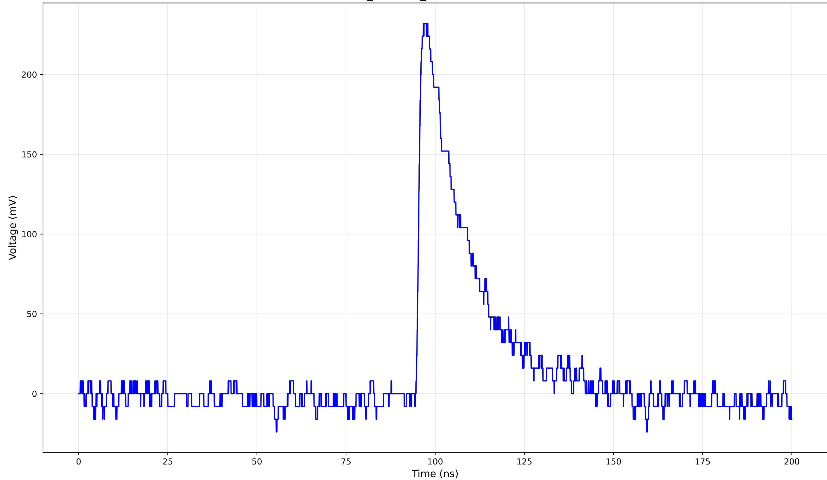
TCT Pulse Waveform - Run 1_80: 1cm_42-Position1 (80.0 V) - Rise Time: 1.32 ns
