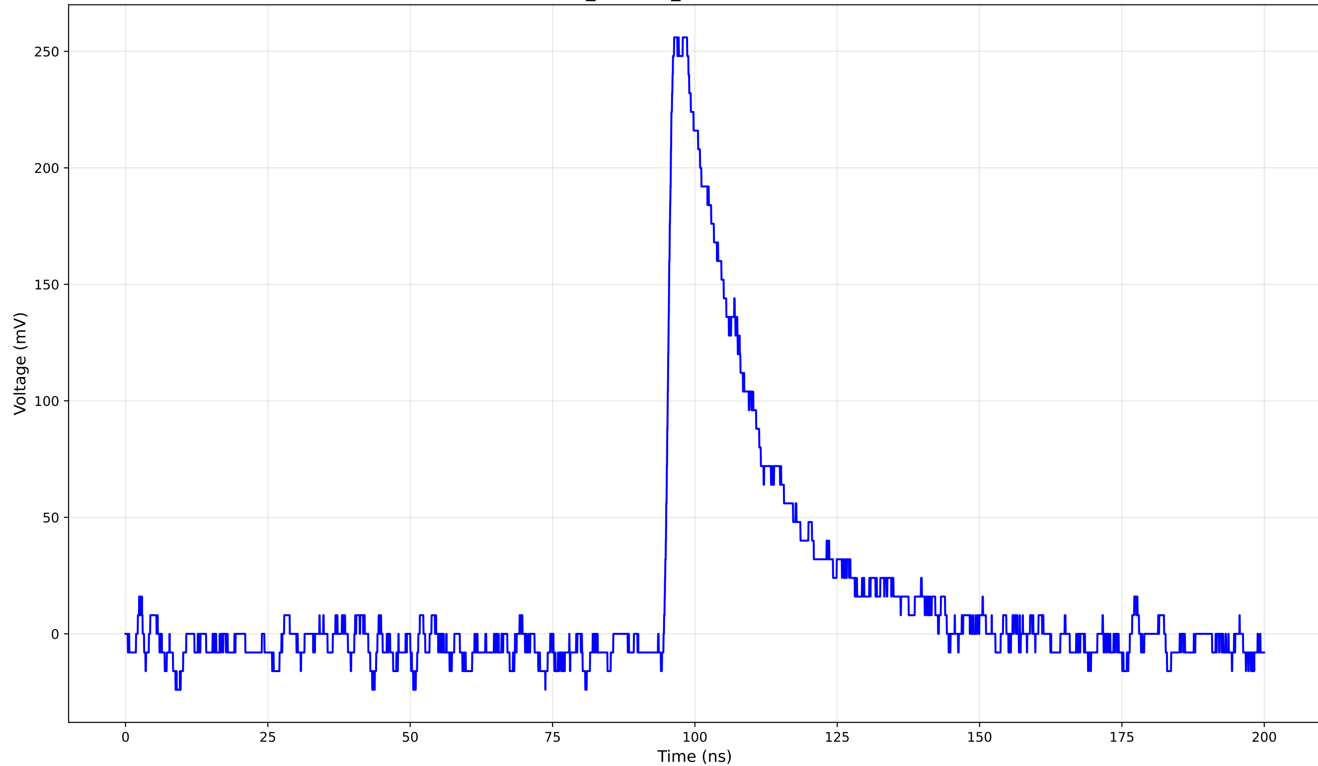
TCT Pulse Waveform - Run 1_90: 1cm_42-Position1 (90.0 V) - Rise Time: 1.25 ns
