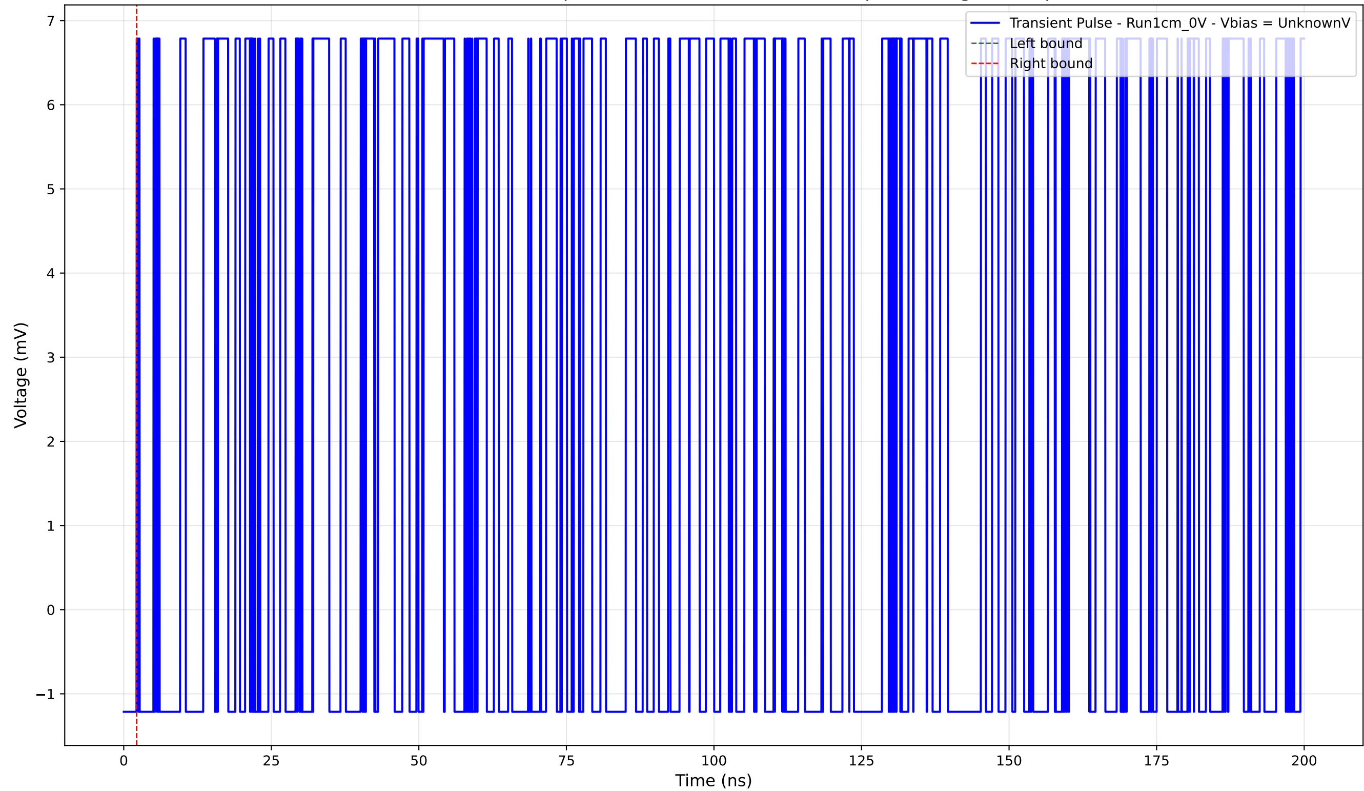
Transient Pulse - Sample: new1cm -Position: 4210.0 \mu\text{m} - Charge: 0.00 pC
