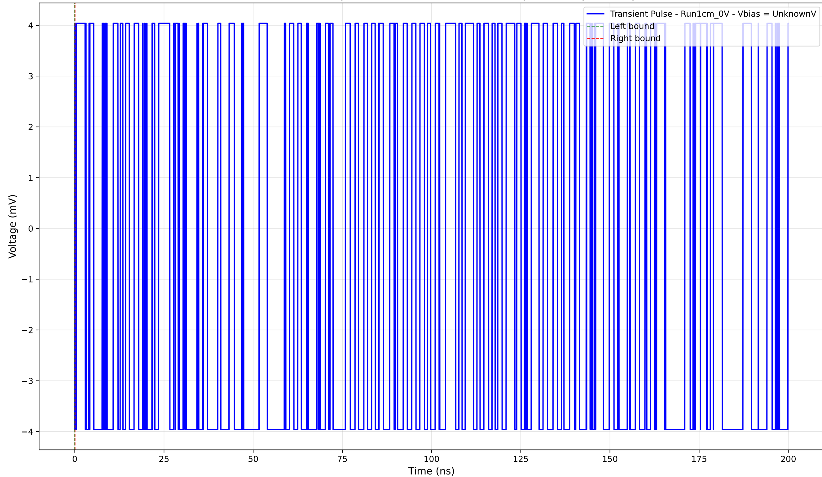
Transient Pulse - Sample: new1cm -Position: 2590.0 \mu\text{m} - Charge: 0.00 pC
