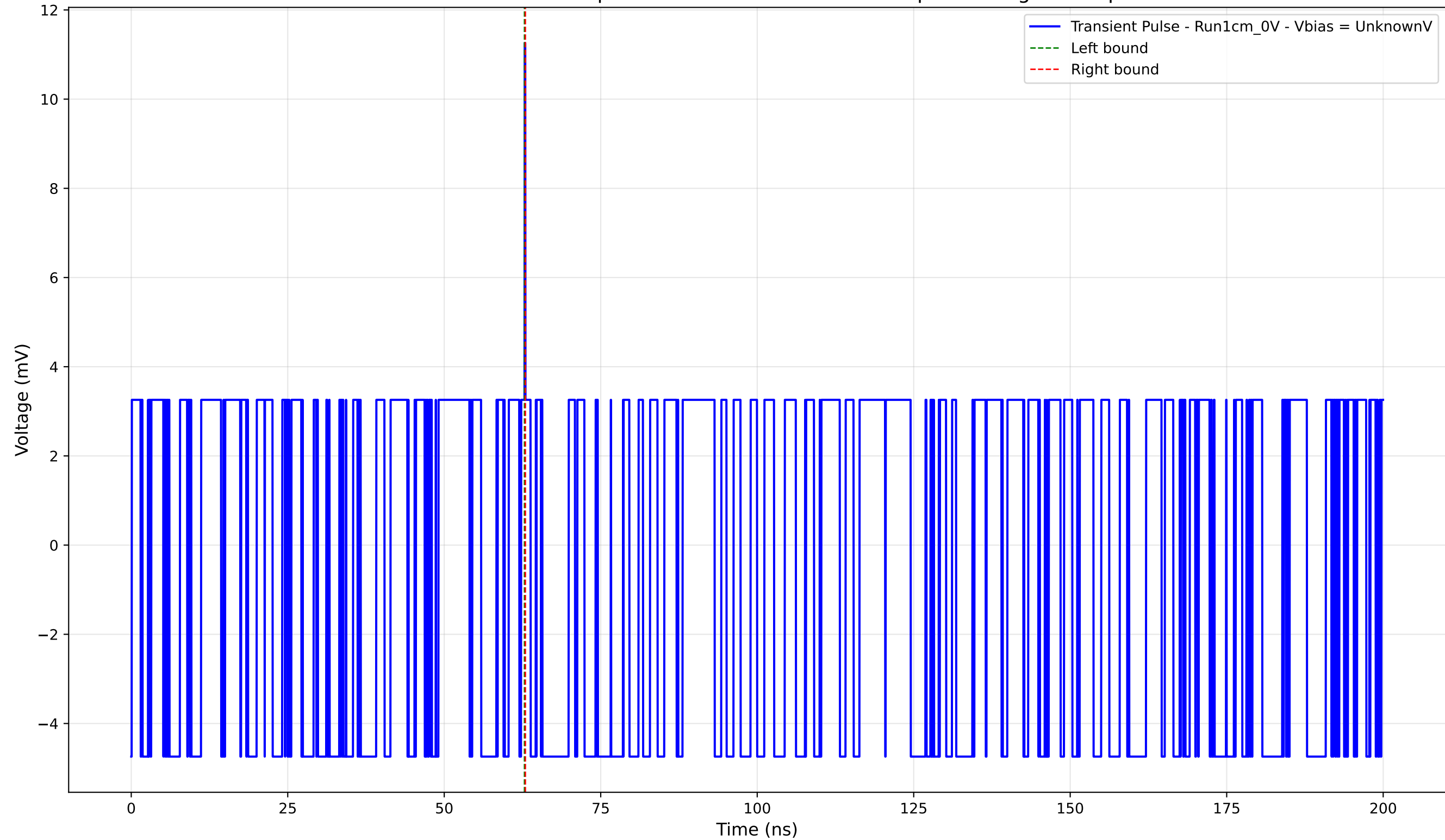
Transient Pulse - Sample: new1cm - Position: 4075.0 \mu\text{m} - Charge: 0.03 pC
