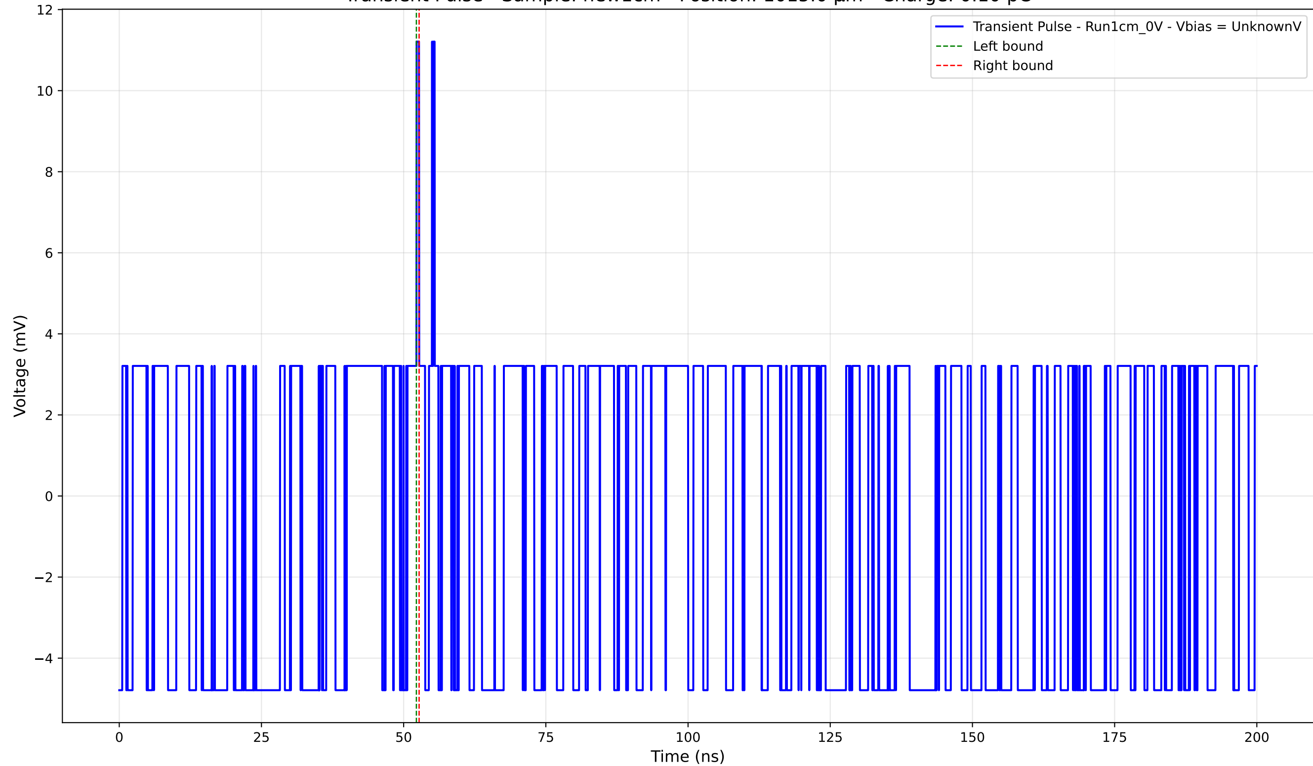
Transient Pulse - Sample: new1cm - Position: 1015.0 \mu\text{m} - Charge: 0.10 pC
