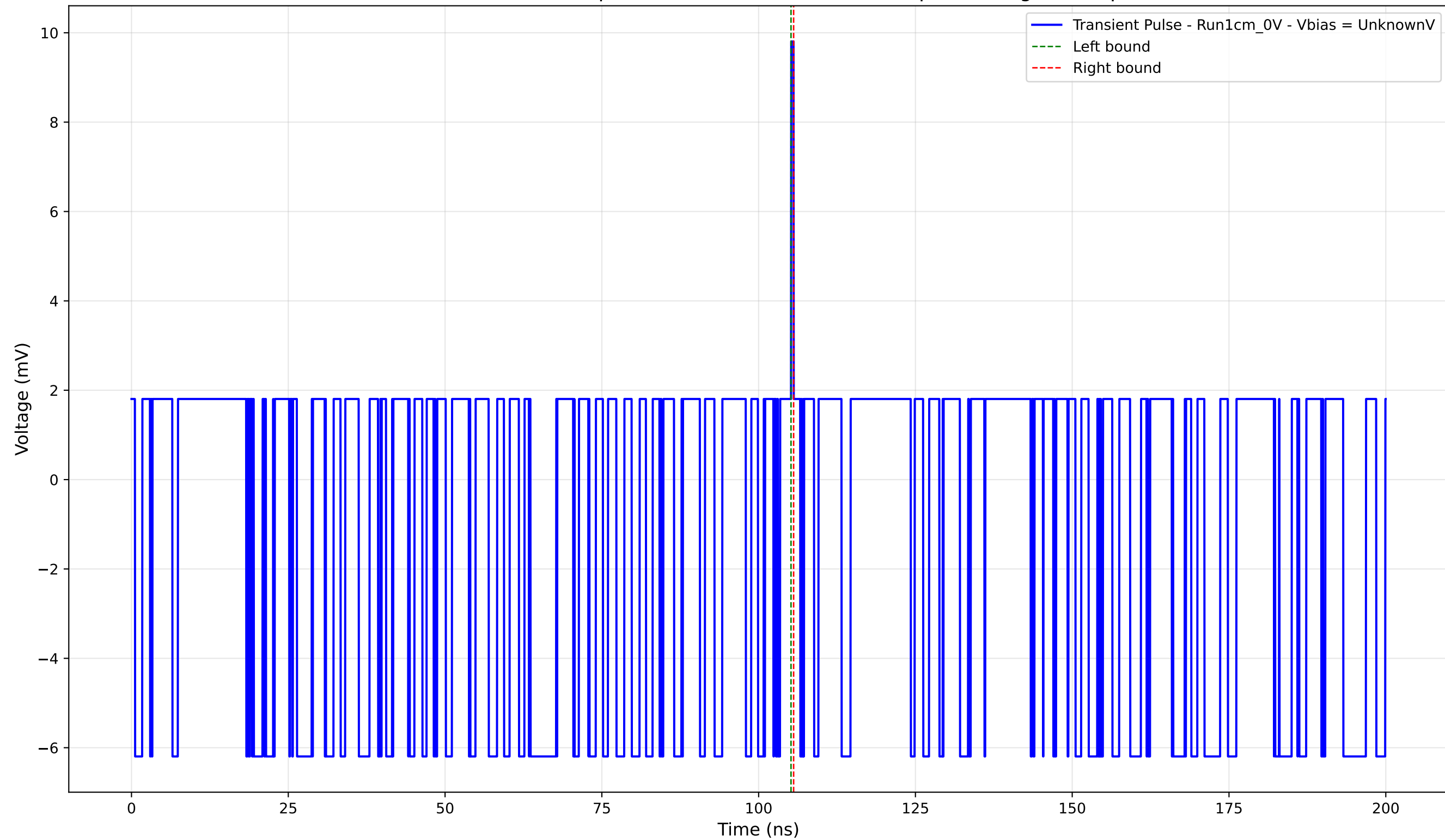
Transient Pulse - Sample: new1cm - Position: 4300.0 \mu\text{m} - Charge: 0.08 pC
