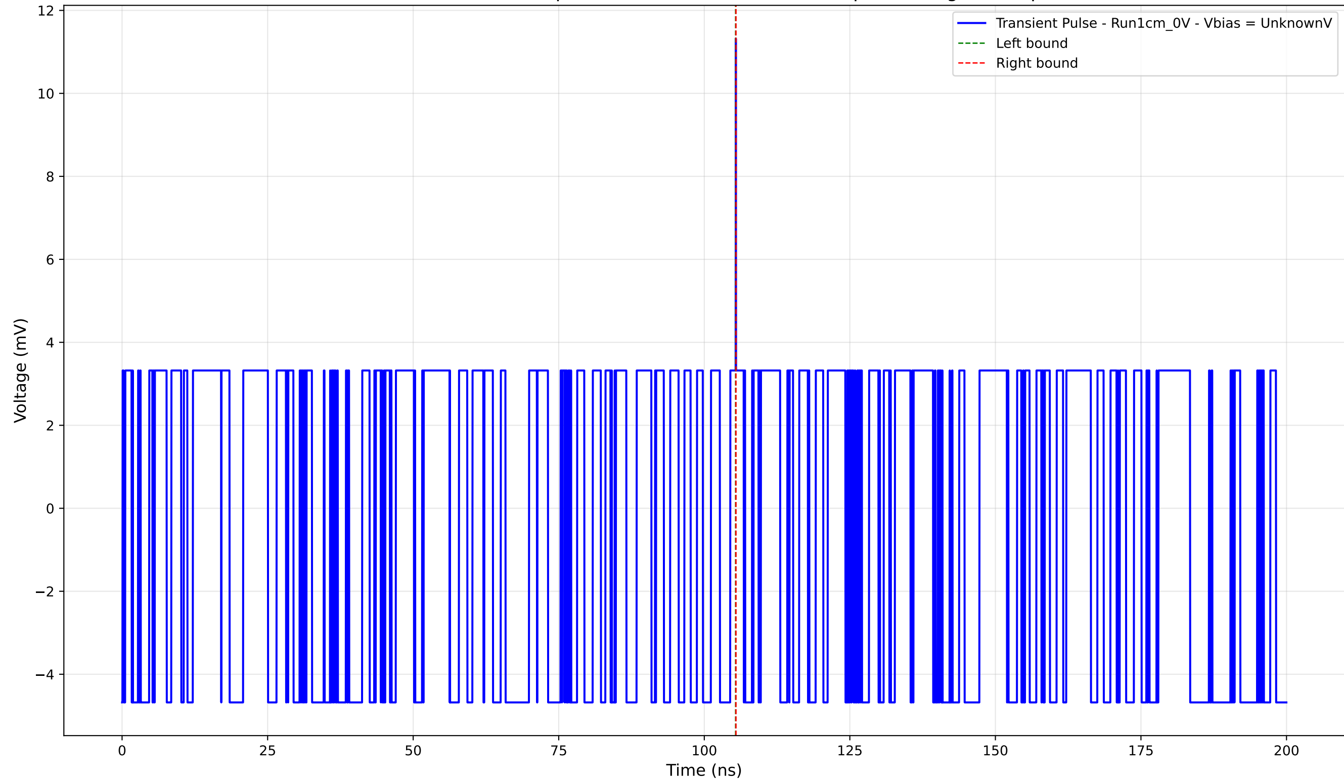
Transient Pulse - Sample: new1cm - Position: 3790.0 \mu\text{m} - Charge: 0.01 pC
