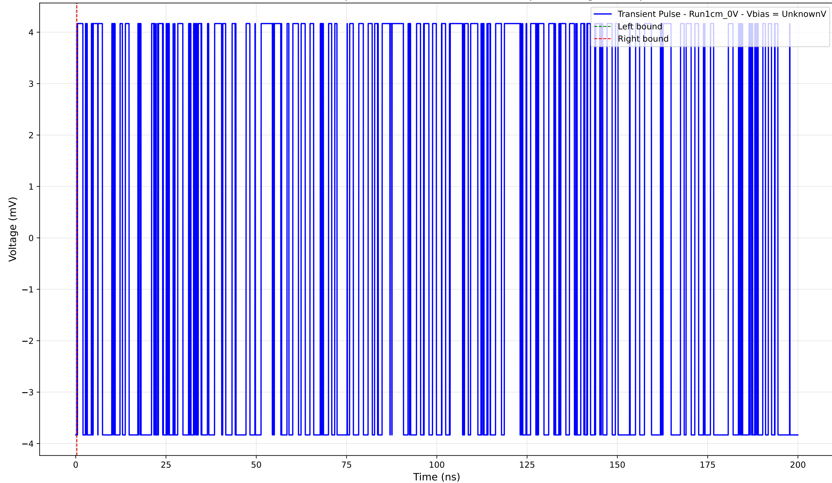
Transient Pulse - Sample: new1cm -Position: 1750.0 \mu\text{m} - Charge: 0.00 pC
