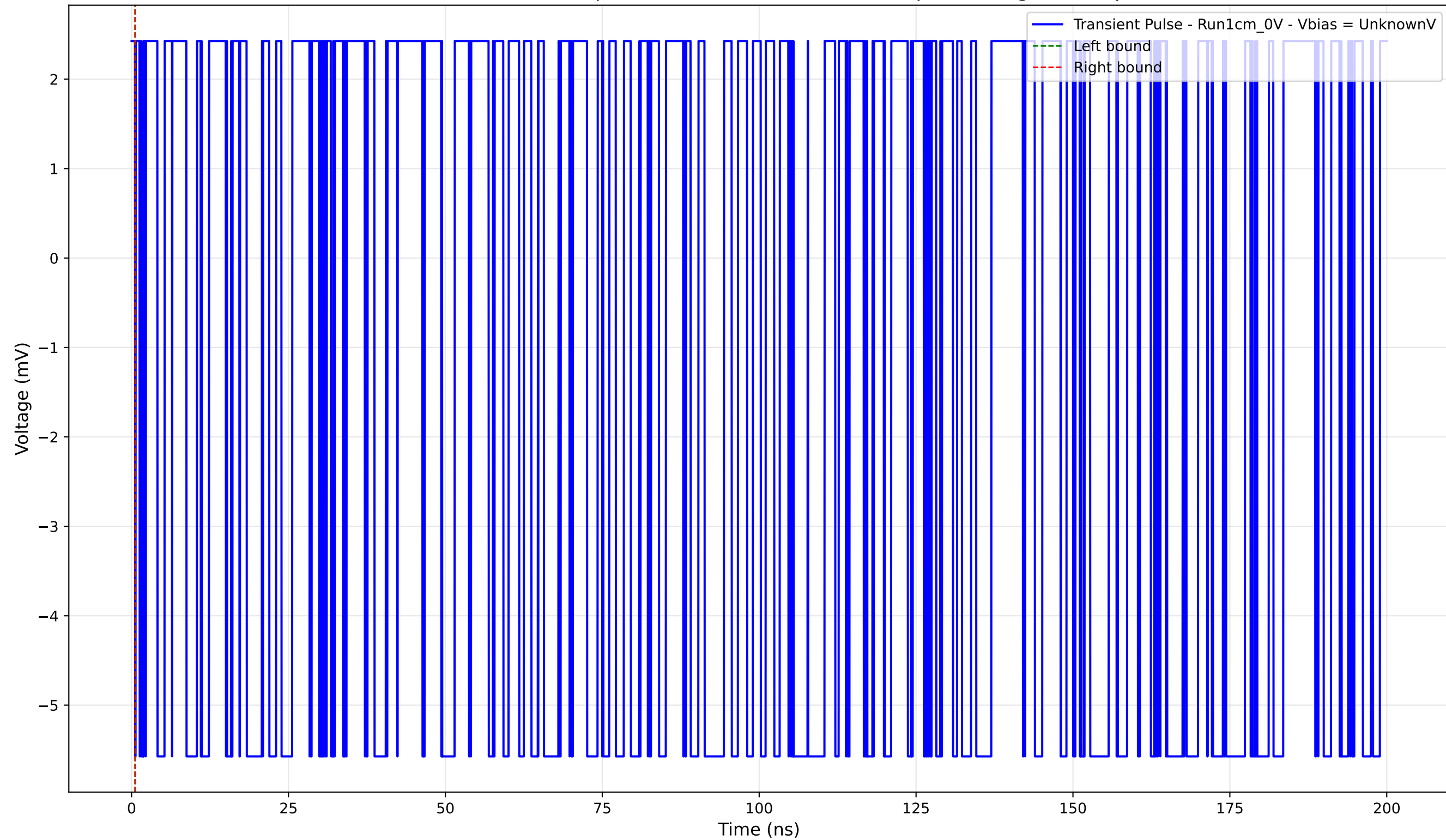
Transient Pulse - Sample: new1cm - Position: 2375.0 \mu\text{m} - Charge: -0.00 pC
