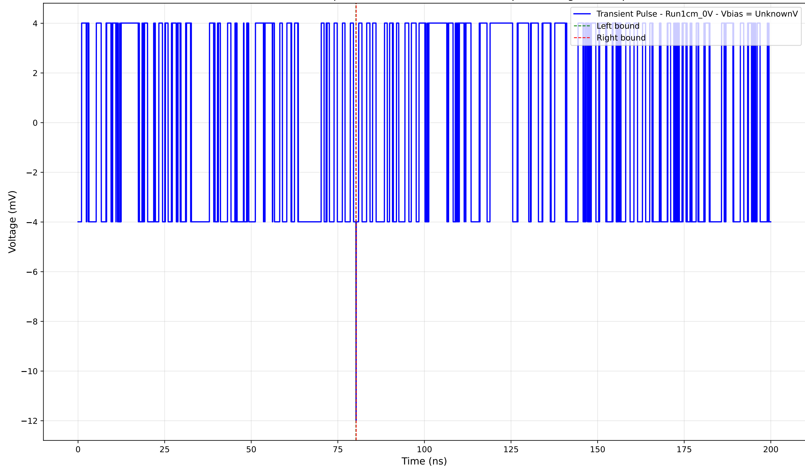
Transient Pulse - Sample: new1cm - Position: 3755.0 \mu\text{m} - Charge: -0.02 pC
