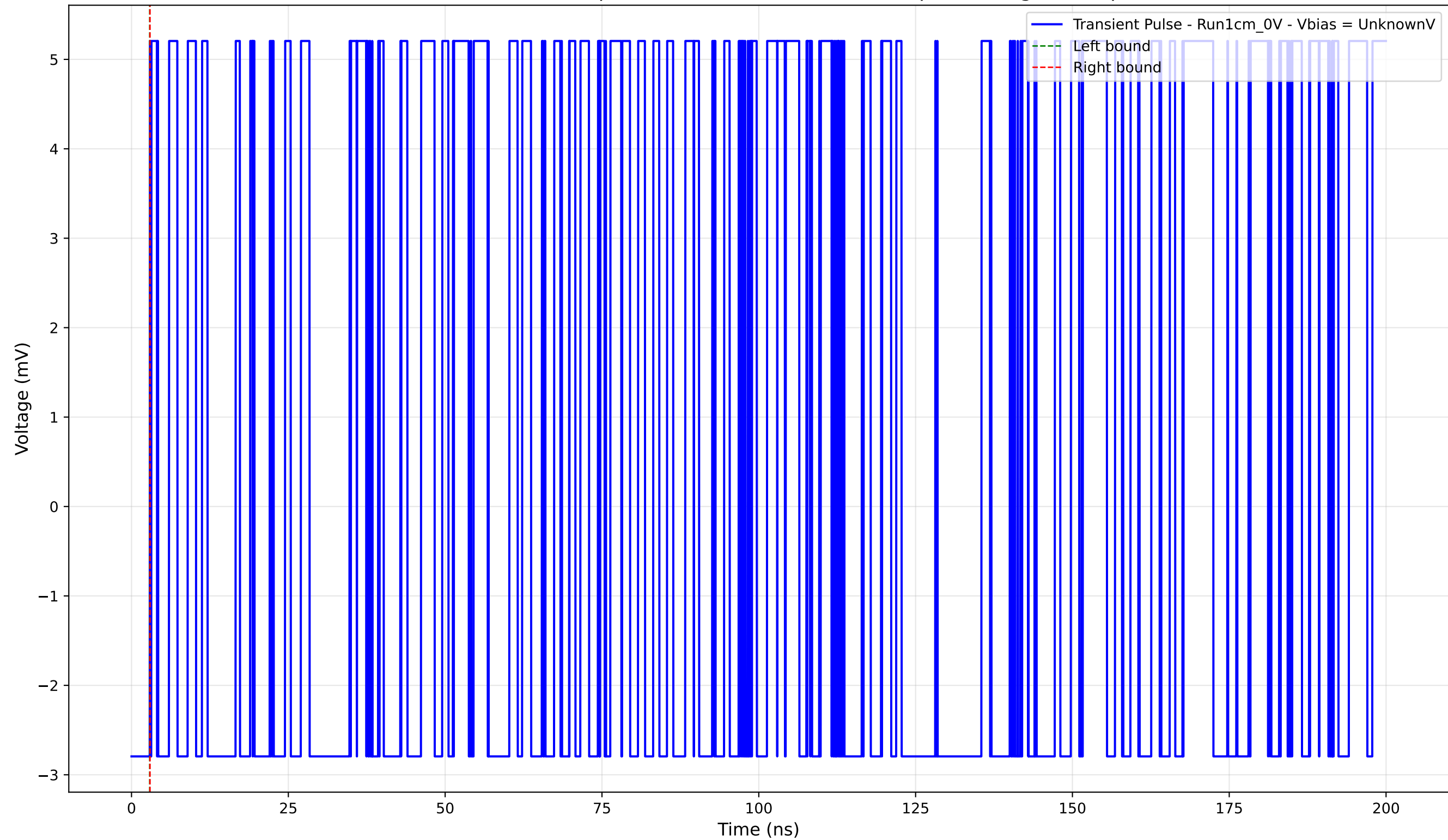
Transient Pulse - Sample: new1cm - Position: 1915.0 \mu\text{m} - Charge: 0.00 pC
