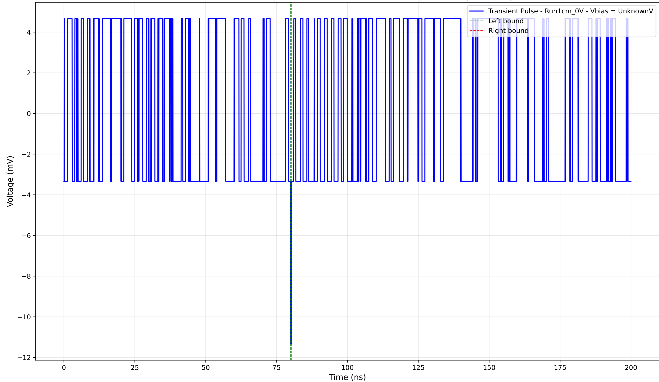
Transient Pulse - Sample: new1cm - Position: 3980.0 \mu\text{m} - Charge: -0.08 pC
