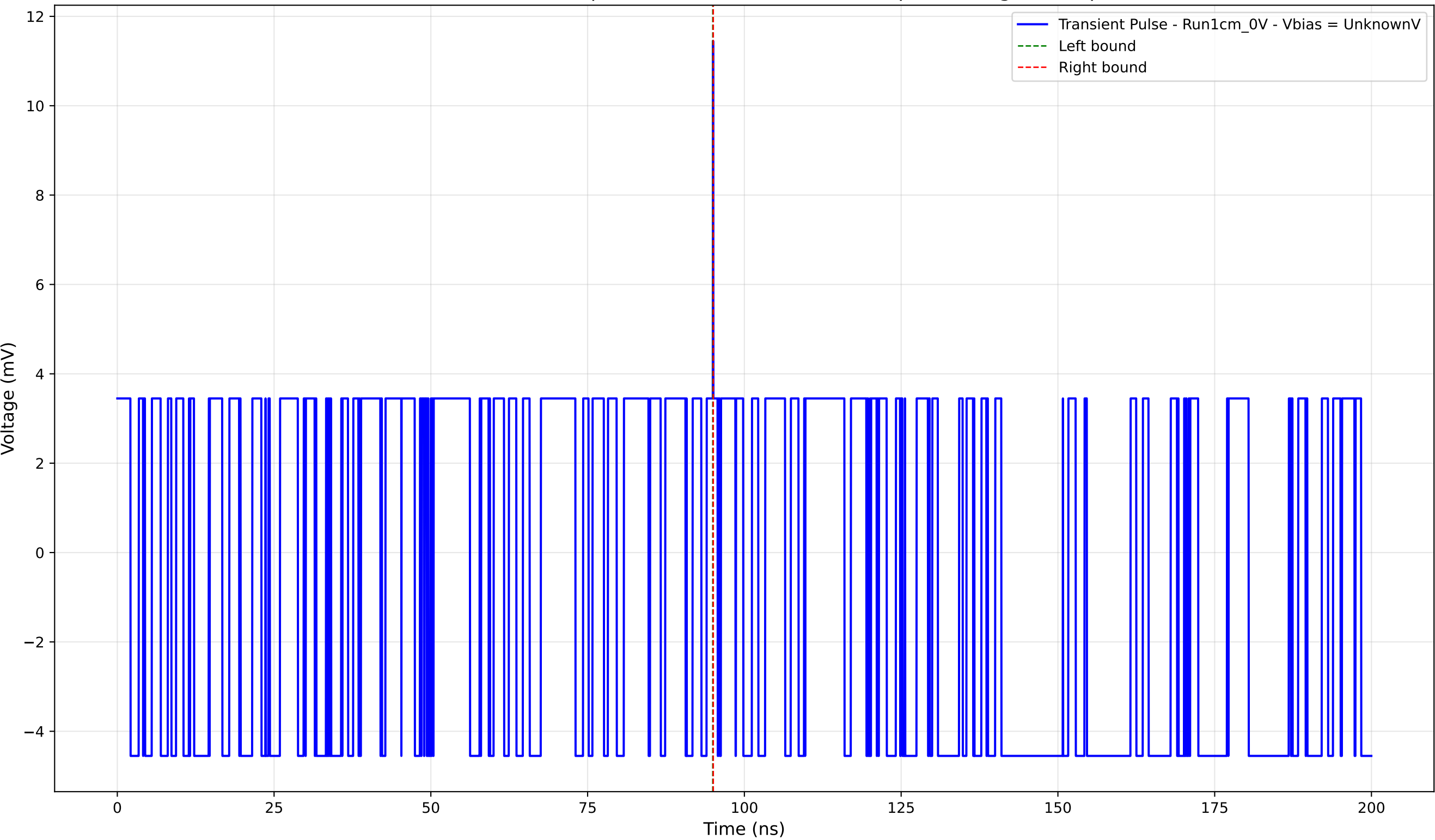
Transient Pulse - Sample: new1cm - Position: 430.0 \mu\text{m} - Charge: 0.02 pC
