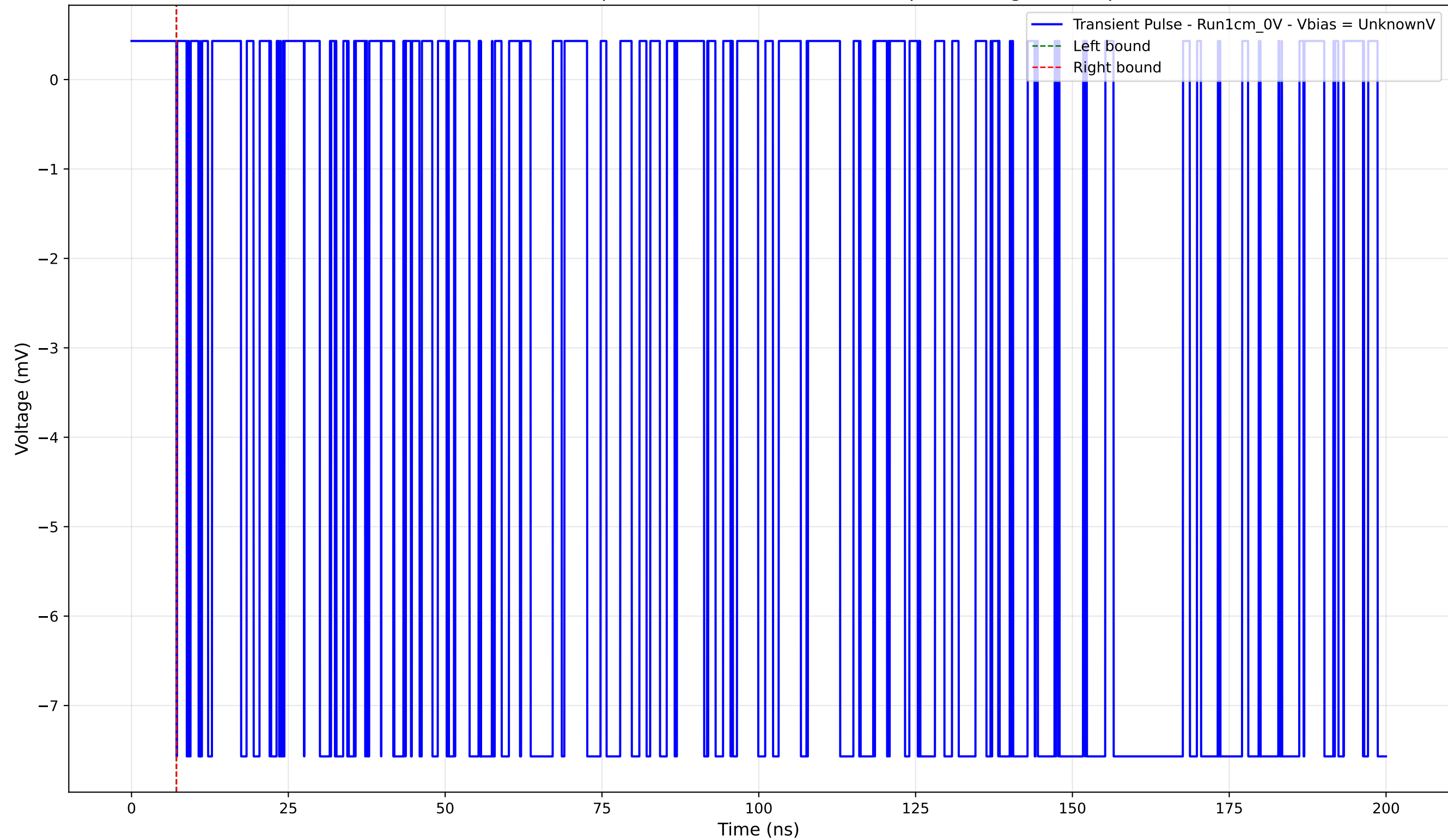
Transient Pulse - Sample: new1cm - Position: 310.0 \mu\text{m} - Charge: -0.00 pC
