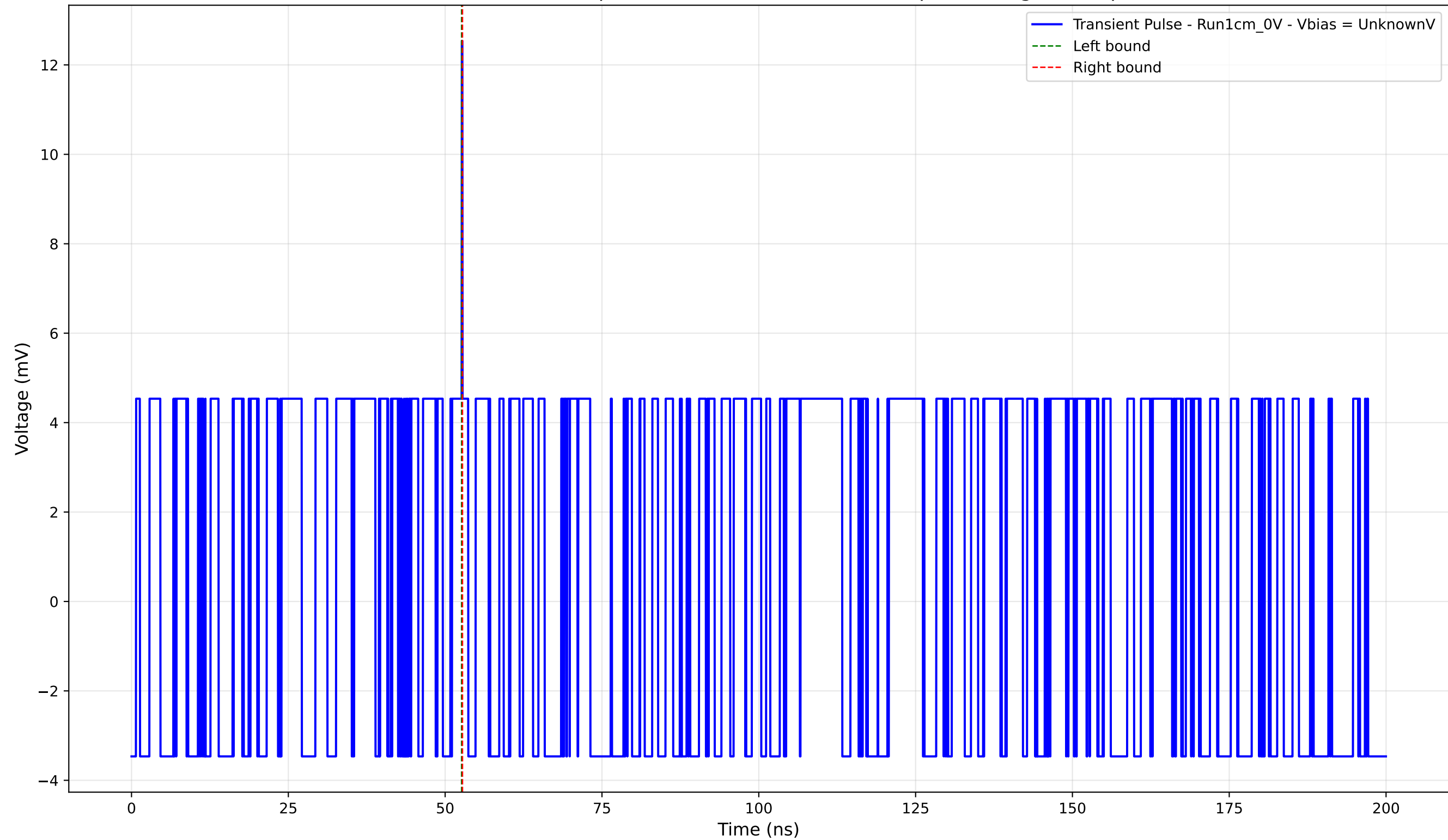
Transient Pulse - Sample: new1cm - Position: 3020.0 \mu\text{m} - Charge: 0.03 pC
