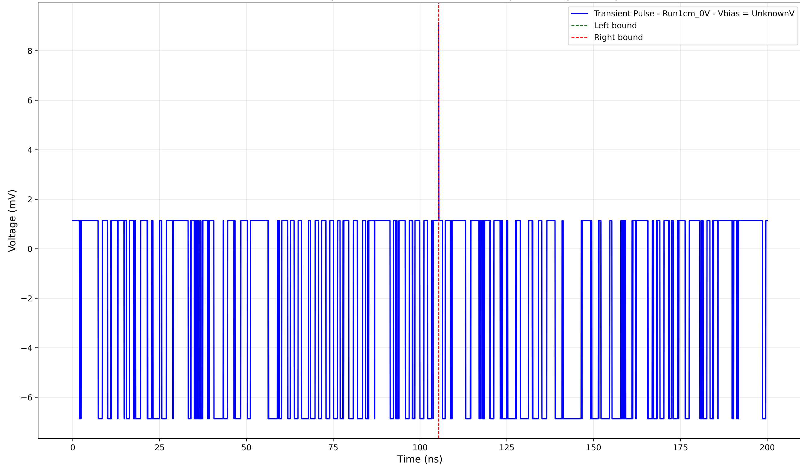
Transient Pulse - Sample: new1cm - Position: 2235.0 \mu\text{m} - Charge: 0.01 pC
