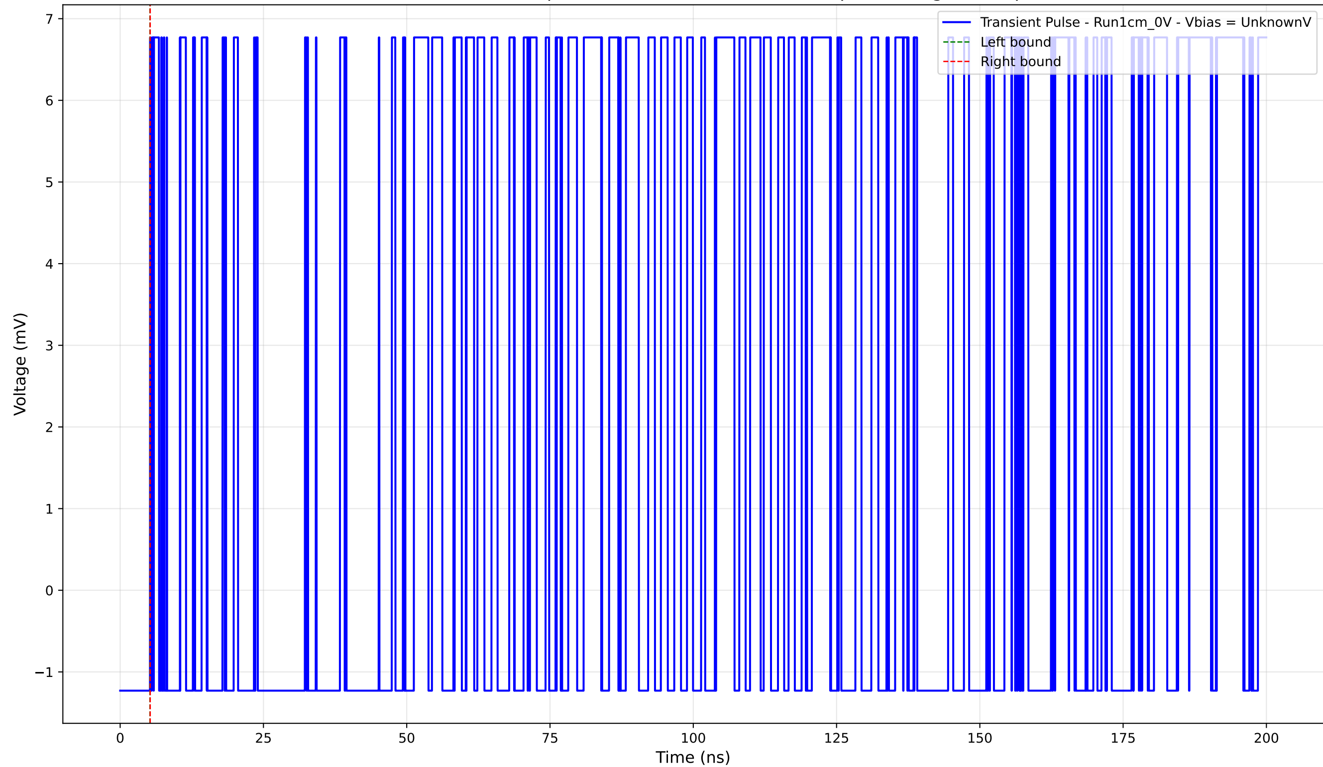
Transient Pulse - Sample: new1cm - Position: 2015.0 \mu\text{m} - Charge: 0.00 pC
