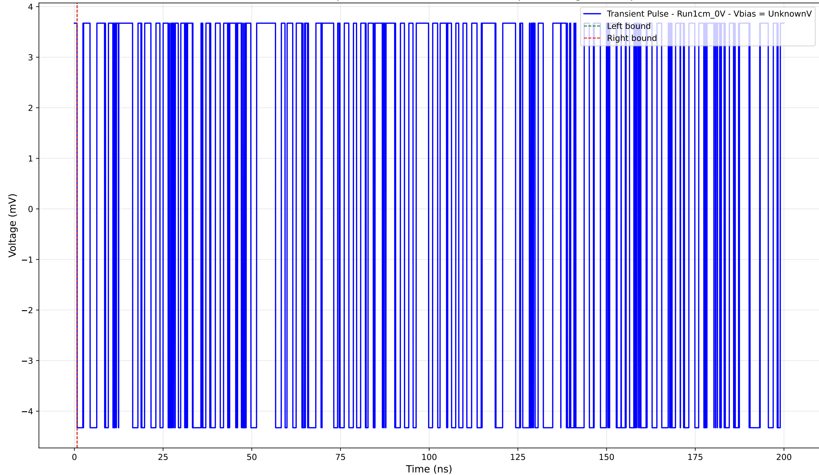
Transient Pulse - Sample: new1cm - Position: 1465.0 \mu\text{m} - Charge: -0.00 pC
