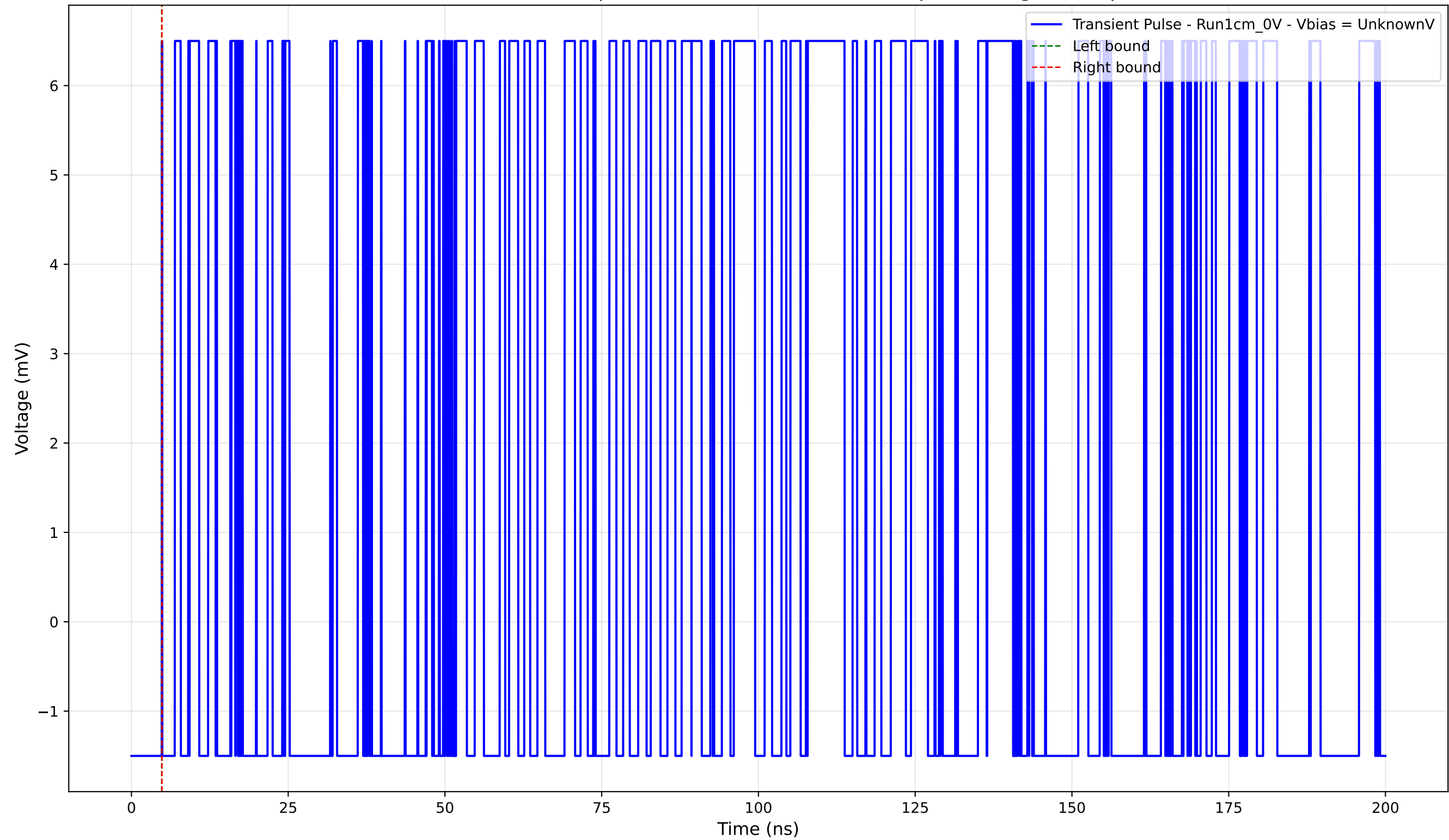
Transient Pulse - Sample: new1cm -Position: 3890.0 \mu\text{m} - Charge: 0.00 pC
