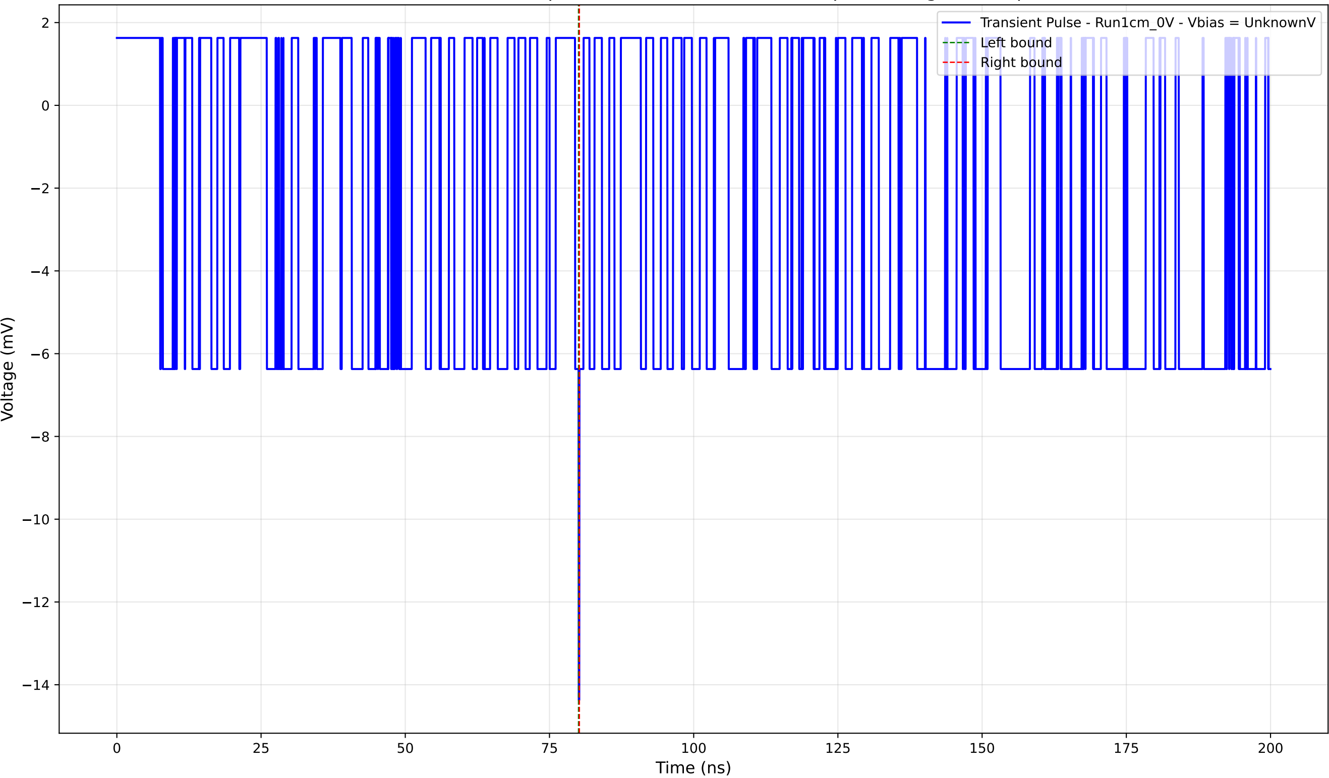
Transient Pulse - Sample: new1cm - Position: 925.0 \mu\text{m} - Charge: -0.04 pC
