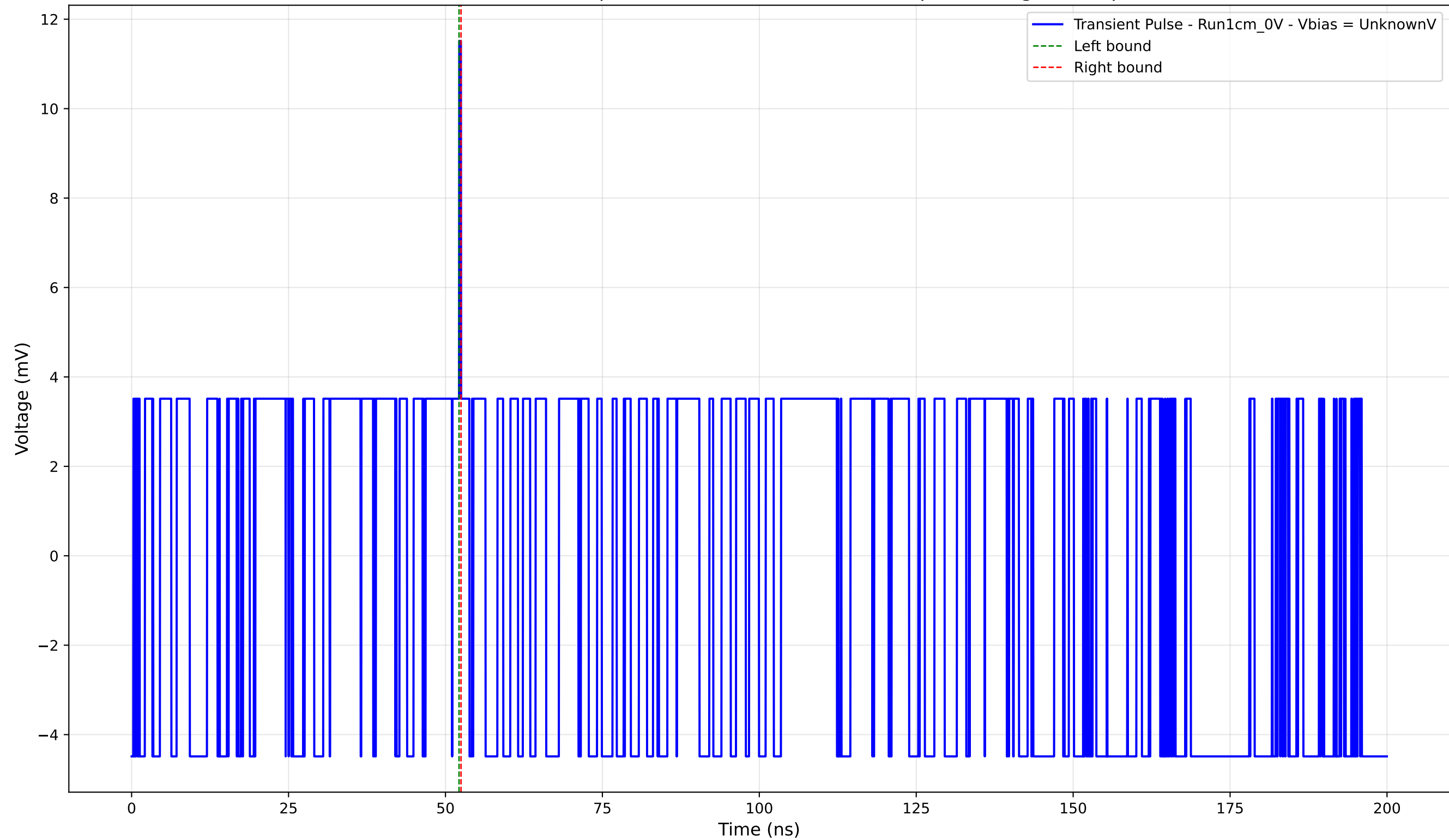
Transient Pulse - Sample: new1cm - Position: 2100.0 \mu\text{m} - Charge: 0.07 pC
