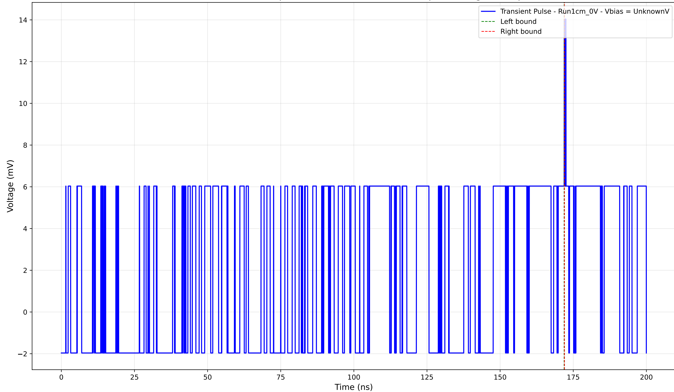
Transient Pulse - Sample: new1cm - Position: 5045.0 \mu\text{m} - Charge: 0.03 pC
