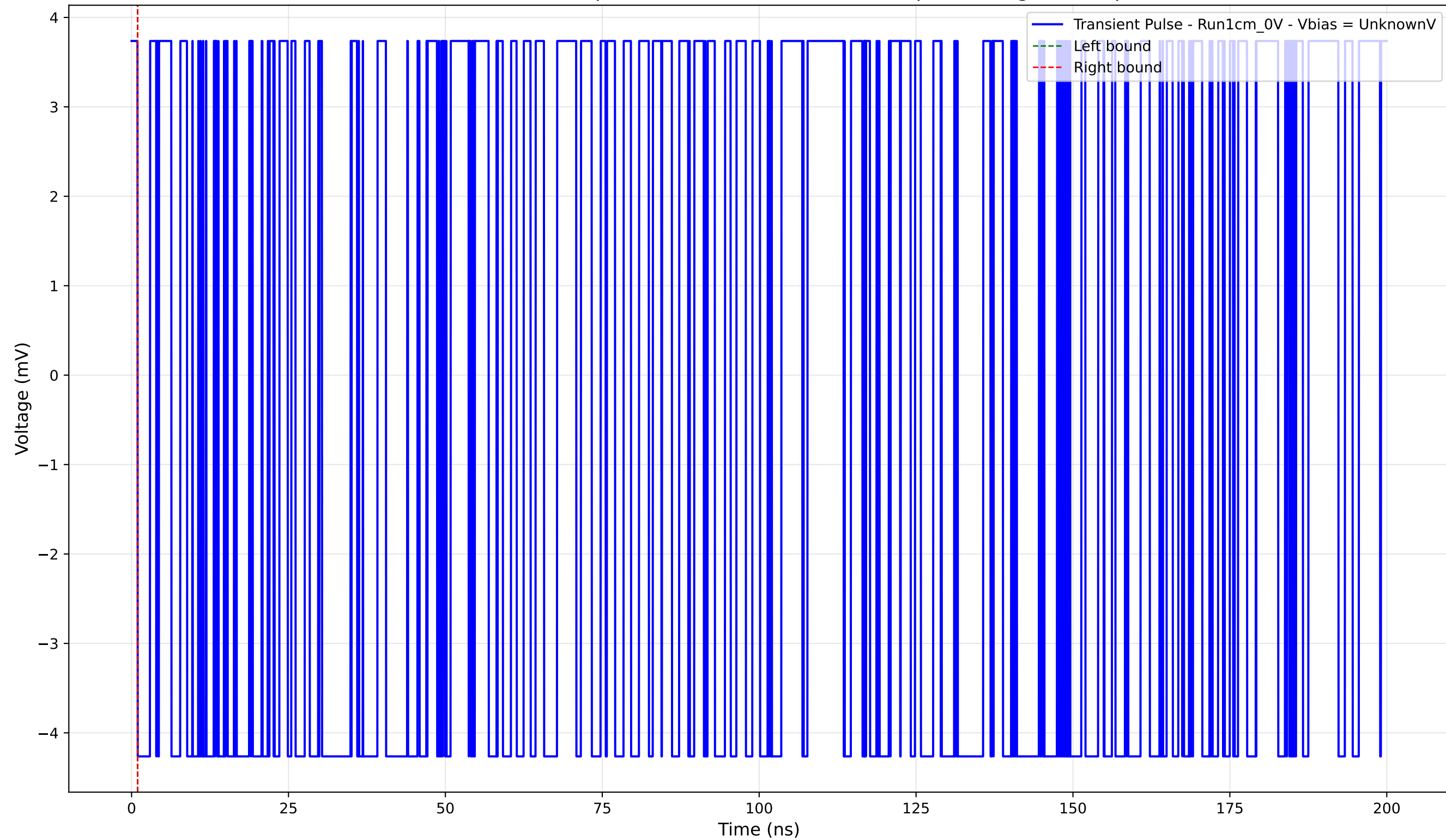
Transient Pulse - Sample: new1cm - Position: 4100.0 \mu\text{m} - Charge: -0.00 pC
