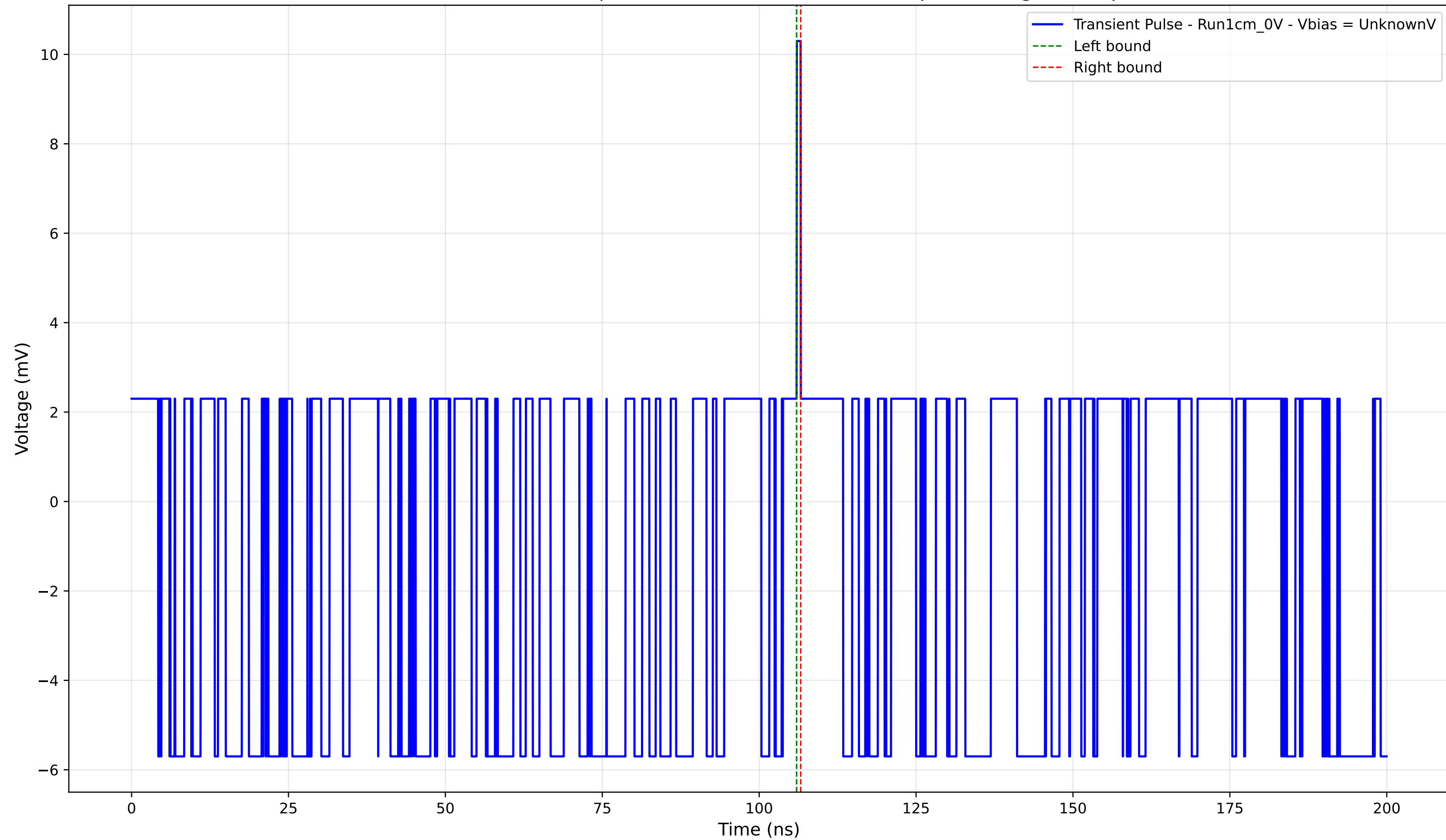
Transient Pulse - Sample: new1cm - Position: 4650.0 \mu\text{m} - Charge: 0.13 pC
