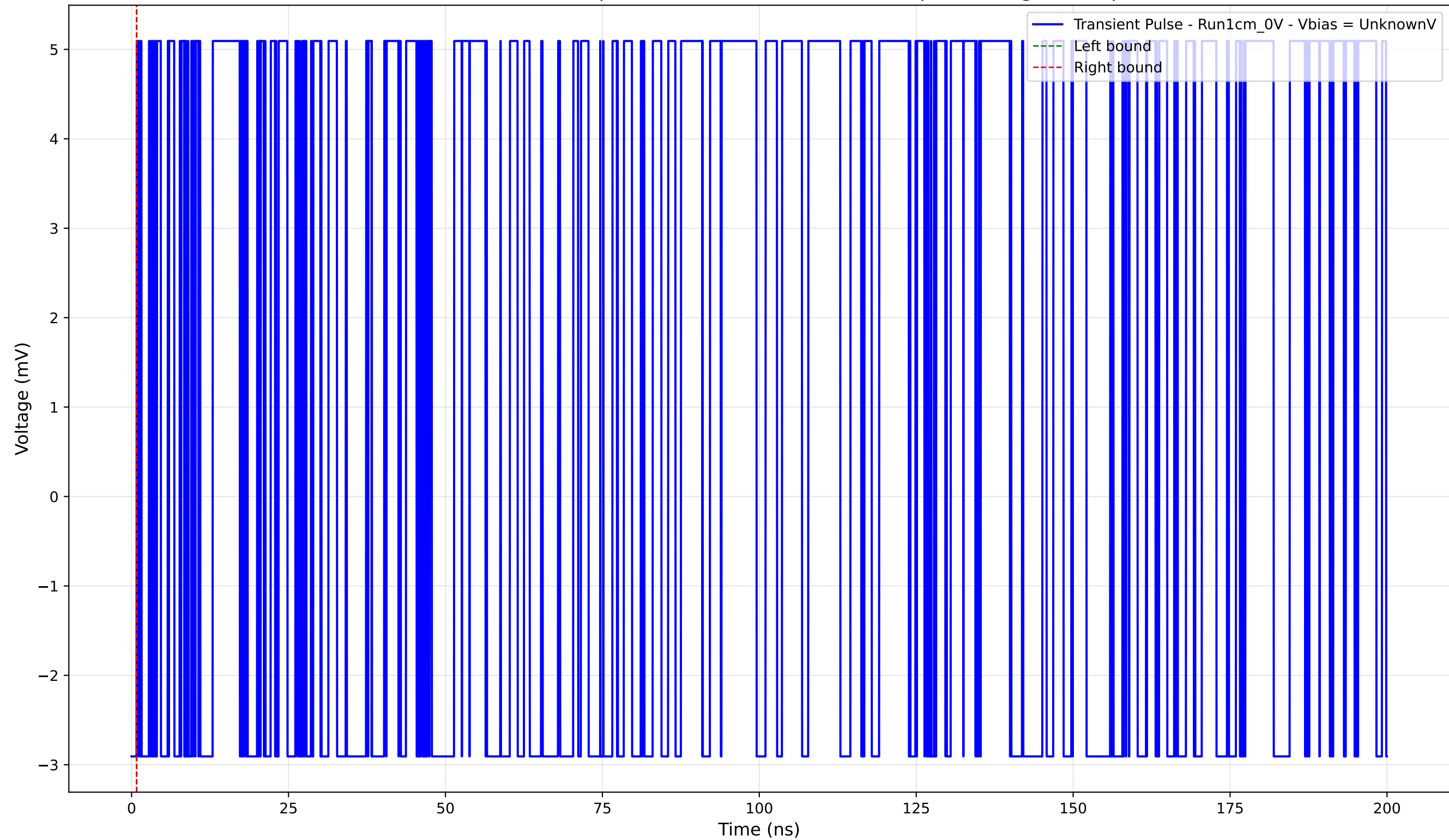
Transient Pulse - Sample: new1cm - Position: 4150.0 \mu\text{m} - Charge: 0.00 pC
