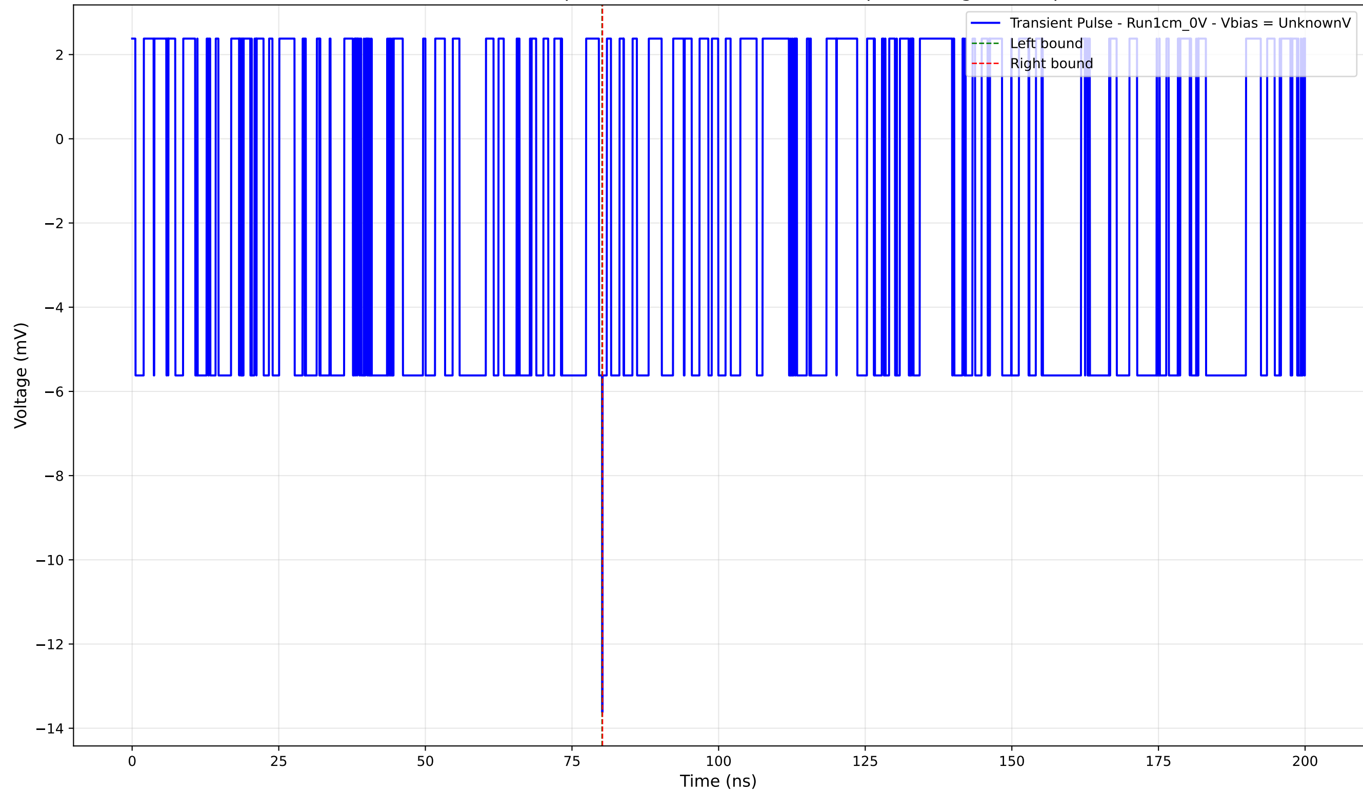
Transient Pulse - Sample: new1cm - Position: 2065.0 \mu\text{m} - Charge: -0.02 pC
