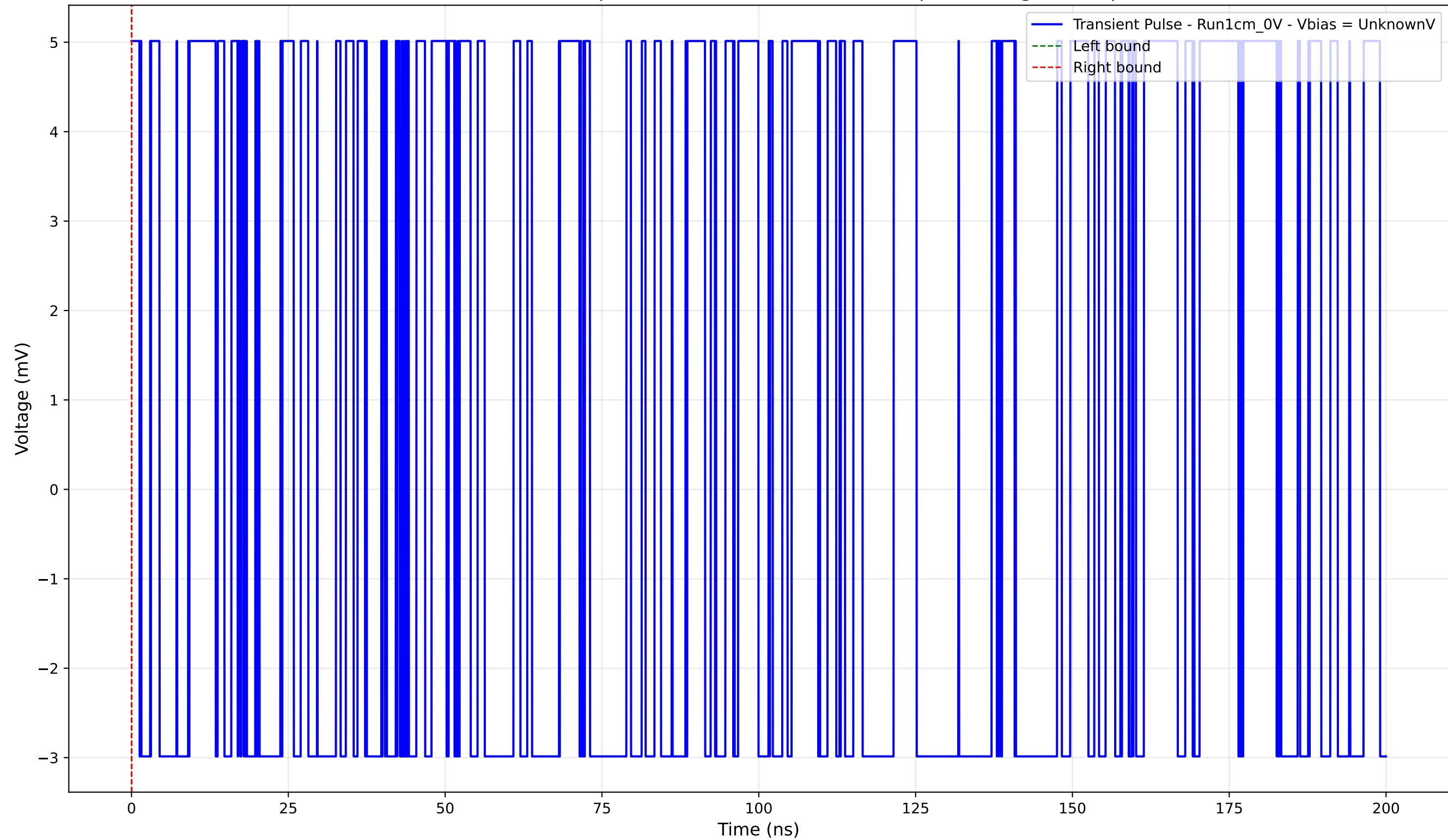
Transient Pulse - Sample: new1cm -Position: 4625.0 \mu\text{m} - Charge: 0.00 pC
