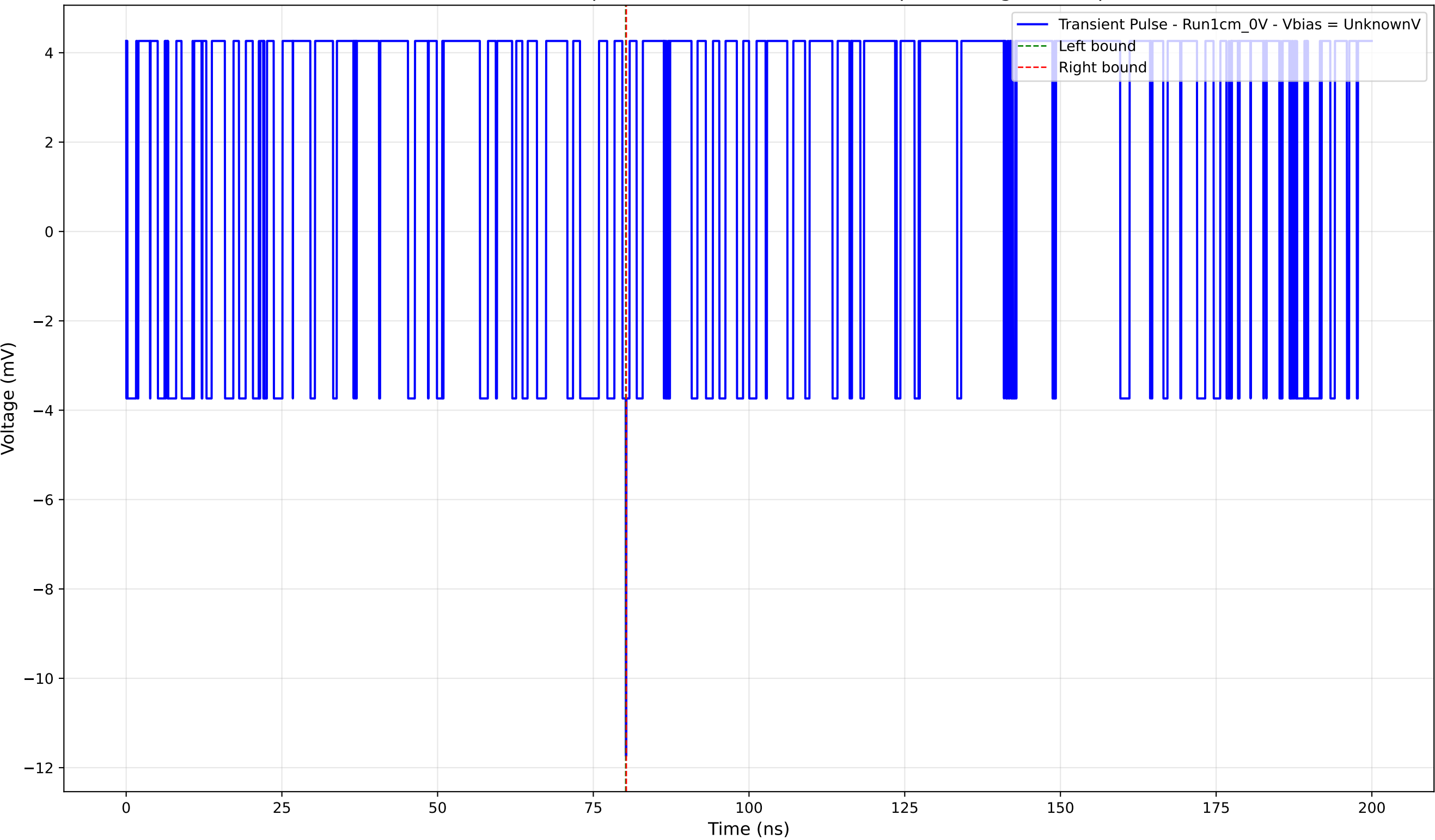
Transient Pulse - Sample: new1cm - Position: 185.0 \mu\text{m} - Charge: -0.02 pC
