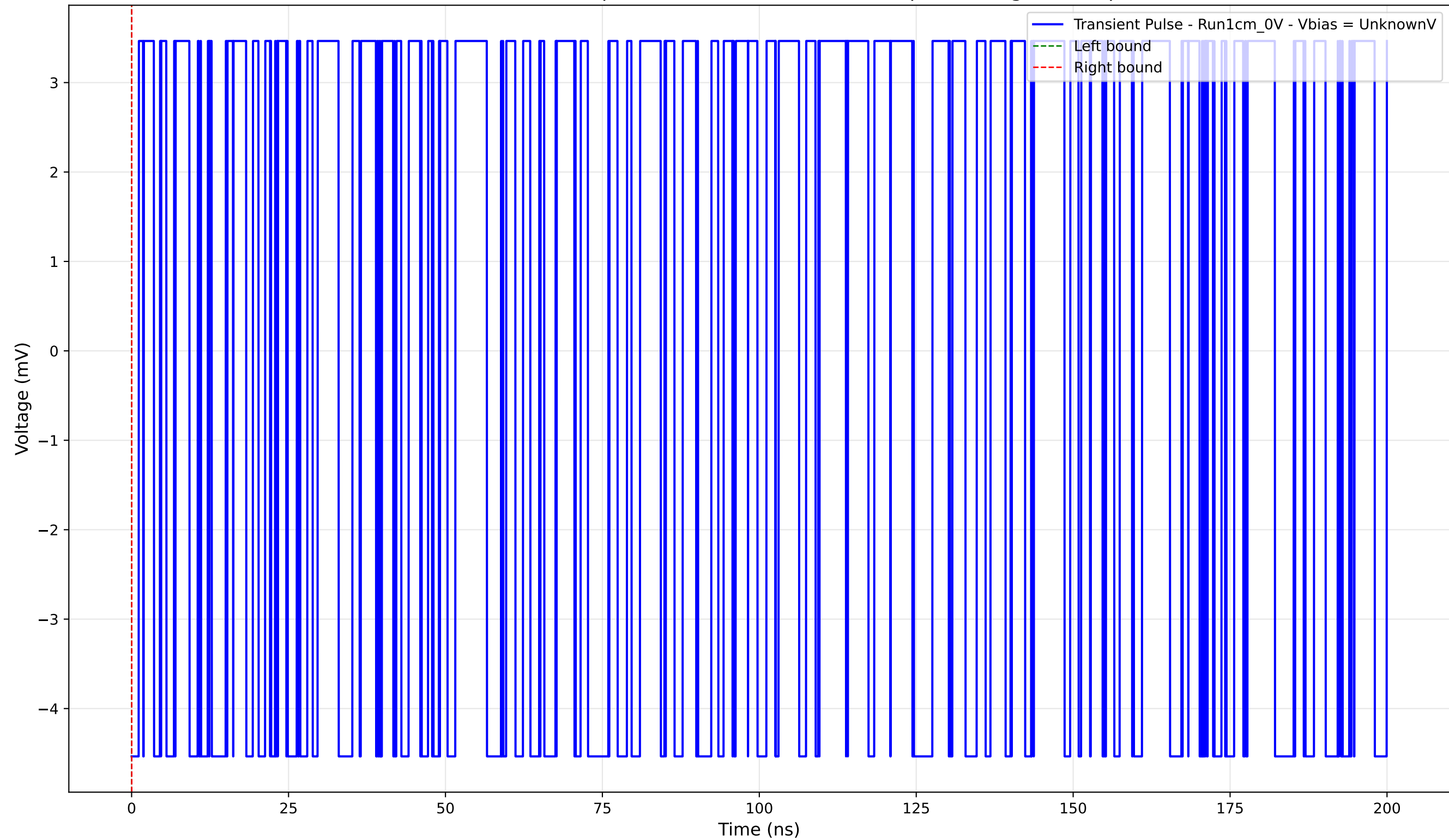
Transient Pulse - Sample: new1cm - Position: 760.0 \mu\text{m} - Charge: -0.00 pC
