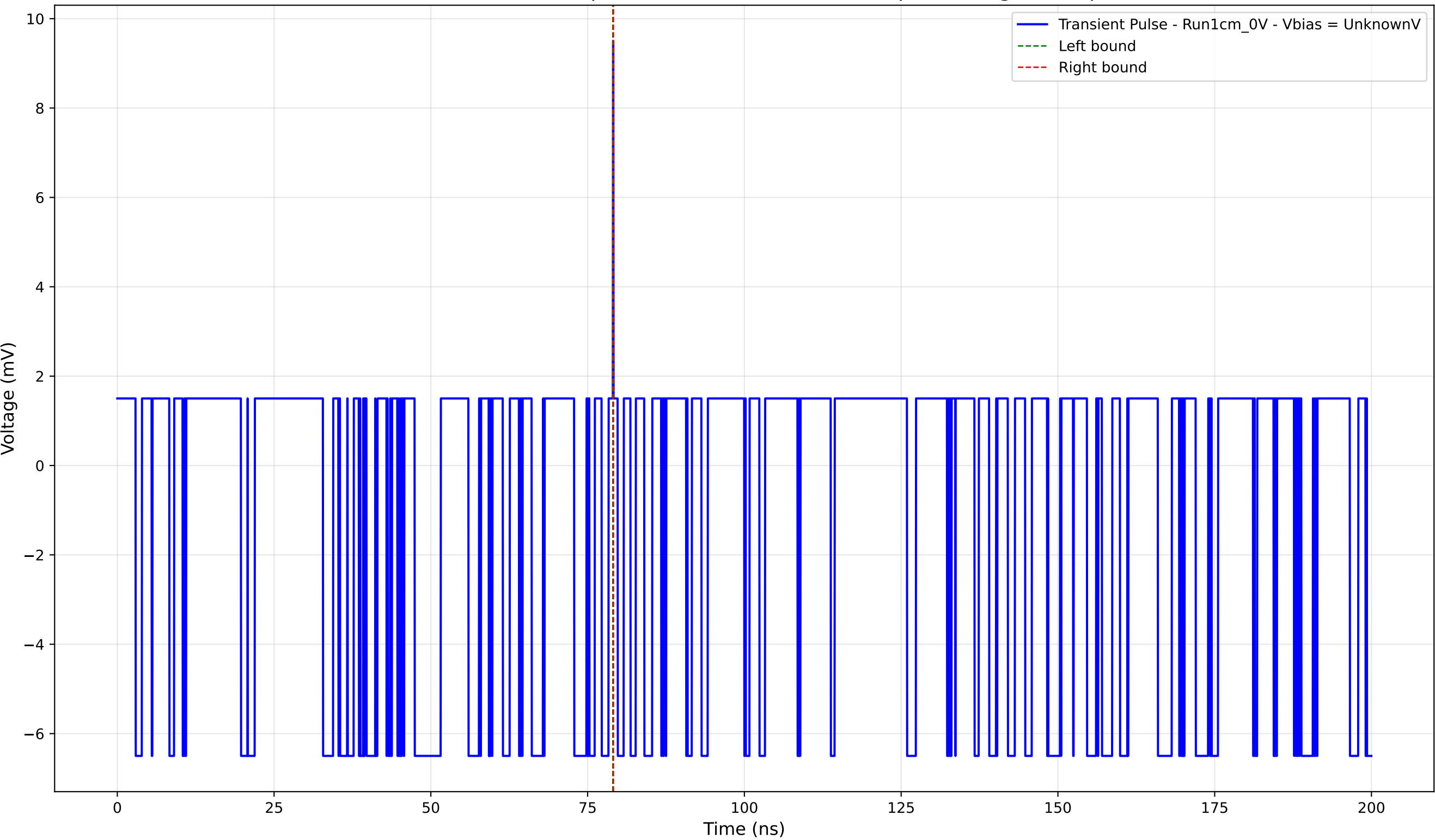
Transient Pulse - Sample: new1cm - Position: 150.0 \mu\text{m} - Charge: 0.02 pC
