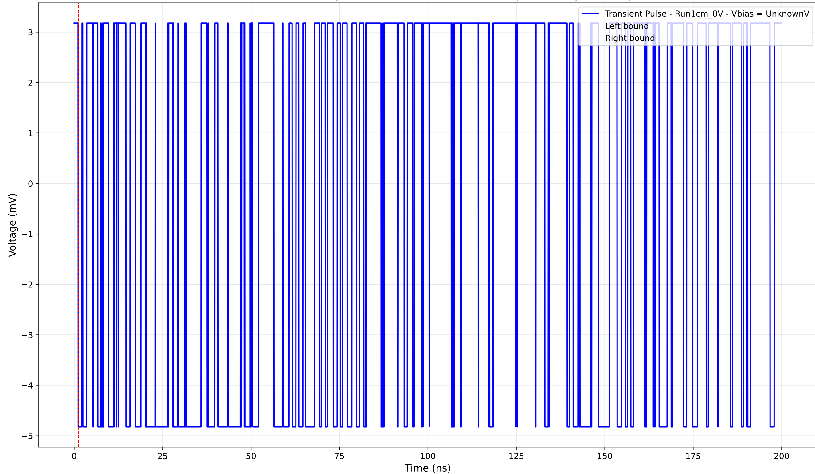
Transient Pulse - Sample: new1cm - Position: 1260.0 \mu\text{m} - Charge: -0.00 pC
