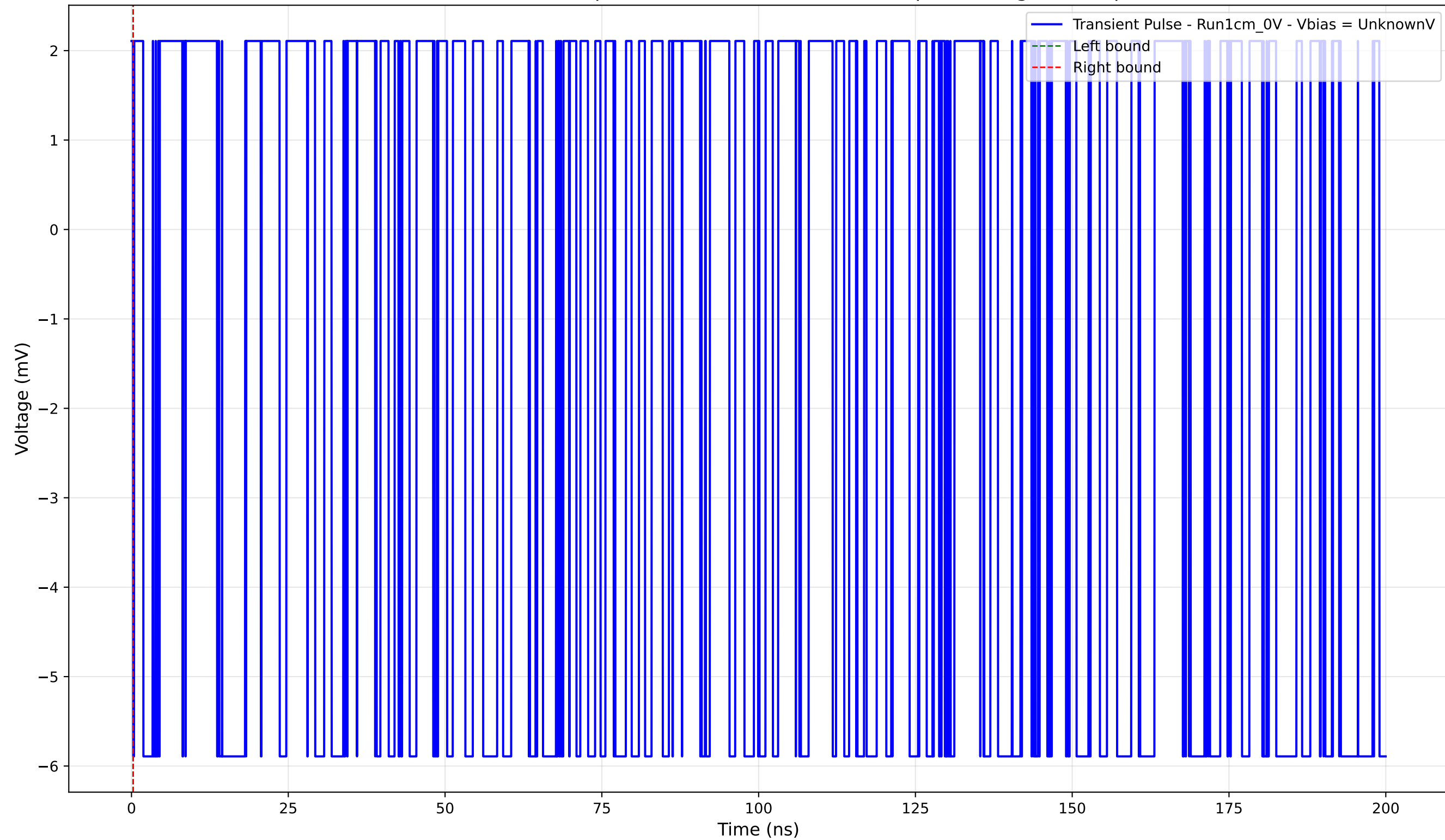
Transient Pulse - Sample: new1cm - Position: 3845.0 \mu\text{m} - Charge: -0.00 pC
