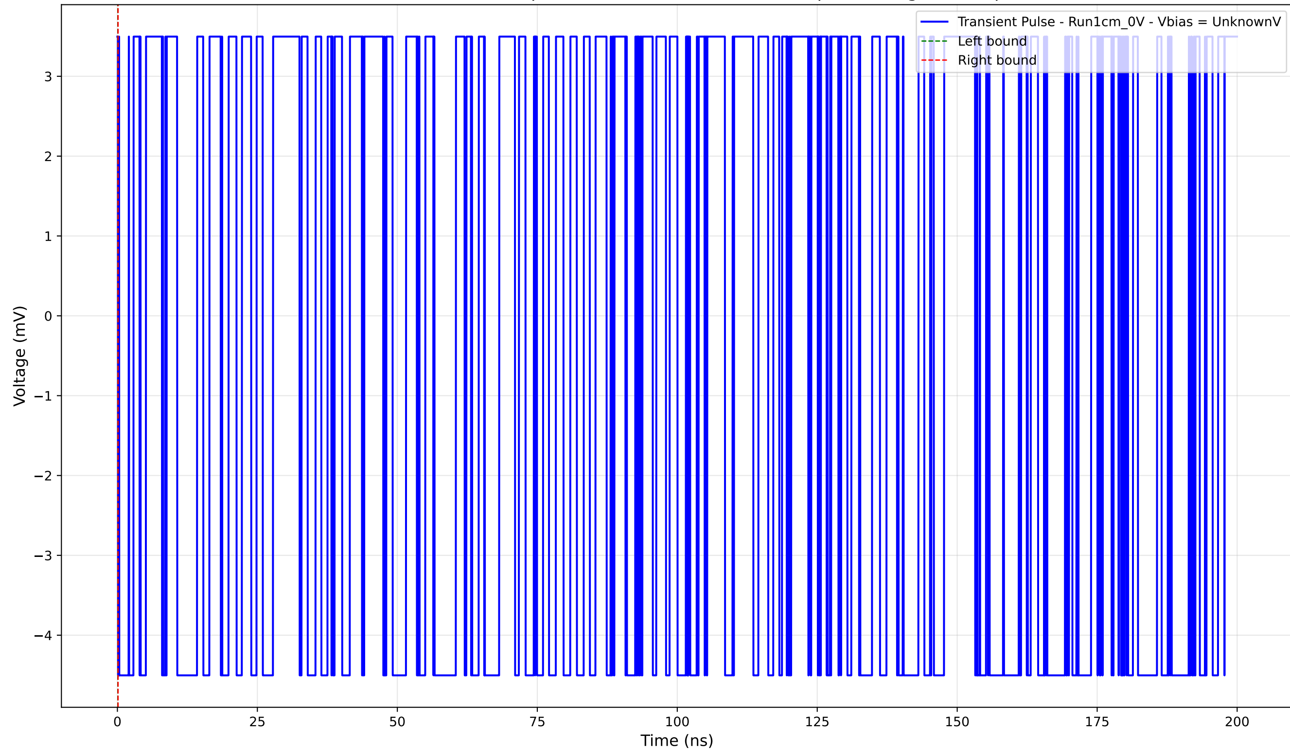
Transient Pulse - Sample: new1cm - Position: 2920.0 \mu\text{m} - Charge: -0.00 pC
