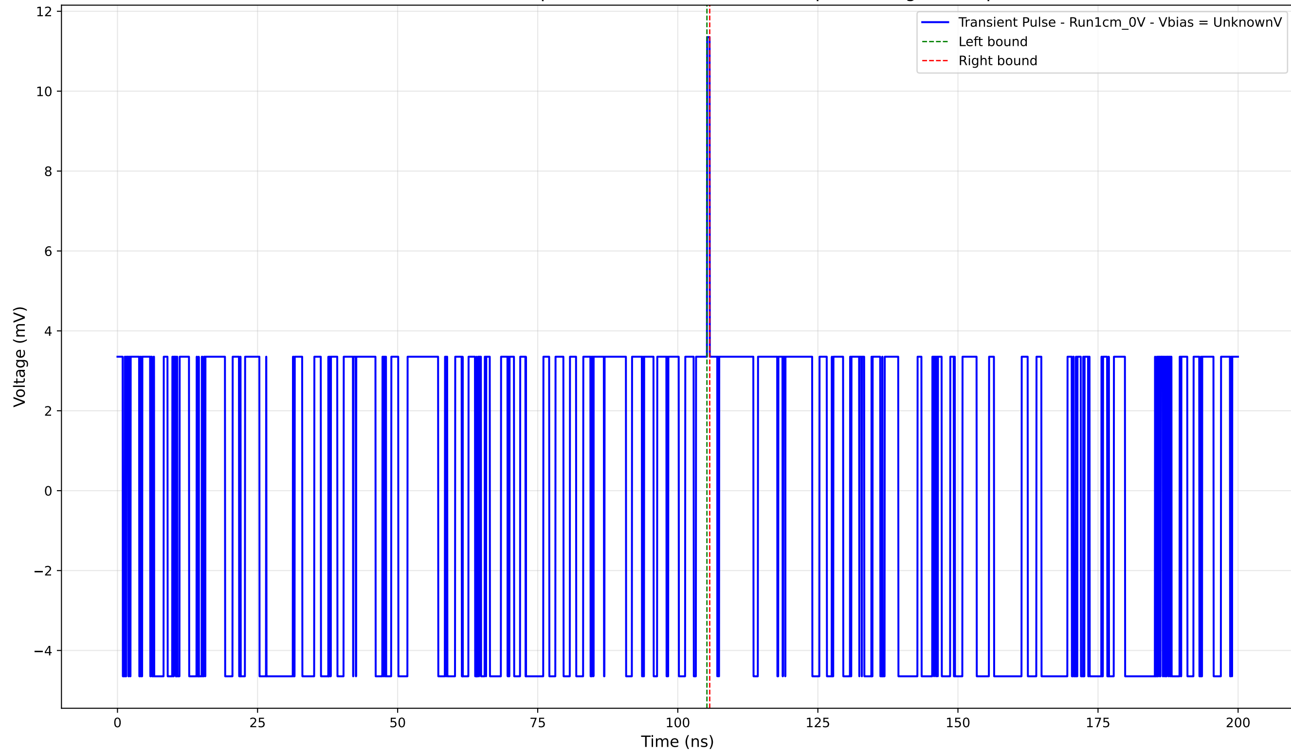
Transient Pulse - Sample: new1cm - Position: 815.0 \mu\text{m} - Charge: 0.11 pC
