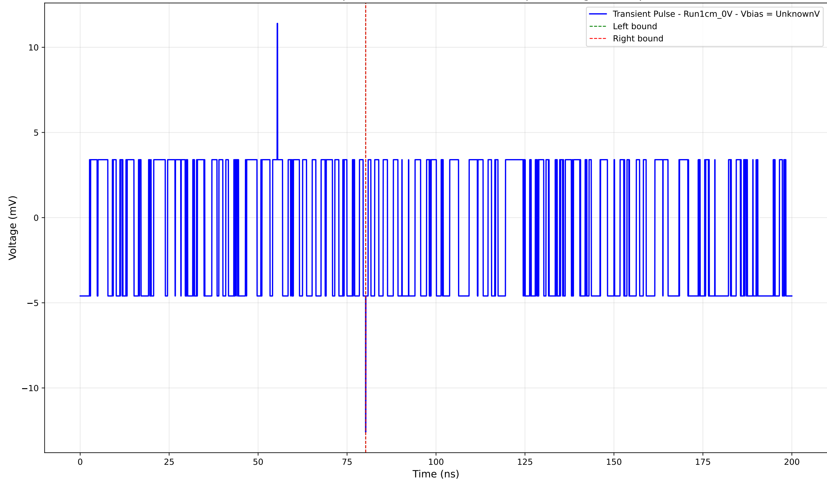
Transient Pulse - Sample: new1cm - Position: 1825.0 \mu\text{m} - Charge: -0.01 pC
