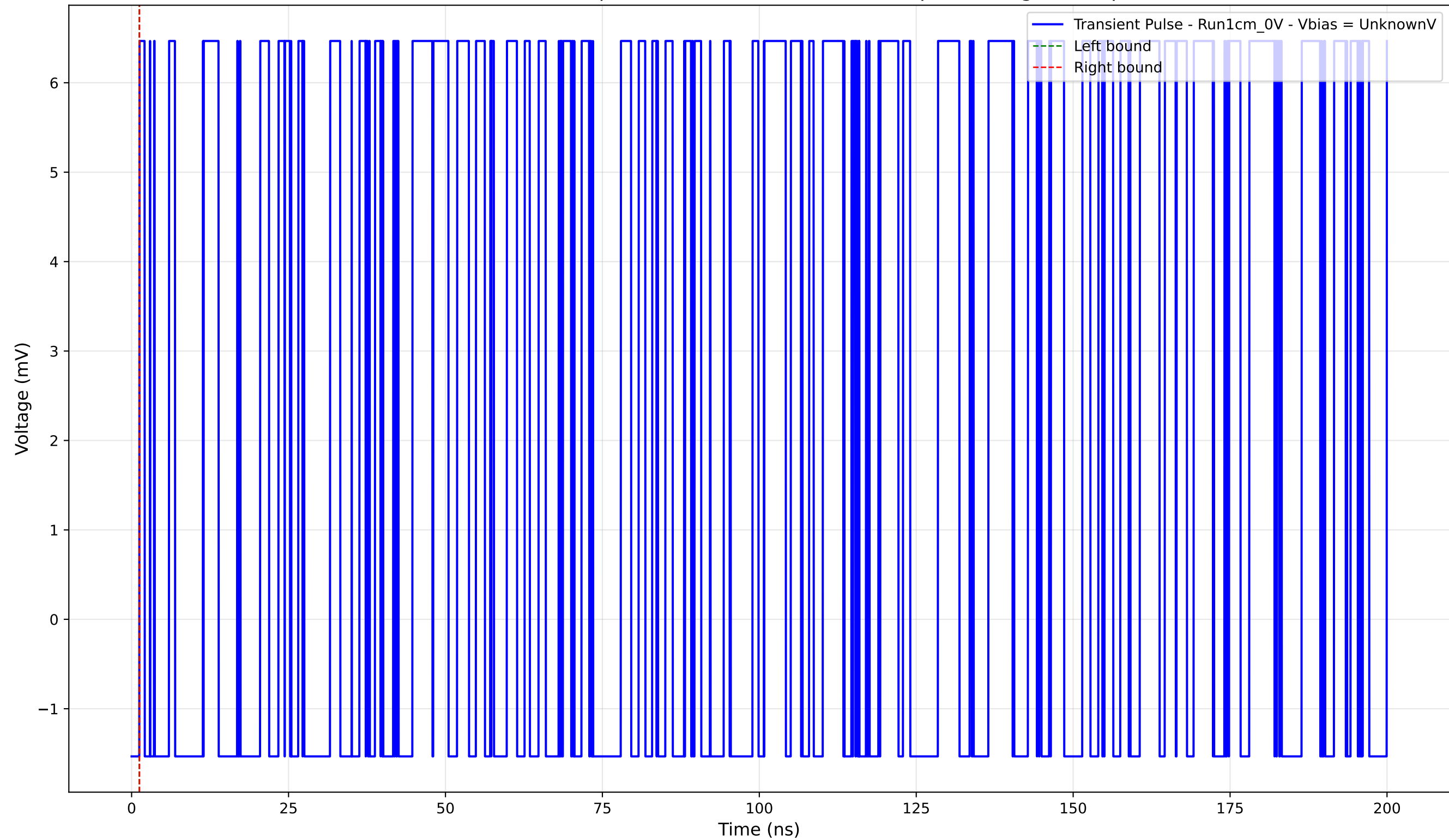
Transient Pulse - Sample: new1cm - Position: 3130.0 \mu\text{m} - Charge: 0.00 pC
