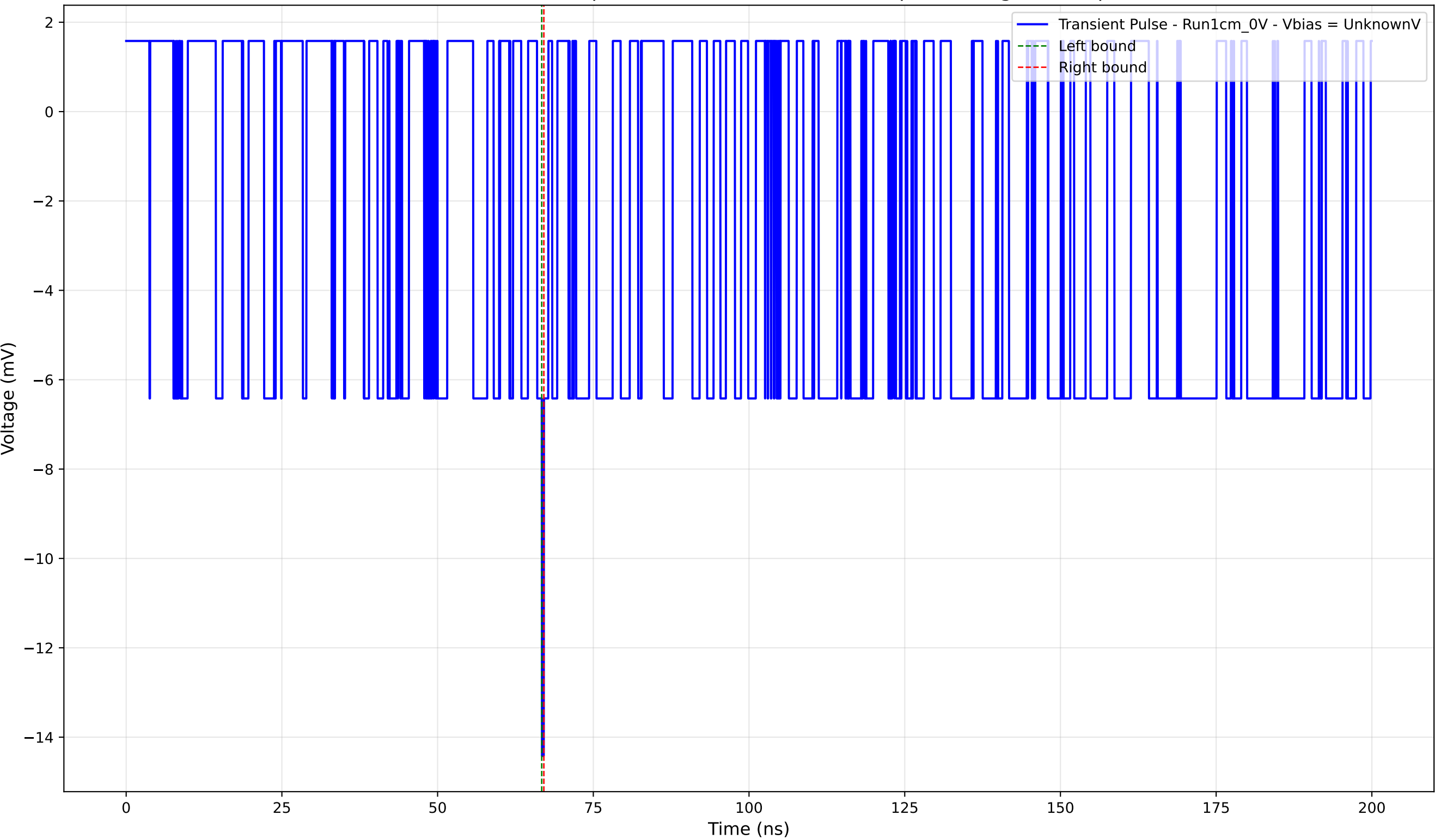
Transient Pulse - Sample: new1cm - Position: 365.0 \mu\text{m} - Charge: -0.09 pC
