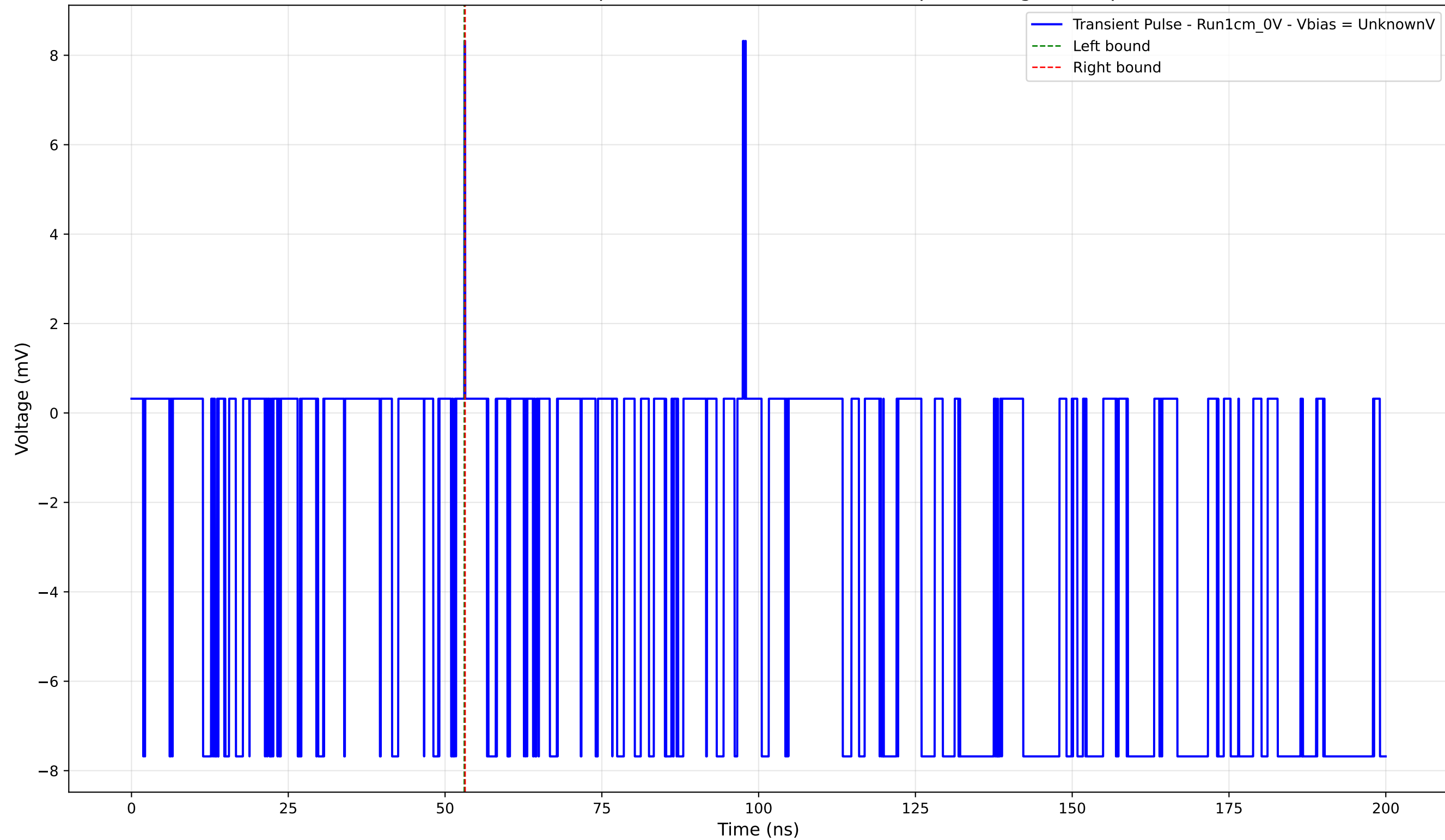
Transient Pulse - Sample: new1cm - Position: 5080.0 \mu\text{m} - Charge: 0.02 pC
