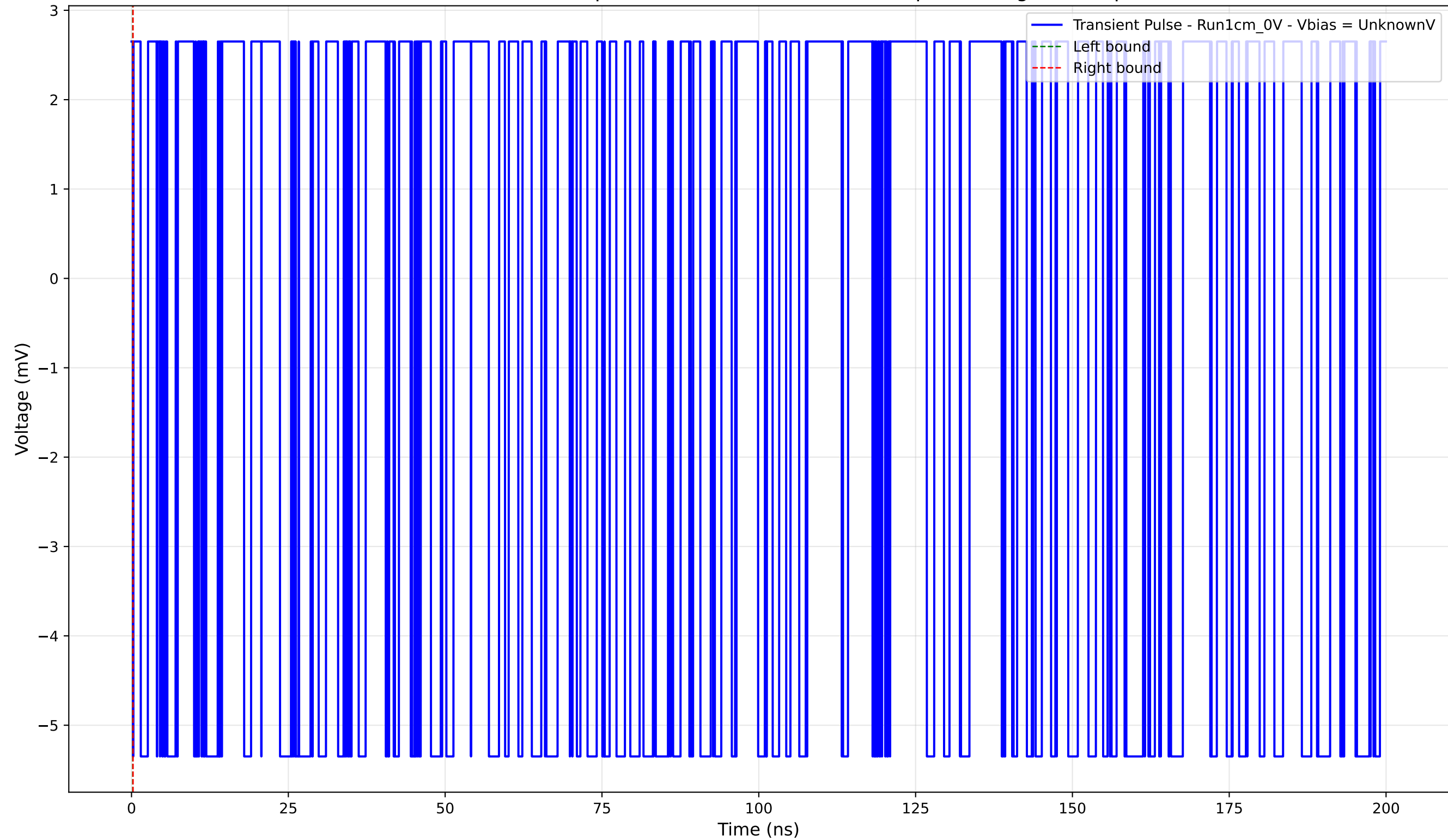
Transient Pulse - Sample: new1cm - Position: 2005.0 \mu\text{m} - Charge: -0.00 pC
