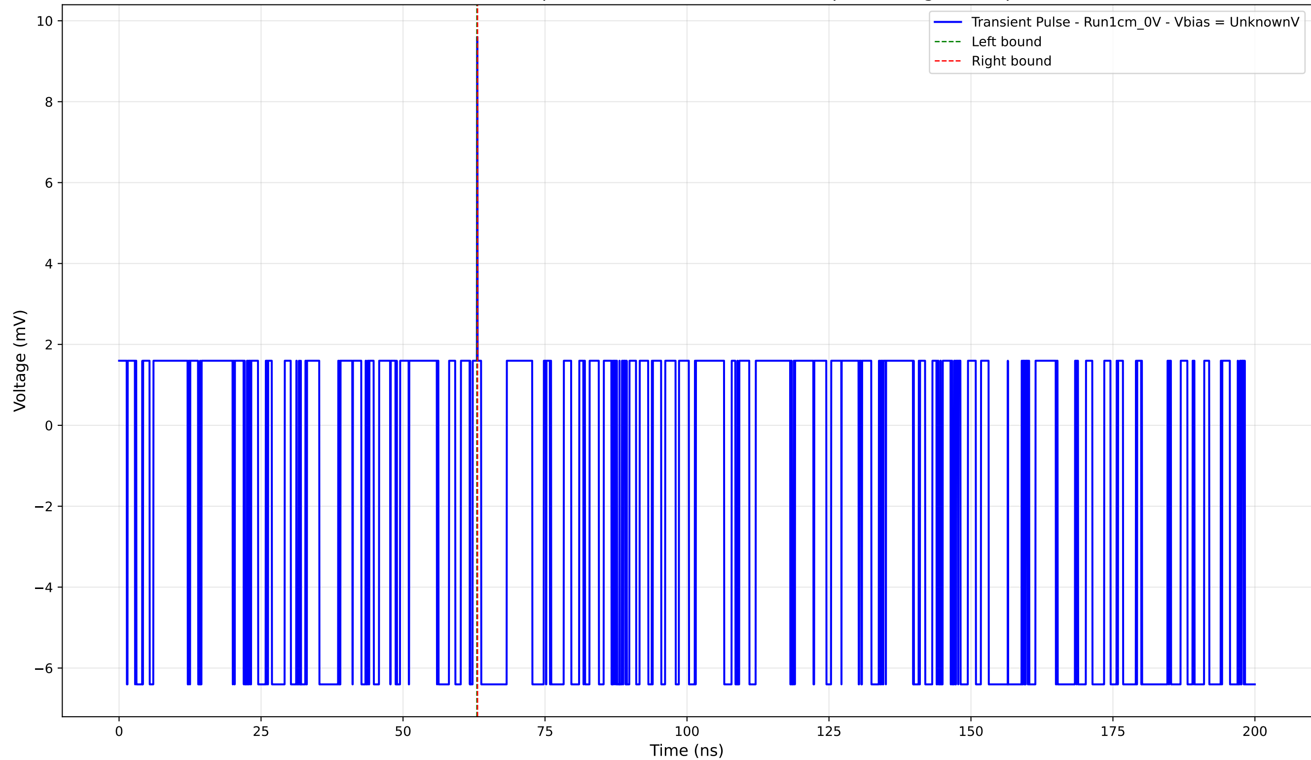
Transient Pulse - Sample: new1cm - Position: 1320.0 \mu\text{m} - Charge: 0.02 pC
