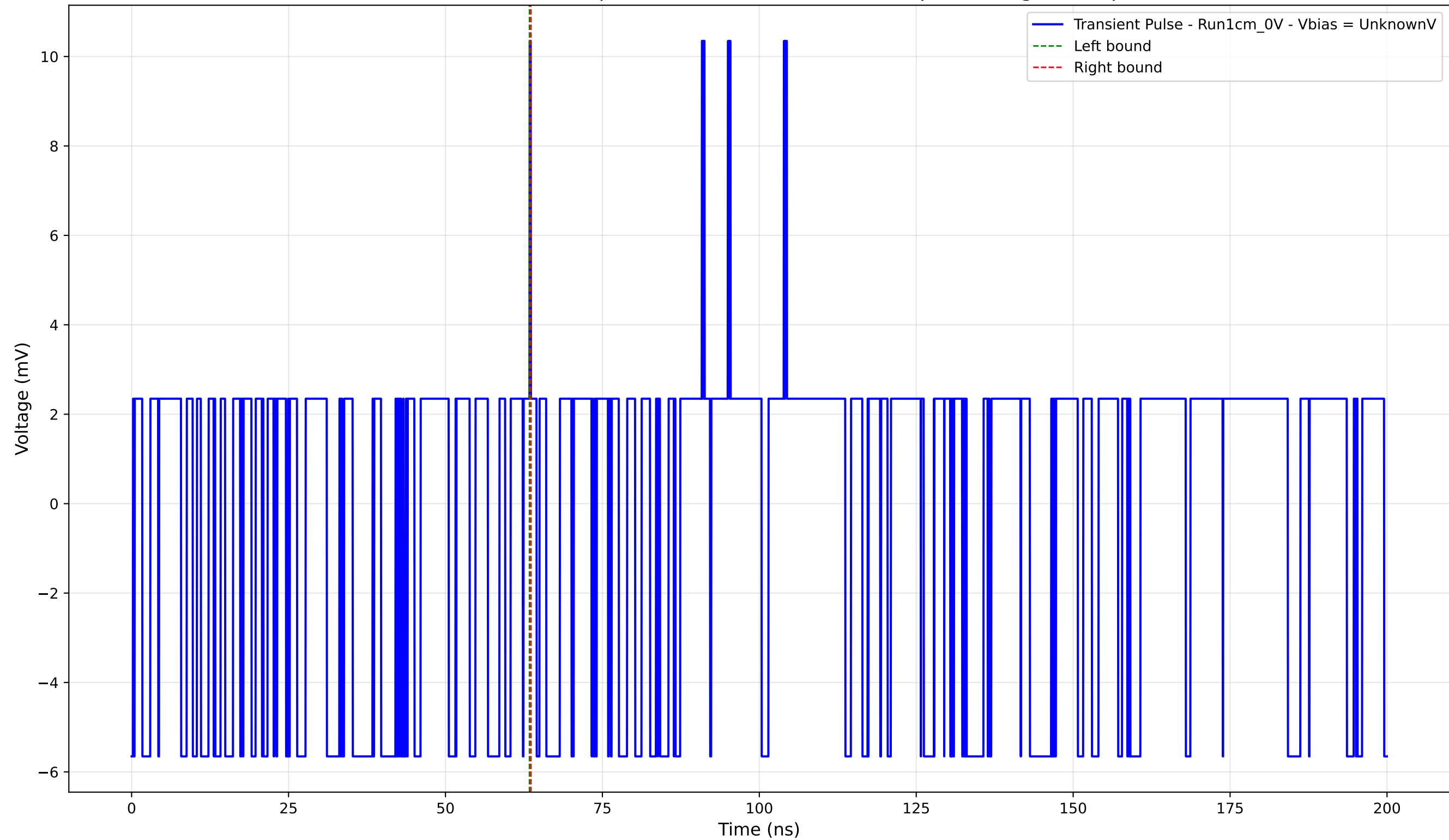
Transient Pulse - Sample: new1cm - Position: 5015.0 \mu\text{m} - Charge: 0.04 pC
