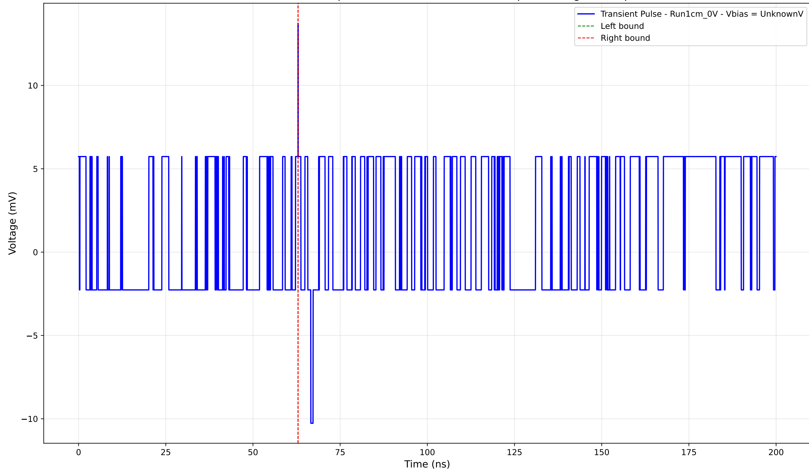
Transient Pulse - Sample: new1cm - Position: 2765.0 \mu\text{m} - Charge: 0.01 pC
