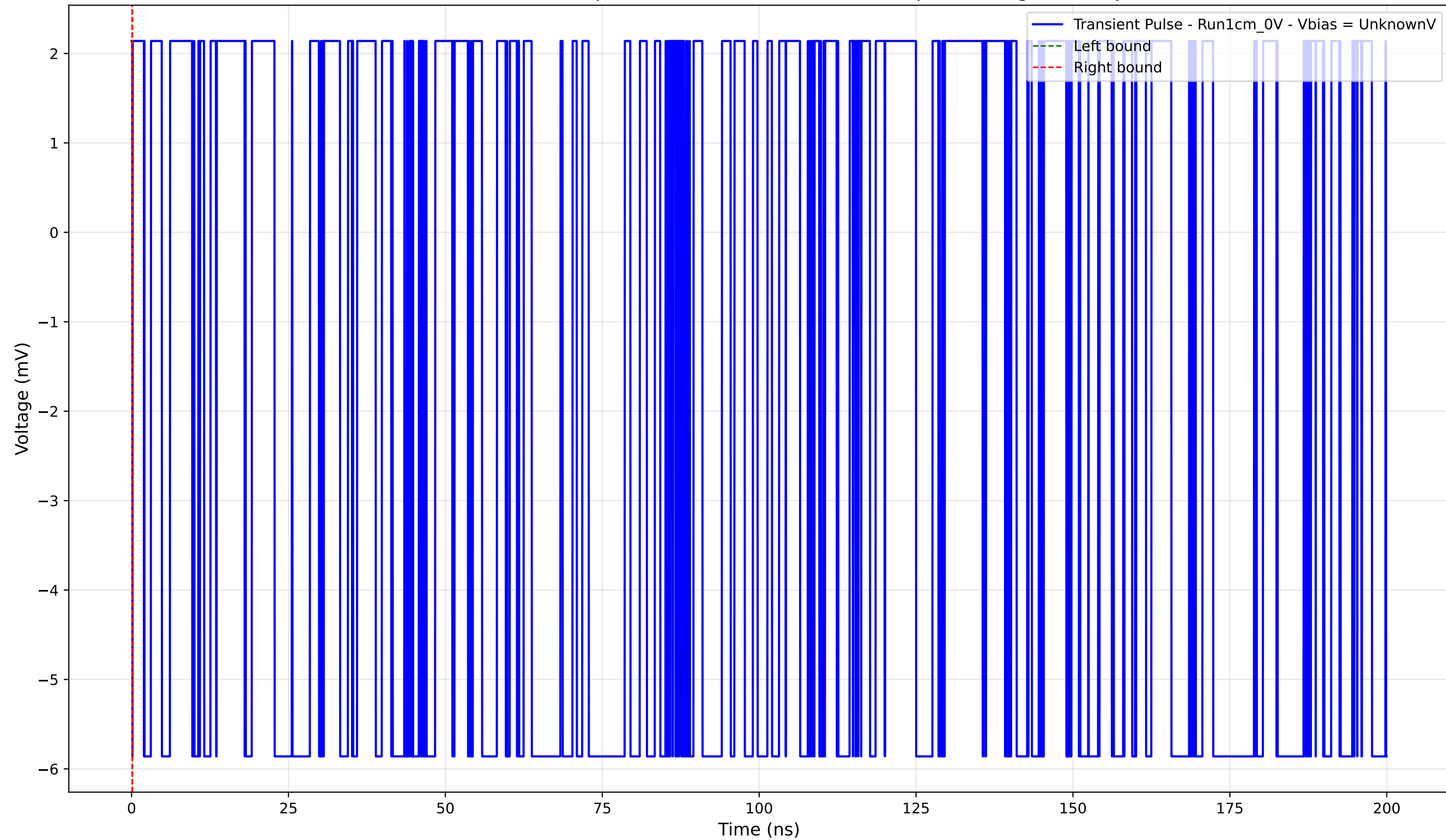
Transient Pulse - Sample: new1cm - Position: 3750.0 \mu\text{m} - Charge: -0.00 pC
