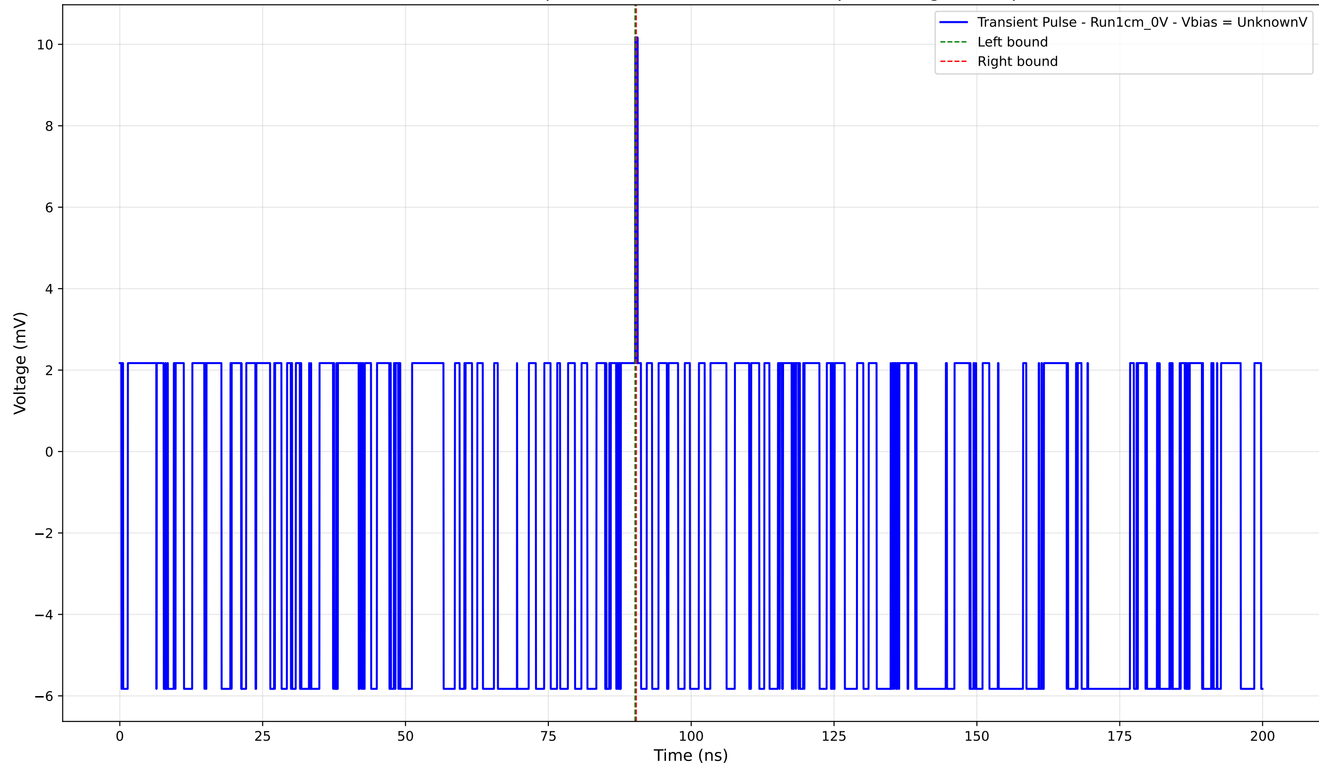
Transient Pulse - Sample: new1cm - Position: 1215.0 \mu\text{m} - Charge: 0.04 pC
