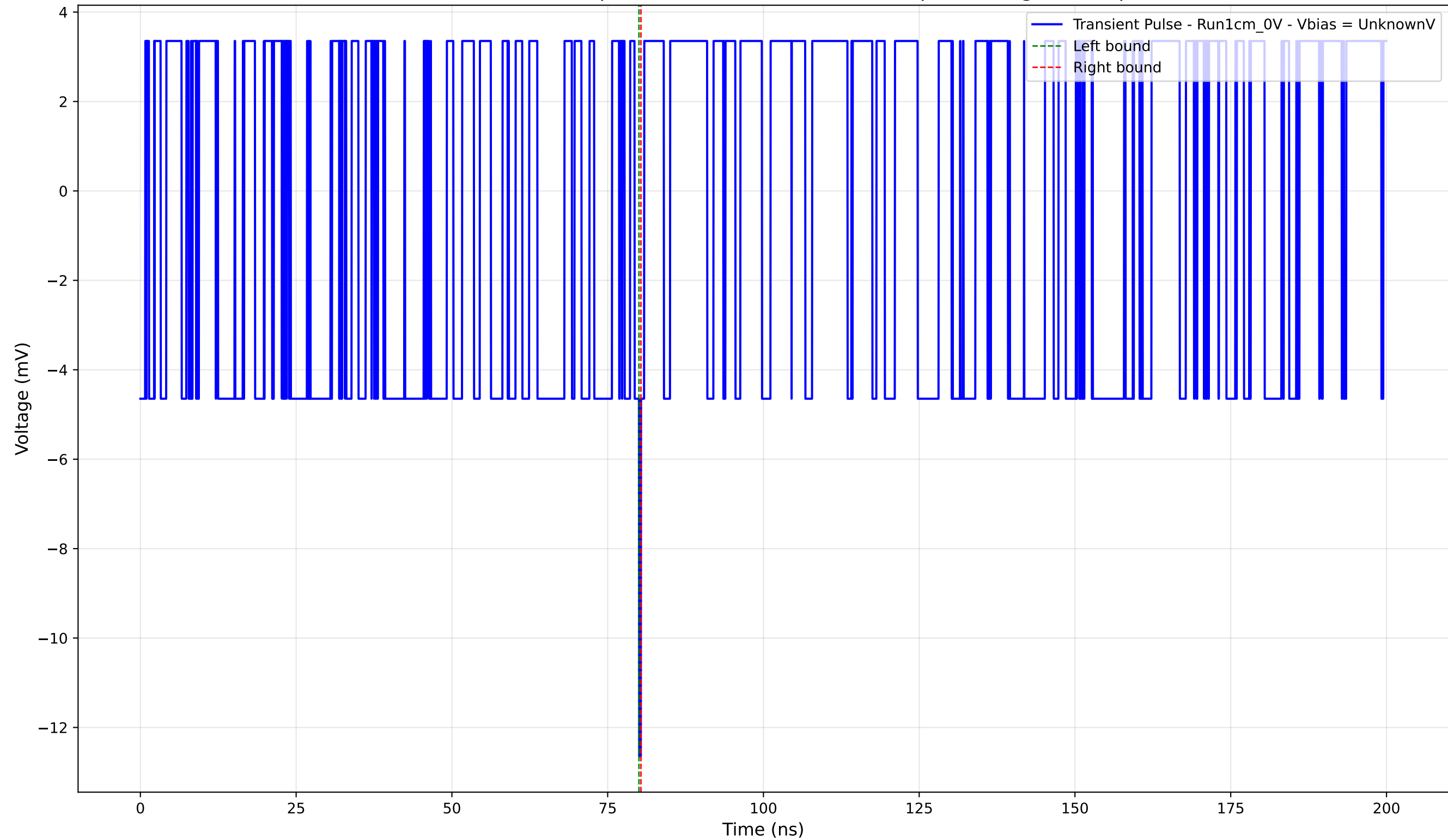
Transient Pulse - Sample: new1cm - Position: 2335.0 \mu\text{m} - Charge: -0.08 pC
