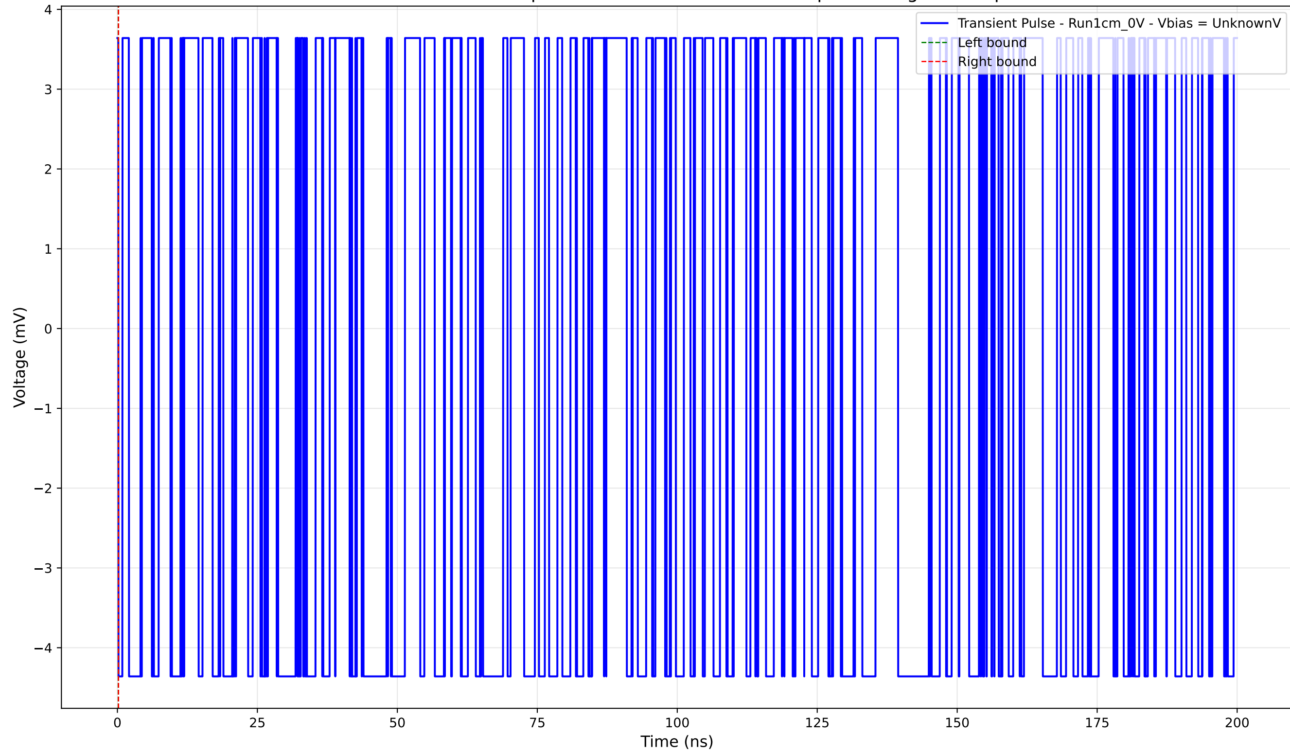
Transient Pulse - Sample: new1cm - Position: 3810.0 \mu\text{m} - Charge: -0.00 pC
