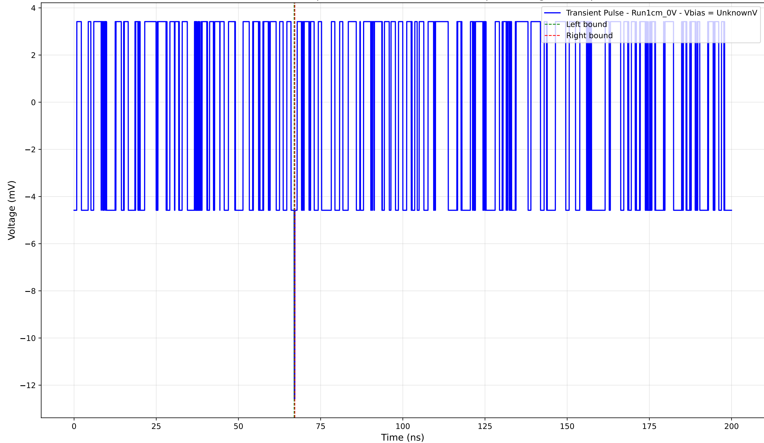
Transient Pulse - Sample: new1cm - Position: 1755.0 \mu\text{m} - Charge: -0.05 pC
