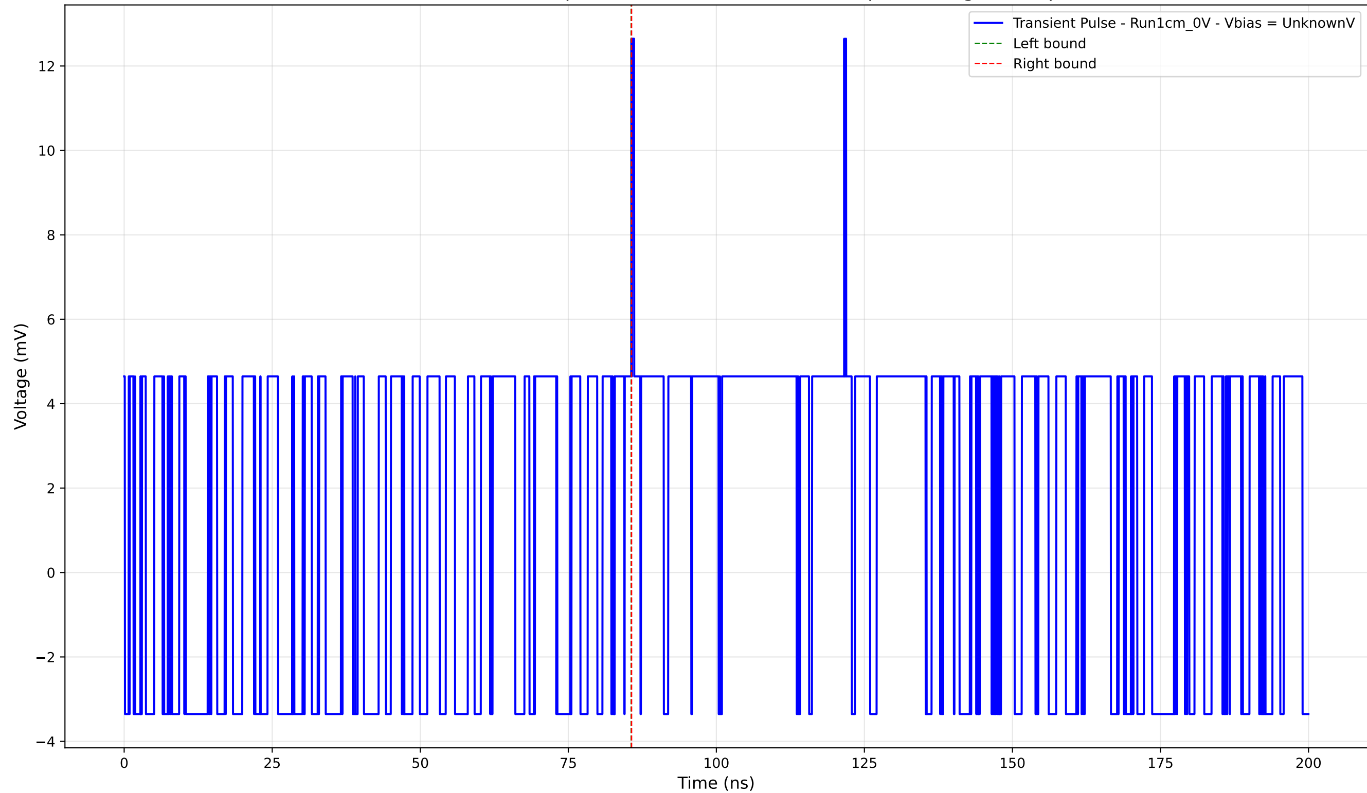
Transient Pulse - Sample: new1cm - Position: 3345.0 \mu\text{m} - Charge: 0.01 pC
