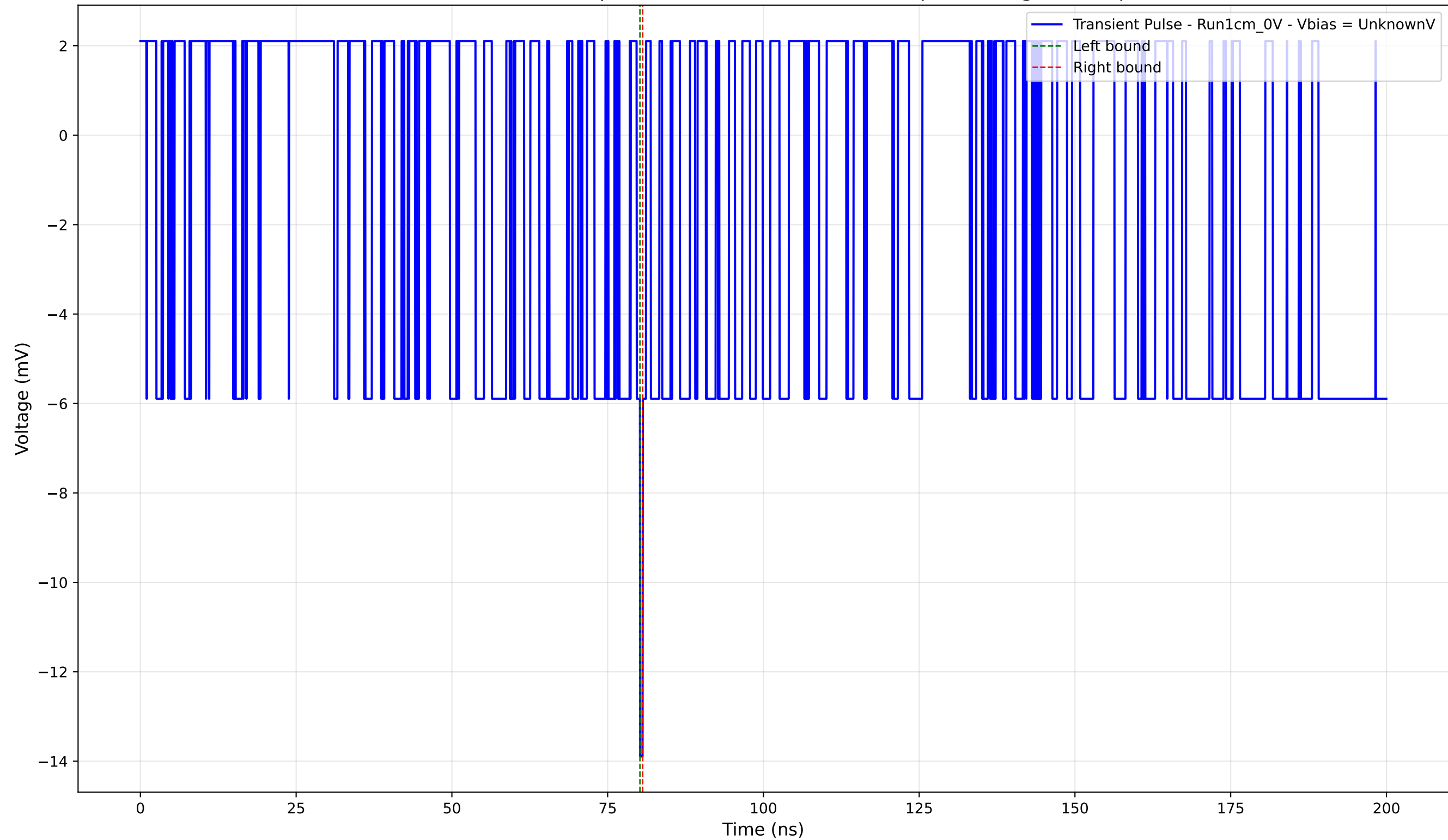
Transient Pulse - Sample: new1cm - Position: 3990.0 \mu\text{m} - Charge: -0.12 pC
