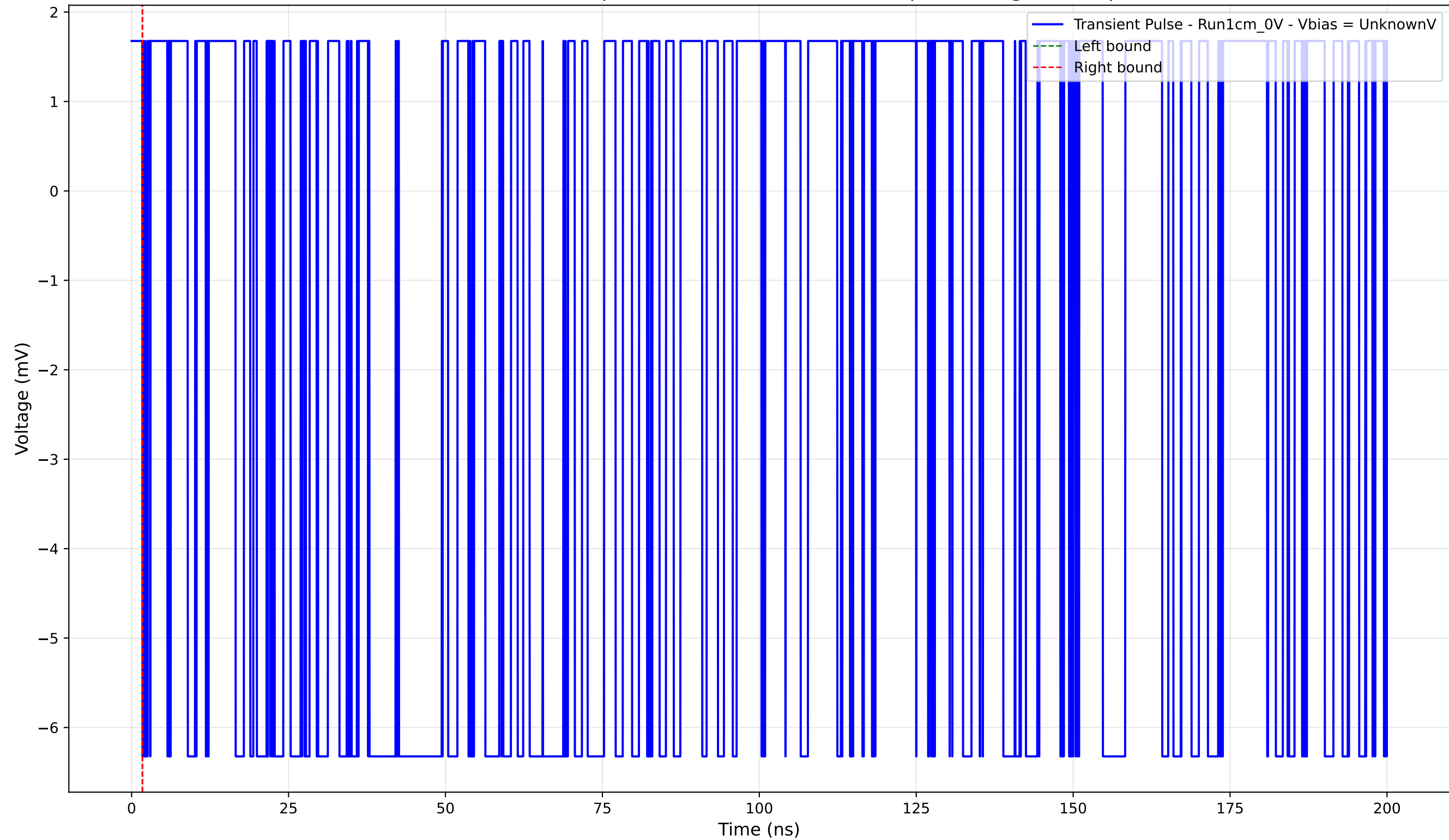
Transient Pulse - Sample: new1cm - Position: 915.0 \mu\text{m} - Charge: -0.00 pC
