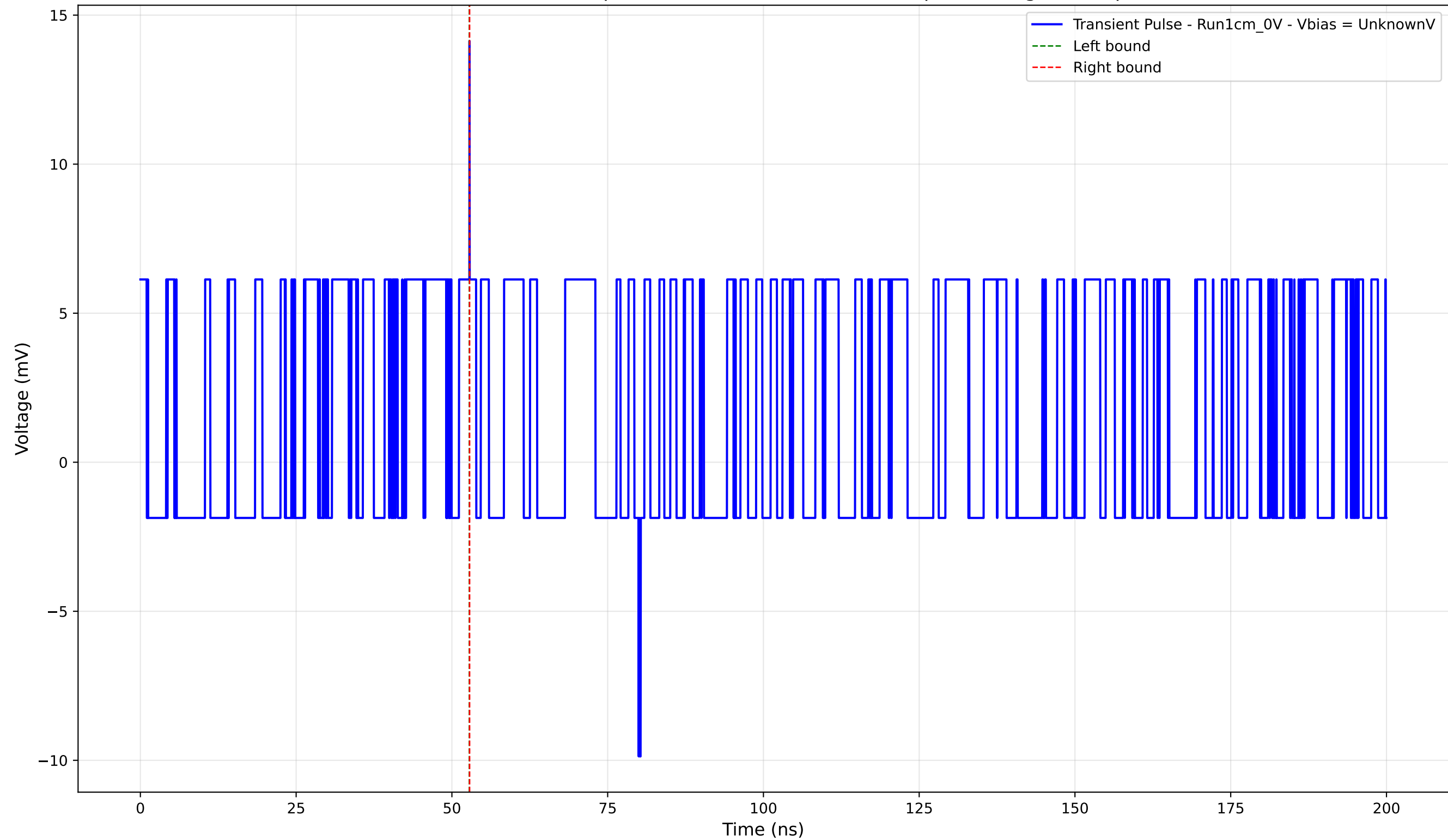
Transient Pulse - Sample: new1cm - Position: 1345.0 \mu\text{m} - Charge: 0.01 pC
