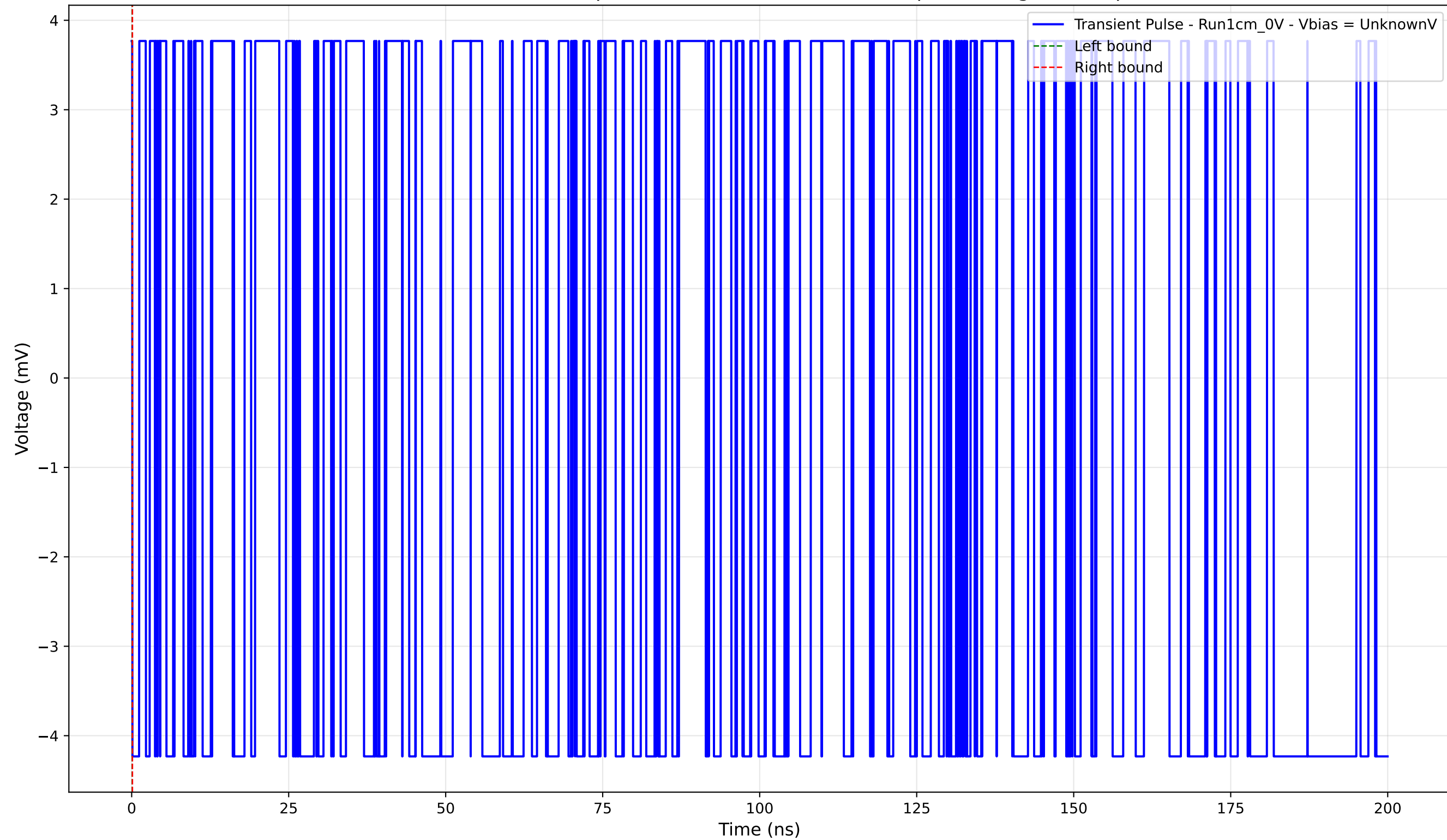
Transient Pulse - Sample: new1cm - Position: 3875.0 \mu\text{m} - Charge: -0.00 pC
