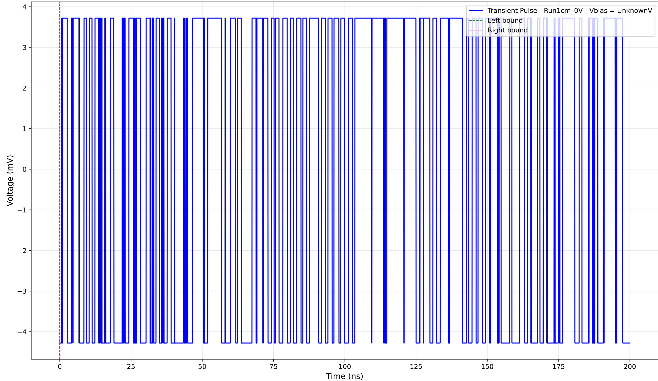
Transient Pulse - Sample: new1cm - Position: 45.0 \mu\text{m} - Charge: -0.00 pC
