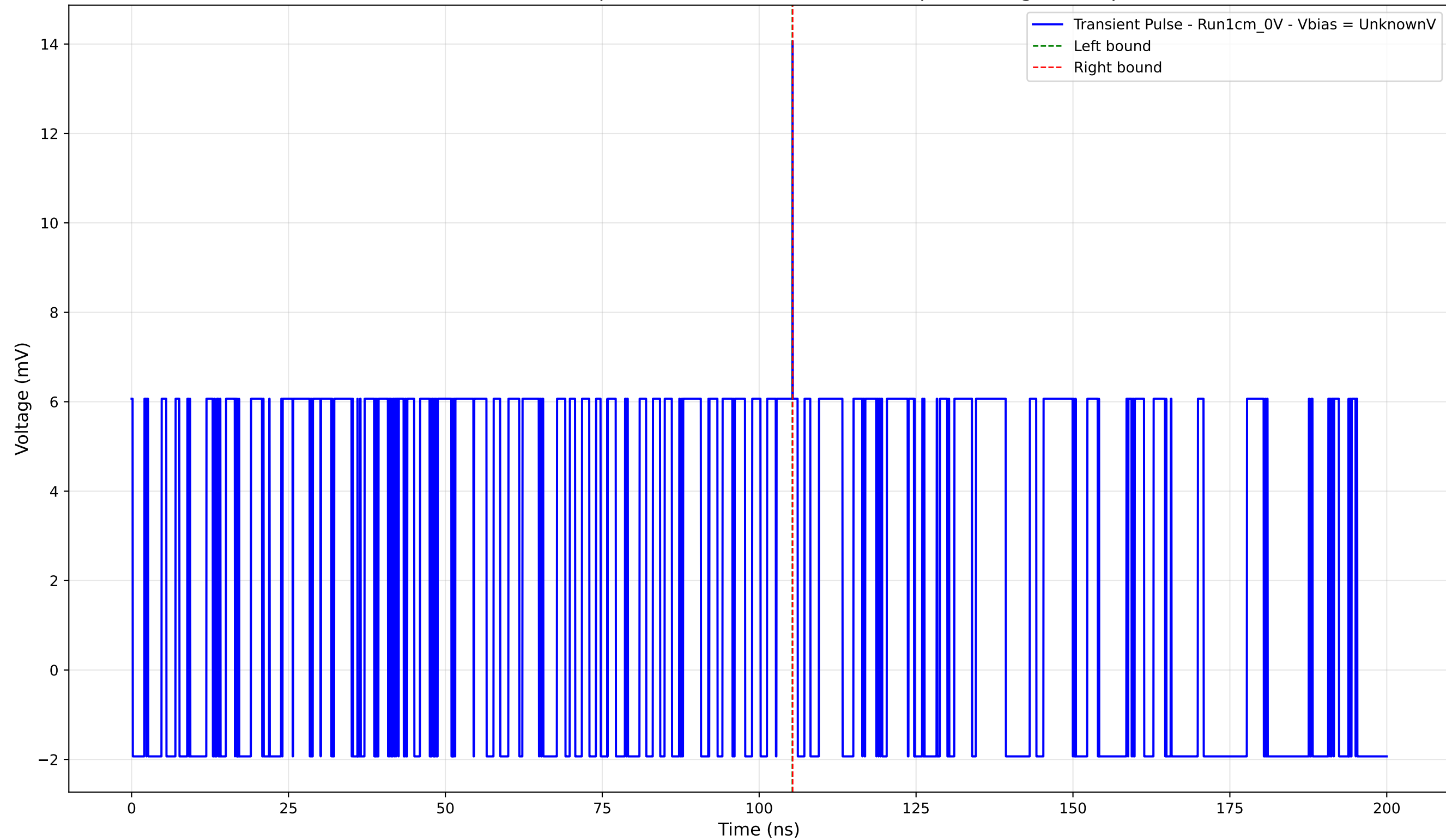
Transient Pulse - Sample: new1cm - Position: 1780.0 \mu\text{m} - Charge: 0.01 pC
