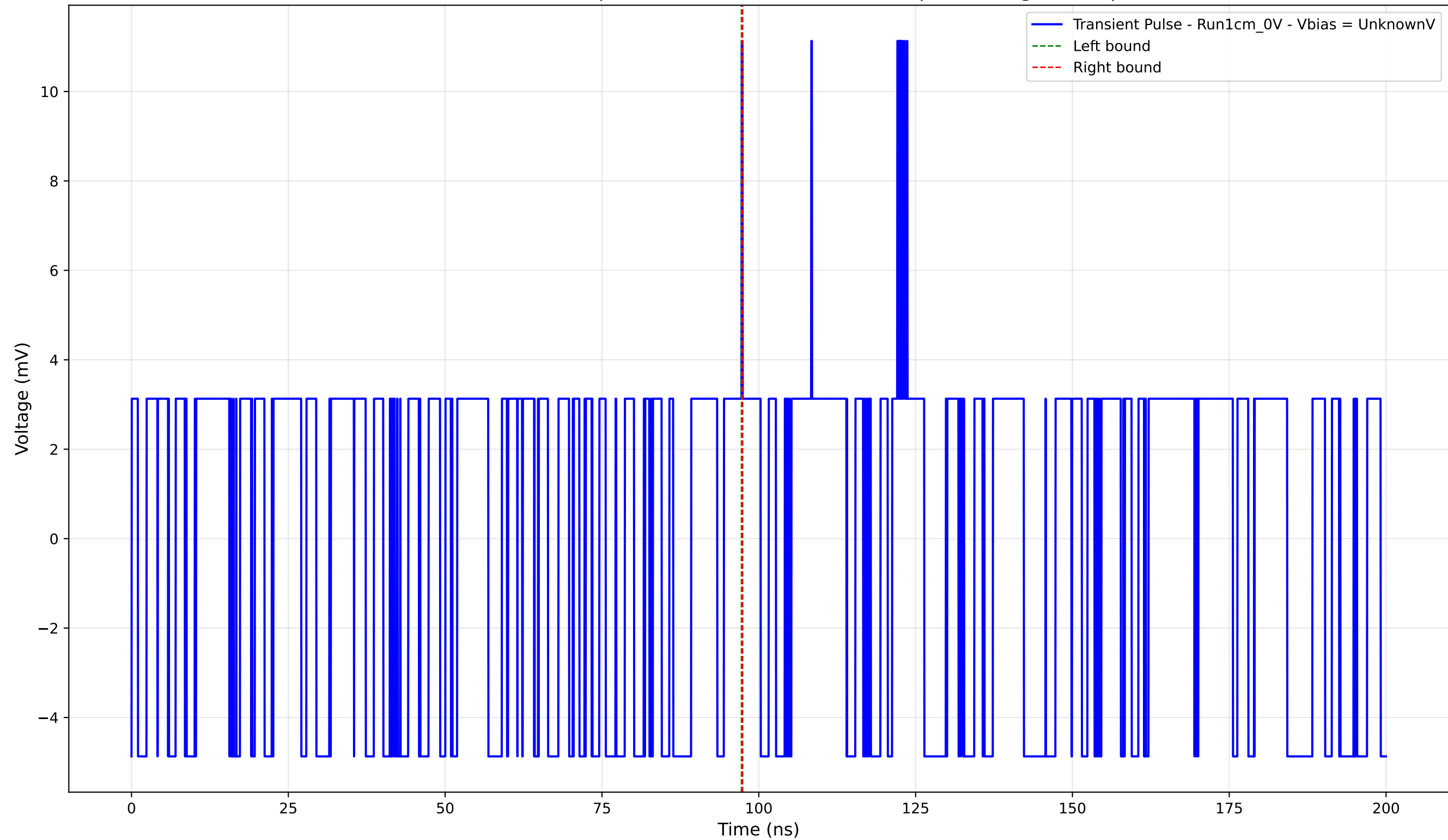
Transient Pulse - Sample: new1cm - Position: 4375.0 \mu\text{m} - Charge: 0.04 pC
