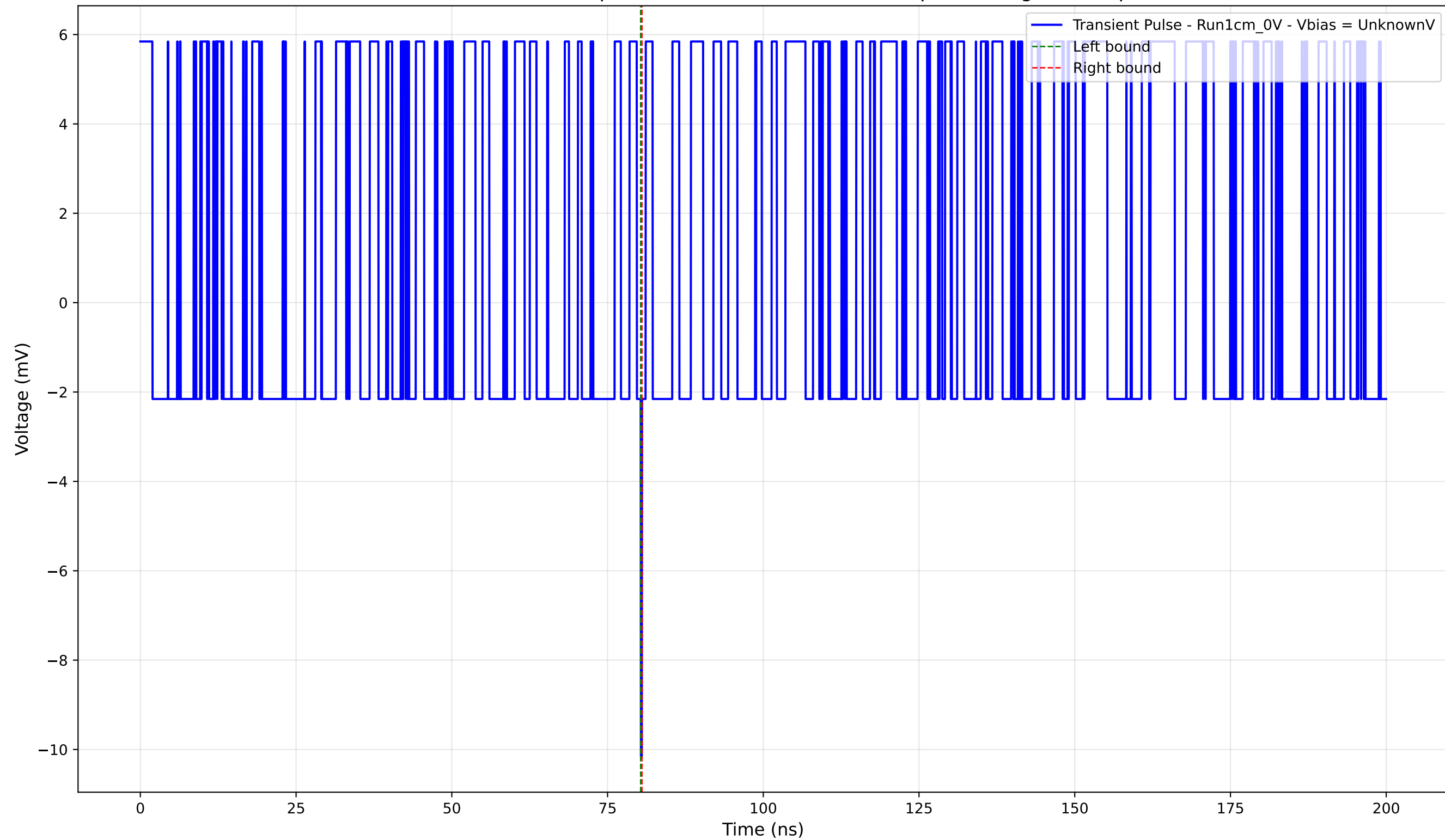
Transient Pulse - Sample: new1cm - Position: 1150.0 \mu\text{m} - Charge: -0.04 pC
