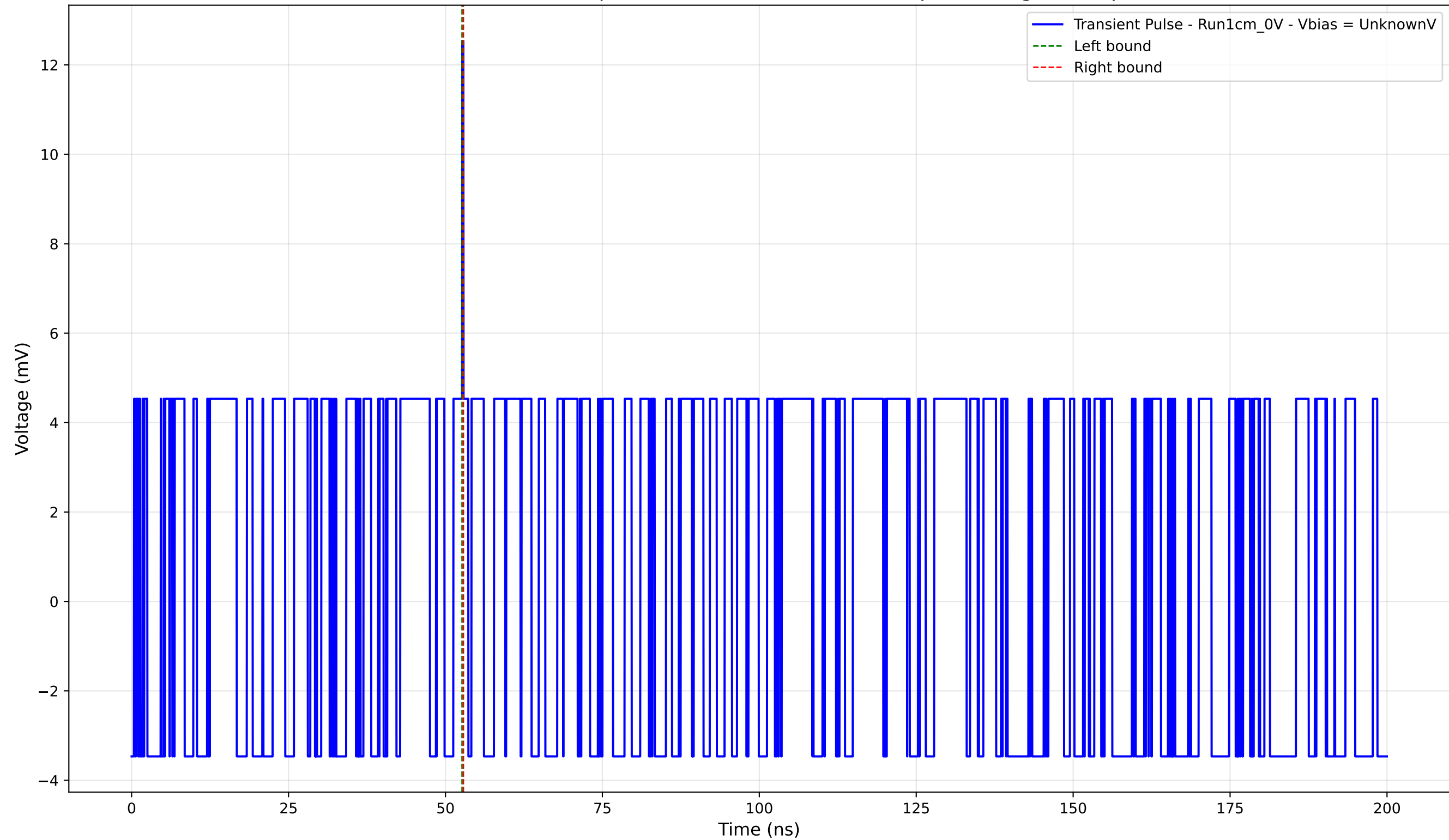
Transient Pulse - Sample: new1cm - Position: 2595.0 \mu\text{m} - Charge: 0.05 pC
