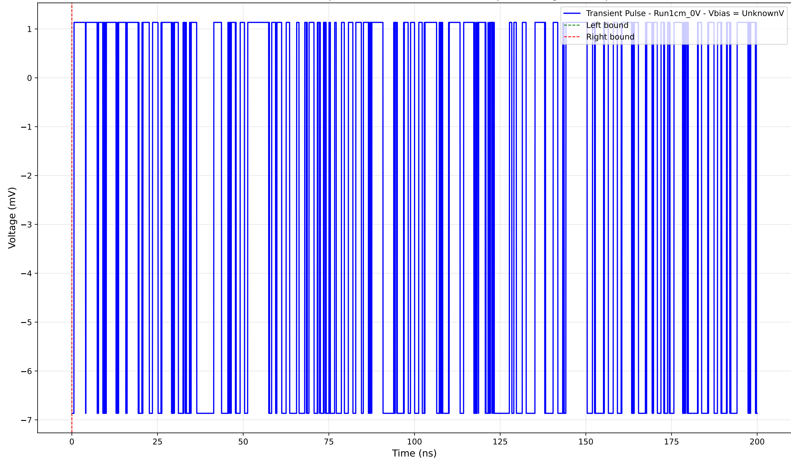
Transient Pulse - Sample: new1cm - Position: 680.0 \mu\text{m} - Charge: -0.00 pC
