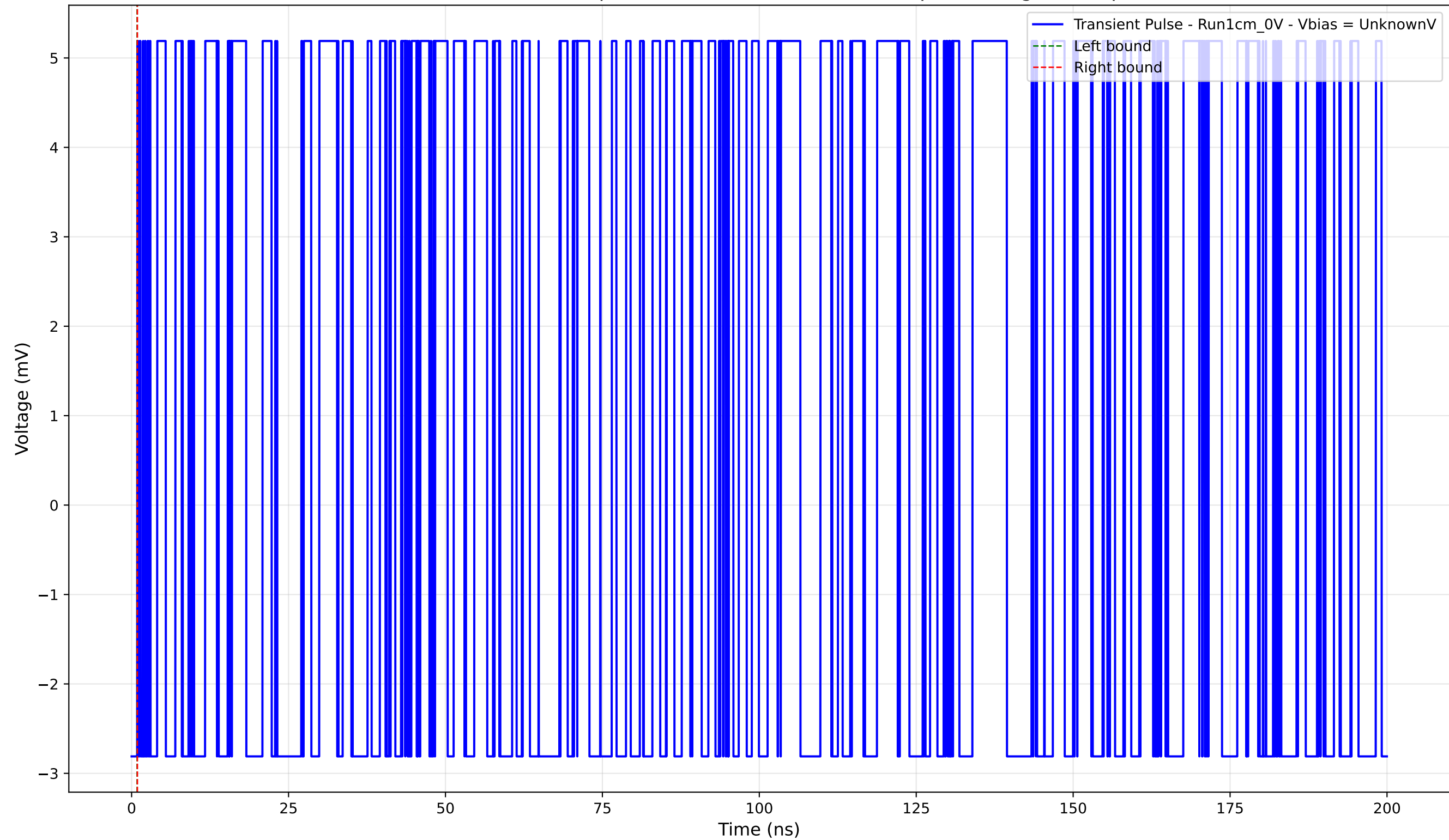
Transient Pulse - Sample: new1cm - Position: 1405.0 \mu\text{m} - Charge: 0.00 pC
