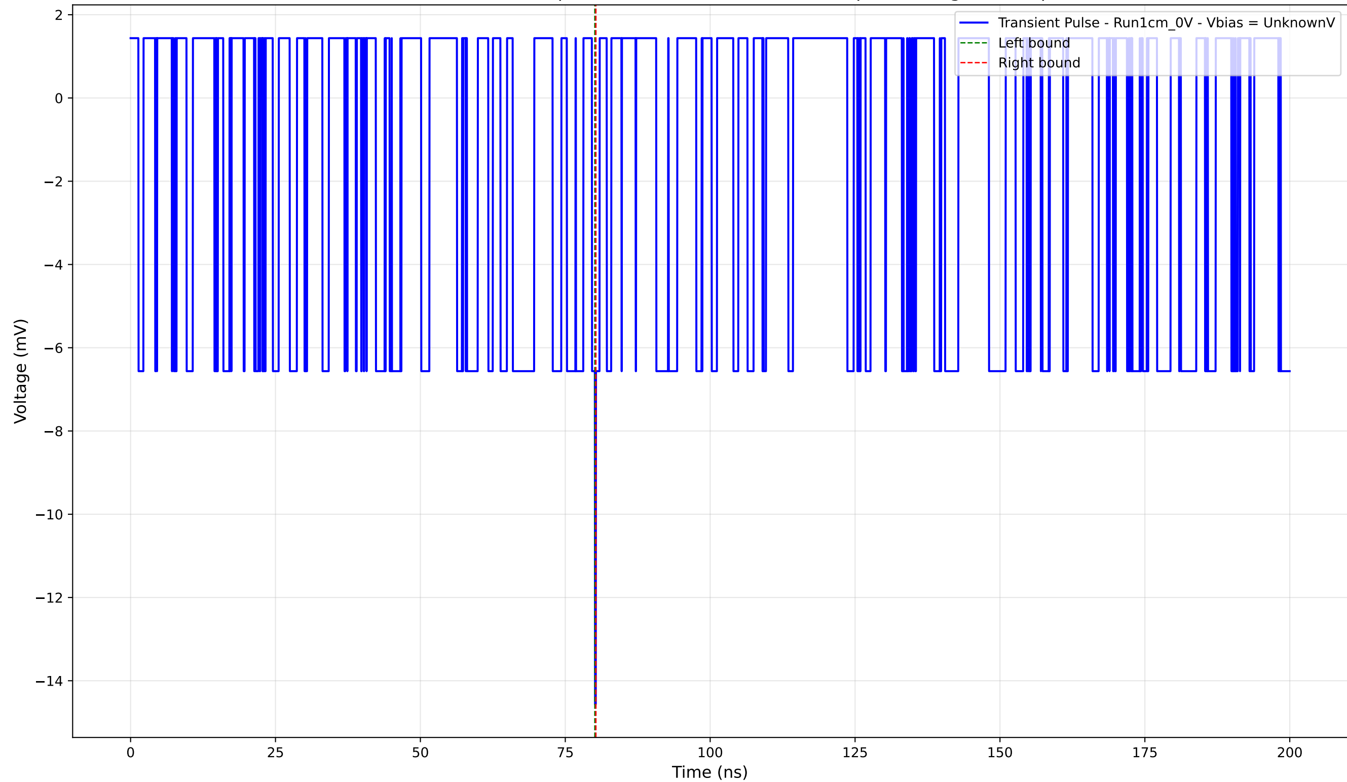
Transient Pulse - Sample: new1cm - Position: 1070.0 \mu\text{m} - Charge: -0.05 pC
