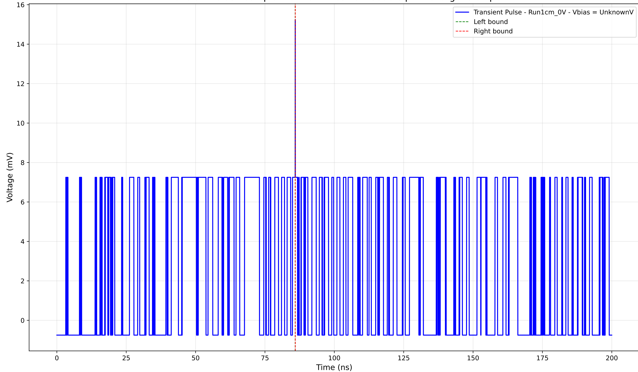
Transient Pulse - Sample: new1cm -Position: 3350.0 \mu\text{m} - Charge: 0.02 pC
