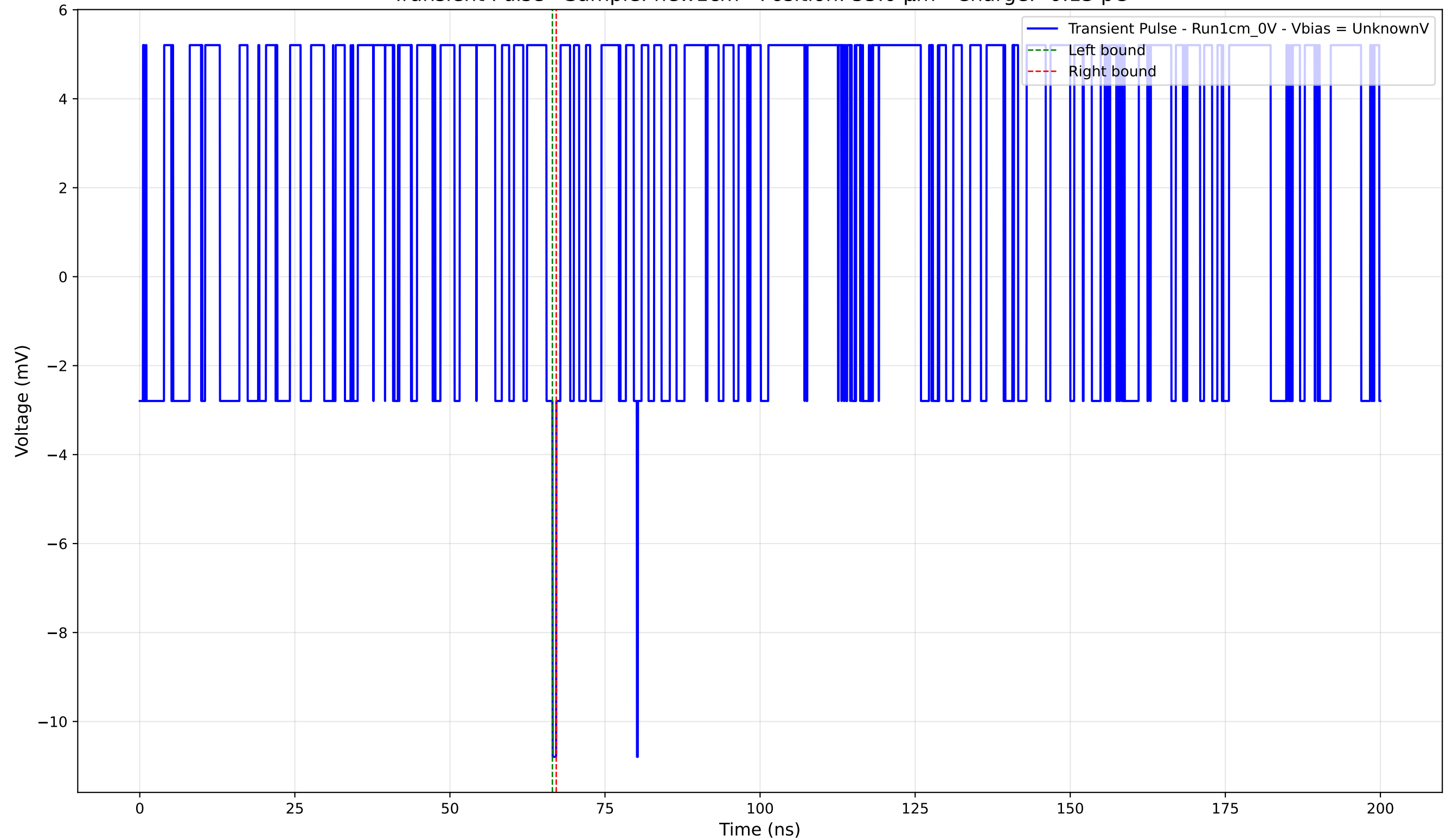
Transient Pulse - Sample: new1cm - Position: 55.0 \mu\text{m} - Charge: -0.13 pC
