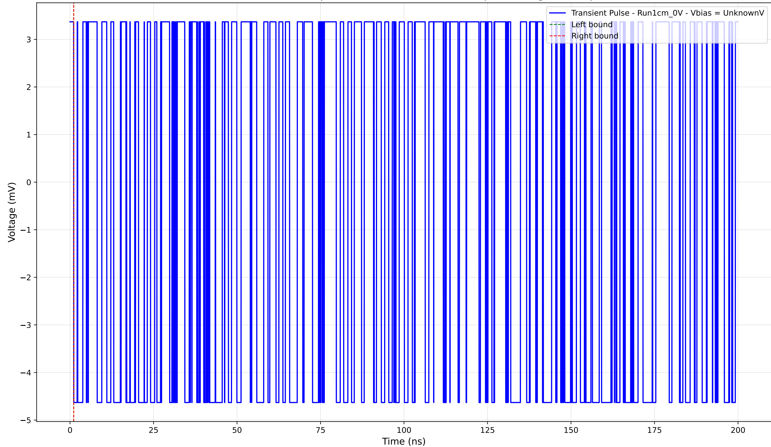
Transient Pulse - Sample: new1cm - Position: 380.0 \mu\text{m} - Charge: -0.00 pC
