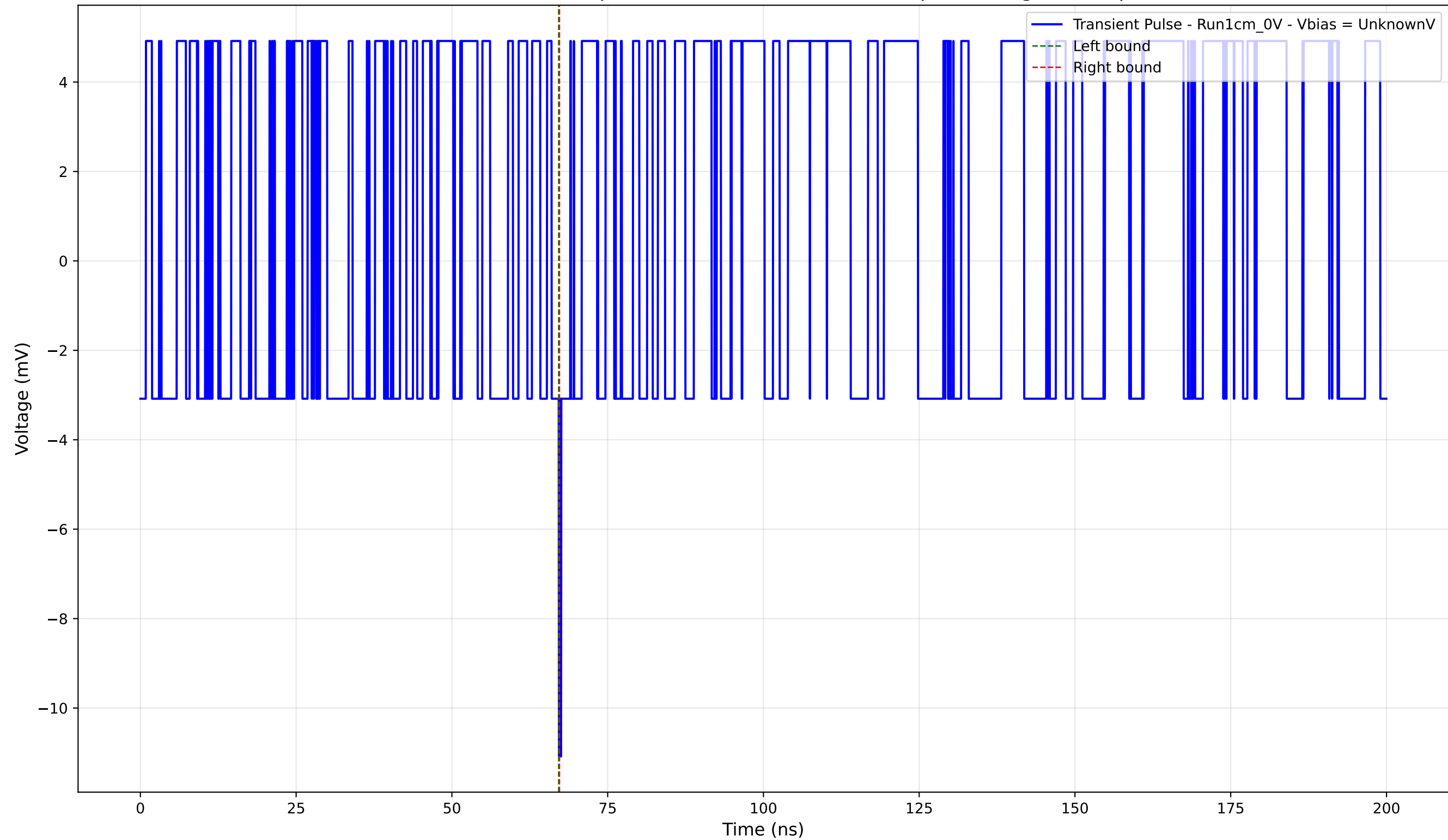
Transient Pulse - Sample: new1cm - Position: 4970.0 \mu\text{m} - Charge: -0.02 pC
