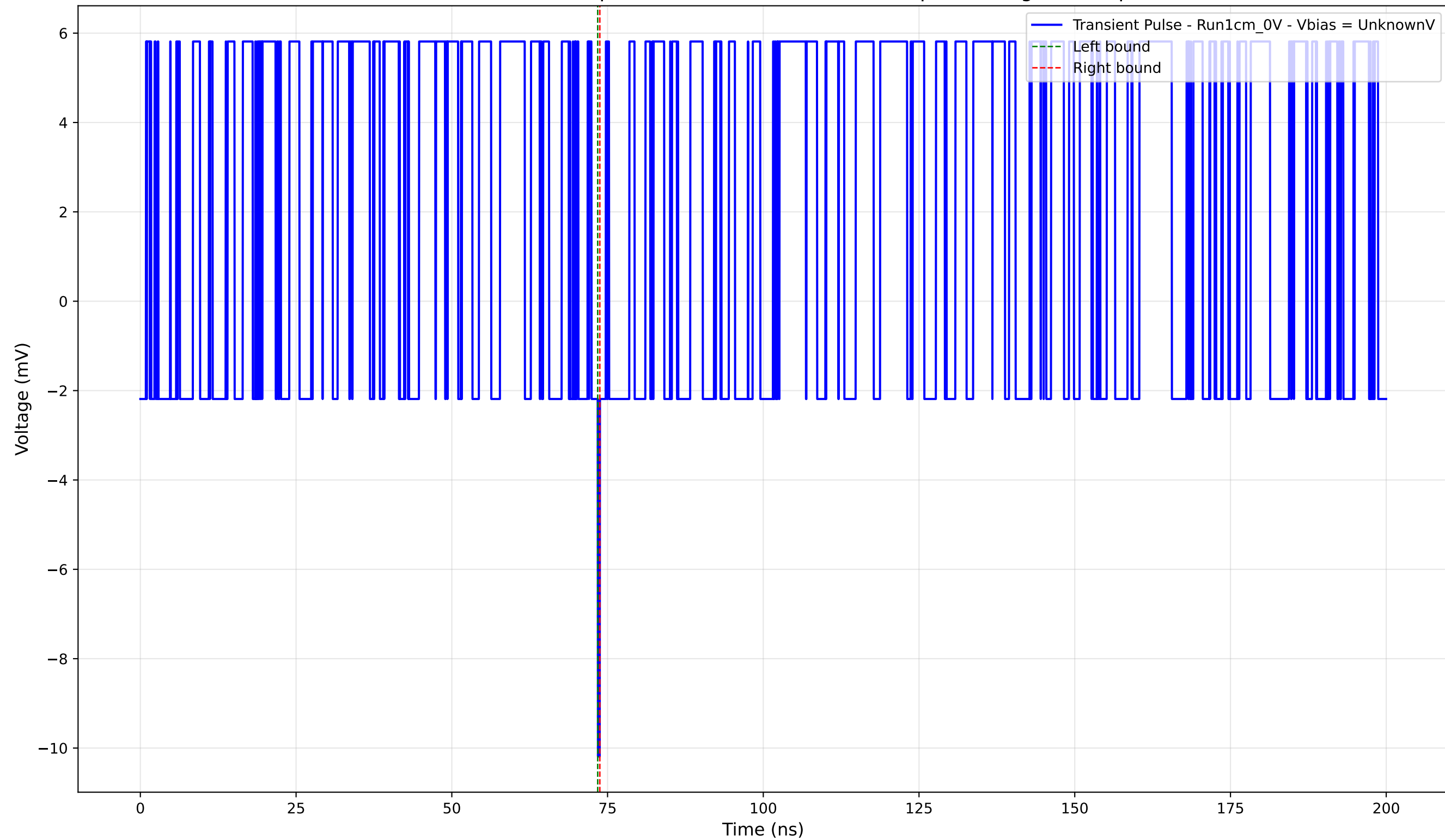
Transient Pulse - Sample: new1cm - Position: 2570.0 \mu\text{m} - Charge: -0.07 pC
