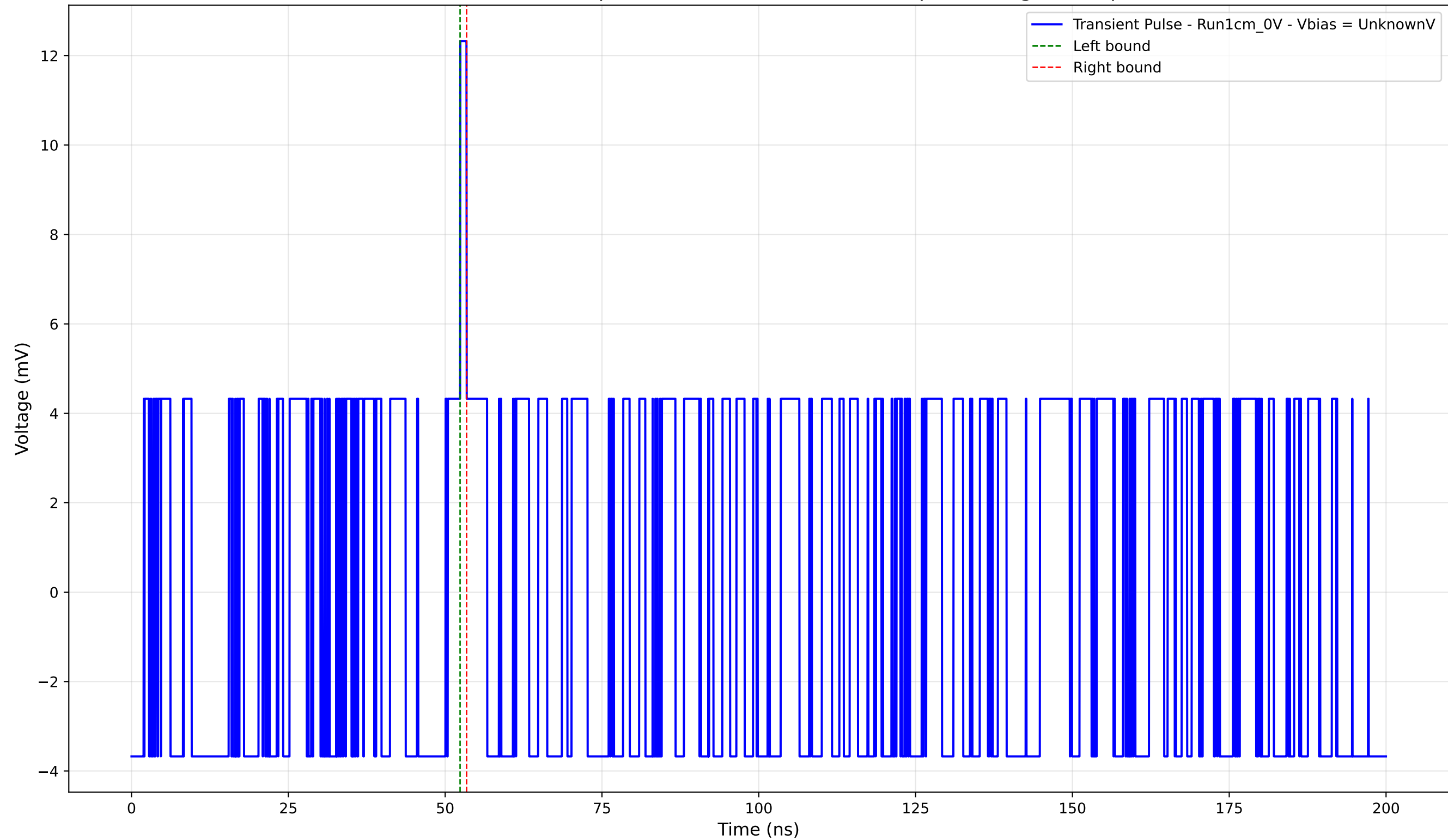
Transient Pulse - Sample: new1cm - Position: 1930.0 \mu\text{m} - Charge: 0.25 pC
