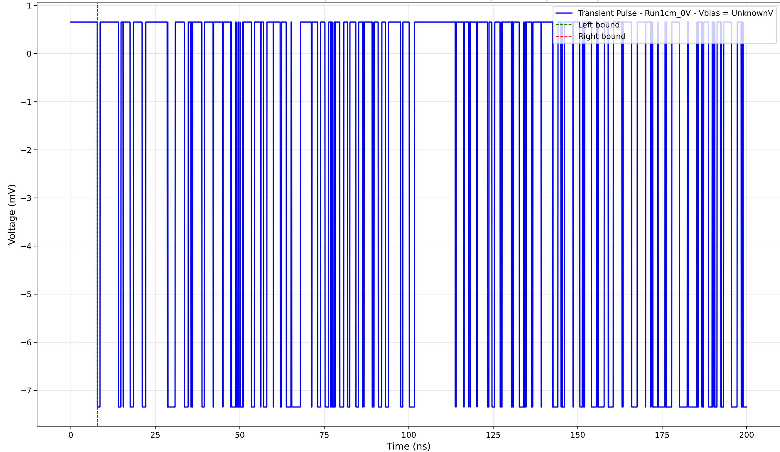
Transient Pulse - Sample: new1cm - Position: 770.0 \mu\text{m} - Charge: -0.00 pC
