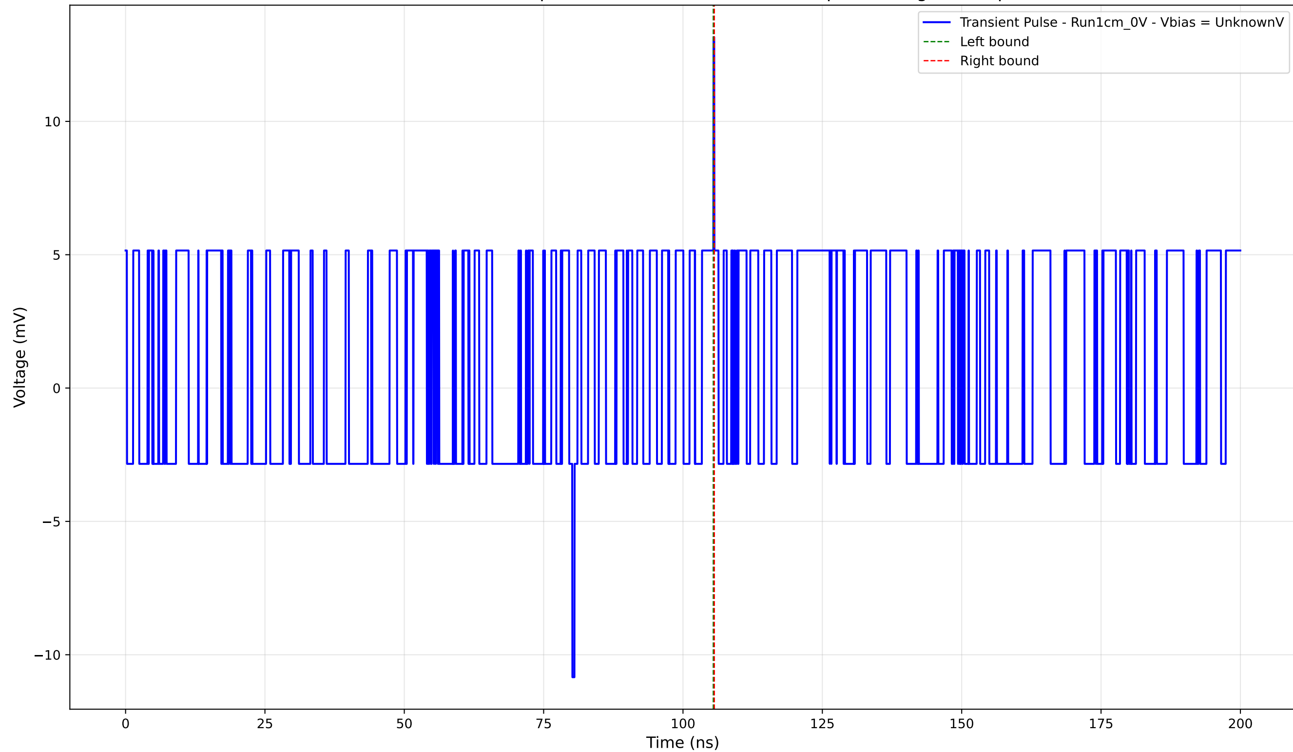
Transient Pulse - Sample: new1cm - Position: 2825.0 \mu\text{m} - Charge: 0.04 pC
