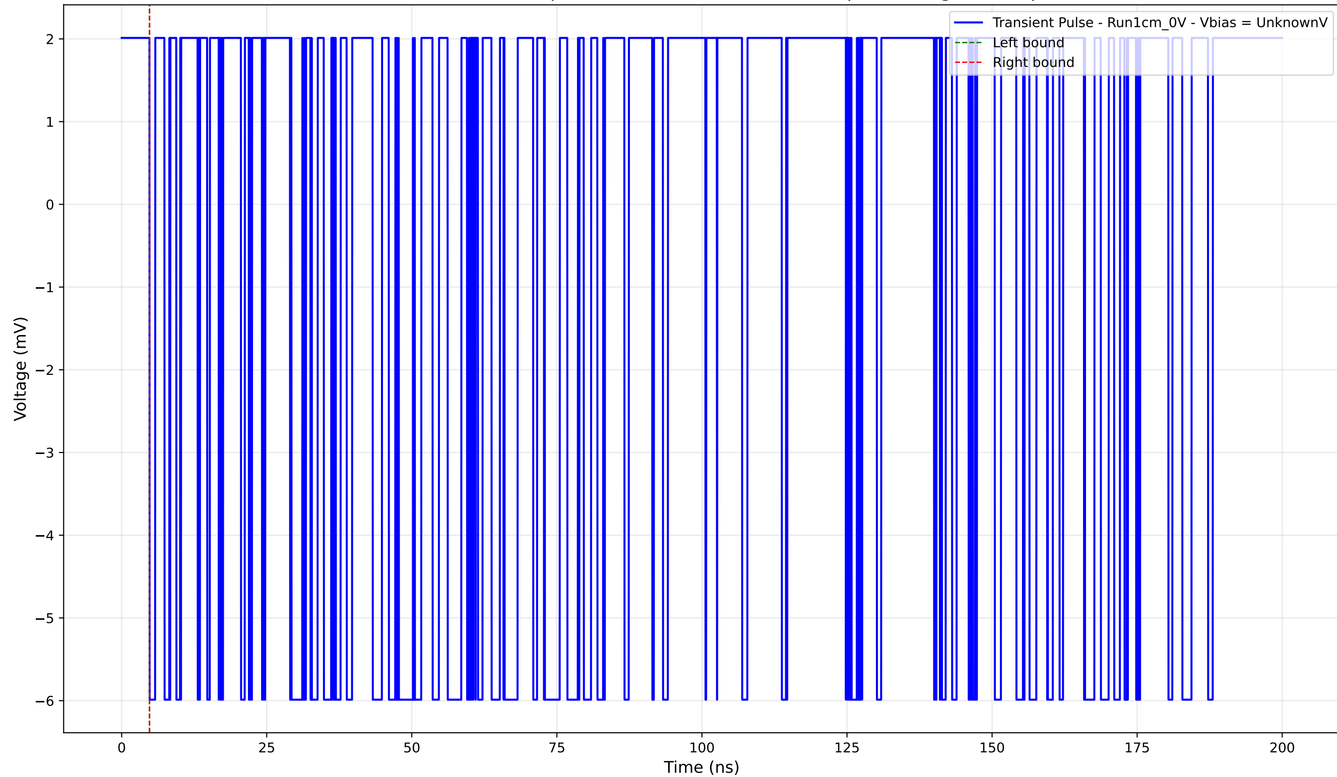
Transient Pulse - Sample: new1cm - Position: 3380.0 \mu\text{m} - Charge: -0.00 pC
