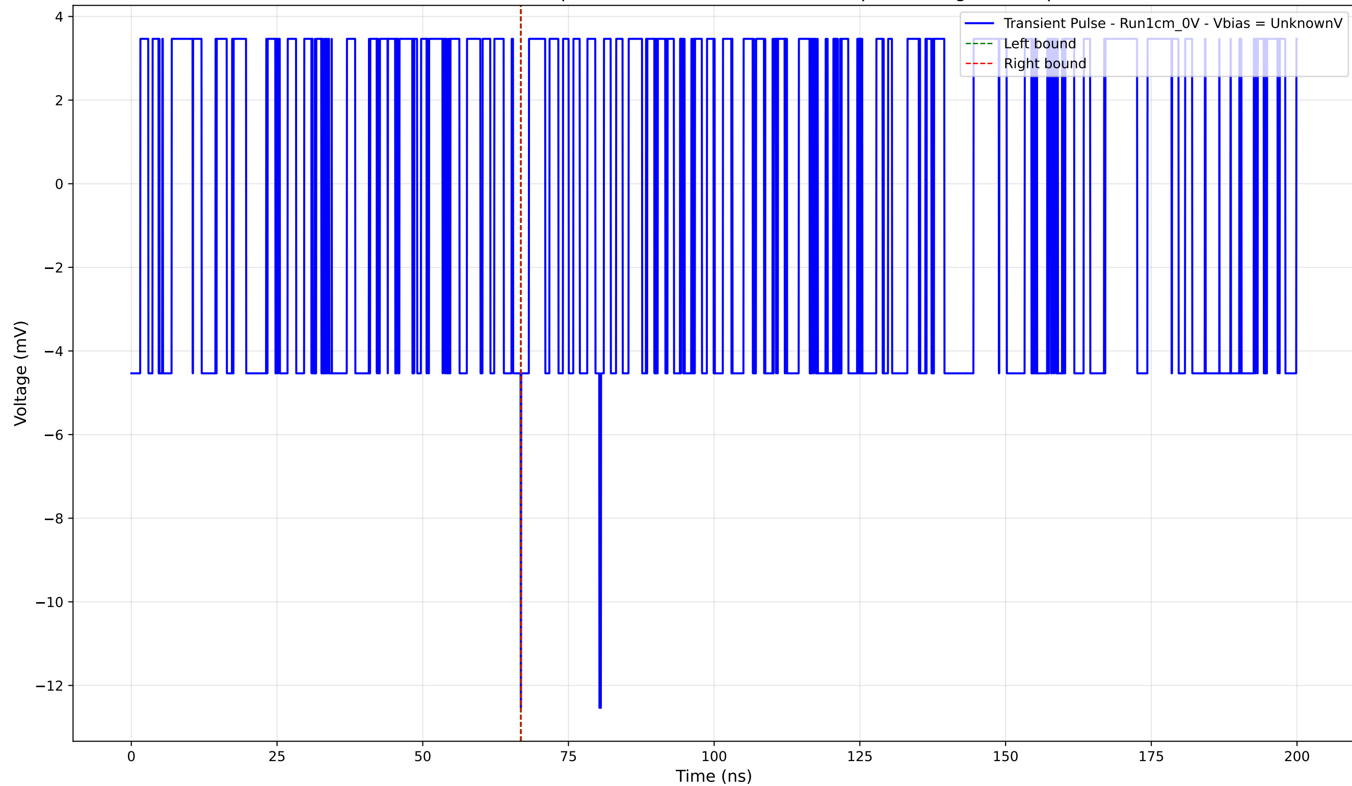
Transient Pulse - Sample: new1cm - Position: 4315.0 \mu\text{m} - Charge: -0.02 pC
