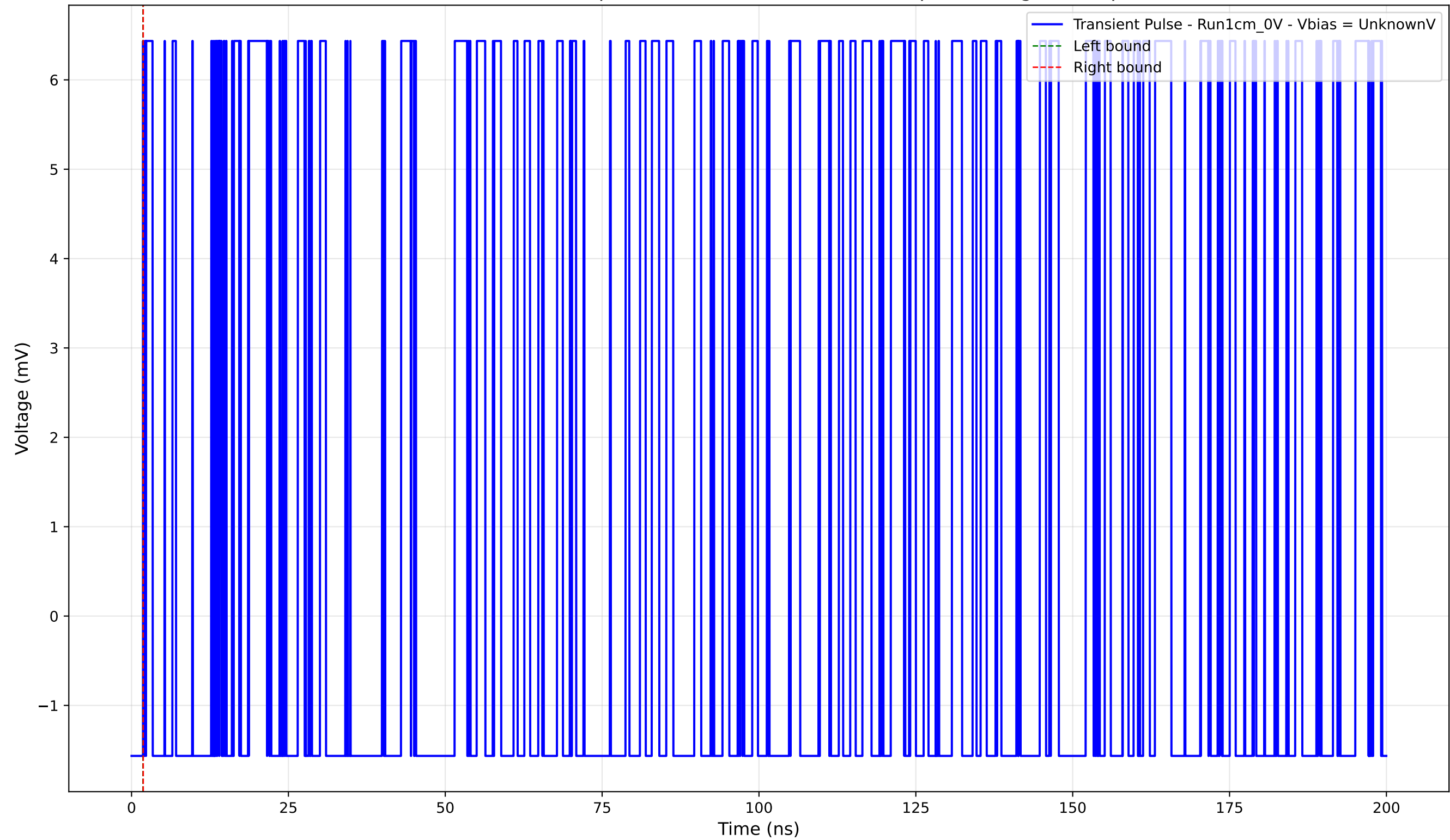
Transient Pulse - Sample: new1cm -Position: 1715.0 \mu\text{m} - Charge: 0.00 pC
