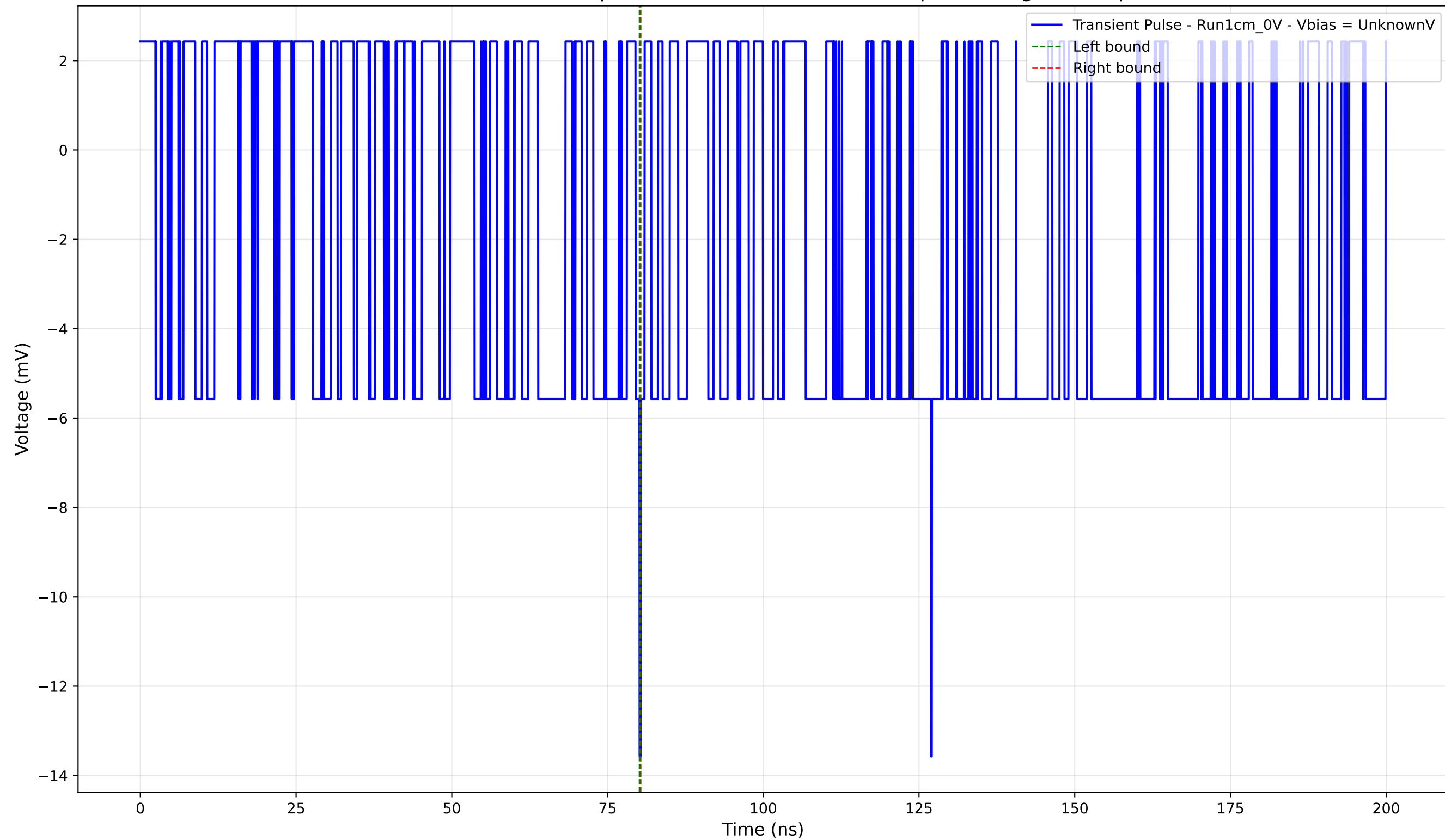
Transient Pulse - Sample: new1cm - Position: 1690.0 \mu\text{m} - Charge: -0.05 pC
