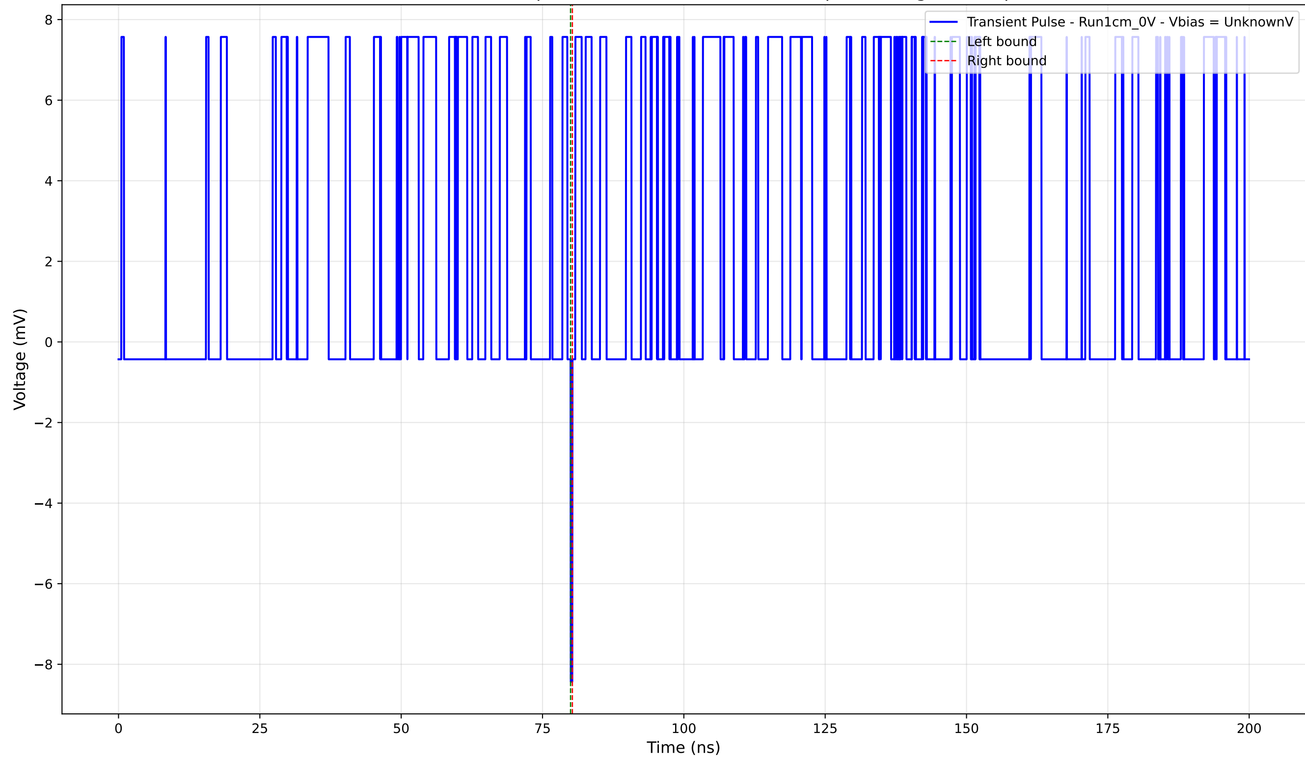
Transient Pulse - Sample: new1cm - Position: 1170.0 \mu\text{m} - Charge: -0.05 pC
