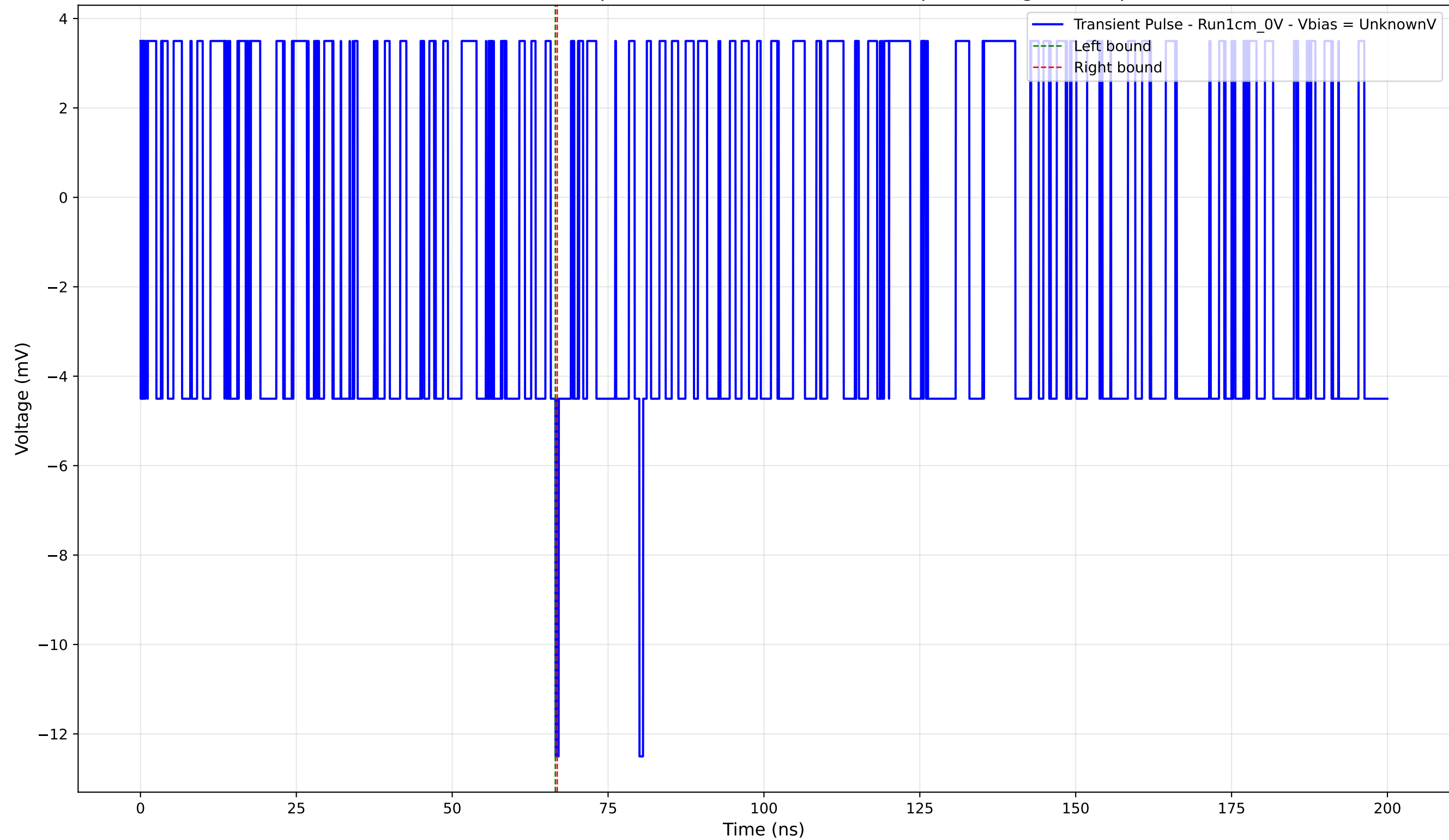
Transient Pulse - Sample: new1cm - Position: 1935.0 \mu\text{m} - Charge: -0.07 pC
