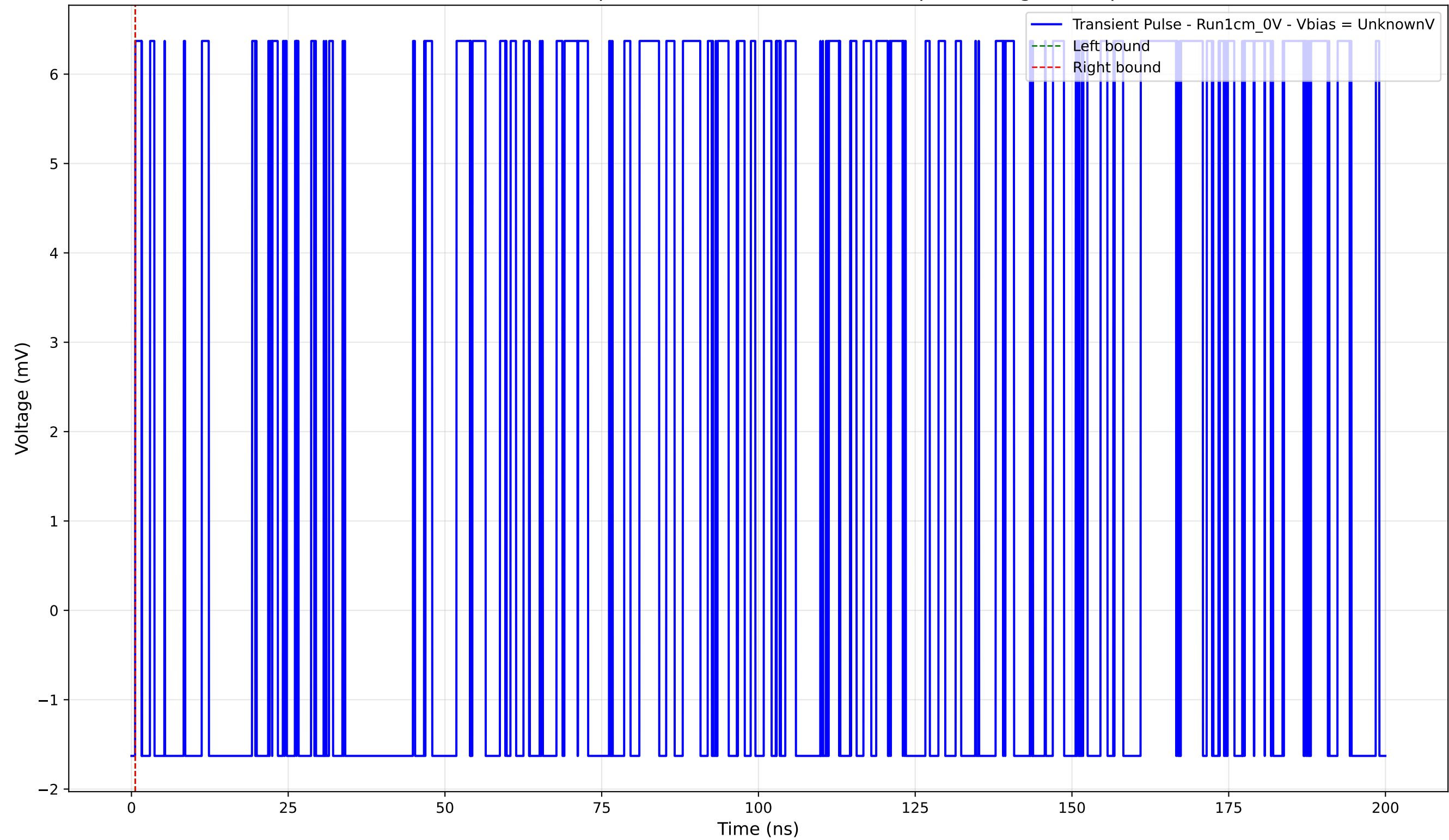
Transient Pulse - Sample: new1cm - Position: 2360.0 \mu\text{m} - Charge: 0.00 pC
