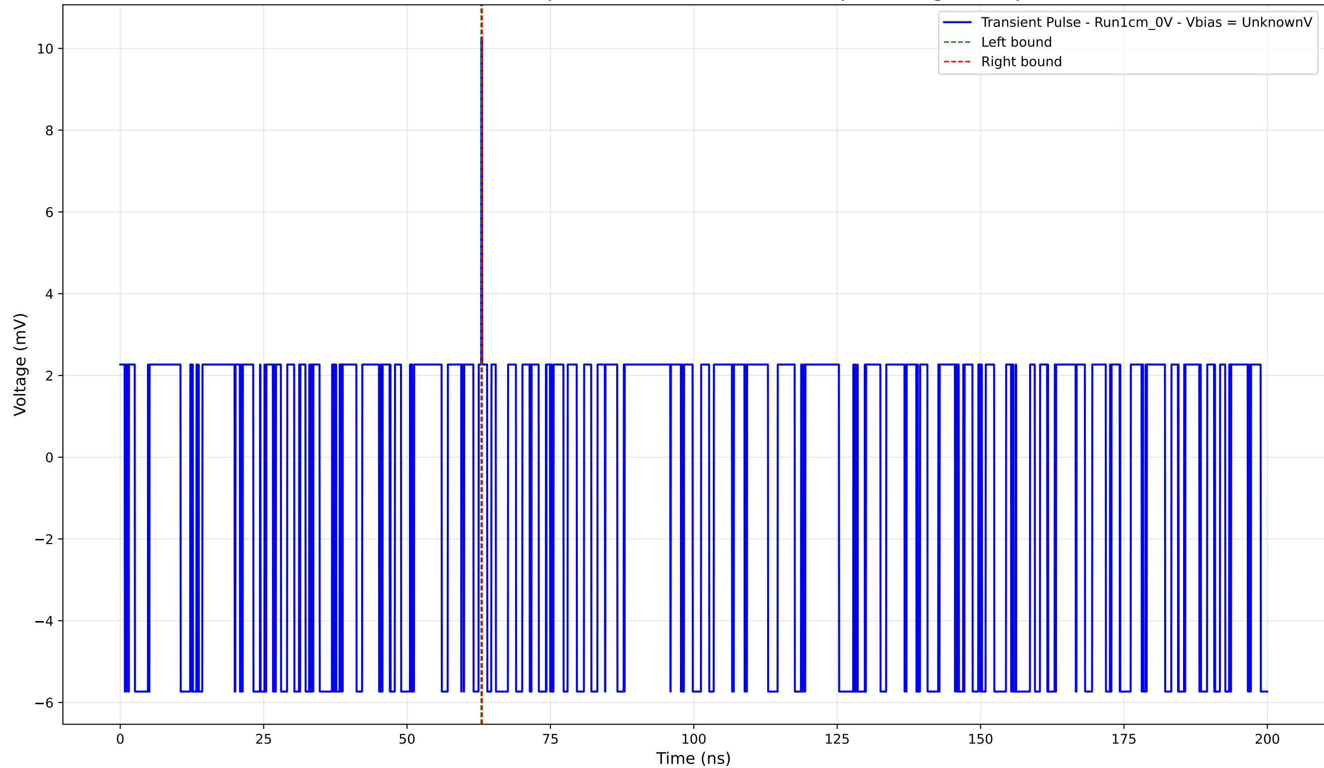
Transient Pulse - Sample: new1cm - Position: 3290.0 \mu\text{m} - Charge: 0.03 pC
