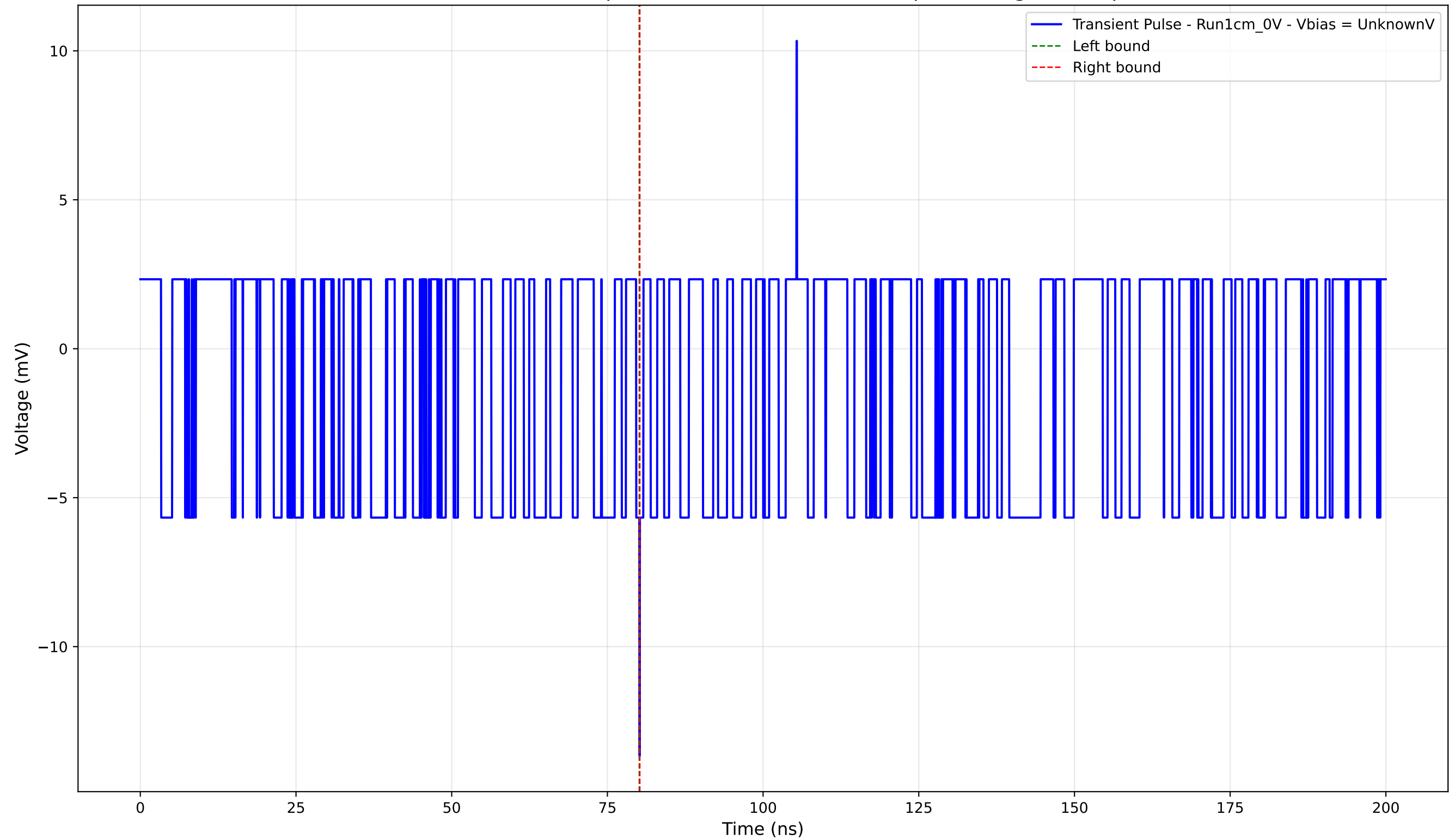
Transient Pulse - Sample: new1cm - Position: 835.0 \mu\text{m} - Charge: -0.02 pC
