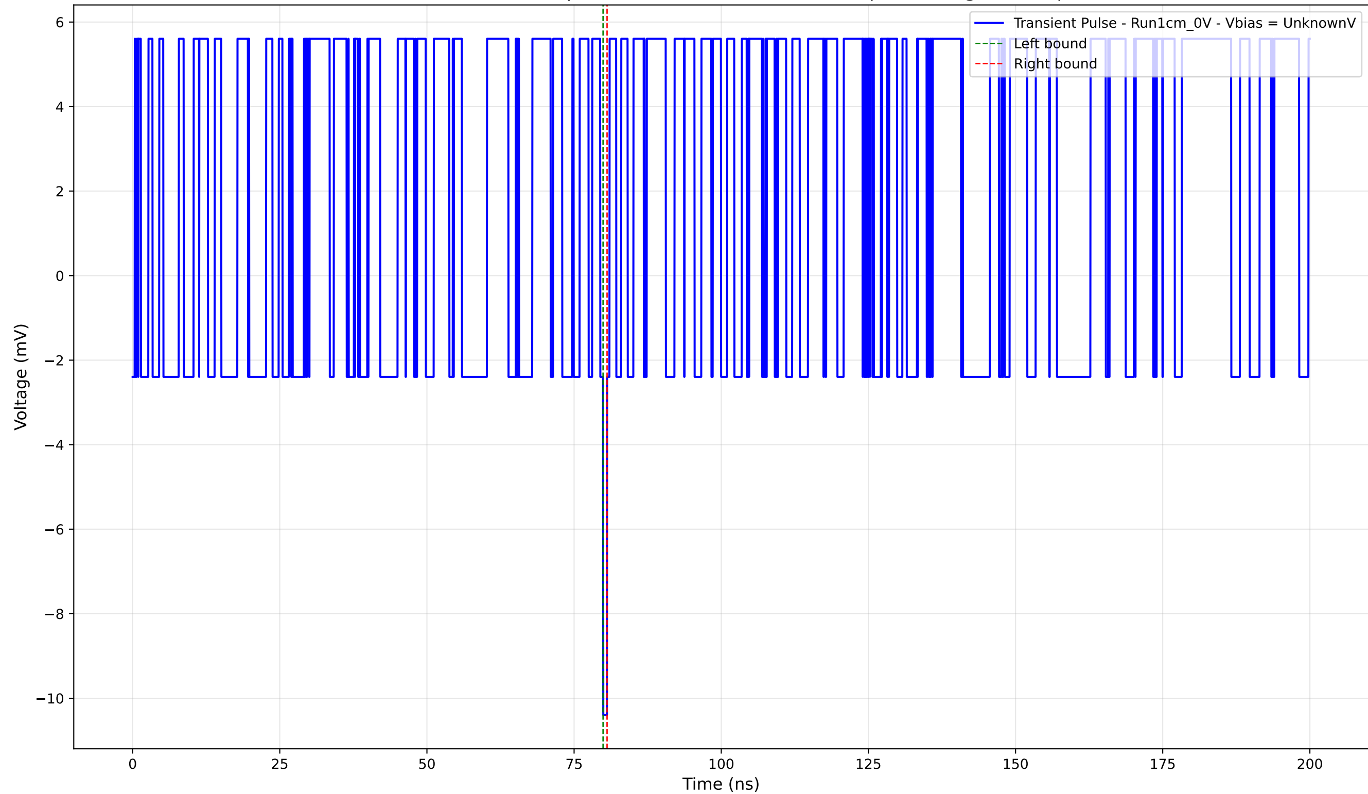
Transient Pulse - Sample: new1cm - Position: 1950.0 \mu\text{m} - Charge: -0.14 pC
