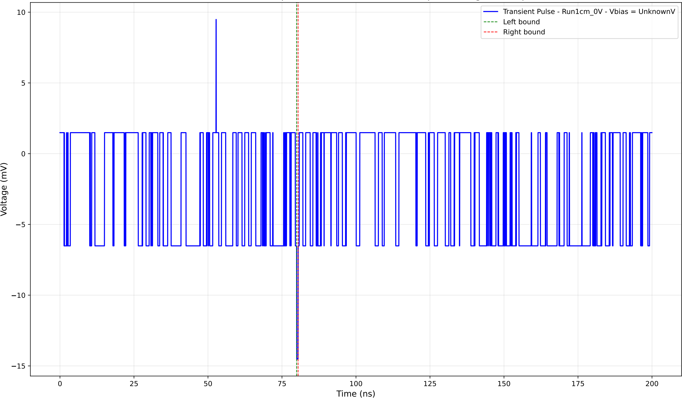
Transient Pulse - Sample: new1cm - Position: 250.0 \mu\text{m} - Charge: -0.14 pC
