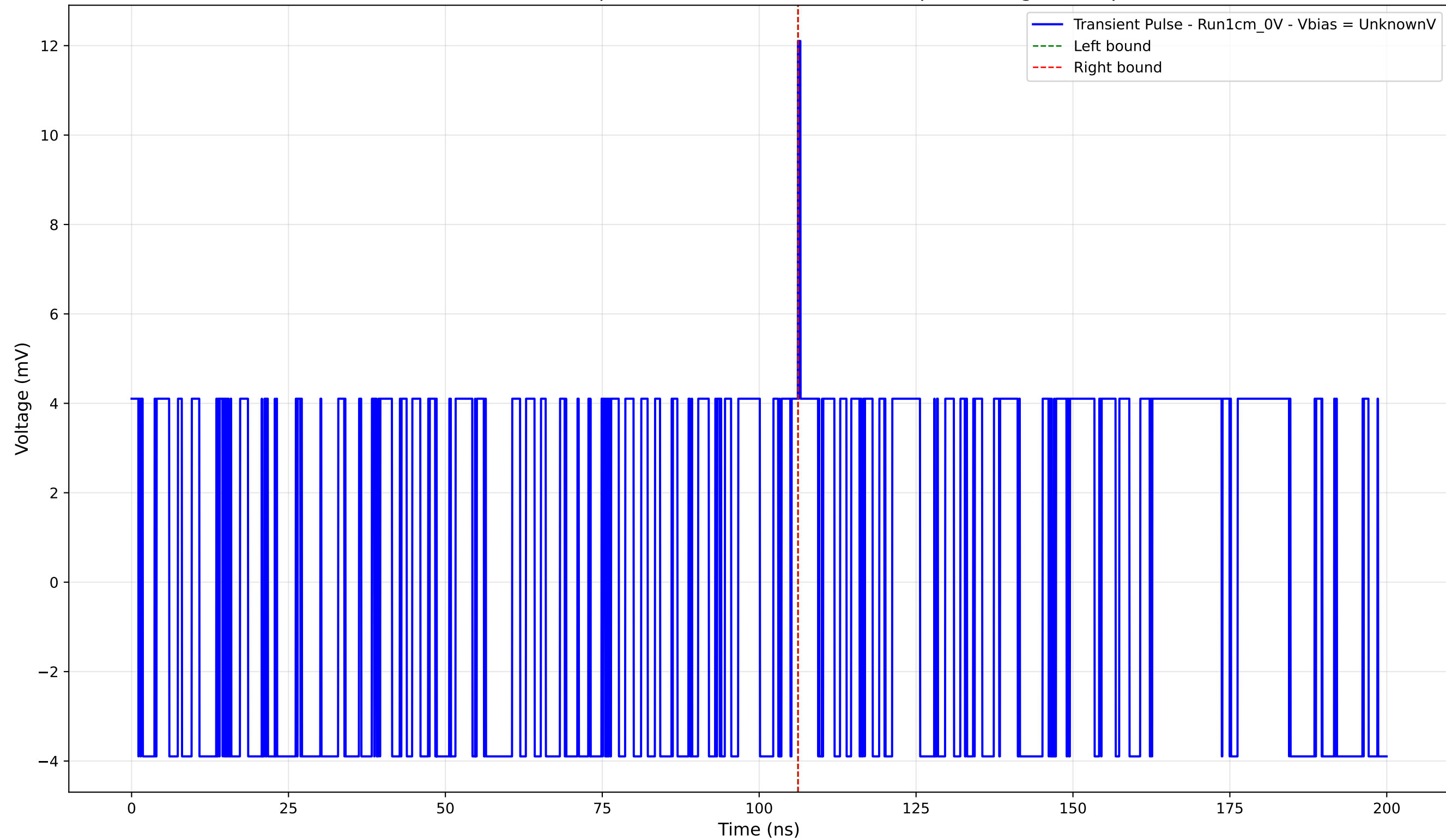
Transient Pulse - Sample: new1cm - Position: 4960.0 \mu\text{m} - Charge: 0.01 pC
