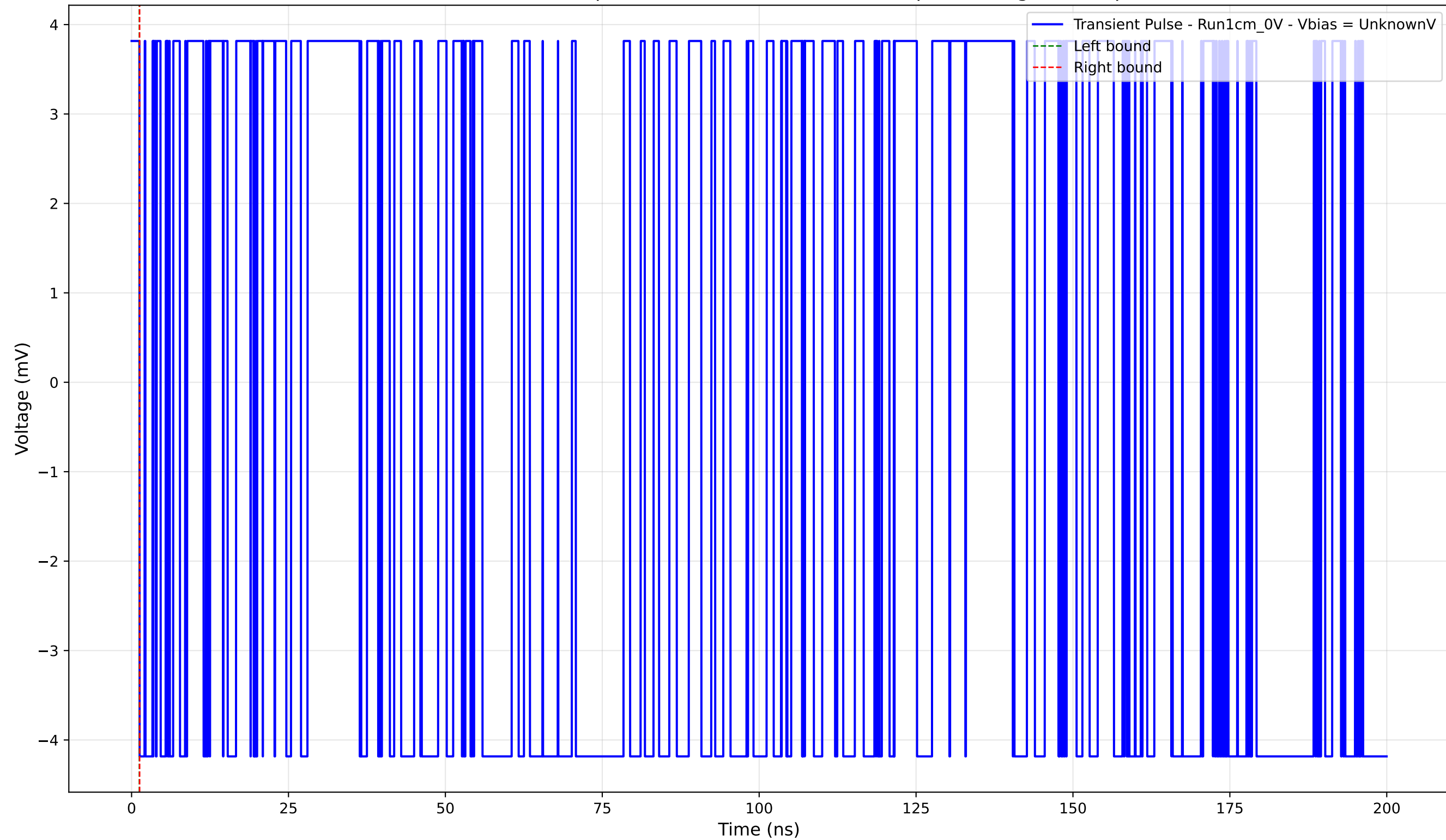
Transient Pulse - Sample: new1cm - Position: 3250.0 \mu\text{m} - Charge: -0.00 pC
