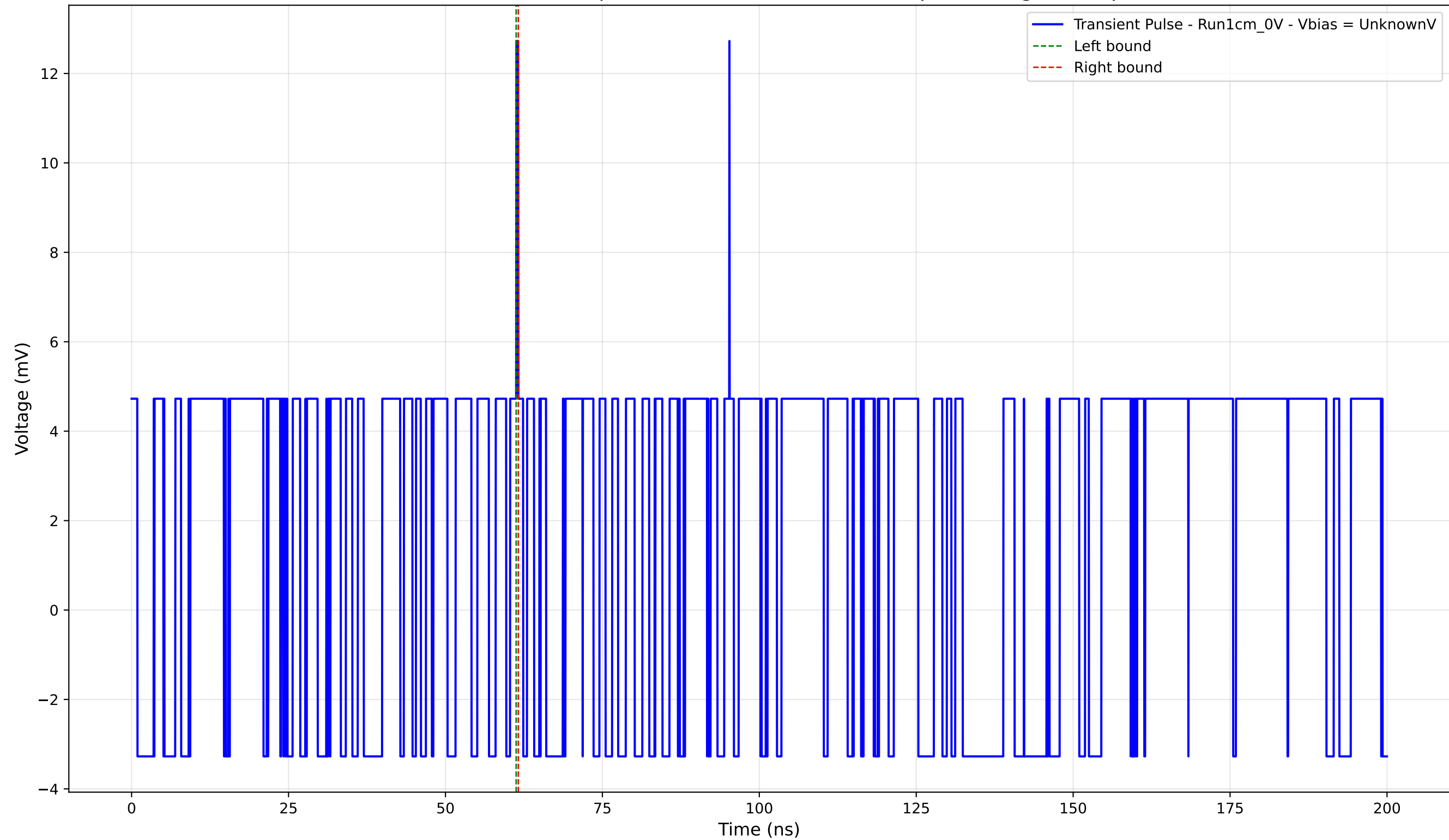
Transient Pulse - Sample: new1cm - Position: 4435.0 \mu\text{m} - Charge: 0.08 pC
