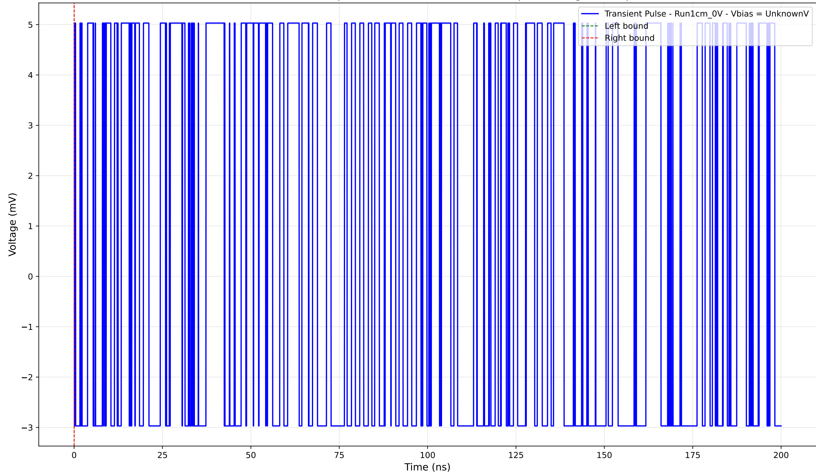
Transient Pulse - Sample: new1cm -Position: 3150.0 \mu\text{m} - Charge: 0.00 pC
