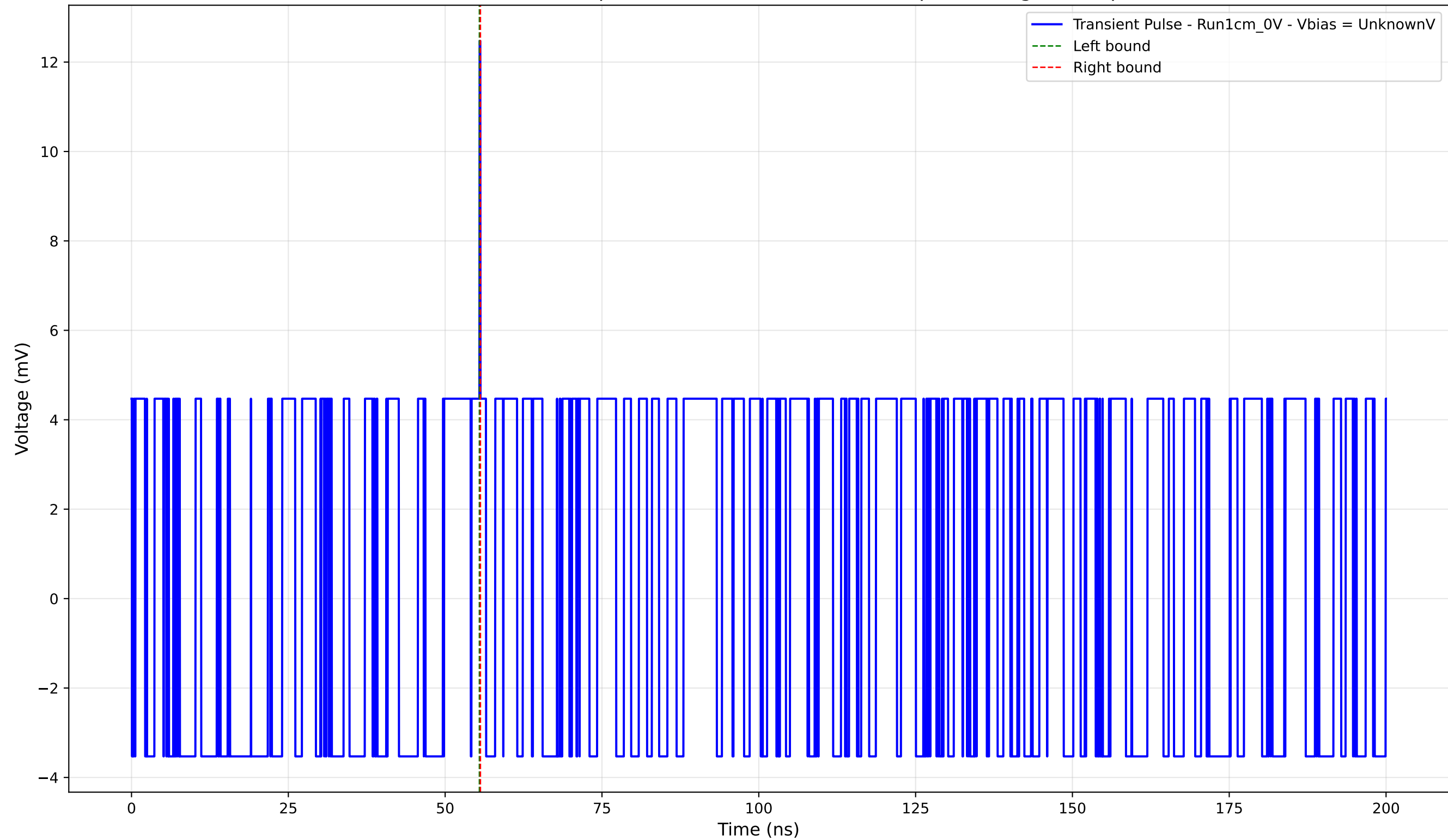
Transient Pulse - Sample: new1cm - Position: 1080.0 \mu\text{m} - Charge: 0.04 pC
