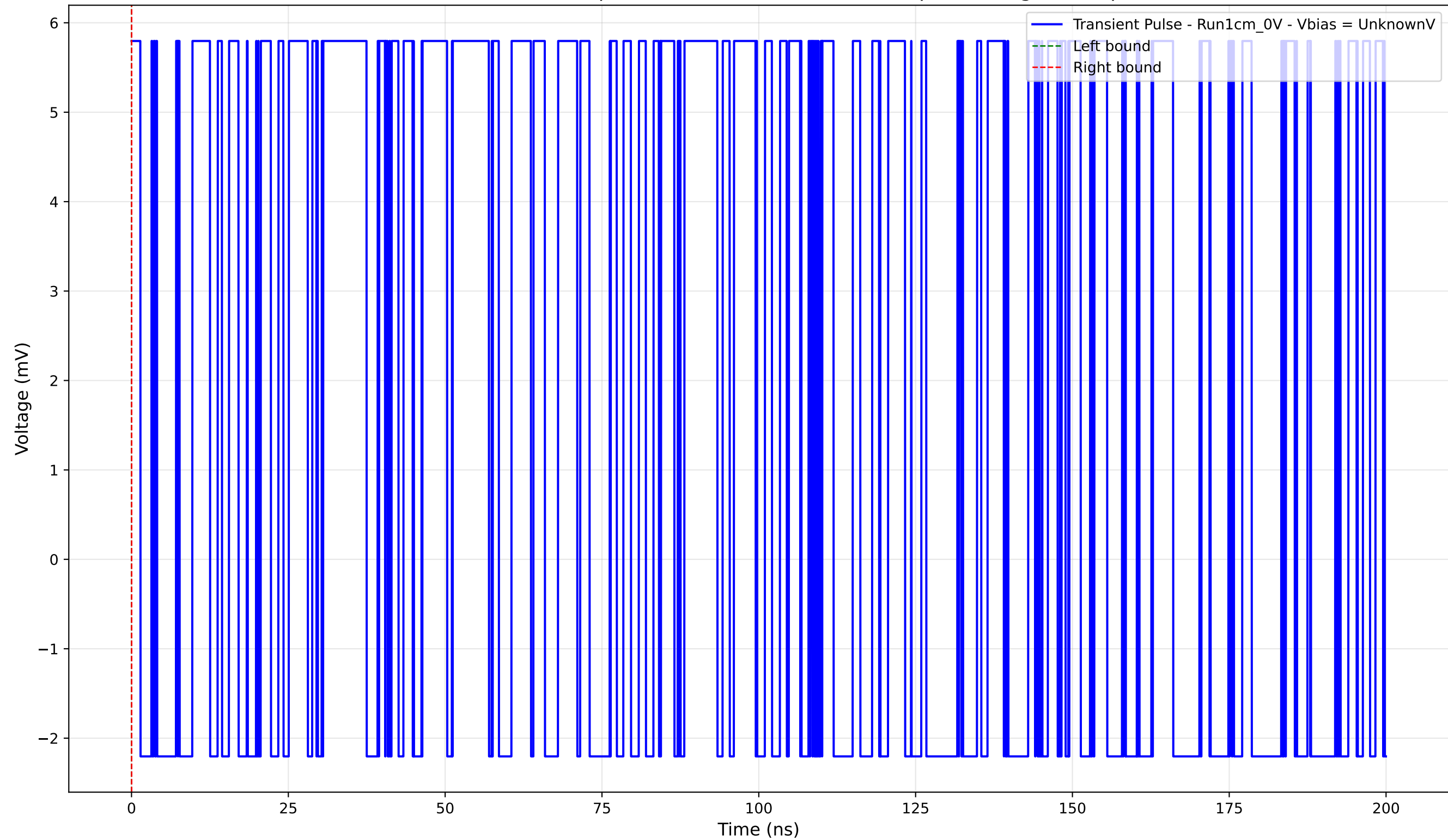
Transient Pulse - Sample: new1cm -Position: 4005.0 \mu\text{m} - Charge: 0.00 pC
