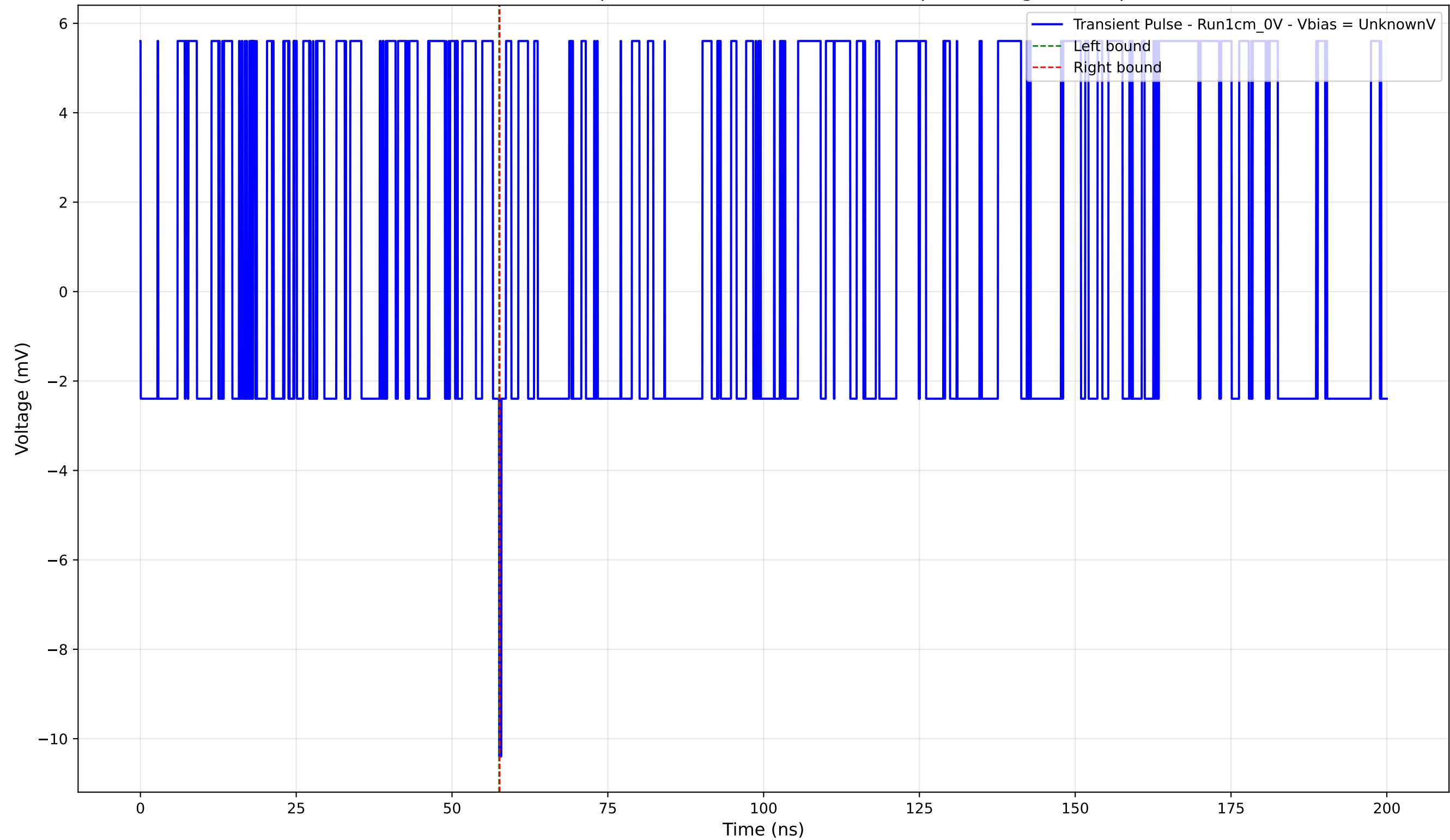
Transient Pulse - Sample: new1cm - Position: 5095.0 \mu\text{m} - Charge: -0.02 pC
