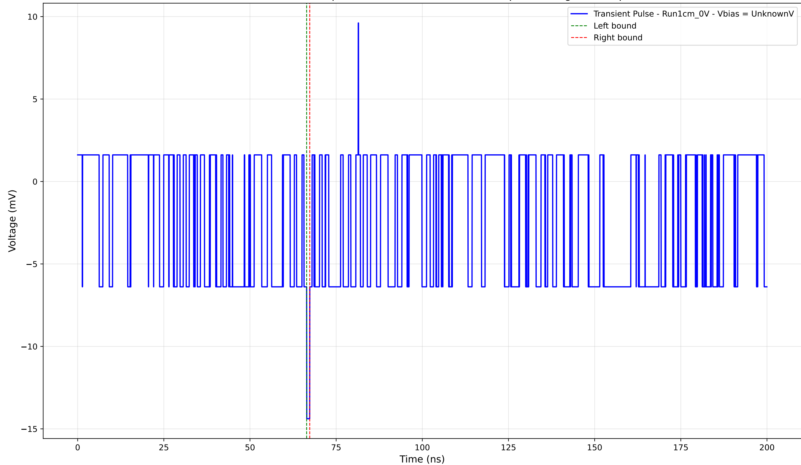
Transient Pulse - Sample: new1cm - Position: 2330.0 \mu\text{m} - Charge: -0.26 pC
