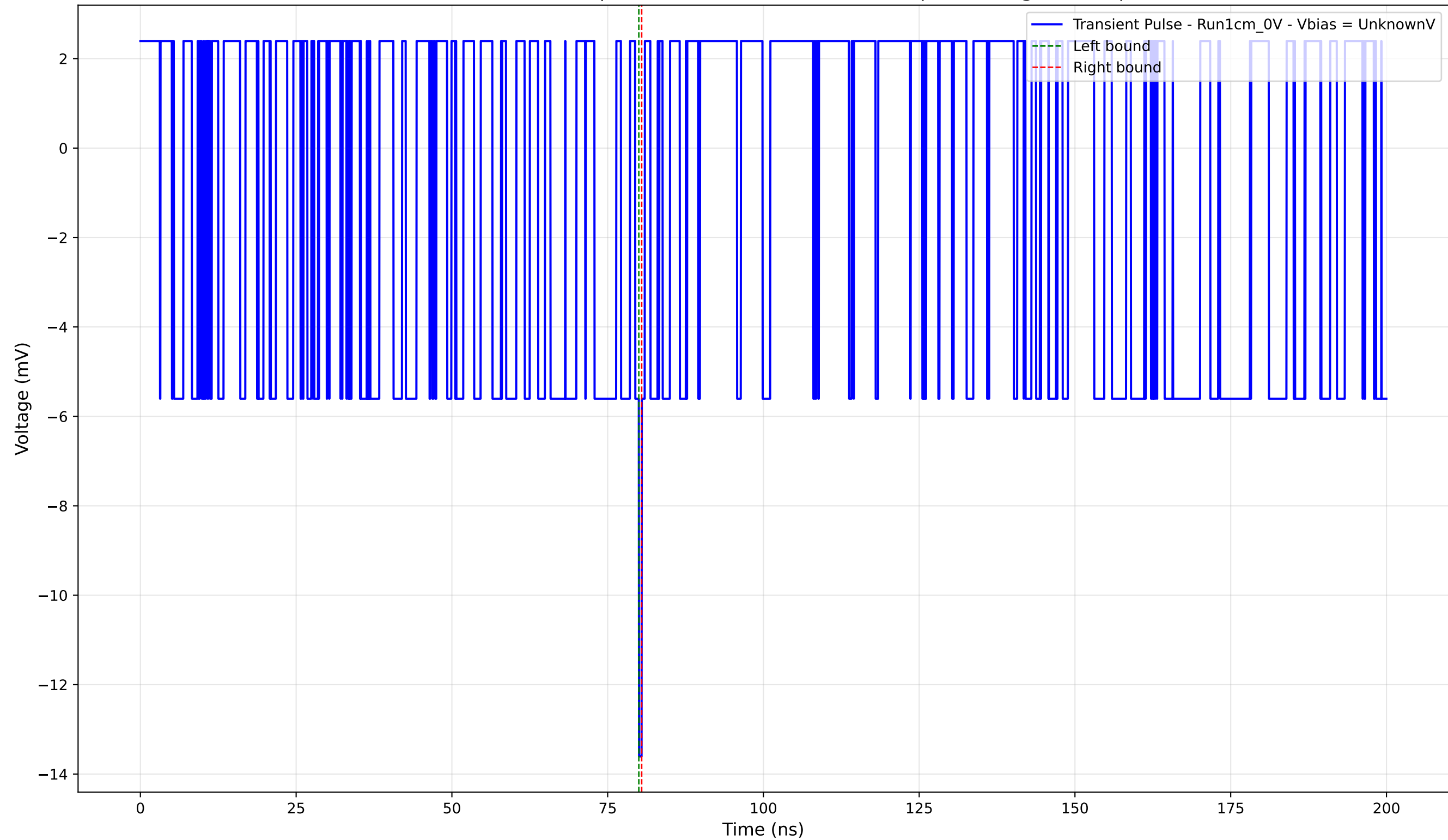
Transient Pulse - Sample: new1cm - Position: 2410.0 \mu\text{m} - Charge: -0.12 pC
