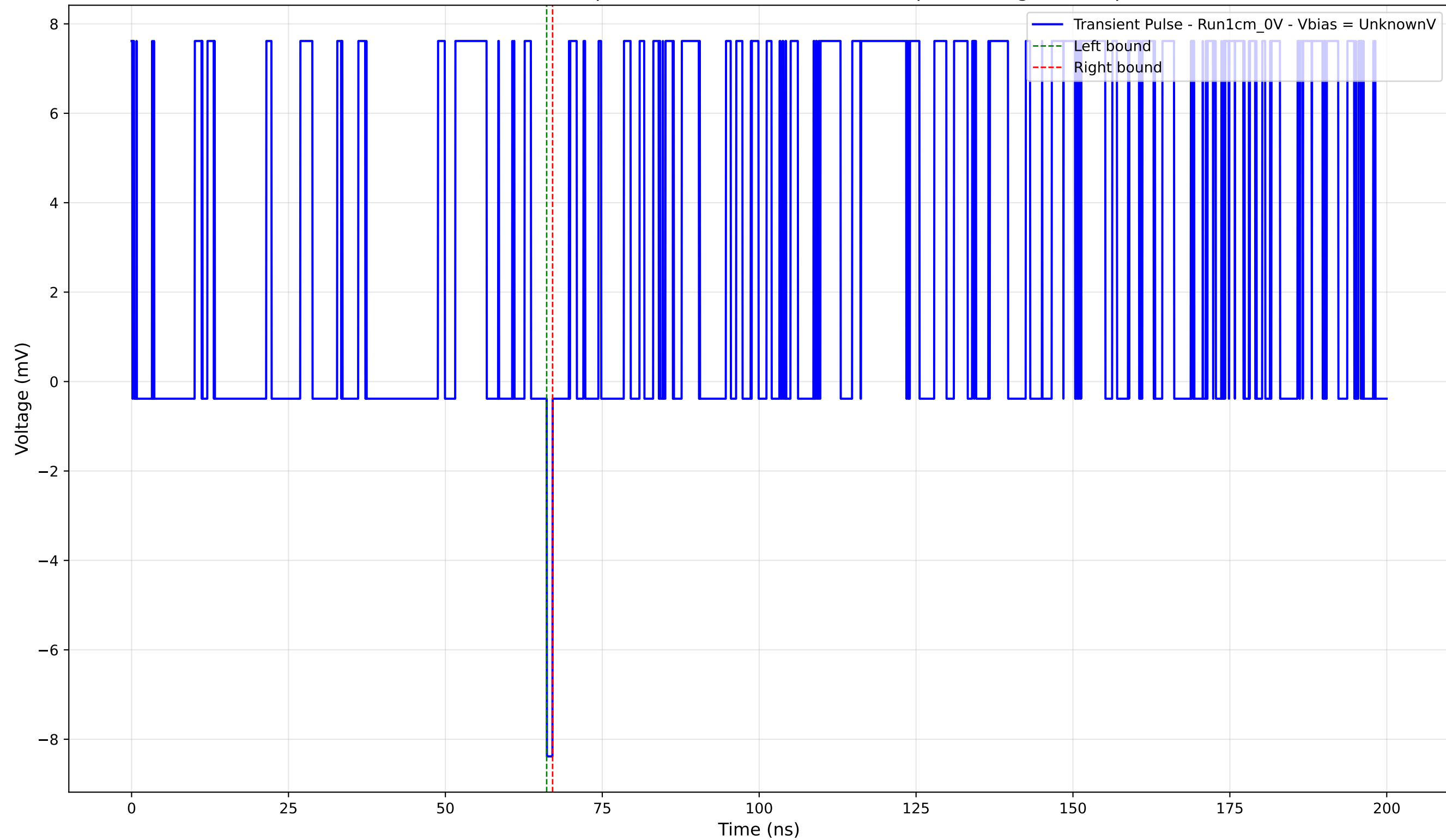
Transient Pulse - Sample: new1cm - Position: 3885.0 \mu\text{m} - Charge: -0.15 pC
