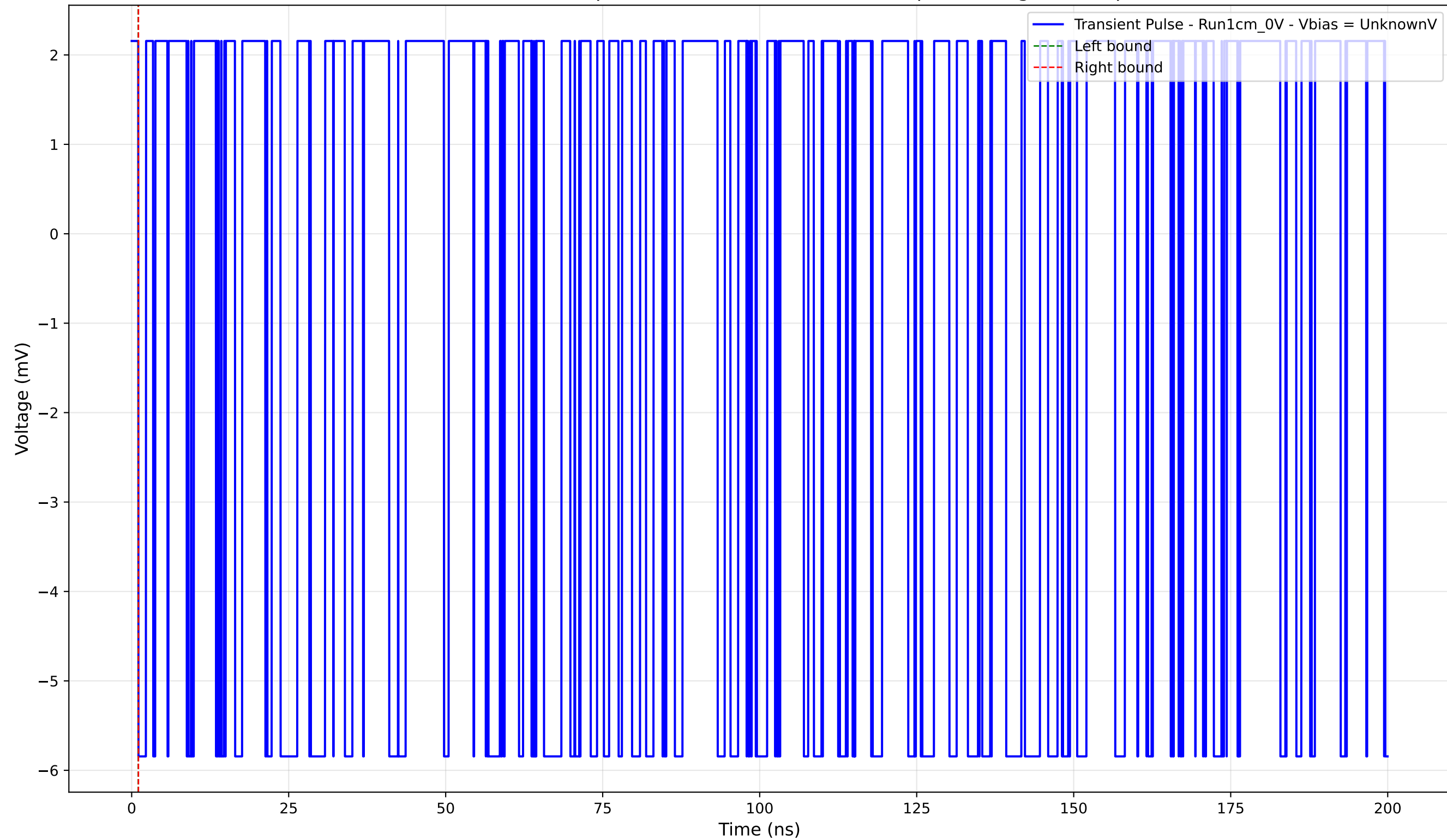
Transient Pulse - Sample: new1cm - Position: 3310.0 \mu\text{m} - Charge: -0.00 pC
