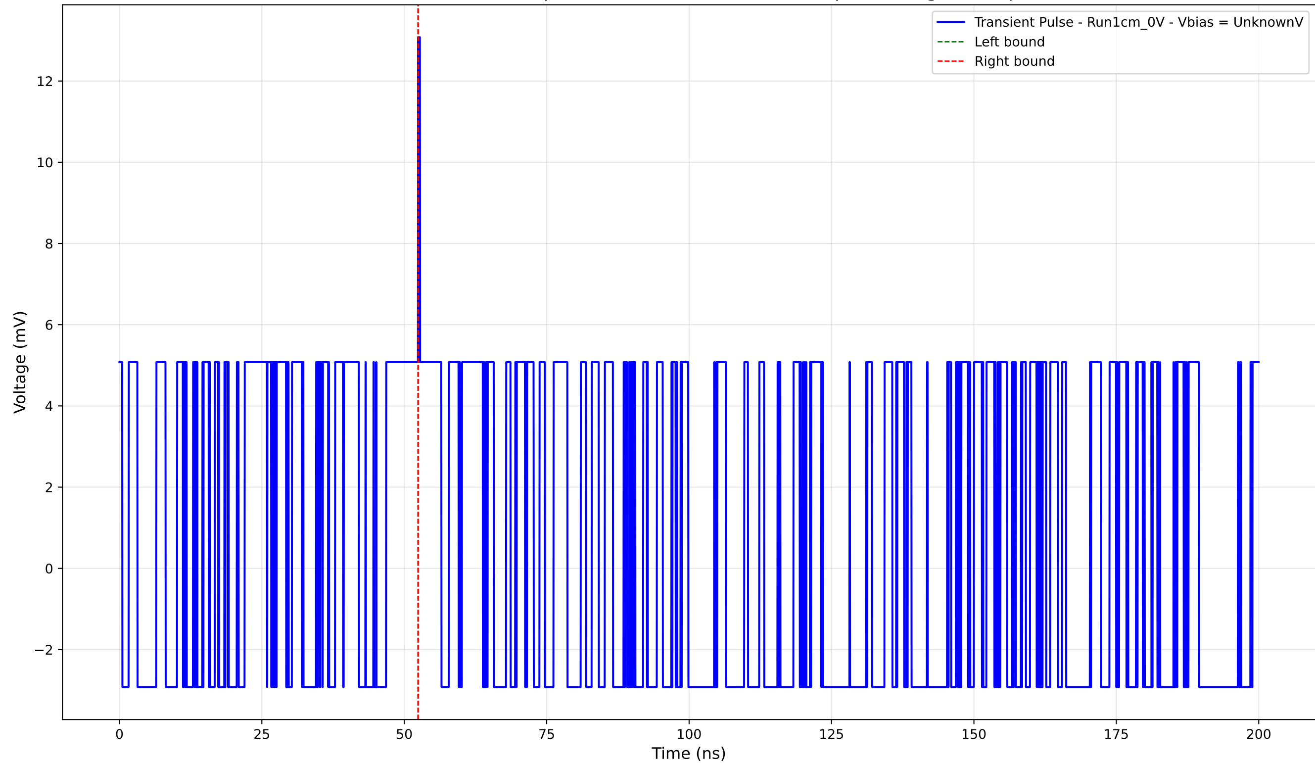
Transient Pulse - Sample: new1cm - Position: 3555.0 \mu\text{m} - Charge: 0.01 pC
