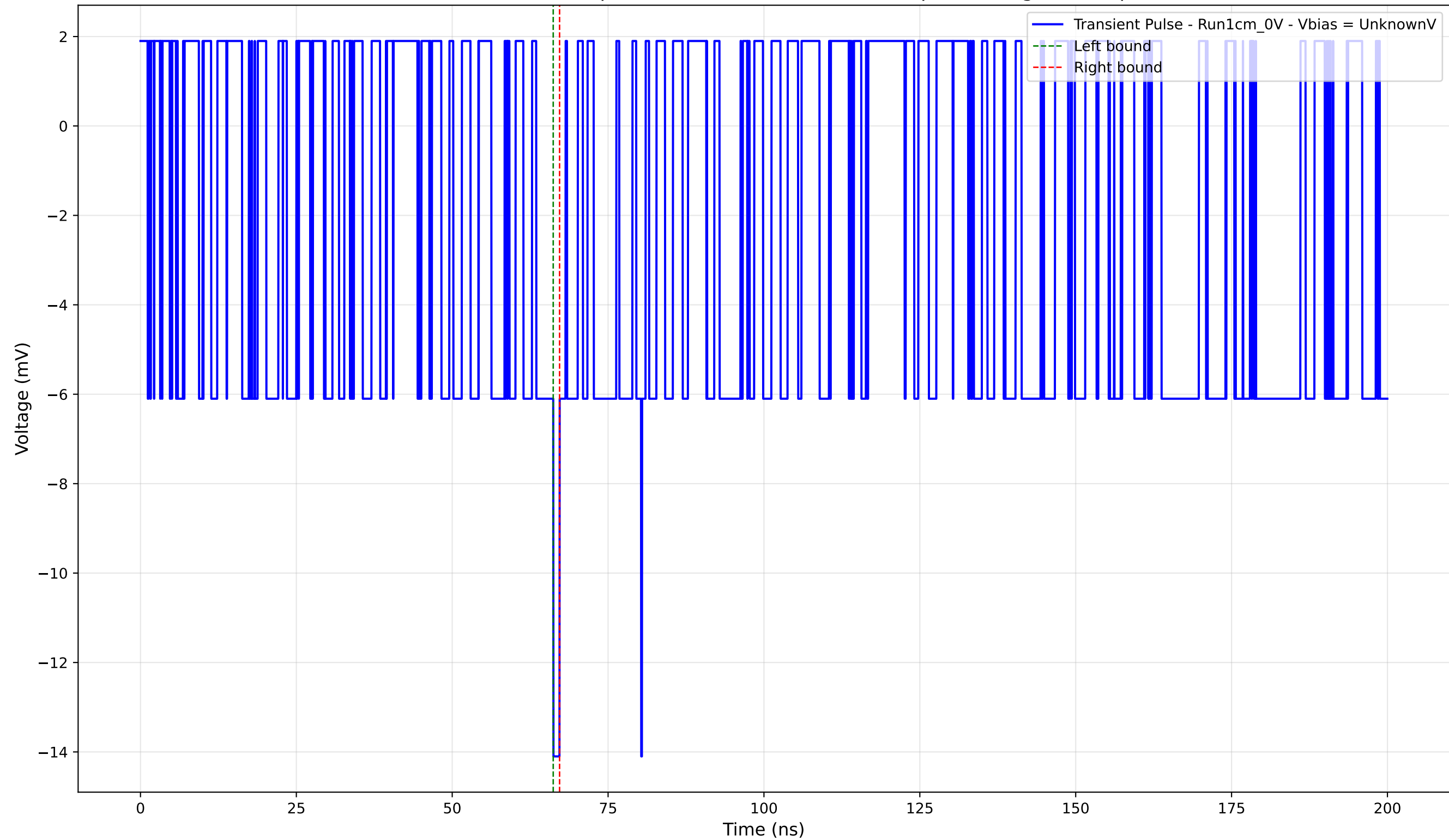
Transient Pulse - Sample: new1cm - Position: 1120.0 \mu\text{m} - Charge: -0.28 pC
