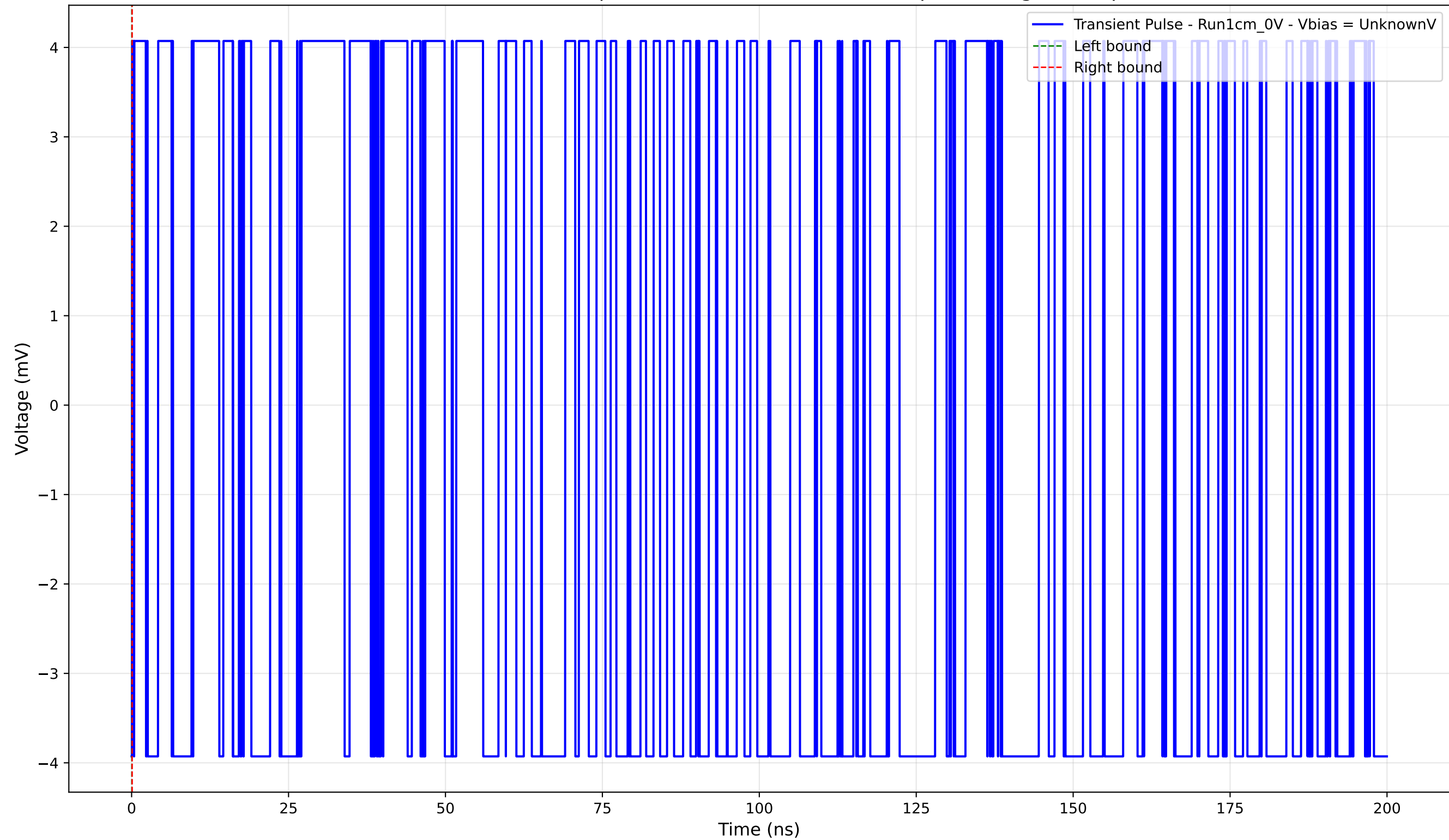
Transient Pulse - Sample: new1cm -Position: 2320.0 \mu\text{m} - Charge: 0.00 pC
