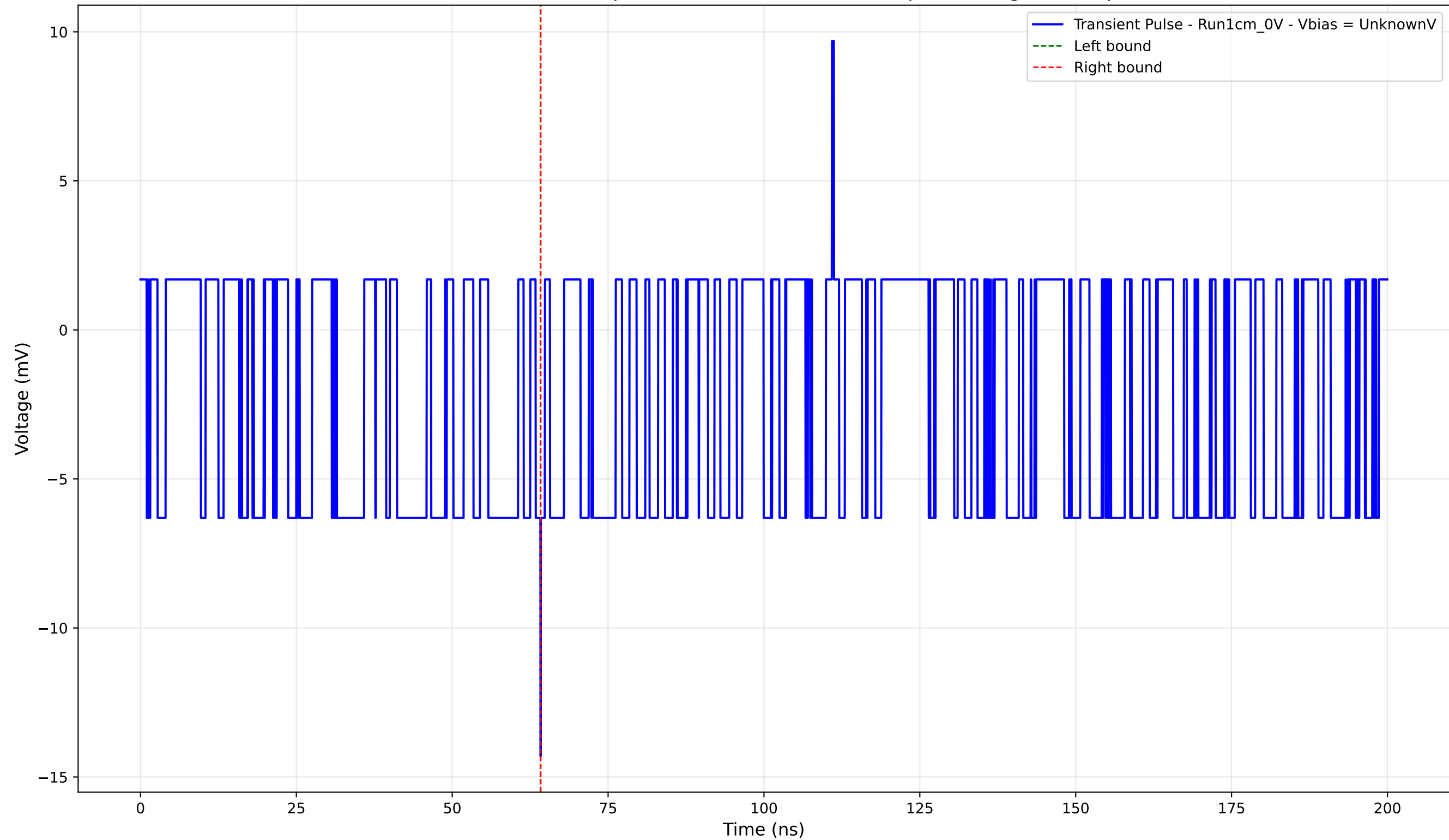
Transient Pulse - Sample: new1cm - Position: 90.0 \mu\text{m} - Charge: -0.01 pC
