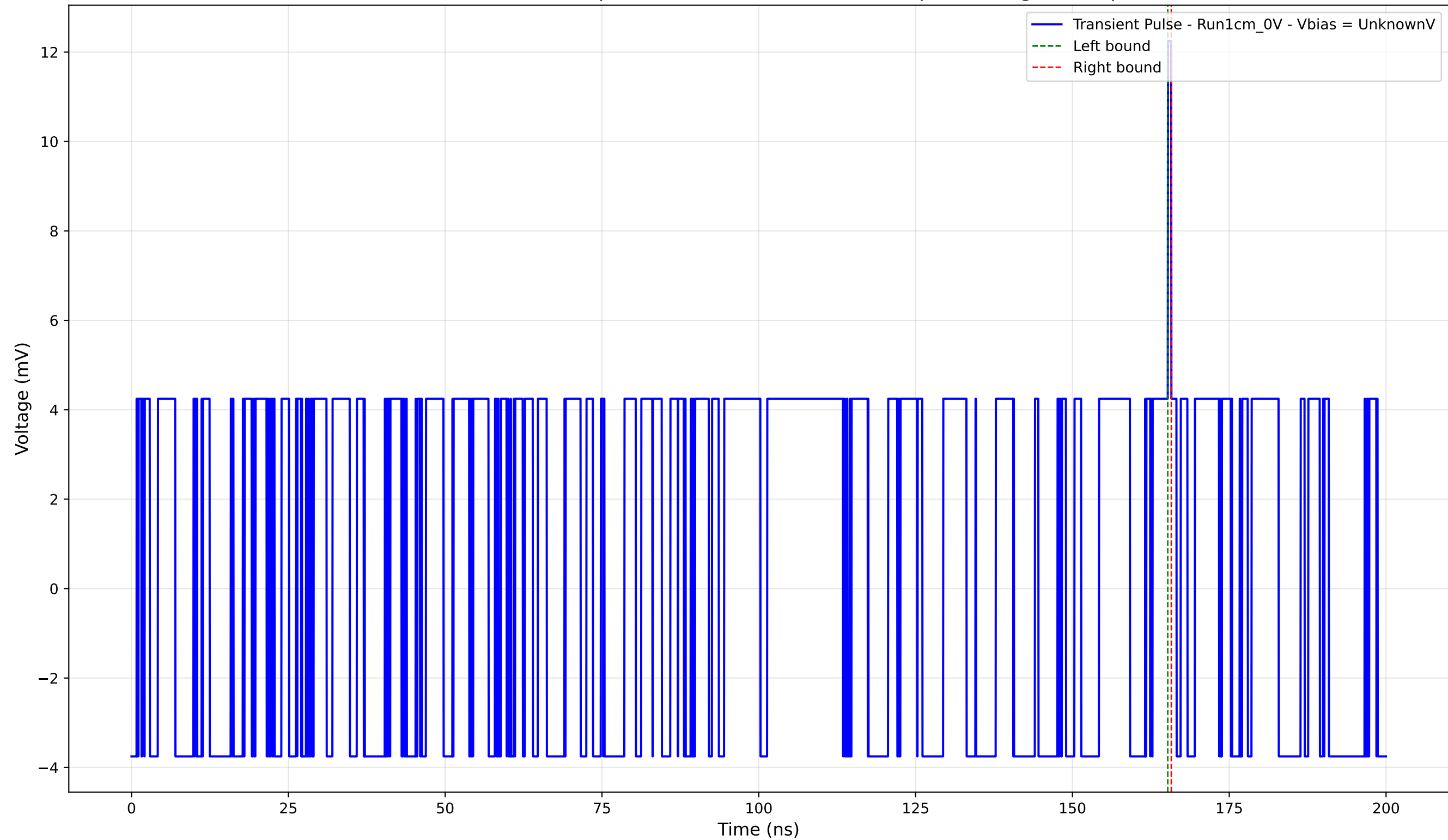
Transient Pulse - Sample: new1cm - Position: 4855.0 \mu\text{m} - Charge: 0.13 pC
