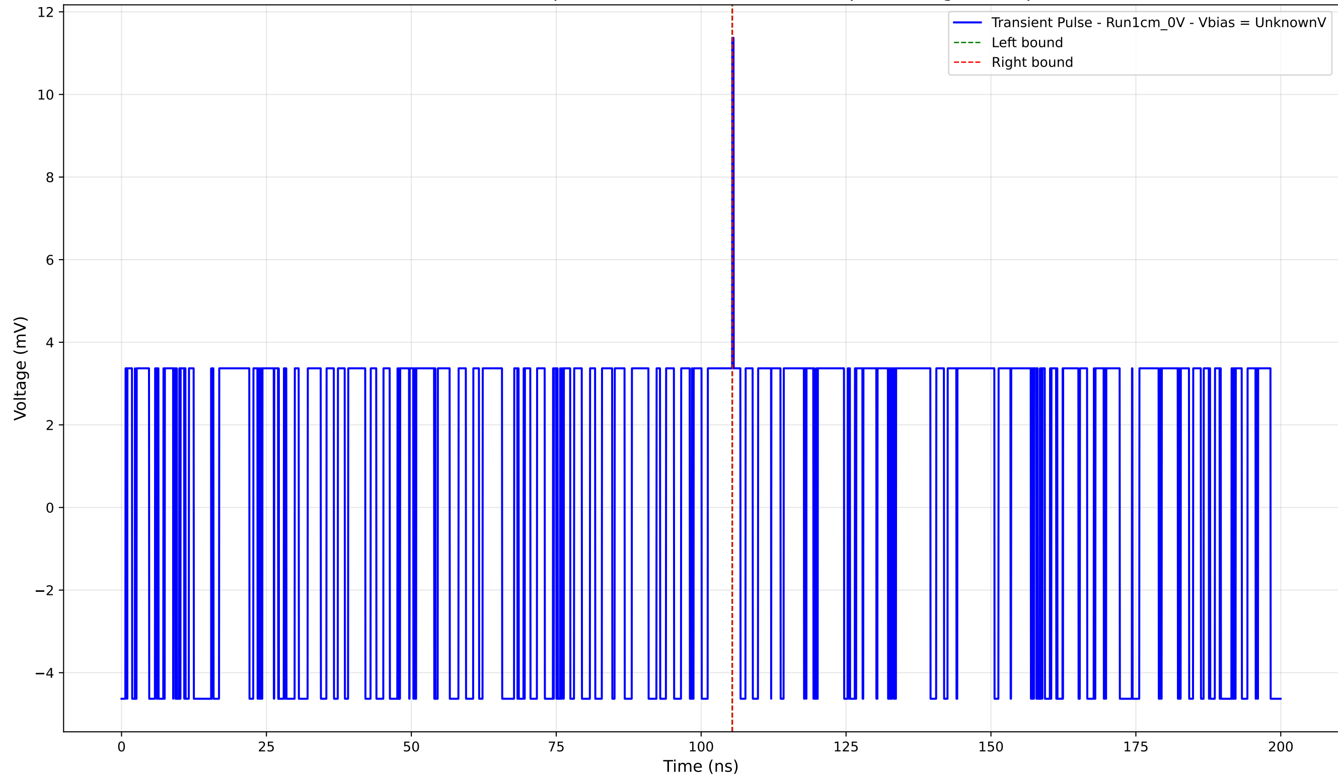
Transient Pulse - Sample: new1cm - Position: 3305.0 \mu\text{m} - Charge: 0.01 pC
