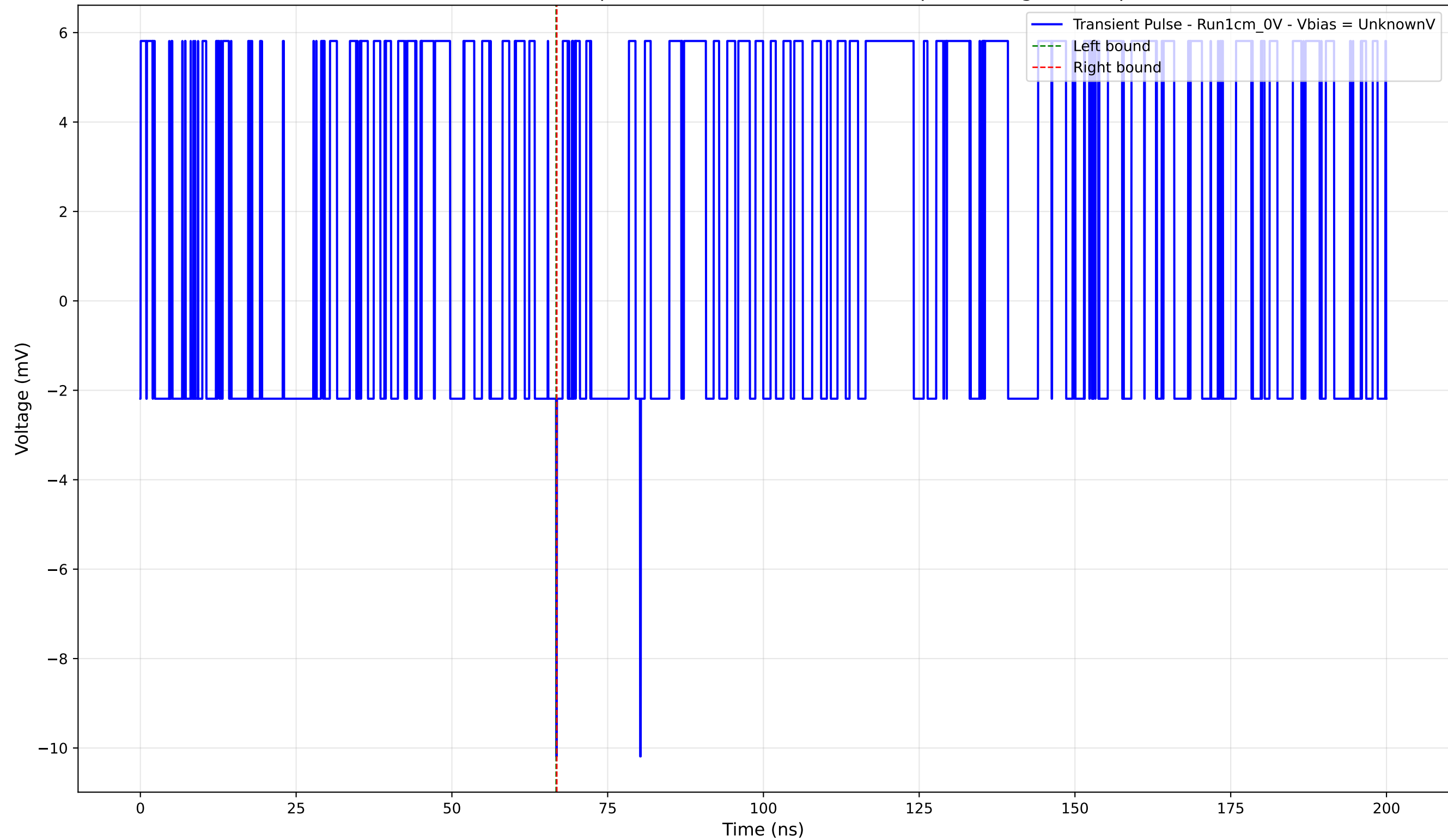
Transient Pulse - Sample: new1cm - Position: 2540.0 \mu\text{m} - Charge: -0.02 pC
