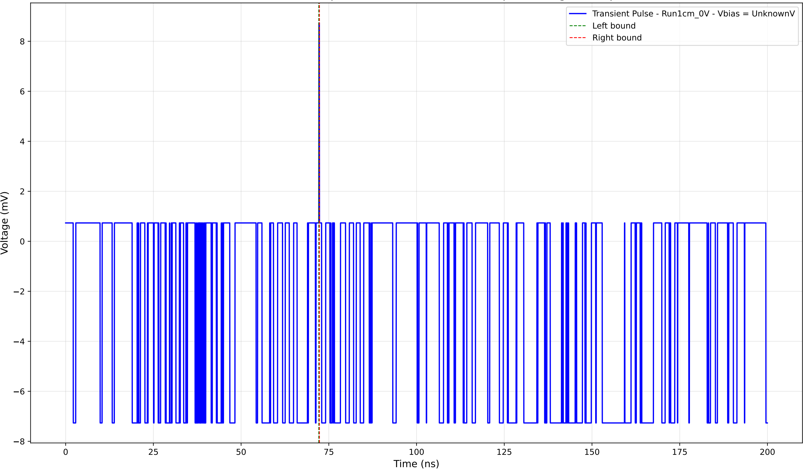
Transient Pulse - Sample: new1cm - Position: 640.0 \mu\text{m} - Charge: 0.03 pC
