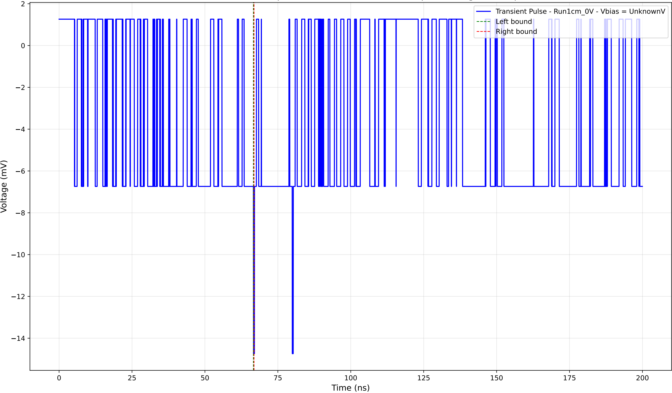
Transient Pulse - Sample: new1cm - Position: 275.0 \mu\text{m} - Charge: -0.06 pC
