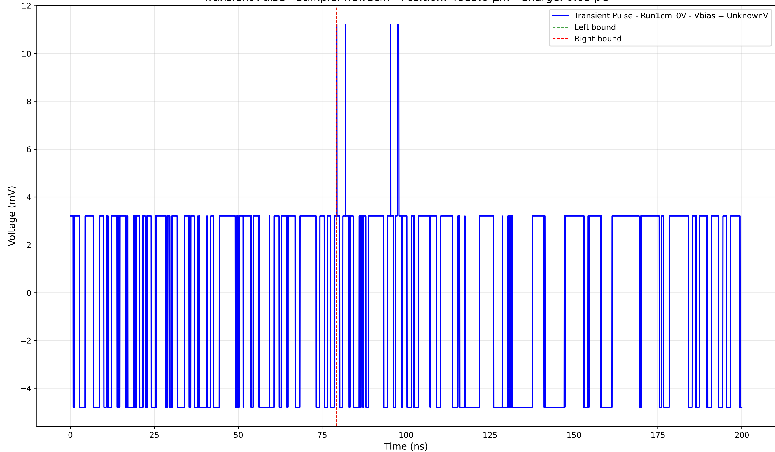
Transient Pulse - Sample: new1cm - Position: 4815.0 \mu\text{m} - Charge: 0.03 pC
