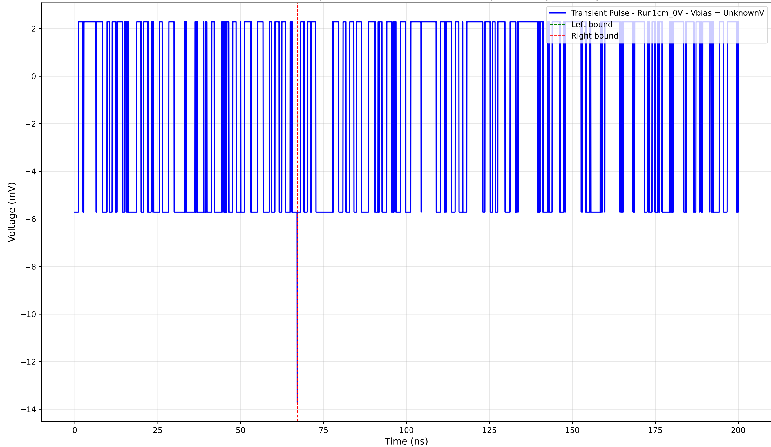
Transient Pulse - Sample: new1cm - Position: 4340.0 \mu\text{m} - Charge: -0.02 pC
