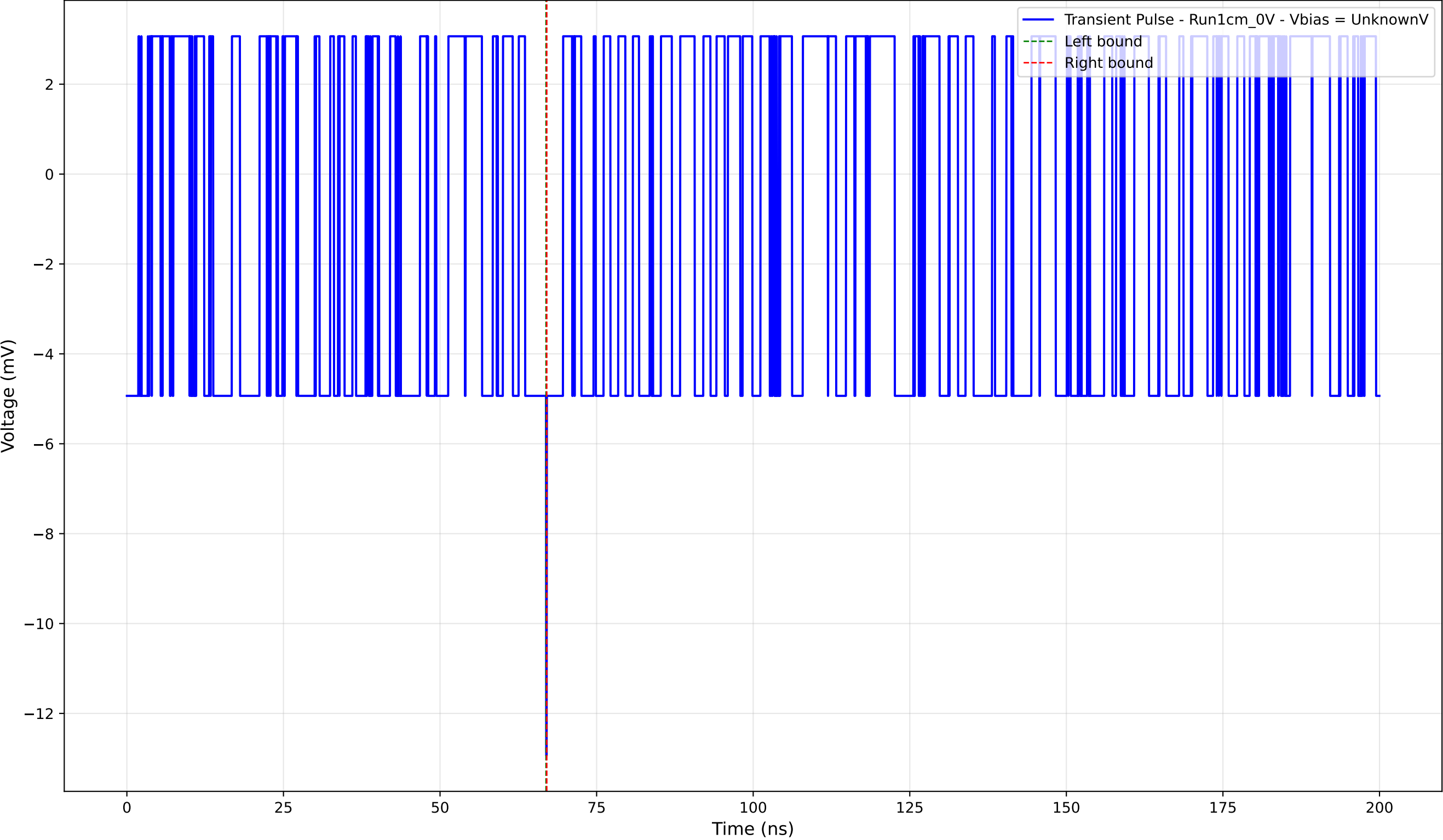
Transient Pulse - Sample: new1cm - Position: 390.0 \mu\text{m} - Charge: -0.03 pC
