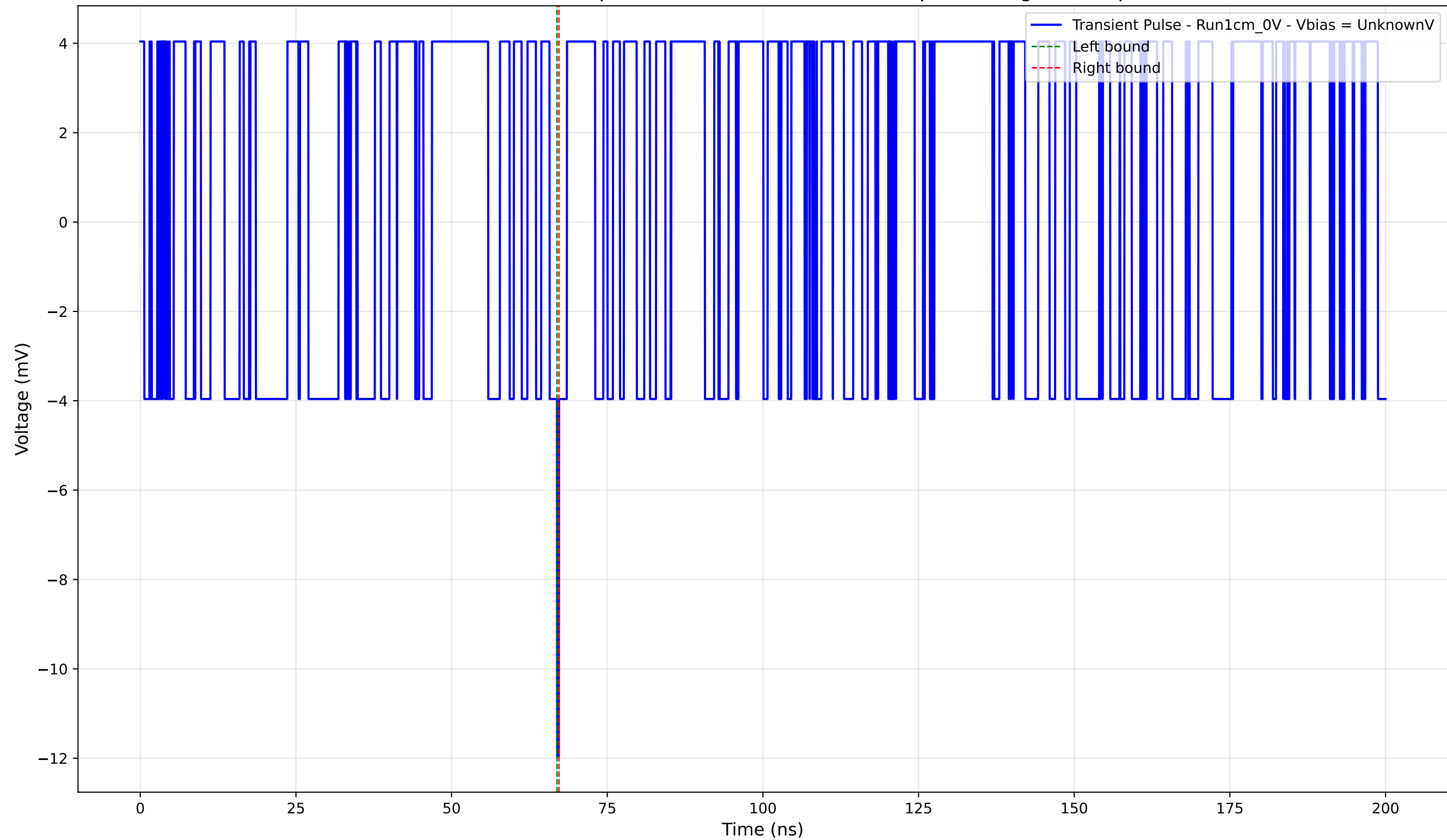
Transient Pulse - Sample: new1cm - Position: 4310.0 \mu\text{m} - Charge: -0.07 pC
