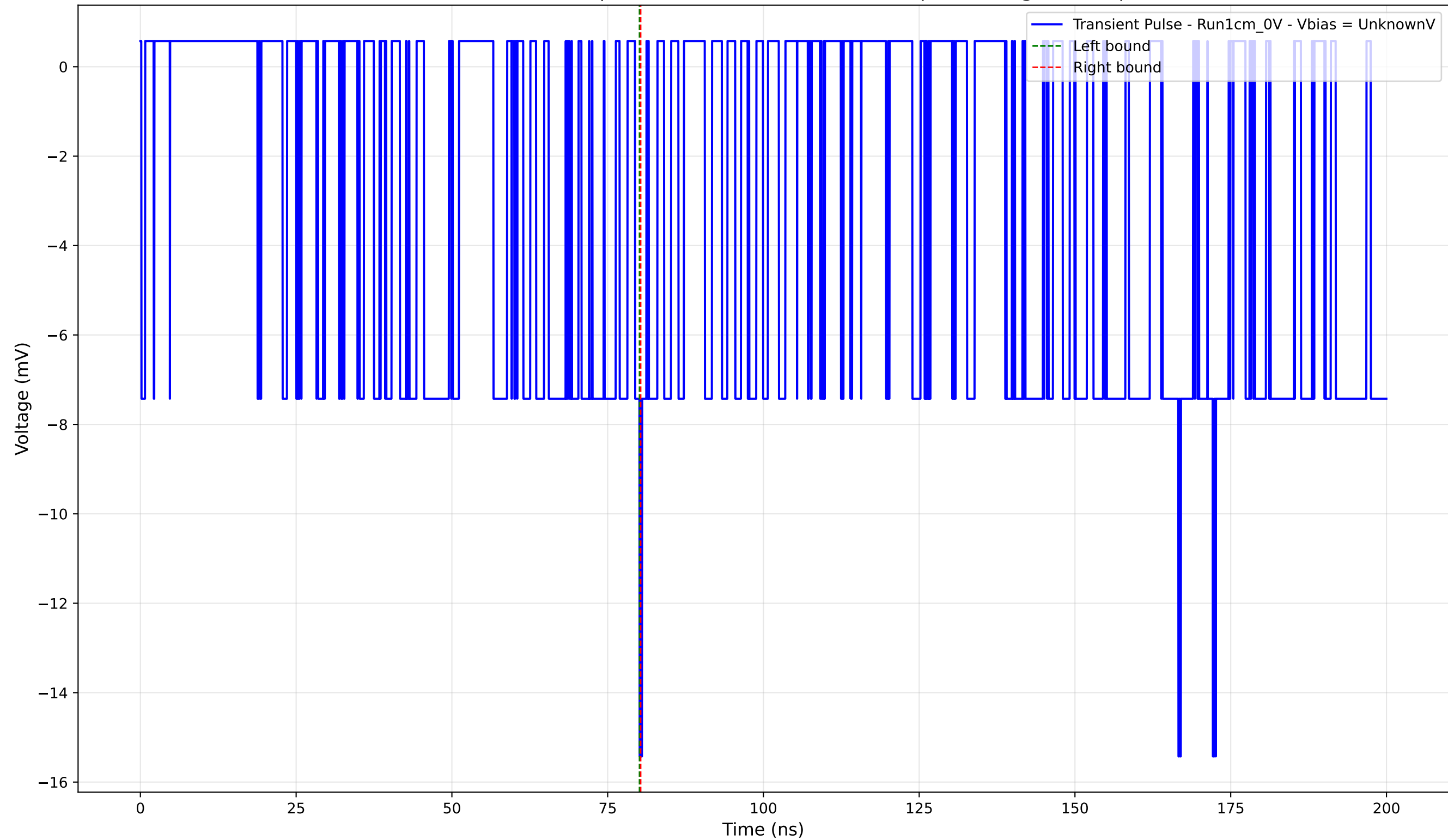
Transient Pulse - Sample: new1cm - Position: 2855.0 \mu\text{m} - Charge: -0.06 pC
