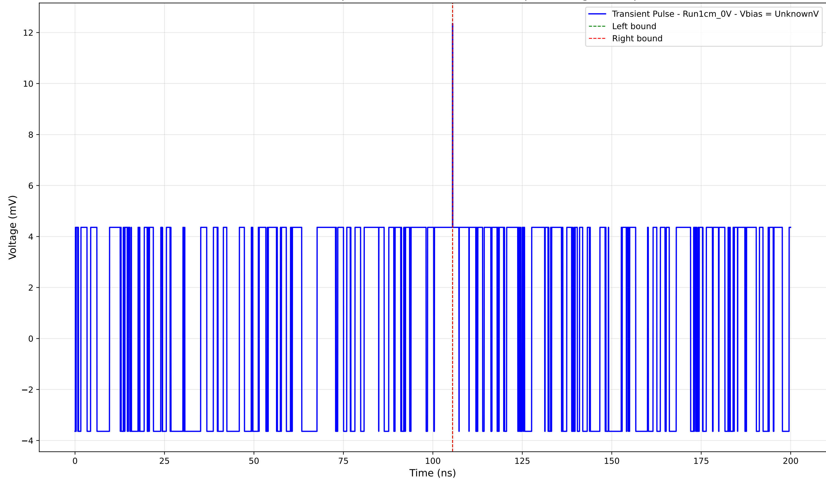
Transient Pulse - Sample: new1cm - Position: 2745.0 \mu\text{m} - Charge: 0.01 pC
