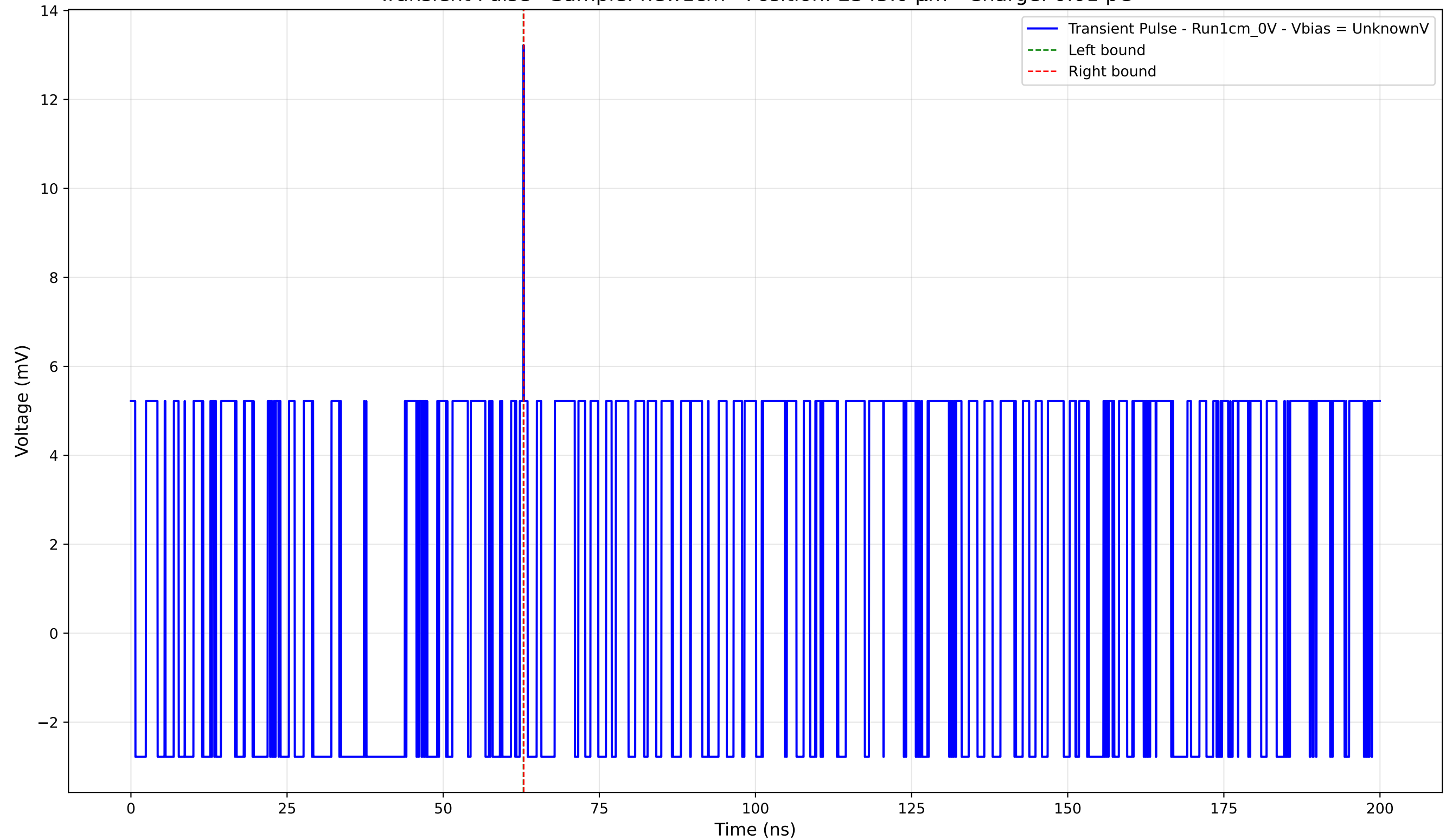
Transient Pulse - Sample: new1cm - Position: 2345.0 \mu\text{m} - Charge: 0.01 pC
