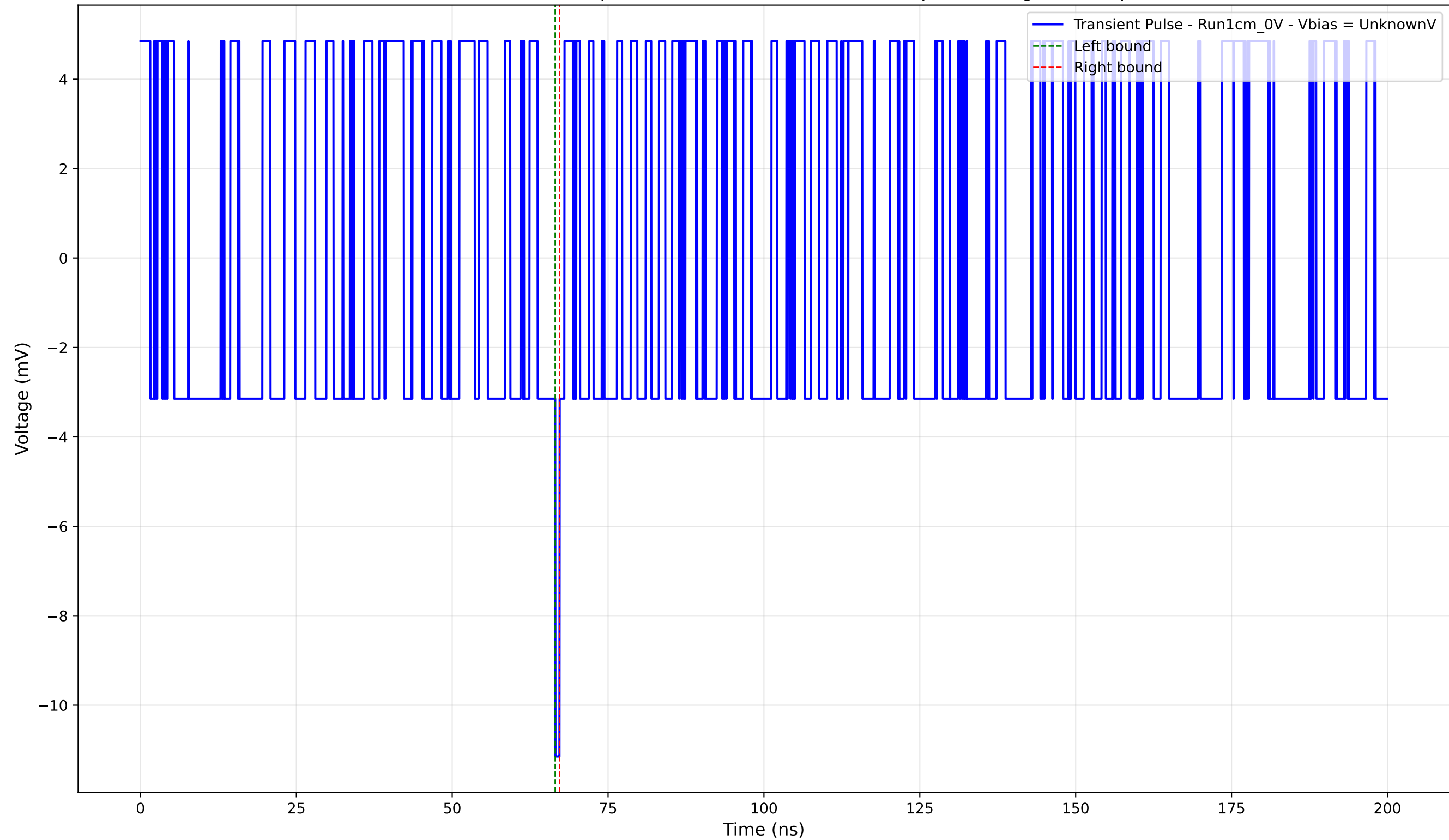
Transient Pulse - Sample: new1cm - Position: 4020.0 \mu\text{m} - Charge: -0.15 pC
