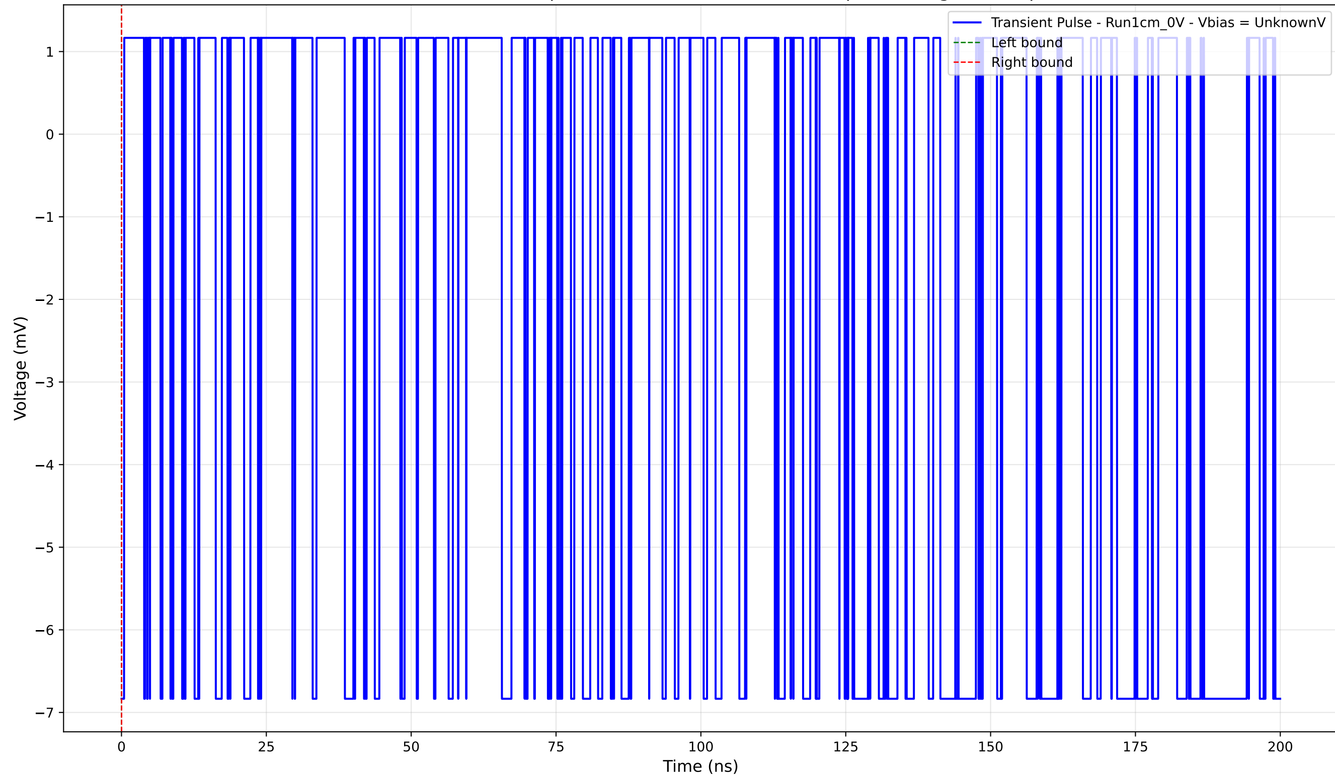
Transient Pulse - Sample: new1cm - Position: 2980.0 \mu\text{m} - Charge: -0.00 pC
