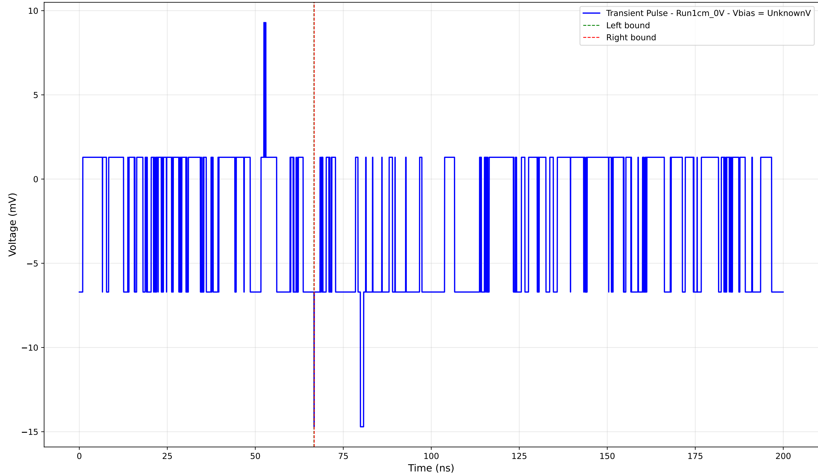
Transient Pulse - Sample: new1cm - Position: 2240.0 \mu\text{m} - Charge: -0.02 pC
