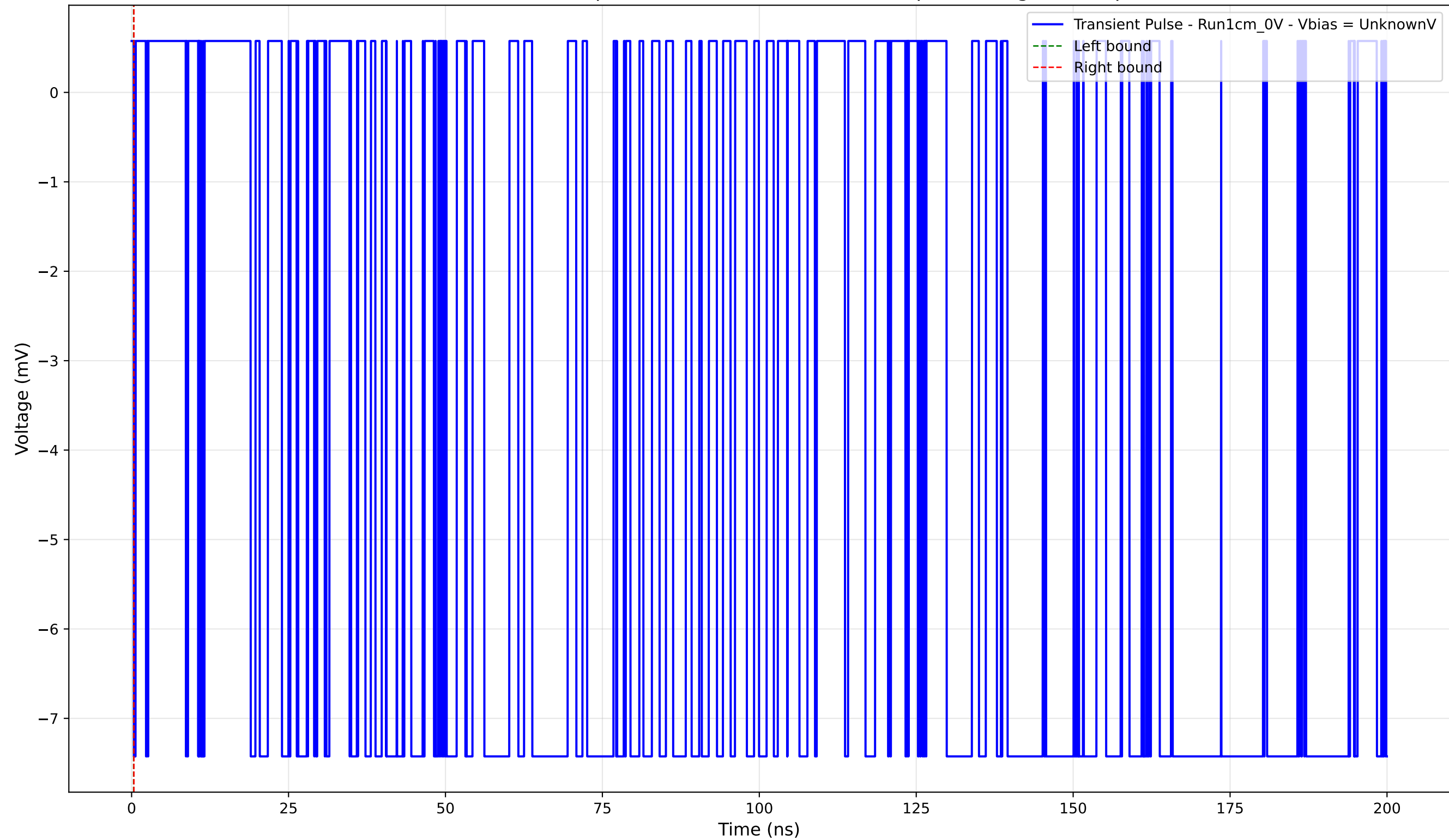
Transient Pulse - Sample: new1cm - Position: 2490.0 \mu\text{m} - Charge: -0.00 pC
