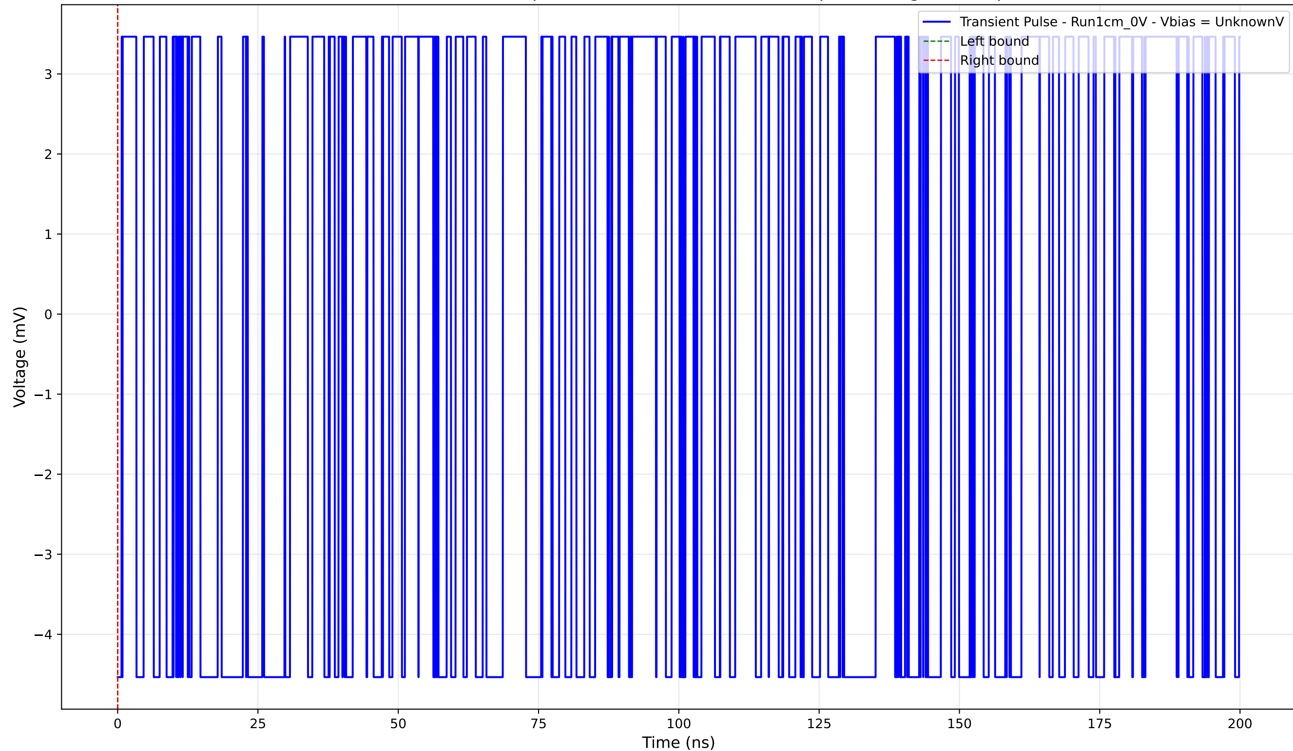
Transient Pulse - Sample: new1cm - Position: 4295.0 \mu\text{m} - Charge: -0.00 pC
