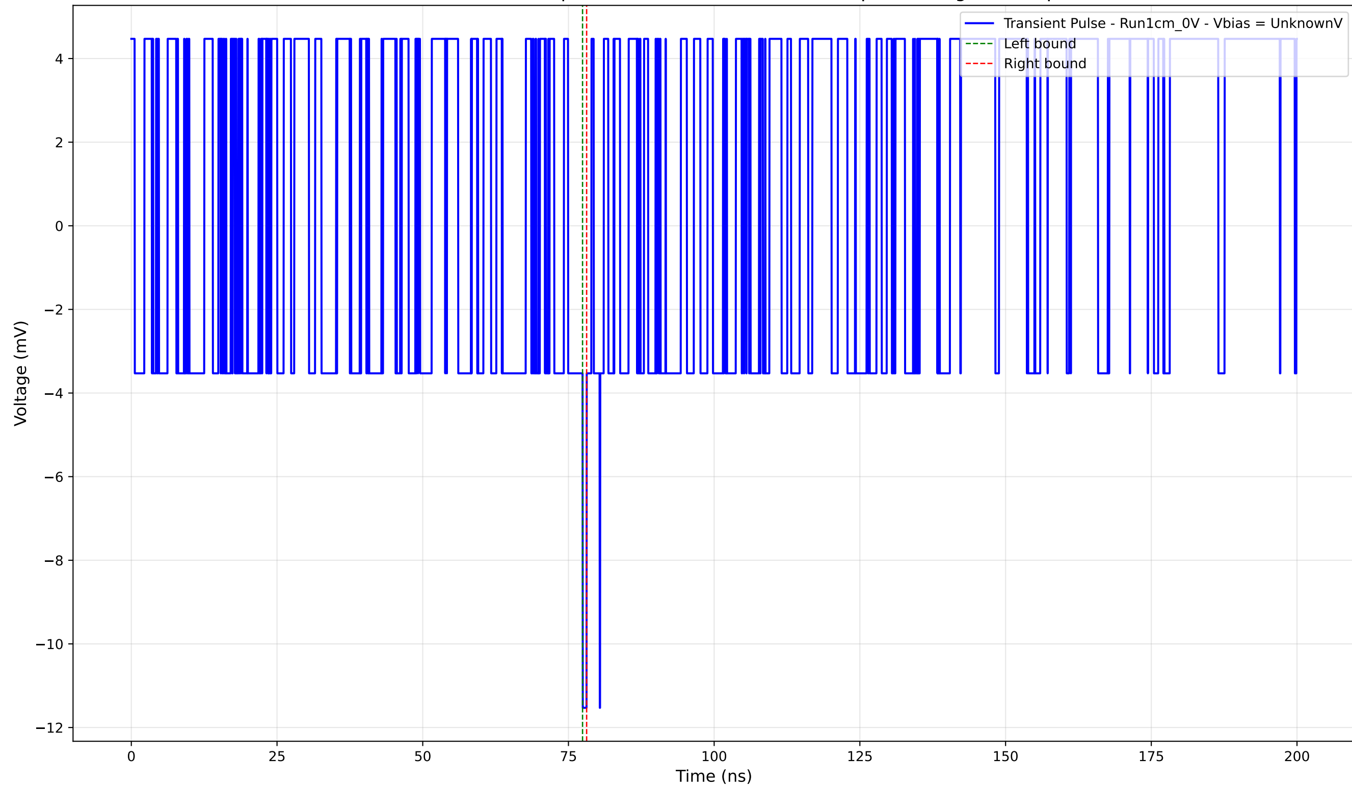
Transient Pulse - Sample: new1cm - Position: 1615.0 \mu\text{m} - Charge: -0.16 pC
