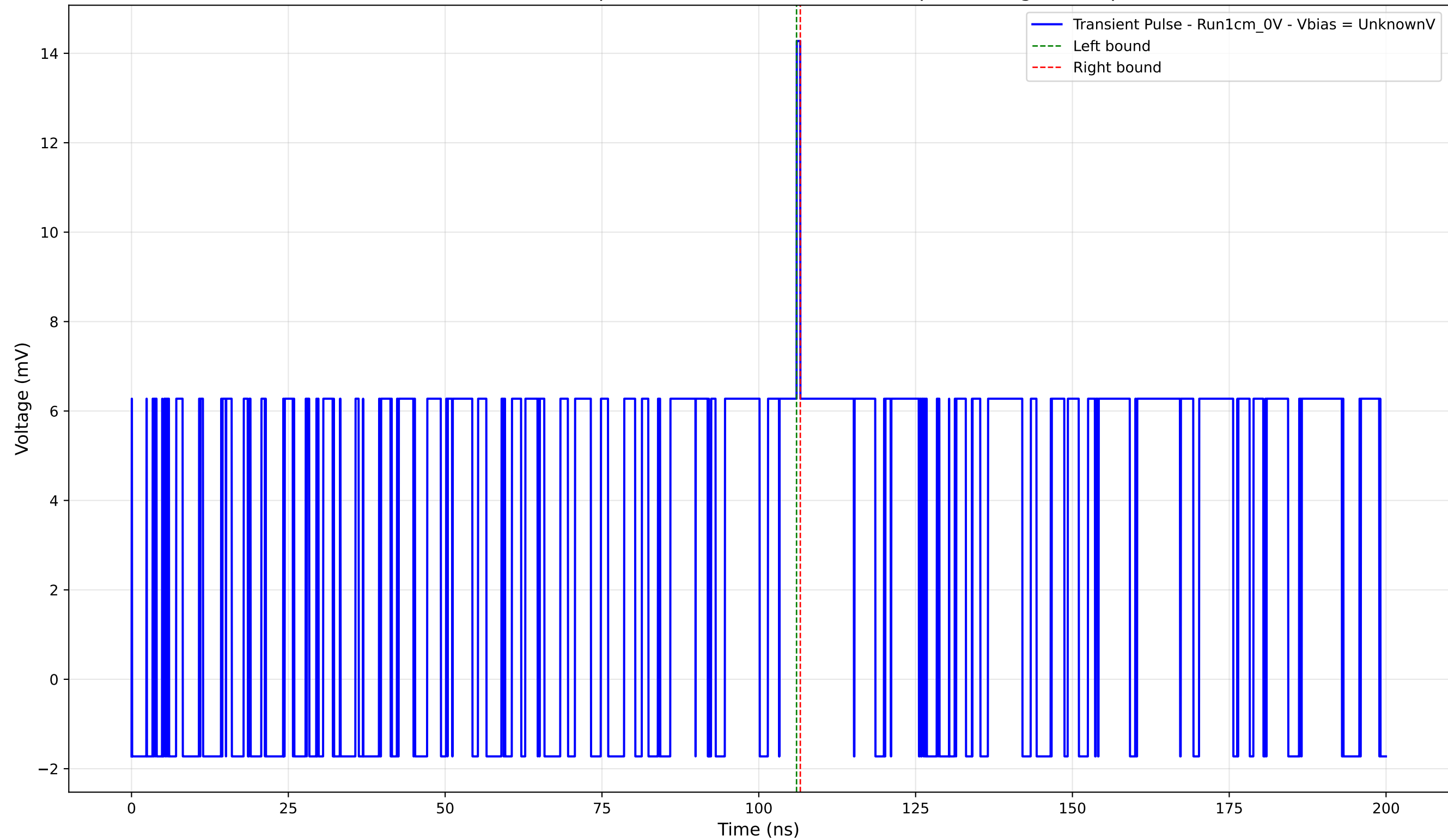
Transient Pulse - Sample: new1cm - Position: 4385.0 \mu\text{m} - Charge: 0.17 pC
