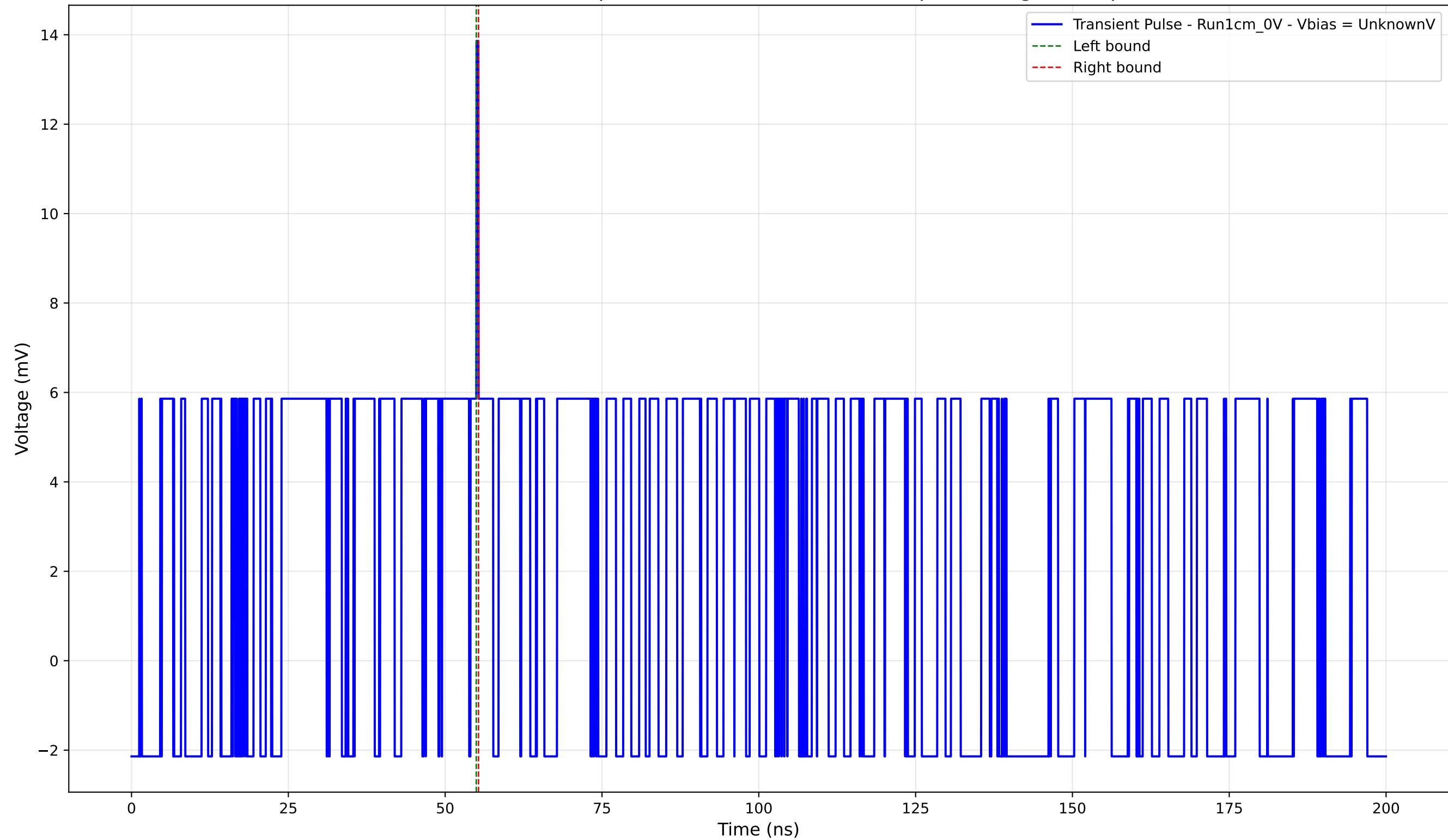
Transient Pulse - Sample: new1cm - Position: 1290.0 \mu\text{m} - Charge: 0.10 pC
