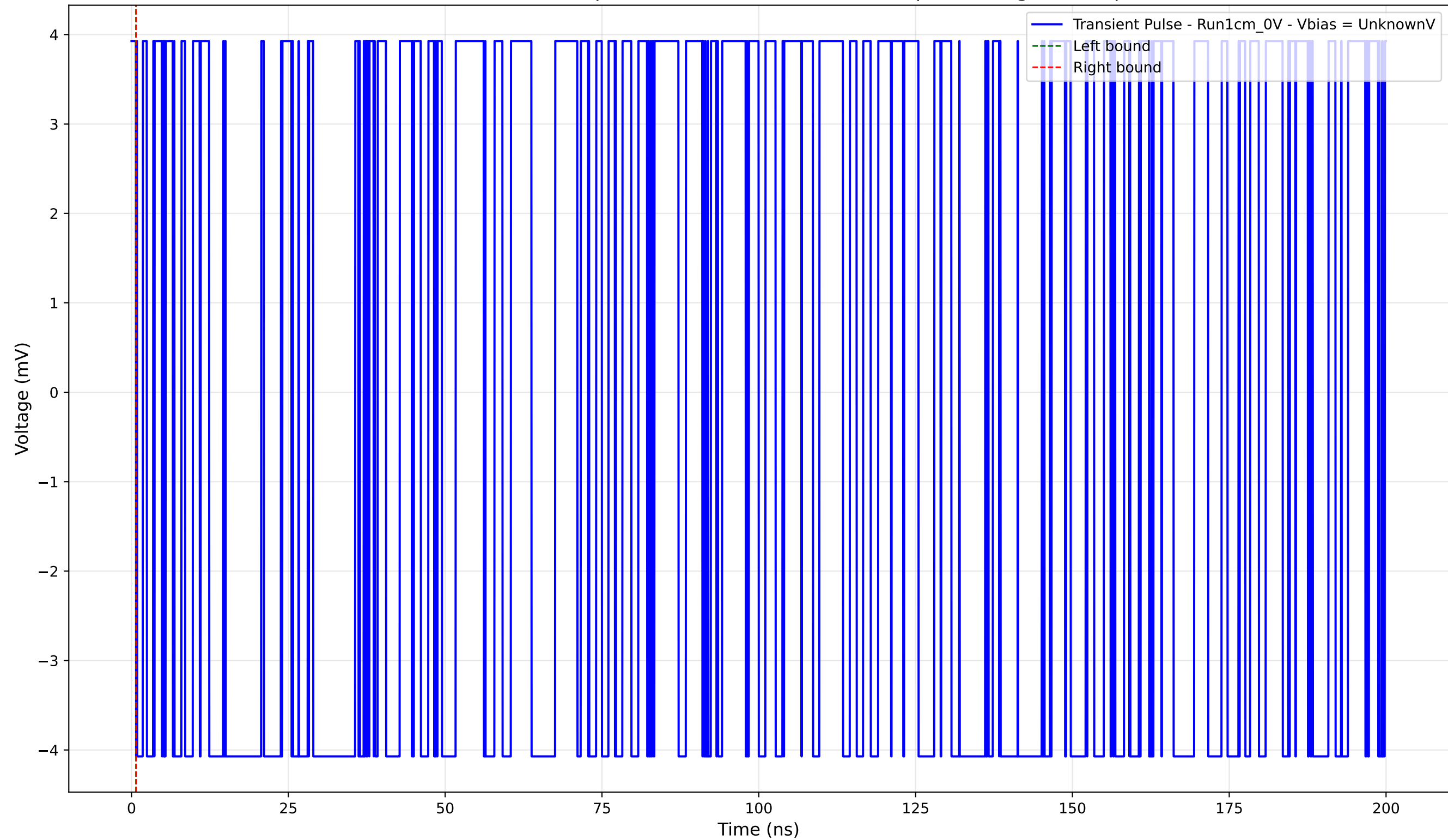
Transient Pulse - Sample: new1cm - Position: 3725.0 \mu\text{m} - Charge: -0.00 pC
