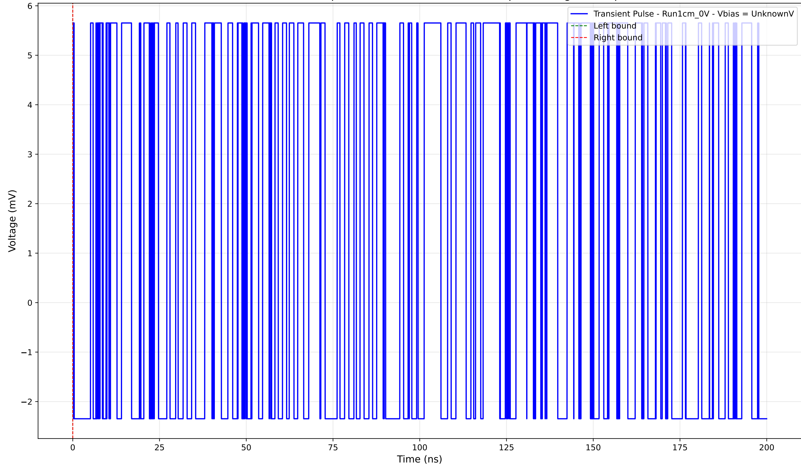
Transient Pulse - Sample: new1cm - Position: 1330.0 \mu\text{m} - Charge: 0.00 pC
