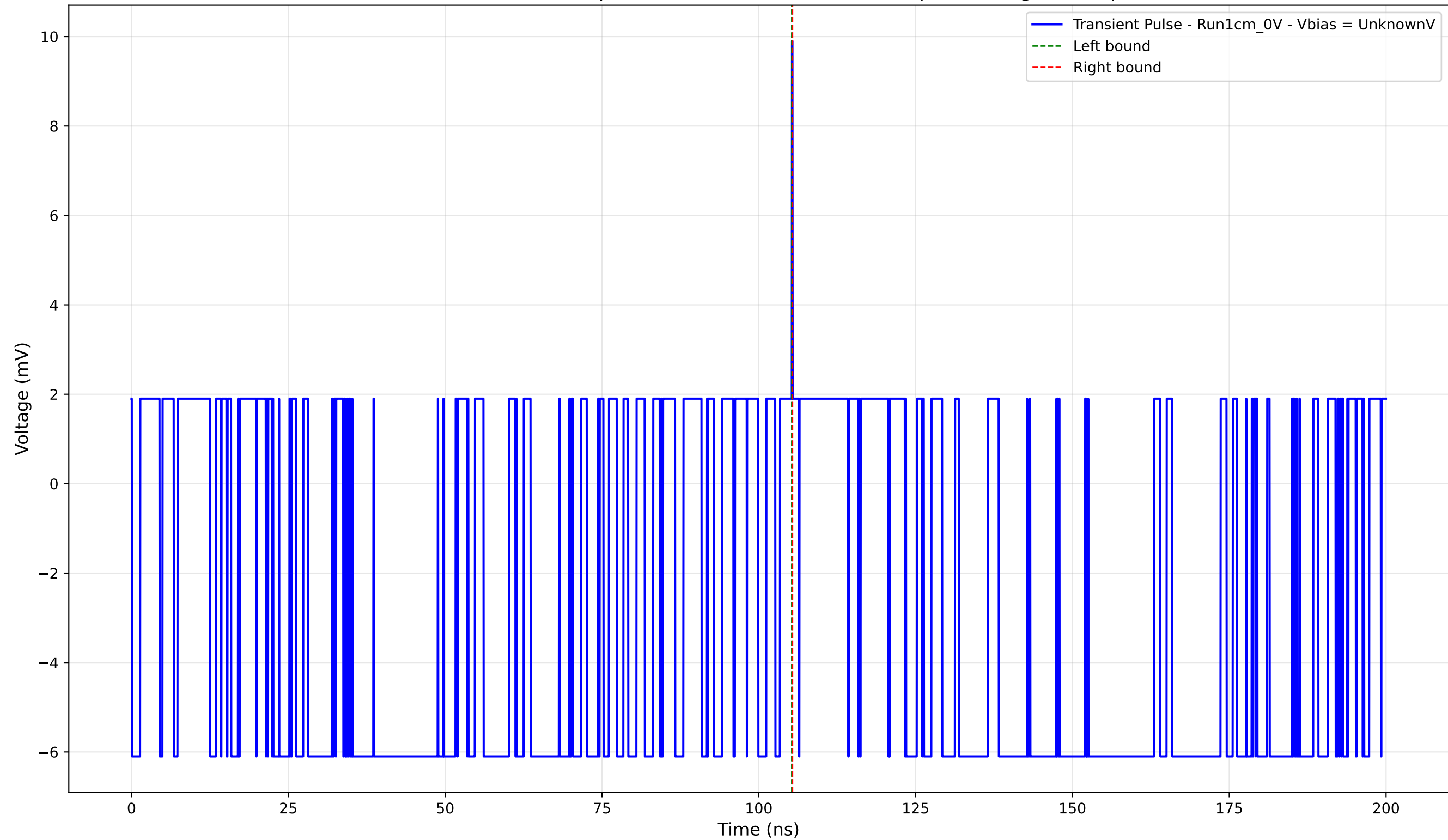
Transient Pulse - Sample: new1cm - Position: 1945.0 \mu\text{m} - Charge: 0.02 pC
