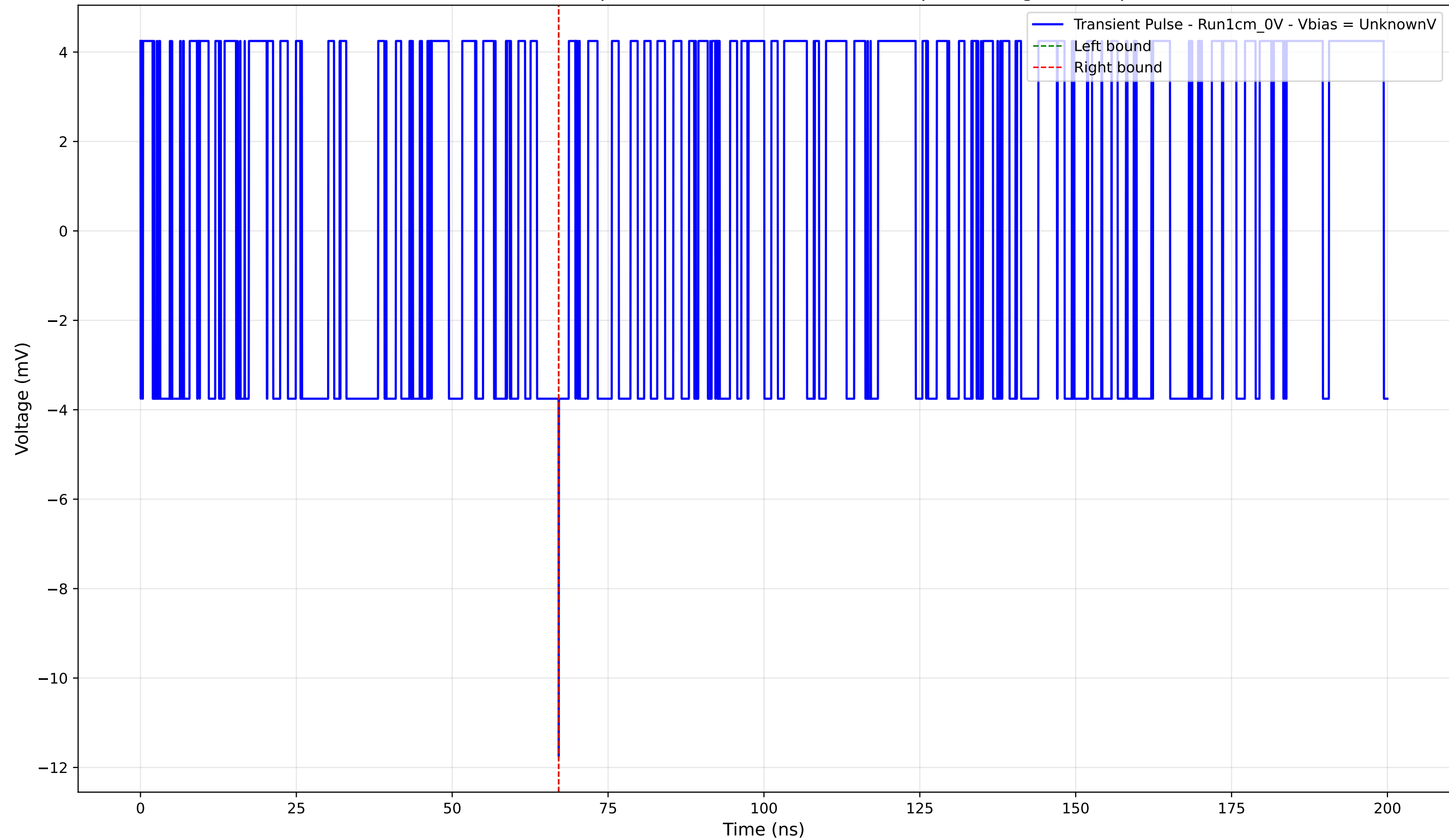
Transient Pulse - Sample: new1cm - Position: 1970.0 \mu\text{m} - Charge: -0.01 pC
