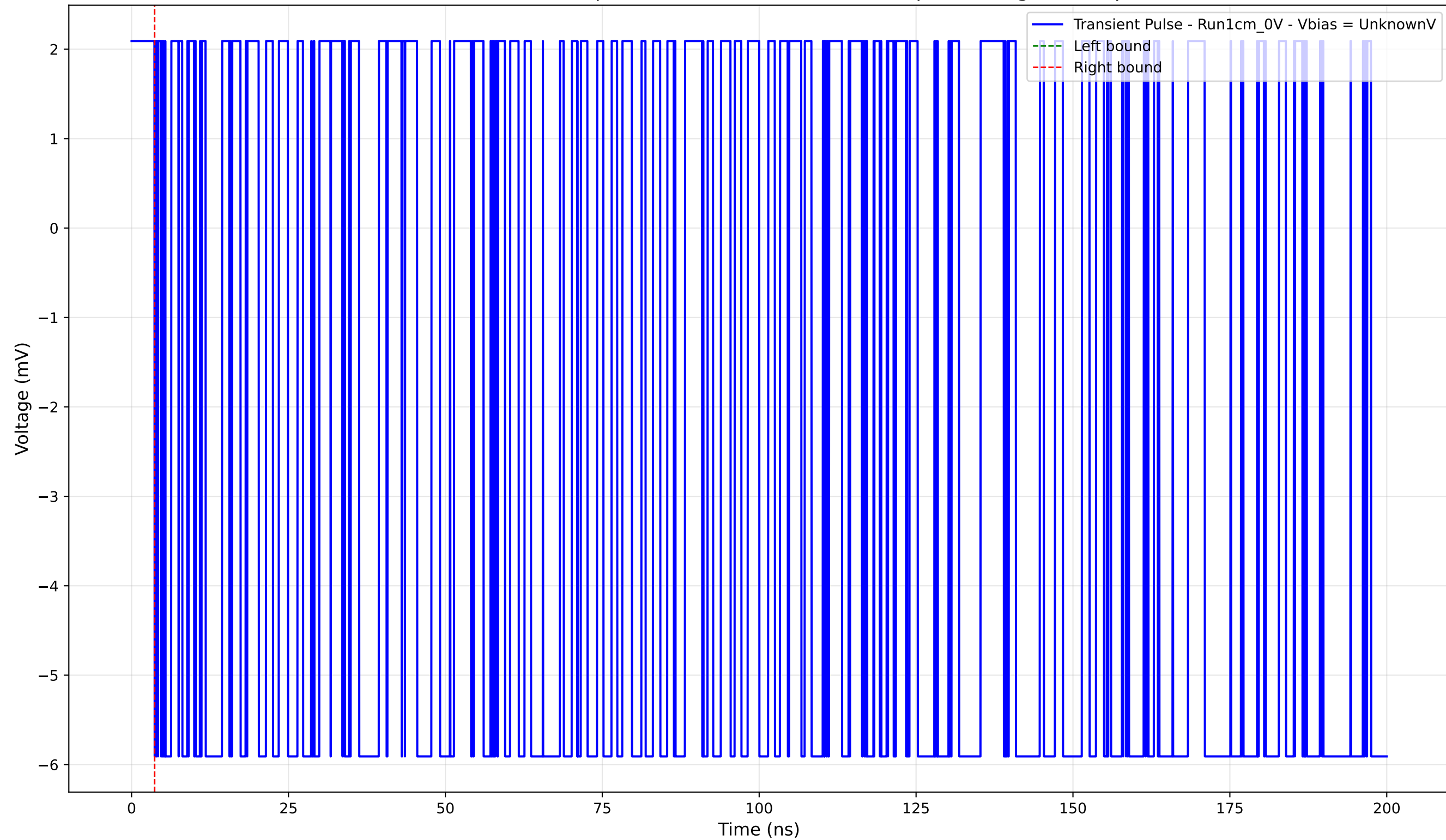
Transient Pulse - Sample: new1cm - Position: 3320.0 \mu\text{m} - Charge: -0.00 pC
