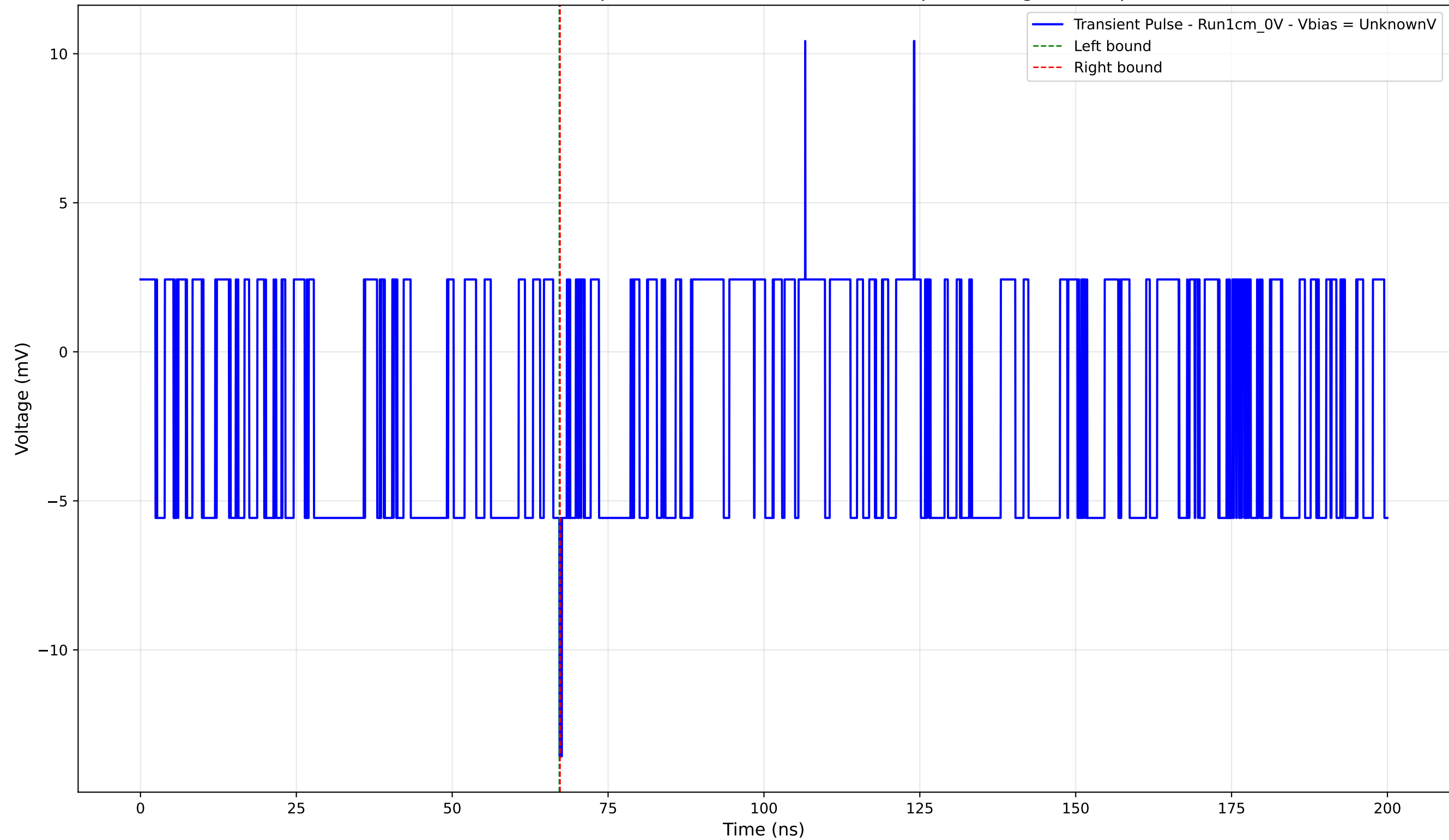
Transient Pulse - Sample: new1cm - Position: 4570.0 \mu\text{m} - Charge: -0.03 pC
