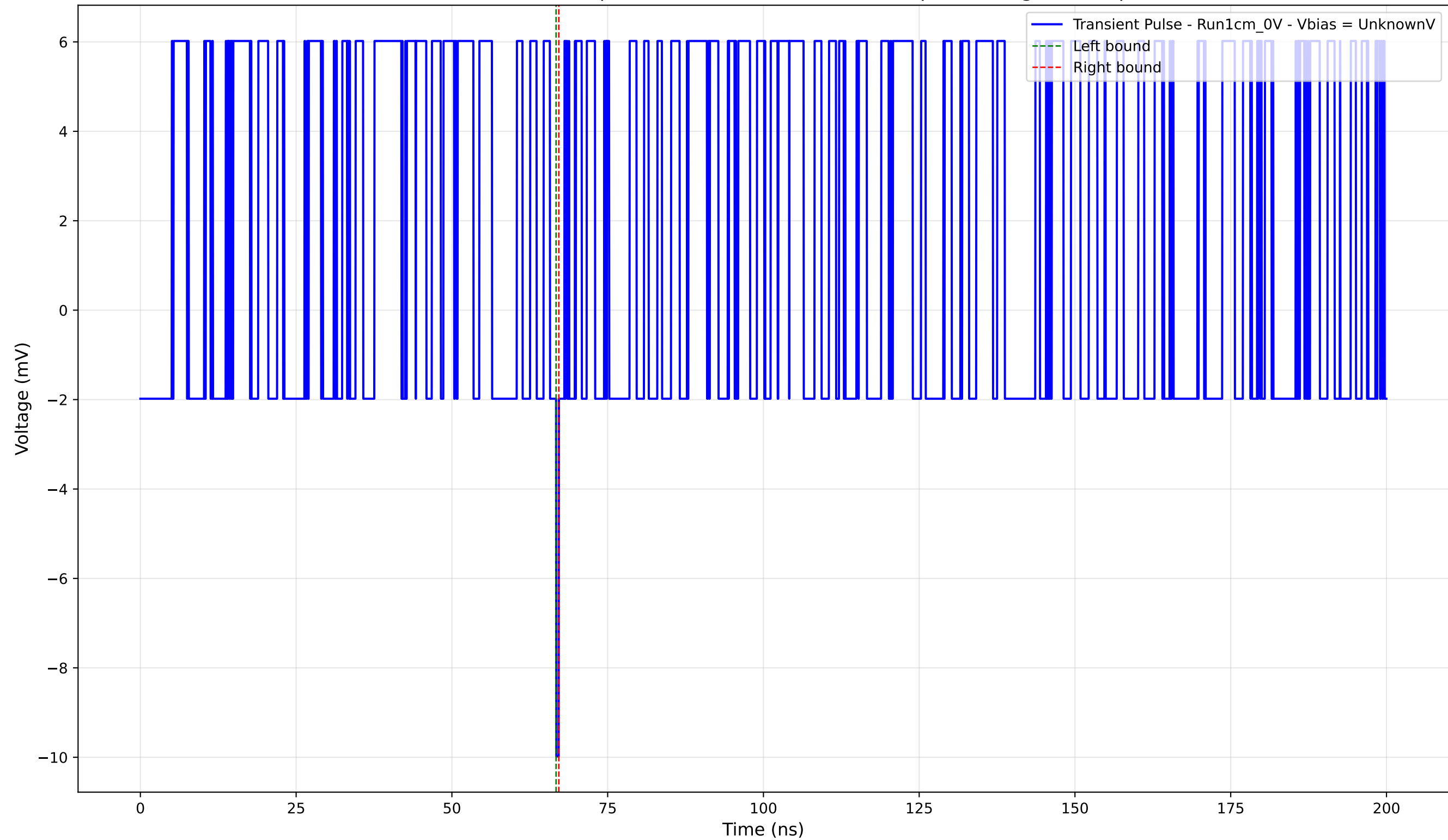
Transient Pulse - Sample: new1cm - Position: 2895.0 \mu\text{m} - Charge: -0.08 pC
