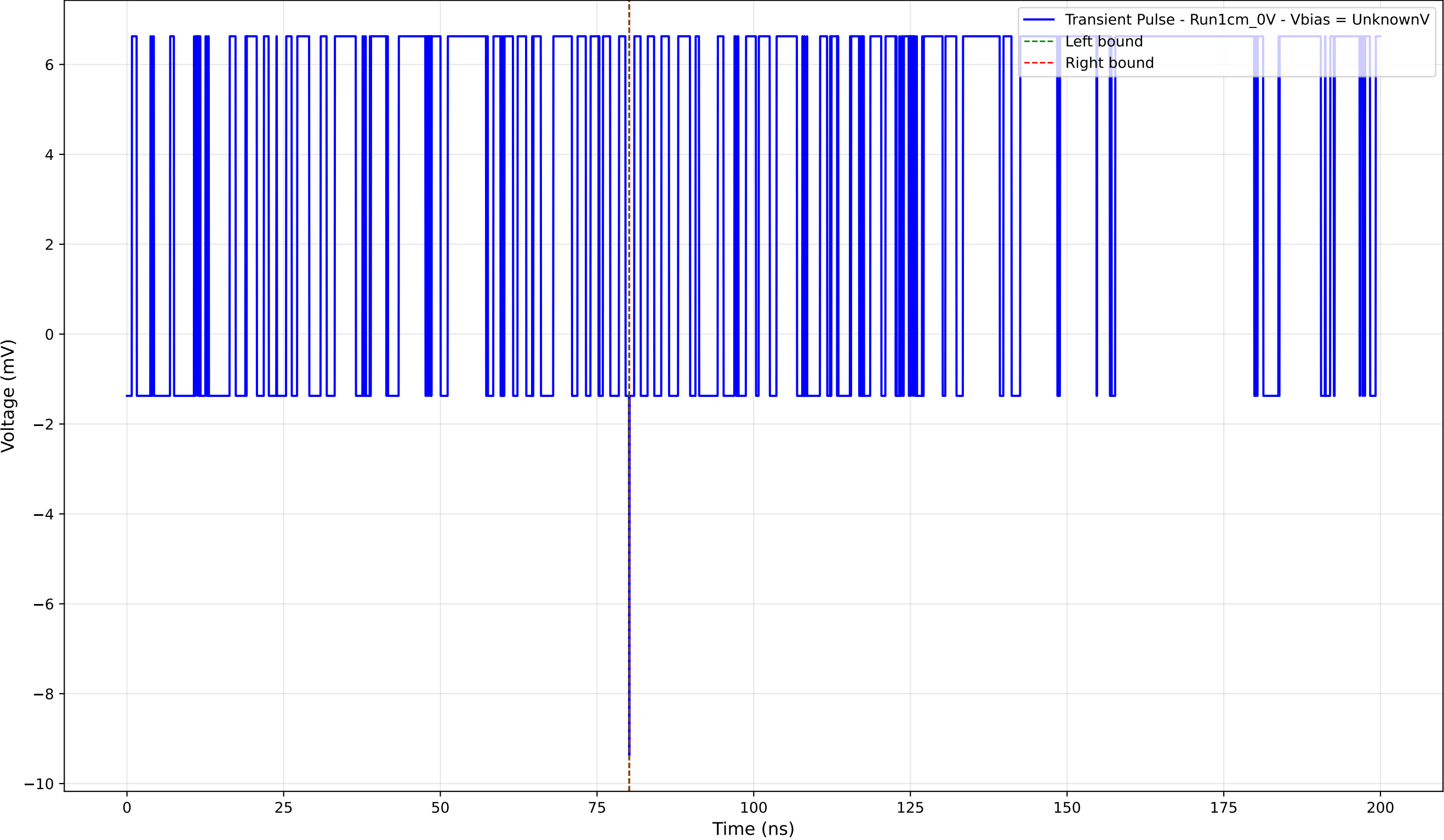
Transient Pulse - Sample: new1cm - Position: 695.0 \mu\text{m} - Charge: -0.01 pC
