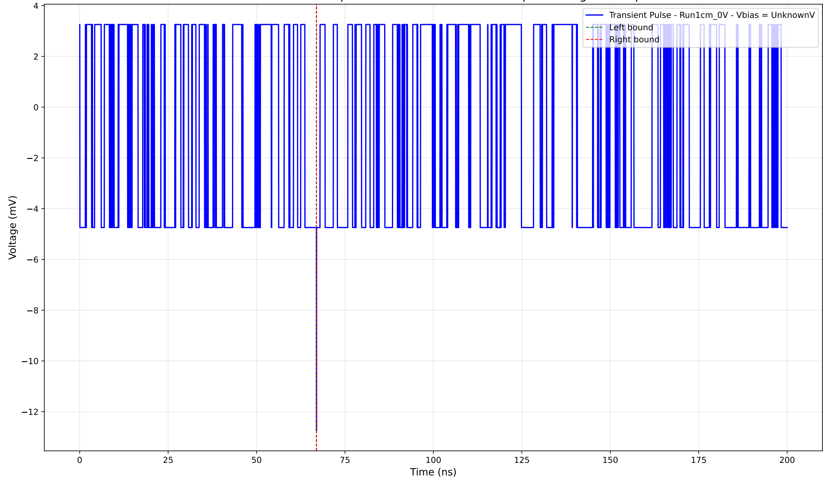
Transient Pulse - Sample: new1cm - Position: 3590.0 \mu\text{m} - Charge: -0.01 pC
