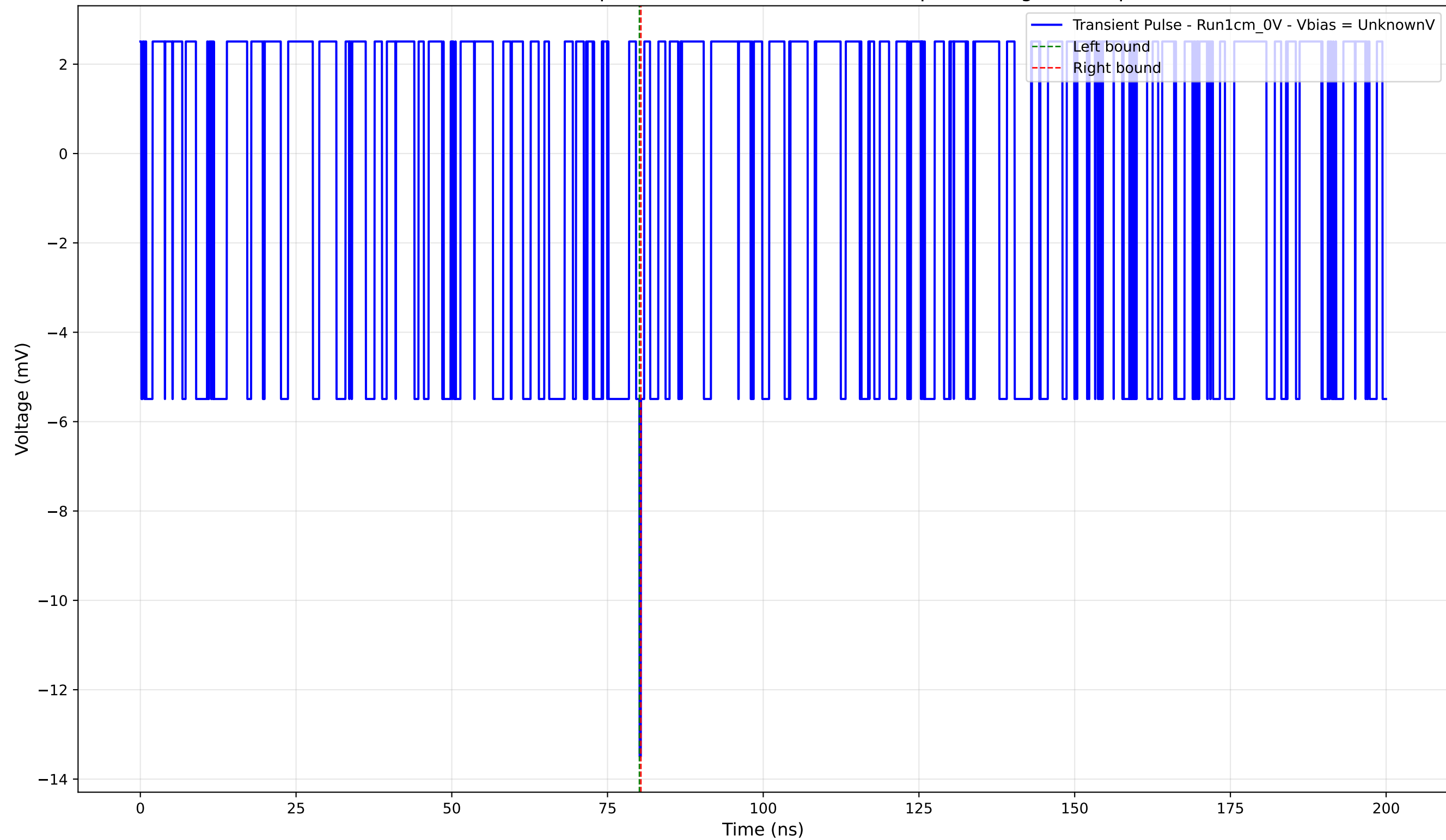
Transient Pulse - Sample: new1cm - Position: 3065.0 \mu\text{m} - Charge: -0.06 pC
