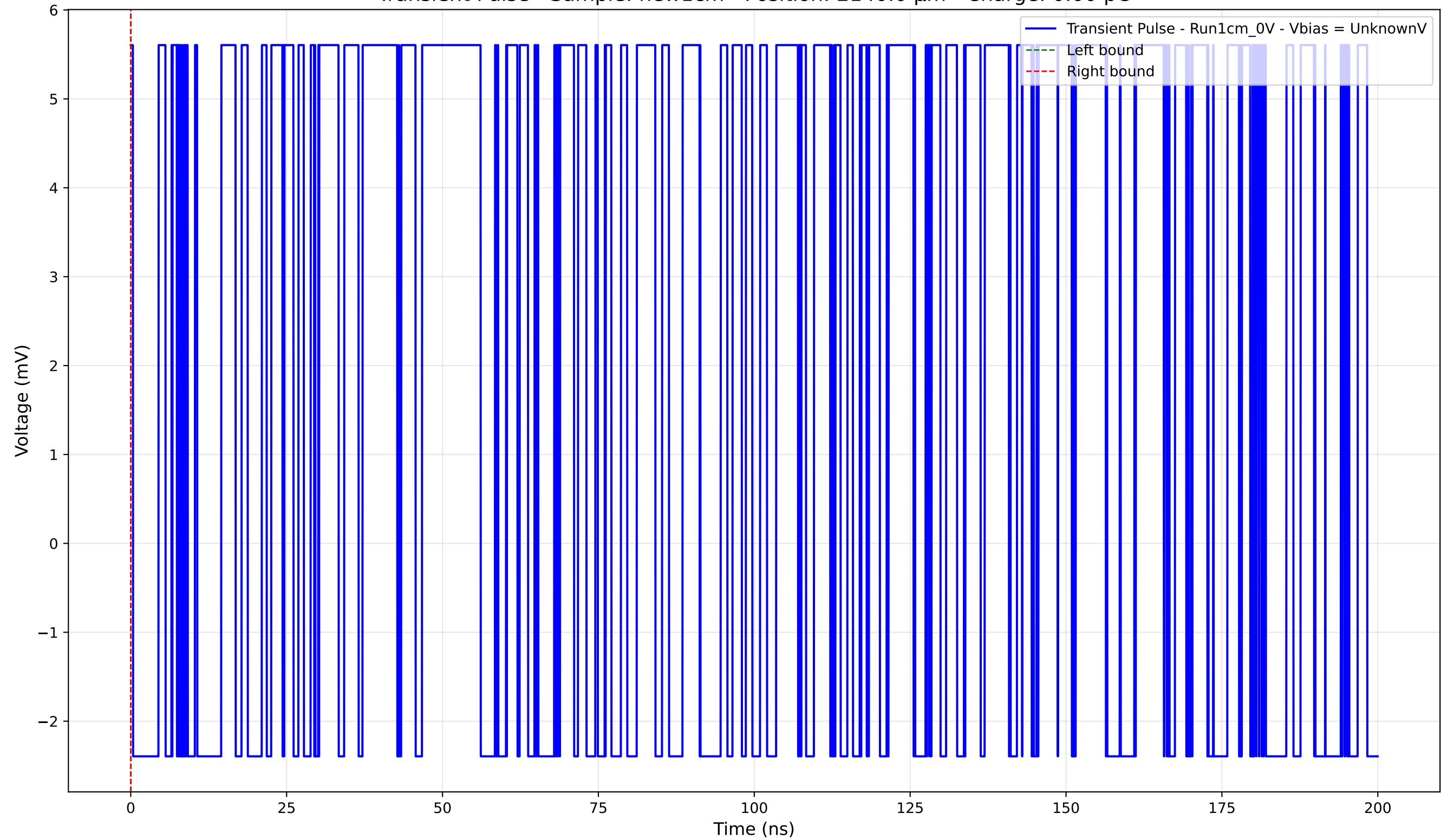
Transient Pulse - Sample: new1cm - Position: 2140.0 \mu\text{m} - Charge: 0.00 pC
