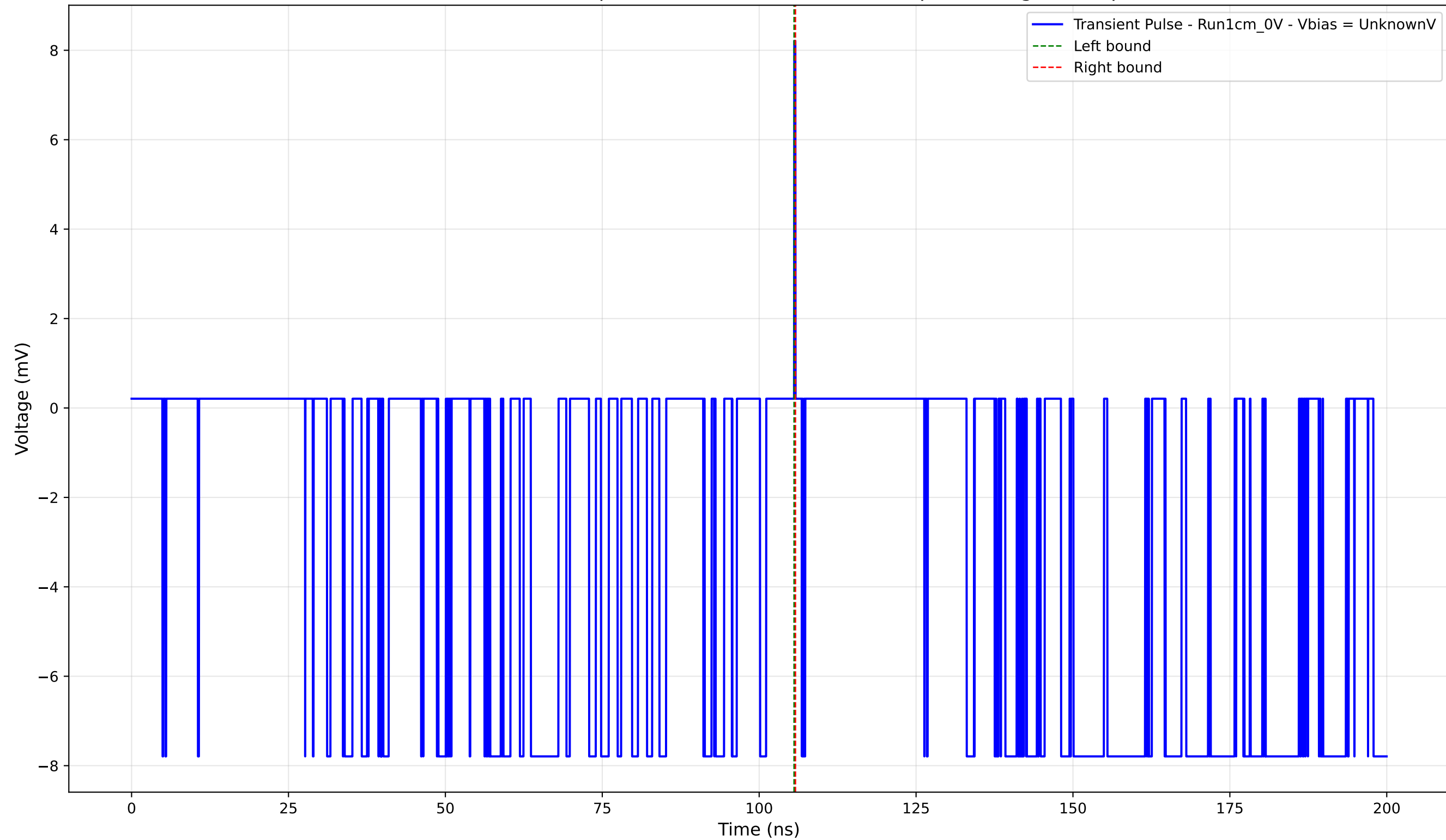
Transient Pulse - Sample: new1cm - Position: 1235.0 \mu\text{m} - Charge: 0.03 pC
