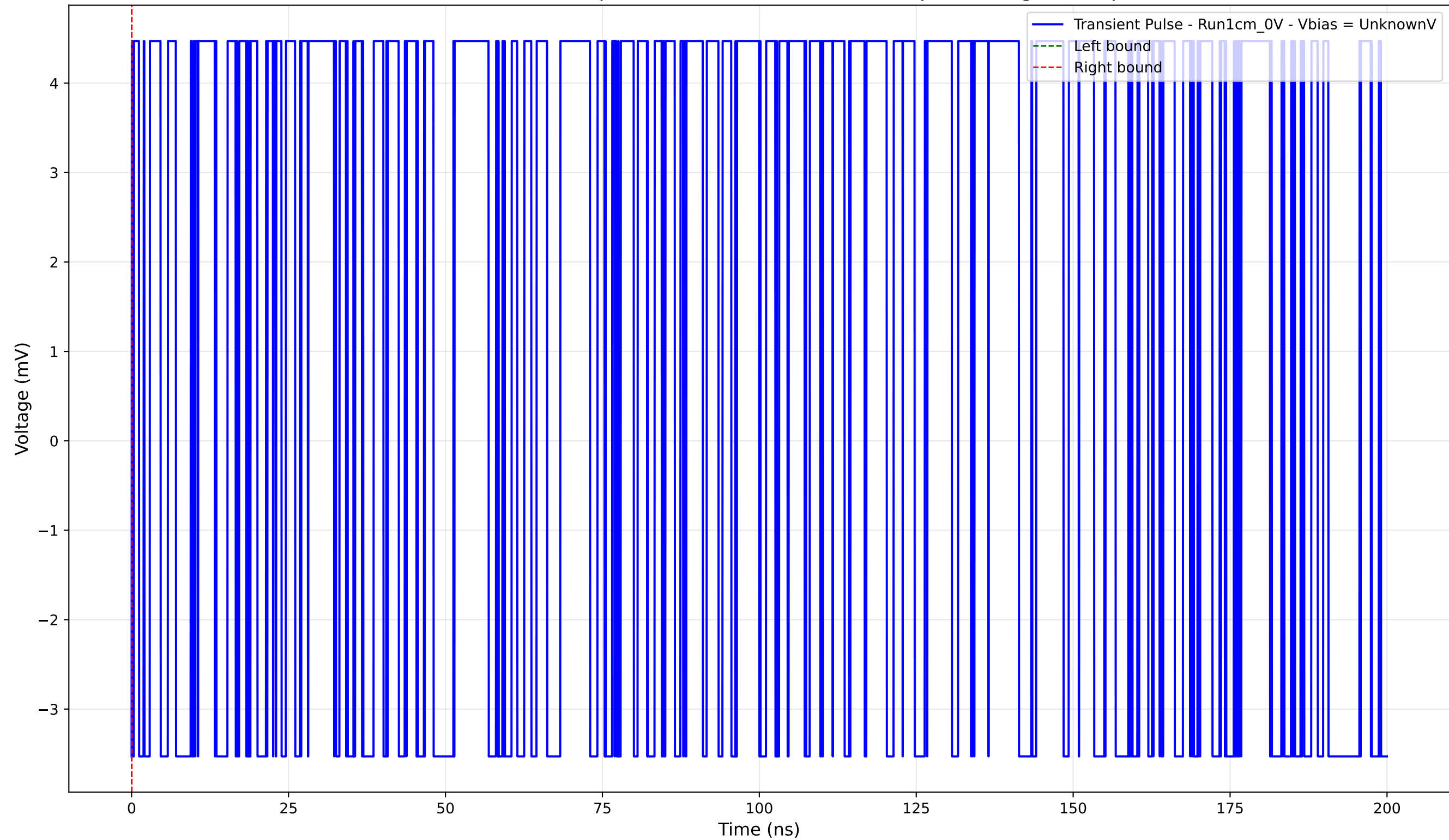
Transient Pulse - Sample: new1cm -Position: 4345.0 \mu\text{m} - Charge: 0.00 pC
