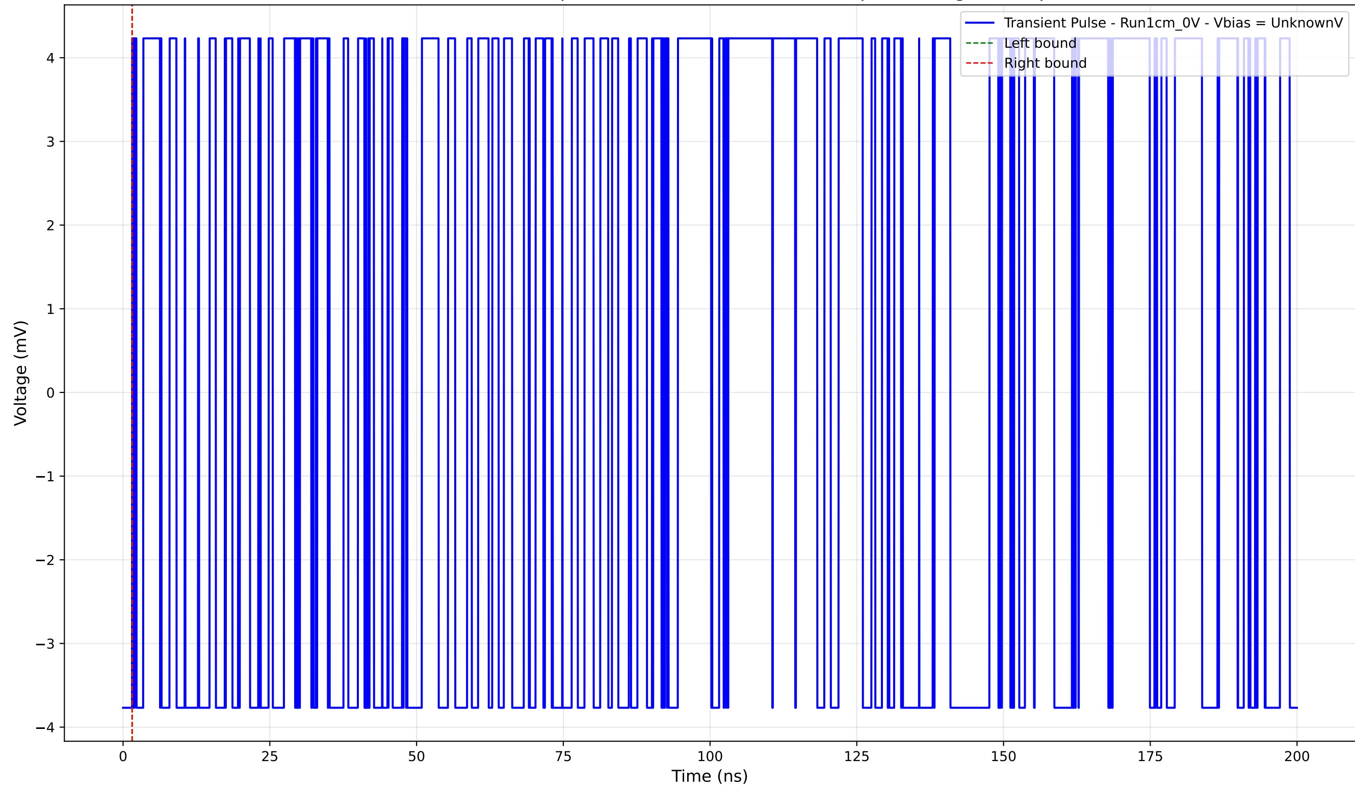
Transient Pulse - Sample: new1cm -Position: 4835.0 \mu\text{m} - Charge: 0.00 pC
