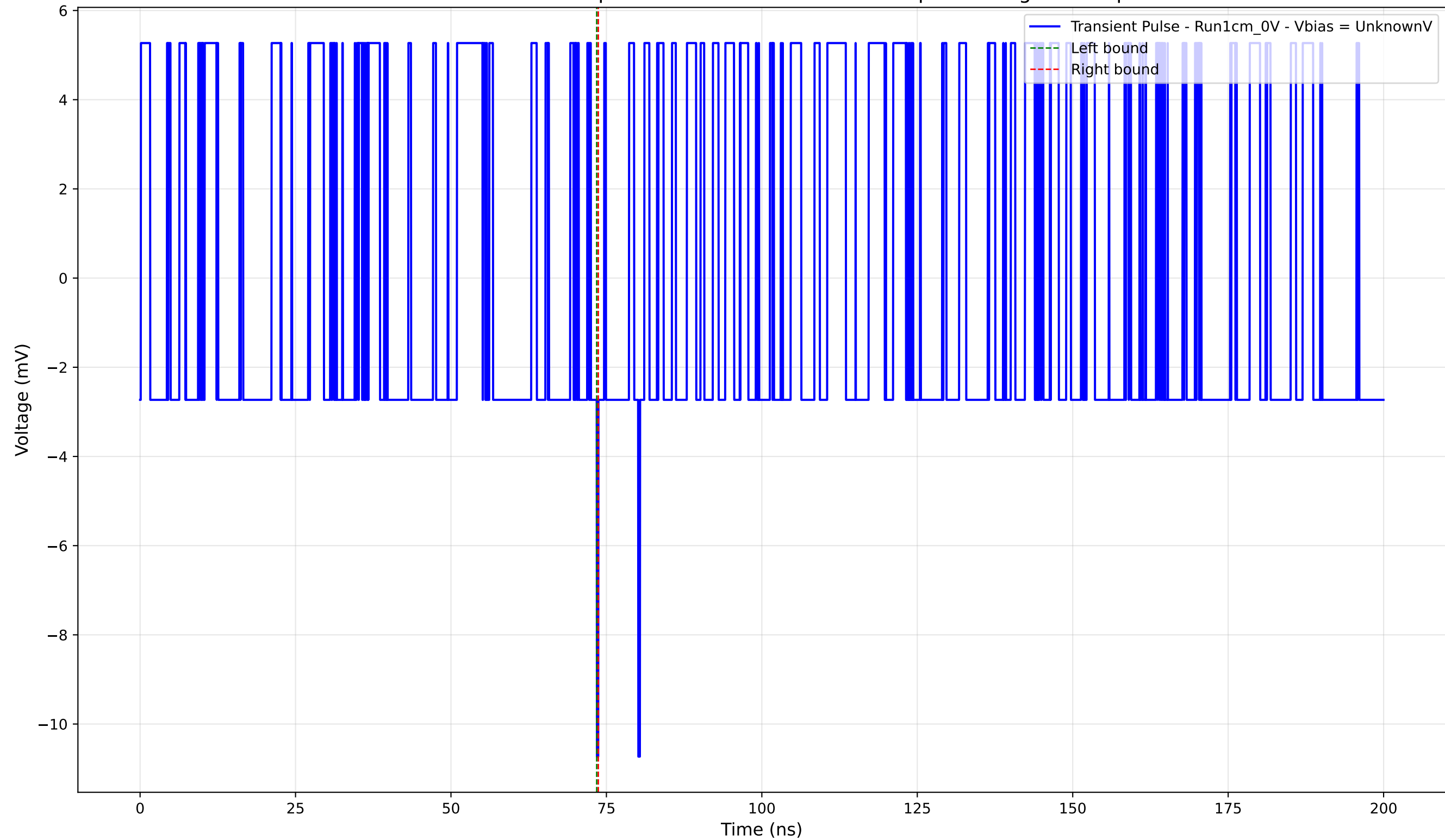
Transient Pulse - Sample: new1cm - Position: 3595.0 \mu\text{m} - Charge: -0.05 pC
