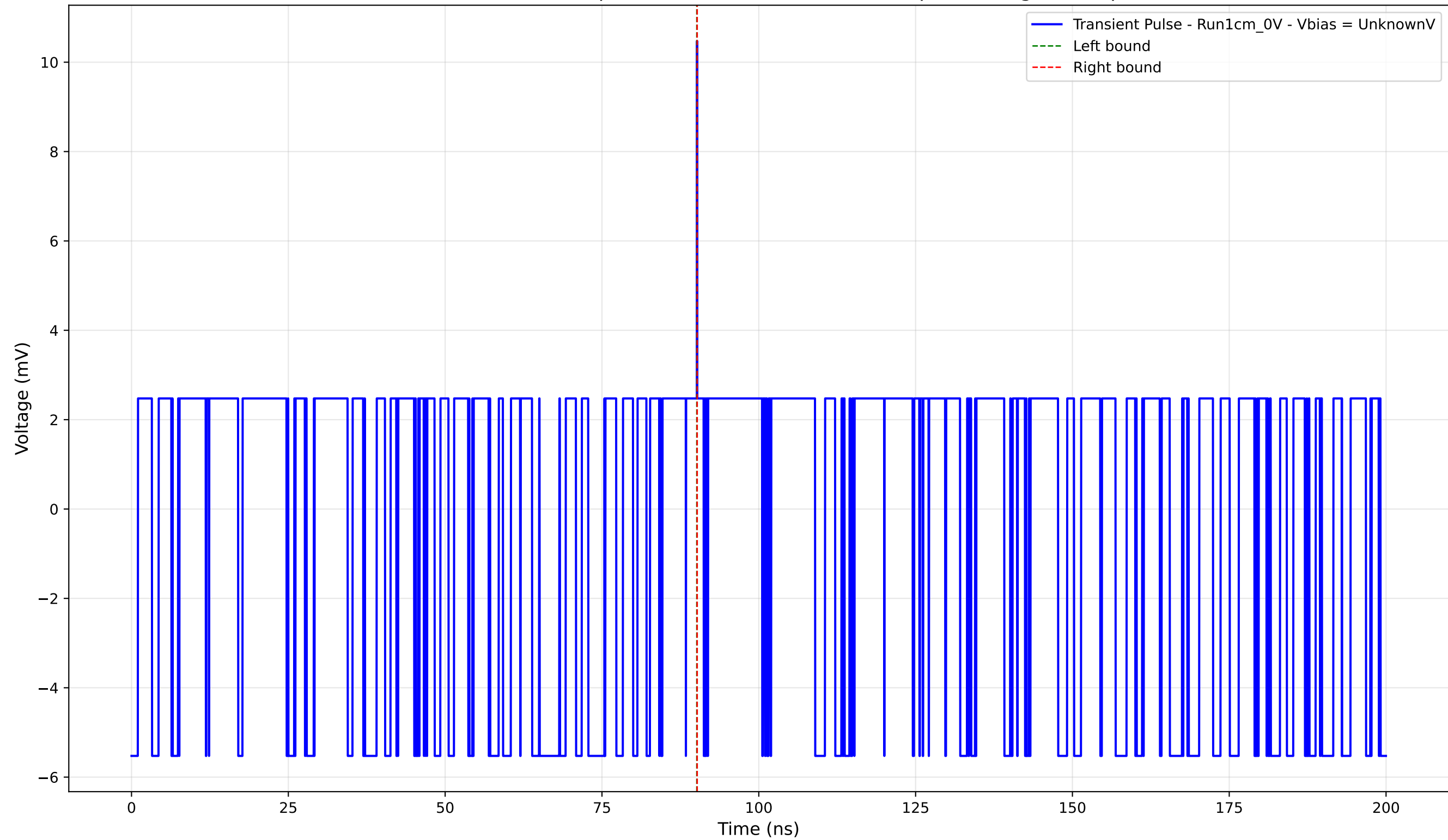
Transient Pulse - Sample: new1cm - Position: 2535.0 \mu\text{m} - Charge: 0.01 pC
