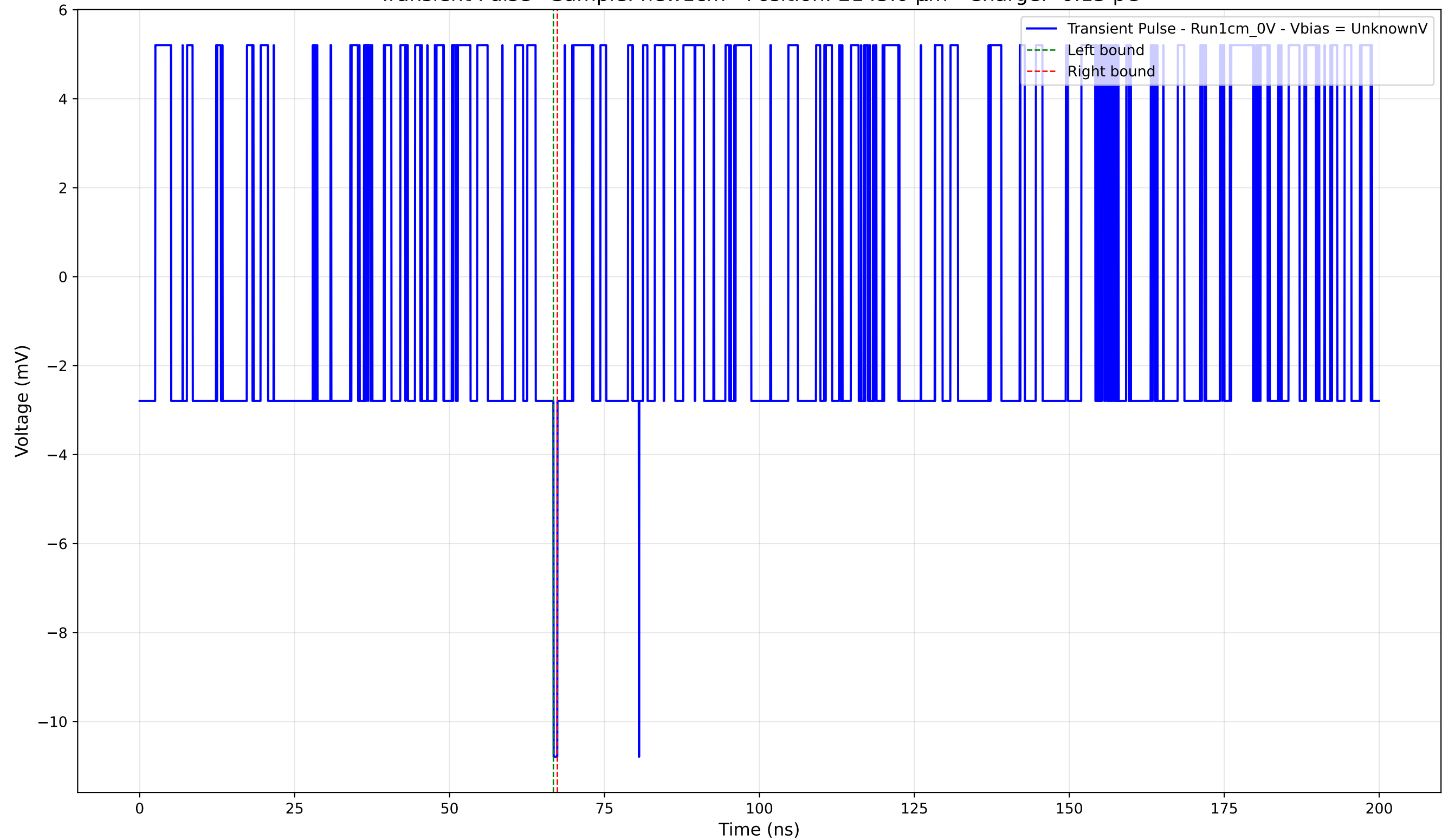
Transient Pulse - Sample: new1cm - Position: 2145.0 \mu\text{m} - Charge: -0.13 pC
