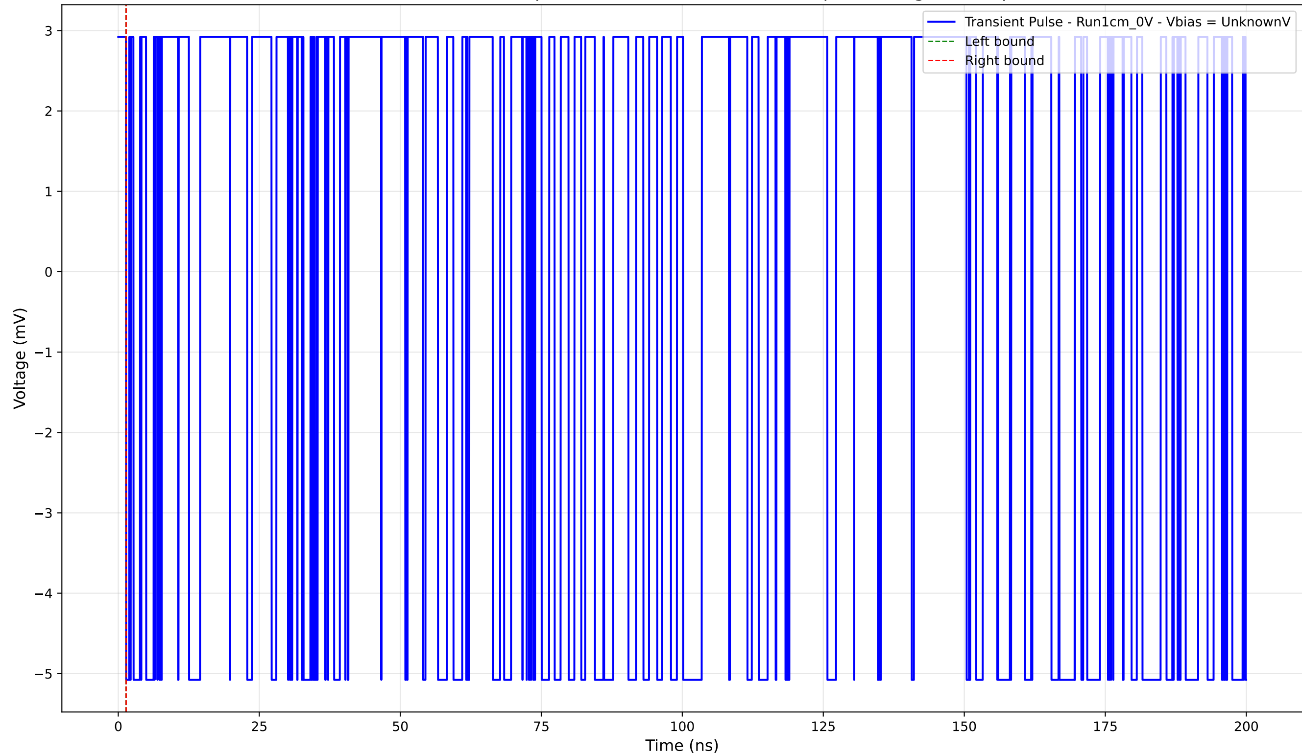
Transient Pulse - Sample: new1cm - Position: 3880.0 \mu\text{m} - Charge: -0.00 pC
