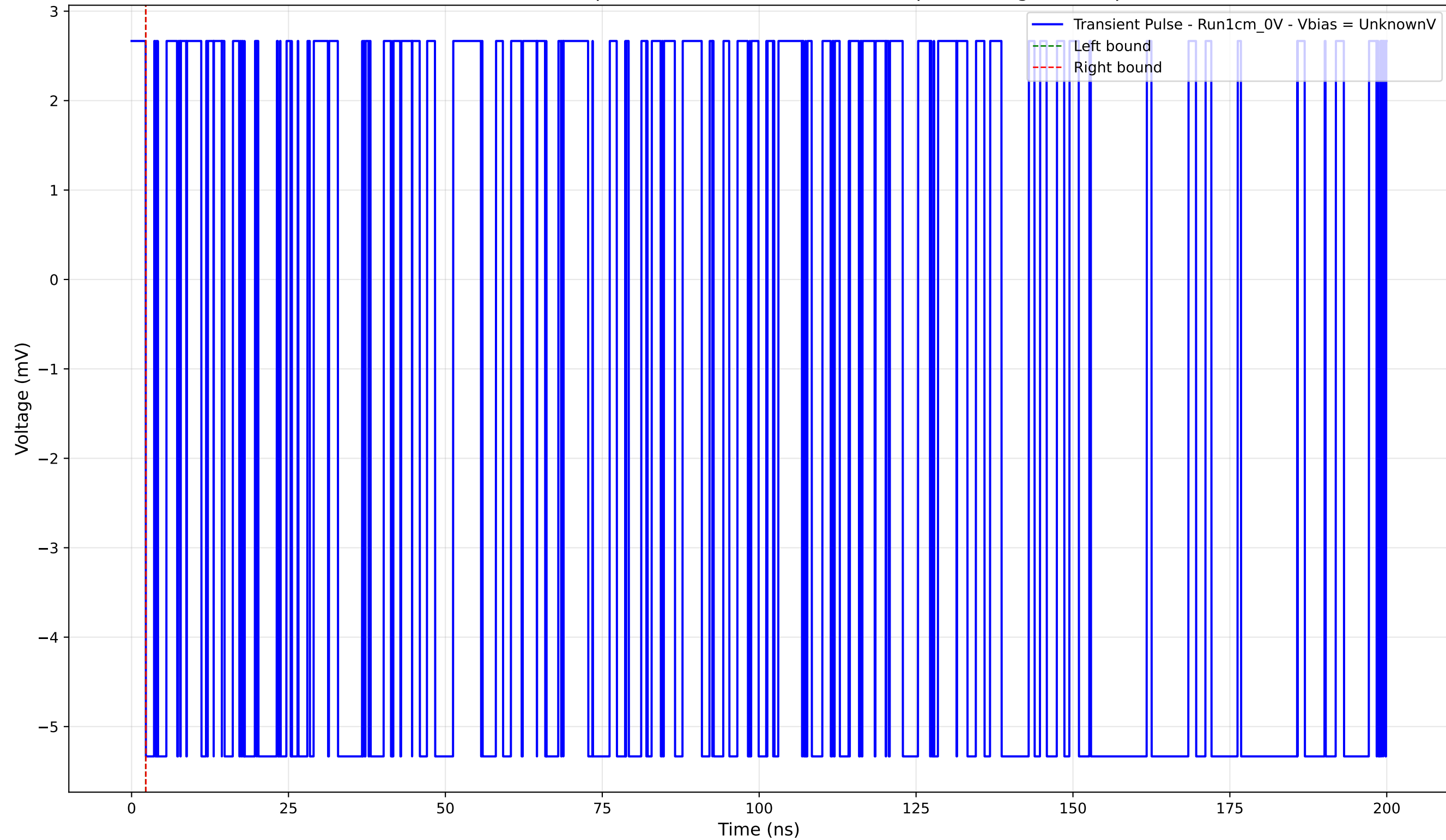
Transient Pulse - Sample: new1cm - Position: 1255.0 \mu\text{m} - Charge: -0.00 pC
