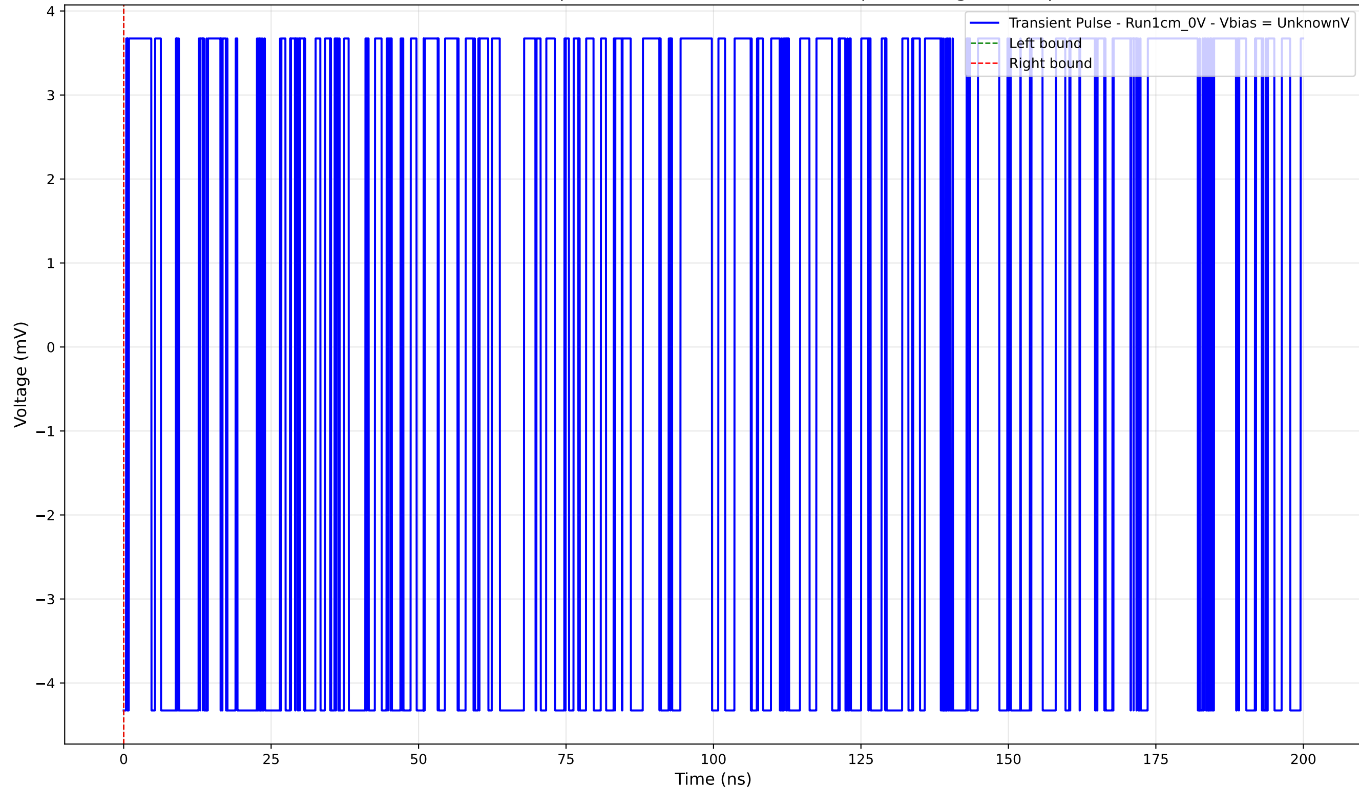
Transient Pulse - Sample: new1cm - Position: 2815.0 \mu\text{m} - Charge: -0.00 pC
