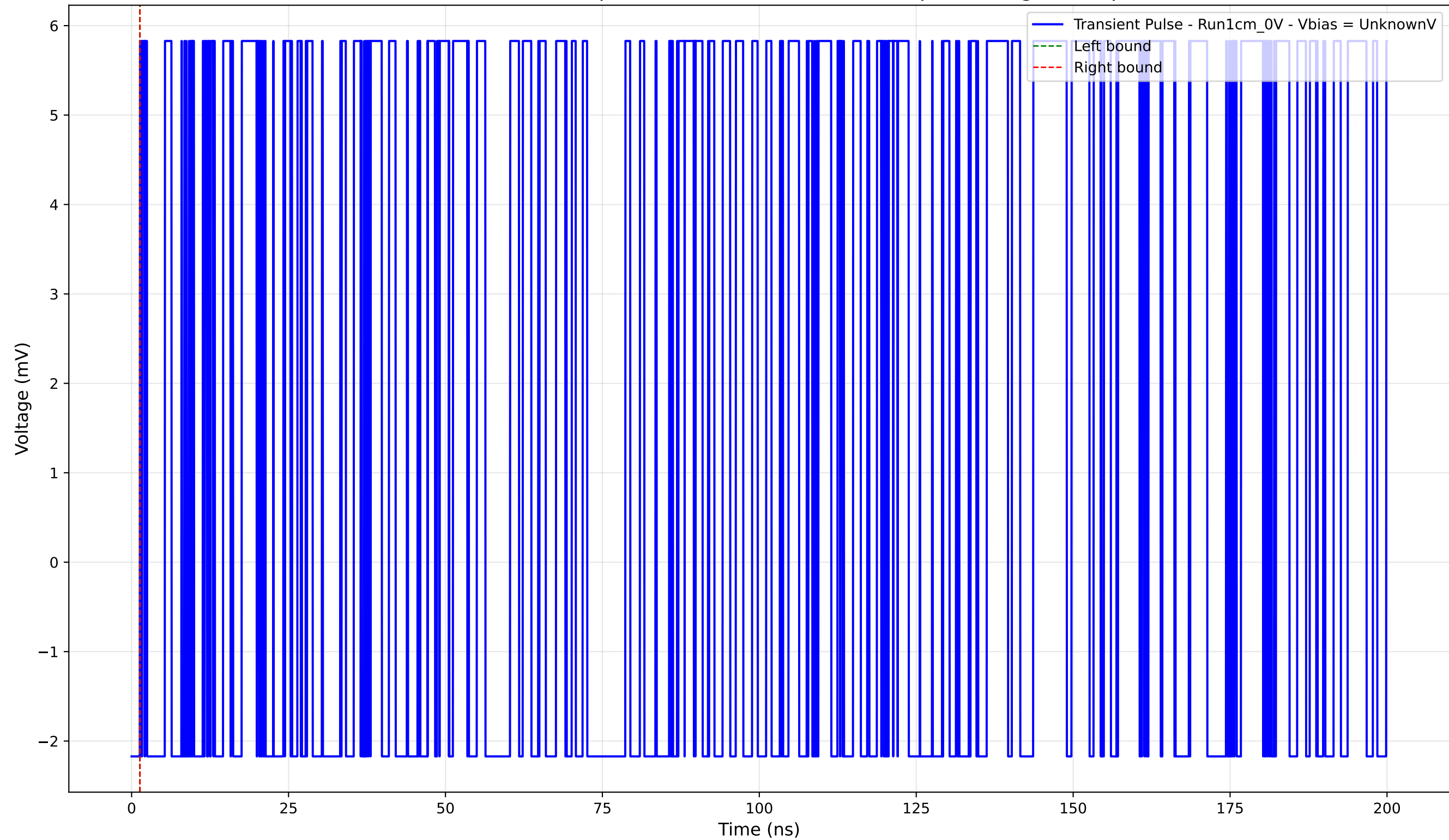
Transient Pulse - Sample: new1cm -Position: 2865.0 \mu\text{m} - Charge: 0.00 pC
