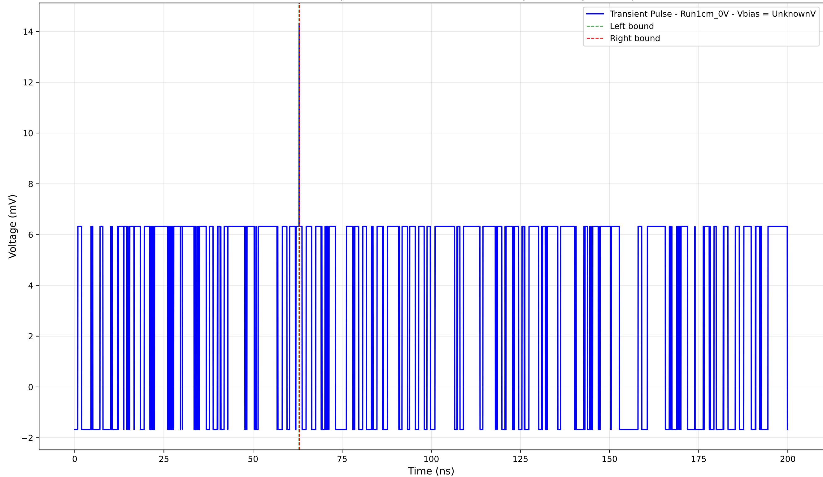
Transient Pulse - Sample: new1cm - Position: 2475.0 \mu\text{m} - Charge: 0.04 pC
