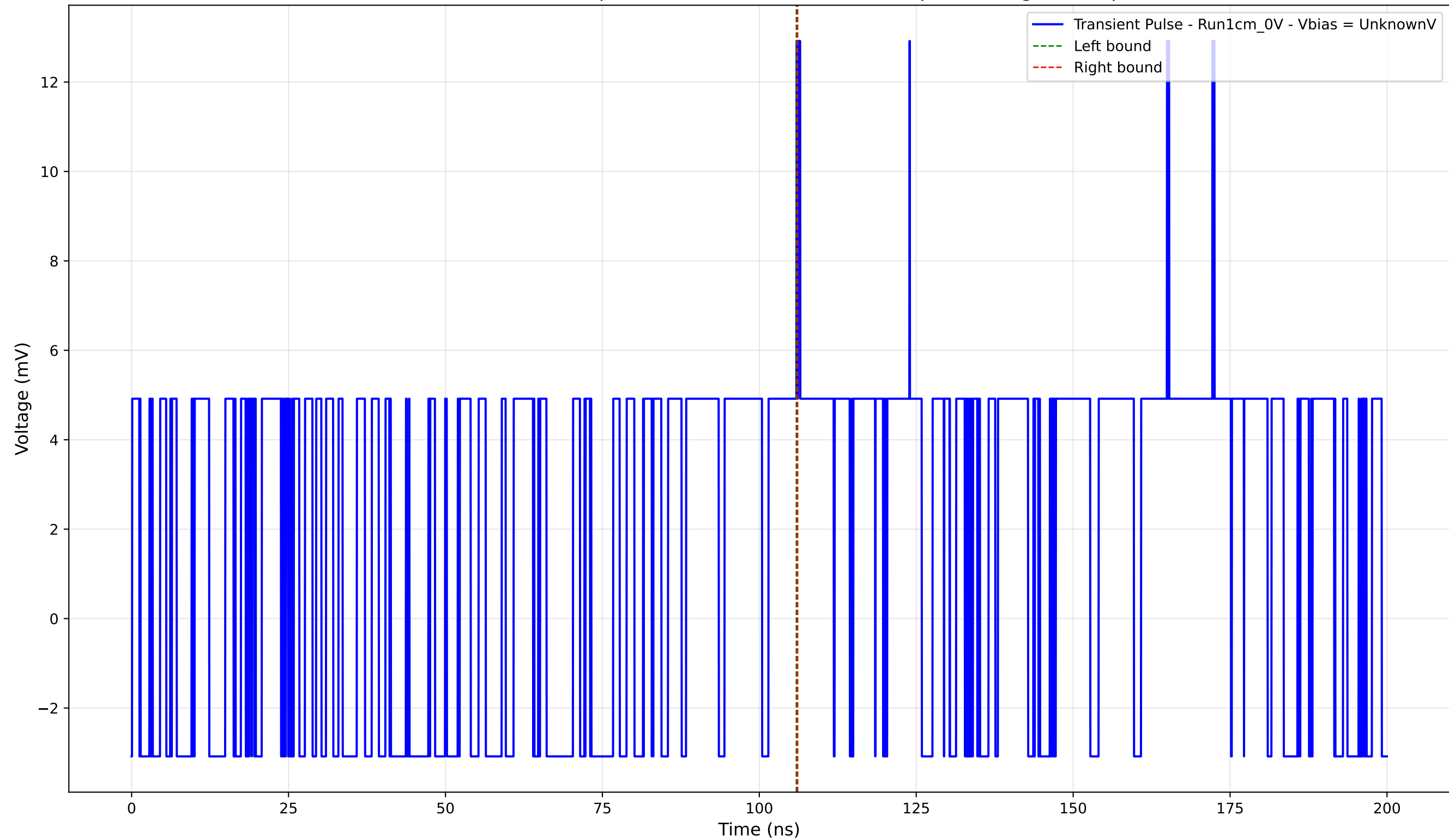
Transient Pulse - Sample: new1cm - Position: 4460.0 \mu\text{m} - Charge: 0.05 pC
