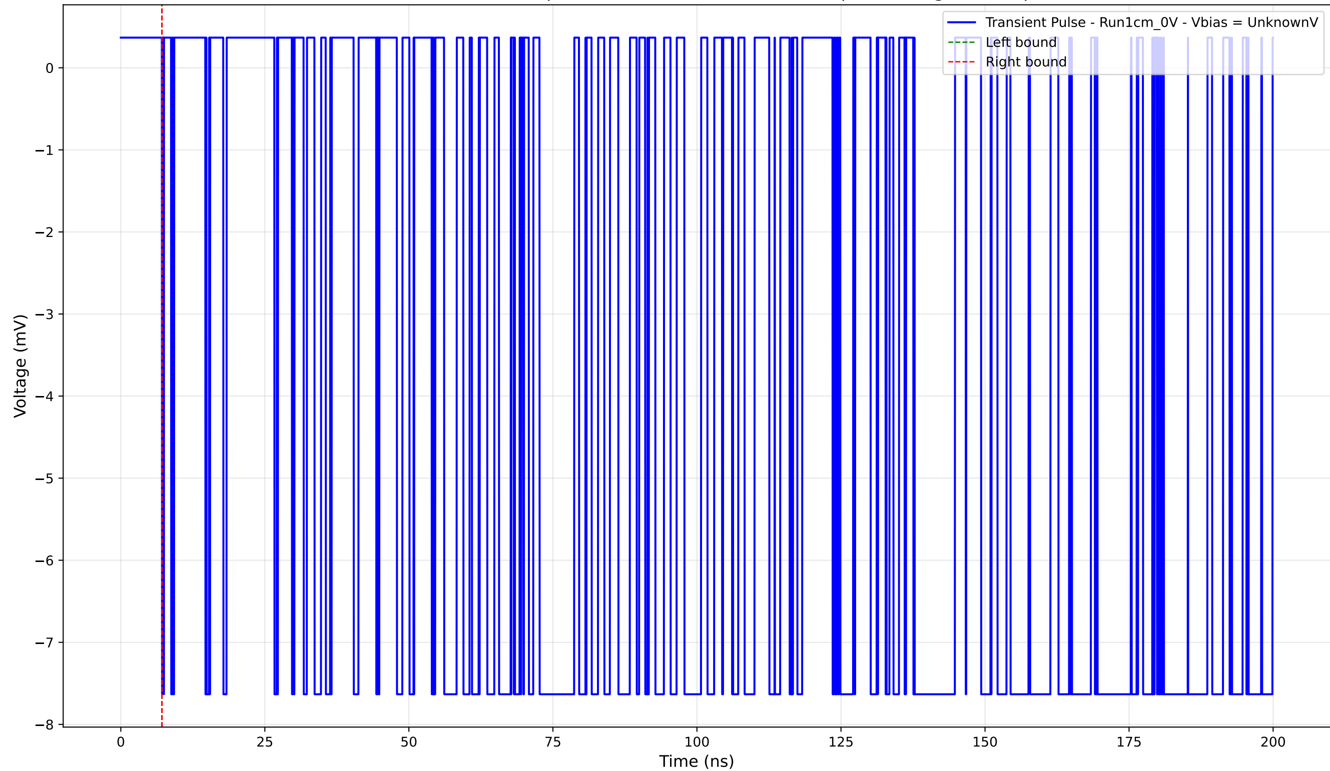
Transient Pulse - Sample: new1cm - Position: 3700.0 \mu\text{m} - Charge: -0.00 pC
