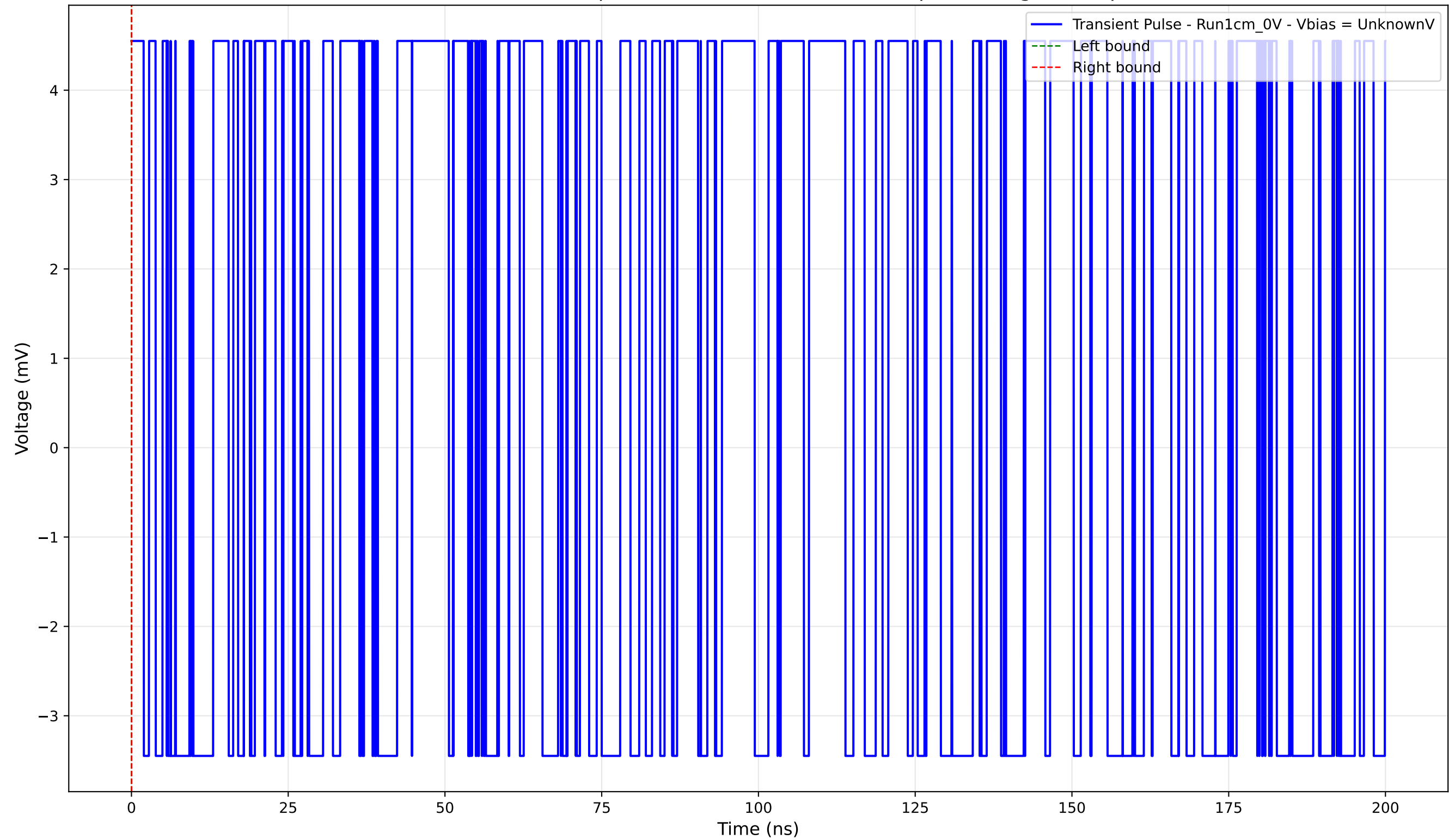
Transient Pulse - Sample: new1cm - Position: 3060.0 \mu\text{m} - Charge: 0.00 pC
