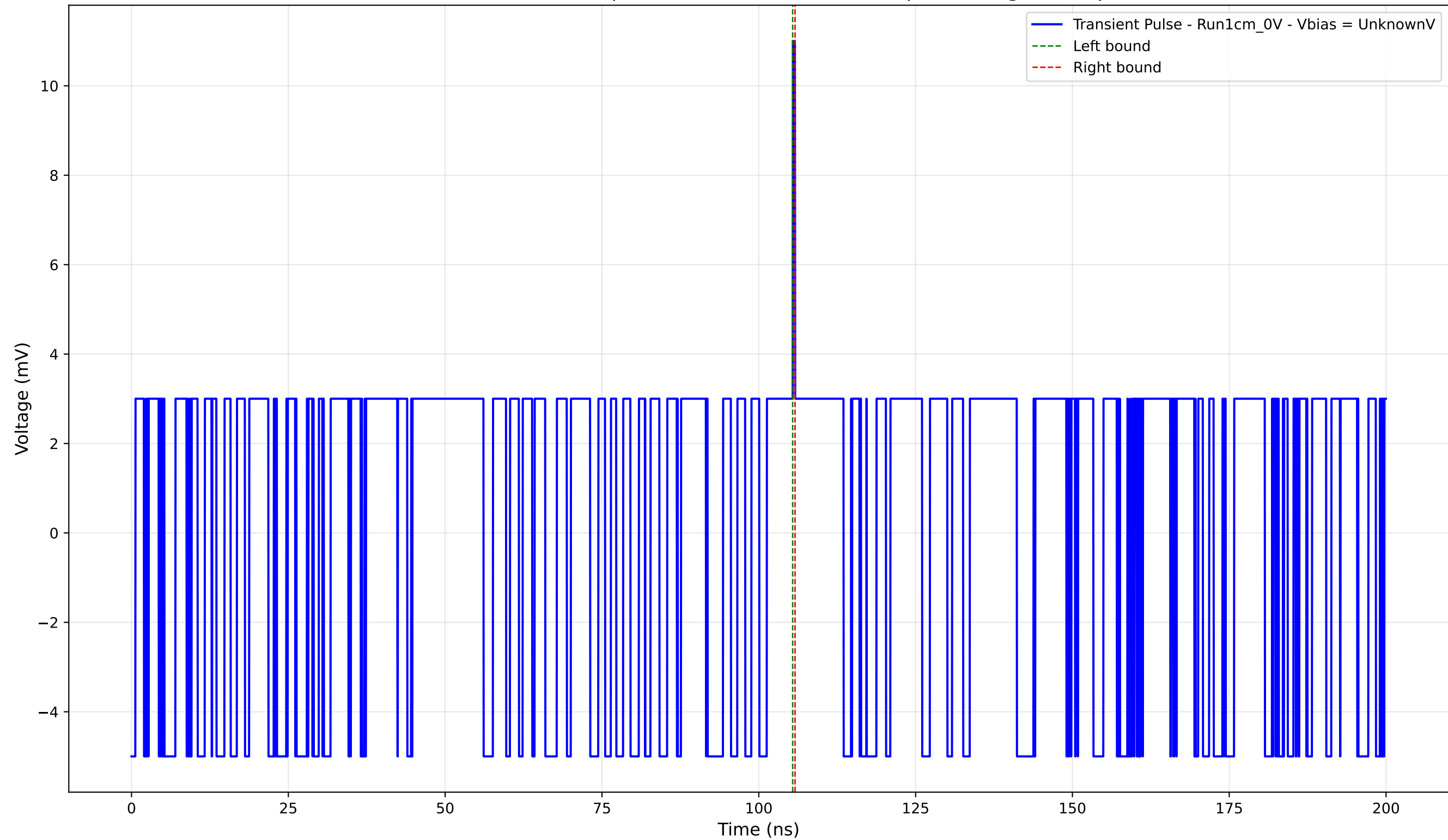
Transient Pulse - Sample: new1cm - Position: 70.0 \mu\text{m} - Charge: 0.08 pC
