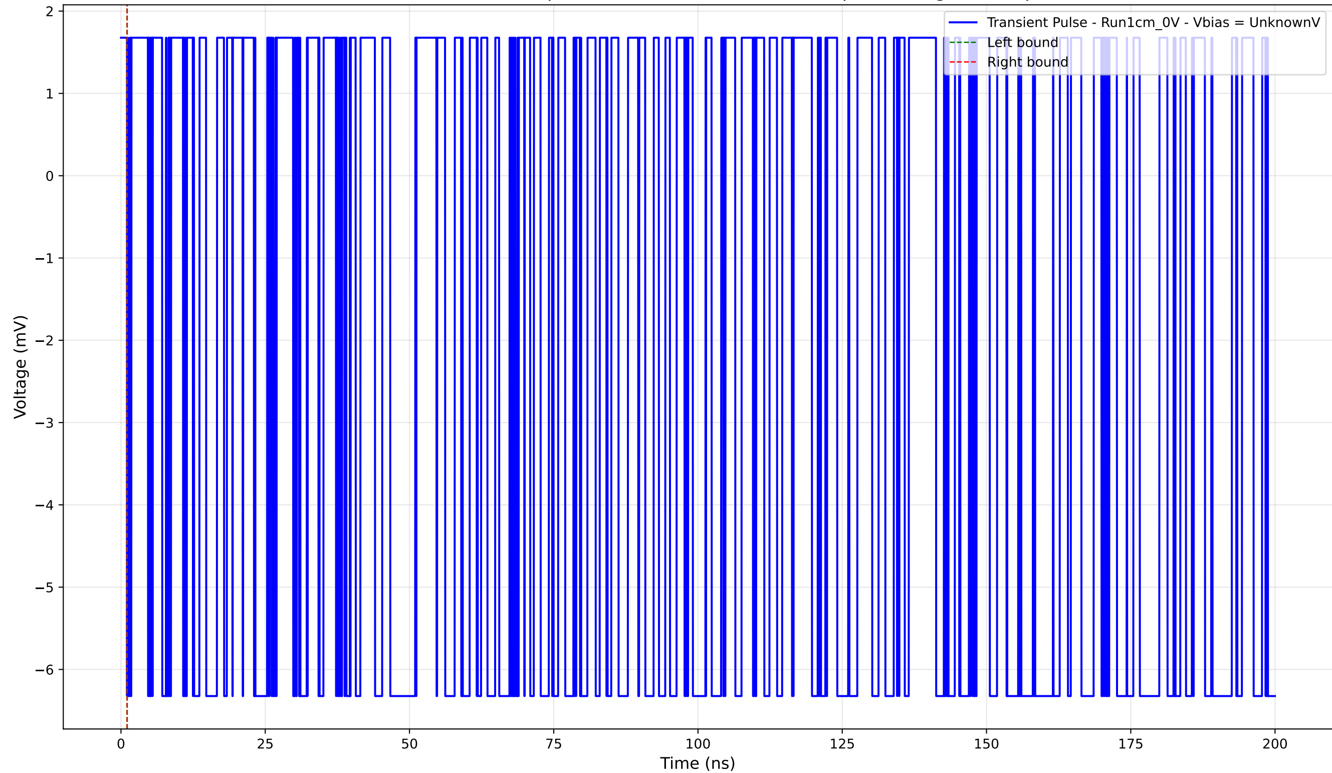
Transient Pulse - Sample: new1cm - Position: 4215.0 \mu\text{m} - Charge: -0.00 pC
