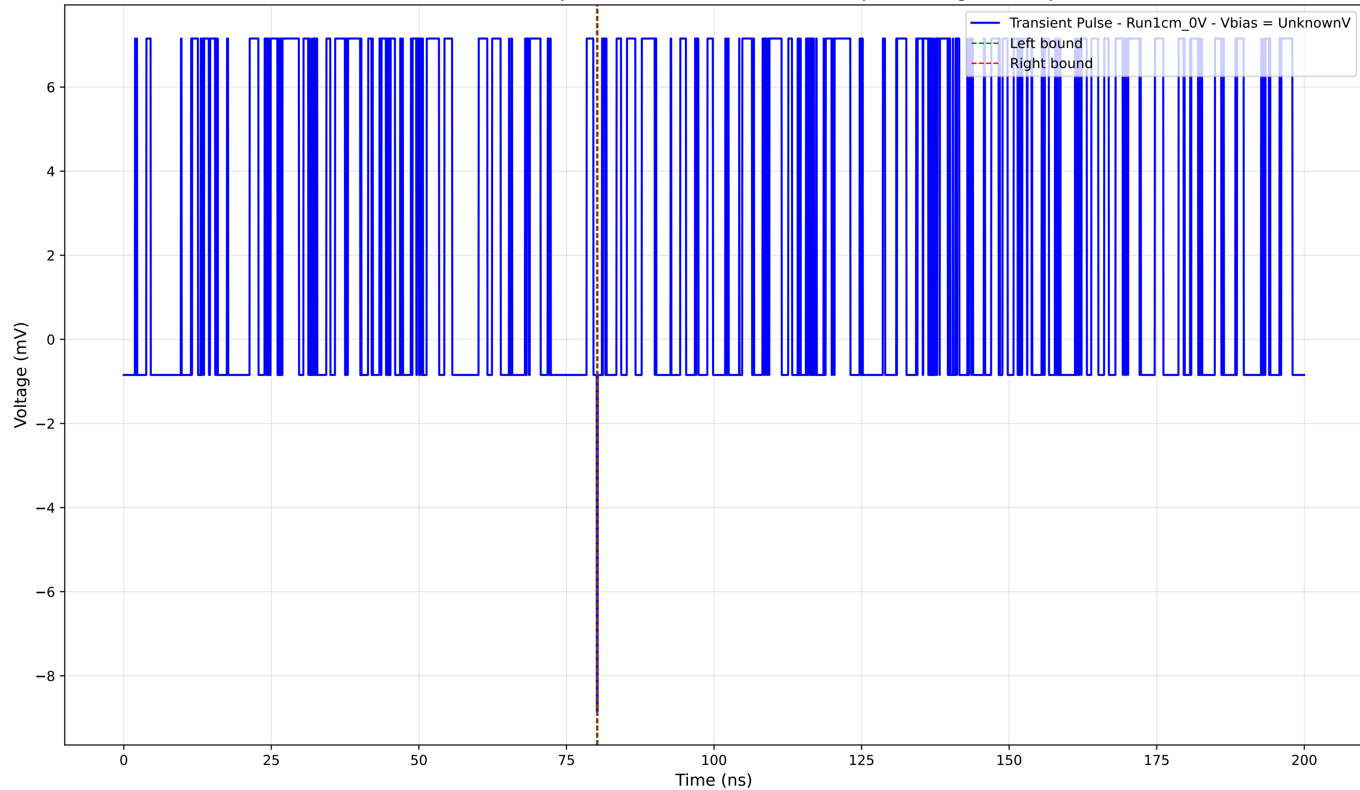
Transient Pulse - Sample: new1cm - Position: 3010.0 \mu\text{m} - Charge: -0.03 pC
