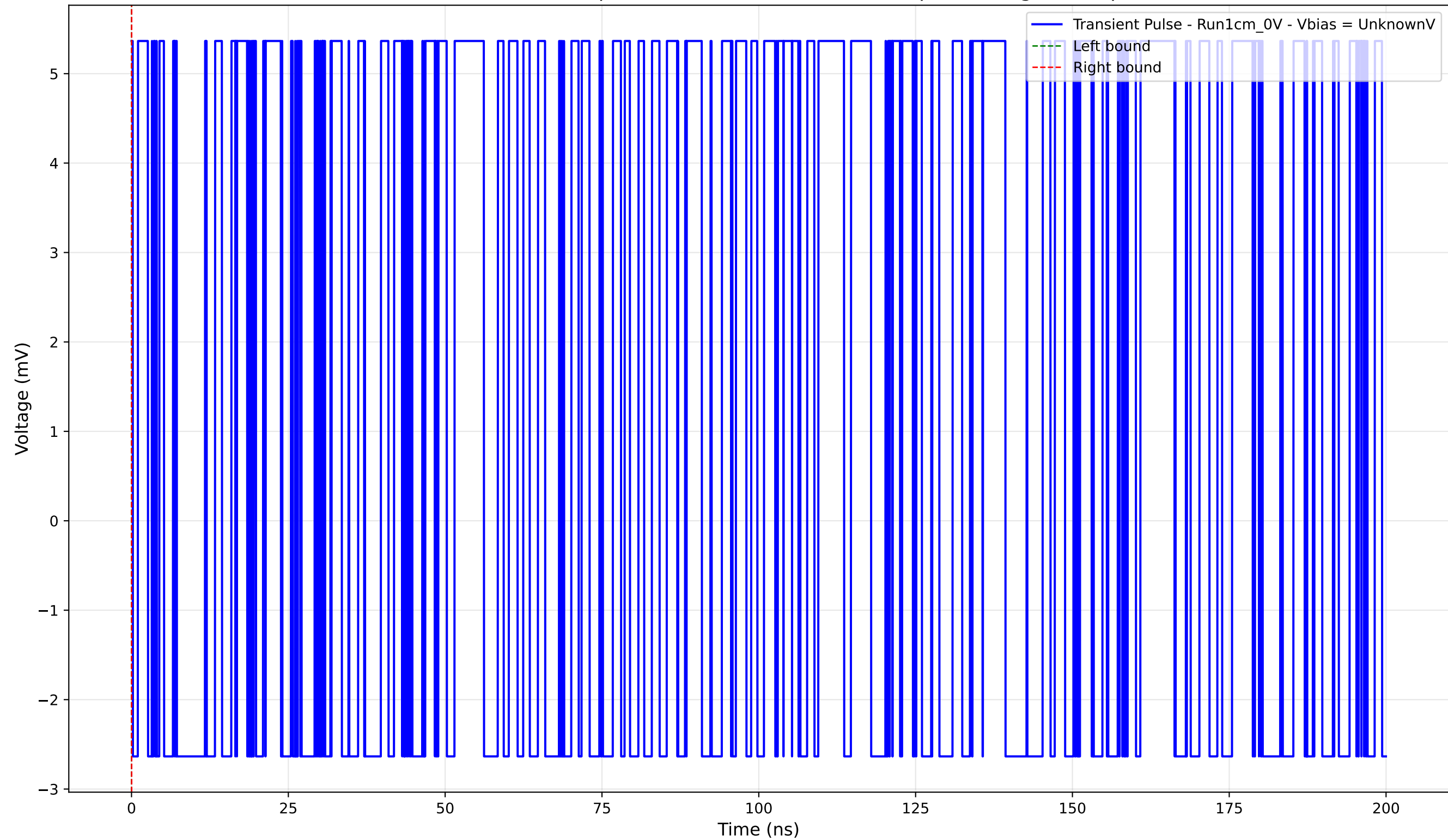
Transient Pulse - Sample: new1cm -Position: 2970.0 \mu\text{m} - Charge: 0.00 pC
