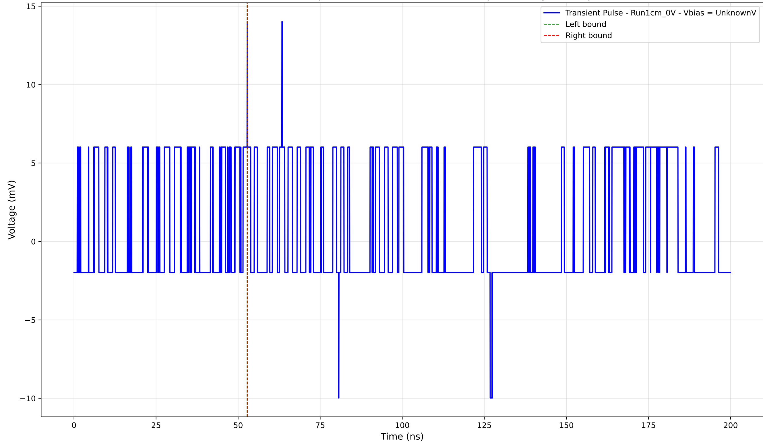
Transient Pulse - Sample: new1cm - Position: 5090.0 \mu\text{m} - Charge: 0.04 pC
