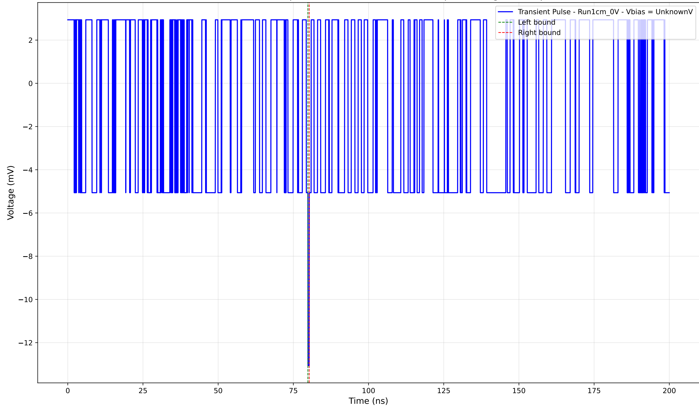
Transient Pulse - Sample: new1cm - Position: 1105.0 \mu\text{m} - Charge: -0.11 pC
