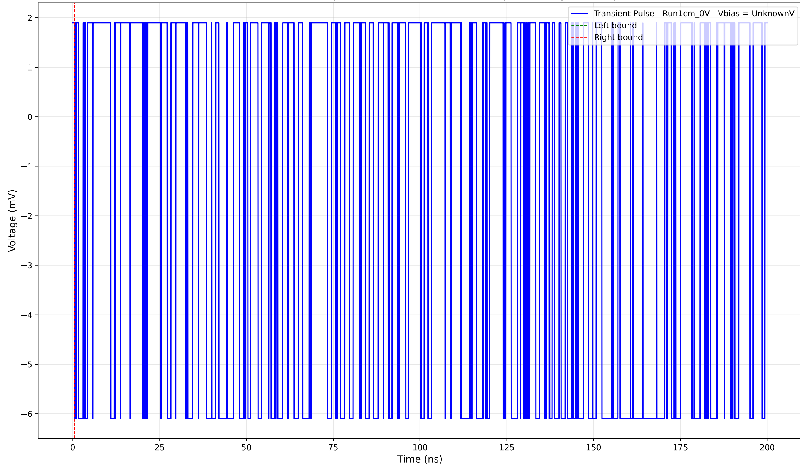
Transient Pulse - Sample: new1cm - Position: 755.0 \mu\text{m} - Charge: -0.00 pC
