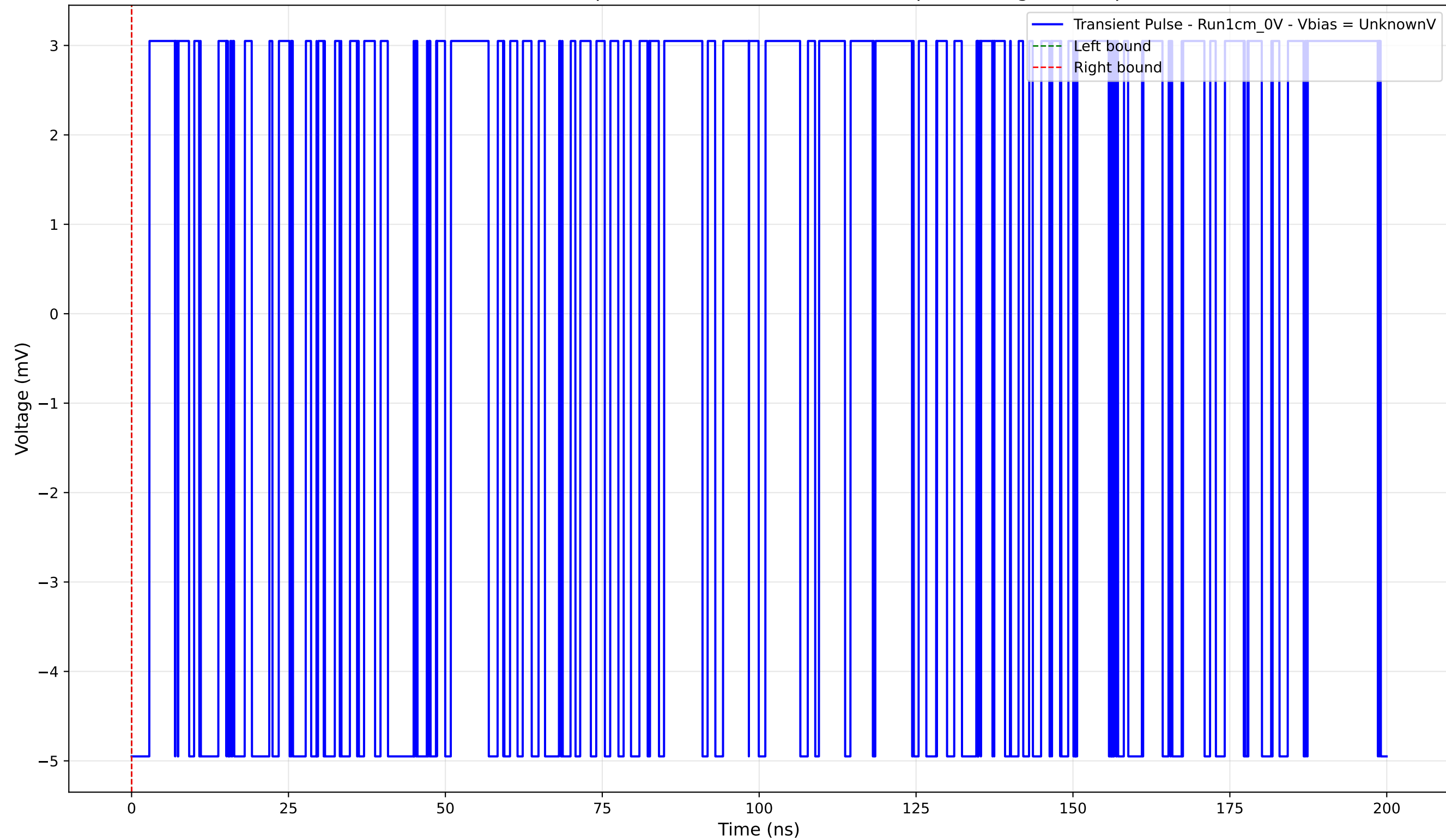
Transient Pulse - Sample: new1cm - Position: 1230.0 \mu\text{m} - Charge: -0.00 pC
