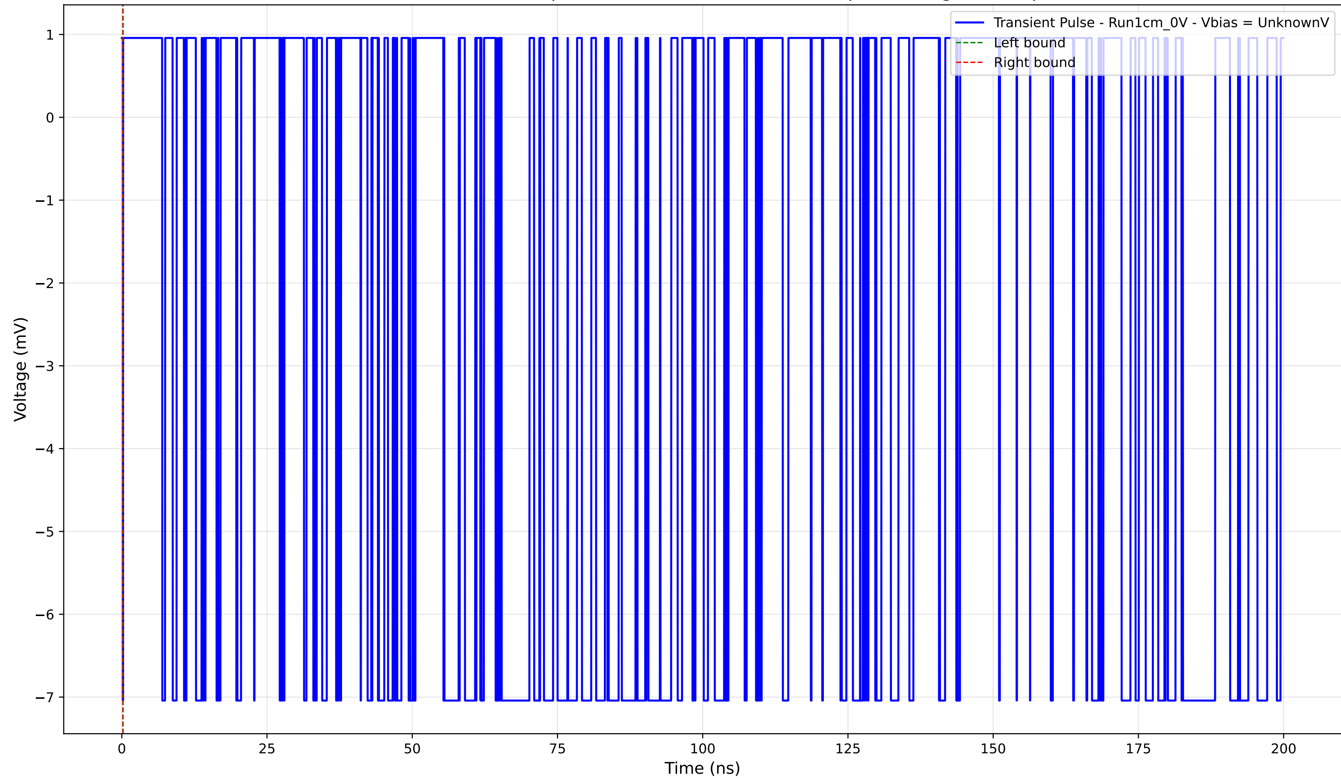
Transient Pulse - Sample: new1cm - Position: 4270.0 \mu\text{m} - Charge: -0.00 pC
