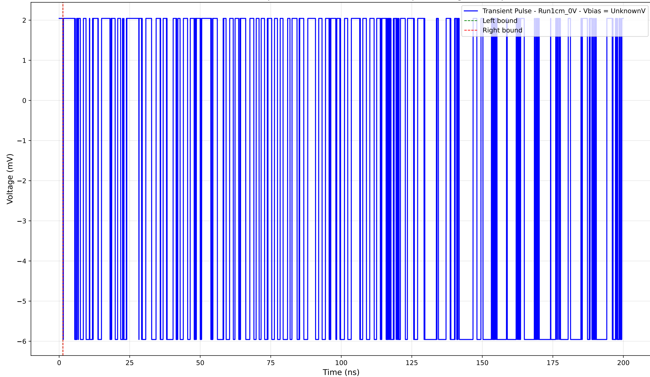
Transient Pulse - Sample: new1cm - Position: 1830.0 \mu\text{m} - Charge: -0.00 pC
