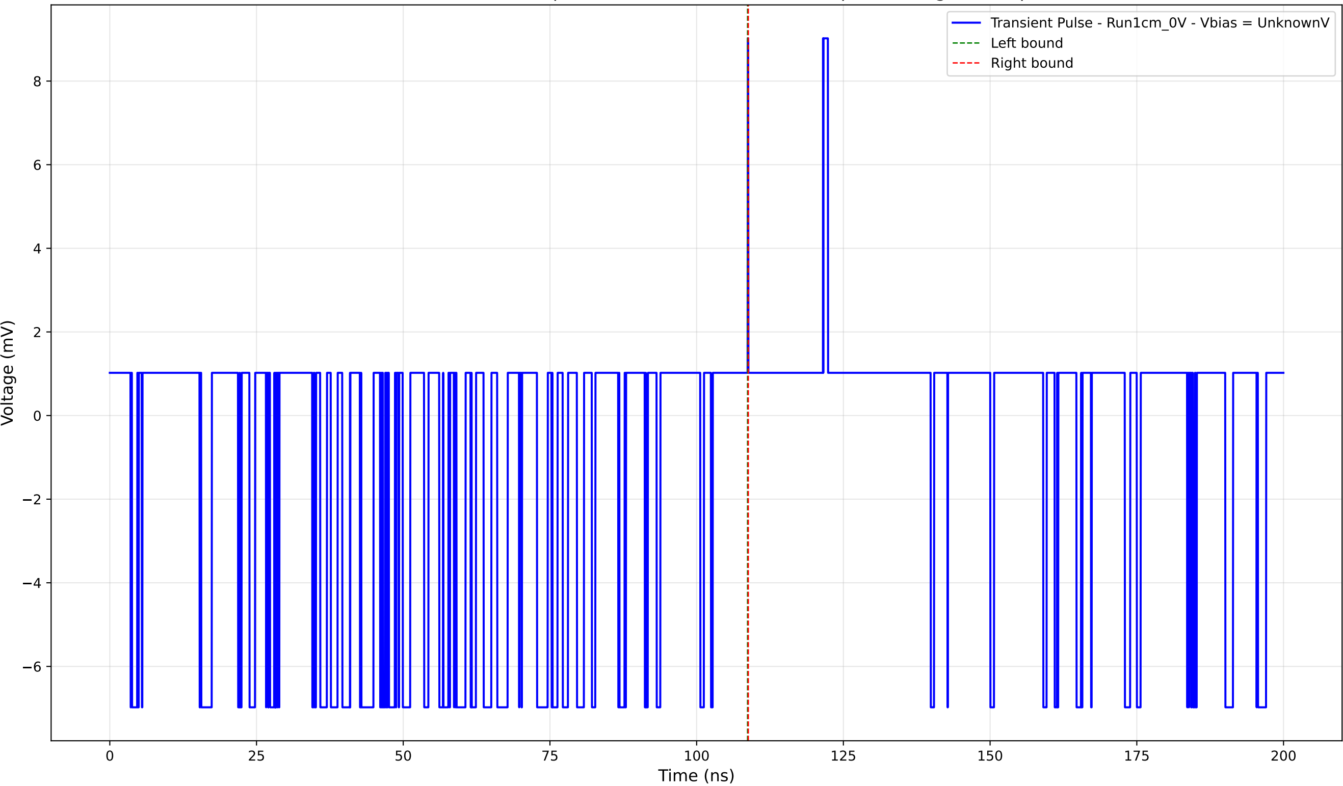
Transient Pulse - Sample: new1cm - Position: 820.0 \mu\text{m} - Charge: 0.02 pC
