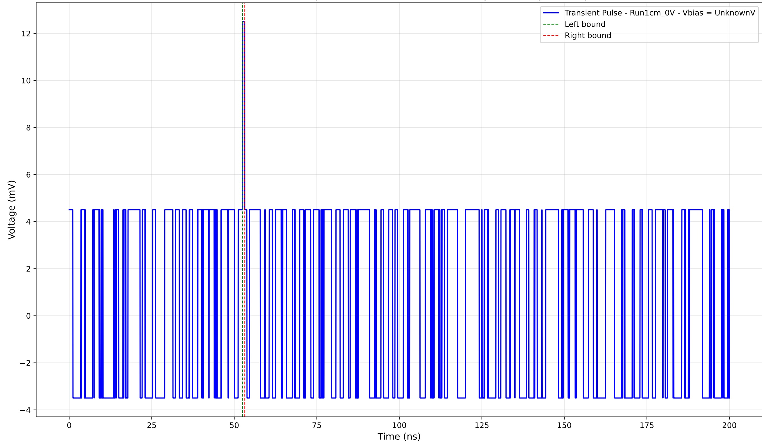
Transient Pulse - Sample: new1cm - Position: 1295.0 \mu\text{m} - Charge: 0.16 pC
