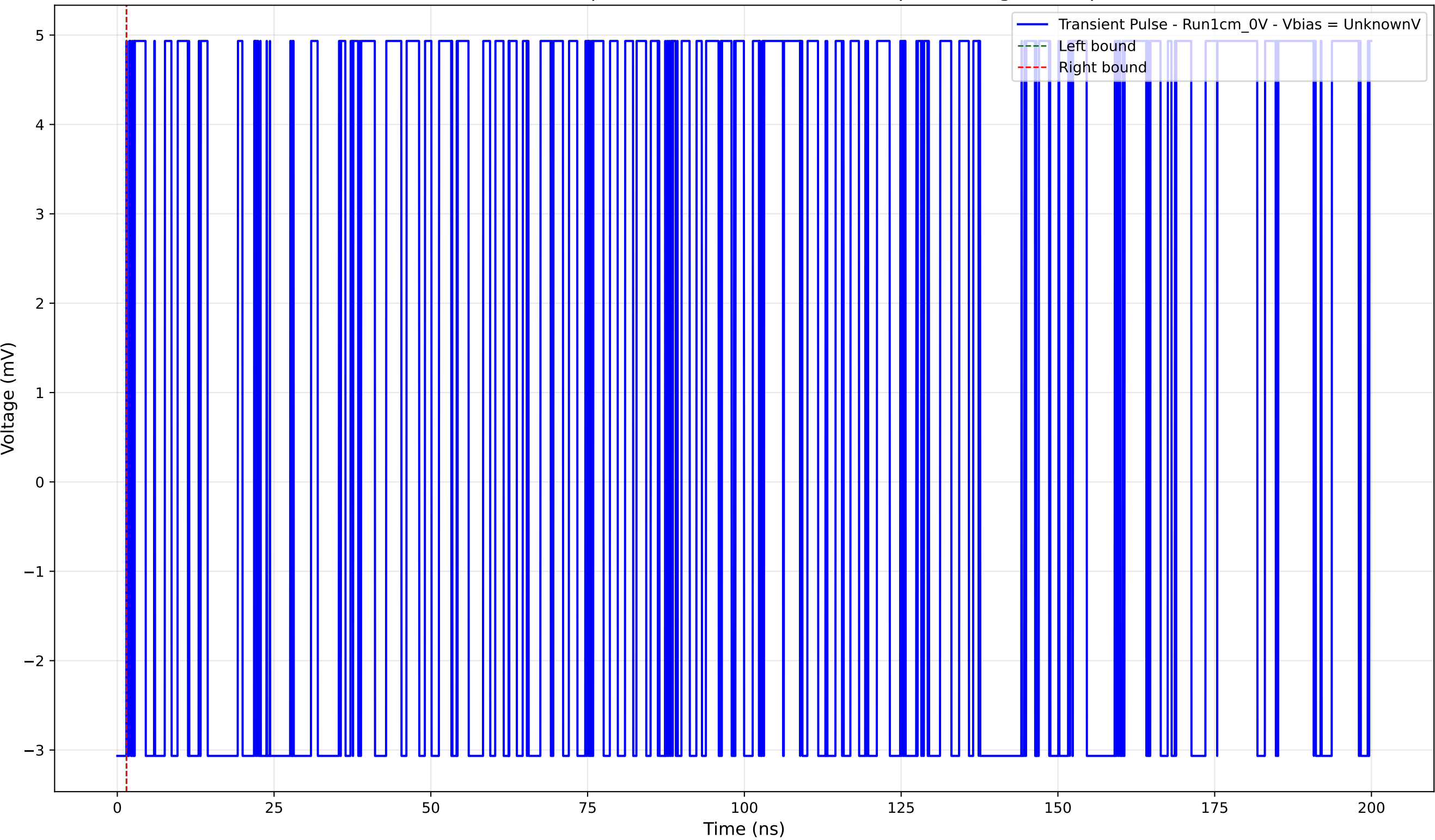
Transient Pulse - Sample: new1cm - Position: 650.0 \mu\text{m} - Charge: 0.00 pC
