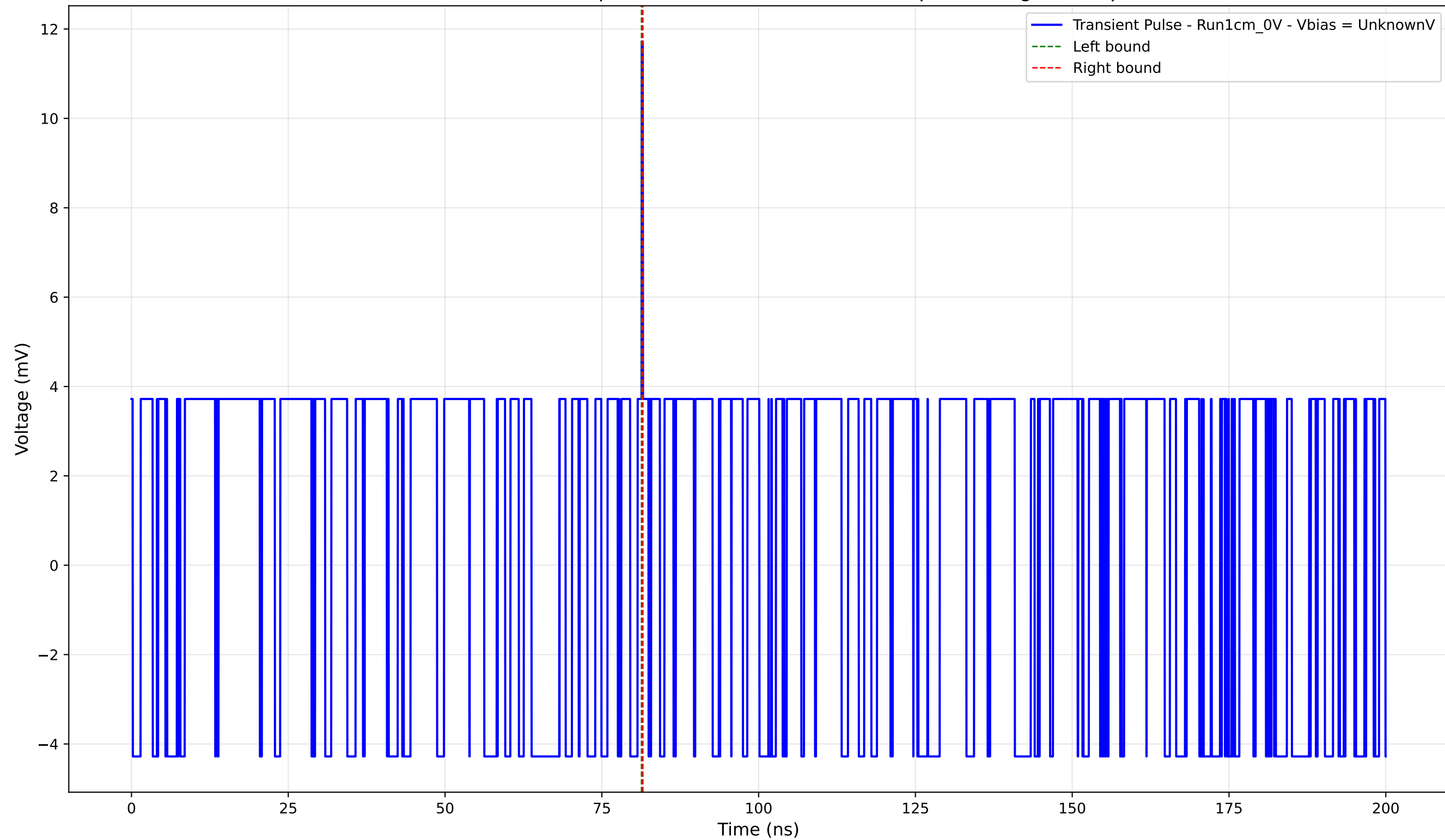
Transient Pulse - Sample: new1cm - Position: 2430.0 \mu\text{m} - Charge: 0.05 pC
