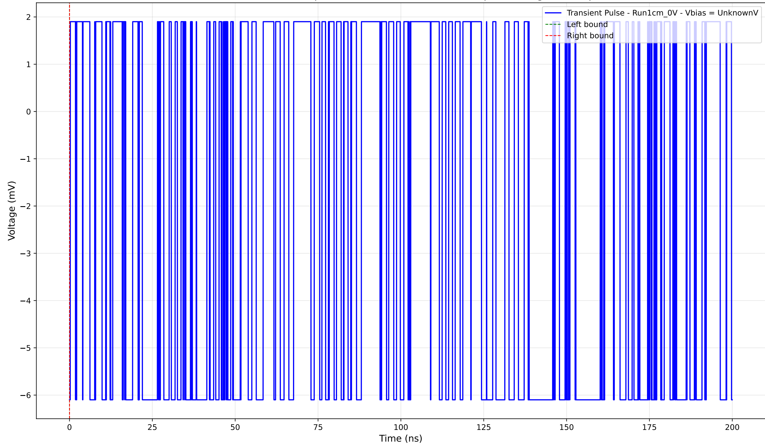
Transient Pulse - Sample: new1cm - Position: 1625.0 \mu\text{m} - Charge: -0.00 pC
