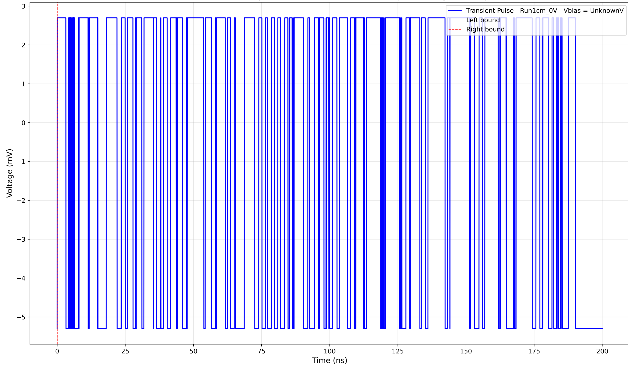
Transient Pulse - Sample: new1cm - Position: 3375.0 \mu\text{m} - Charge: -0.00 pC
