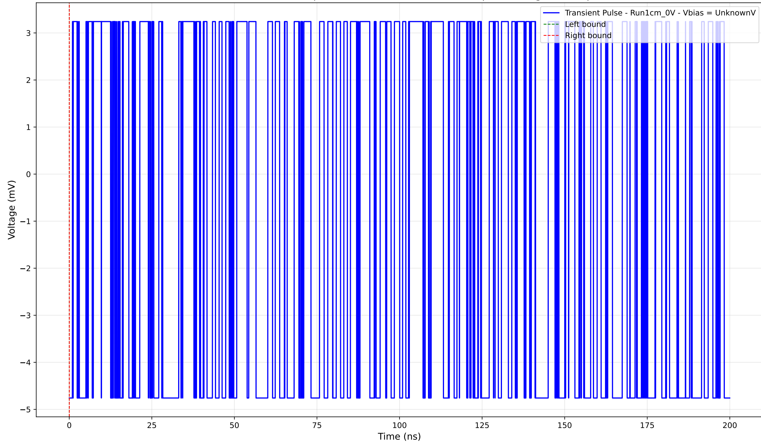
Transient Pulse - Sample: new1cm - Position: 1195.0 \mu\text{m} - Charge: -0.00 pC
