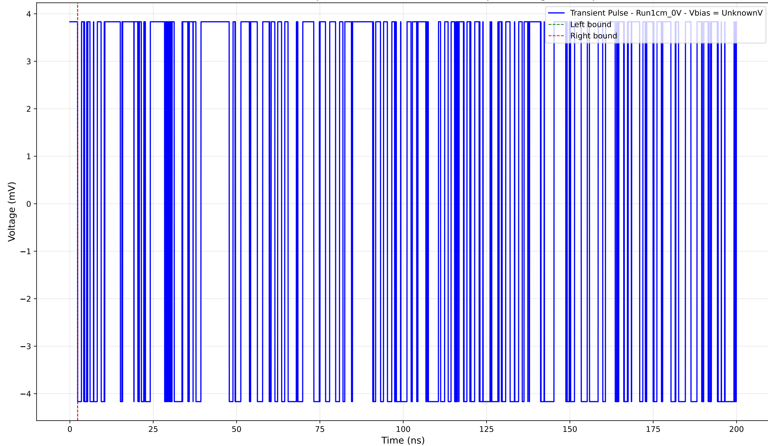
Transient Pulse - Sample: new1cm - Position: 1055.0 \mu\text{m} - Charge: -0.00 pC
