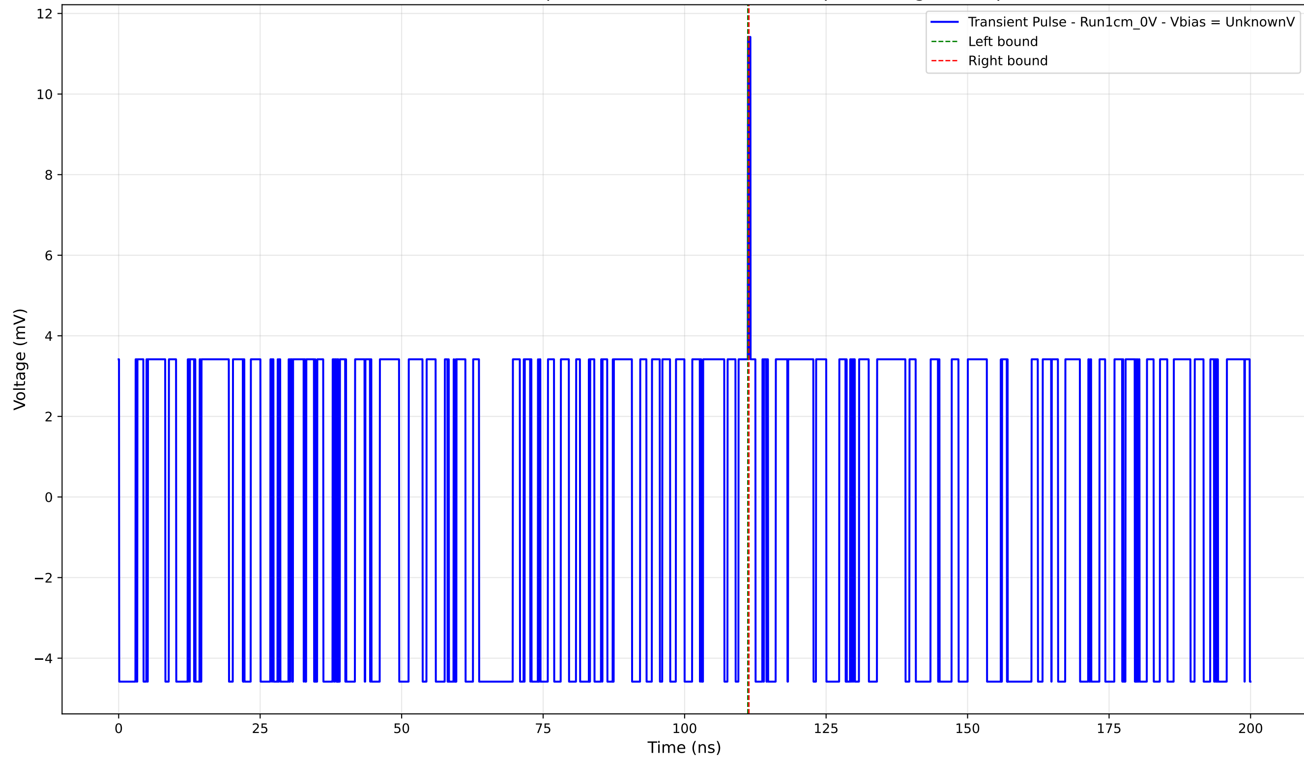
Transient Pulse - Sample: new1cm - Position: 655.0 \mu\text{m} - Charge: 0.04 pC
