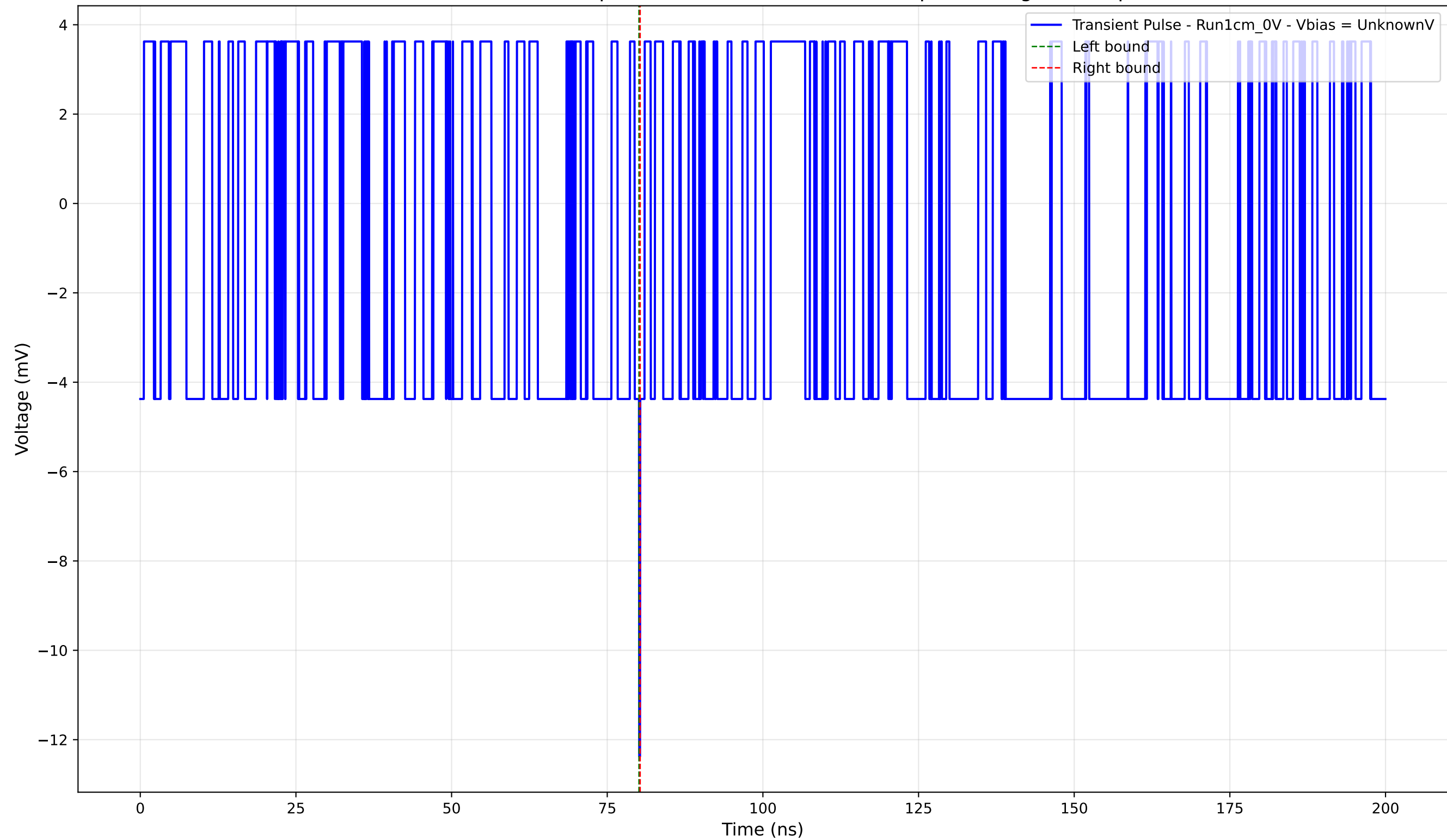
Transient Pulse - Sample: new1cm - Position: 1410.0 \mu\text{m} - Charge: -0.04 pC
