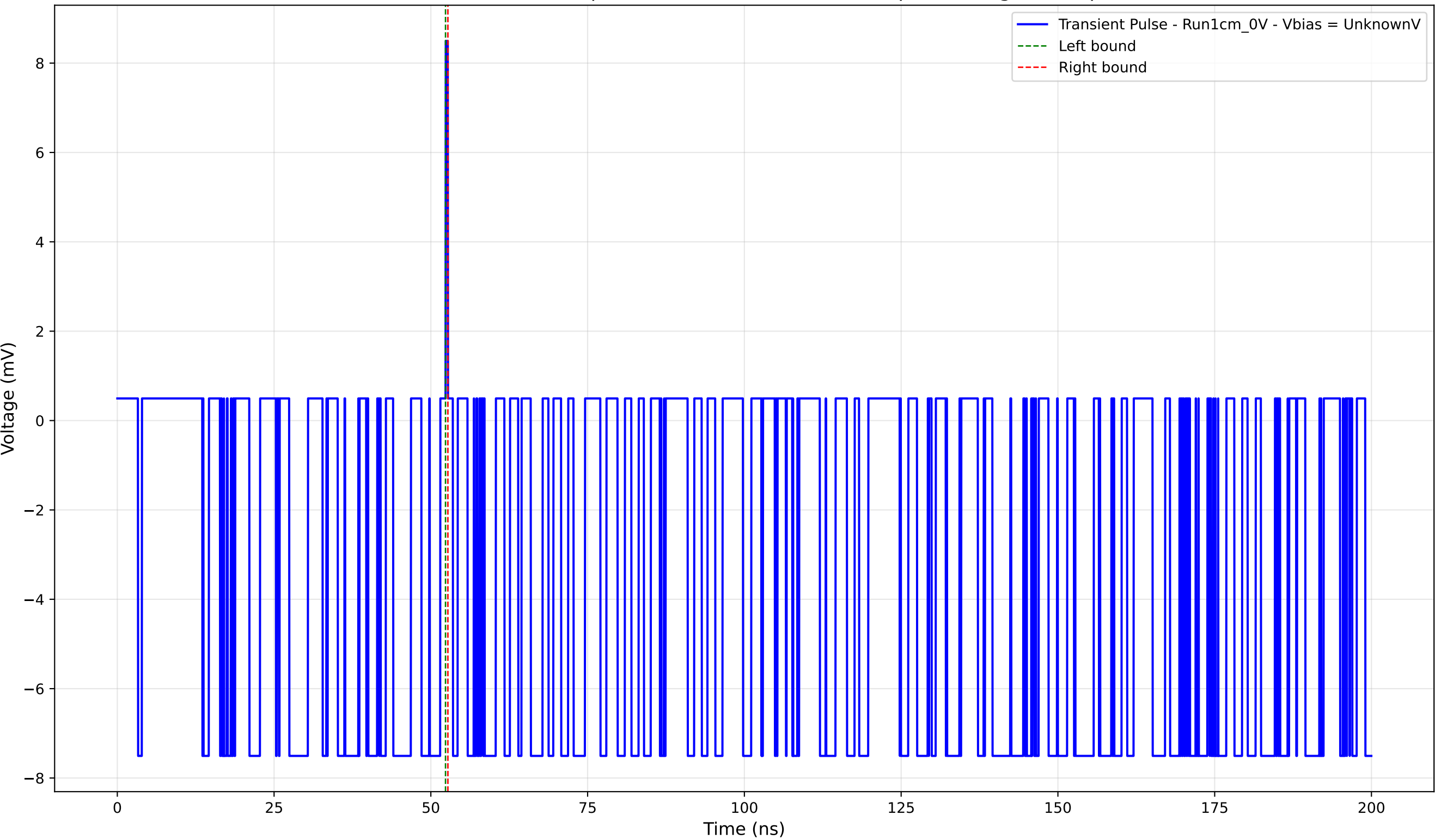
Transient Pulse - Sample: new1cm - Position: 480.0 \mu\text{m} - Charge: 0.06 pC
