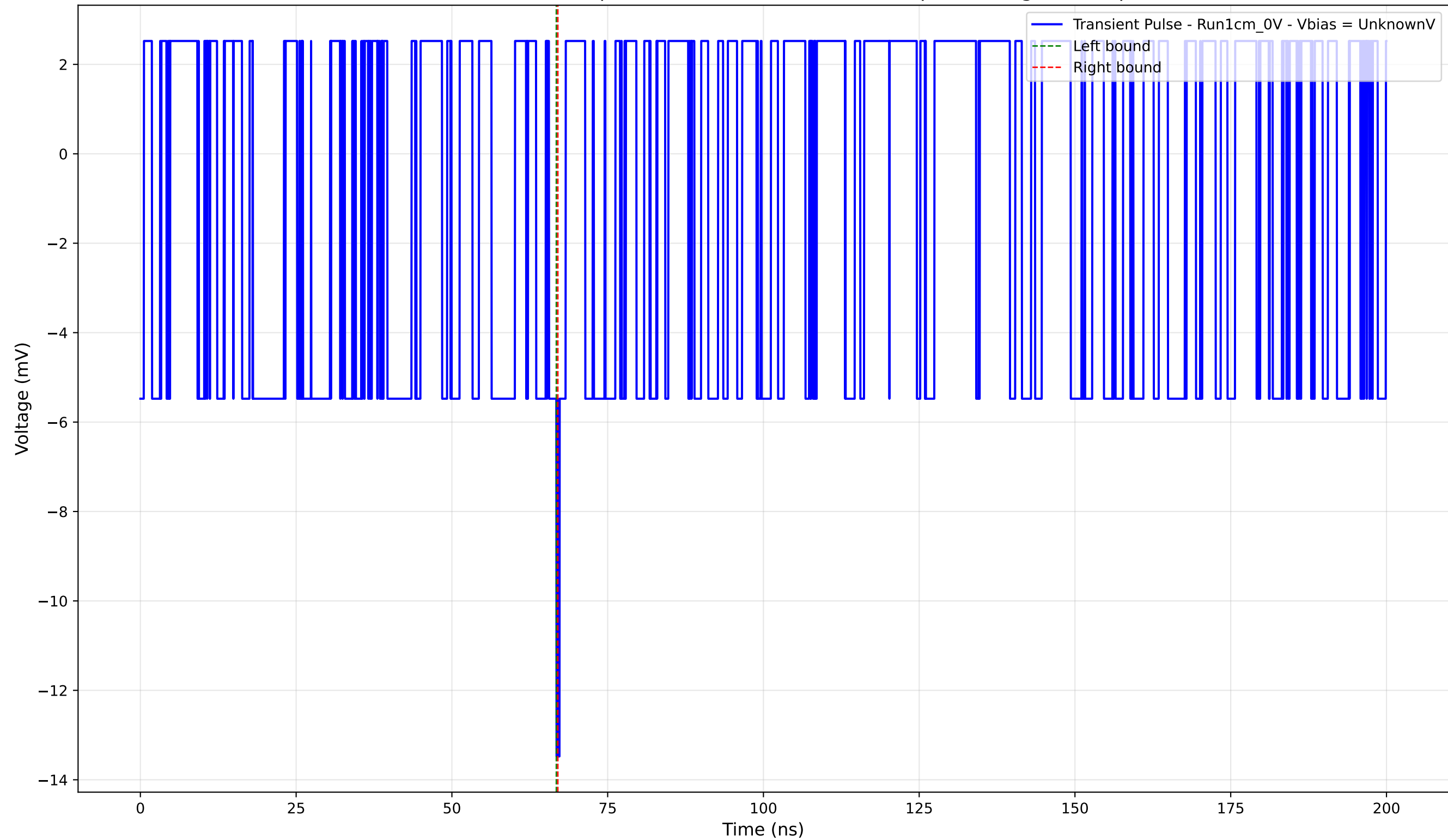
Transient Pulse - Sample: new1cm - Position: 2265.0 \mu\text{m} - Charge: -0.06 pC
