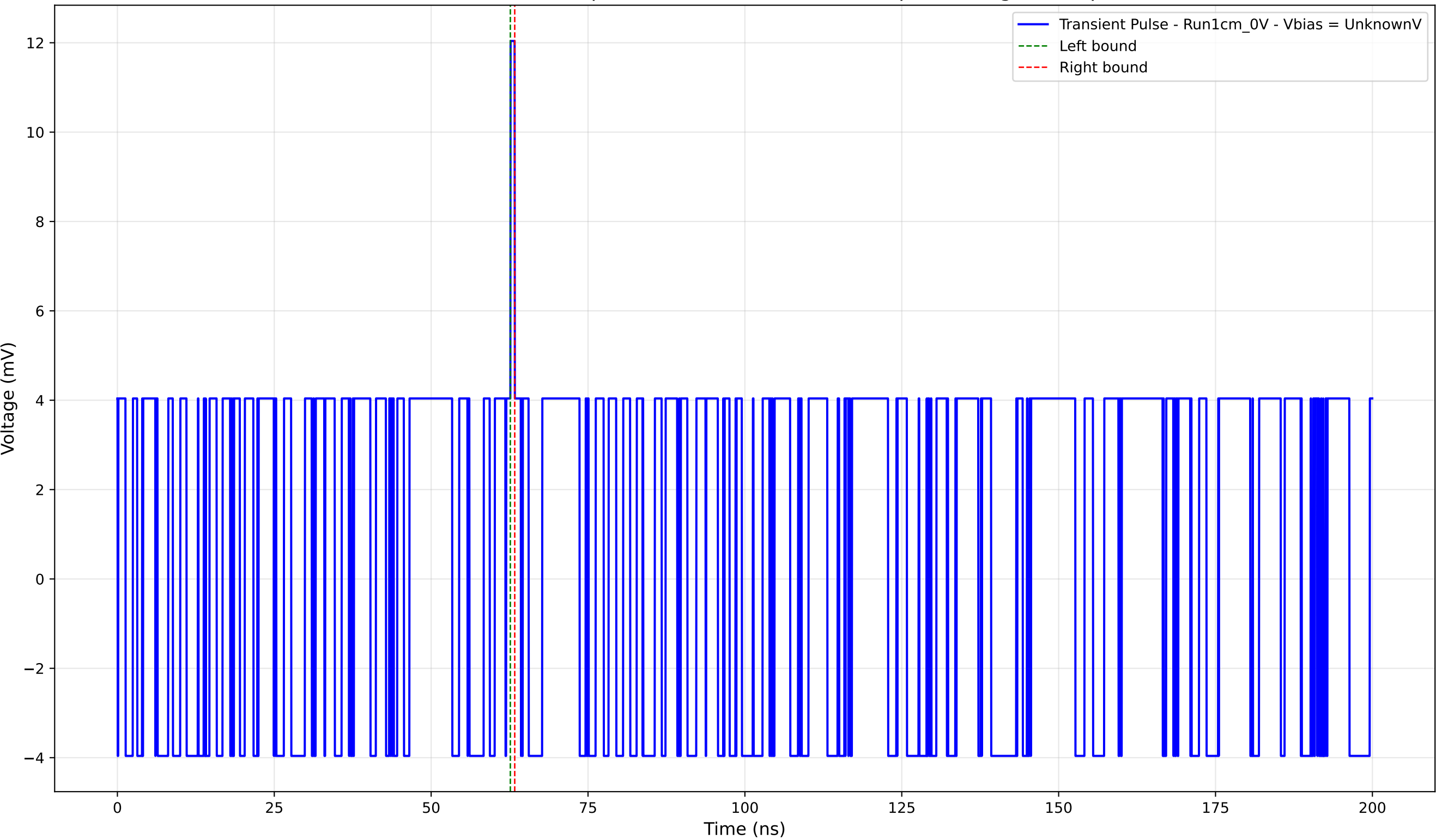
Transient Pulse - Sample: new1cm - Position: 980.0 \mu\text{m} - Charge: 0.17 pC
