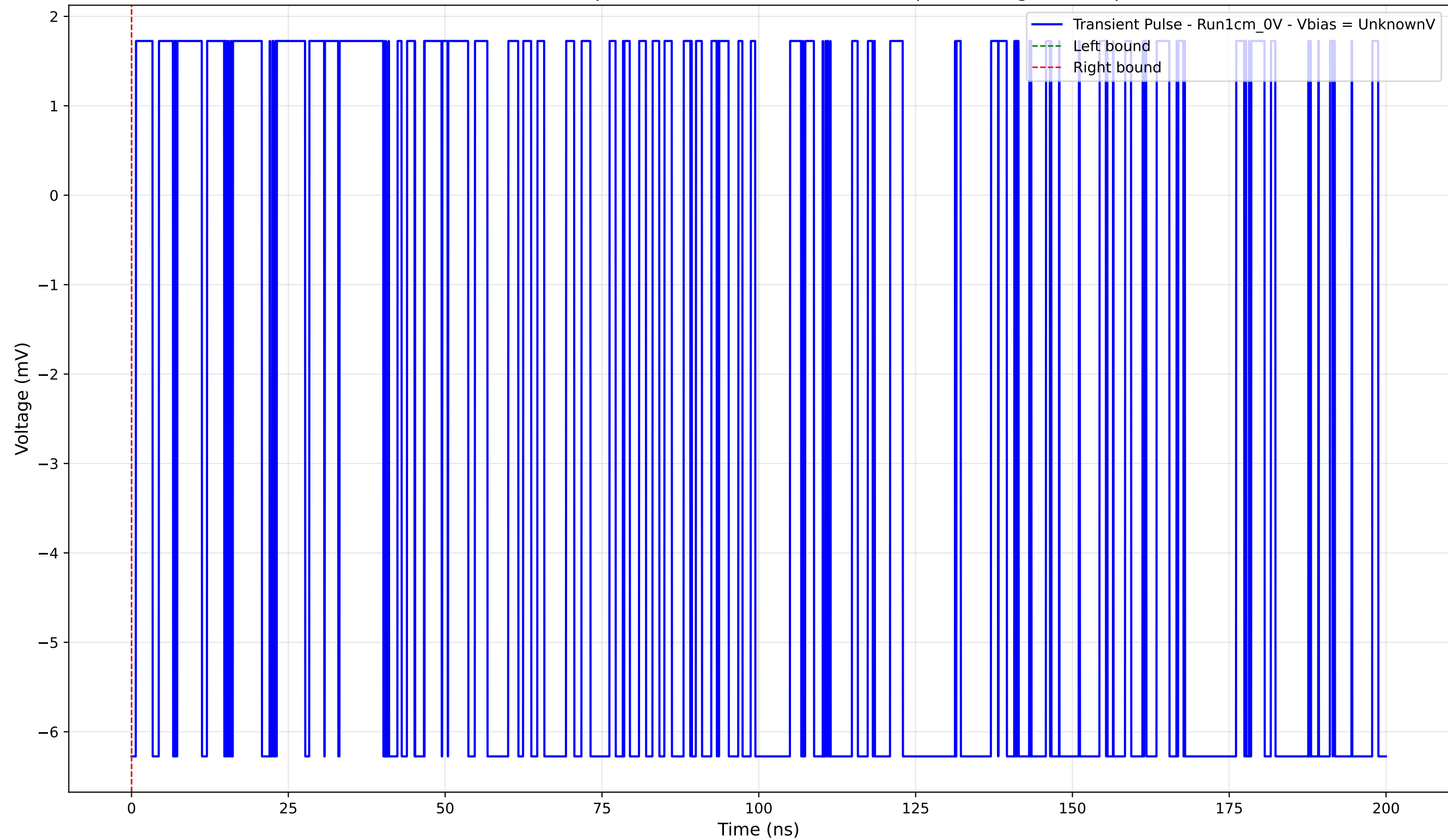
Transient Pulse - Sample: new1cm - Position: 3545.0 \mu\text{m} - Charge: -0.00 pC
