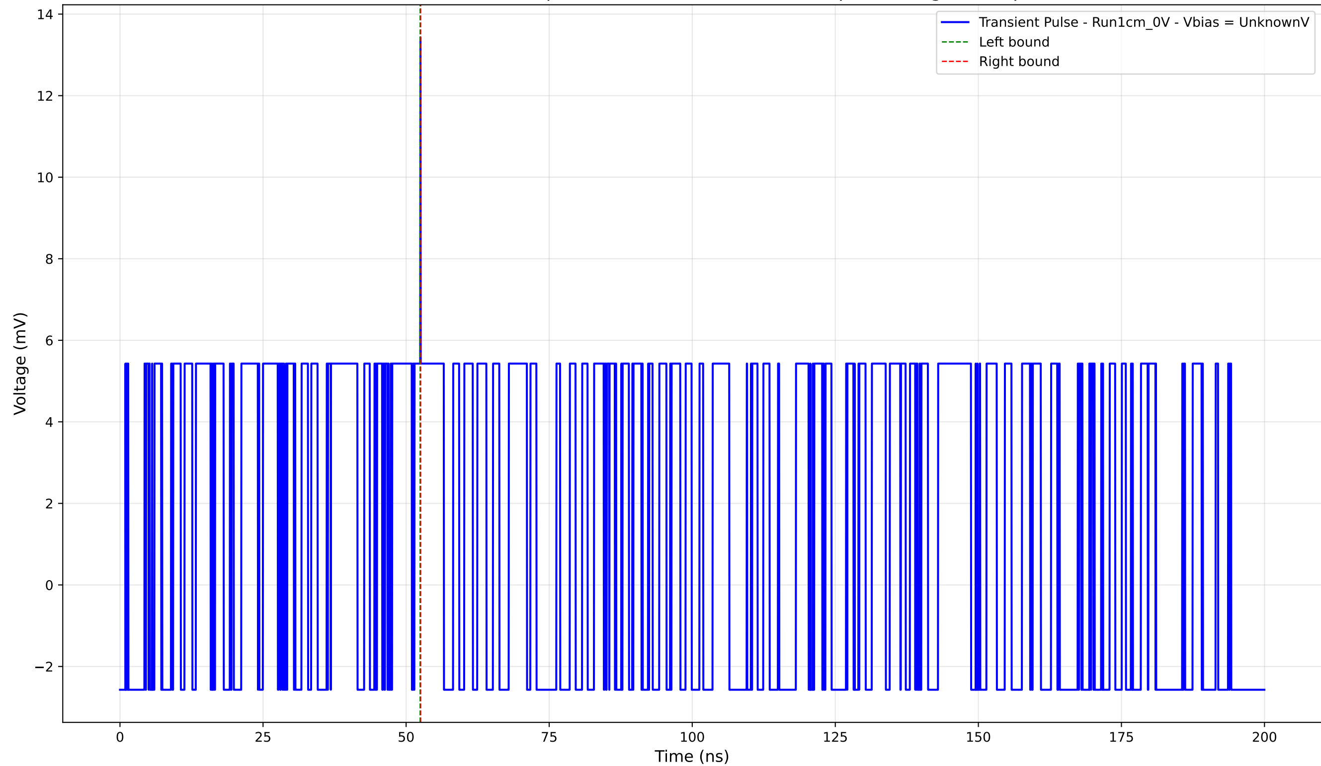
Transient Pulse - Sample: new1cm - Position: 1770.0 \mu\text{m} - Charge: 0.02 pC
