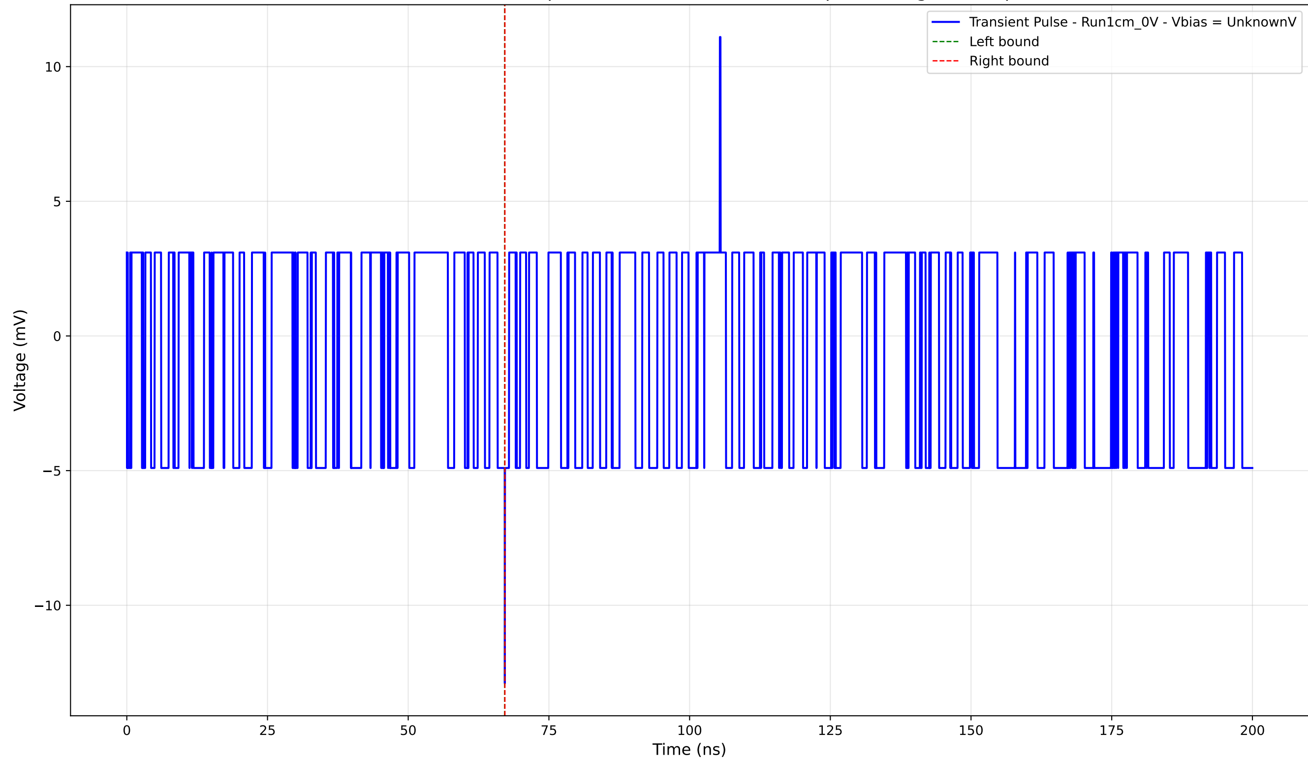
Transient Pulse - Sample: new1cm - Position: 865.0 \mu\text{m} - Charge: -0.01 pC
