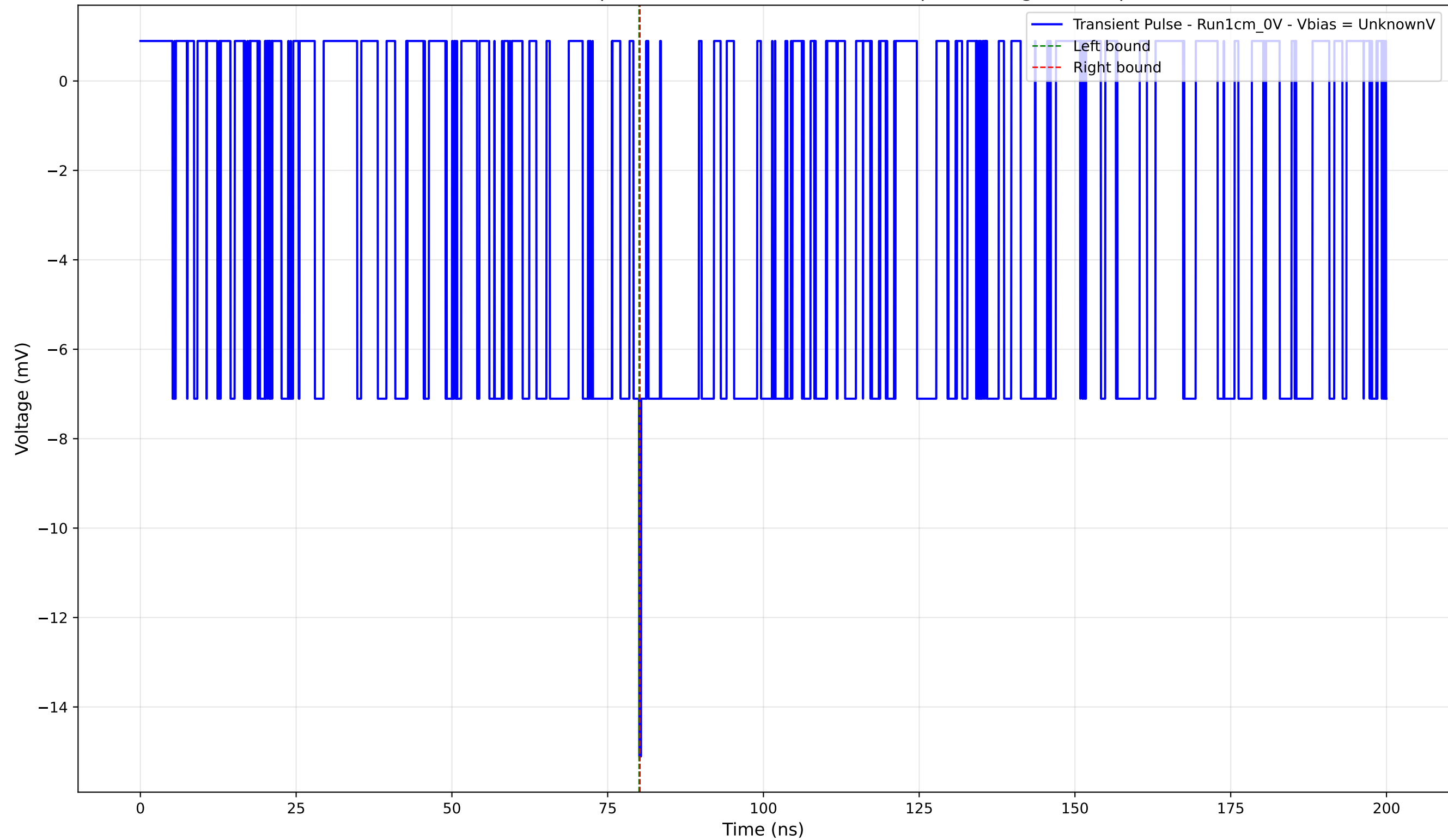
Transient Pulse - Sample: new1cm - Position: 3575.0 \mu\text{m} - Charge: -0.04 pC
