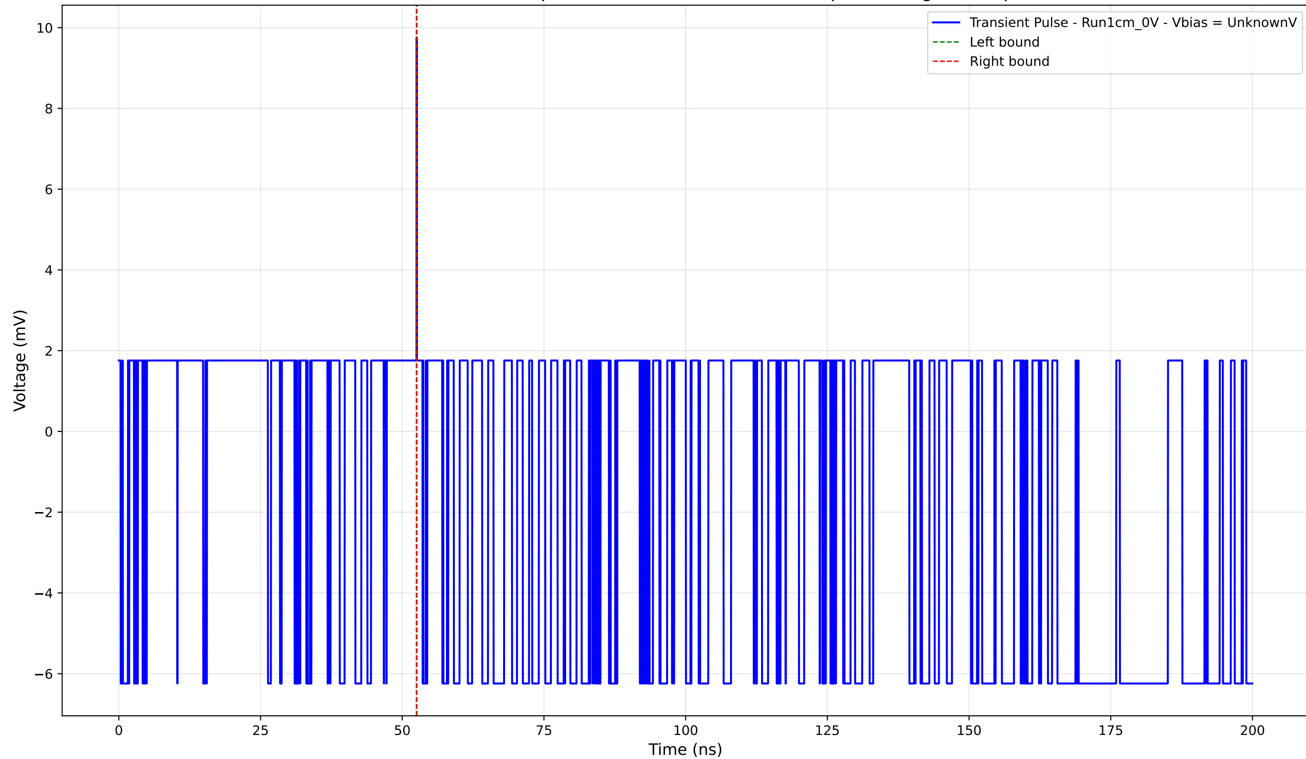
Transient Pulse - Sample: new1cm - Position: 3430.0 \mu\text{m} - Charge: 0.01 pC
