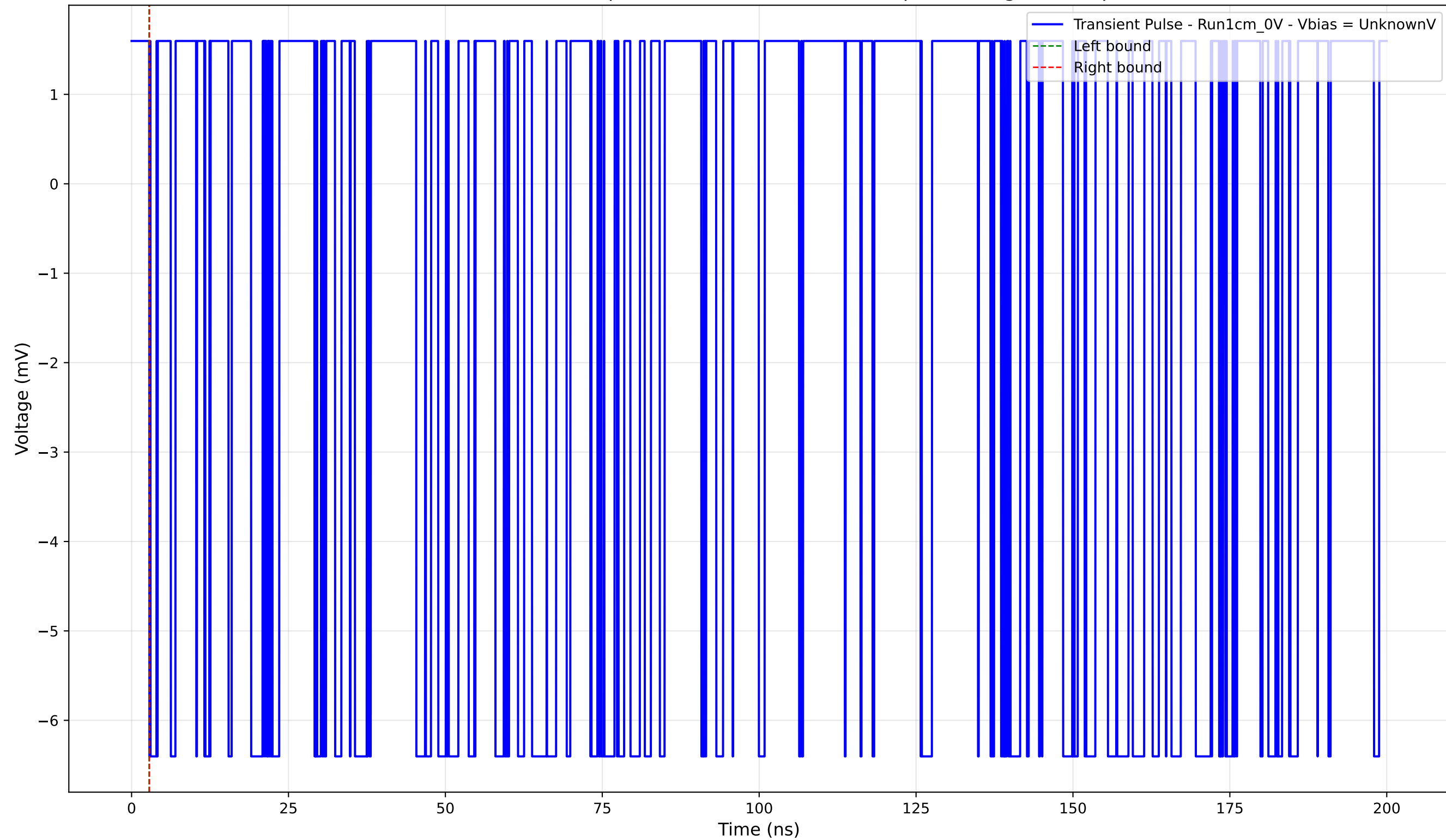
Transient Pulse - Sample: new1cm - Position: 75.0 \mu\text{m} - Charge: -0.00 pC
