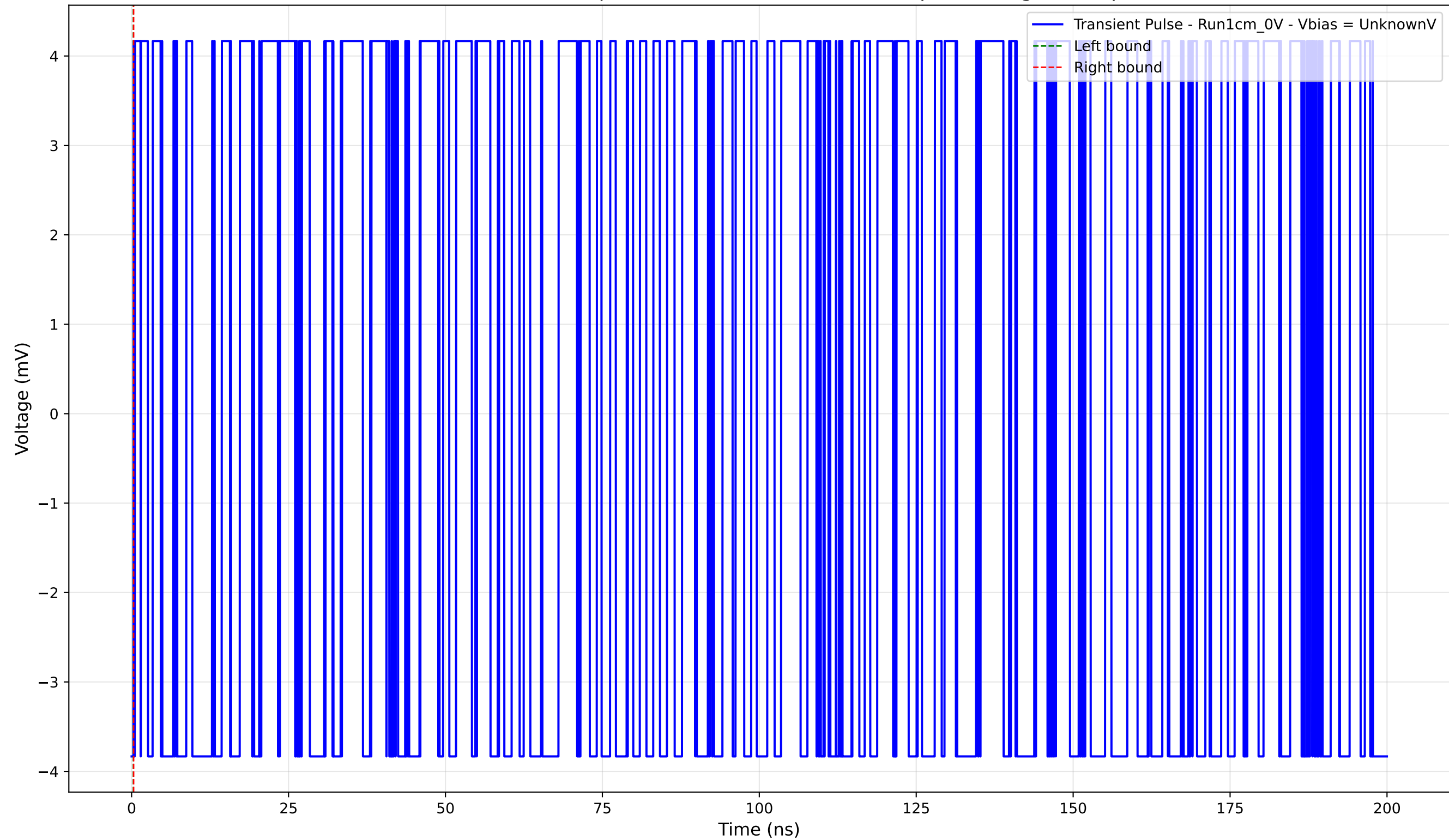
Transient Pulse - Sample: new1cm -Position: 3240.0 \mu\text{m} - Charge: 0.00 pC
