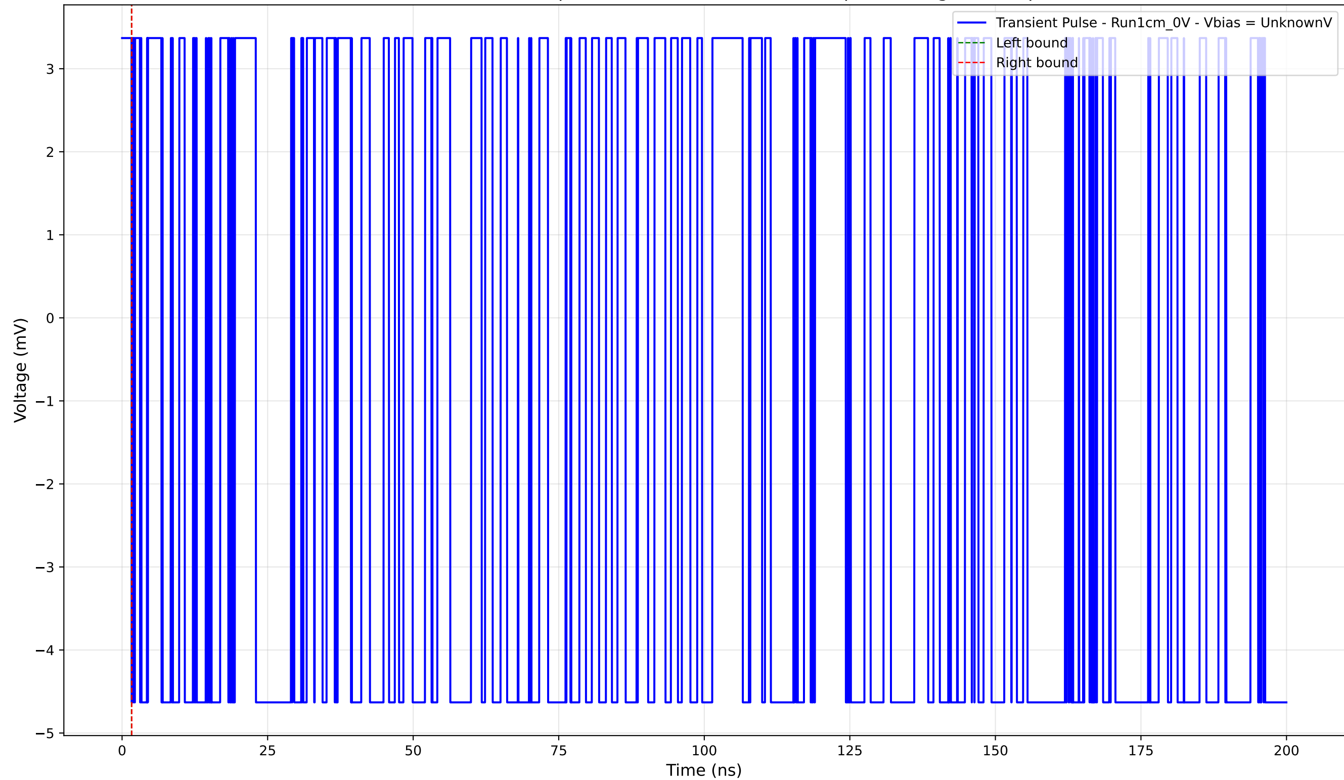
Transient Pulse - Sample: new1cm - Position: 550.0 \mu\text{m} - Charge: -0.00 pC
