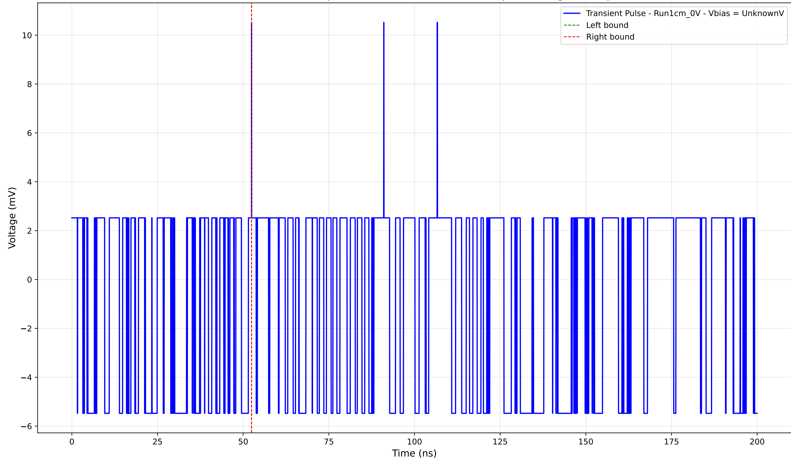
Transient Pulse - Sample: new1cm - Position: 4745.0 \mu\text{m} - Charge: 0.01 pC
