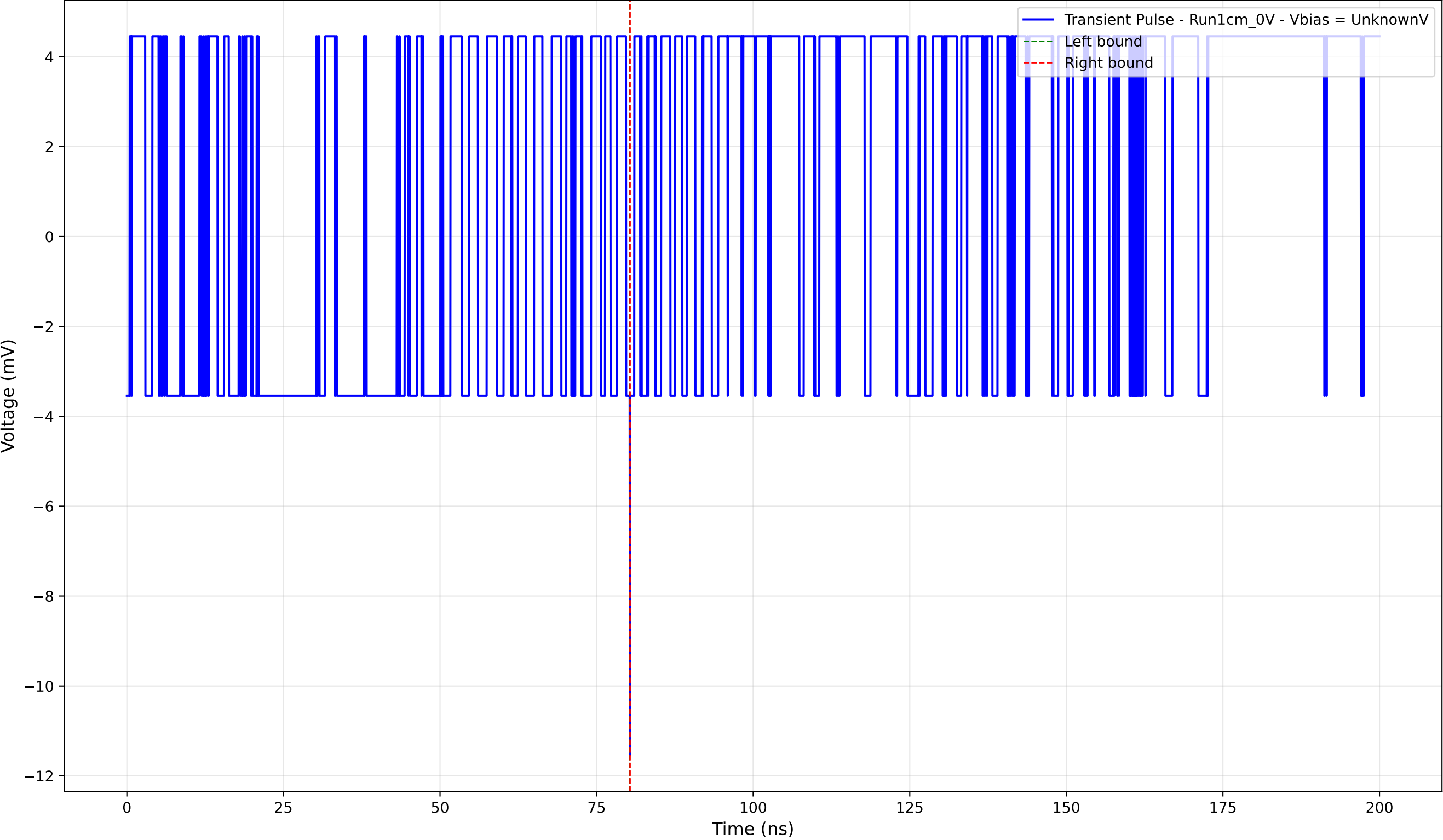
Transient Pulse - Sample: new1cm - Position: 705.0 \mu\text{m} - Charge: -0.01 pC
