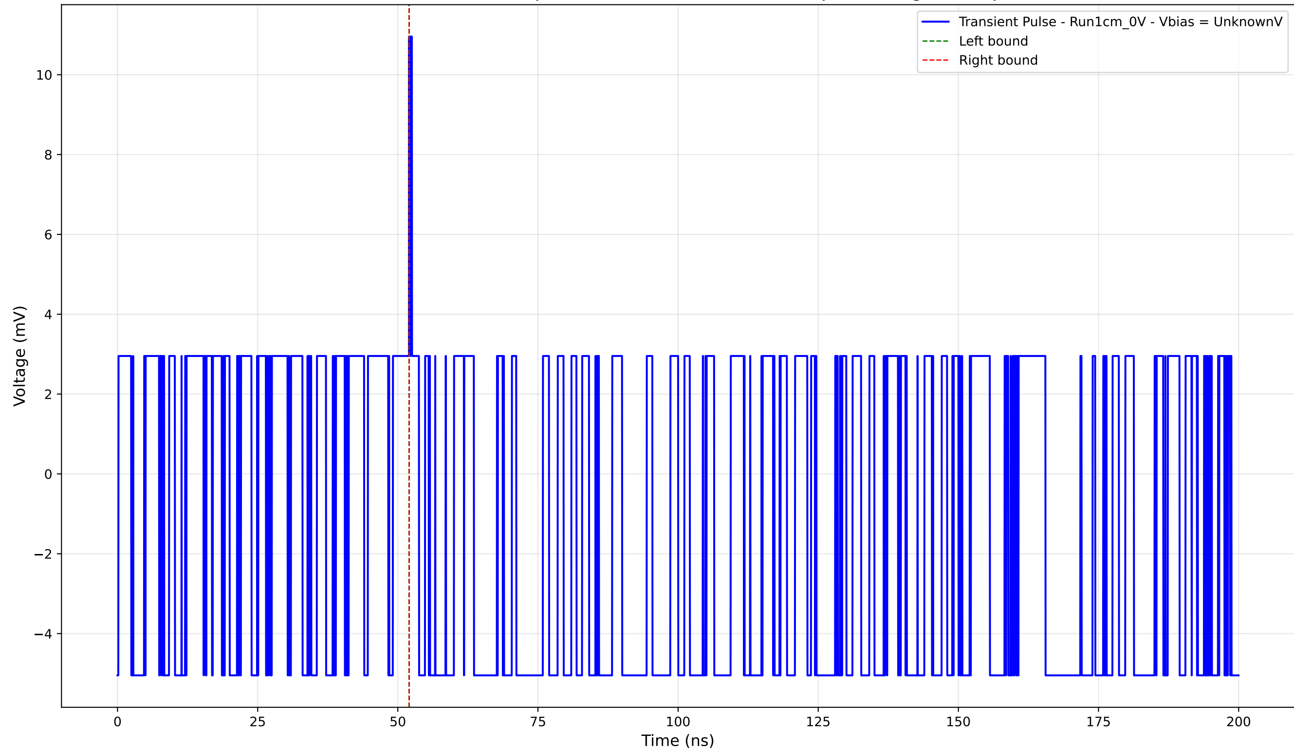
Transient Pulse - Sample: new1cm - Position: 2960.0 \mu\text{m} - Charge: 0.01 pC
