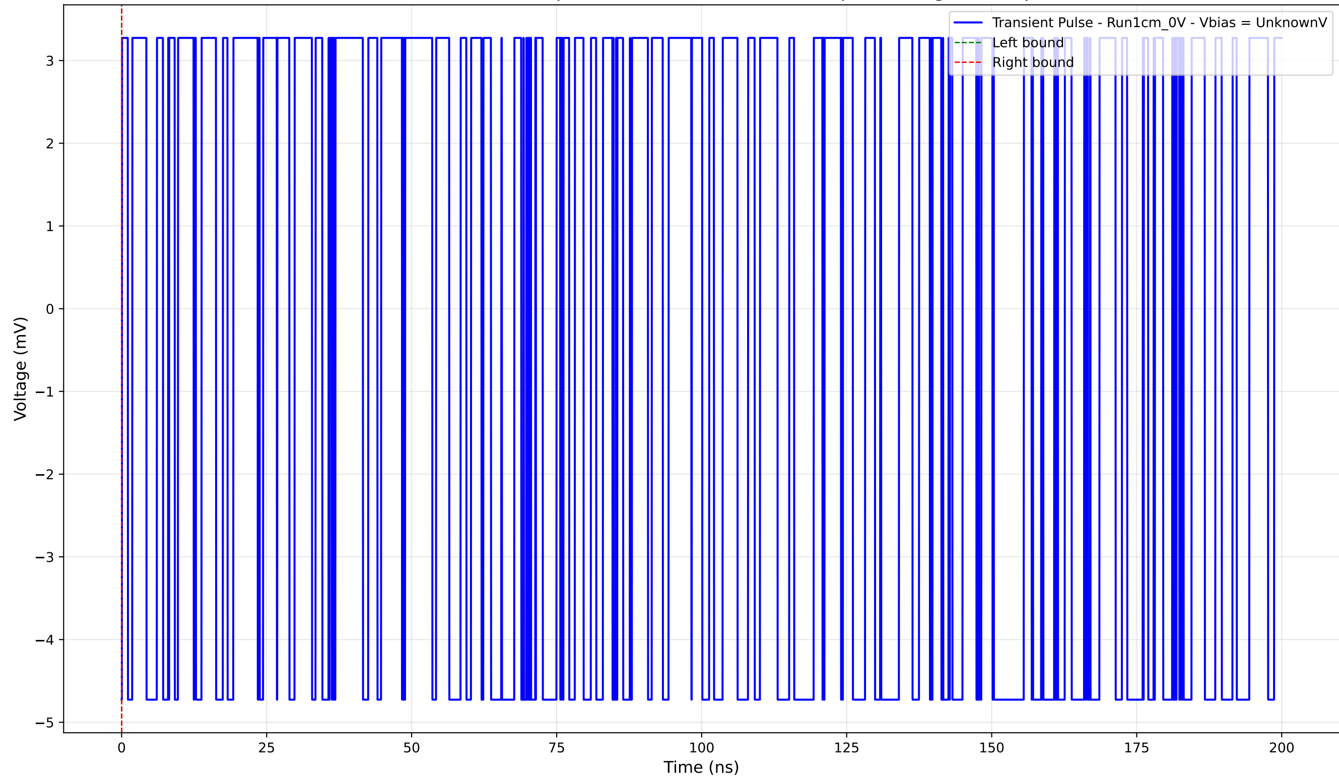
Transient Pulse - Sample: new1cm - Position: 200.0 \mu\text{m} - Charge: -0.00 pC
