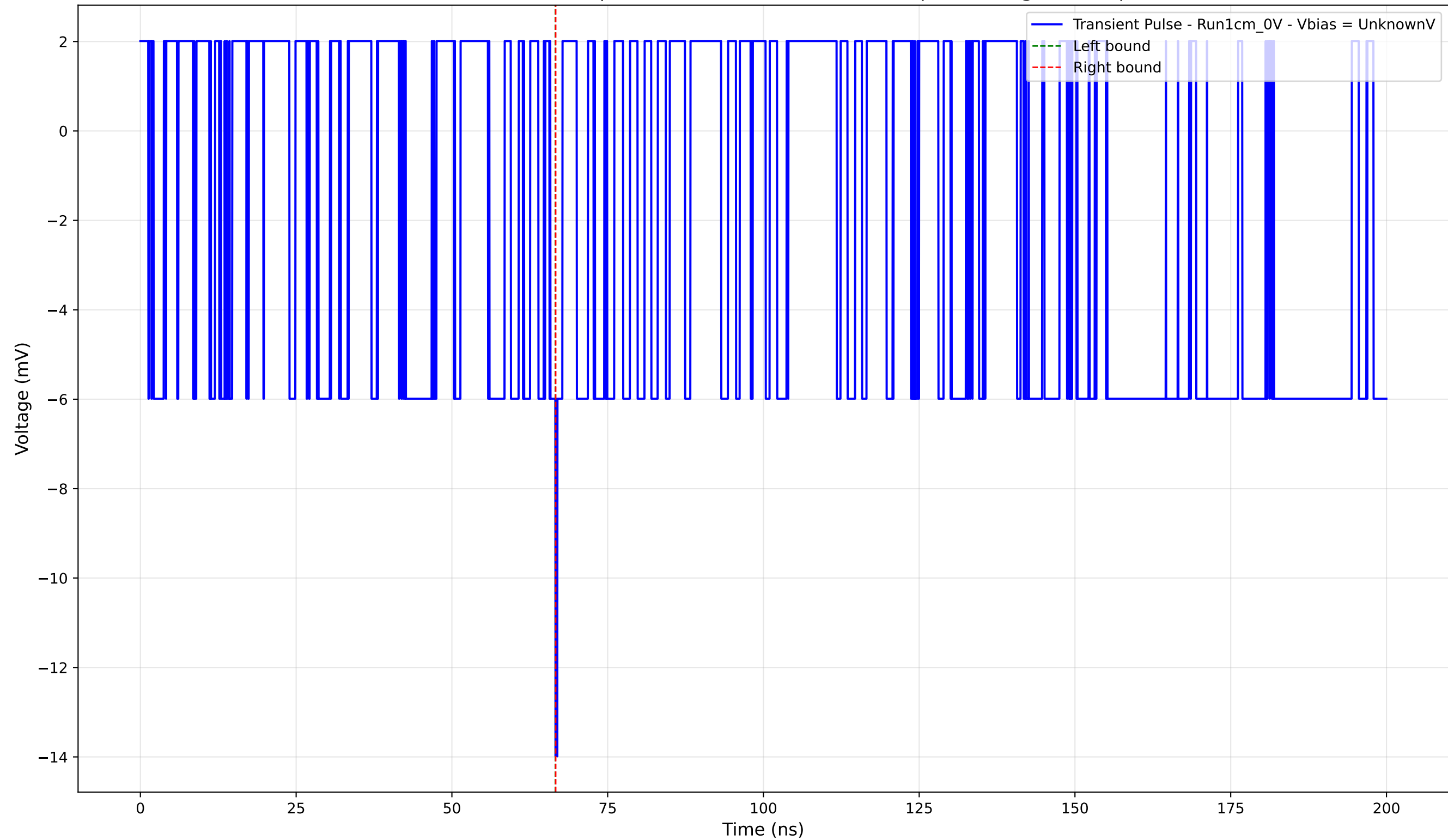
Transient Pulse - Sample: new1cm - Position: 3805.0 \mu\text{m} - Charge: -0.01 pC
