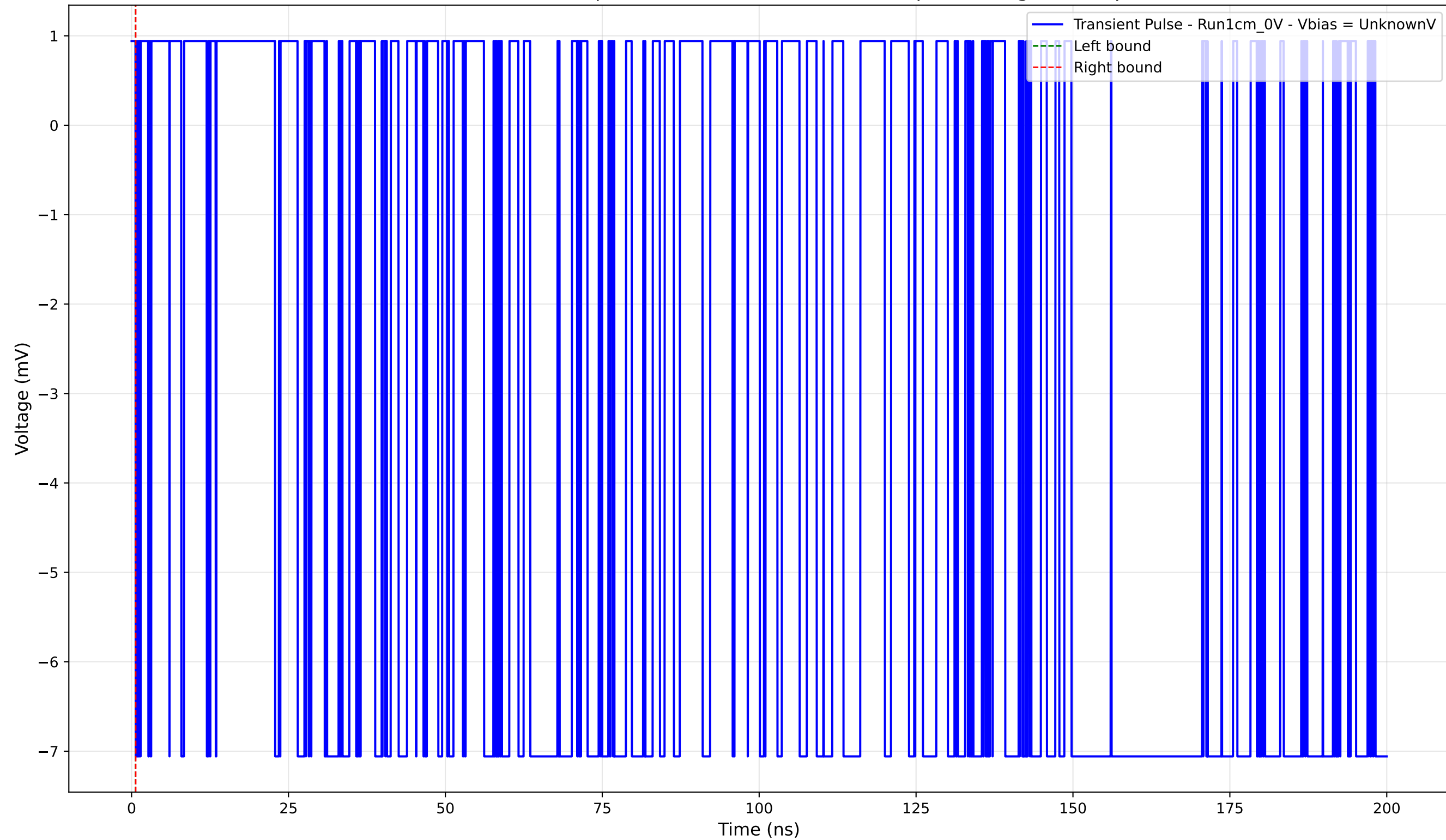
Transient Pulse - Sample: new1cm - Position: 3485.0 \mu\text{m} - Charge: -0.00 pC
