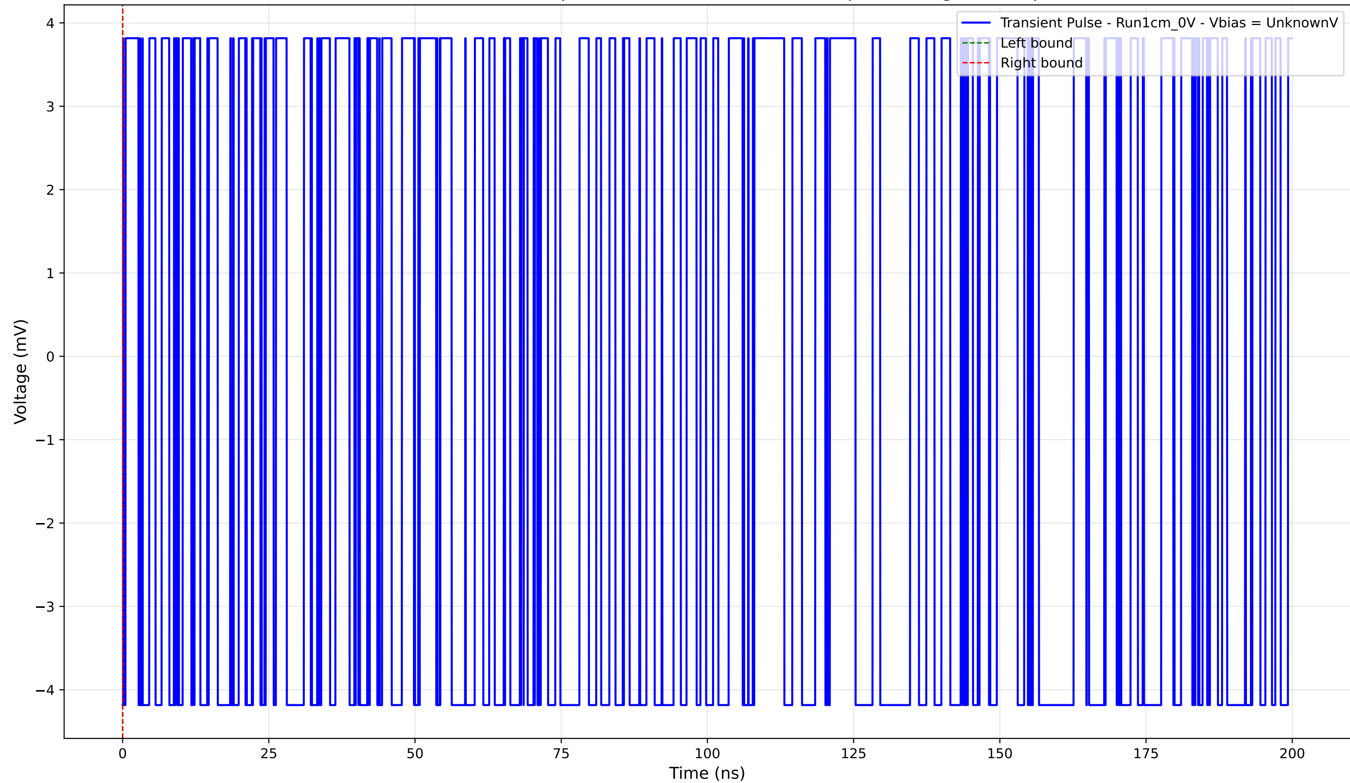
Transient Pulse - Sample: new1cm - Position: 285.0 \mu\text{m} - Charge: -0.00 pC
