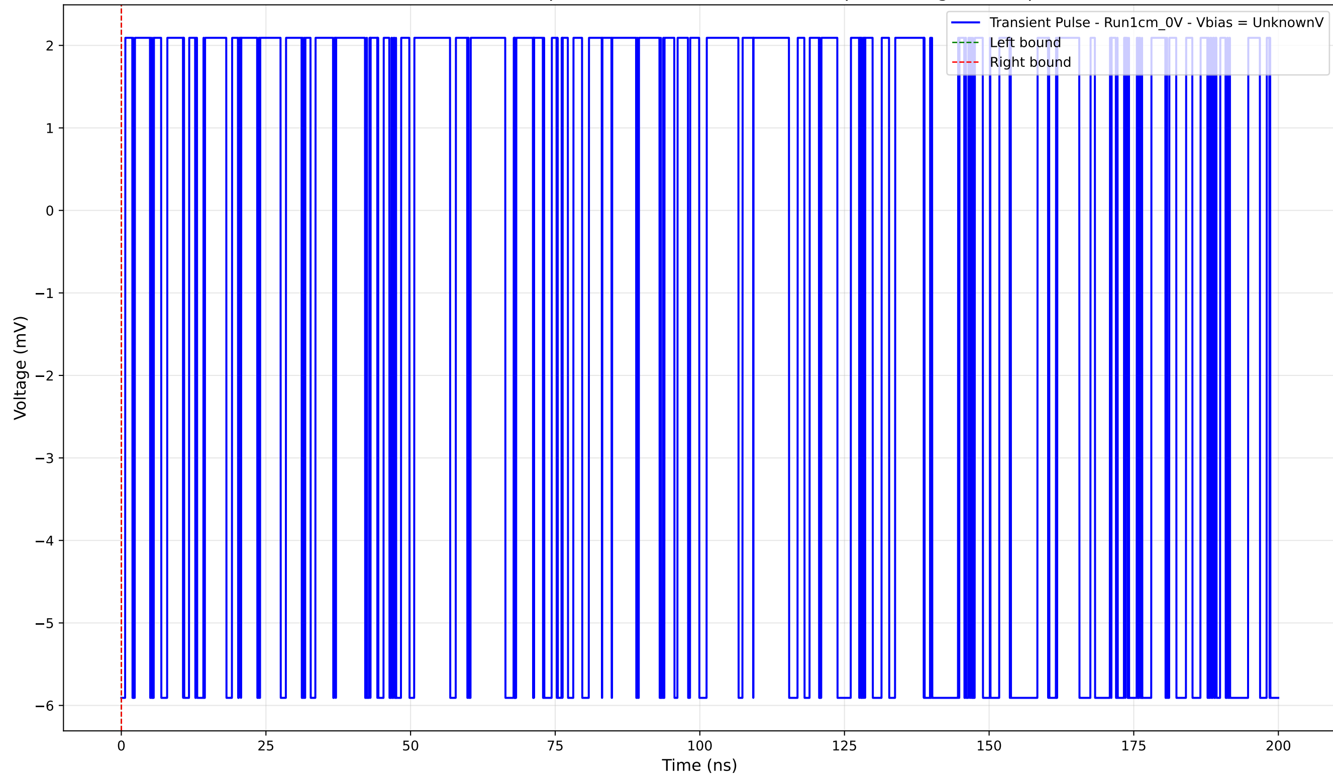
Transient Pulse - Sample: new1cm - Position: 2625.0 \mu\text{m} - Charge: -0.00 pC
