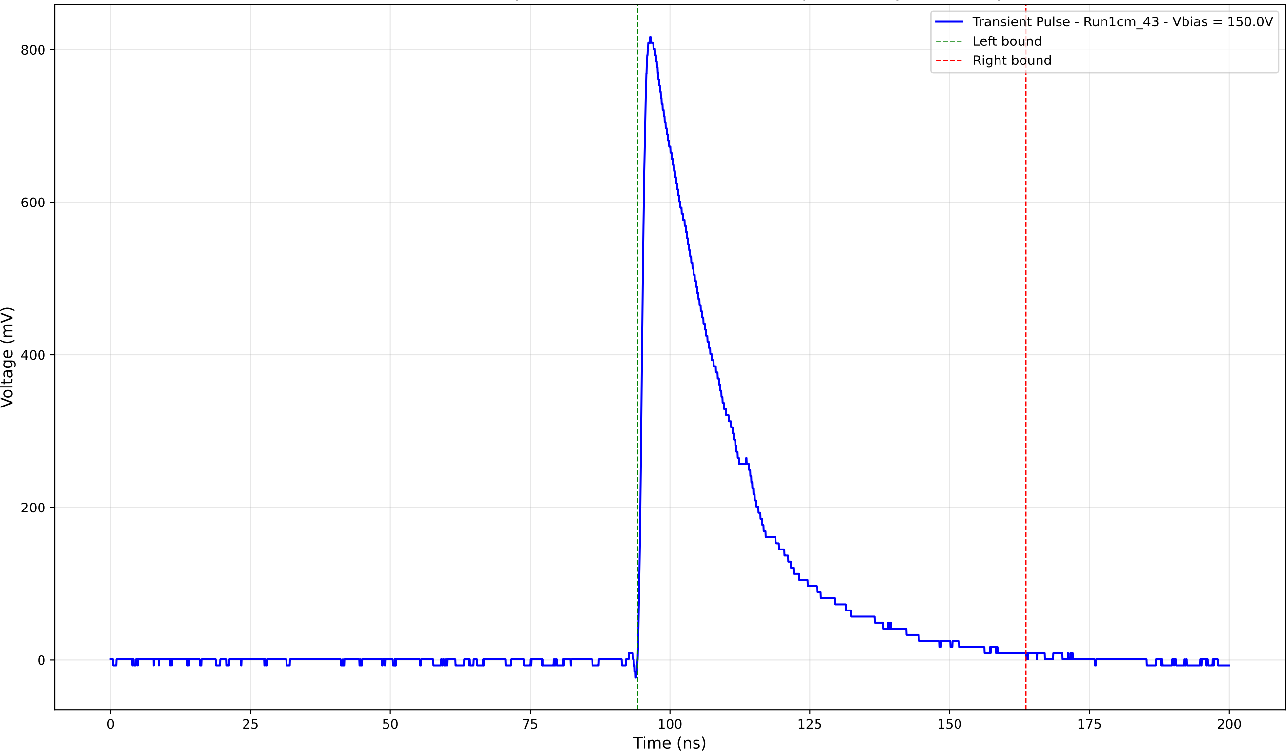
Transient Pulse - Sample: new1cm - Position: 4455.0 \mu\text{m} - Charge: 259.07 pC
