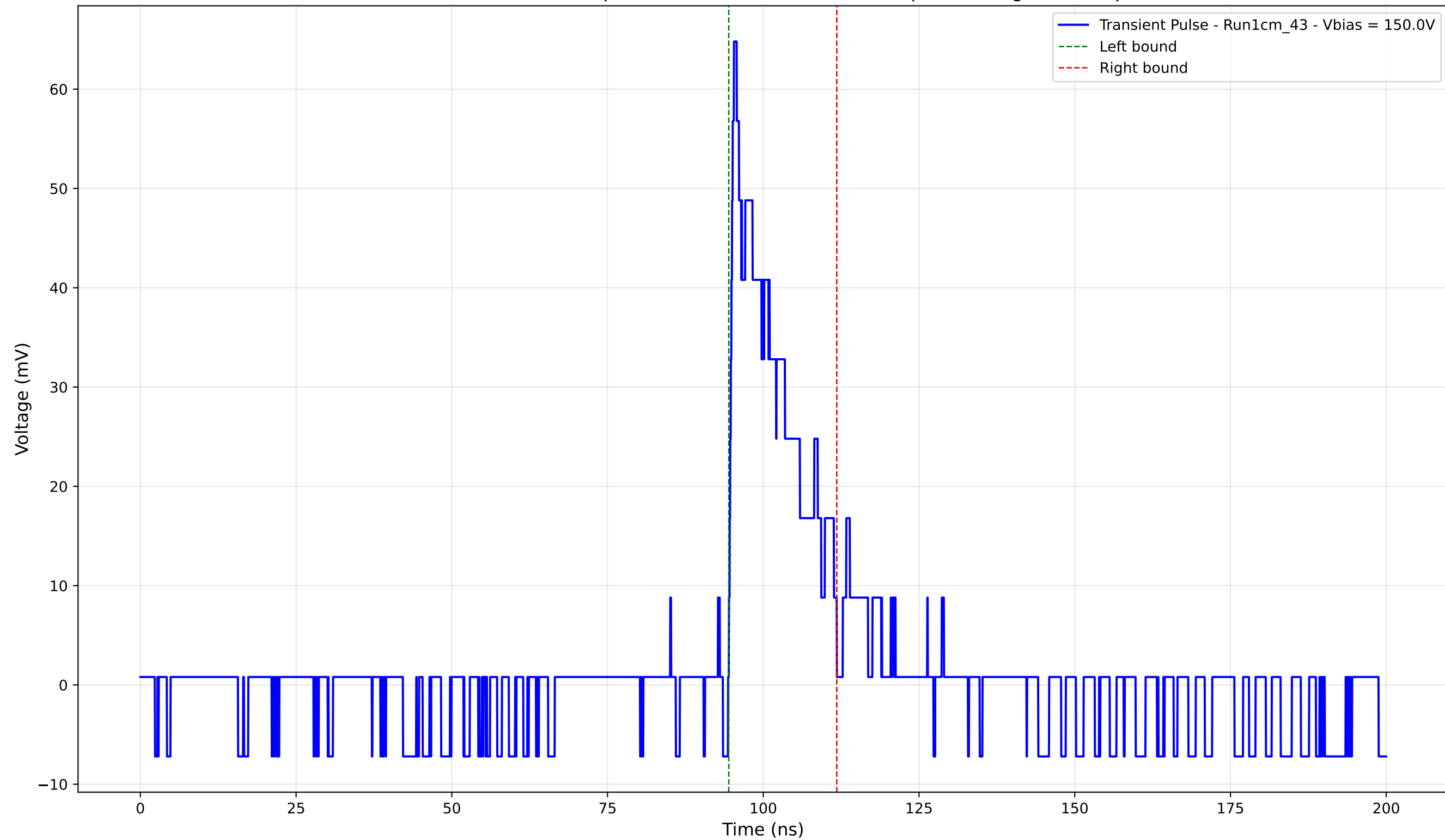
Transient Pulse - Sample: new1cm - Position: 170.0 \mu\text{m} - Charge: 10.50 pC
