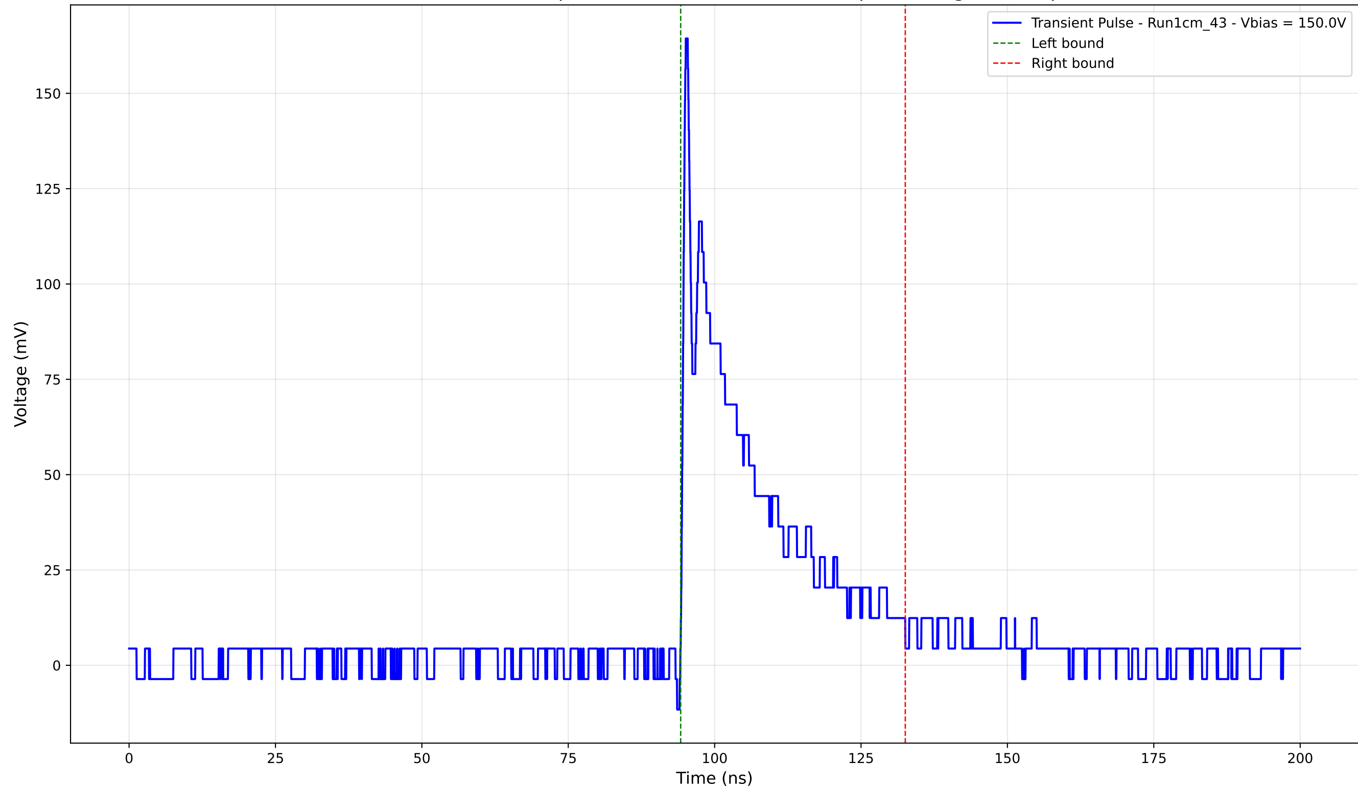
Transient Pulse - Sample: new1cm - Position: 2705.0 \mu\text{m} - Charge: 34.04 pC
