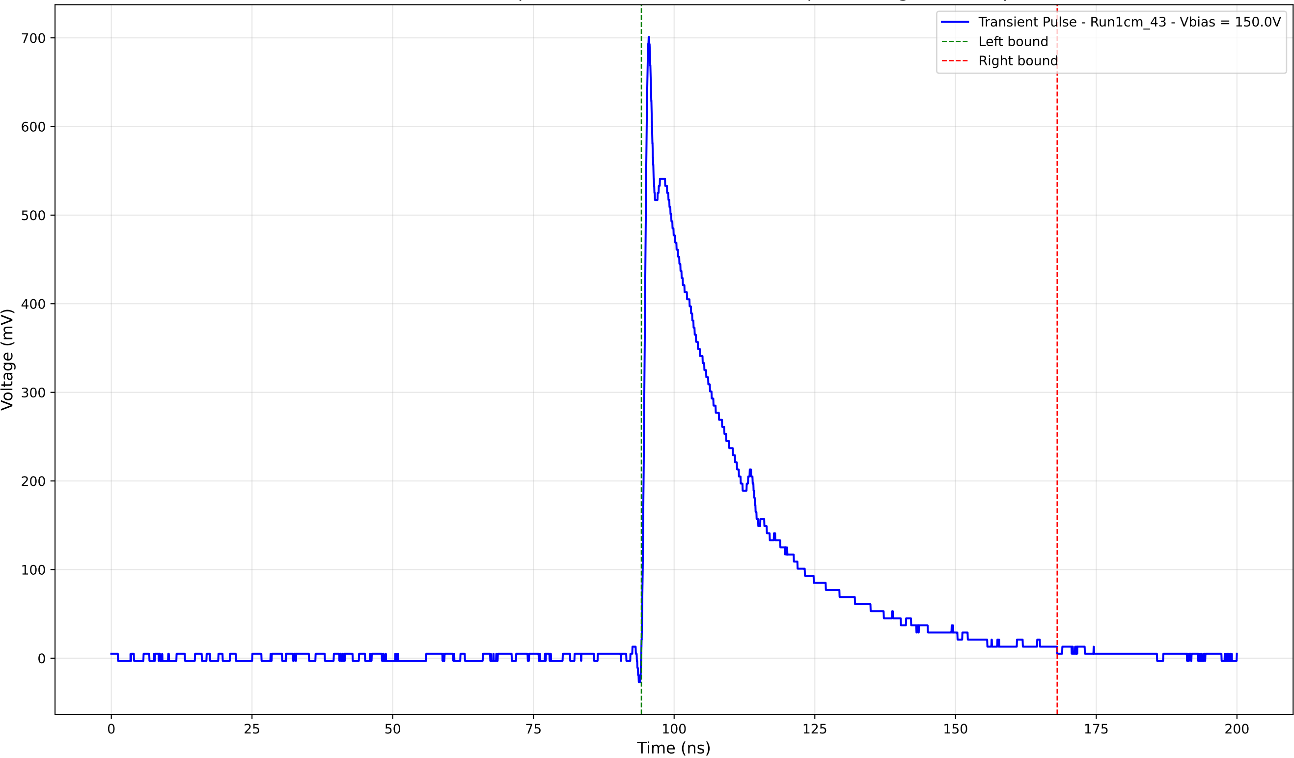
Transient Pulse - Sample: new1cm - Position: 2295.0 \mu\text{m} - Charge: 204.00 pC
