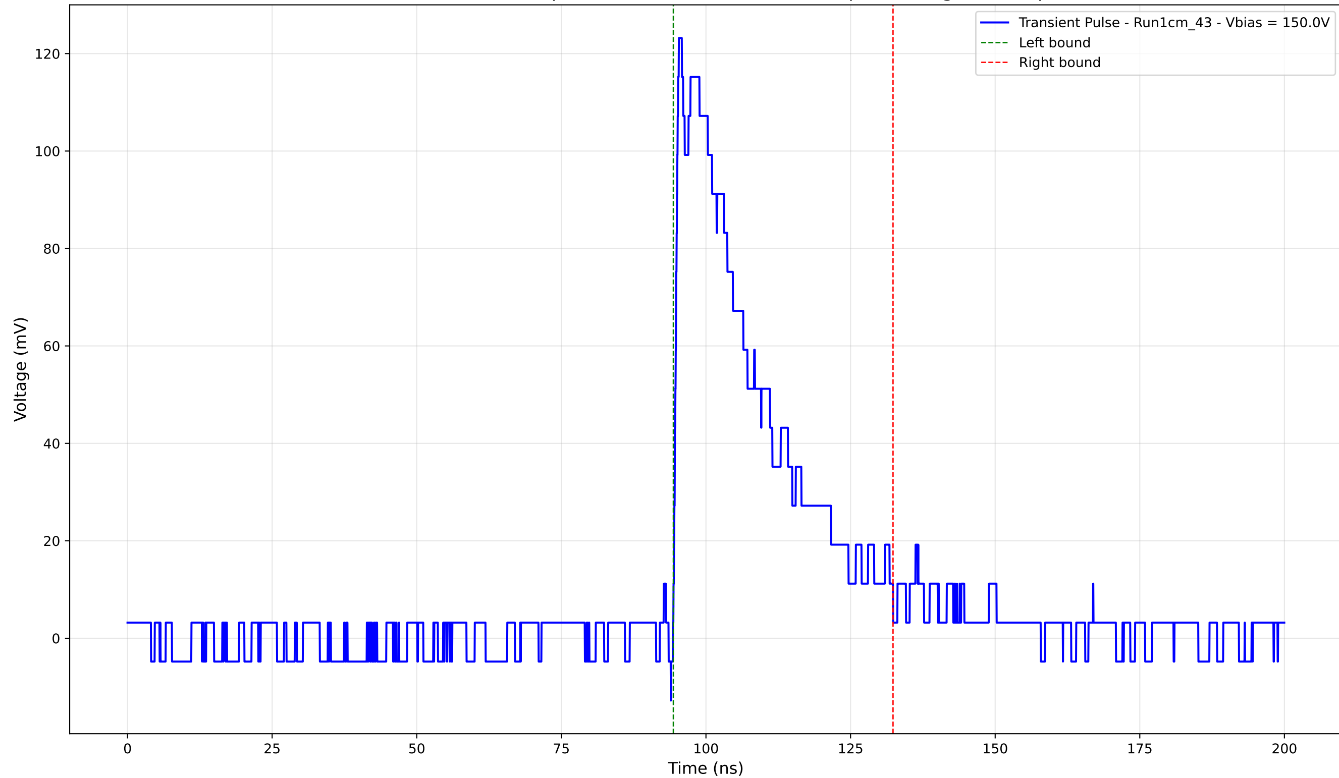
Transient Pulse - Sample: new1cm - Position: 3200.0 \mu\text{m} - Charge: 37.35 pC
