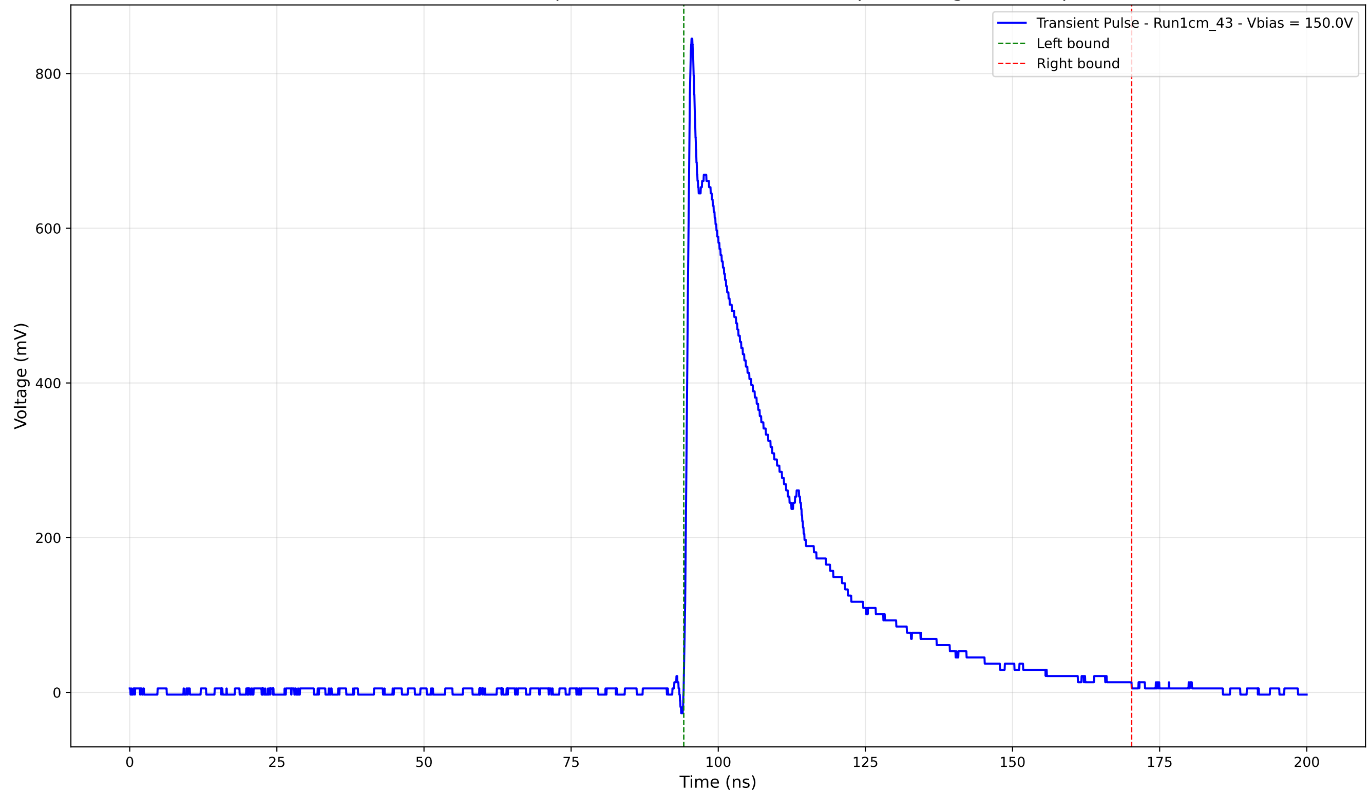
Transient Pulse - Sample: new1cm - Position: 3085.0 \mu\text{m} - Charge: 254.26 pC
