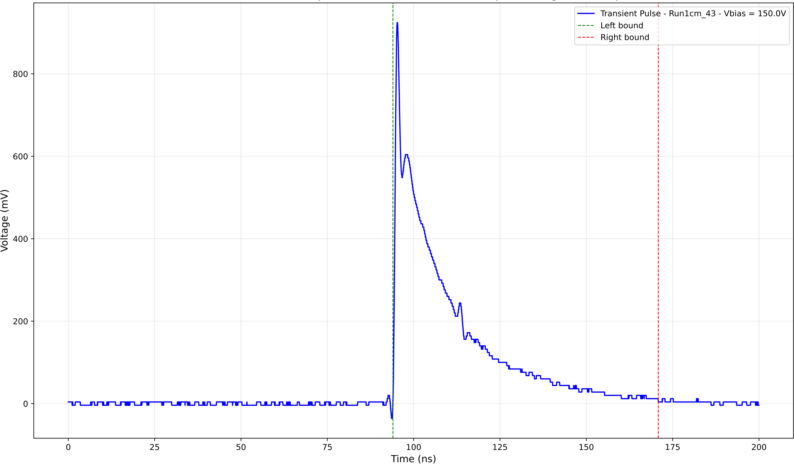
Transient Pulse - Sample: new1cm - Position: 2580.0 \mu\text{m} - Charge: 233.31 pC
