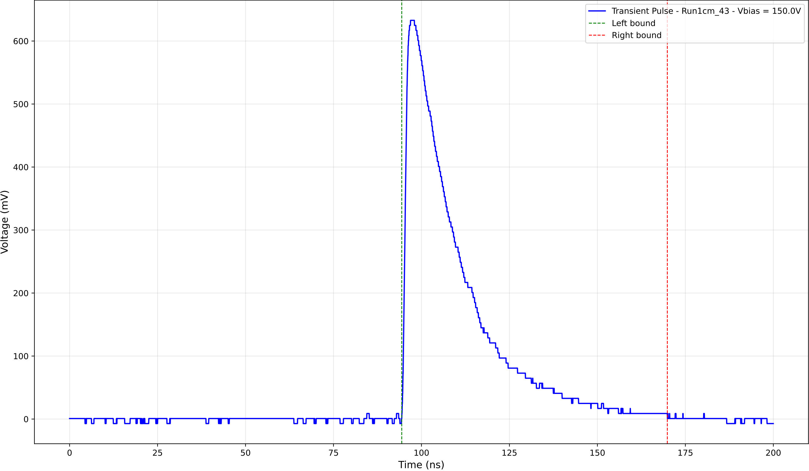
Transient Pulse - Sample: new1cm - Position: 1460.0 \mu\text{m} - Charge: 213.88 pC
