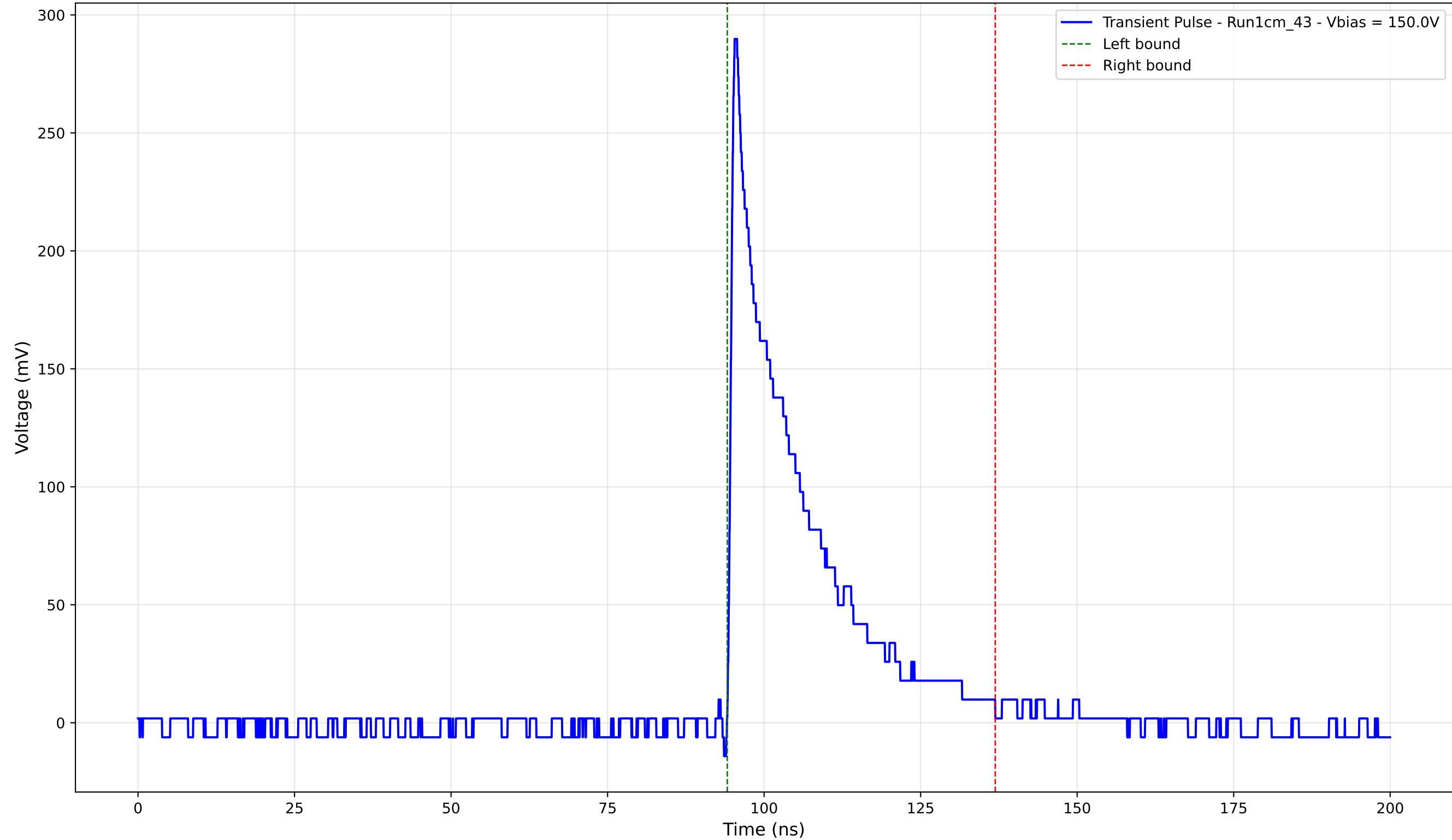
Transient Pulse - Sample: new1cm - Position: 5015.0 \mu\text{m} - Charge: 60.15 pC
