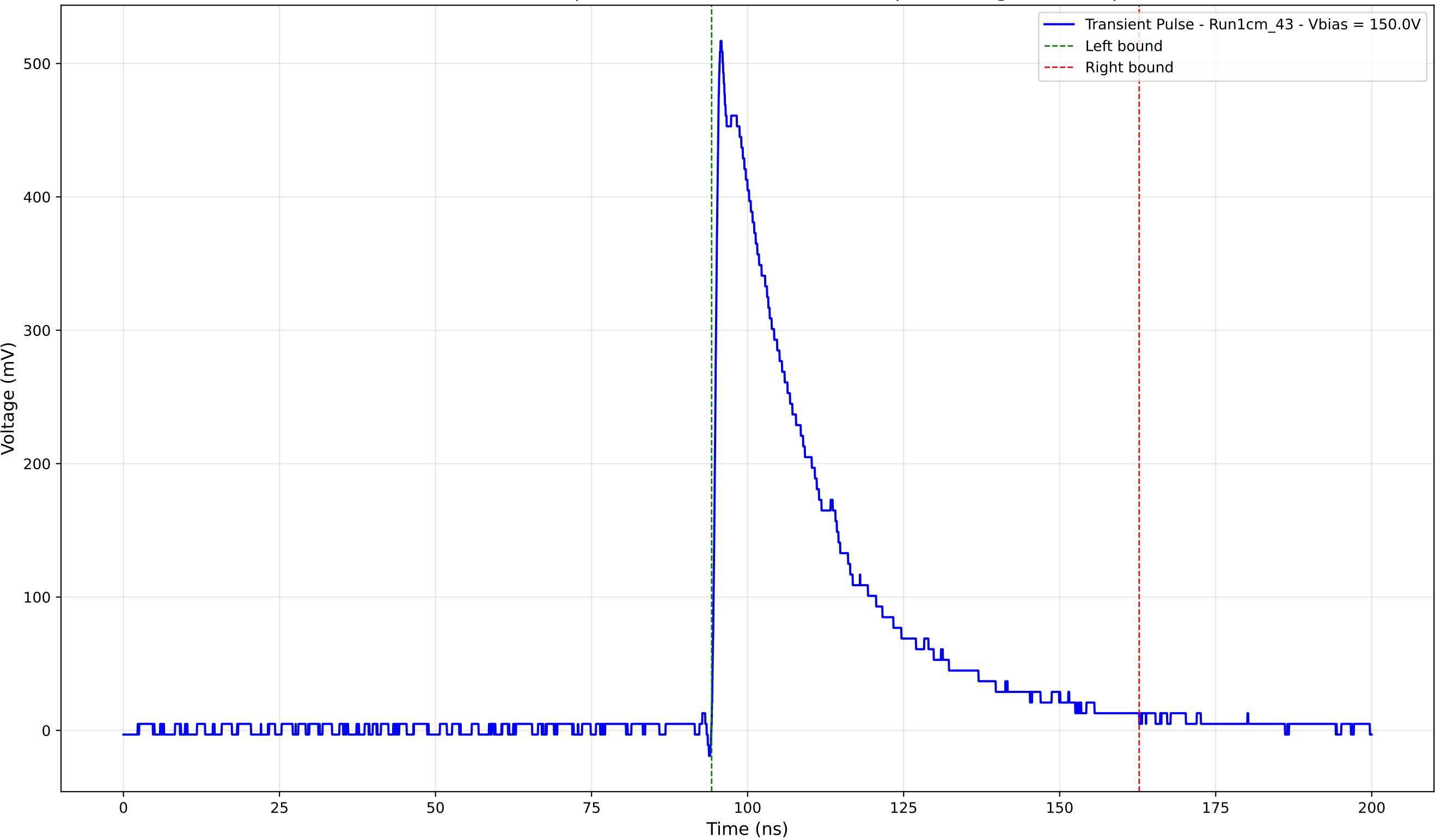
Transient Pulse - Sample: new1cm - Position: 3270.0 \mu\text{m} - Charge: 167.41 pC
