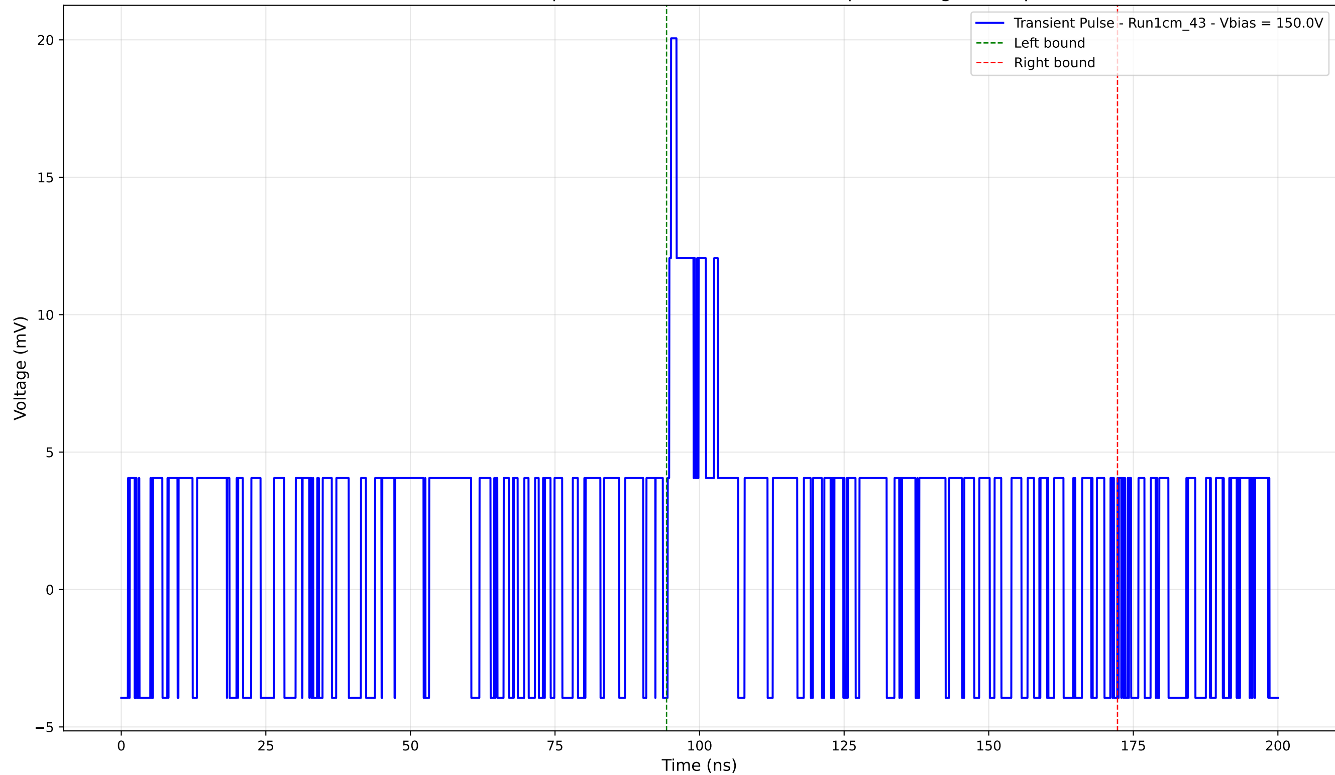
Transient Pulse - Sample: new1cm - Position: 5090.0 \mu\text{m} - Charge: 4.16 pC
