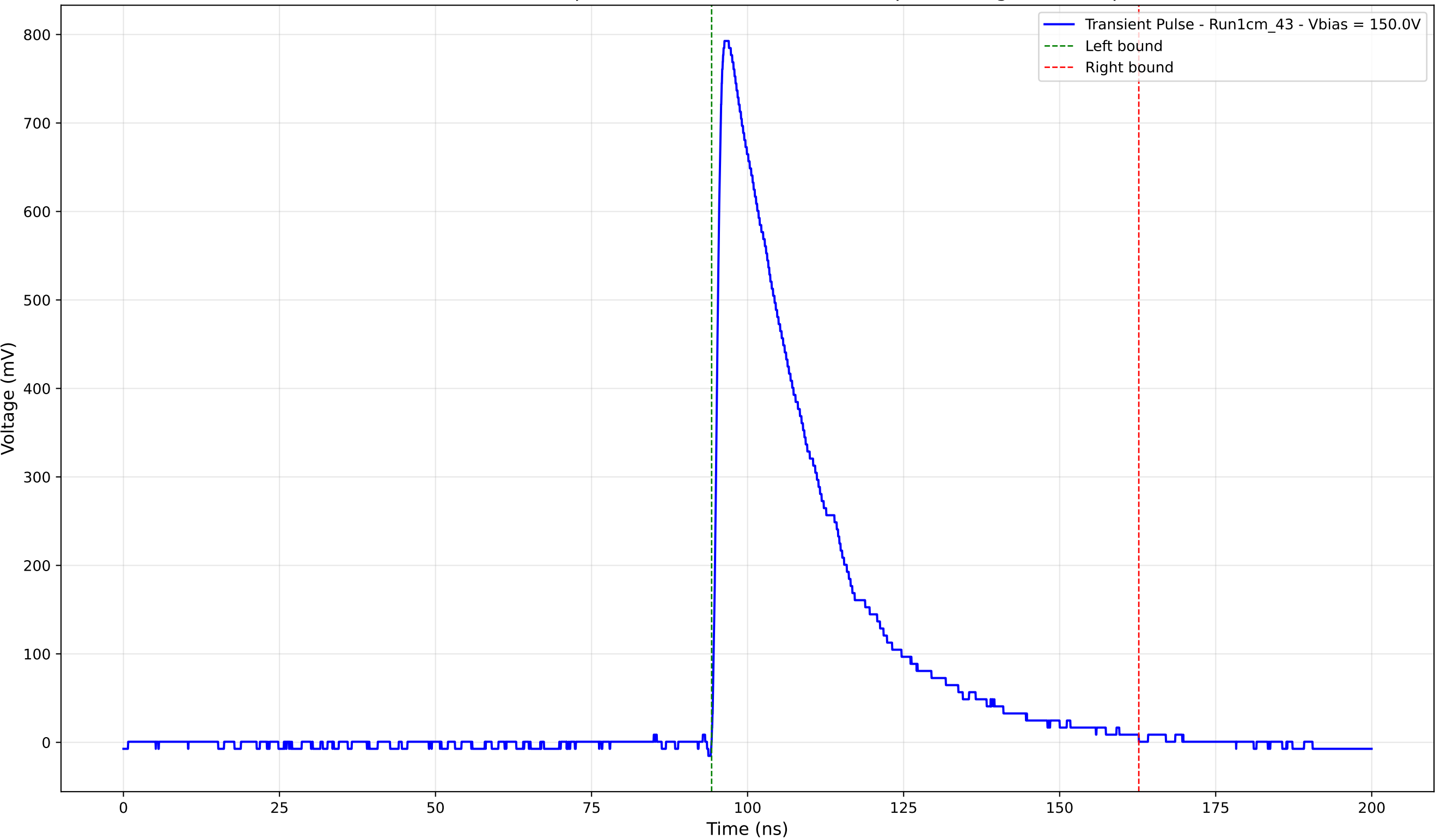
Transient Pulse - Sample: new1cm - Position: 4360.0 \mu\text{m} - Charge: 255.44 pC
