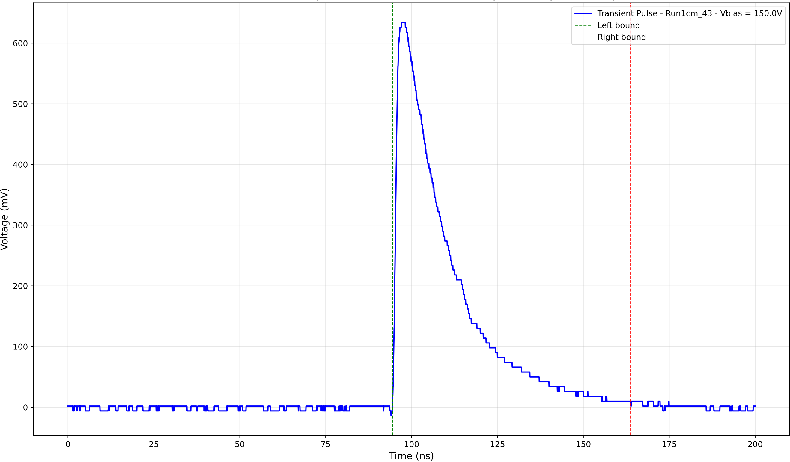
Transient Pulse - Sample: new1cm - Position: 1475.0 \mu\text{m} - Charge: 214.55 pC
