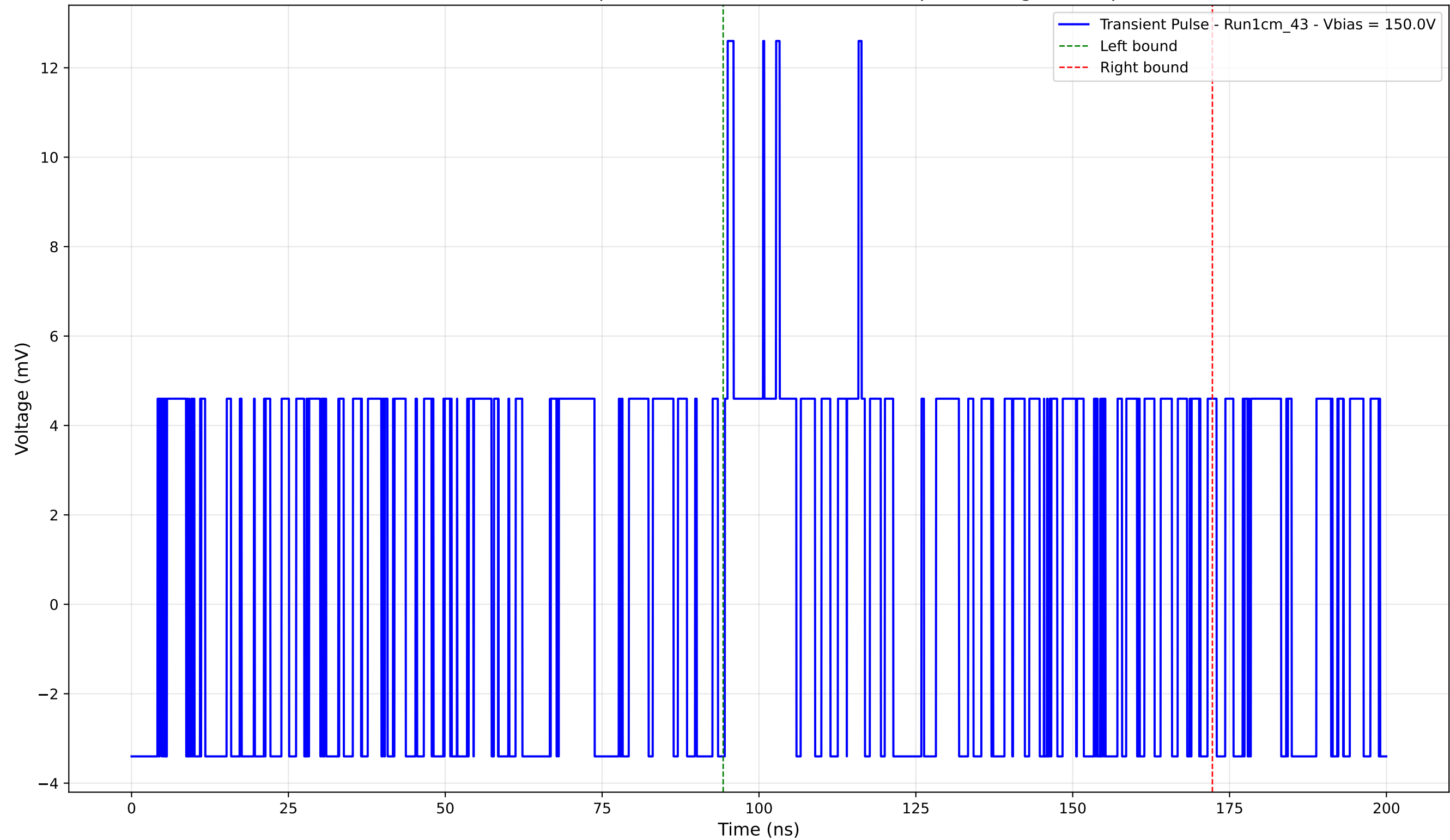
Transient Pulse - Sample: new1cm - Position: 5155.0 \mu\text{m} - Charge: 2.90 pC
