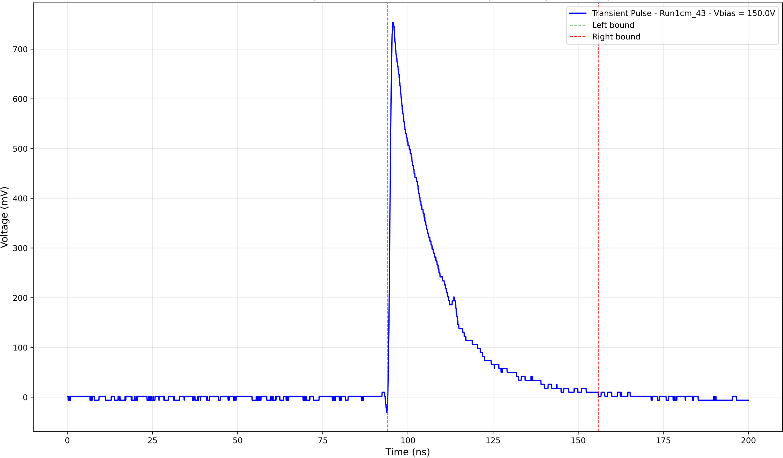
Transient Pulse - Sample: new1cm - Position: 4835.0 \mu\text{m} - Charge: 198.26 pC
