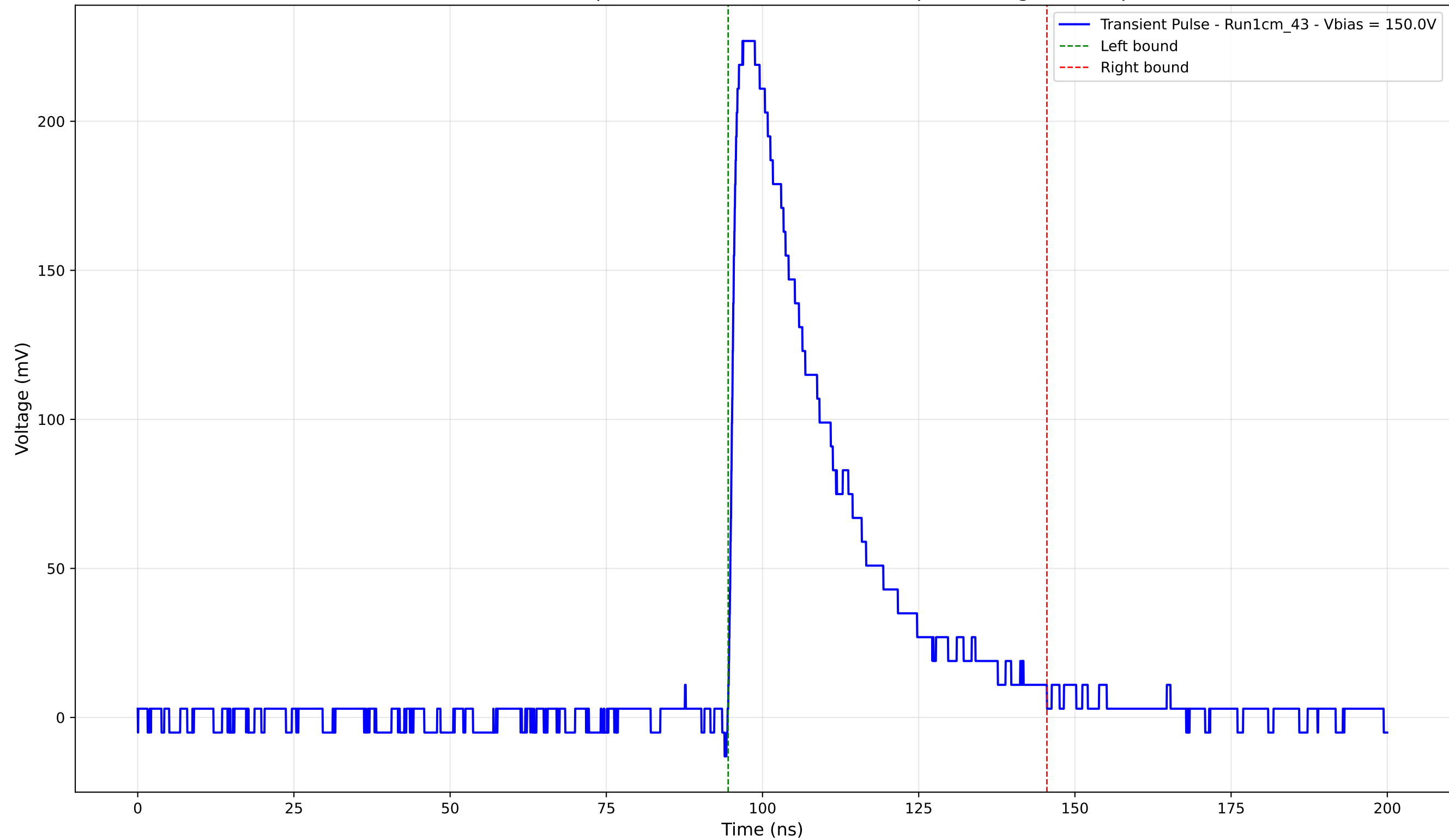
Transient Pulse - Sample: new1cm - Position: 1725.0 \mu\text{m} - Charge: 75.59 pC
