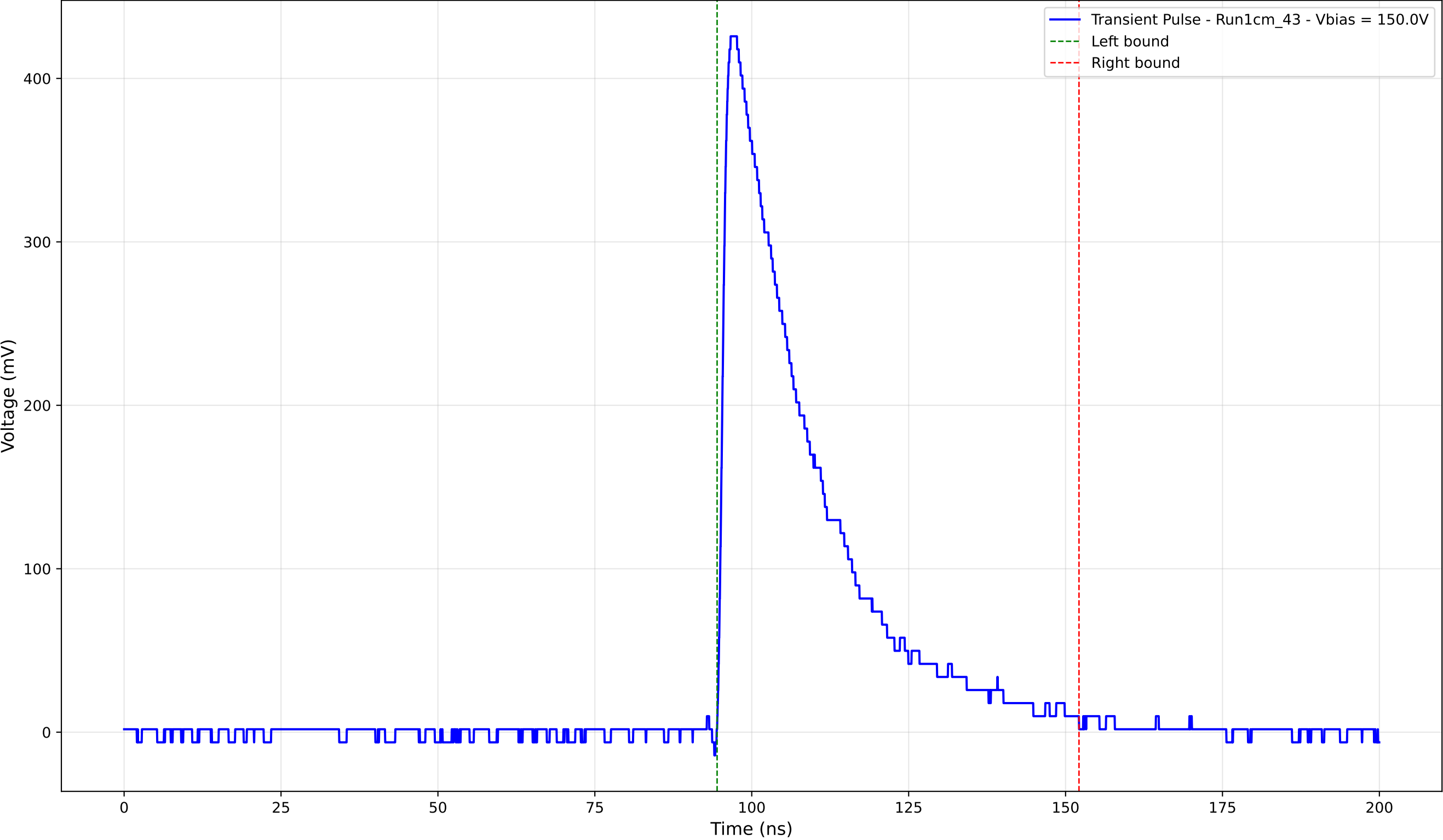
Transient Pulse - Sample: new1cm - Position: 1120.0 \mu\text{m} - Charge: 130.46 pC
