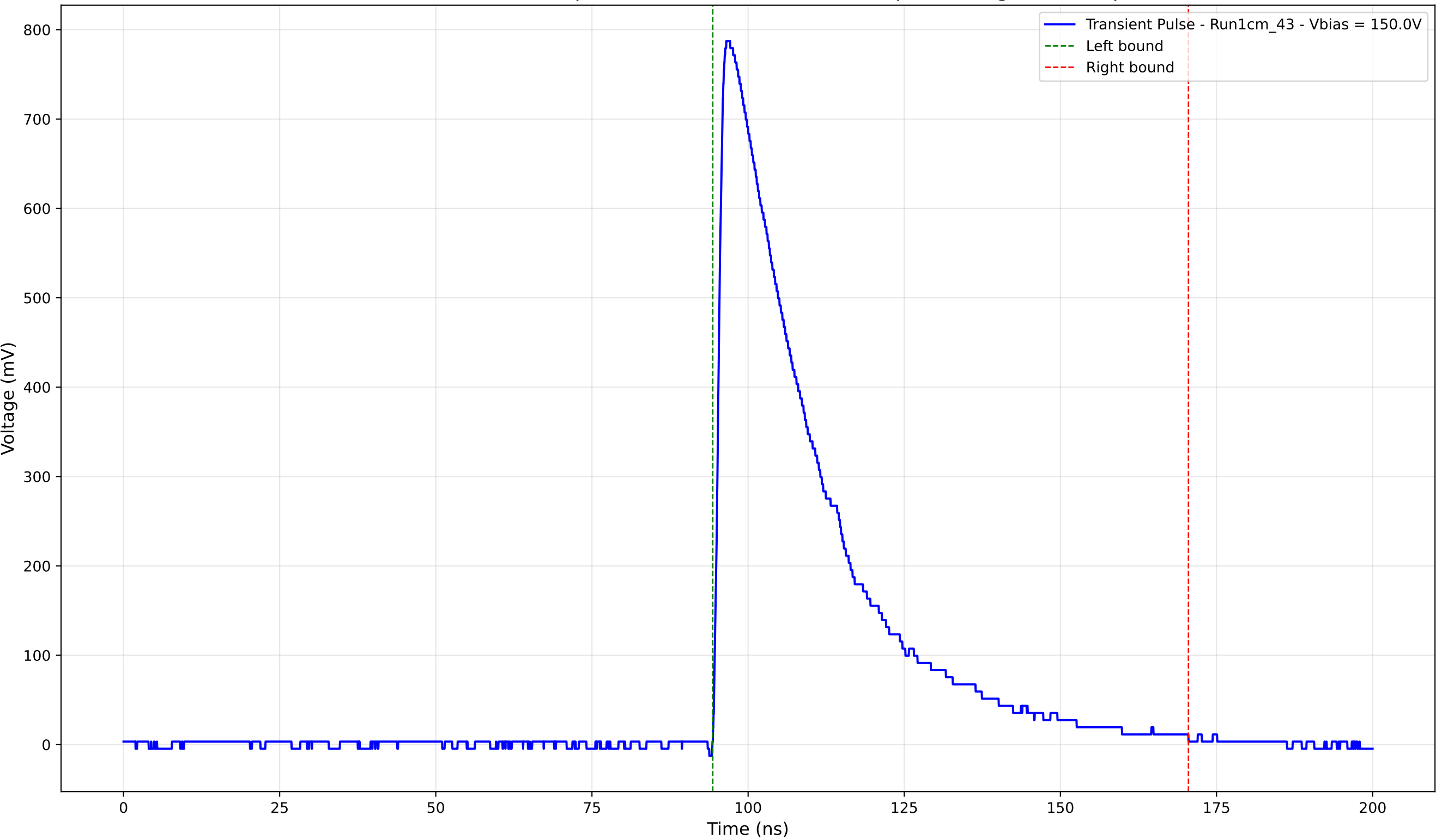
Transient Pulse - Sample: new1cm - Position: 4035.0 \mu\text{m} - Charge: 269.93 pC
