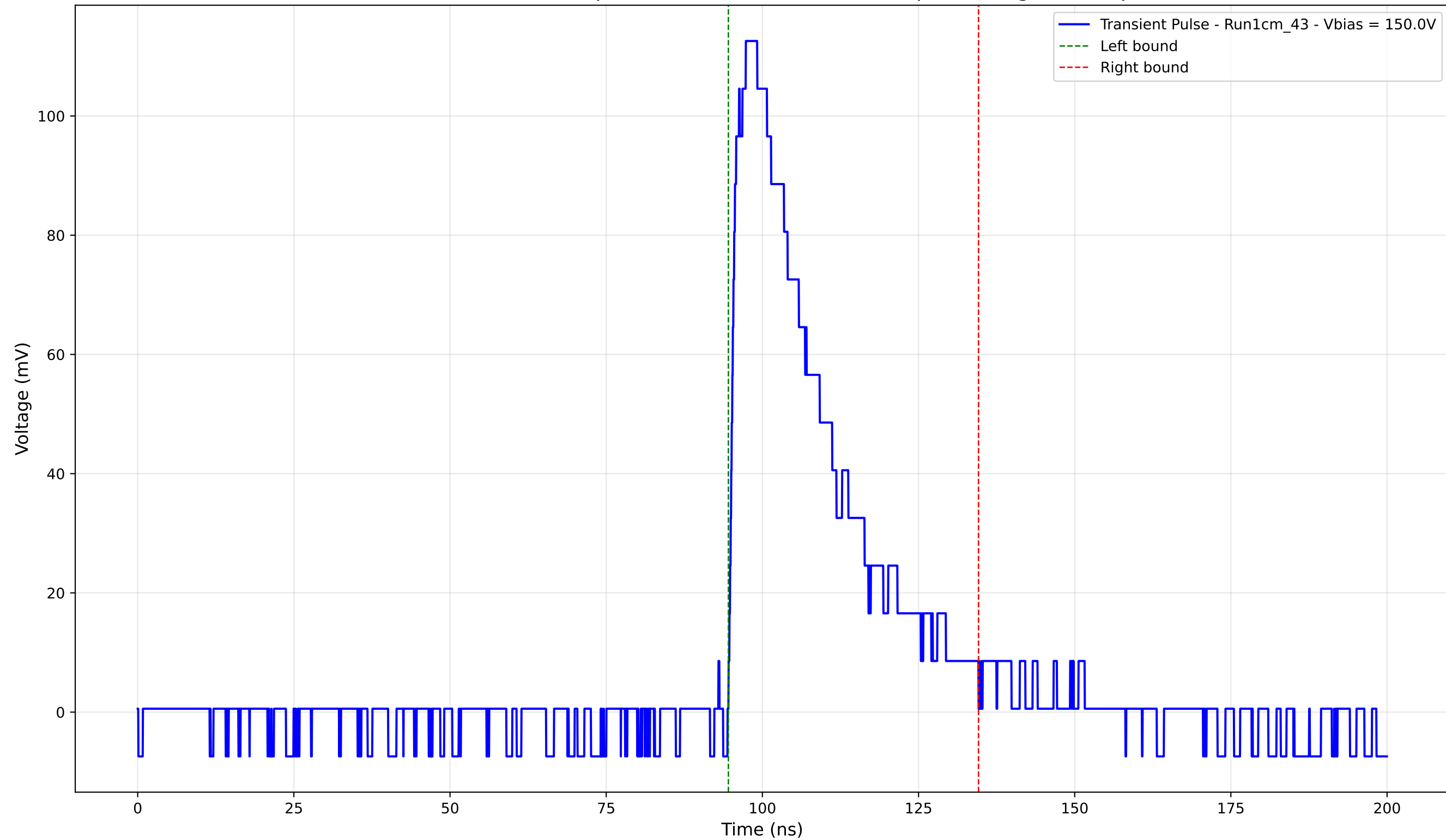
Transient Pulse - Sample: new1cm - Position: 3710.0 \mu\text{m} - Charge: 35.45 pC
