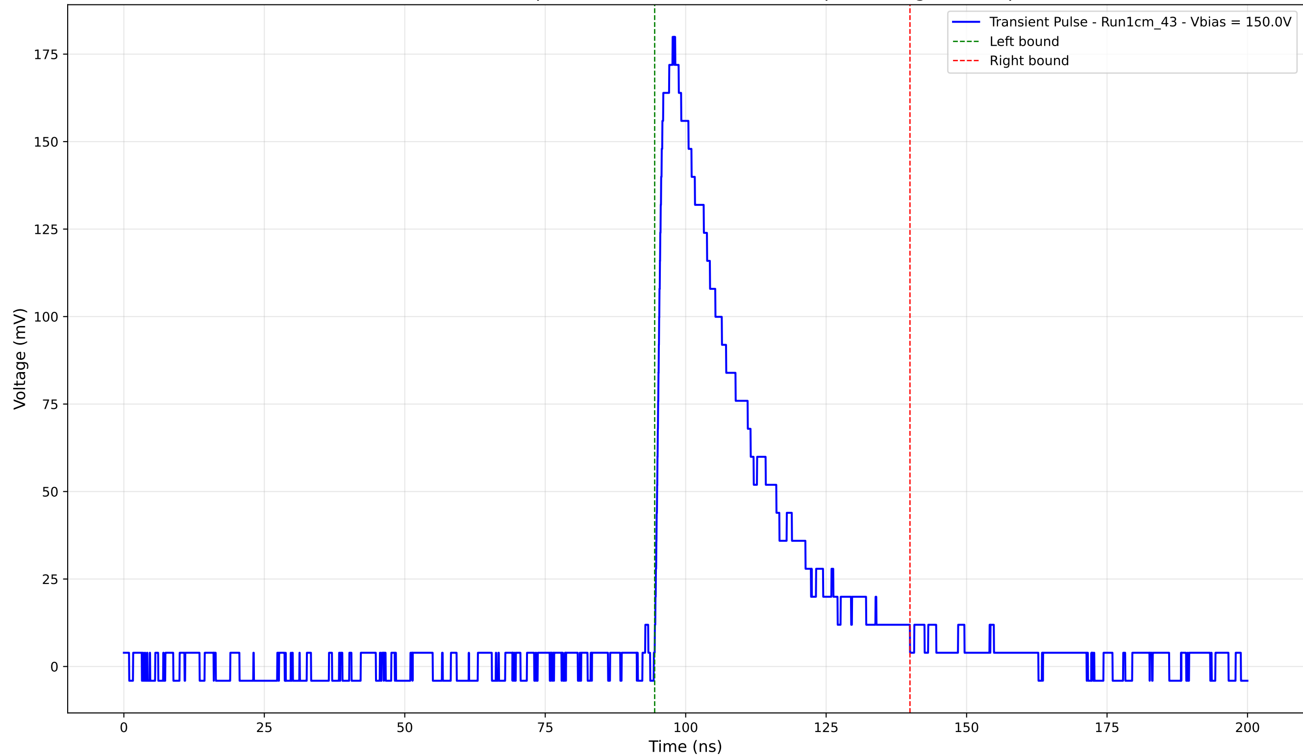
Transient Pulse - Sample: new1cm - Position: 4235.0 \mu\text{m} - Charge: 55.83 pC
