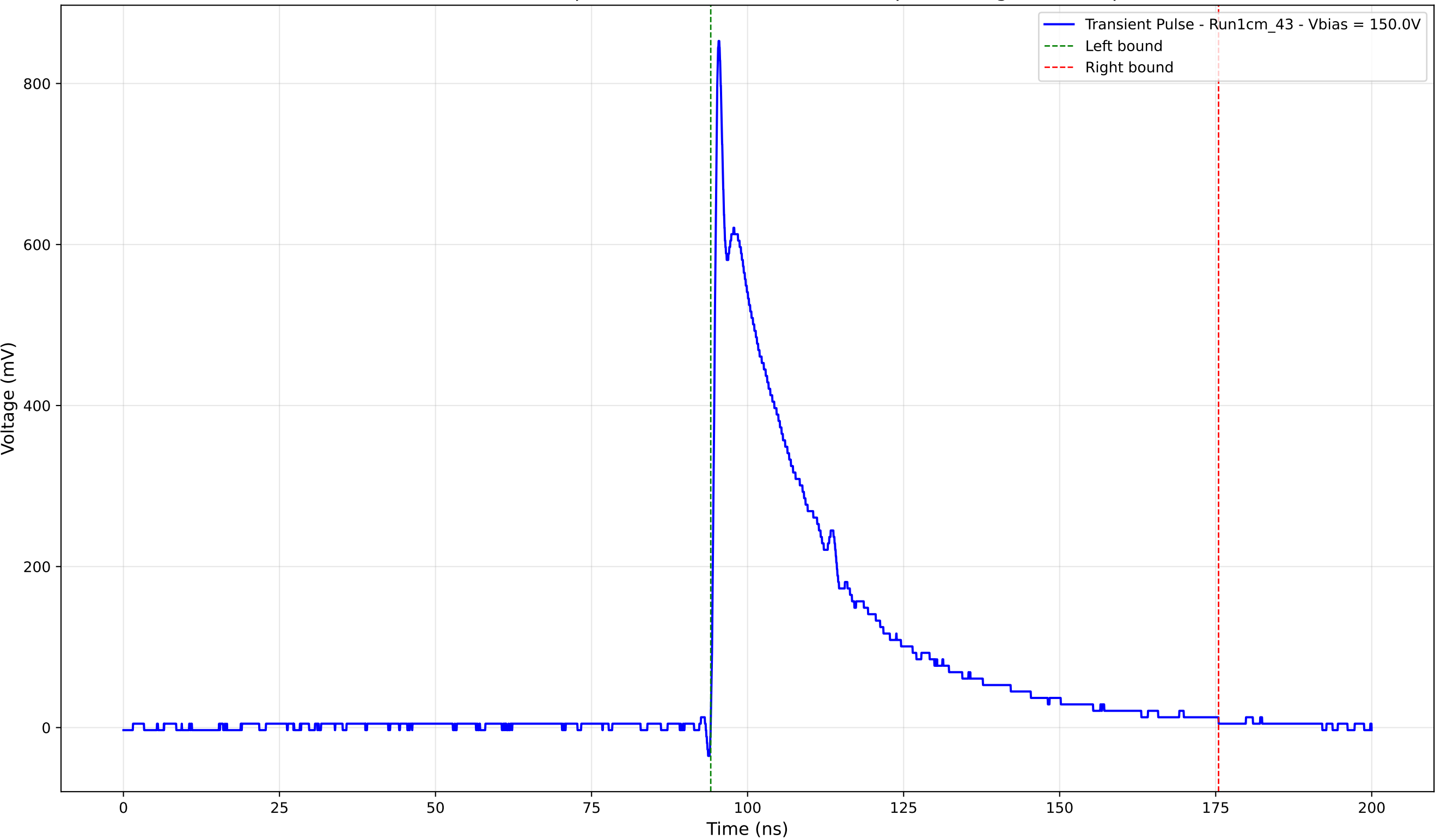
Transient Pulse - Sample: new1cm - Position: 2410.0 \mu\text{m} - Charge: 238.45 pC
