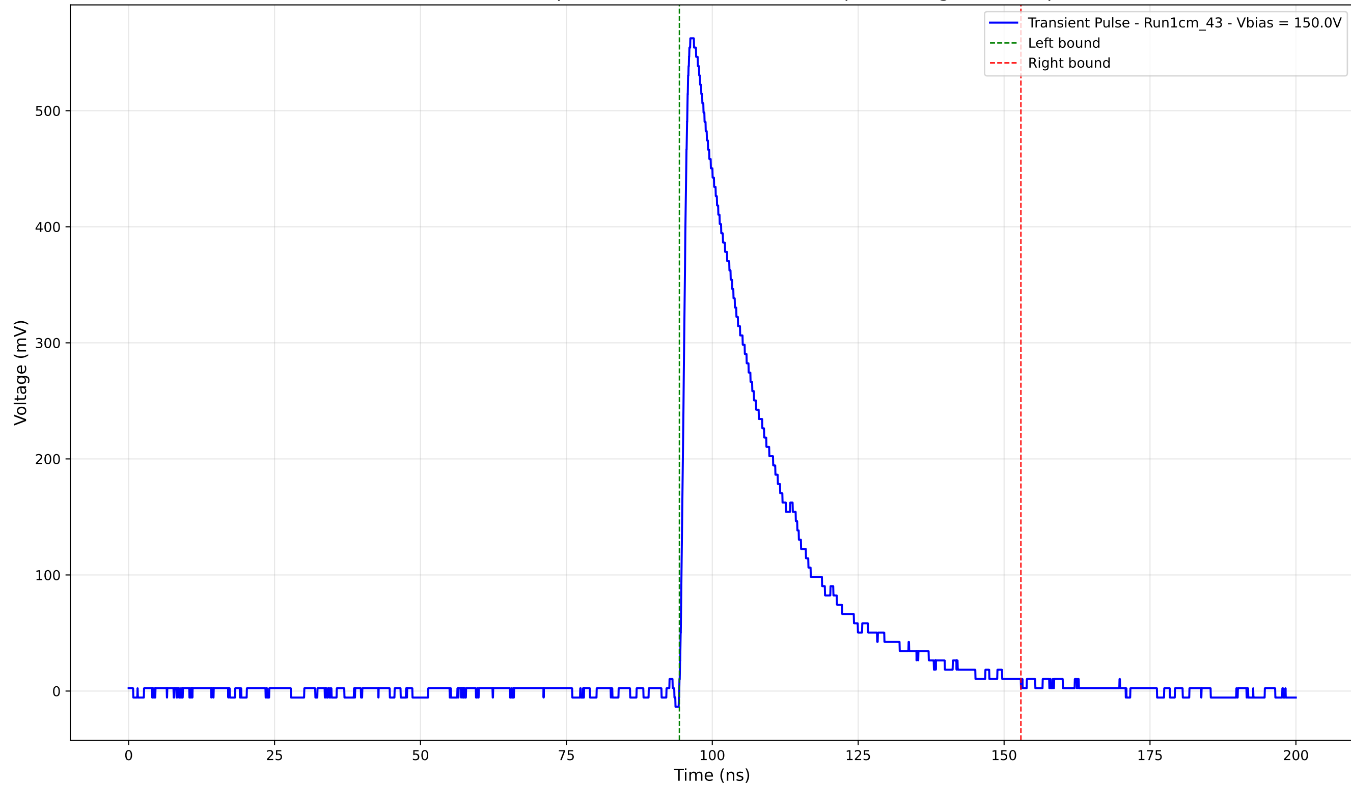
Transient Pulse - Sample: new1cm - Position: 760.0 \mu\text{m} - Charge: 162.89 pC
