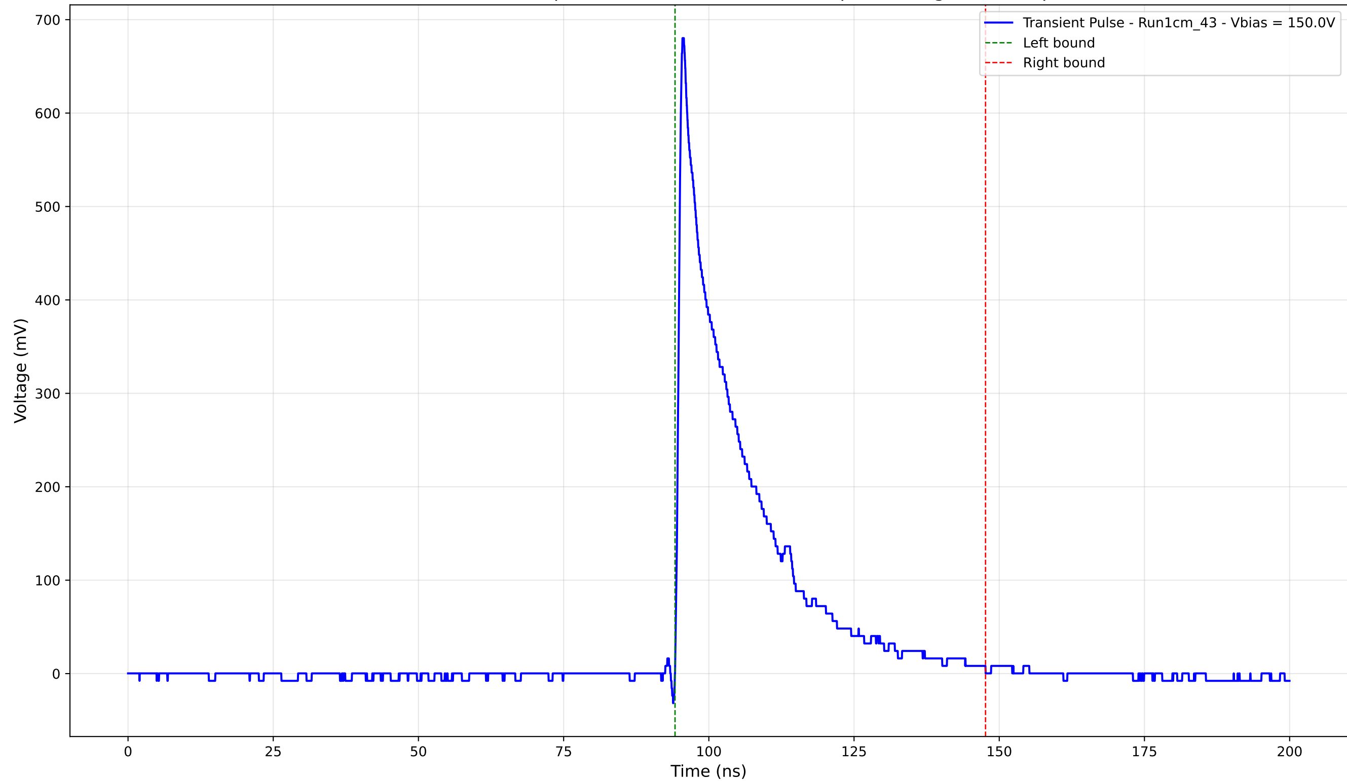
Transient Pulse - Sample: new1cm - Position: 260.0 \mu\text{m} - Charge: 143.97 pC
