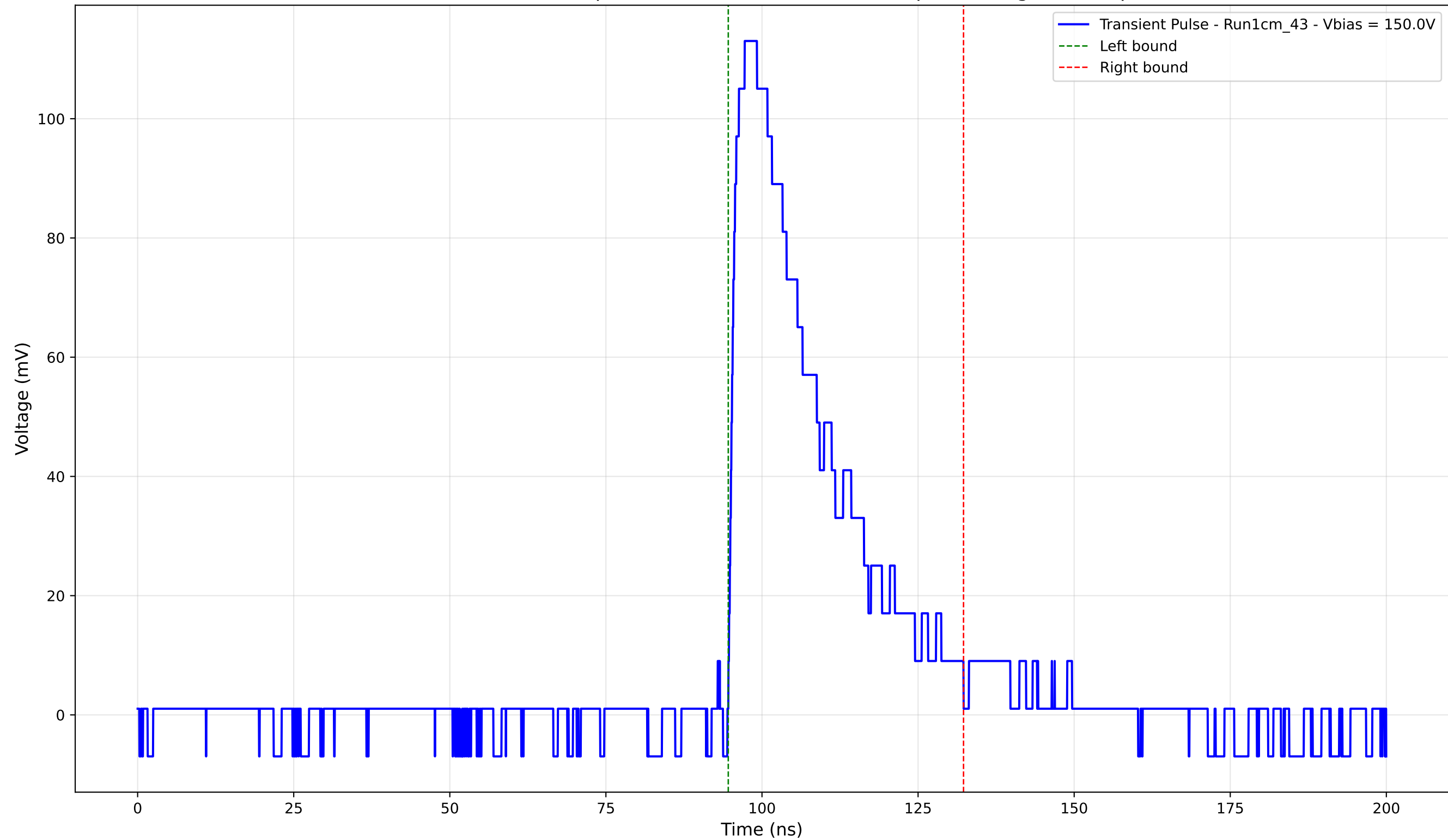
Transient Pulse - Sample: new1cm - Position: 4215.0 \mu\text{m} - Charge: 34.74 pC
