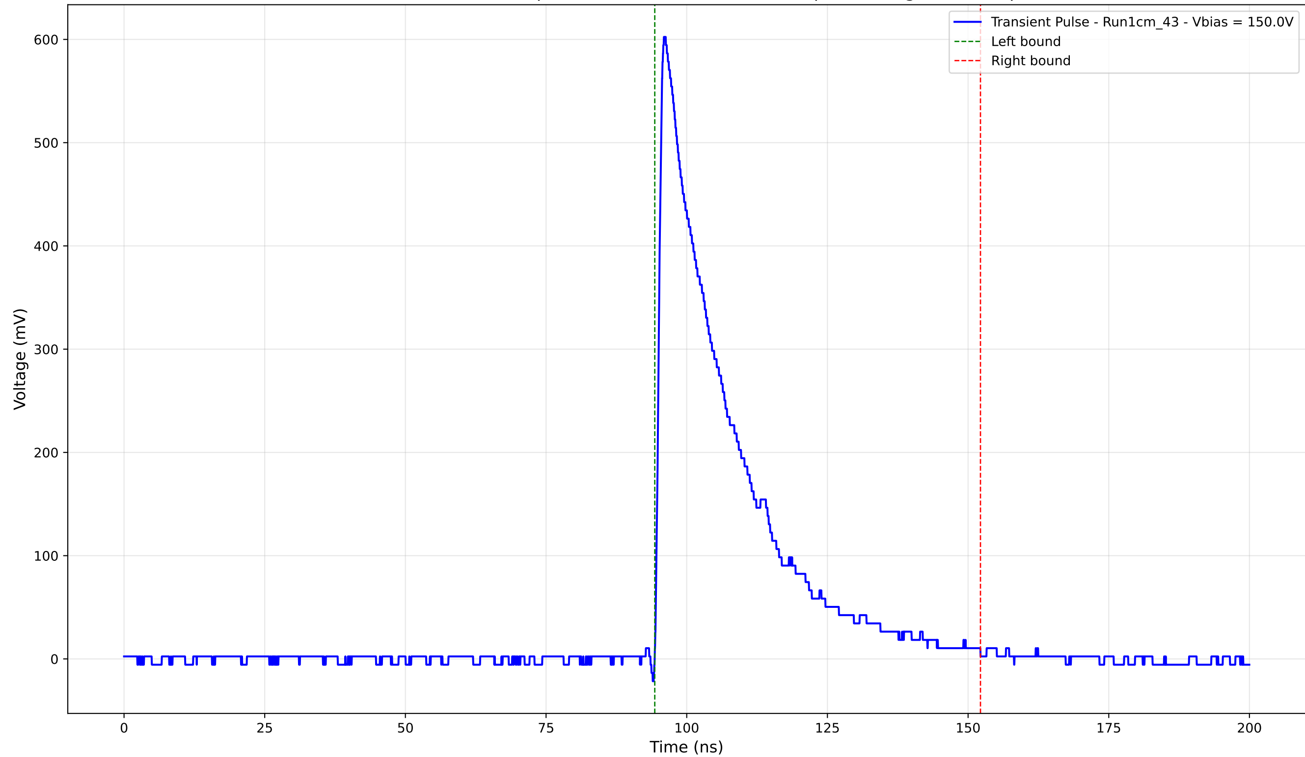
Transient Pulse - Sample: new1cm - Position: 595.0 \mu\text{m} - Charge: 159.14 pC
