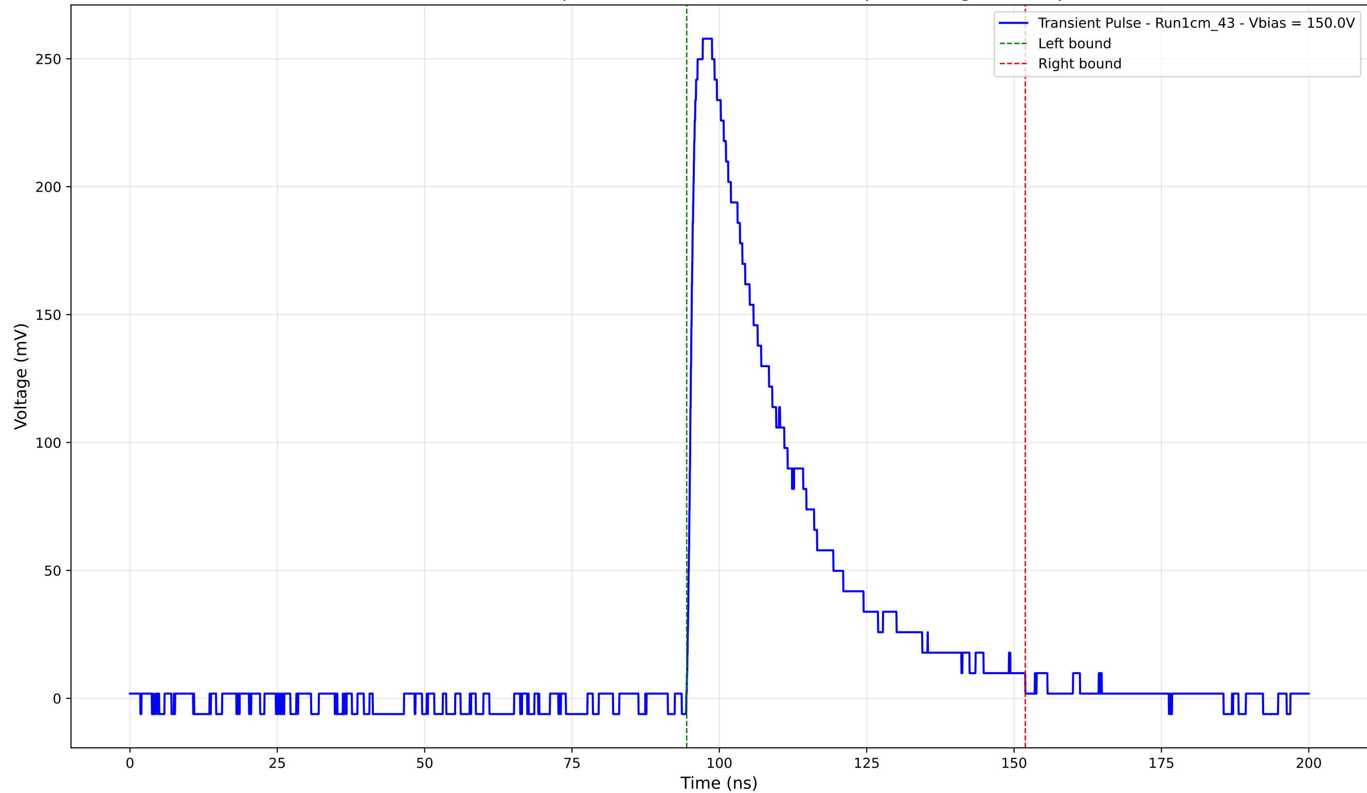
Transient Pulse - Sample: new1cm - Position: 1730.0 \mu\text{m} - Charge: 86.75 pC
