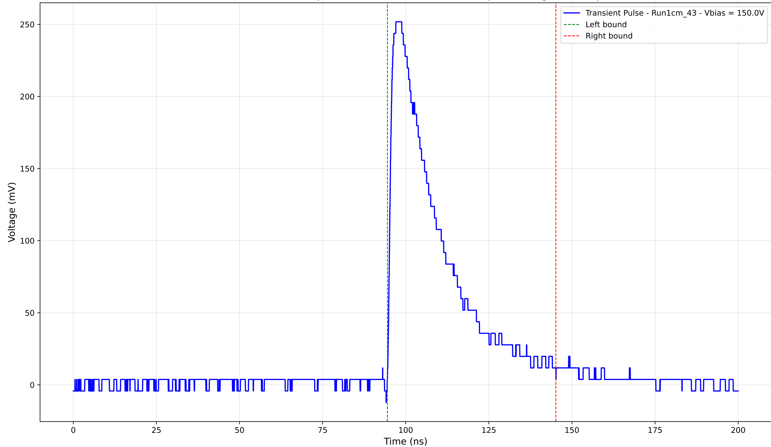
Transient Pulse - Sample: new1cm - Position: 1645.0 \mu\text{m} - Charge: 83.36 pC
