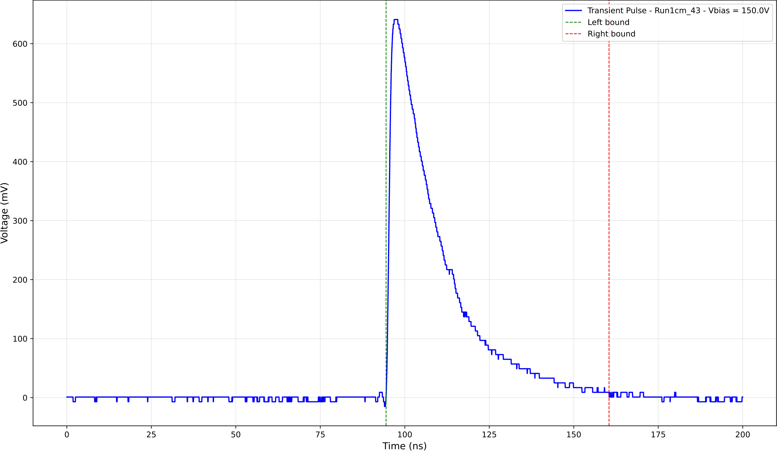
Transient Pulse - Sample: new1cm - Position: 1405.0 \mu\text{m} - Charge: 212.77 pC
