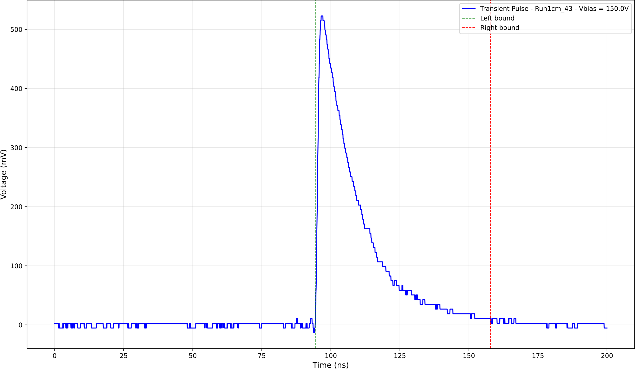
Transient Pulse - Sample: new1cm - Position: 4155.0 \mu\text{m} - Charge: 164.36 pC
