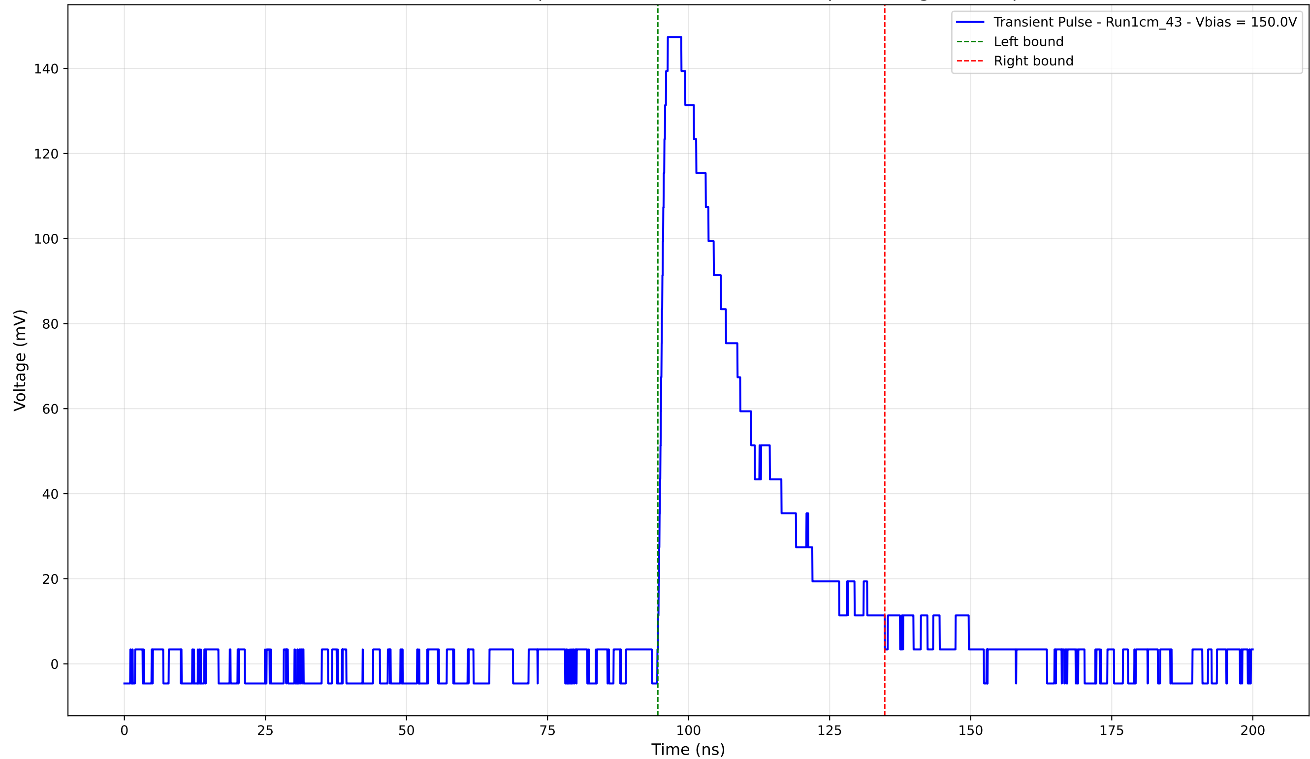
Transient Pulse - Sample: new1cm - Position: 4200.0 \mu\text{m} - Charge: 46.27 pC
