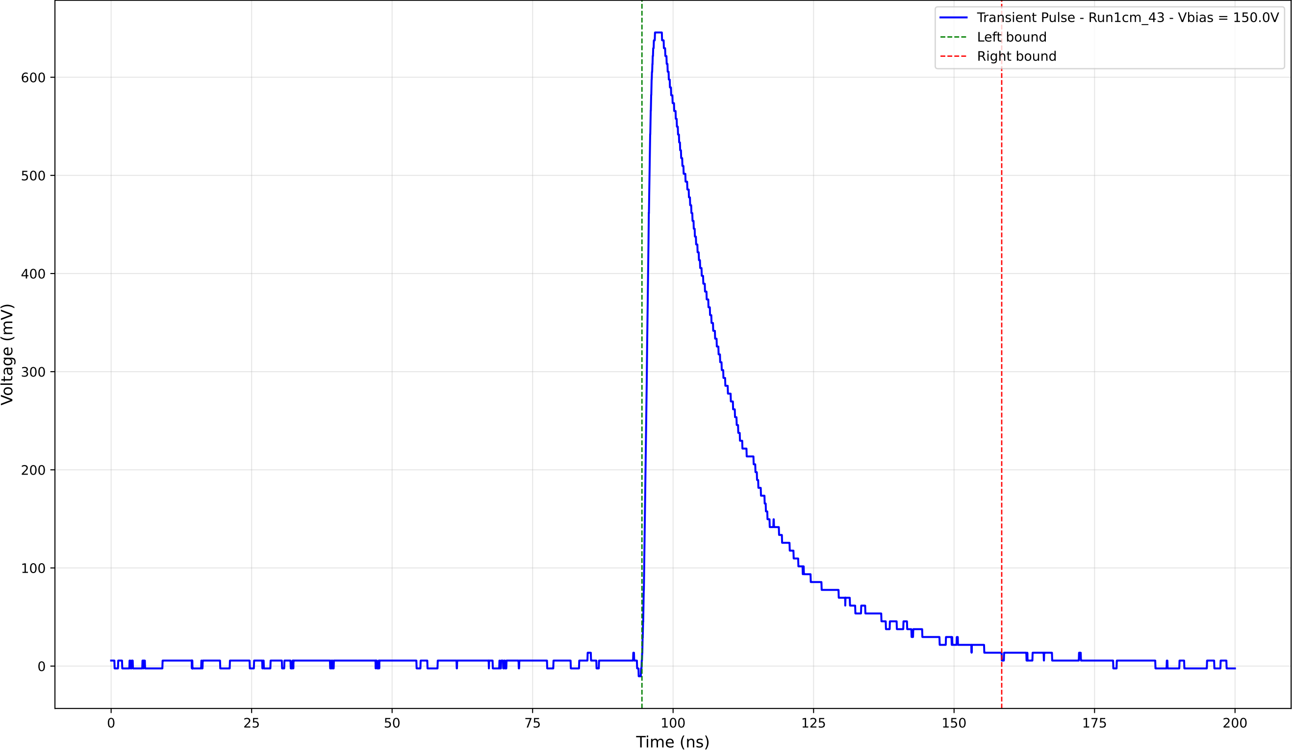
Transient Pulse - Sample: new1cm - Position: 1350.0 \mu\text{m} - Charge: 217.42 pC
