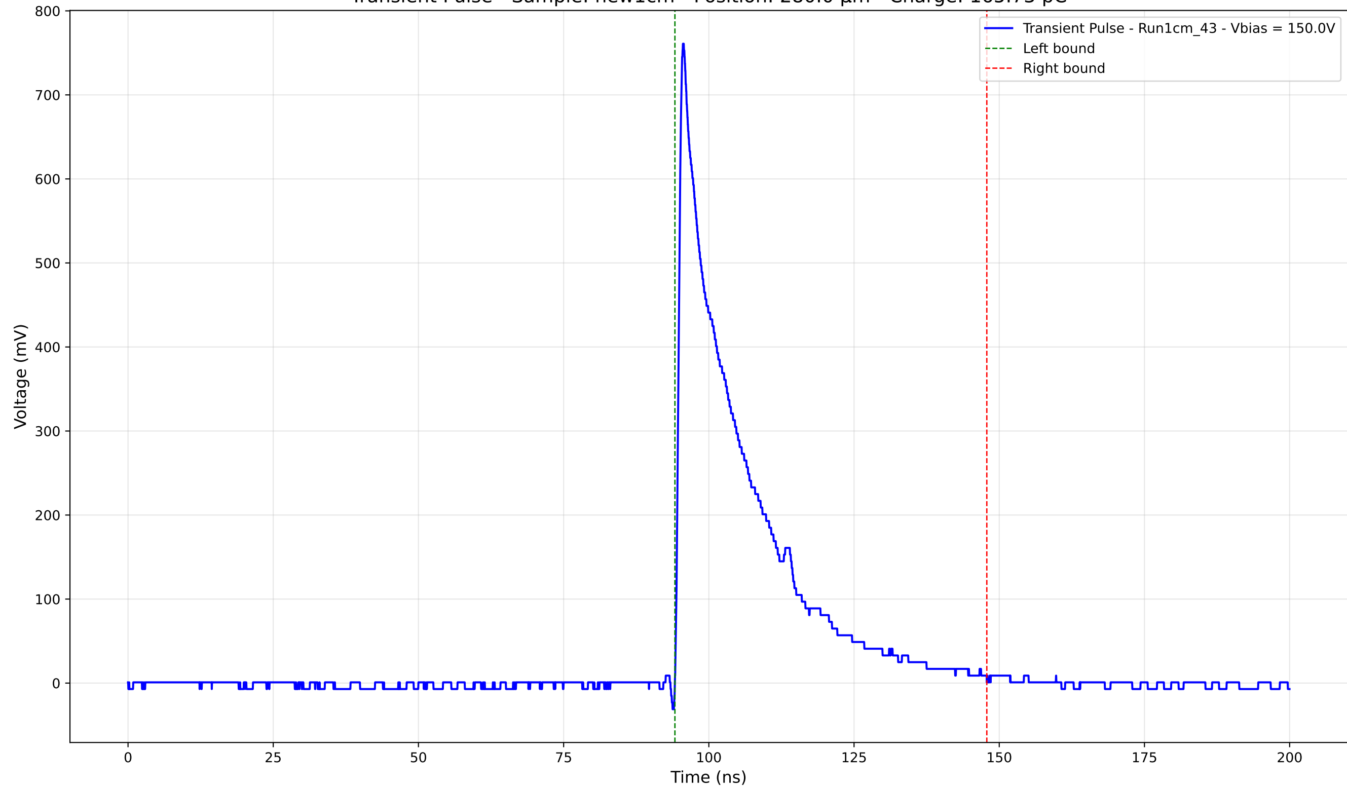
Transient Pulse - Sample: new1cm - Position: 280.0 \mu\text{m} - Charge: 165.73 pC
