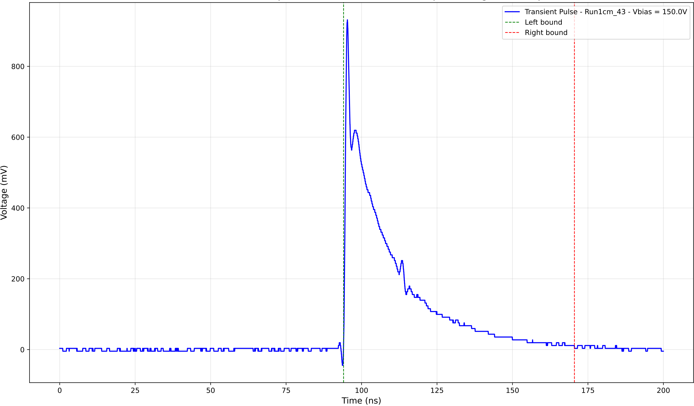
Transient Pulse - Sample: new1cm - Position: 2560.0 \mu\text{m} - Charge: 235.97 pC
