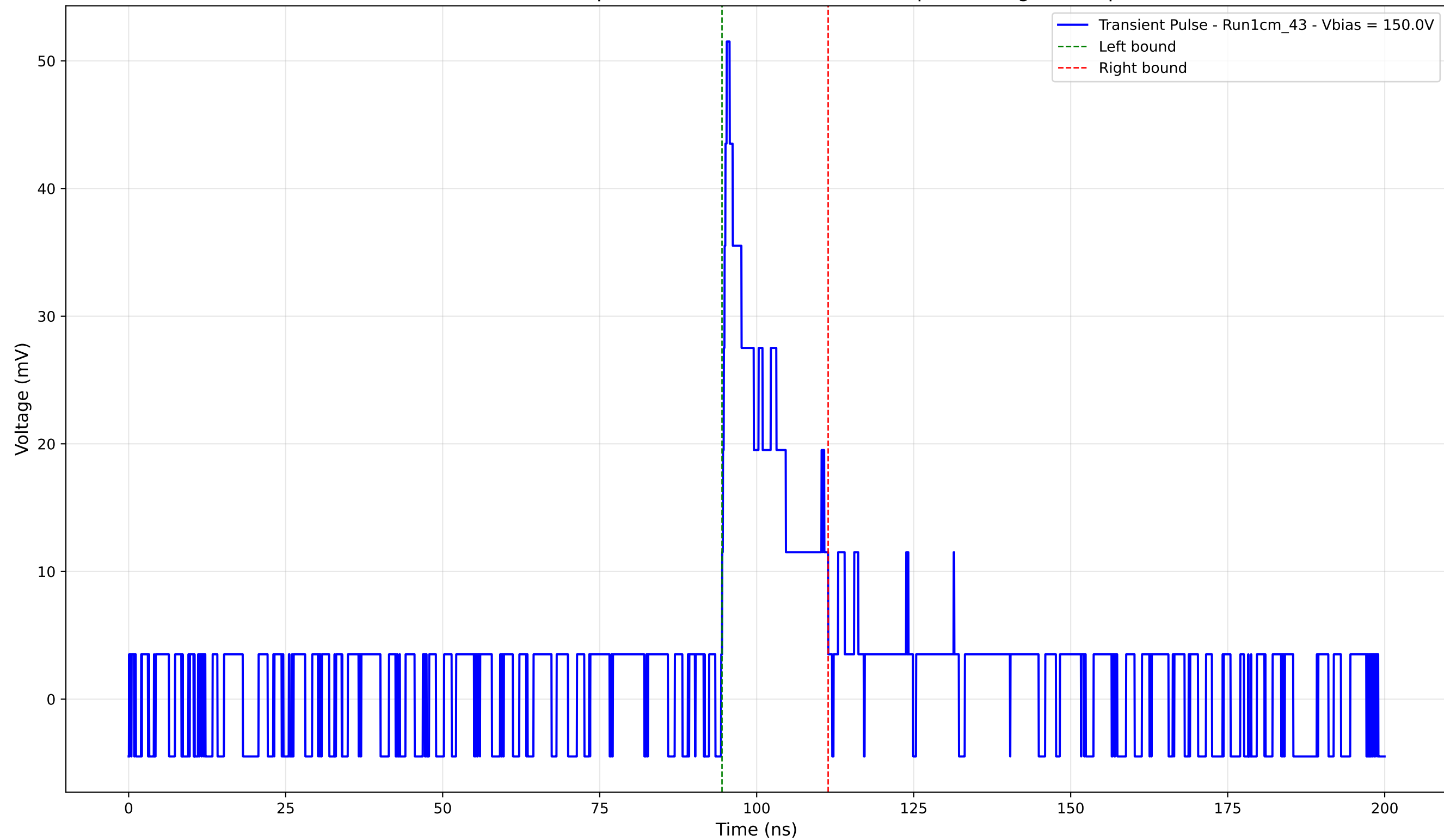
Transient Pulse - Sample: new1cm -Position: 5055.0 \mu\text{m} - Charge: 7.25 pC
