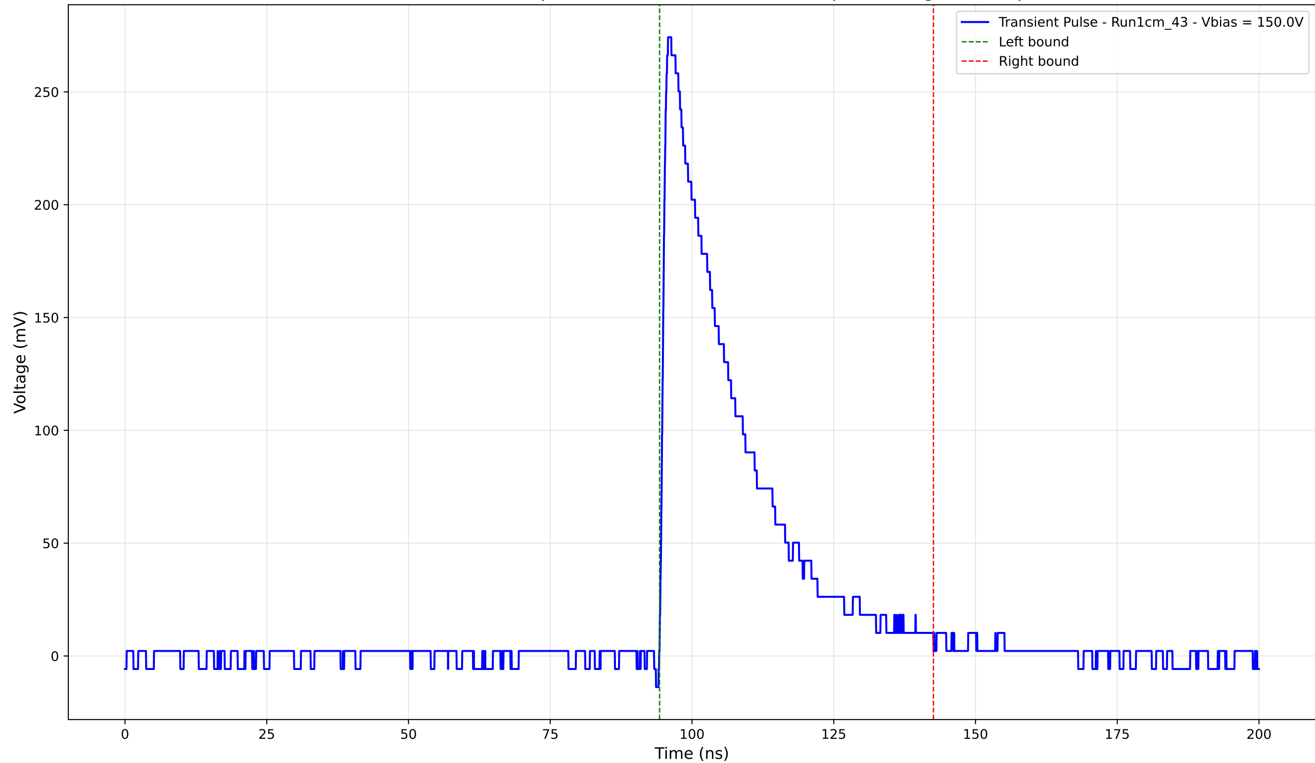
Transient Pulse - Sample: new1cm - Position: 4685.0 \mu\text{m} - Charge: 75.18 pC
