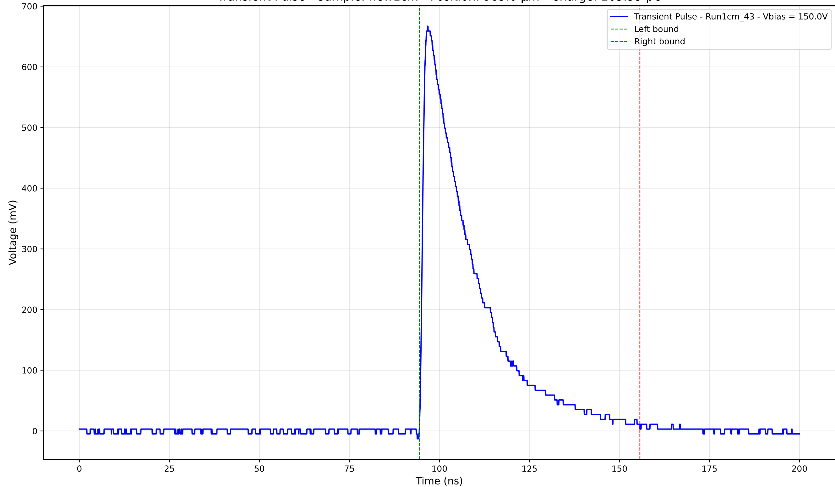
Transient Pulse - Sample: new1cm - Position: 985.0 \mu\text{m} - Charge: 205.55 pC
