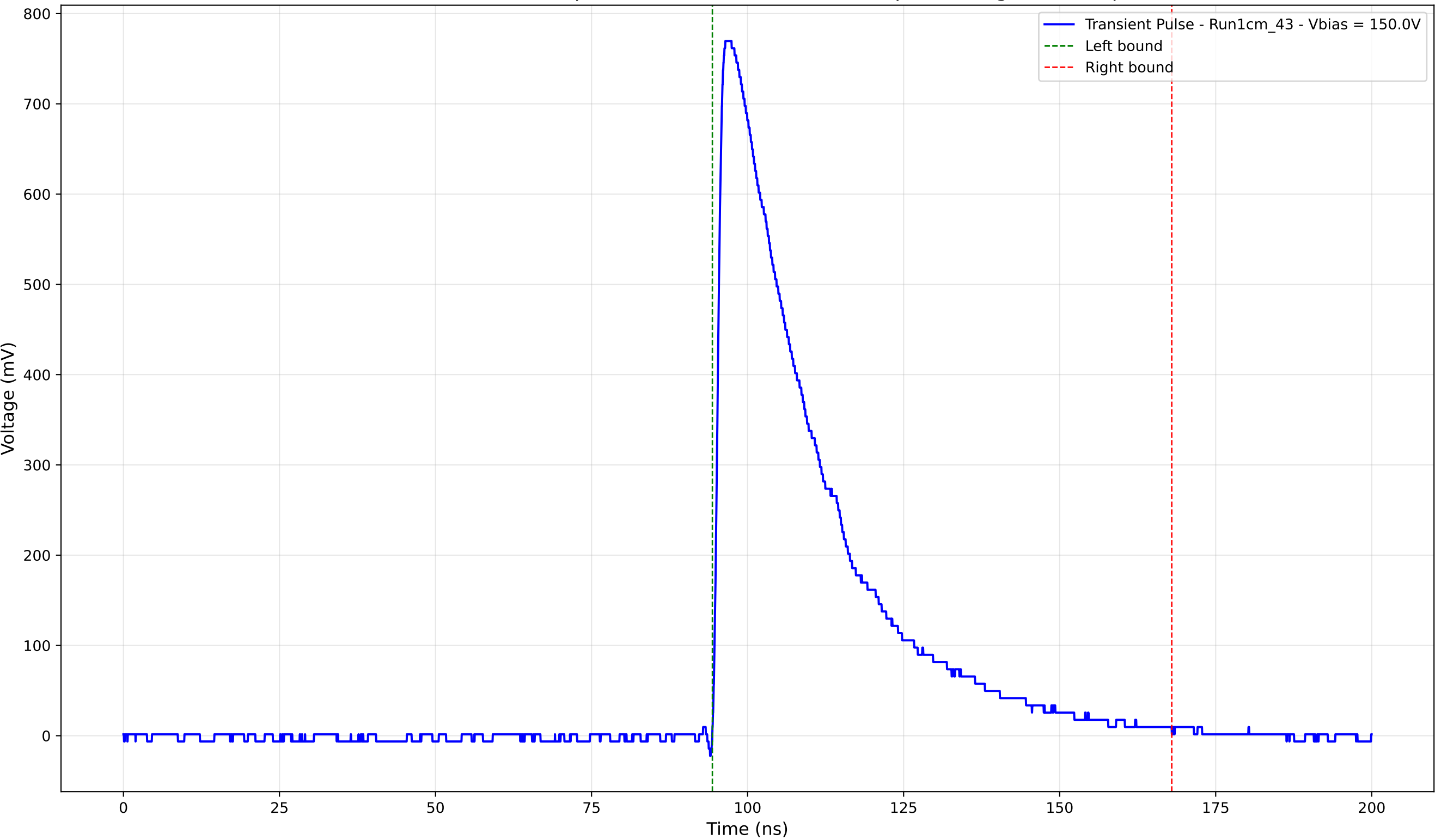
Transient Pulse - Sample: new1cm - Position: 3860.0 \mu\text{m} - Charge: 266.39 pC
