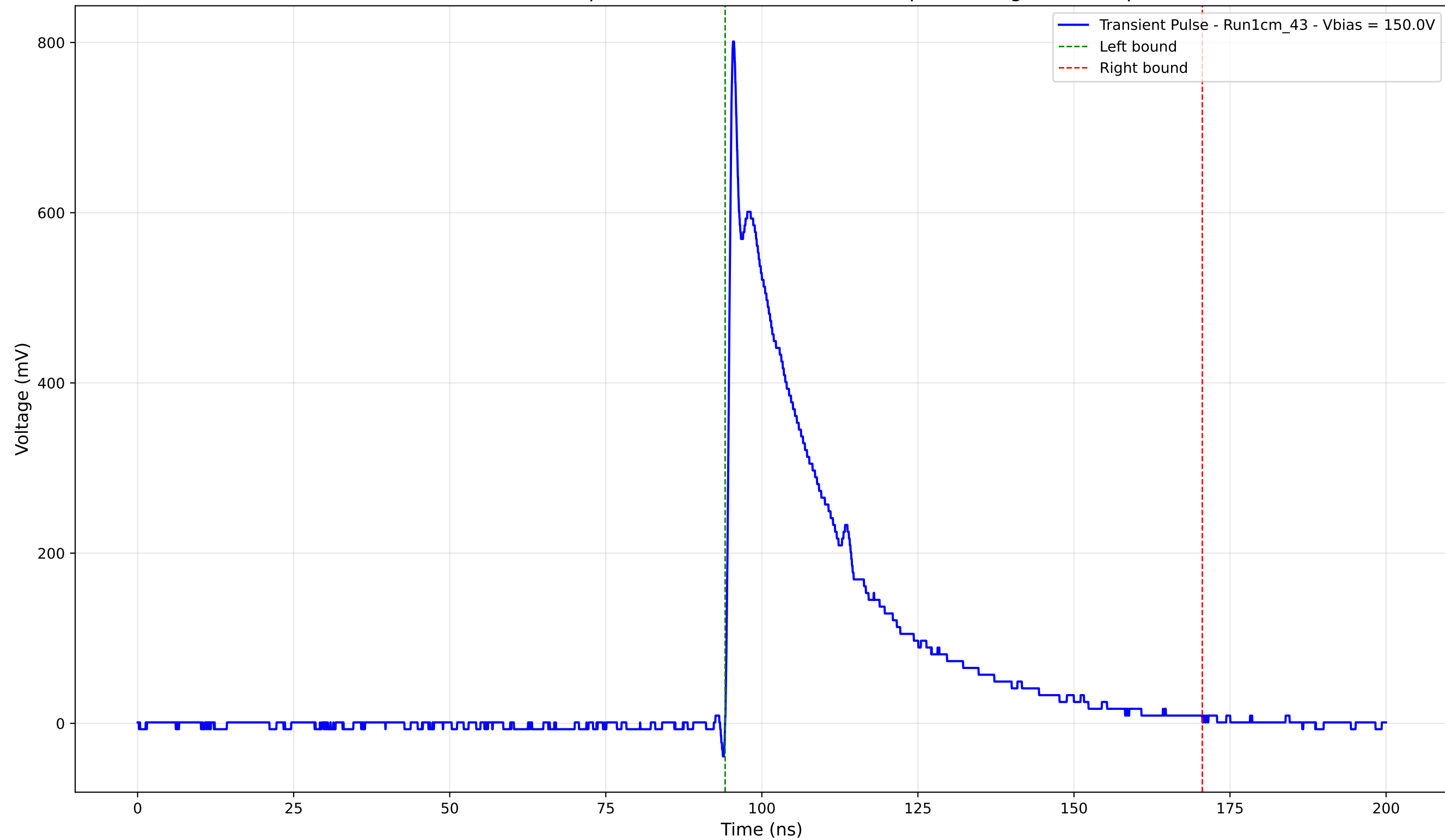
Transient Pulse - Sample: new1cm - Position: 2355.0 \mu\text{m} - Charge: 224.92 pC
