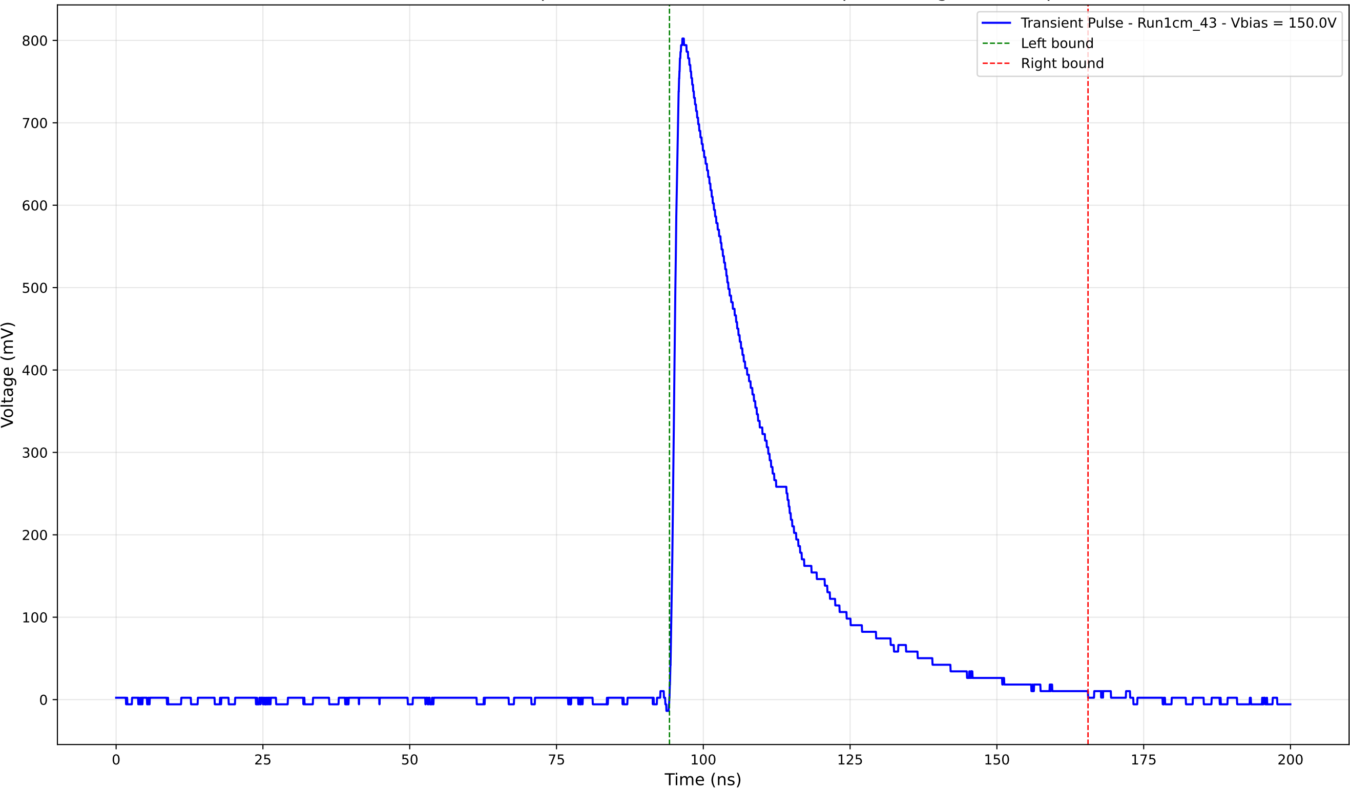
Transient Pulse - Sample: new1cm - Position: 4370.0 \mu\text{m} - Charge: 258.80 pC
