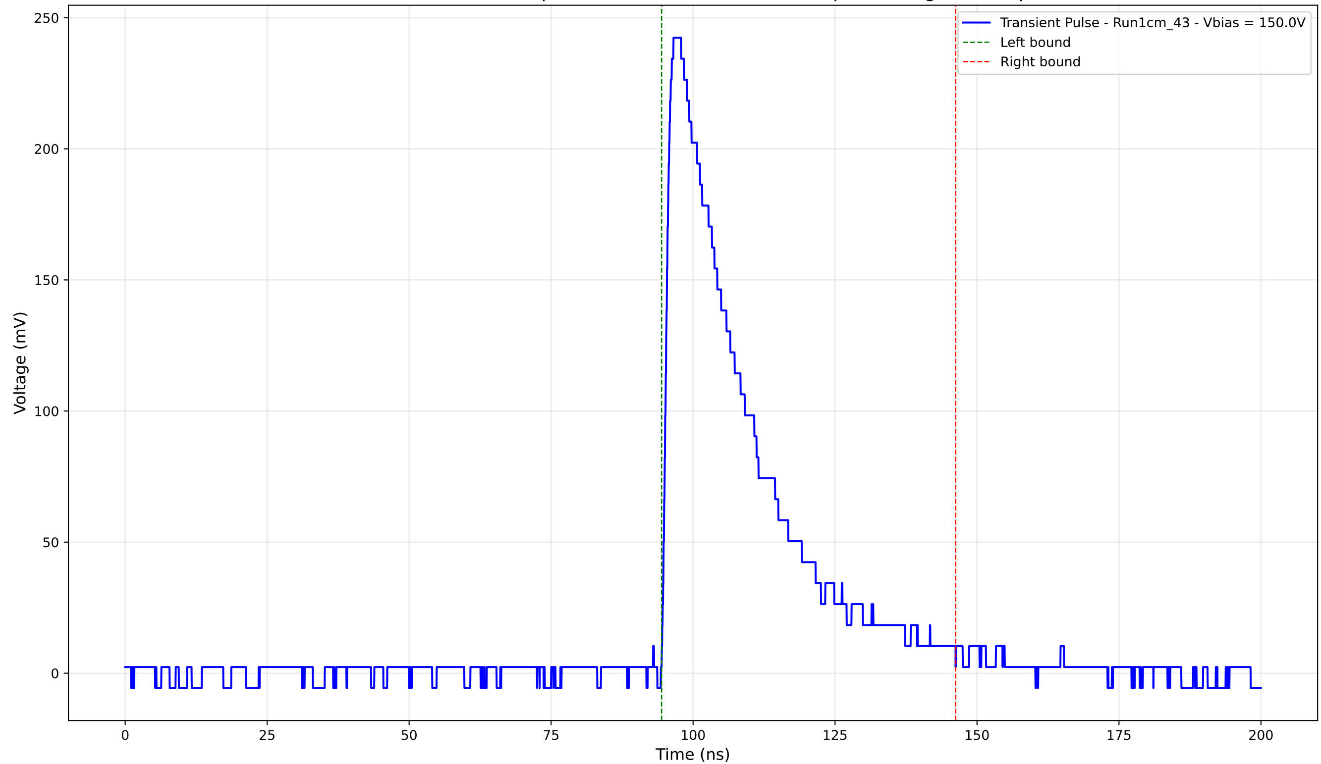
Transient Pulse - Sample: new1cm - Position: 4185.0 \mu\text{m} - Charge: 74.99 pC
