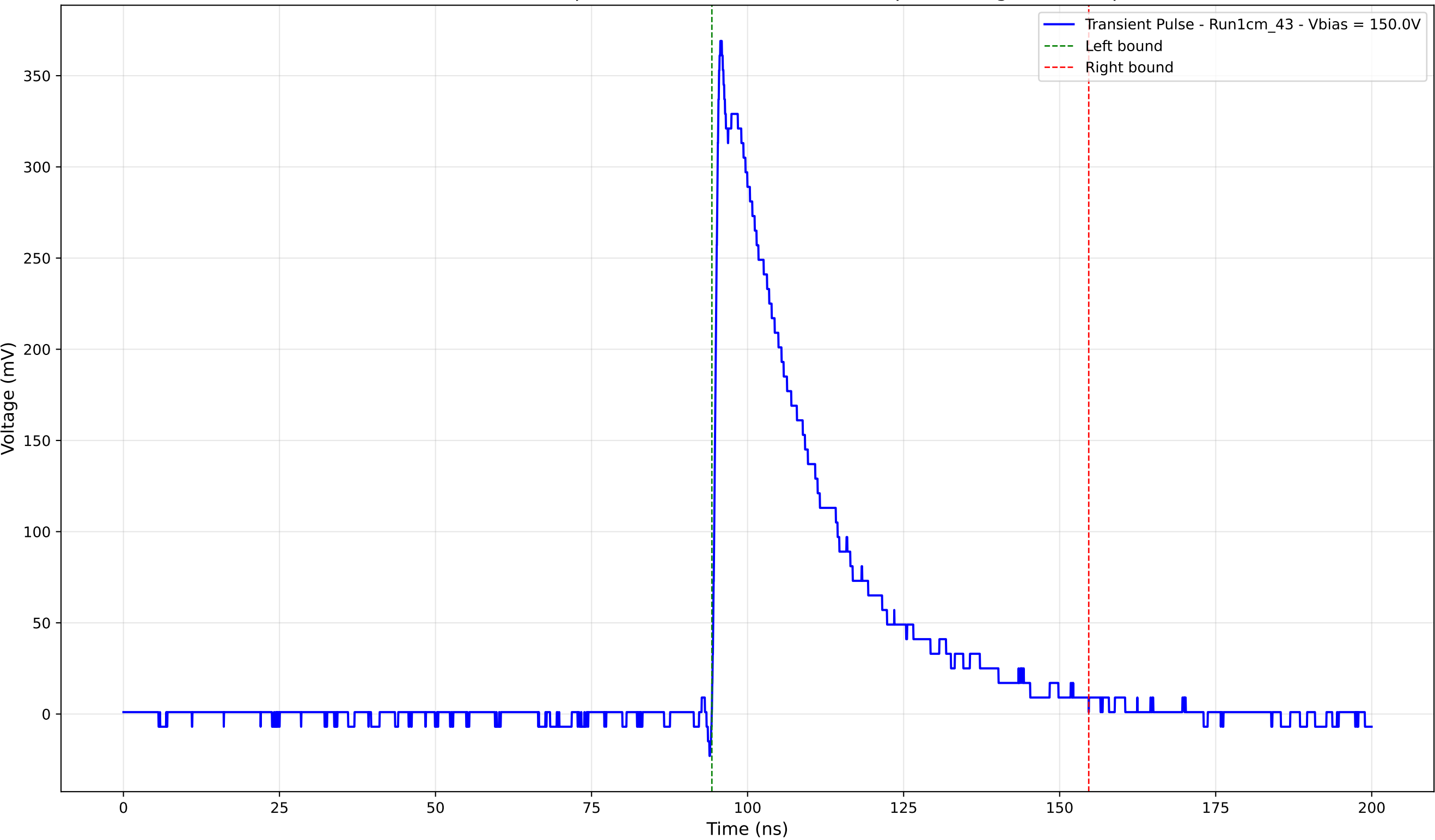
Transient Pulse - Sample: new1cm - Position: 2130.0 \mu\text{m} - Charge: 114.35 pC
