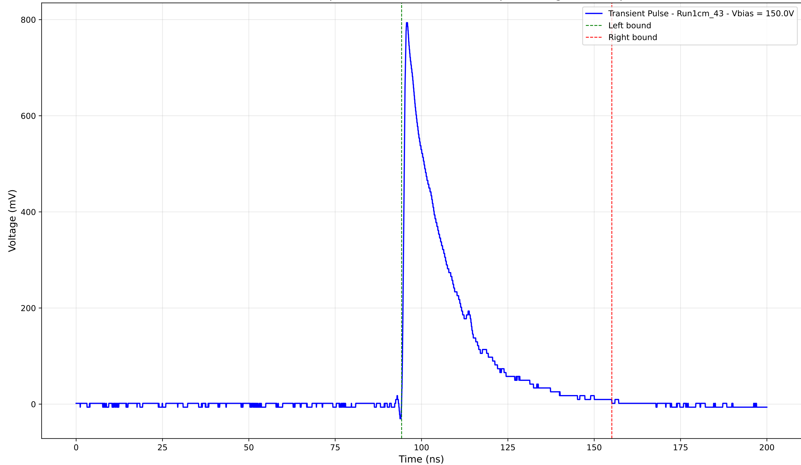
Transient Pulse - Sample: new1cm - Position: 420.0 \mu\text{m} - Charge: 196.86 pC
