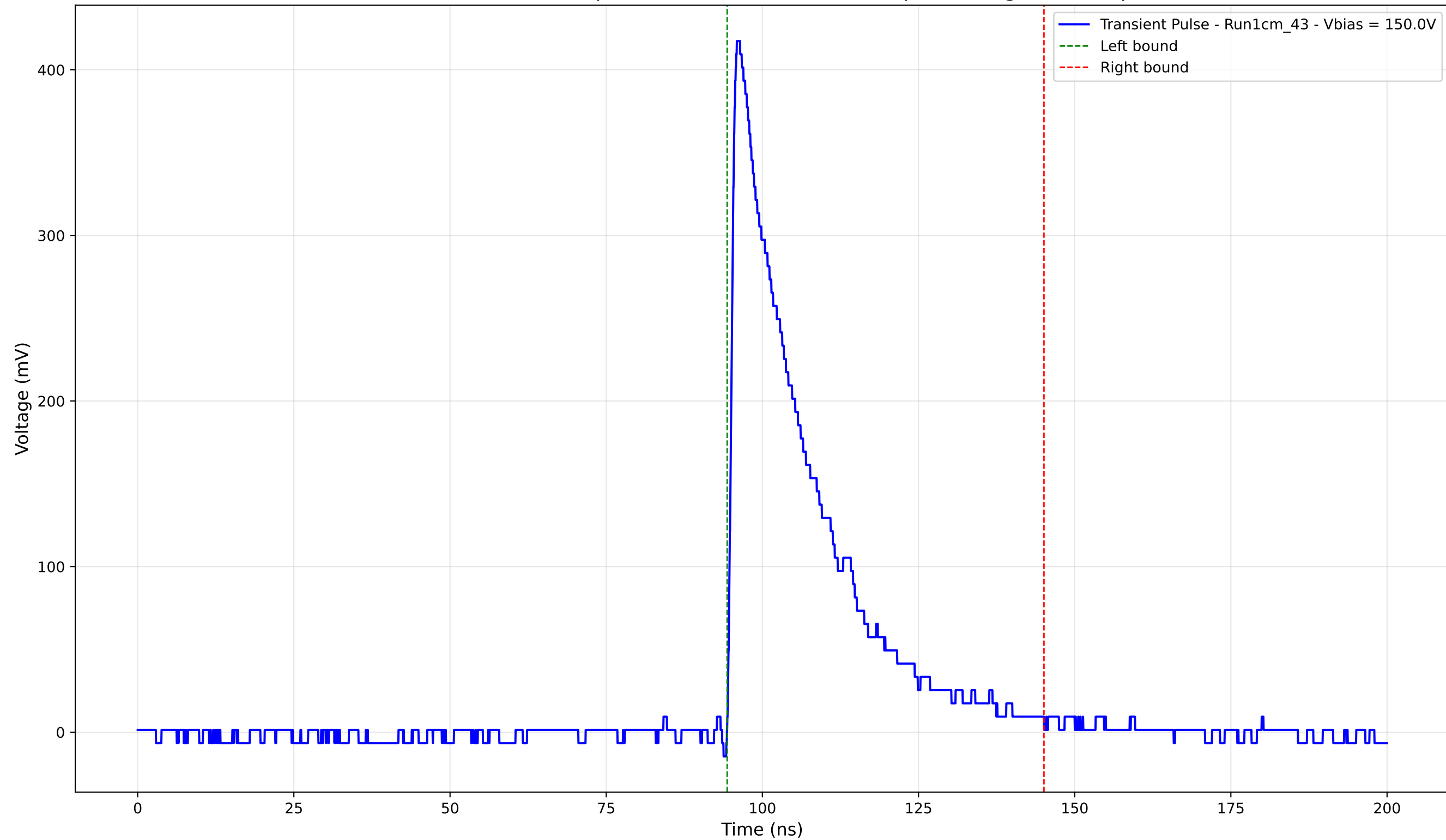
Transient Pulse - Sample: new1cm - Position: 620.0 \mu\text{m} - Charge: 106.50 pC
