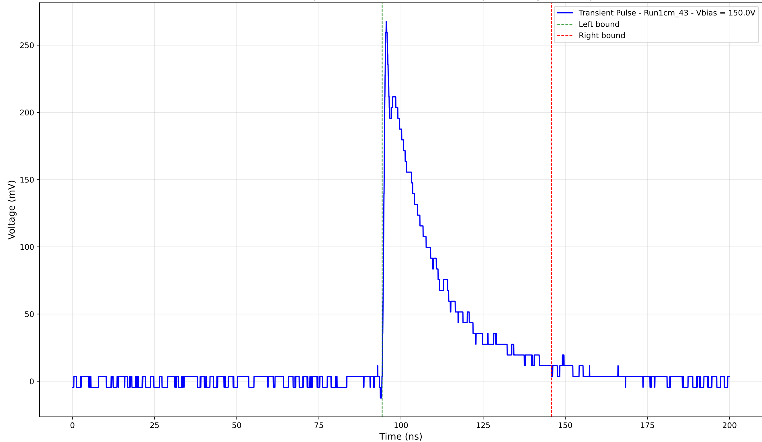
Transient Pulse - Sample: new1cm - Position: 2225.0 \mu\text{m} - Charge: 73.93 pC
