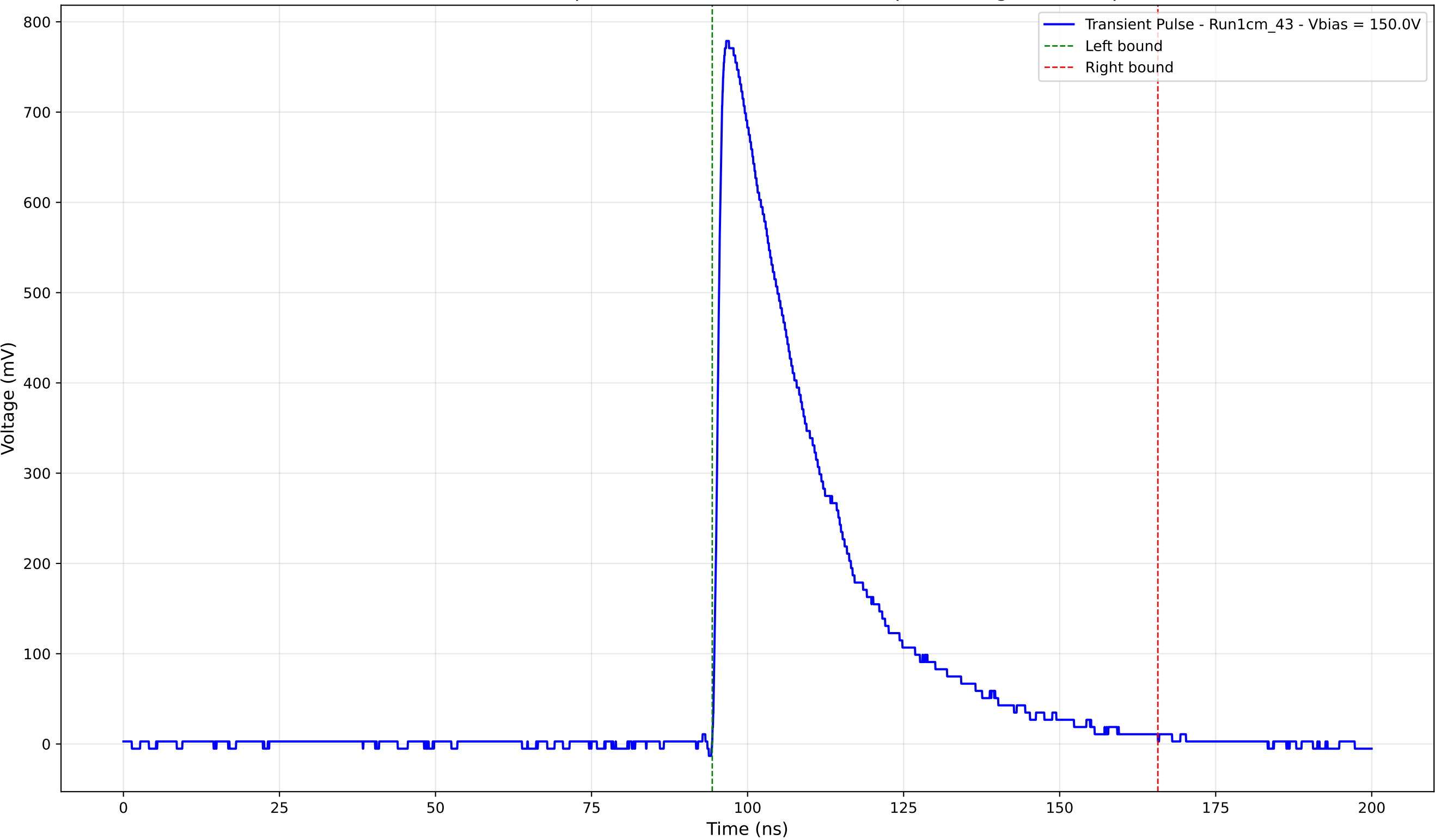
Transient Pulse - Sample: new1cm - Position: 3910.0 \mu\text{m} - Charge: 267.66 pC
