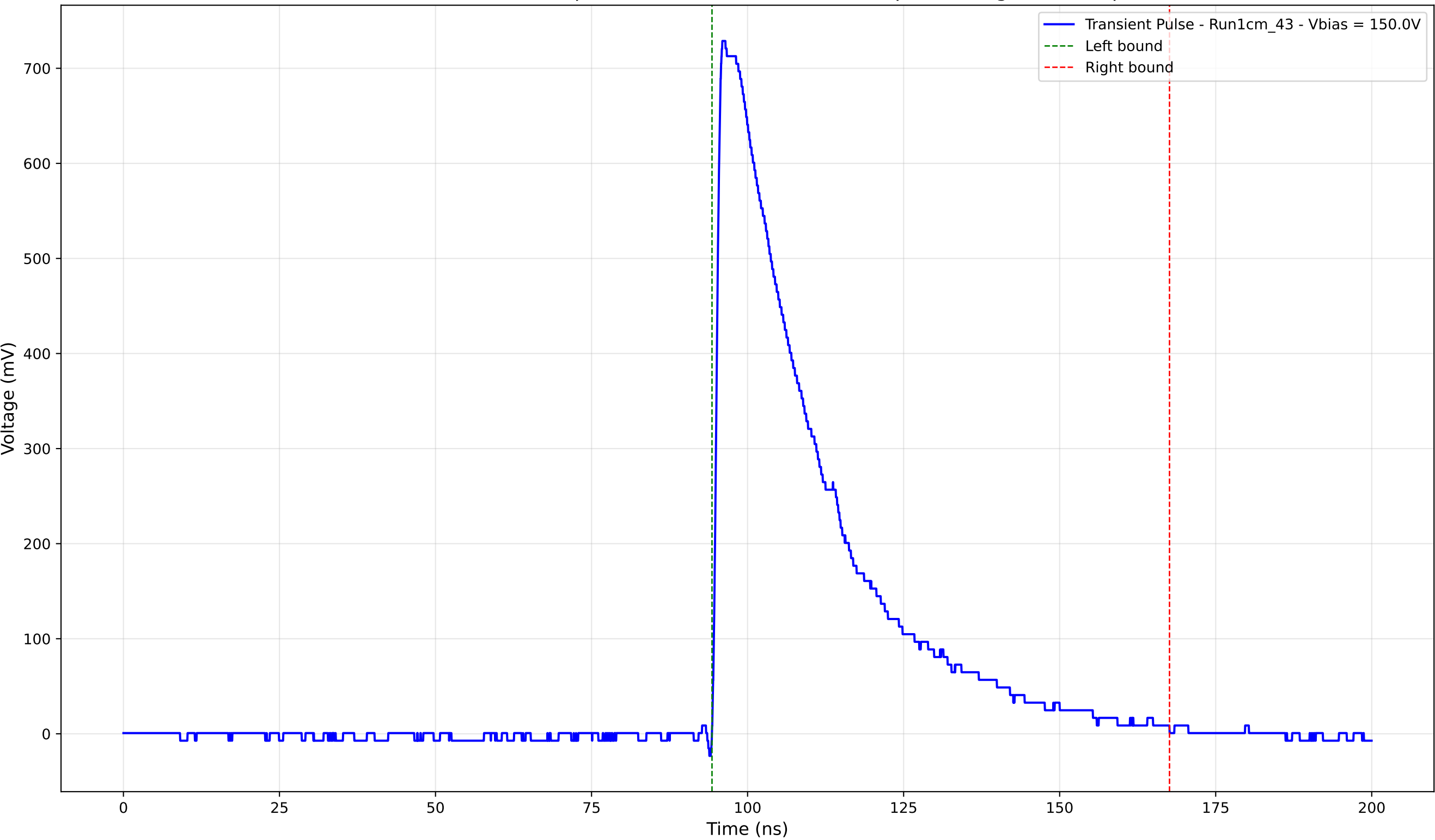
Transient Pulse - Sample: new1cm - Position: 3505.0 \mu\text{m} - Charge: 256.83 pC
