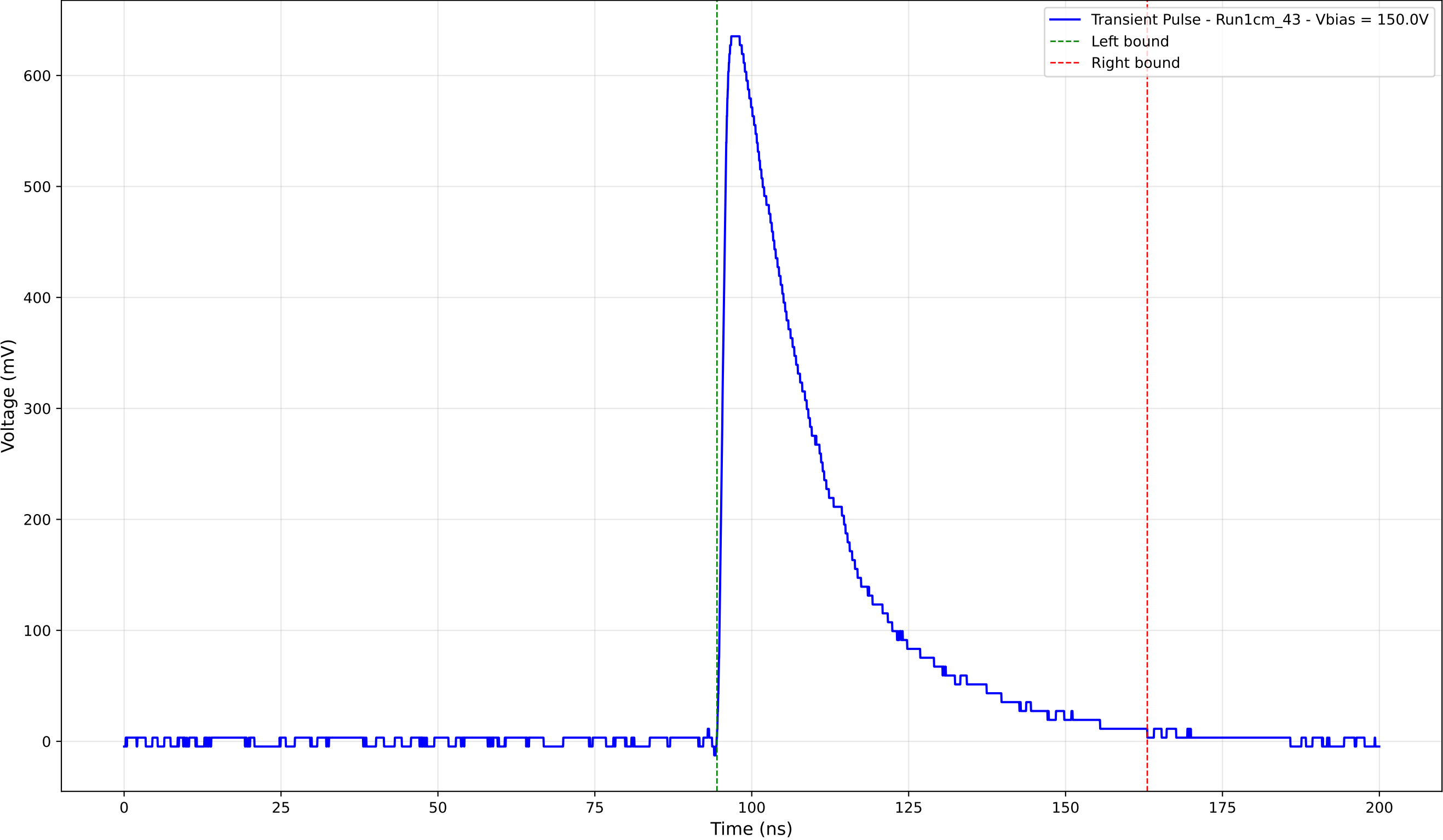
Transient Pulse - Sample: new1cm - Position: 1420.0 \mu\text{m} - Charge: 214.79 pC
