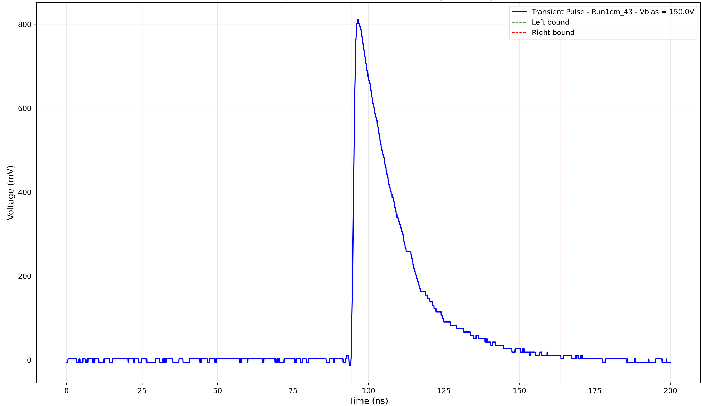
Transient Pulse - Sample: new1cm - Position: 4400.0 \mu\text{m} - Charge: 260.29 pC
