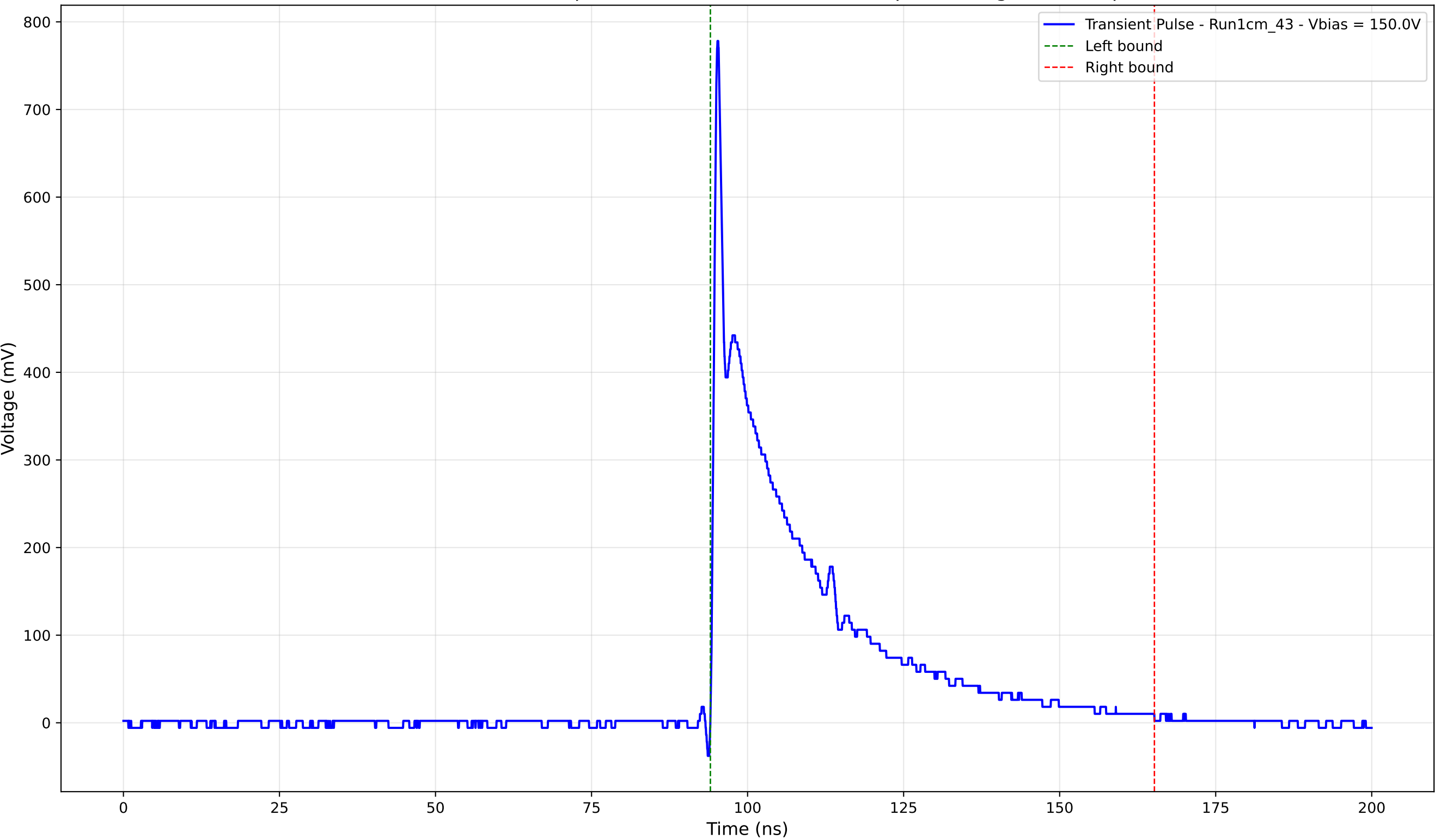
Transient Pulse - Sample: new1cm - Position: 2630.0 \mu\text{m} - Charge: 164.42 pC
