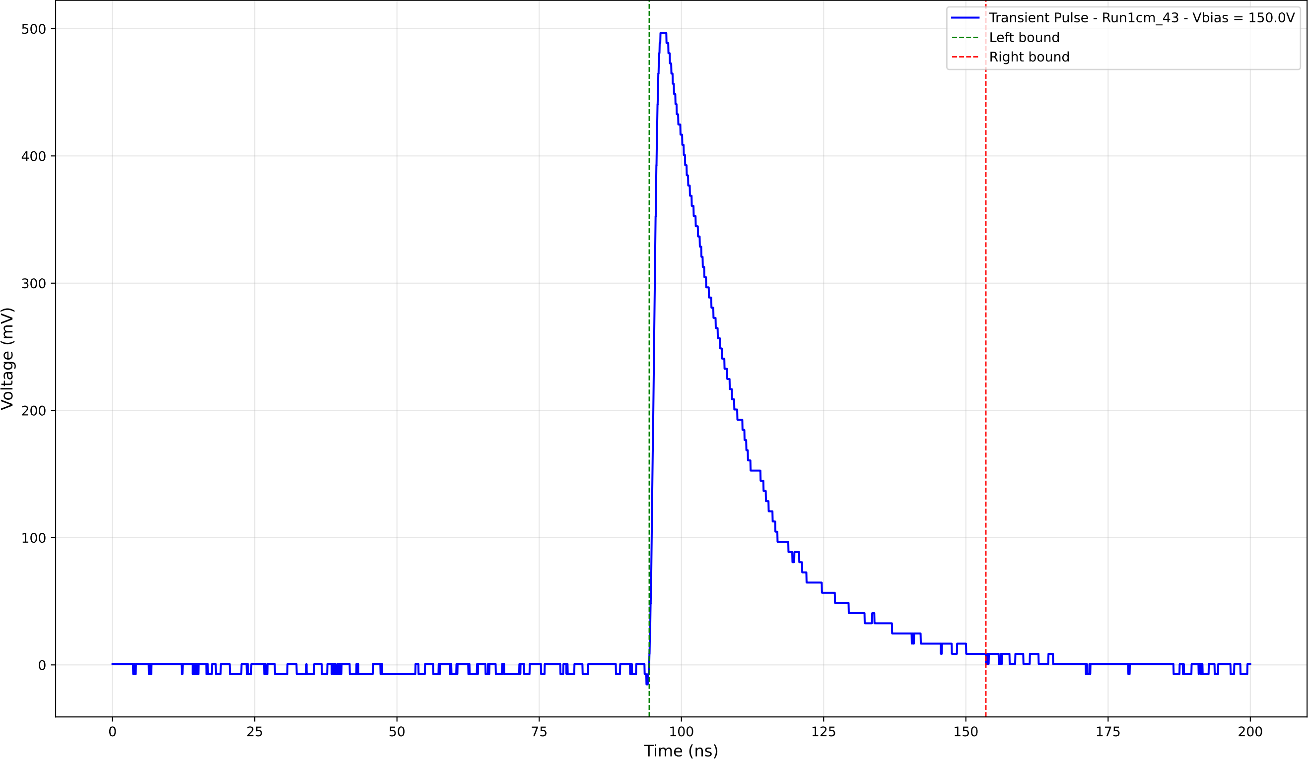
Transient Pulse - Sample: new1cm - Position: 4275.0 \mu\text{m} - Charge: 153.09 pC
