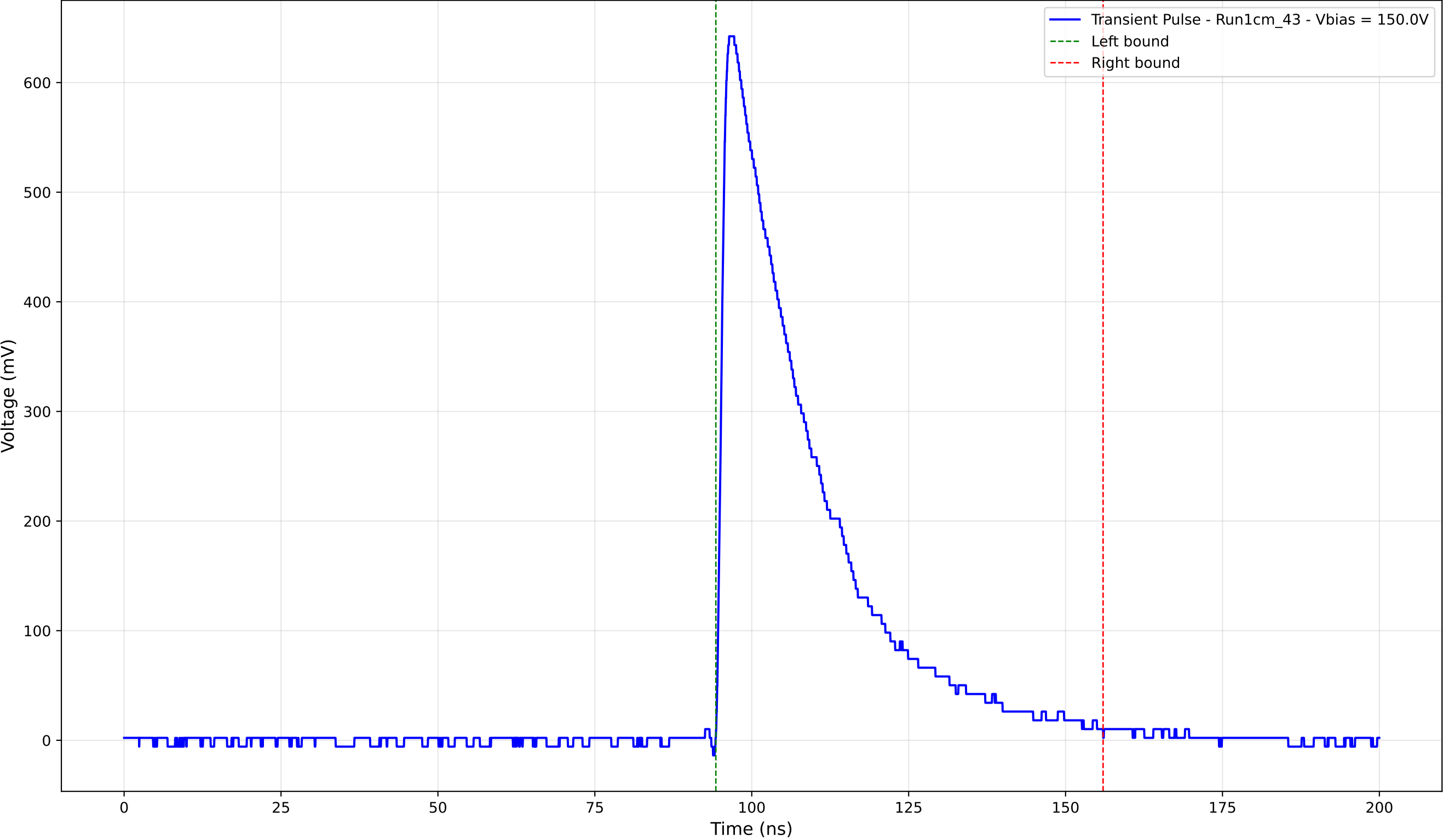
Transient Pulse - Sample: new1cm - Position: 4295.0 \mu\text{m} - Charge: 202.00 pC
