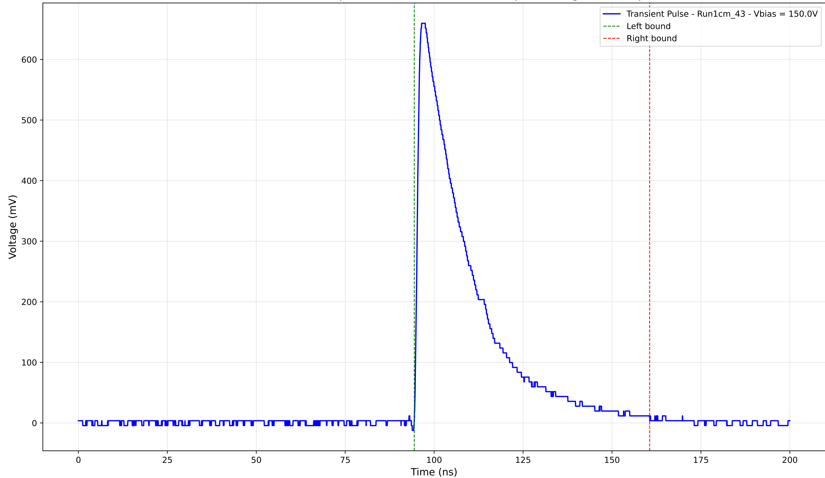
Transient Pulse - Sample: new1cm - Position: 955.0 \mu\text{m} - Charge: 206.85 pC
