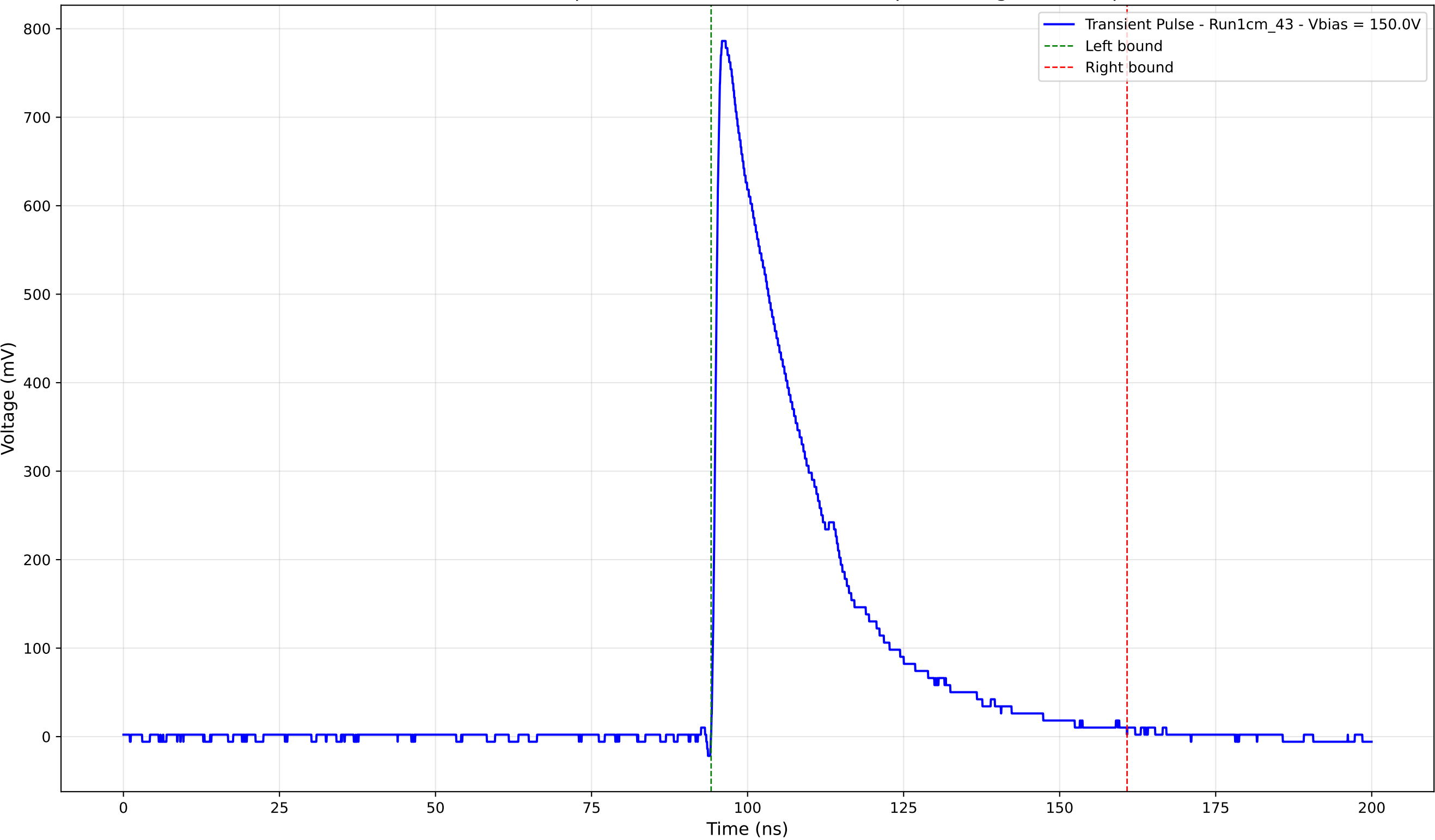
Transient Pulse - Sample: new1cm - Position: 4590.0 \mu\text{m} - Charge: 240.12 pC
