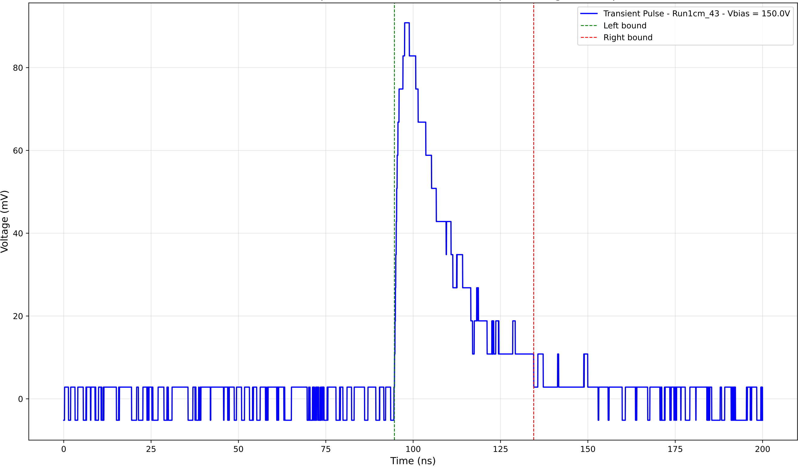
Transient Pulse - Sample: new1cm - Position: 1690.0 \mu\text{m} - Charge: 28.29 pC
