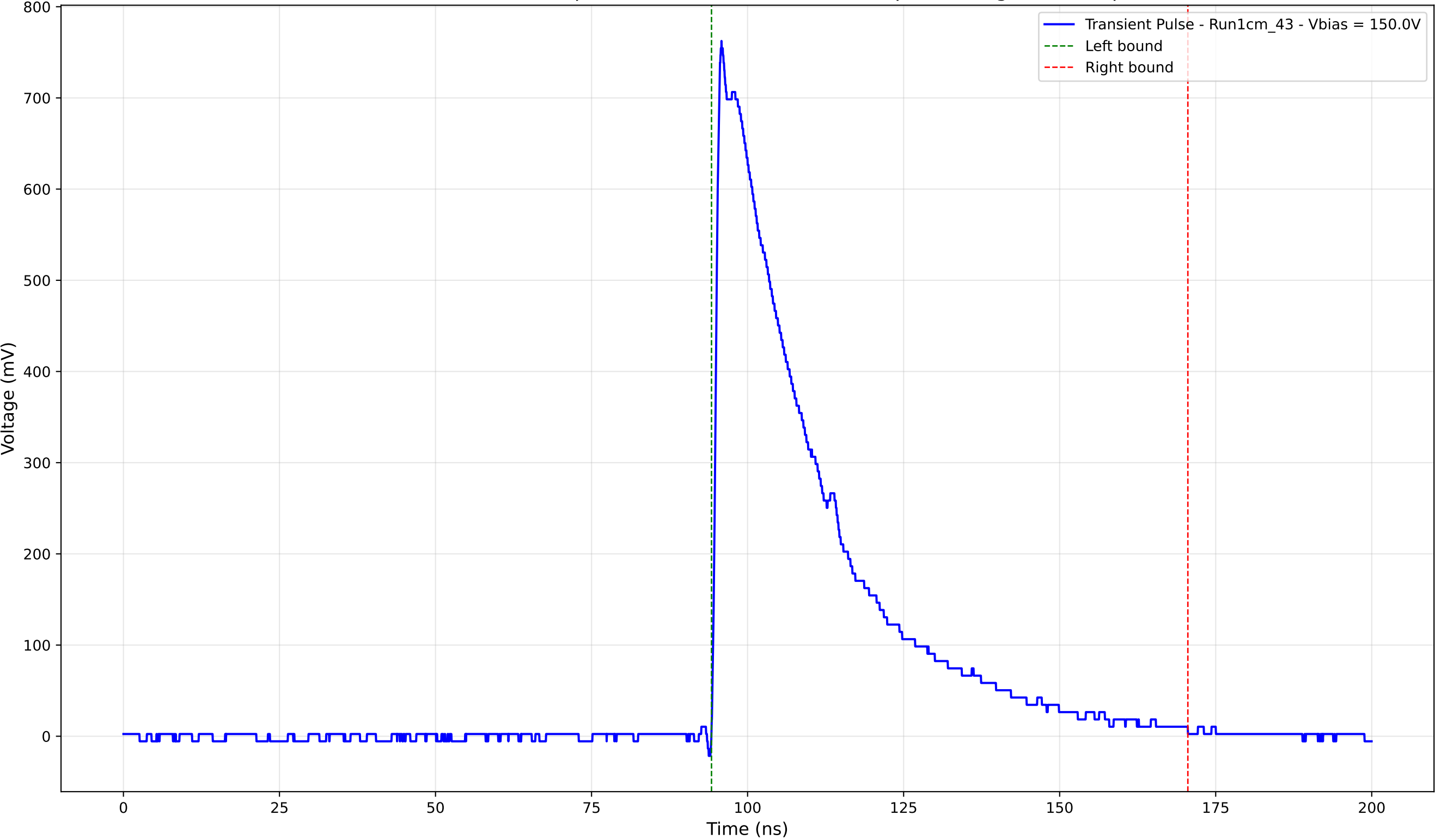
Transient Pulse - Sample: new1cm - Position: 3345.0 \mu\text{m} - Charge: 259.91 pC
