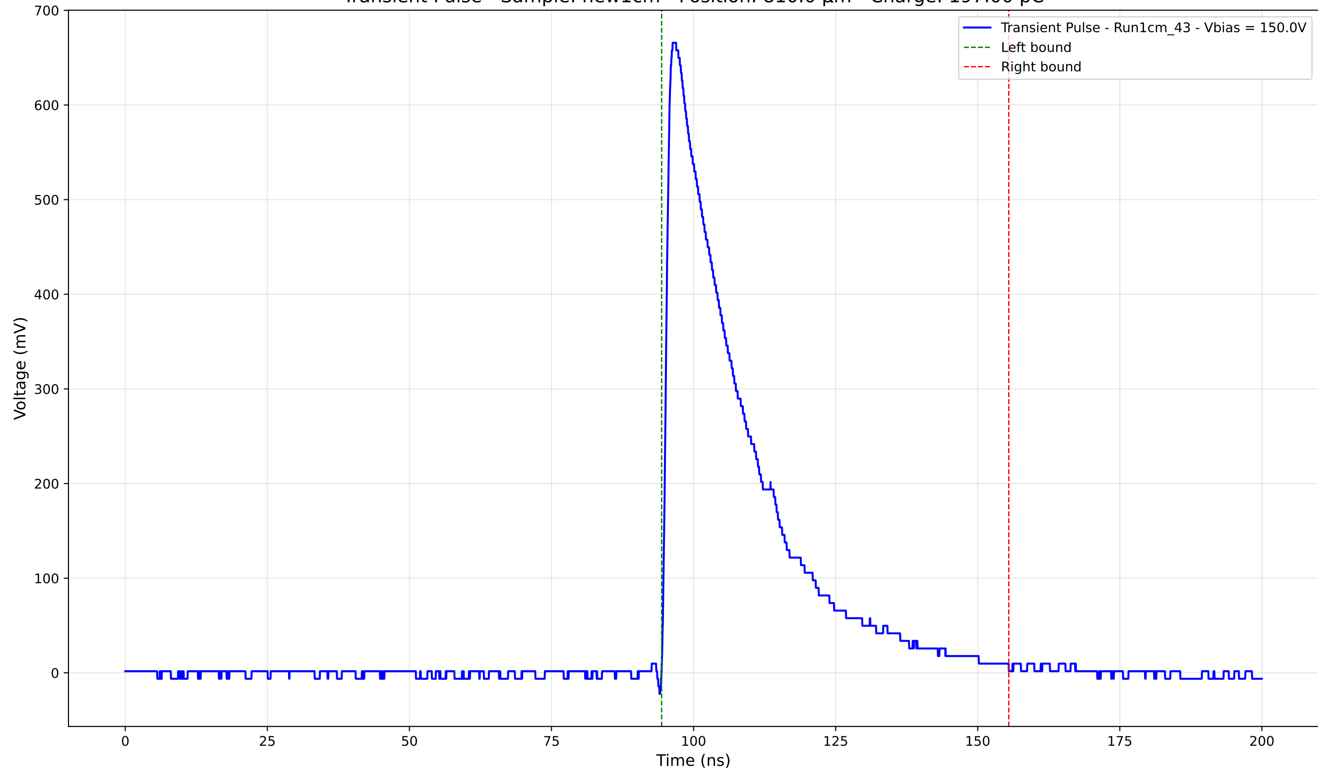
Transient Pulse - Sample: new1cm - Position: 810.0 \mu\text{m} - Charge: 197.00 pC
