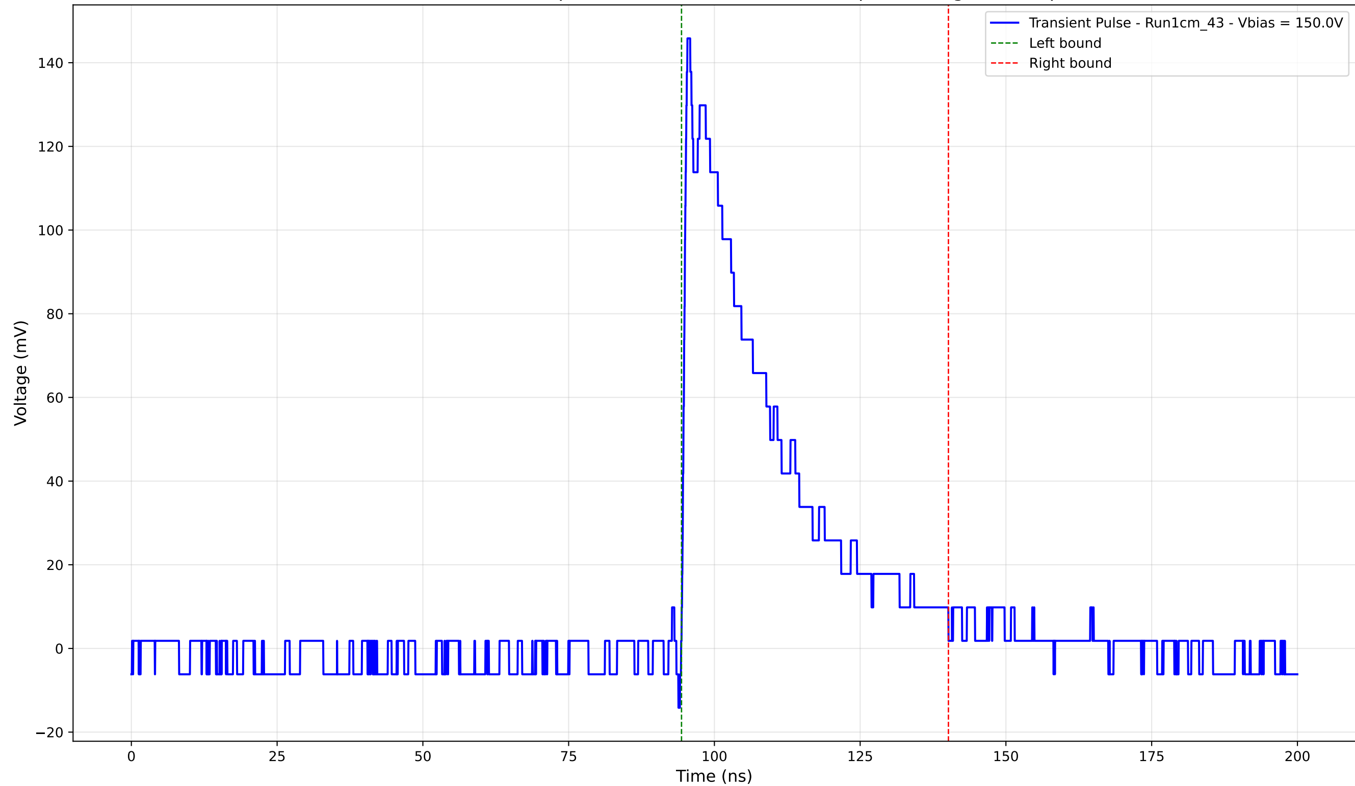
Transient Pulse - Sample: new1cm - Position: 3195.0 \mu\text{m} - Charge: 43.07 pC
