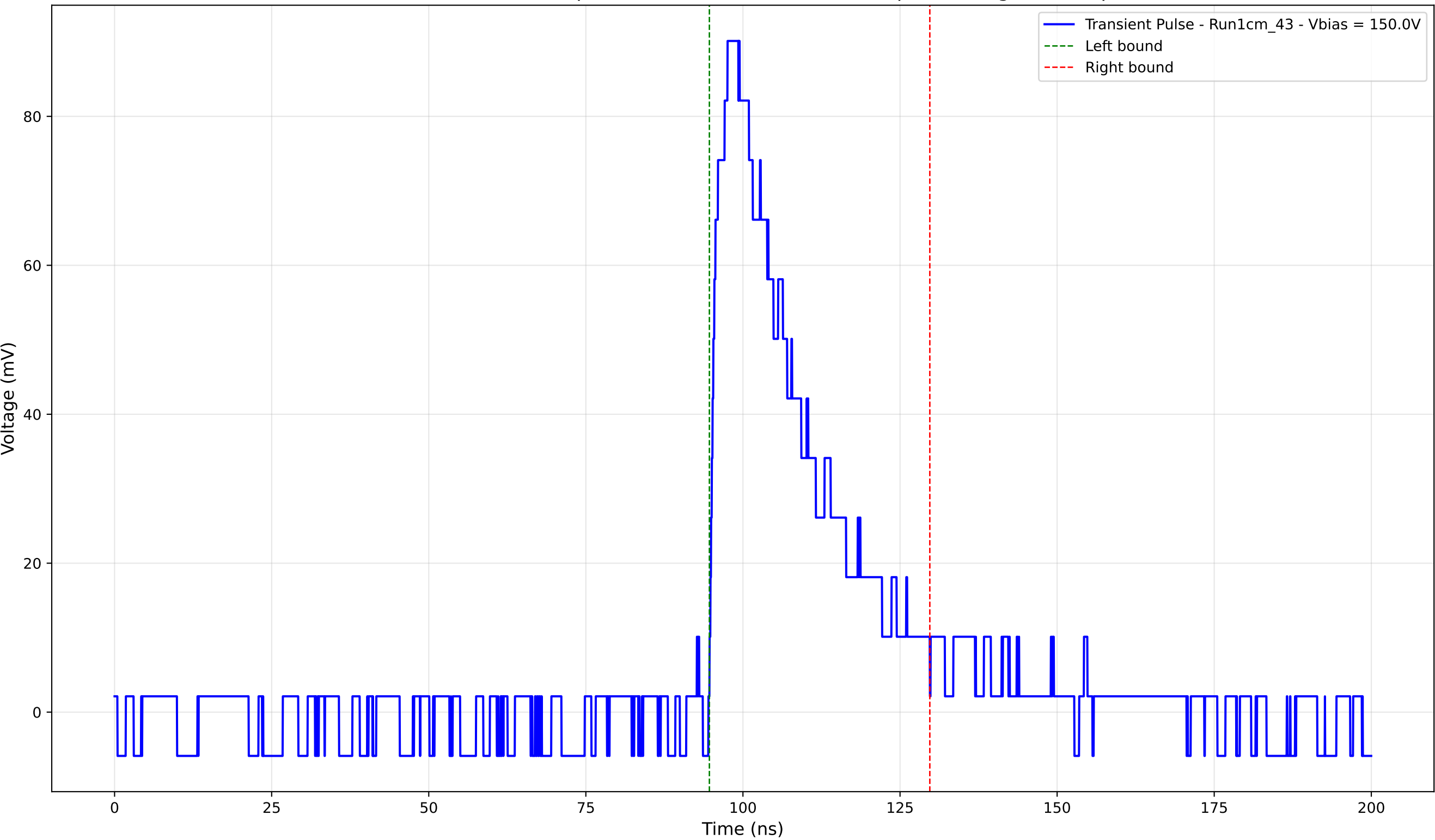
Transient Pulse - Sample: new1cm - Position: 1685.0 \mu\text{m} - Charge: 26.90 pC
