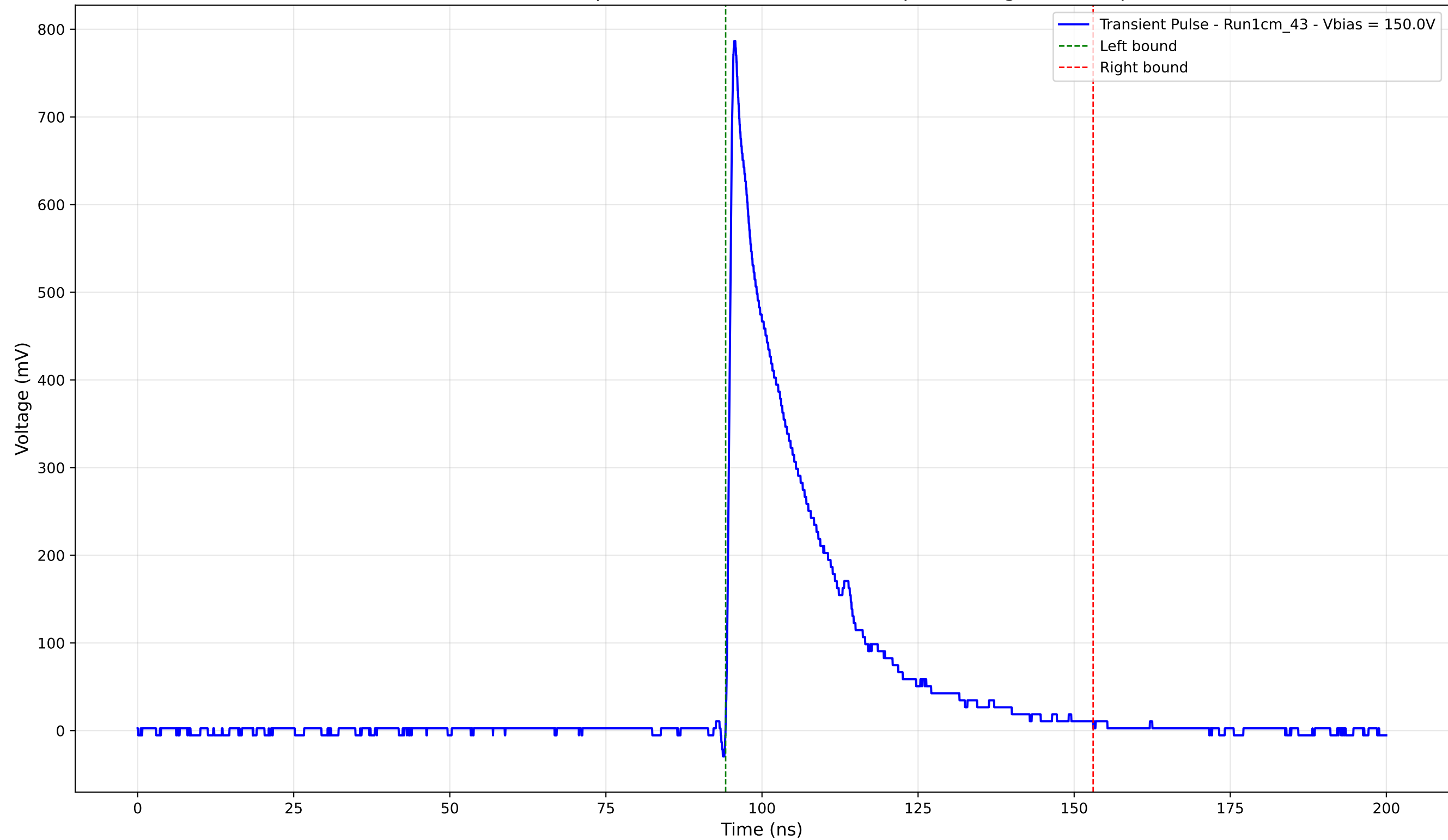
Transient Pulse - Sample: new1cm - Position: 300.0 \mu\text{m} - Charge: 178.02 pC
