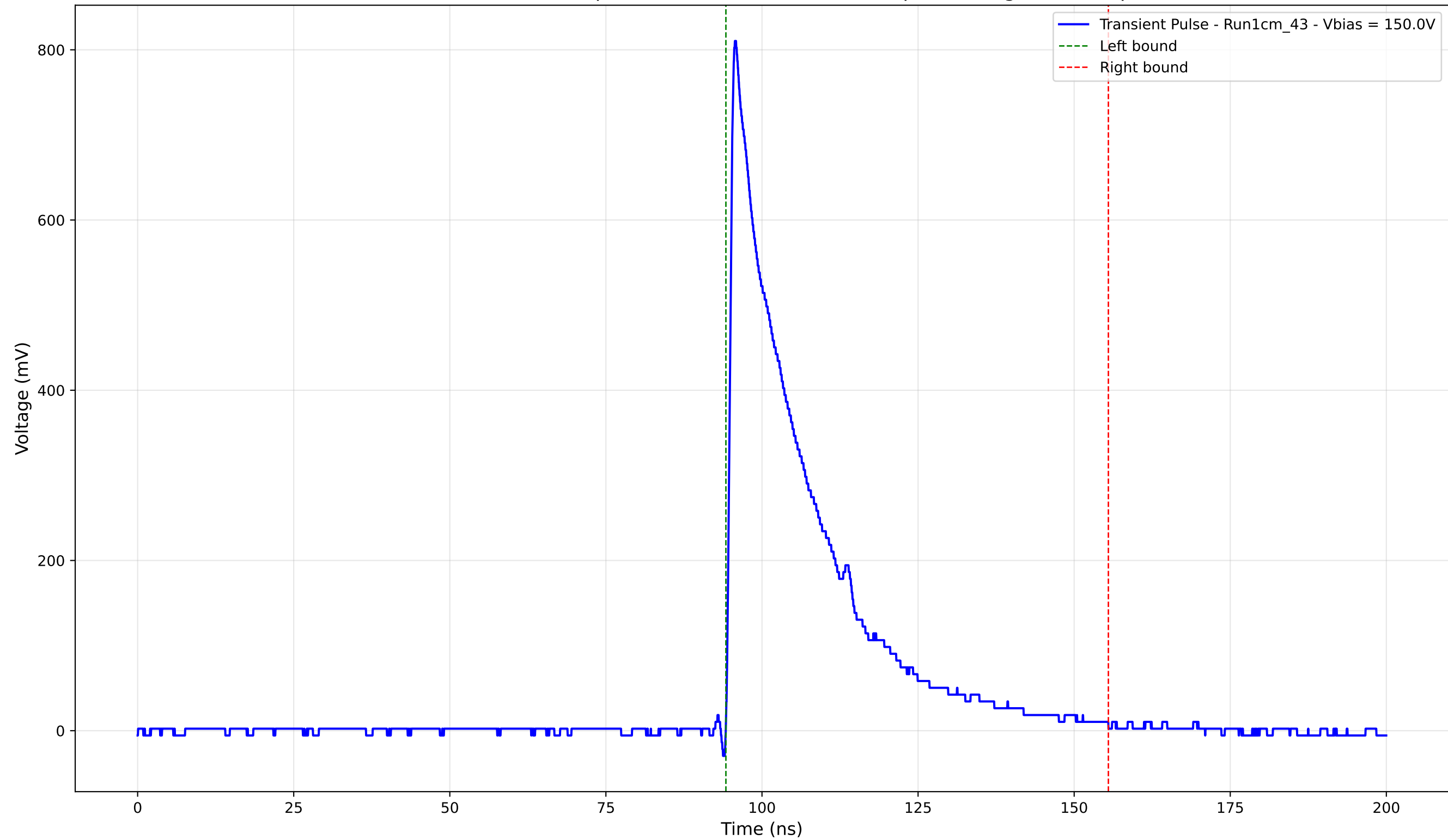
Transient Pulse - Sample: new1cm - Position: 390.0 \mu\text{m} - Charge: 198.17 pC
