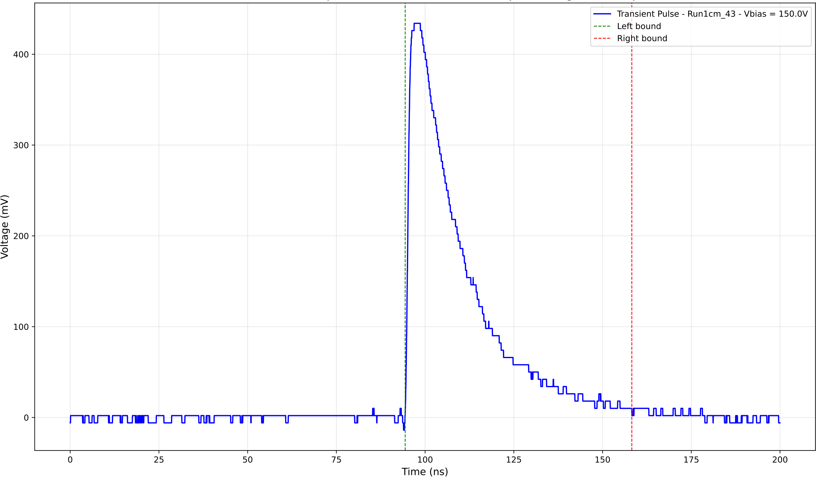
Transient Pulse - Sample: new1cm - Position: 1760.0 \mu\text{m} - Charge: 149.89 pC
