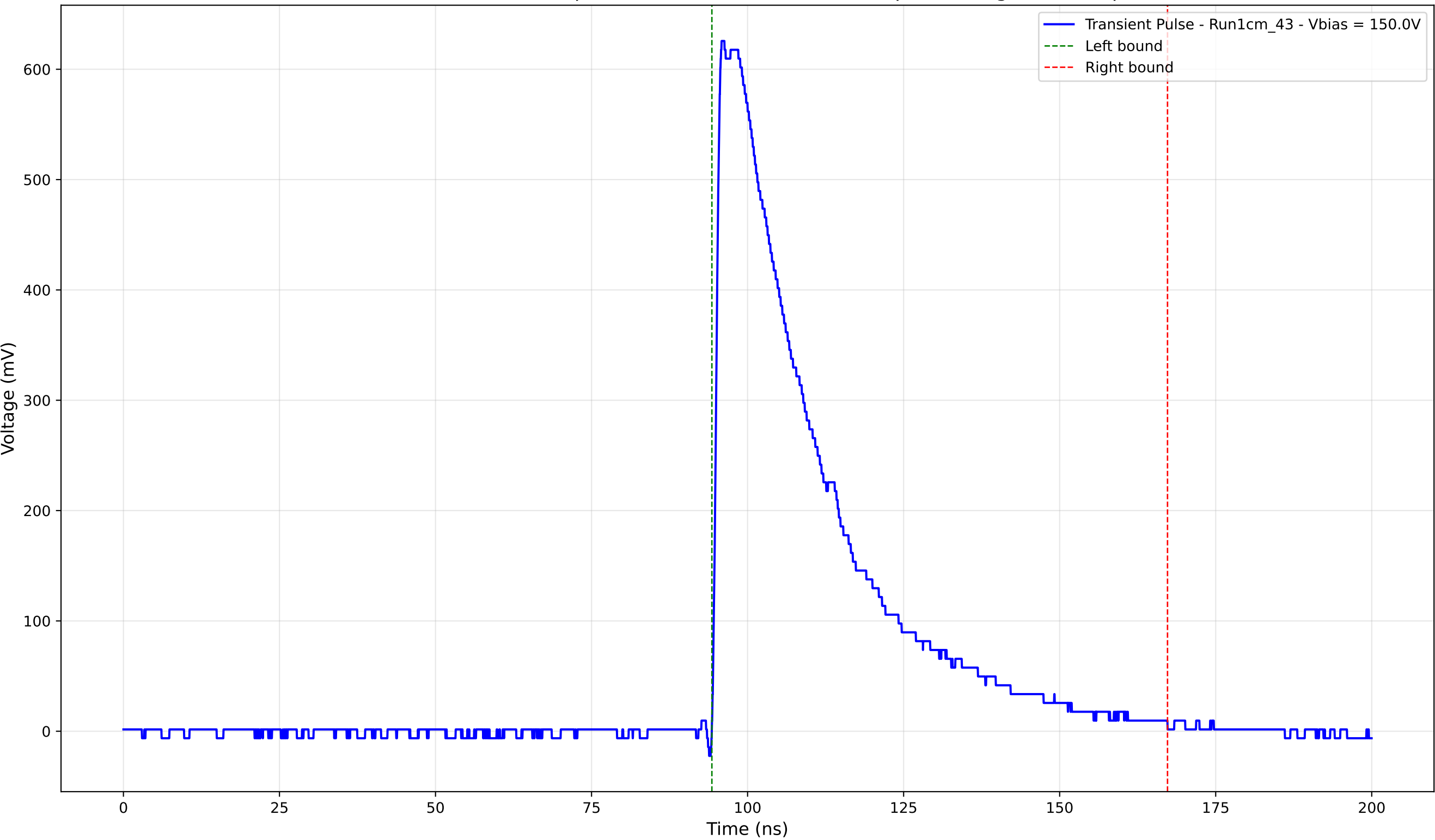
Transient Pulse - Sample: new1cm - Position: 1955.0 \mu\text{m} - Charge: 224.04 pC
