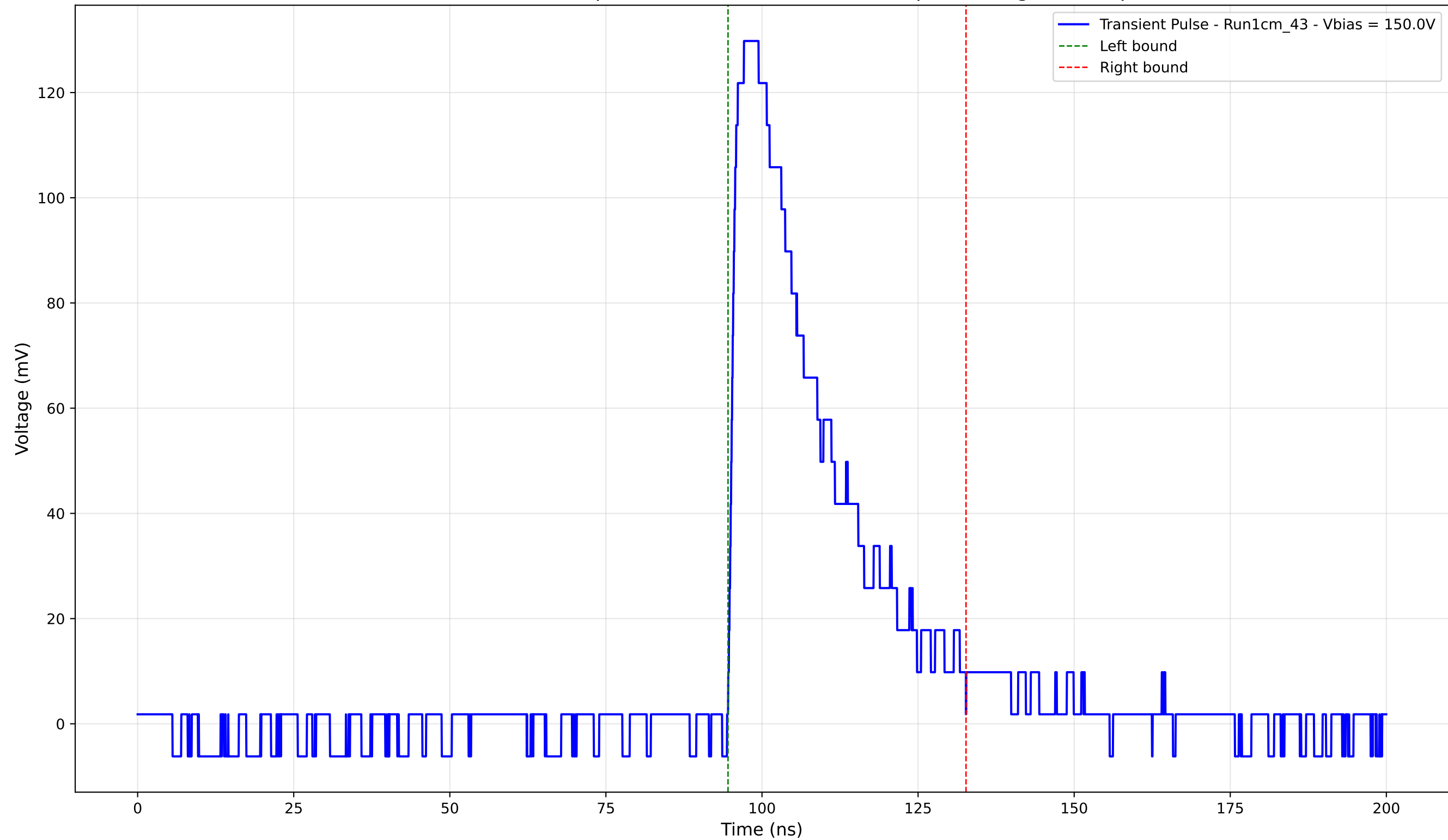
Transient Pulse - Sample: new1cm - Position: 3720.0 \mu\text{m} - Charge: 40.95 pC
