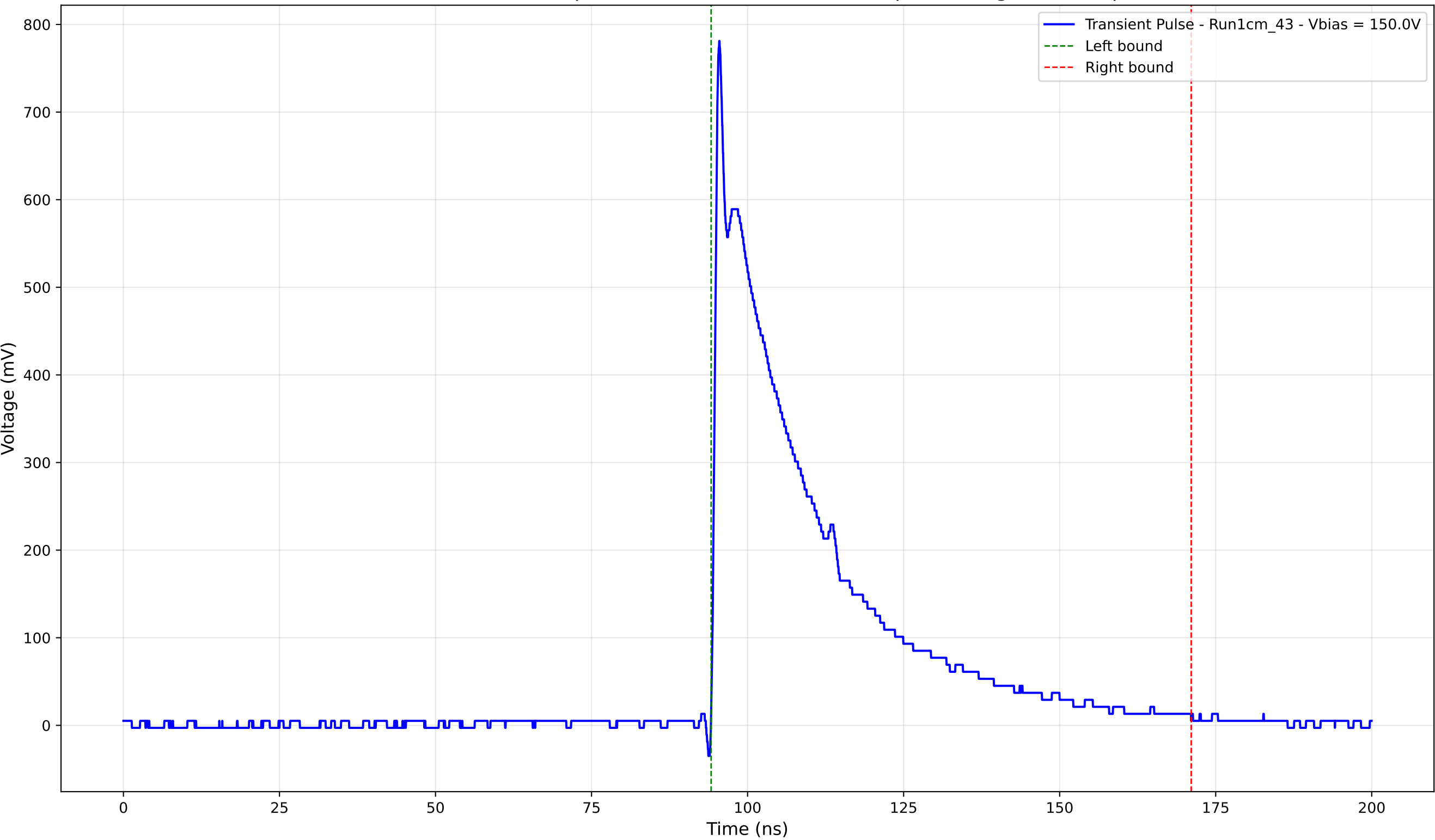
Transient Pulse - Sample: new1cm - Position: 2335.0 \mu\text{m} - Charge: 224.89 pC
