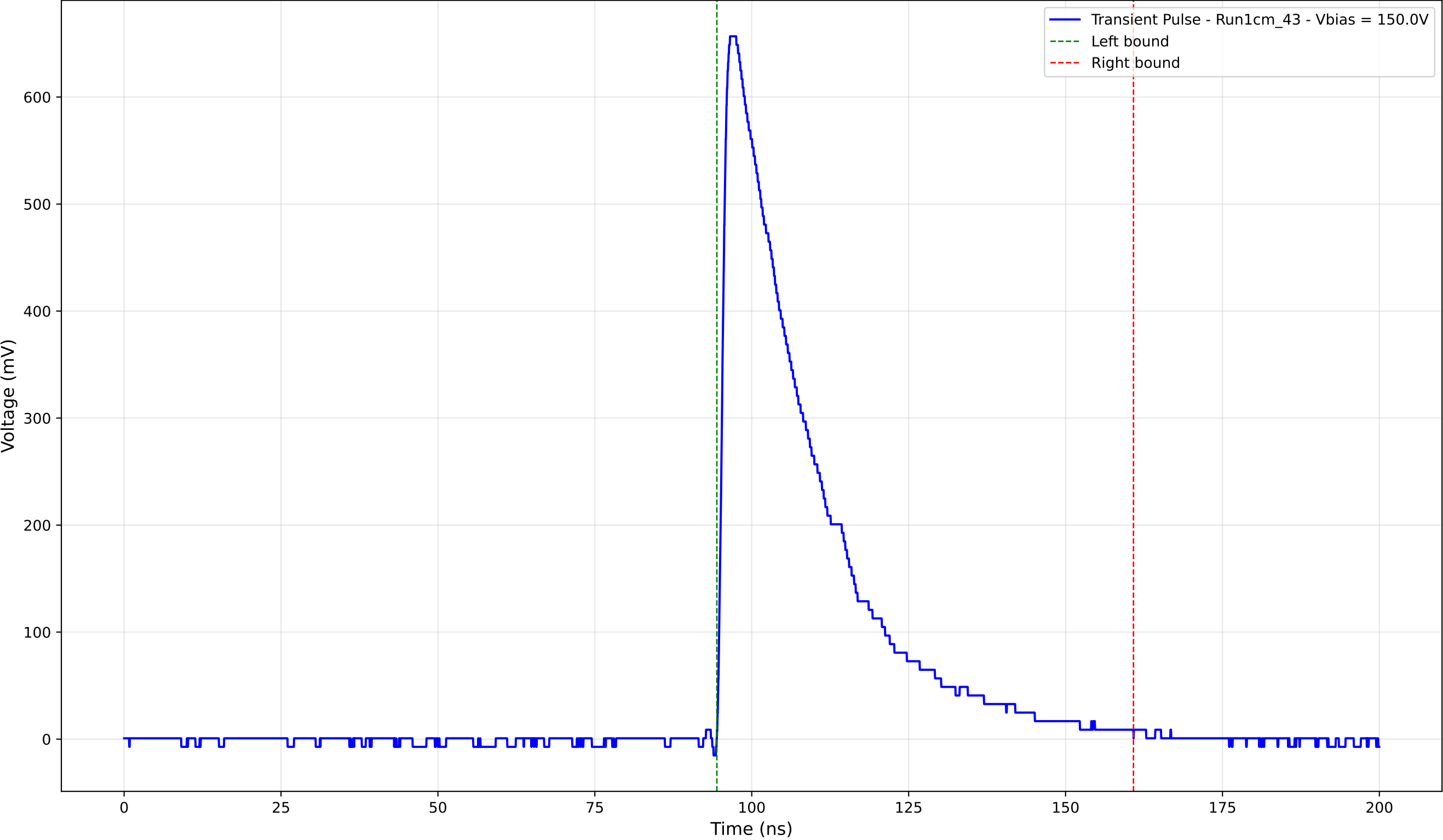
Transient Pulse - Sample: new1cm - Position: 1010.0 \mu\text{m} - Charge: 203.49 pC
