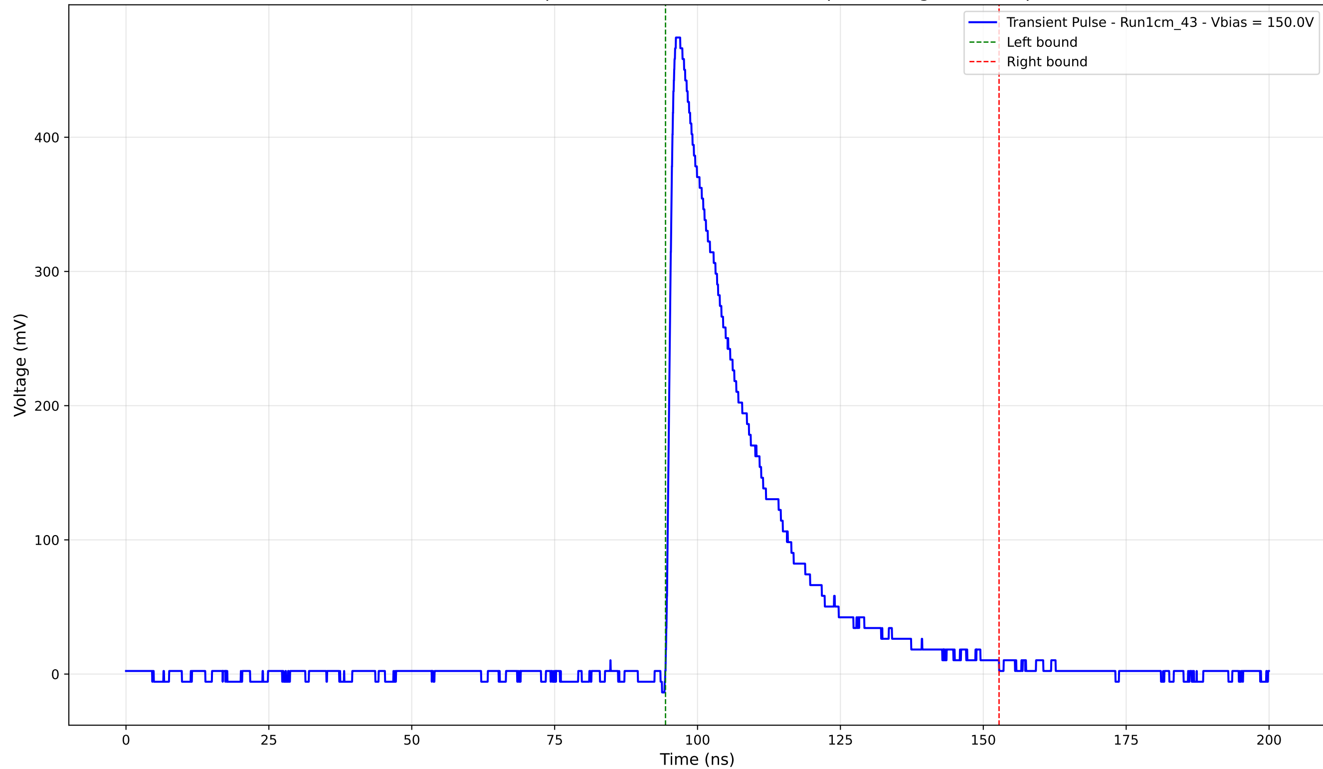
Transient Pulse - Sample: new1cm - Position: 745.0 \mu\text{m} - Charge: 135.56 pC
