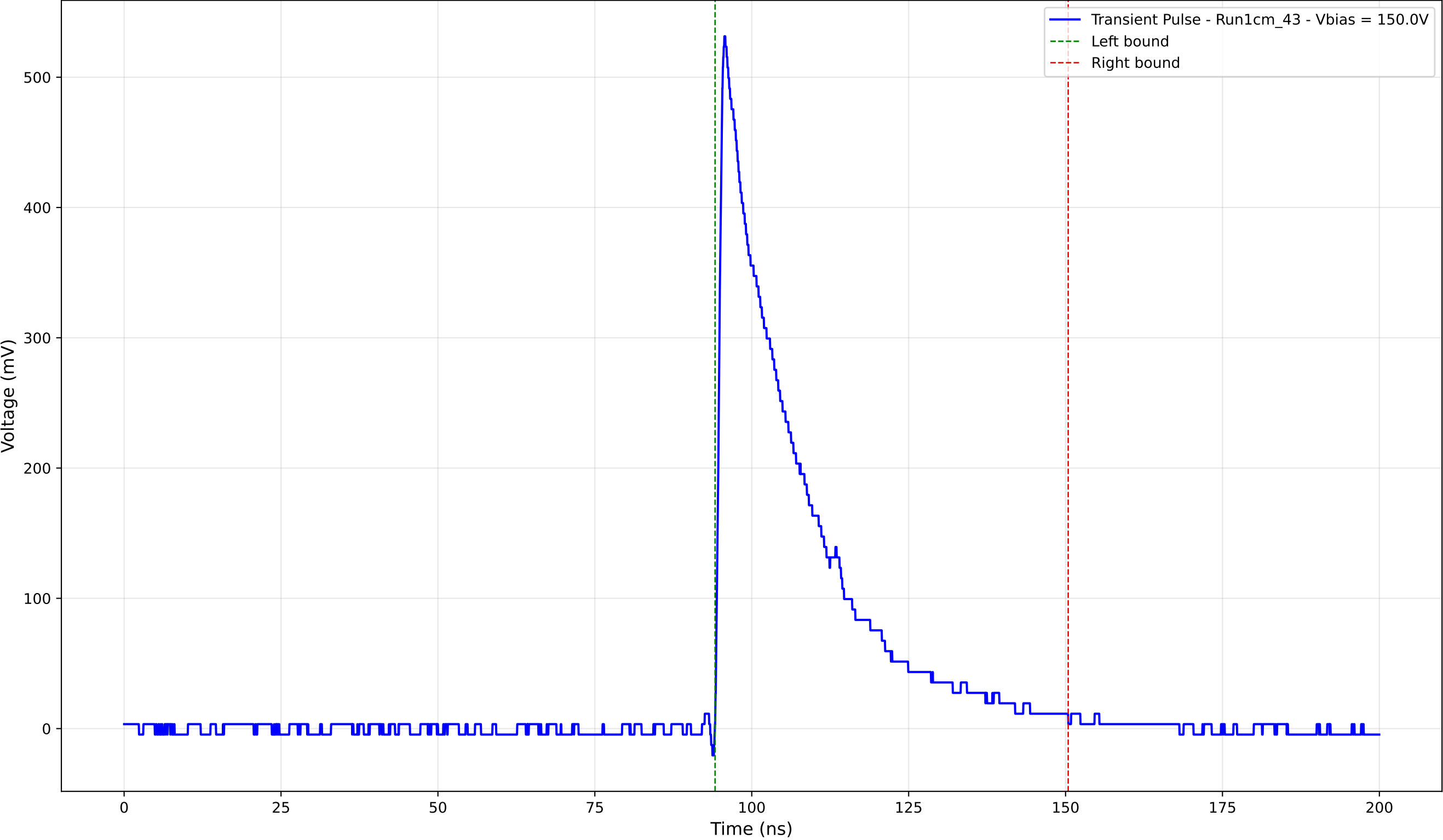
Transient Pulse - Sample: new1cm - Position: 4780.0 \mu\text{m} - Charge: 138.07 pC
