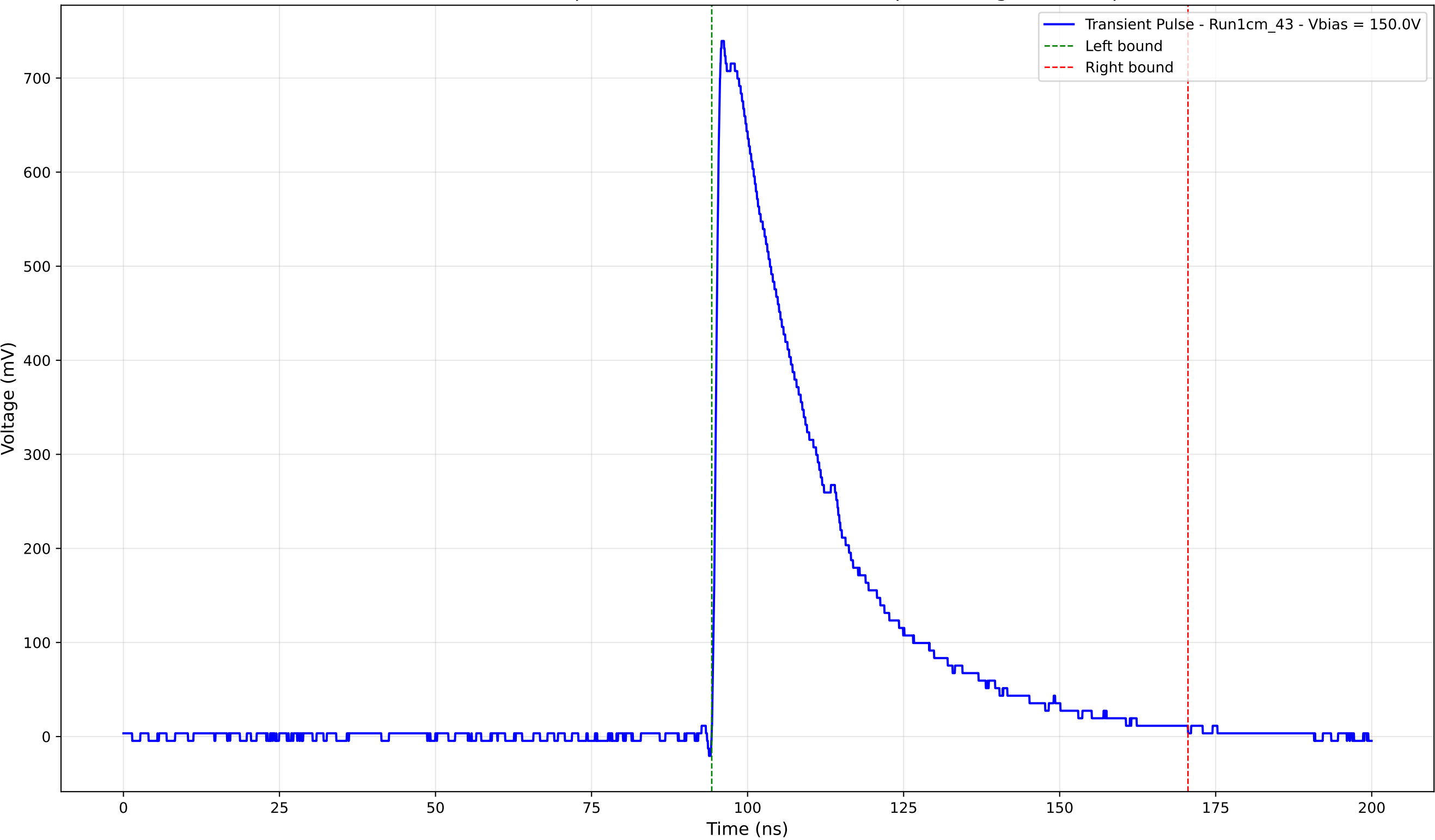
Transient Pulse - Sample: new1cm - Position: 3430.0 \mu\text{m} - Charge: 261.75 pC
