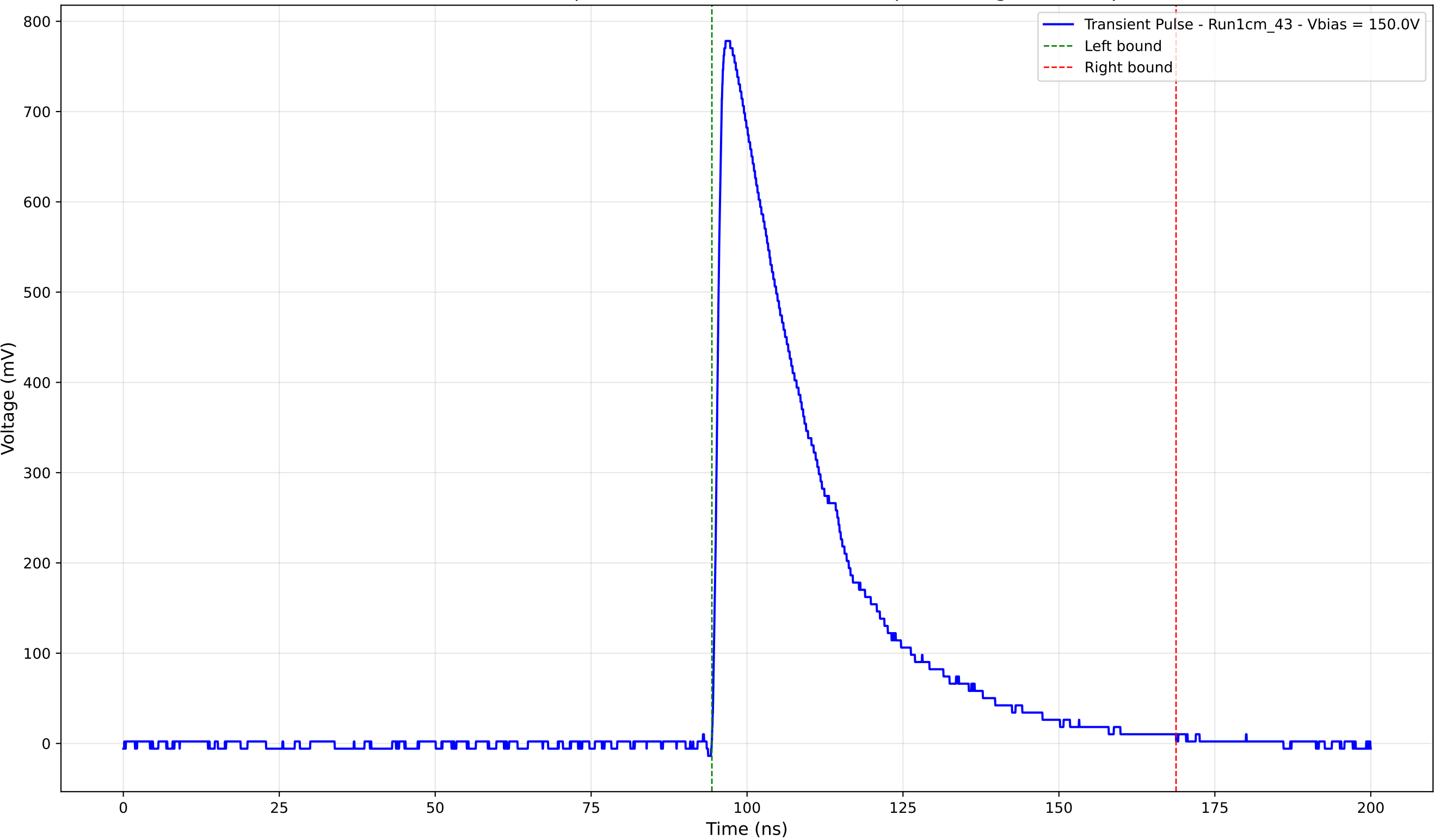
Transient Pulse - Sample: new1cm - Position: 3955.0 \mu\text{m} - Charge: 265.27 pC
