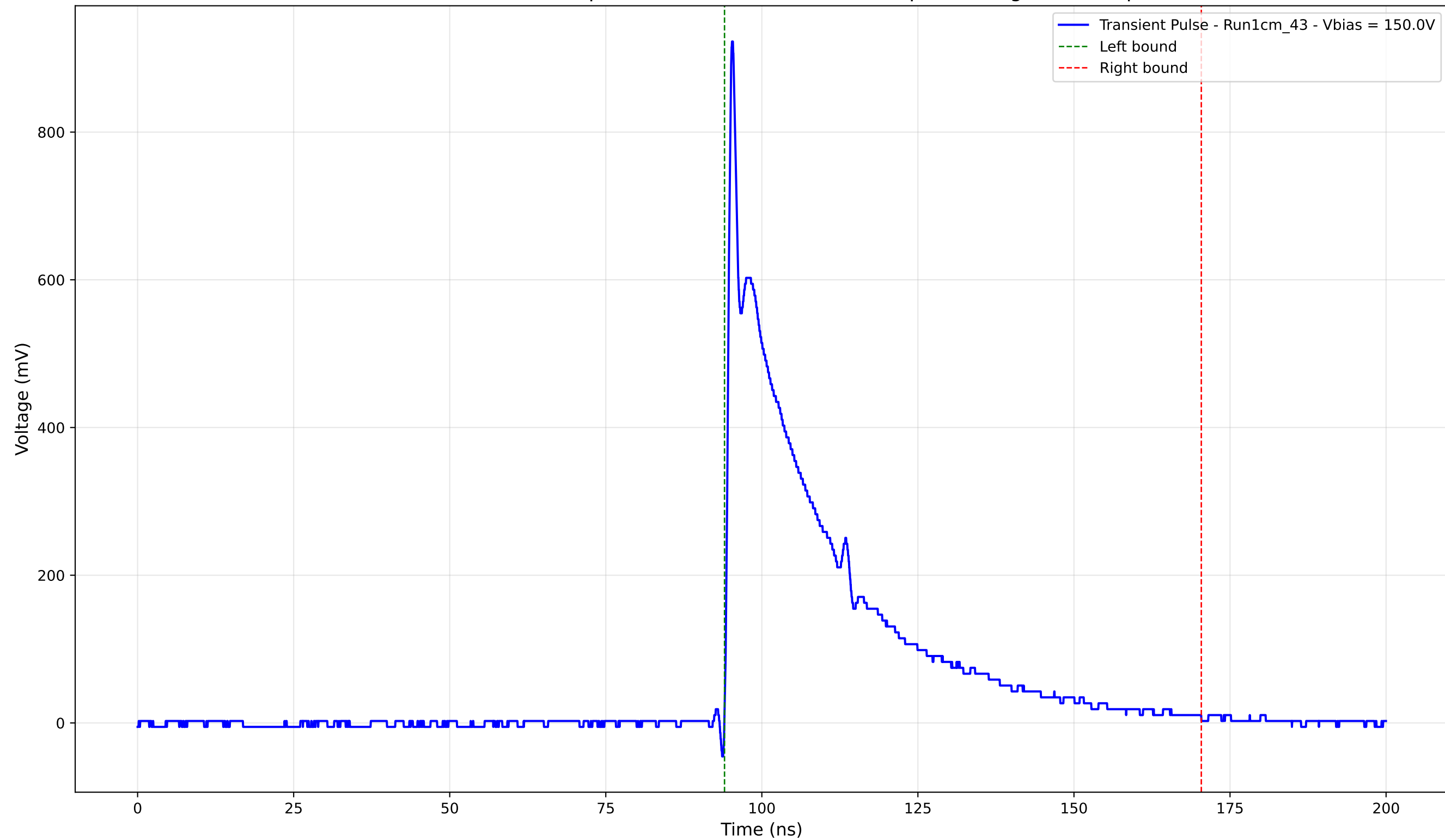
Transient Pulse - Sample: new1cm - Position: 2575.0 \mu\text{m} - Charge: 231.50 pC
