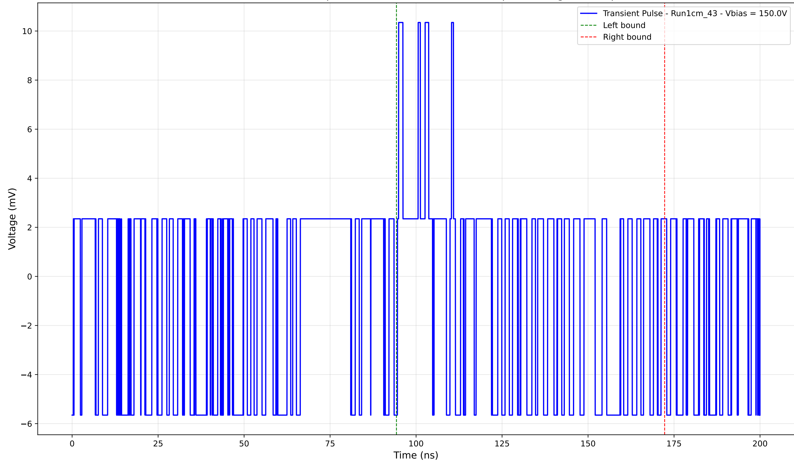
Transient Pulse - Sample: new1cm - Position: 5185.0 \mu\text{m} - Charge: -0.13 pC
