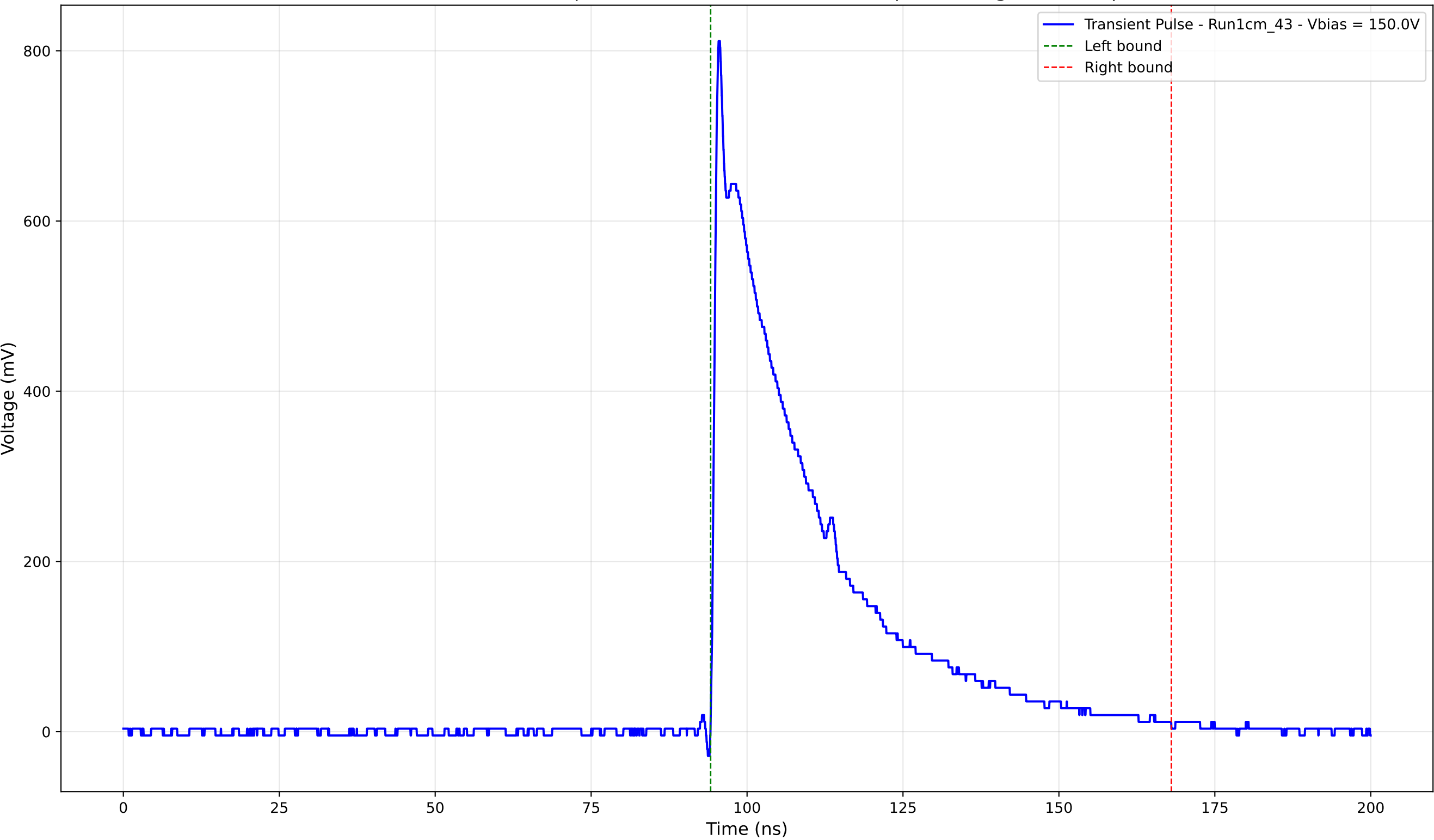
Transient Pulse - Sample: new1cm - Position: 3105.0 \mu\text{m} - Charge: 244.05 pC
