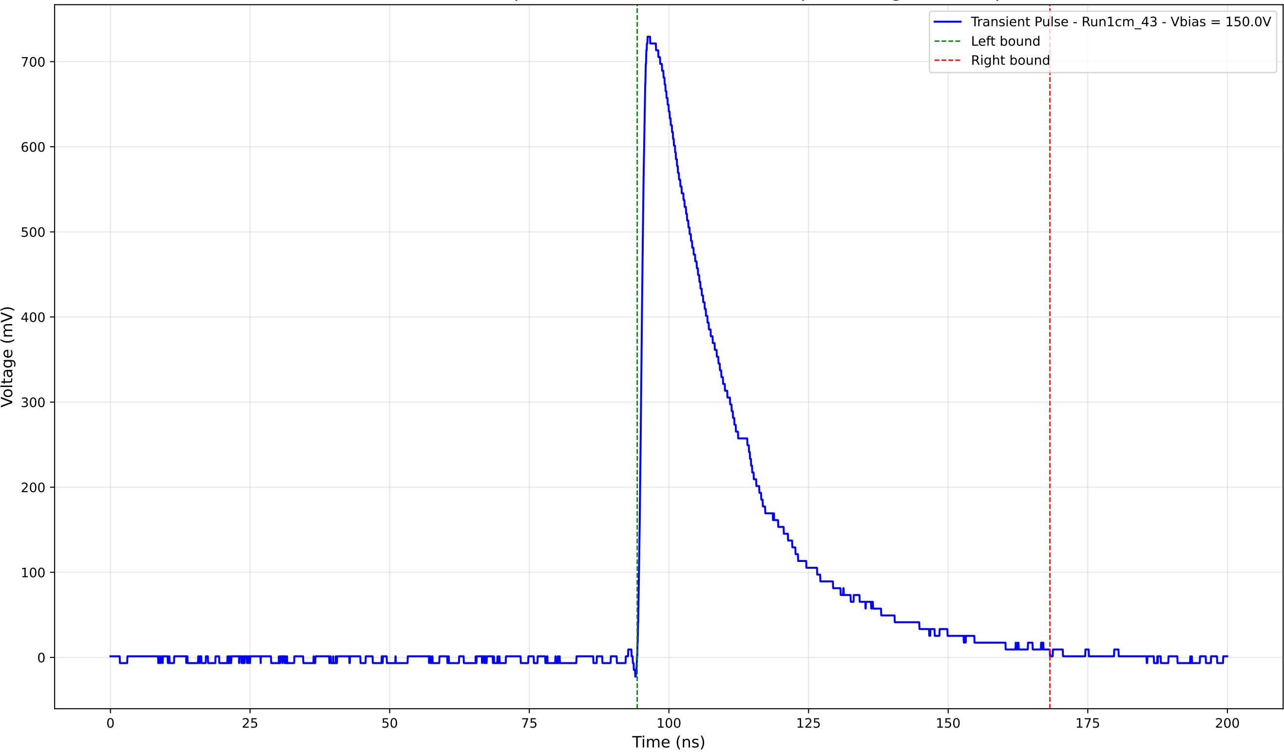
Transient Pulse - Sample: new1cm - Position: 3605.0 \mu\text{m} - Charge: 254.96 pC
