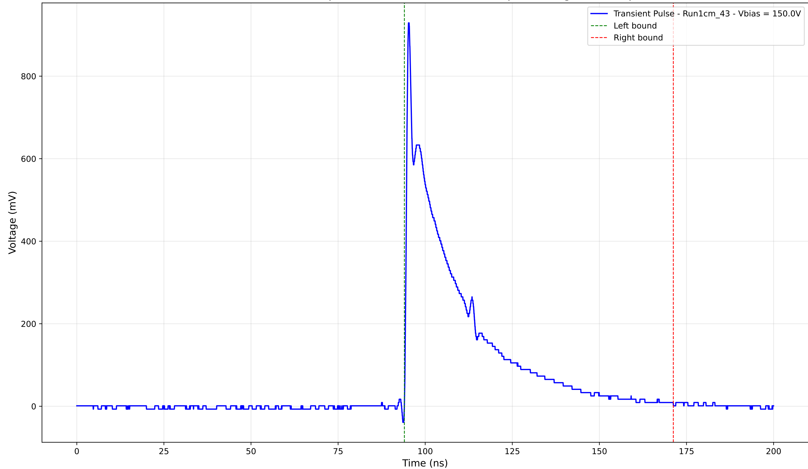
Transient Pulse - Sample: new1cm - Position: 2845.0 \mu\text{m} - Charge: 240.28 pC
