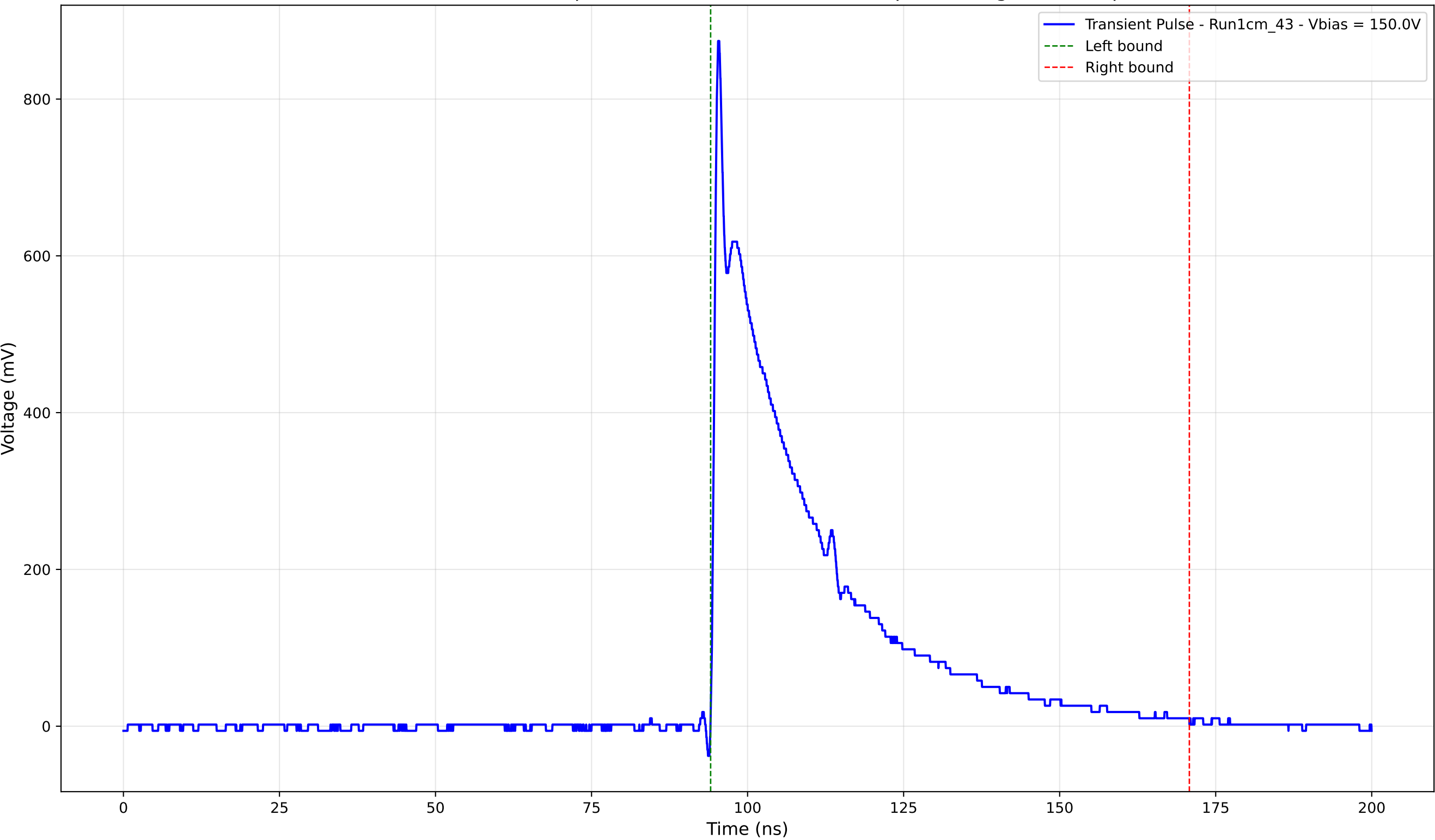
Transient Pulse - Sample: new1cm - Position: 2450.0 \mu\text{m} - Charge: 235.49 pC
