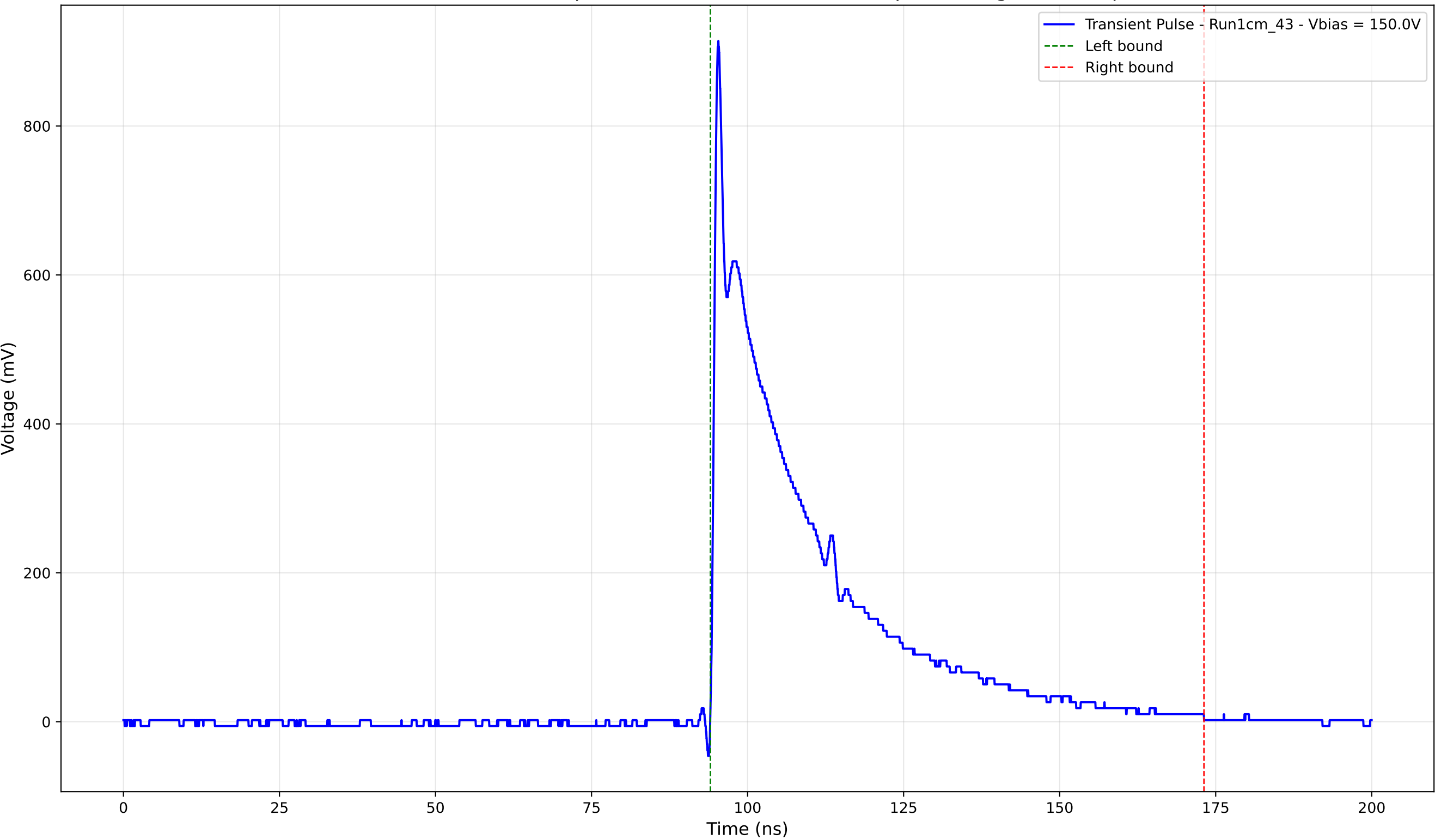
Transient Pulse - Sample: new1cm - Position: 2520.0 \mu\text{m} - Charge: 236.01 pC
