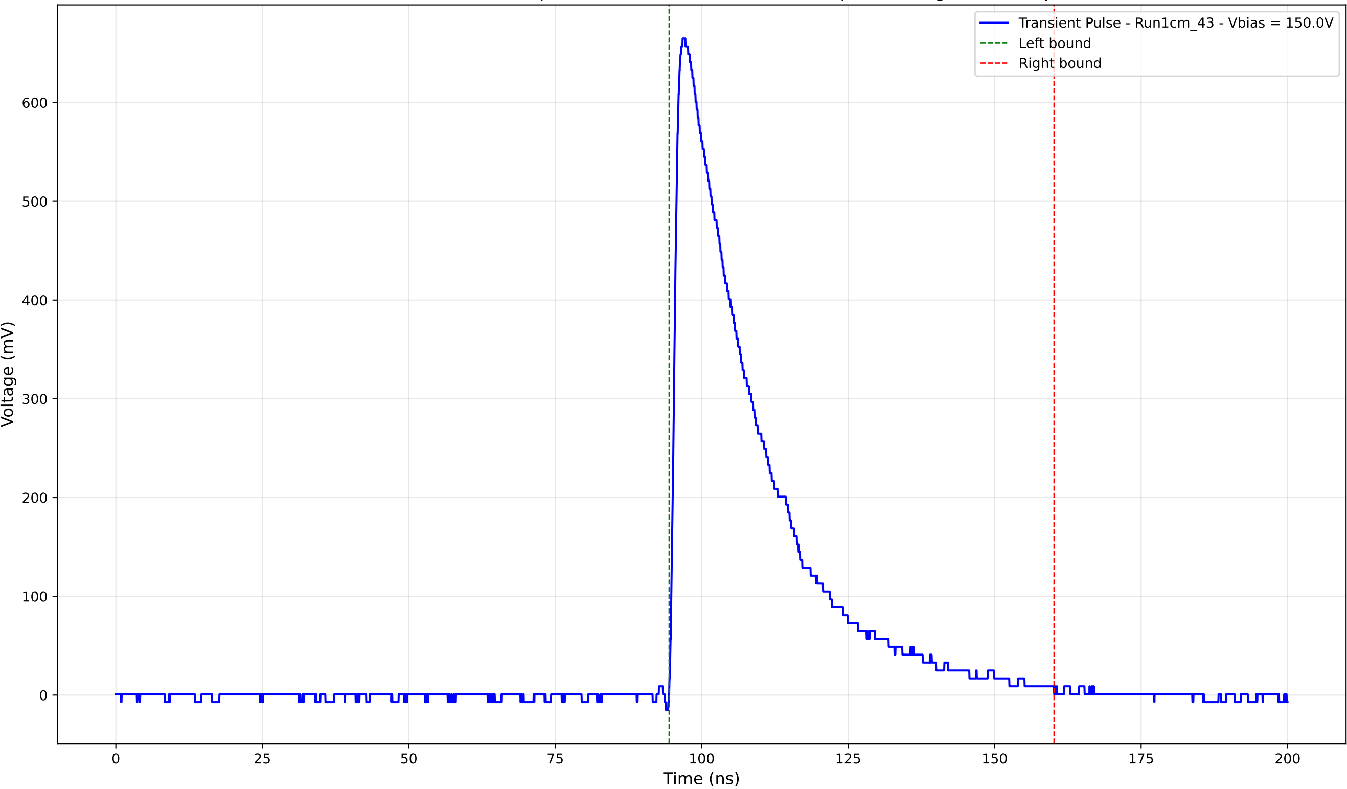
Transient Pulse - Sample: new1cm - Position: 1030.0 \mu\text{m} - Charge: 206.53 pC
