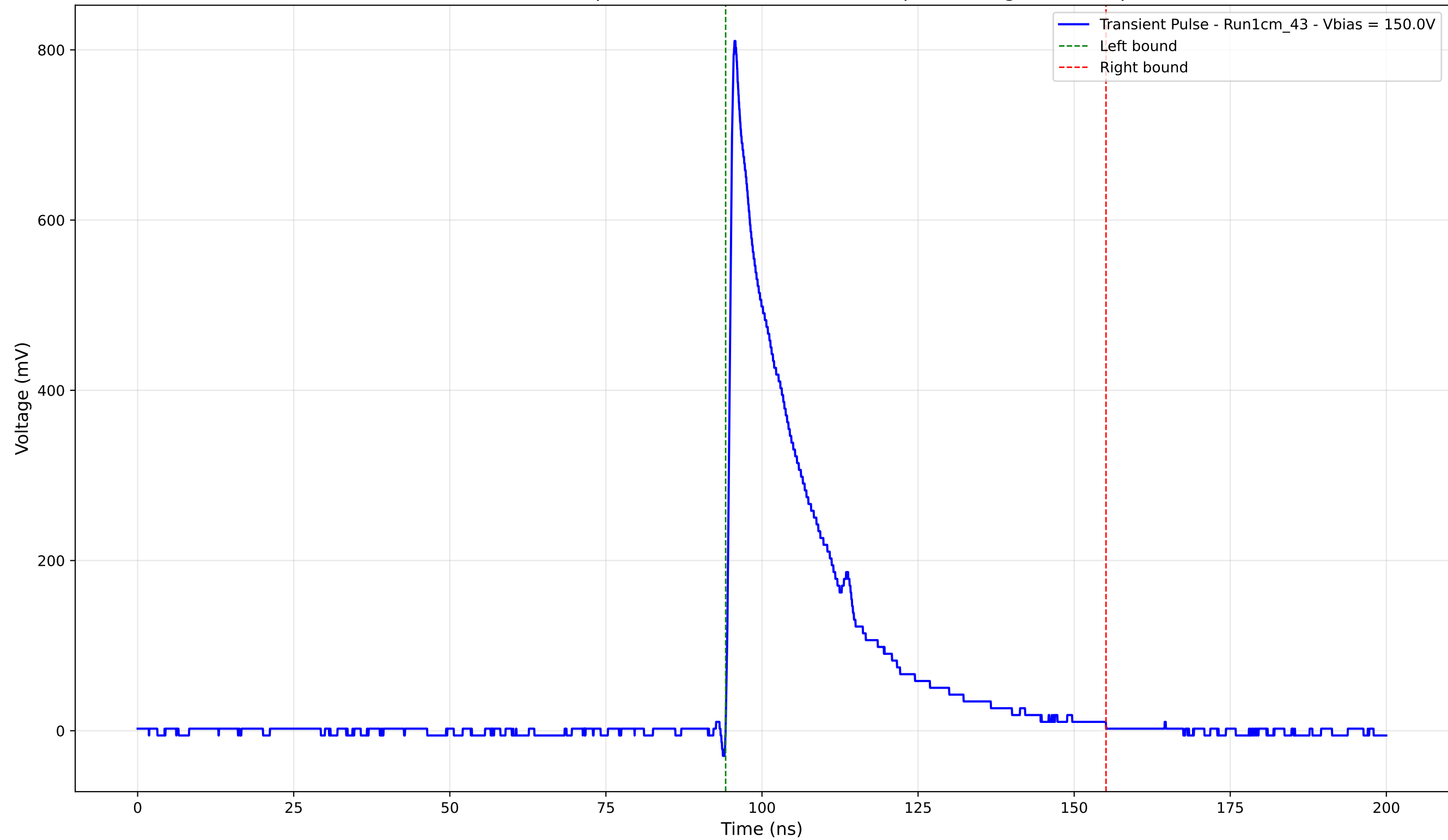
Transient Pulse - Sample: new1cm - Position: 330.0 \mu\text{m} - Charge: 189.31 pC
