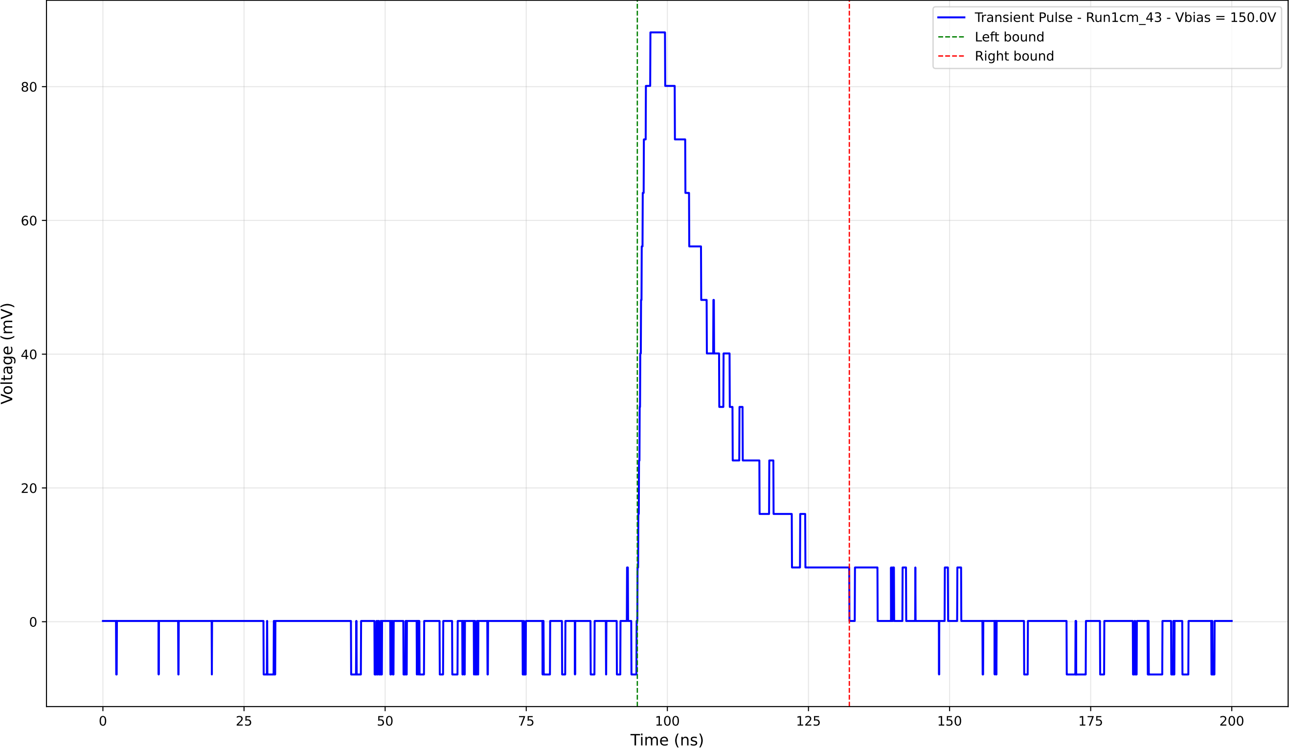
Transient Pulse - Sample: new1cm - Position: 1180.0 \mu\text{m} - Charge: 26.59 pC
