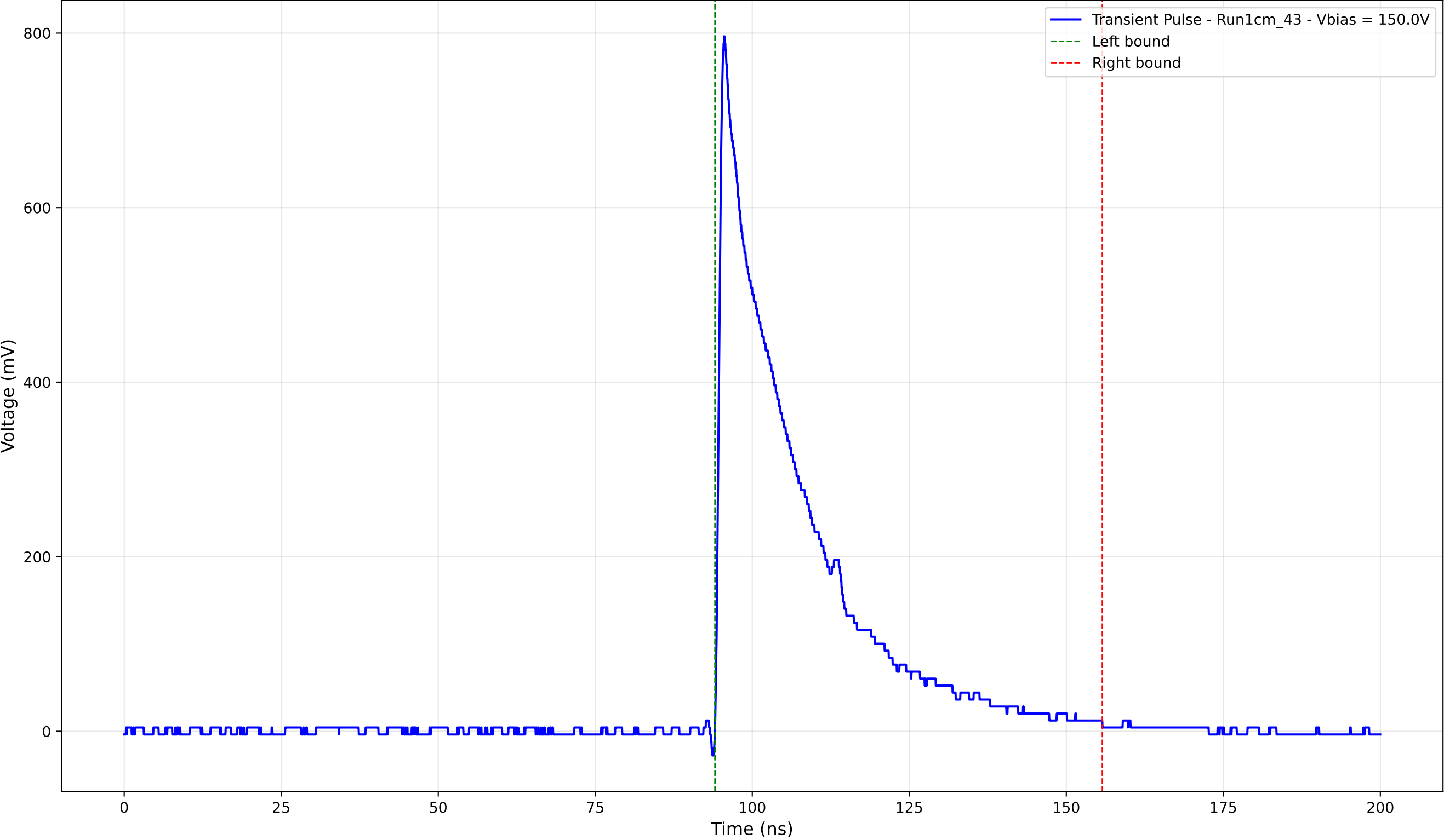
Transient Pulse - Sample: new1cm - Position: 4915.0 \mu\text{m} - Charge: 199.84 pC
