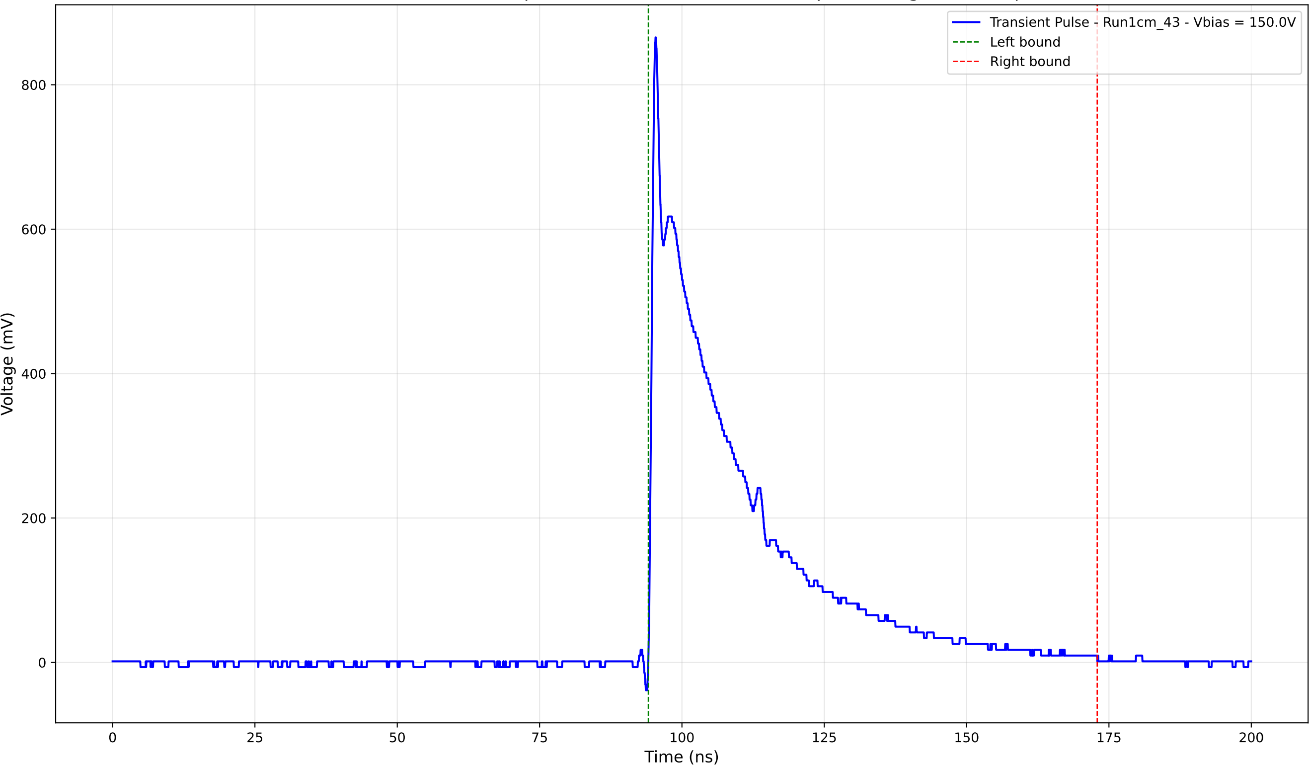
Transient Pulse - Sample: new1cm - Position: 2430.0 \mu\text{m} - Charge: 232.42 pC
