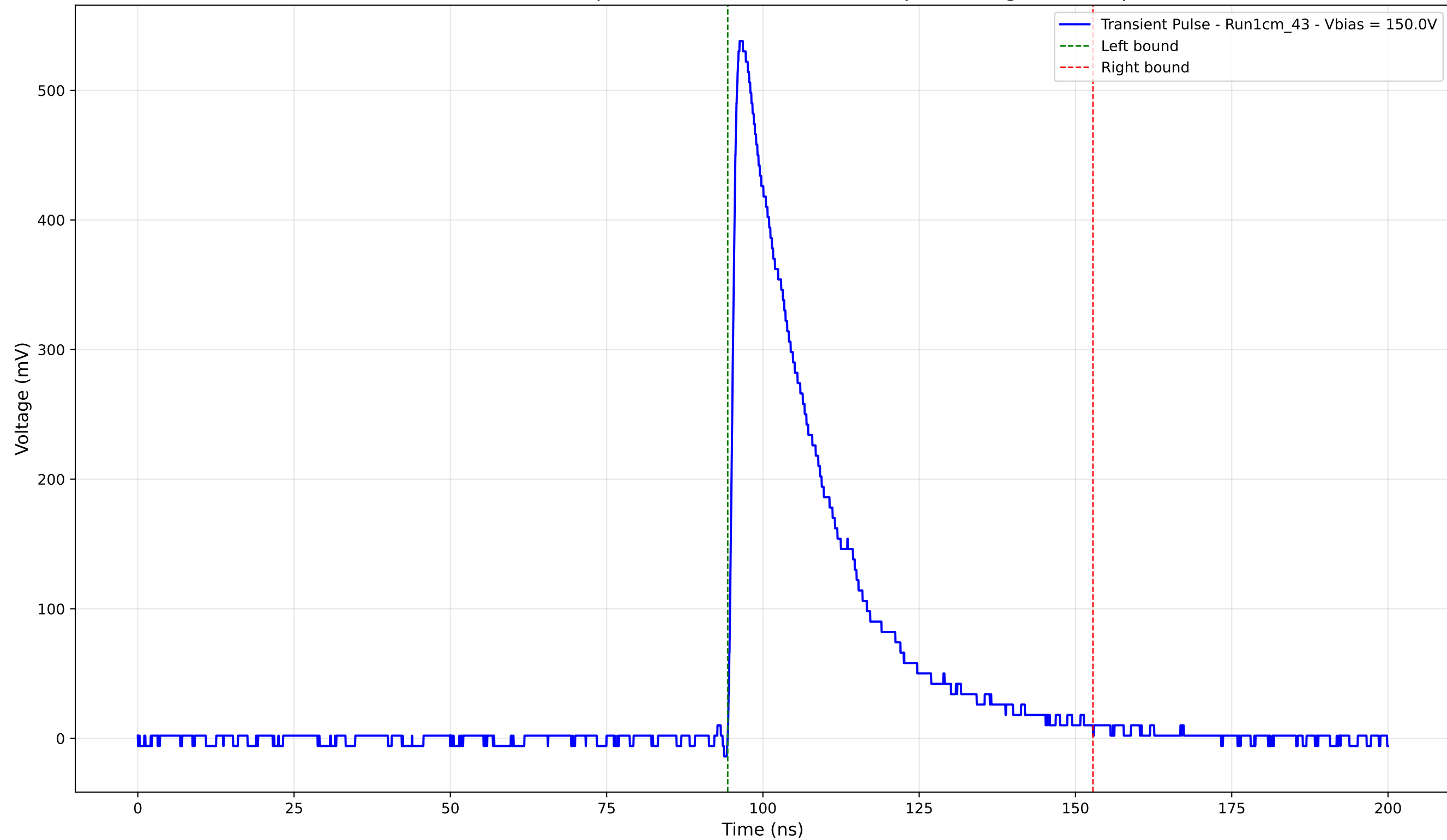
Transient Pulse - Sample: new1cm - Position: 755.0 \mu\text{m} - Charge: 154.46 pC
