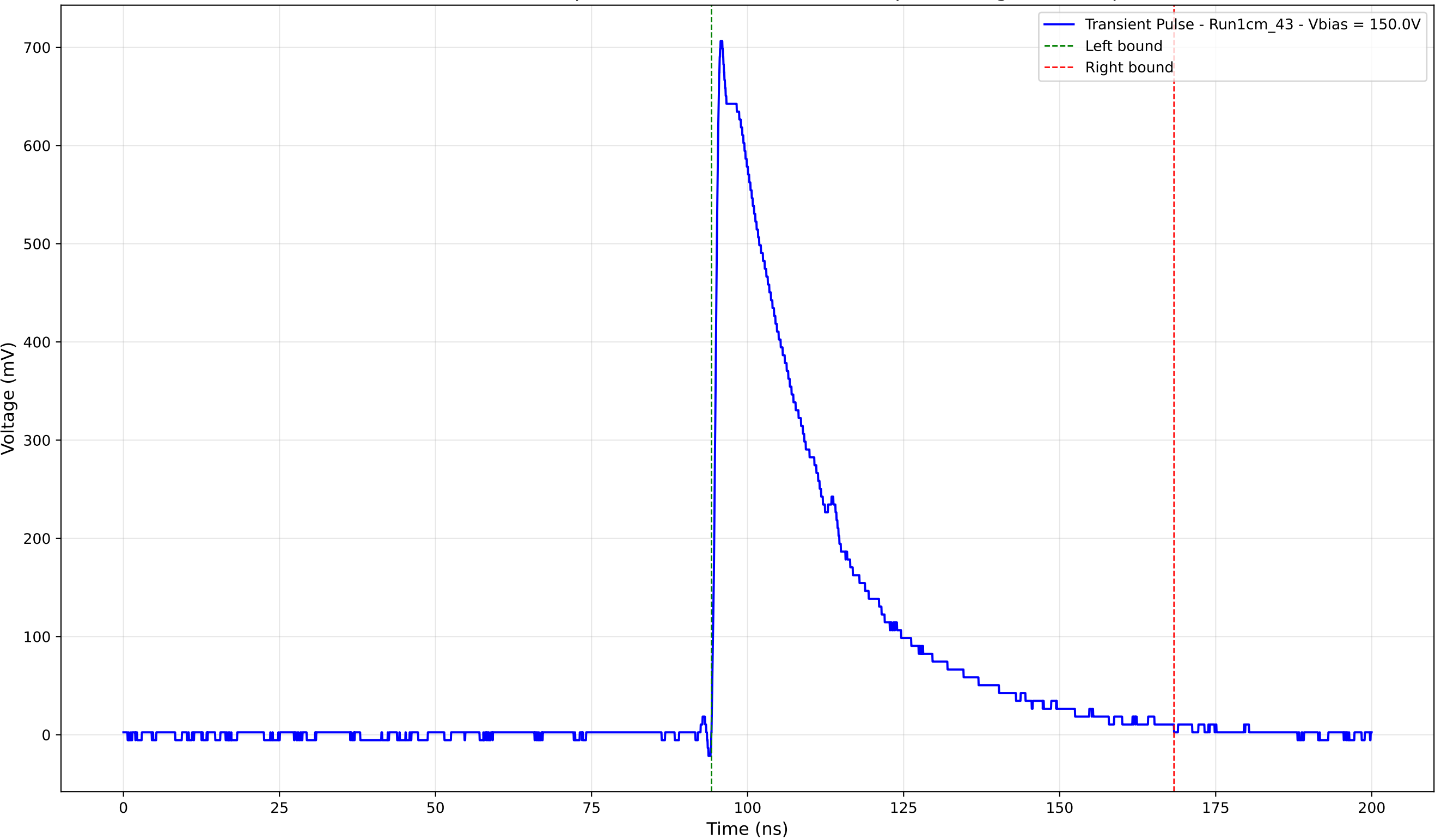
Transient Pulse - Sample: new1cm - Position: 3305.0 \mu\text{m} - Charge: 236.07 pC
