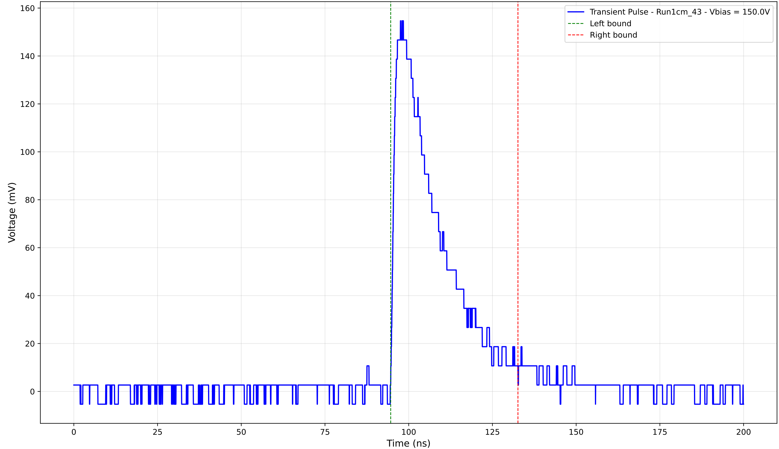
Transient Pulse - Sample: new1cm - Position: 1205.0 \mu\text{m} - Charge: 45.78 pC
