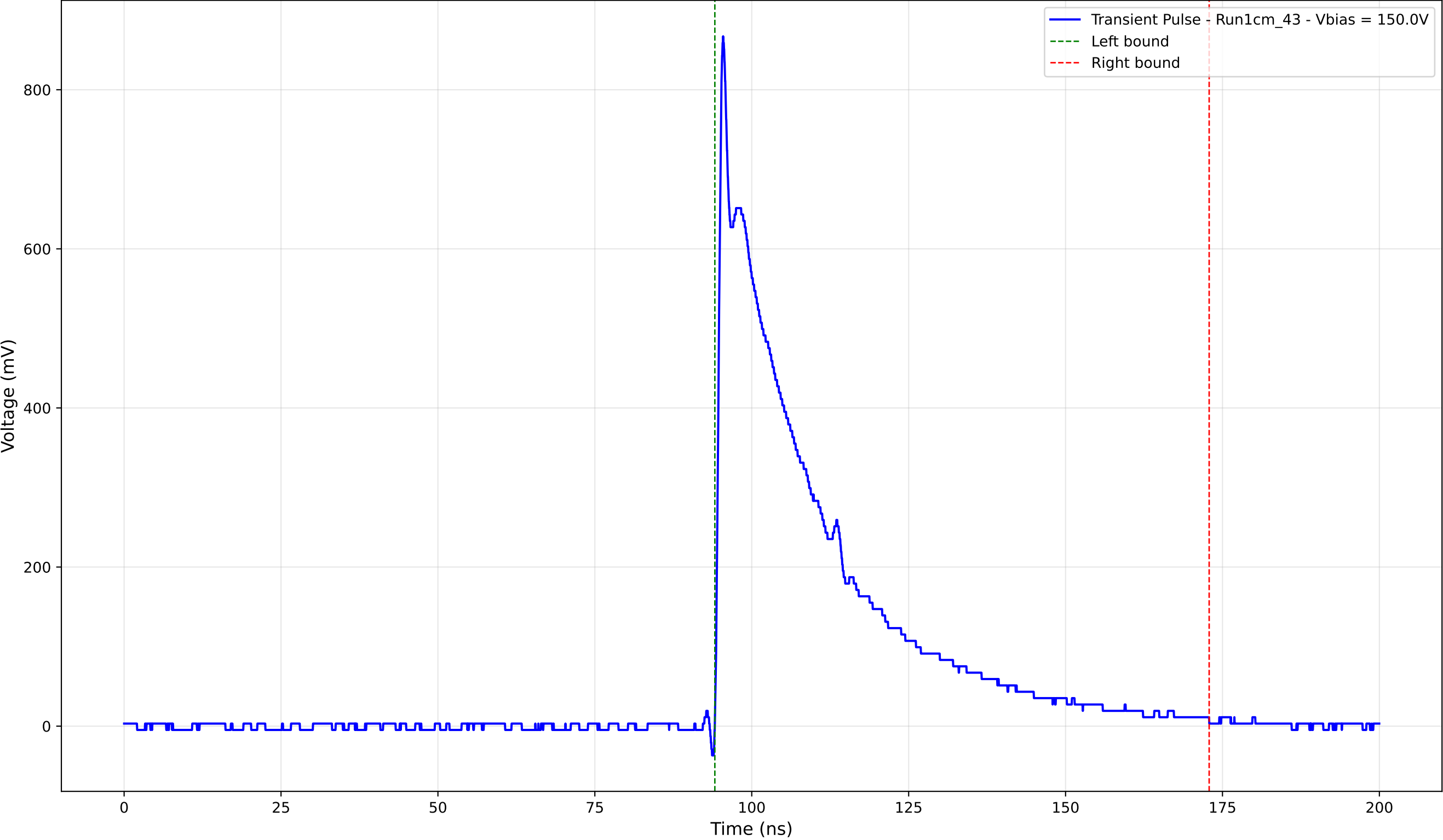
Transient Pulse - Sample: new1cm - Position: 3025.0 \mu\text{m} - Charge: 248.43 pC
