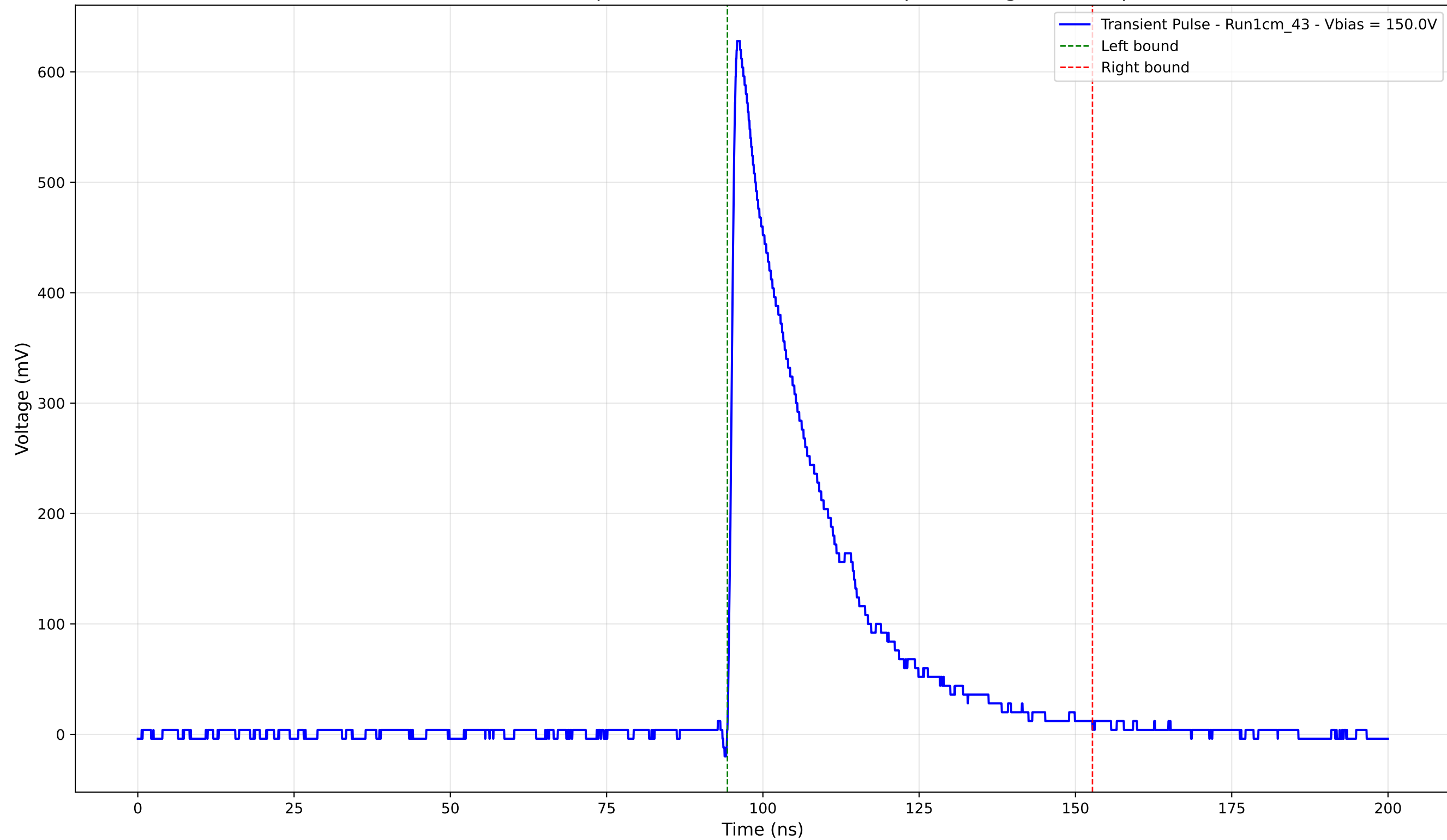
Transient Pulse - Sample: new1cm - Position: 590.0 \mu\text{m} - Charge: 168.93 pC
