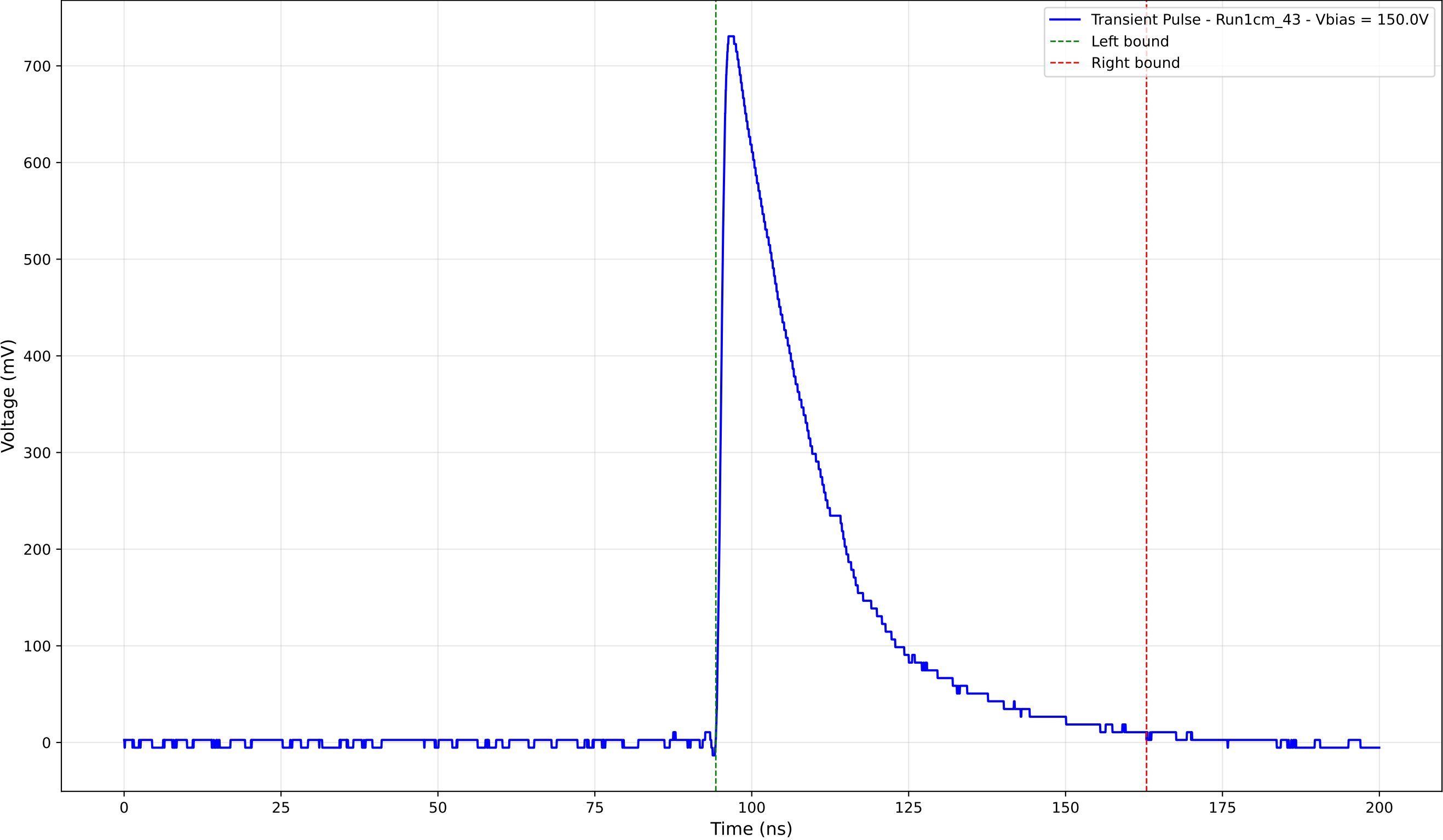
Transient Pulse - Sample: new1cm - Position: 4315.0 \mu\text{m} - Charge: 236.03 pC
