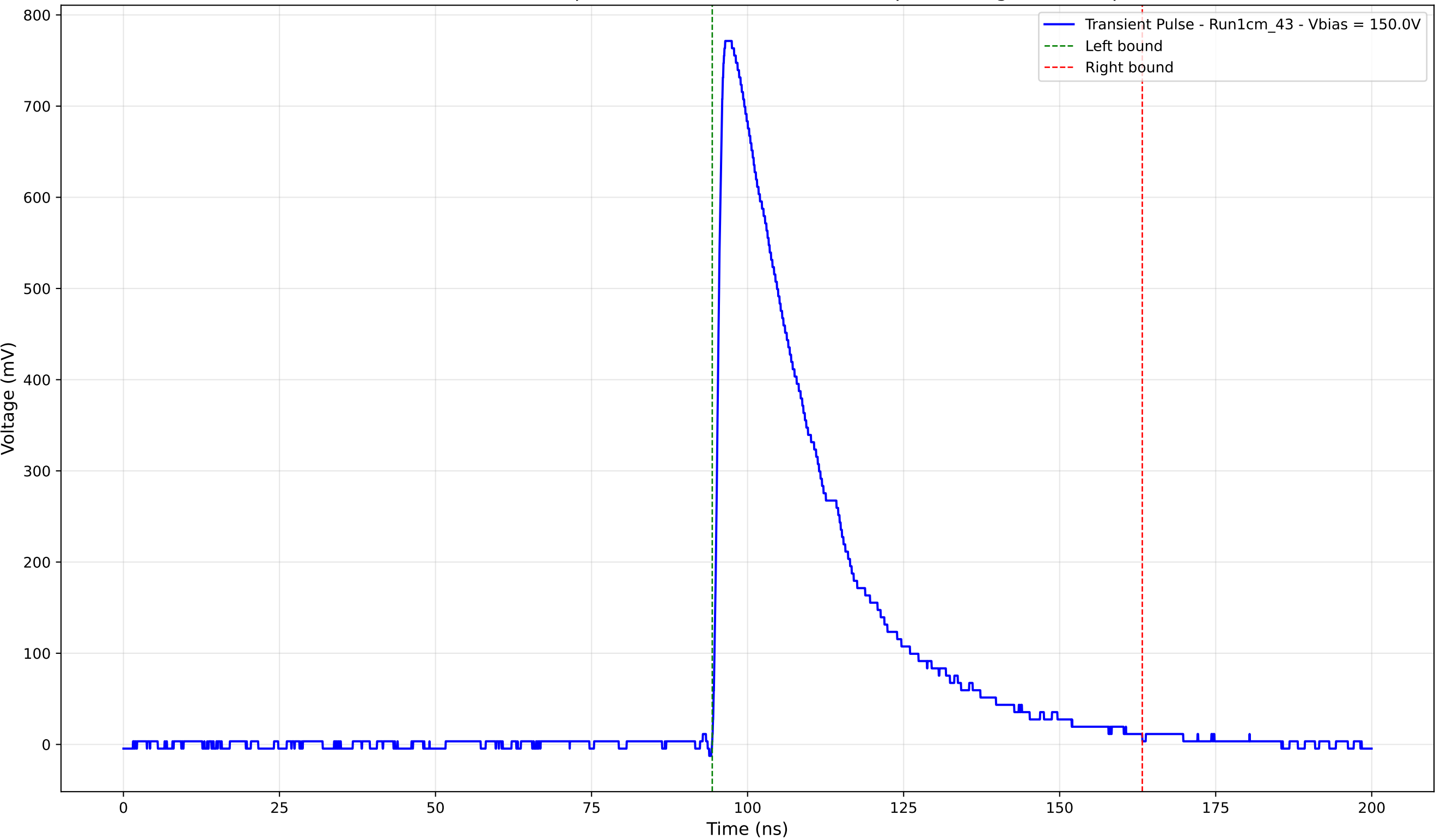
Transient Pulse - Sample: new1cm - Position: 3940.0 \mu\text{m} - Charge: 265.02 pC
