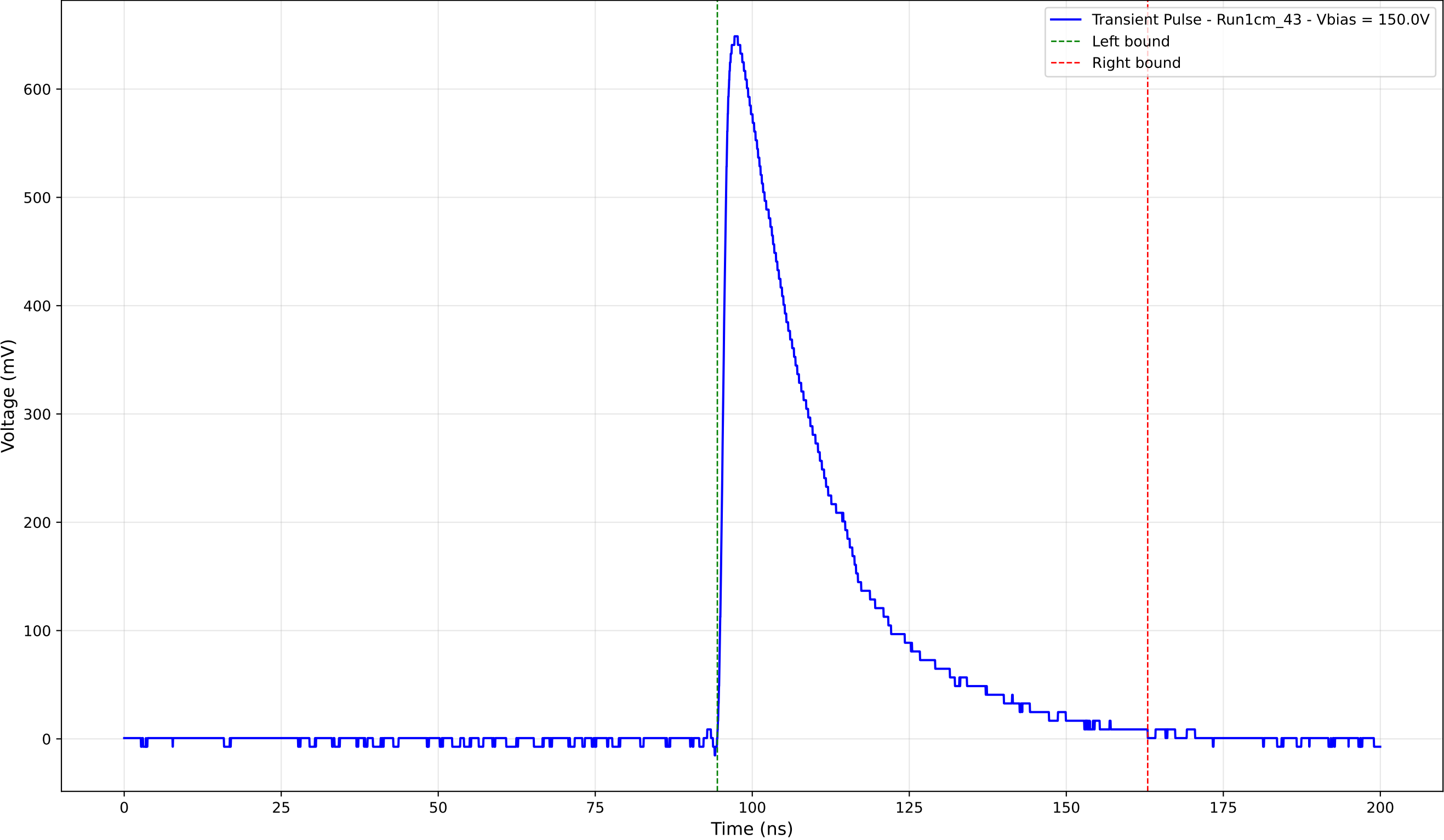
Transient Pulse - Sample: new1cm - Position: 1370.0 \mu\text{m} - Charge: 213.58 pC
