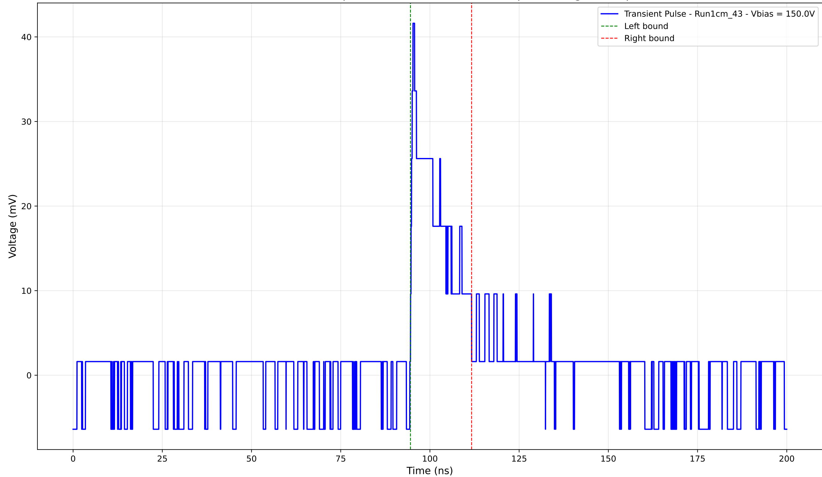
Transient Pulse - Sample: new1cm - Position: 155.0 \mu\text{m} - Charge: 6.43 pC
