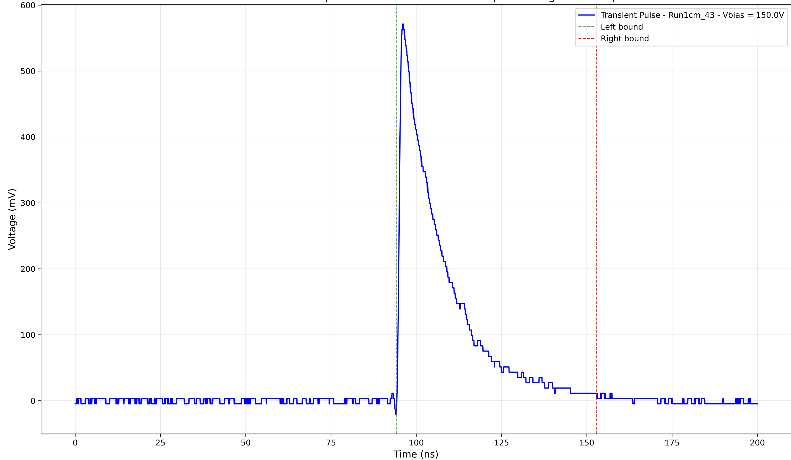
Transient Pulse - Sample: new1cm - Position: 600.0 \mu\text{m} - Charge: 152.04 pC
