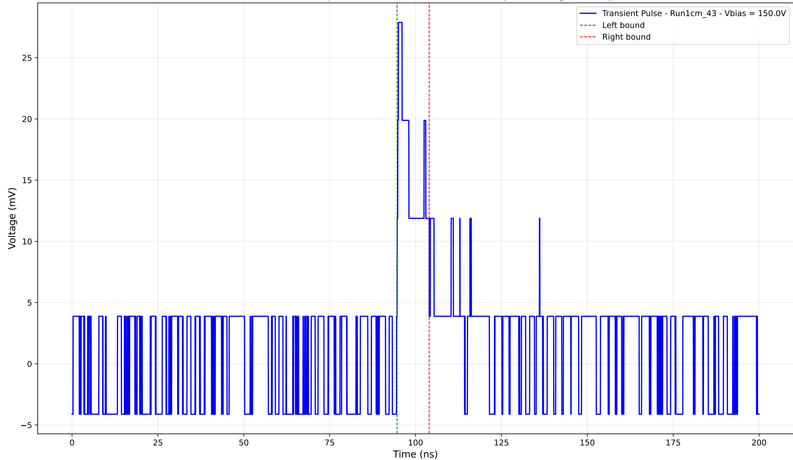
Transient Pulse - Sample: new1cm - Position: 5065.0 \mu\text{m} - Charge: 2.99 pC
