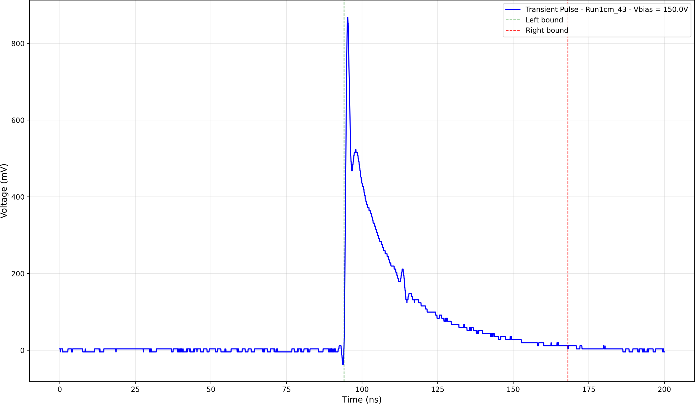
Transient Pulse - Sample: new1cm - Position: 2615.0 \mu\text{m} - Charge: 200.06 pC
