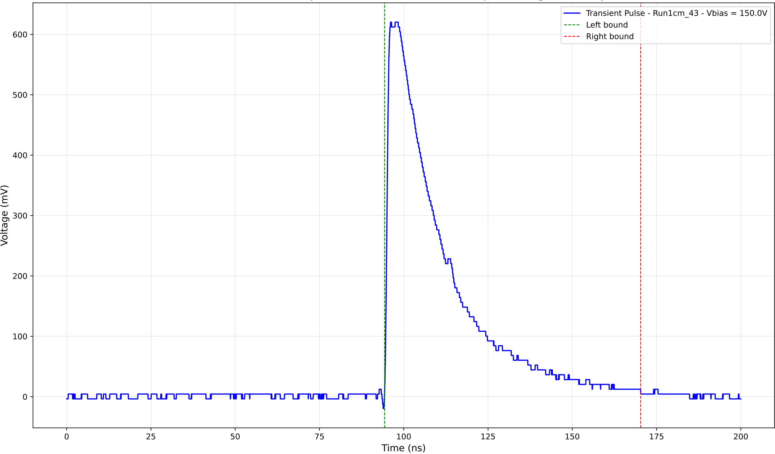
Transient Pulse - Sample: new1cm - Position: 1905.0 \mu\text{m} - Charge: 226.83 pC
