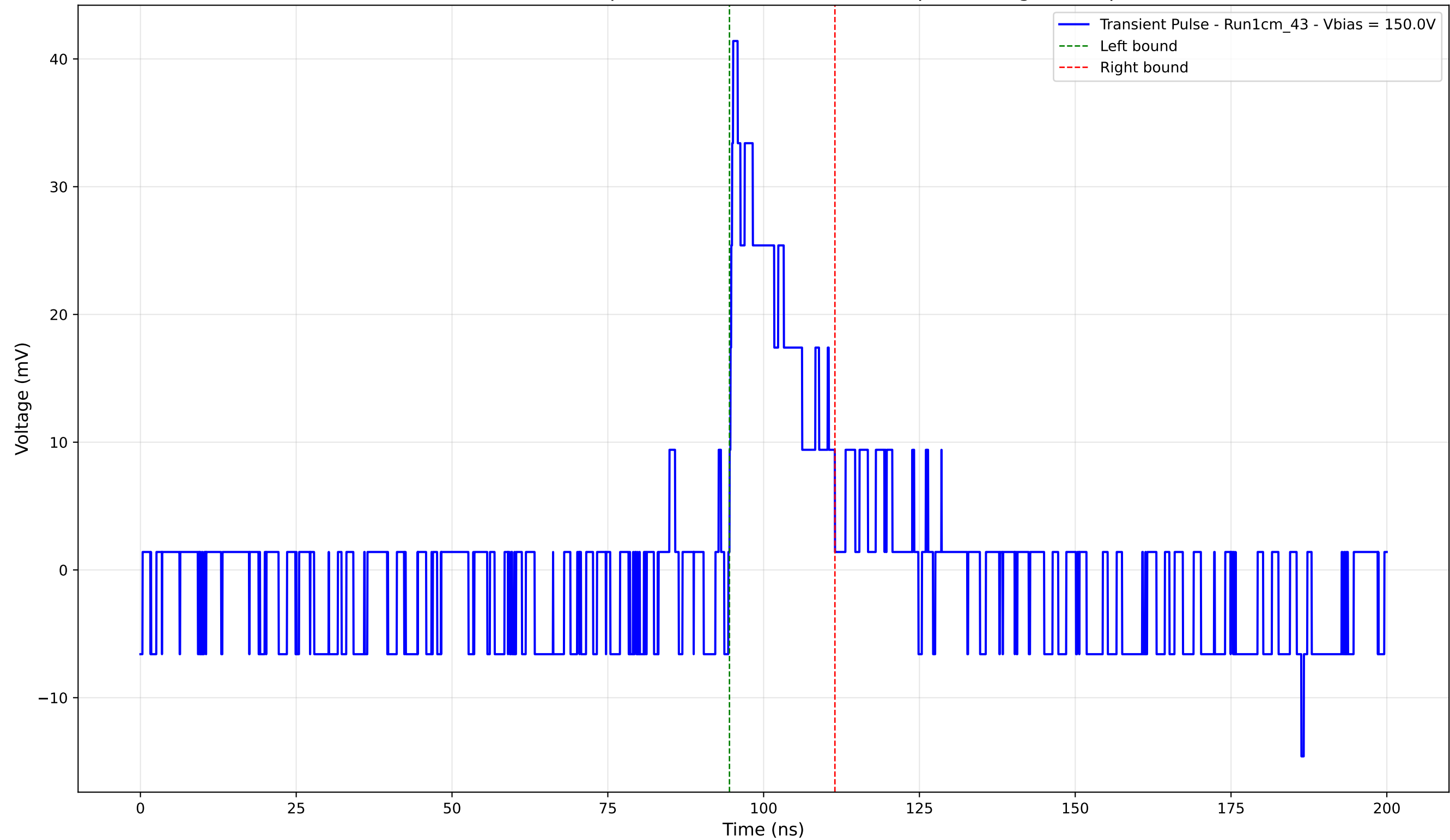
Transient Pulse - Sample: new1cm - Position: 160.0 \mu\text{m} - Charge: 6.93 pC
