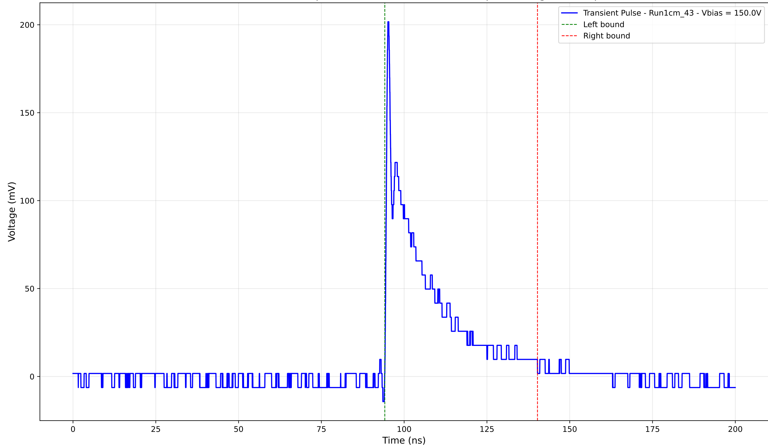
Transient Pulse - Sample: new1cm - Position: 2685.0 \mu\text{m} - Charge: 38.39 pC
