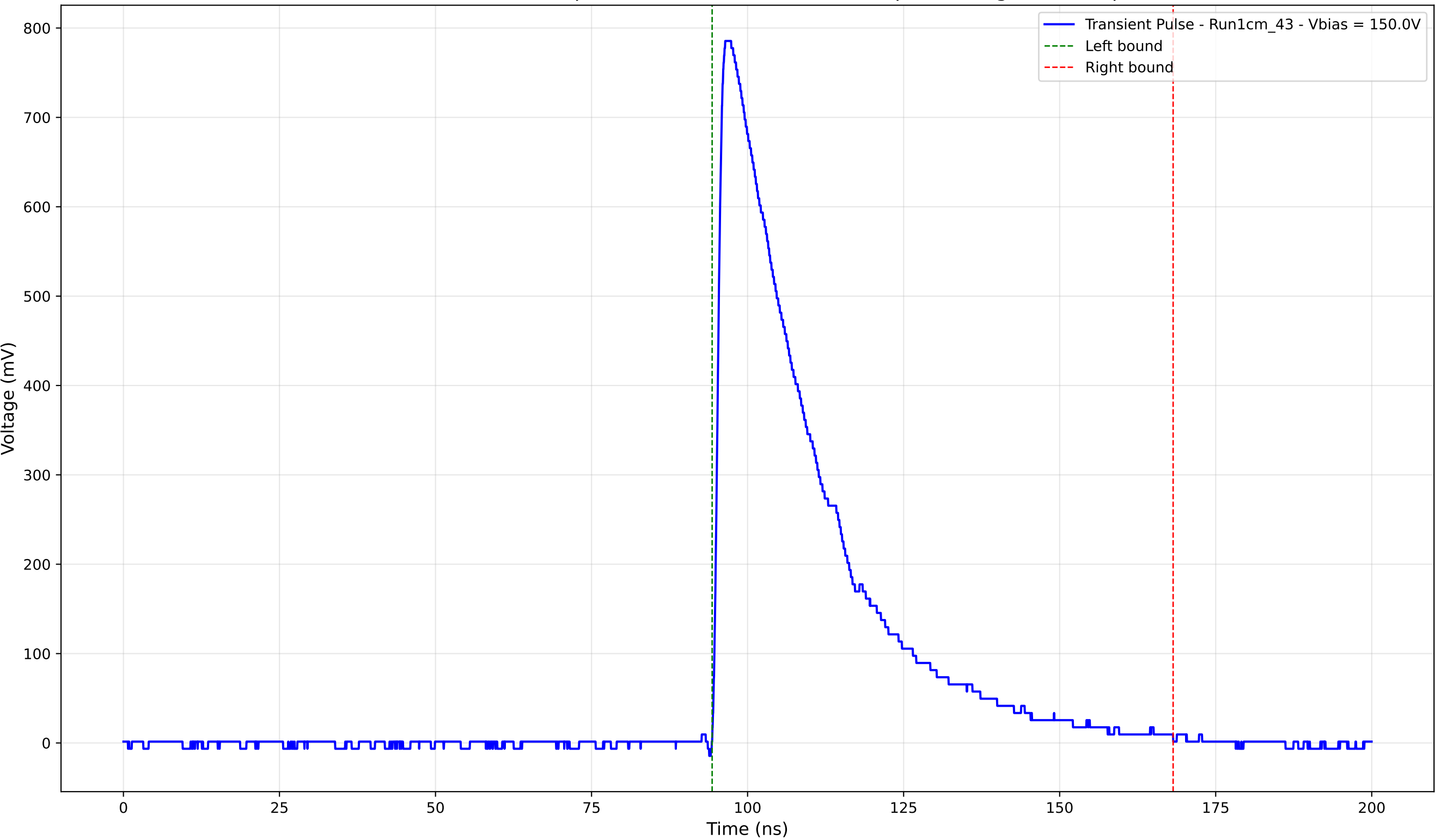
Transient Pulse - Sample: new1cm - Position: 4080.0 \mu\text{m} - Charge: 265.28 pC
