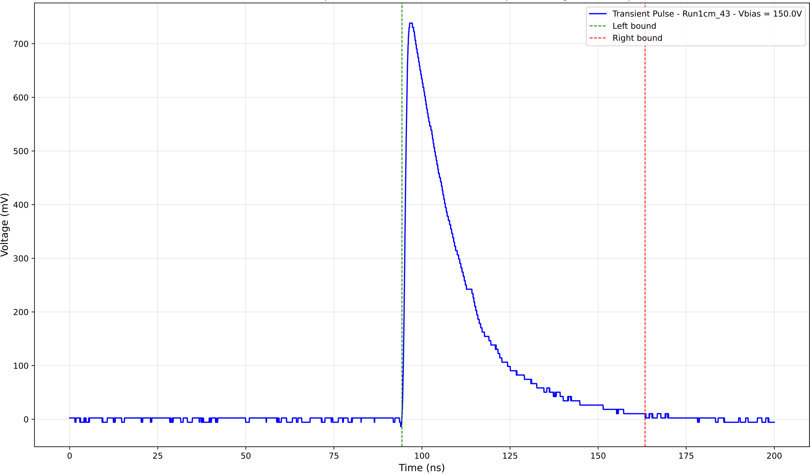
Transient Pulse - Sample: new1cm - Position: 4120.0 \mu\text{m} - Charge: 243.25 pC
