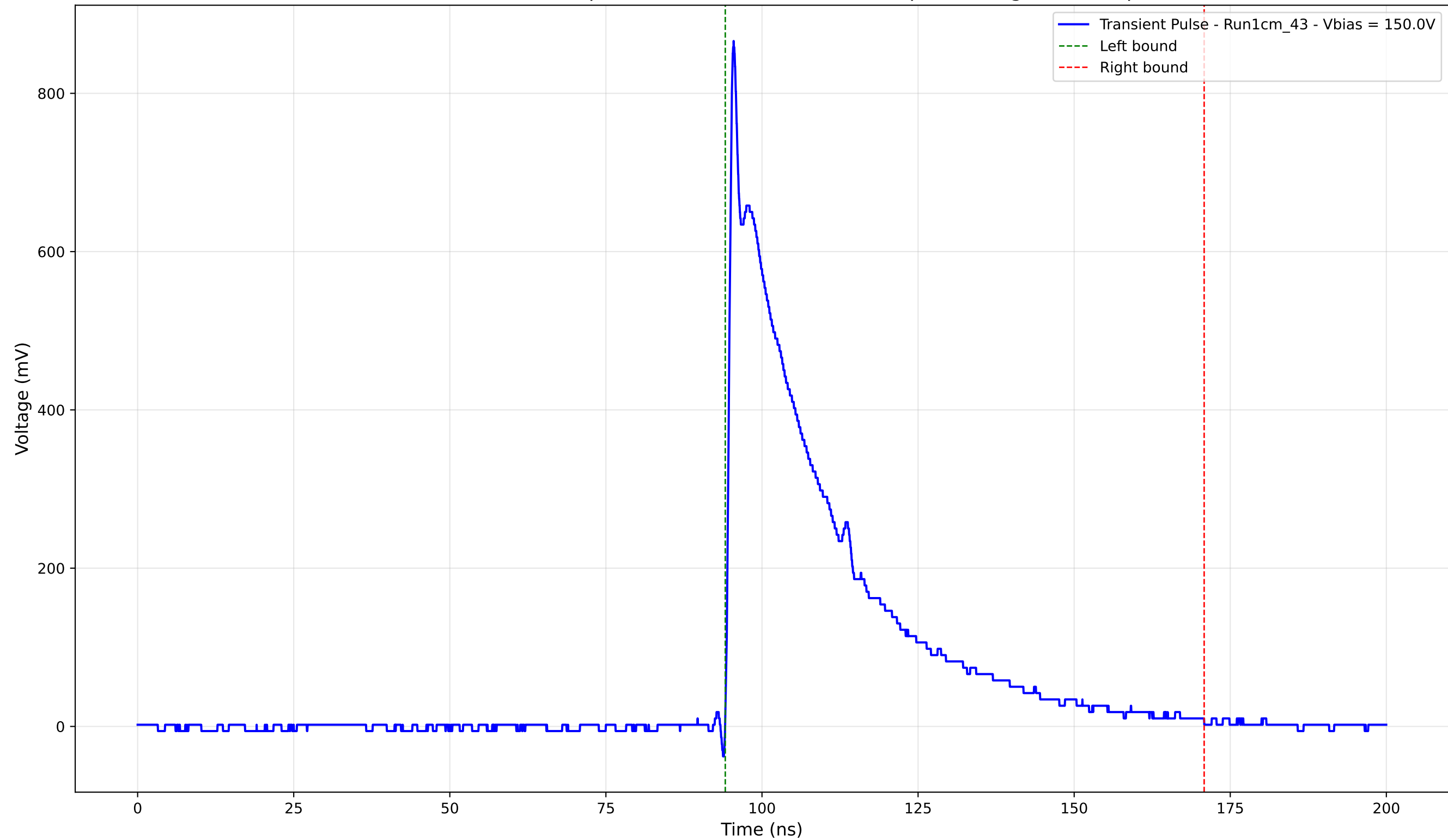
Transient Pulse - Sample: new1cm - Position: 3035.0 \mu\text{m} - Charge: 247.89 pC
