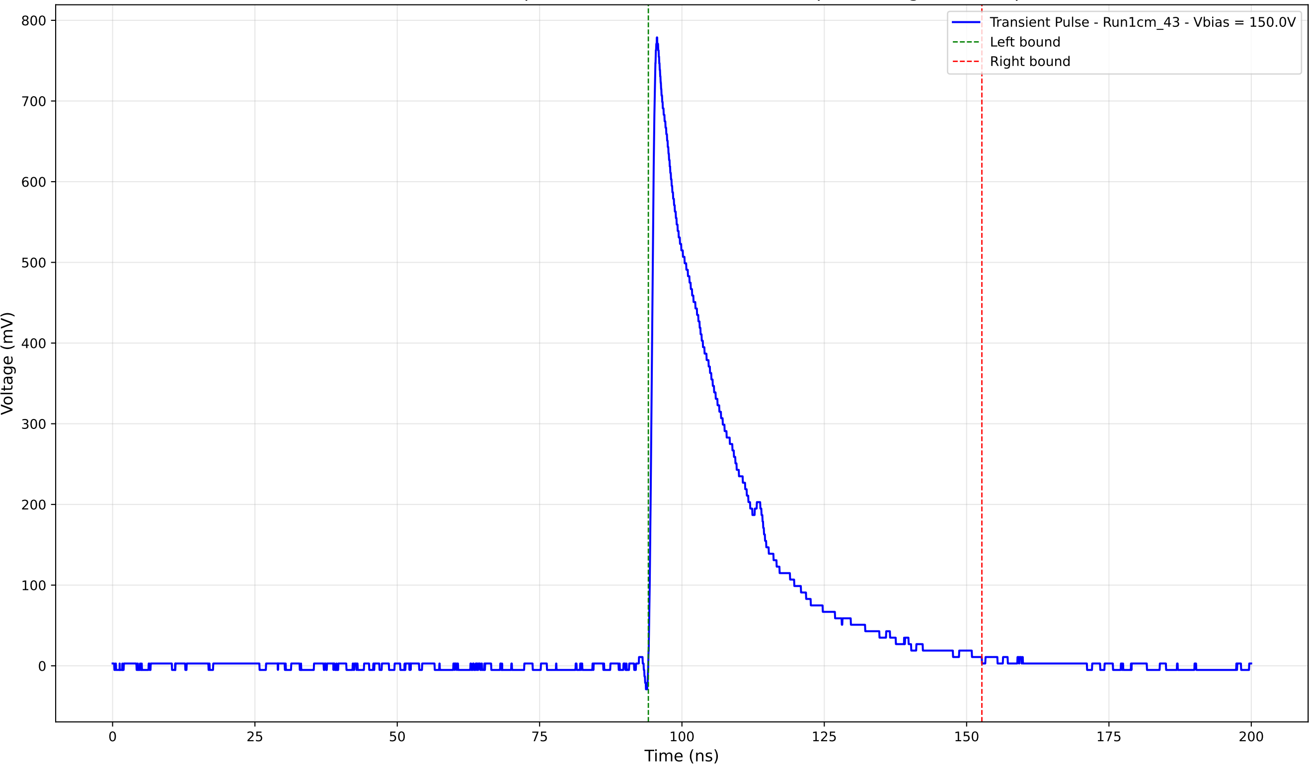
Transient Pulse - Sample: new1cm - Position: 4860.0 \mu\text{m} - Charge: 201.43 pC
