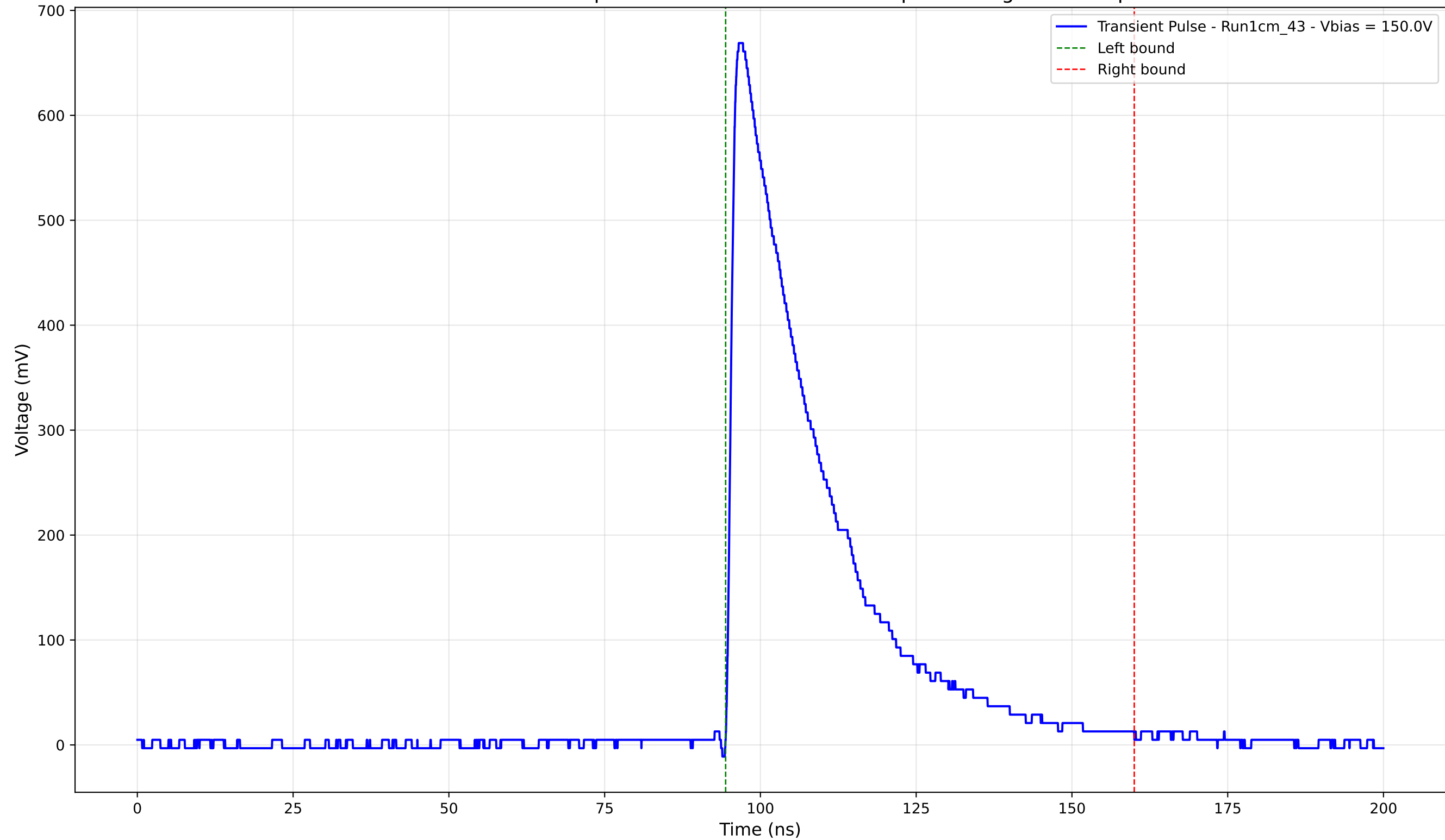
Transient Pulse - Sample: new1cm - Position: 935.0 \mu\text{m} - Charge: 207.43 pC
