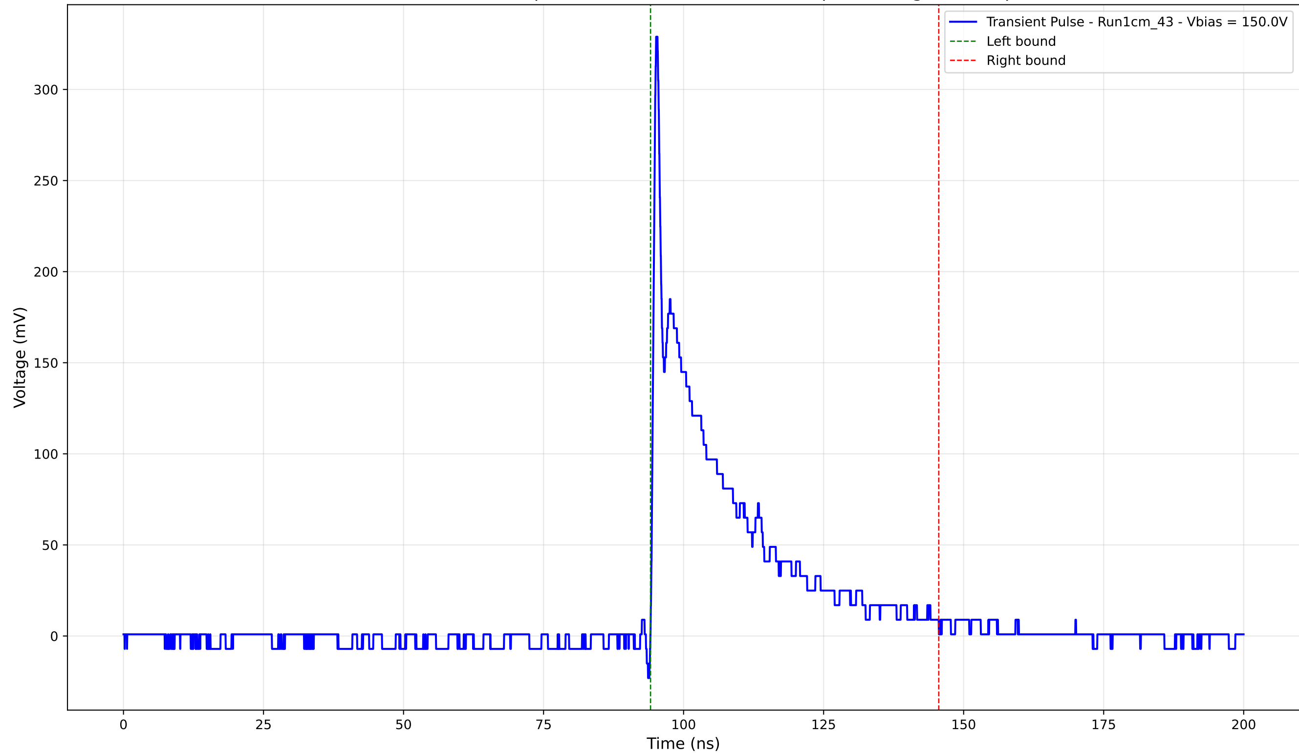
Transient Pulse - Sample: new1cm - Position: 2670.0 \mu\text{m} - Charge: 61.57 pC
