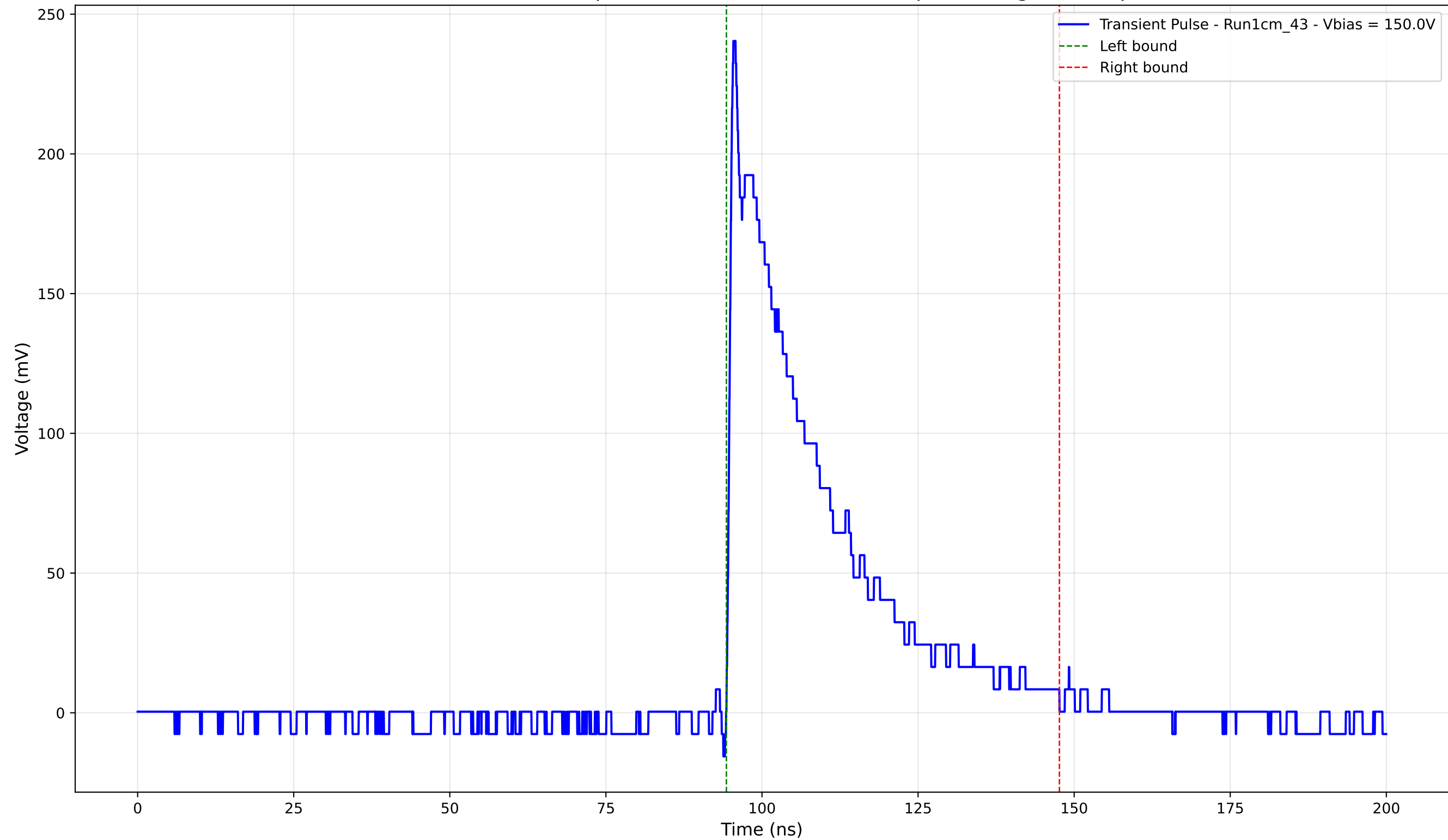
Transient Pulse - Sample: new1cm - Position: 3180.0 \mu\text{m} - Charge: 65.83 pC
