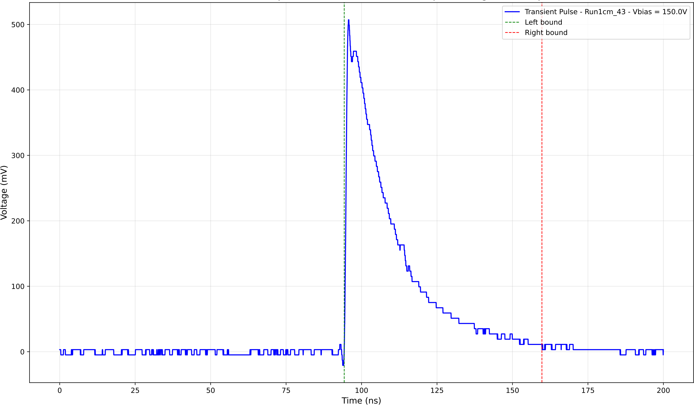
Transient Pulse - Sample: new1cm - Position: 2110.0 \mu\text{m} - Charge: 163.70 pC
