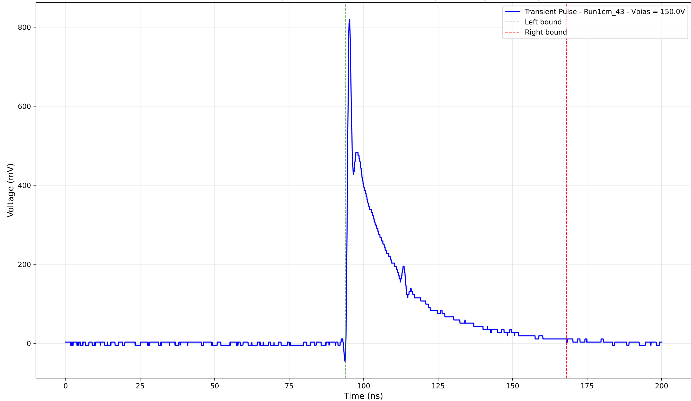
Transient Pulse - Sample: new1cm - Position: 2775.0 \mu\text{m} - Charge: 183.06 pC
