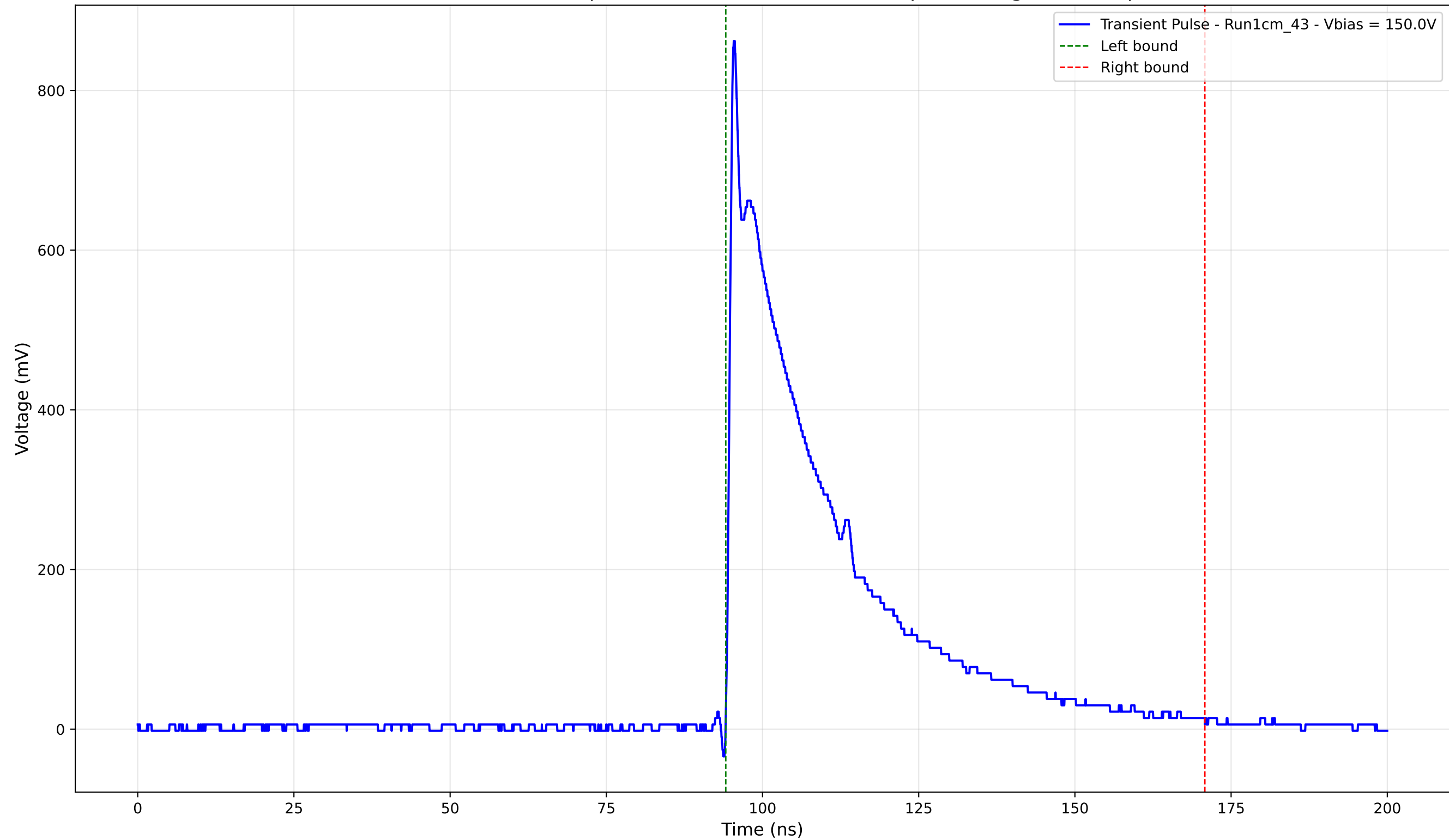
Transient Pulse - Sample: new1cm - Position: 3040.0 \mu\text{m} - Charge: 254.56 pC
