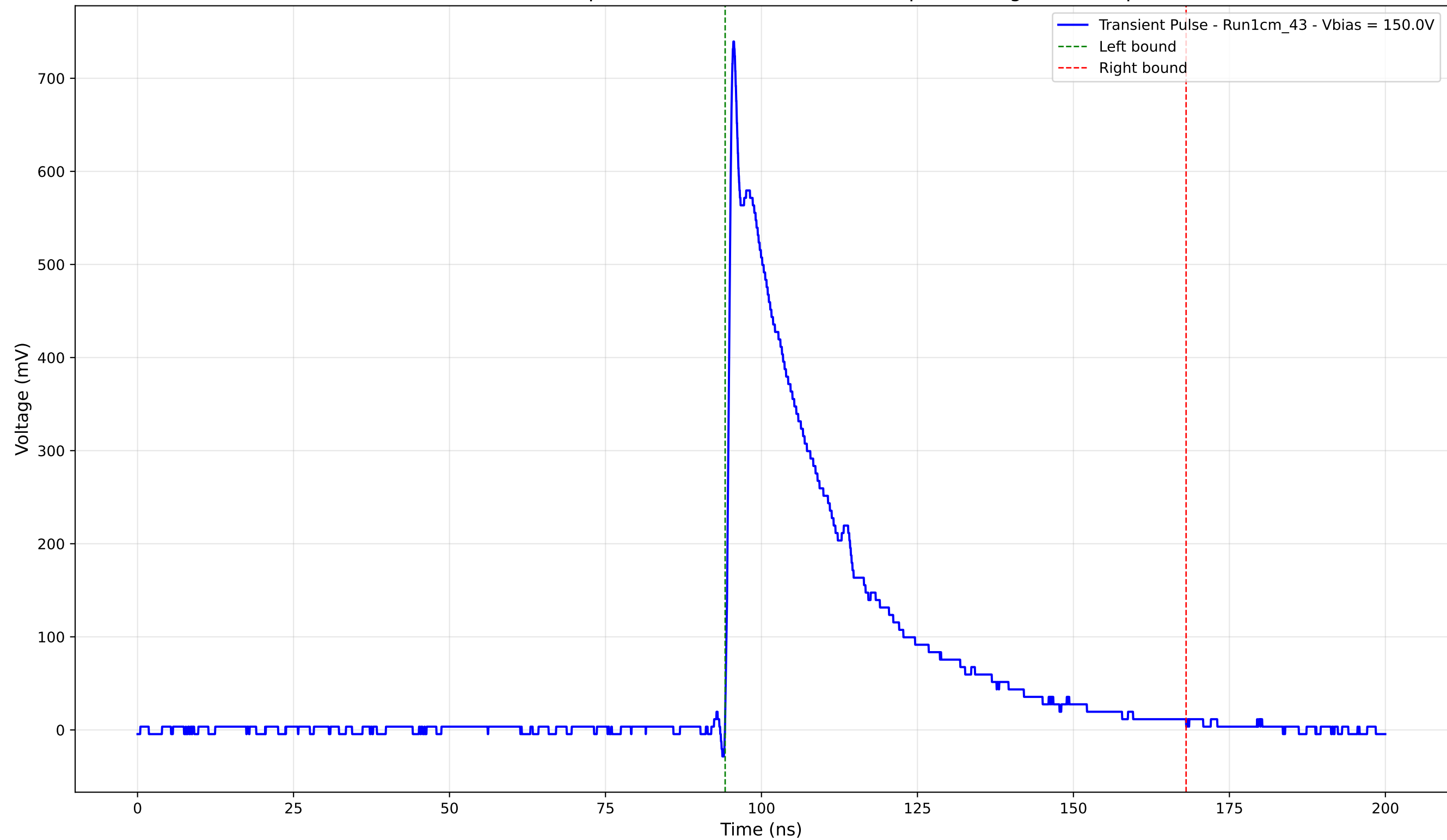
Transient Pulse - Sample: new1cm - Position: 3125.0 \mu\text{m} - Charge: 216.39 pC
