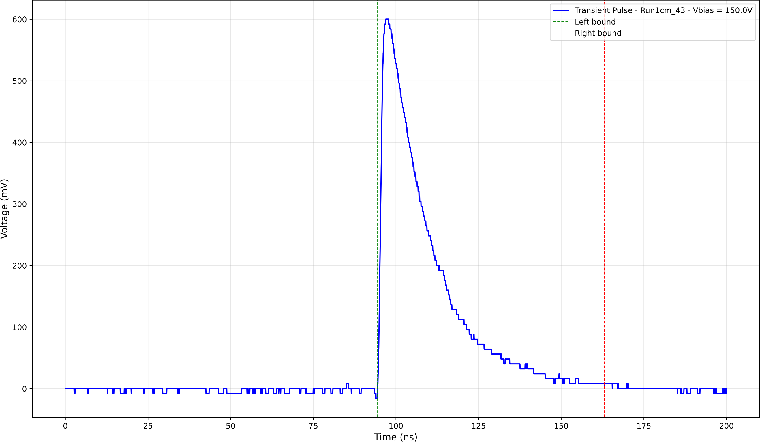
Transient Pulse - Sample: new1cm - Position: 1295.0 \mu\text{m} - Charge: 193.91 pC
