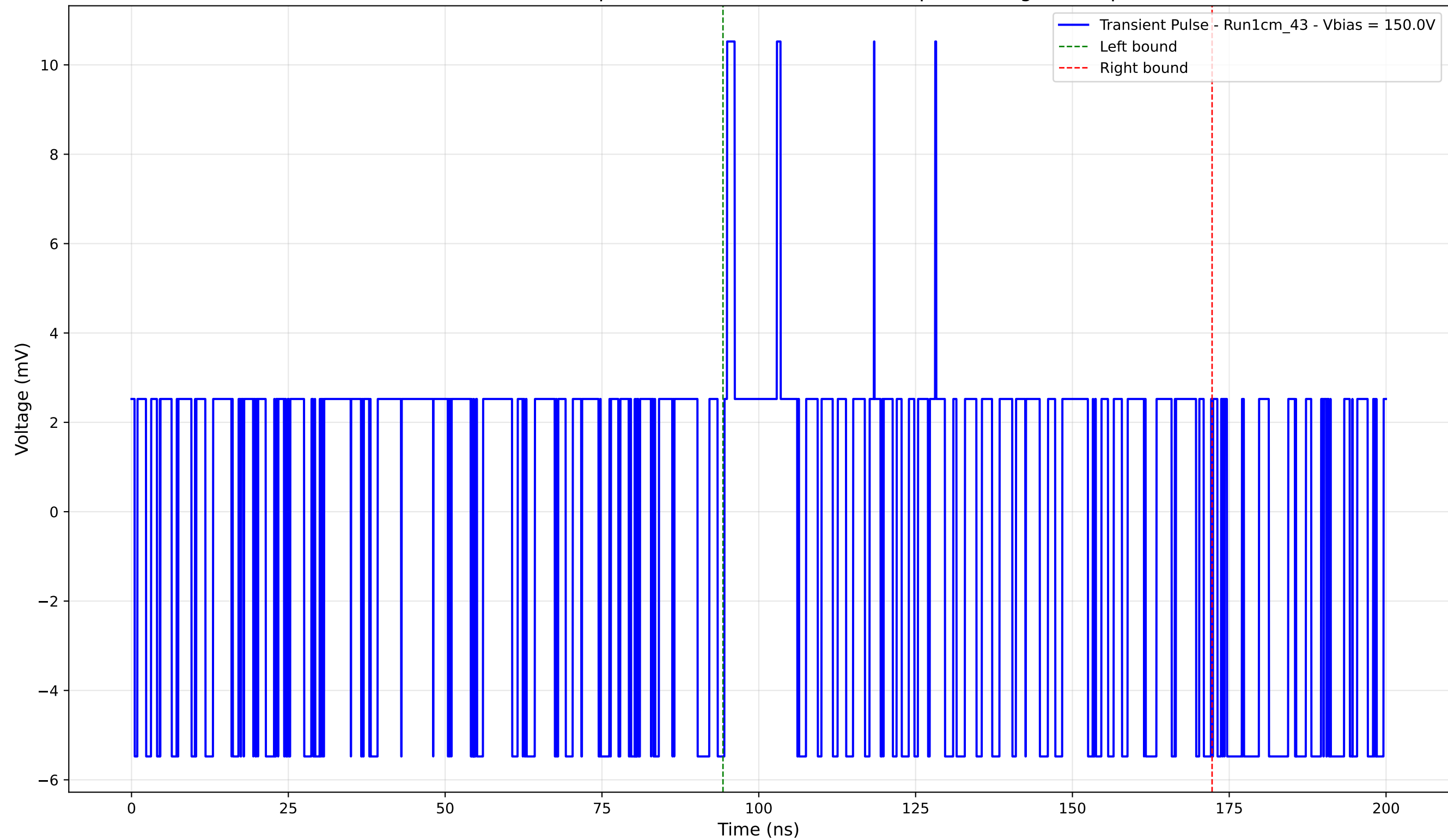
Transient Pulse - Sample: new1cm - Position: 5165.0 \mu\text{m} - Charge: 0.57 pC
