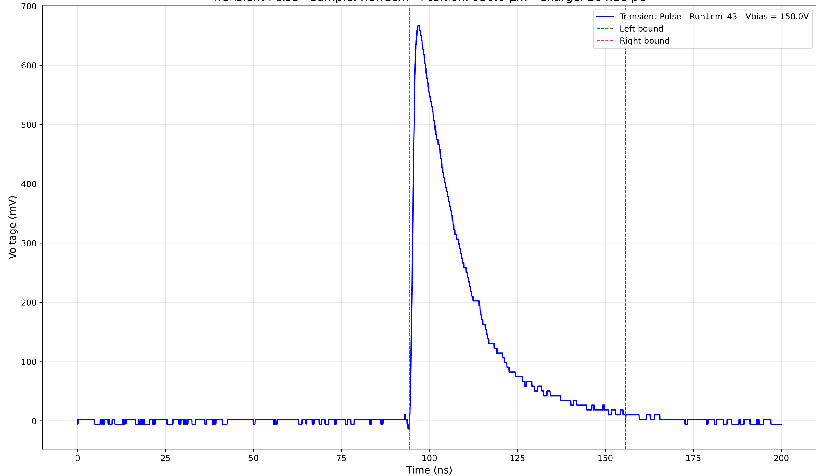
Transient Pulse - Sample: new1cm - Position: 950.0 \mu\text{m} - Charge: 204.18 pC
