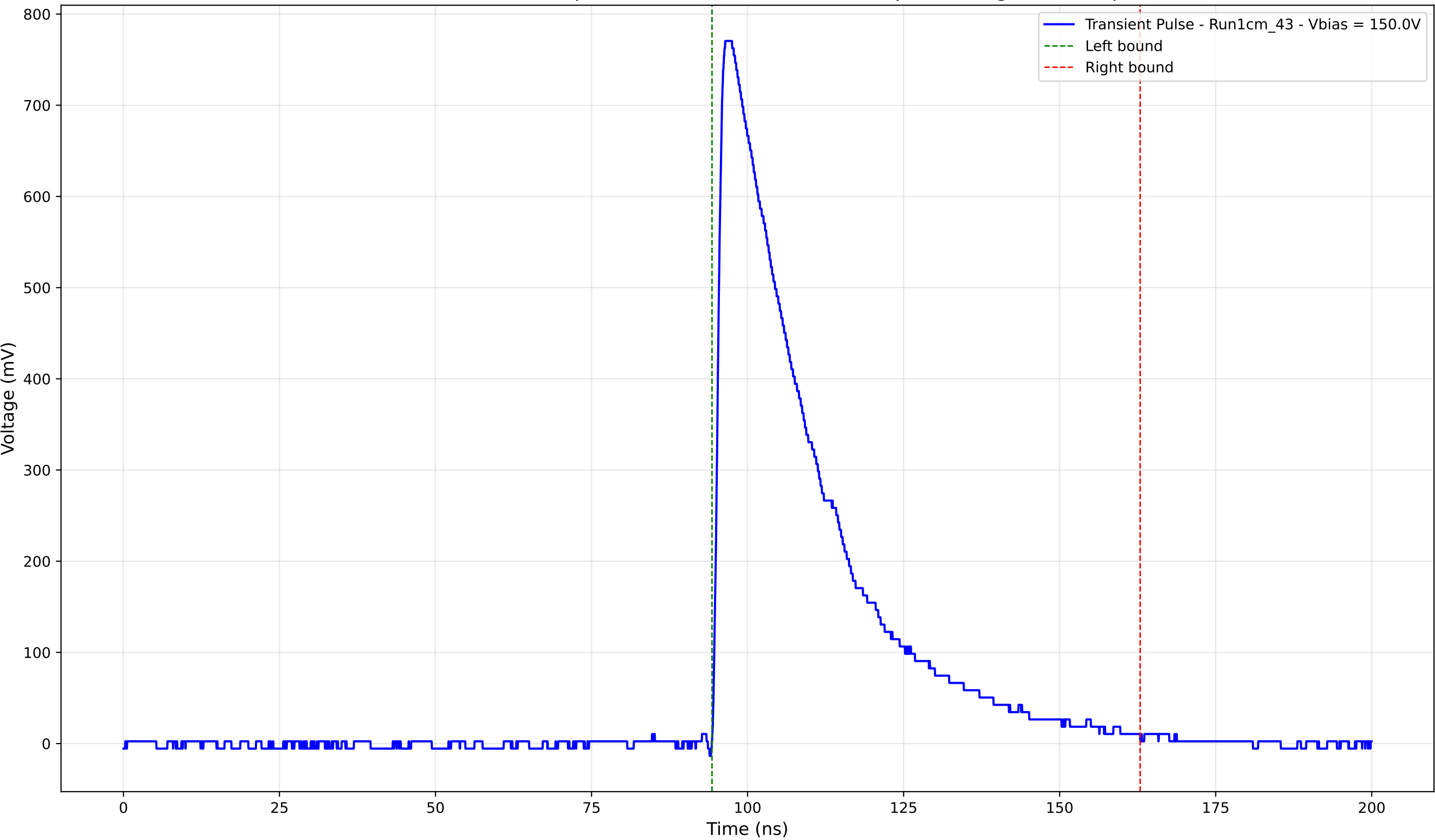
Transient Pulse - Sample: new1cm - Position: 4100.0 \mu\text{m} - Charge: 259.26 pC
