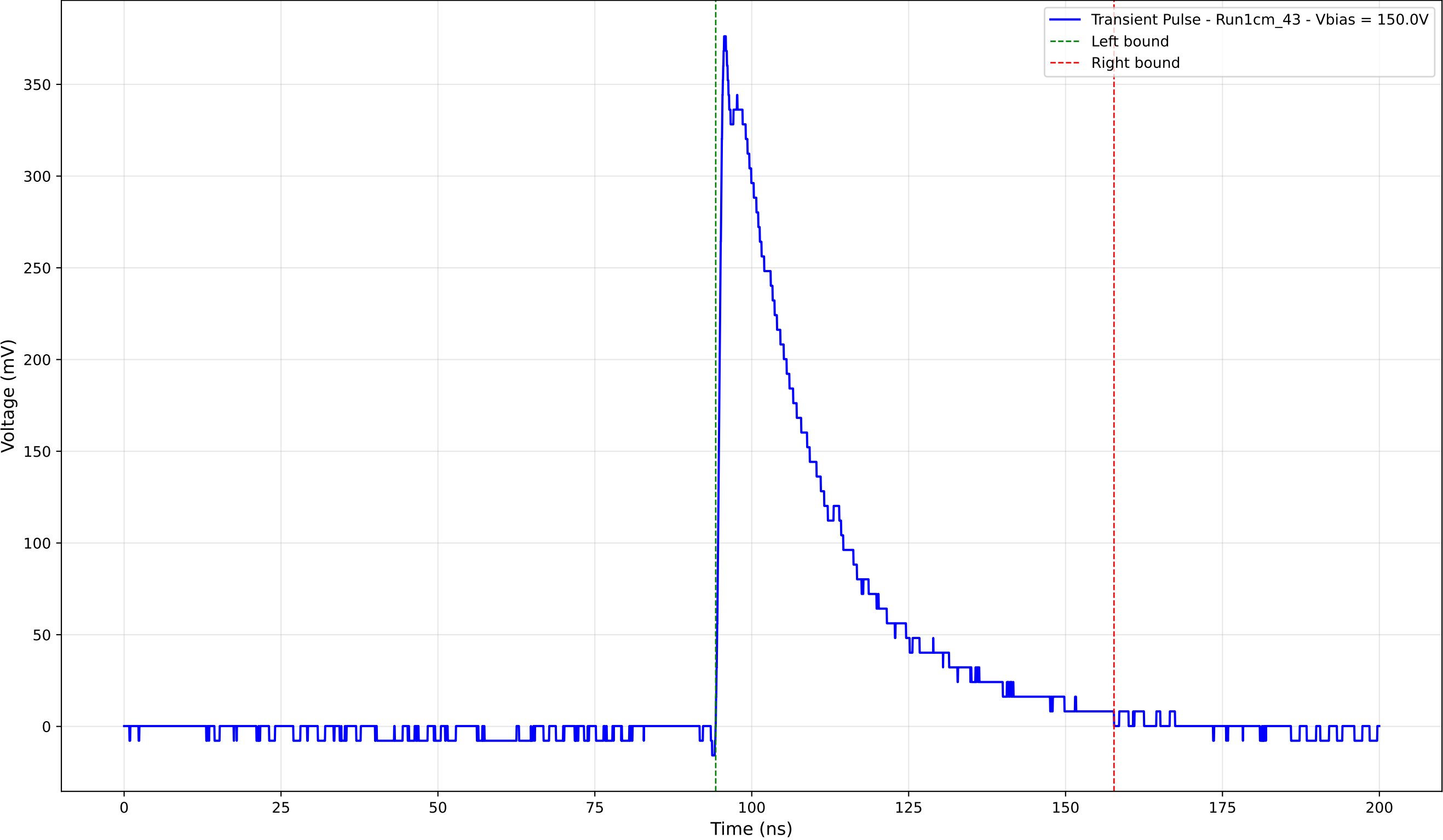
Transient Pulse - Sample: new1cm - Position: 3255.0 \mu\text{m} - Charge: 117.42 pC
