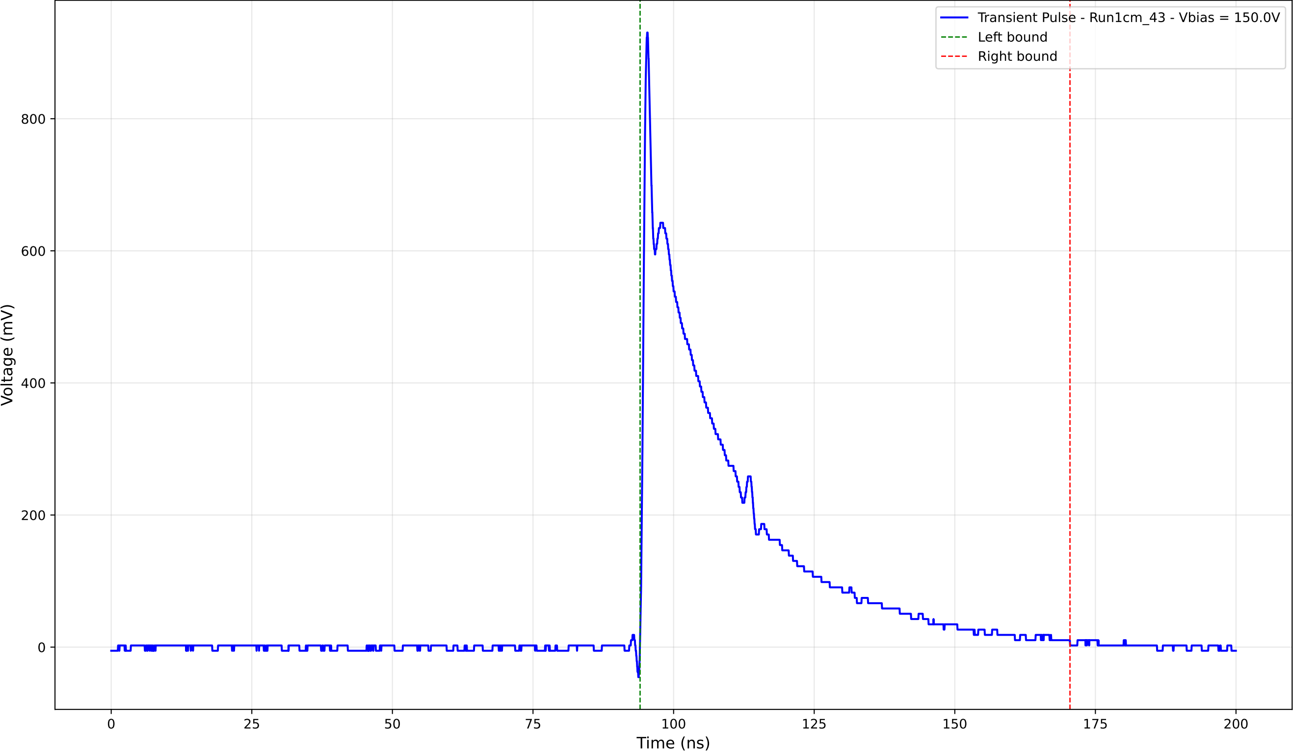
Transient Pulse - Sample: new1cm - Position: 2870.0 \mu\text{m} - Charge: 244.70 pC
