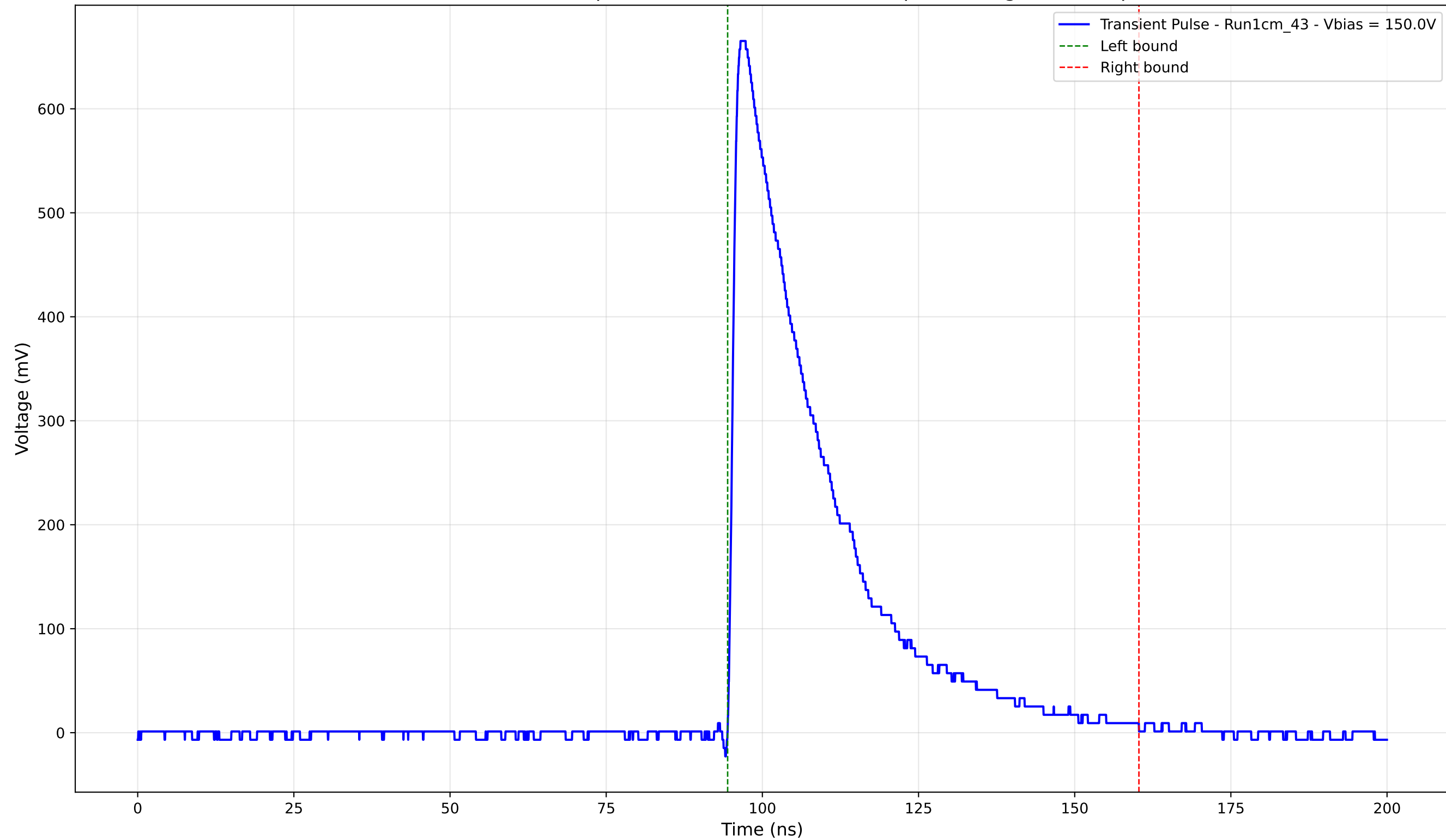
Transient Pulse - Sample: new1cm - Position: 930.0 \mu\text{m} - Charge: 203.71 pC
