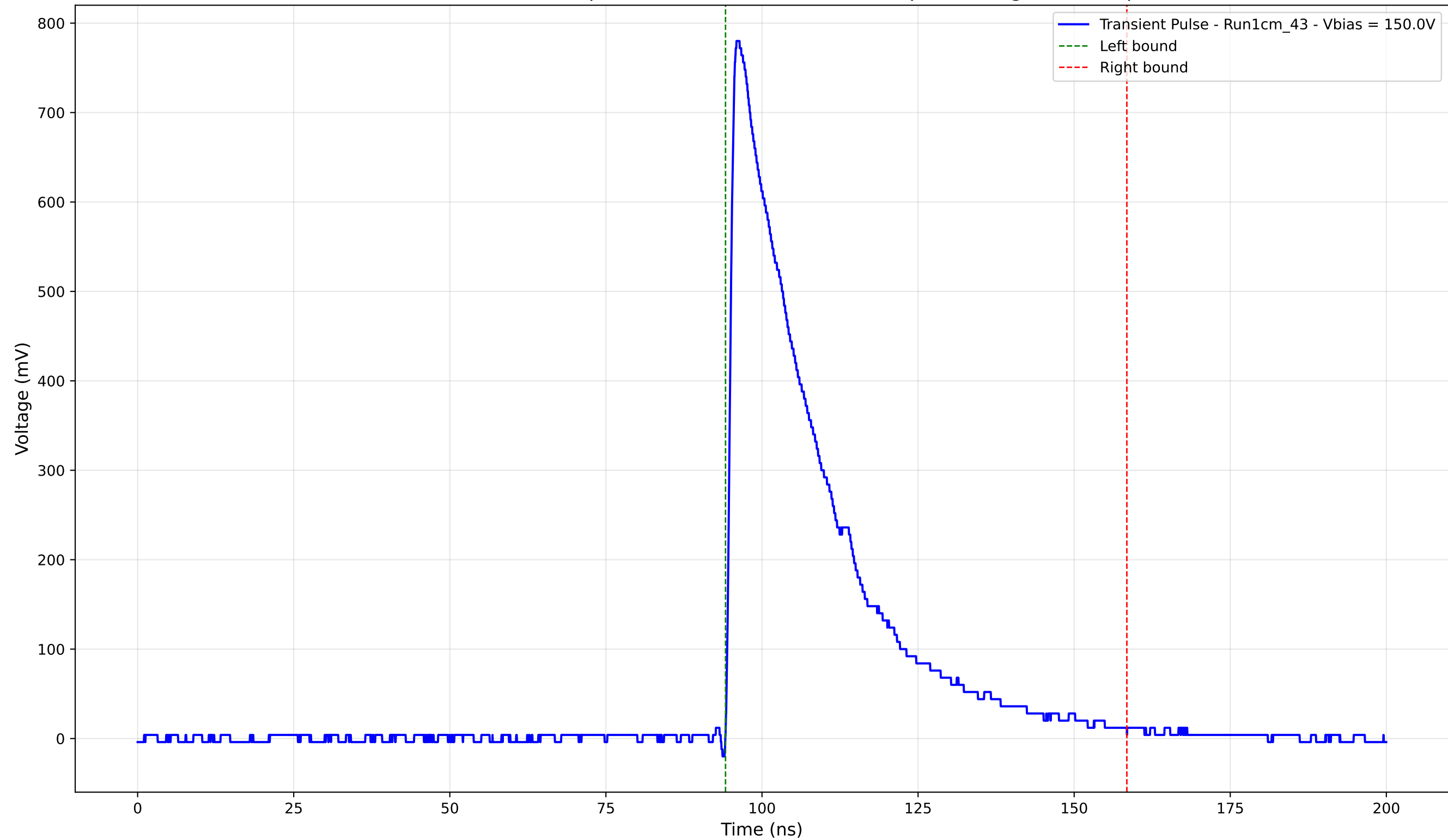
Transient Pulse - Sample: new1cm - Position: 4600.0 \mu\text{m} - Charge: 238.01 pC
