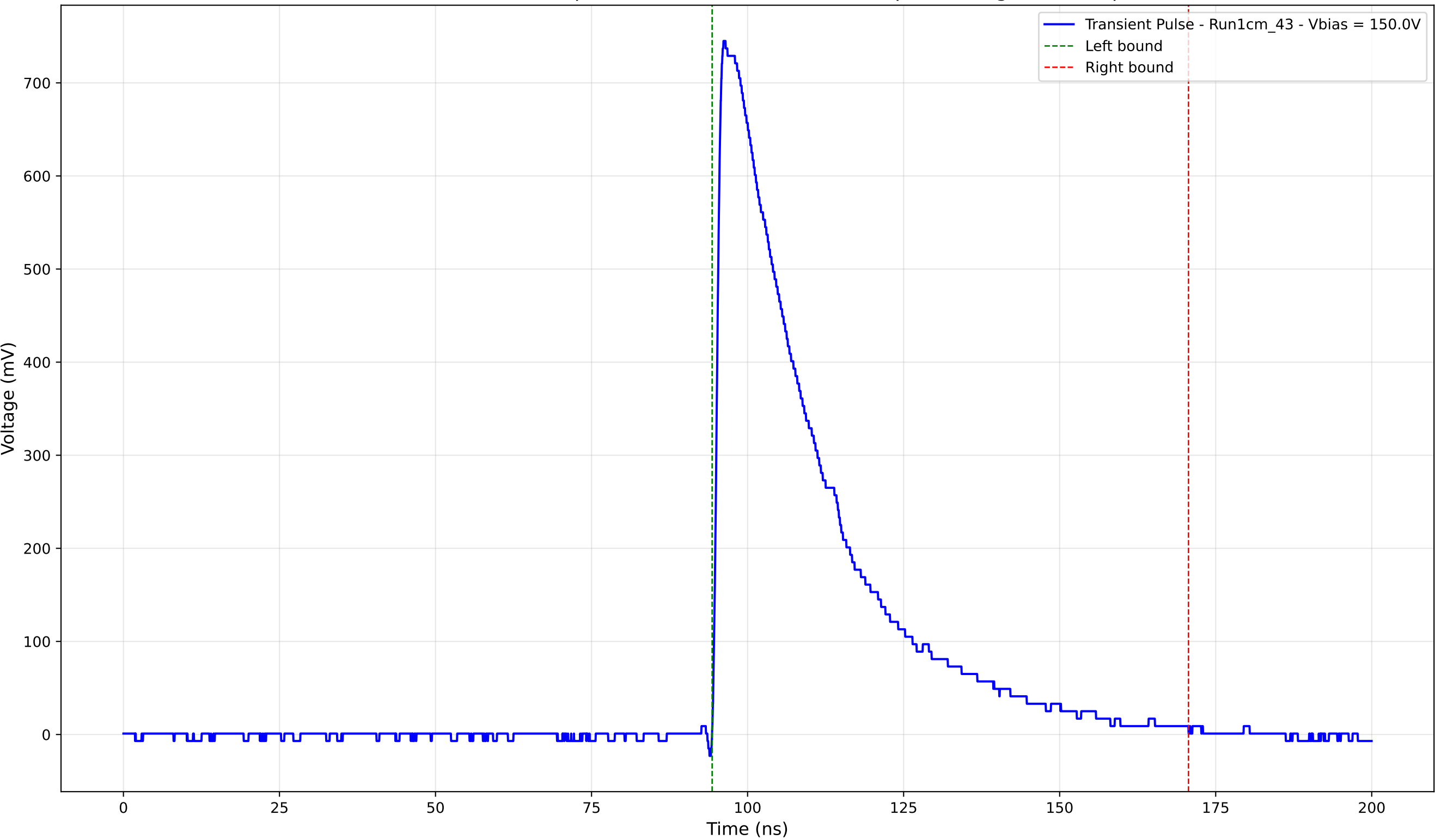
Transient Pulse - Sample: new1cm - Position: 3580.0 \mu\text{m} - Charge: 261.15 pC
