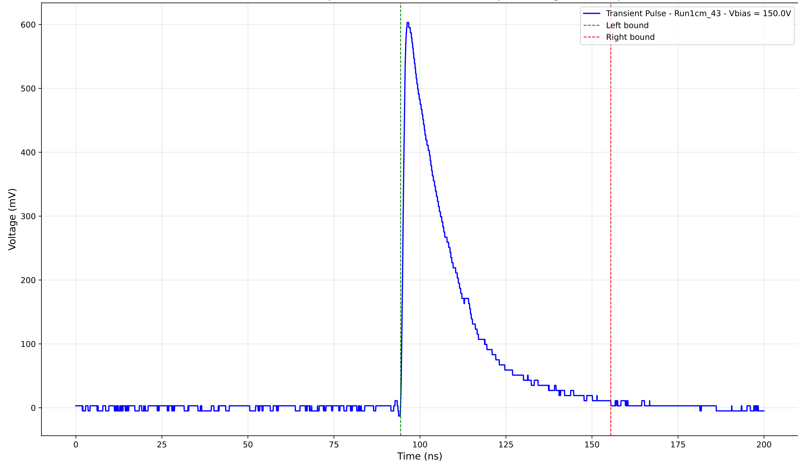
Transient Pulse - Sample: new1cm - Position: 770.0 \mu\text{m} - Charge: 176.62 pC
