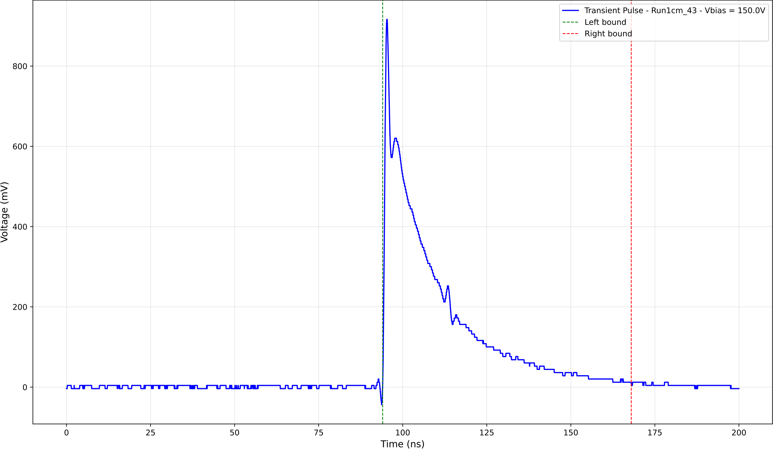
Transient Pulse - Sample: new1cm - Position: 2535.0 \mu\text{m} - Charge: 237.17 pC
