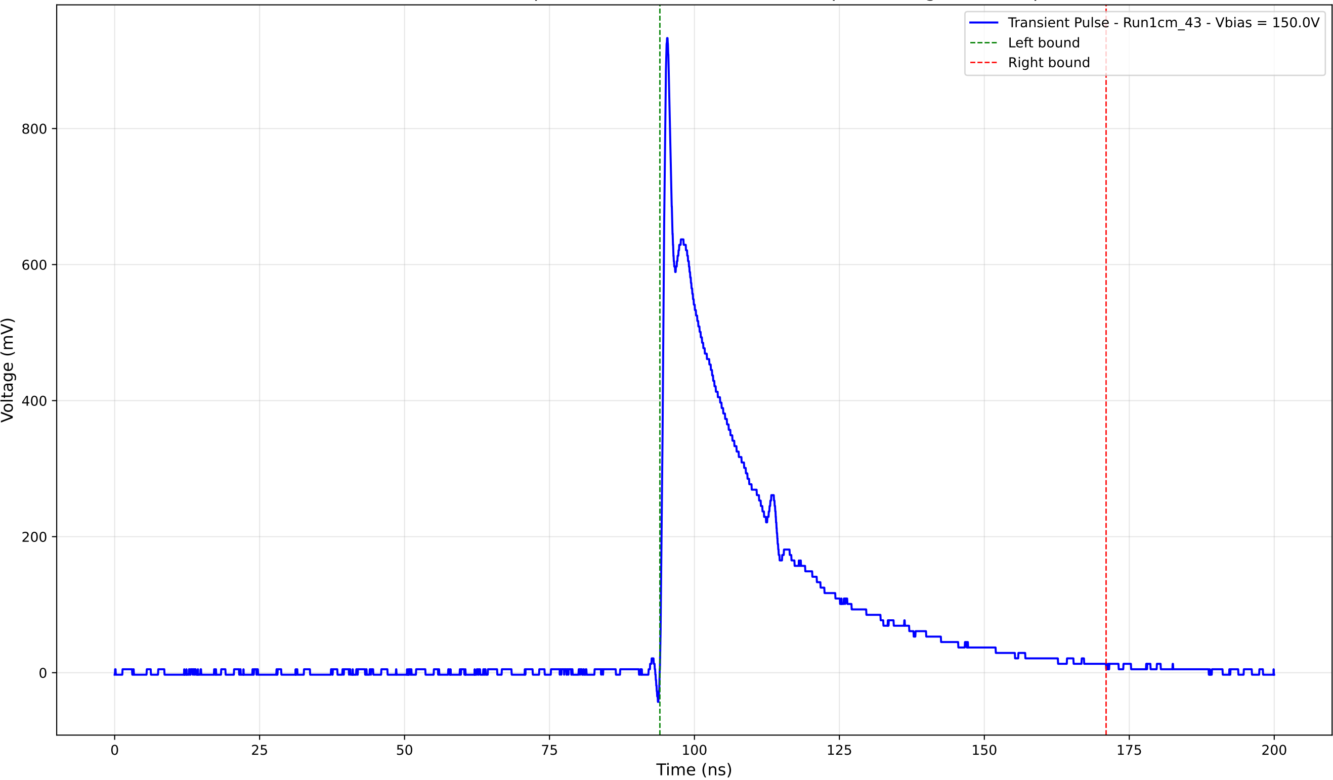
Transient Pulse - Sample: new1cm - Position: 2855.0 \mu\text{m} - Charge: 245.95 pC
