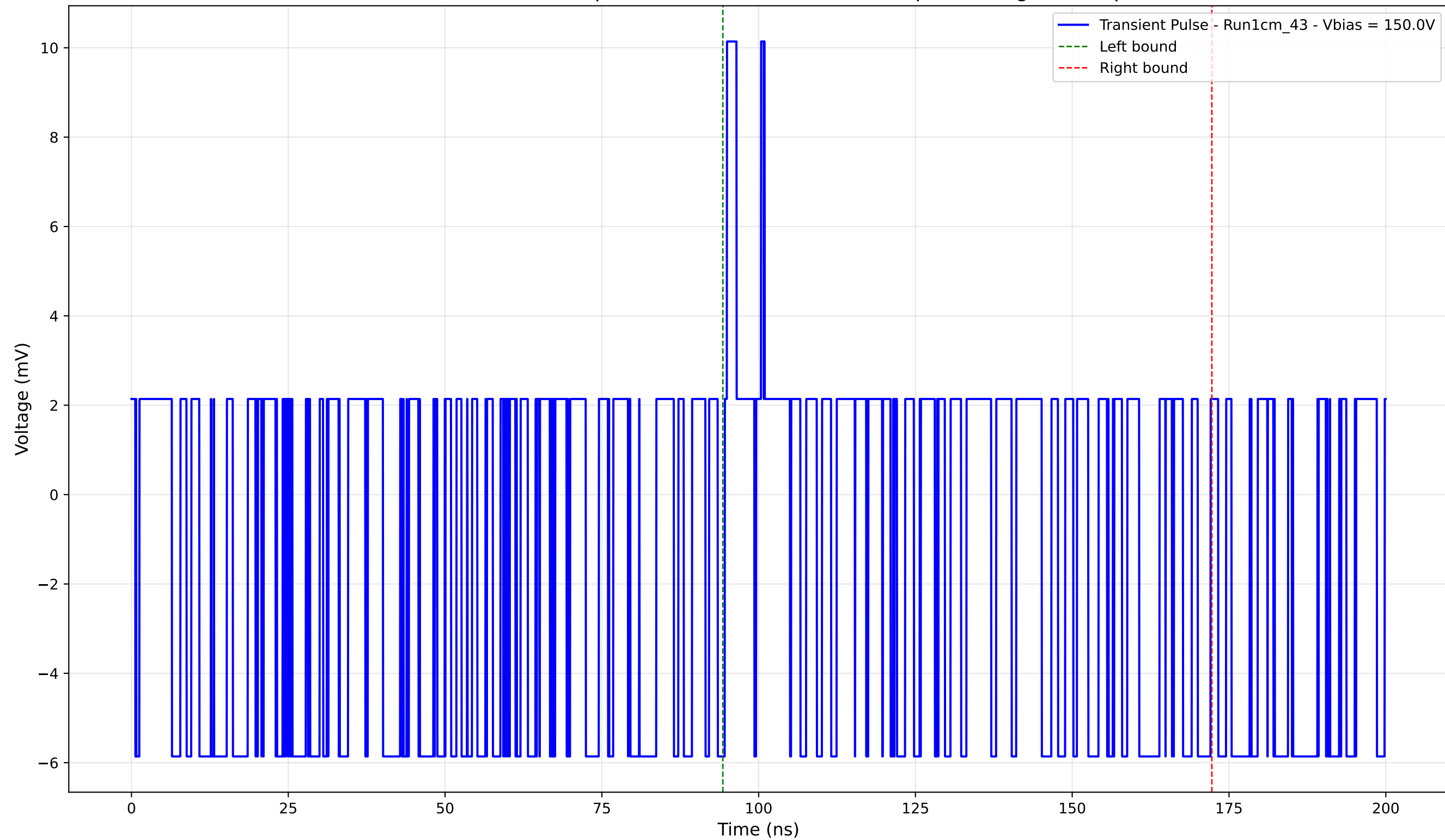
Transient Pulse - Sample: new1cm - Position: 5115.0 \mu\text{m} - Charge: -0.11 pC
