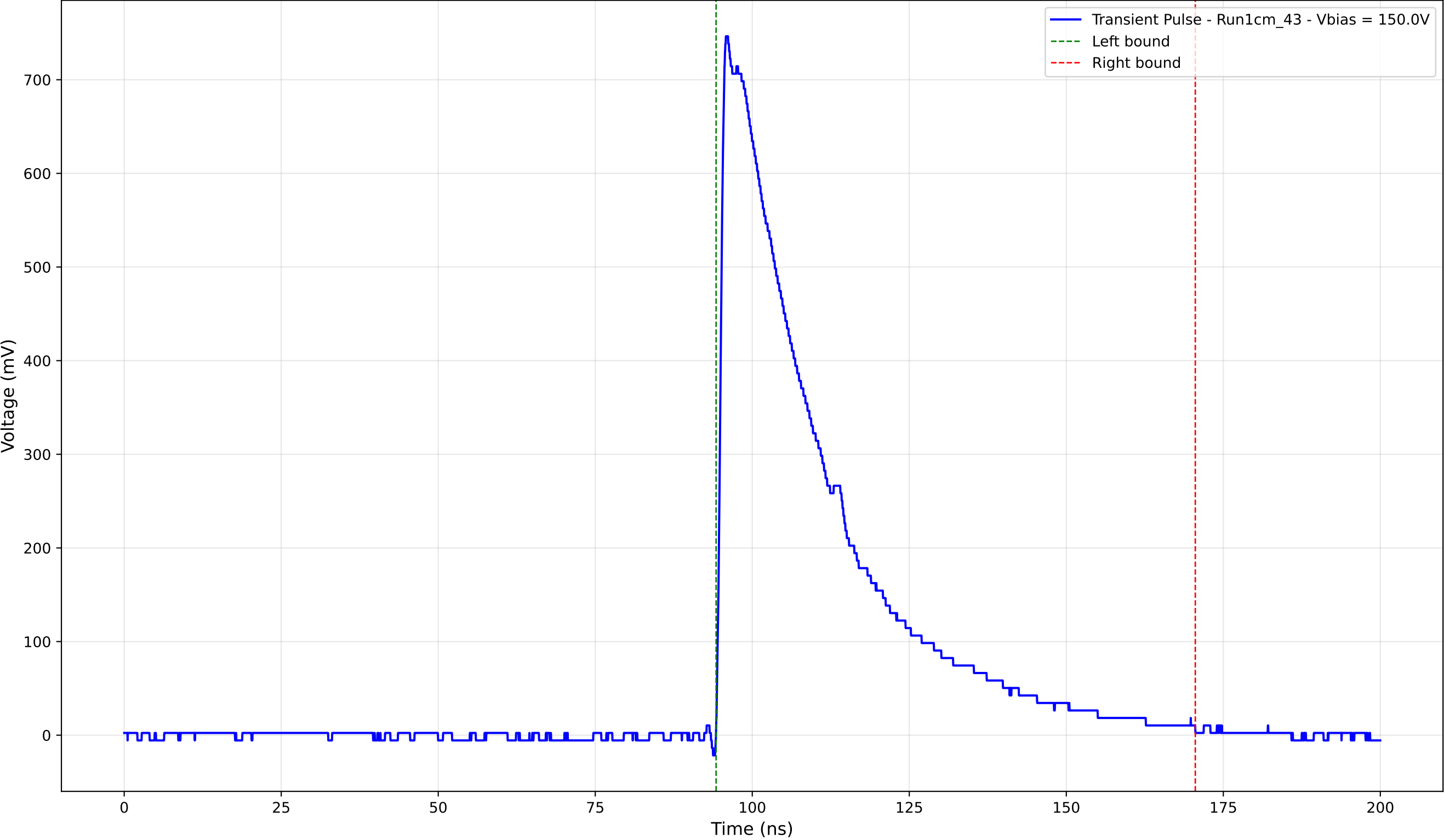
Transient Pulse - Sample: new1cm - Position: 3395.0 \mu\text{m} - Charge: 261.84 pC
