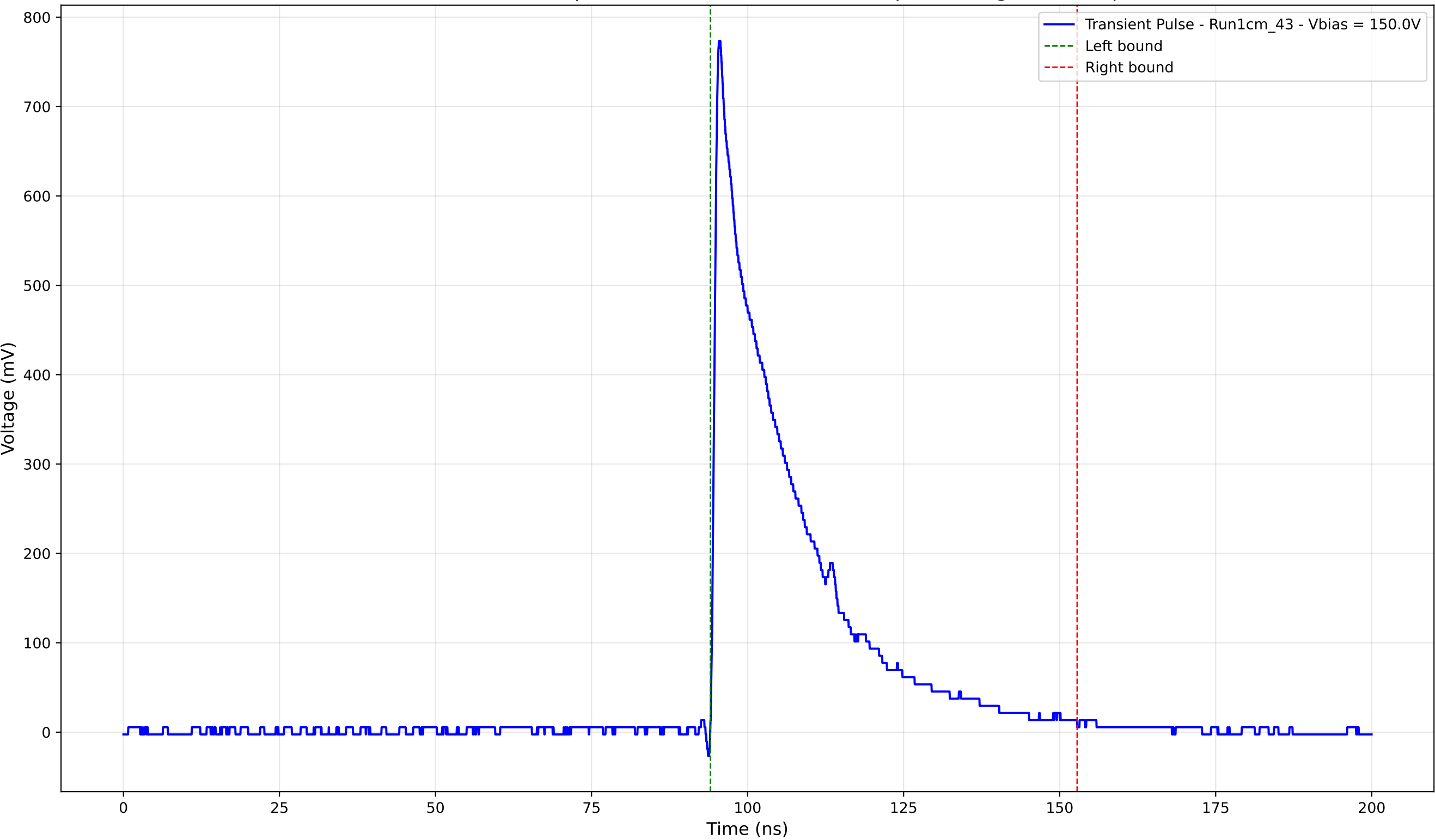
Transient Pulse - Sample: new1cm - Position: 4950.0 \mu\text{m} - Charge: 188.03 pC
