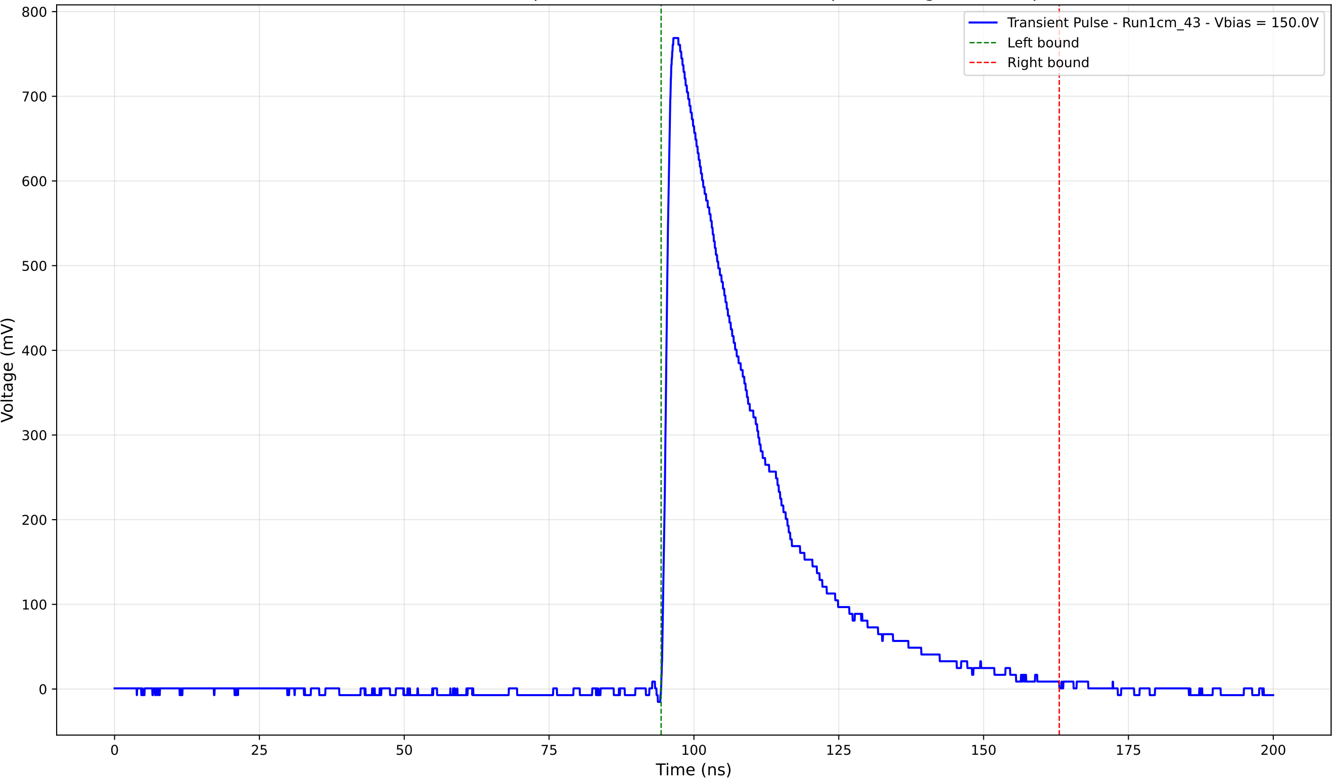
Transient Pulse - Sample: new1cm - Position: 4105.0 \mu\text{m} - Charge: 254.69 pC
