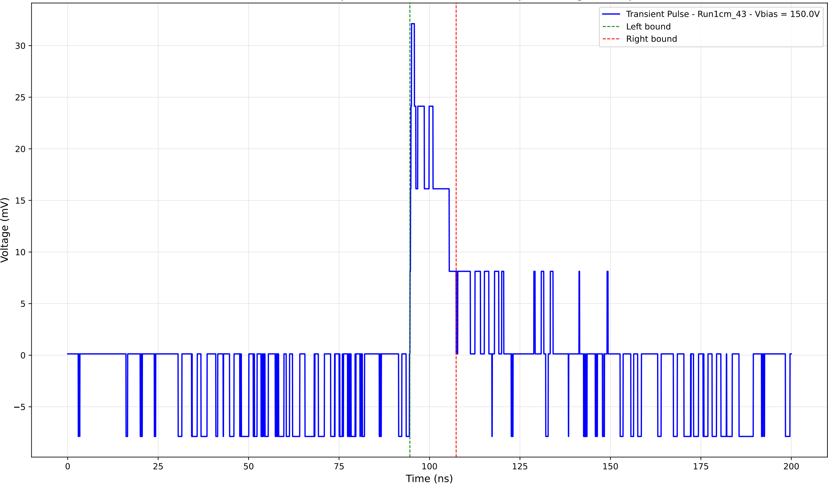
Transient Pulse - Sample: new1cm - Position: 150.0 \mu\text{m} - Charge: 4.60 pC
