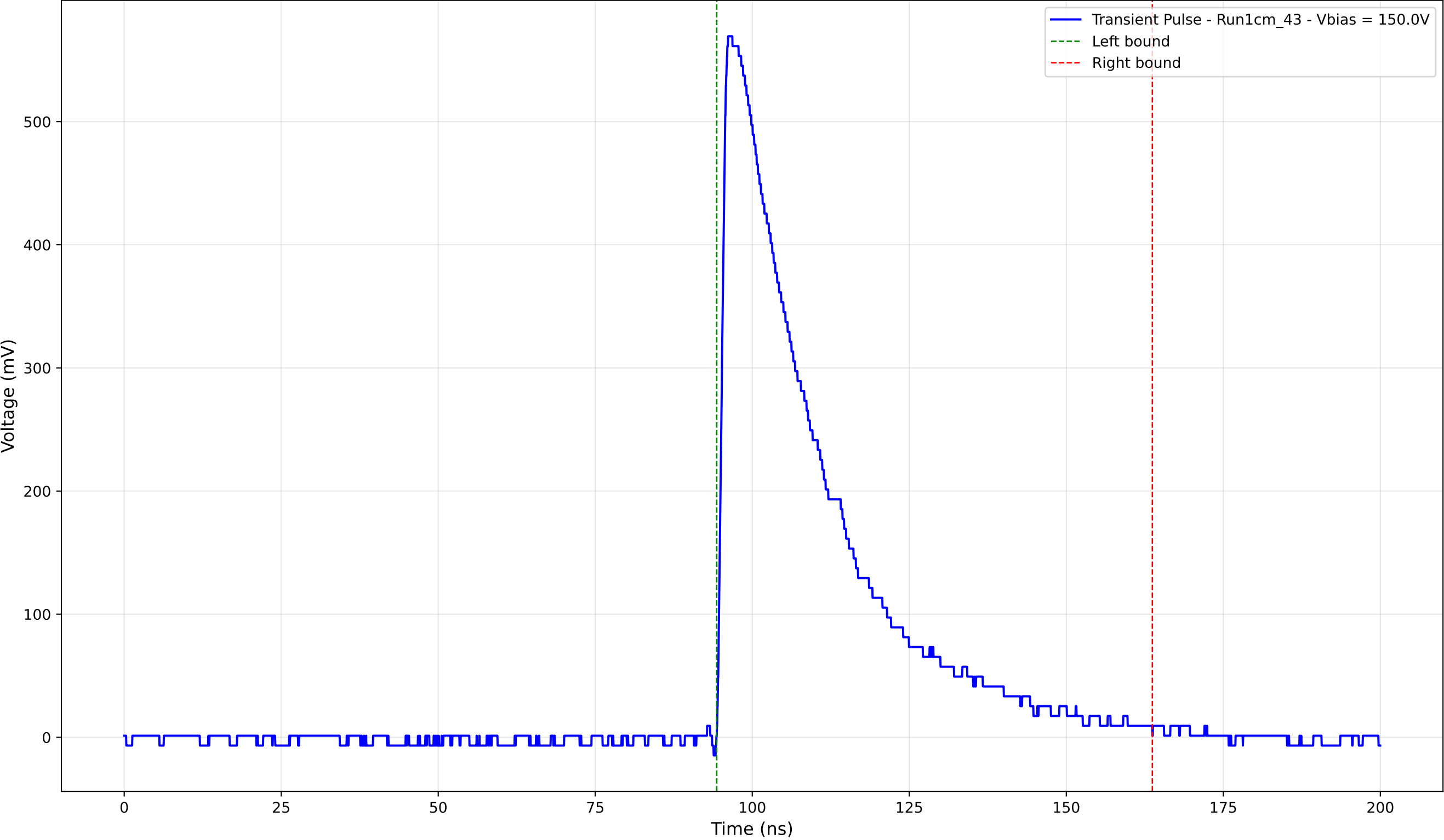
Transient Pulse - Sample: new1cm - Position: 3640.0 \mu\text{m} - Charge: 192.39 pC
