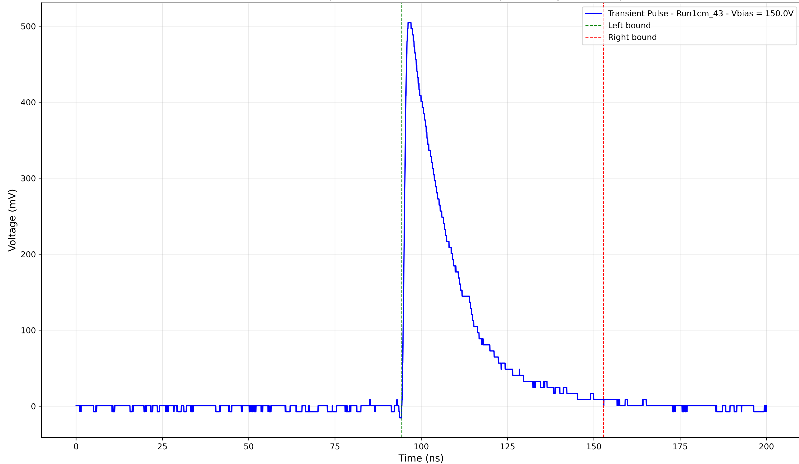
Transient Pulse - Sample: new1cm - Position: 750.0 \mu\text{m} - Charge: 144.95 pC
