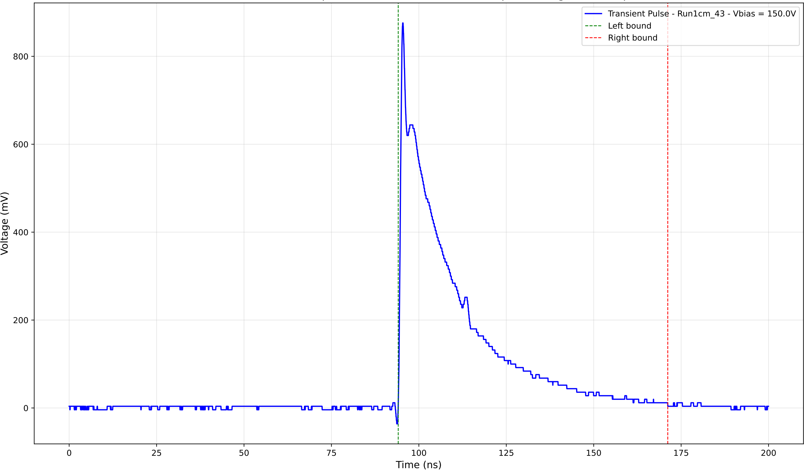
Transient Pulse - Sample: new1cm - Position: 2995.0 \mu\text{m} - Charge: 247.02 pC
