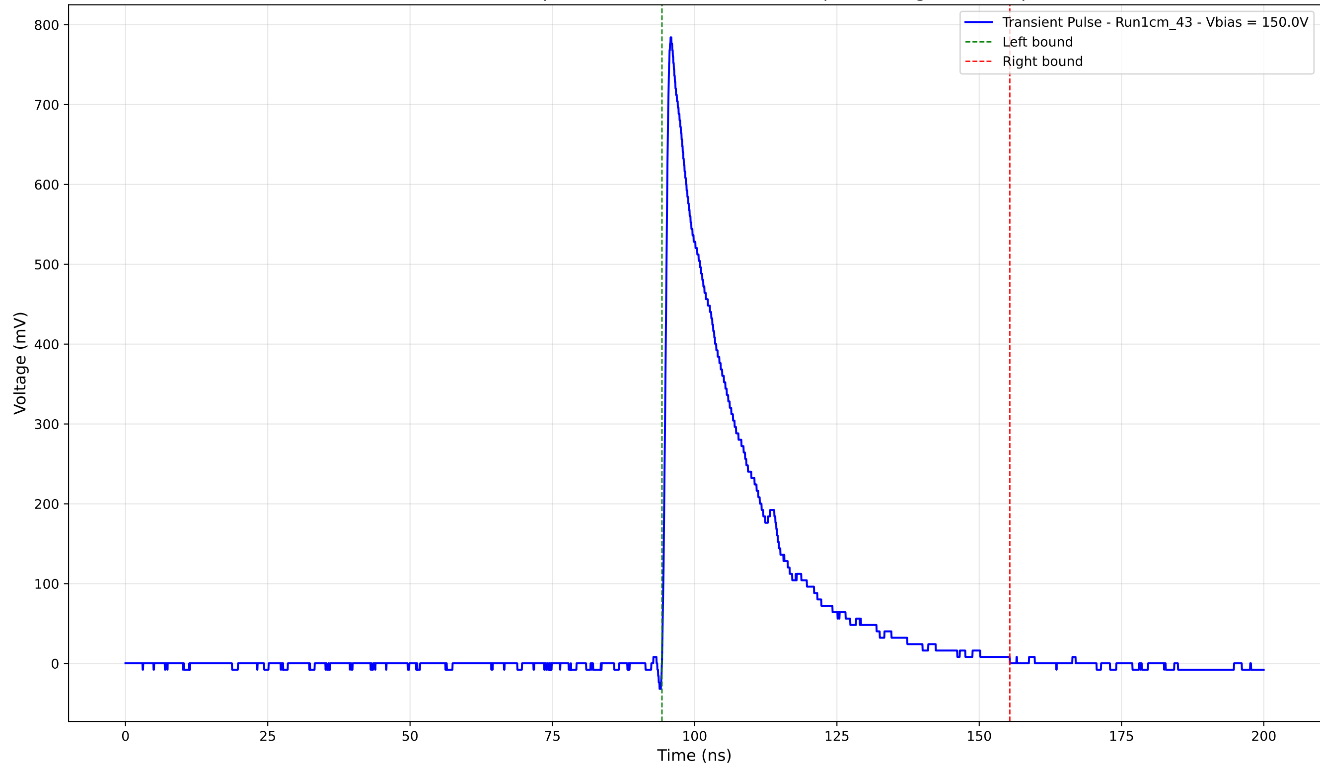
Transient Pulse - Sample: new1cm - Position: 455.0 \mu\text{m} - Charge: 196.90 pC
