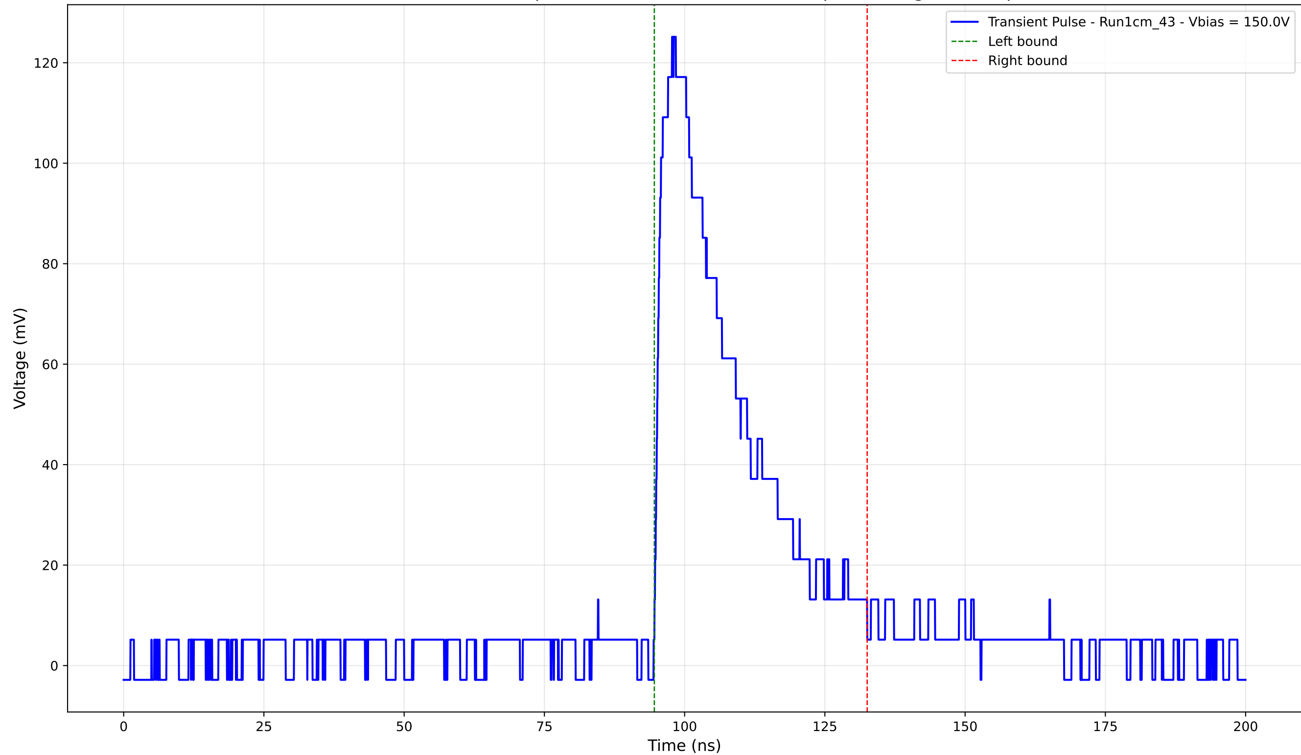
Transient Pulse - Sample: new1cm - Position: 4220.0 \mu\text{m} - Charge: 38.08 pC
