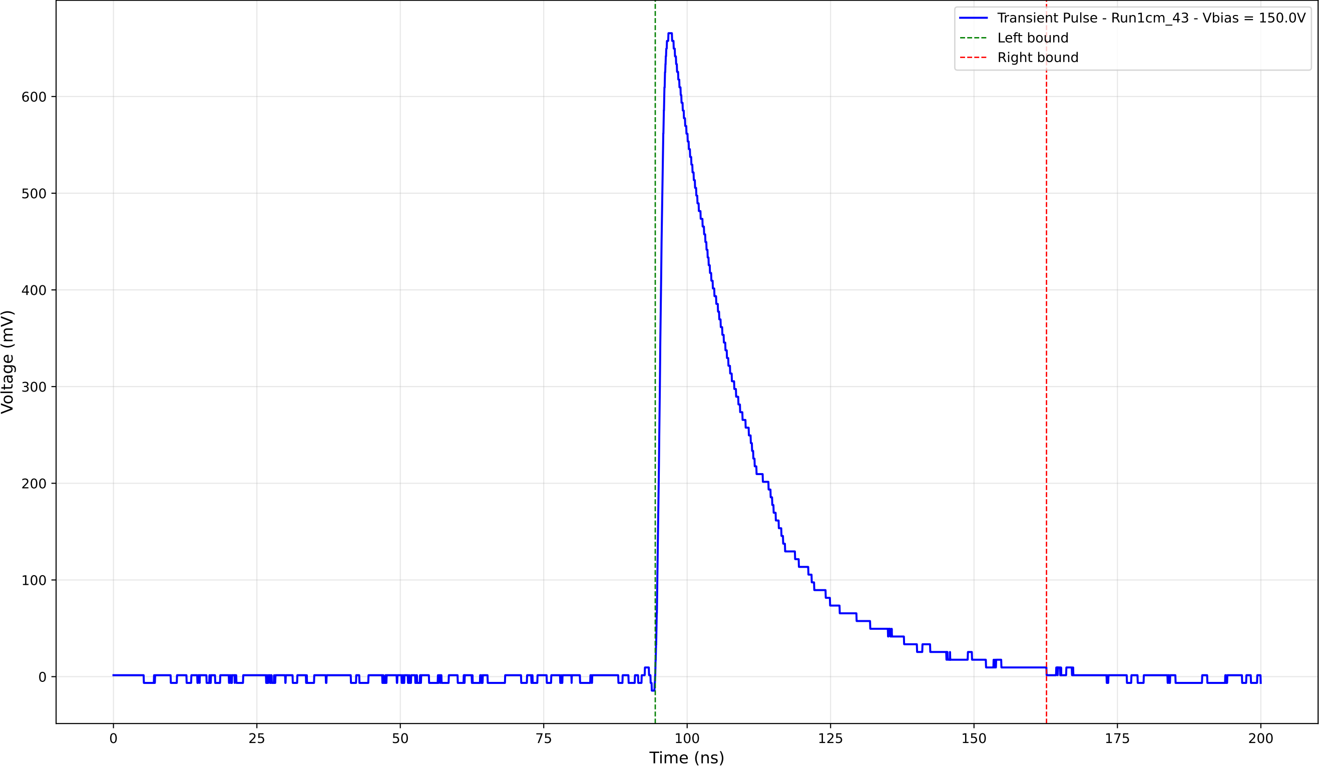
Transient Pulse - Sample: new1cm - Position: 1005.0 \mu\text{m} - Charge: 207.09 pC
