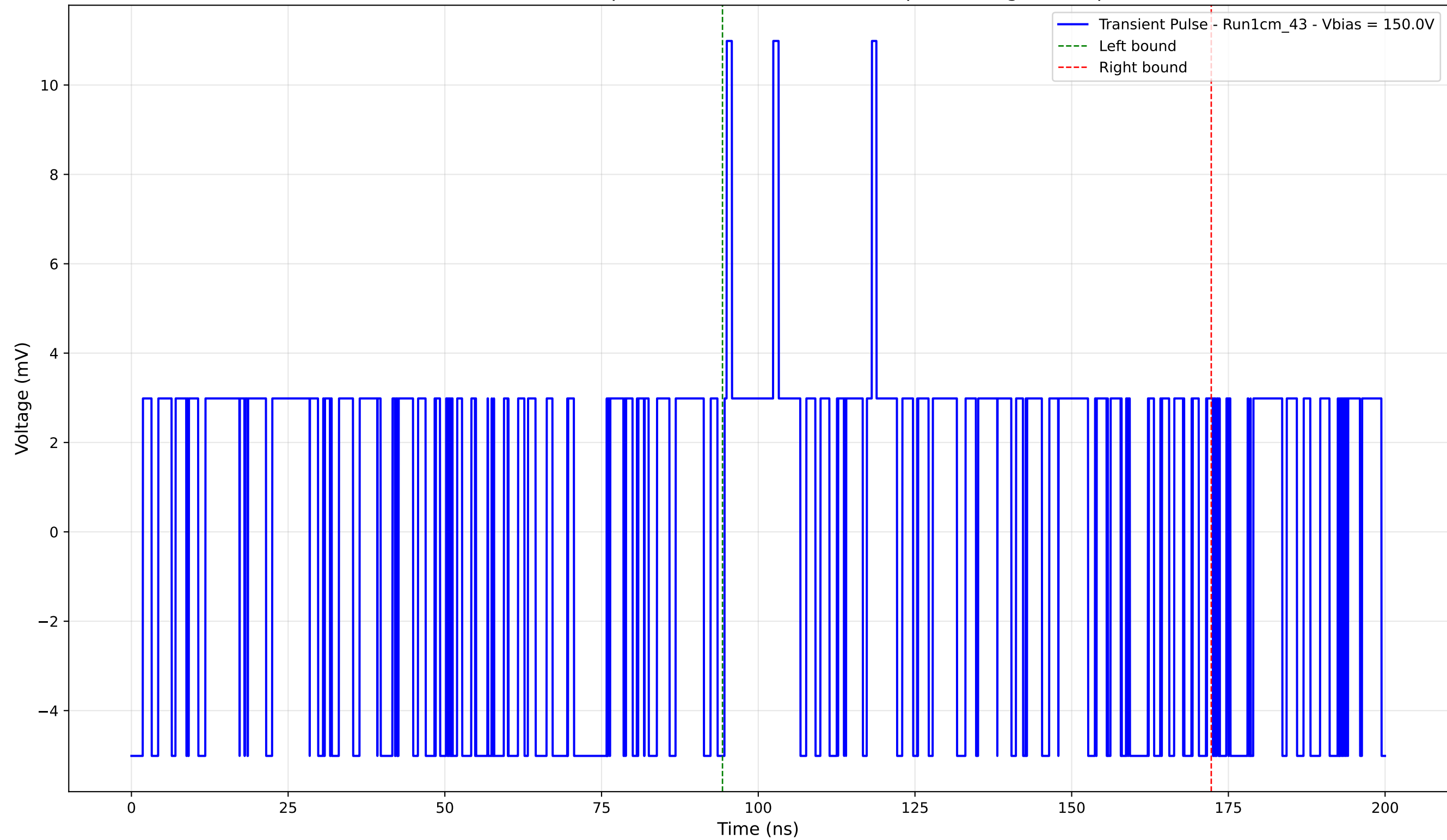
Transient Pulse - Sample: new1cm - Position: 15.0 \mu\text{m} - Charge: 1.76 pC
