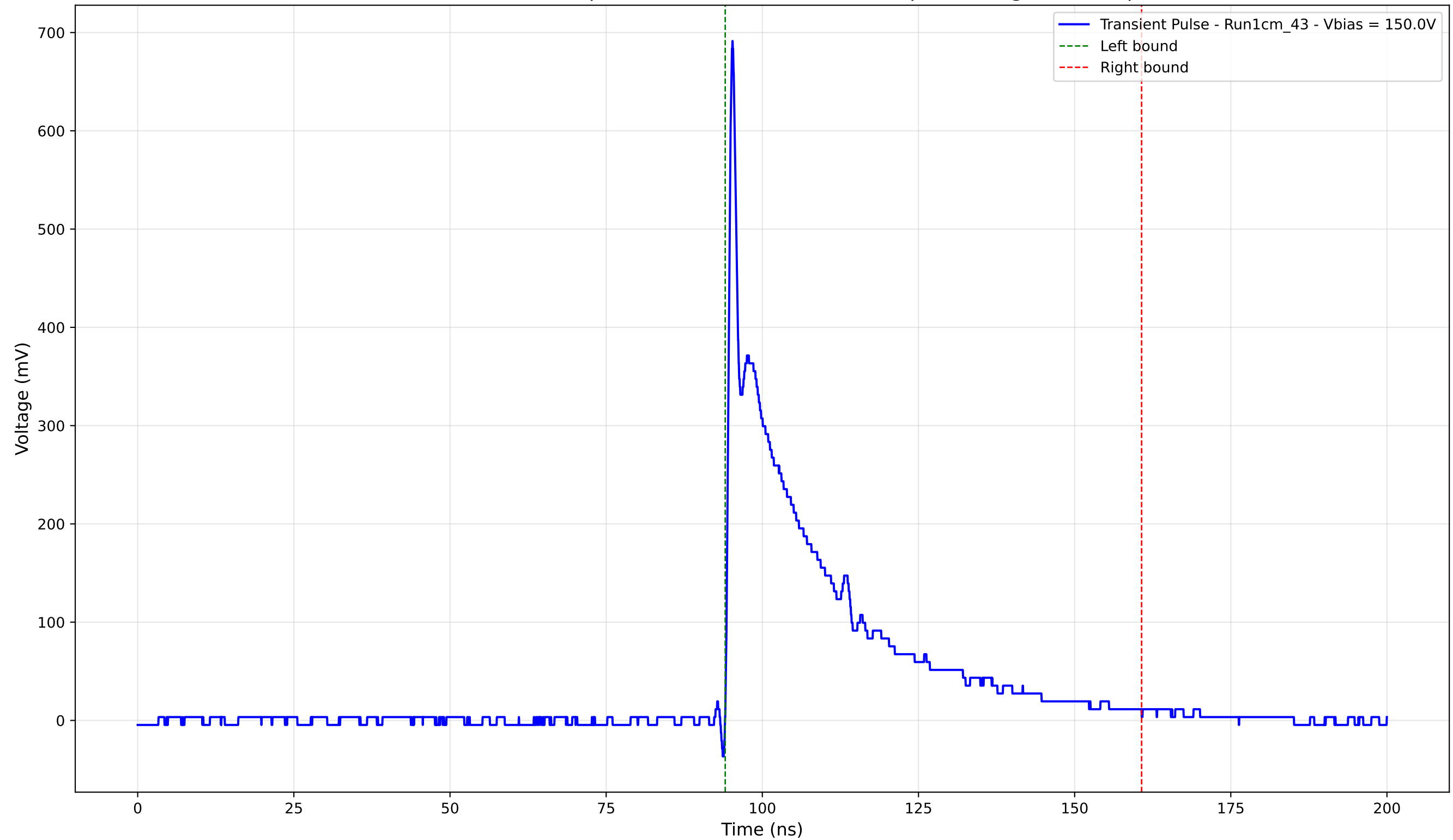
Transient Pulse - Sample: new1cm - Position: 2640.0 \mu\text{m} - Charge: 139.89 pC
