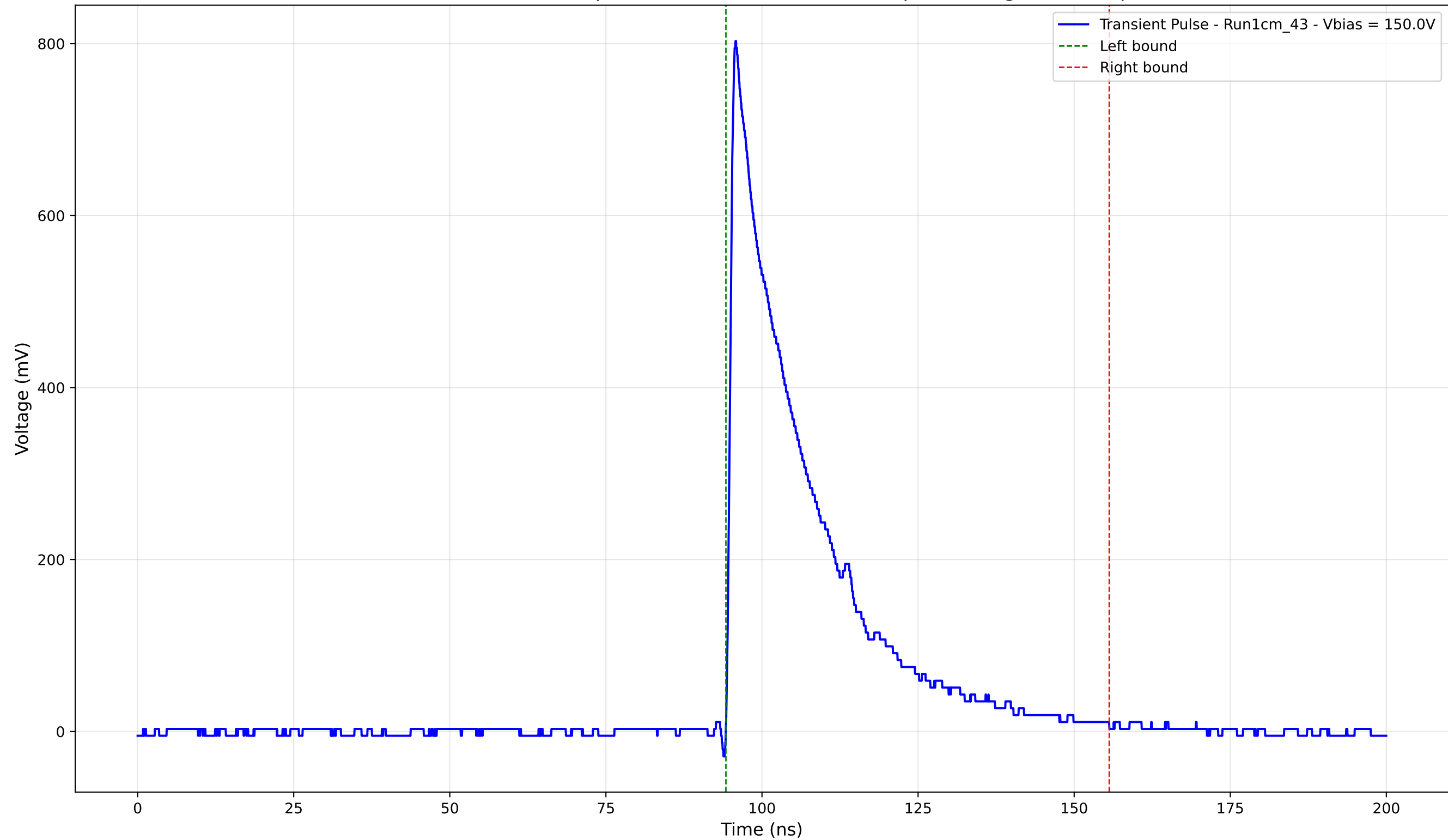
Transient Pulse - Sample: new1cm - Position: 430.0 \mu\text{m} - Charge: 201.32 pC
