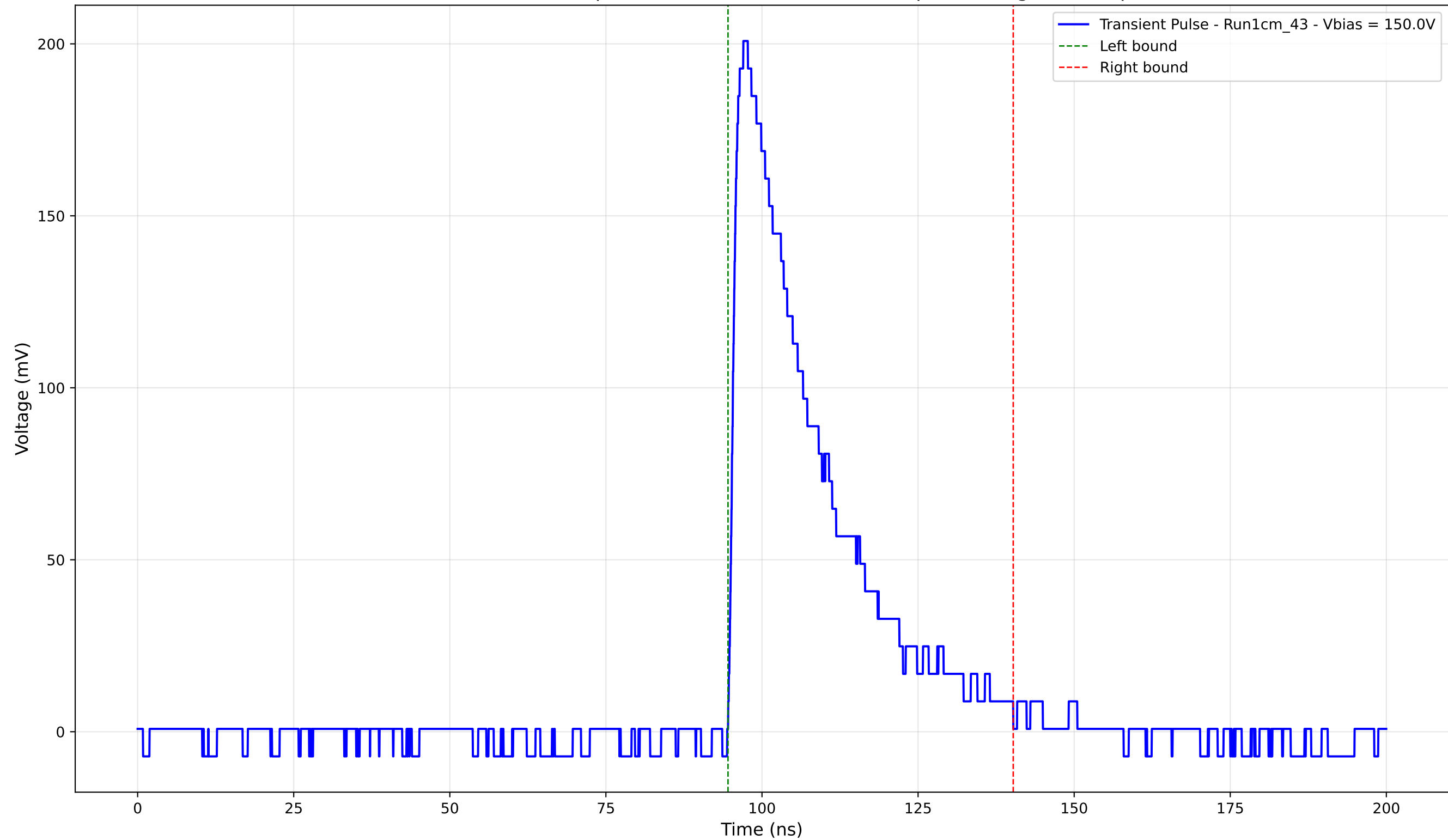
Transient Pulse - Sample: new1cm - Position: 1150.0 \mu\text{m} - Charge: 58.85 pC
