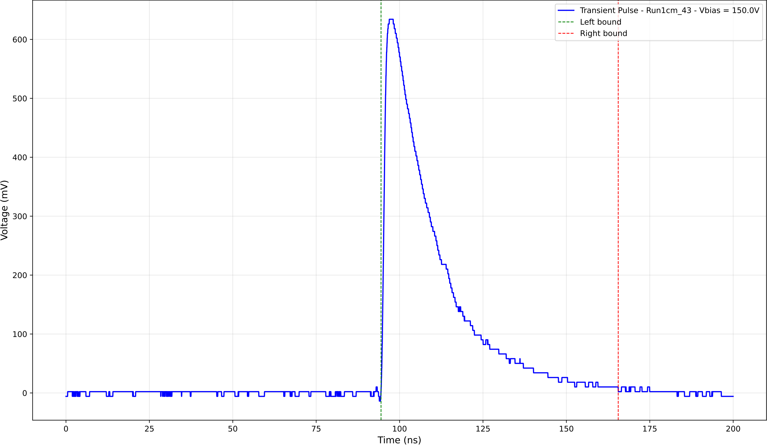
Transient Pulse - Sample: new1cm - Position: 1510.0 \mu\text{m} - Charge: 216.66 pC
