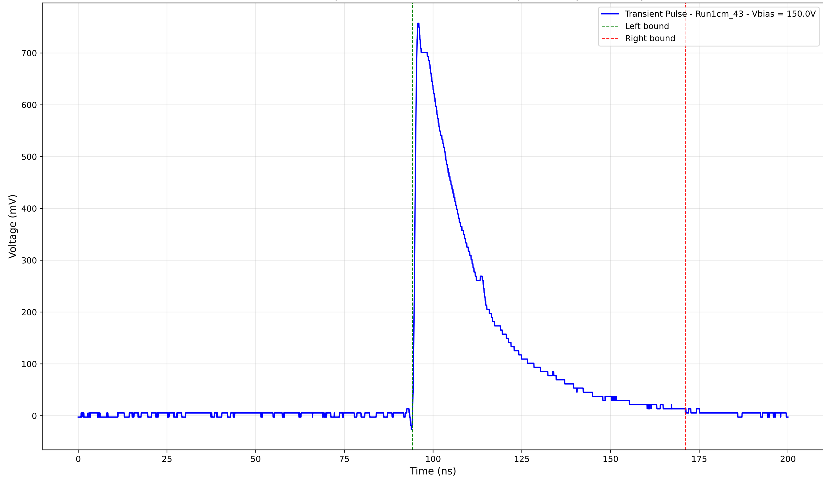
Transient Pulse - Sample: new1cm - Position: 3340.0 \mu\text{m} - Charge: 264.14 pC
