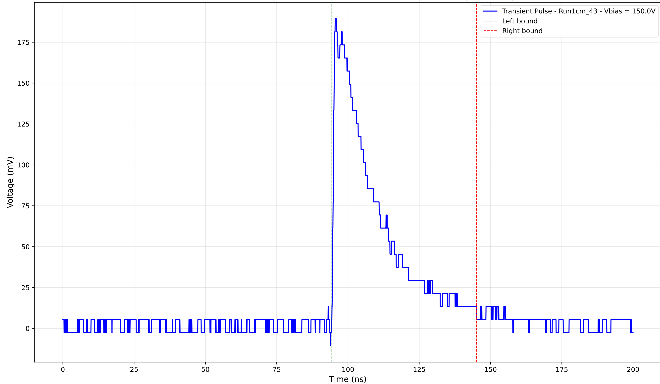
Transient Pulse - Sample: new1cm - Position: 2155.0 \mu\text{m} - Charge: 61.58 pC
