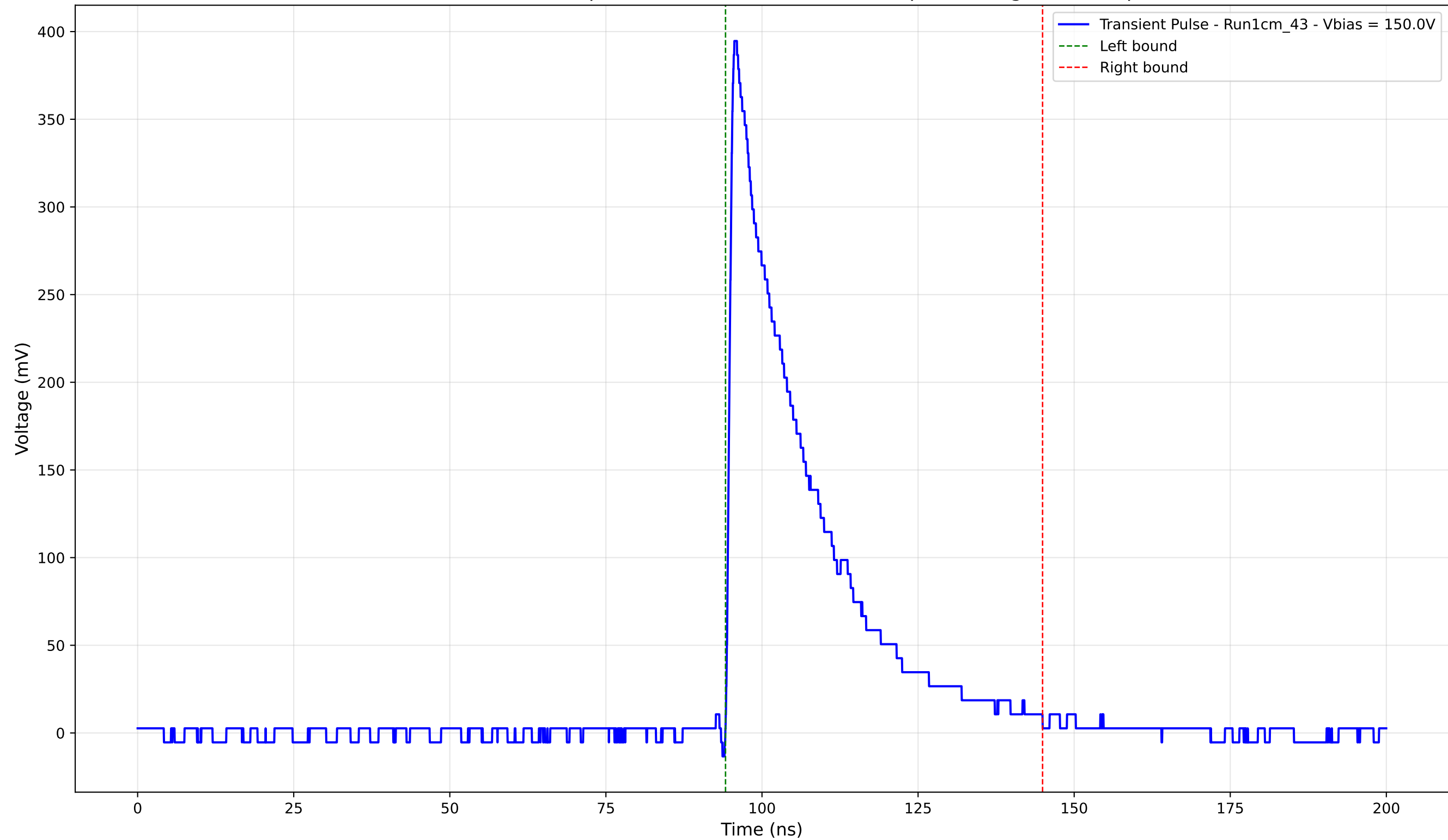
Transient Pulse - Sample: new1cm - Position: 4765.0 \mu\text{m} - Charge: 100.61 pC
