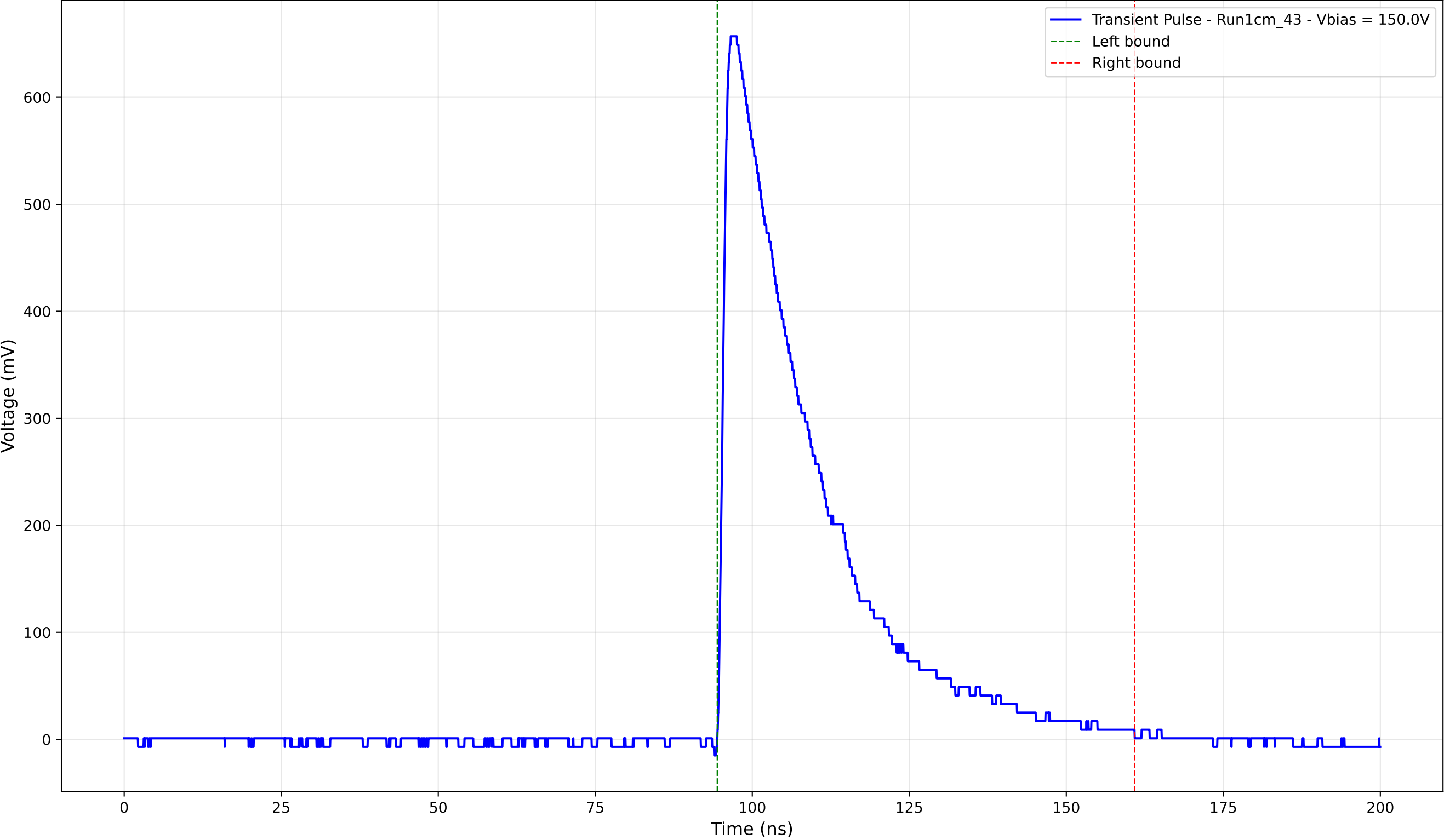
Transient Pulse - Sample: new1cm - Position: 1045.0 \mu\text{m} - Charge: 205.31 pC
