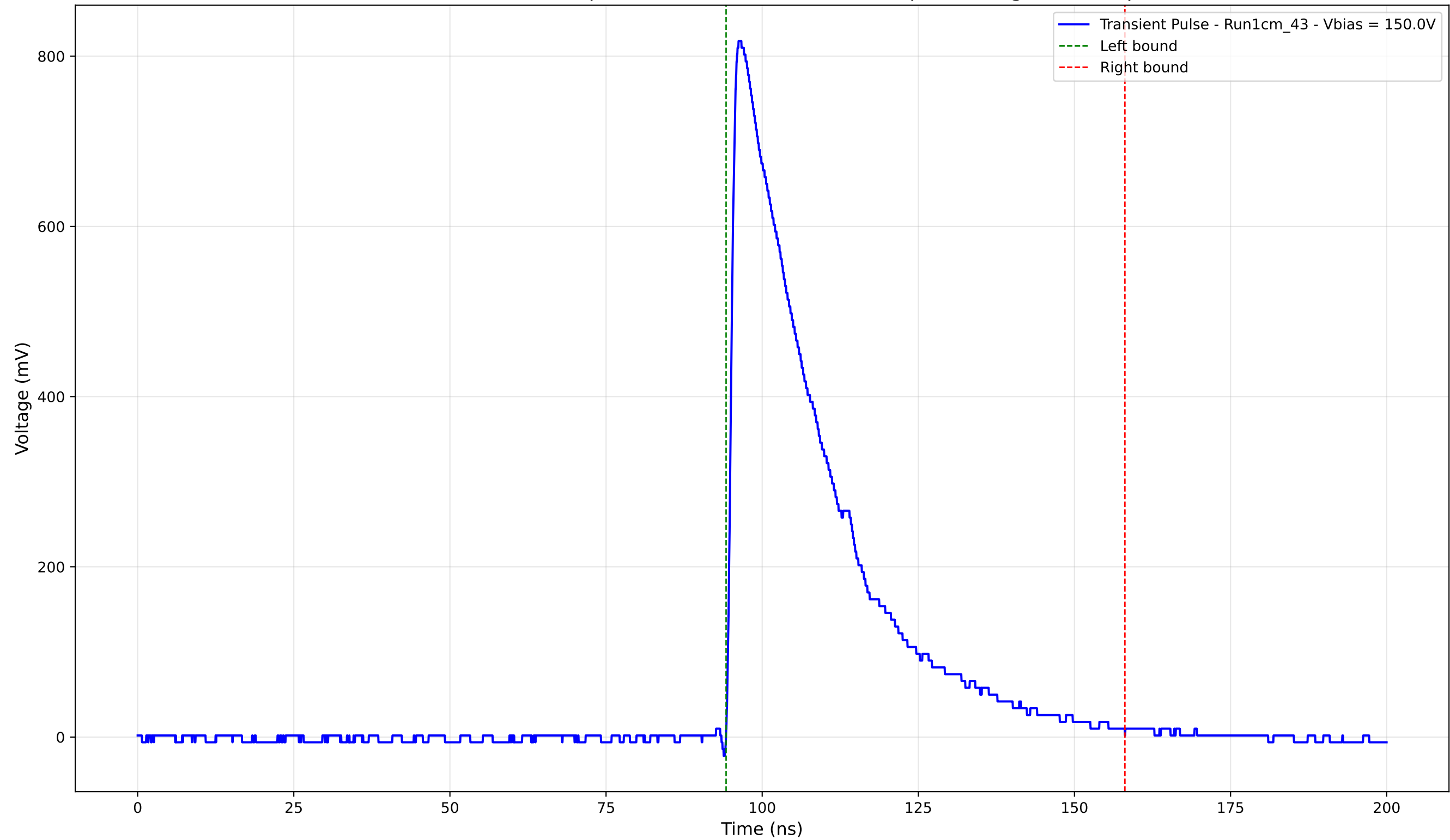
Transient Pulse - Sample: new1cm - Position: 4440.0 \mu\text{m} - Charge: 259.60 pC
