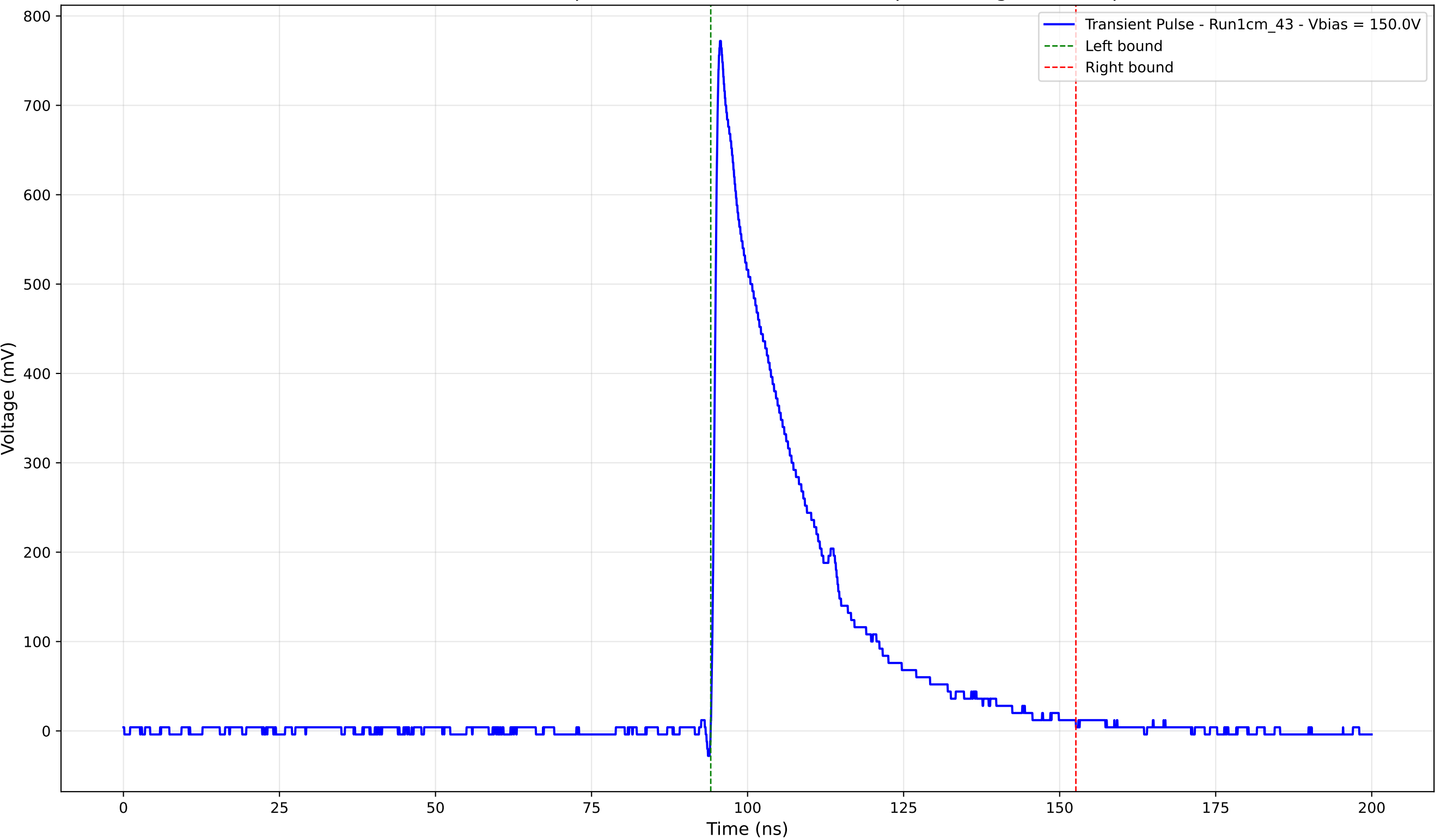
Transient Pulse - Sample: new1cm - Position: 4850.0 \mu\text{m} - Charge: 201.56 pC
