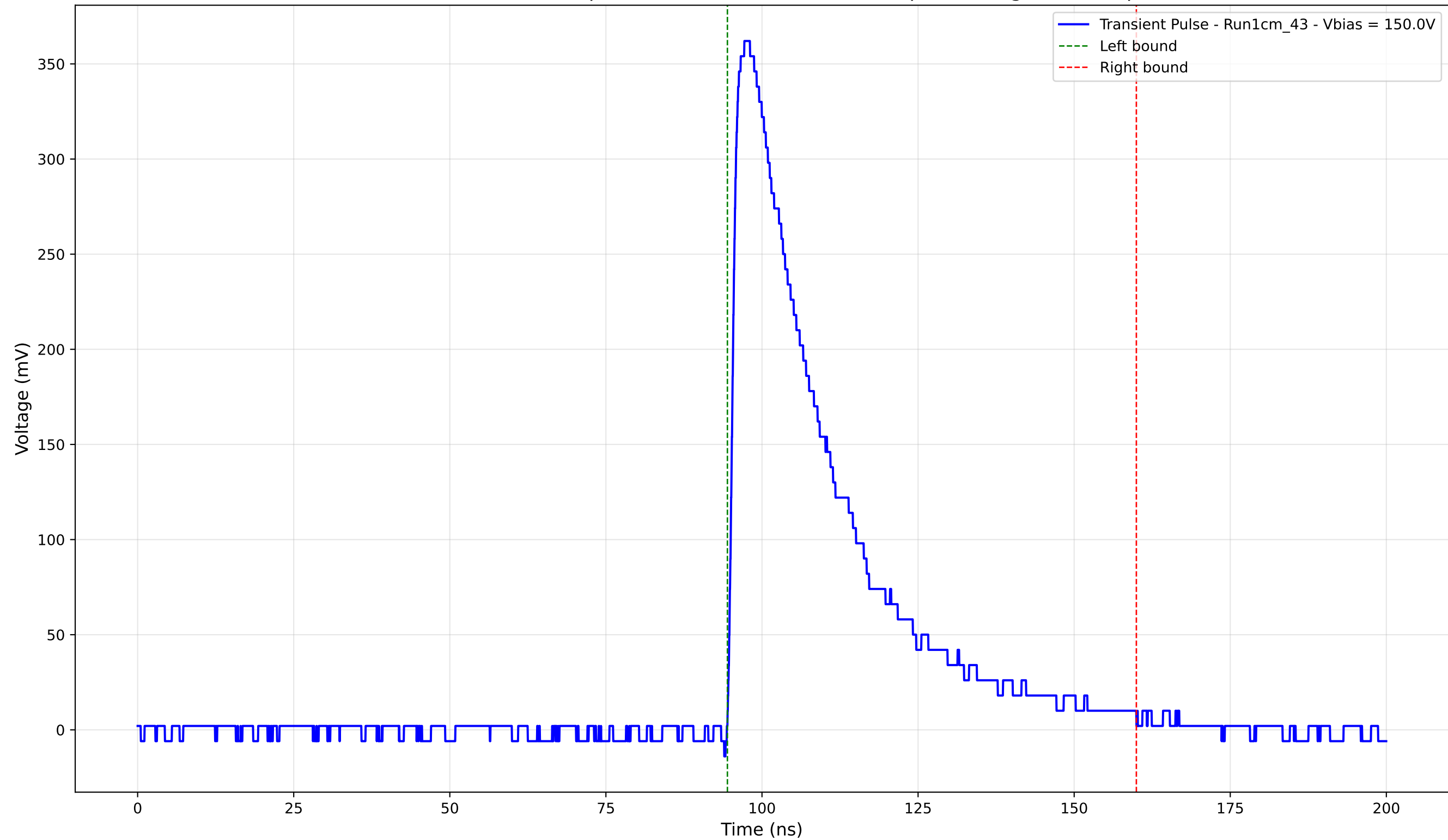
Transient Pulse - Sample: new1cm - Position: 1630.0 \mu\text{m} - Charge: 120.97 pC
