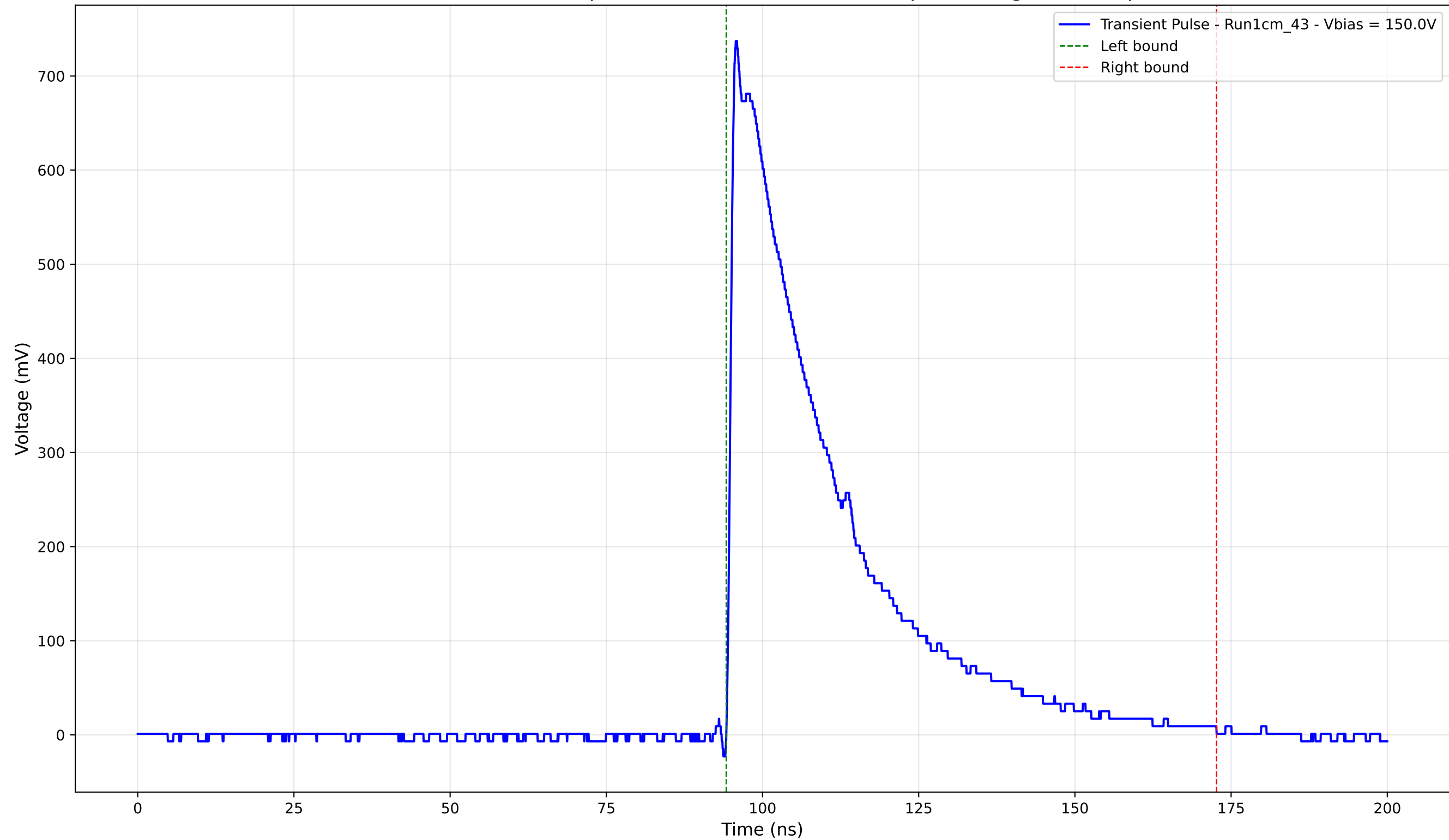
Transient Pulse - Sample: new1cm - Position: 3320.0 \mu\text{m} - Charge: 250.28 pC
