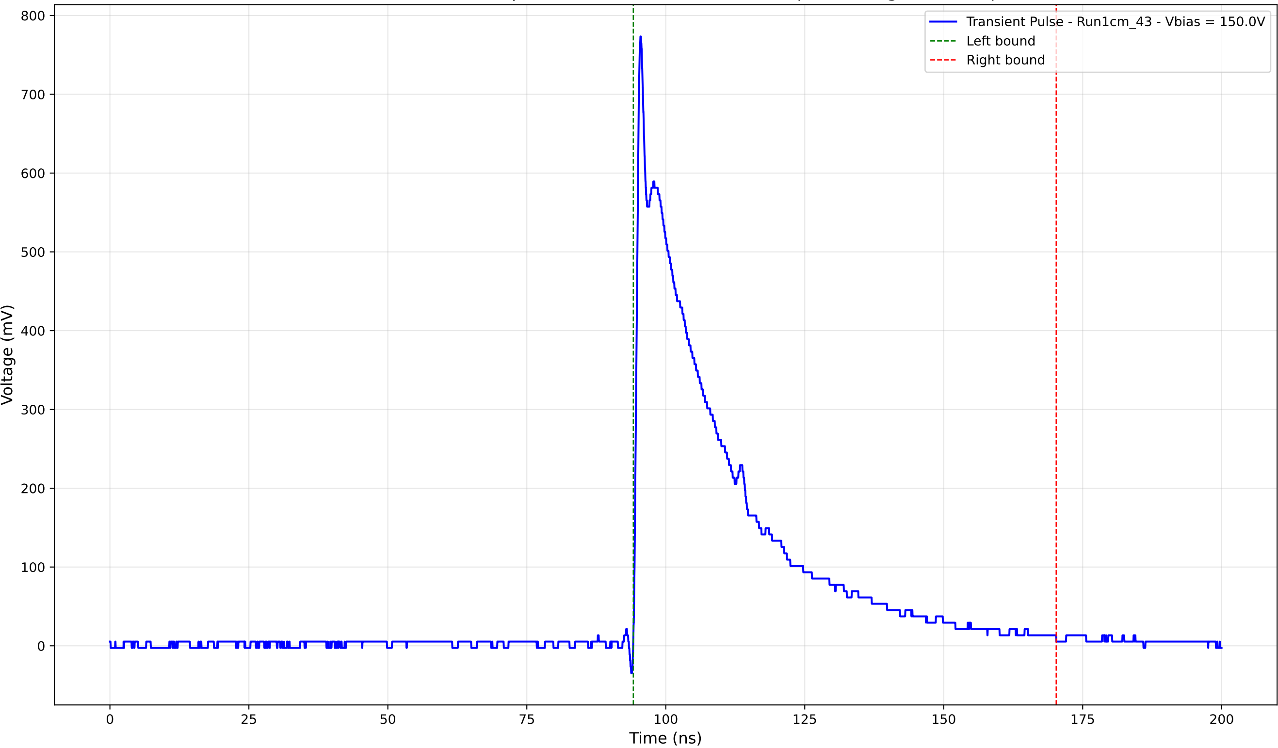
Transient Pulse - Sample: new1cm - Position: 2330.0 \mu\text{m} - Charge: 223.53 pC
