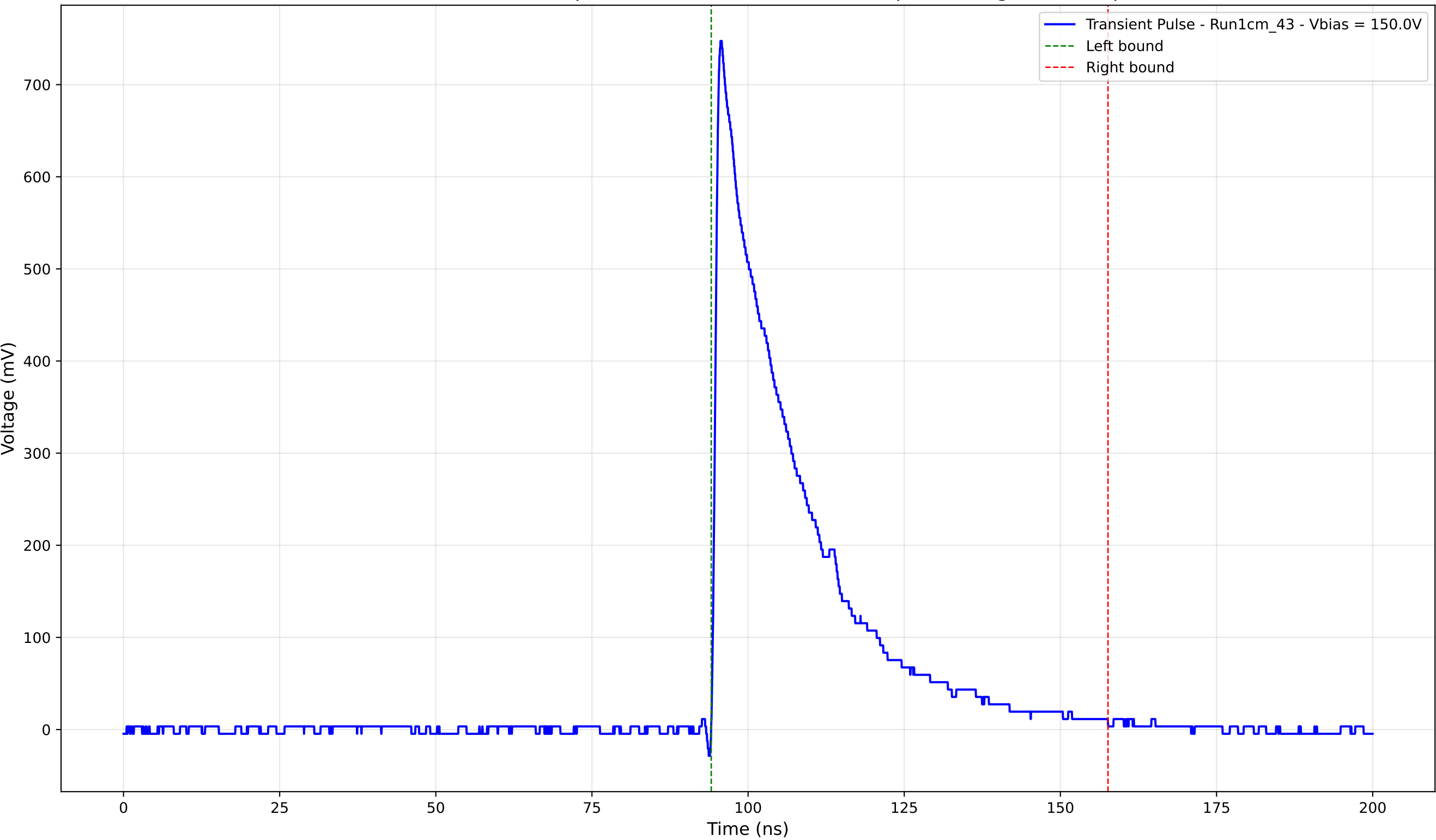
Transient Pulse - Sample: new1cm - Position: 4830.0 \mu\text{m} - Charge: 199.13 pC
