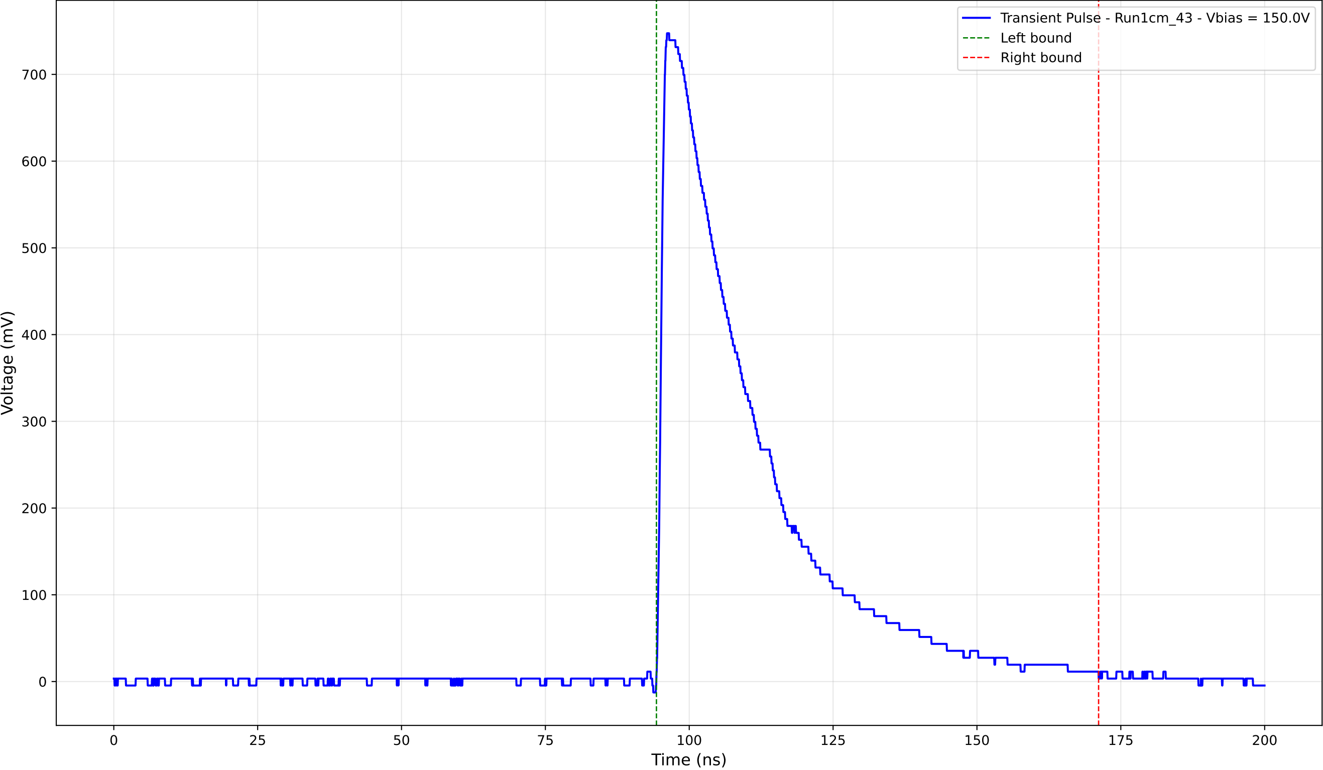
Transient Pulse - Sample: new1cm - Position: 3570.0 \mu\text{m} - Charge: 266.61 pC
