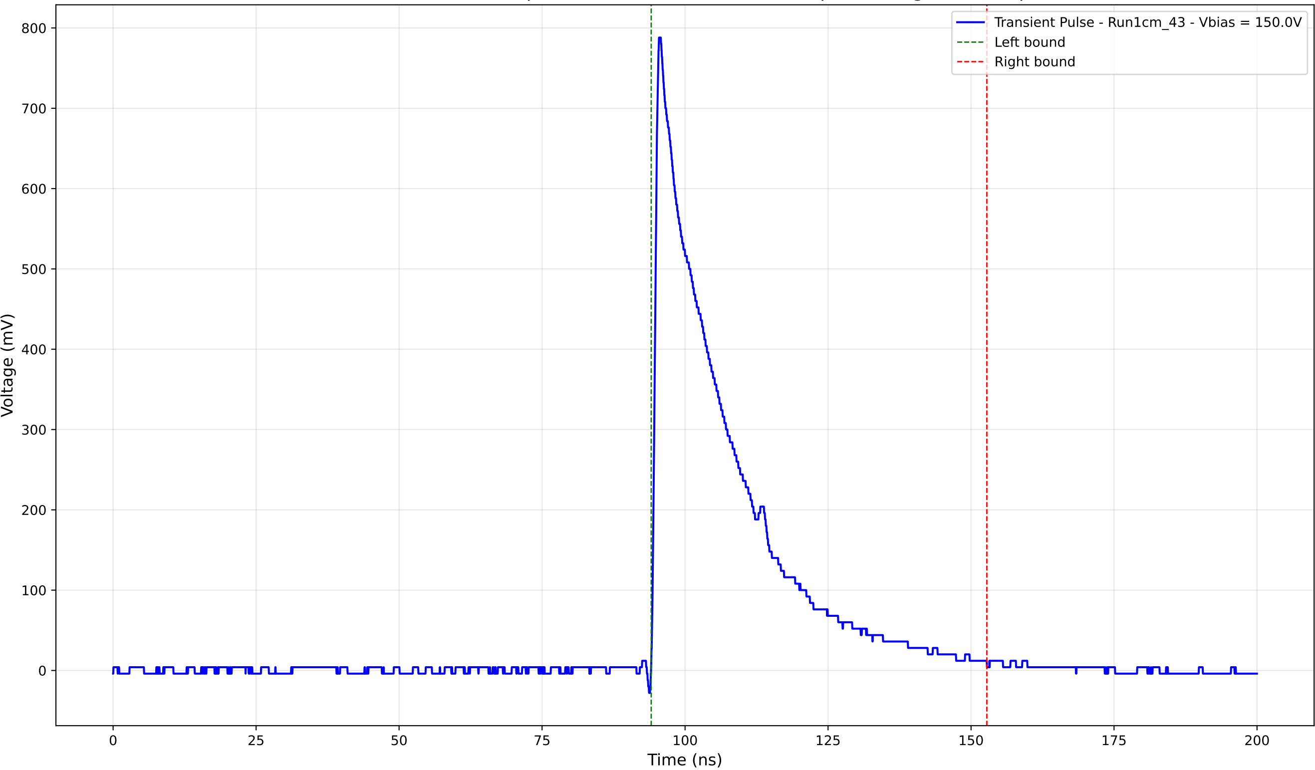
Transient Pulse - Sample: new1cm - Position: 4885.0 \mu\text{m} - Charge: 203.83 pC
