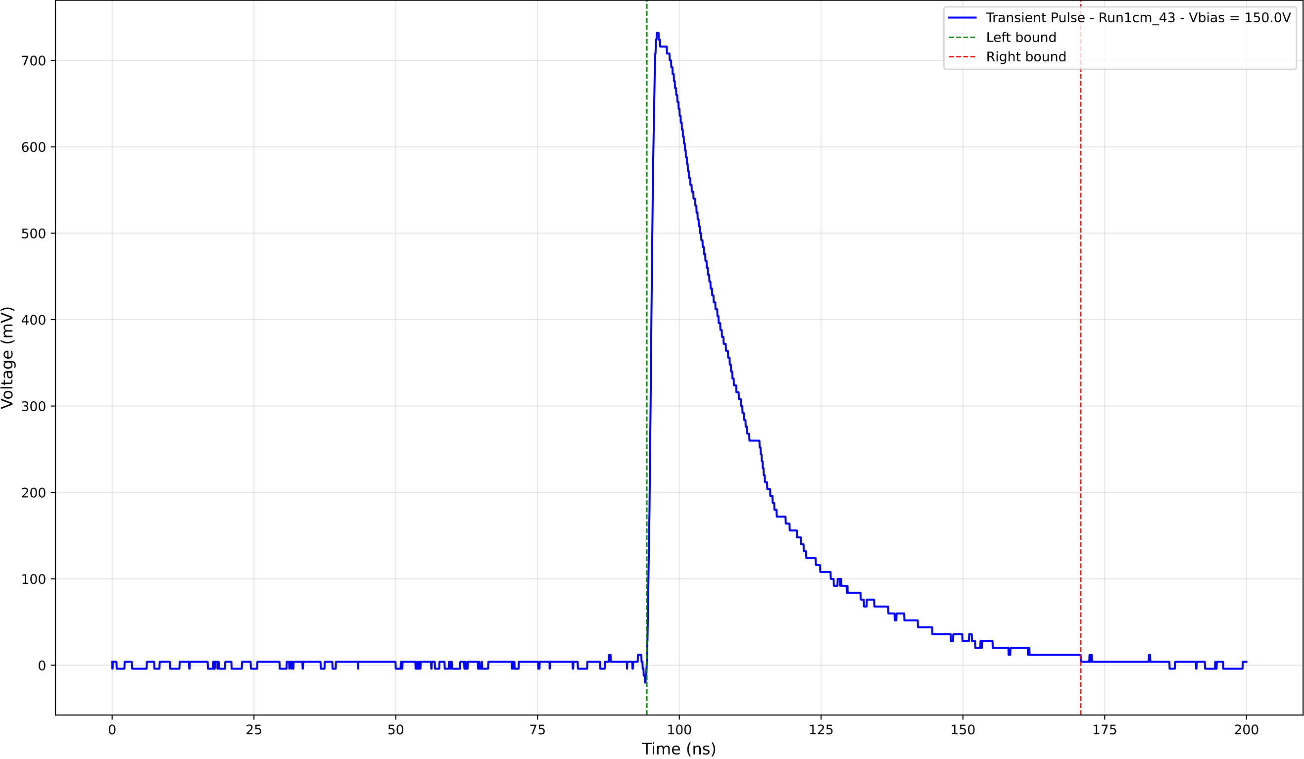
Transient Pulse - Sample: new1cm - Position: 3495.0 \mu\text{m} - Charge: 260.89 pC
