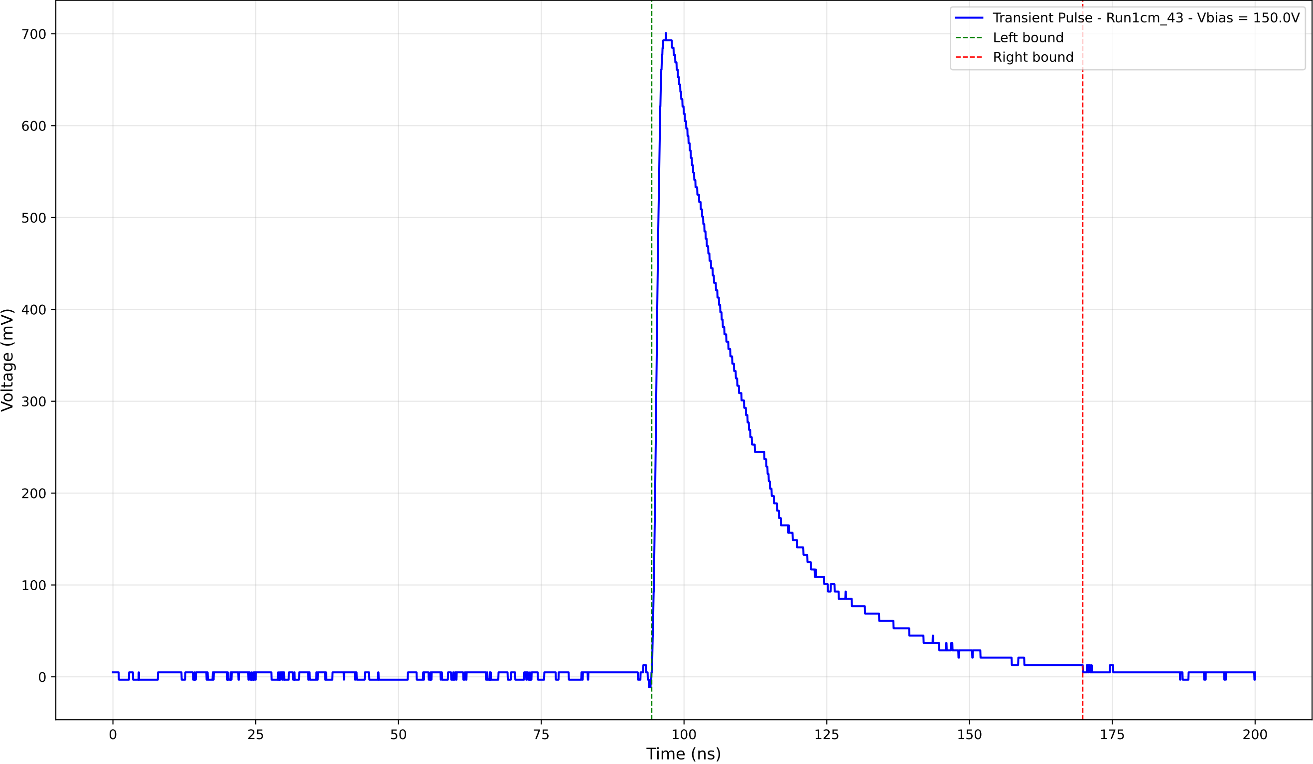
Transient Pulse - Sample: new1cm - Position: 3800.0 \mu\text{m} - Charge: 243.54 pC
