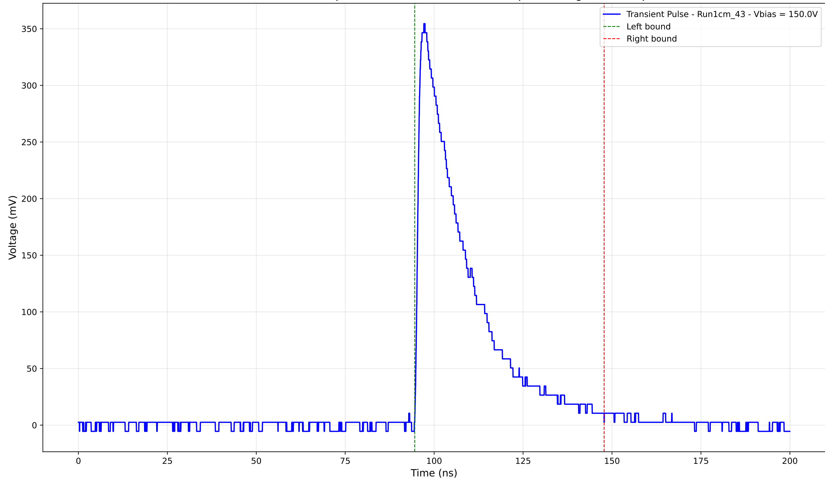
Transient Pulse - Sample: new1cm - Position: 1130.0 \mu\text{m} - Charge: 105.55 pC
