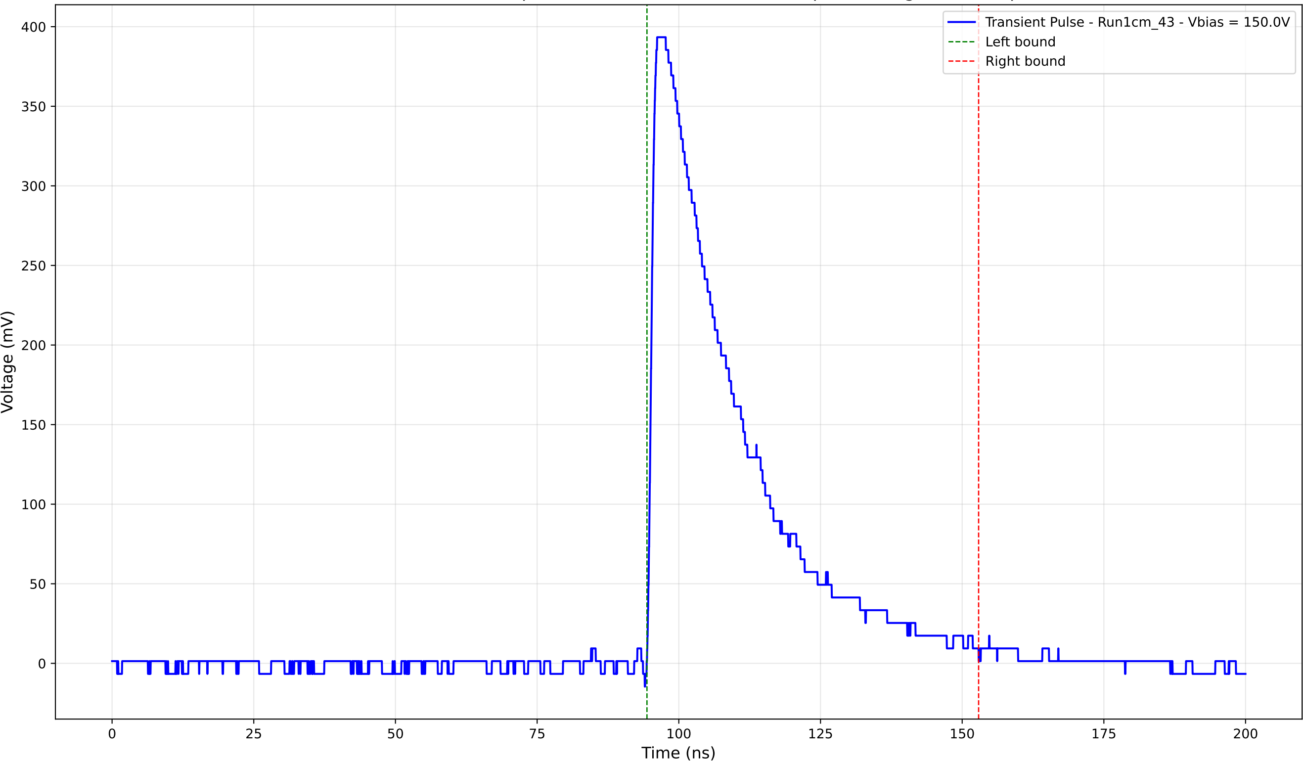
Transient Pulse - Sample: new1cm - Position: 3660.0 \mu\text{m} - Charge: 129.83 pC
