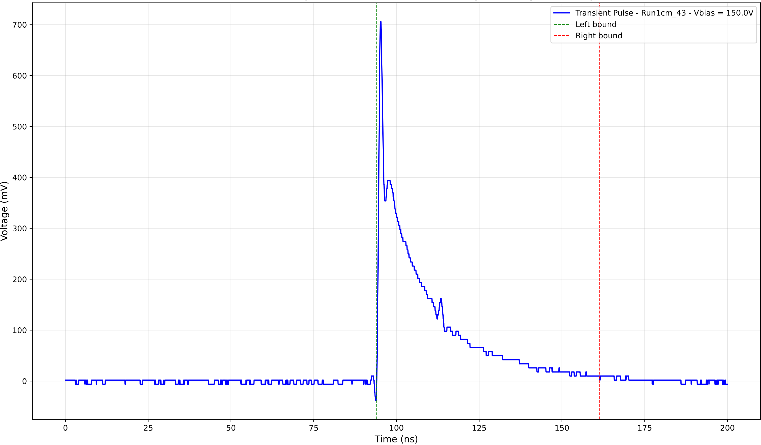
Transient Pulse - Sample: new1cm - Position: 2760.0 \mu\text{m} - Charge: 146.45 pC
