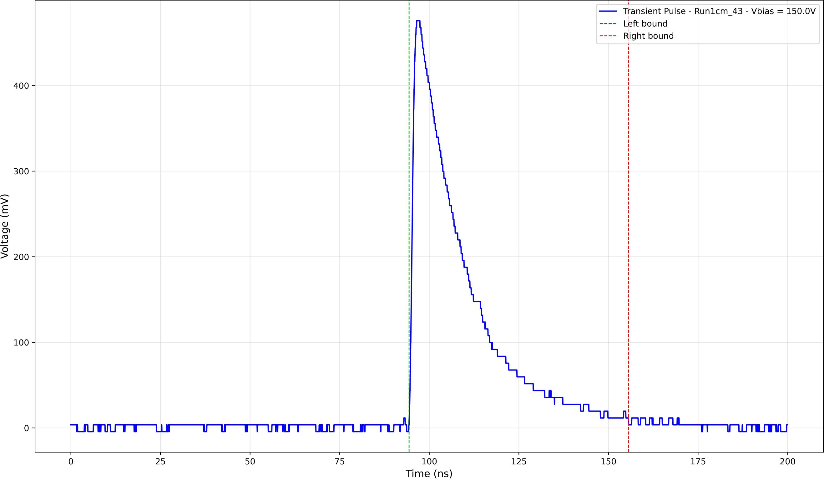
Transient Pulse - Sample: new1cm - Position: 4160.0 \mu\text{m} - Charge: 150.53 pC
