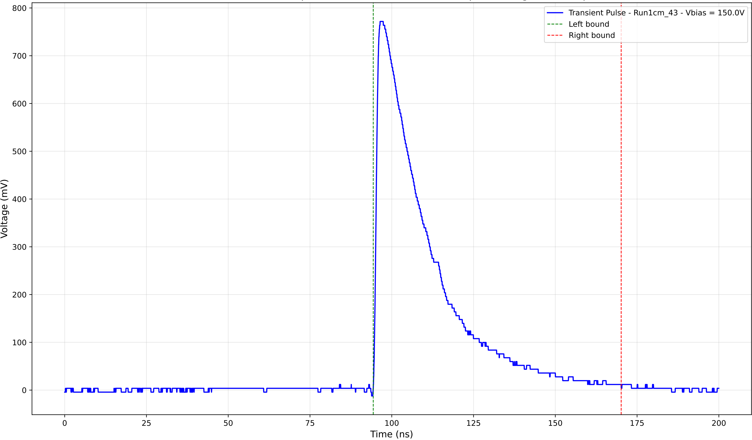
Transient Pulse - Sample: new1cm - Position: 3865.0 \mu\text{m} - Charge: 270.31 pC
