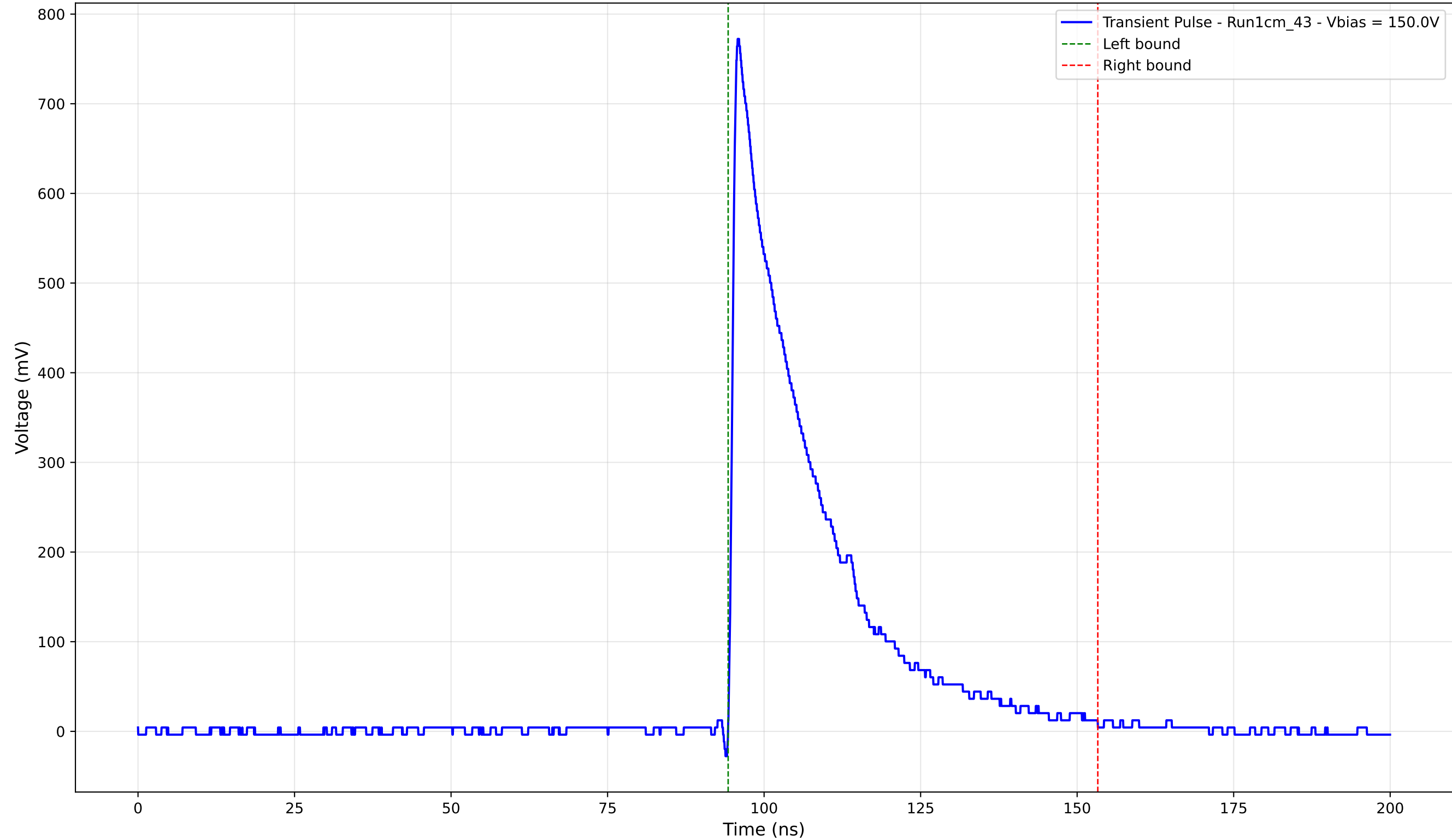
Transient Pulse - Sample: new1cm - Position: 485.0 \mu\text{m} - Charge: 200.79 pC
