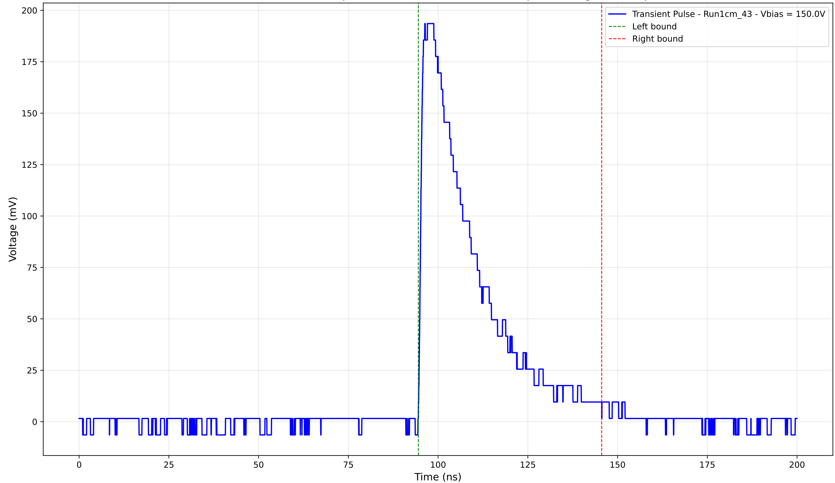
Transient Pulse - Sample: new1cm - Position: 3685.0 \mu\text{m} - Charge: 63.37 pC
