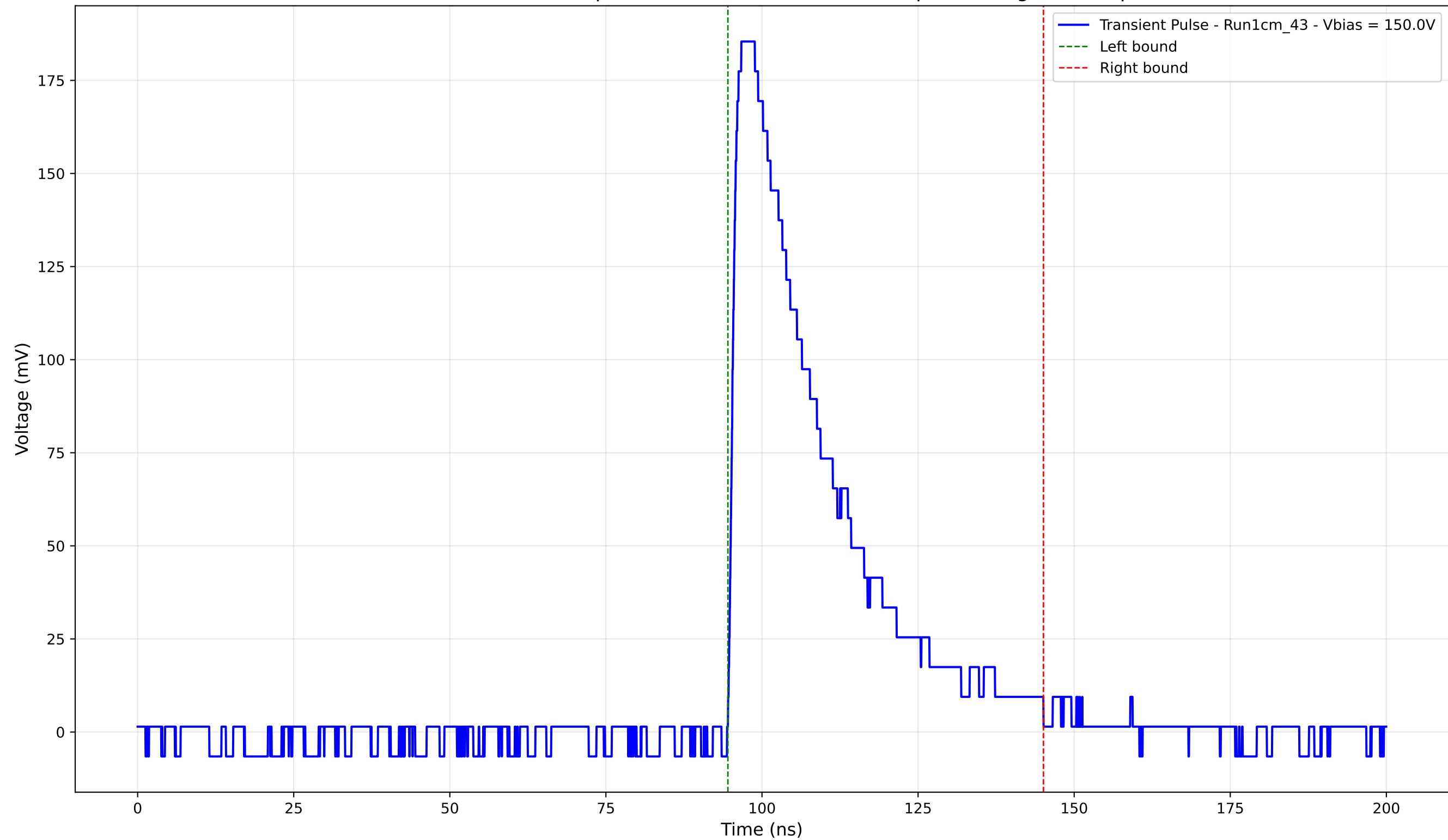
Transient Pulse - Sample: new1cm - Position: 1655.0 \mu\text{m} - Charge: 59.43 pC
