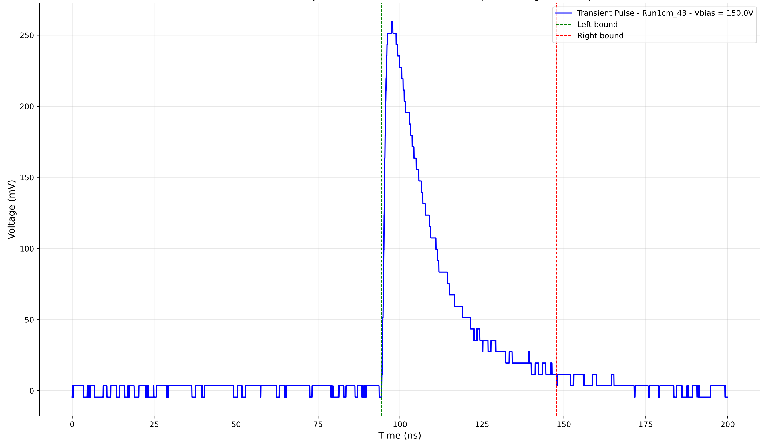
Transient Pulse - Sample: new1cm - Position: 3740.0 \mu\text{m} - Charge: 85.50 pC
