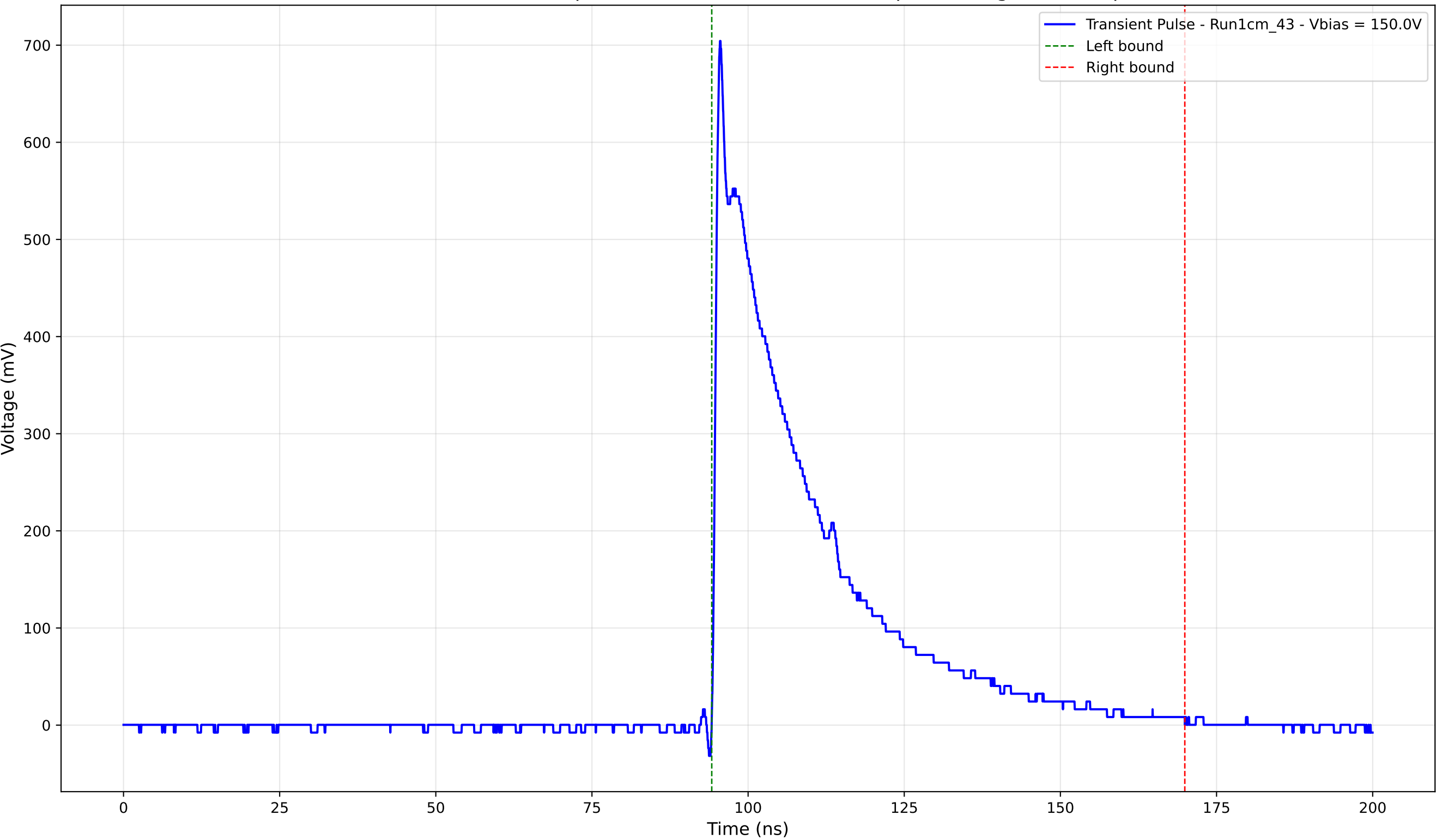
Transient Pulse - Sample: new1cm - Position: 3130.0 \mu\text{m} - Charge: 201.54 pC
