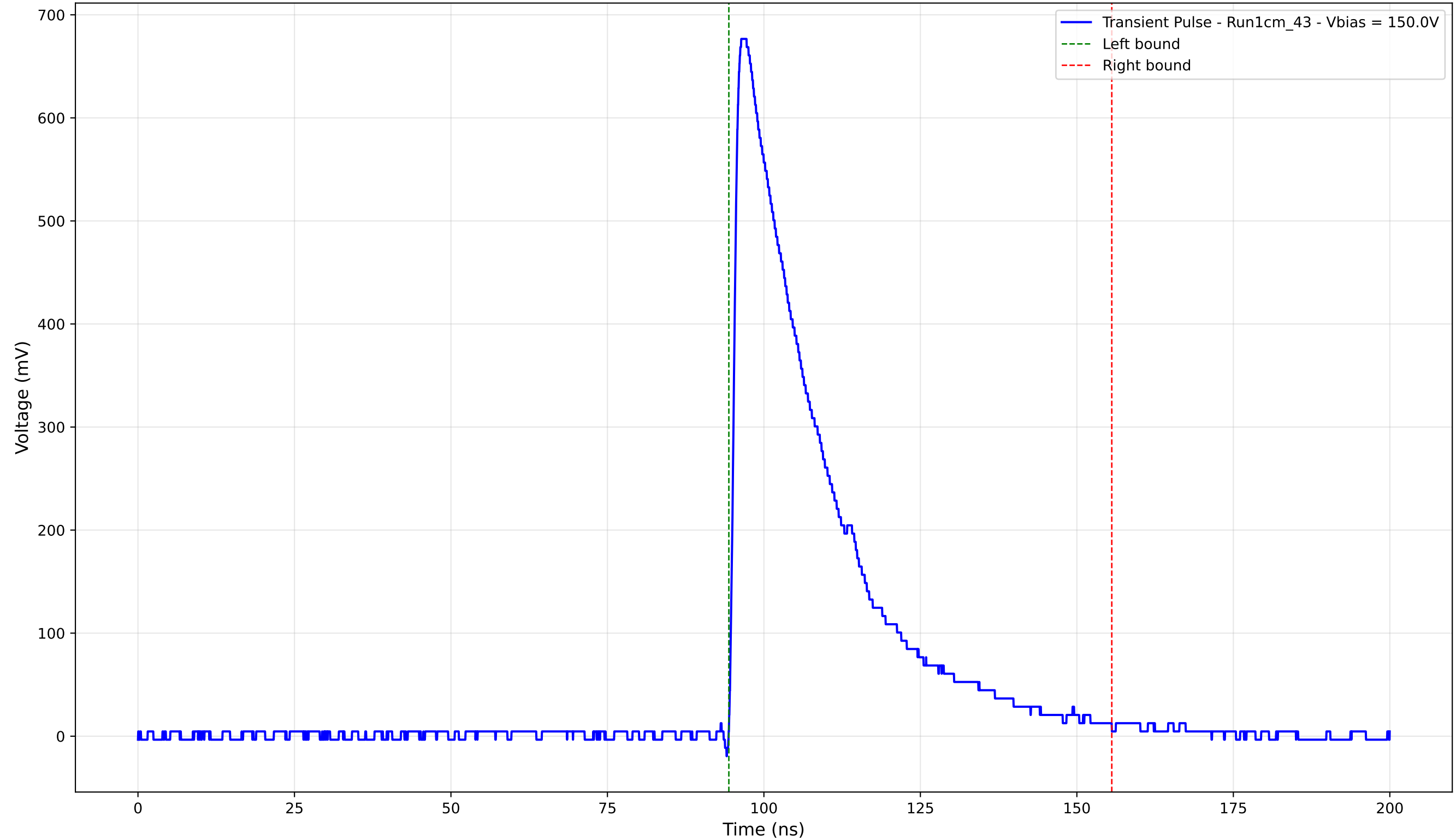
Transient Pulse - Sample: new1cm - Position: 875.0 \mu\text{m} - Charge: 206.77 pC
