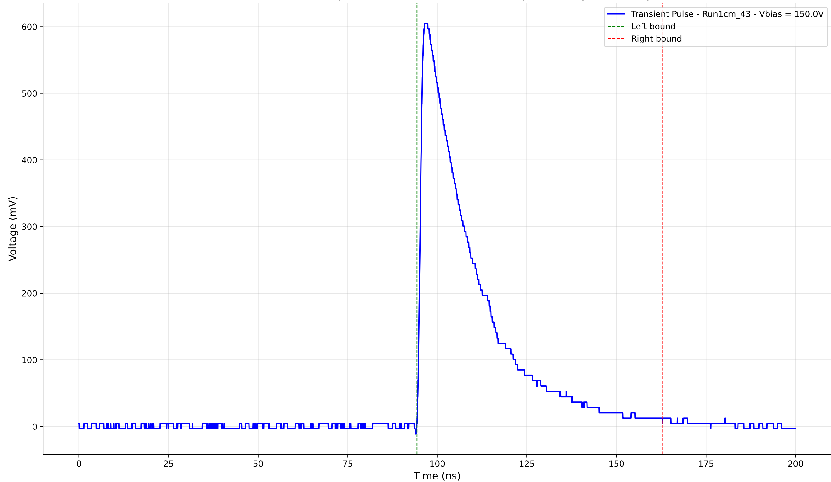
Transient Pulse - Sample: new1cm - Position: 4145.0 \mu\text{m} - Charge: 196.76 pC
