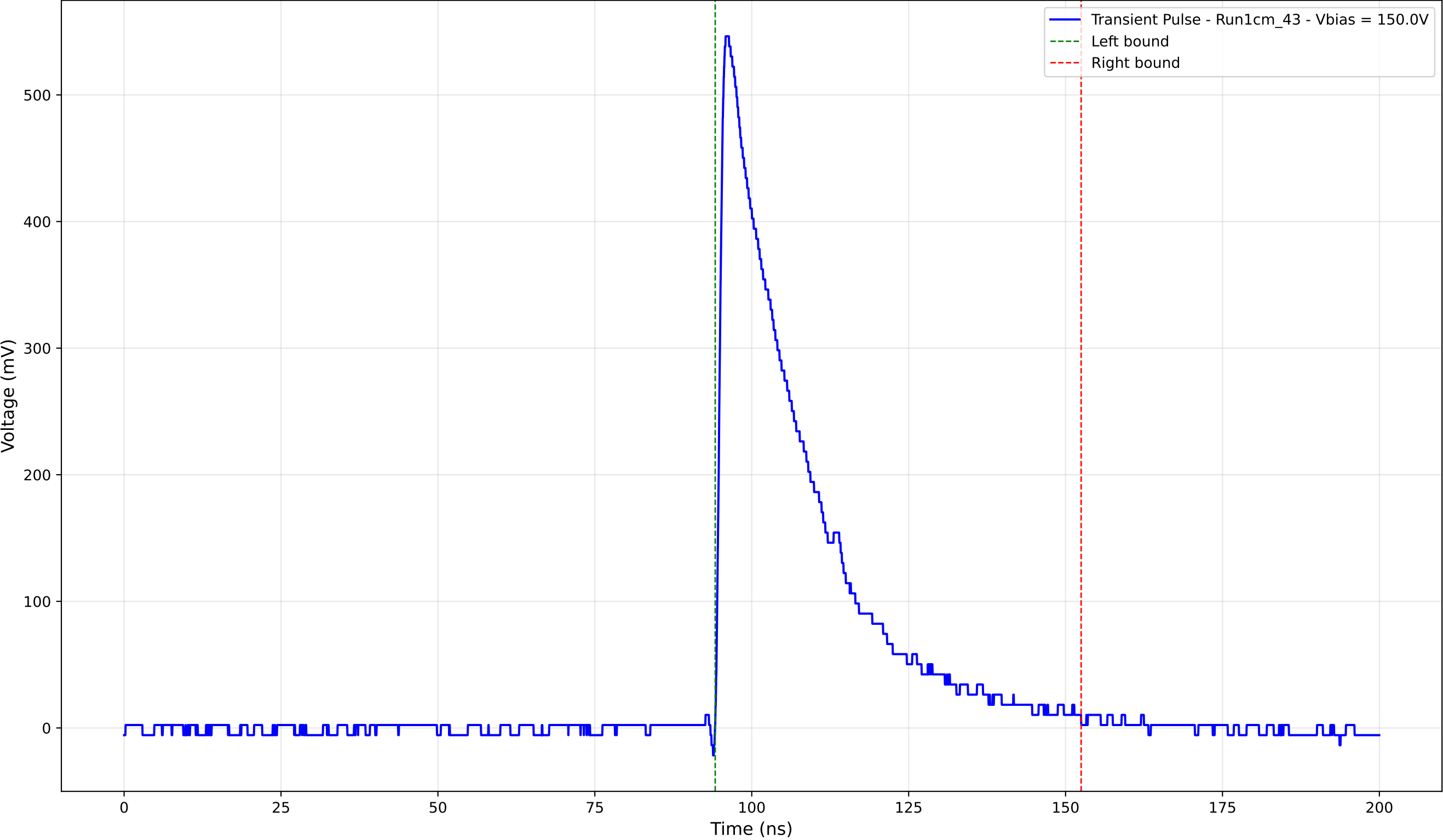
Transient Pulse - Sample: new1cm - Position: 4655.0 \mu\text{m} - Charge: 154.48 pC
