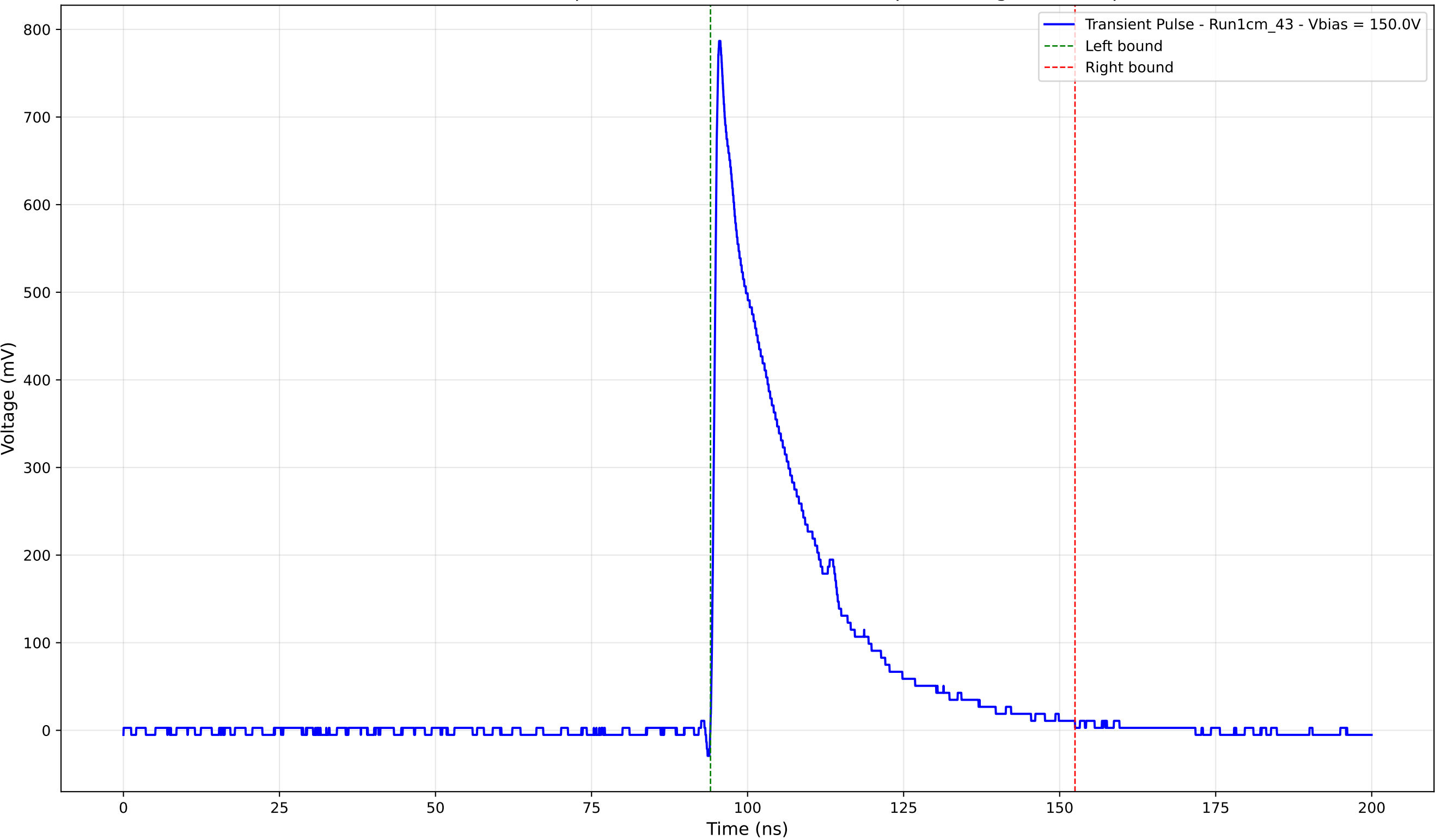
Transient Pulse - Sample: new1cm - Position: 4930.0 \mu\text{m} - Charge: 192.15 pC
