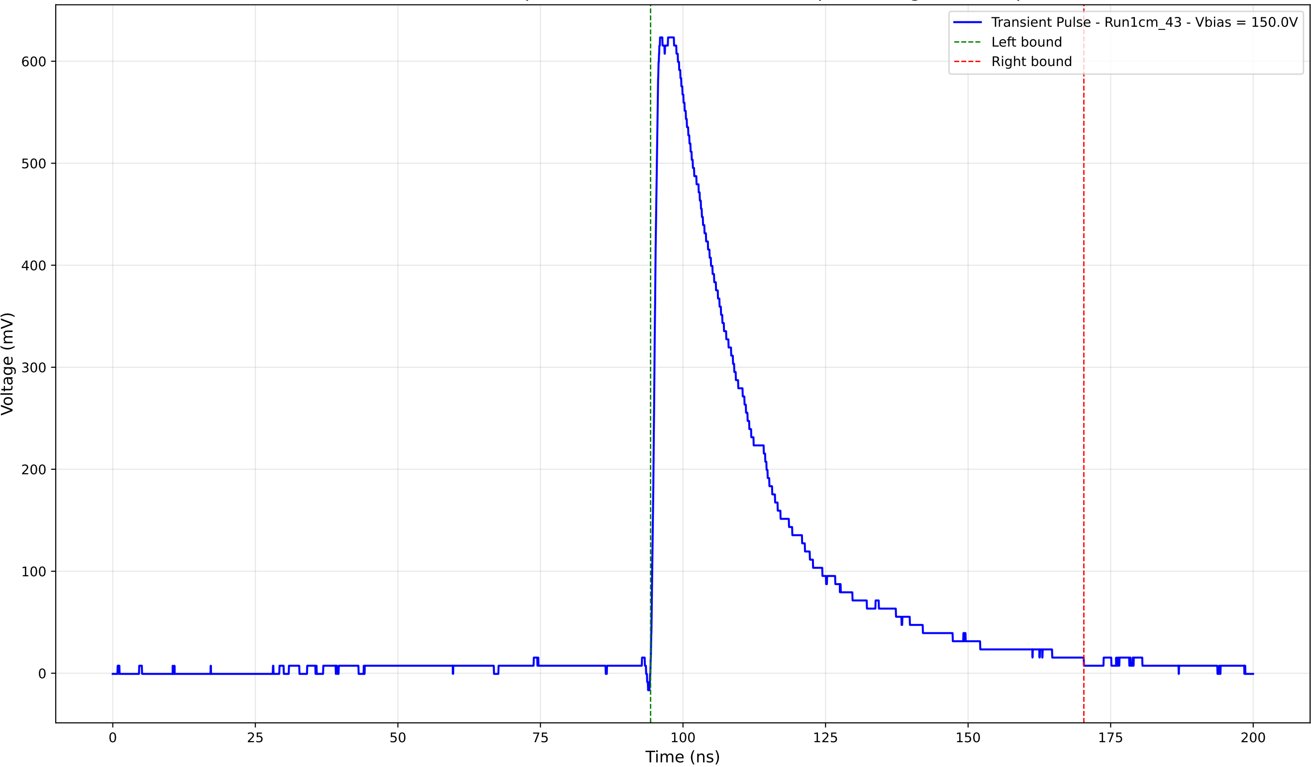
Transient Pulse - Sample: new1cm - Position: 1915.0 \mu\text{m} - Charge: 230.87 pC
