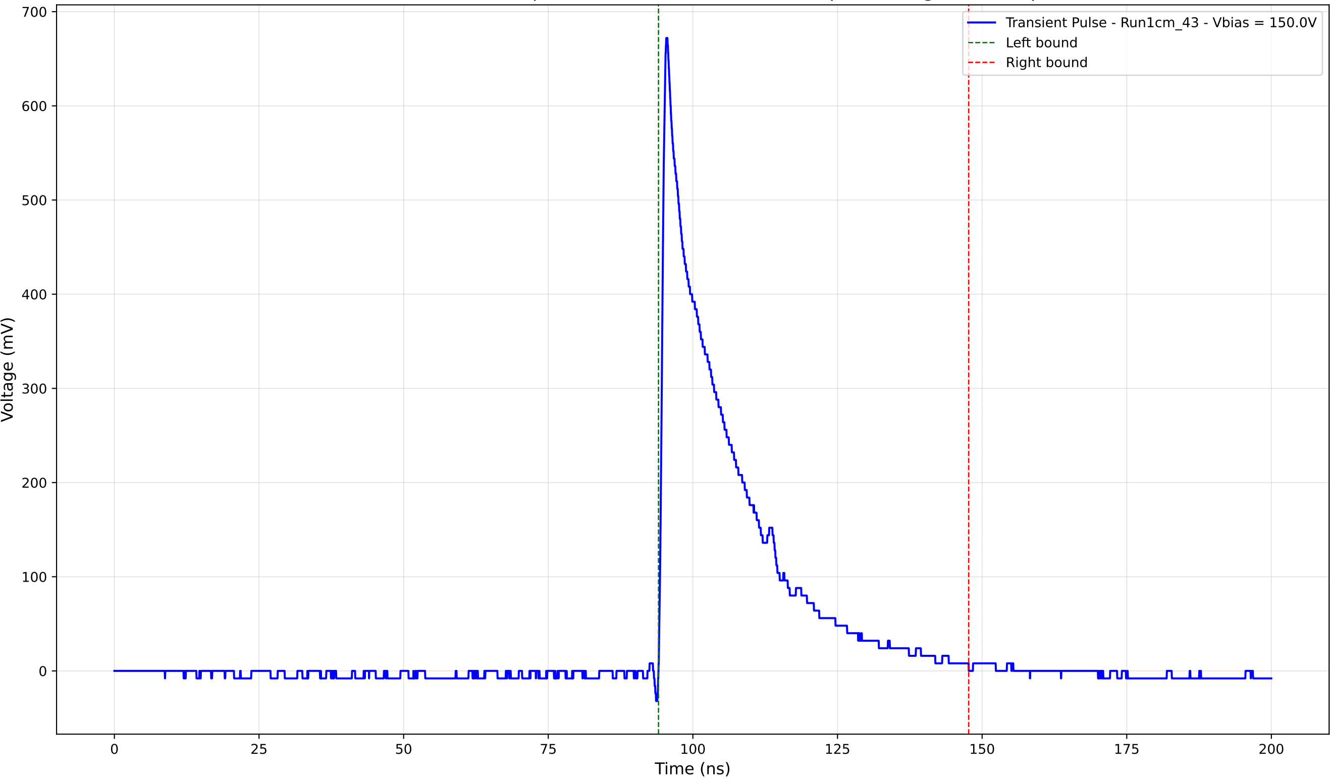
Transient Pulse - Sample: new1cm - Position: 4975.0 \mu\text{m} - Charge: 150.89 pC
