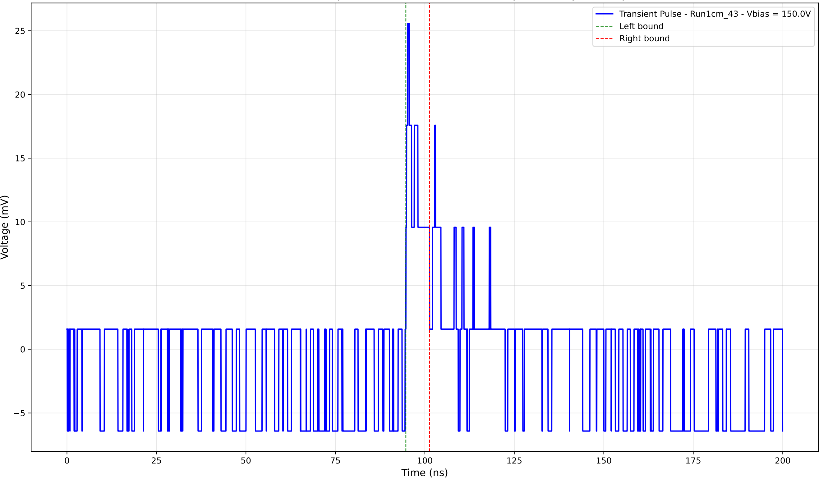
Transient Pulse - Sample: new1cm - Position: 125.0 \mu\text{m} - Charge: 1.71 pC
