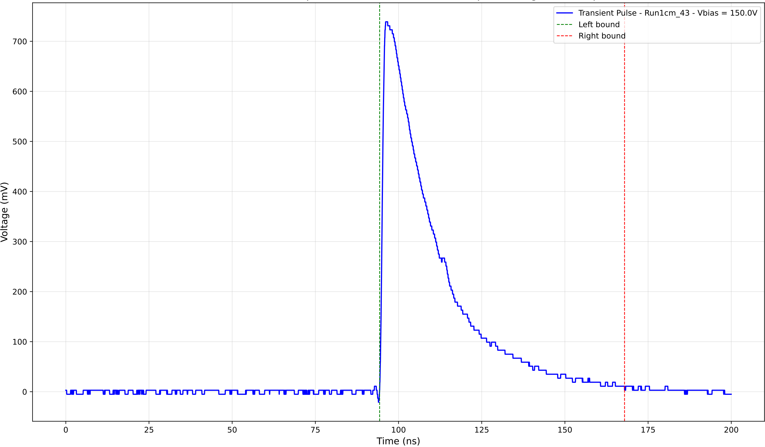
Transient Pulse - Sample: new1cm - Position: 3595.0 \mu\text{m} - Charge: 262.04 pC
