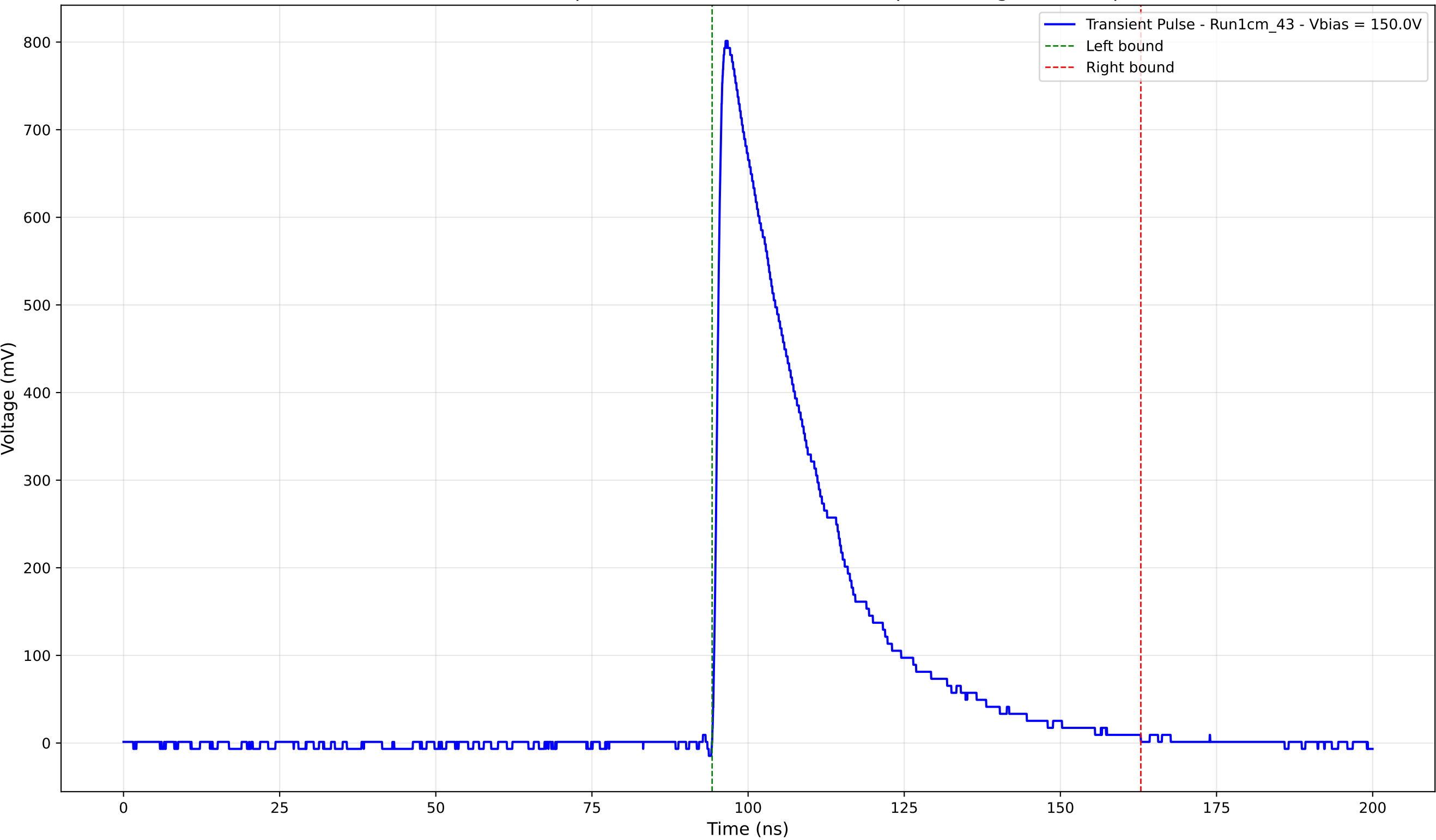
Transient Pulse - Sample: new1cm - Position: 4365.0 \mu\text{m} - Charge: 256.90 pC
