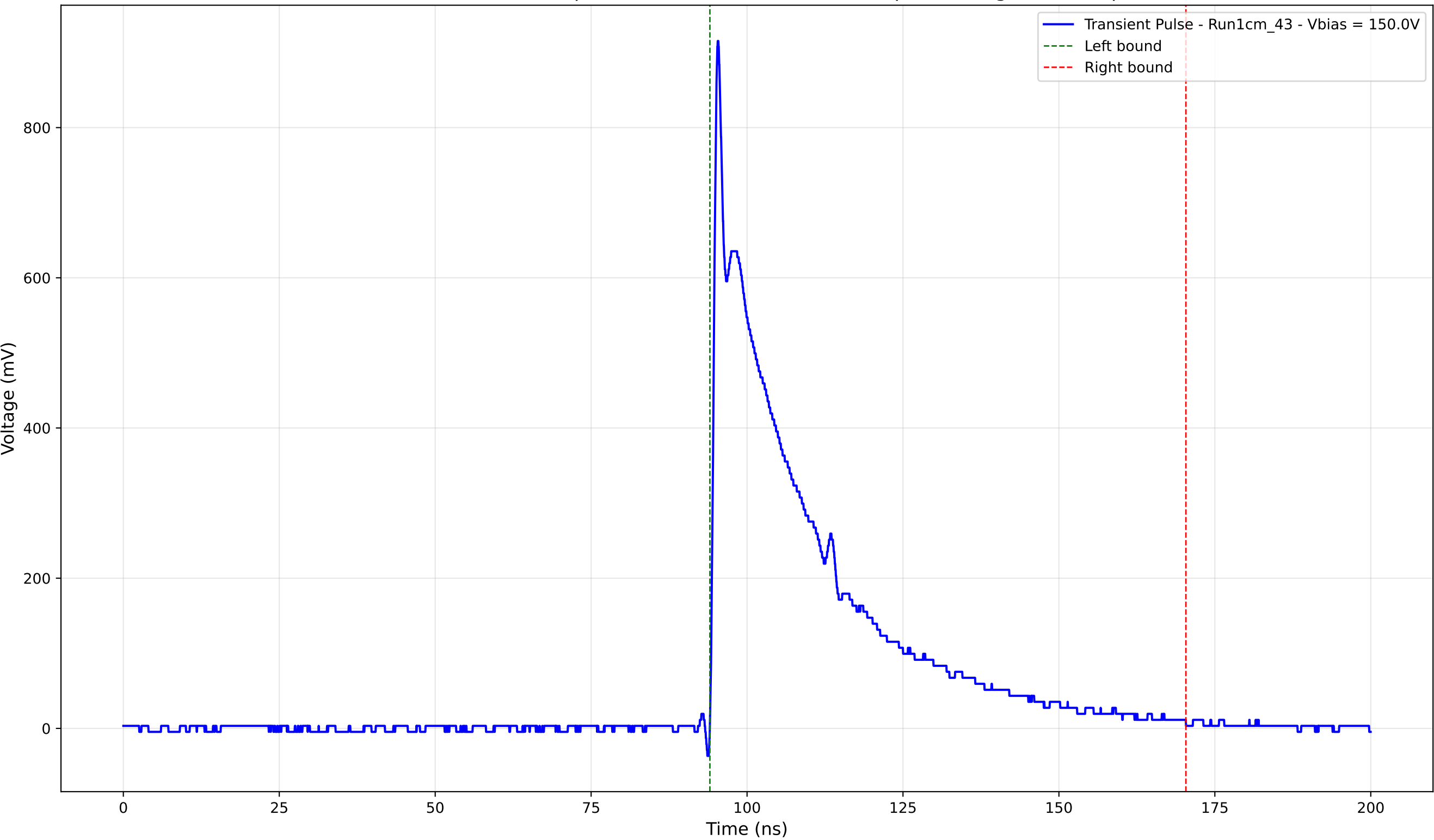
Transient Pulse - Sample: new1cm - Position: 2900.0 \mu\text{m} - Charge: 243.44 pC
