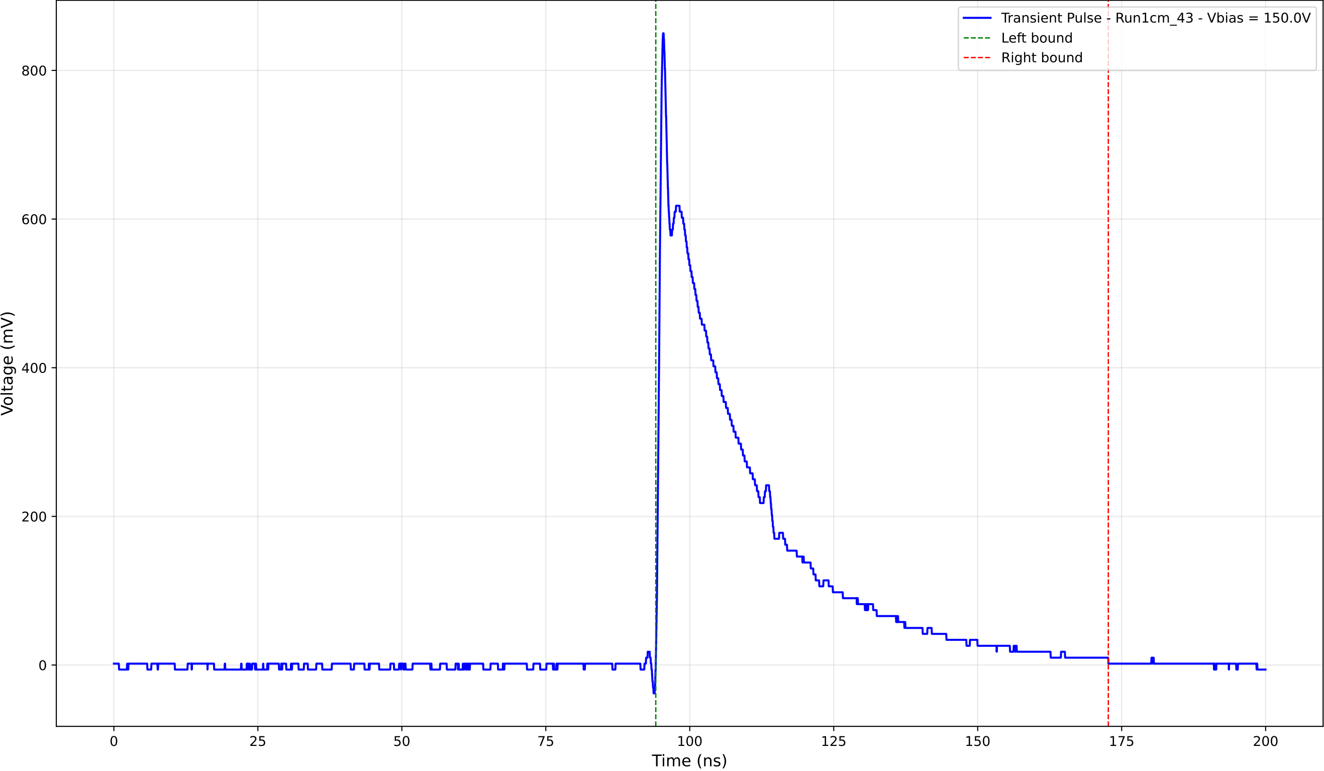
Transient Pulse - Sample: new1cm - Position: 2405.0 \mu\text{m} - Charge: 234.42 pC
