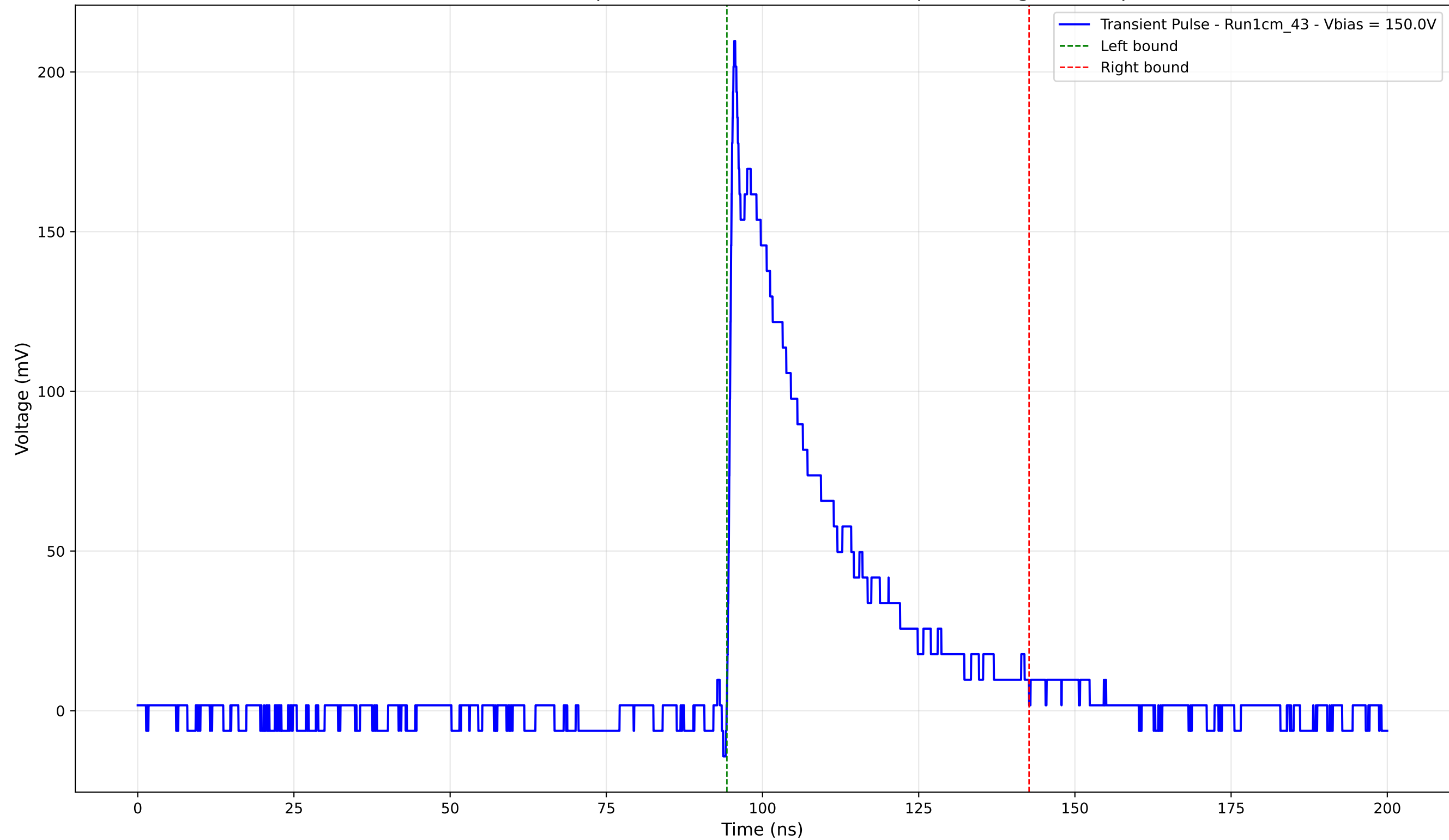
Transient Pulse - Sample: new1cm - Position: 3185.0 \mu\text{m} - Charge: 55.67 pC
