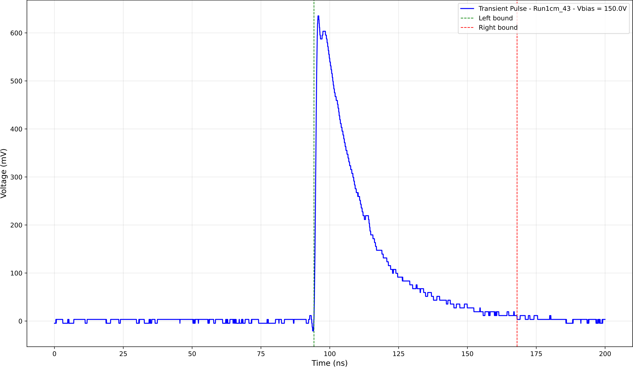
Transient Pulse - Sample: new1cm - Position: 2045.0 \mu\text{m} - Charge: 221.71 pC
