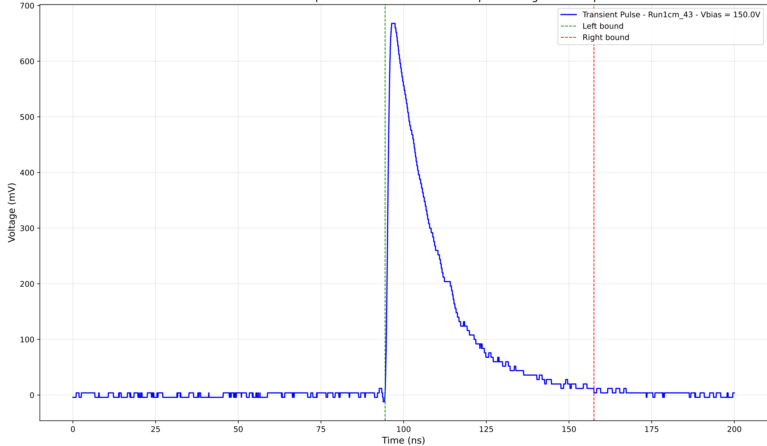
Transient Pulse - Sample: new1cm - Position: 905.0 \mu\text{m} - Charge: 205.82 pC
