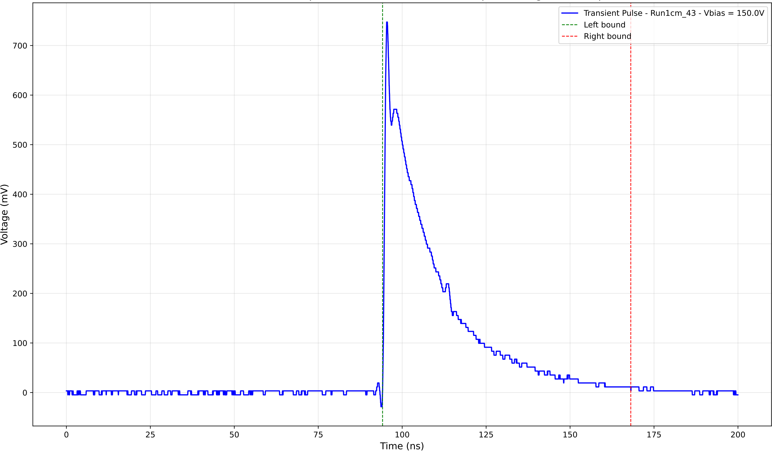
Transient Pulse - Sample: new1cm - Position: 2320.0 \mu\text{m} - Charge: 215.36 pC
