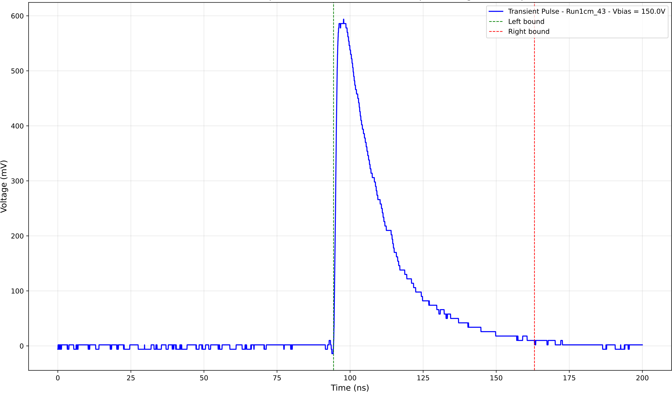
Transient Pulse - Sample: new1cm - Position: 1840.0 \mu\text{m} - Charge: 208.55 pC
