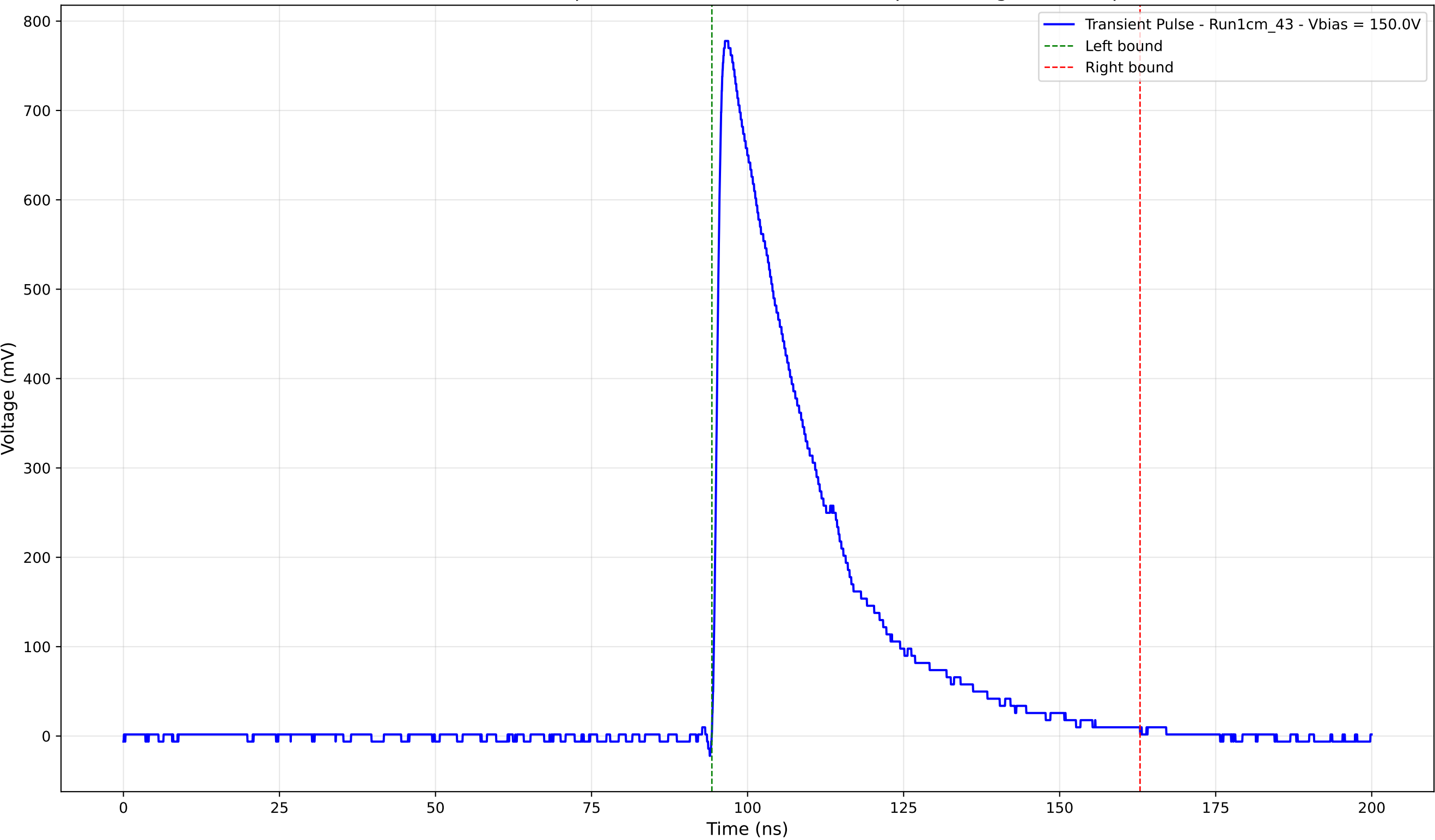
Transient Pulse - Sample: new1cm - Position: 4340.0 \mu\text{m} - Charge: 250.71 pC
