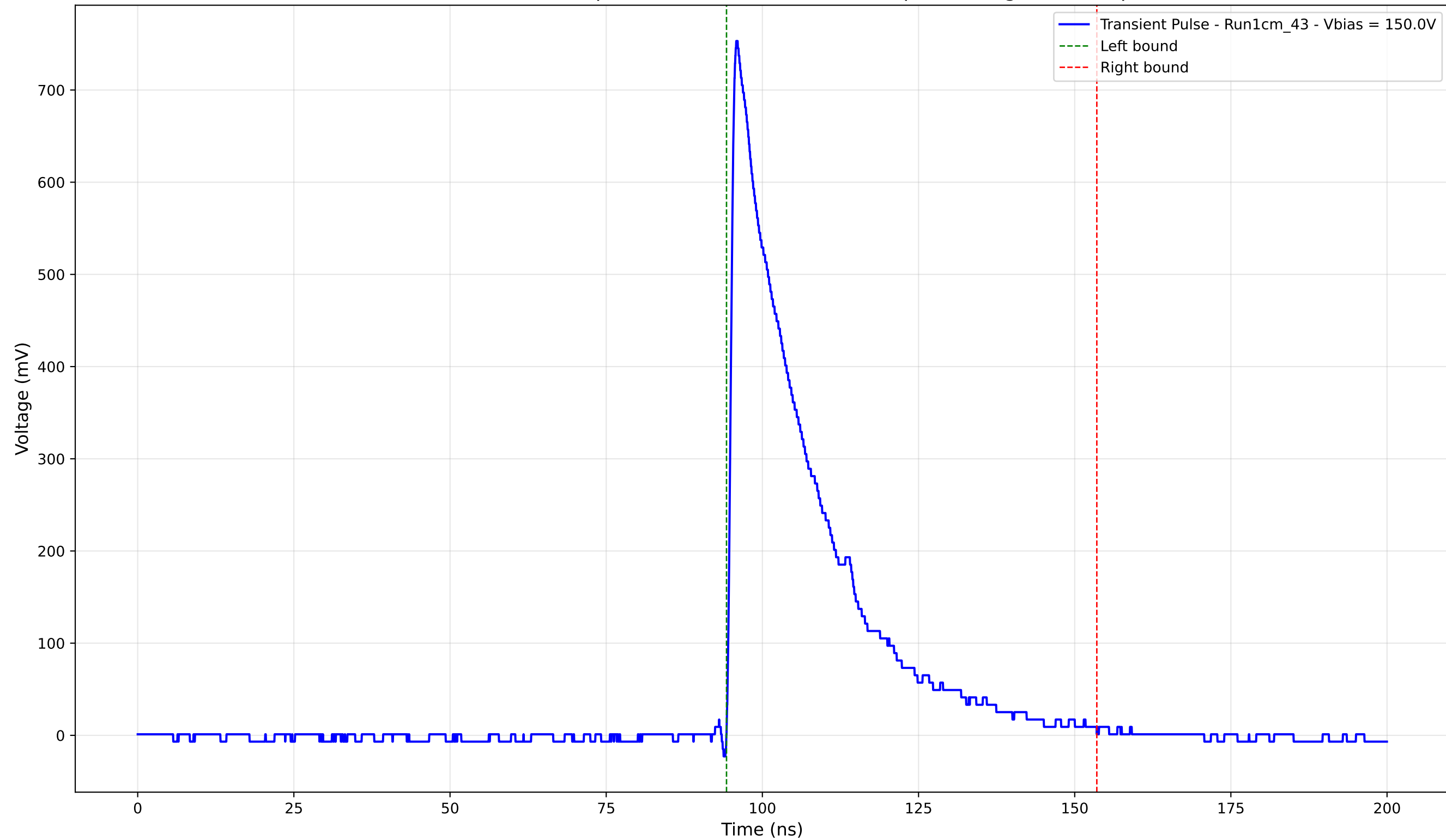
Transient Pulse - Sample: new1cm - Position: 510.0 \mu\text{m} - Charge: 196.70 pC
