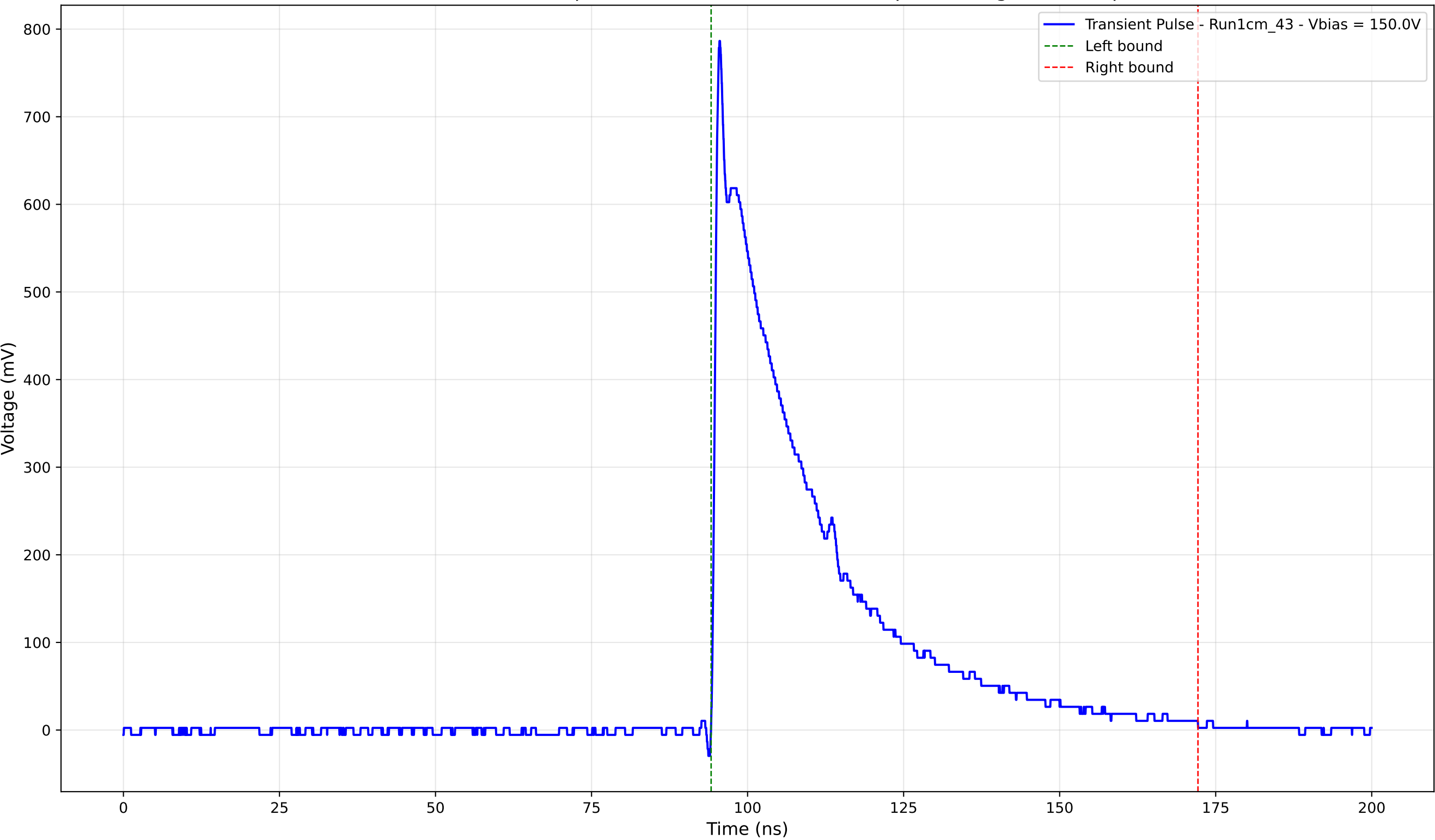
Transient Pulse - Sample: new1cm - Position: 3115.0 \mu\text{m} - Charge: 233.00 pC
