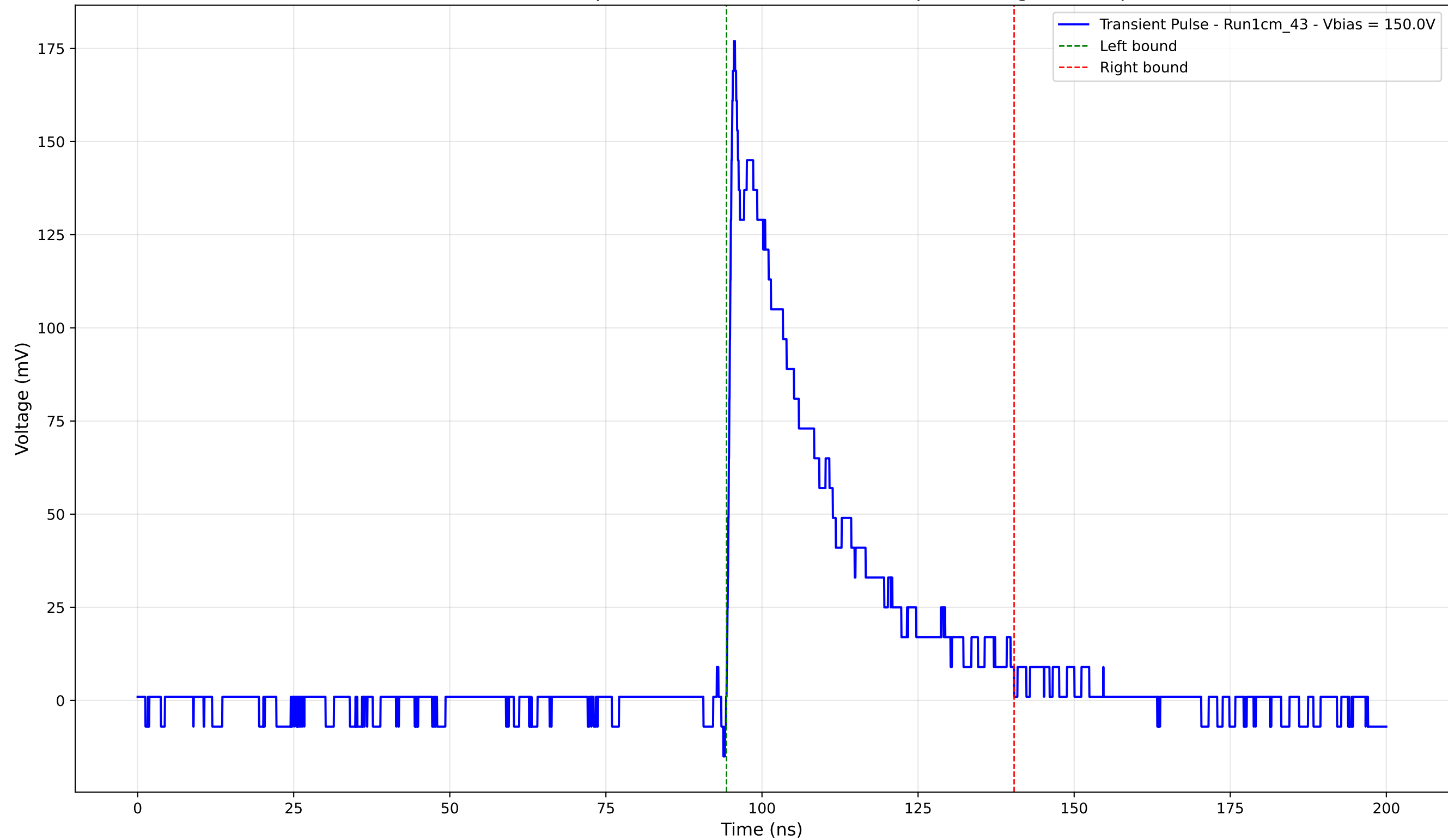
Transient Pulse - Sample: new1cm - Position: 3190.0 \mu\text{m} - Charge: 47.85 pC
