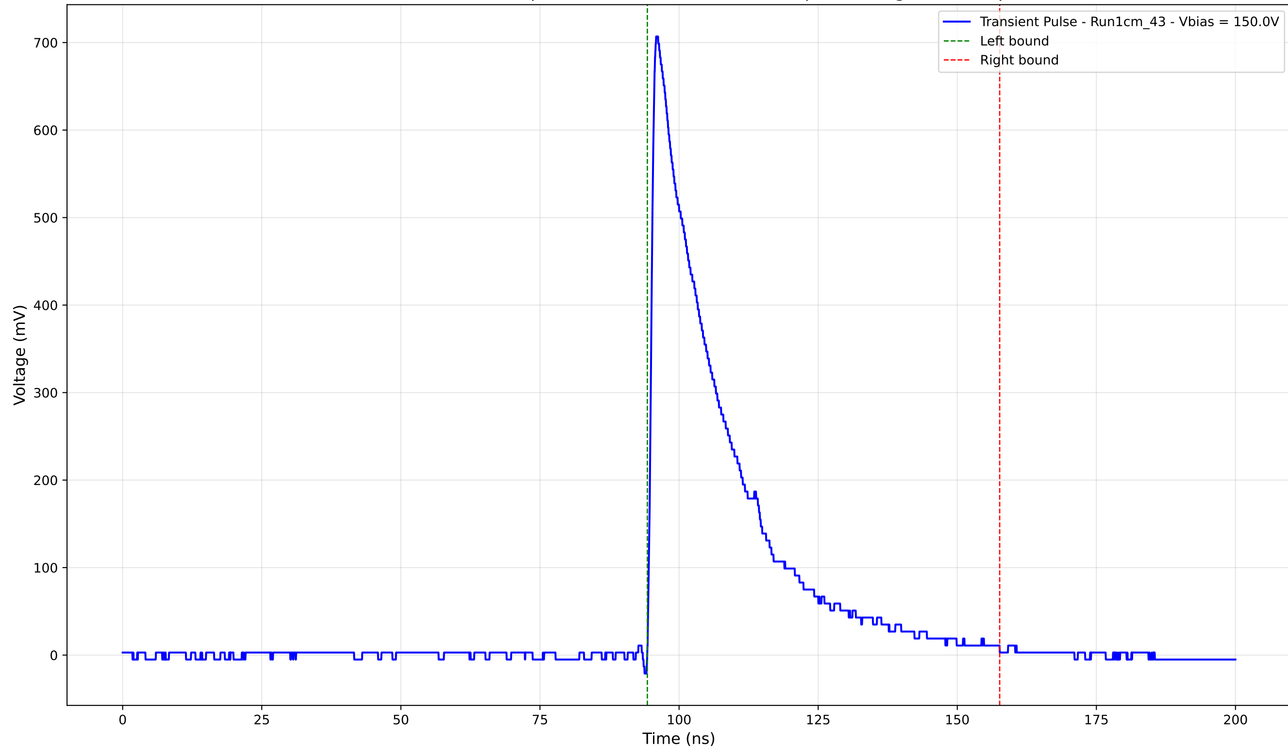
Transient Pulse - Sample: new1cm - Position: 565.0 \mu\text{m} - Charge: 191.84 pC
