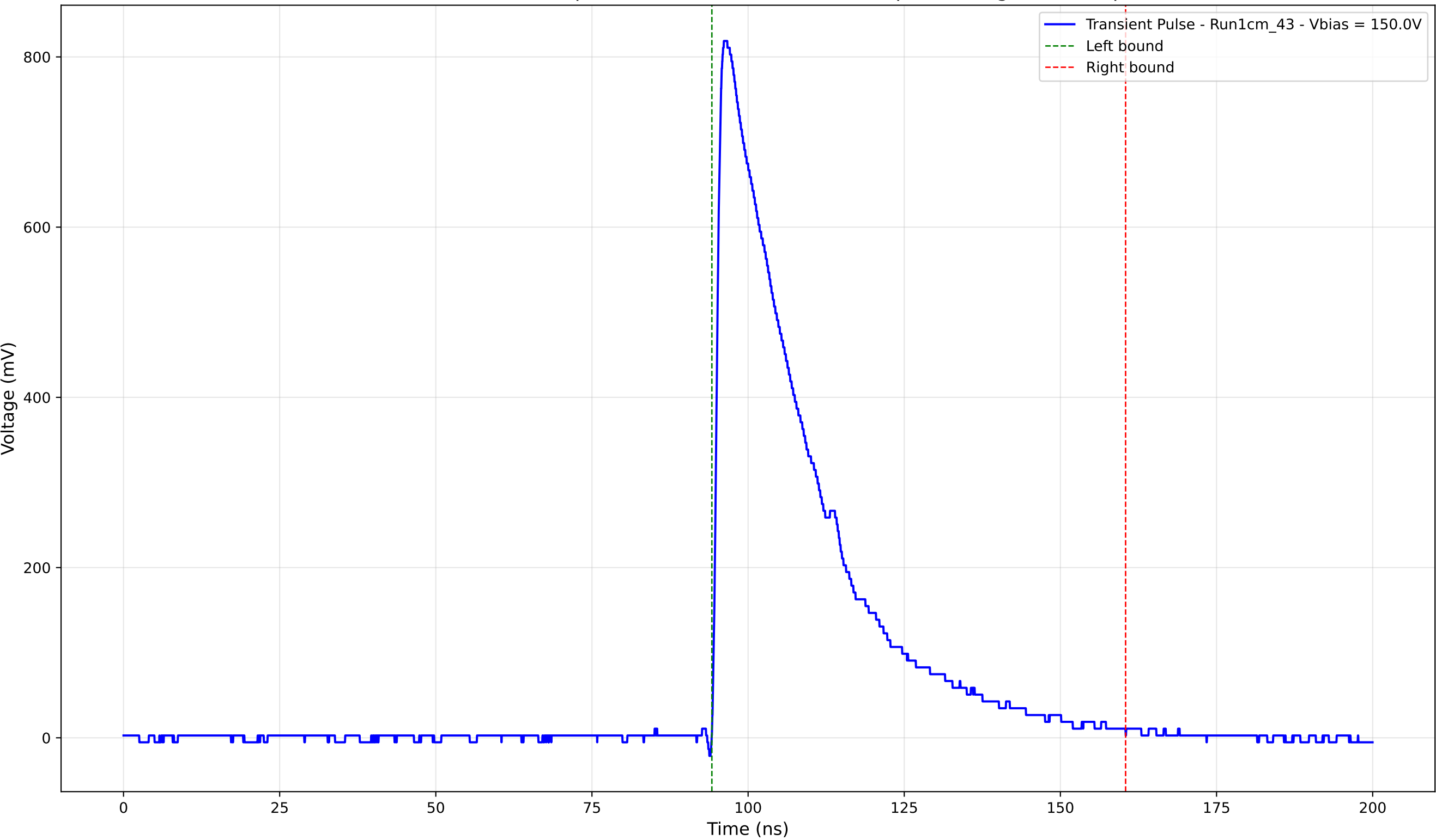
Transient Pulse - Sample: new1cm - Position: 4490.0 \mu\text{m} - Charge: 260.11 pC
