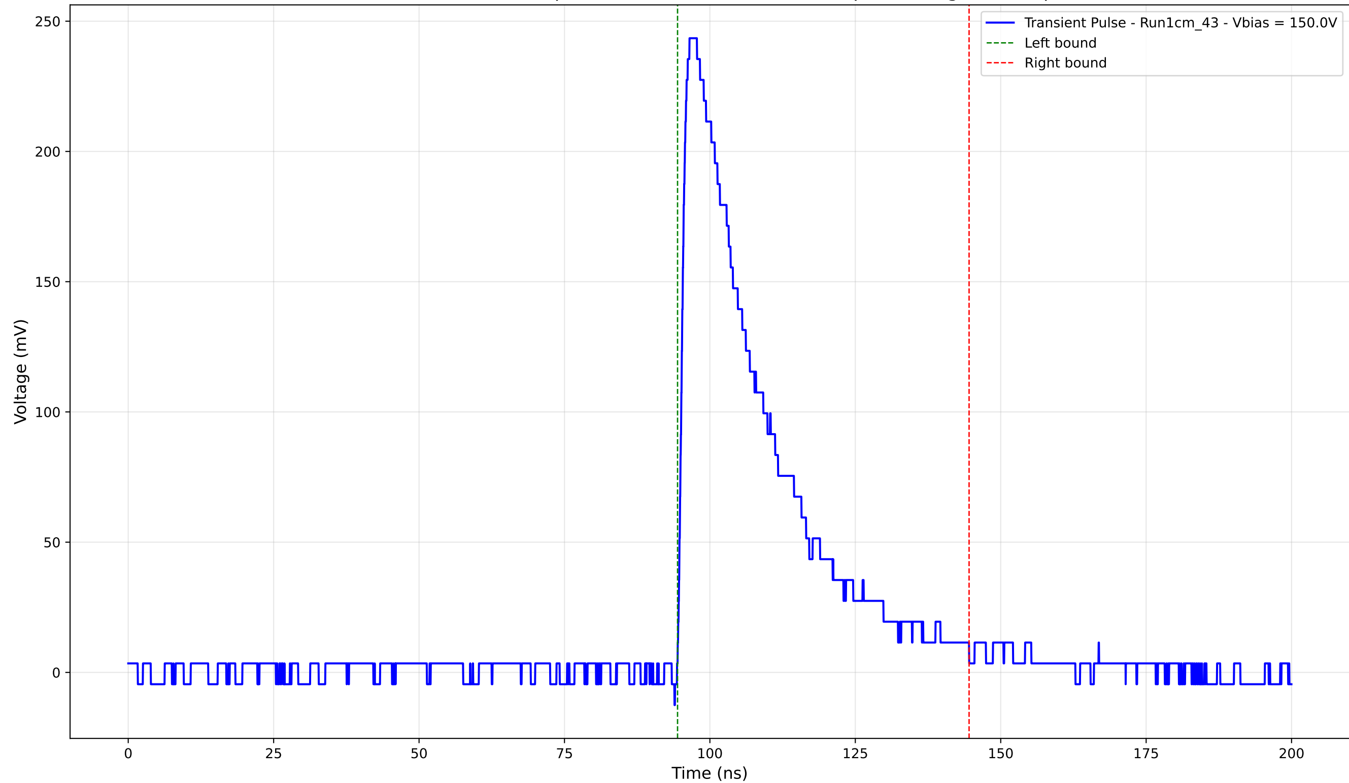
Transient Pulse - Sample: new1cm - Position: 4245.0 \mu\text{m} - Charge: 75.47 pC
