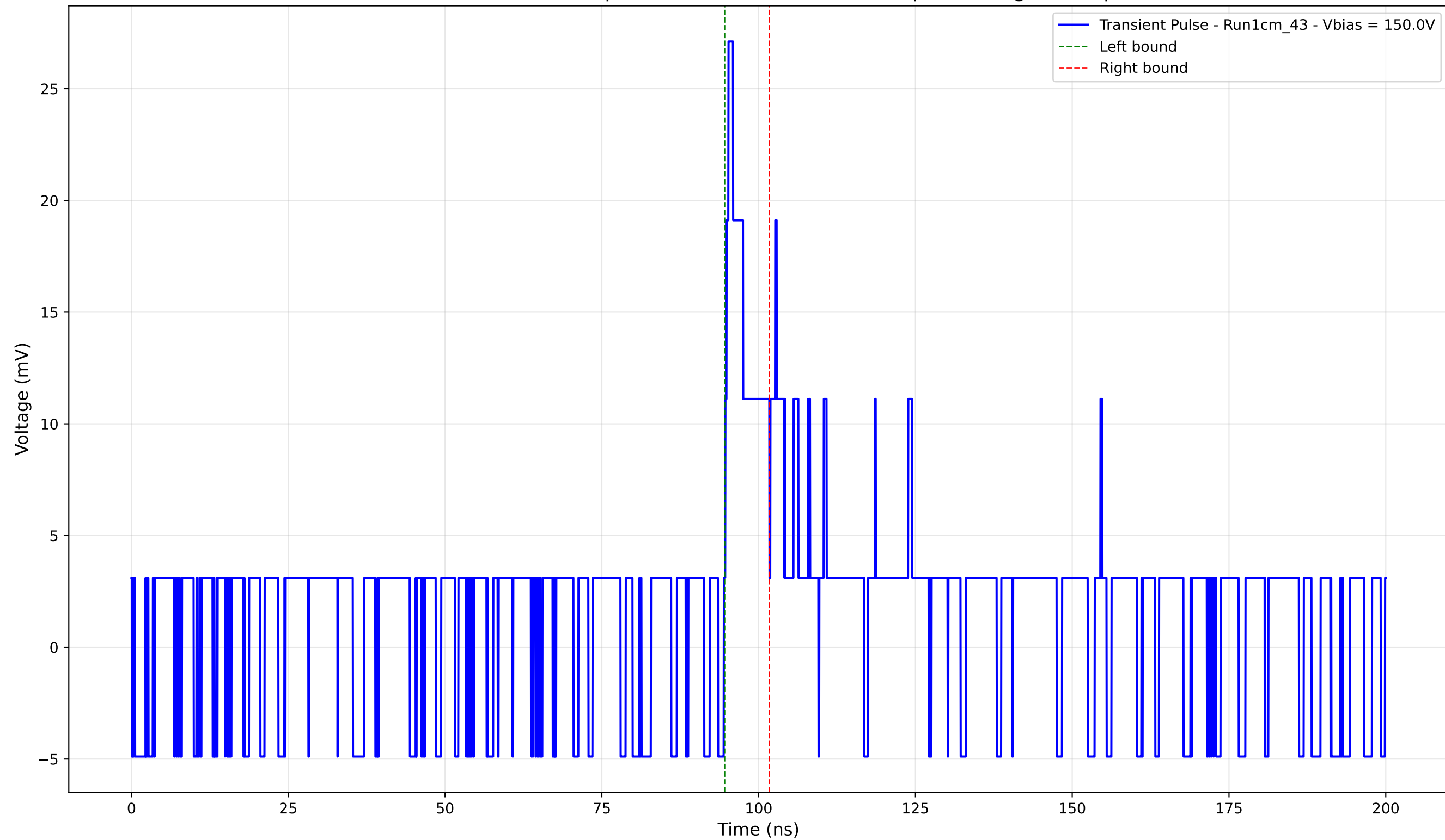
Transient Pulse - Sample: new1cm - Position: 120.0 \mu\text{m} - Charge: 2.11 pC
