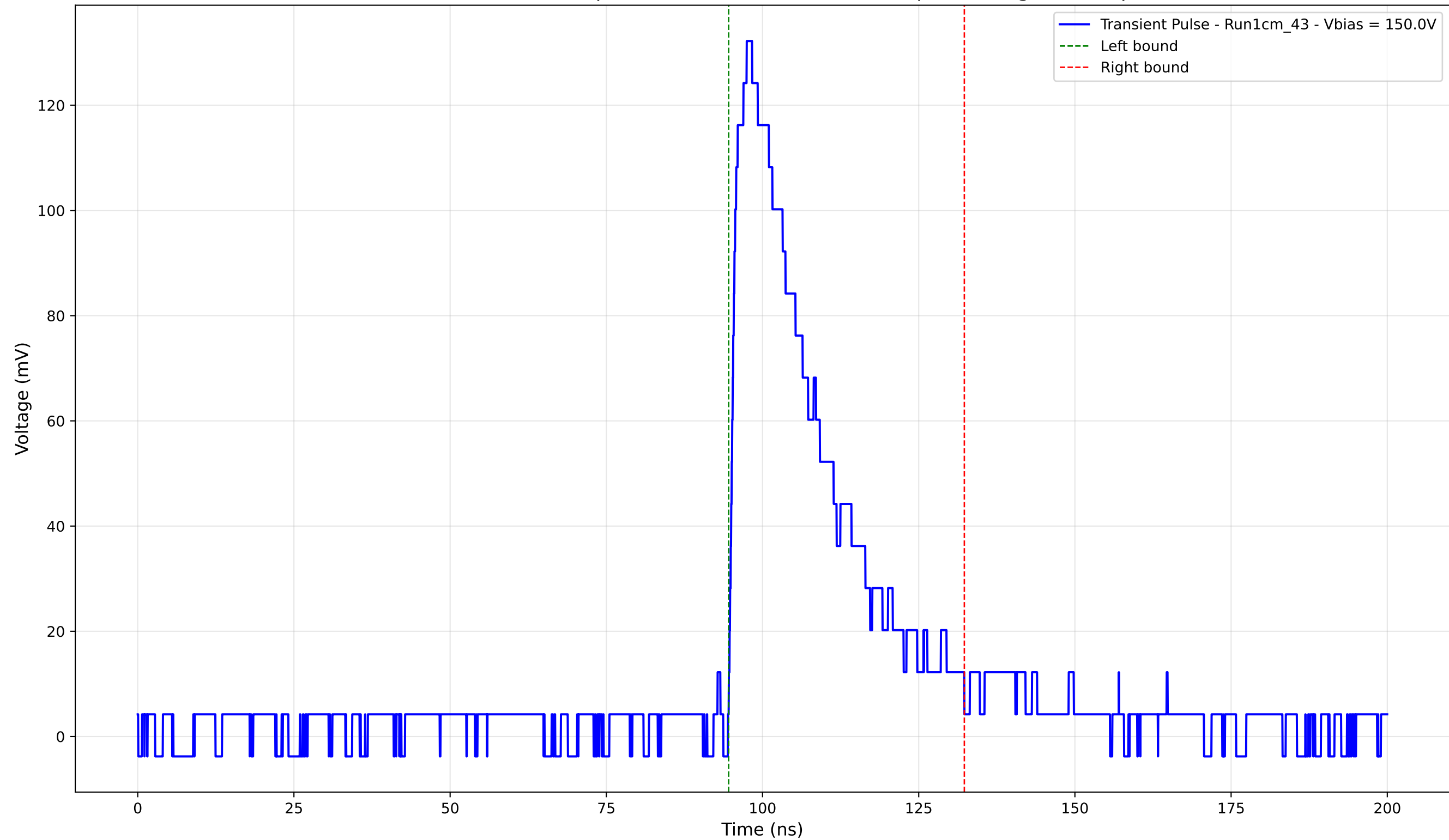
Transient Pulse - Sample: new1cm - Position: 4225.0 \mu\text{m} - Charge: 39.56 pC
