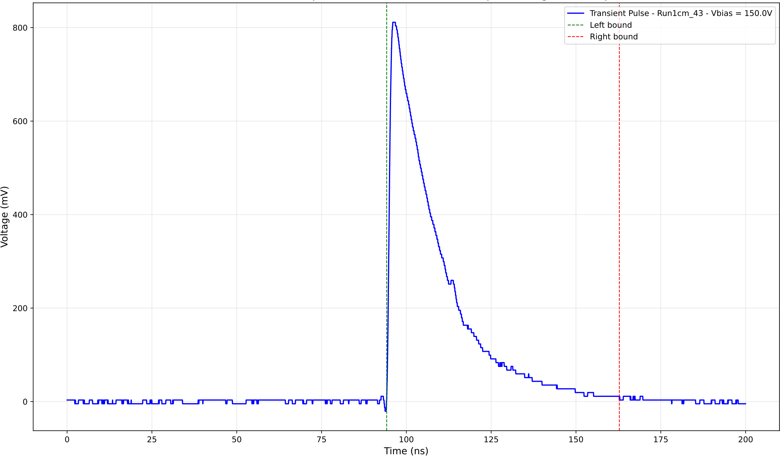
Transient Pulse - Sample: new1cm - Position: 4525.0 \mu\text{m} - Charge: 256.81 pC
