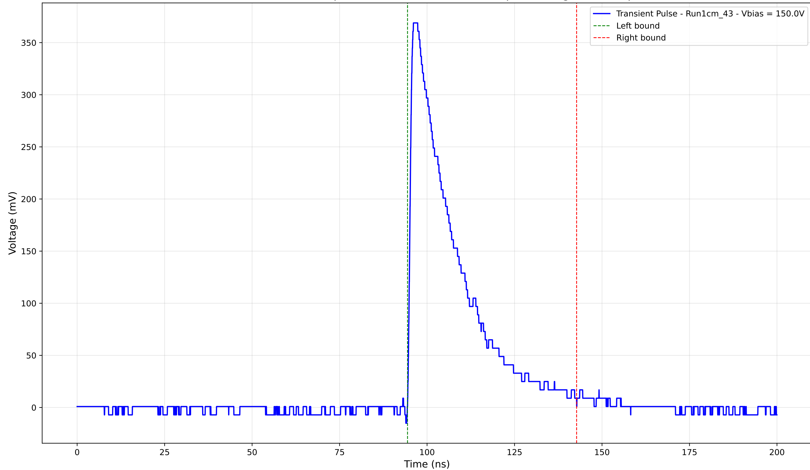
Transient Pulse - Sample: new1cm - Position: 730.0 \mu\text{m} - Charge: 103.51 pC
