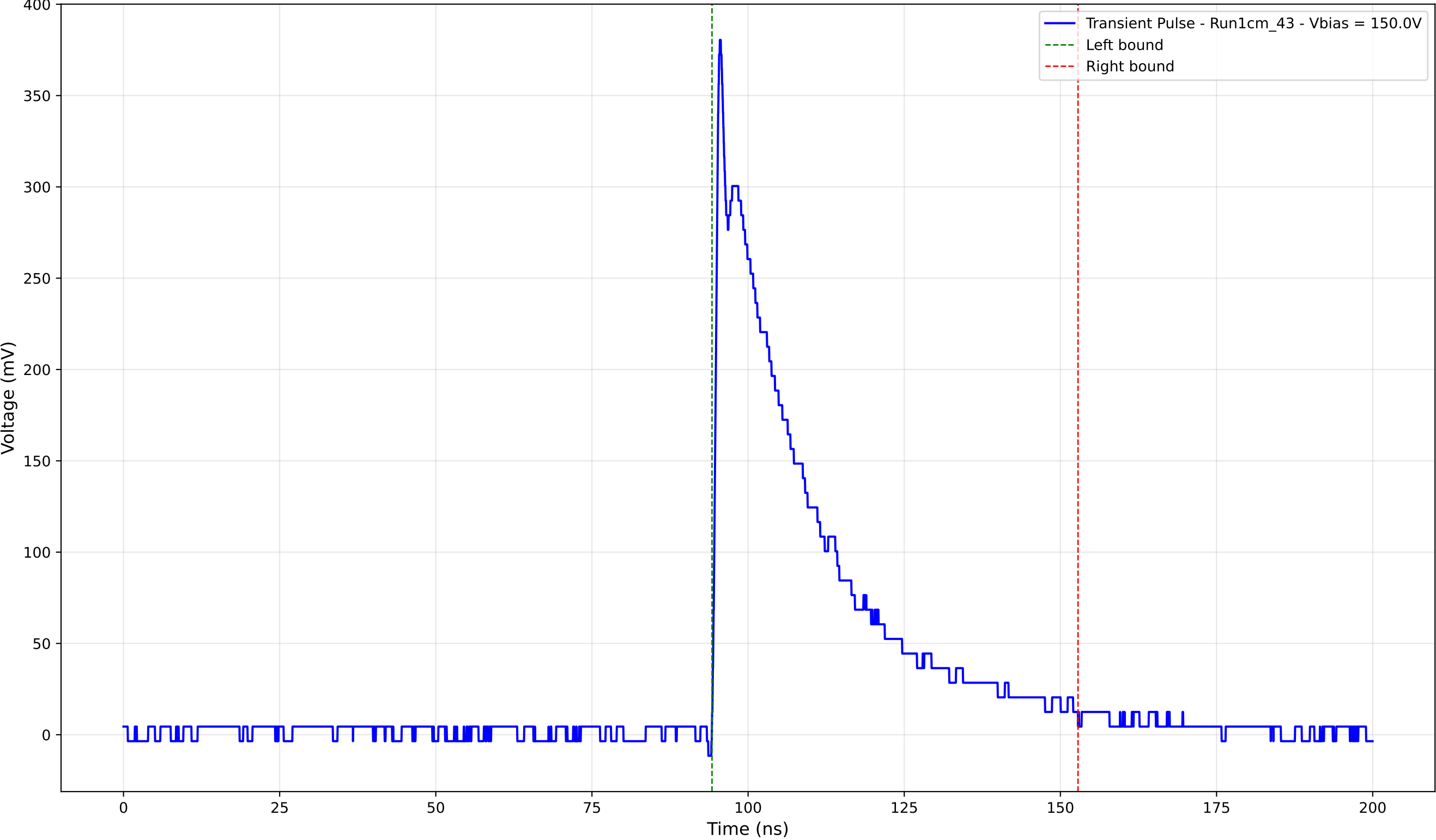
Transient Pulse - Sample: new1cm - Position: 2240.0 \mu\text{m} - Charge: 108.66 pC
