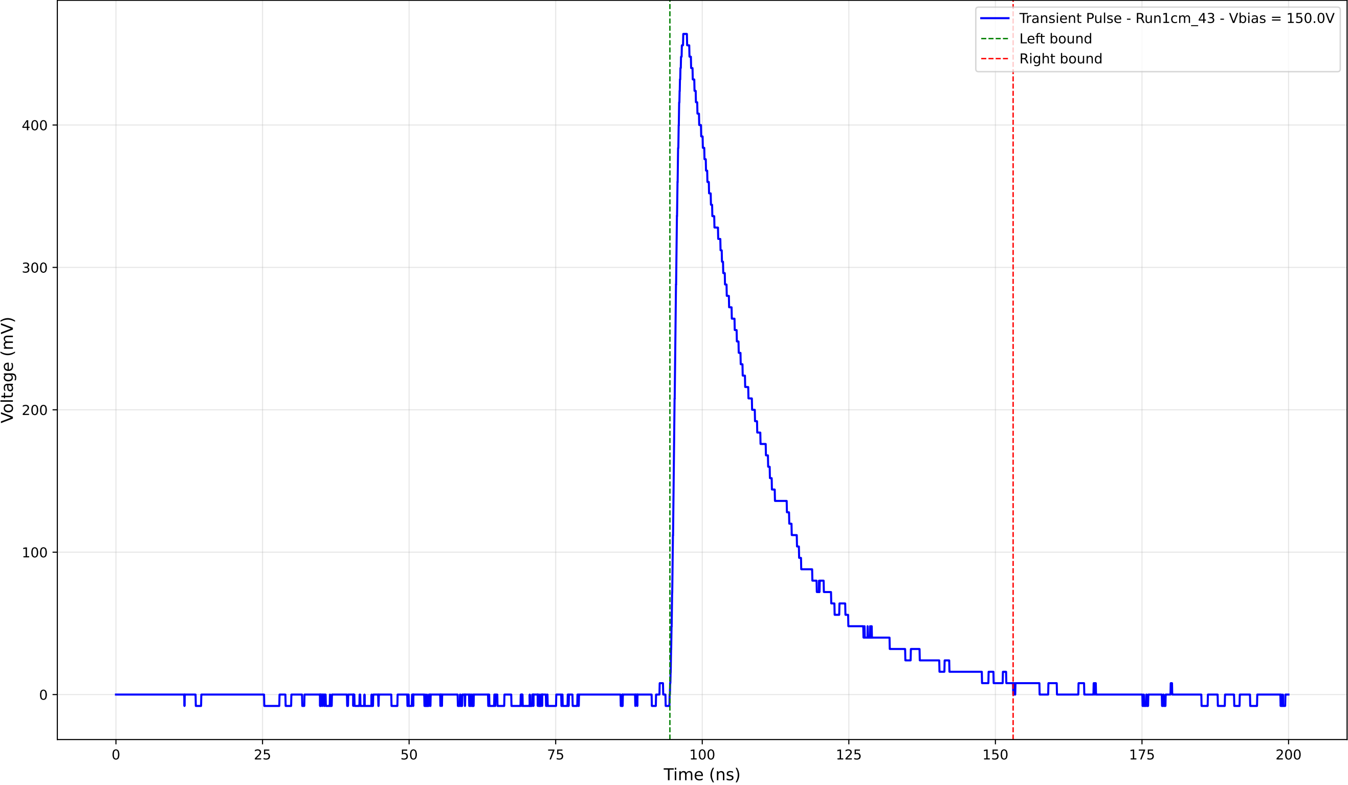
Transient Pulse - Sample: new1cm - Position: 1115.0 \mu\text{m} - Charge: 140.11 pC
