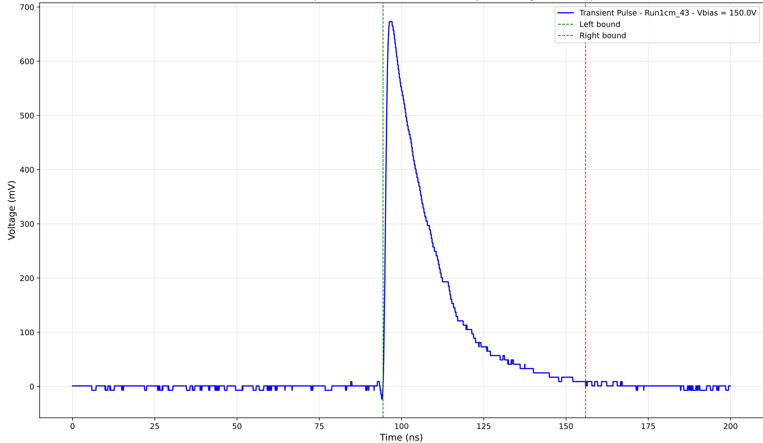
Transient Pulse - Sample: new1cm - Position: 825.0 \mu\text{m} - Charge: 200.70 pC
