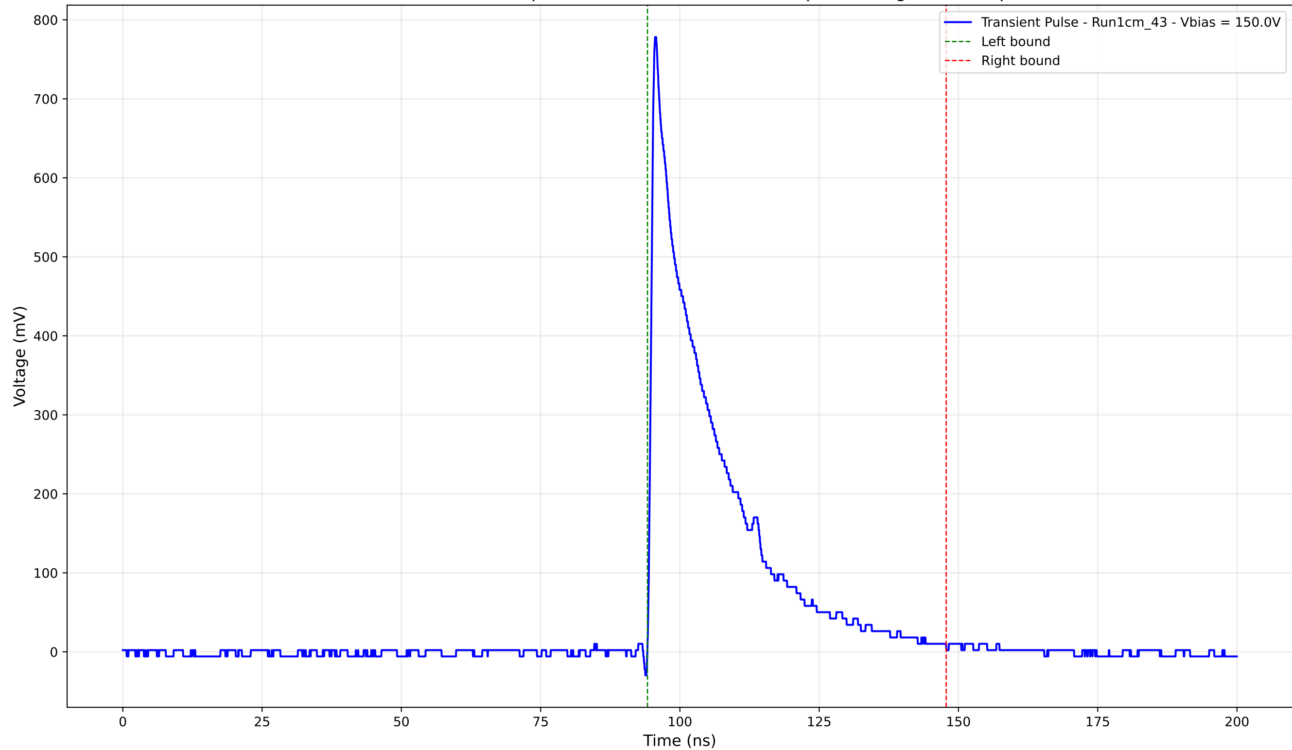
Transient Pulse - Sample: new1cm - Position: 295.0 \mu\text{m} - Charge: 172.75 pC
