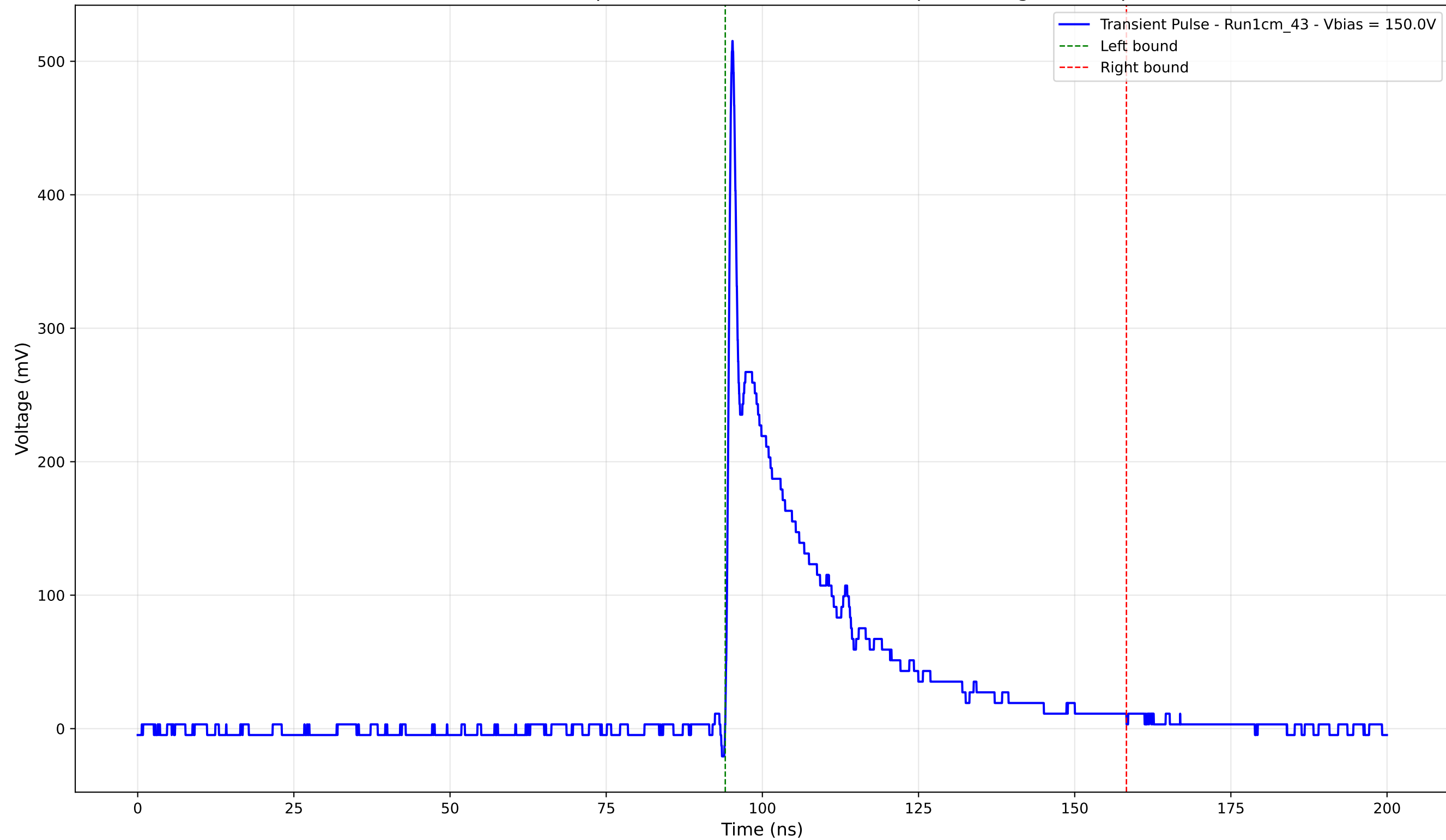
Transient Pulse - Sample: new1cm - Position: 2655.0 \mu\text{m} - Charge: 99.59 pC
