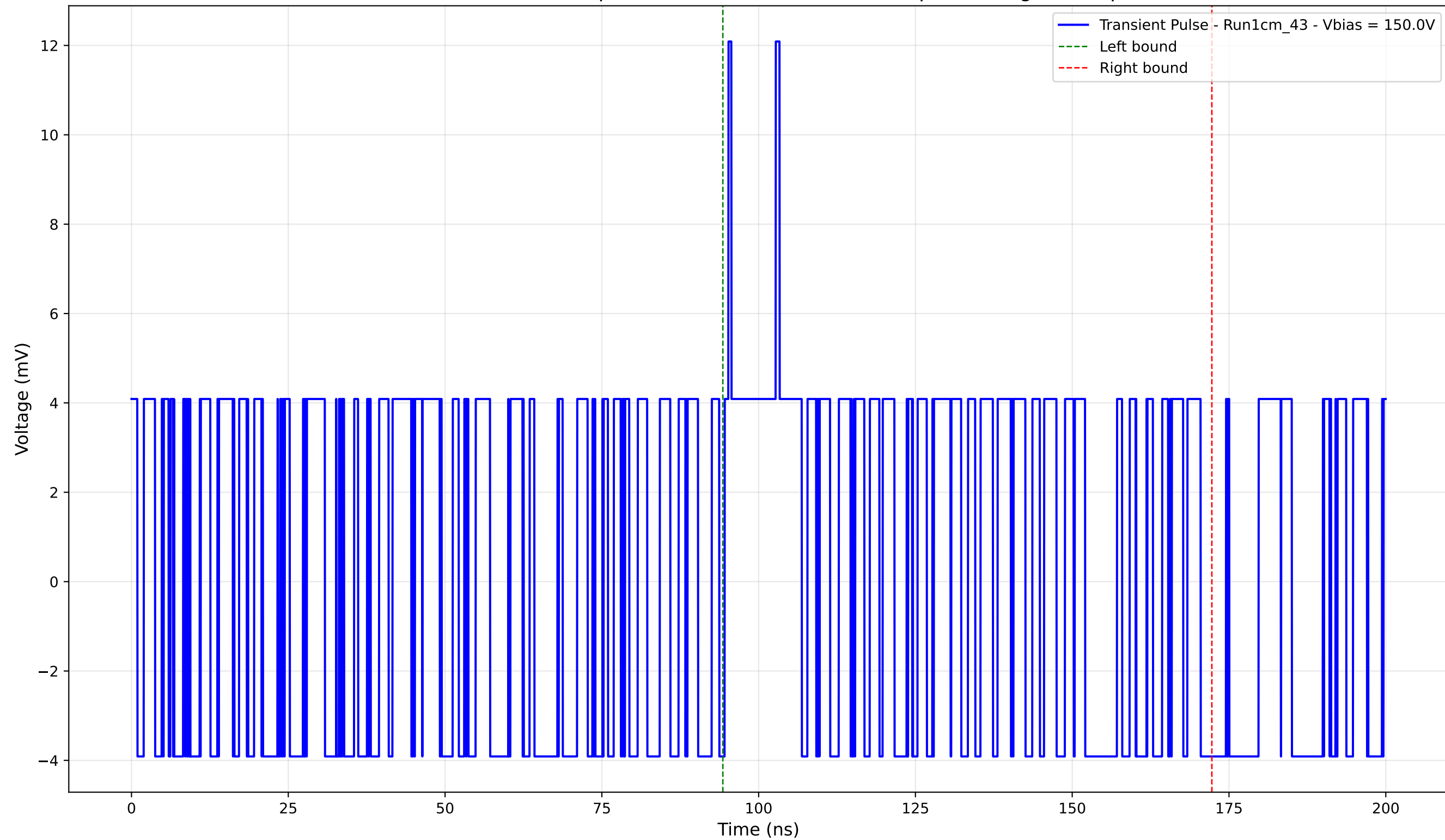
Transient Pulse - Sample: new1cm - Position: 5195.0 \mu\text{m} - Charge: 2.19 pC
