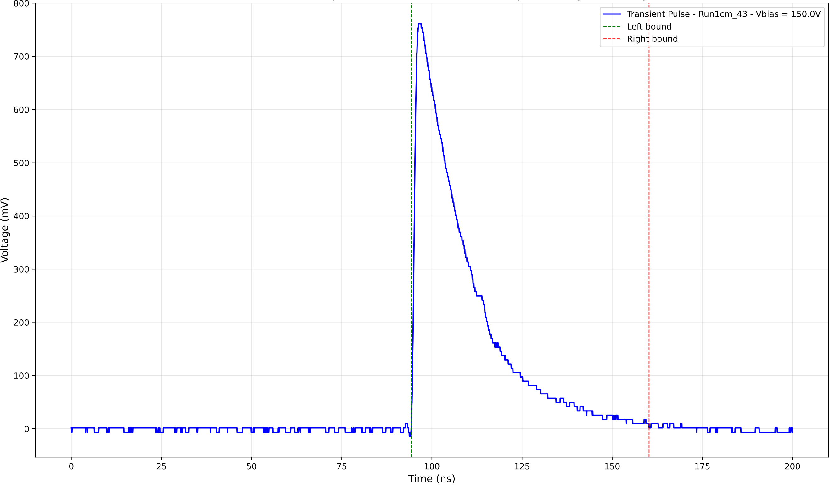
Transient Pulse - Sample: new1cm - Position: 4330.0 \mu\text{m} - Charge: 244.82 pC
