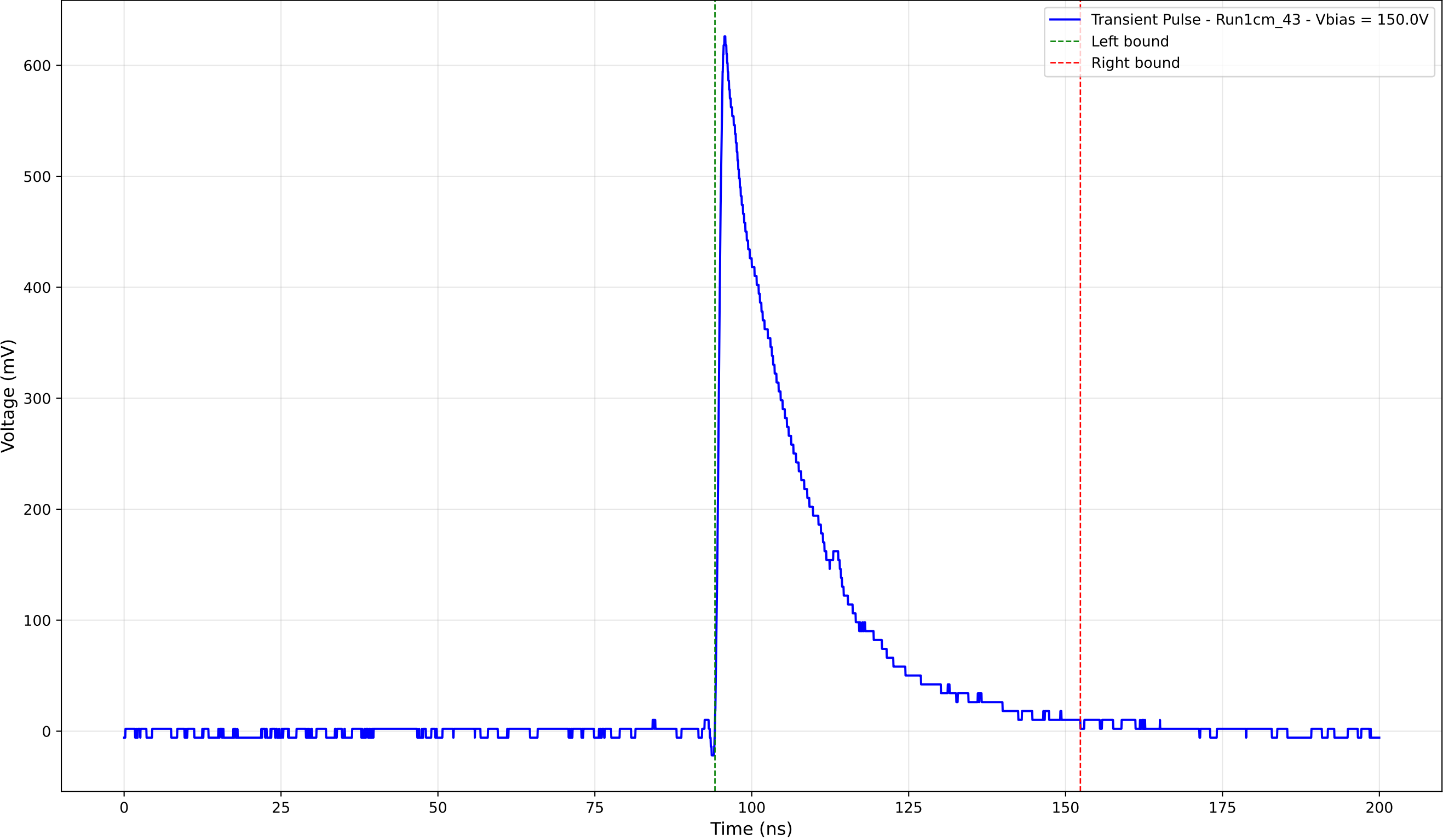
Transient Pulse - Sample: new1cm - Position: 4795.0 \mu\text{m} - Charge: 161.51 pC
