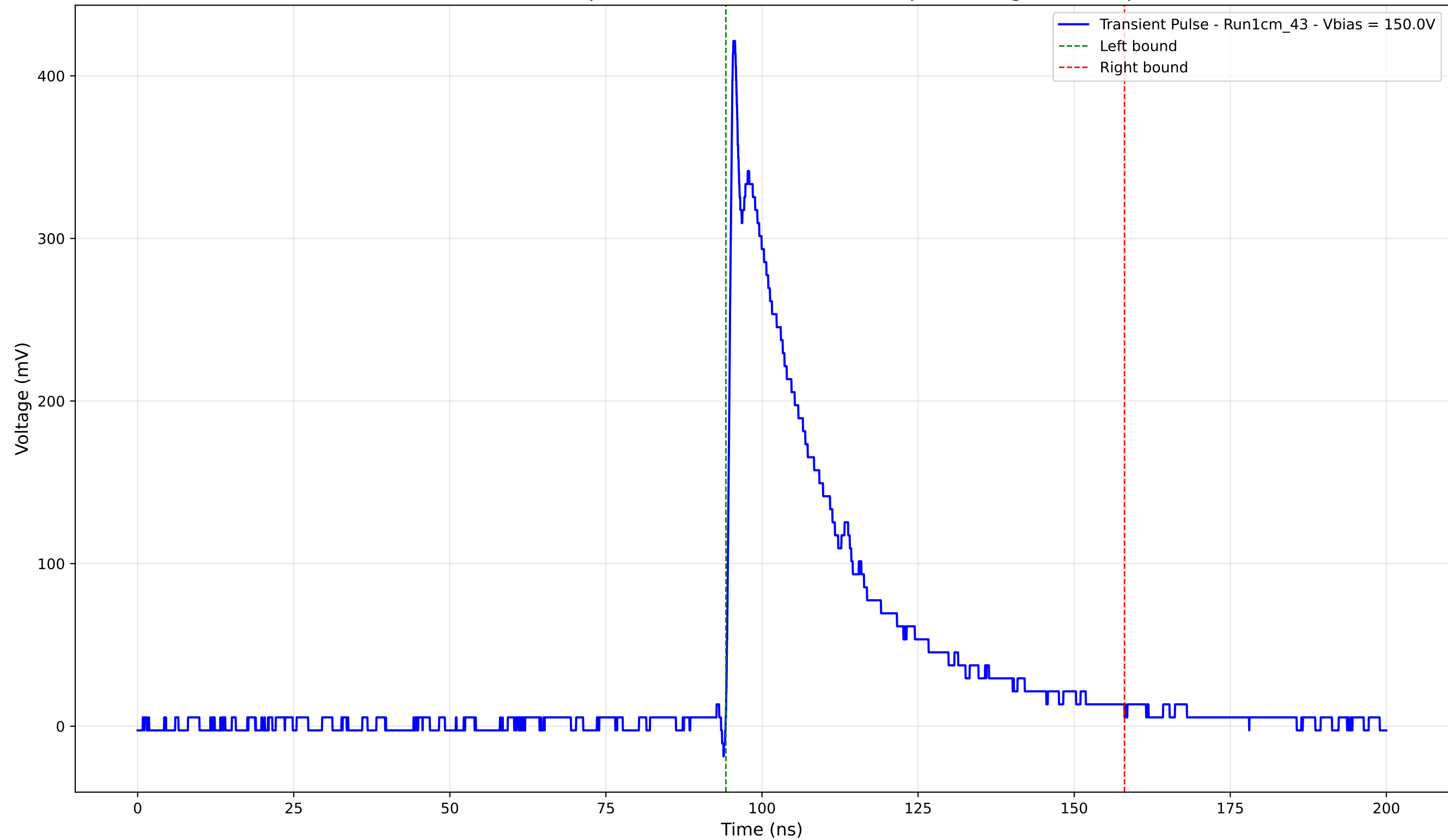
Transient Pulse - Sample: new1cm - Position: 2245.0 \mu\text{m} - Charge: 122.55 pC
