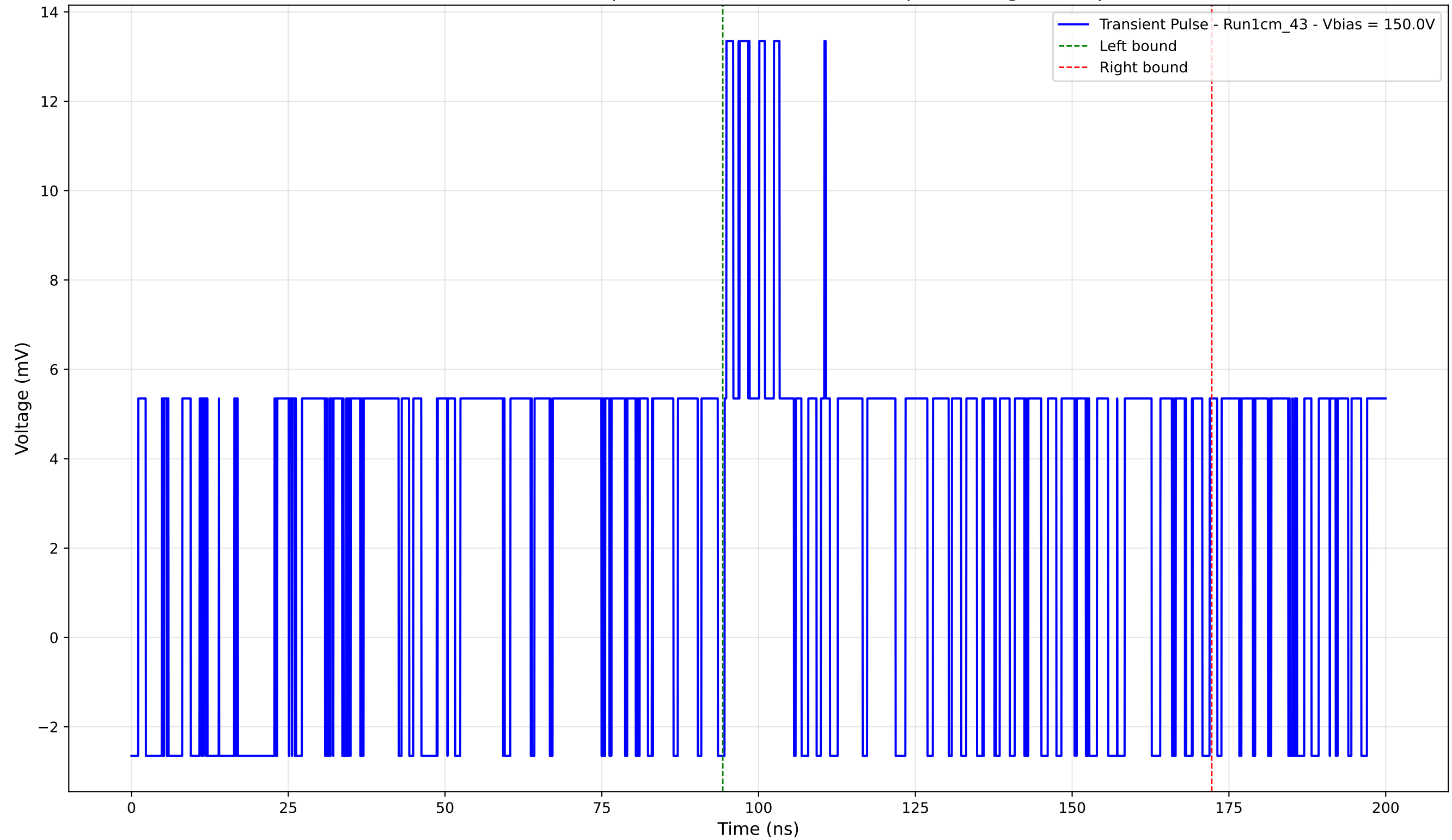
Transient Pulse - Sample: new1cm - Position: 85.0 \mu\text{m} - Charge: 5.71 pC
