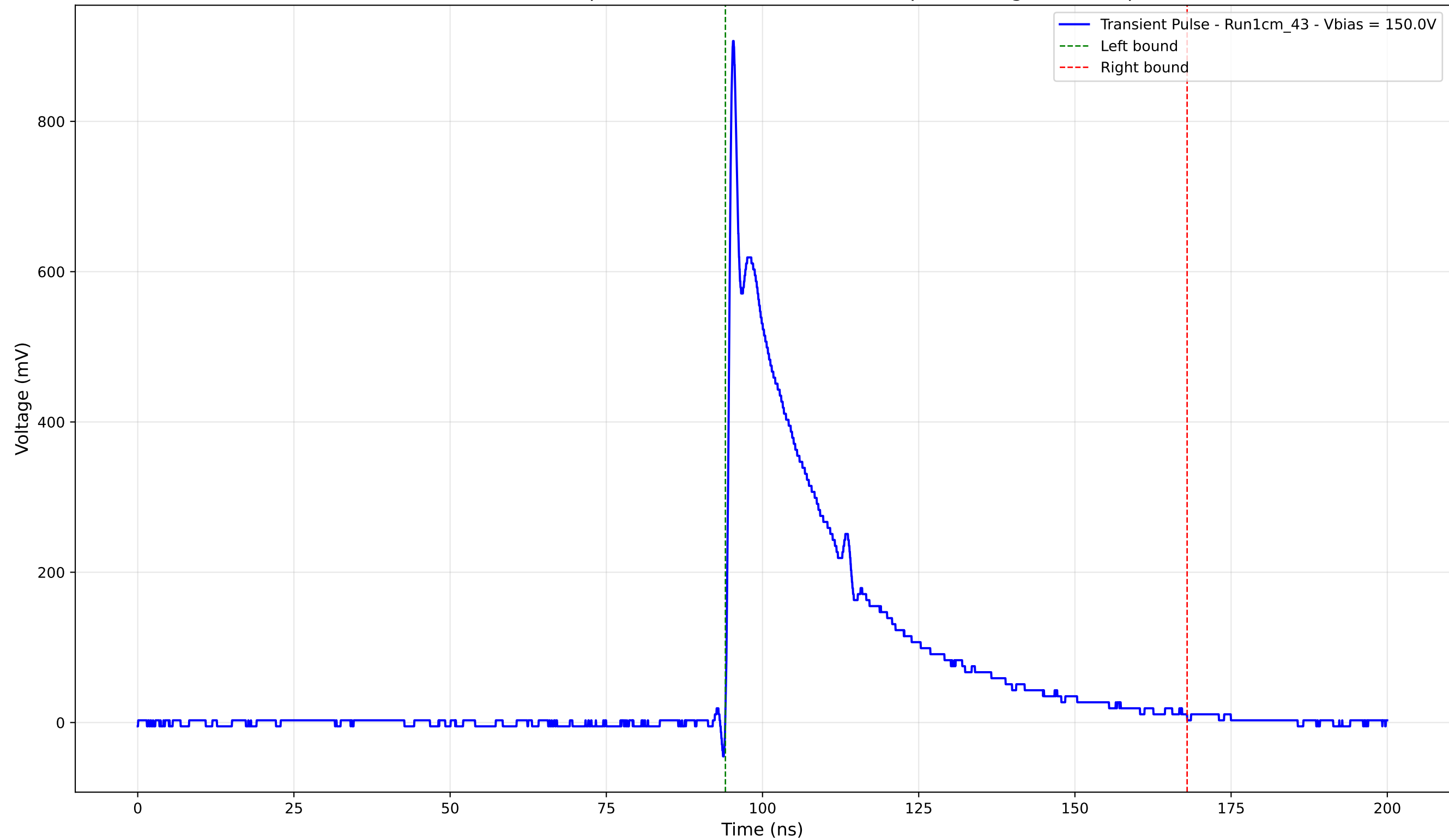
Transient Pulse - Sample: new1cm - Position: 2515.0 \mu\text{m} - Charge: 236.23 pC
