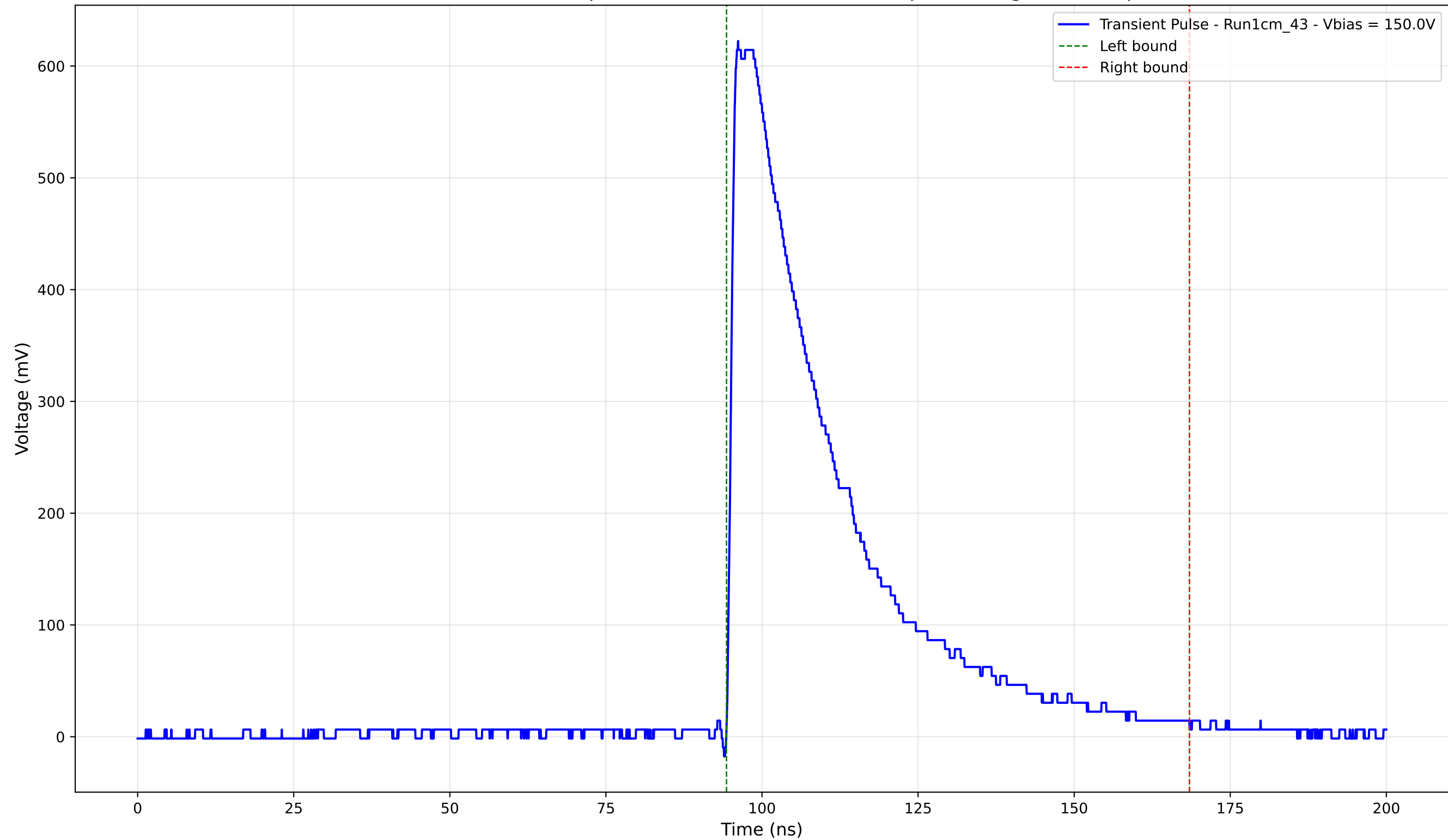
Transient Pulse - Sample: new1cm - Position: 1895.0 \mu\text{m} - Charge: 226.54 pC
