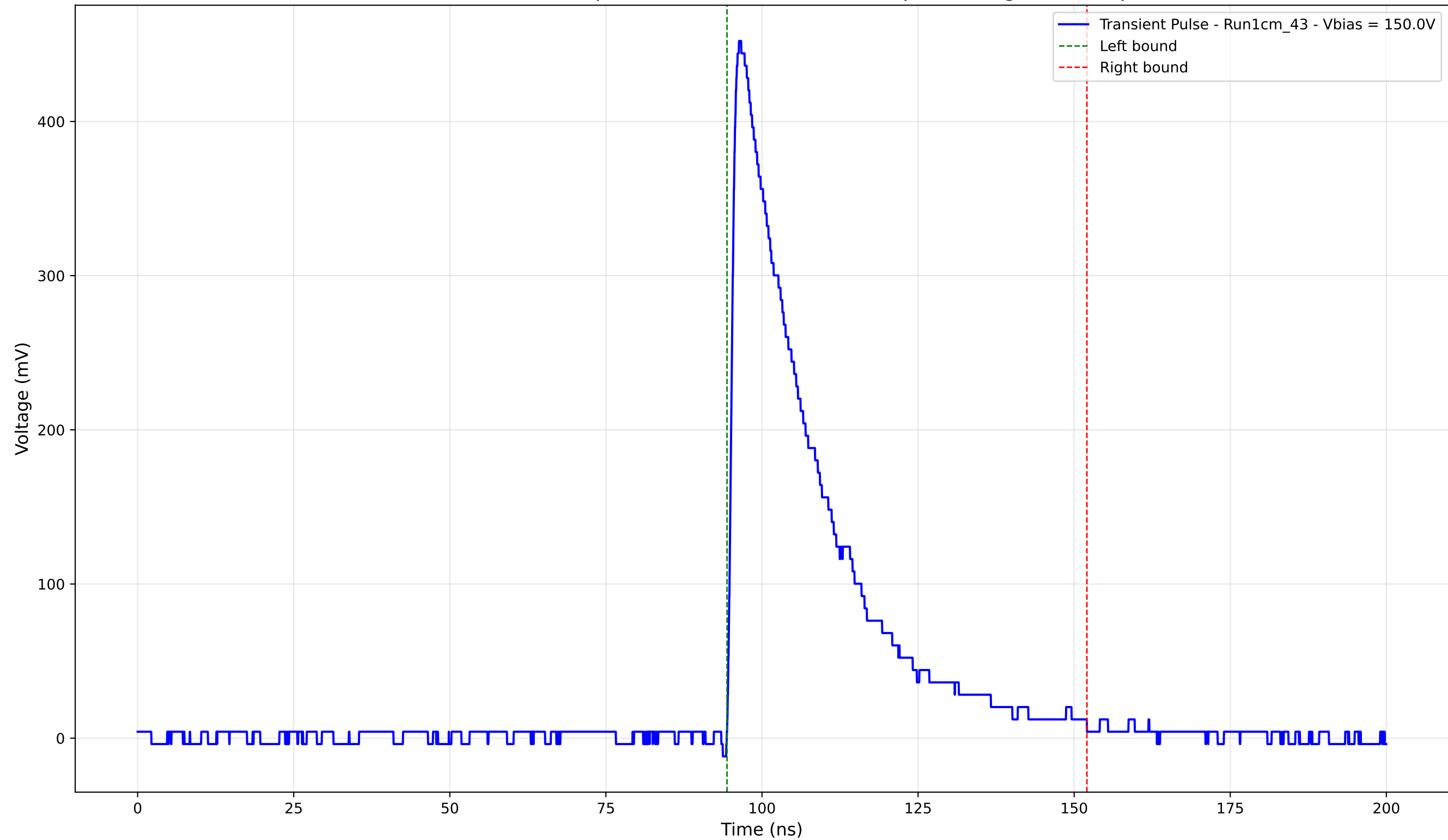
Transient Pulse - Sample: new1cm - Position: 740.0 \mu\text{m} - Charge: 128.88 pC
