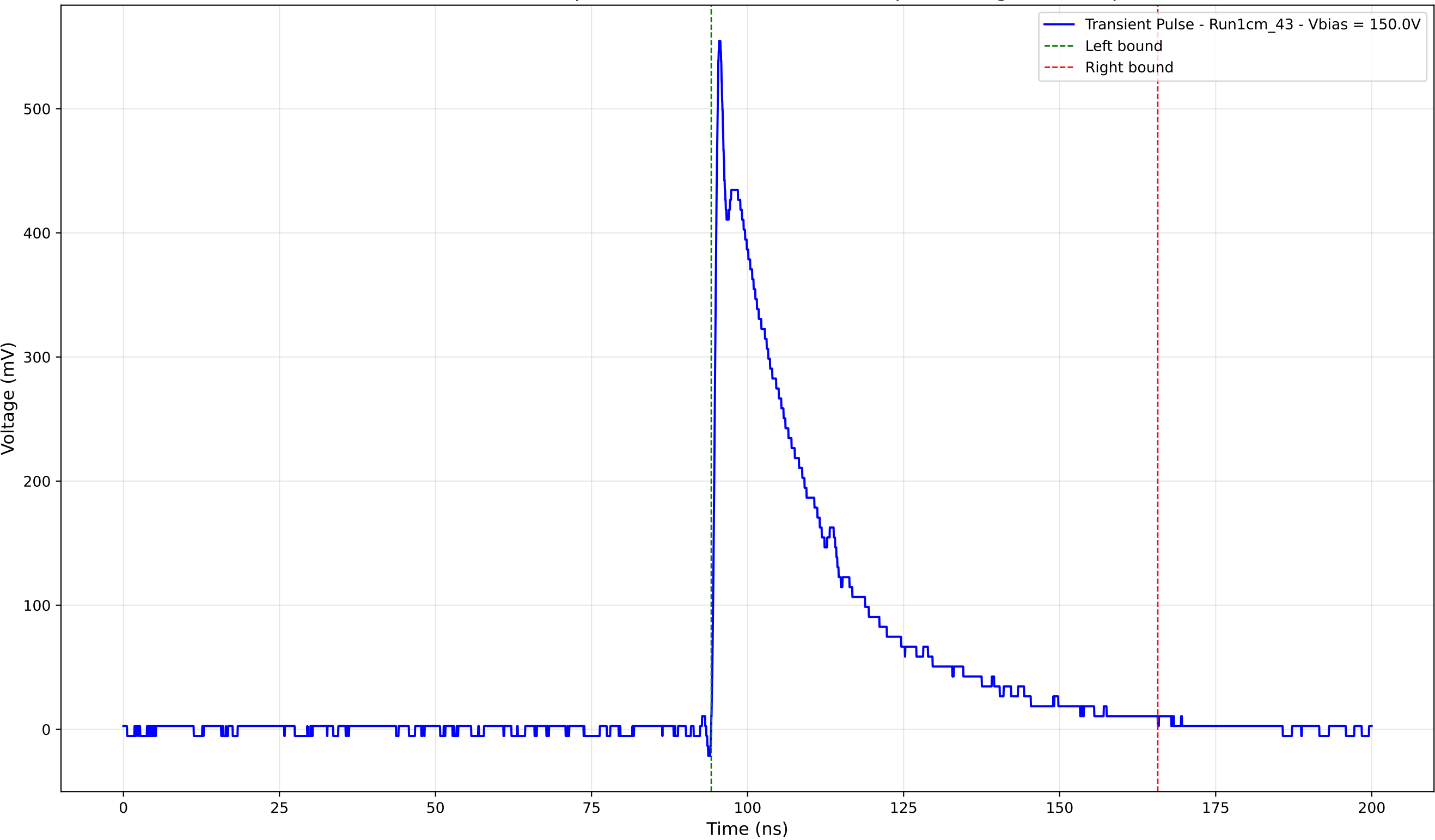
Transient Pulse - Sample: new1cm - Position: 2265.0 \mu\text{m} - Charge: 161.09 pC
