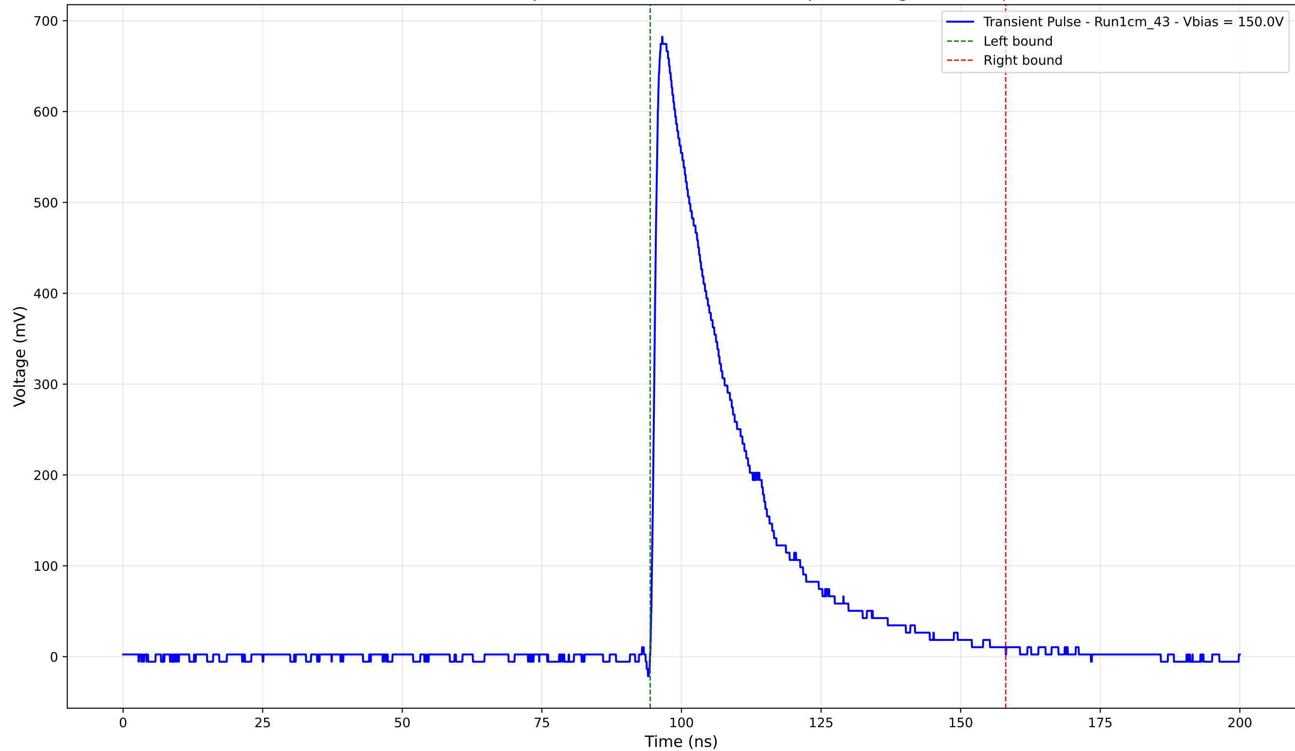
Transient Pulse - Sample: new1cm - Position: 845.0 \mu\text{m} - Charge: 204.06 pC
