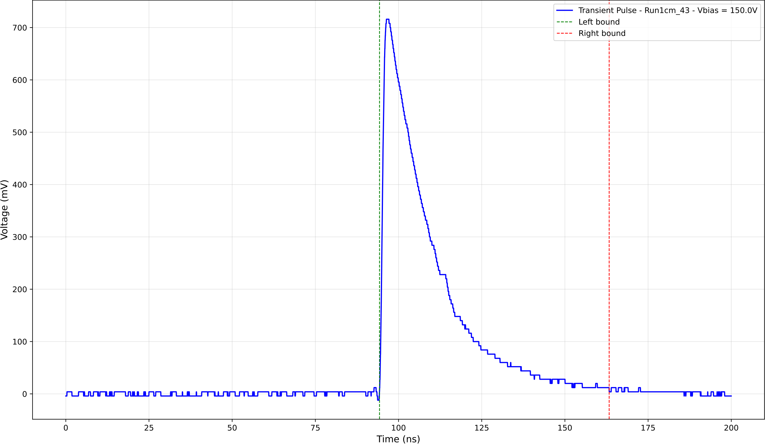
Transient Pulse - Sample: new1cm - Position: 4310.0 \mu\text{m} - Charge: 230.11 pC
