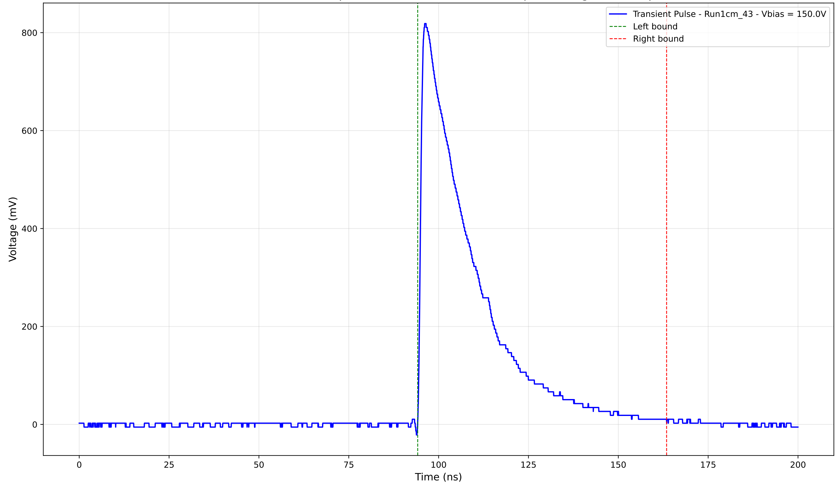
Transient Pulse - Sample: new1cm - Position: 4520.0 \mu\text{m} - Charge: 257.54 pC
