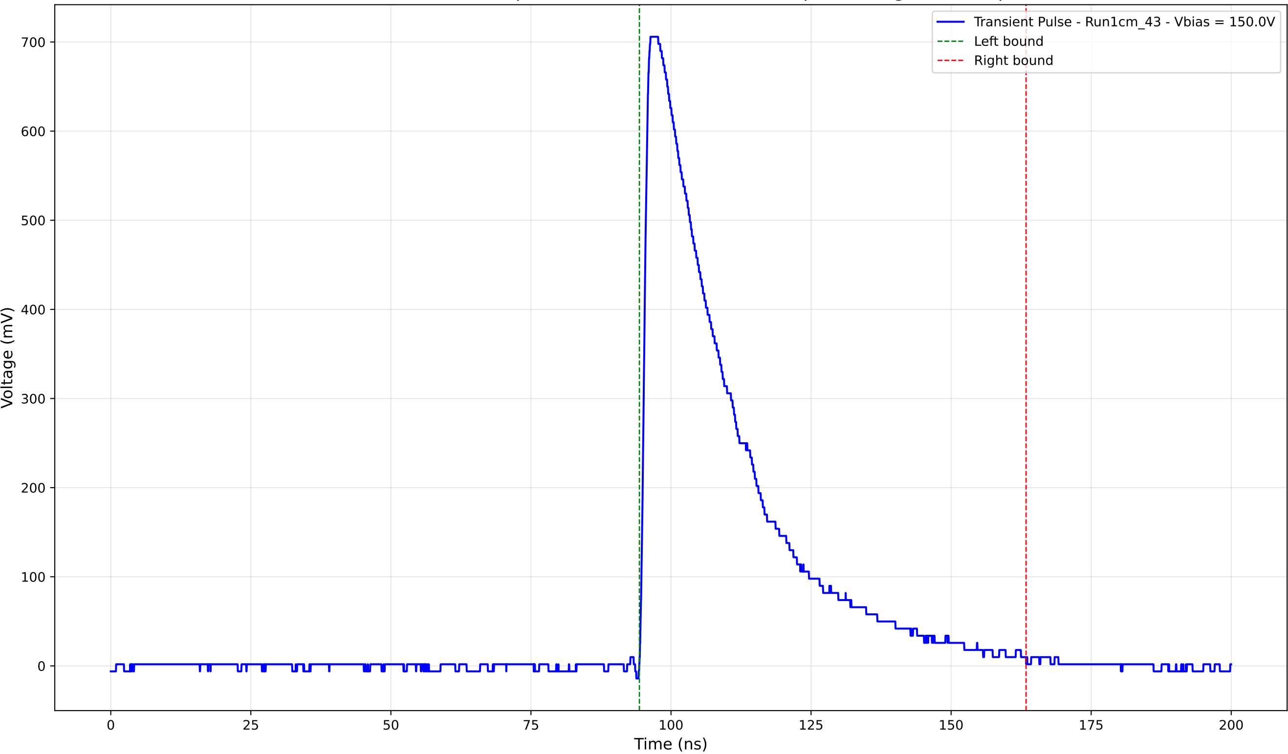
Transient Pulse - Sample: new1cm - Position: 3805.0 \mu\text{m} - Charge: 243.40 pC
