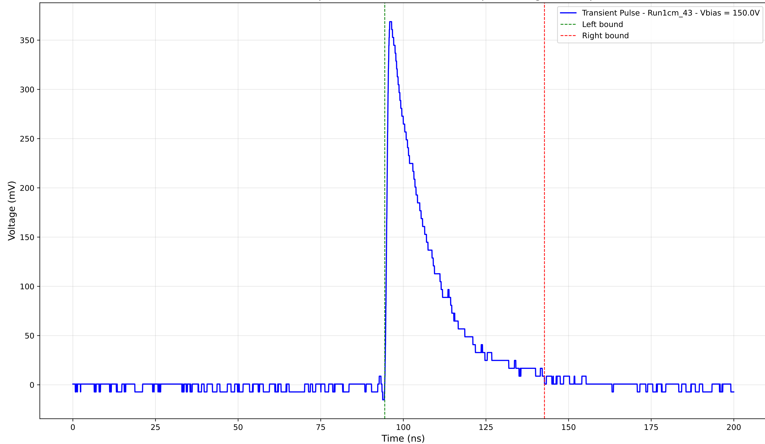
Transient Pulse - Sample: new1cm - Position: 625.0 \mu\text{m} - Charge: 95.12 pC
