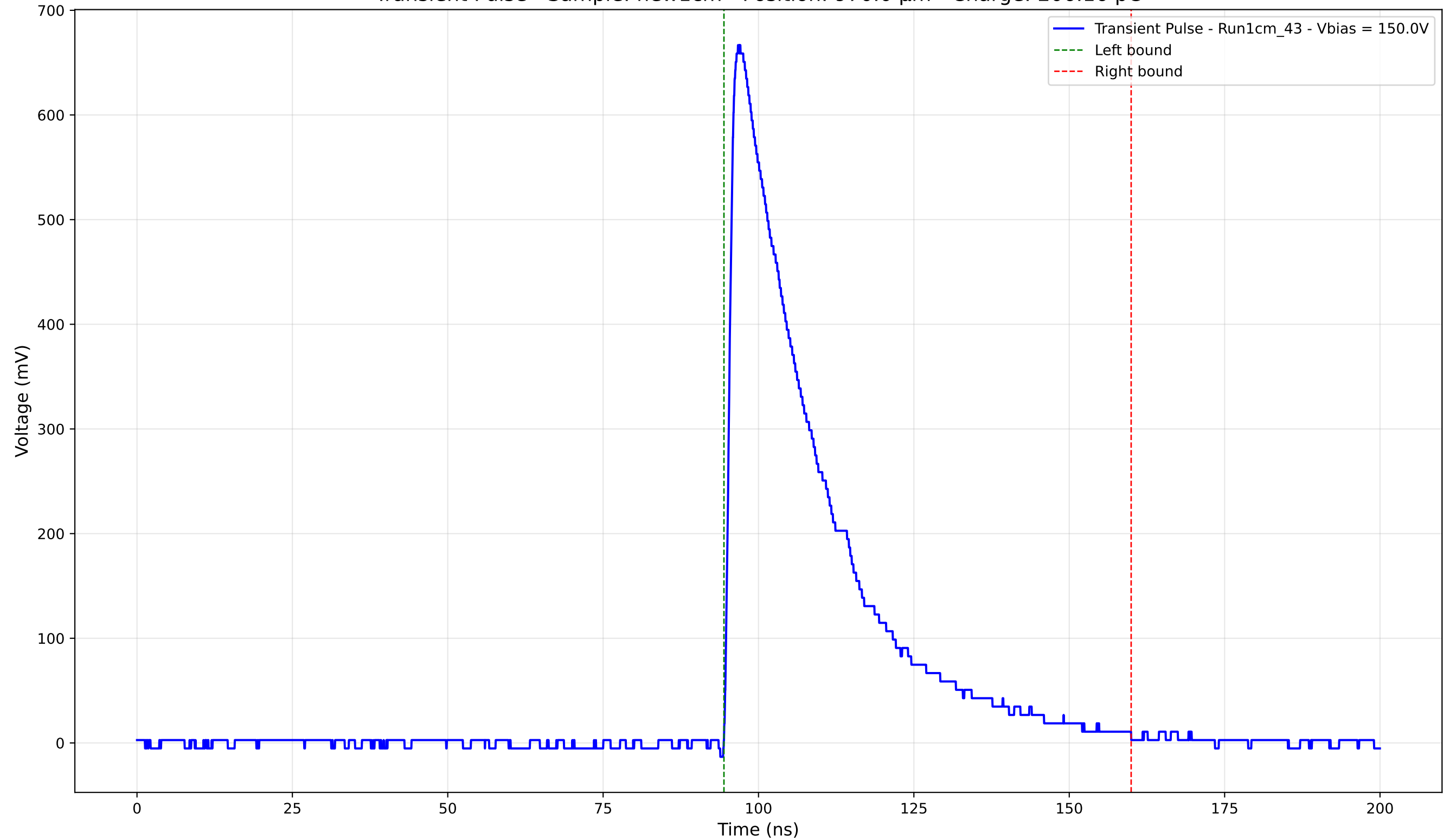
Transient Pulse - Sample: new1cm - Position: 970.0 \mu\text{m} - Charge: 206.16 pC
