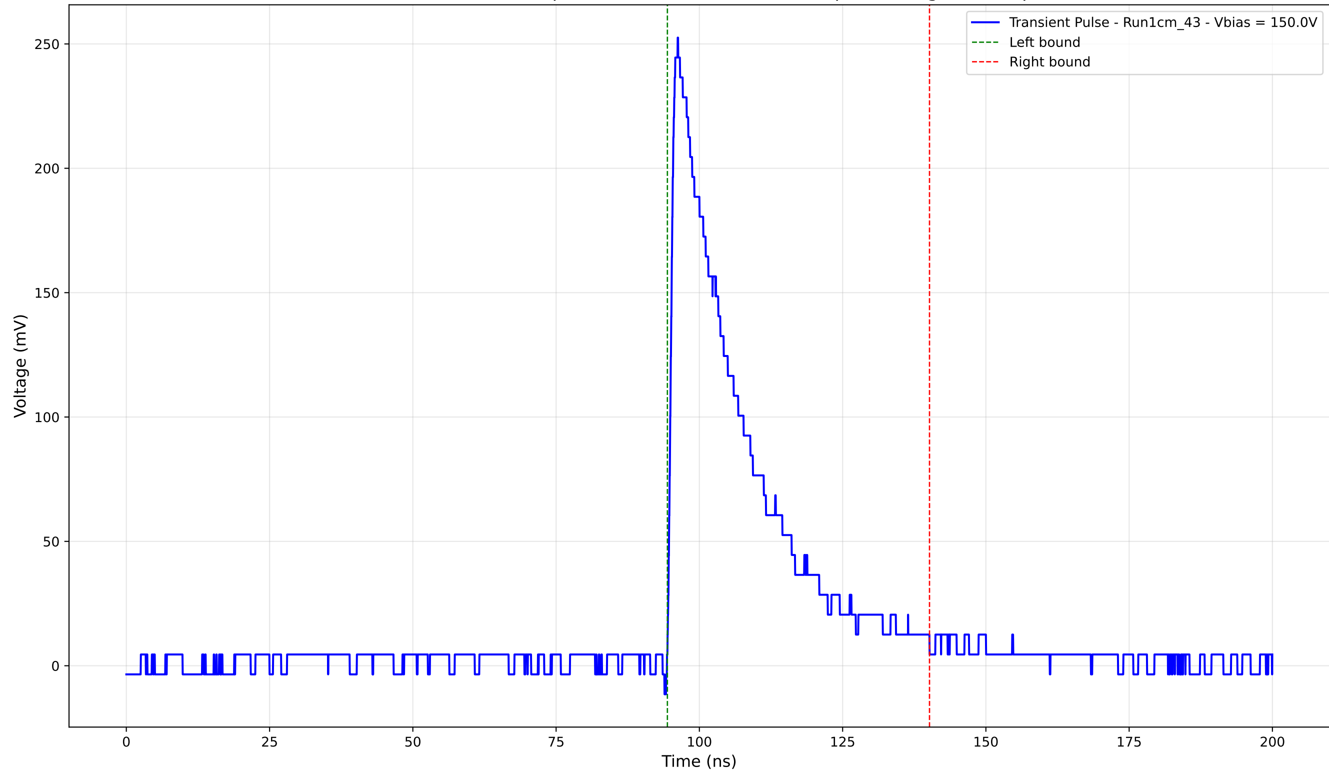
Transient Pulse - Sample: new1cm - Position: 640.0 \mu\text{m} - Charge: 65.52 pC
