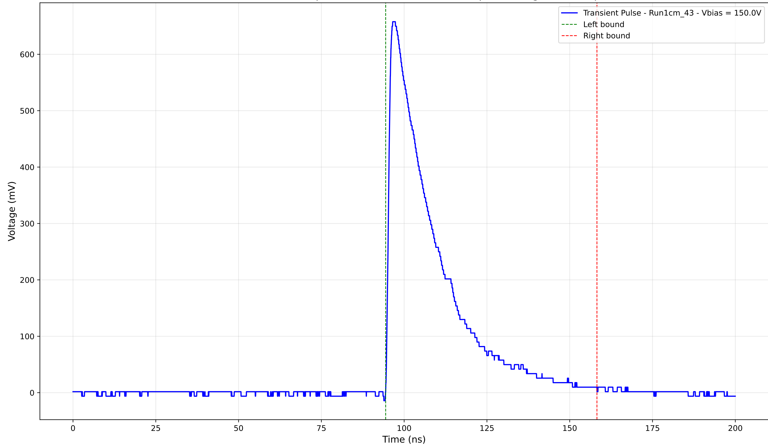
Transient Pulse - Sample: new1cm - Position: 960.0 \mu\text{m} - Charge: 202.19 pC
