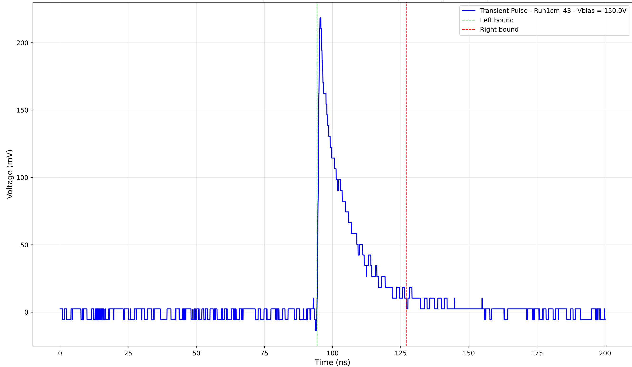
Transient Pulse - Sample: new1cm - Position: 200.0 \mu\text{m} - Charge: 40.93 pC
