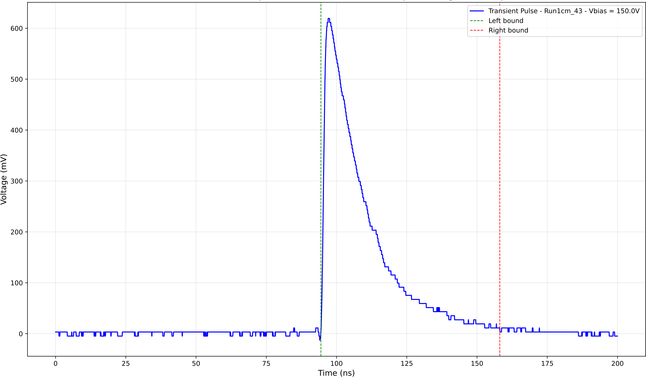
Transient Pulse - Sample: new1cm - Position: 1300.0 \mu\text{m} - Charge: 201.54 pC
