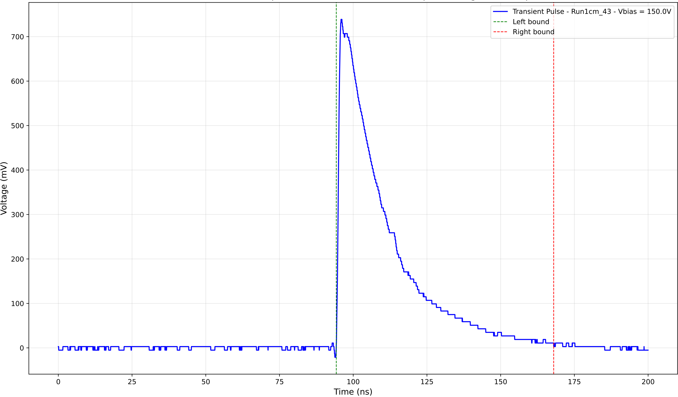
Transient Pulse - Sample: new1cm - Position: 3420.0 \mu\text{m} - Charge: 258.52 pC
