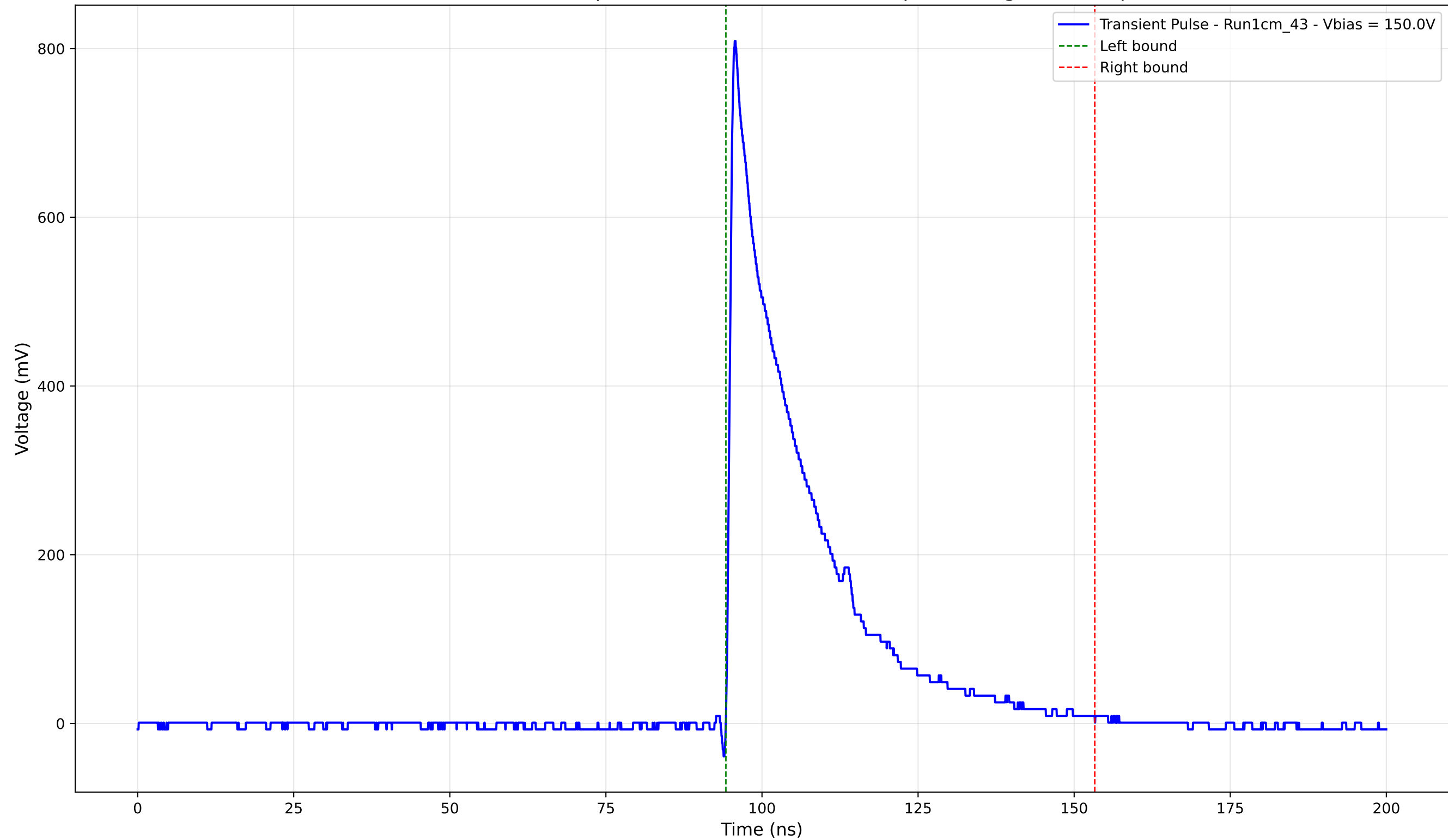
Transient Pulse - Sample: new1cm - Position: 350.0 \mu\text{m} - Charge: 190.45 pC
