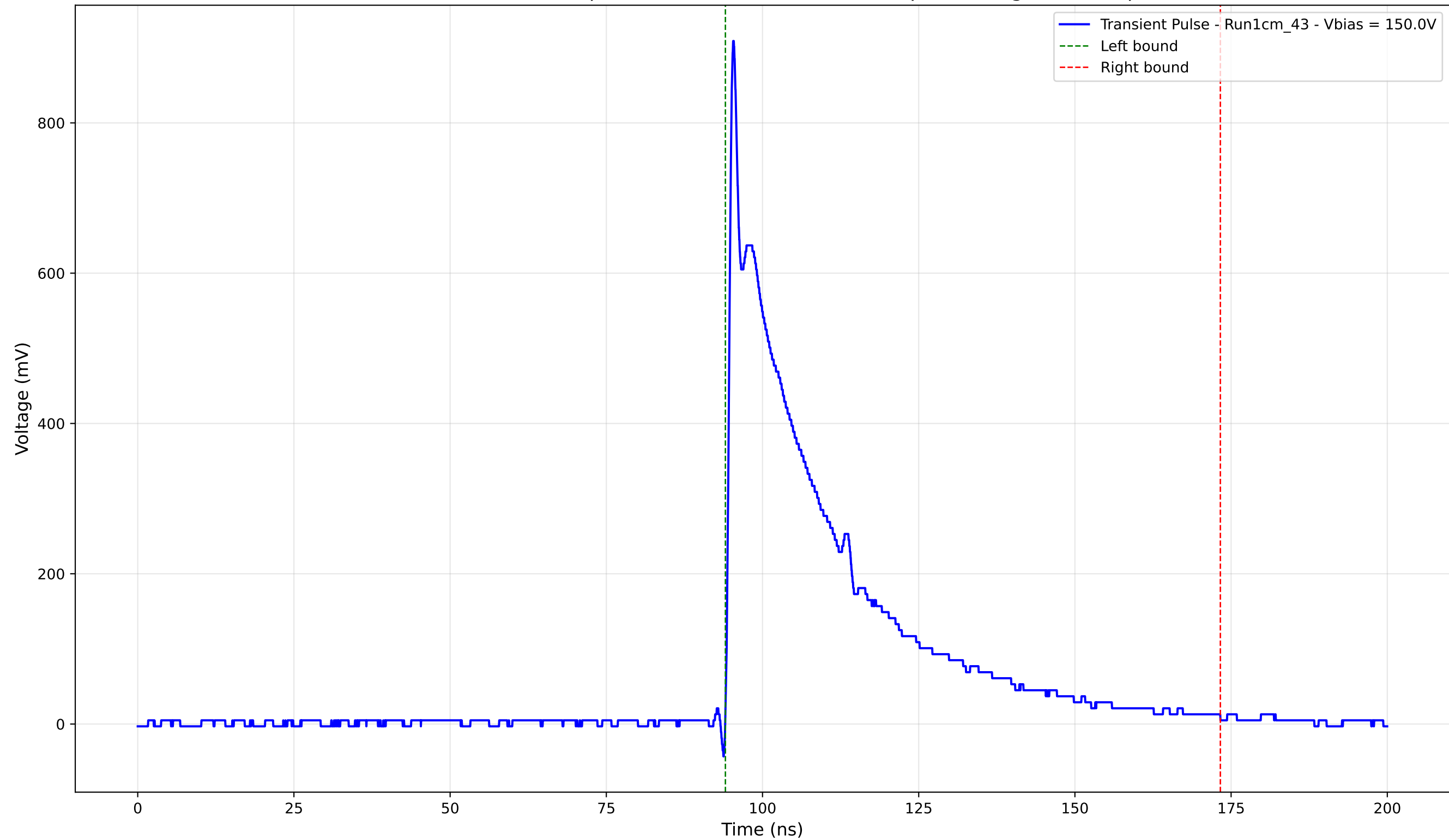
Transient Pulse - Sample: new1cm - Position: 2920.0 \mu\text{m} - Charge: 247.08 pC
