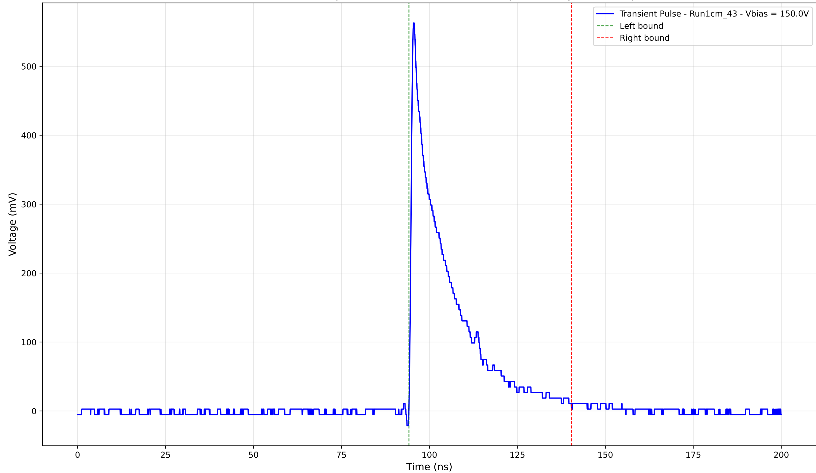
Transient Pulse - Sample: new1cm - Position: 240.0 \mu\text{m} - Charge: 115.30 pC
