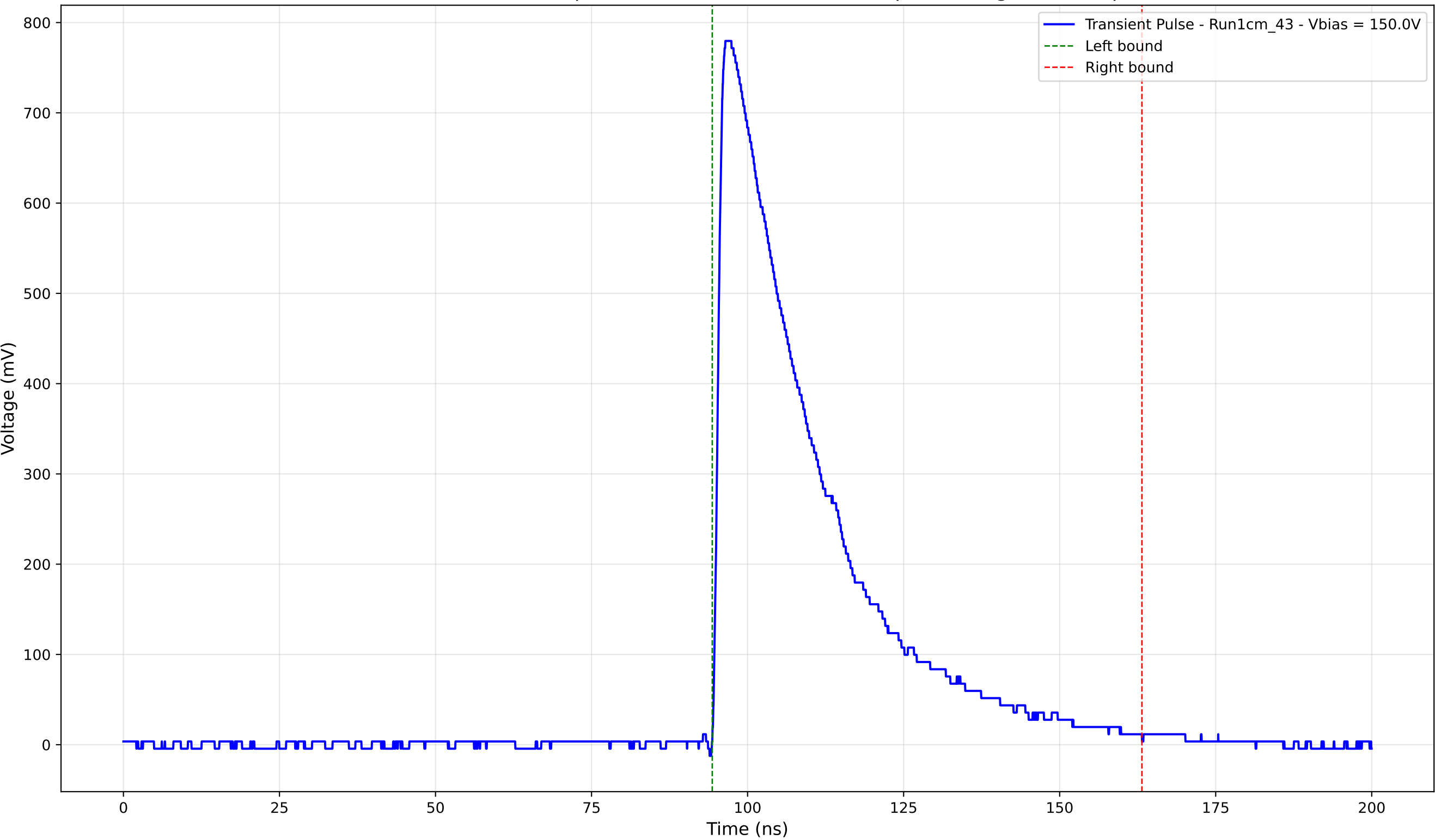
Transient Pulse - Sample: new1cm - Position: 3970.0 \mu\text{m} - Charge: 267.48 pC
