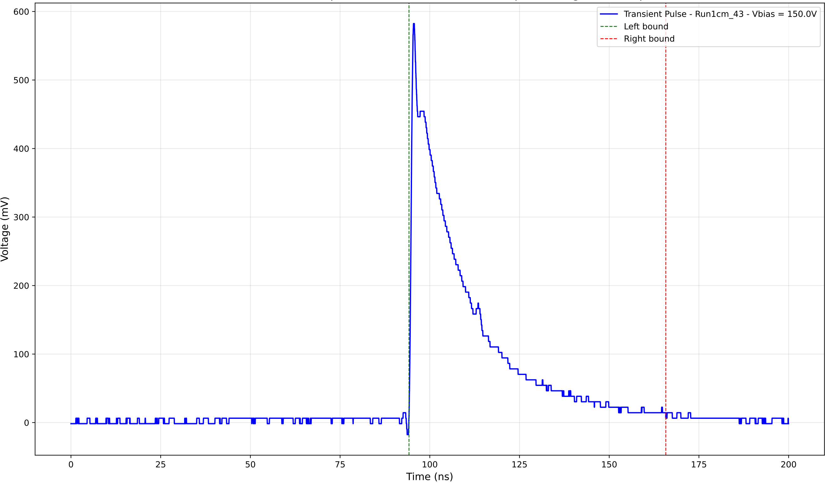
Transient Pulse - Sample: new1cm - Position: 3145.0 \mu\text{m} - Charge: 170.07 pC
