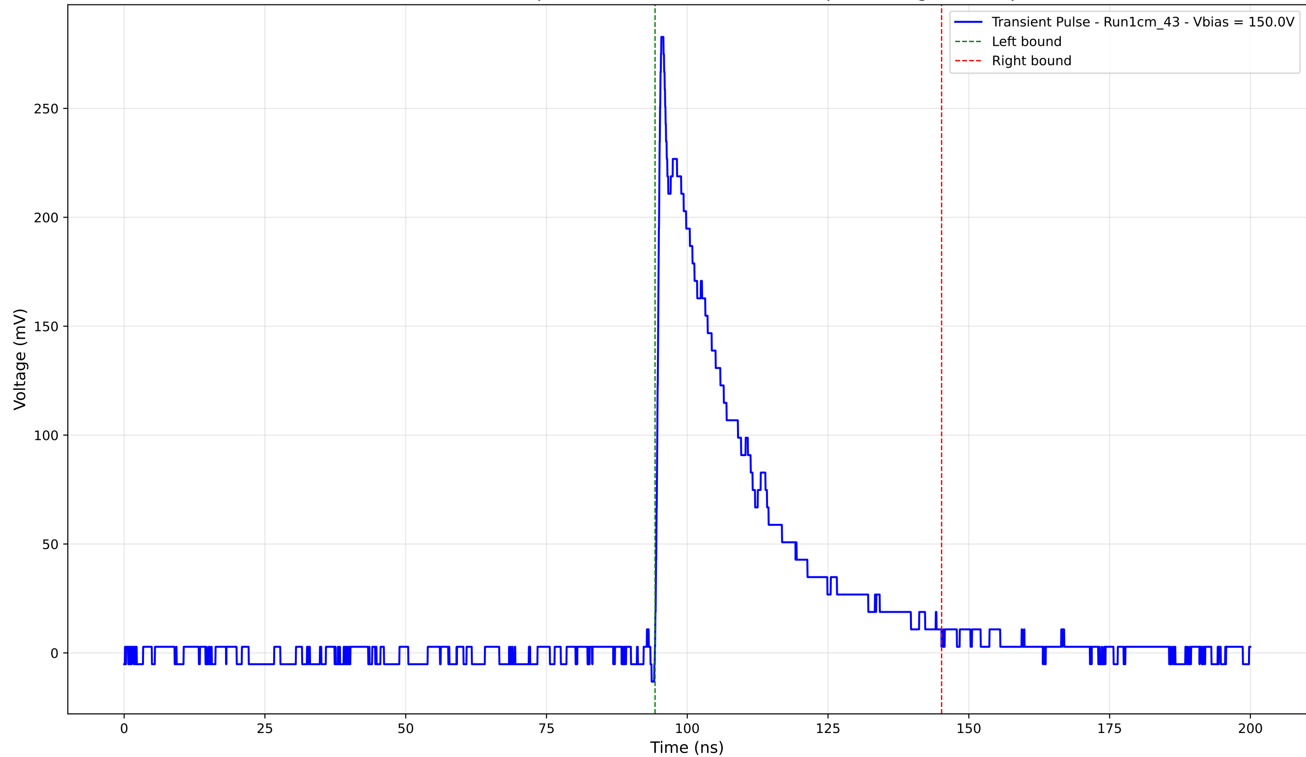
Transient Pulse - Sample: new1cm - Position: 3175.0 \mu\text{m} - Charge: 76.76 pC
