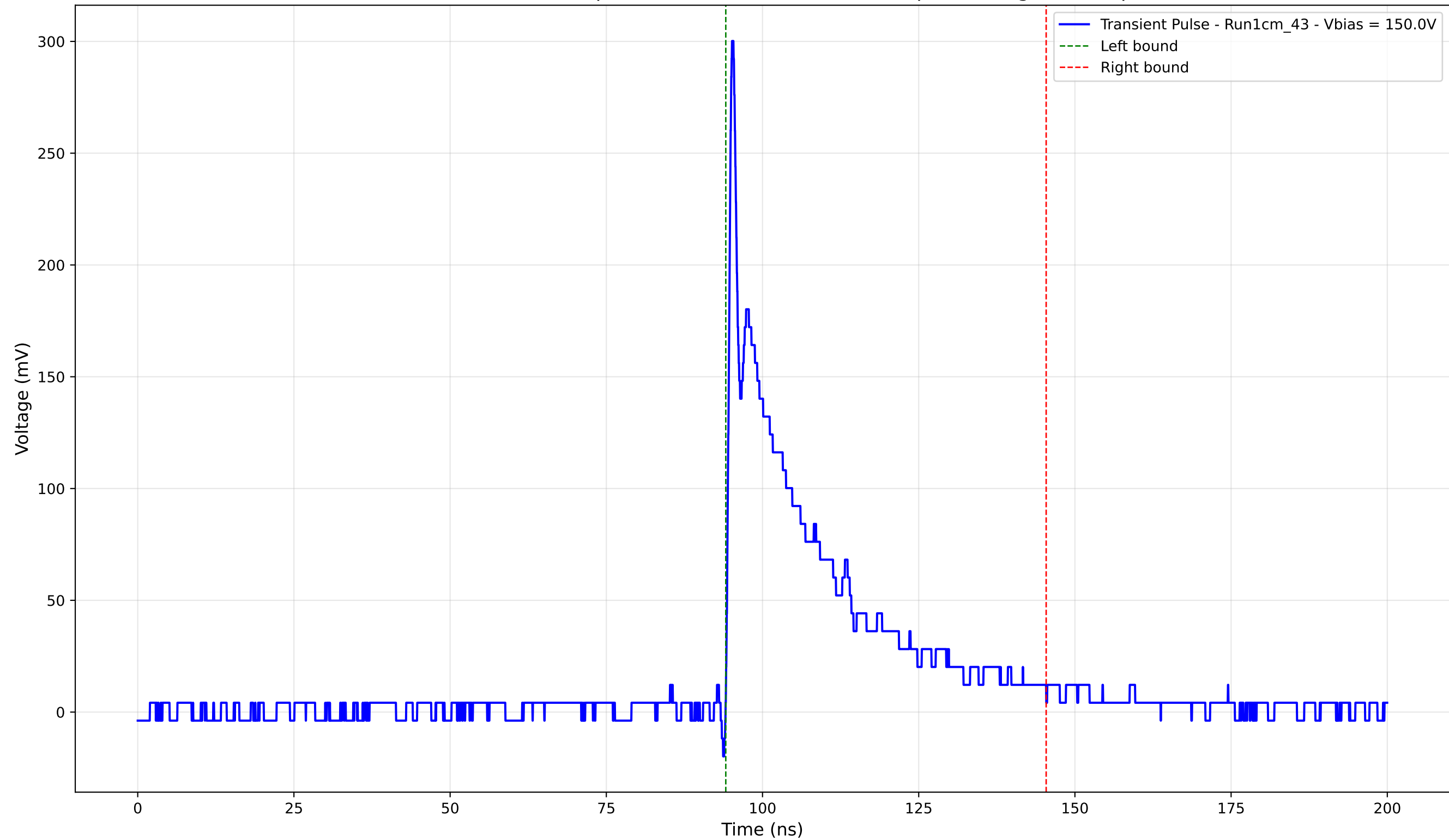
Transient Pulse - Sample: new1cm - Position: 2725.0 \mu\text{m} - Charge: 60.20 pC
