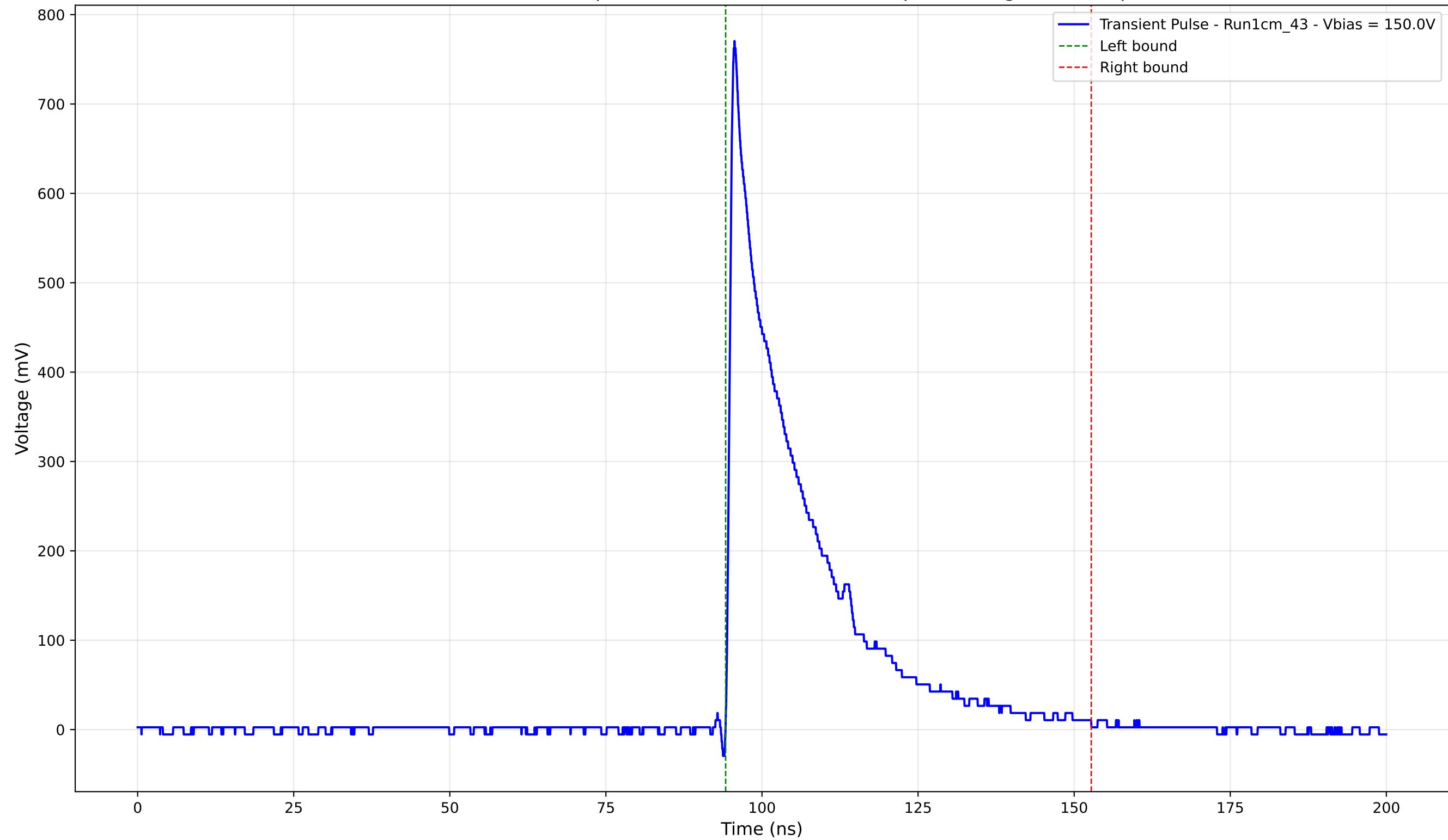
Transient Pulse - Sample: new1cm - Position: 285.0 \mu\text{m} - Charge: 170.62 pC
