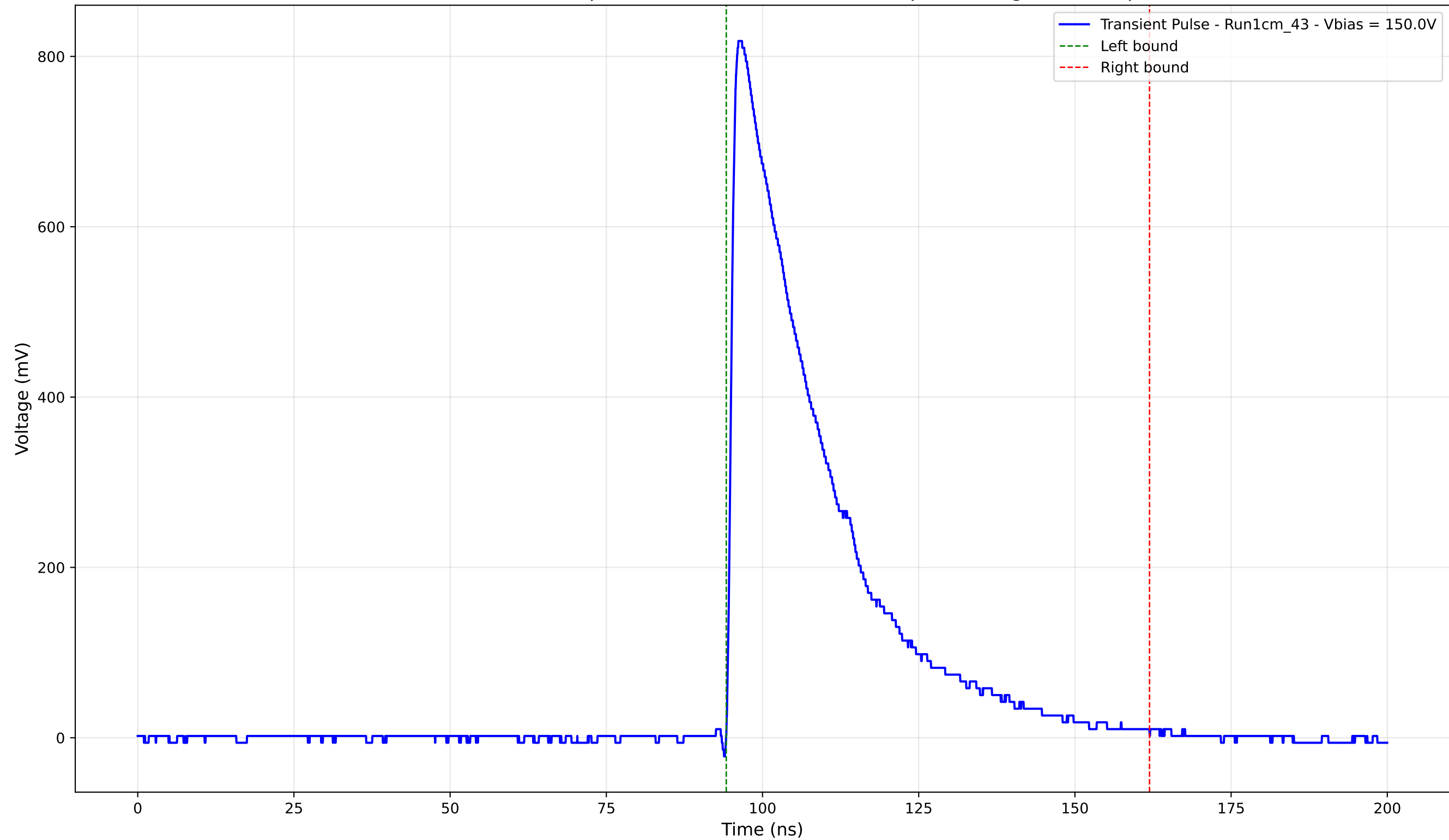
Transient Pulse - Sample: new1cm - Position: 4485.0 \mu\text{m} - Charge: 261.22 pC
