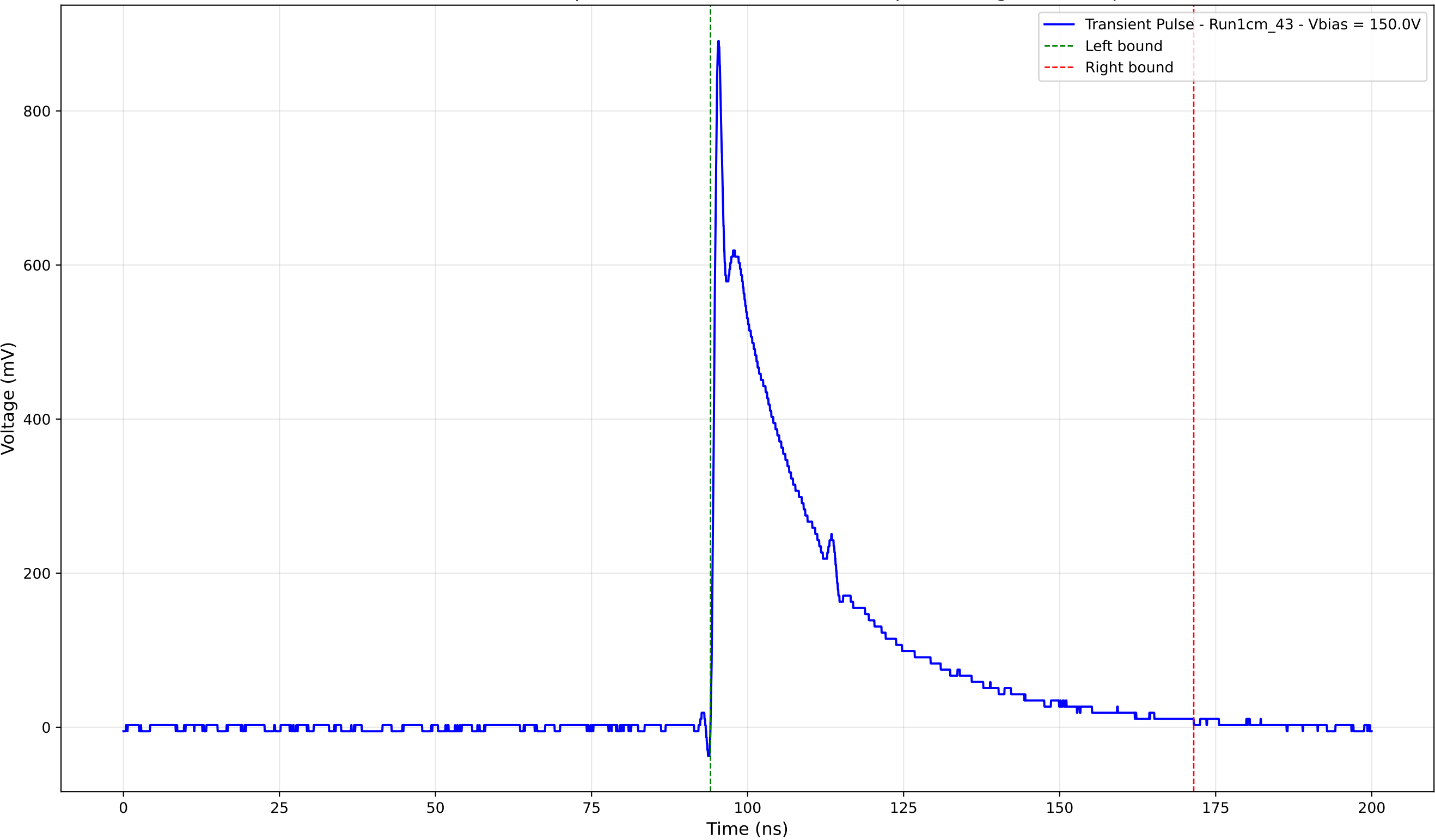
Transient Pulse - Sample: new1cm - Position: 2480.0 \mu\text{m} - Charge: 235.06 pC
