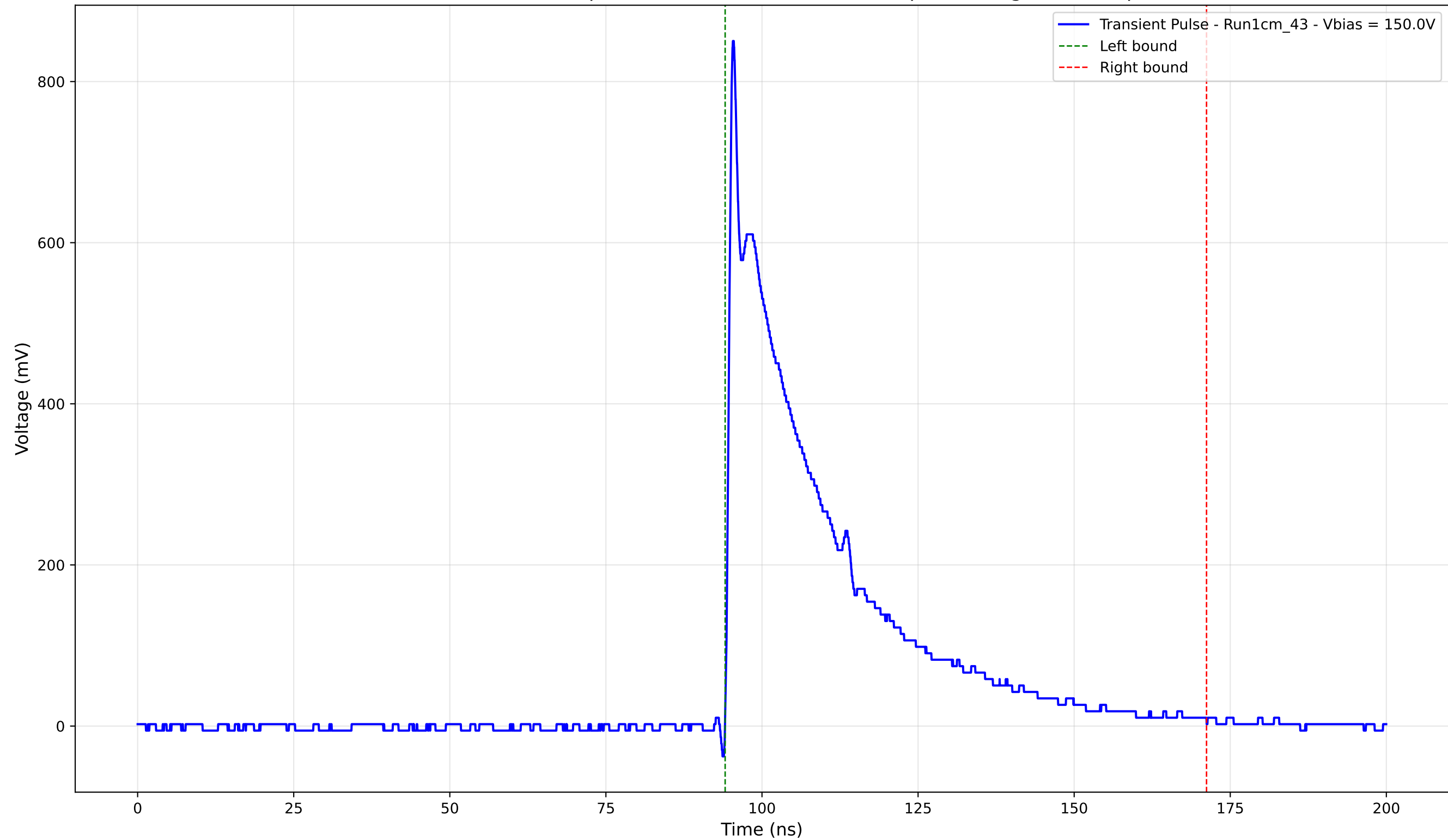
Transient Pulse - Sample: new1cm - Position: 2415.0 \mu\text{m} - Charge: 231.41 pC
