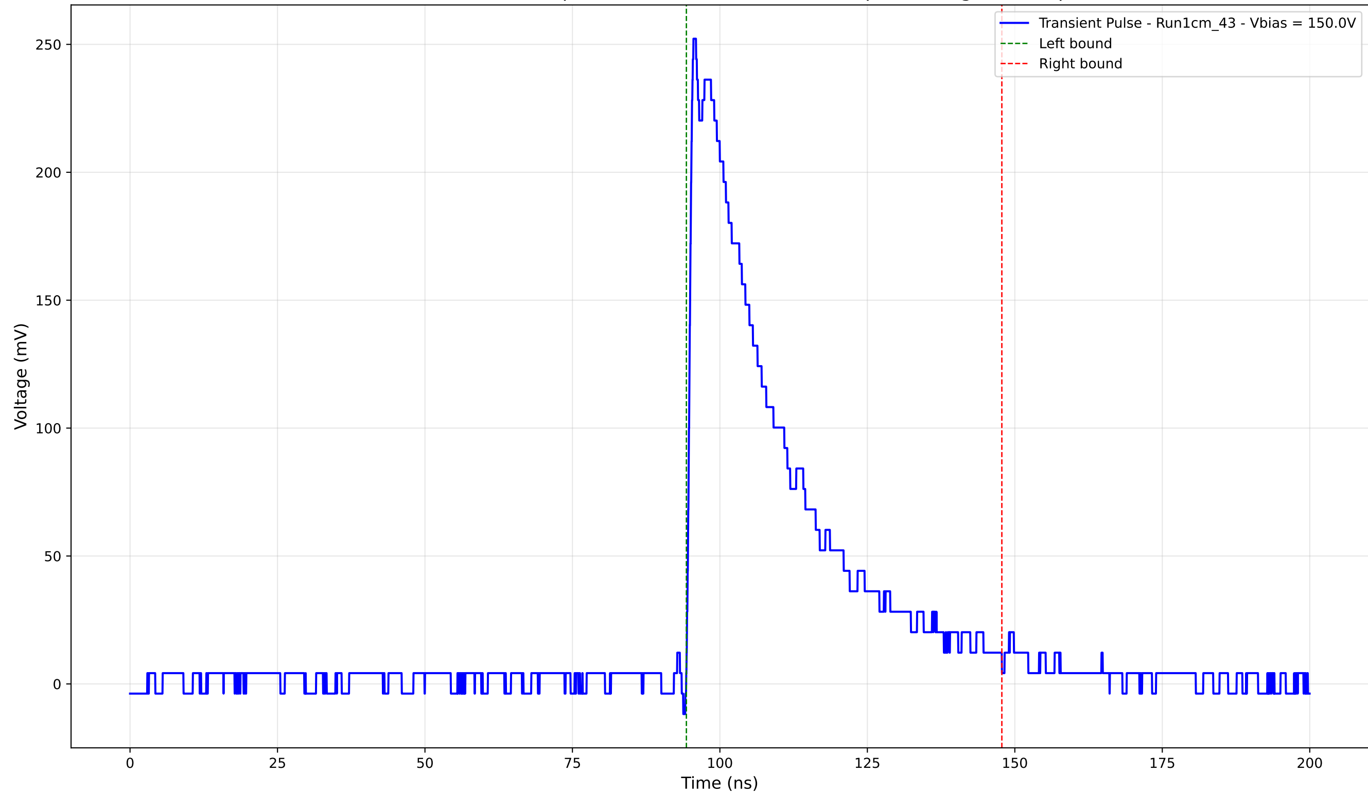
Transient Pulse - Sample: new1cm - Position: 2145.0 \mu\text{m} - Charge: 81.92 pC
