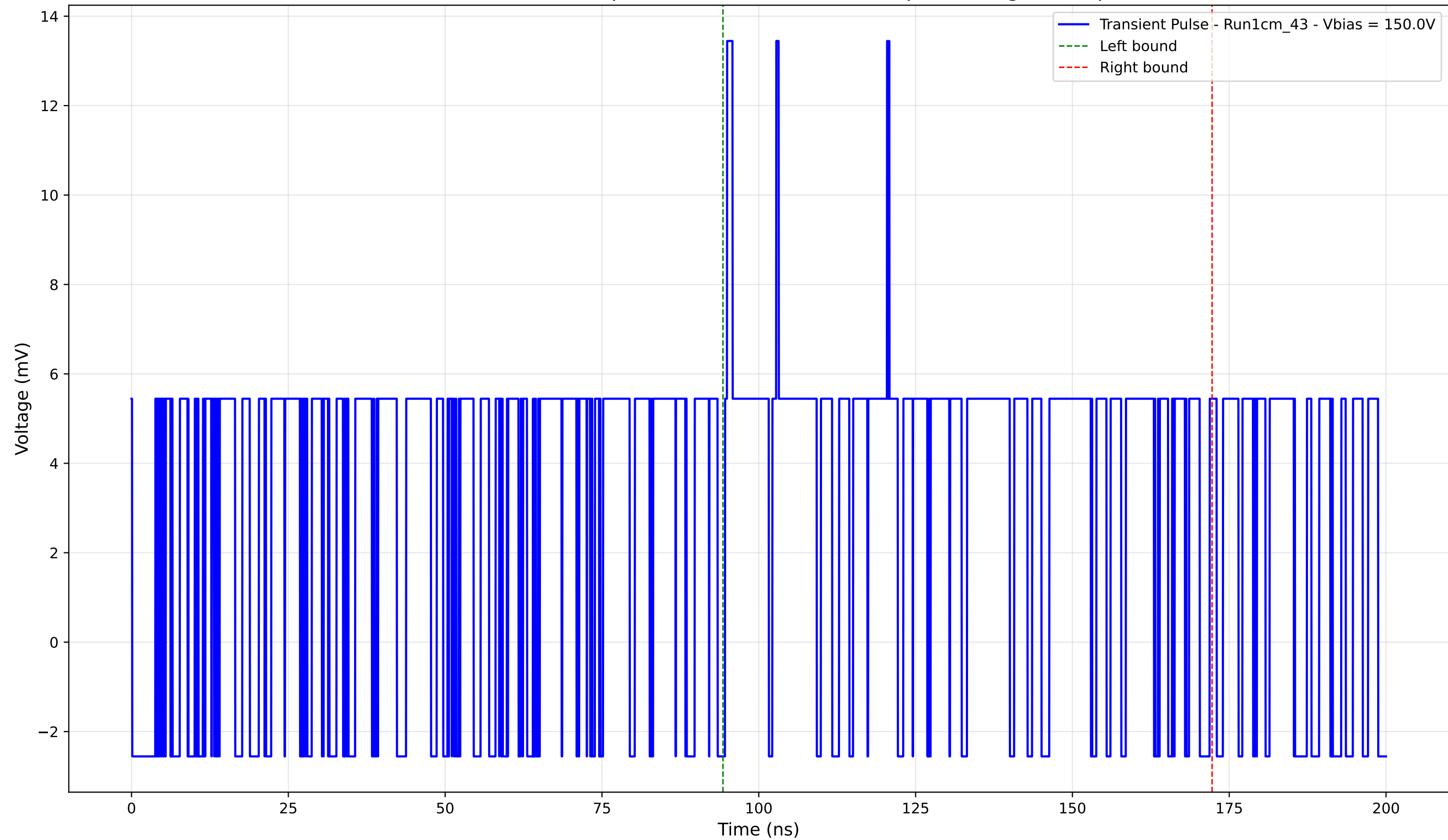
Transient Pulse - Sample: new1cm - Position: 60.0 \mu\text{m} - Charge: 6.46 pC
