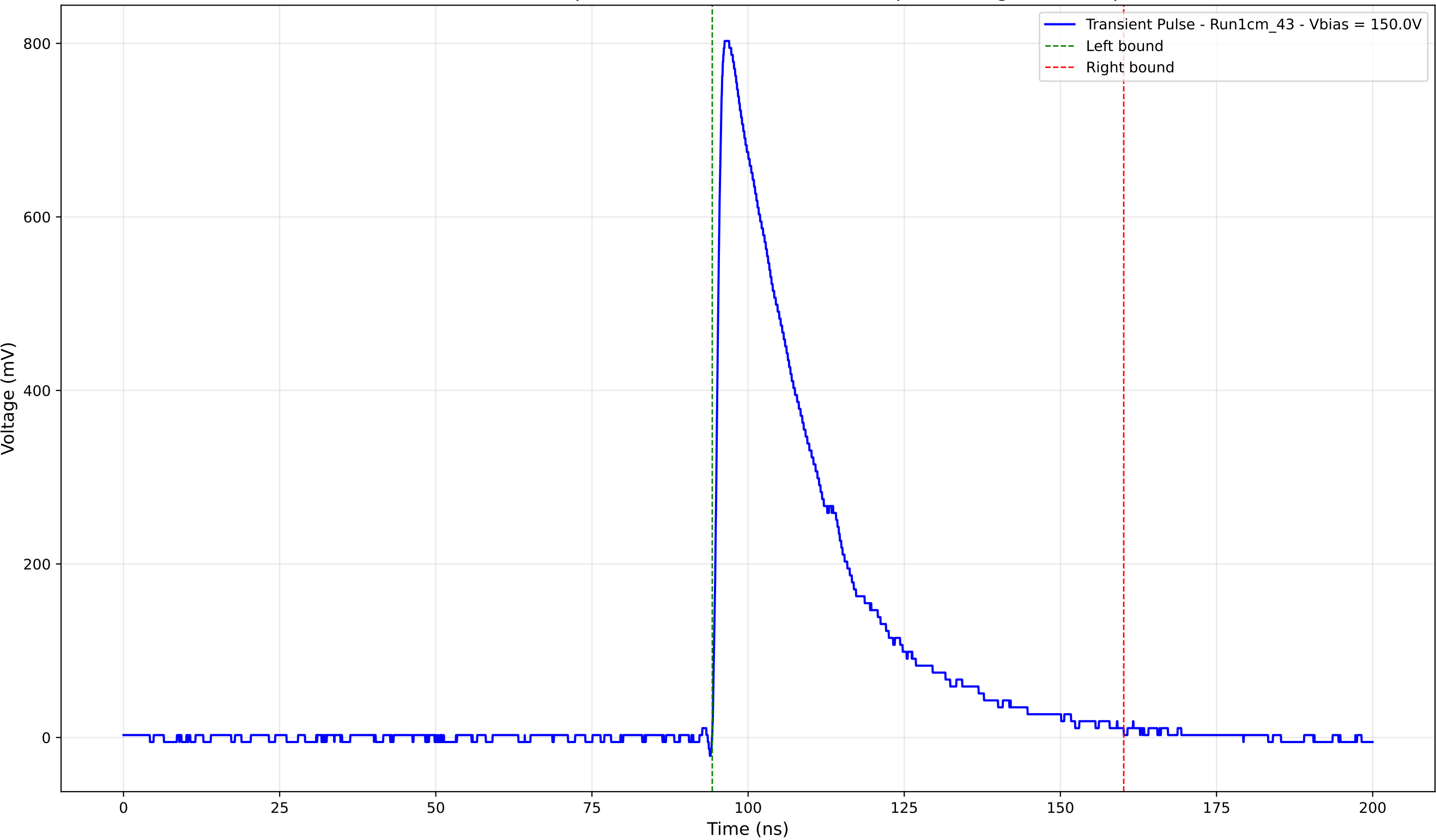
Transient Pulse - Sample: new1cm - Position: 4380.0 \mu\text{m} - Charge: 260.06 pC
