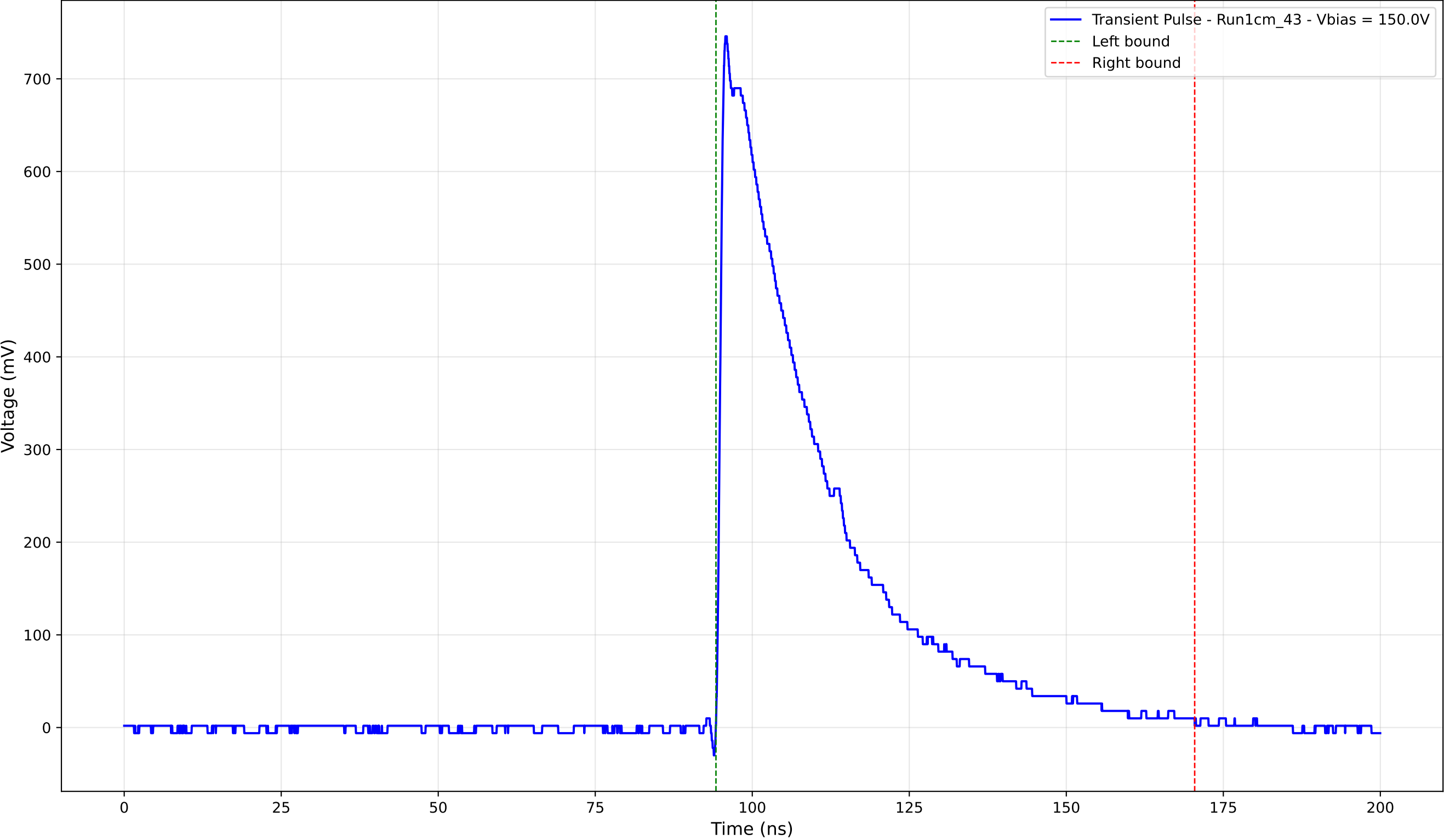
Transient Pulse - Sample: new1cm - Position: 3330.0 \mu\text{m} - Charge: 254.79 pC
