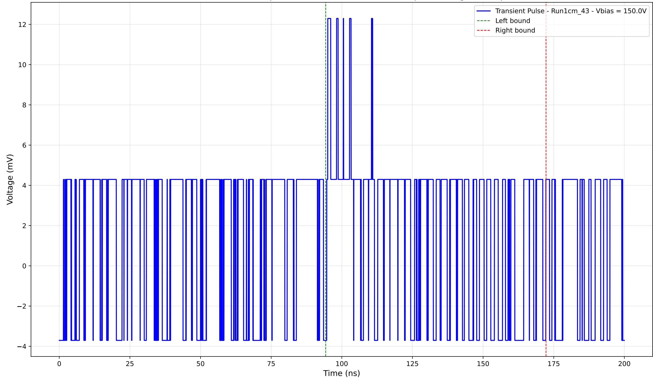
Transient Pulse - Sample: new1cm - Position: 5120.0 \mu\text{m} - Charge: 3.58 pC
