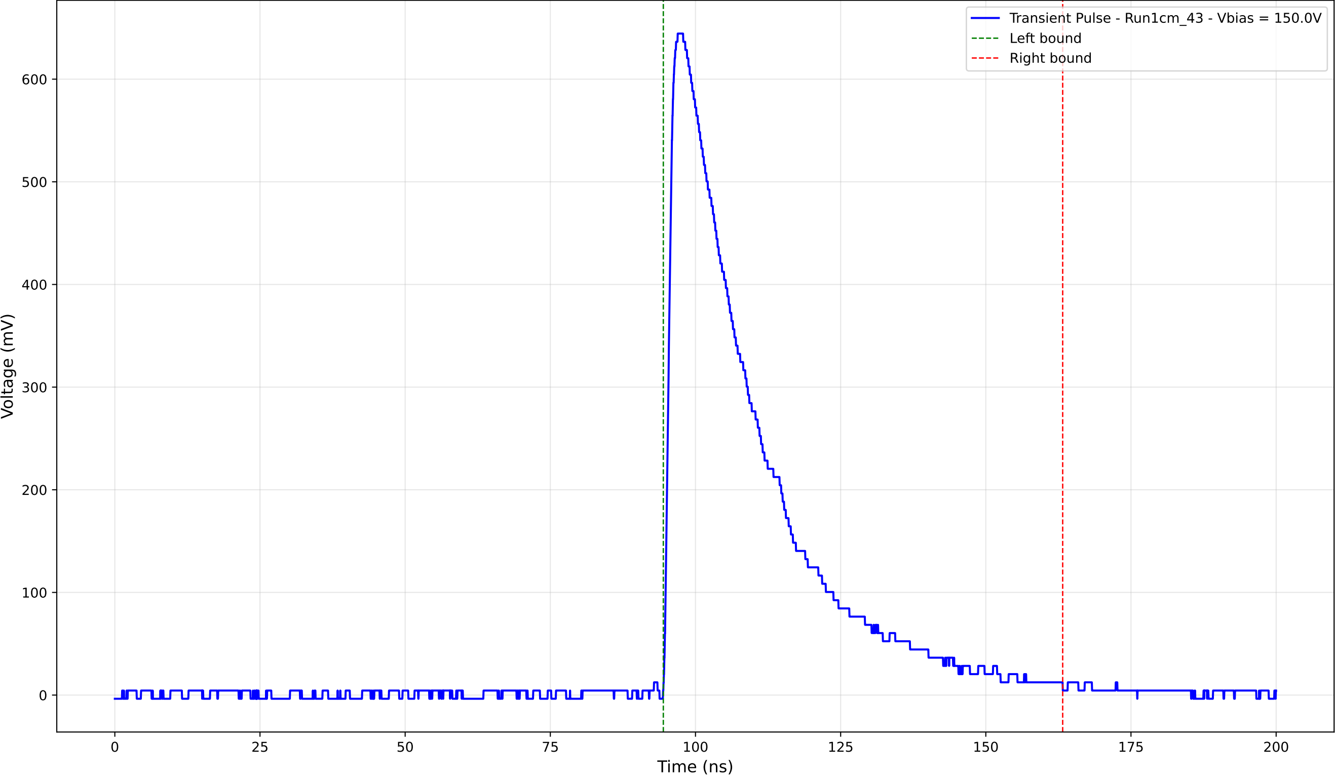
Transient Pulse - Sample: new1cm - Position: 1390.0 \mu\text{m} - Charge: 216.80 pC
