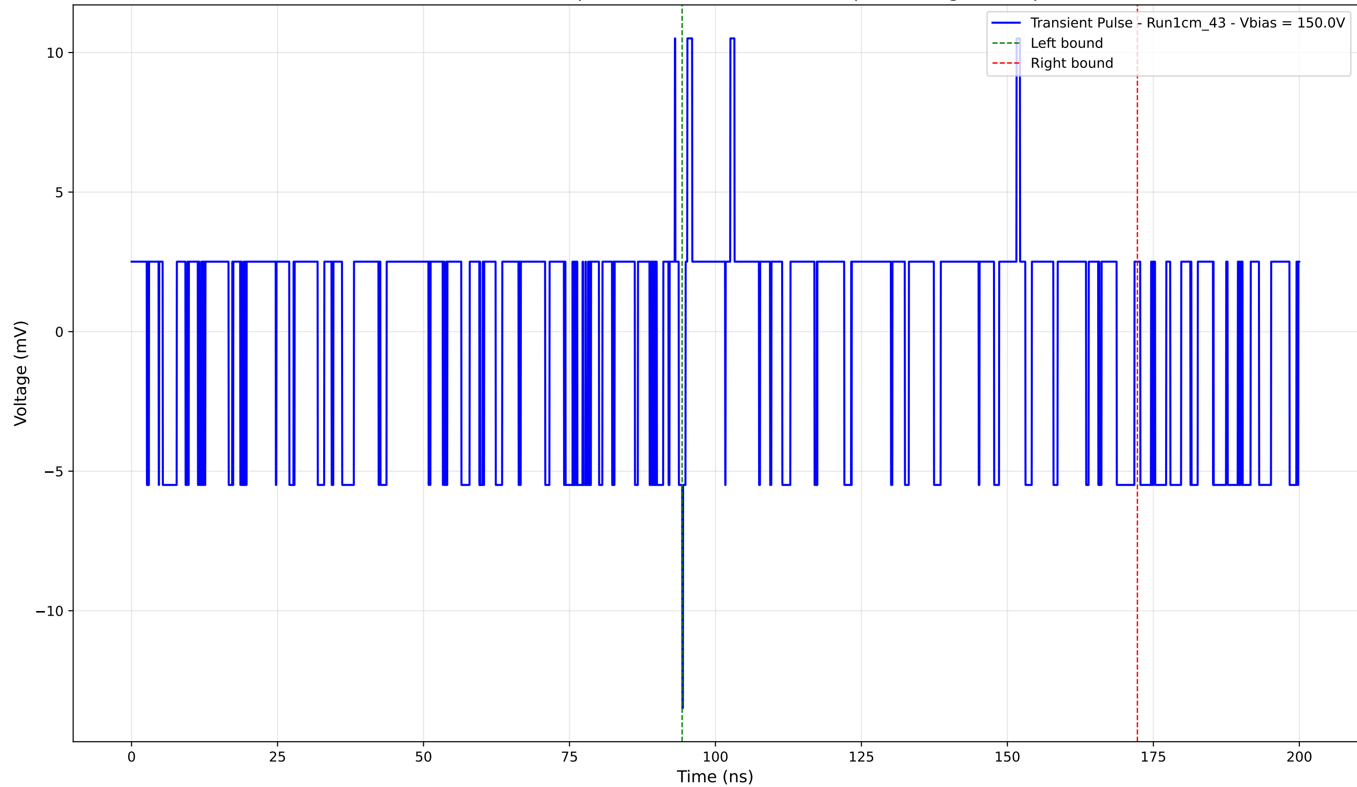
Transient Pulse - Sample: new1cm - Position: 35.0 \mu\text{m} - Charge: 2.17 pC
