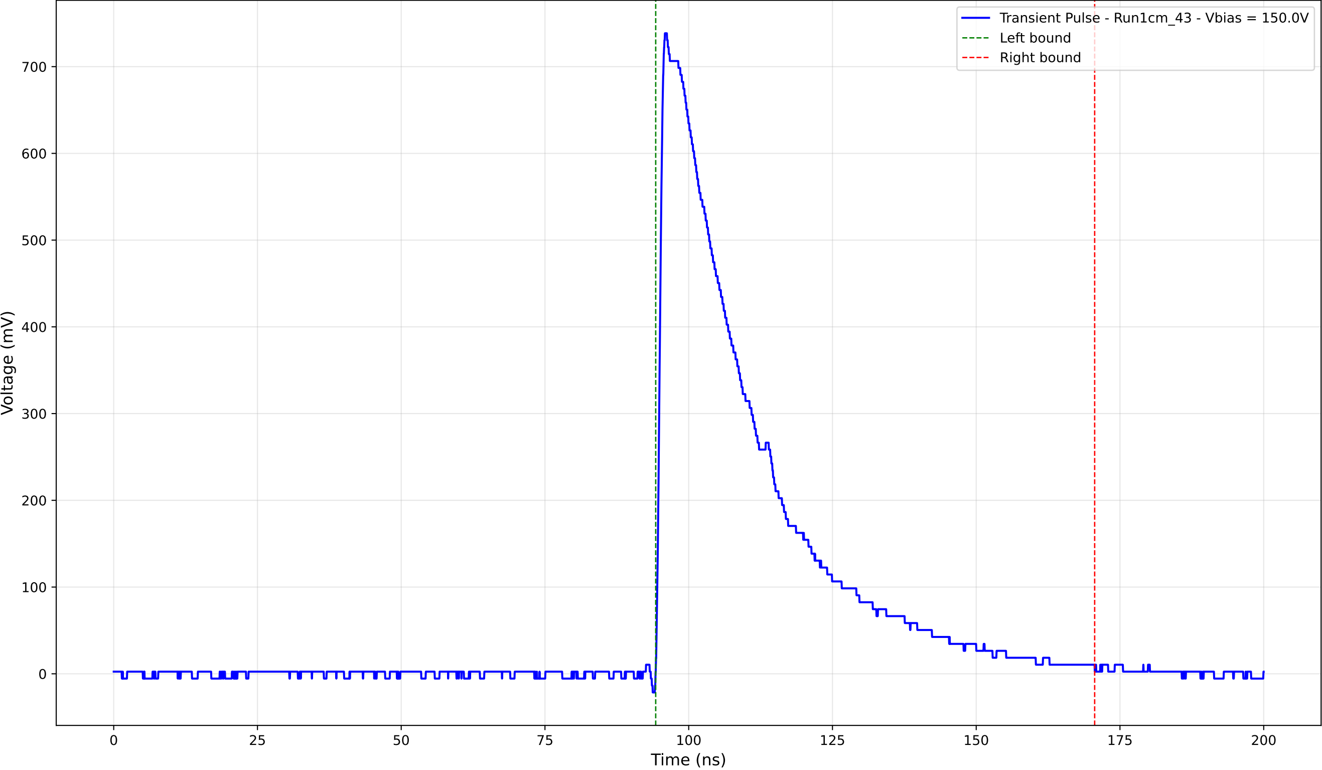
Transient Pulse - Sample: new1cm - Position: 3425.0 \mu\text{m} - Charge: 260.04 pC
