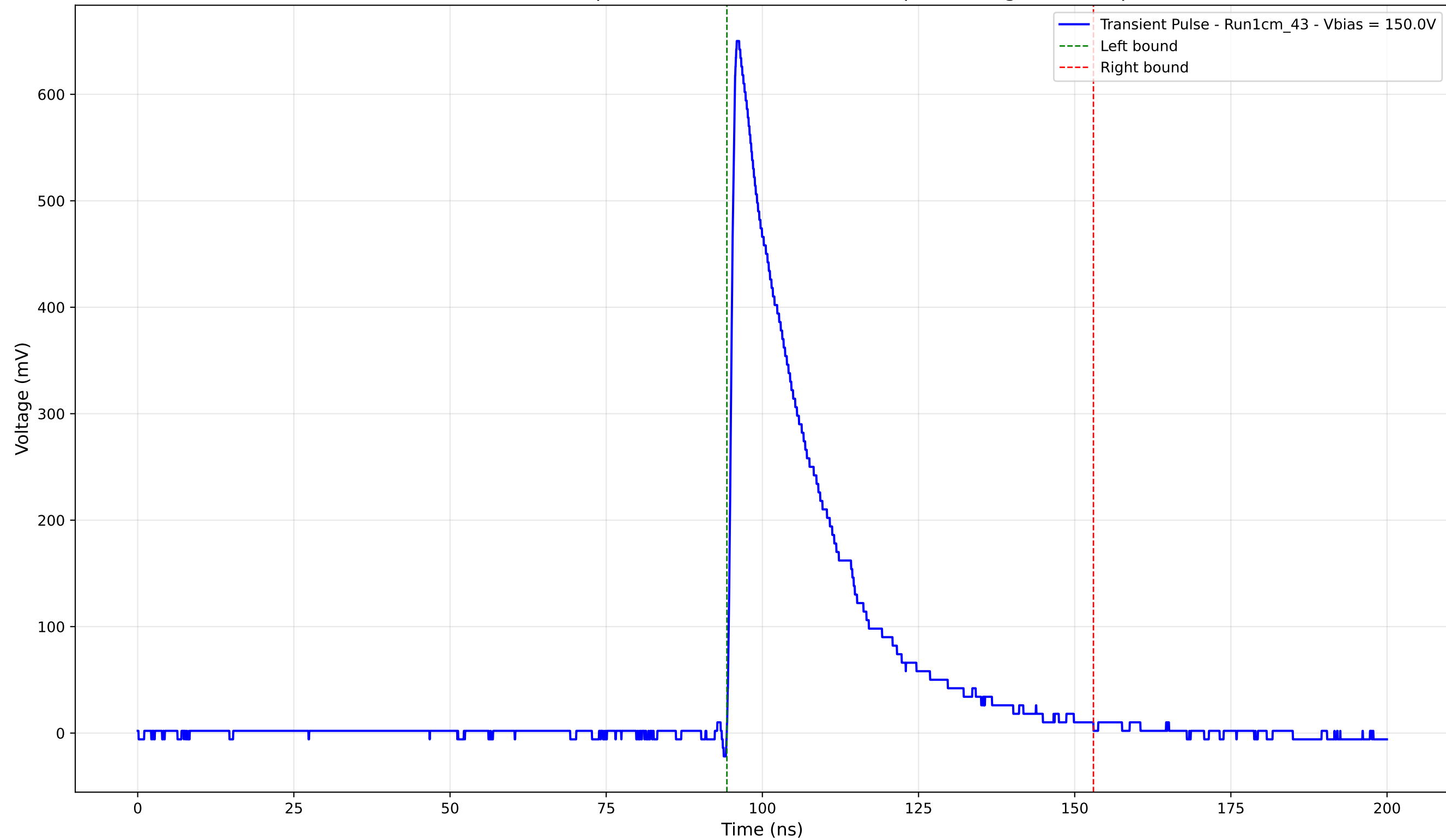
Transient Pulse - Sample: new1cm - Position: 585.0 \mu\text{m} - Charge: 173.44 pC
