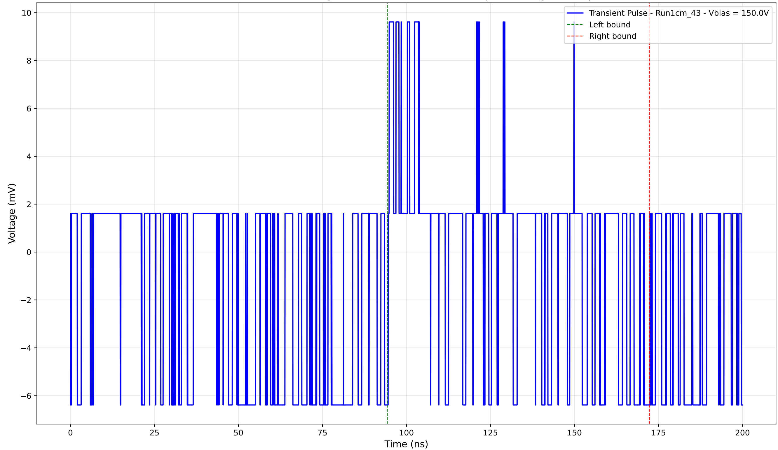
Transient Pulse - Sample: new1cm - Position: 80.0 \mu\text{m} - Charge: 0.50 pC
