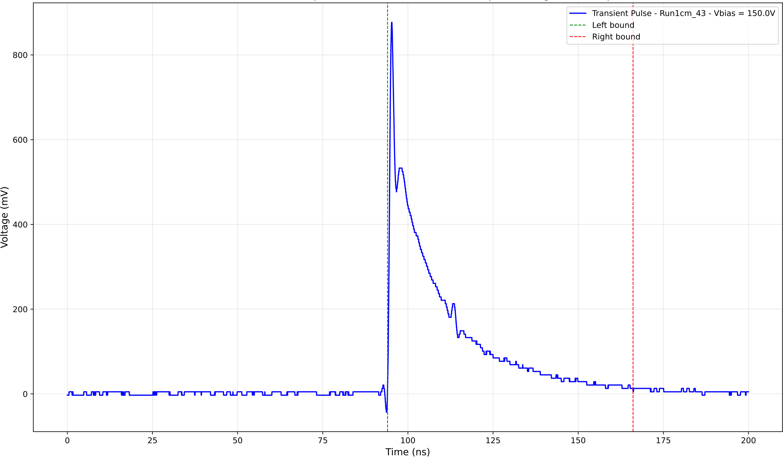
Transient Pulse - Sample: new1cm - Position: 2785.0 \mu\text{m} - Charge: 204.92 pC
