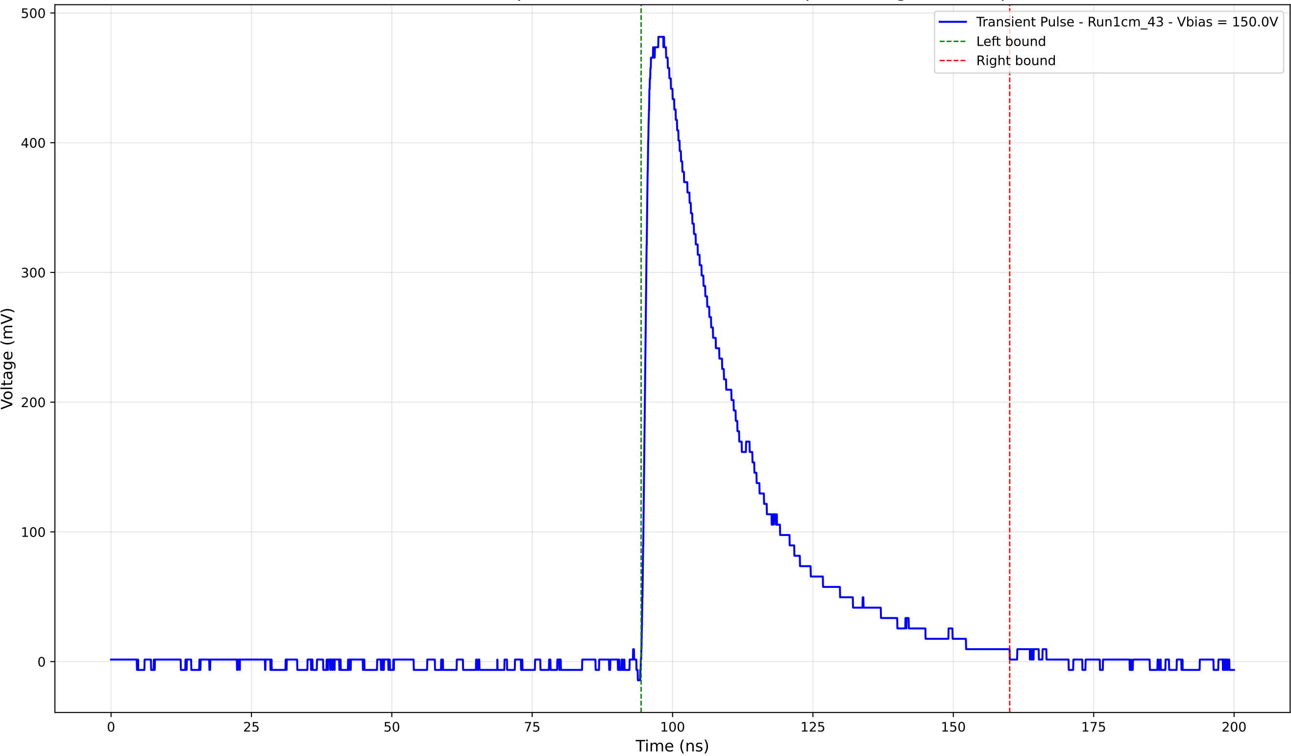
Transient Pulse - Sample: new1cm - Position: 1770.0 \mu\text{m} - Charge: 165.14 pC
