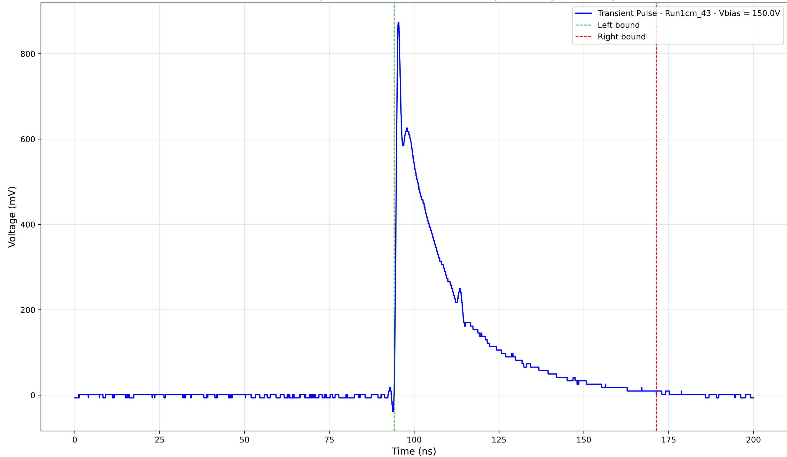
Transient Pulse - Sample: new1cm - Position: 2445.0 \mu\text{m} - Charge: 237.15 pC
