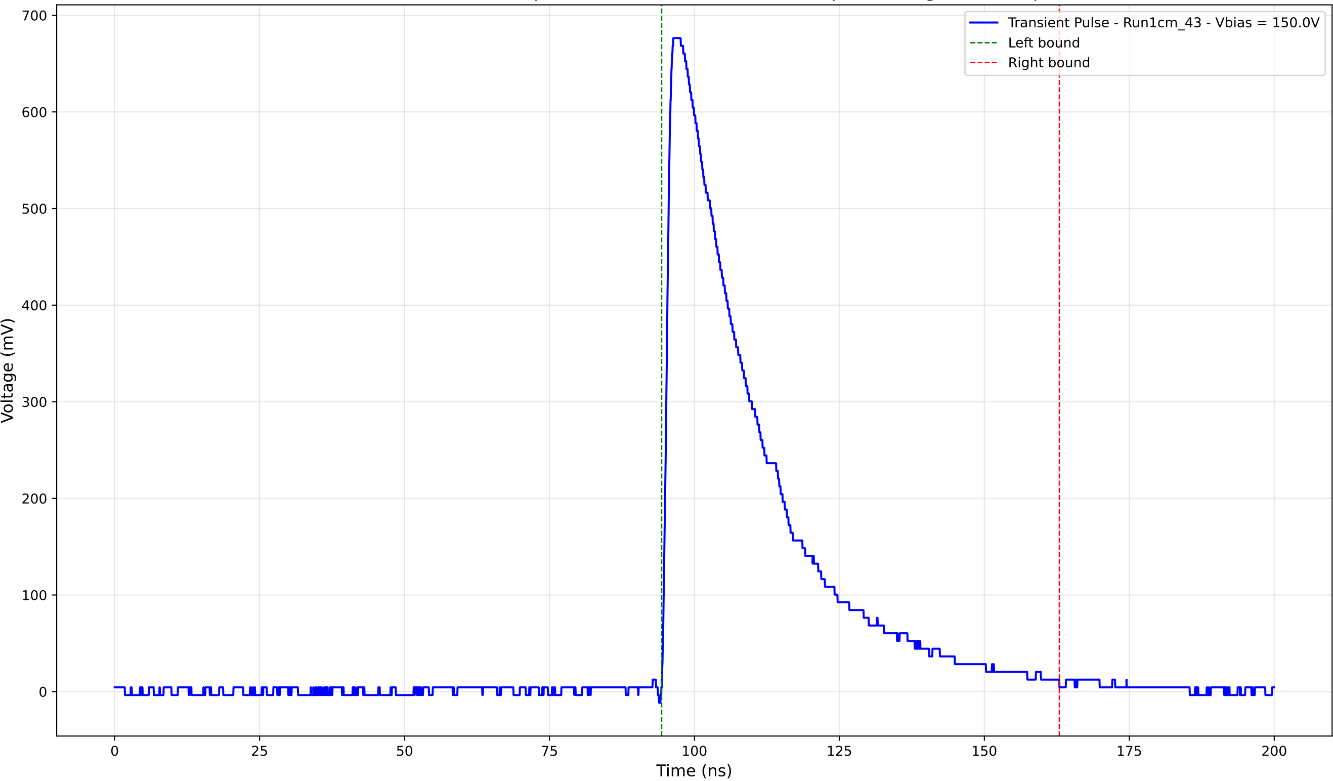
Transient Pulse - Sample: new1cm - Position: 3795.0 \mu\text{m} - Charge: 233.32 pC
