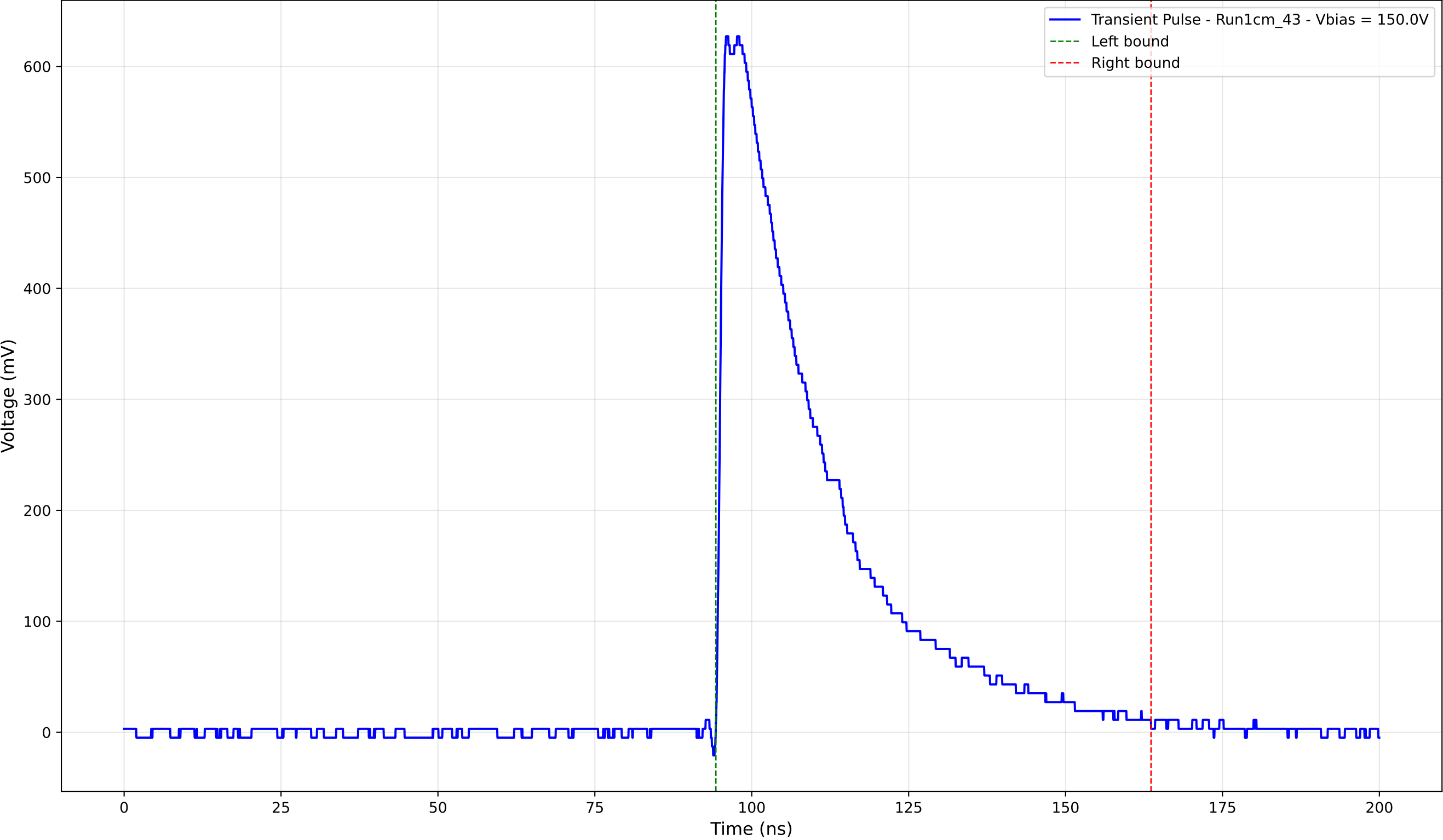
Transient Pulse - Sample: new1cm - Position: 1950.0 \mu\text{m} - Charge: 224.79 pC
