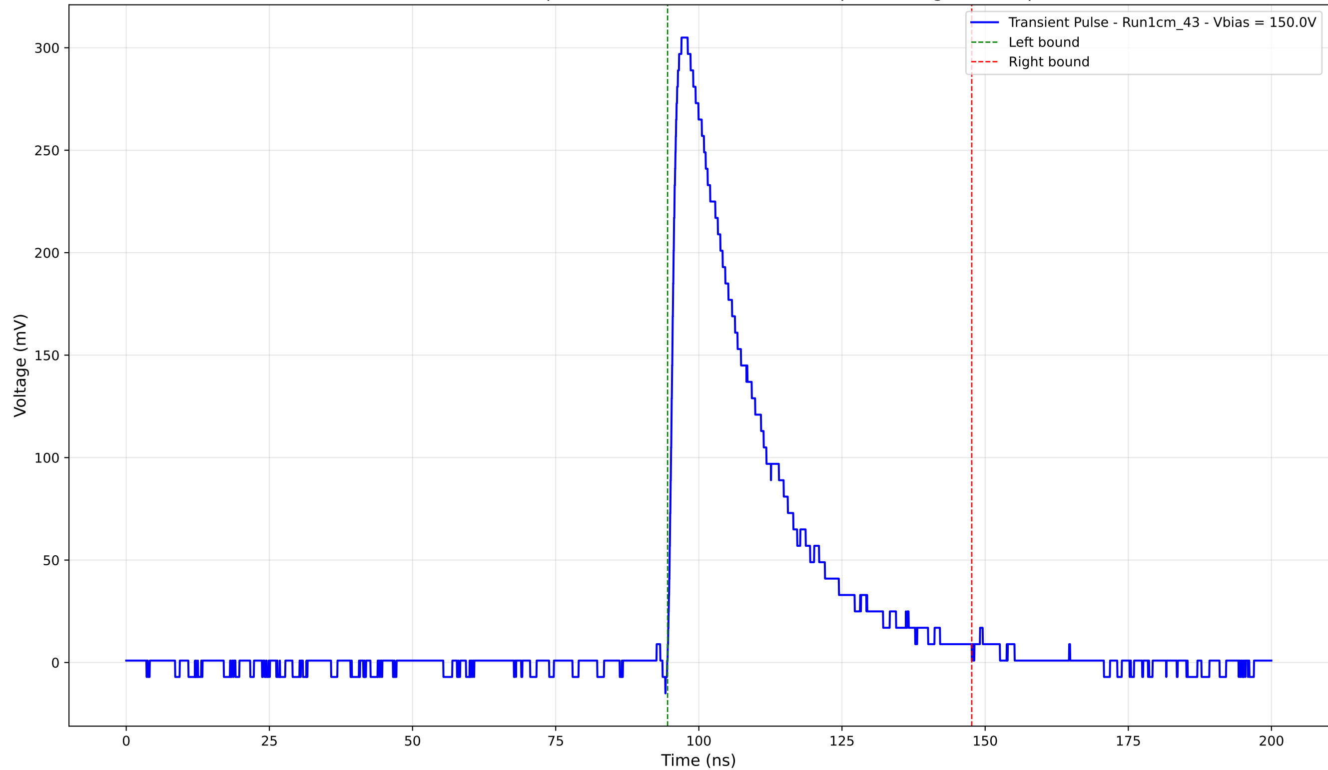
Transient Pulse - Sample: new1cm - Position: 1230.0 \mu\text{m} - Charge: 94.09 pC
