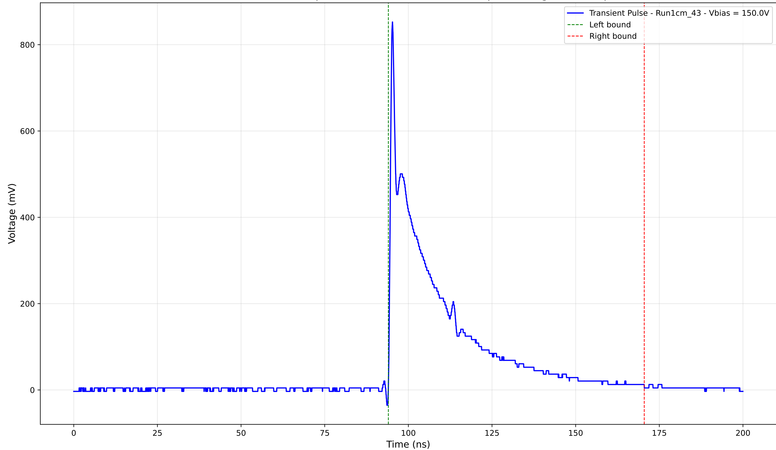
Transient Pulse - Sample: new1cm - Position: 2620.0 \mu\text{m} - Charge: 192.69 pC
