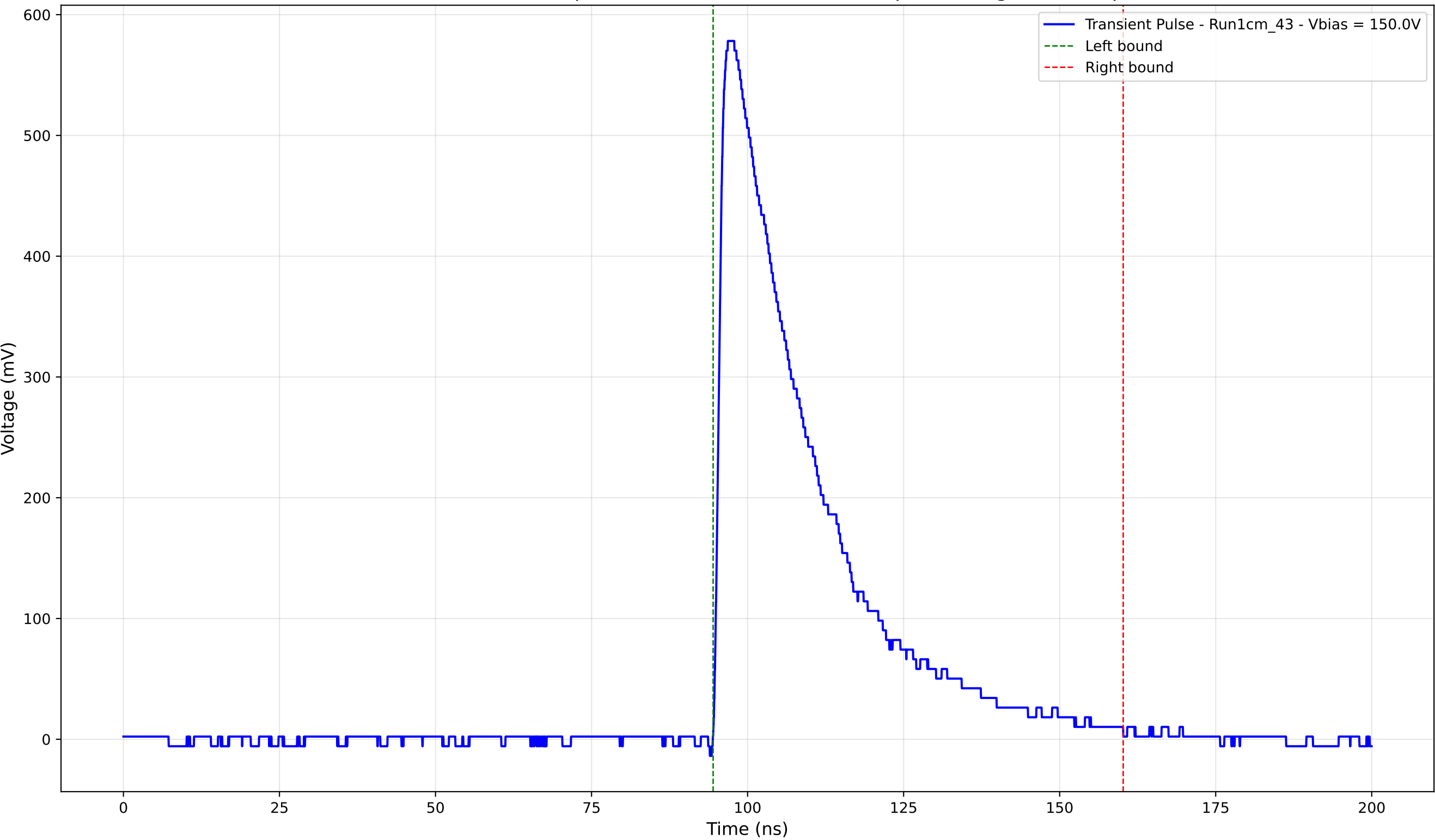
Transient Pulse - Sample: new1cm - Position: 1280.0 \mu\text{m} - Charge: 188.30 pC
