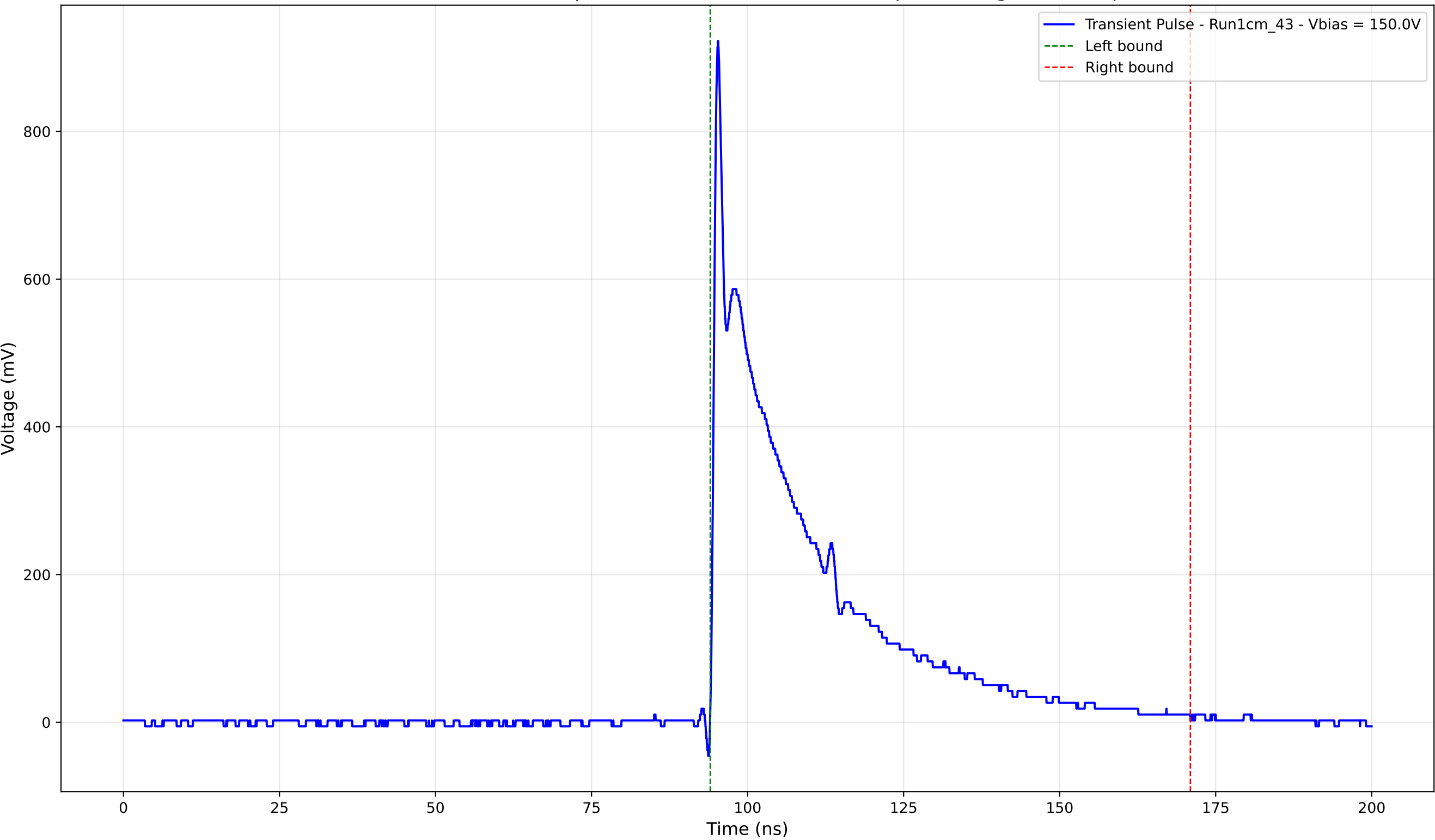
Transient Pulse - Sample: new1cm - Position: 2595.0 \mu\text{m} - Charge: 224.57 pC
