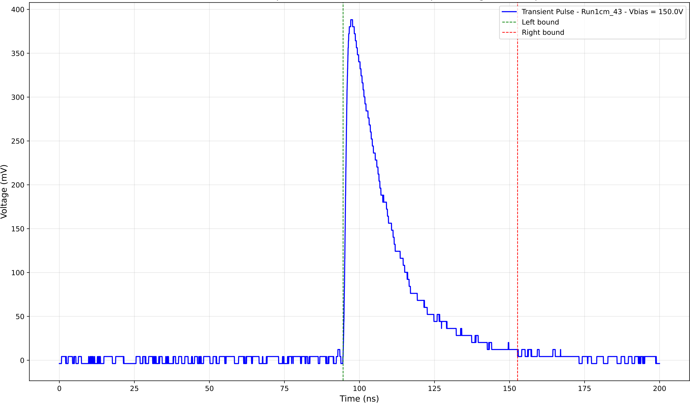
Transient Pulse - Sample: new1cm - Position: 1240.0 \mu\text{m} - Charge: 122.91 pC
