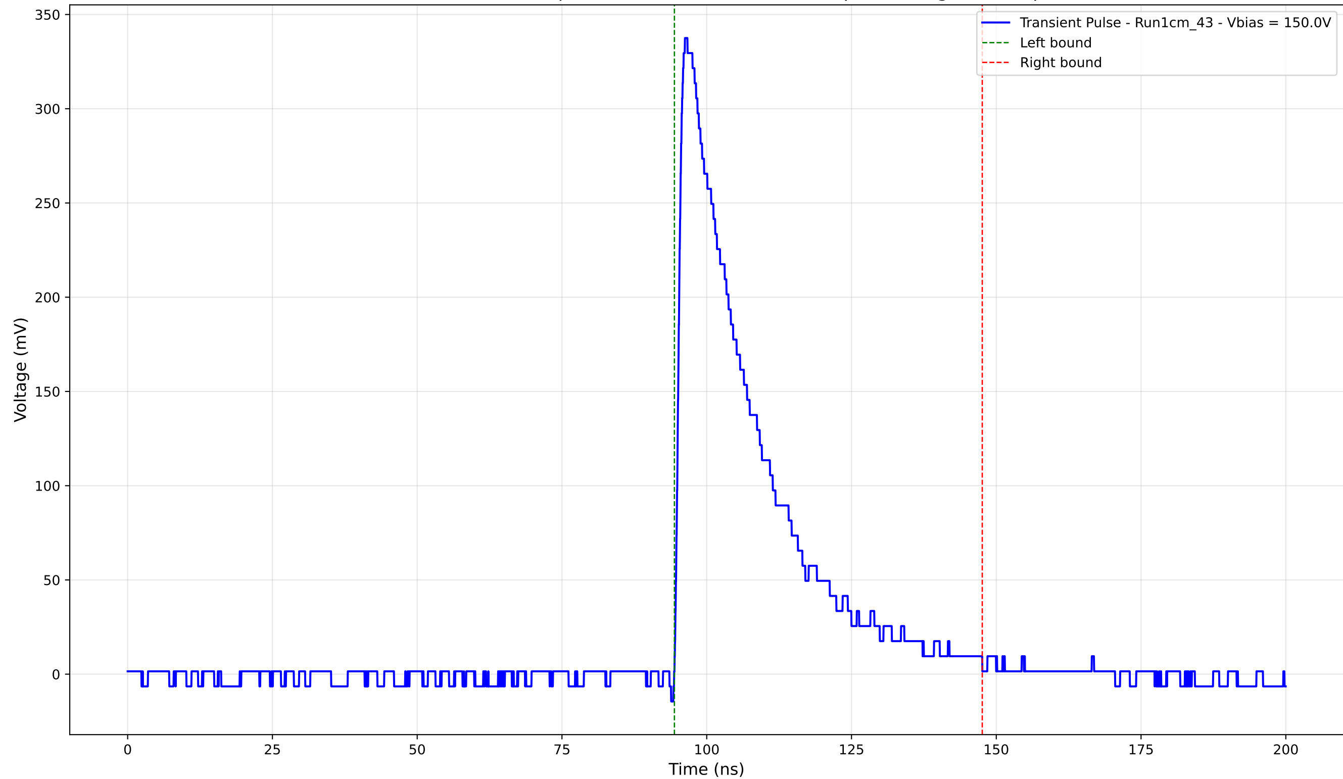
Transient Pulse - Sample: new1cm - Position: 725.0 \mu\text{m} - Charge: 93.72 pC
