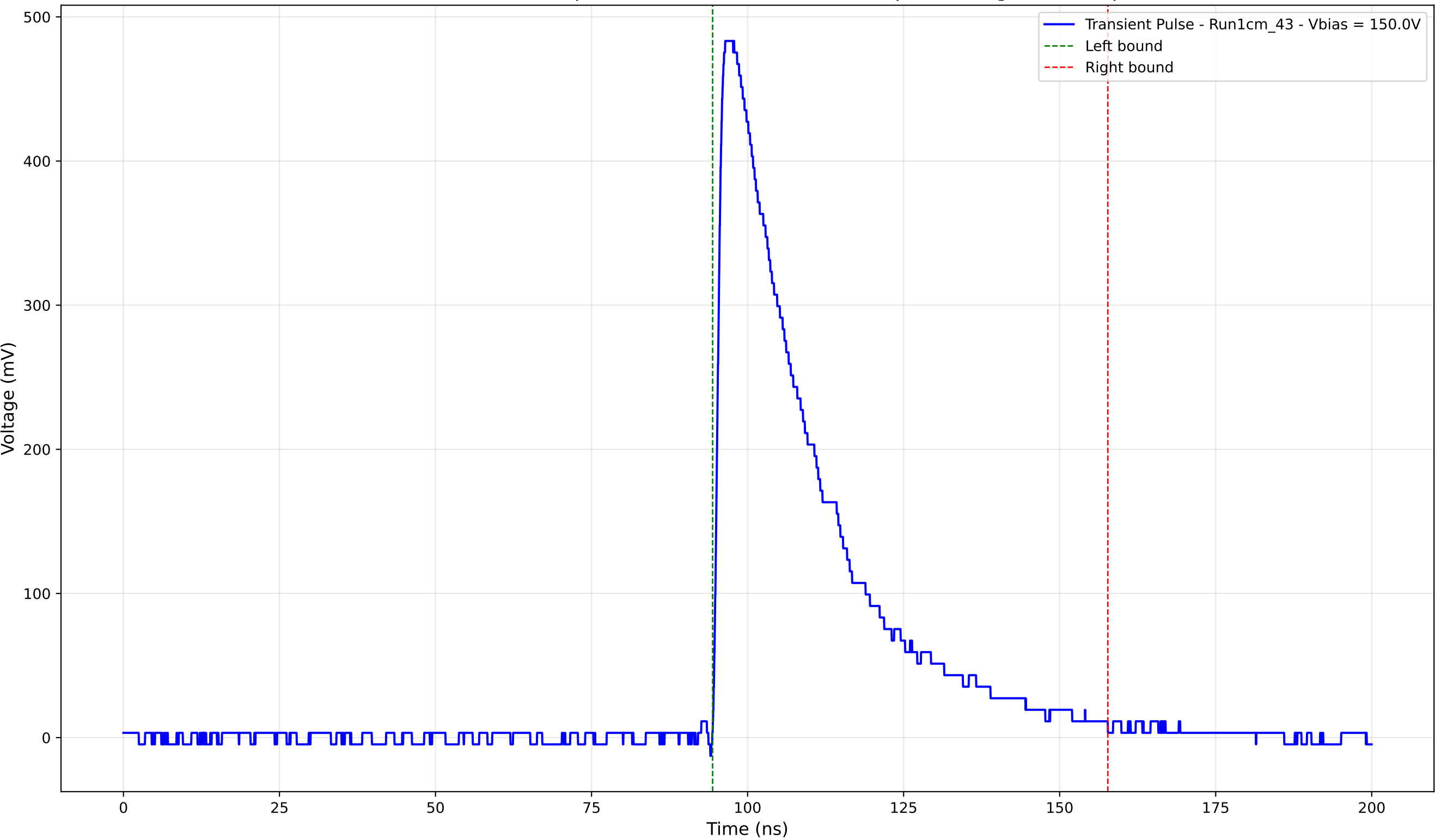
Transient Pulse - Sample: new1cm - Position: 3765.0 \mu\text{m} - Charge: 161.79 pC
