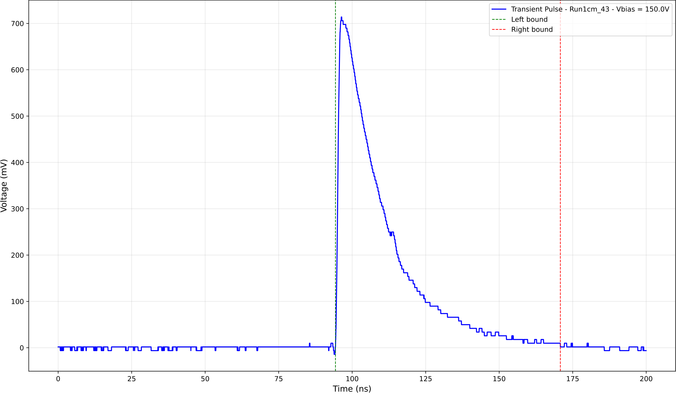
Transient Pulse - Sample: new1cm - Position: 3615.0 \mu\text{m} - Charge: 247.39 pC
