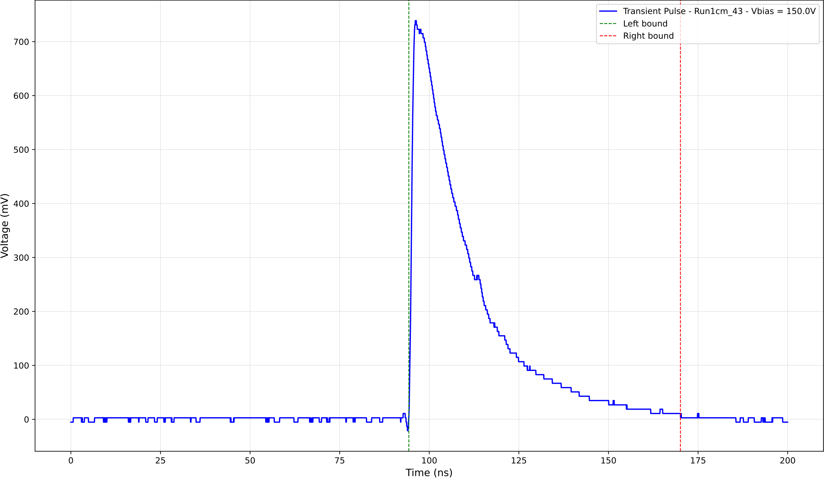
Transient Pulse - Sample: new1cm - Position: 3535.0 \mu\text{m} - Charge: 262.17 pC
