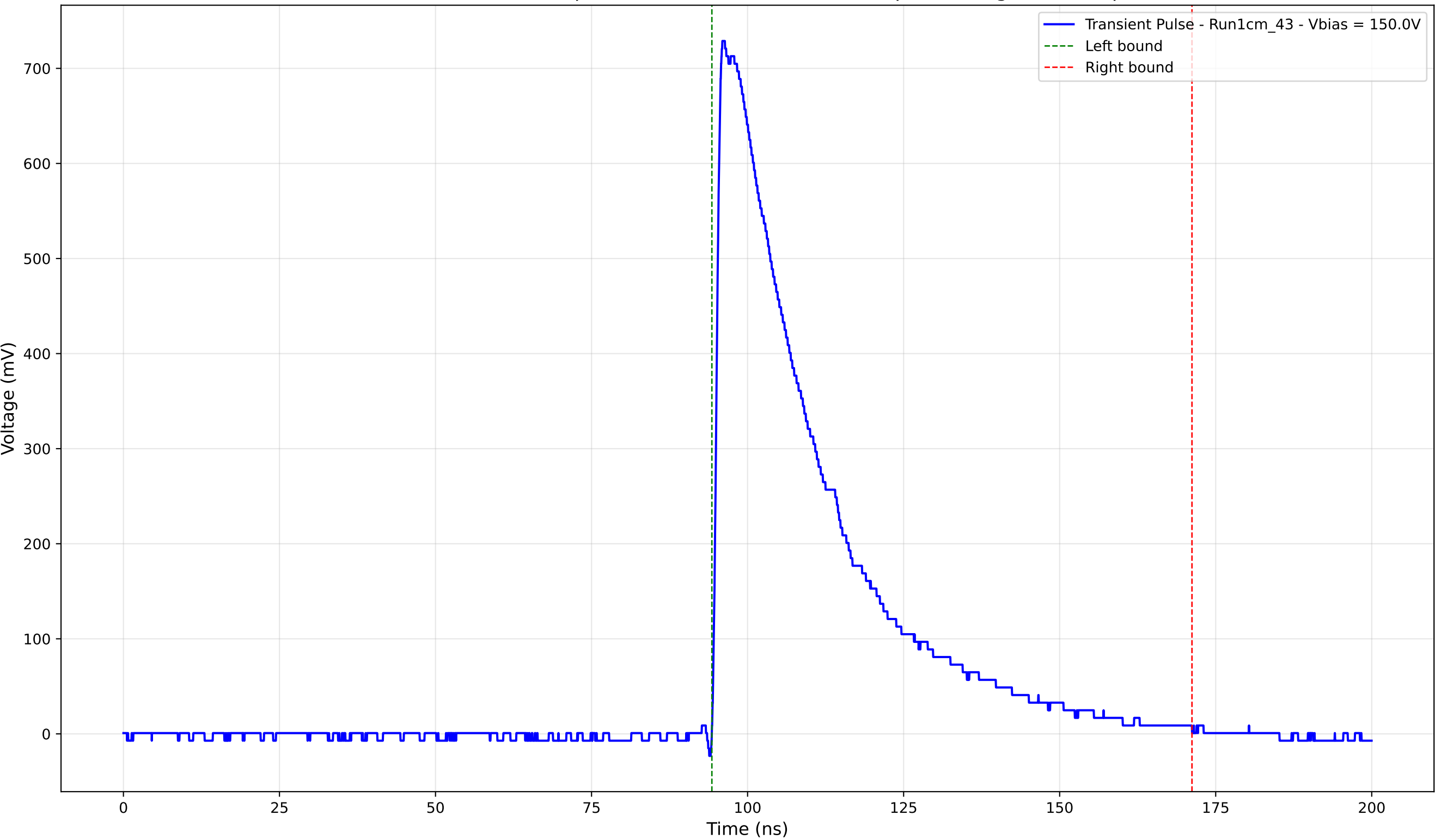
Transient Pulse - Sample: new1cm - Position: 3490.0 \mu\text{m} - Charge: 257.38 pC
