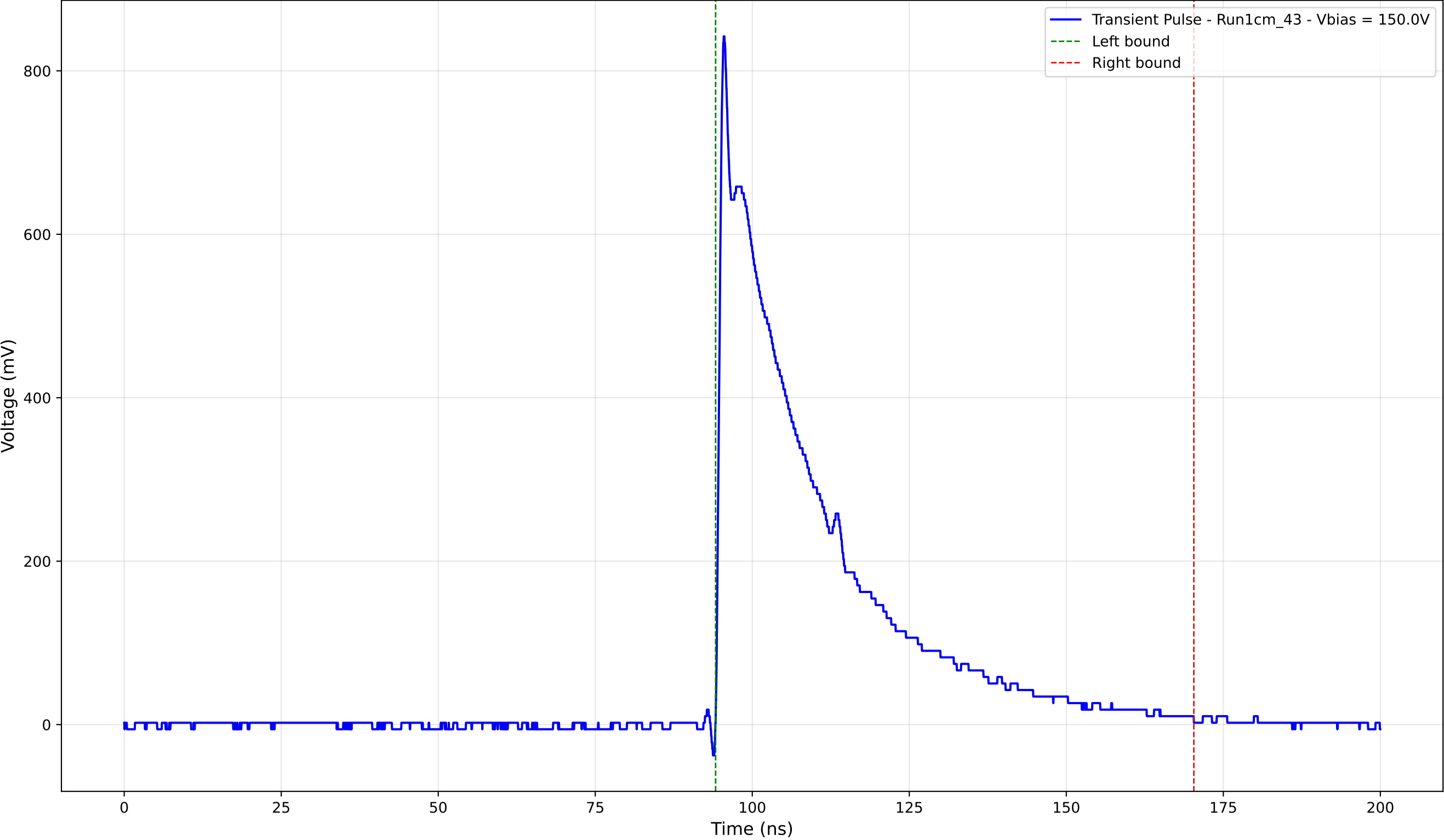
Transient Pulse - Sample: new1cm - Position: 3080.0 \mu\text{m} - Charge: 247.86 pC
