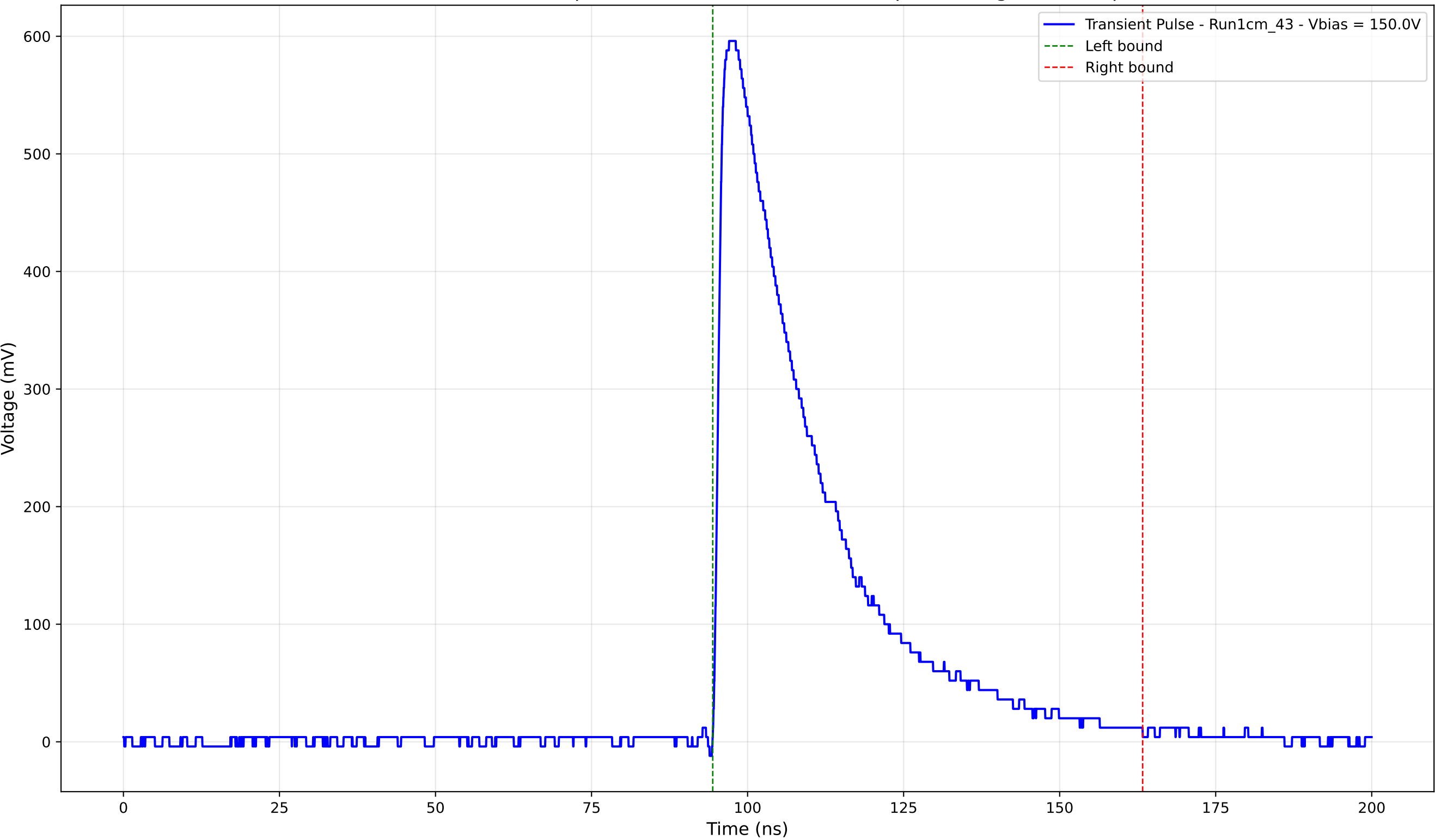
Transient Pulse - Sample: new1cm - Position: 1585.0 \mu\text{m} - Charge: 204.79 pC
