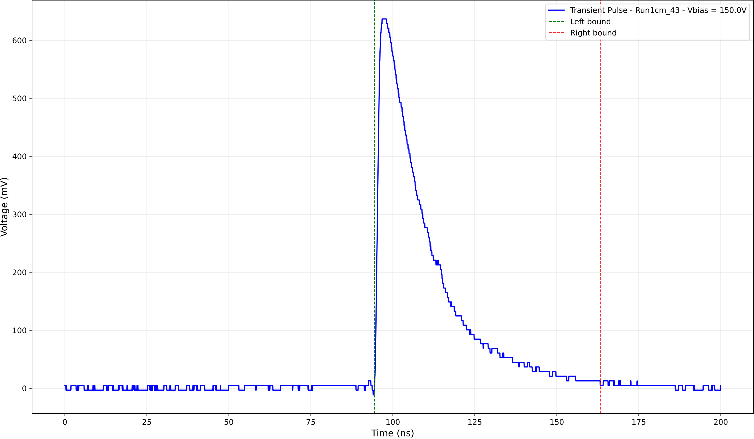
Transient Pulse - Sample: new1cm - Position: 1480.0 \mu\text{m} - Charge: 217.71 pC
