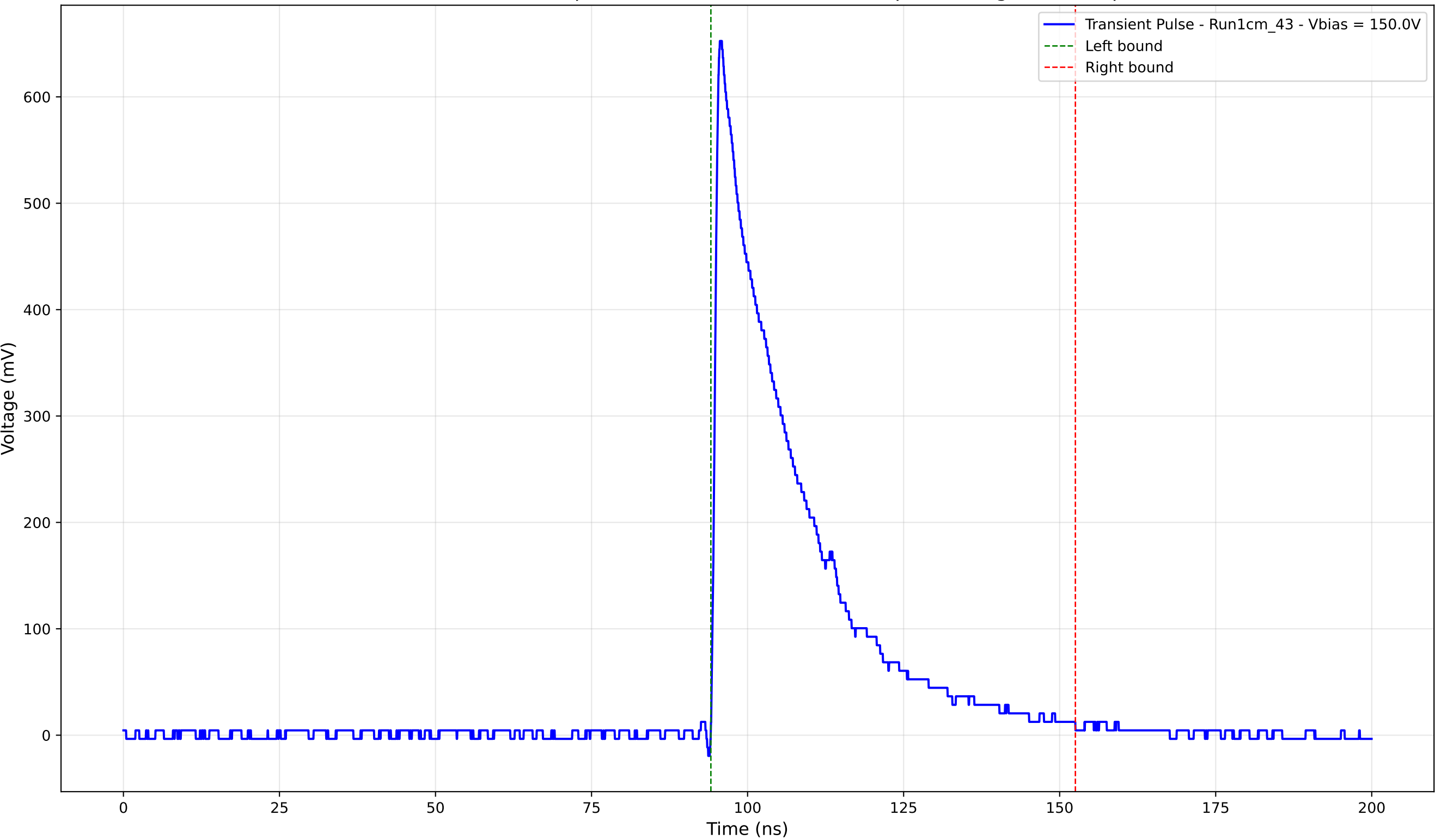
Transient Pulse - Sample: new1cm - Position: 4800.0 \mu\text{m} - Charge: 172.65 pC
