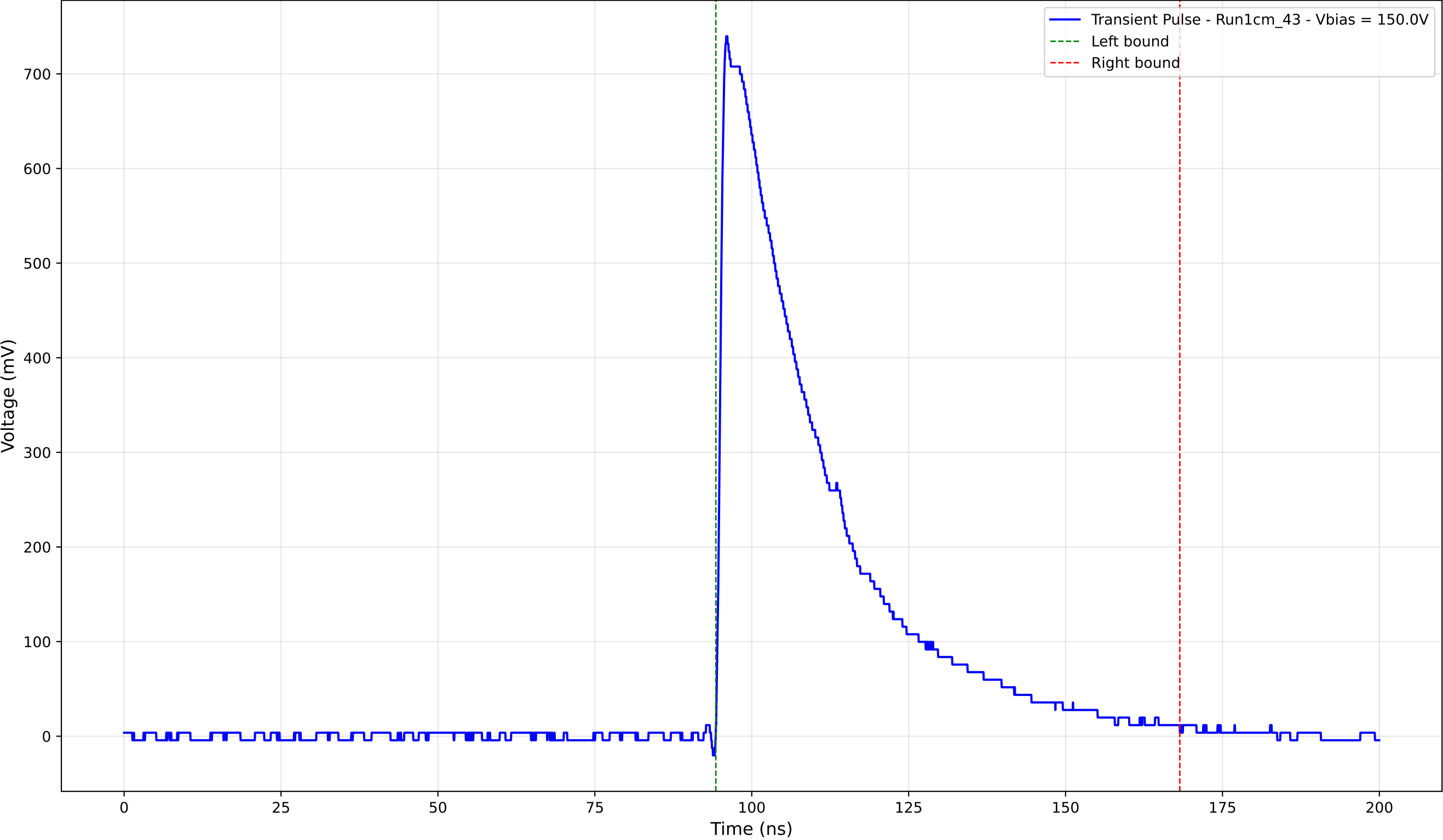
Transient Pulse - Sample: new1cm - Position: 3435.0 \mu\text{m} - Charge: 260.01 pC
