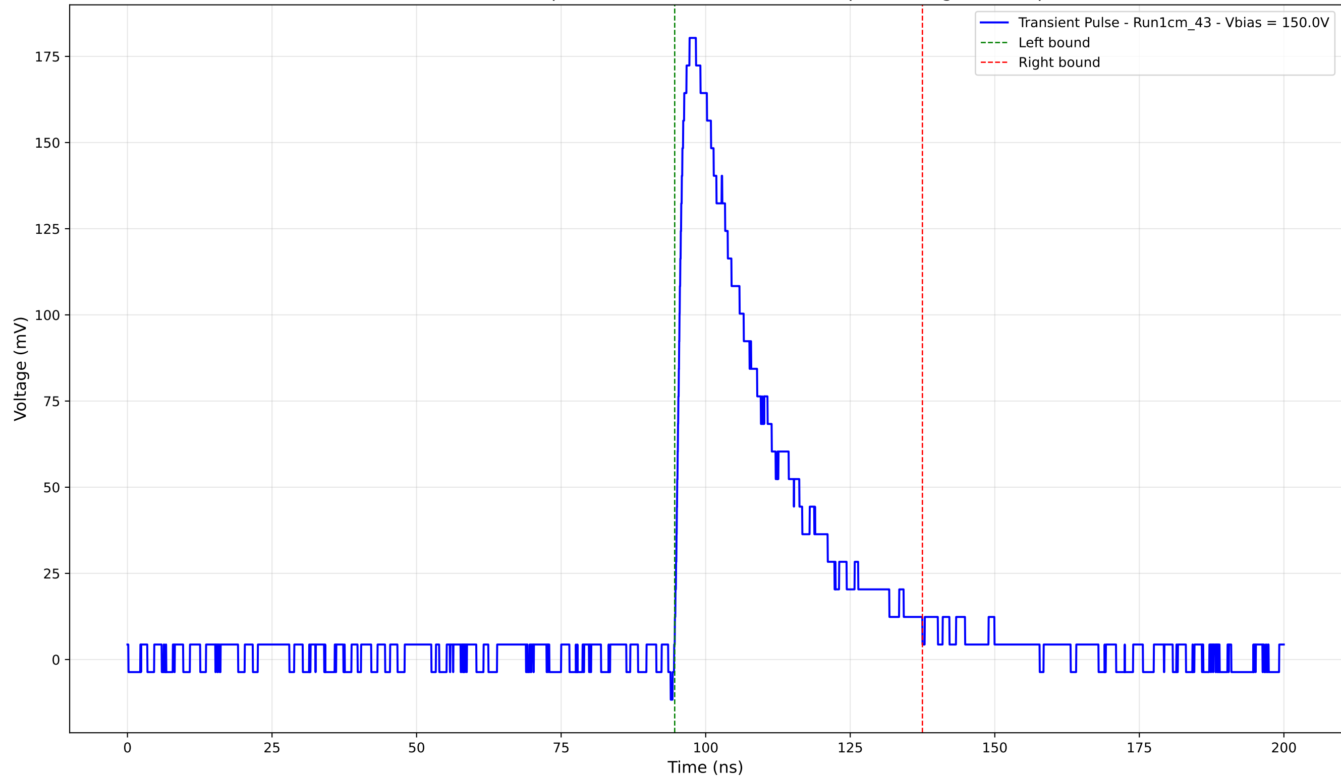
Transient Pulse - Sample: new1cm - Position: 1210.0 \mu\text{m} - Charge: 55.81 pC
