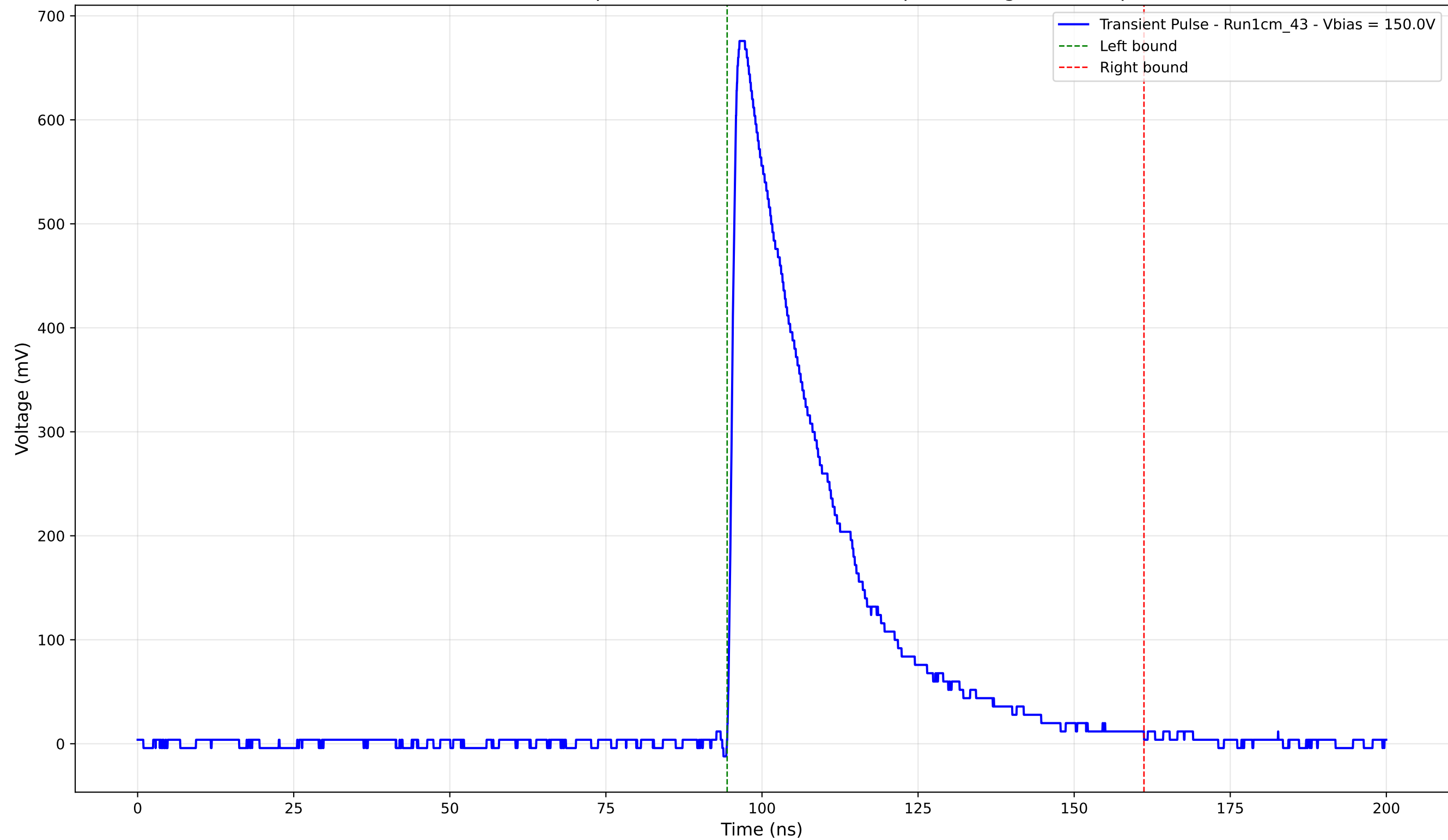
Transient Pulse - Sample: new1cm - Position: 885.0 \mu\text{m} - Charge: 207.69 pC
