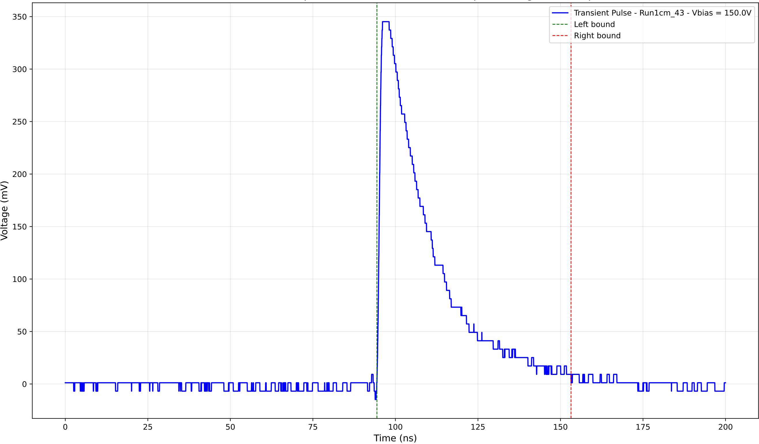
Transient Pulse - Sample: new1cm - Position: 3665.0 \mu\text{m} - Charge: 114.92 pC
