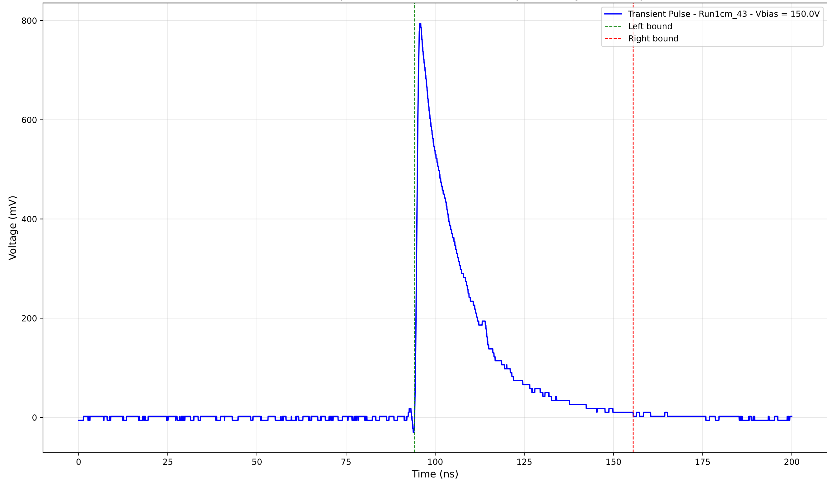
Transient Pulse - Sample: new1cm - Position: 435.0 \mu\text{m} - Charge: 201.10 pC
