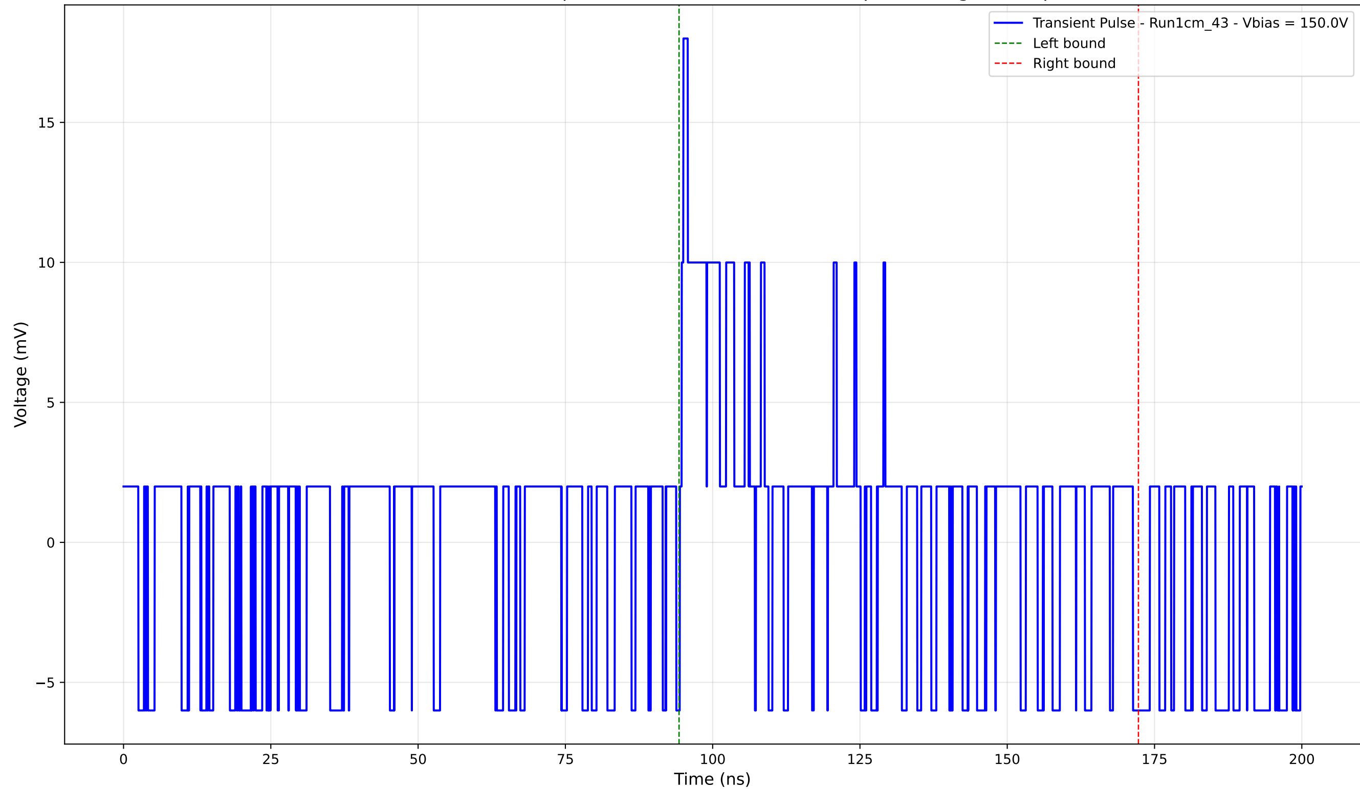
Transient Pulse - Sample: new1cm - Position: 5085.0 \mu\text{m} - Charge: 2.49 pC
