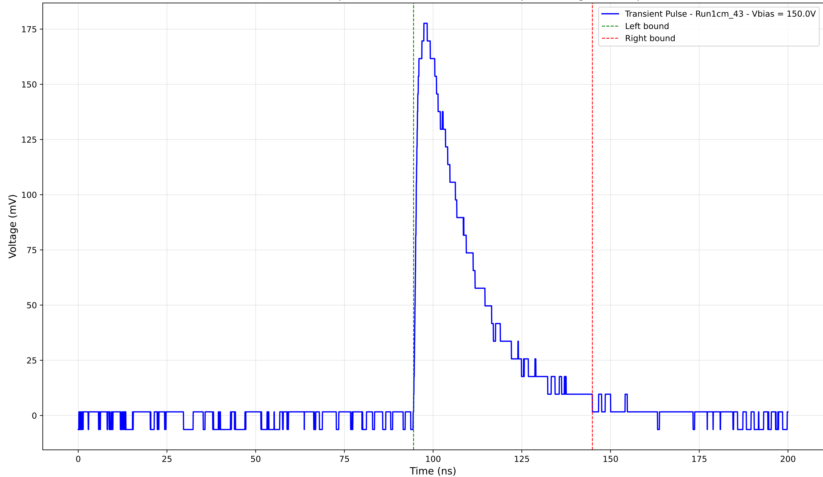
Transient Pulse - Sample: new1cm - Position: 1715.0 \mu\text{m} - Charge: 57.45 pC
