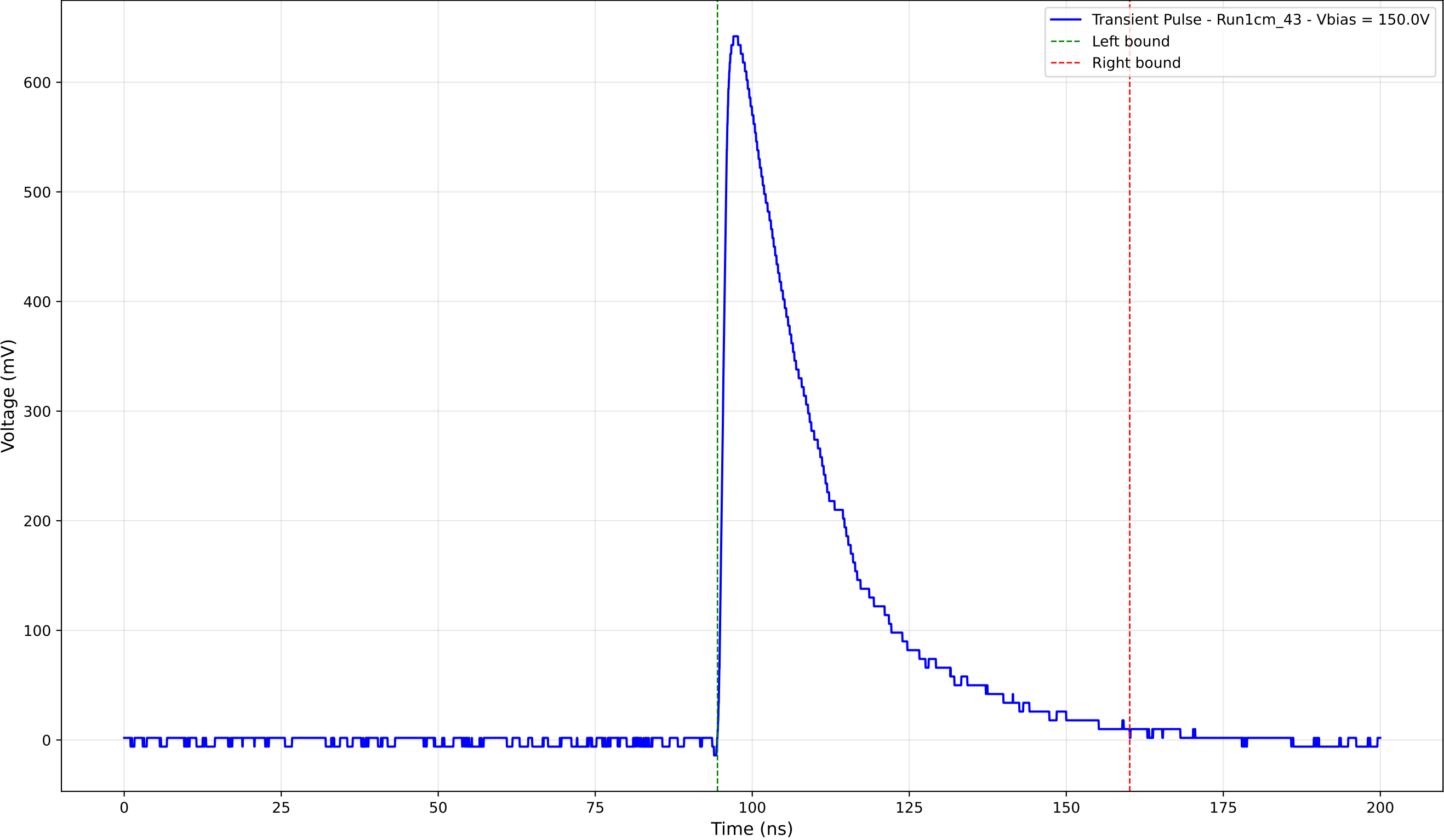
Transient Pulse - Sample: new1cm - Position: 1395.0 \mu\text{m} - Charge: 213.11 pC
