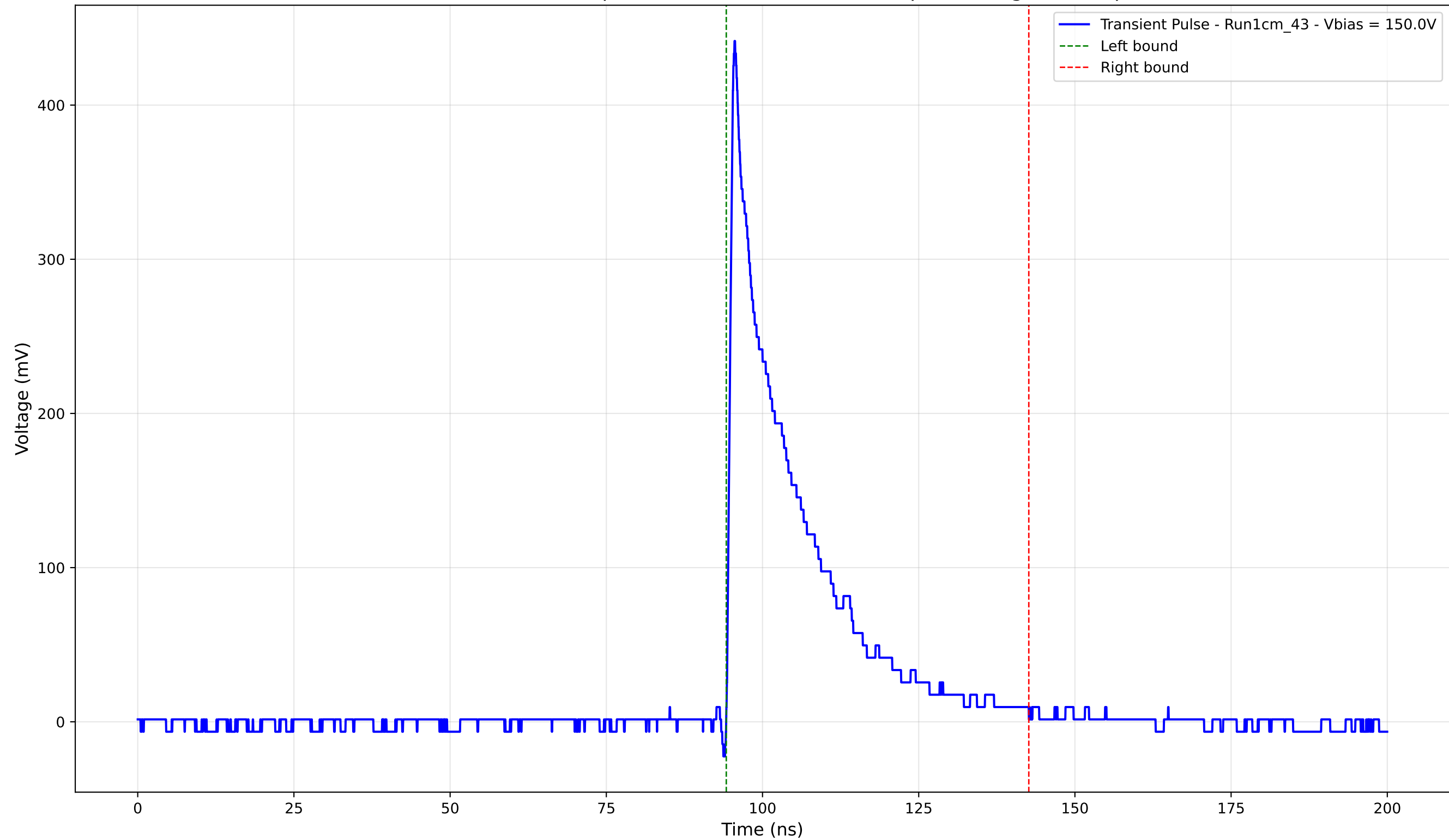
Transient Pulse - Sample: new1cm - Position: 225.0 \mu\text{m} - Charge: 87.38 pC
