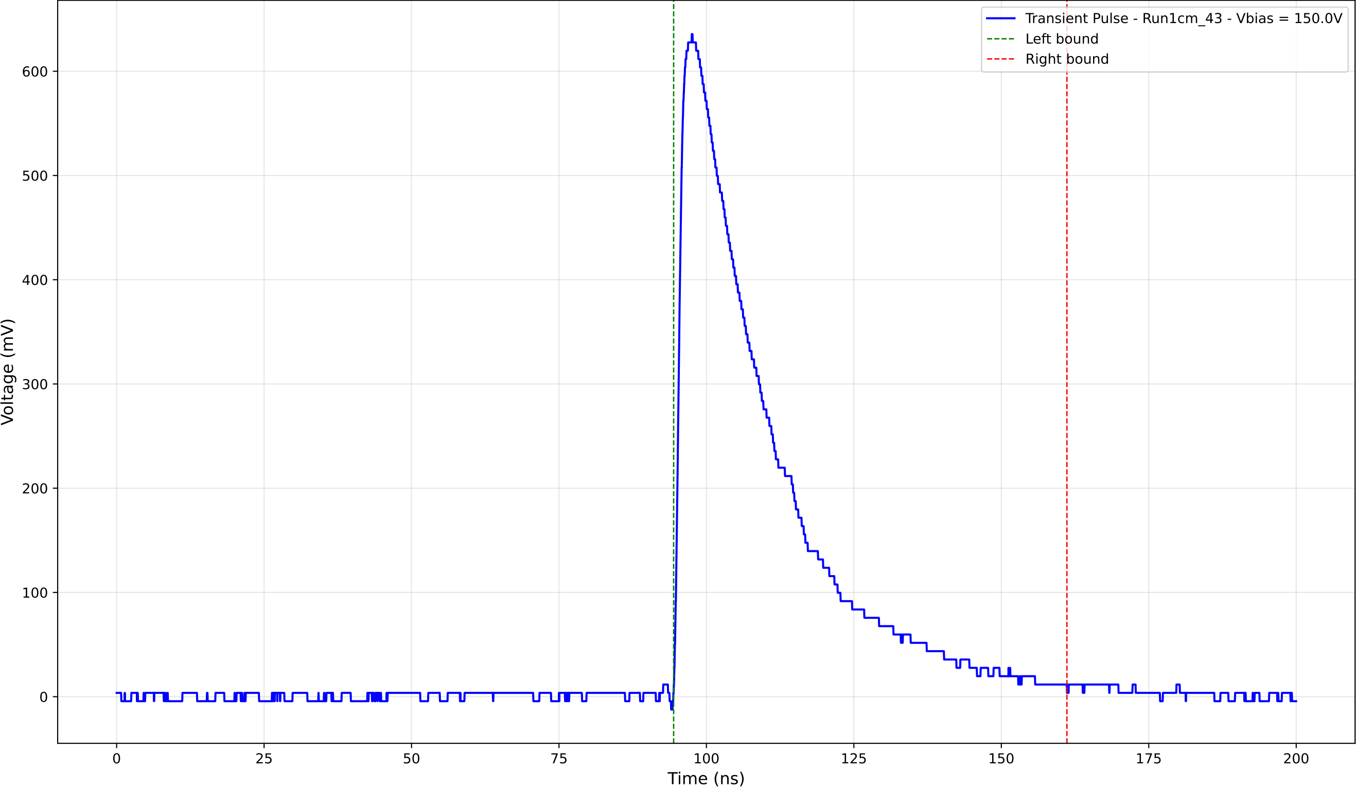
Transient Pulse - Sample: new1cm - Position: 1545.0 \mu\text{m} - Charge: 214.89 pC
