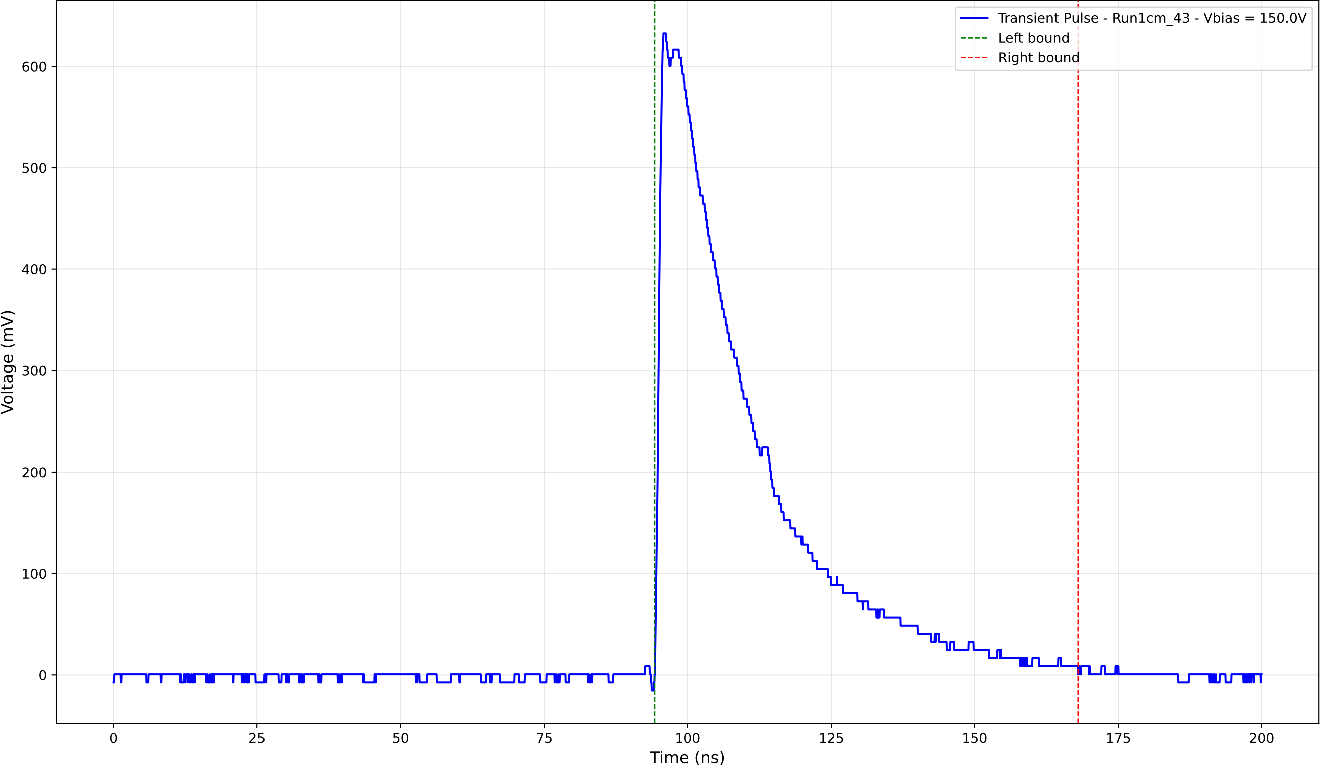
Transient Pulse - Sample: new1cm - Position: 1990.0 \mu\text{m} - Charge: 223.11 pC
