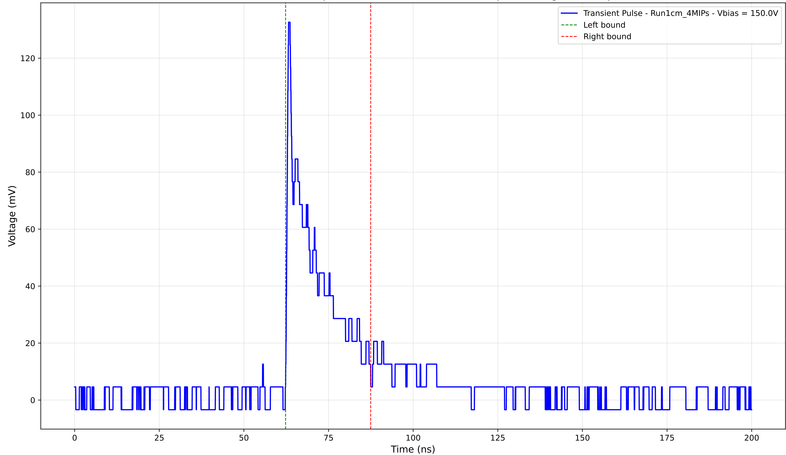
Transient Pulse - Sample: new1cm - Position: 3410.0 \mu\text{m} - Charge: 21.92 pC
