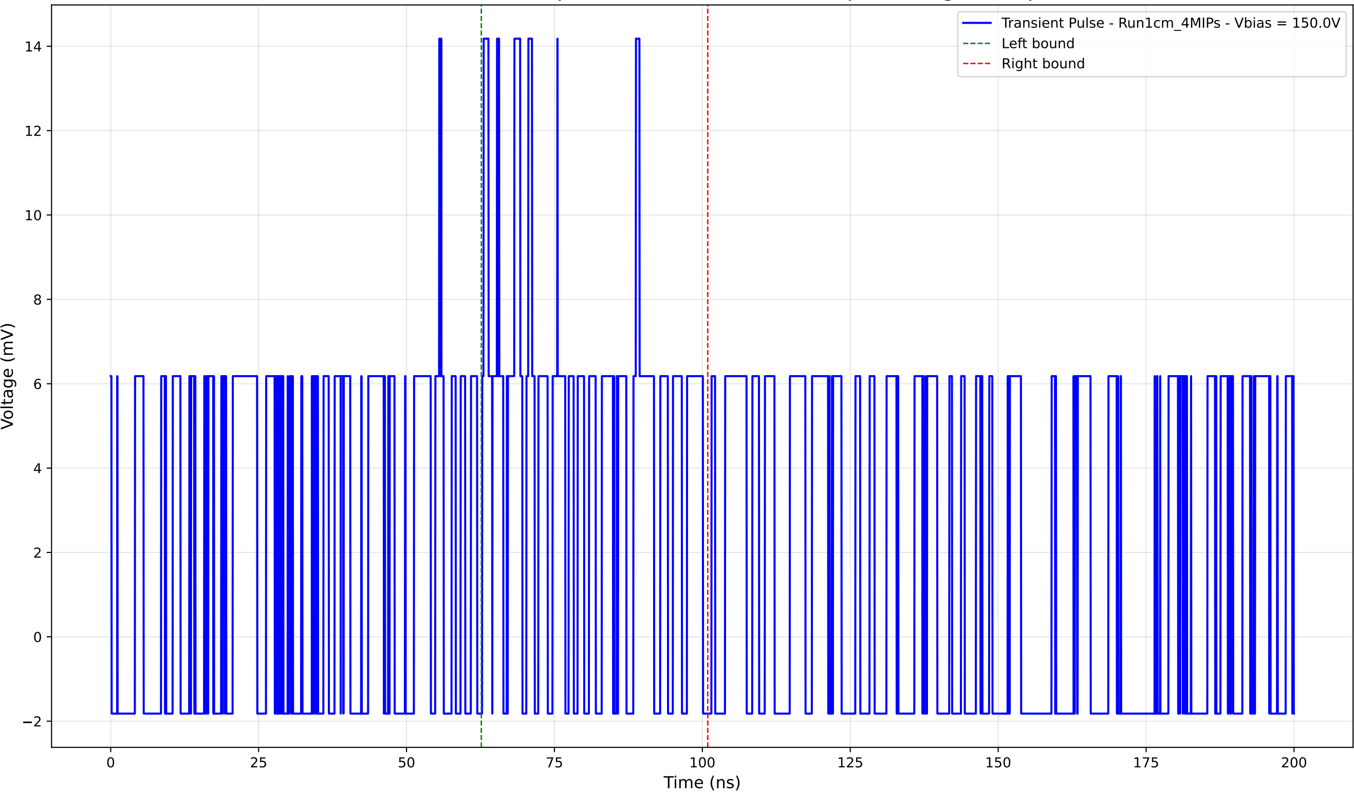
Transient Pulse - Sample: new1cm - Position: 185.0 \mu\text{m} - Charge: 3.46 pC
