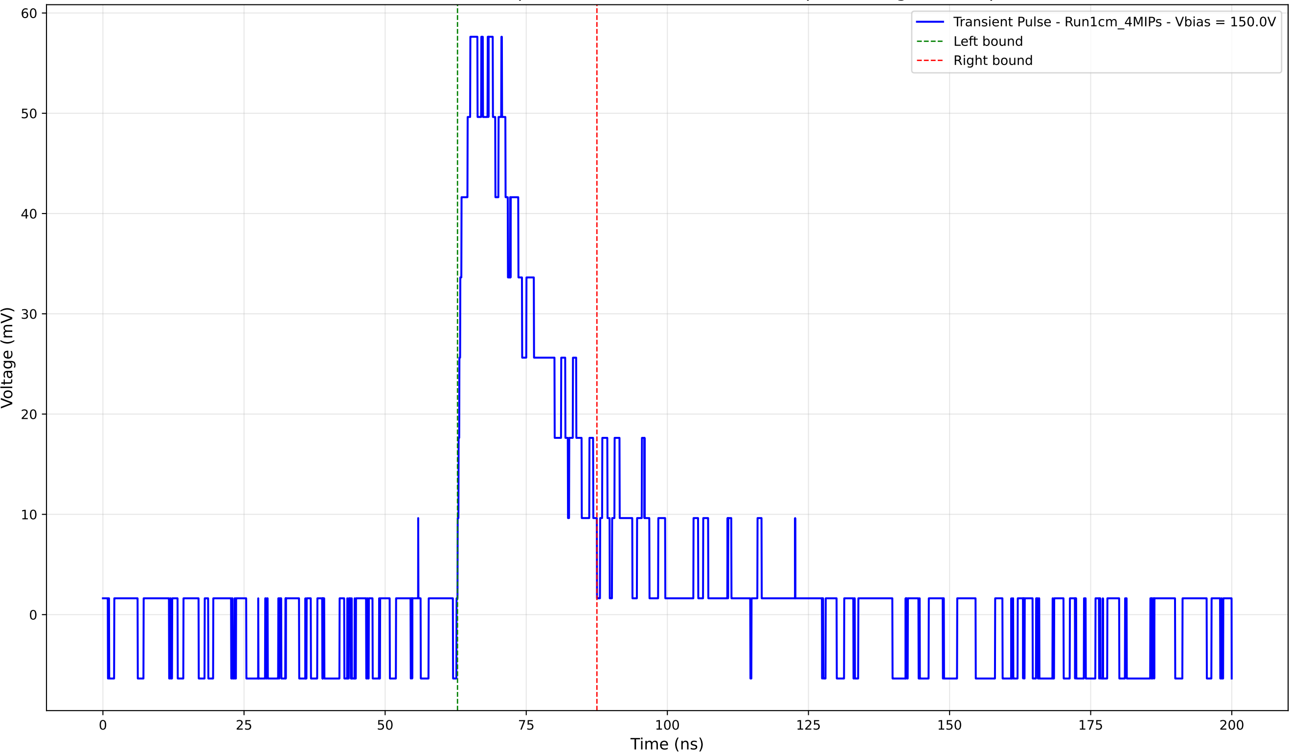
Transient Pulse - Sample: new1cm - Position: 2095.0 \mu\text{m} - Charge: 16.15 pC
