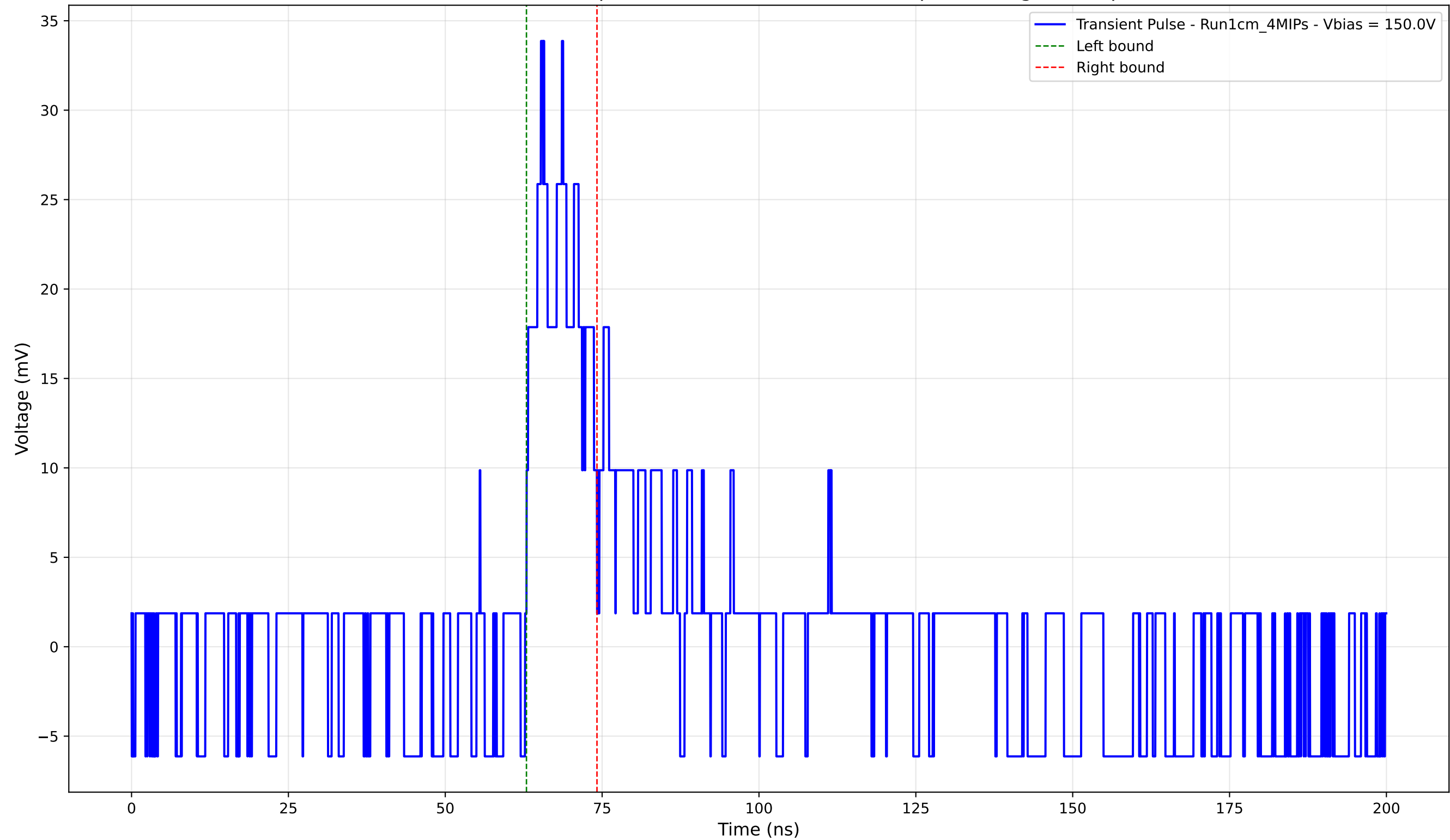
Transient Pulse - Sample: new1cm - Position: 1145.0 \mu\text{m} - Charge: 4.59 pC
