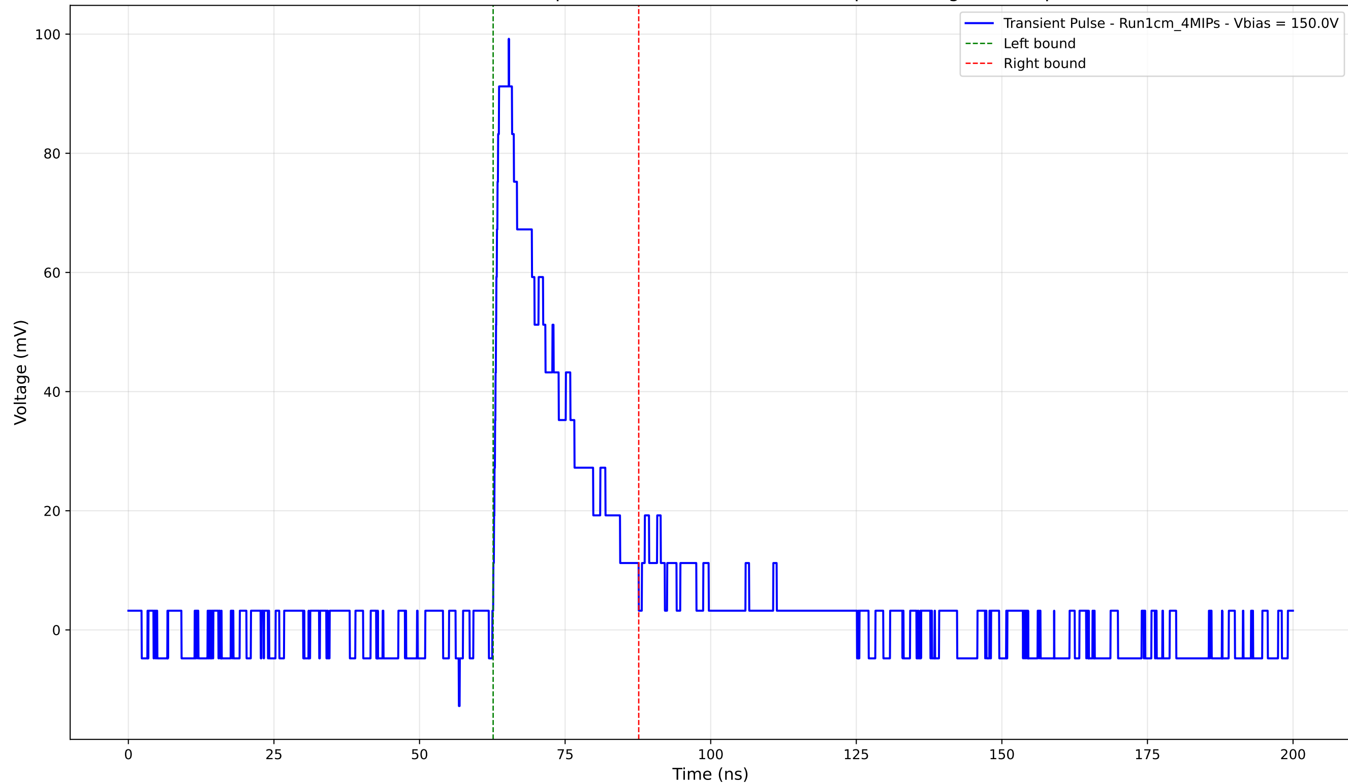
Transient Pulse - Sample: new1cm - Position: 4325.0 \mu\text{m} - Charge: 20.84 pC
