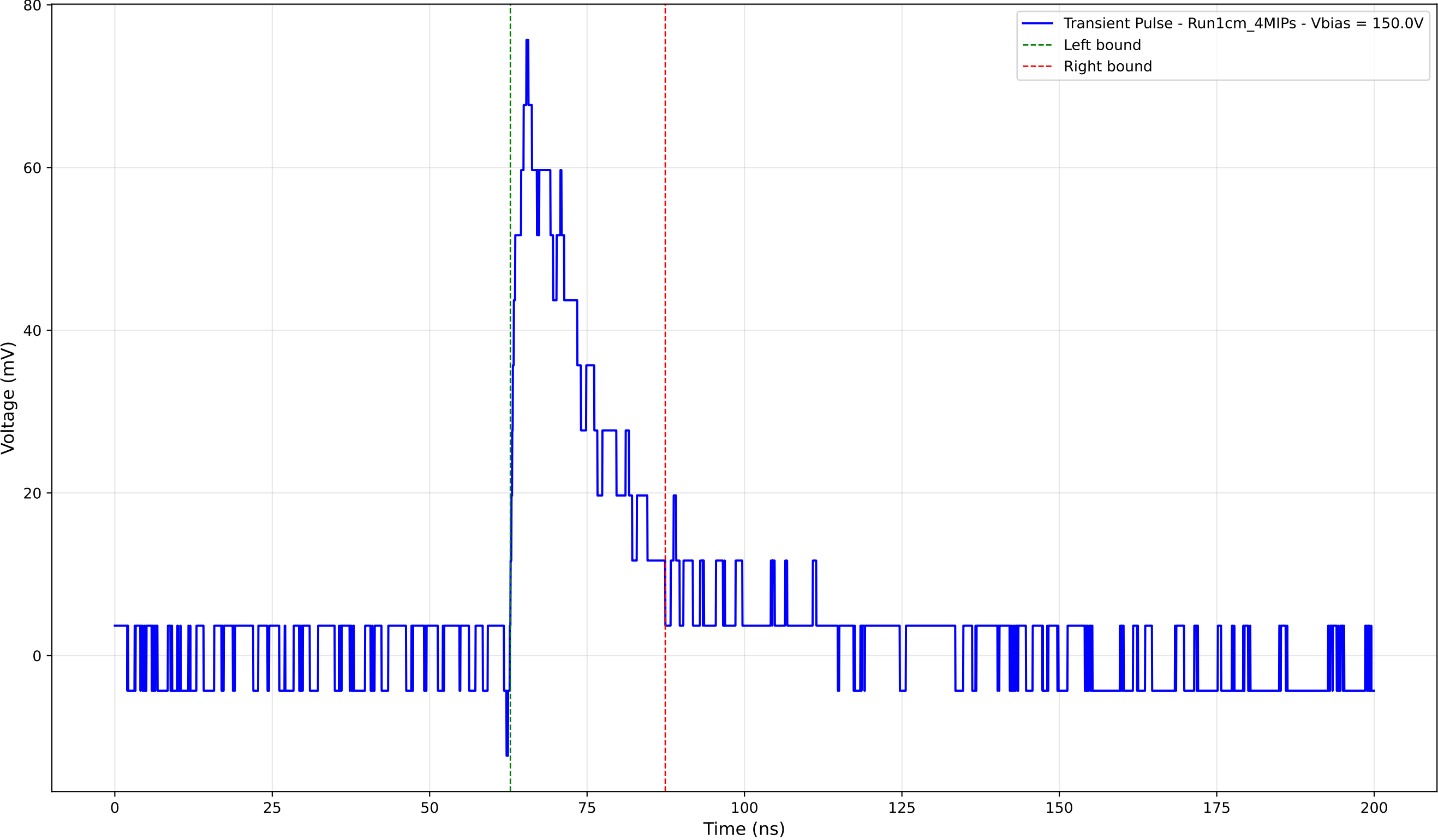
Transient Pulse - Sample: new1cm - Position: 1075.0 \mu\text{m} - Charge: 17.41 pC
