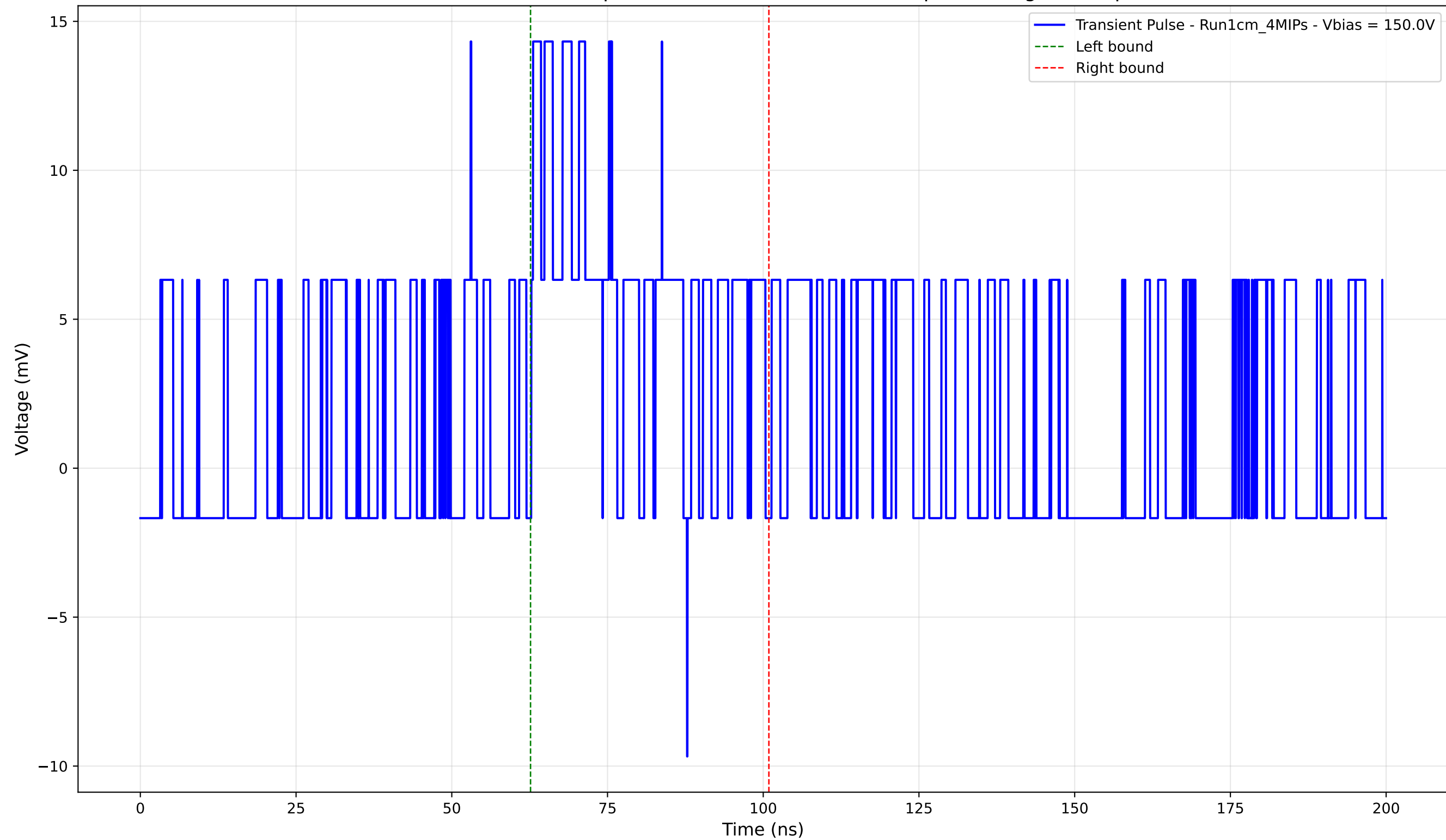
Transient Pulse - Sample: new1cm - Position: 4725.0 \mu\text{m} - Charge: 4.64 pC
