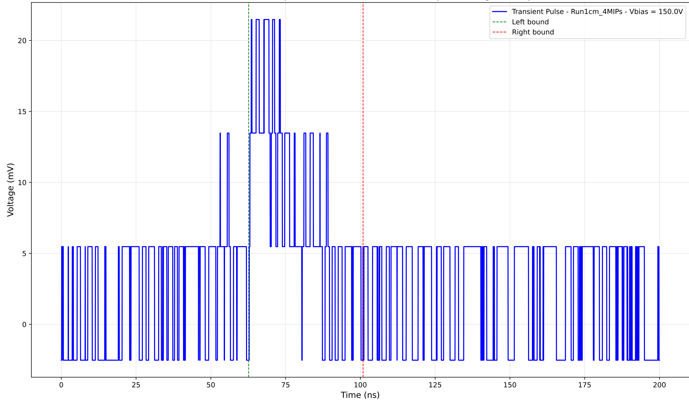
Transient Pulse - Sample: new1cm -Position: 1665.0 \mu\text{m} - Charge: 6.26 pC
