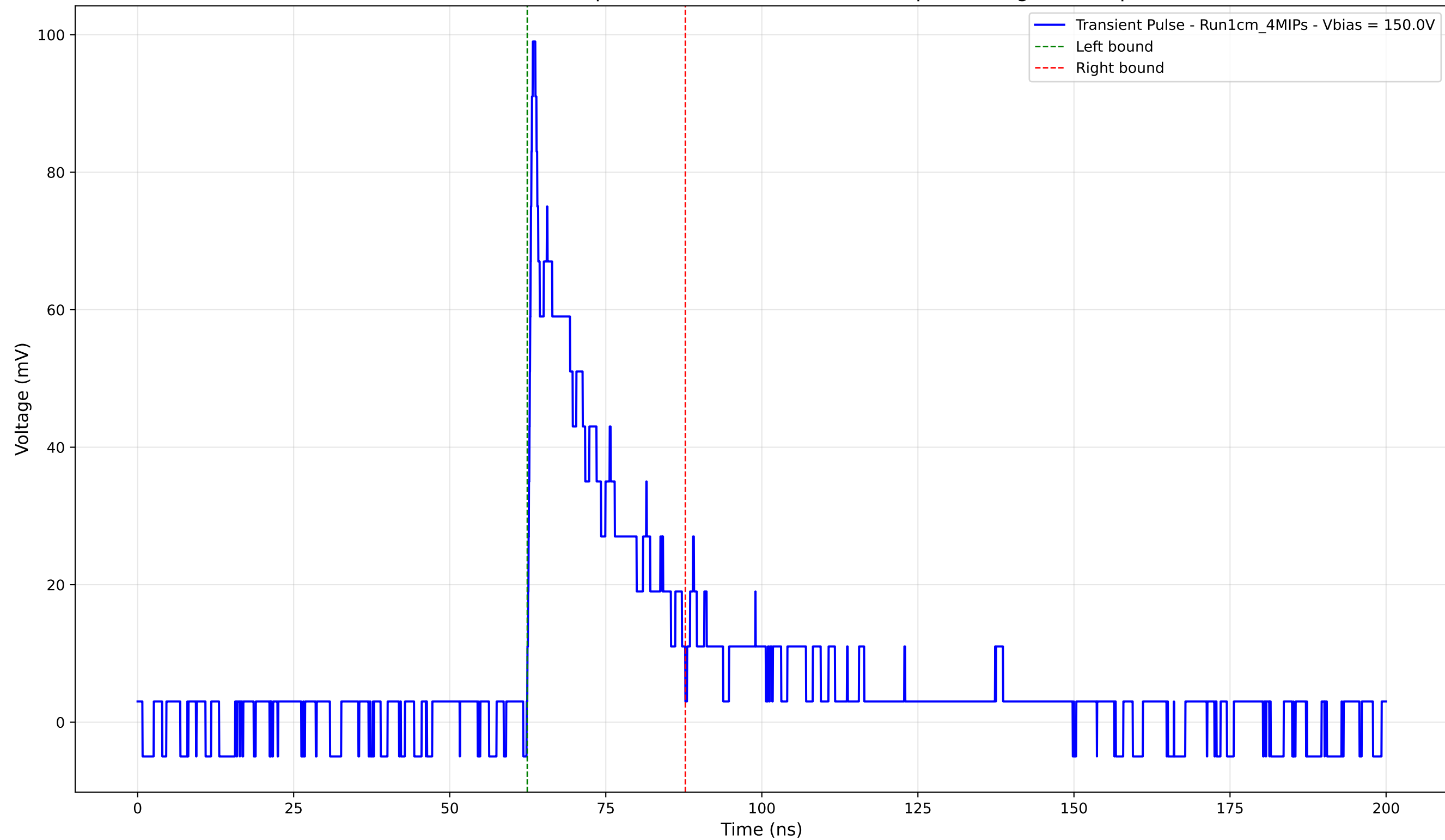
Transient Pulse - Sample: new1cm - Position: 2870.0 \mu\text{m} - Charge: 19.46 pC
