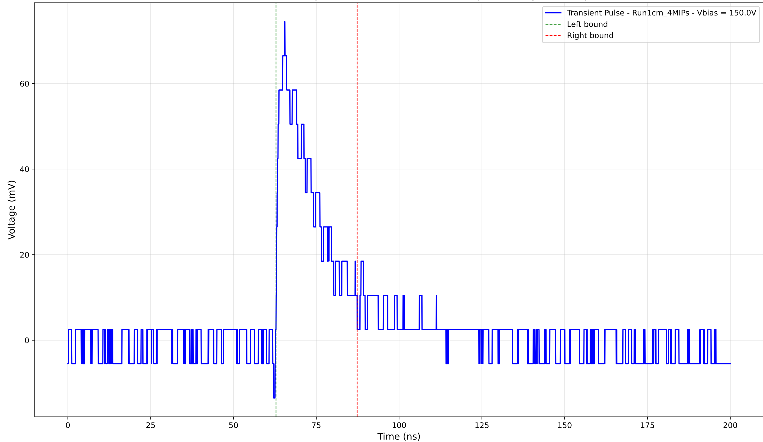
Transient Pulse - Sample: new1cm -Position: 990.0 \mu\text{m} - Charge: 16.43 pC
