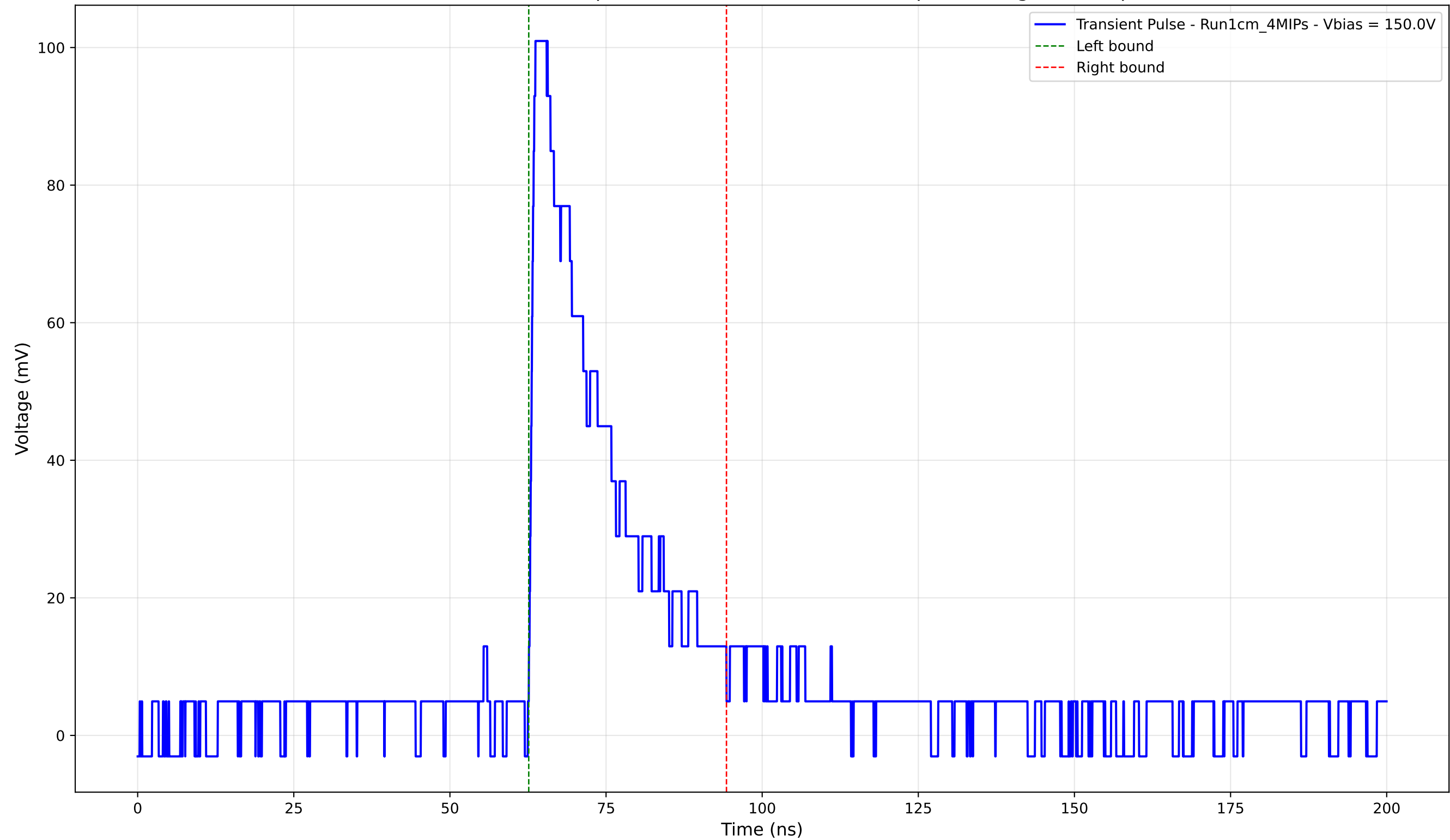
Transient Pulse - Sample: new1cm - Position: 4095.0 \mu\text{m} - Charge: 25.84 pC
