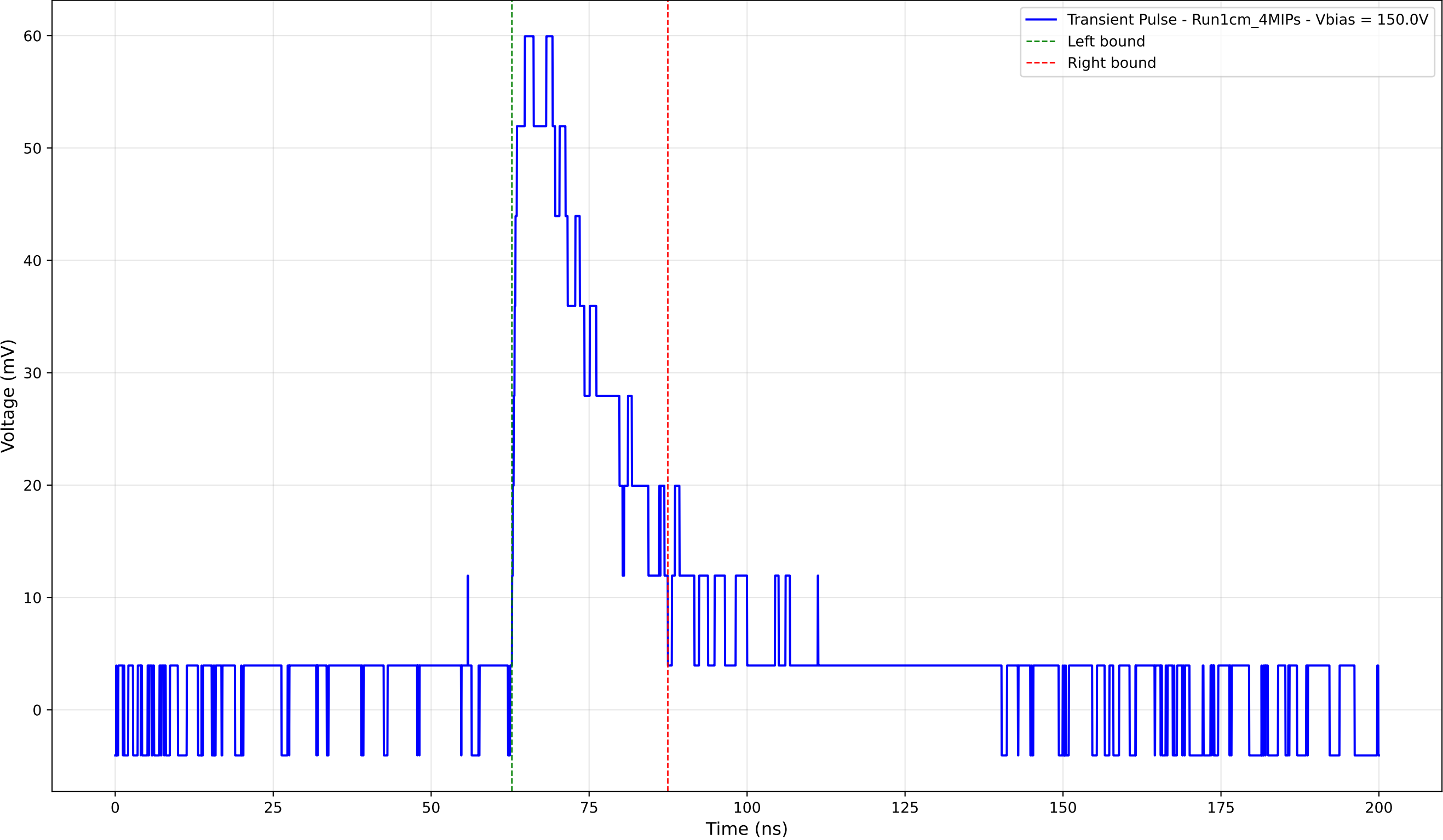
Transient Pulse - Sample: new1cm - Position: 2305.0 \mu\text{m} - Charge: 17.06 pC
