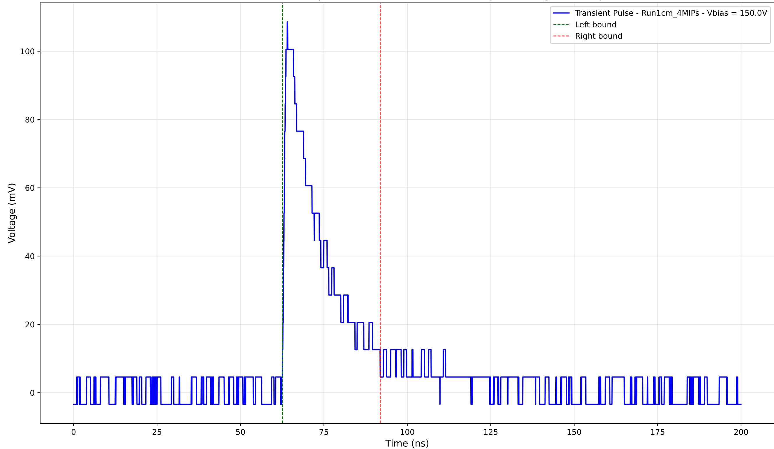
Transient Pulse - Sample: new1cm - Position: 4430.0 \mu\text{m} - Charge: 24.84 pC
