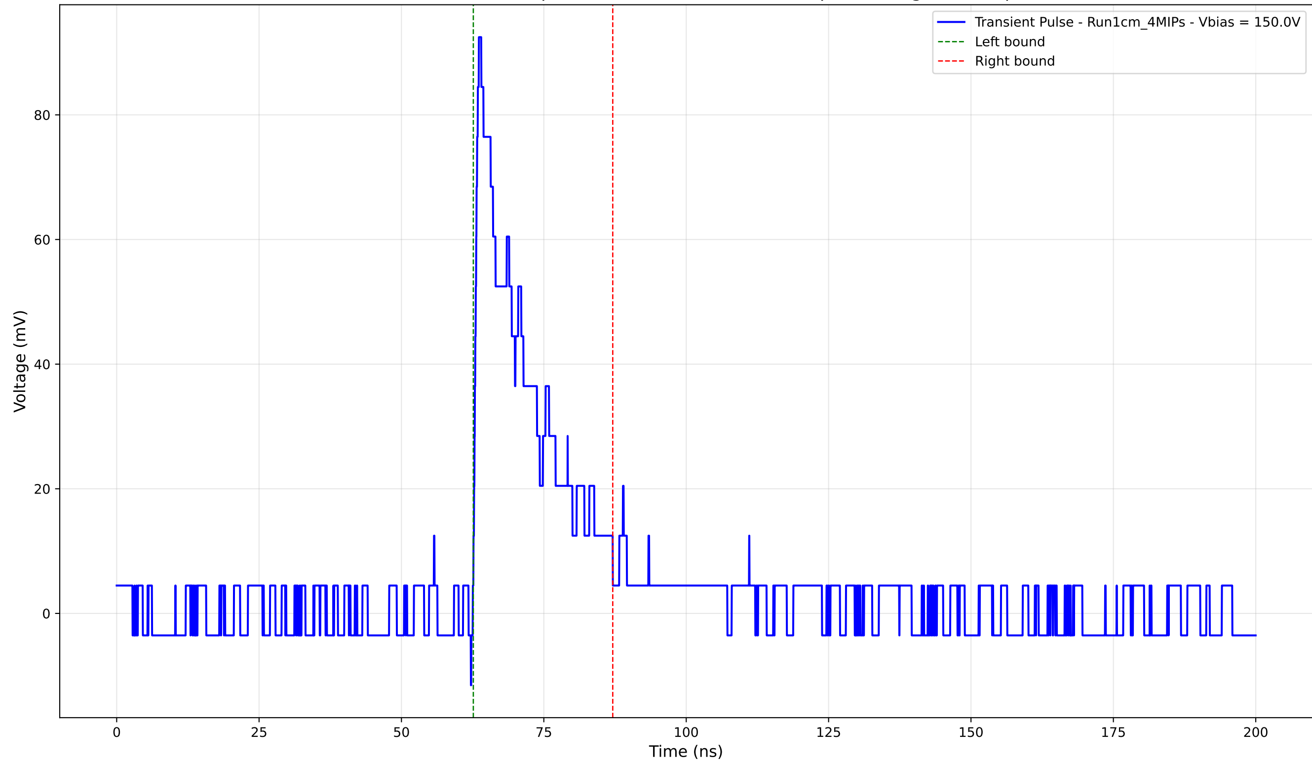
Transient Pulse - Sample: new1cm -Position: 425.0 \mu\text{m} - Charge: 17.39 pC
