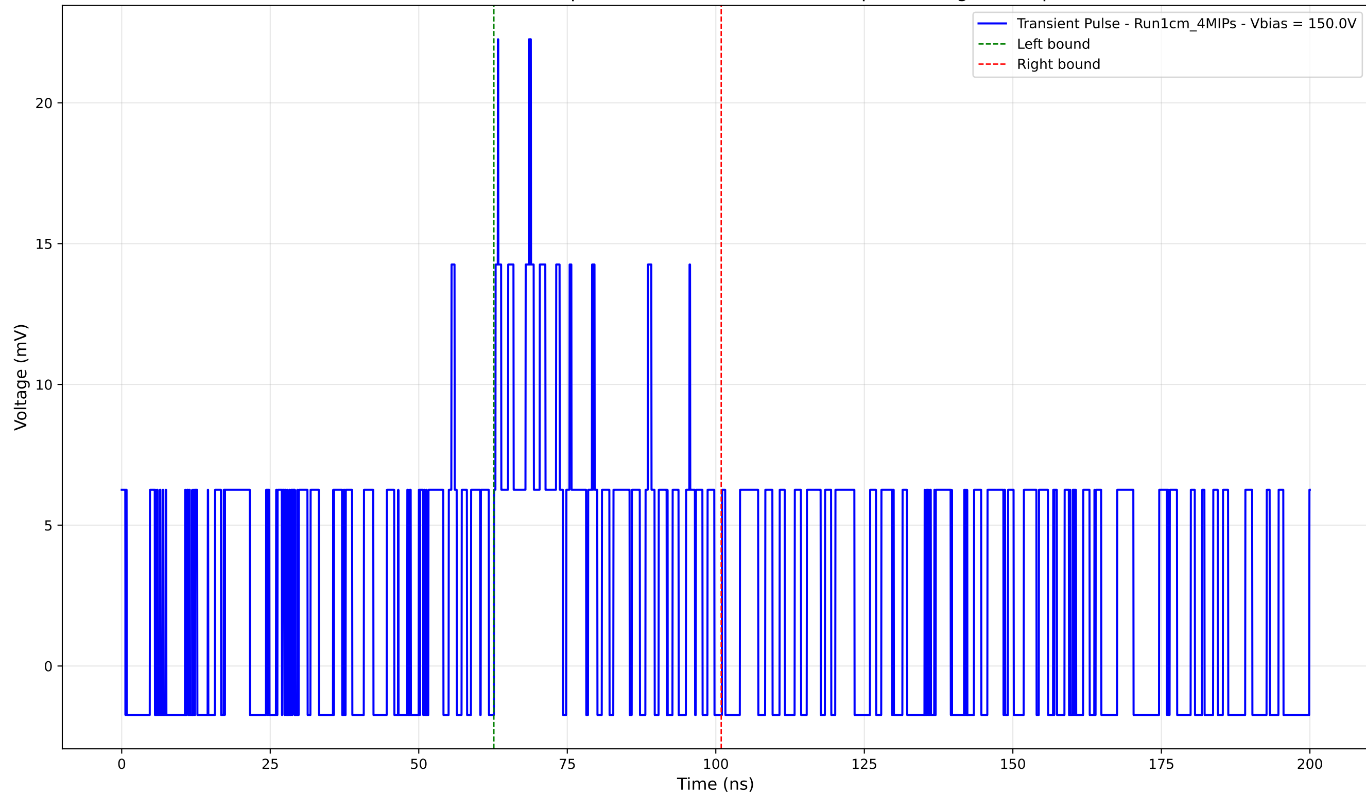
Transient Pulse - Sample: new1cm - Position: 695.0 \mu\text{m} - Charge: 4.45 pC
