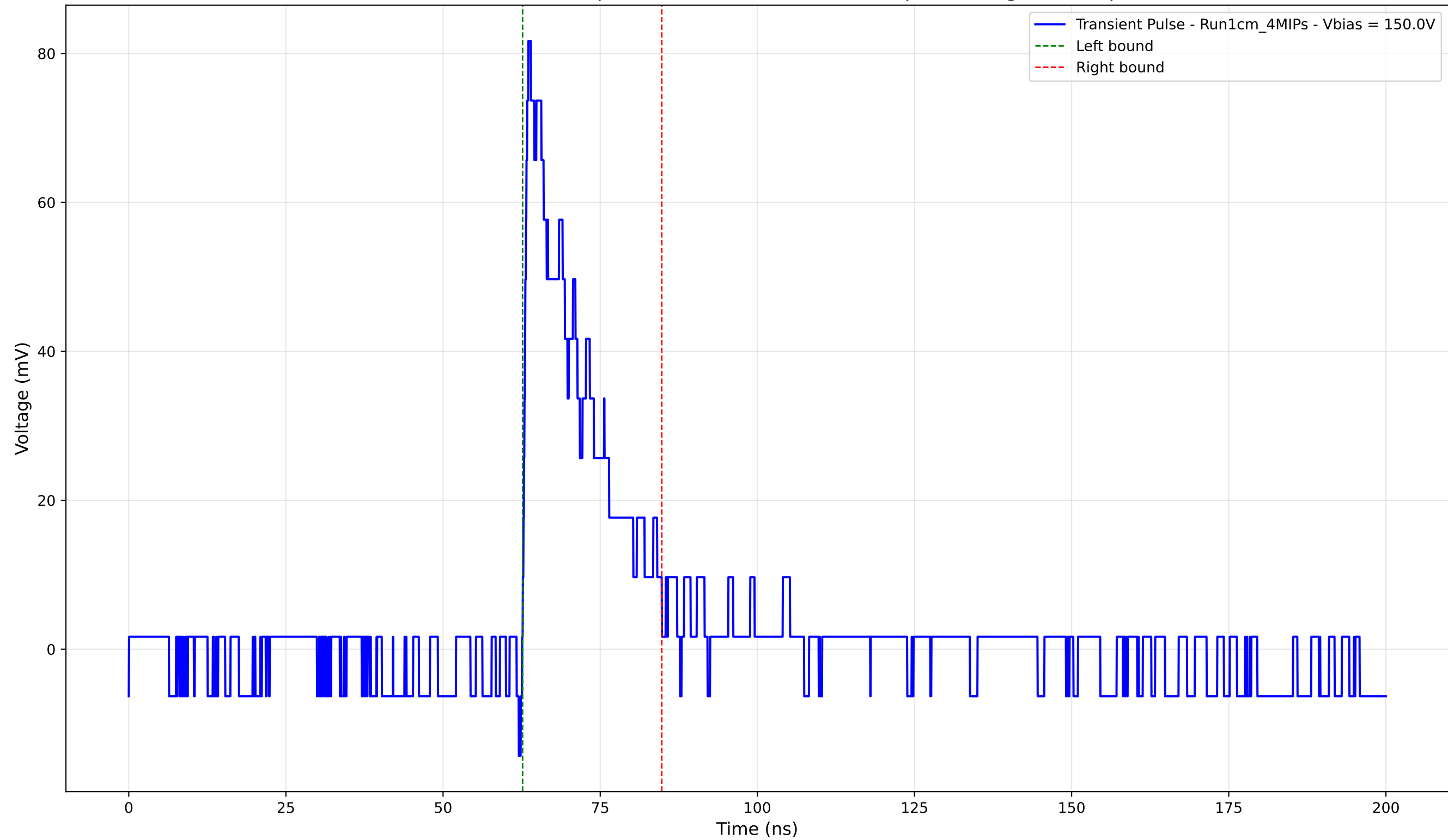
Transient Pulse - Sample: new1cm - Position: 525.0 \mu\text{m} - Charge: 15.19 pC
