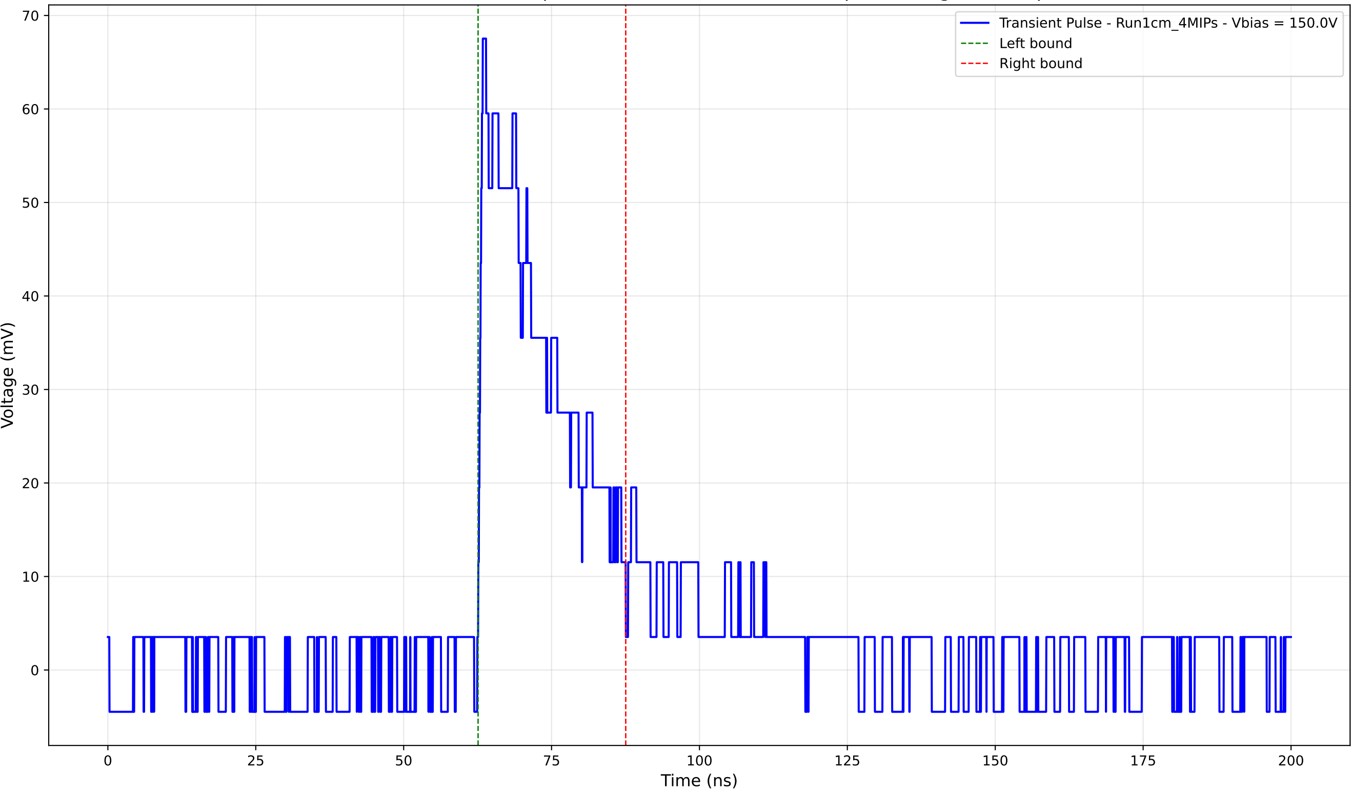
Transient Pulse - Sample: new1cm - Position: 2620.0 \mu\text{m} - Charge: 17.11 pC
