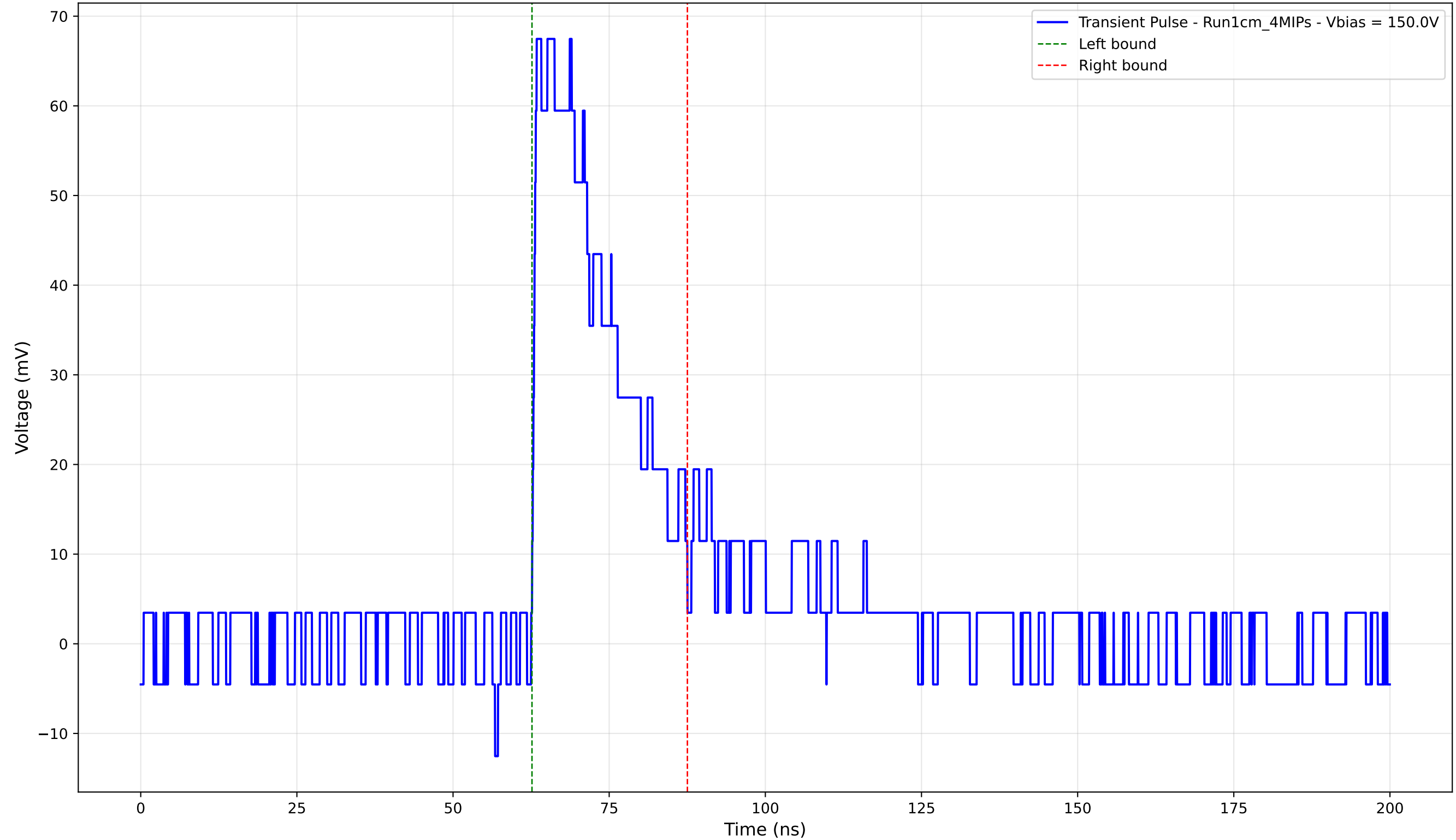
Transient Pulse - Sample: new1cm - Position: 2505.0 \mu\text{m} - Charge: 18.72 pC
