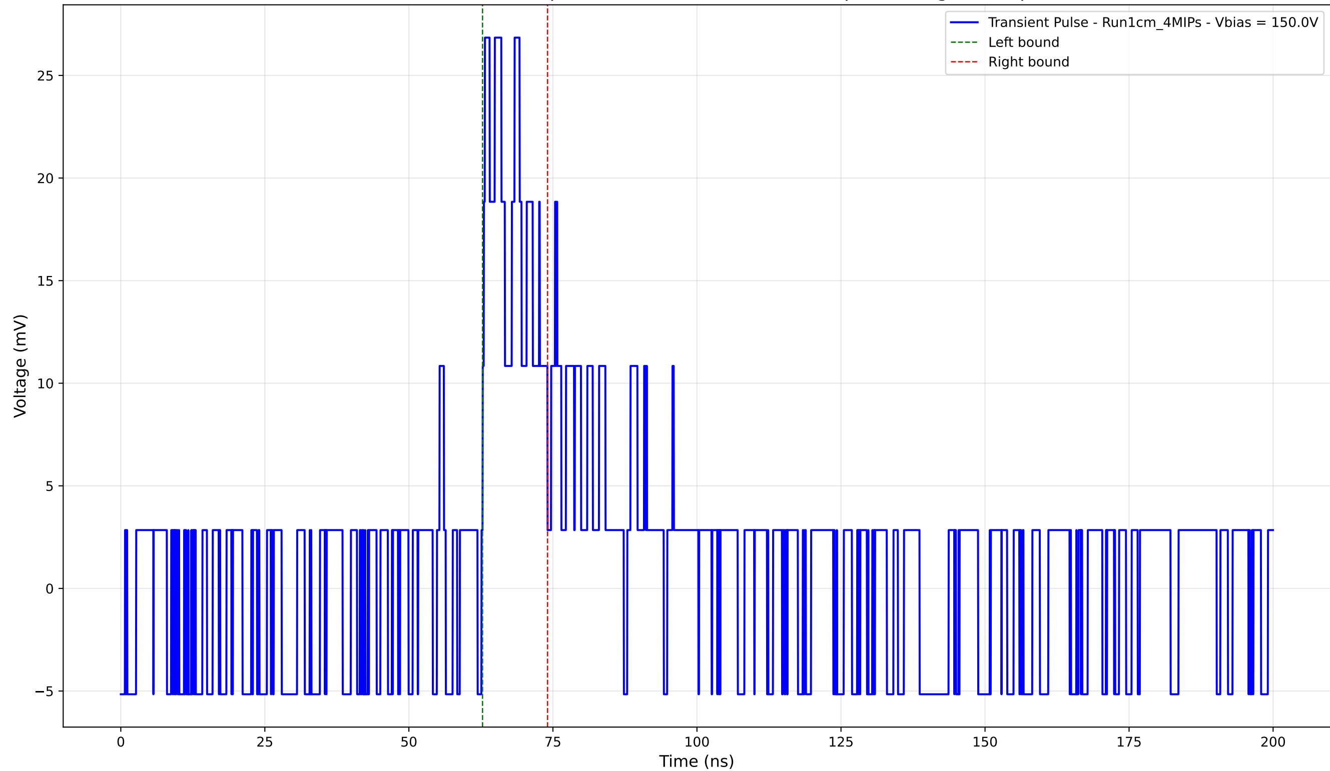
Transient Pulse - Sample: new1cm - Position: 3745.0 \mu\text{m} - Charge: 3.95 pC
