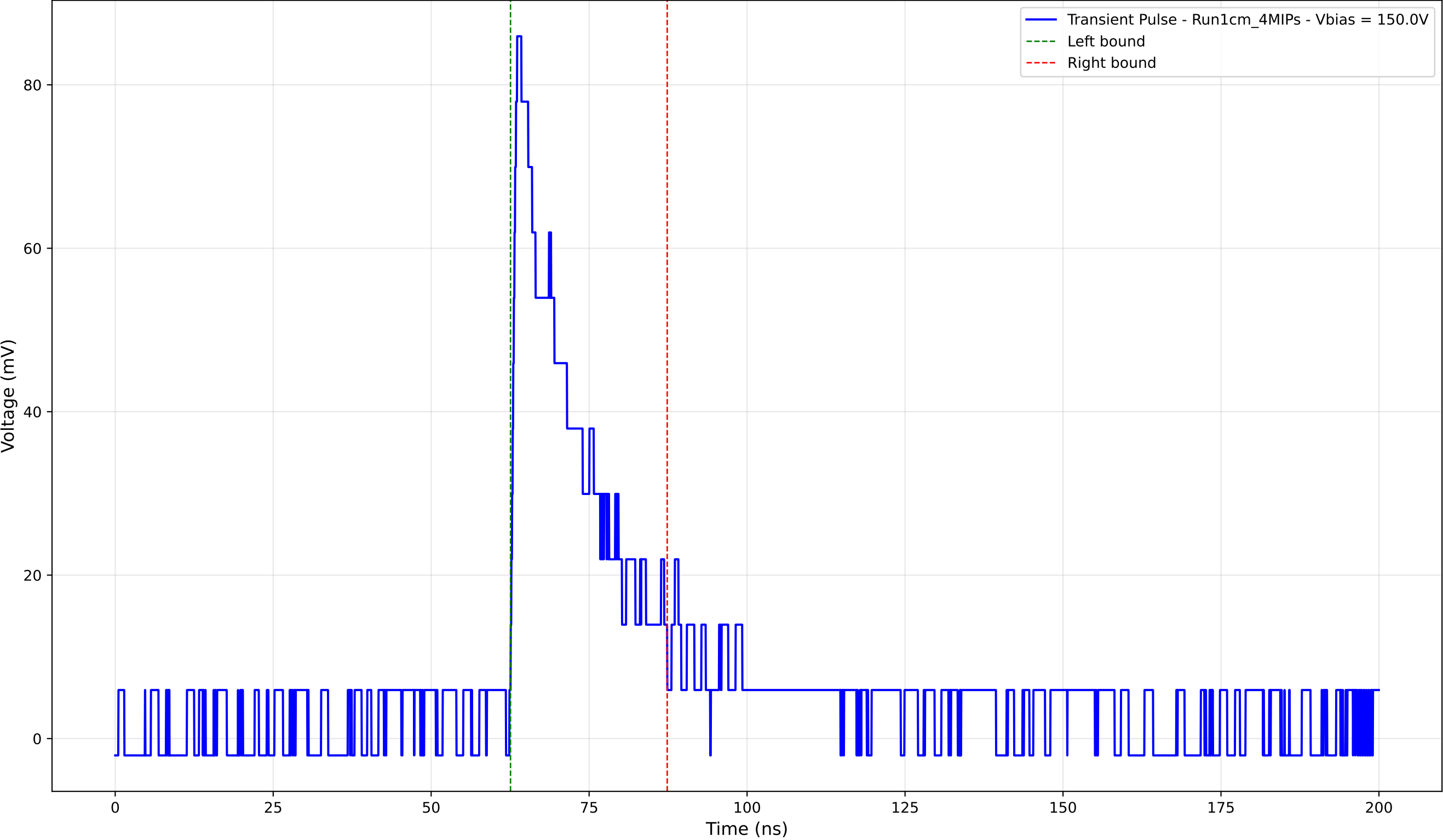
Transient Pulse - Sample: new1cm - Position: 4650.0 \mu\text{m} - Charge: 18.29 pC
