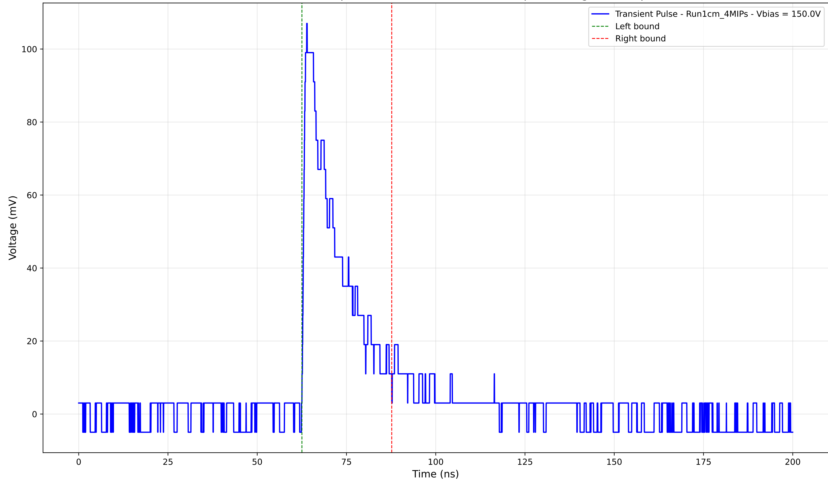
Transient Pulse - Sample: new1cm - Position: 4590.0 \mu\text{m} - Charge: 21.78 pC
