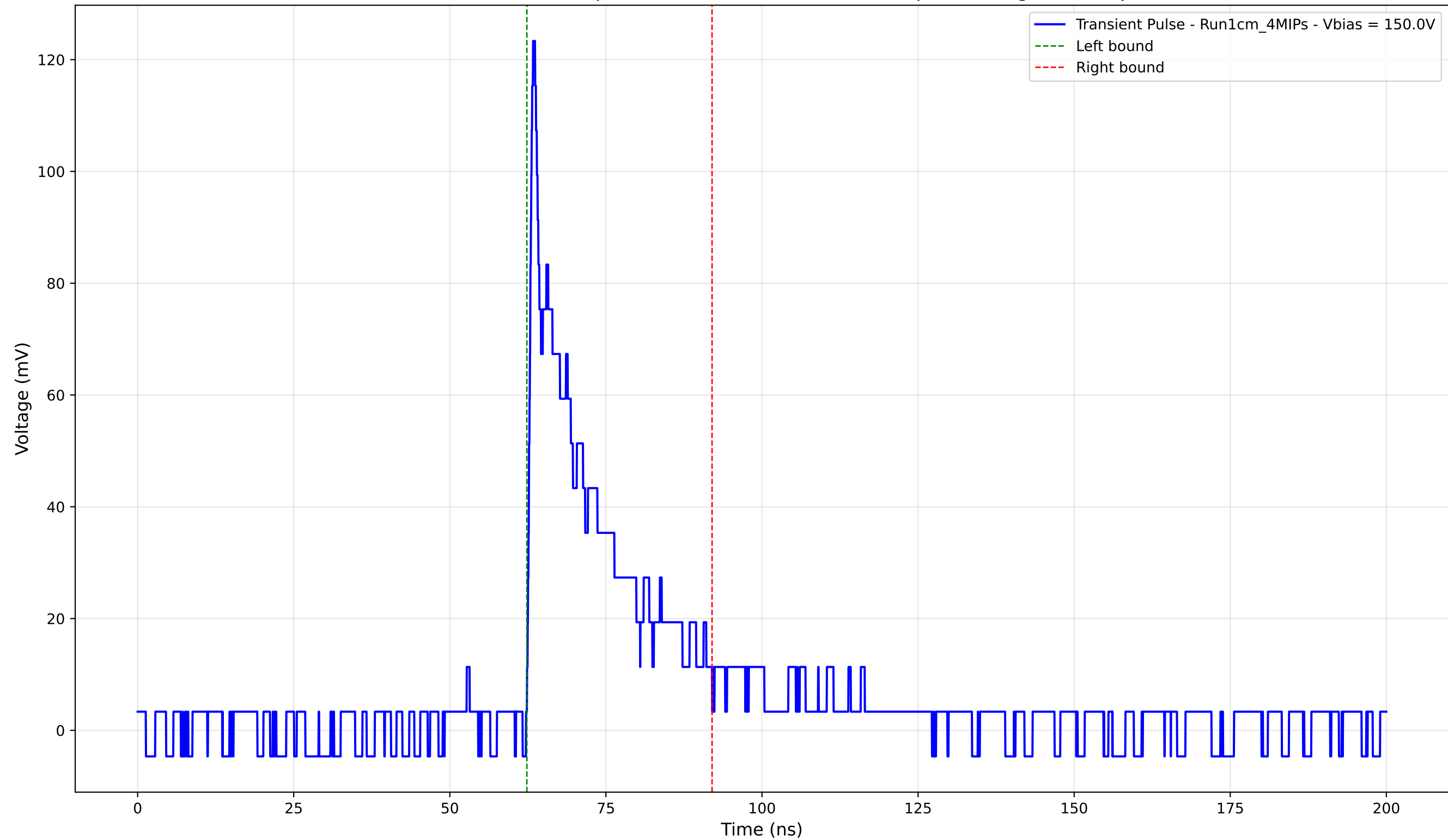
Transient Pulse - Sample: new1cm - Position: 3480.0 \mu\text{m} - Charge: 22.34 pC
