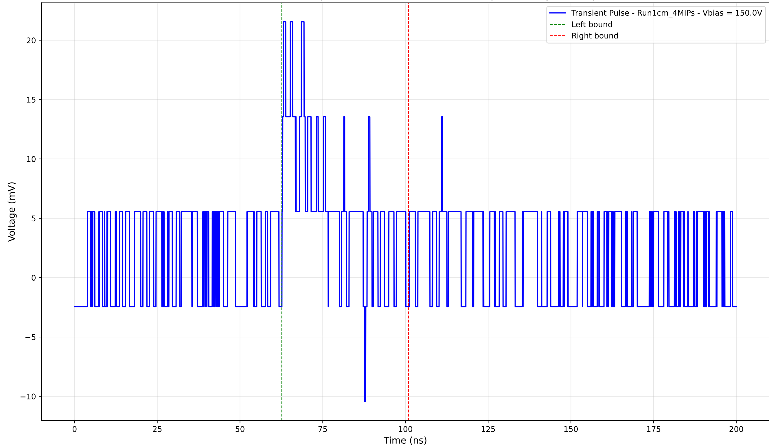
Transient Pulse - Sample: new1cm - Position: 4715.0 \mu\text{m} - Charge: 4.83 pC
