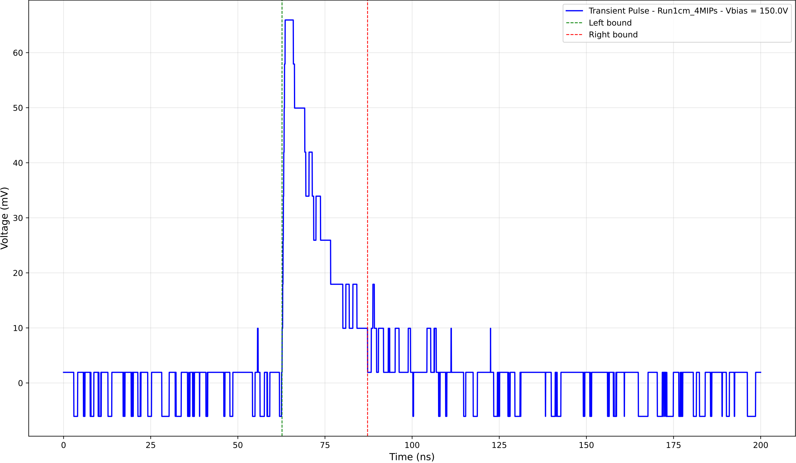
Transient Pulse - Sample: new1cm - Position: 4160.0 \mu\text{m} - Charge: 14.71 pC
