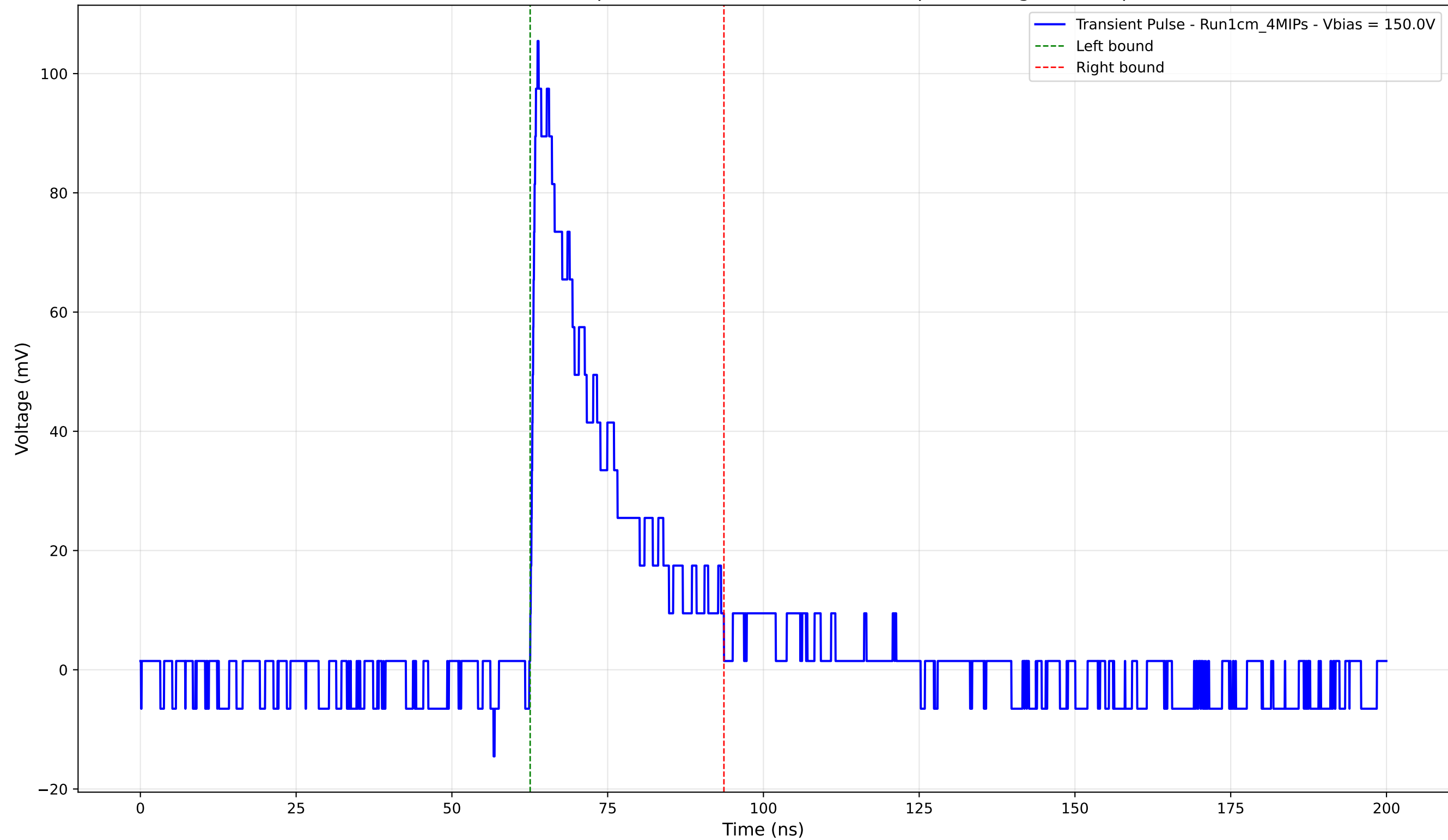
Transient Pulse - Sample: new1cm - Position: 3850.0 \mu\text{m} - Charge: 22.88 pC
