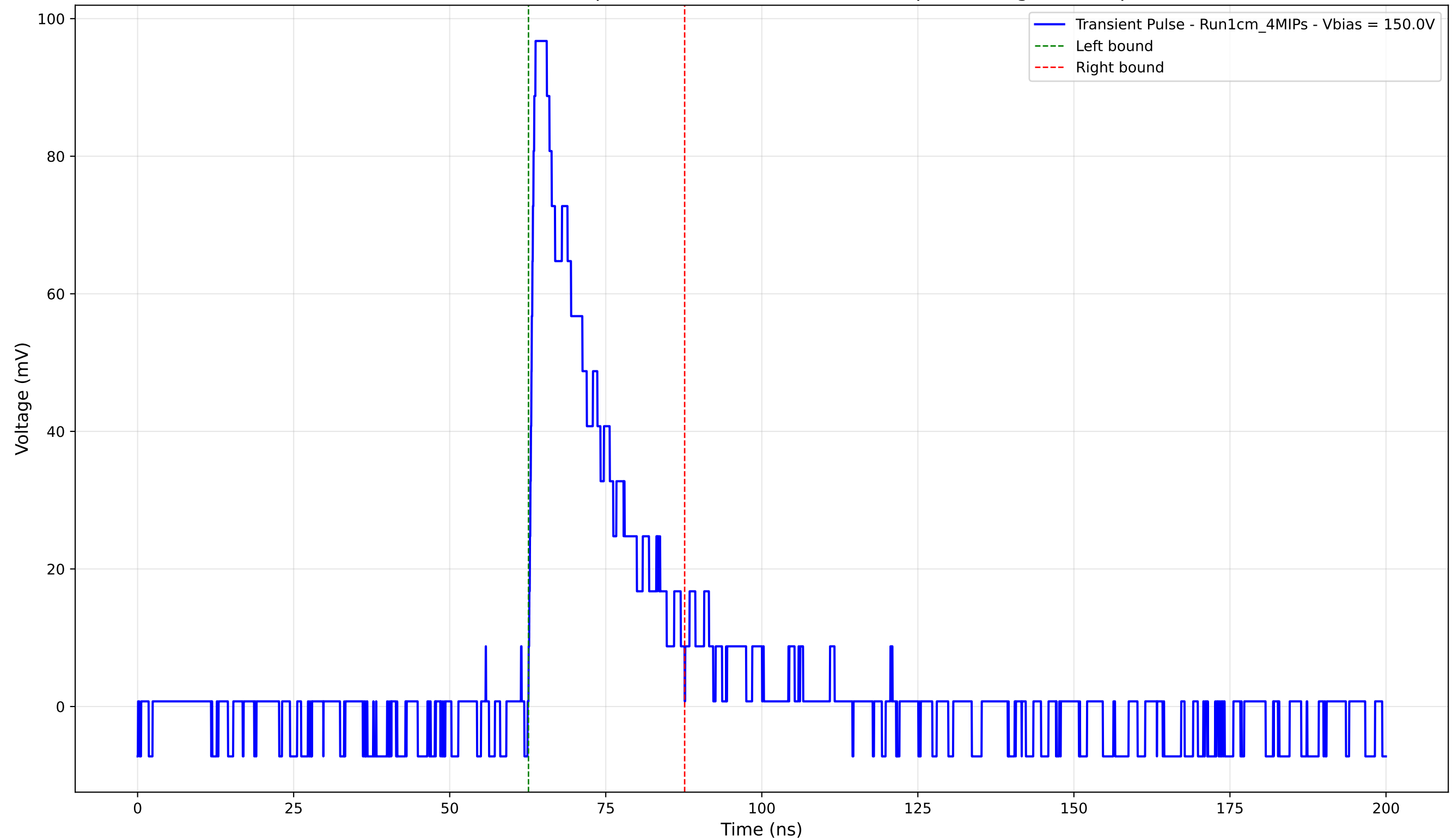
Transient Pulse - Sample: new1cm - Position: 4365.0 \mu\text{m} - Charge: 21.00 pC
