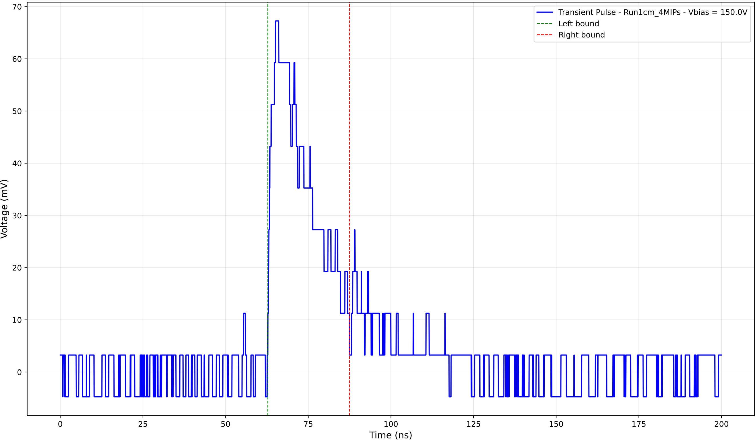
Transient Pulse - Sample: new1cm - Position: 2075.0 \mu\text{m} - Charge: 17.88 pC
