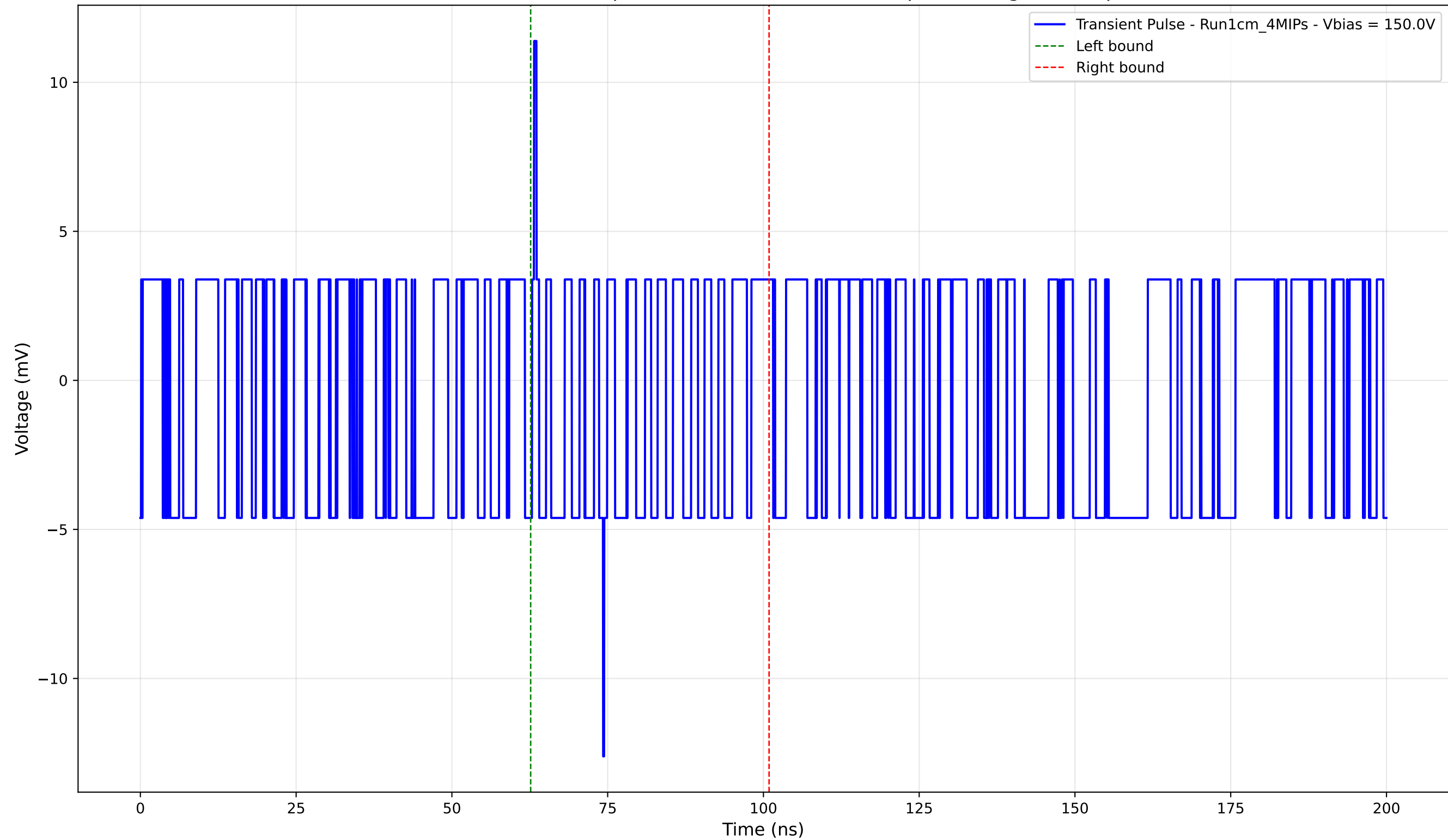
Transient Pulse - Sample: new1cm - Position: 30.0 \mu\text{m} - Charge: -0.34 pC
