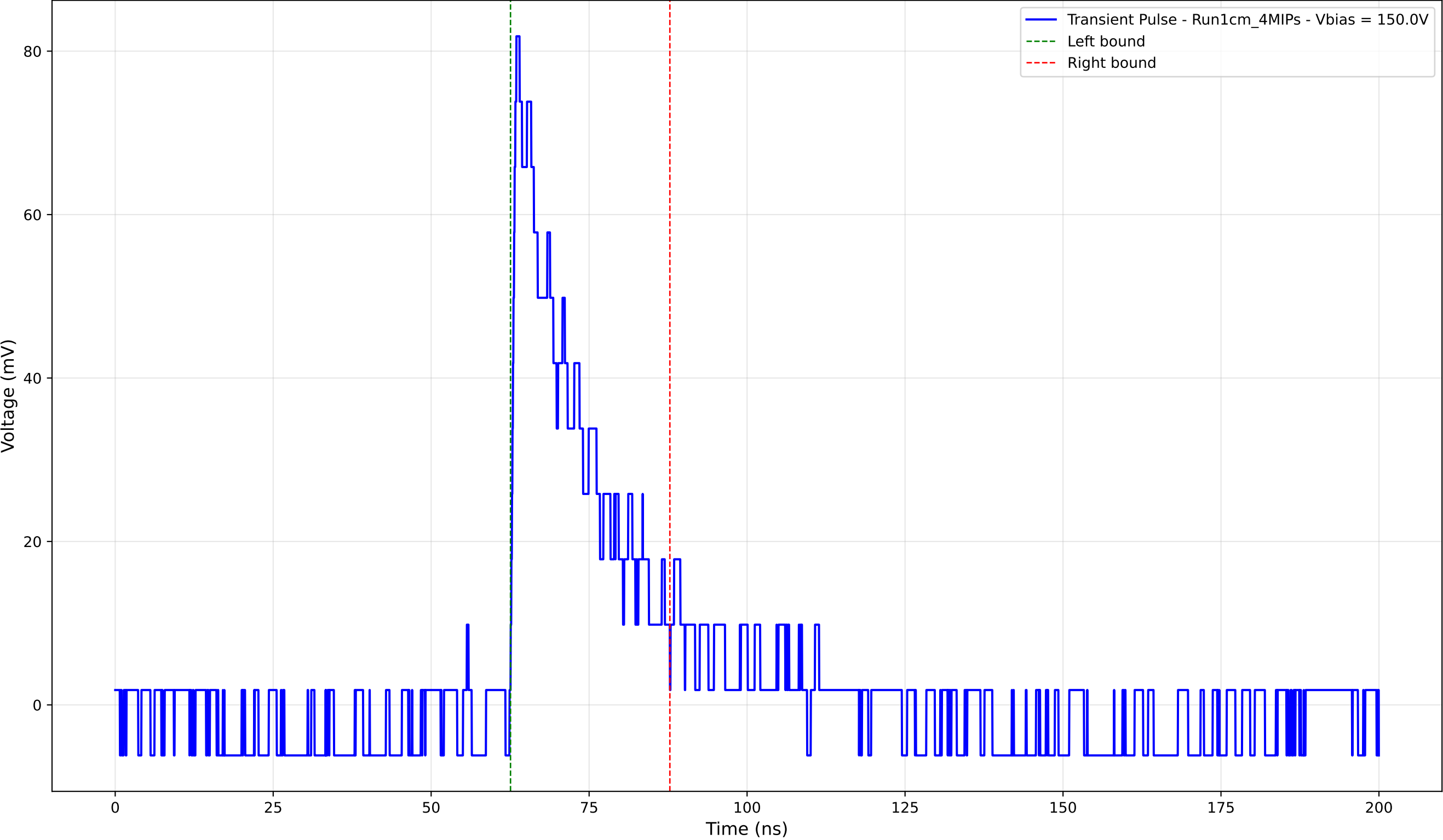
Transient Pulse - Sample: new1cm - Position: 3795.0 \mu\text{m} - Charge: 17.13 pC
