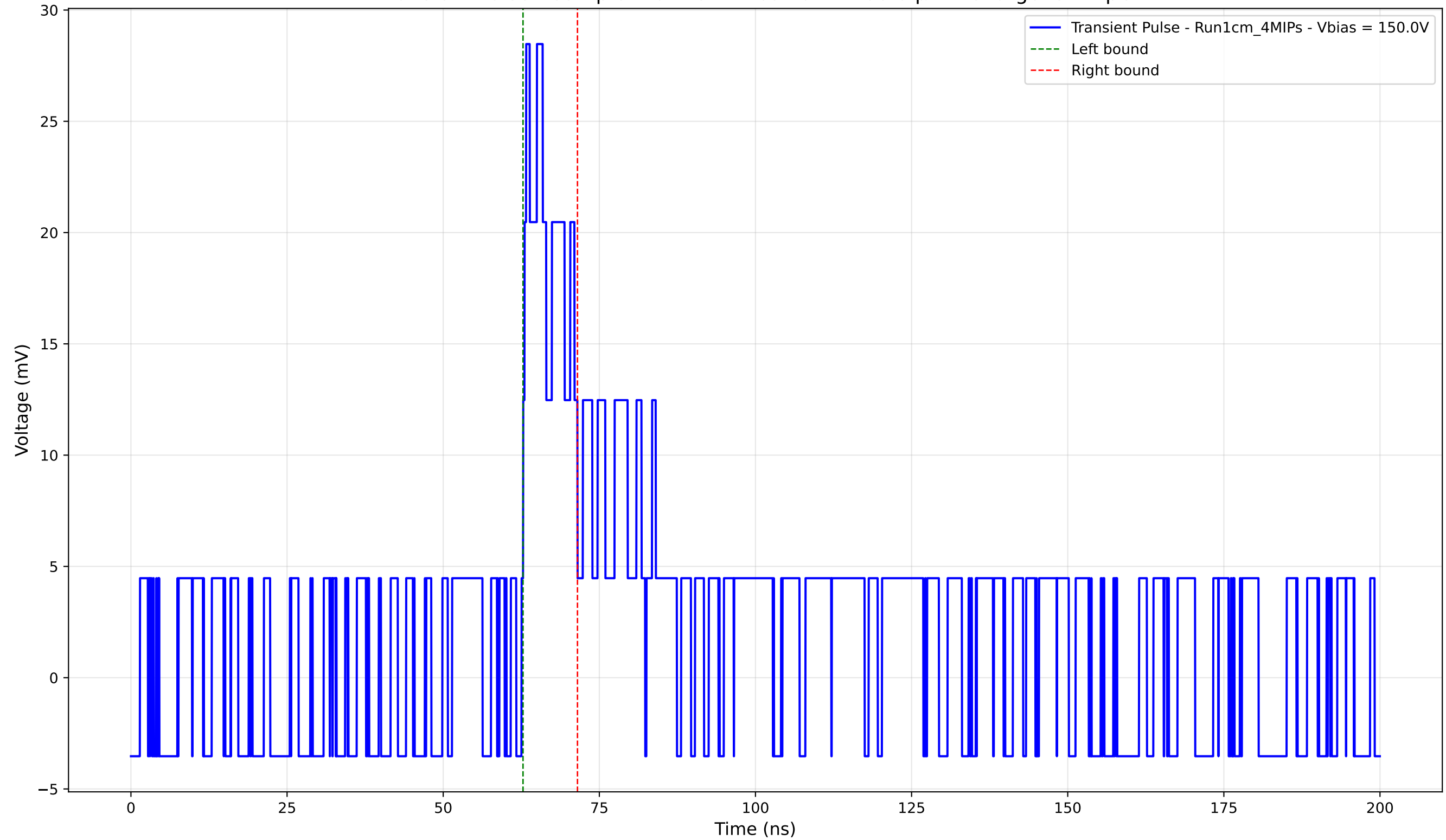
Transient Pulse - Sample: new1cm - Position: 4700.0 \mu\text{m} - Charge: 3.41 pC
