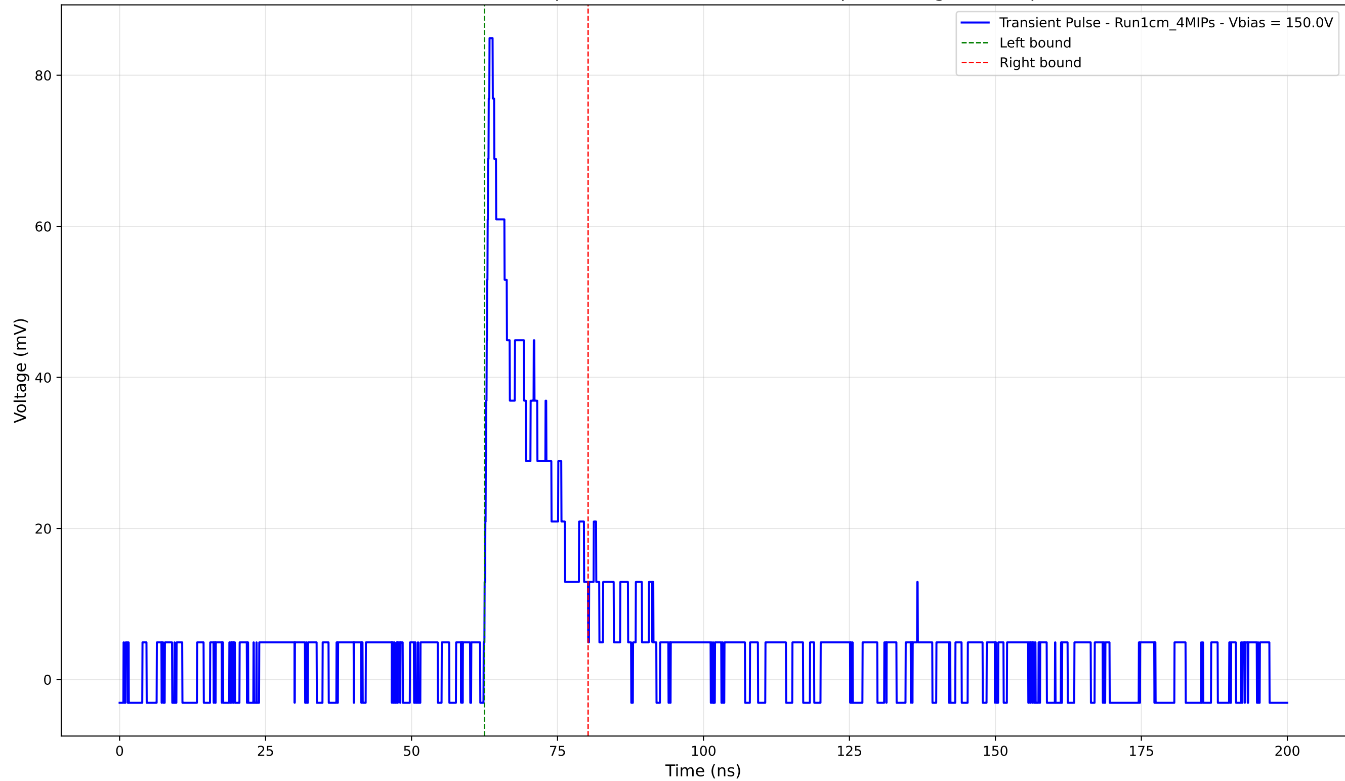
Transient Pulse - Sample: new1cm -Position: 275.0 \mu\text{m} - Charge: 12.47 pC
