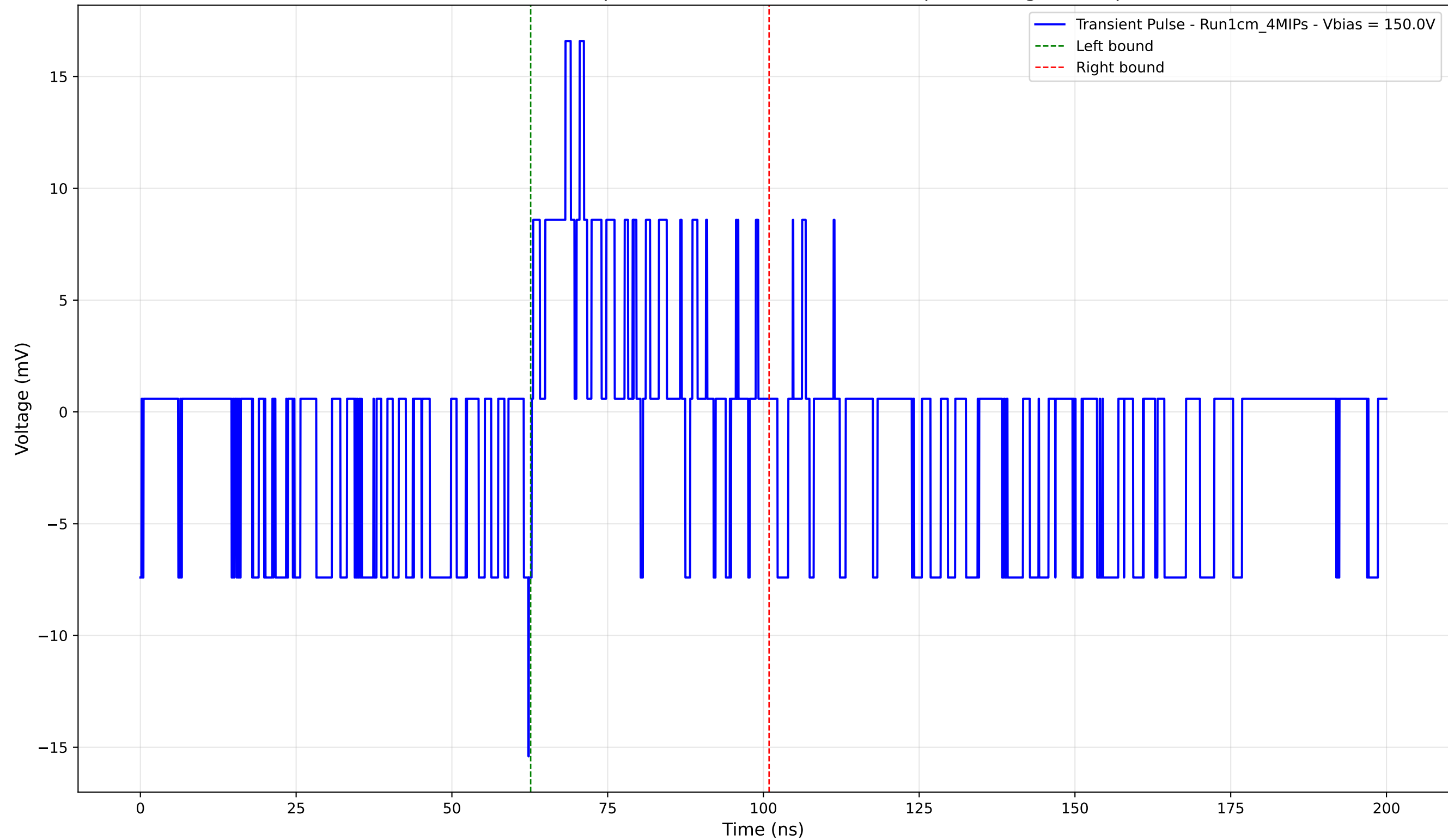
Transient Pulse - Sample: new1cm - Position: 1720.0 \mu\text{m} - Charge: 2.77 pC
