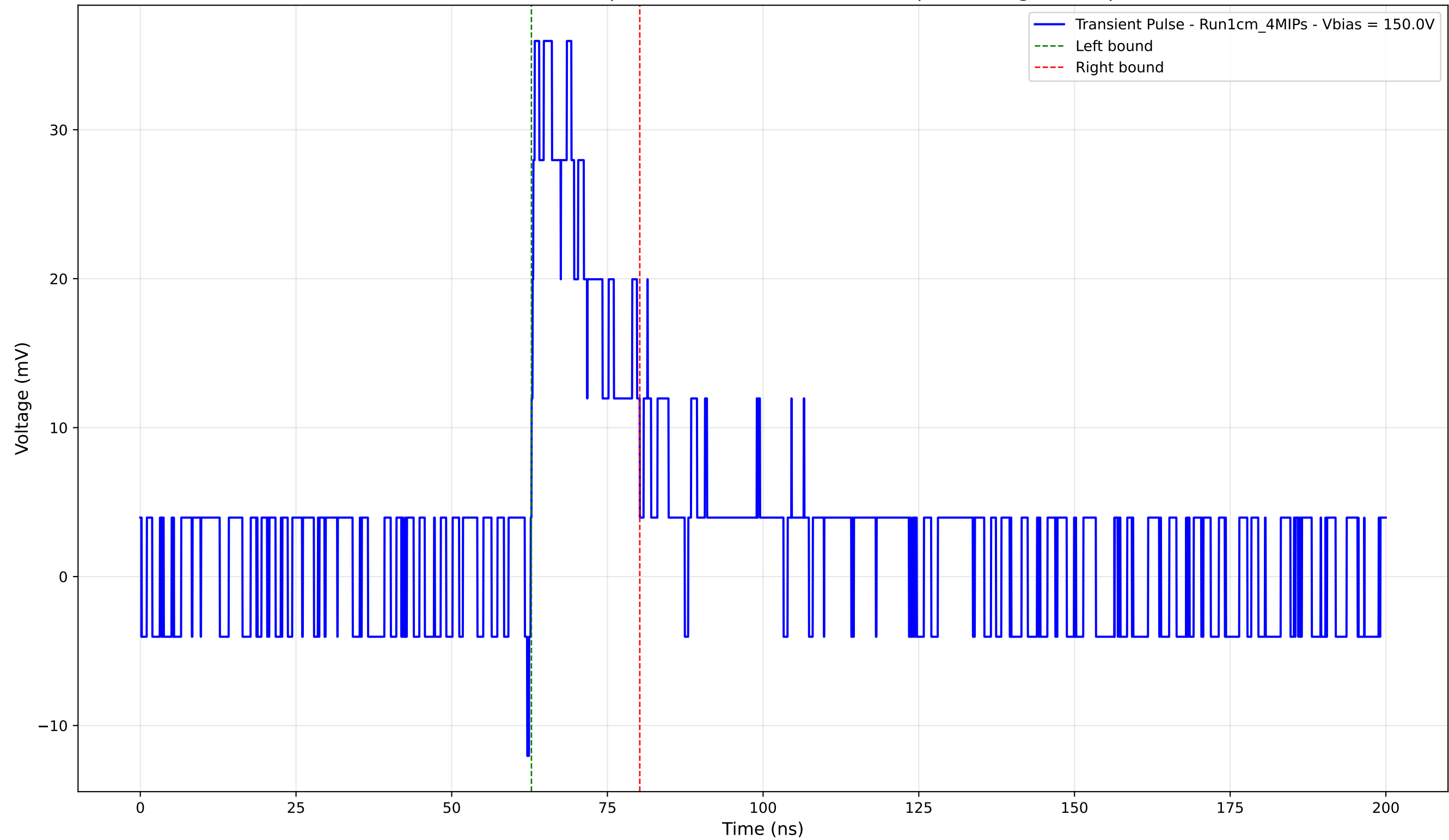
Transient Pulse - Sample: new1cm - Position: 740.0 \mu\text{m} - Charge: 7.85 pC
