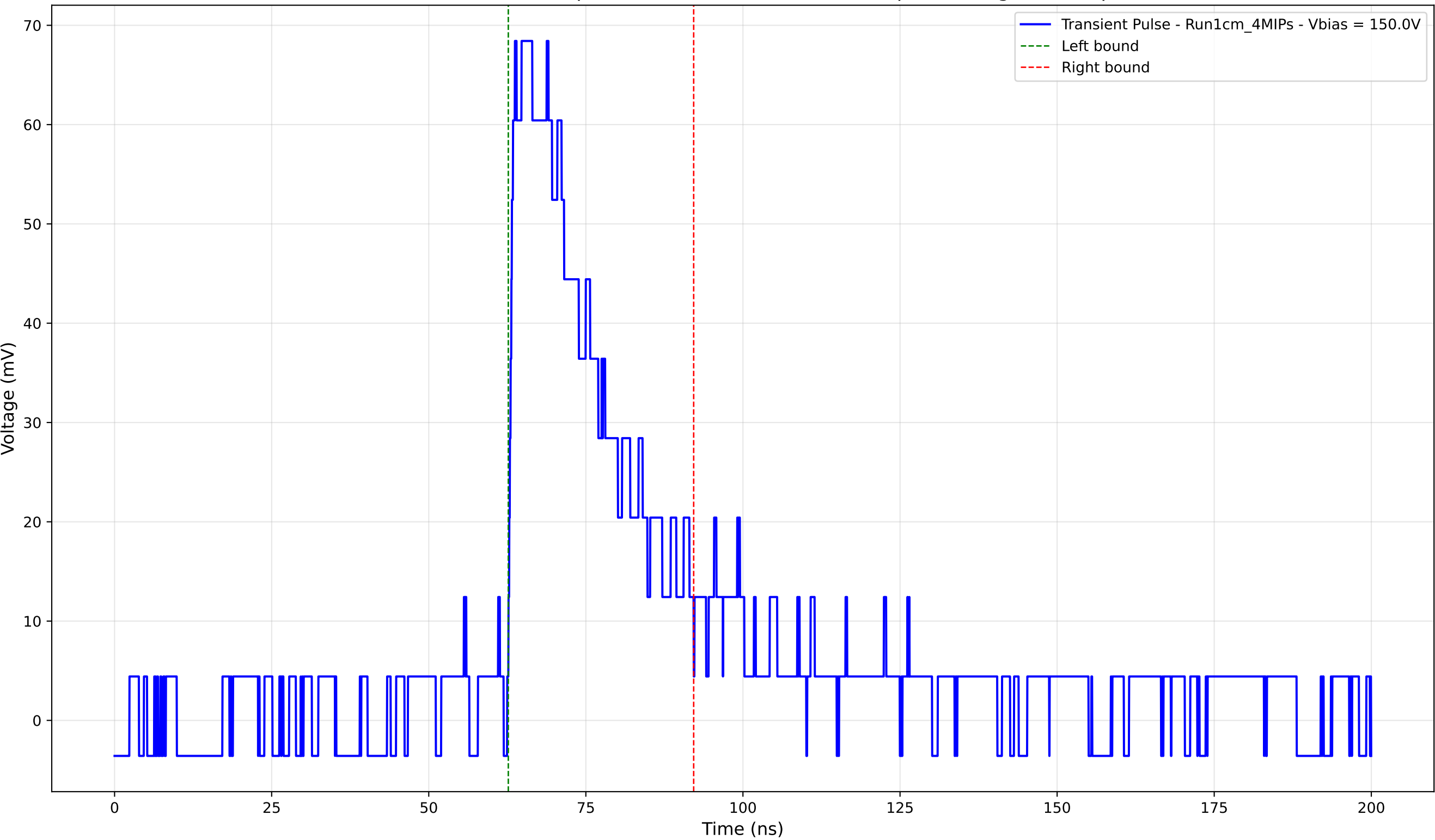
Transient Pulse - Sample: new1cm - Position: 2400.0 \mu\text{m} - Charge: 21.44 pC
