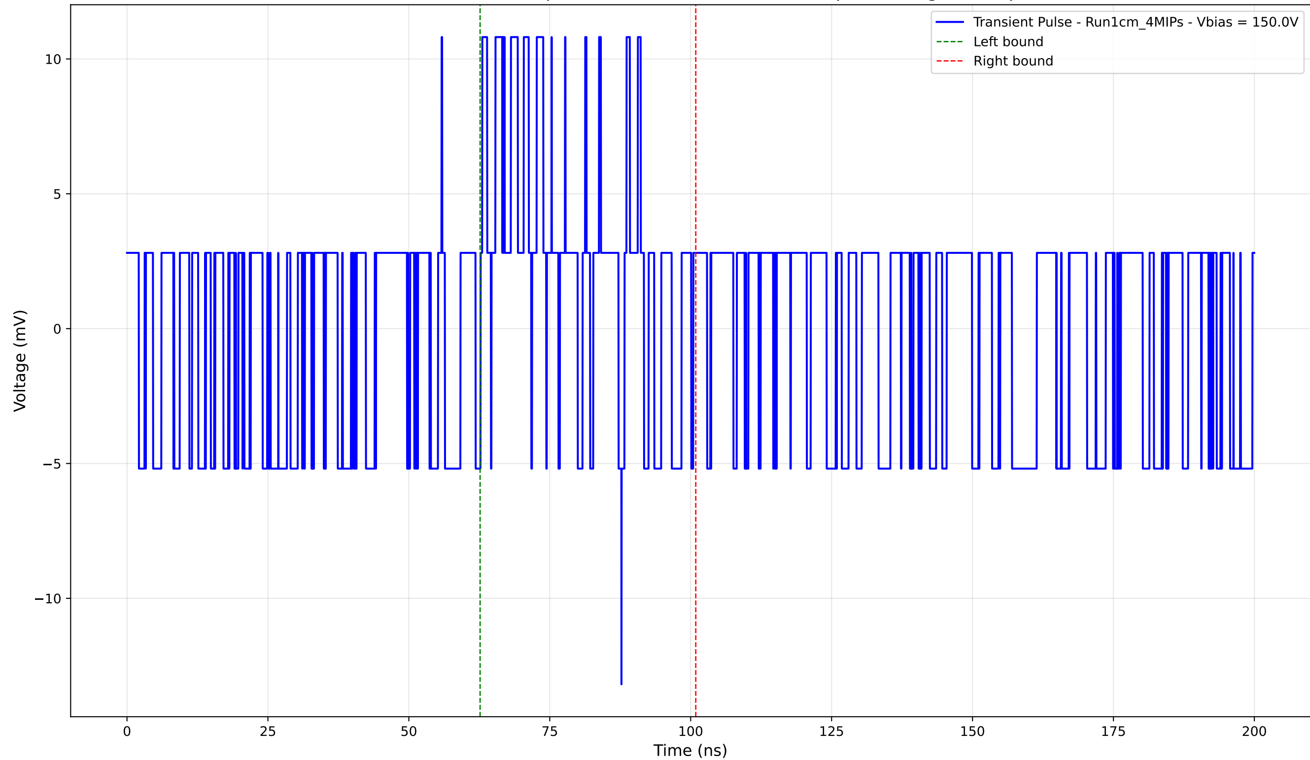
Transient Pulse - Sample: new1cm - Position: 1710.0 \mu\text{m} - Charge: 2.18 pC
