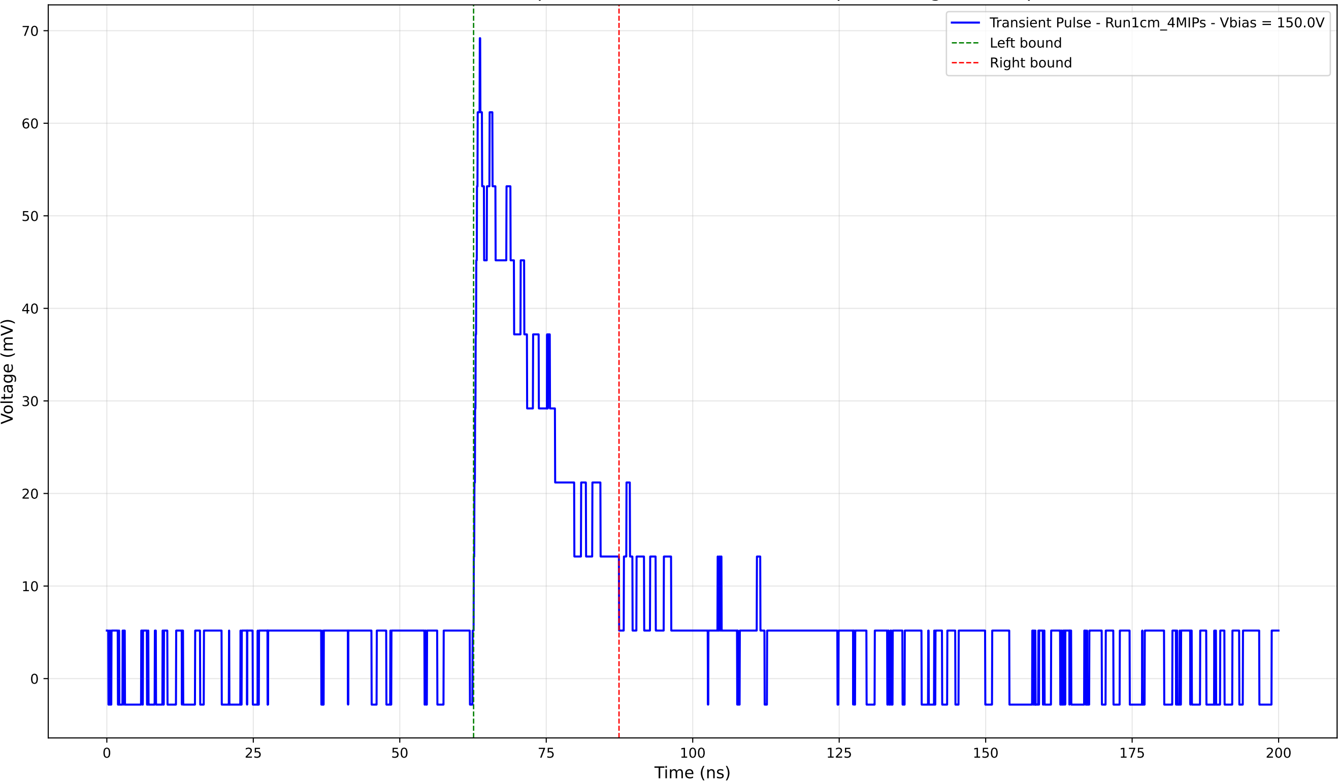
Transient Pulse - Sample: new1cm - Position: 2630.0 \mu\text{m} - Charge: 15.33 pC
