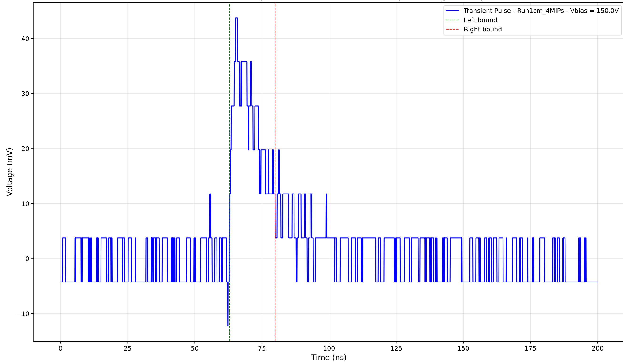
Transient Pulse - Sample: new1cm - Position: 1135.0 \mu\text{m} - Charge: 8.38 pC
