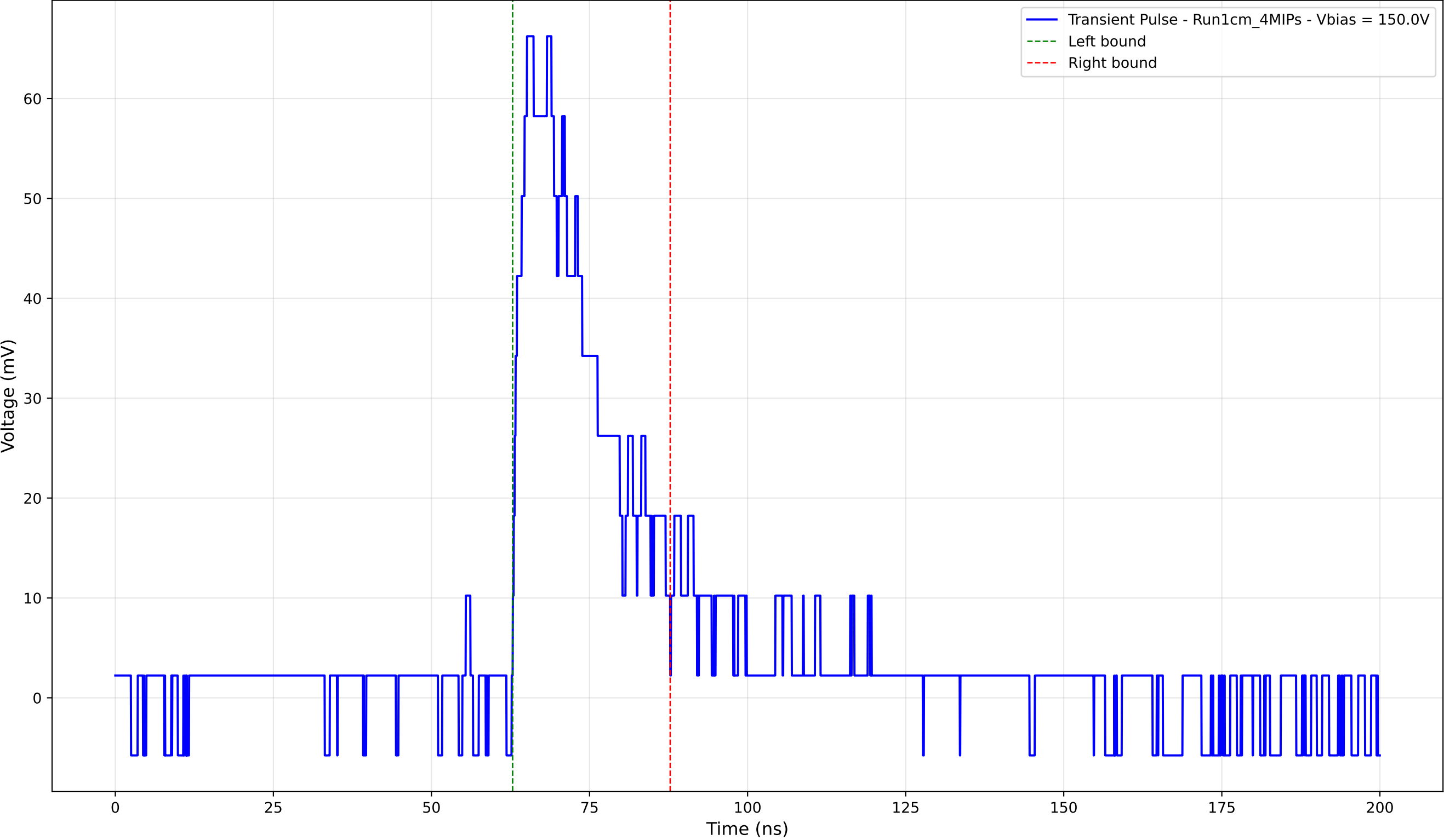
Transient Pulse - Sample: new1cm - Position: 2010.0 \mu\text{m} - Charge: 17.66 pC
