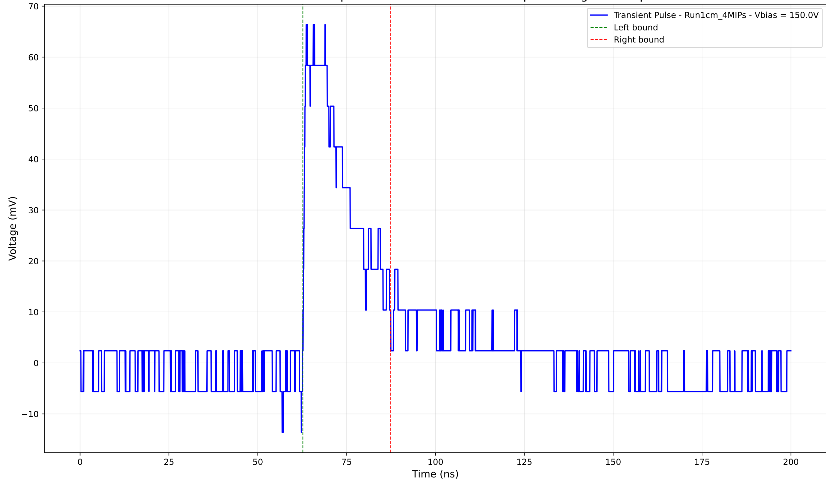
Transient Pulse - Sample: new1cm - Position: 2425.0 \mu\text{m} - Charge: 17.83 pC
