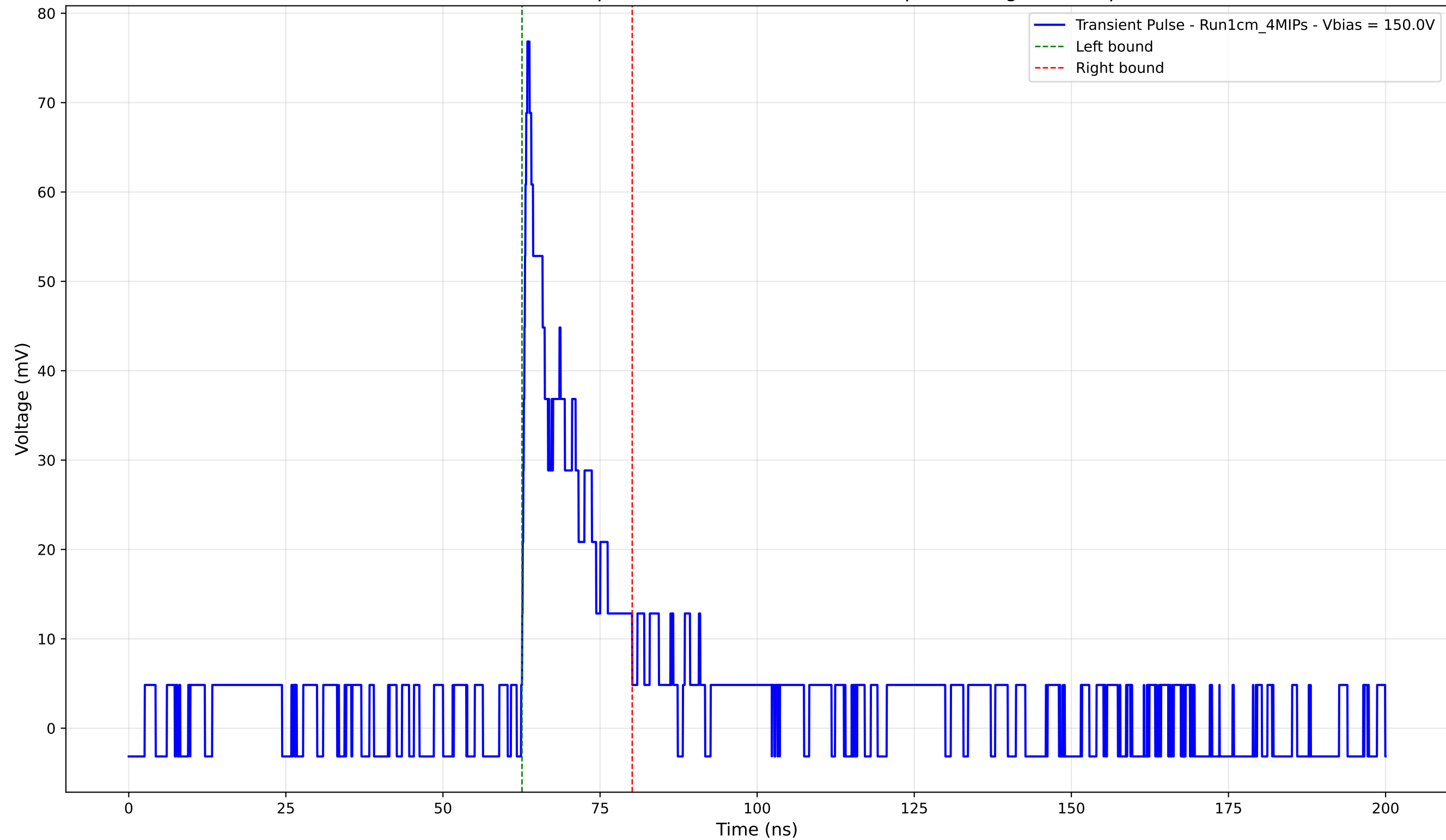
Transient Pulse - Sample: new1cm -Position: 260.0 \mu\text{m} - Charge: 10.59 pC
