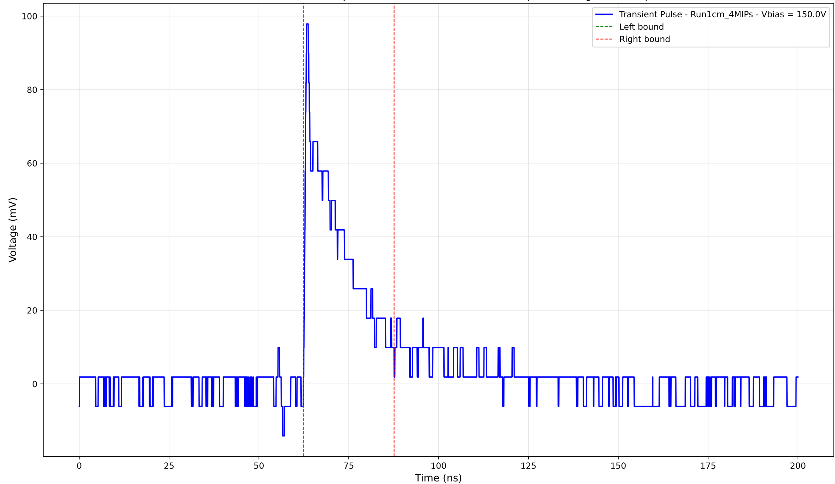
Transient Pulse - Sample: new1cm - Position: 2855.0 \mu\text{m} - Charge: 18.56 pC
