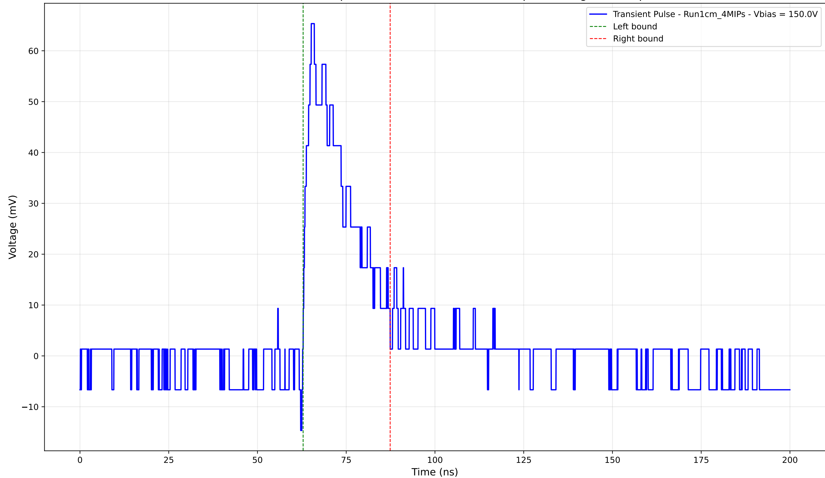
Transient Pulse - Sample: new1cm - Position: 1315.0 \mu\text{m} - Charge: 15.81 pC
