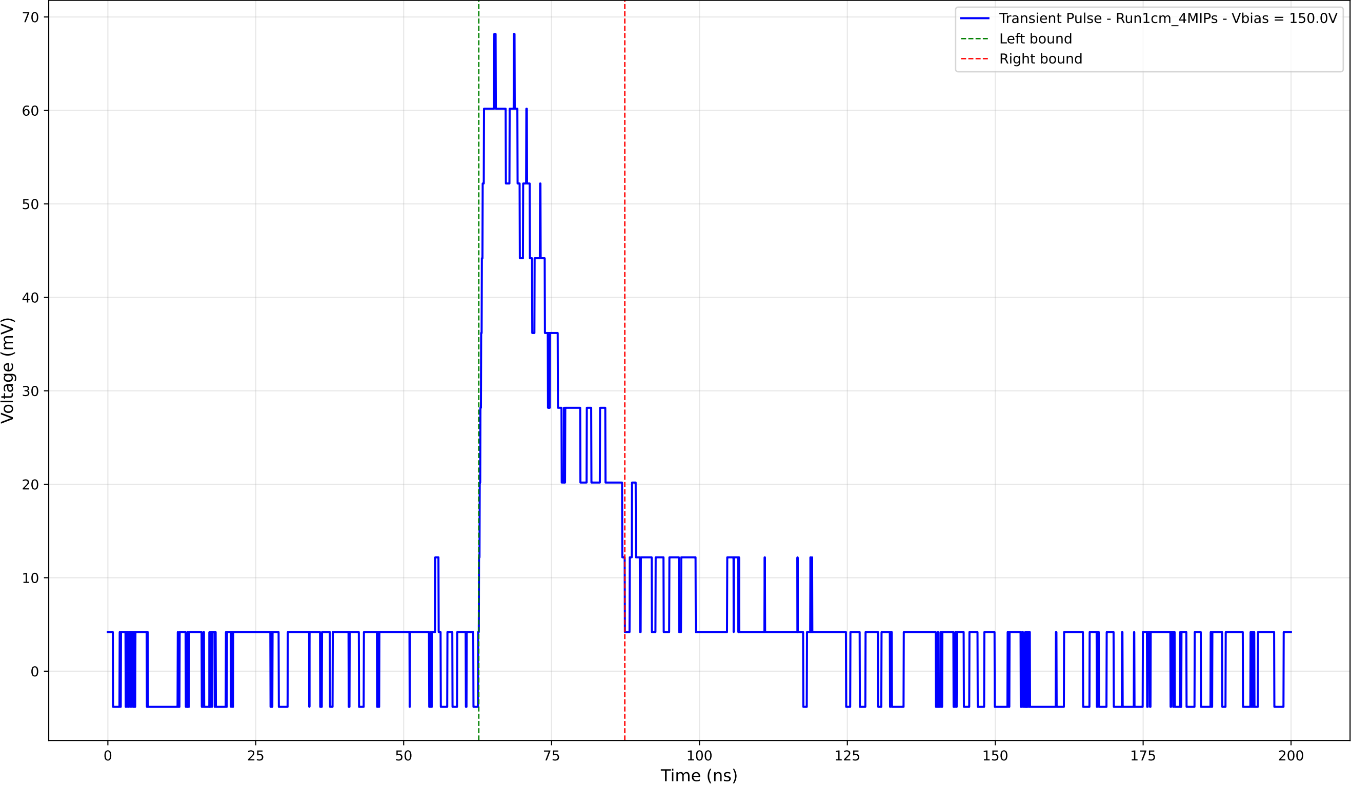
Transient Pulse - Sample: new1cm - Position: 2335.0 \mu\text{m} - Charge: 18.53 pC
