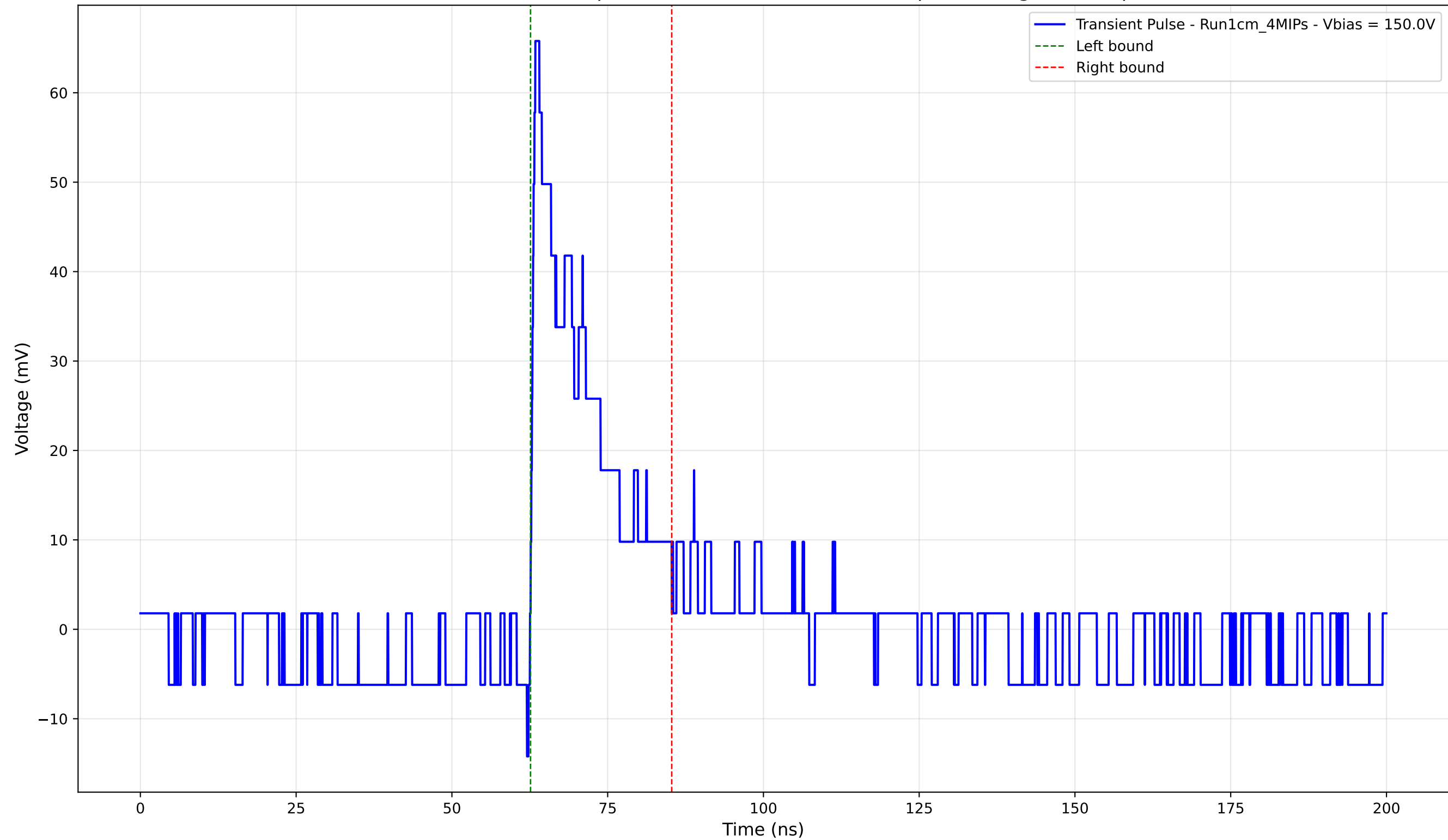
Transient Pulse - Sample: new1cm - Position: 4800.0 \mu\text{m} - Charge: 11.38 pC
