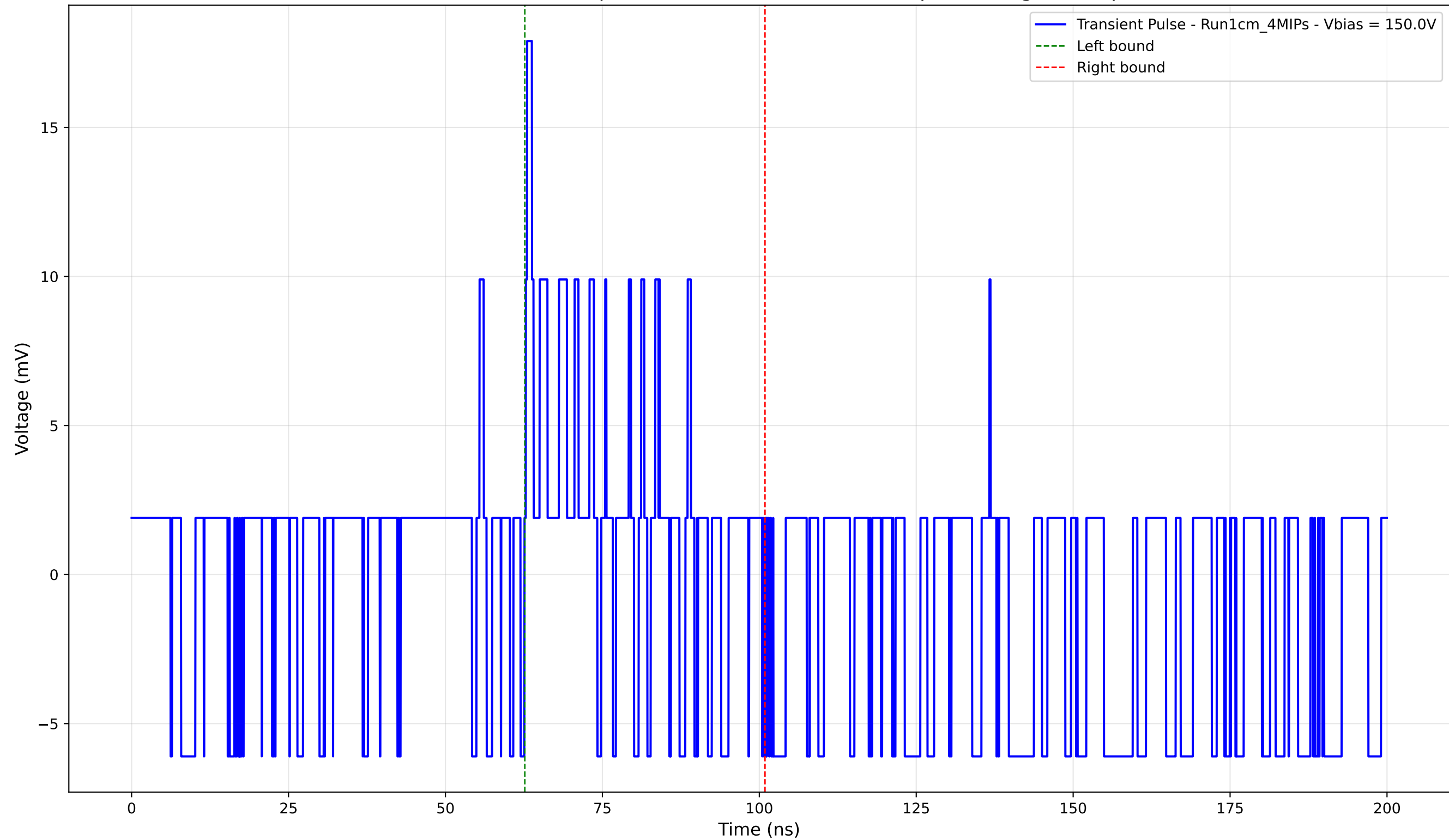
Transient Pulse - Sample: new1cm - Position: 3220.0 \mu\text{m} - Charge: 1.76 pC
