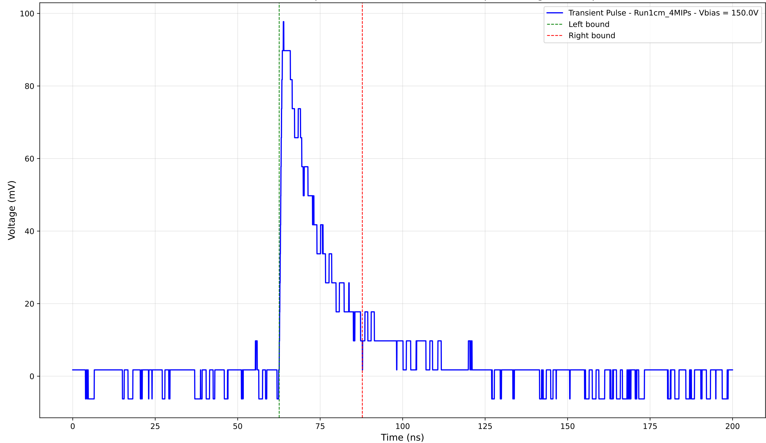
Transient Pulse - Sample: new1cm - Position: 3990.0 \mu\text{m} - Charge: 21.45 pC
