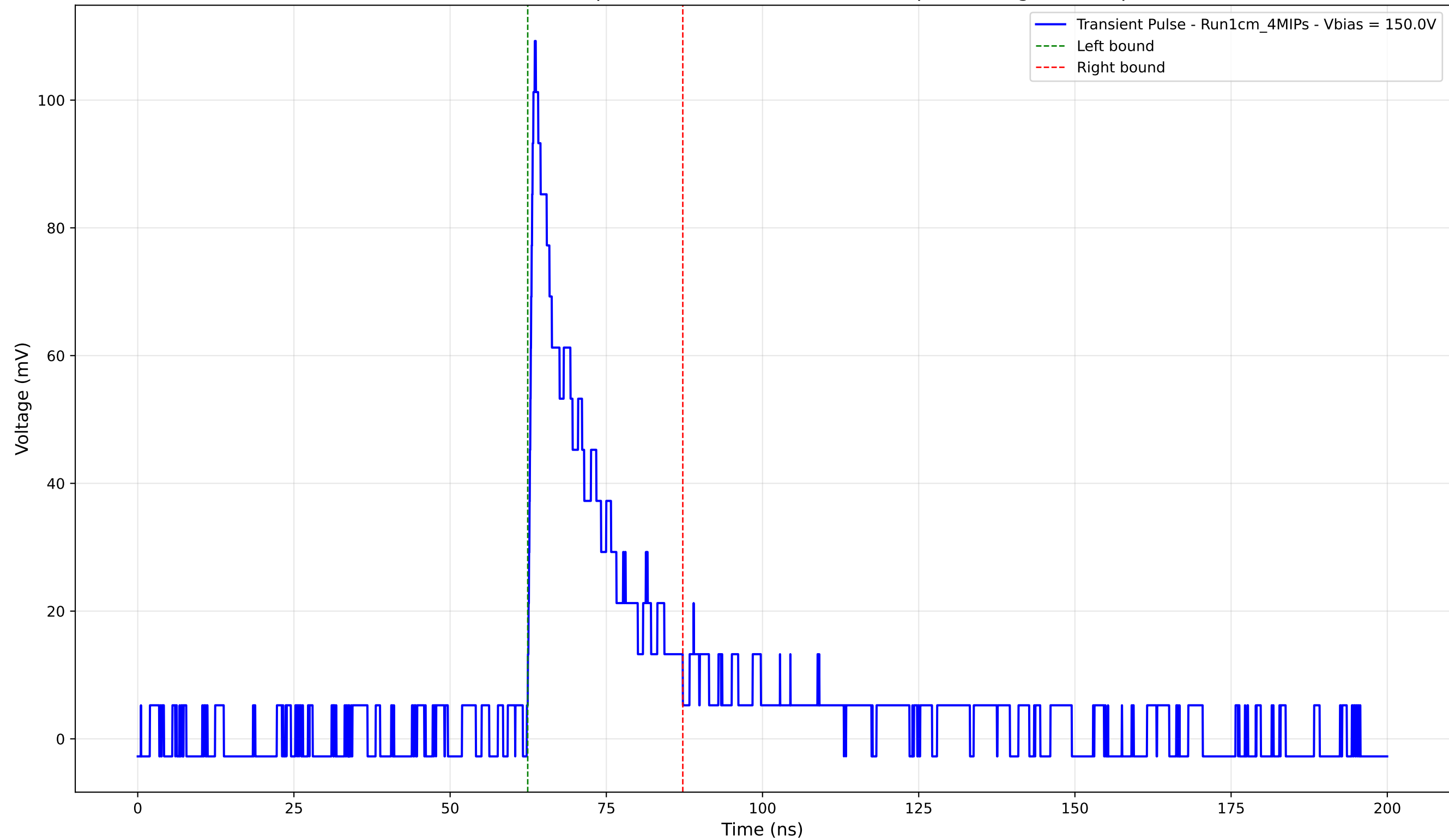
Transient Pulse - Sample: new1cm - Position: 4910.0 \mu\text{m} - Charge: 19.38 pC
