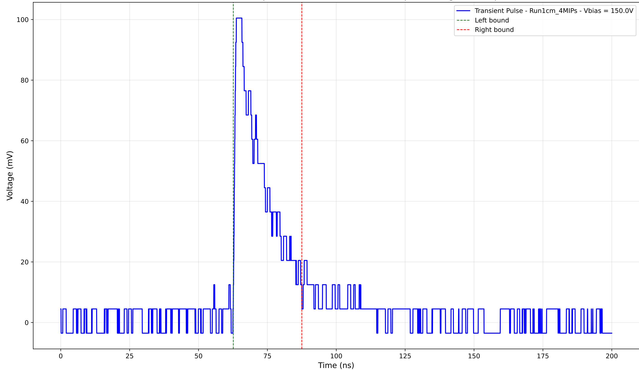
Transient Pulse - Sample: new1cm - Position: 4380.0 \mu\text{m} - Charge: 23.51 pC
