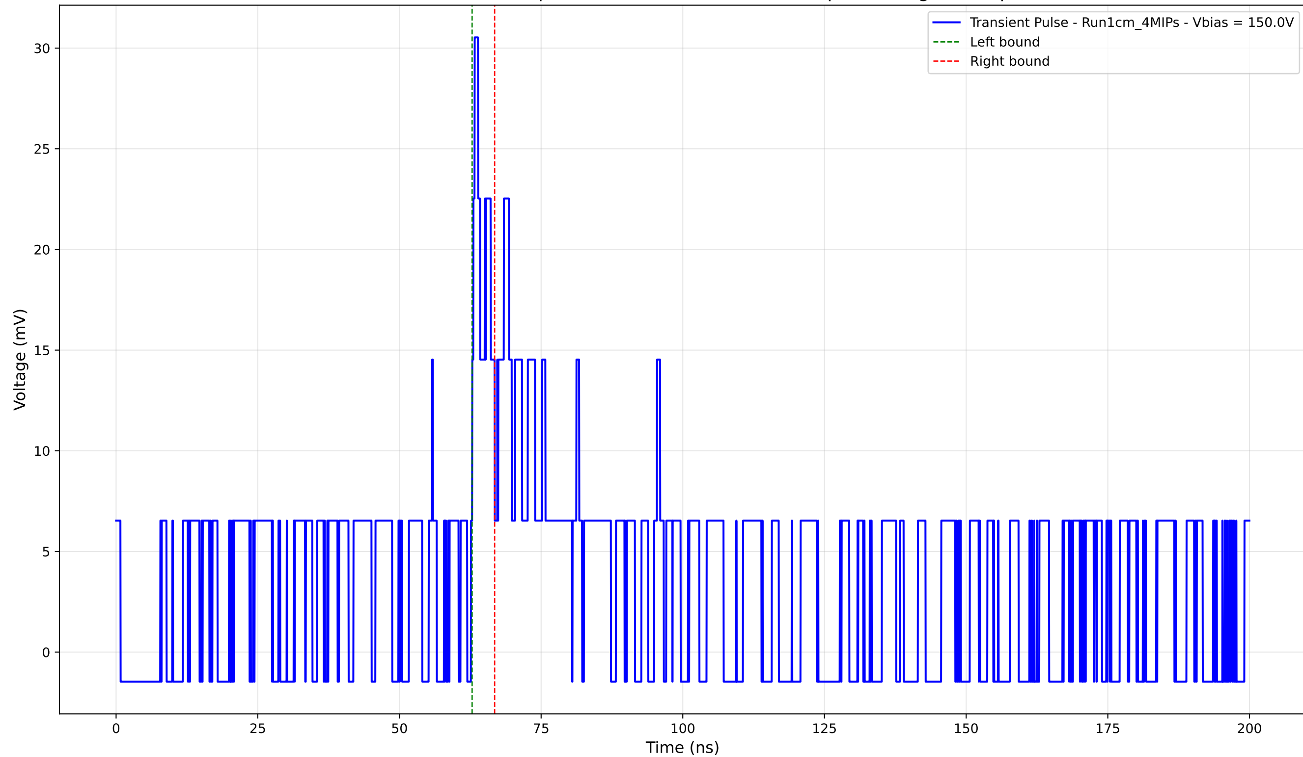
Transient Pulse - Sample: new1cm -Position: 4750.0 \mu\text{m} - Charge: 1.60 pC
