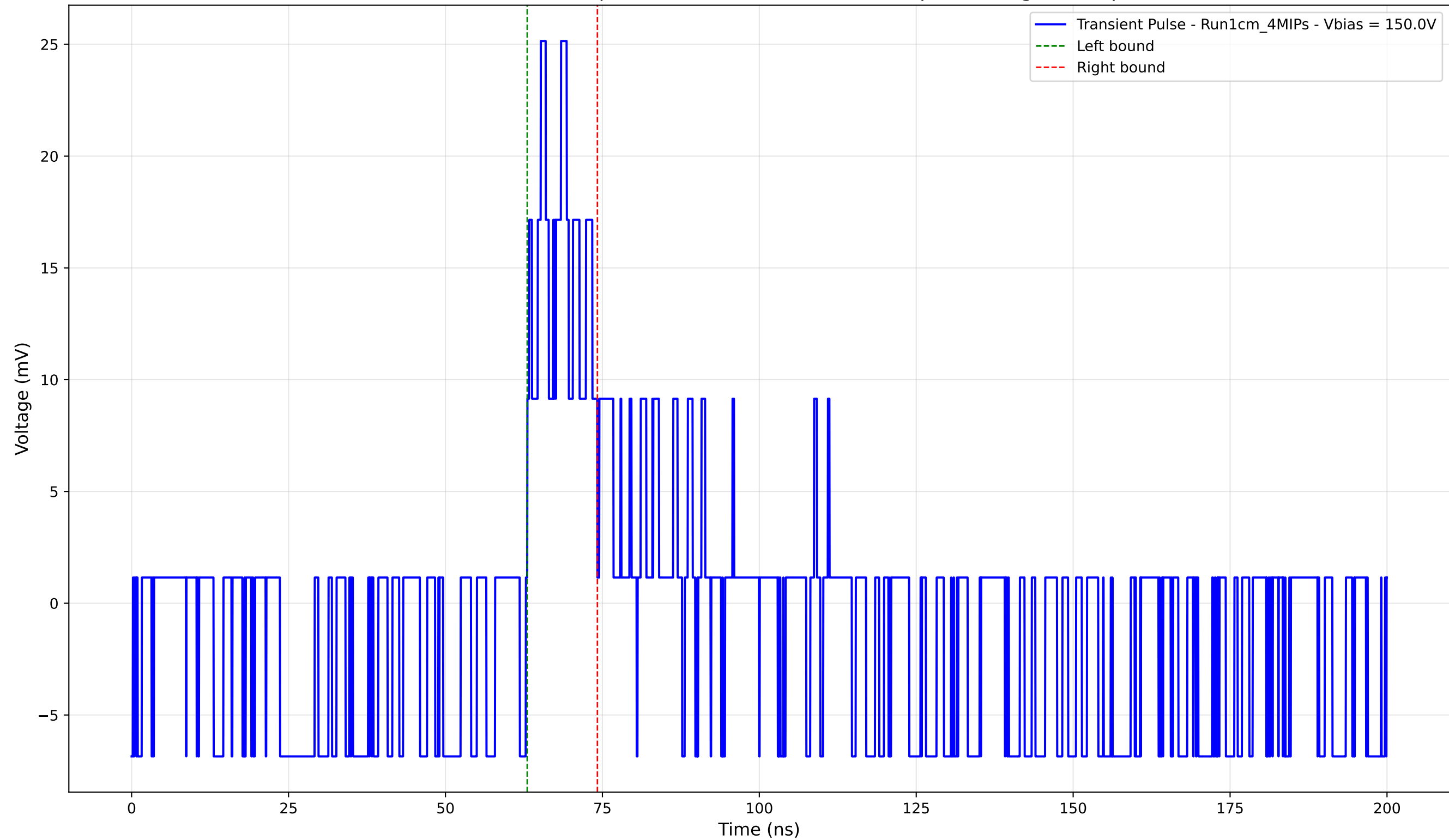
Transient Pulse - Sample: new1cm - Position: 1230.0 \mu\text{m} - Charge: 3.38 pC
