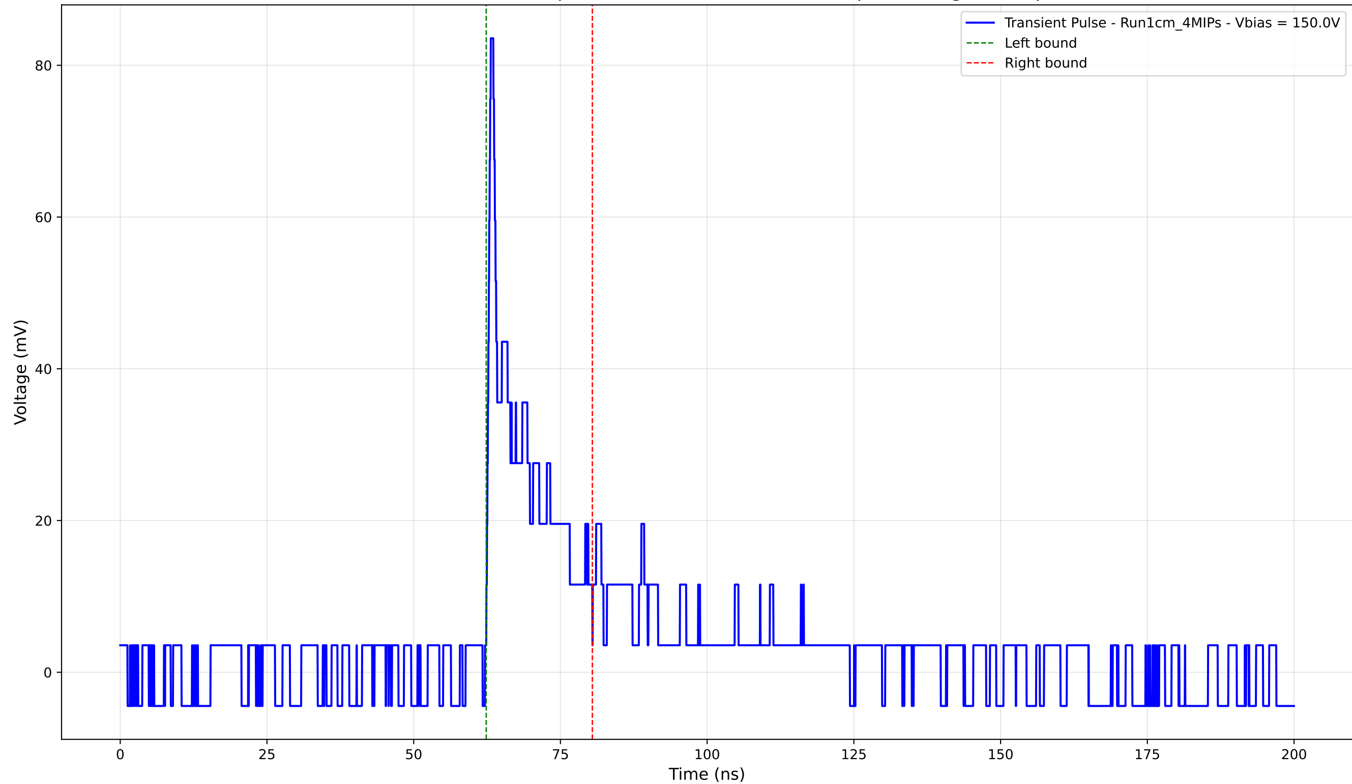
Transient Pulse - Sample: new1cm -Position: 3160.0 \mu\text{m} - Charge: 9.79 pC
