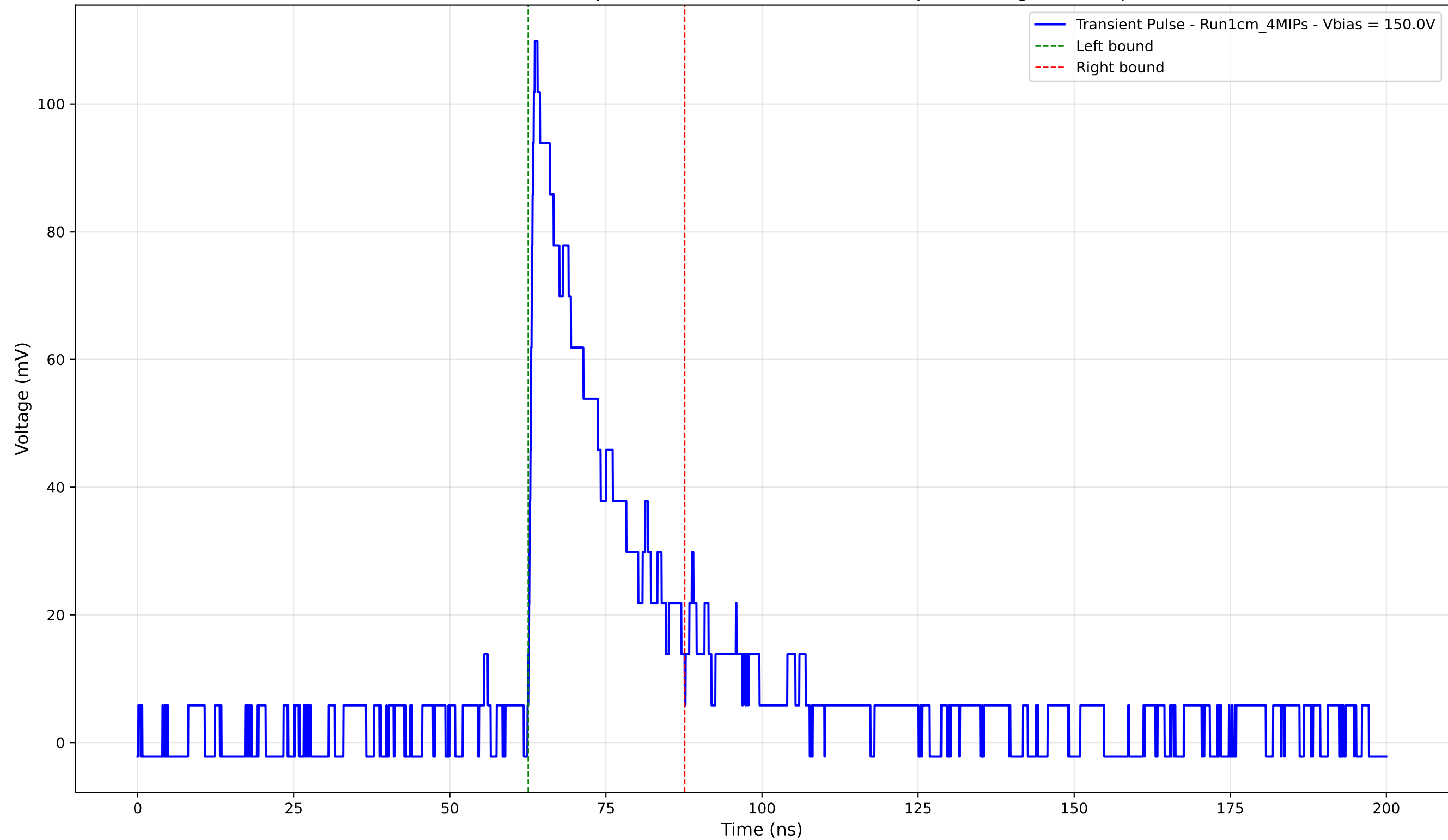
Transient Pulse - Sample: new1cm - Position: 3860.0 \mu\text{m} - Charge: 24.51 pC
