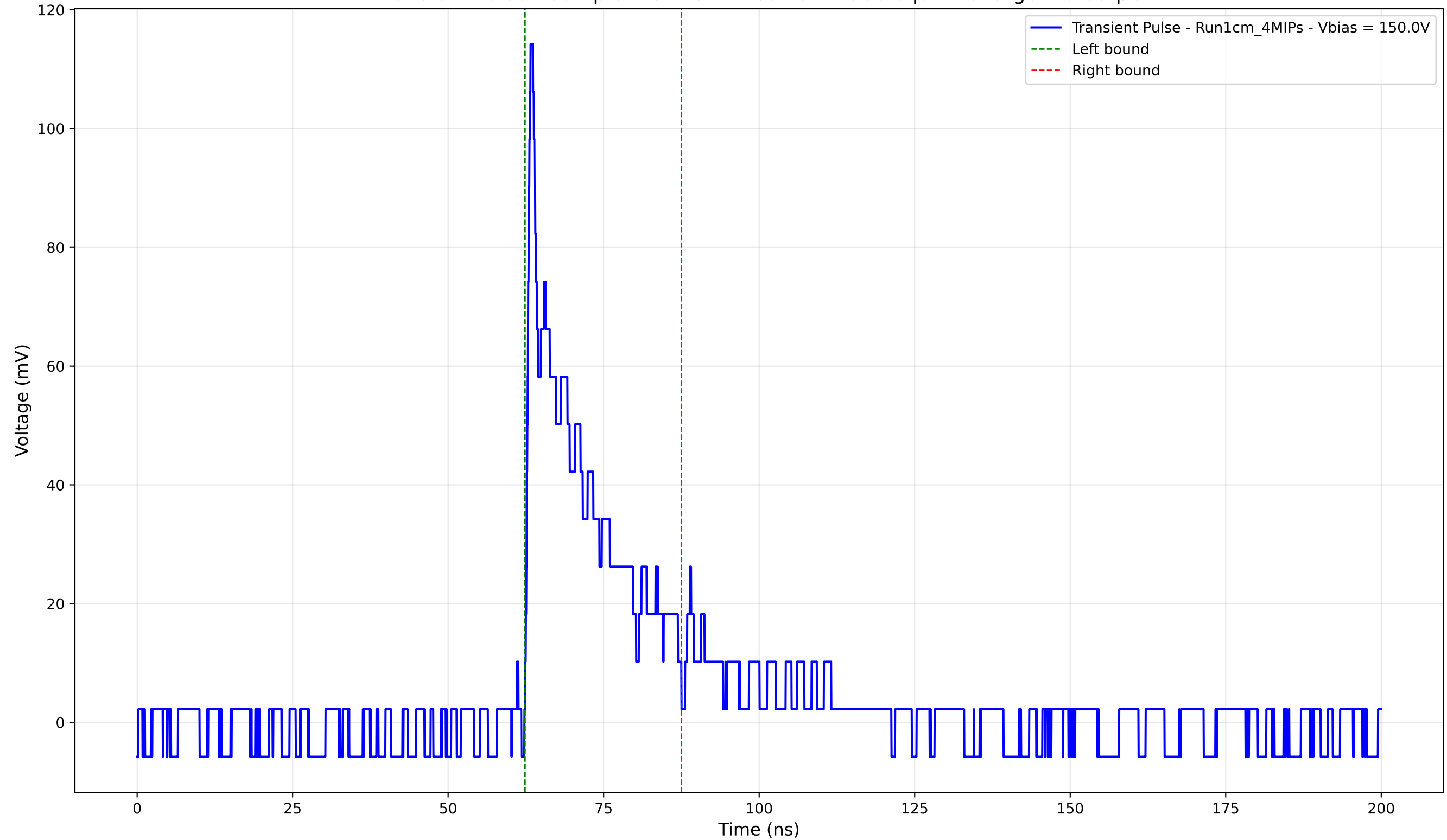
Transient Pulse - Sample: new1cm - Position: 2980.0 \mu\text{m} - Charge: 19.09 pC
