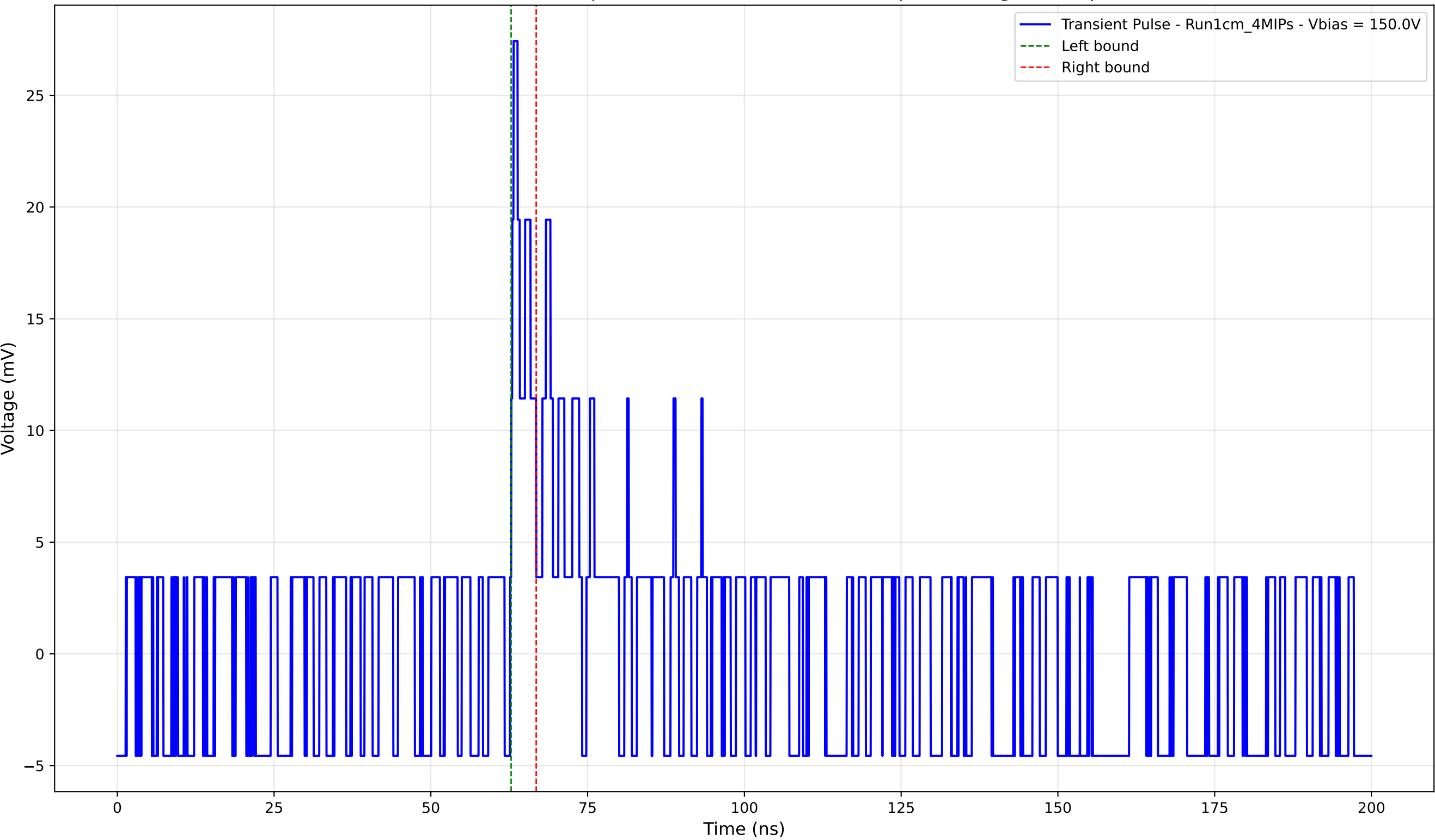
Transient Pulse - Sample: new1cm - Position: 210.0 \mu\text{m} - Charge: 1.35 pC
