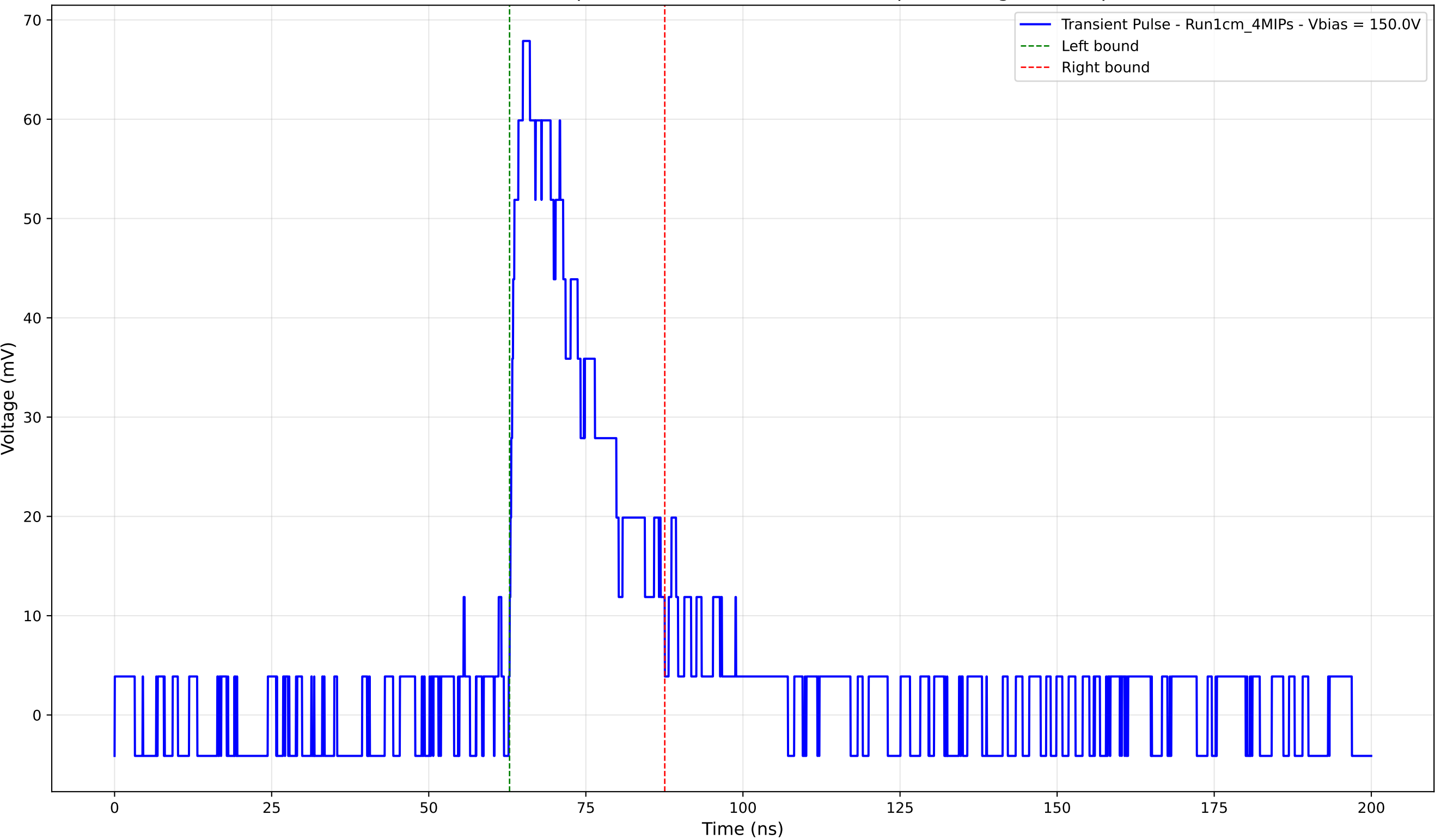
Transient Pulse - Sample: new1cm - Position: 1030.0 \mu\text{m} - Charge: 17.75 pC
