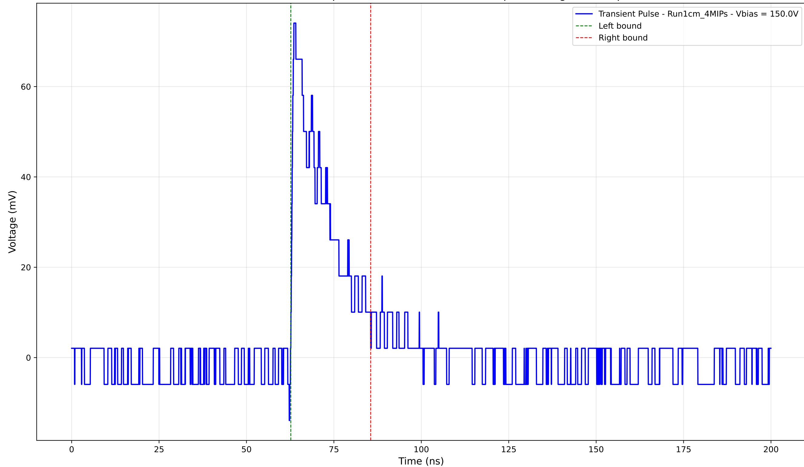
Transient Pulse - Sample: new1cm - Position: 570.0 \mu\text{m} - Charge: 14.92 pC
