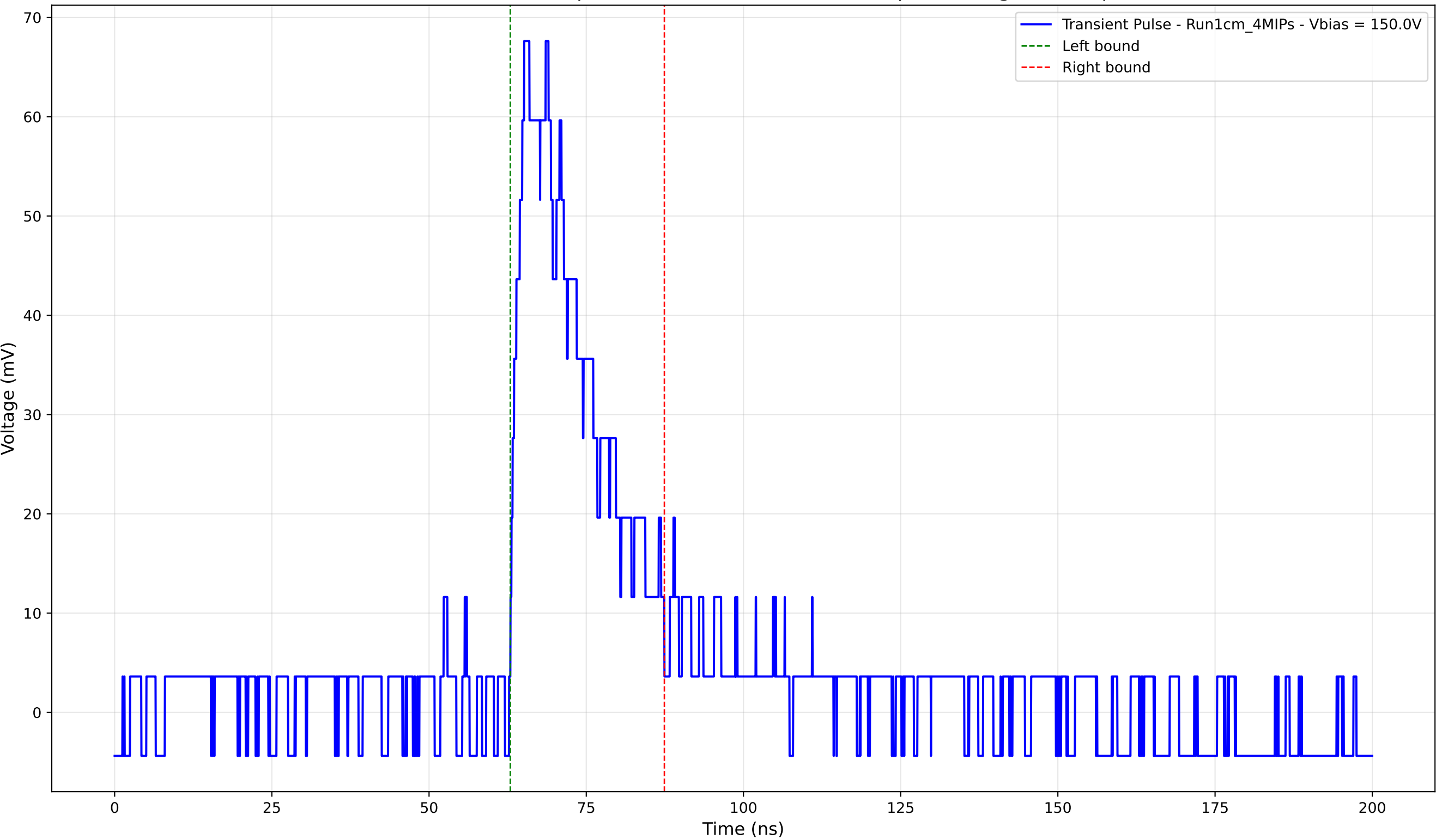
Transient Pulse - Sample: new1cm - Position: 1415.0 \mu\text{m} - Charge: 17.11 pC
