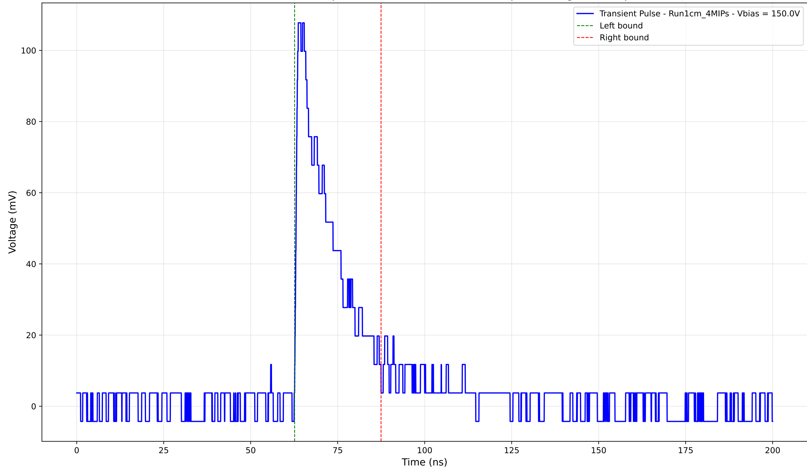
Transient Pulse - Sample: new1cm - Position: 4495.0 \mu\text{m} - Charge: 23.50 pC
