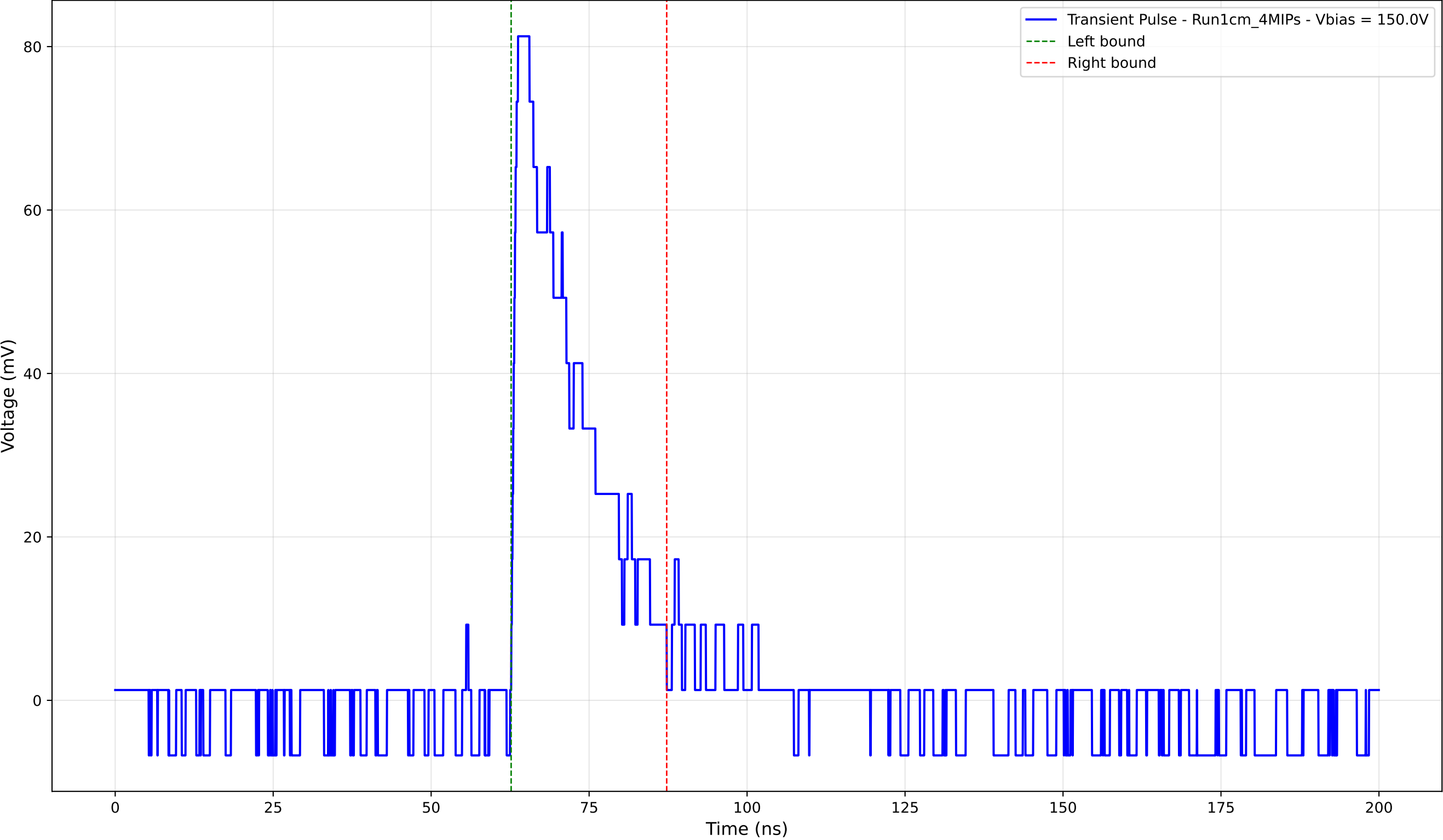
Transient Pulse - Sample: new1cm - Position: 4305.0 \mu\text{m} - Charge: 18.10 pC
