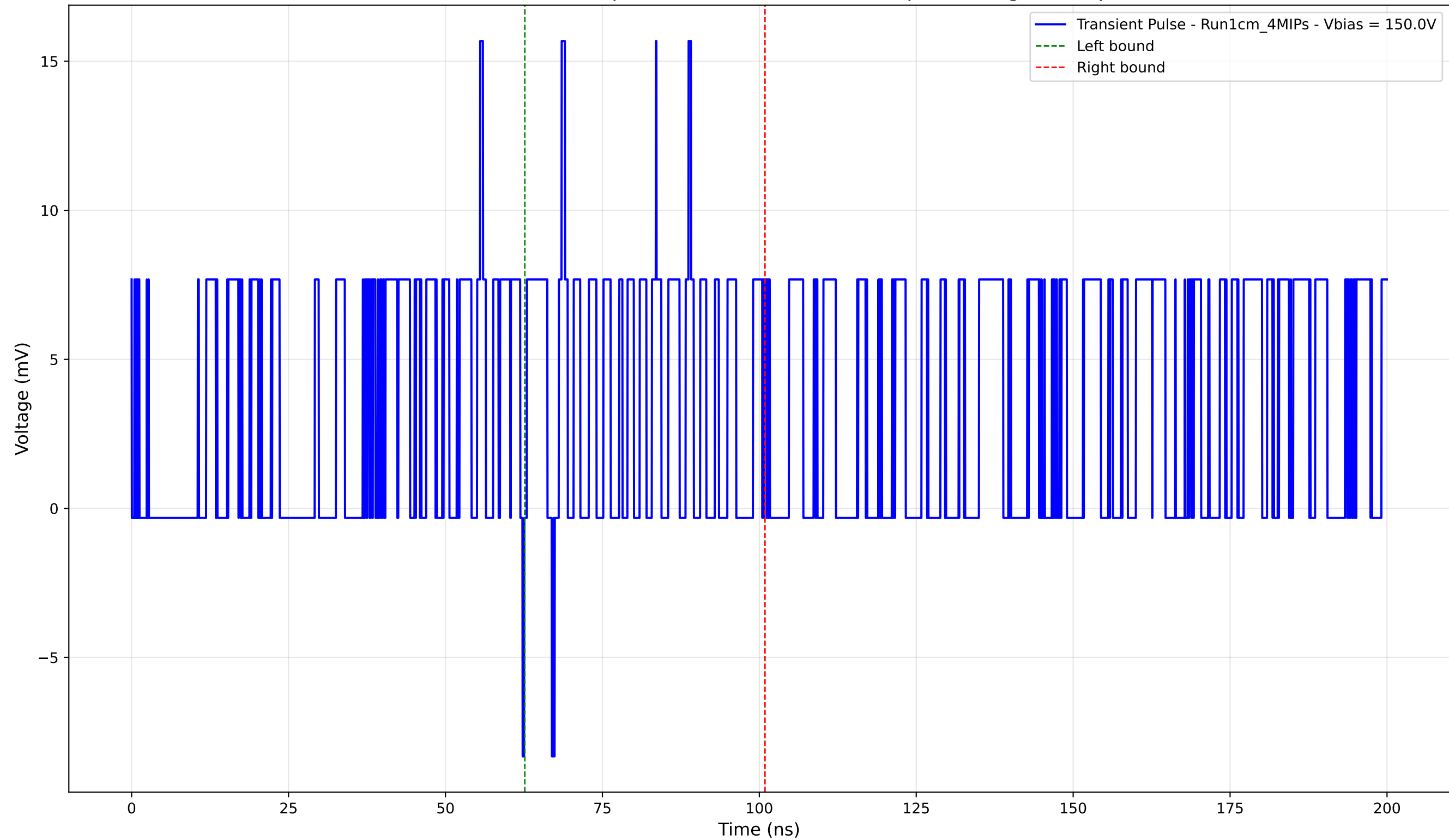
Transient Pulse - Sample: new1cm - Position: 65.0 \mu\text{m} - Charge: 3.09 pC
