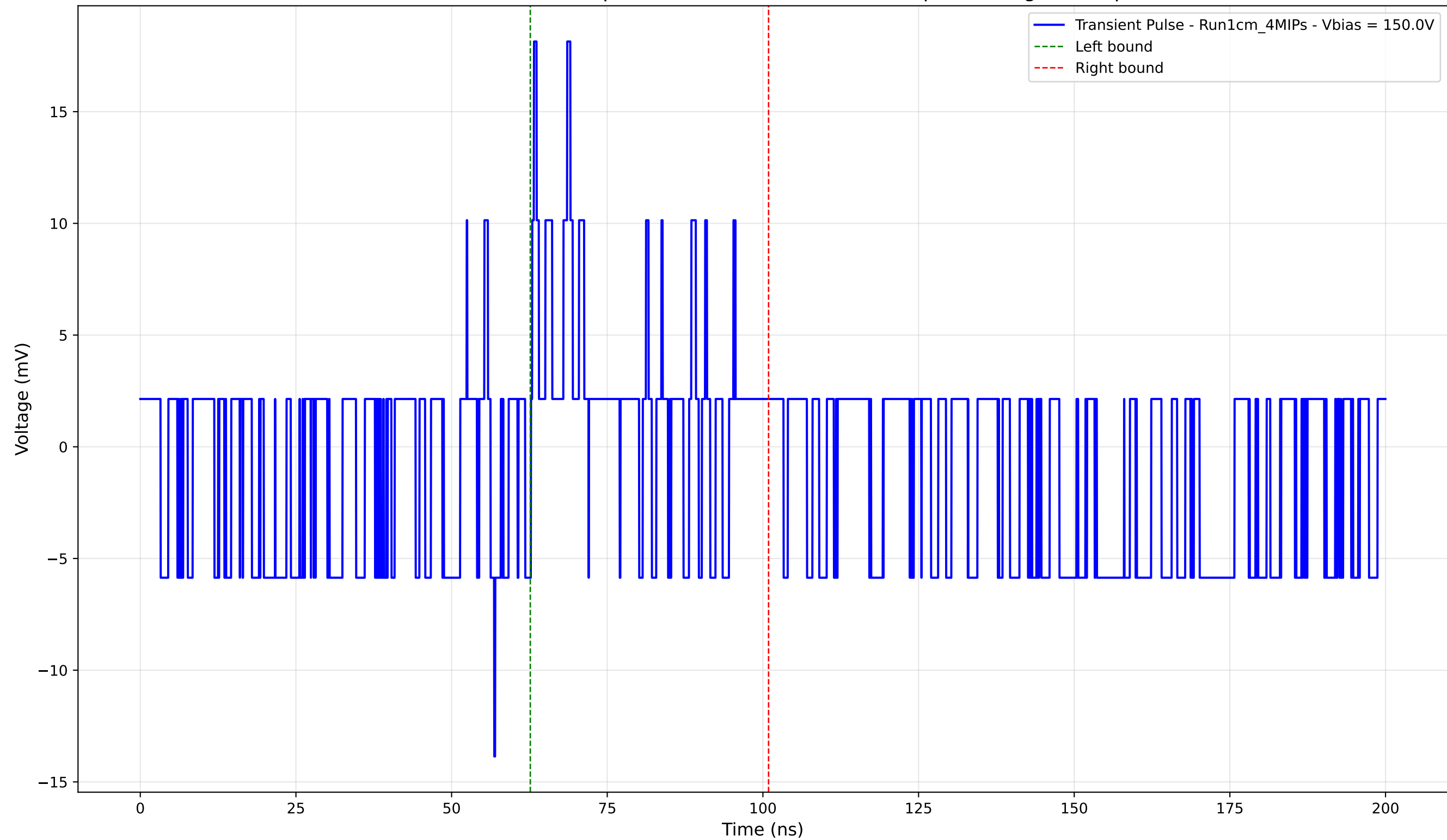
Transient Pulse - Sample: new1cm - Position: 3715.0 \mu\text{m} - Charge: 1.98 pC
