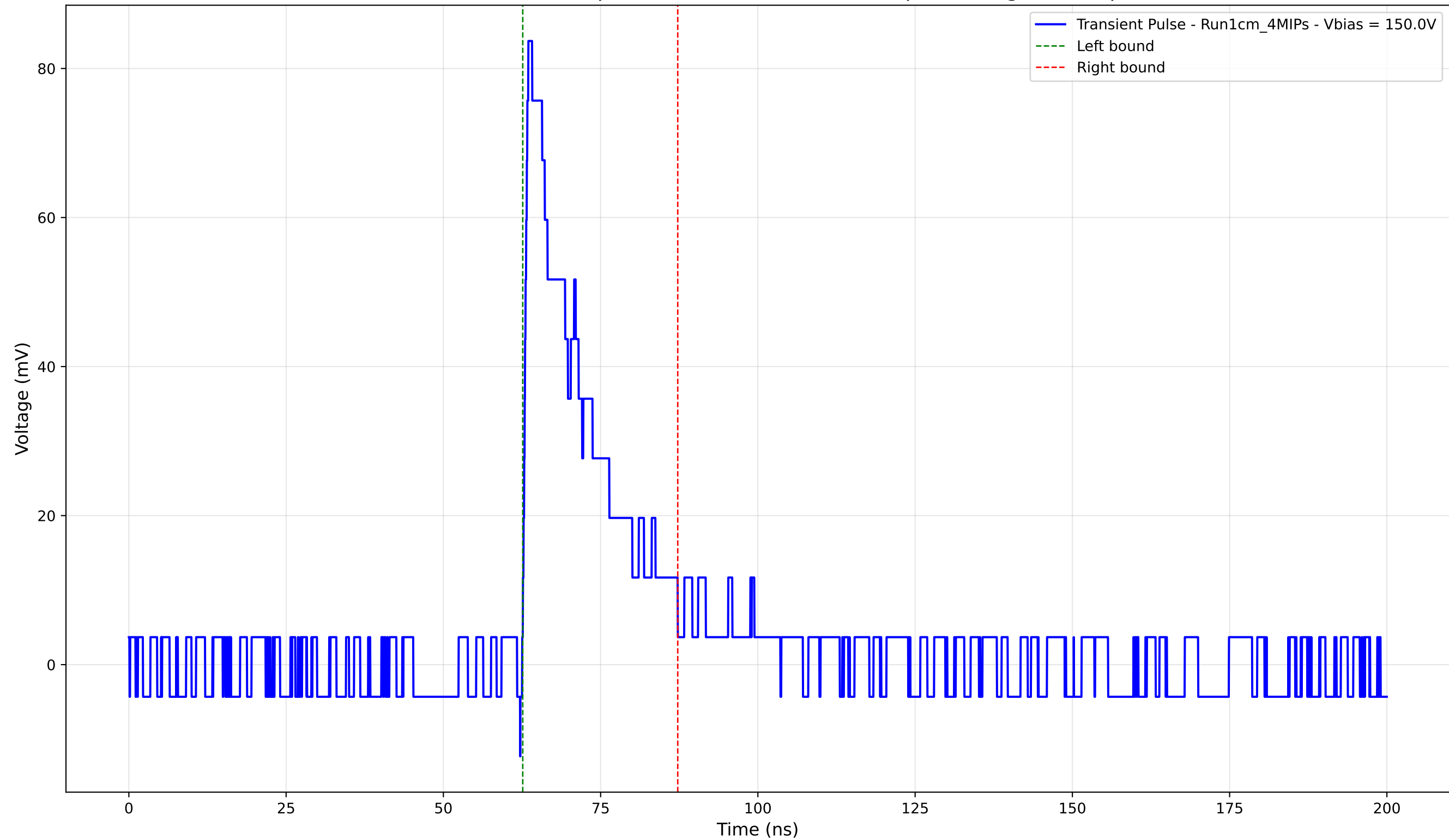
Transient Pulse - Sample: new1cm -Position: 480.0 \mu\text{m} - Charge: 16.44 pC
