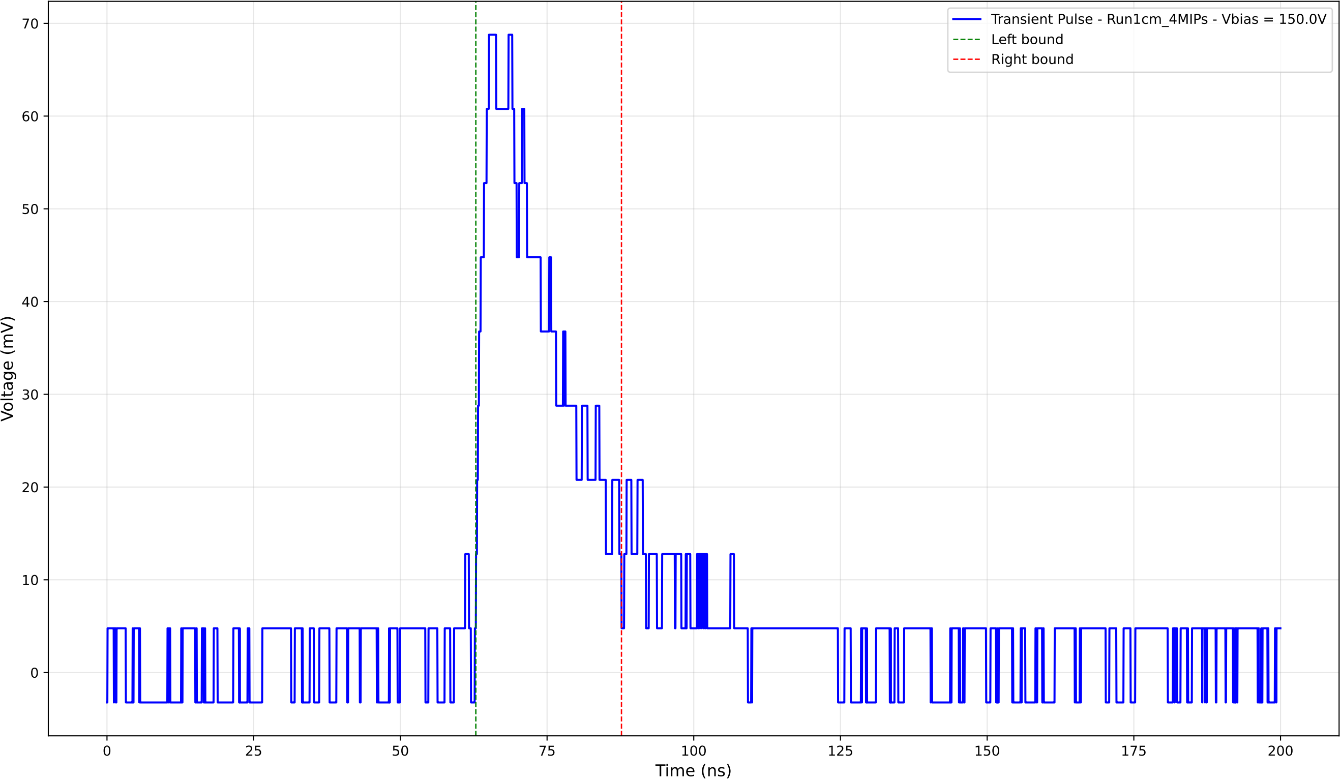
Transient Pulse - Sample: new1cm - Position: 1505.0 \mu\text{m} - Charge: 19.07 pC
