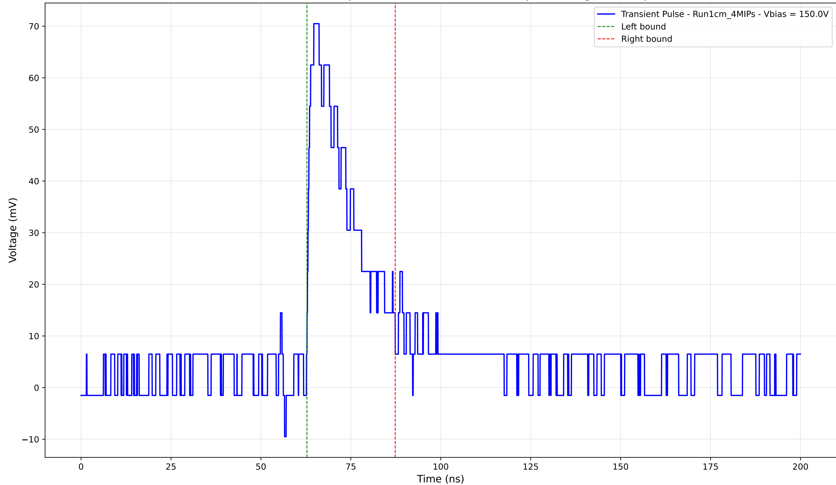
Transient Pulse - Sample: new1cm - Position: 975.0 \mu\text{m} - Charge: 18.37 pC
