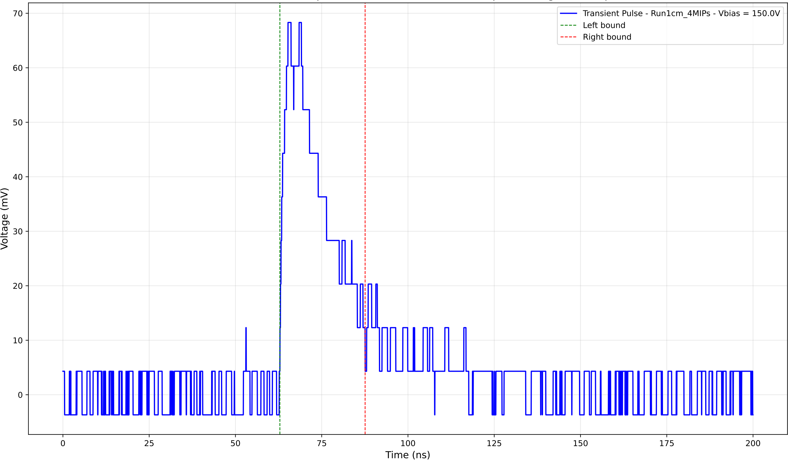
Transient Pulse - Sample: new1cm - Position: 1880.0 \mu\text{m} - Charge: 18.52 pC
