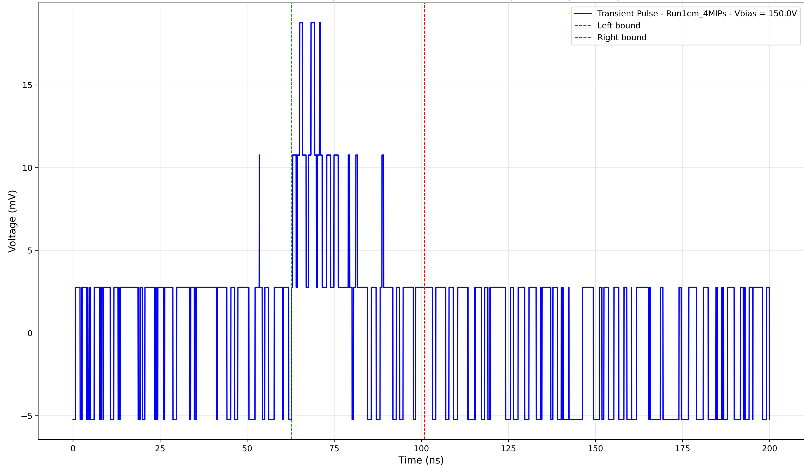
Transient Pulse - Sample: new1cm - Position: 1165.0 \mu\text{m} - Charge: 3.36 pC
