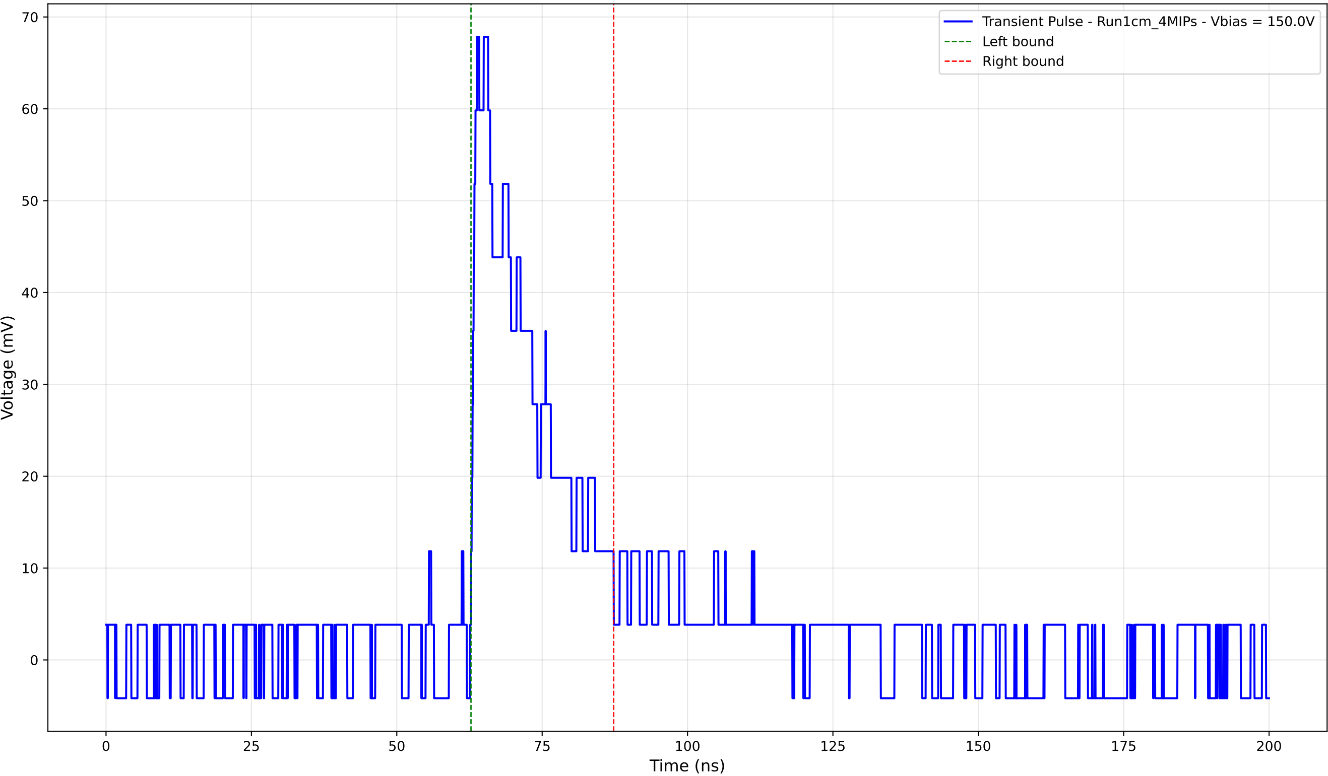
Transient Pulse - Sample: new1cm - Position: 4285.0 \mu\text{m} - Charge: 15.00 pC
