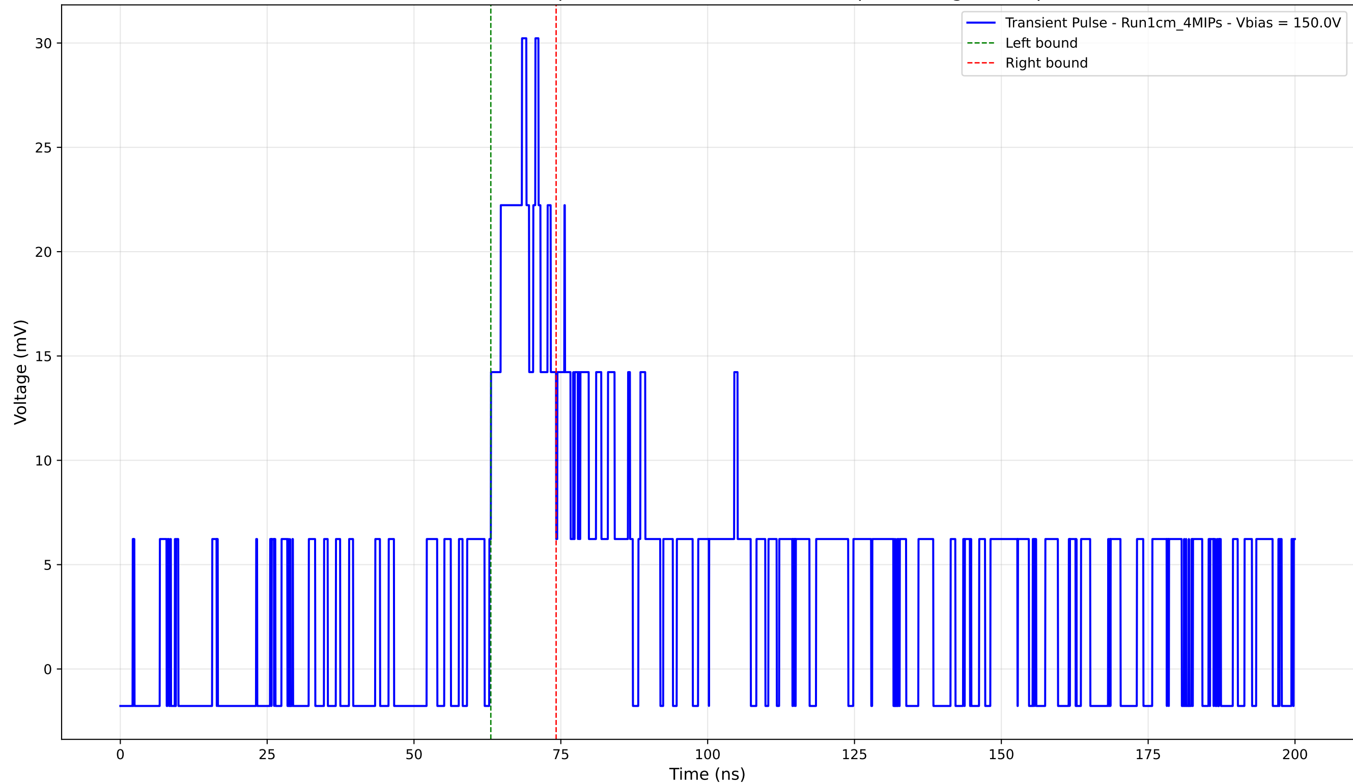
Transient Pulse - Sample: new1cm -Position: 1660.0 \mu\text{m} - Charge: 4.43 pC
