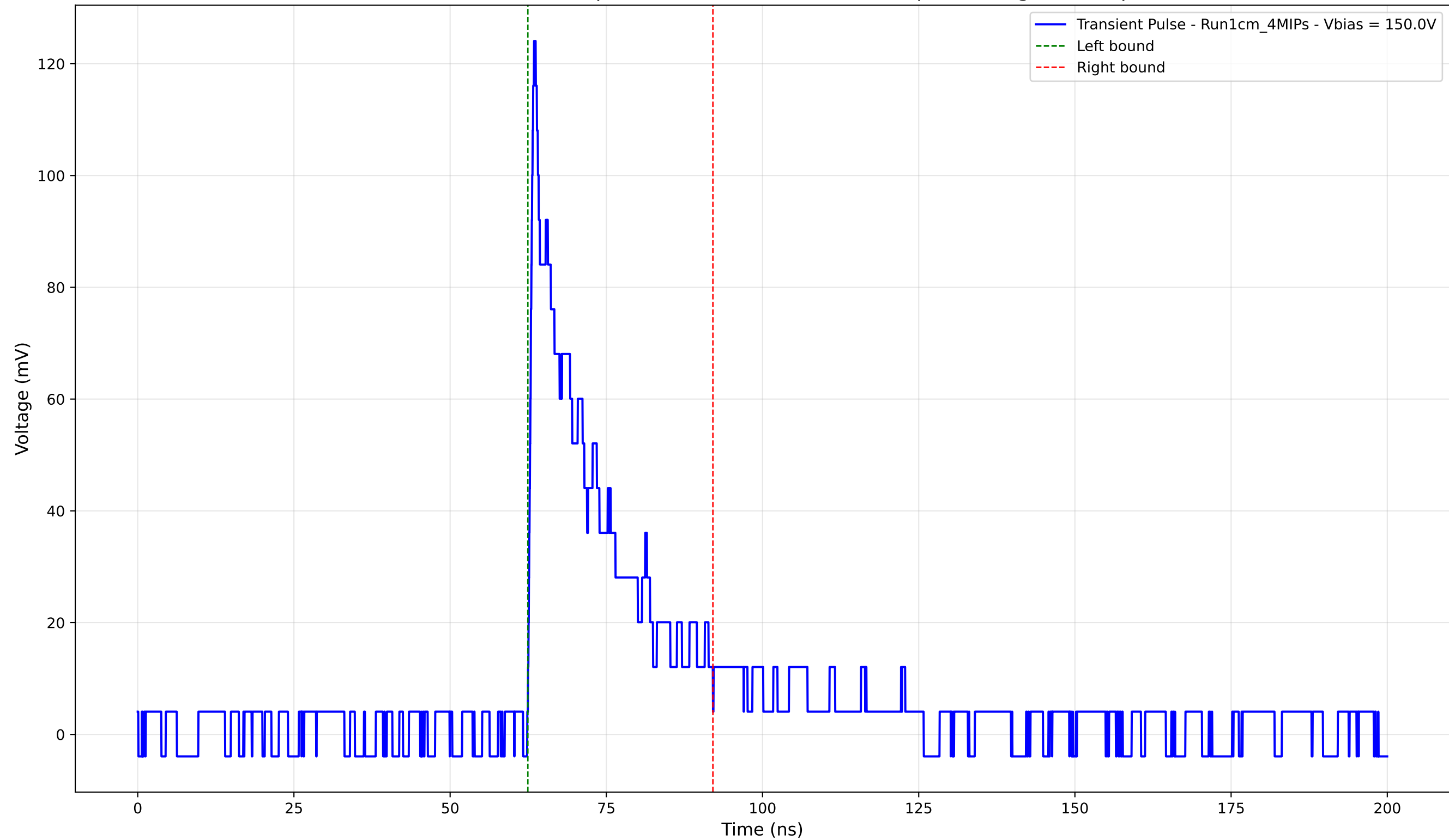
Transient Pulse - Sample: new1cm - Position: 3575.0 \mu\text{m} - Charge: 23.62 pC
