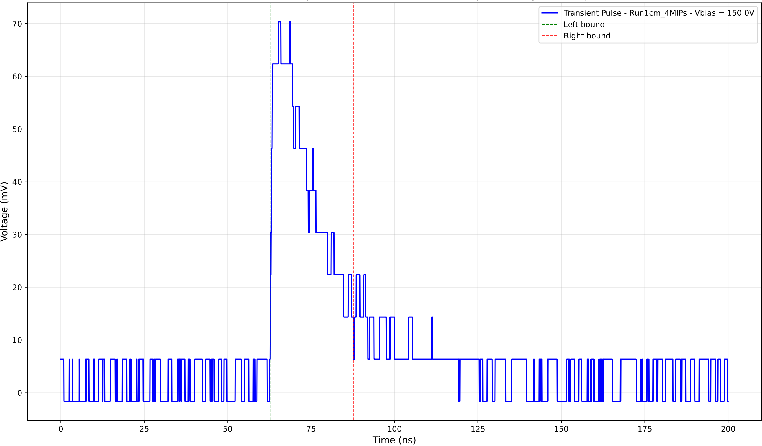
Transient Pulse - Sample: new1cm - Position: 2350.0 \mu\text{m} - Charge: 19.79 pC
