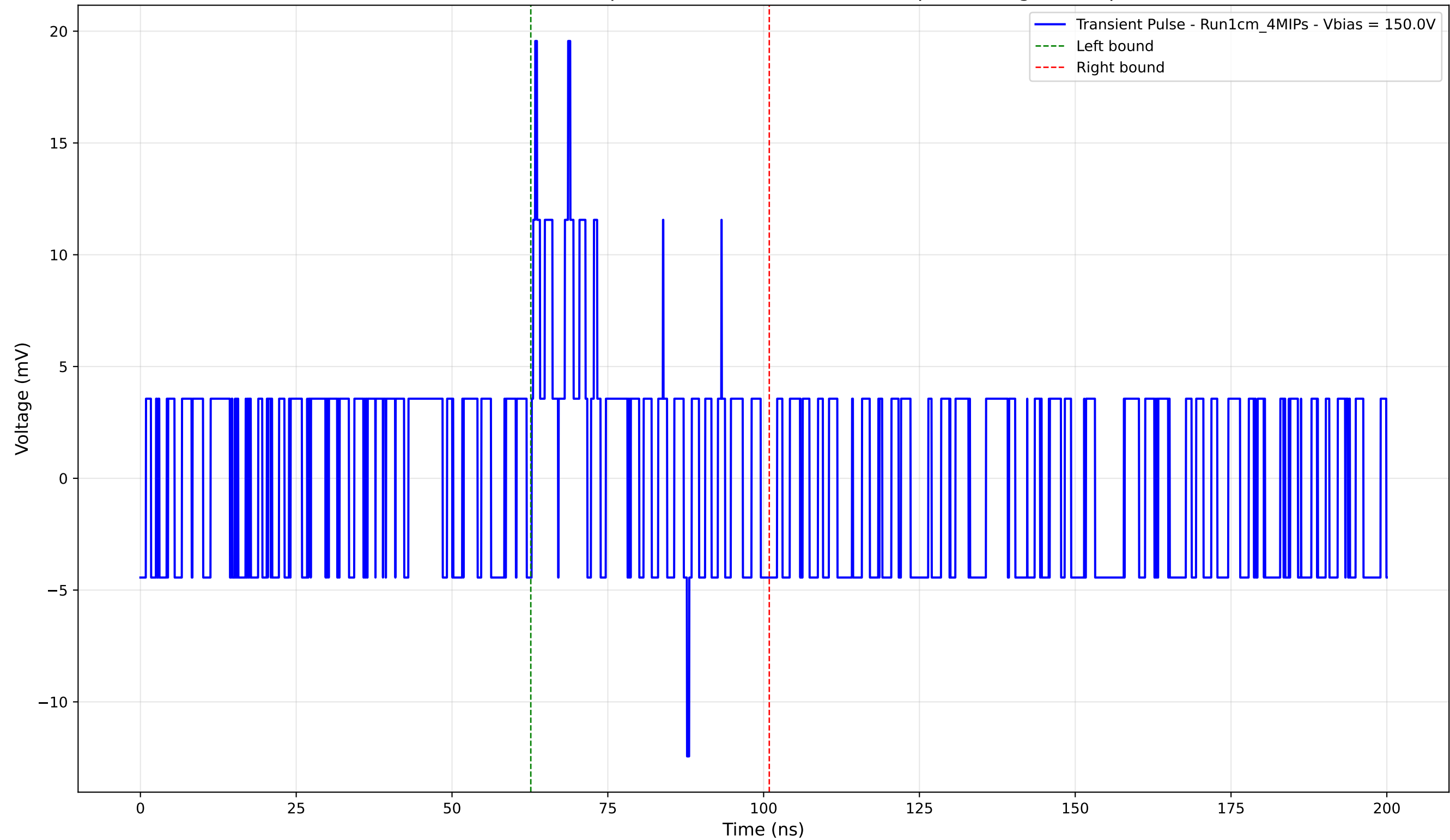
Transient Pulse - Sample: new1cm - Position: 675.0 \mu\text{m} - Charge: 1.76 pC
