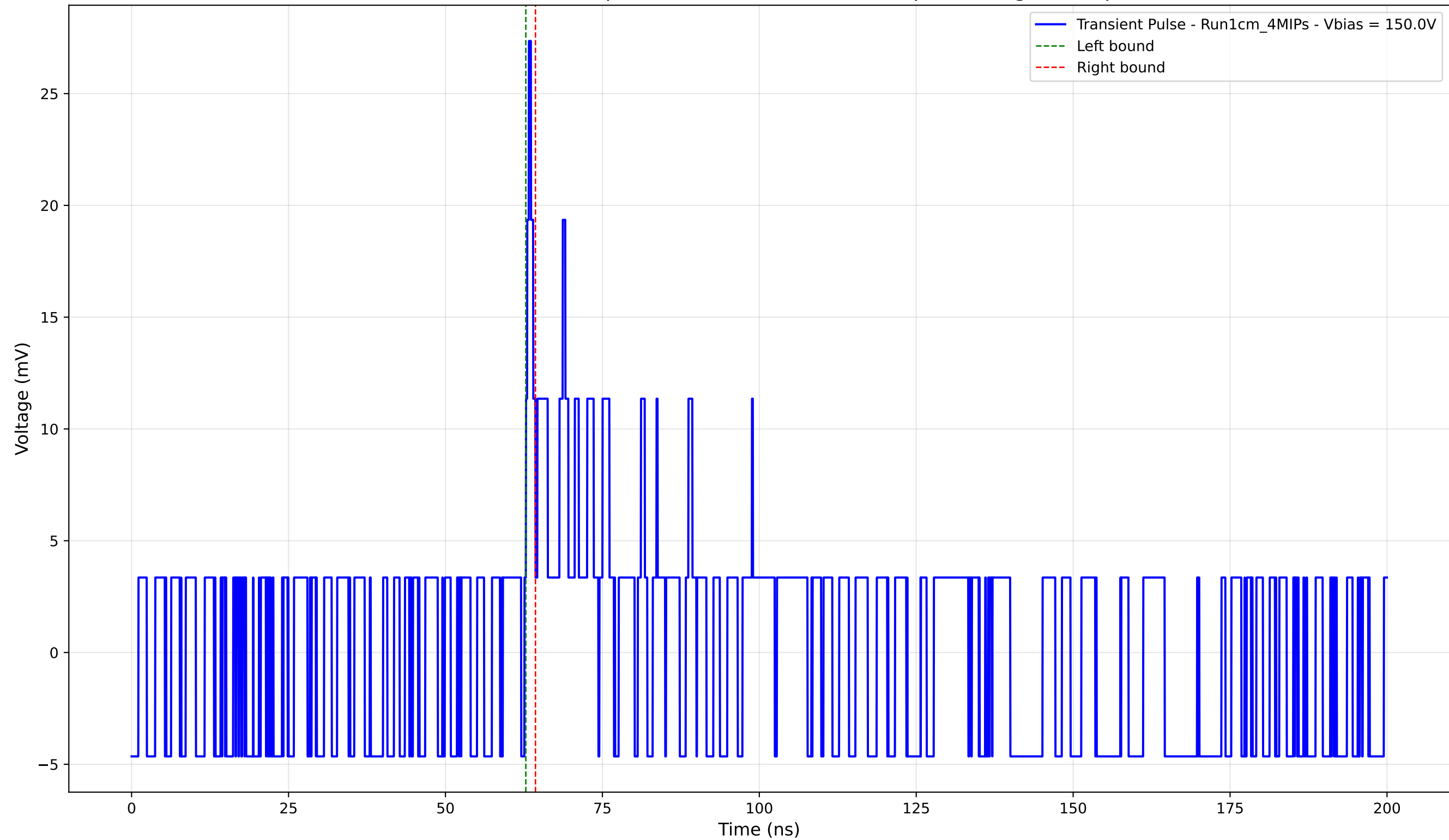
Transient Pulse - Sample: new1cm - Position: 205.0 \mu\text{m} - Charge: 0.55 pC
