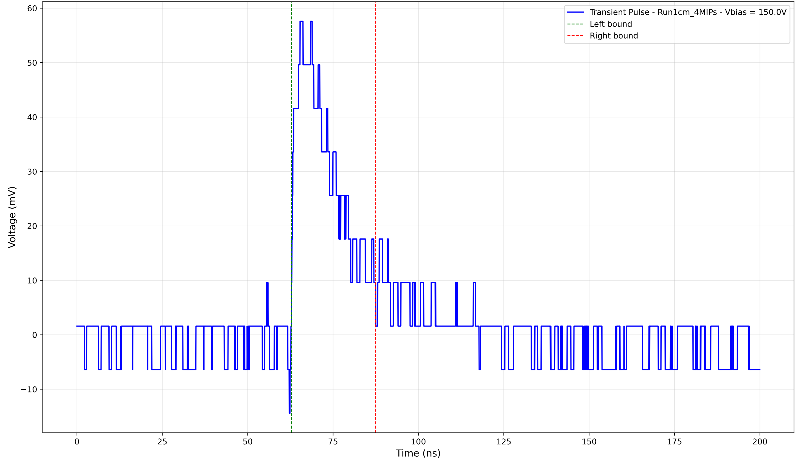
Transient Pulse - Sample: new1cm - Position: 2105.0 \mu\text{m} - Charge: 14.82 pC
