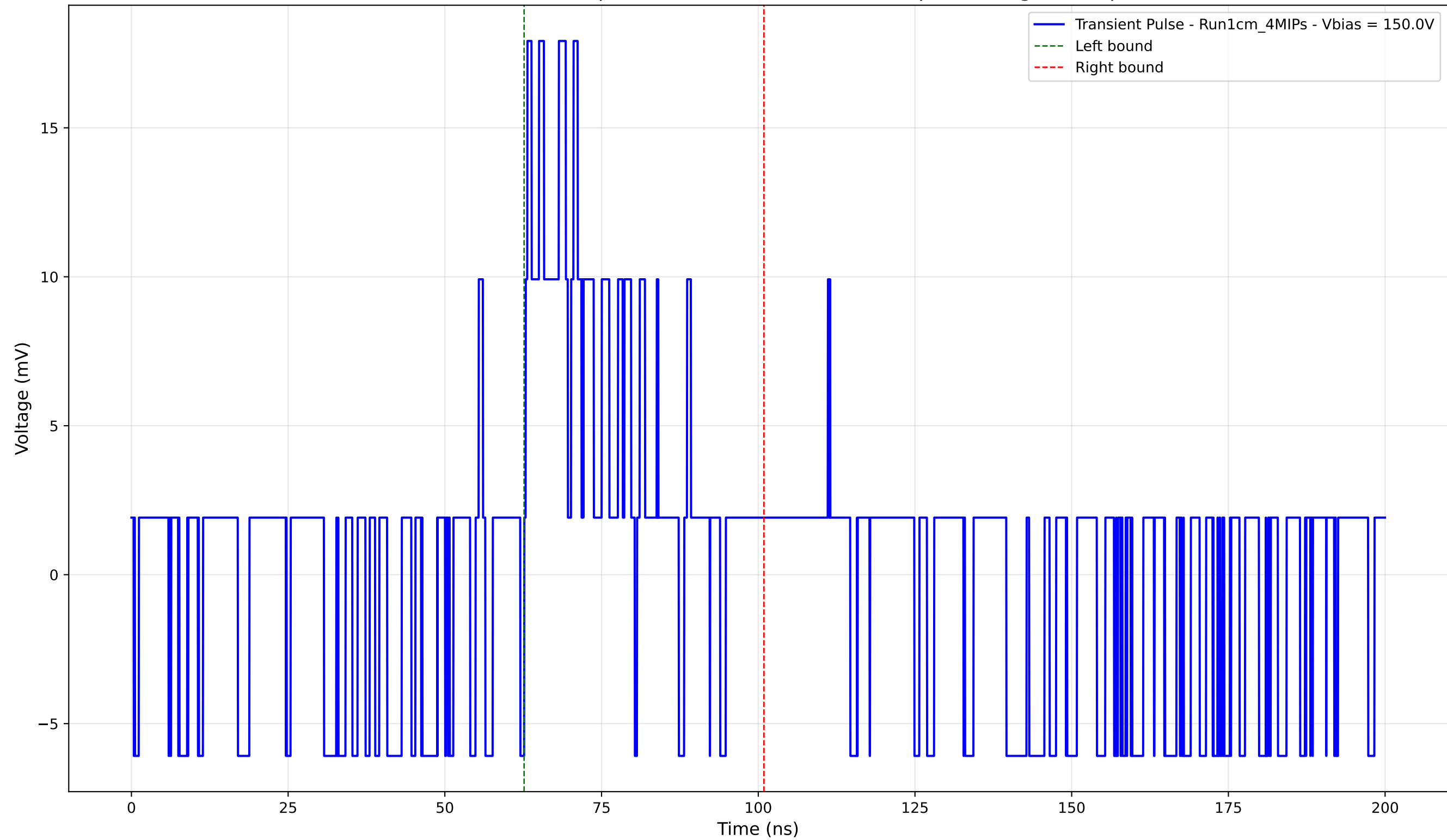
Transient Pulse - Sample: new1cm - Position: 2225.0 \mu\text{m} - Charge: 4.01 pC
