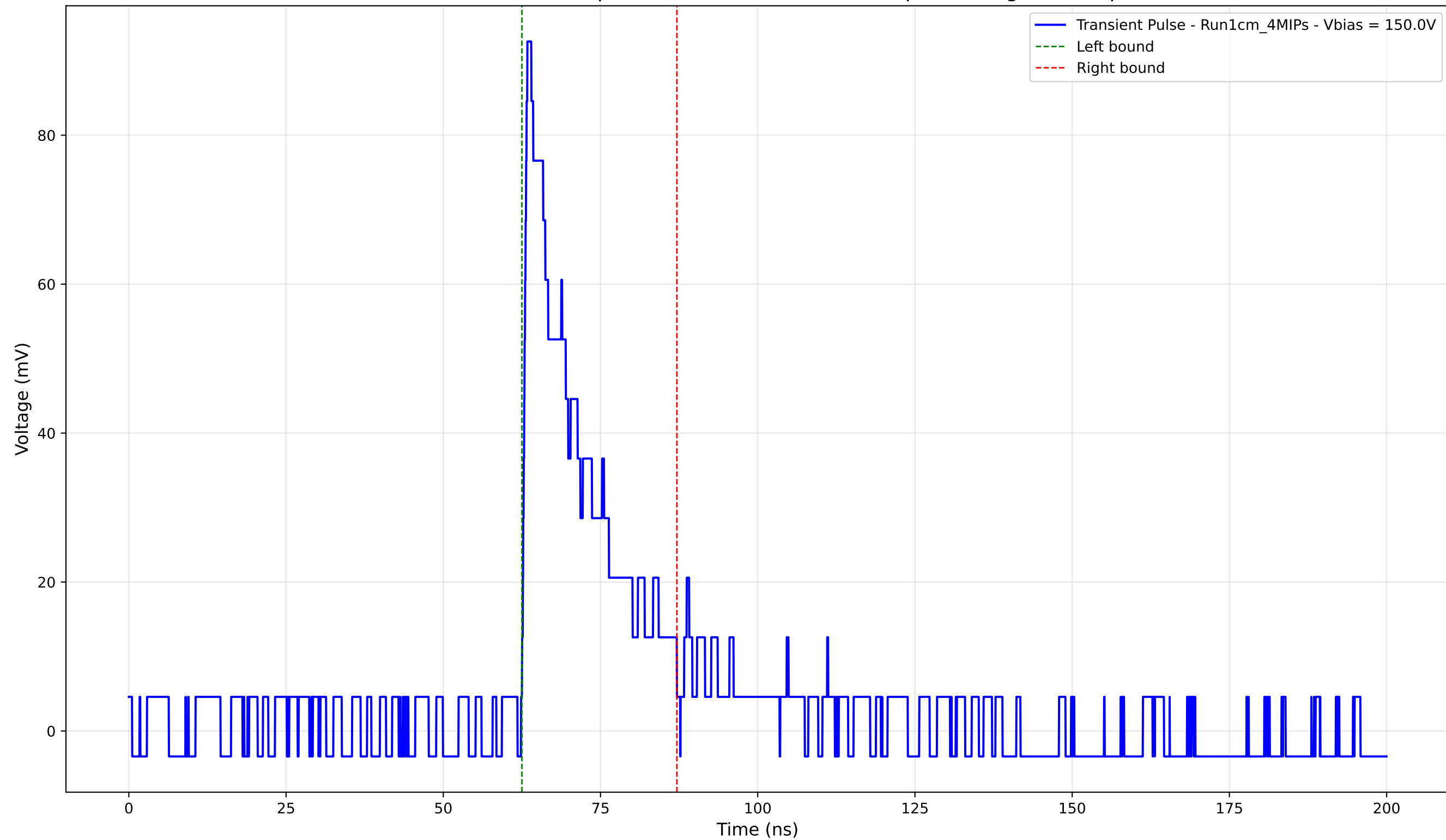
Transient Pulse - Sample: new1cm -Position: 370.0 \mu\text{m} - Charge: 17.38 pC
