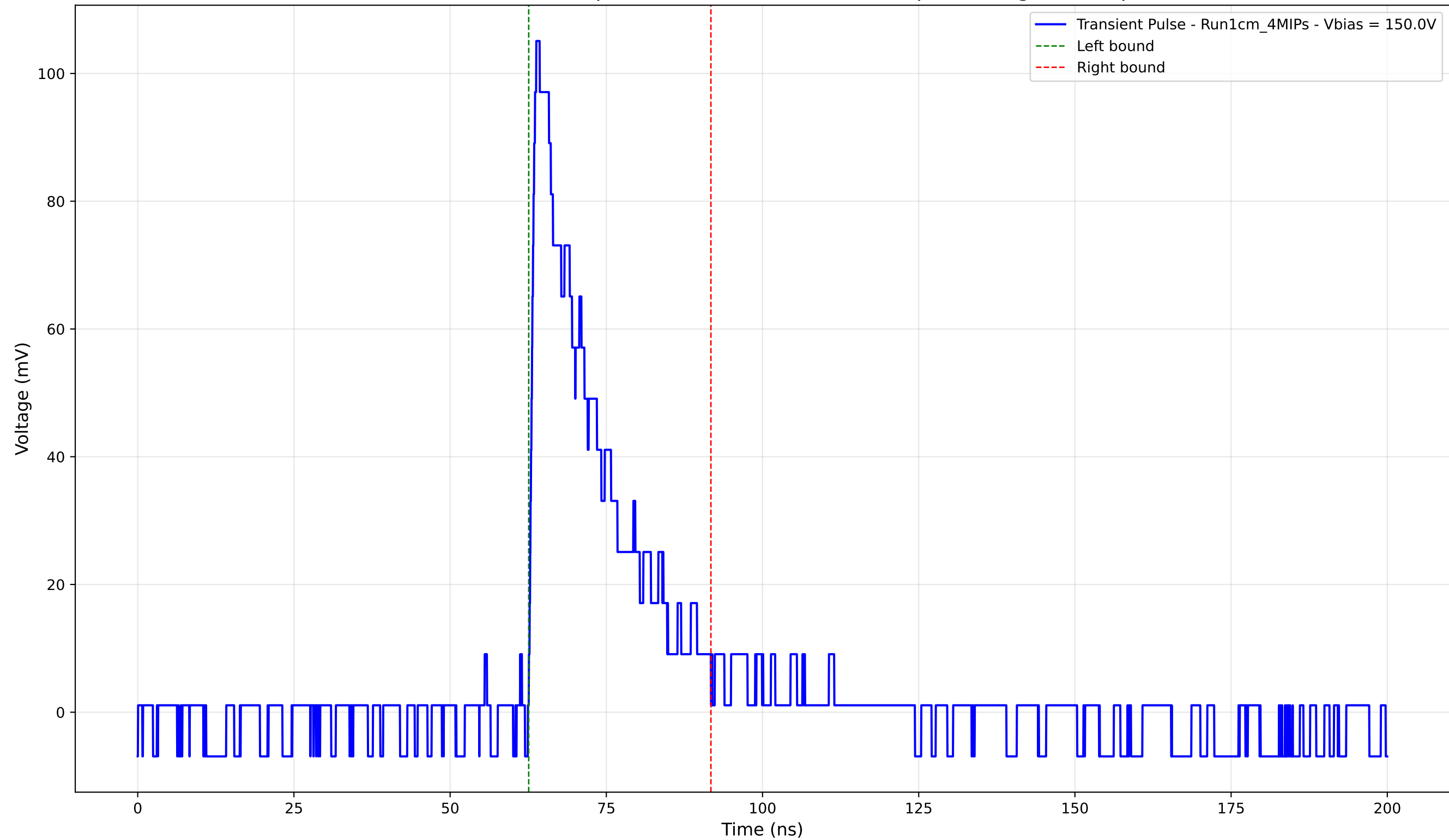
Transient Pulse - Sample: new1cm - Position: 4420.0 \mu\text{m} - Charge: 22.74 pC
