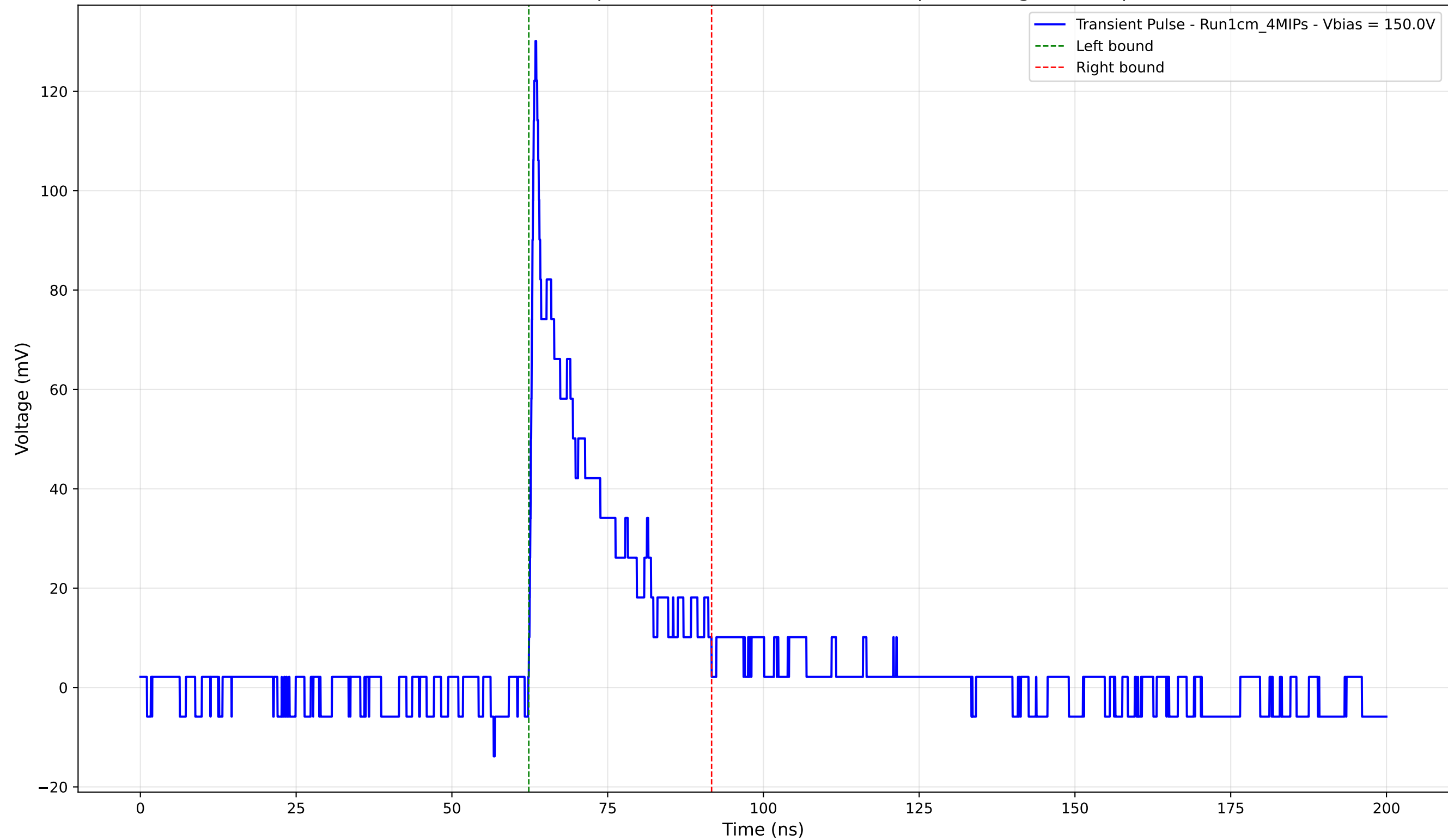
Transient Pulse - Sample: new1cm - Position: 3465.0 \mu\text{m} - Charge: 21.69 pC
