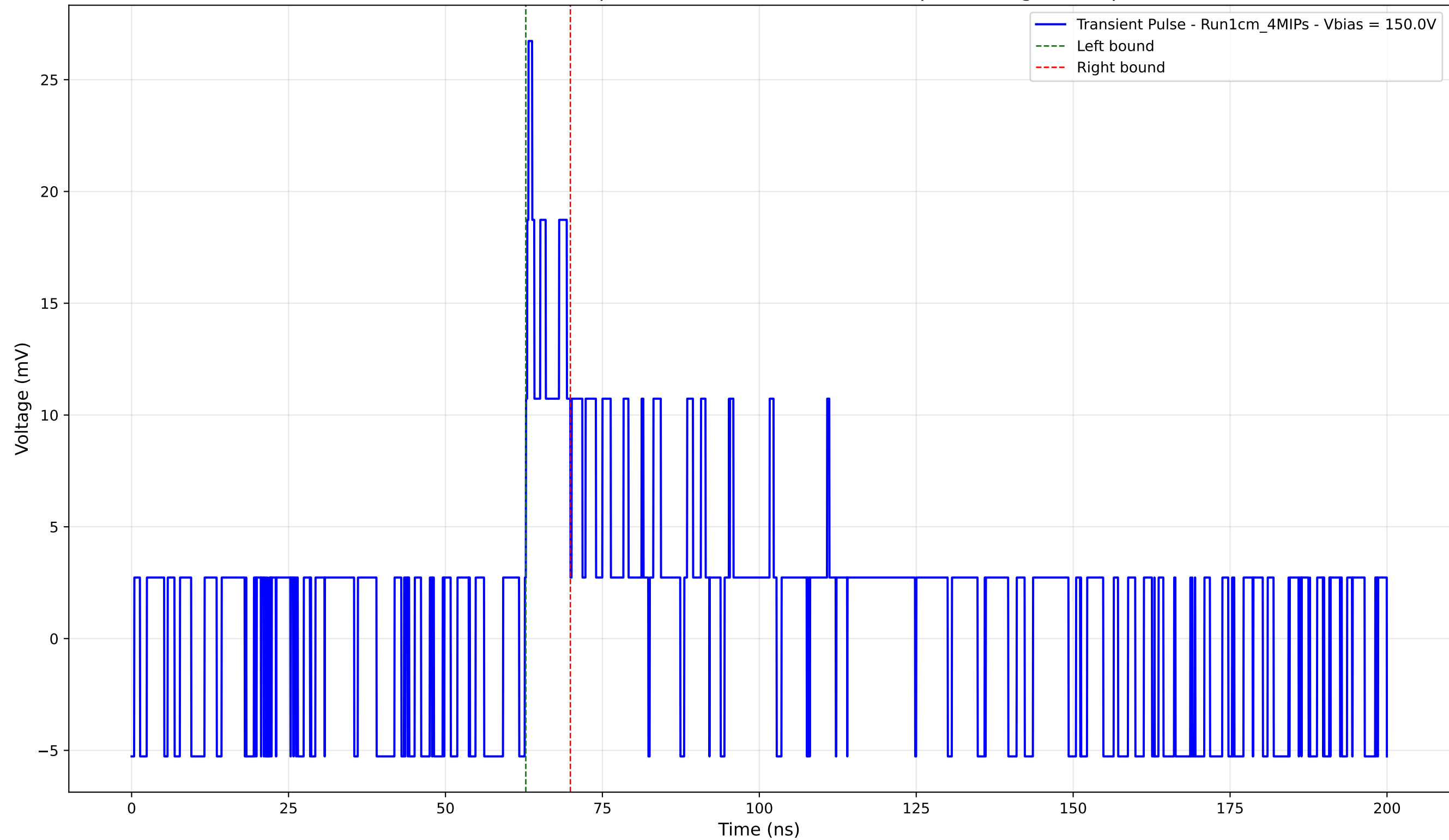
Transient Pulse - Sample: new1cm - Position: 2735.0 \mu\text{m} - Charge: 2.14 pC
