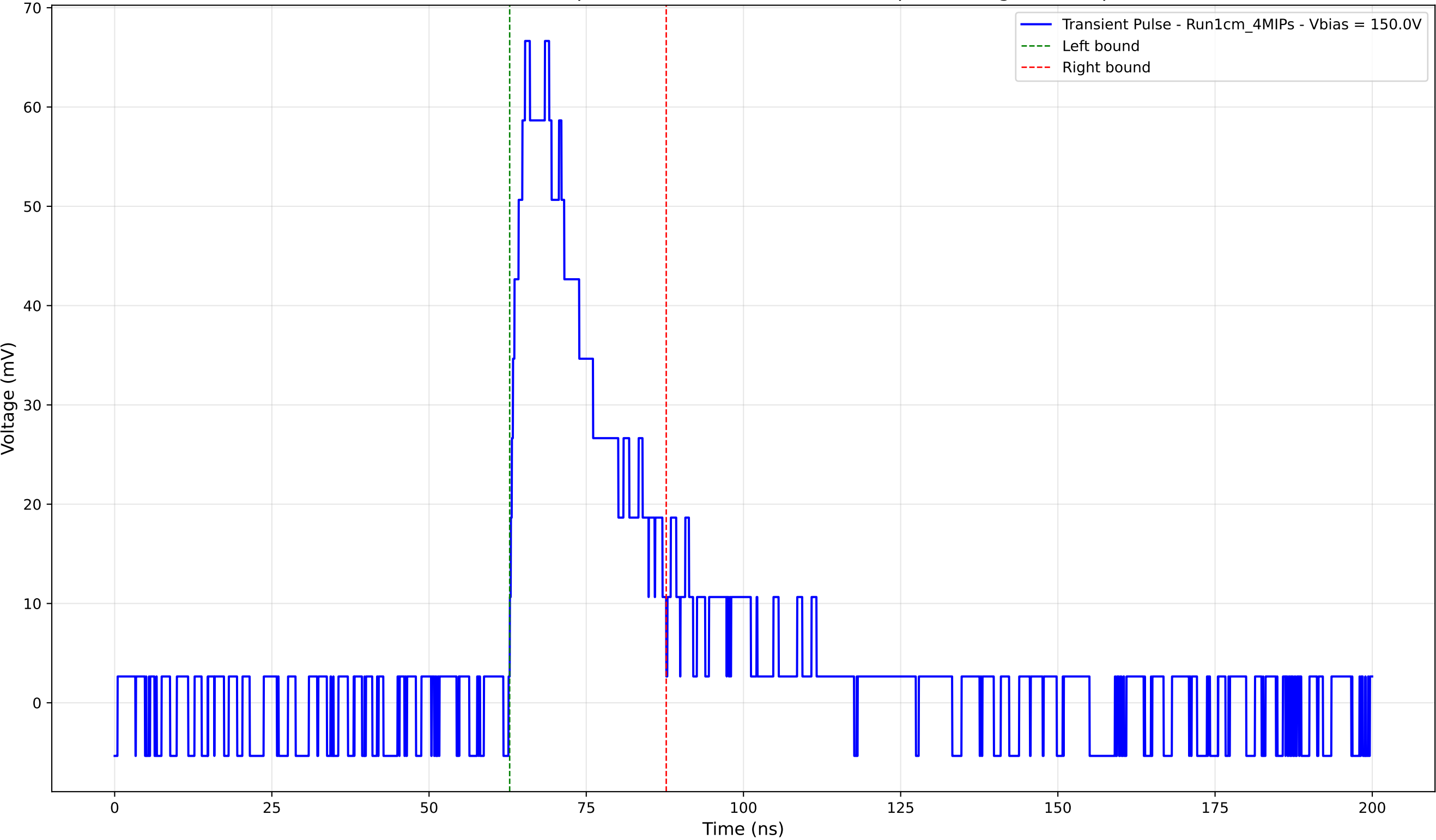
Transient Pulse - Sample: new1cm - Position: 1915.0 \mu\text{m} - Charge: 17.99 pC
