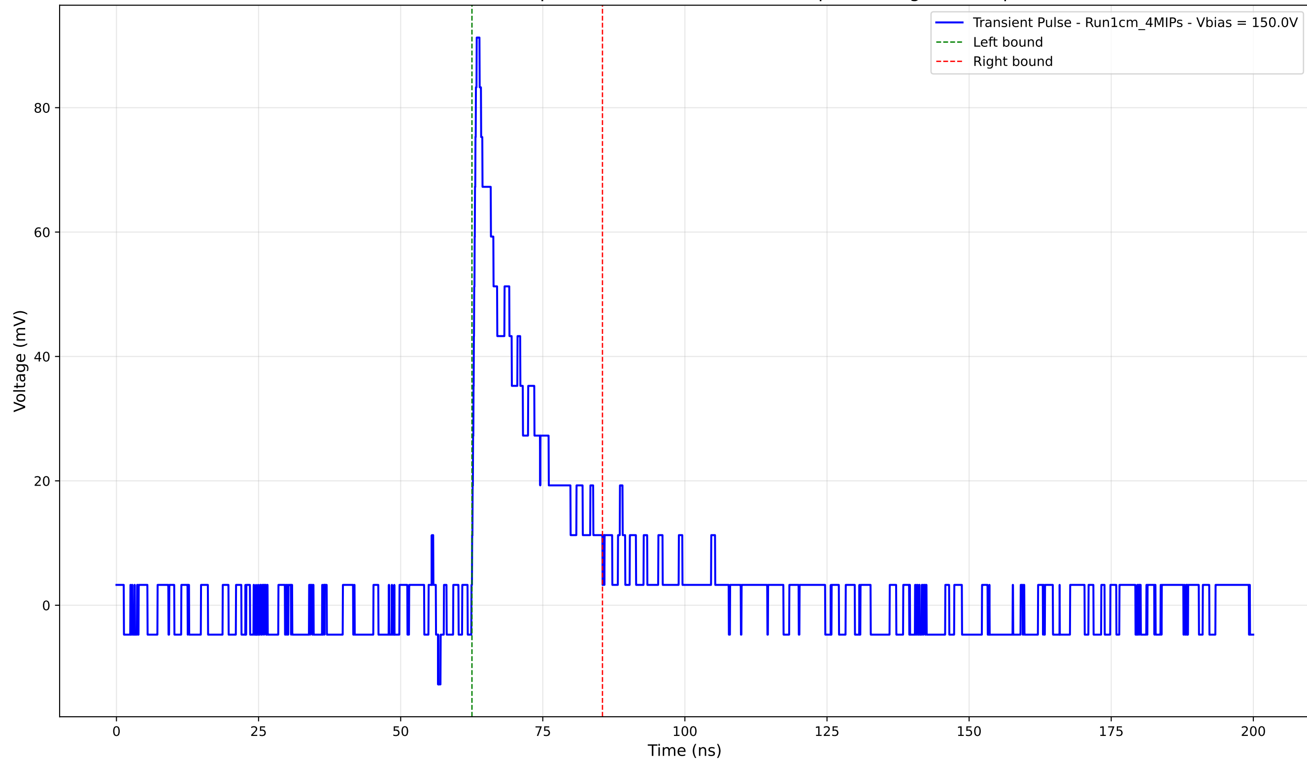
Transient Pulse - Sample: new1cm -Position: 305.0 \mu\text{m} - Charge: 15.22 pC
