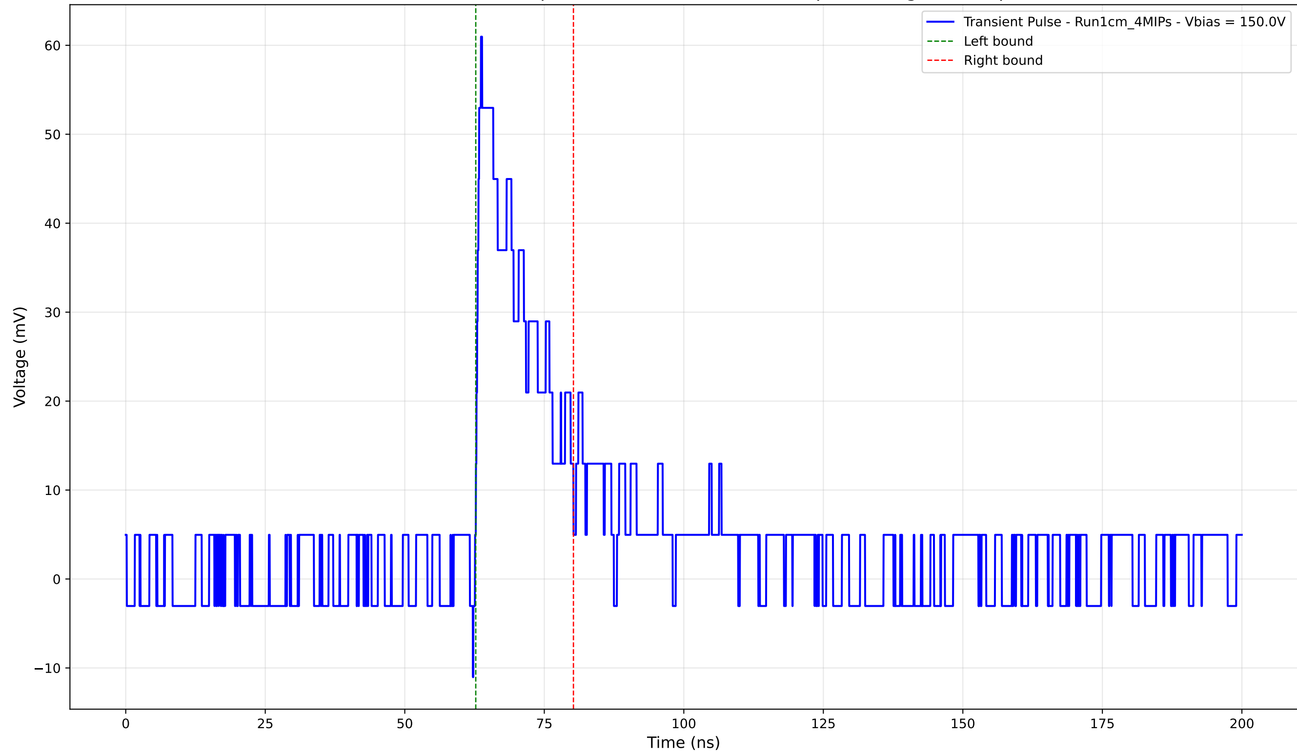
Transient Pulse - Sample: new1cm - Position: 615.0 \mu\text{m} - Charge: 10.97 pC
