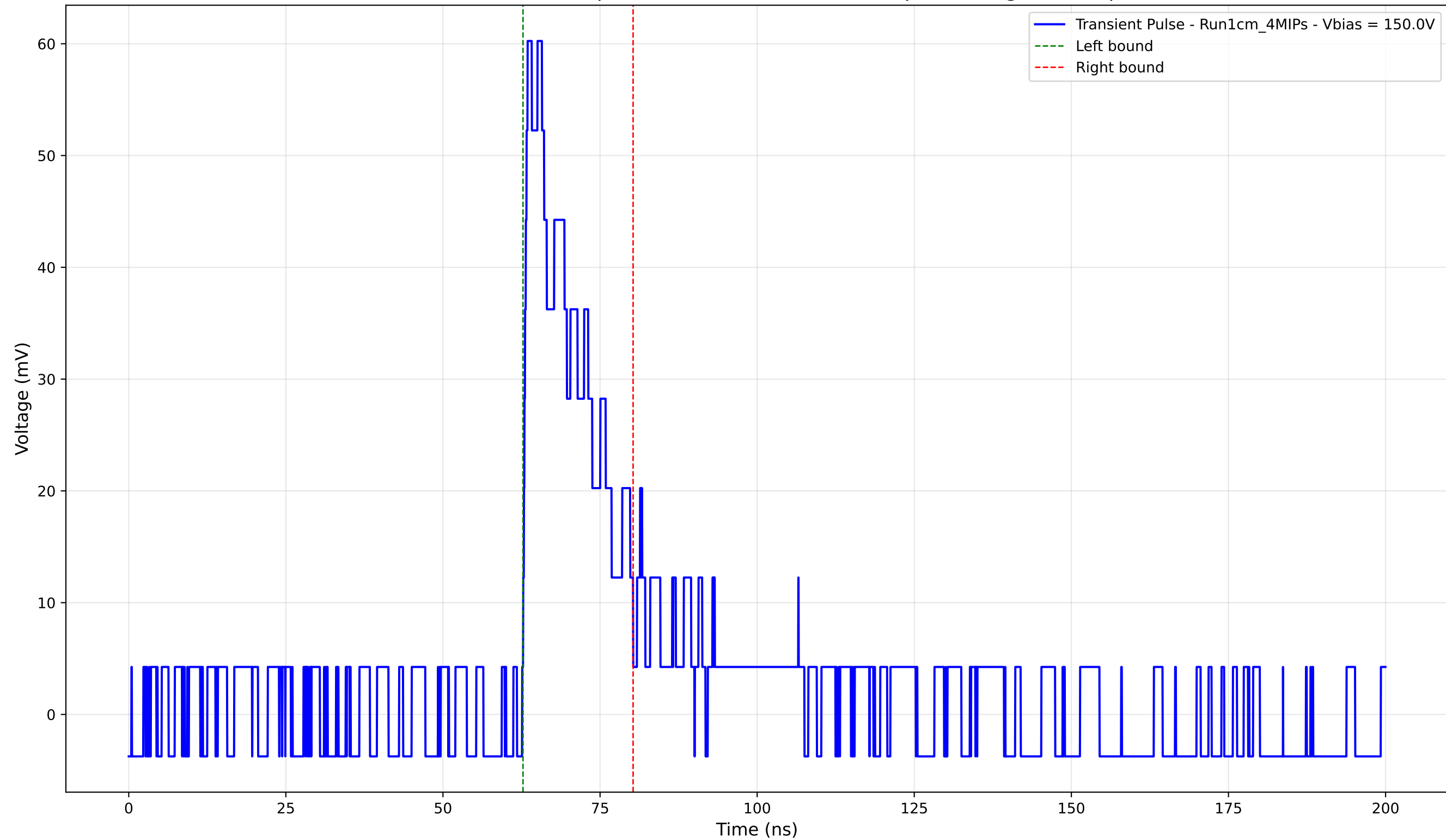
Transient Pulse - Sample: new1cm -Position: 605.0 \mu\text{m} - Charge: 11.41 pC
