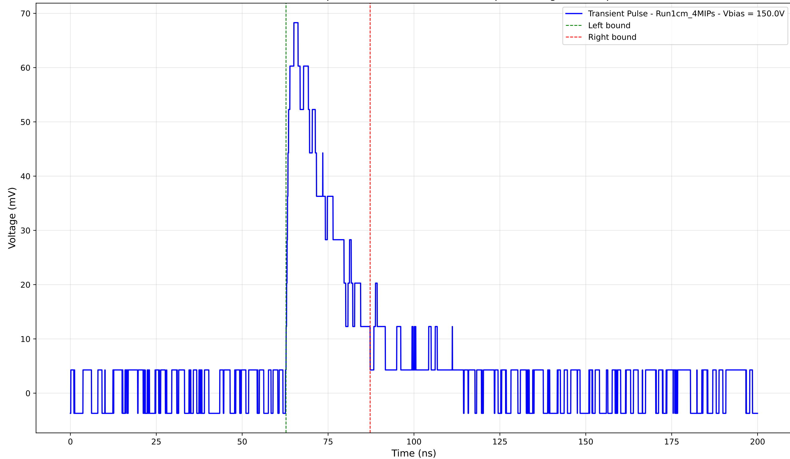
Transient Pulse - Sample: new1cm -Position: 935.0 \mu\text{m} - Charge: 17.37 pC
