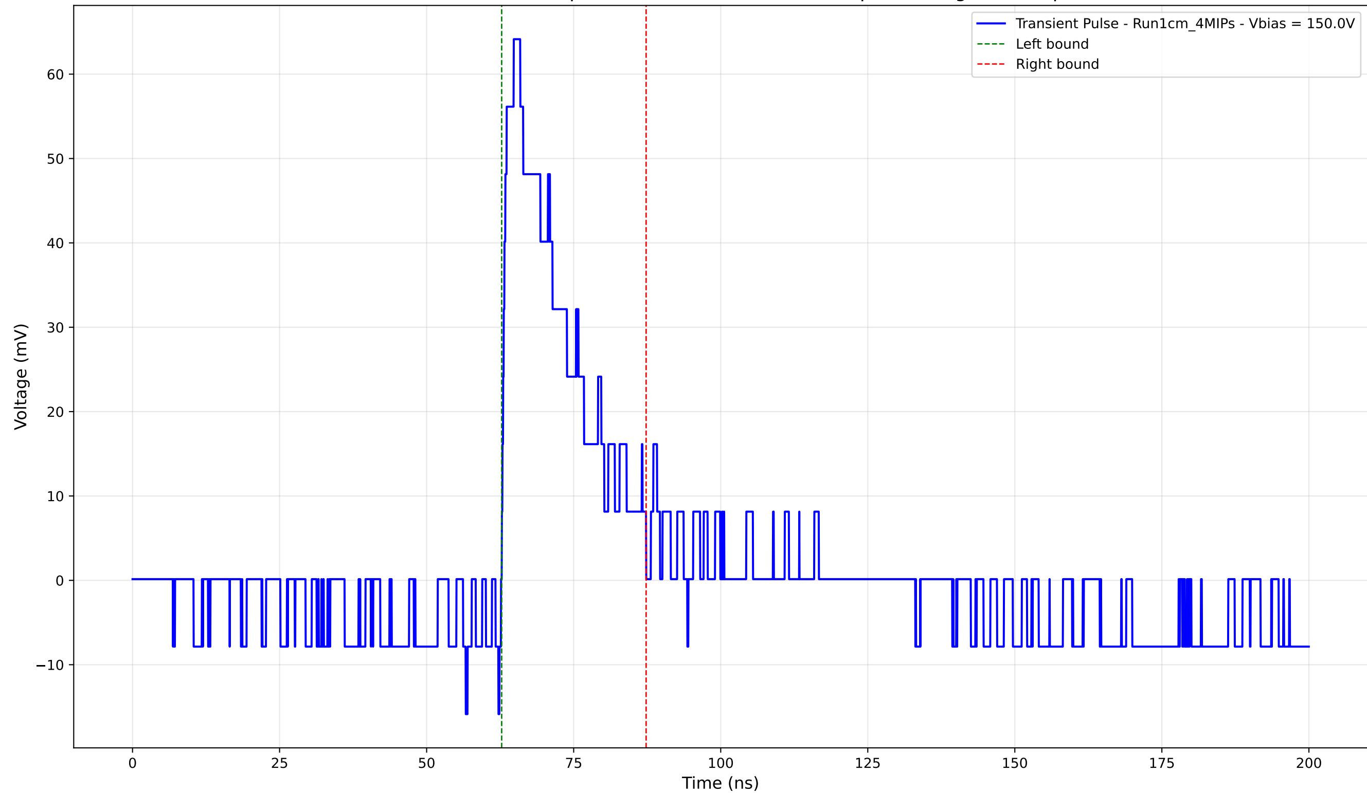
Transient Pulse - Sample: new1cm - Position: 795.0 \mu\text{m} - Charge: 14.17 pC
