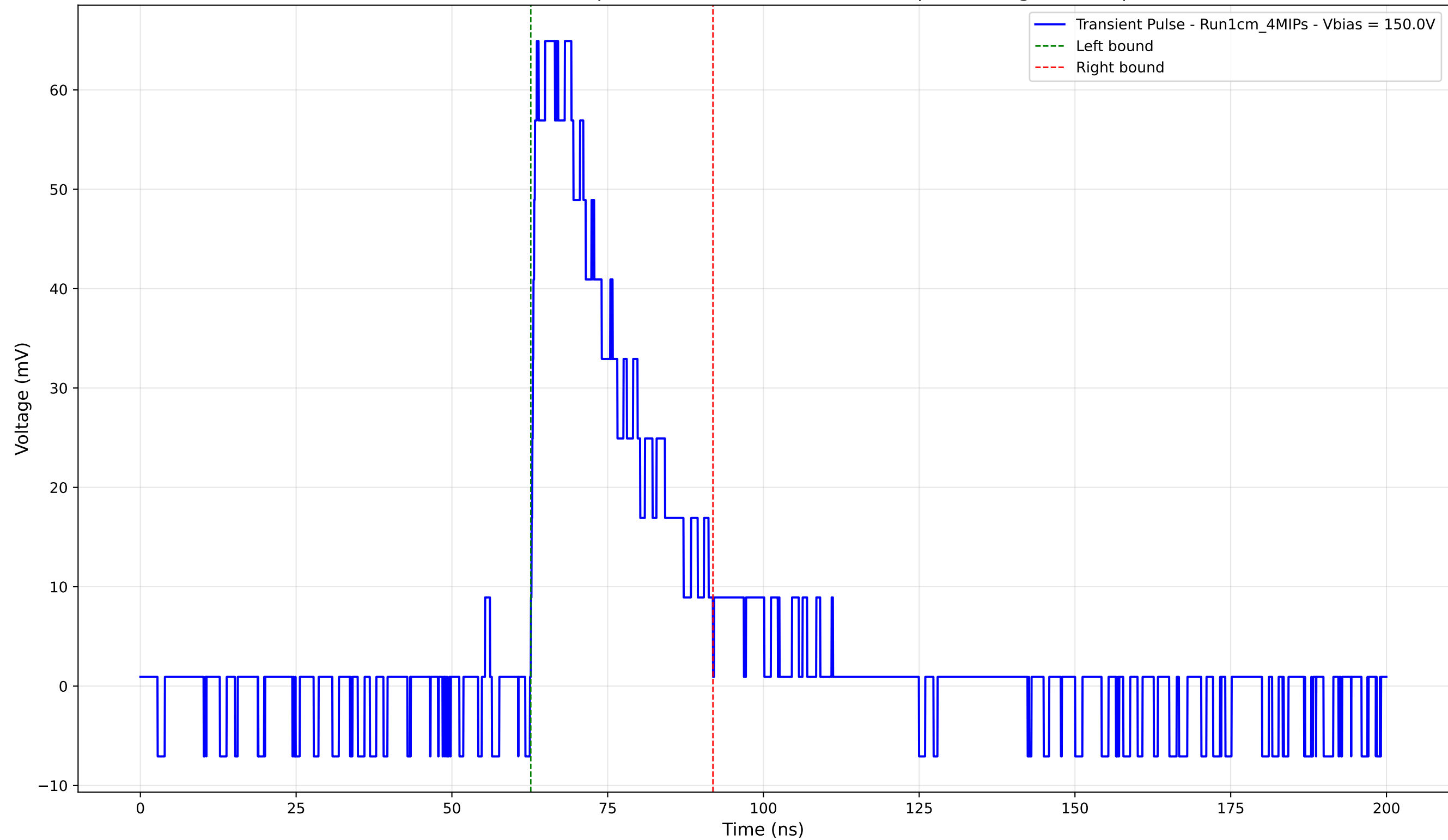
Transient Pulse - Sample: new1cm - Position: 2365.0 \mu\text{m} - Charge: 19.75 pC
