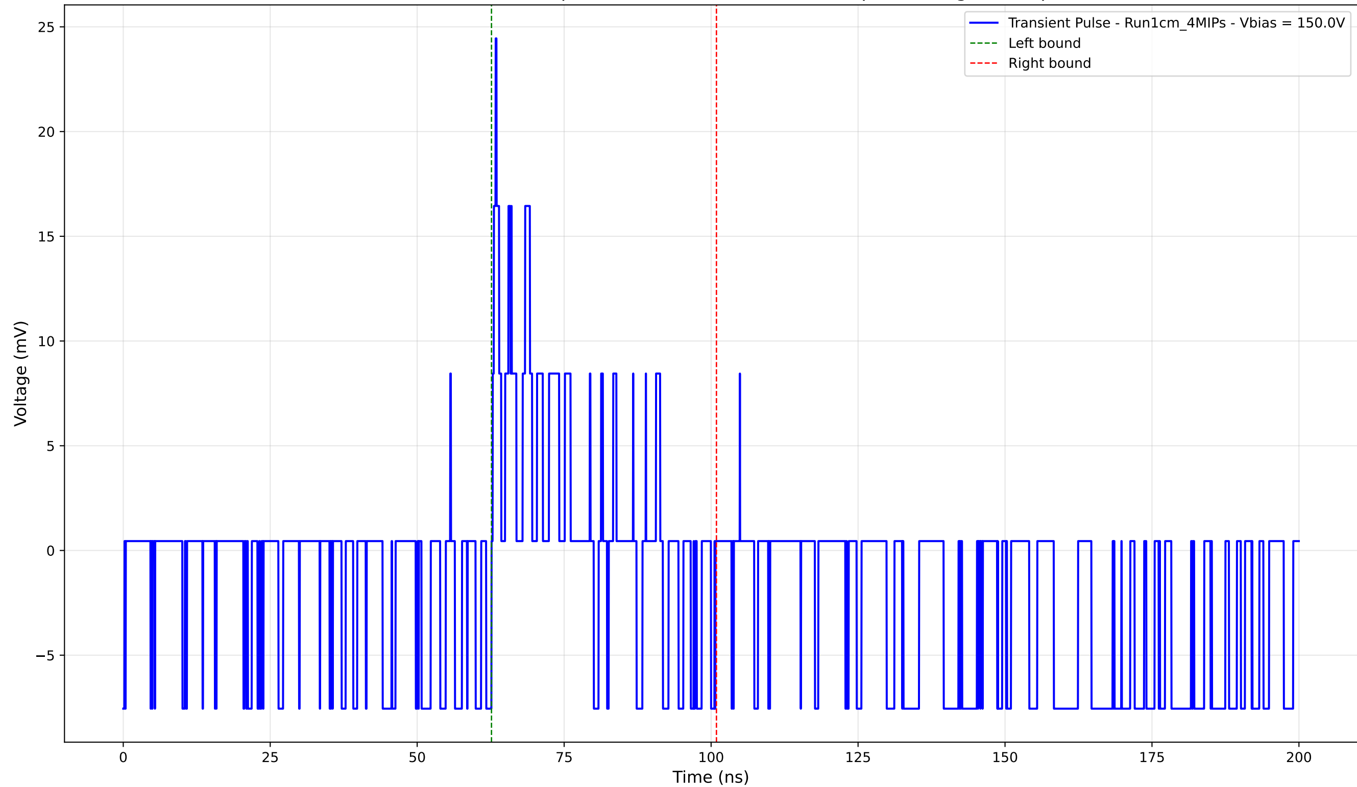
Transient Pulse - Sample: new1cm - Position: 2685.0 \mu\text{m} - Charge: 1.41 pC
