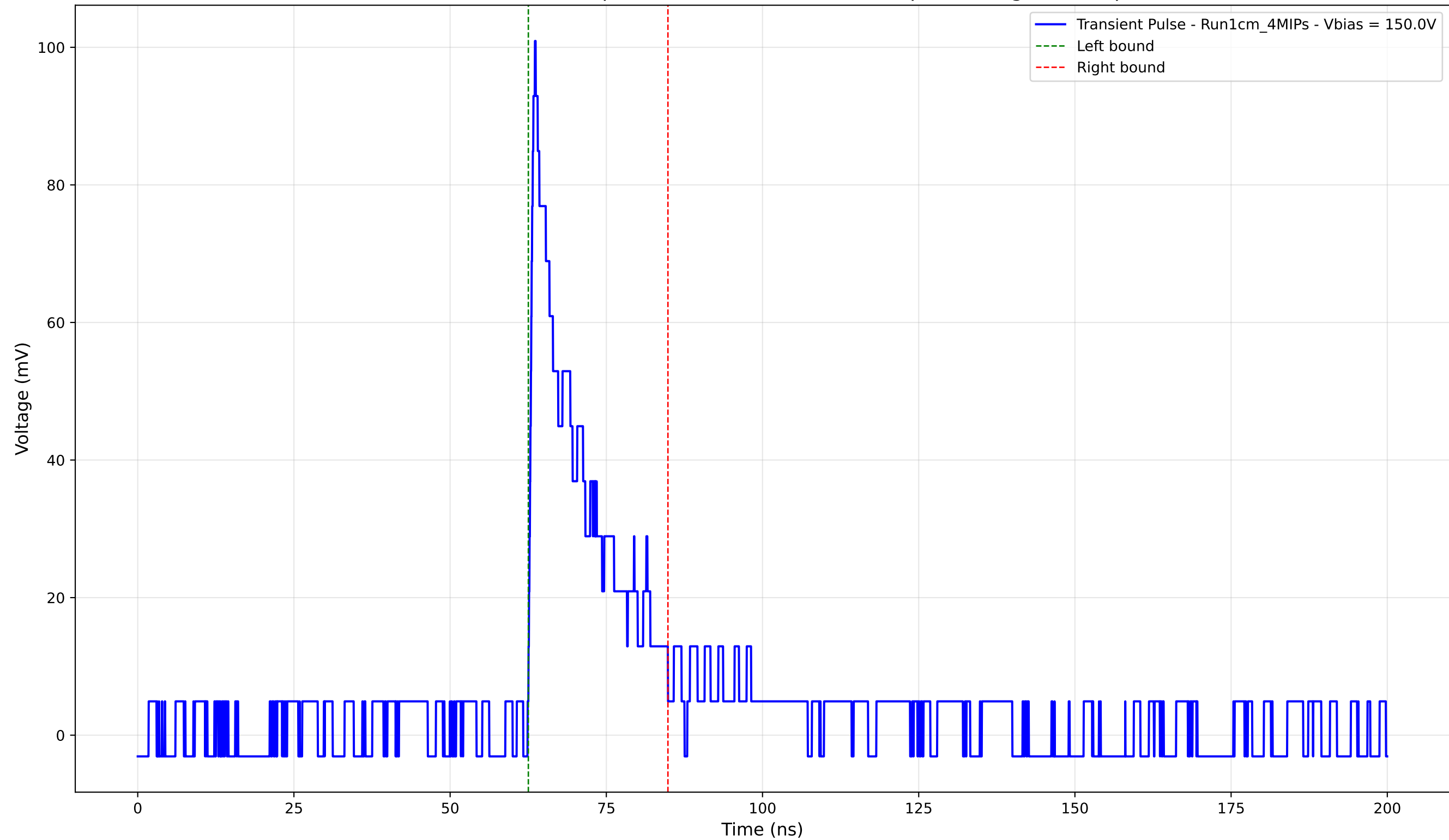
Transient Pulse - Sample: new1cm - Position: 315.0 \mu\text{m} - Charge: 16.20 pC
