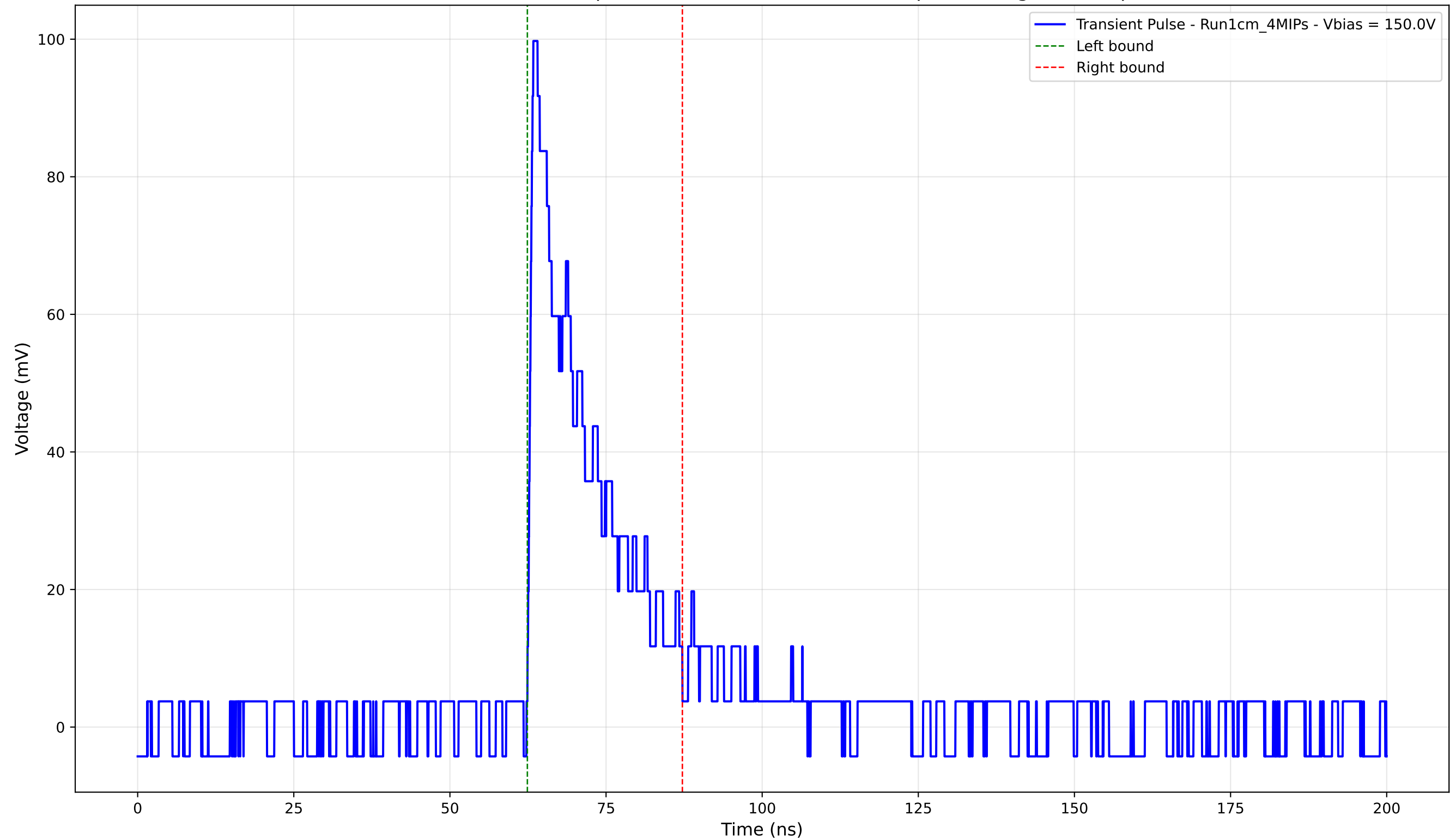
Transient Pulse - Sample: new1cm - Position: 4865.0 \mu\text{m} - Charge: 19.41 pC
