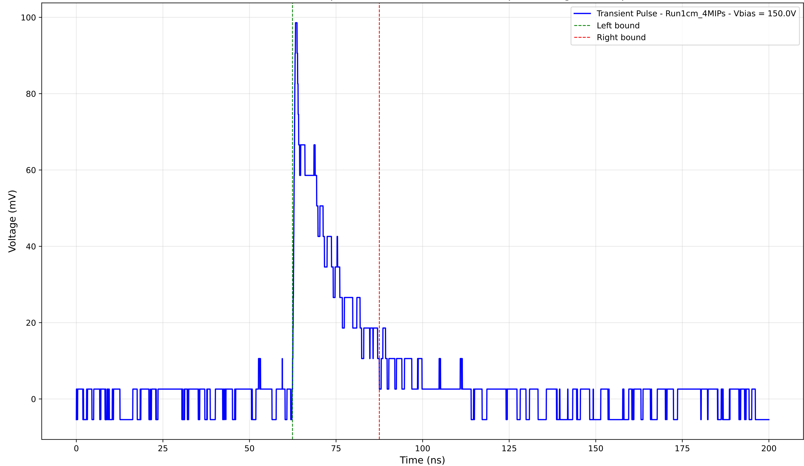
Transient Pulse - Sample: new1cm - Position: 2840.0 \mu\text{m} - Charge: 18.94 pC
