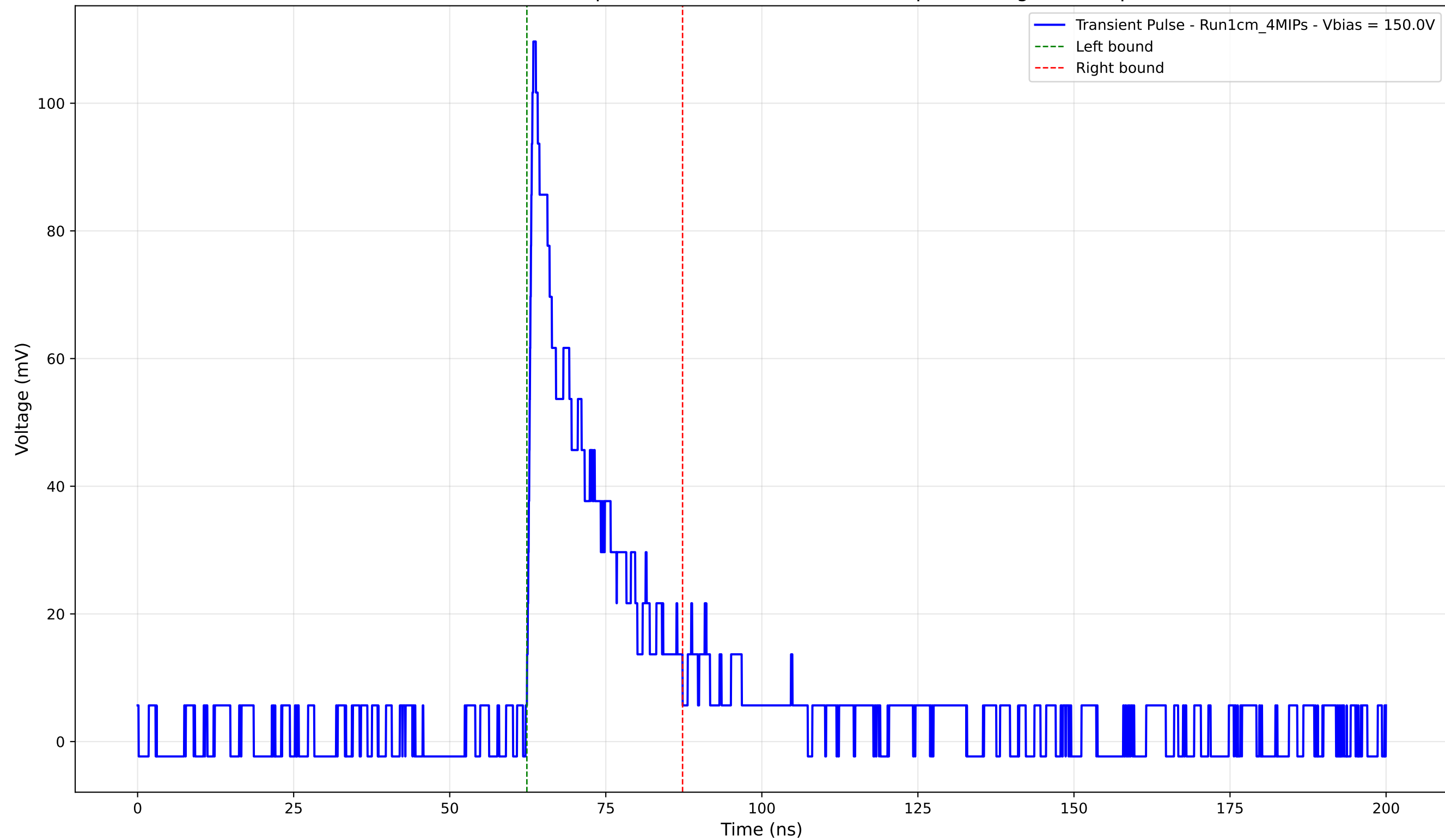
Transient Pulse - Sample: new1cm - Position: 4915.0 \mu\text{m} - Charge: 20.01 pC
