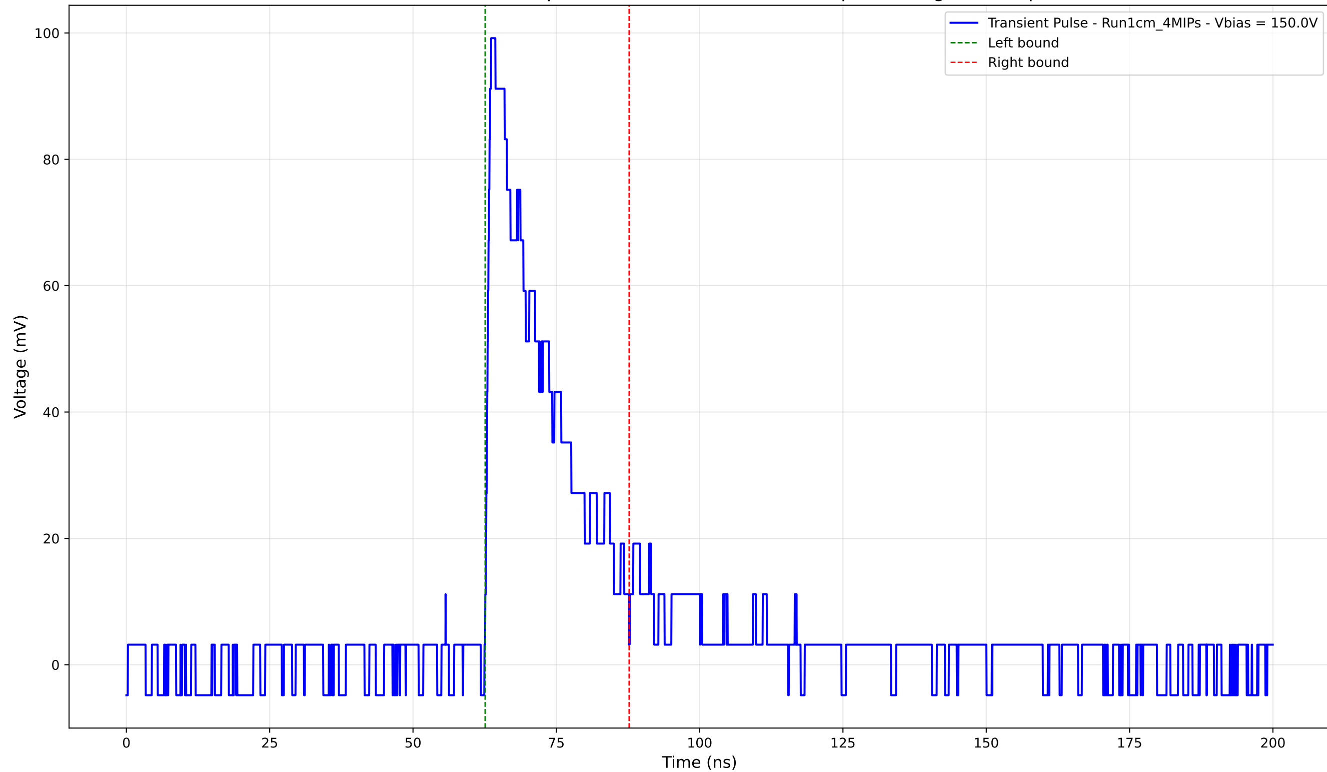
Transient Pulse - Sample: new1cm - Position: 3925.0 \mu\text{m} - Charge: 22.29 pC
