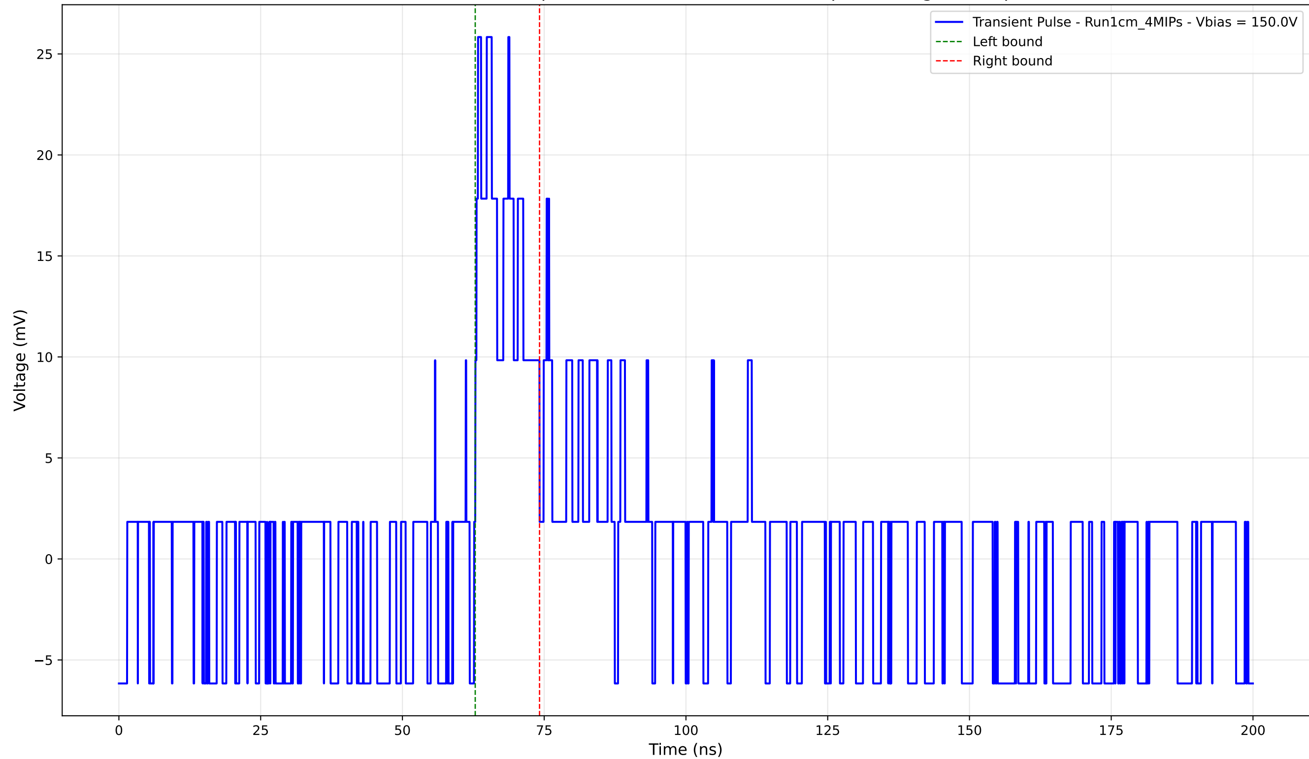
Transient Pulse - Sample: new1cm - Position: 4195.0 \mu\text{m} - Charge: 3.53 pC
