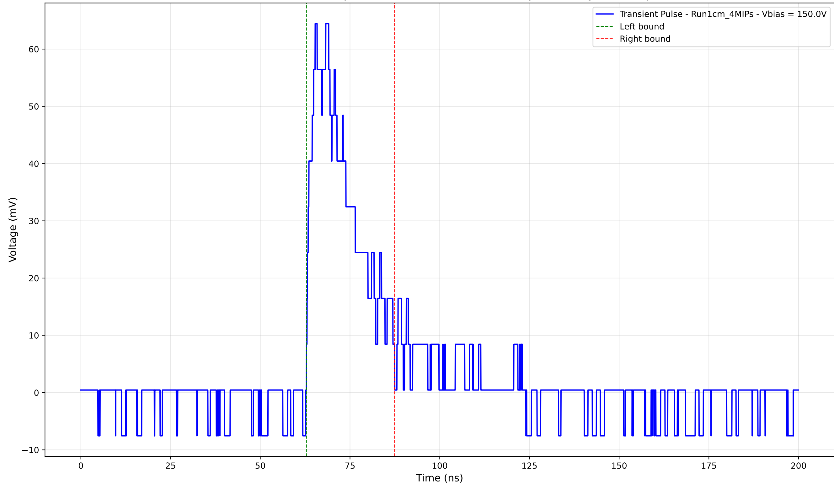
Transient Pulse - Sample: new1cm - Position: 1920.0 \mu\text{m} - Charge: 16.53 pC
