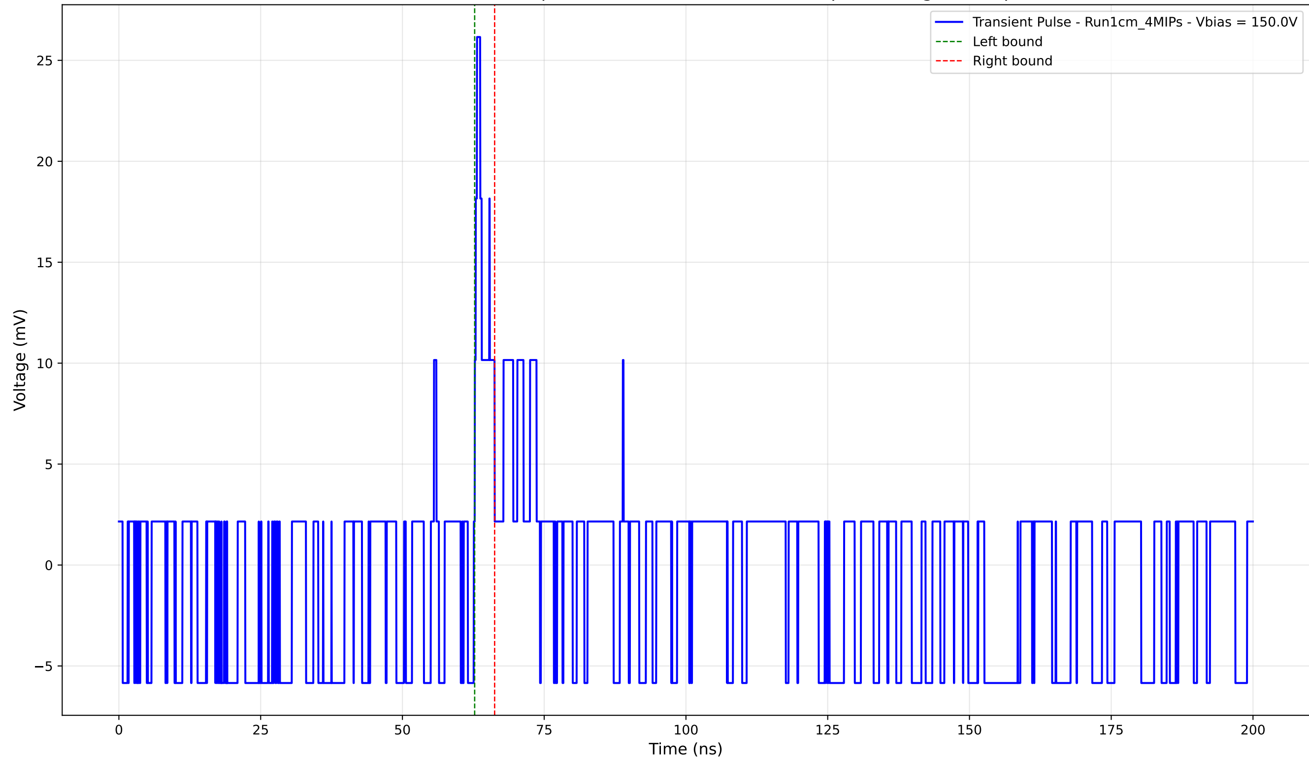
Transient Pulse - Sample: new1cm - Position: 5035.0 \mu\text{m} - Charge: 0.99 pC
