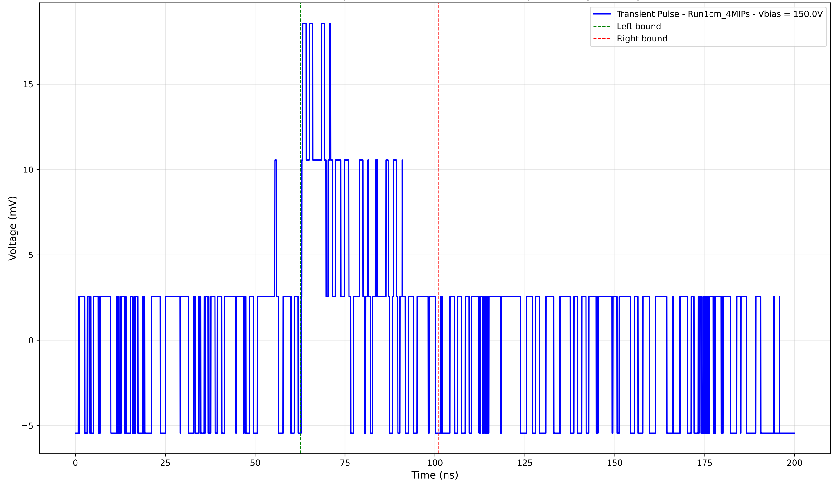
Transient Pulse - Sample: new1cm - Position: 4205.0 \mu\text{m} - Charge: 3.64 pC
