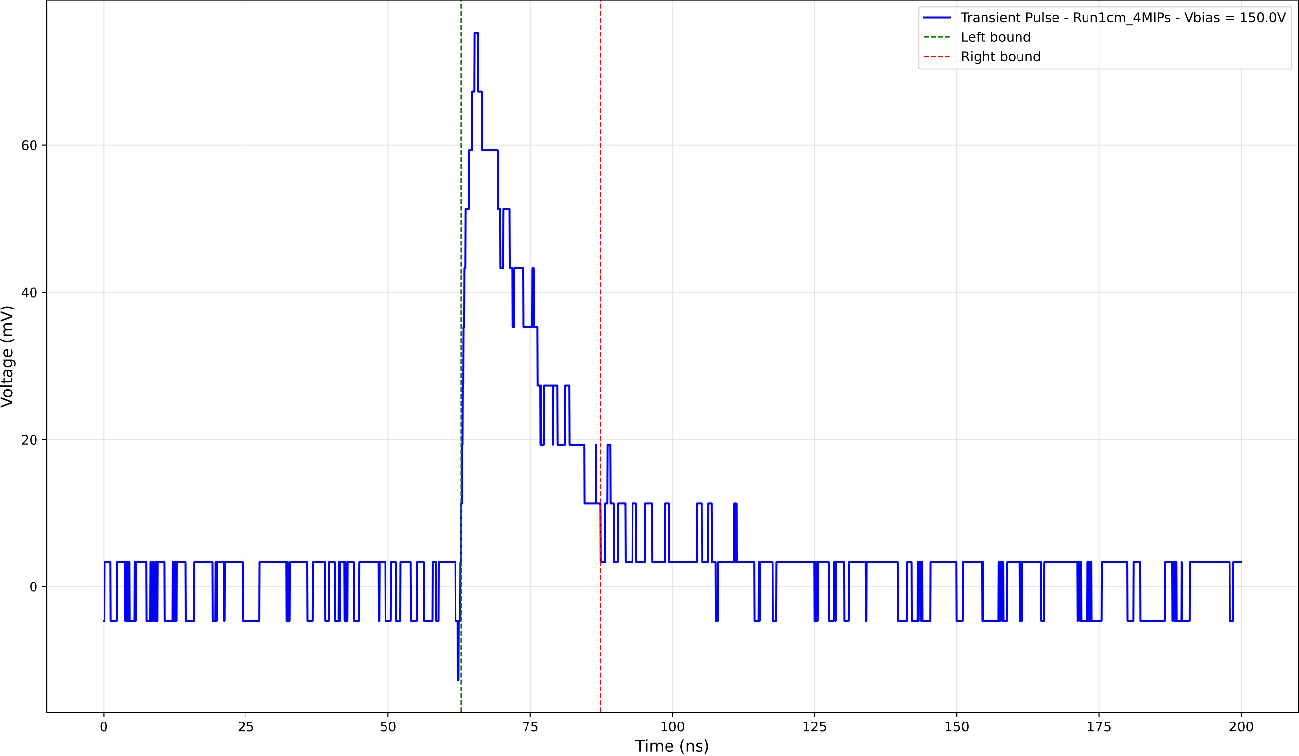
Transient Pulse - Sample: new1cm - Position: 1050.0 \mu\text{m} - Charge: 17.75 pC
