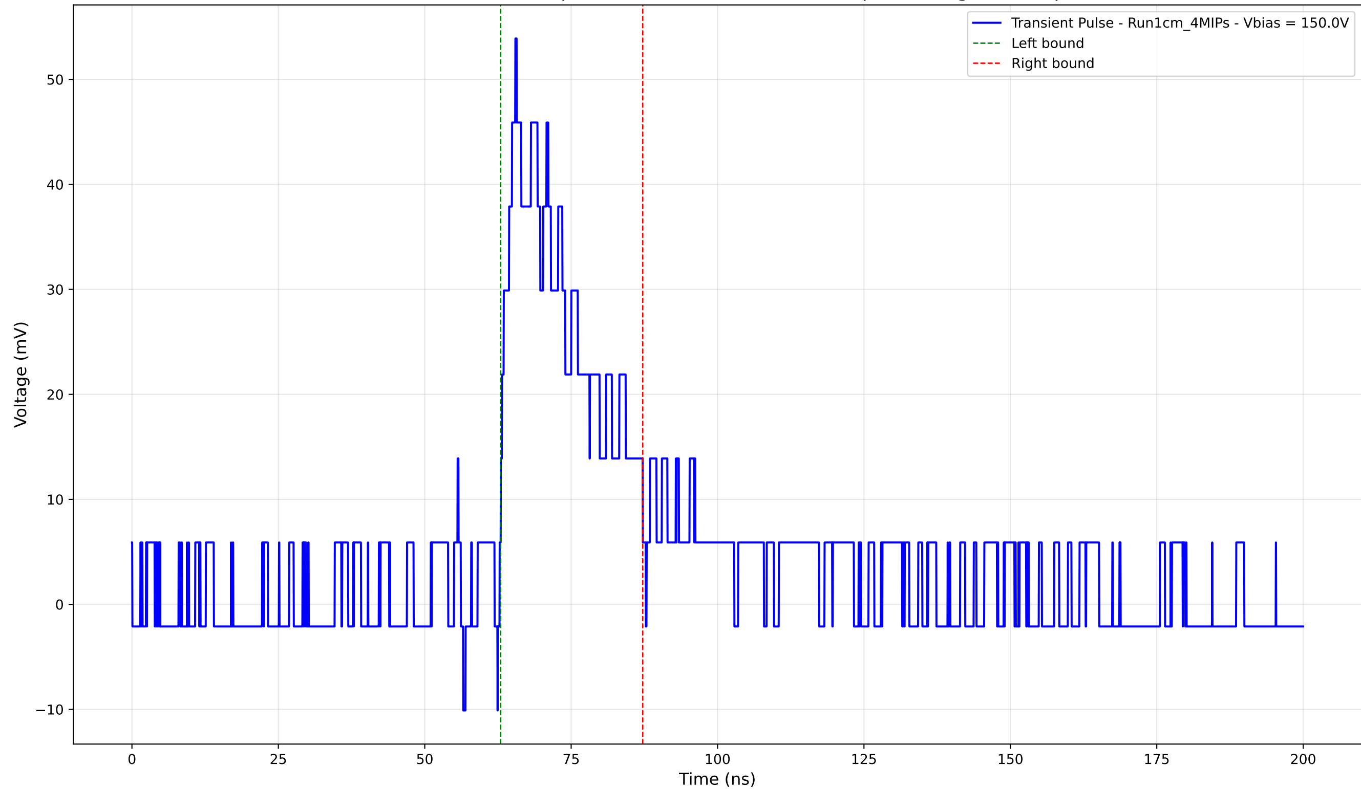
Transient Pulse - Sample: new1cm - Position: 1625.0 \mu\text{m} - Charge: 13.30 pC
