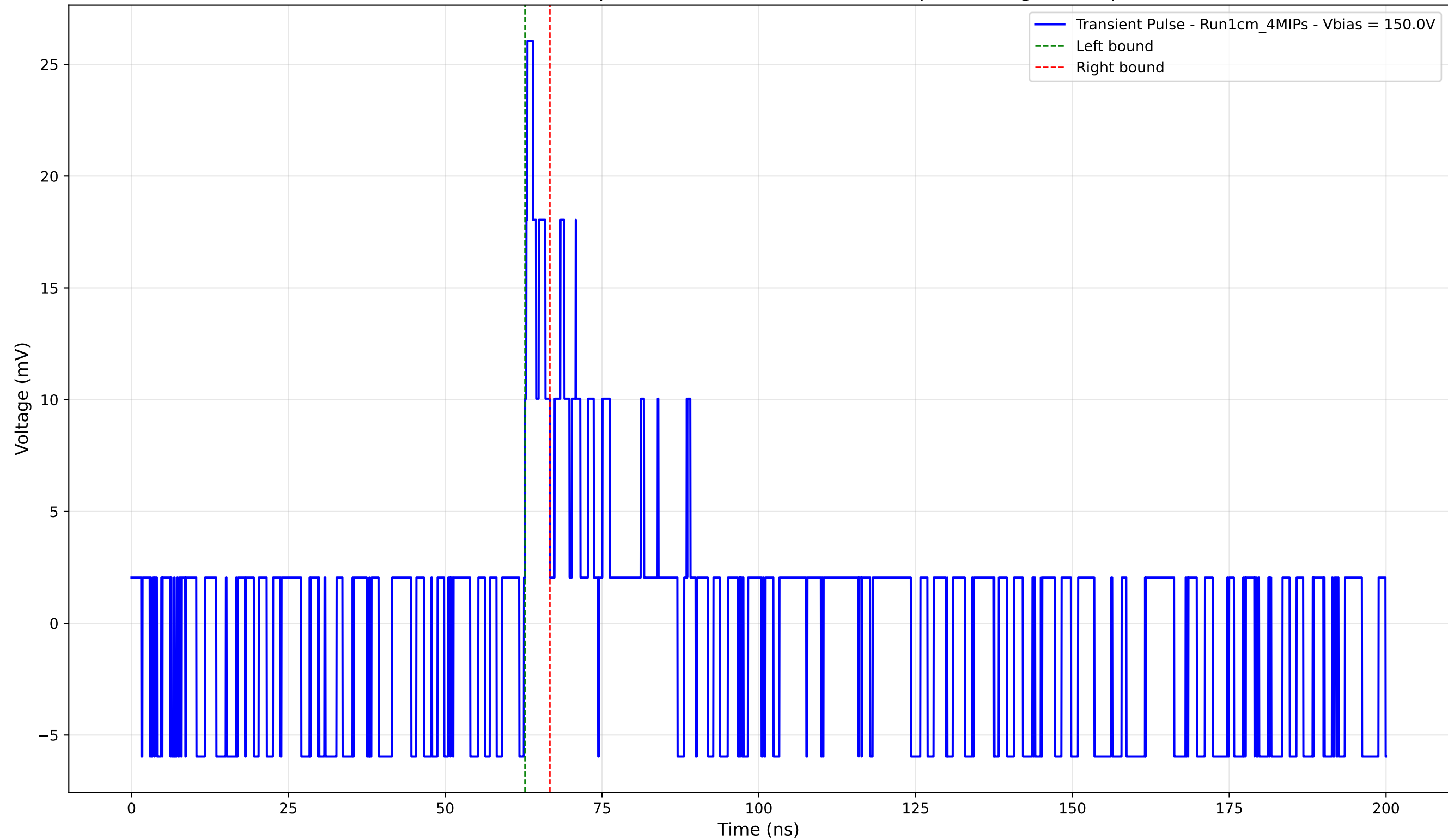
Transient Pulse - Sample: new1cm - Position: 5030.0 \mu\text{m} - Charge: 1.36 pC
