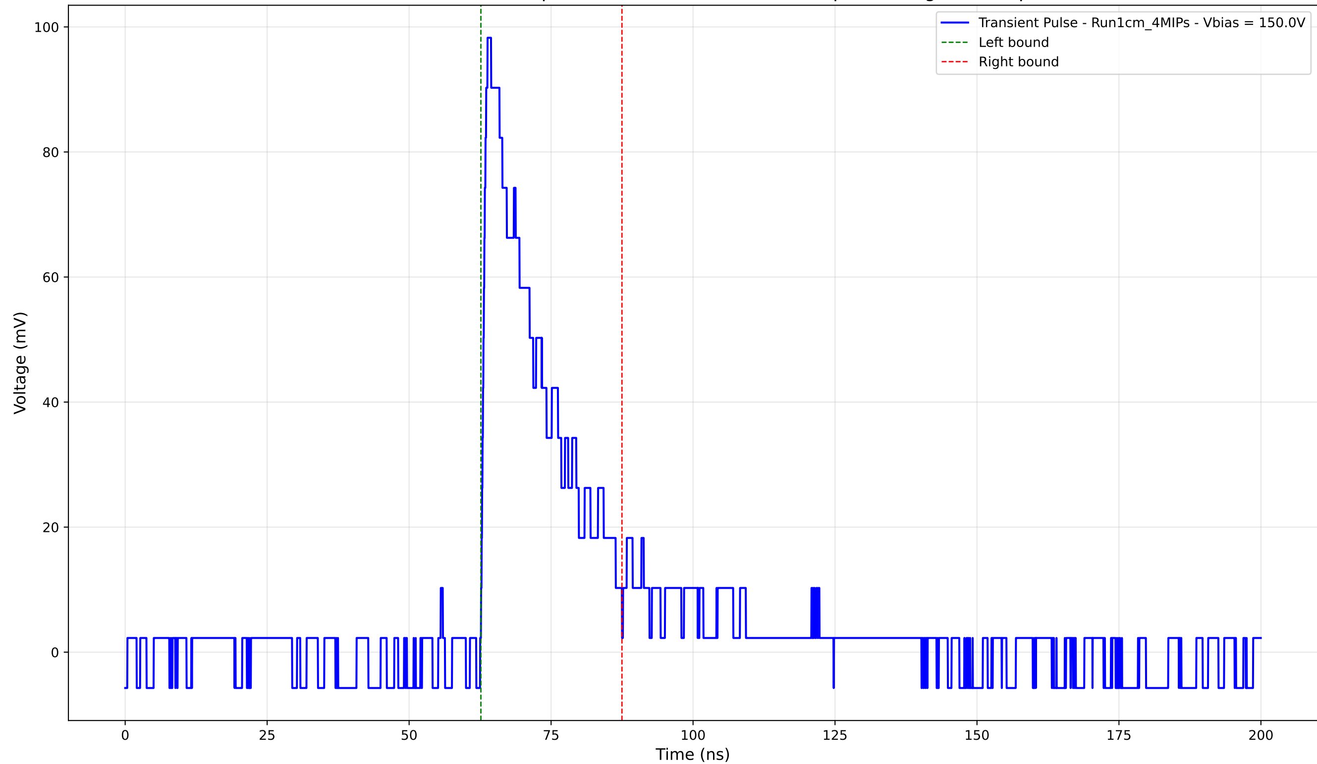
Transient Pulse - Sample: new1cm - Position: 4075.0 \mu\text{m} - Charge: 21.81 pC
