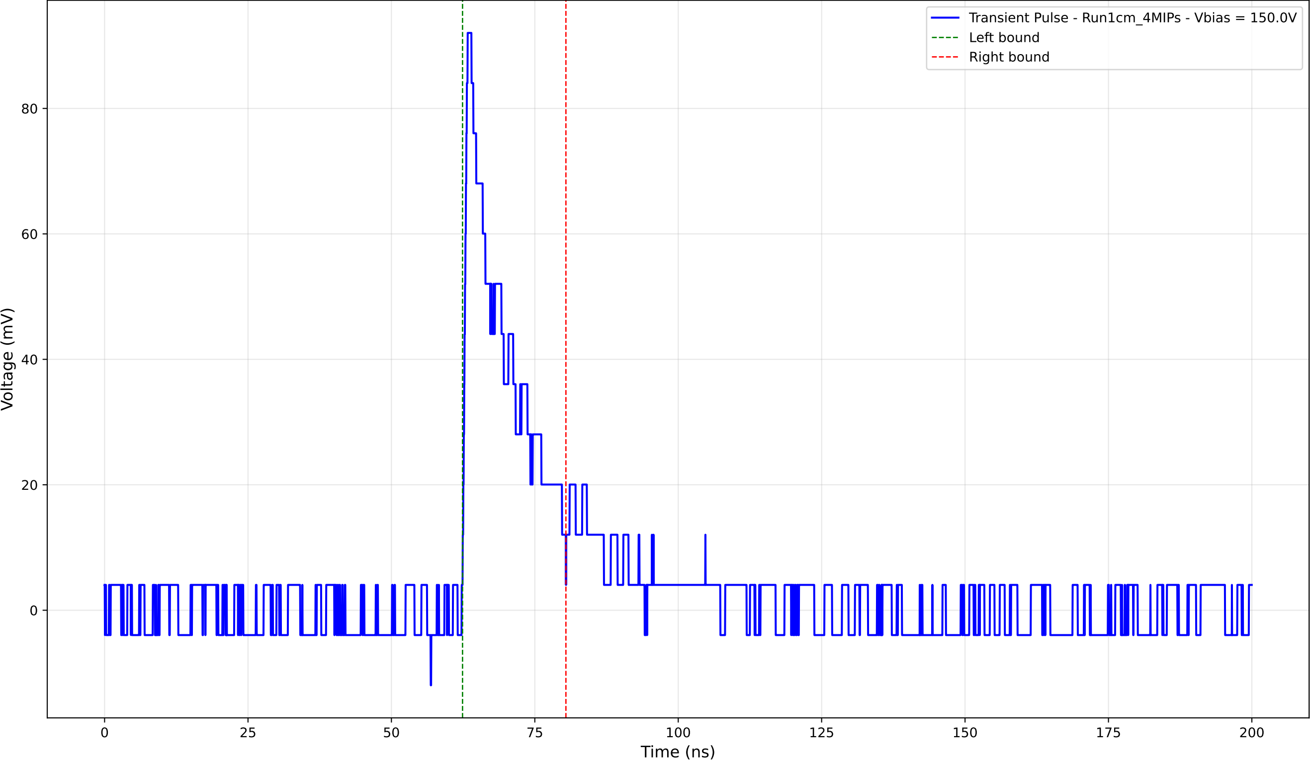
Transient Pulse - Sample: new1cm - Position: 4965.0 \mu\text{m} - Charge: 14.58 pC
