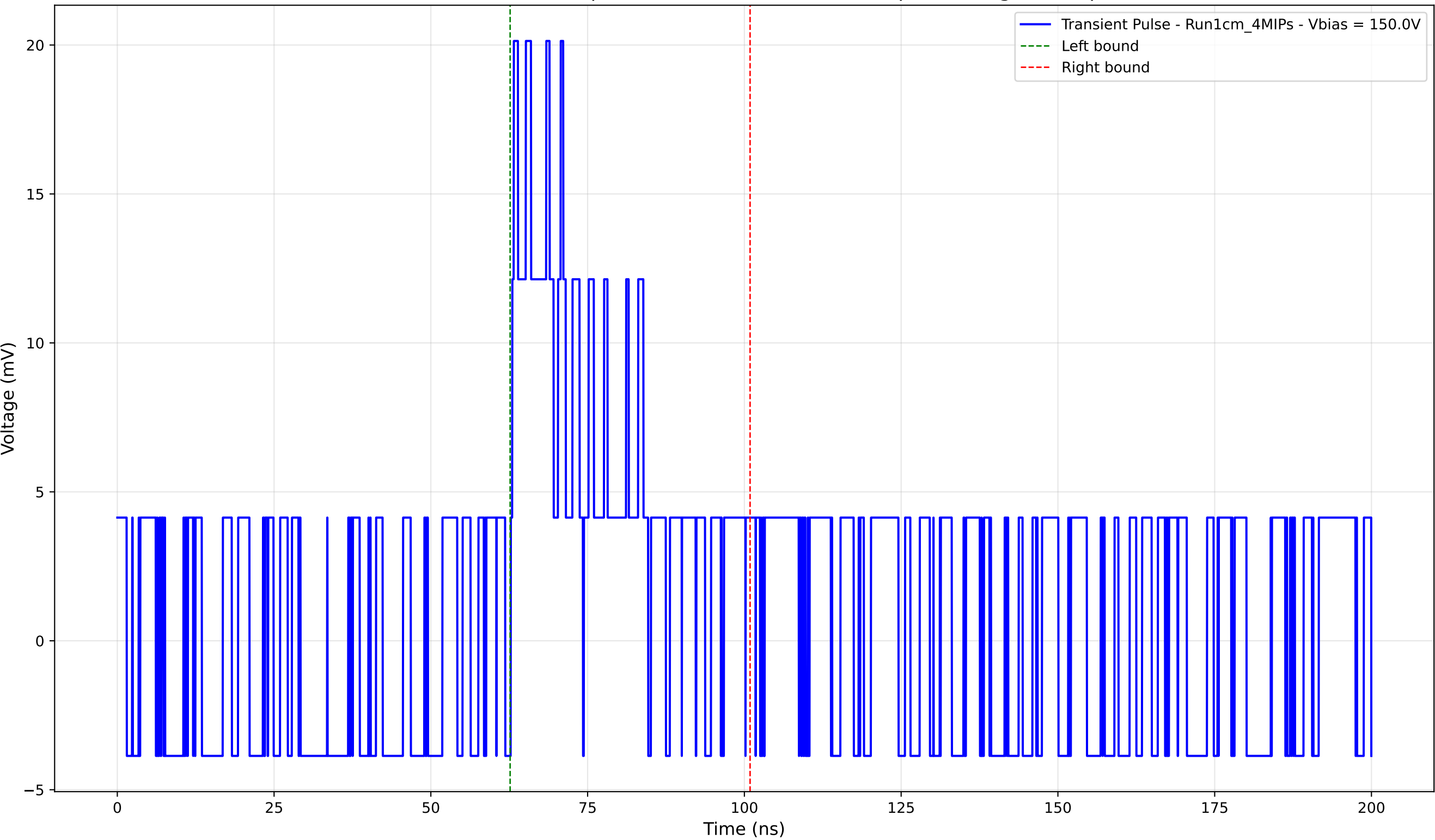
Transient Pulse - Sample: new1cm - Position: 660.0 \mu\text{m} - Charge: 4.98 pC
