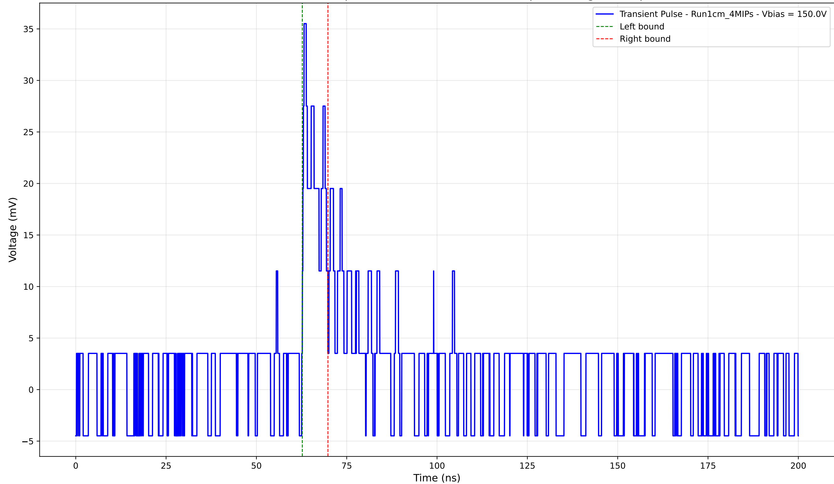
Transient Pulse - Sample: new1cm - Position: 3685.0 \mu\text{m} - Charge: 3.07 pC
