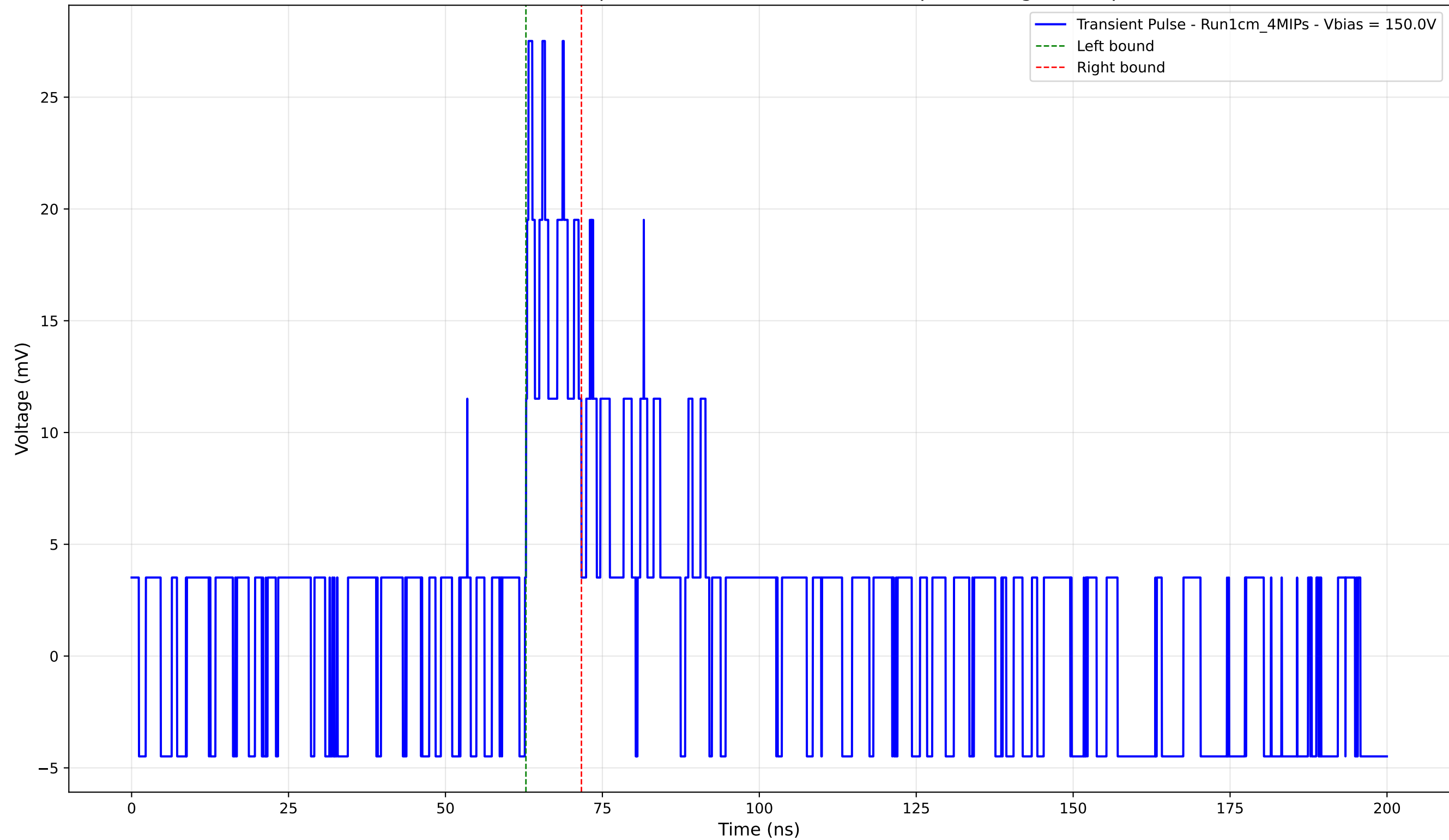
Transient Pulse - Sample: new1cm - Position: 2740.0 \mu\text{m} - Charge: 3.04 pC
