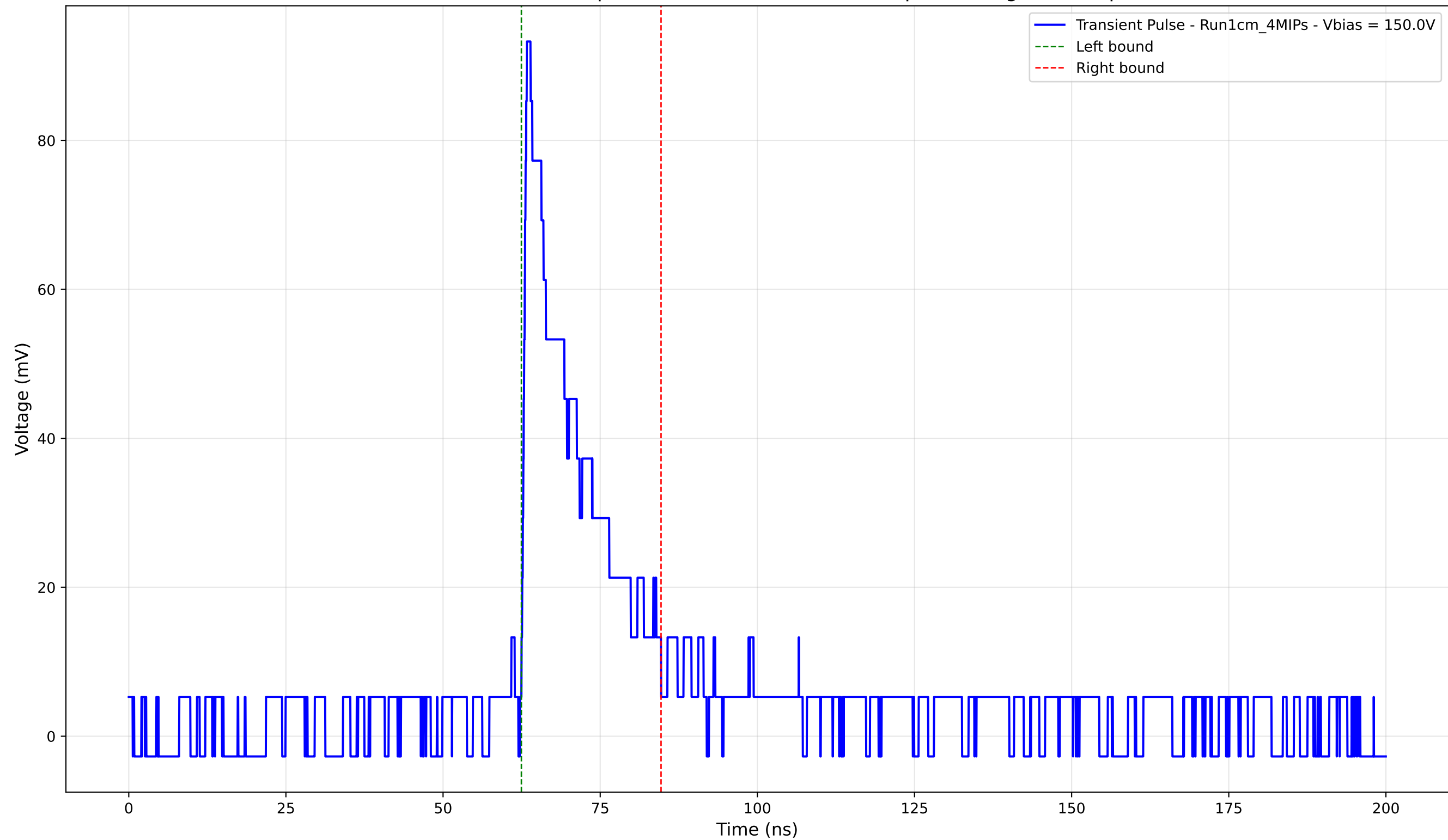
Transient Pulse - Sample: new1cm -Position: 330.0 \mu\text{m} - Charge: 16.76 pC
