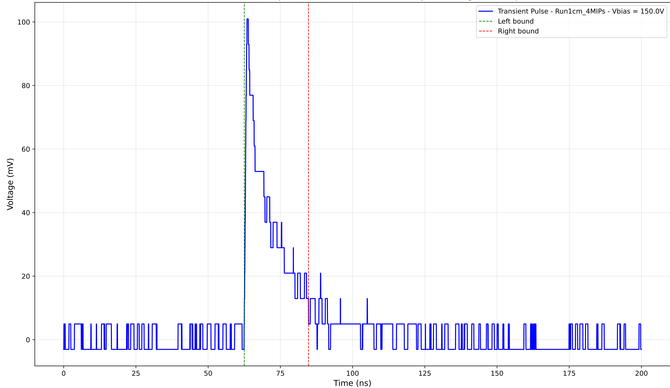
Transient Pulse - Sample: new1cm - Position: 345.0 \mu\text{m} - Charge: 16.71 pC
