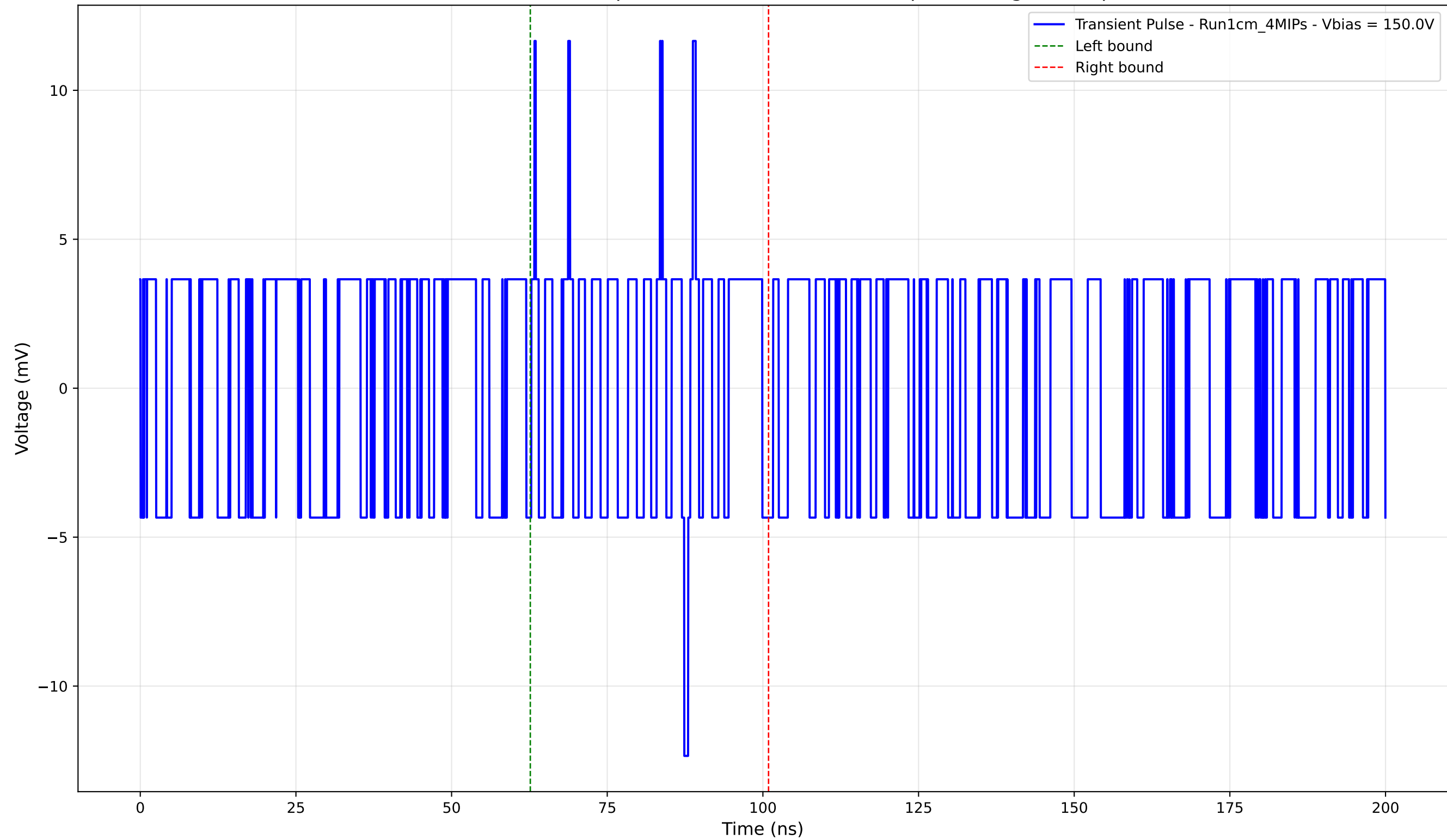
Transient Pulse - Sample: new1cm - Position: 90.0 \mu\text{m} - Charge: 0.46 pC
