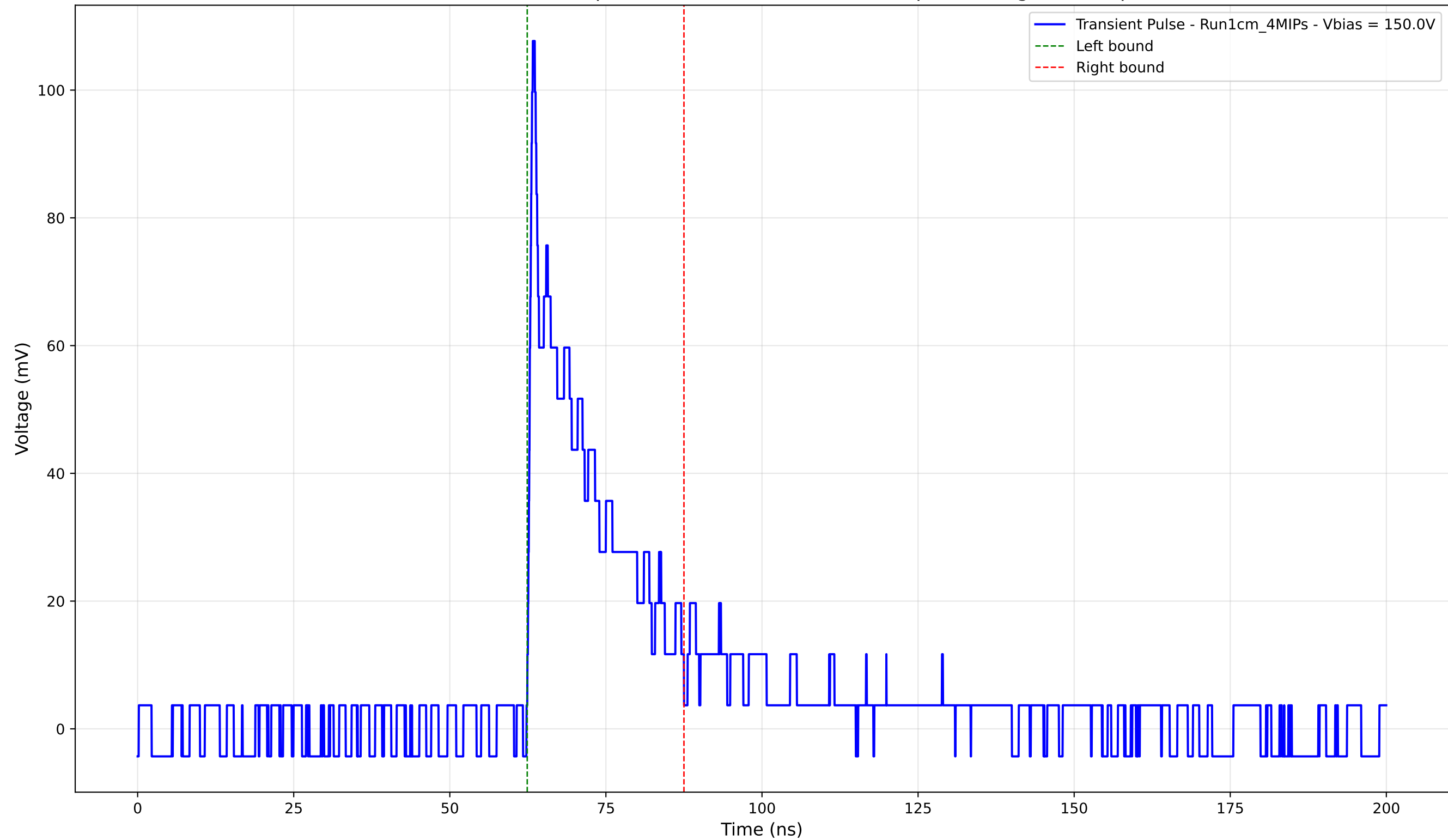
Transient Pulse - Sample: new1cm - Position: 2910.0 \mu\text{m} - Charge: 19.10 pC
