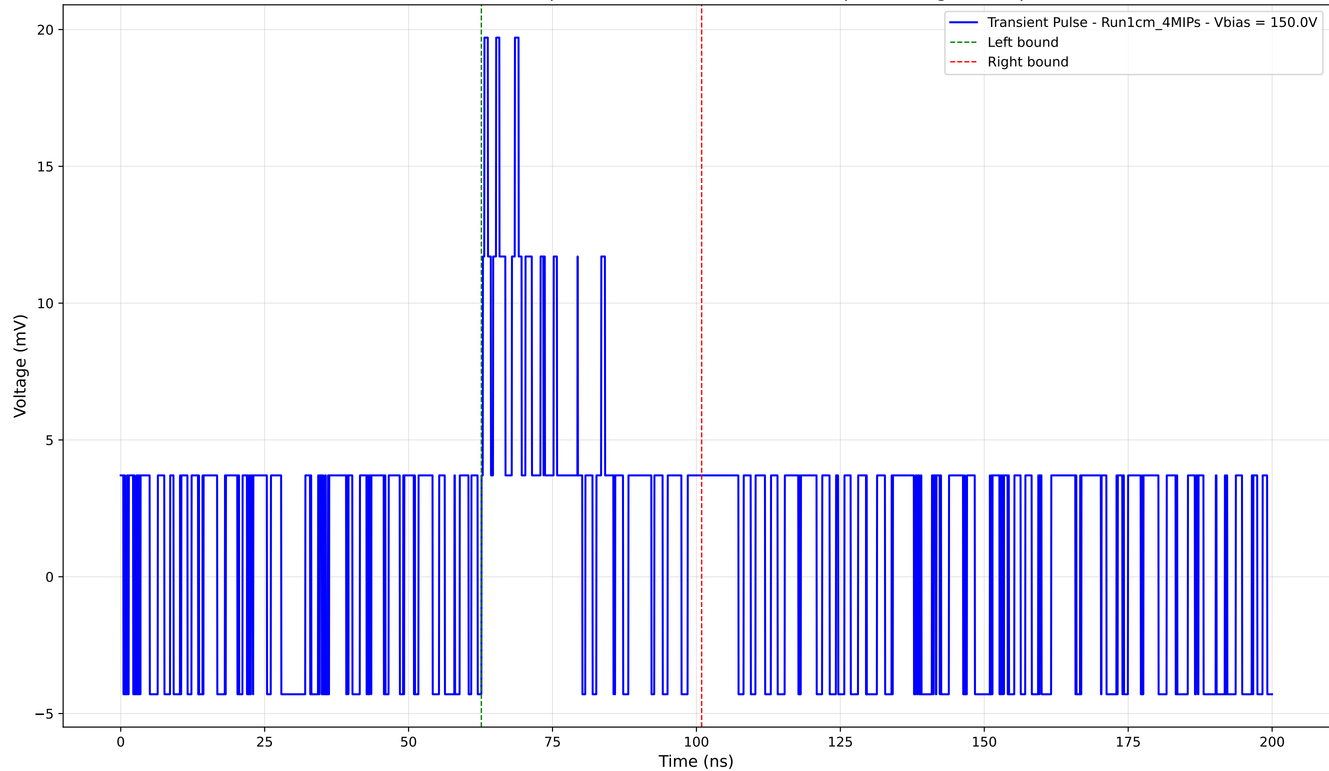
Transient Pulse - Sample: new1cm - Position: 4230.0 \mu\text{m} - Charge: 3.73 pC
