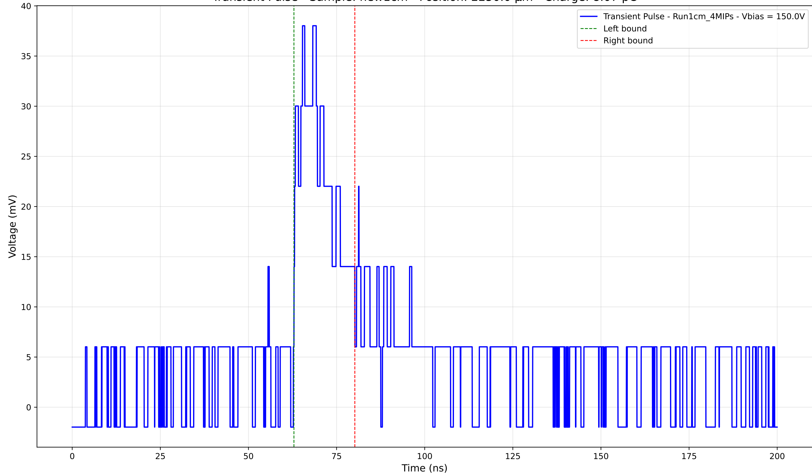
Transient Pulse - Sample: new1cm -Position: 2250.0 \mu\text{m} - Charge: 8.07 pC
