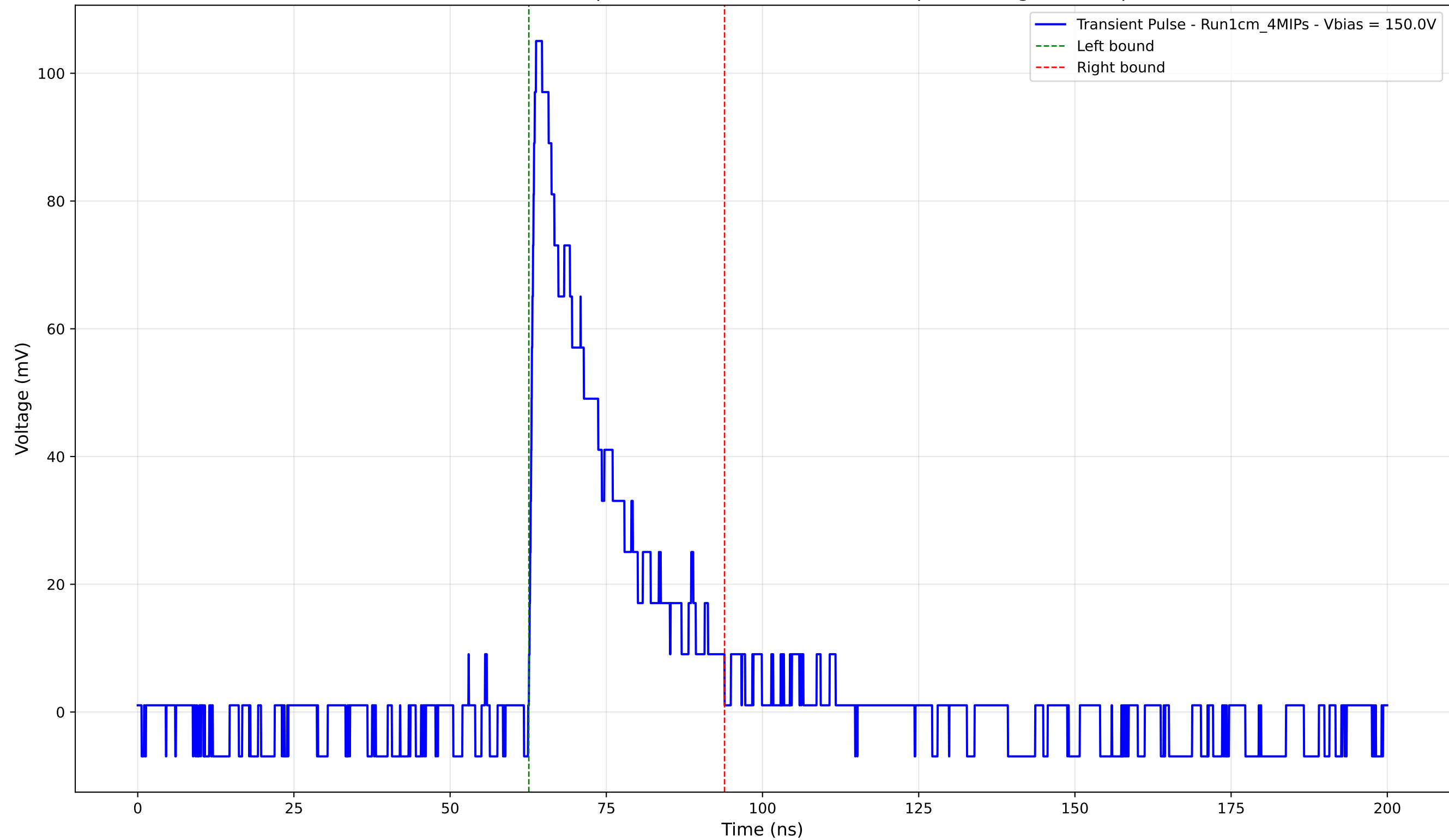
Transient Pulse - Sample: new1cm - Position: 4490.0 \mu\text{m} - Charge: 23.67 pC
