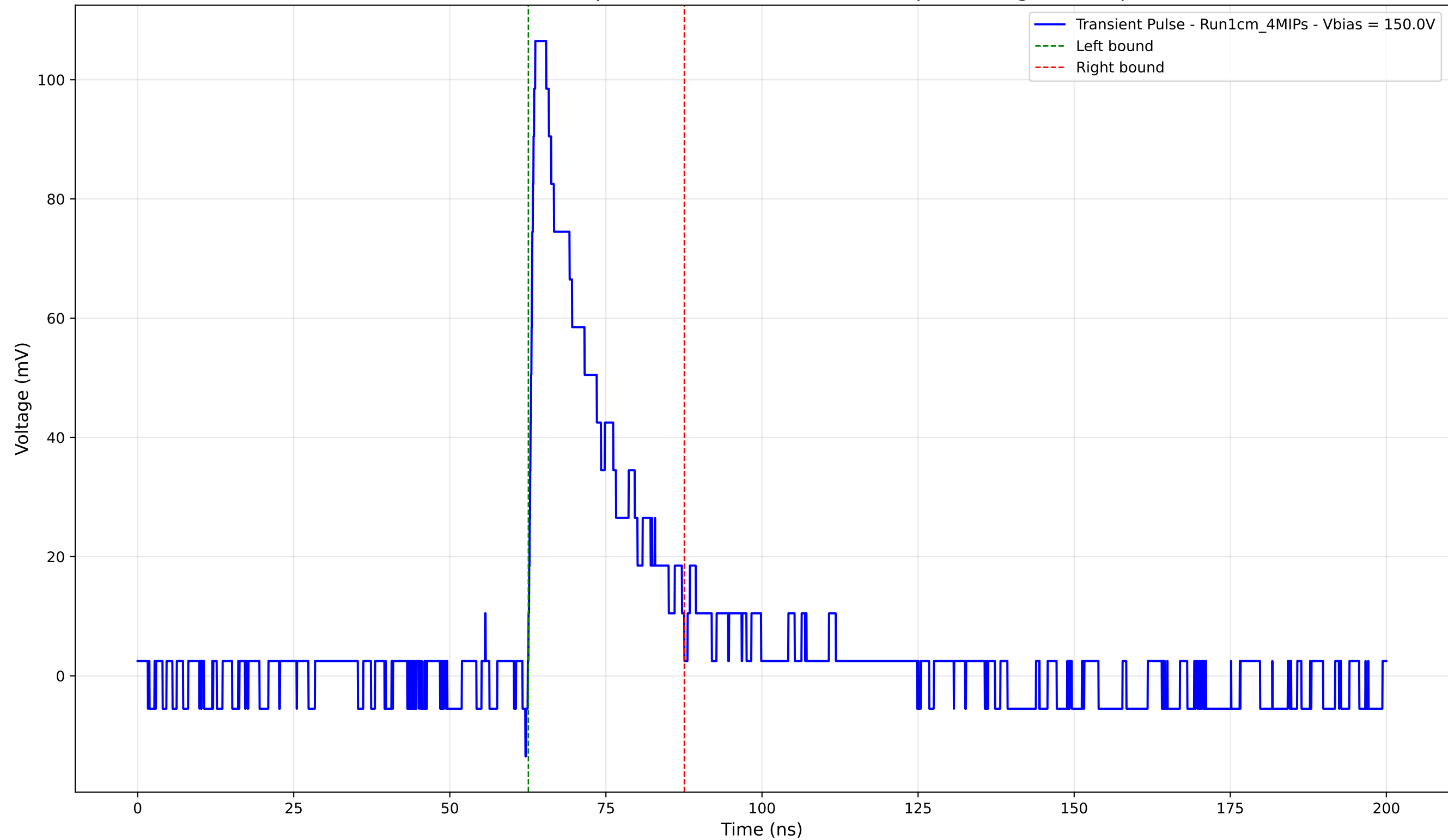
Transient Pulse - Sample: new1cm - Position: 4510.0 \mu\text{m} - Charge: 23.06 pC
