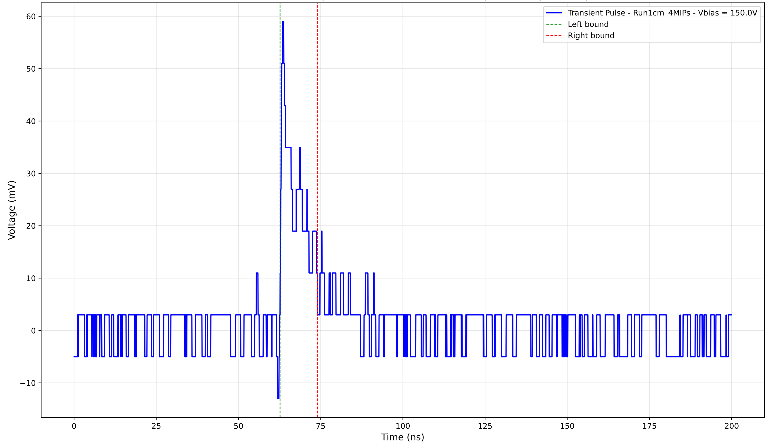
Transient Pulse - Sample: new1cm - Position: 240.0 \mu\text{m} - Charge: 5.89 pC
