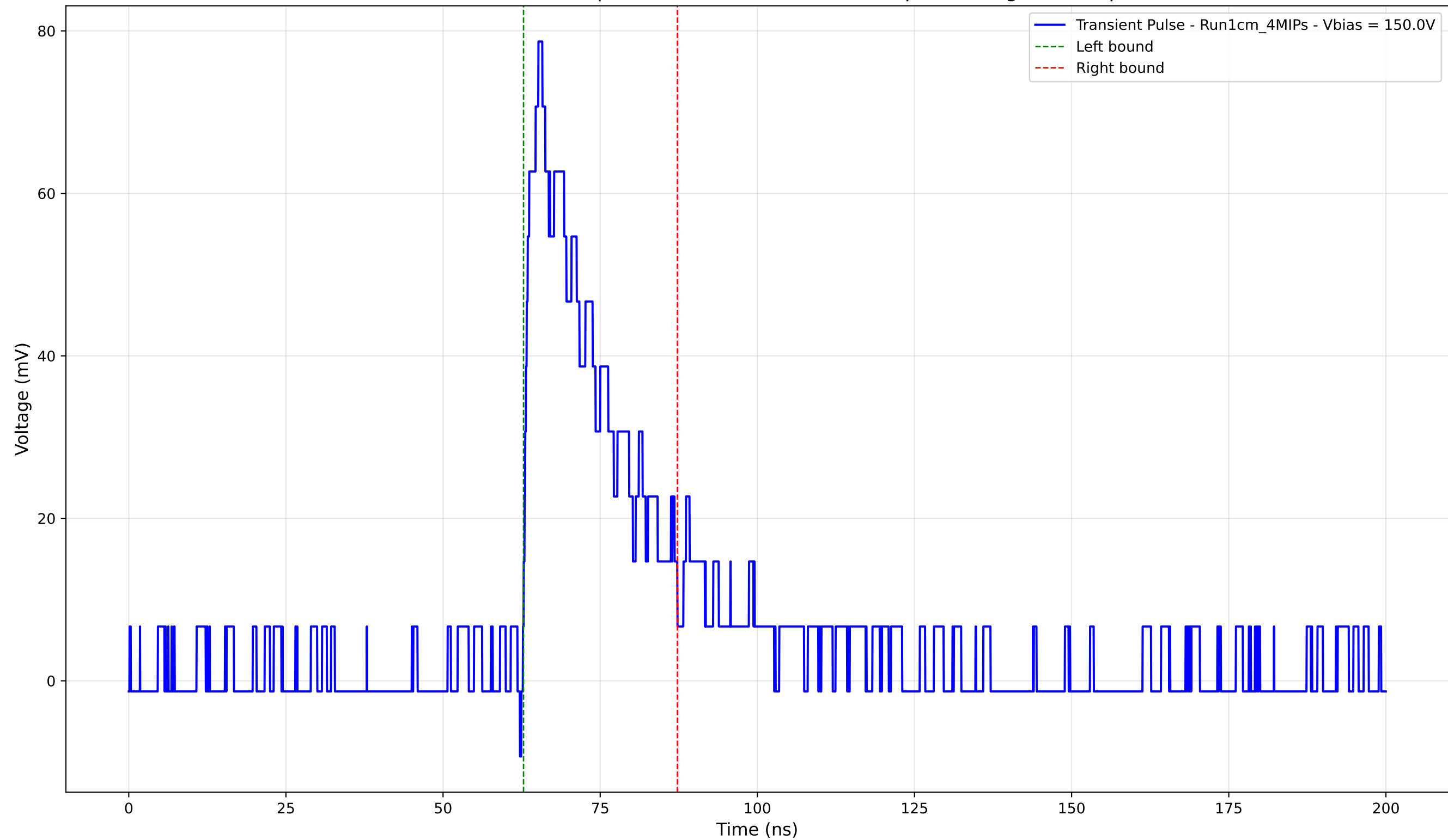
Transient Pulse - Sample: new1cm -Position: 910.0 \mu\text{m} - Charge: 18.91 pC
