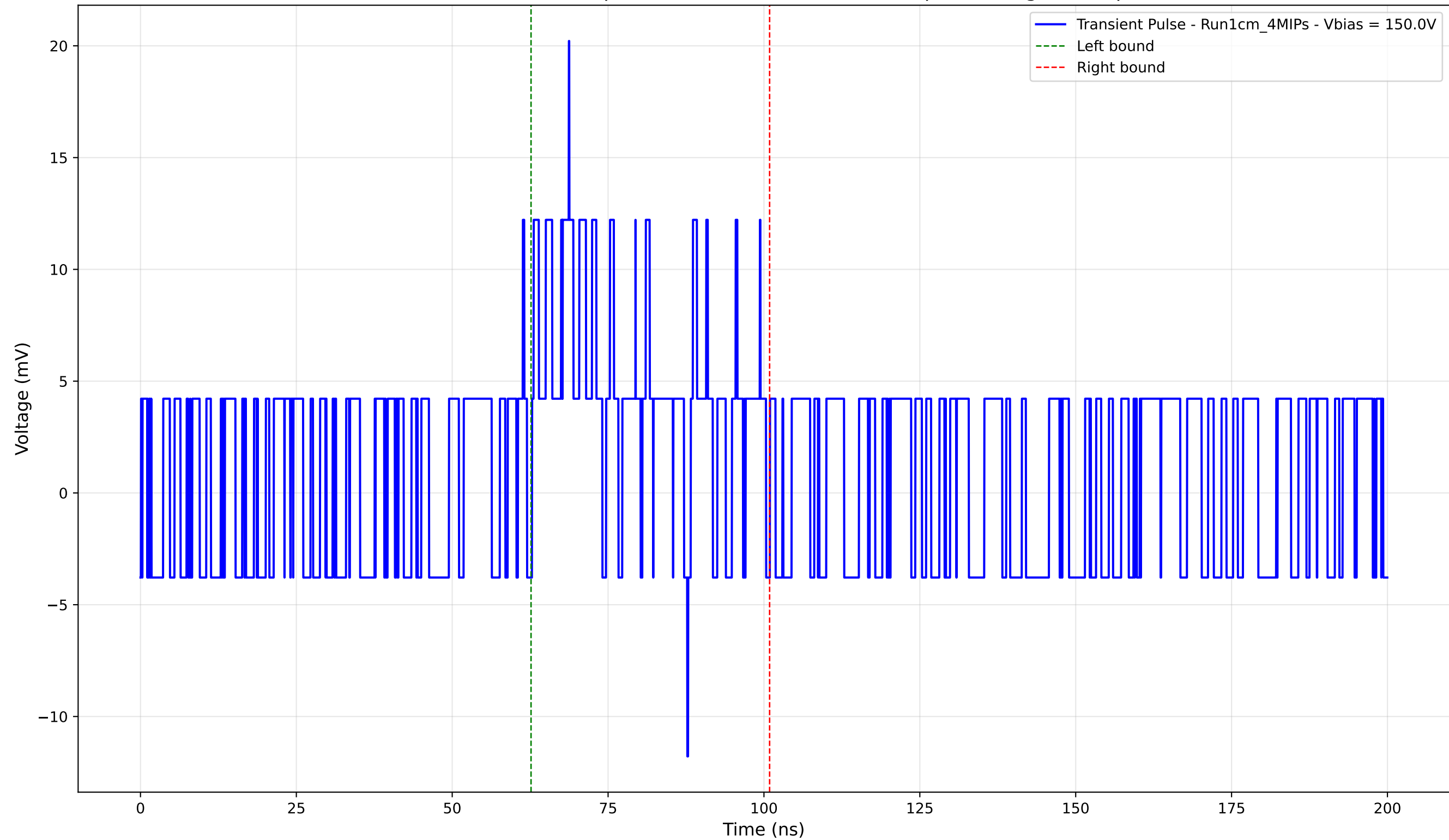
Transient Pulse - Sample: new1cm - Position: 2190.0 \mu\text{m} - Charge: 3.66 pC
