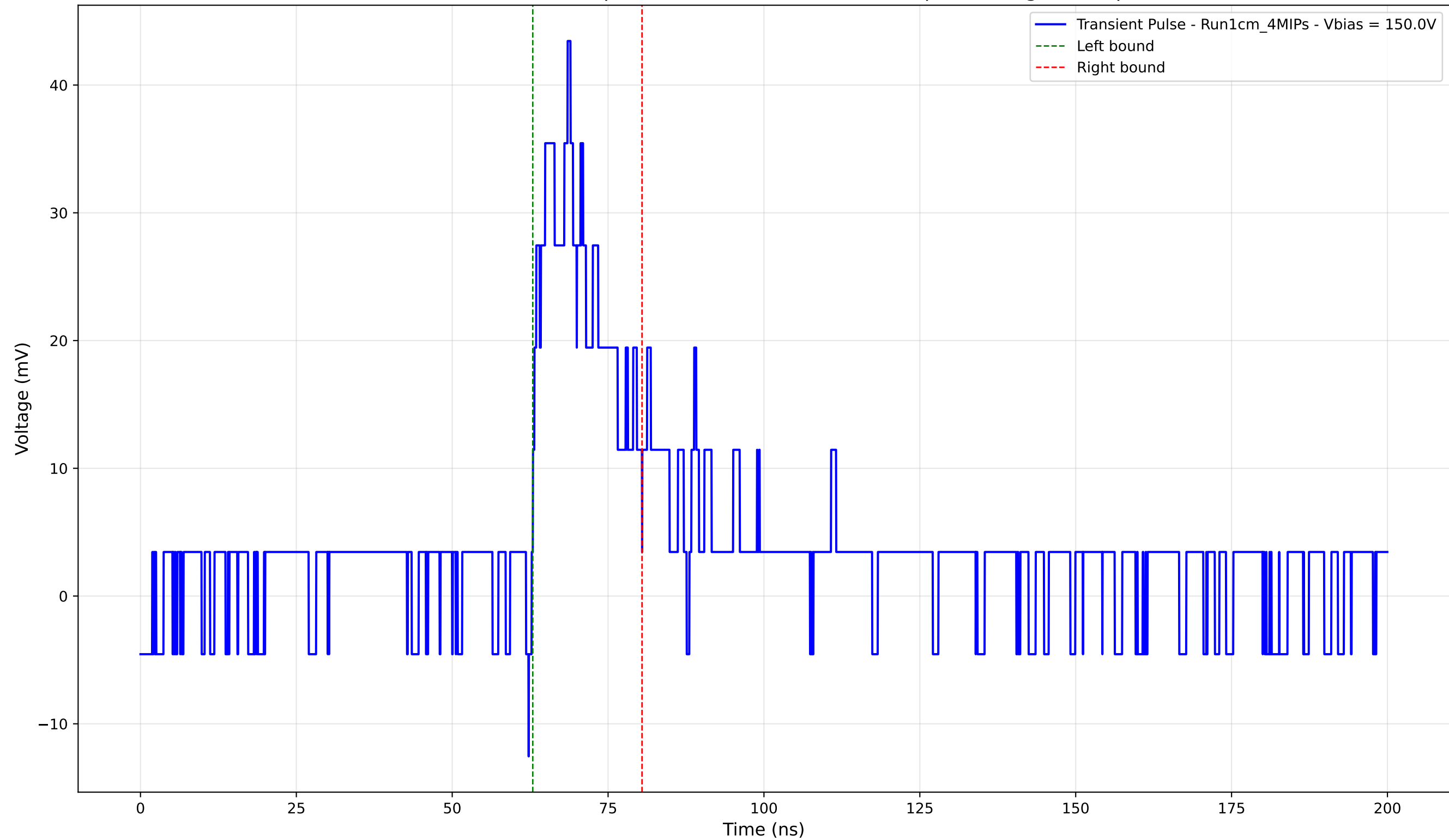
Transient Pulse - Sample: new1cm - Position: 1640.0 \mu\text{m} - Charge: 8.29 pC
