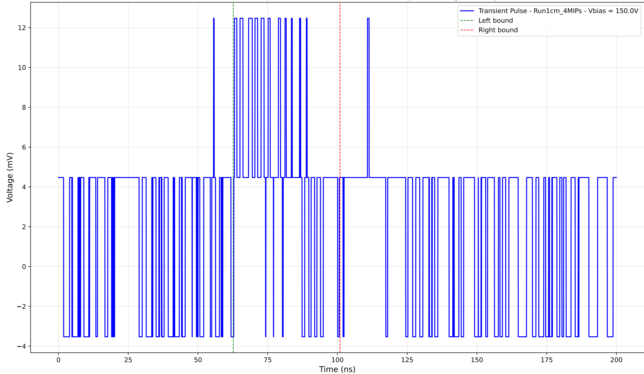
Transient Pulse - Sample: new1cm - Position: 2180.0 \mu\text{m} - Charge: 3.91 pC
