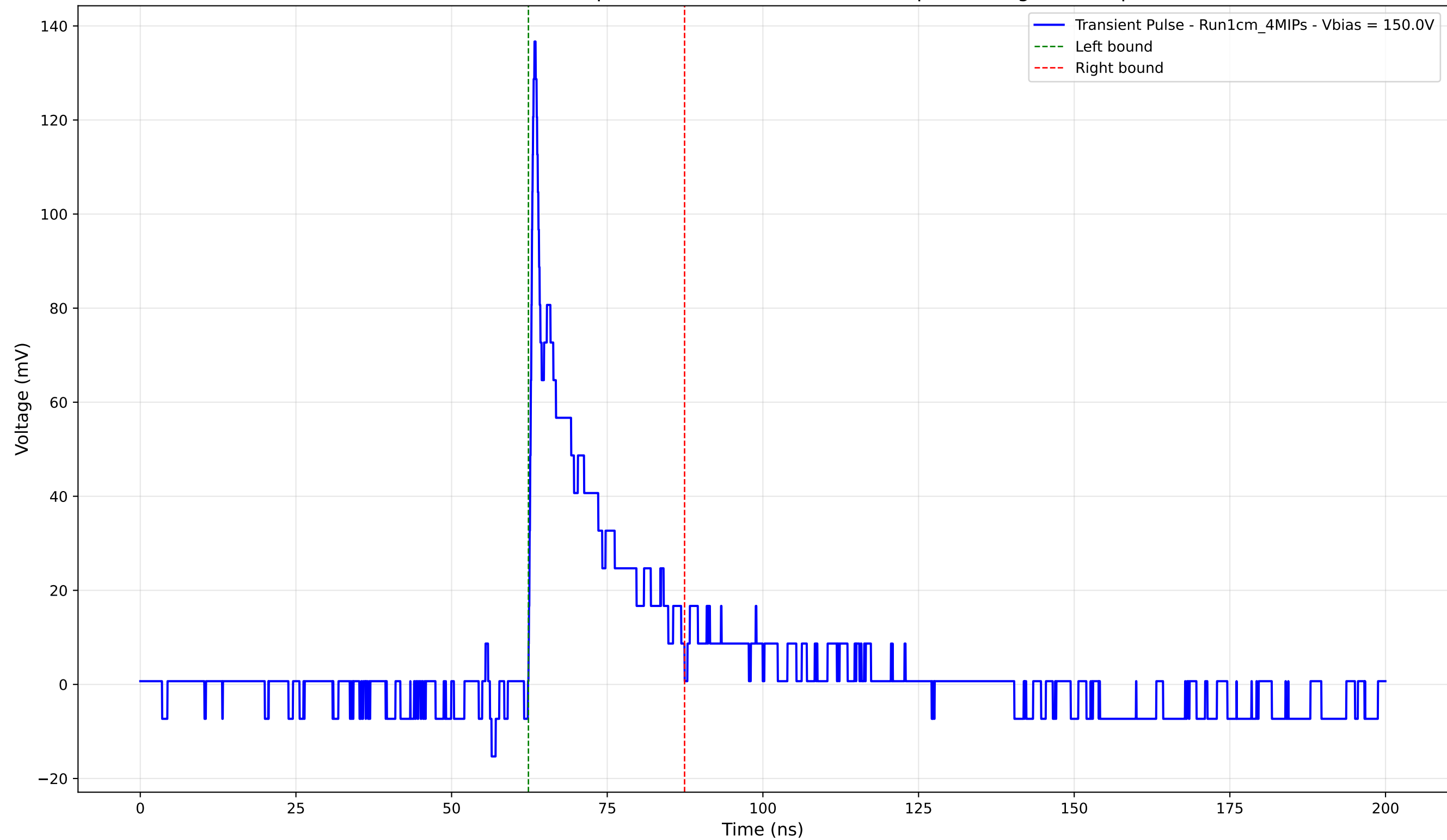
Transient Pulse - Sample: new1cm - Position: 3390.0 \mu\text{m} - Charge: 19.68 pC
