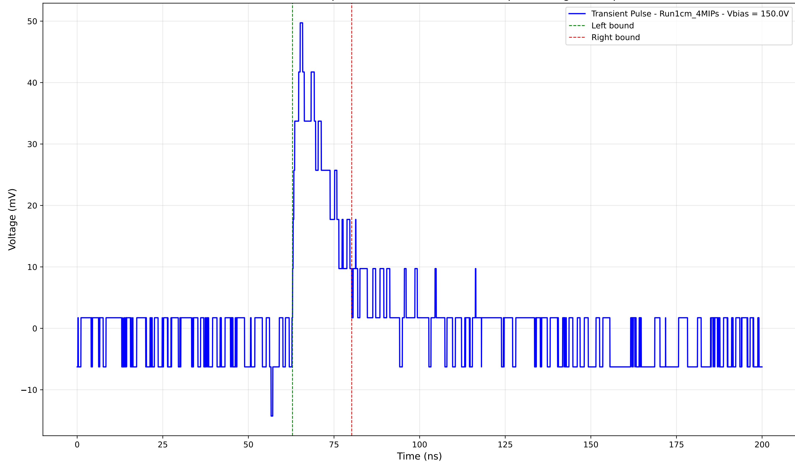
Transient Pulse - Sample: new1cm - Position: 1125.0 \mu\text{m} - Charge: 9.12 pC
