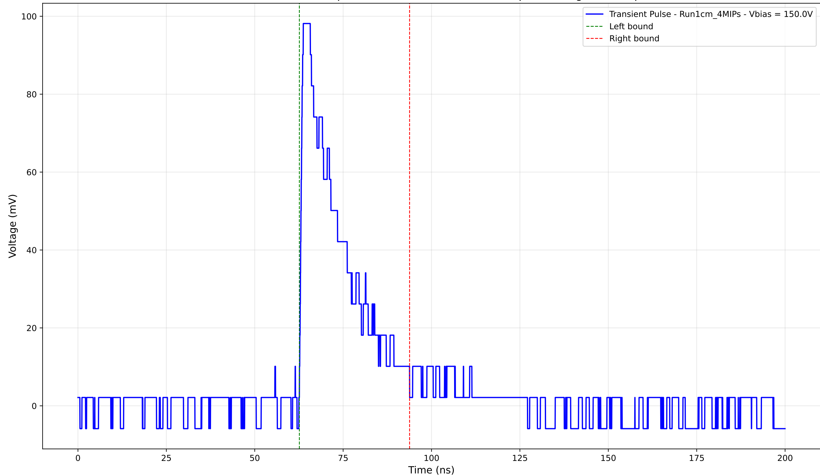
Transient Pulse - Sample: new1cm - Position: 4405.0 \mu\text{m} - Charge: 24.24 pC
