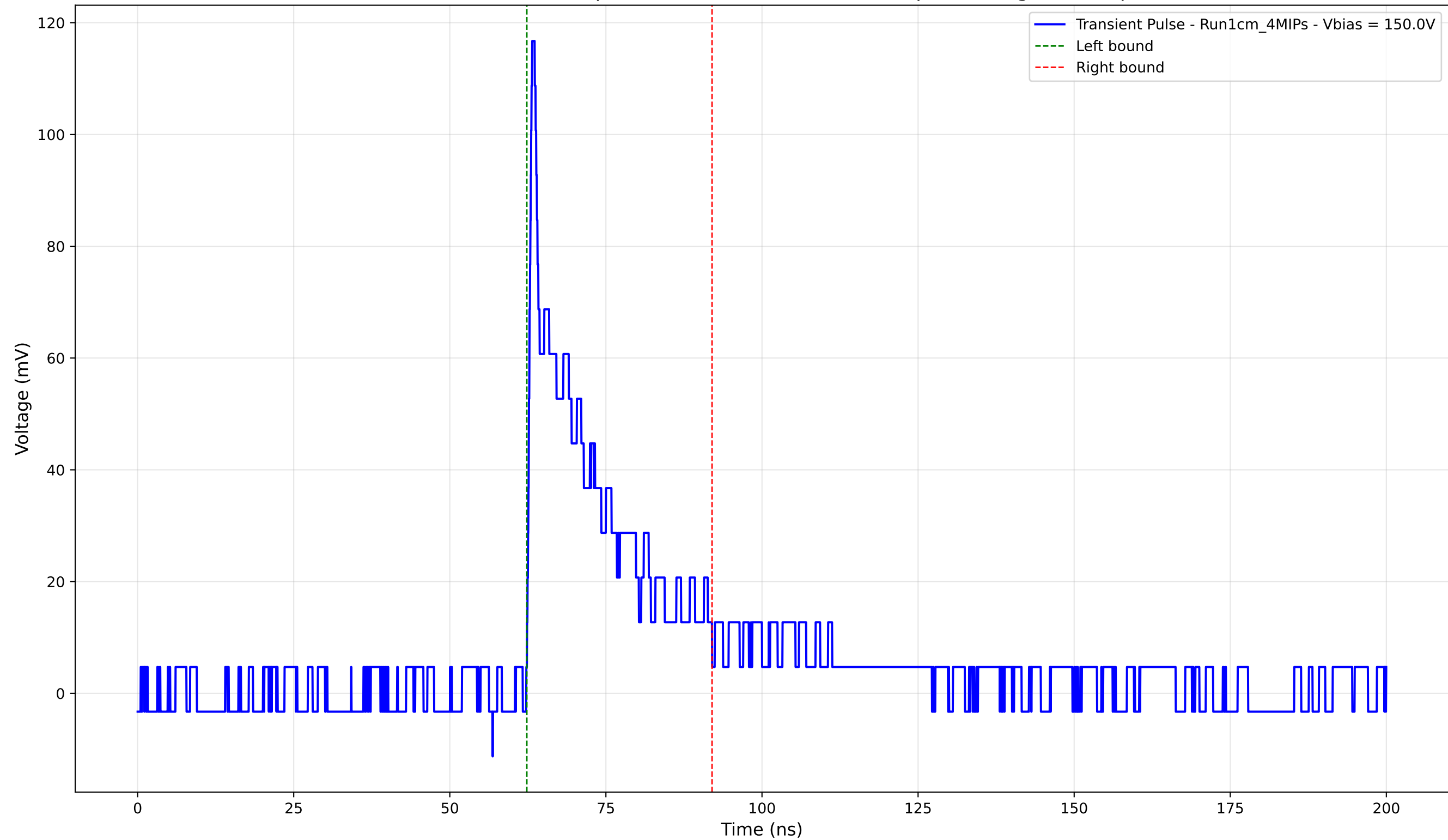
Transient Pulse - Sample: new1cm - Position: 3015.0 \mu\text{m} - Charge: 20.89 pC
