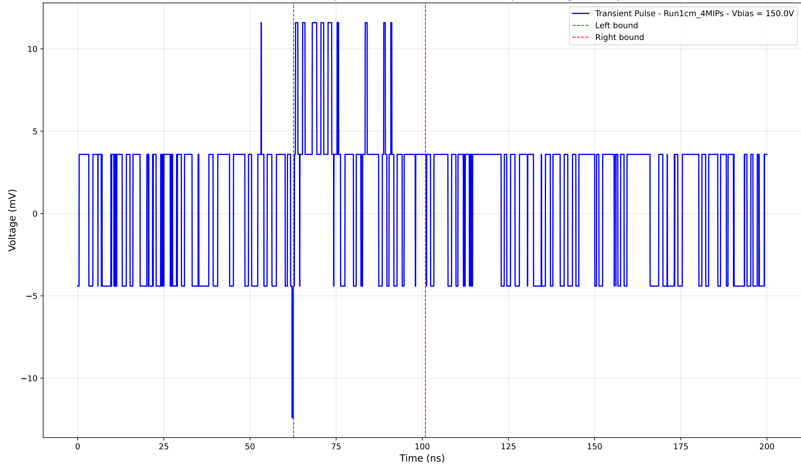
Transient Pulse - Sample: new1cm - Position: 2200.0 \mu\text{m} - Charge: 2.77 pC
