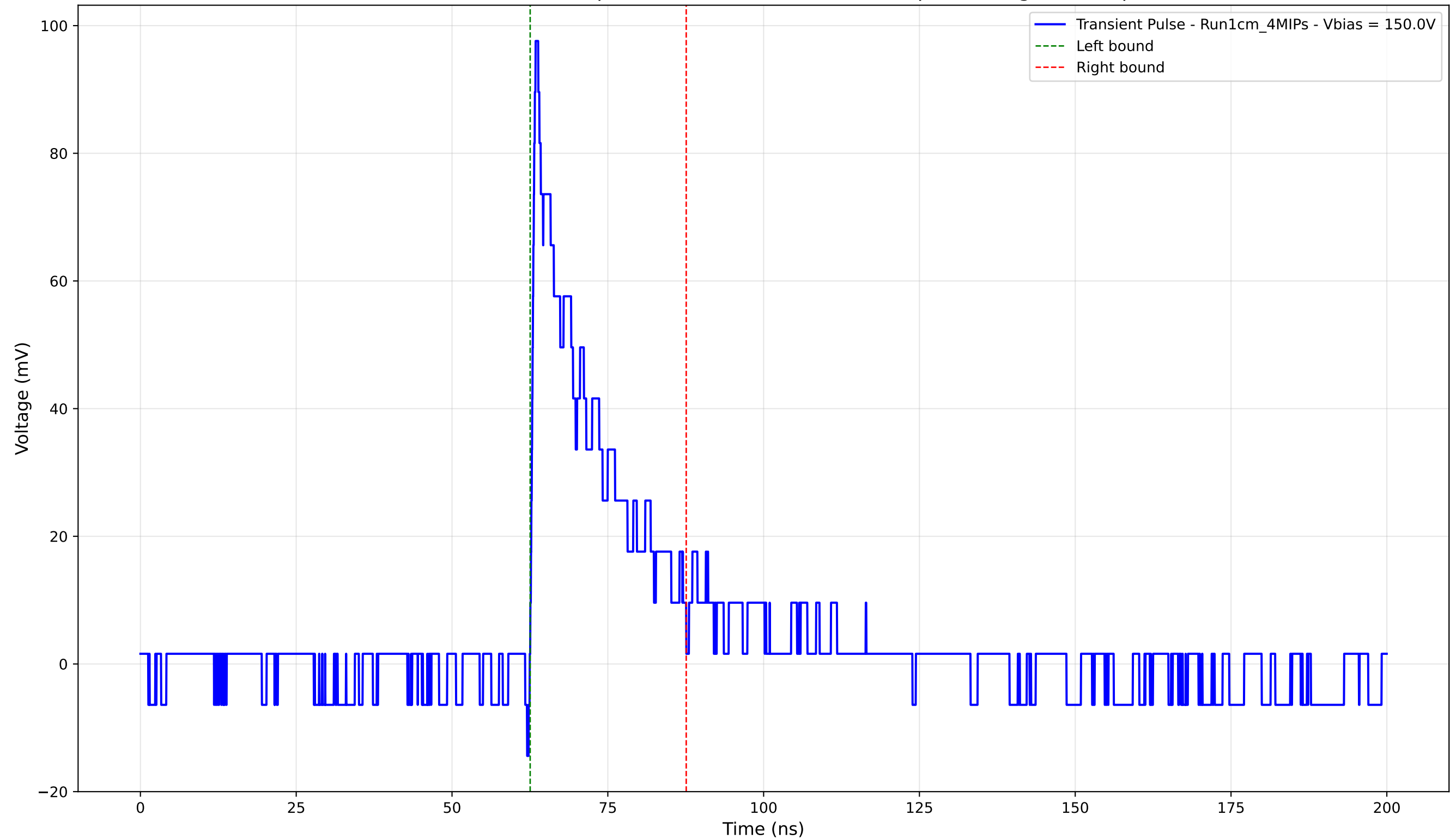
Transient Pulse - Sample: new1cm - Position: 3635.0 \mu\text{m} - Charge: 18.03 pC
