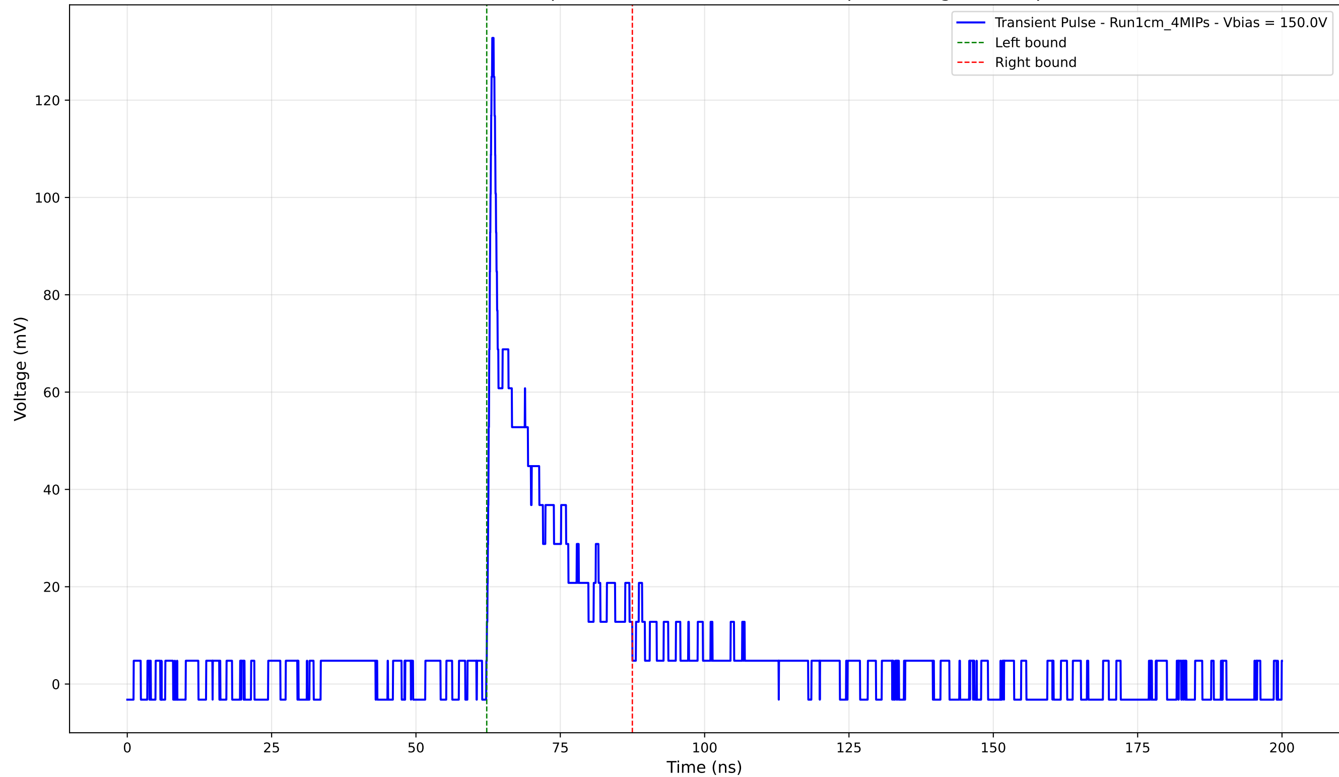
Transient Pulse - Sample: new1cm - Position: 3310.0 \mu\text{m} - Charge: 18.68 pC
