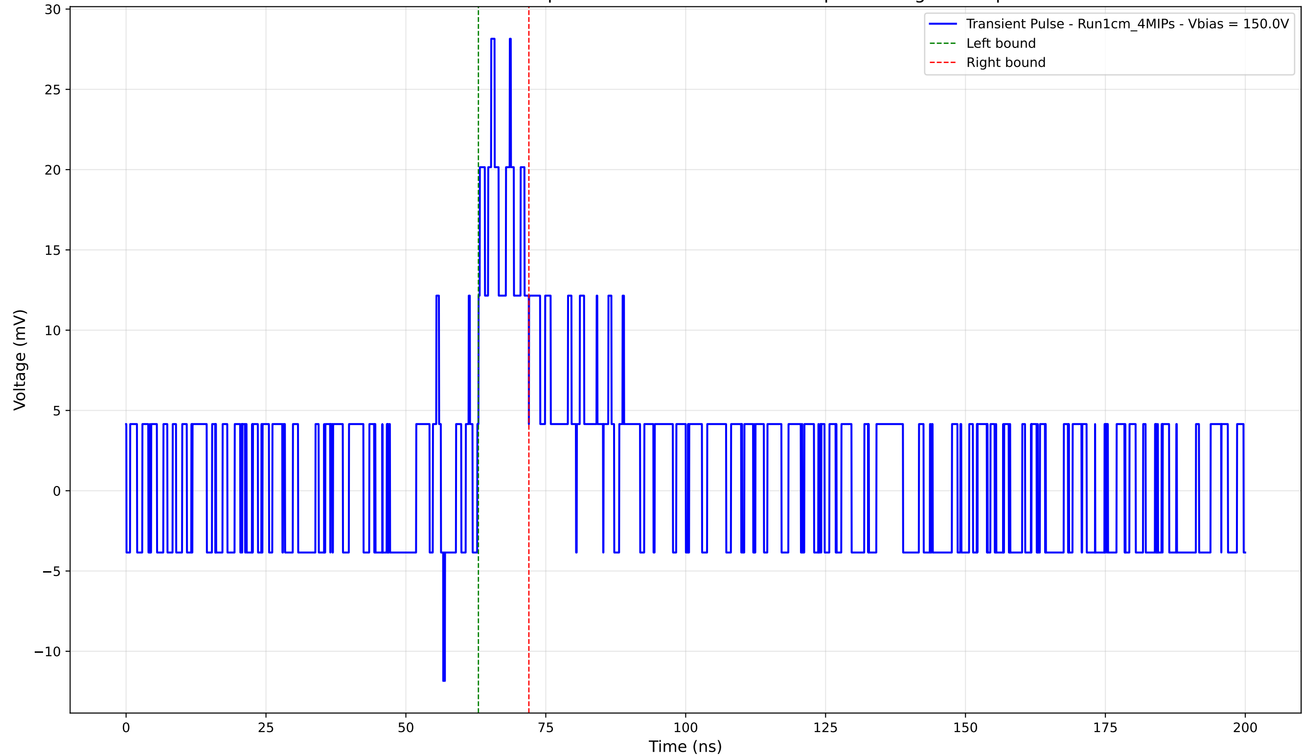
Transient Pulse - Sample: new1cm - Position: 720.0 \mu\text{m} - Charge: 3.11 pC
