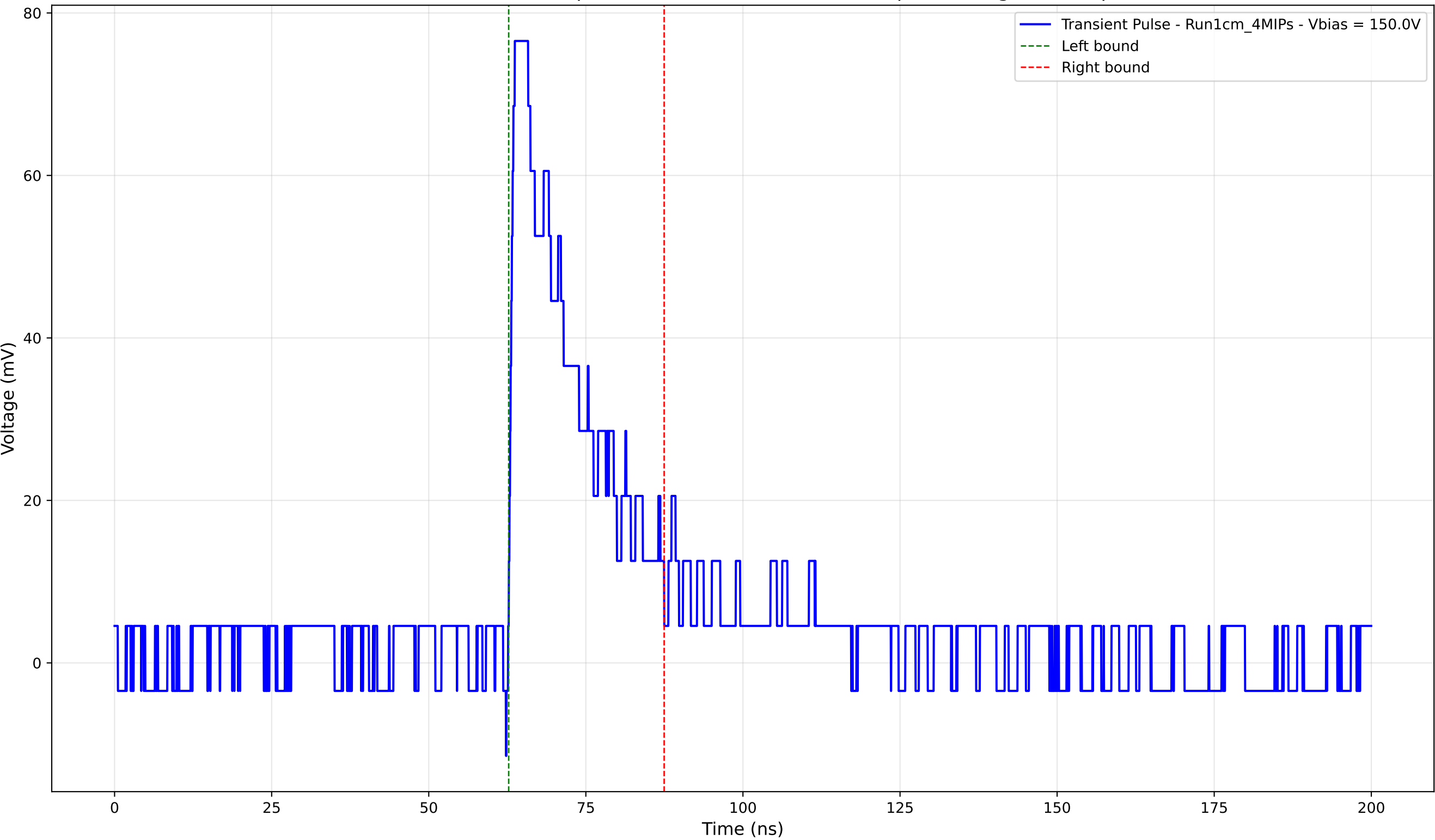
Transient Pulse - Sample: new1cm - Position: 4295.0 \mu\text{m} - Charge: 17.57 pC
