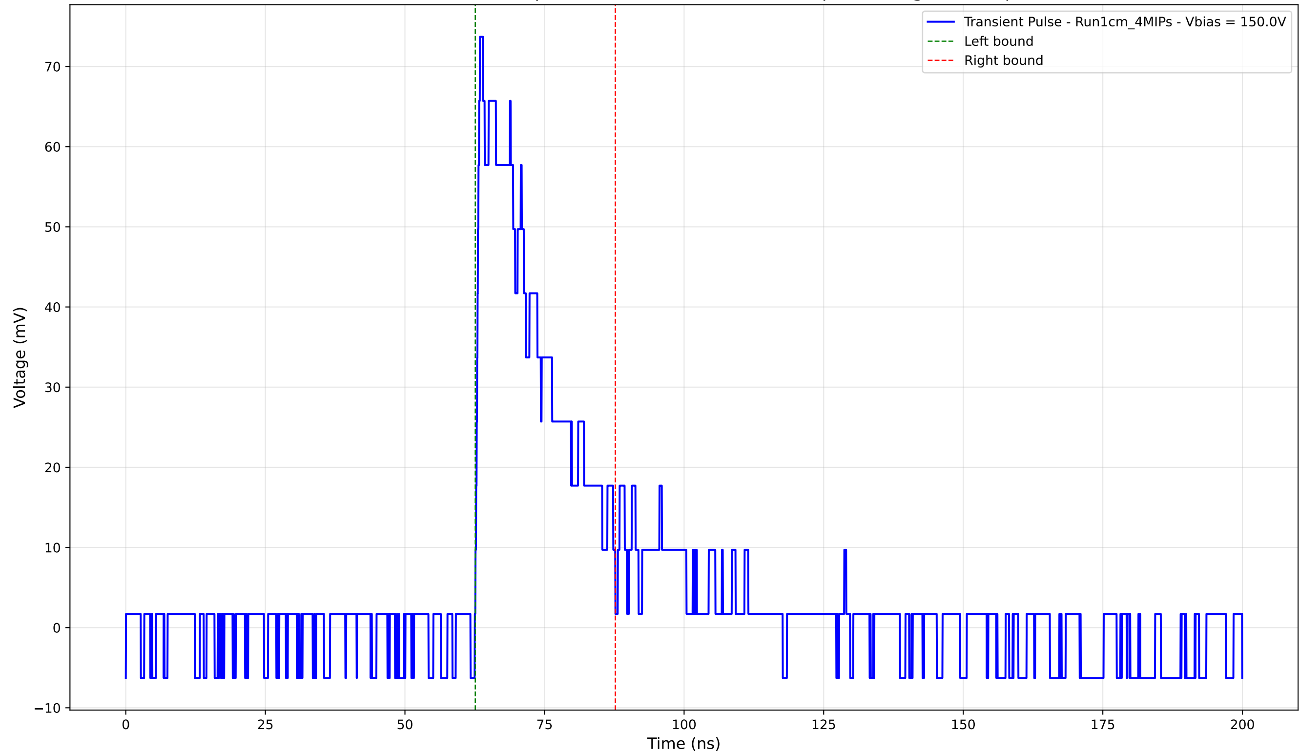
Transient Pulse - Sample: new1cm - Position: 2575.0 \mu\text{m} - Charge: 18.03 pC
