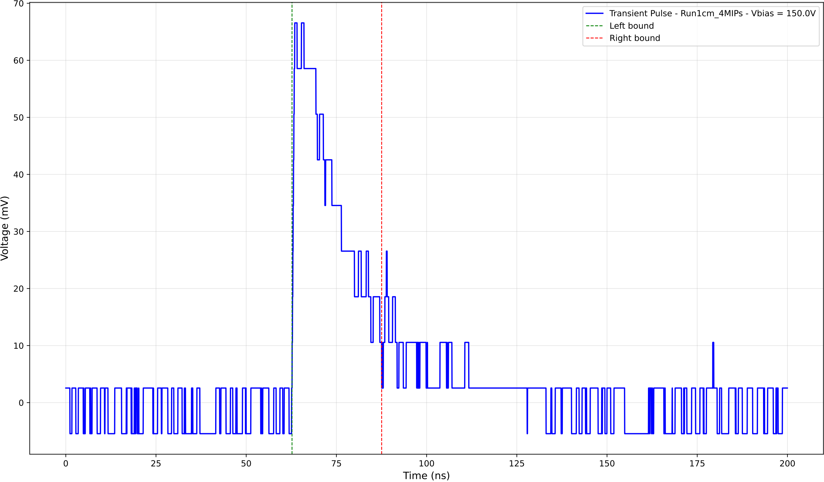
Transient Pulse - Sample: new1cm - Position: 2470.0 \mu\text{m} - Charge: 18.17 pC
