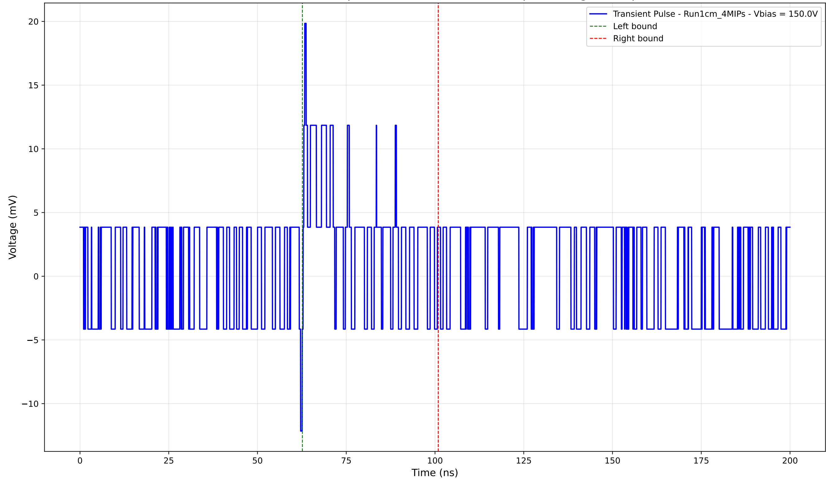
Transient Pulse - Sample: new1cm - Position: 705.0 \mu\text{m} - Charge: 2.47 pC
