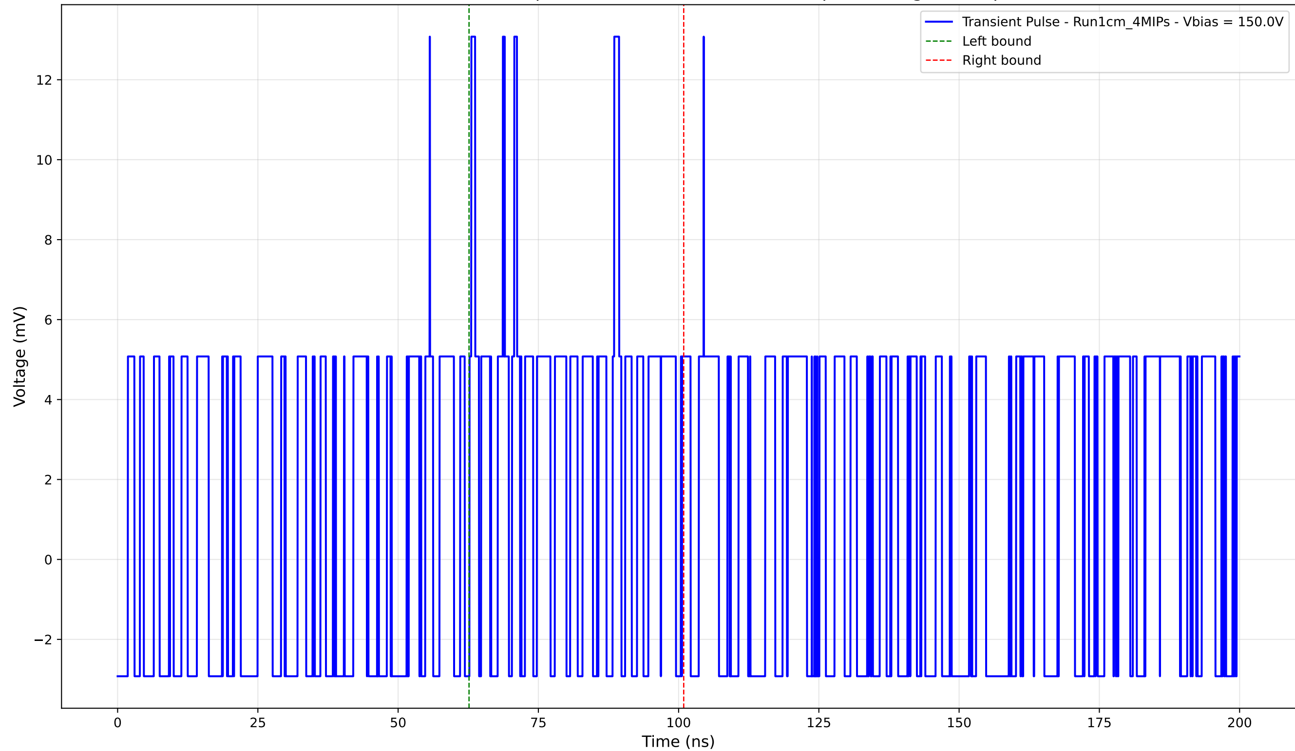
Transient Pulse - Sample: new1cm - Position: 5060.0 \mu\text{m} - Charge: 2.40 pC
