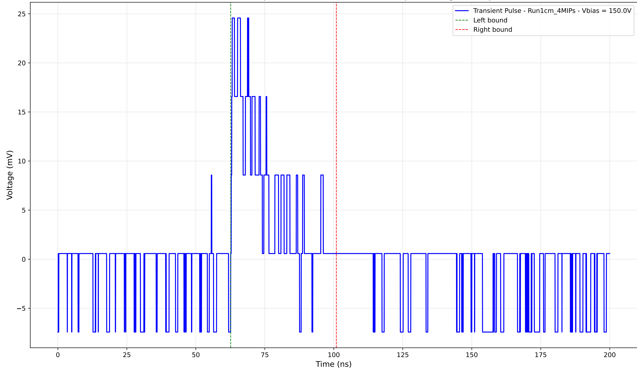
Transient Pulse - Sample: new1cm - Position: 2670.0 \mu\text{m} - Charge: 4.91 pC
