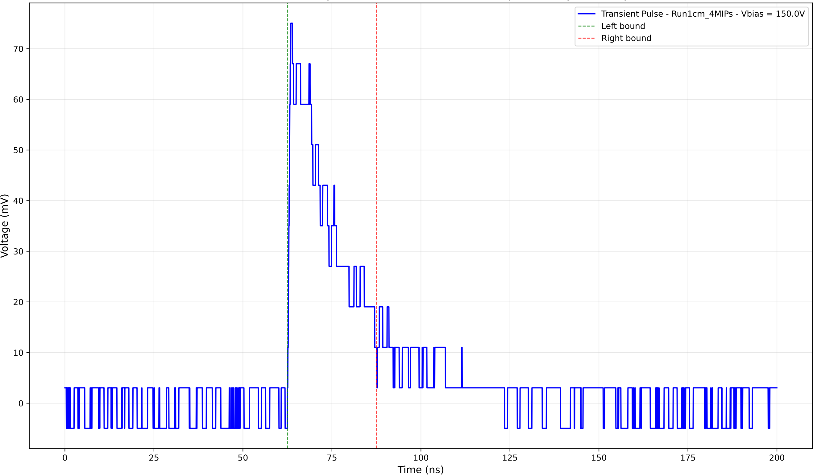
Transient Pulse - Sample: new1cm - Position: 2580.0 \mu\text{m} - Charge: 18.73 pC
