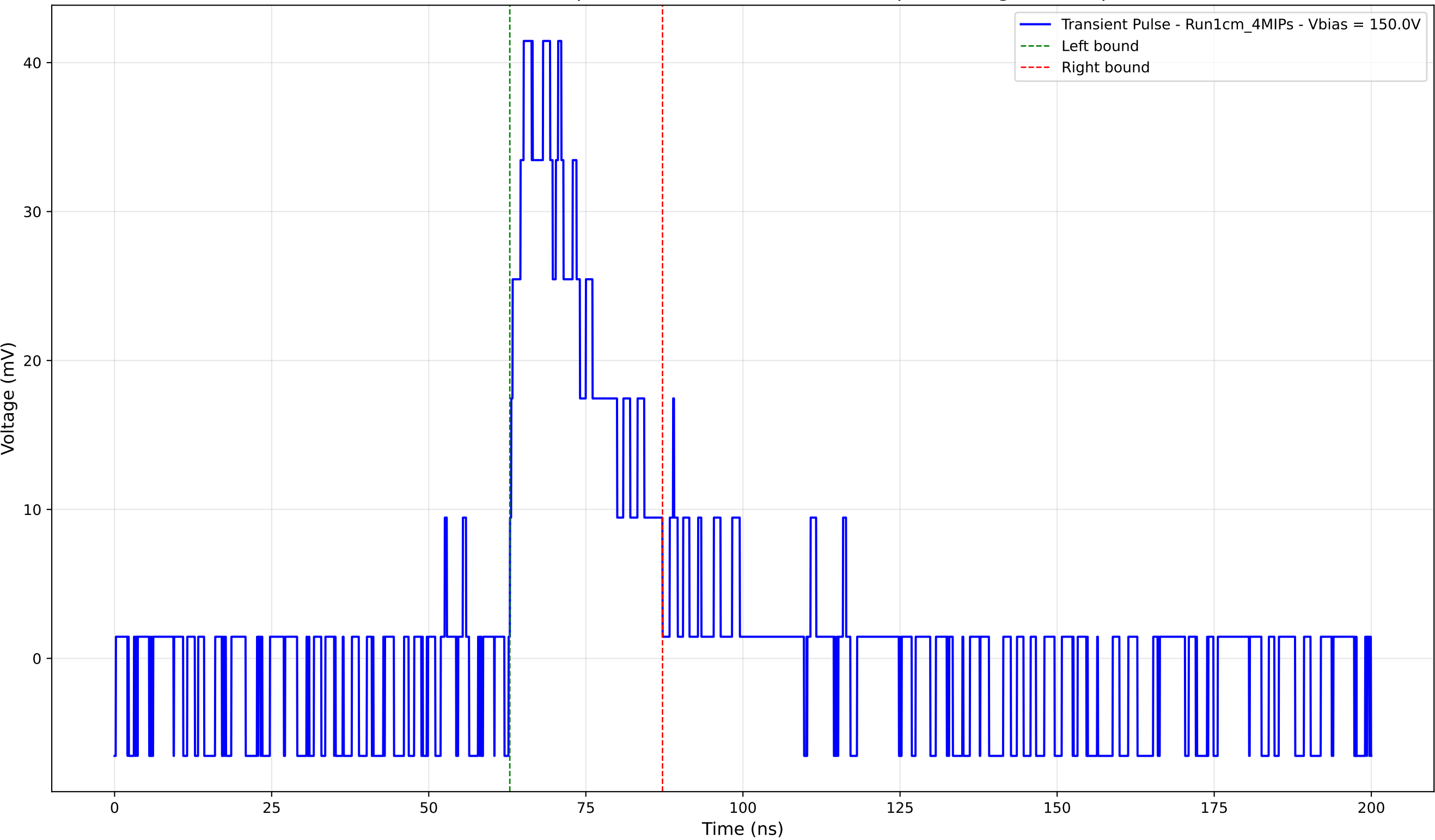
Transient Pulse - Sample: new1cm - Position: 1765.0 \mu\text{m} - Charge: 11.11 pC
