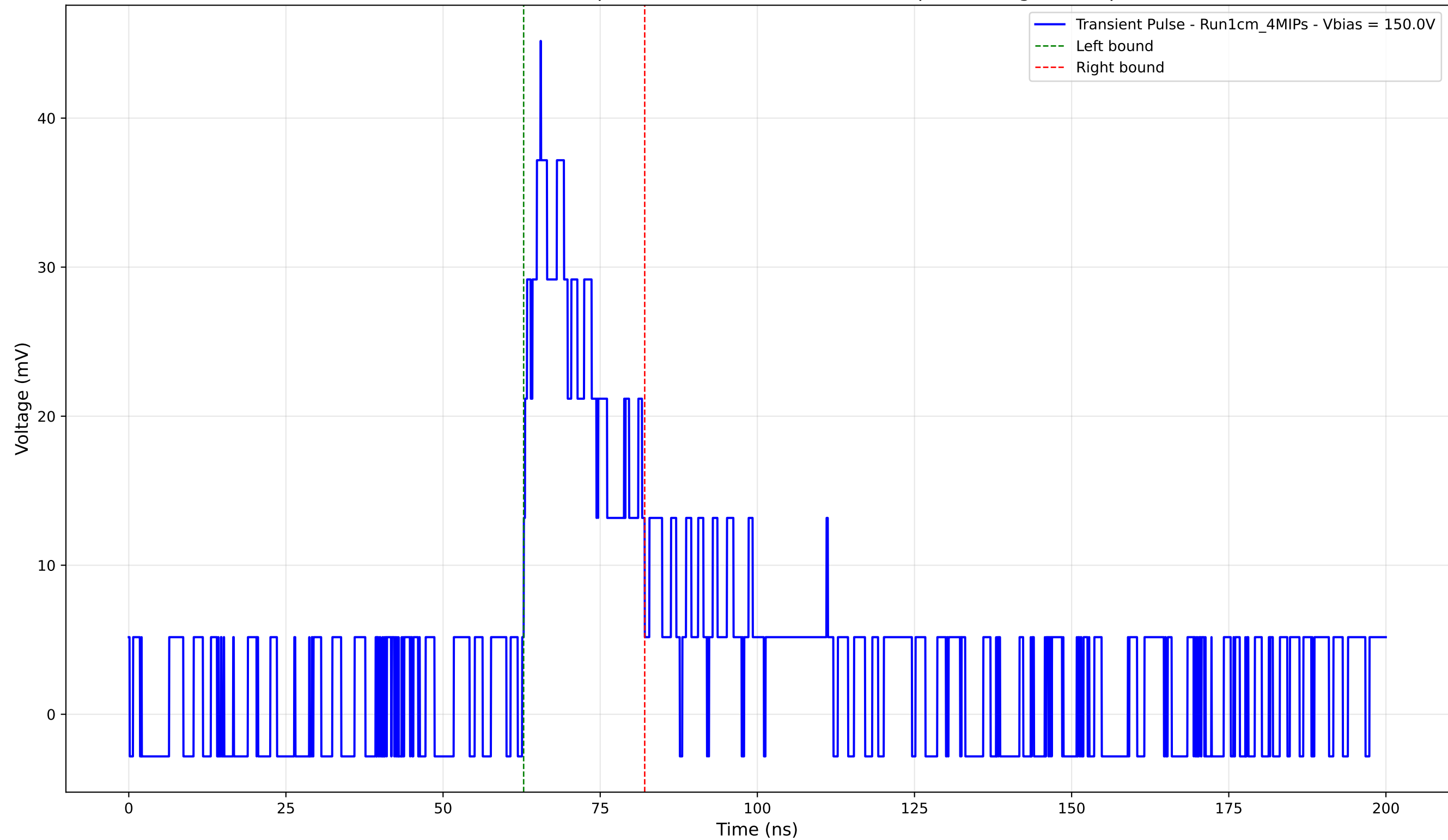
Transient Pulse - Sample: new1cm -Position: 1140.0 \mu\text{m} - Charge: 9.15 pC
