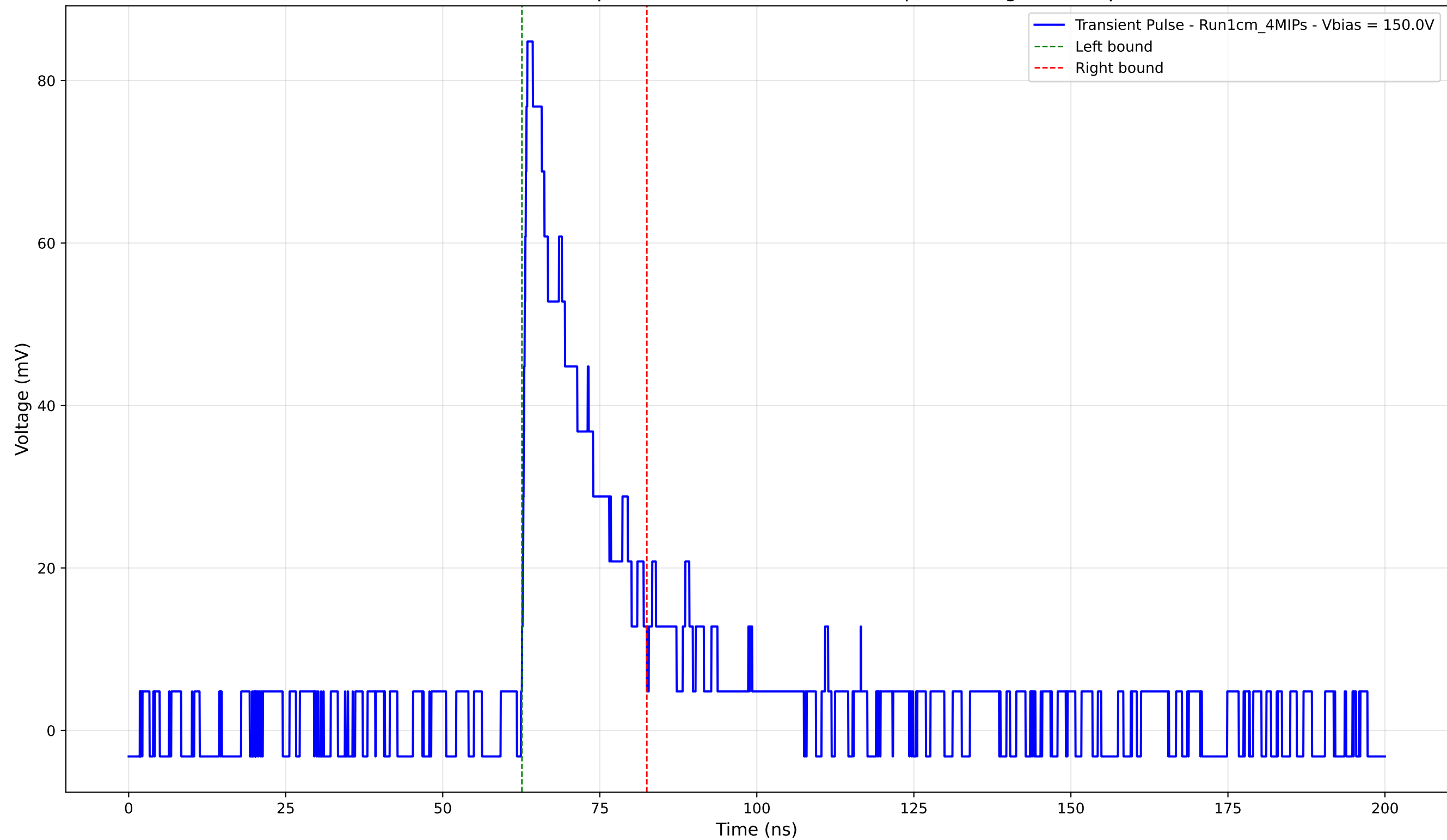
Transient Pulse - Sample: new1cm -Position: 505.0 \mu\text{m} - Charge: 16.20 pC
