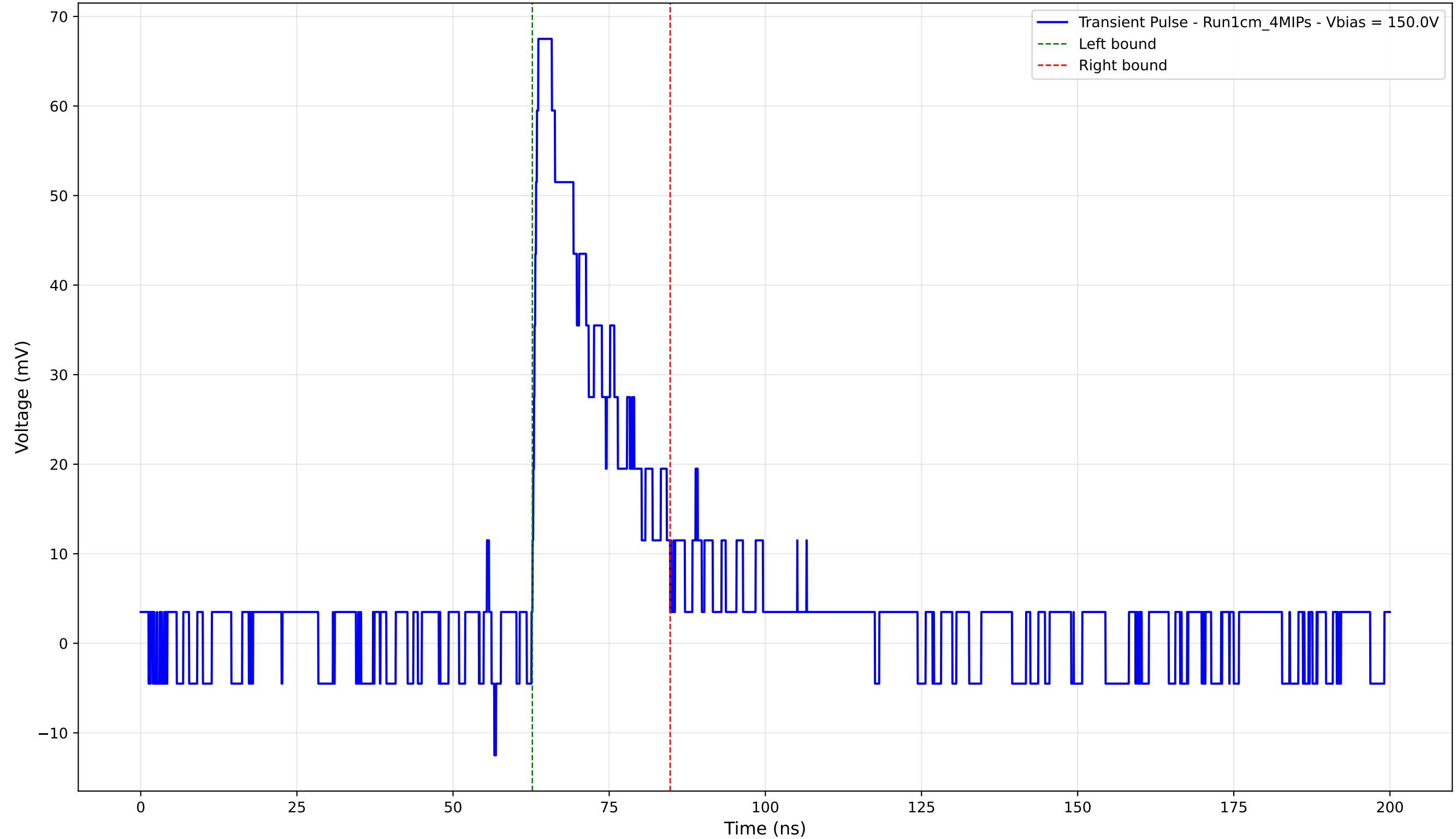
Transient Pulse - Sample: new1cm - Position: 4290.0 \mu\text{m} - Charge: 15.12 pC
