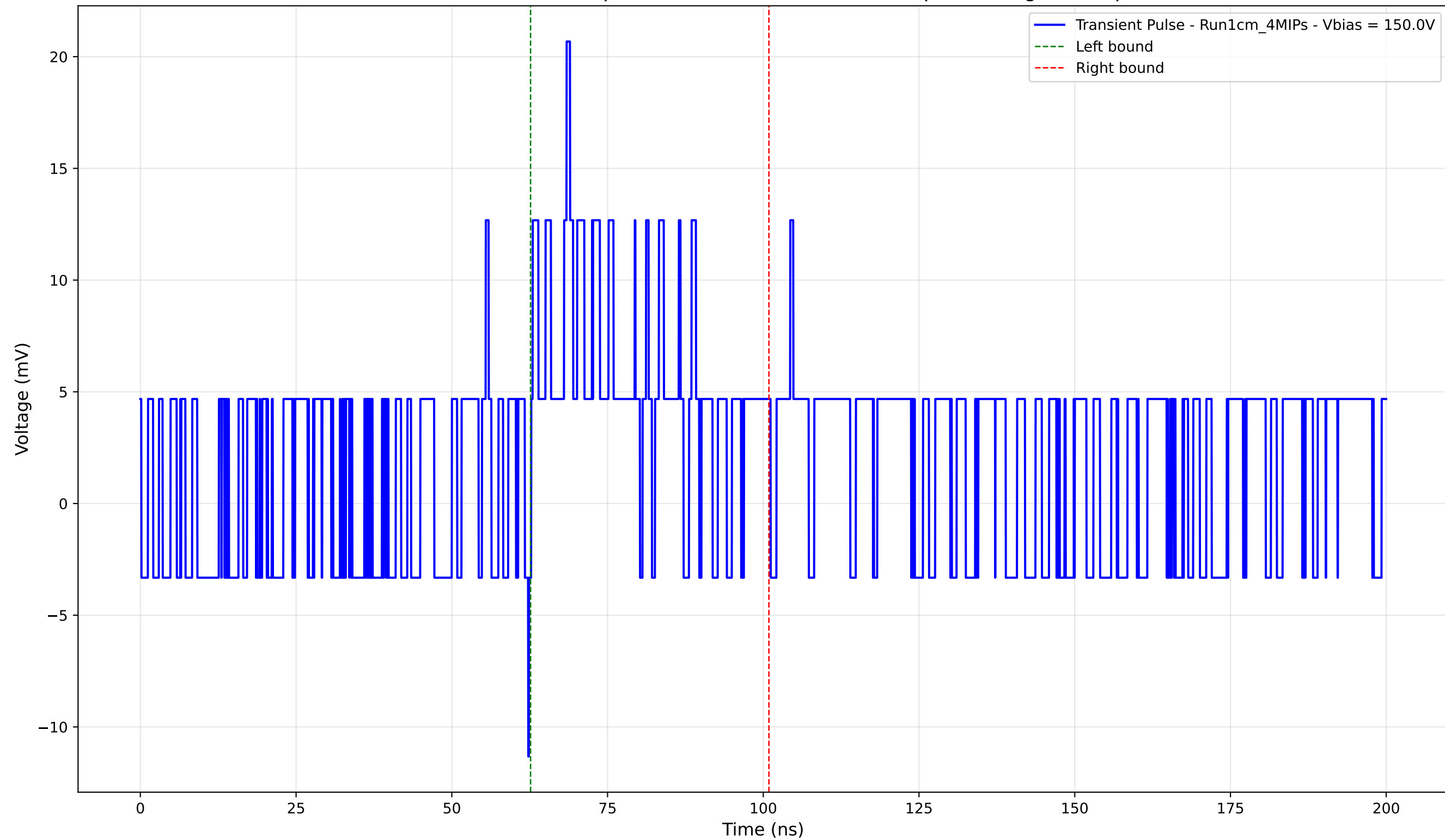
Transient Pulse - Sample: new1cm - Position: 2215.0 \mu\text{m} - Charge: 4.40 pC
