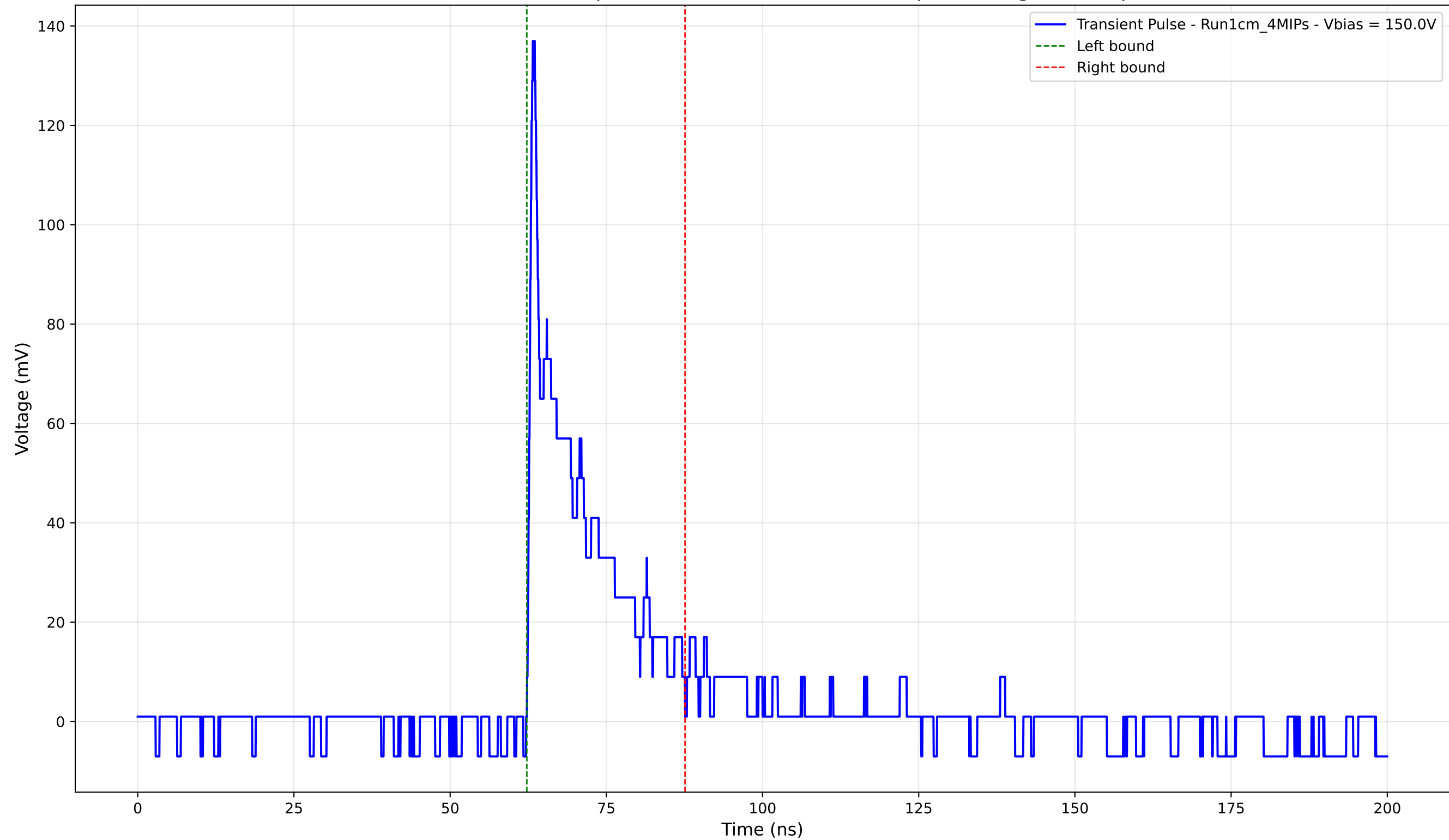
Transient Pulse - Sample: new1cm - Position: 3385.0 \mu\text{m} - Charge: 19.79 pC
