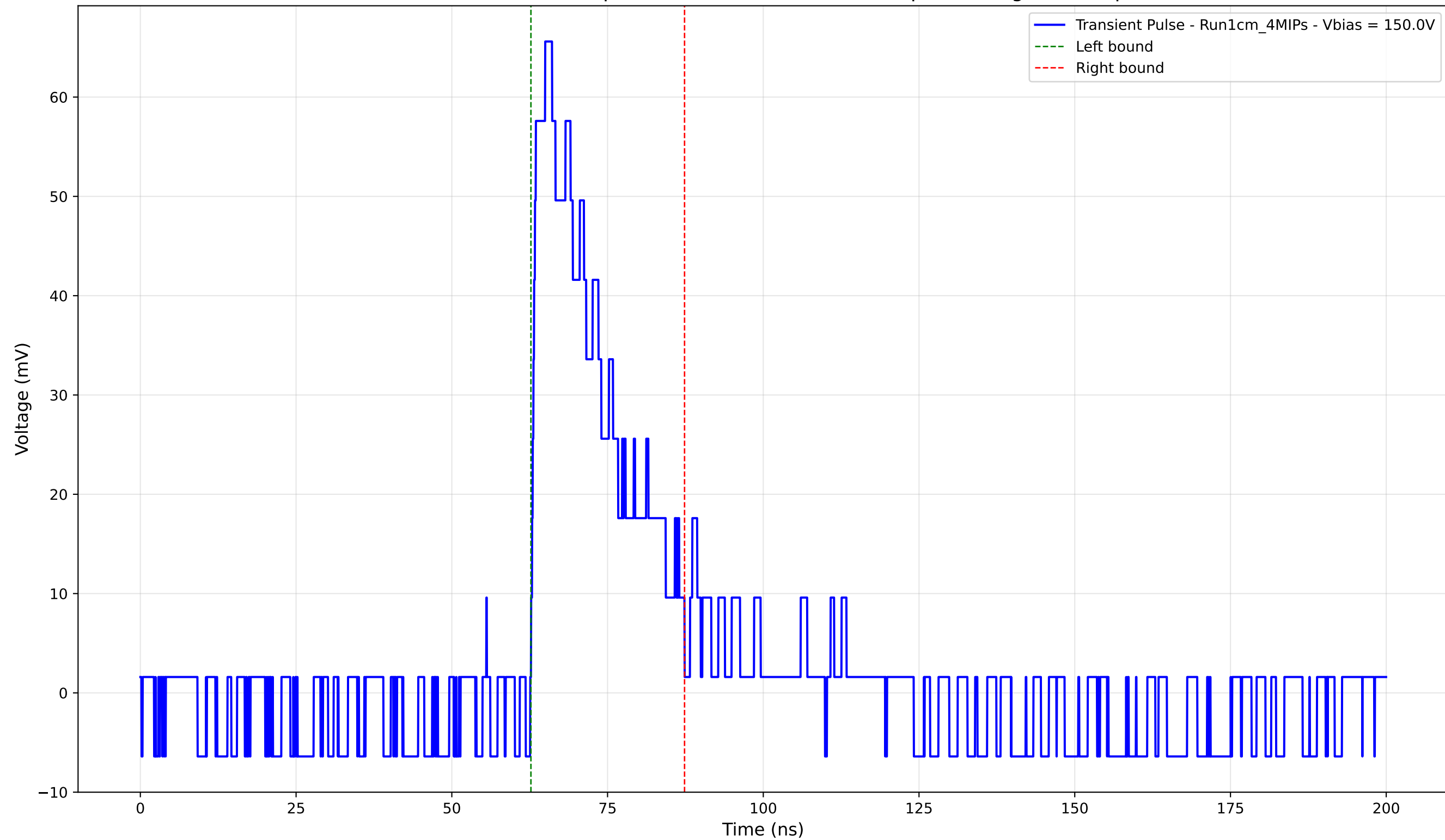
Transient Pulse - Sample: new1cm - Position: 790.0 \mu\text{m} - Charge: 15.83 pC
