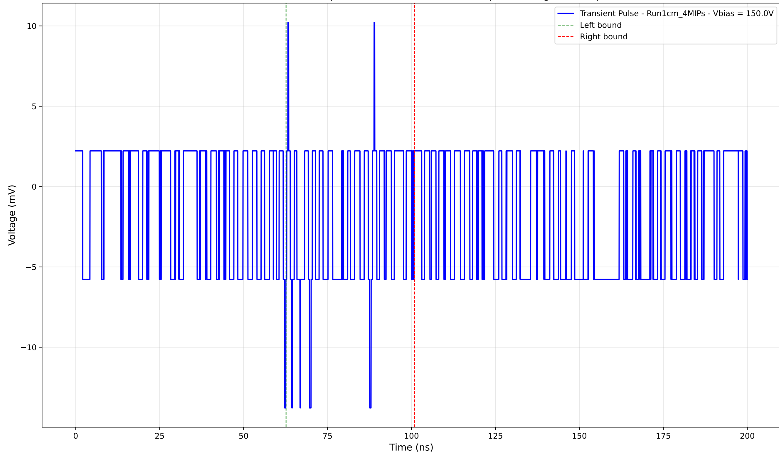
Transient Pulse - Sample: new1cm - Position: 60.0 \mu\text{m} - Charge: -1.39 pC
