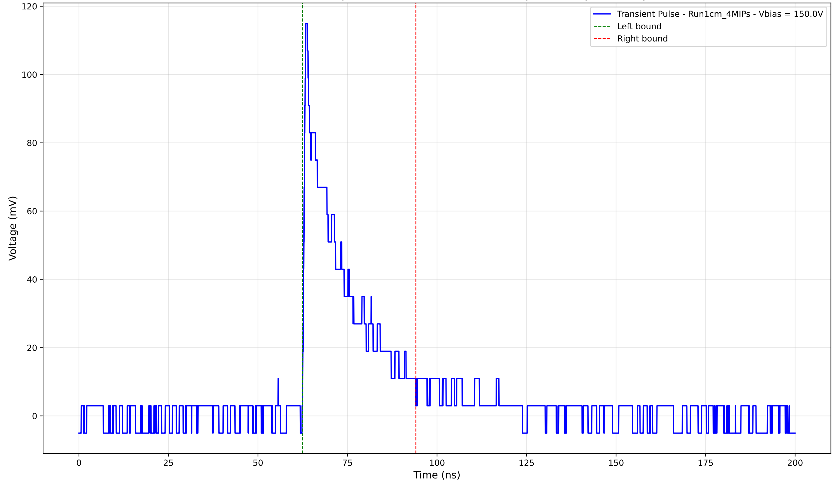
Transient Pulse - Sample: new1cm - Position: 3590.0 \mu\text{m} - Charge: 23.74 pC
