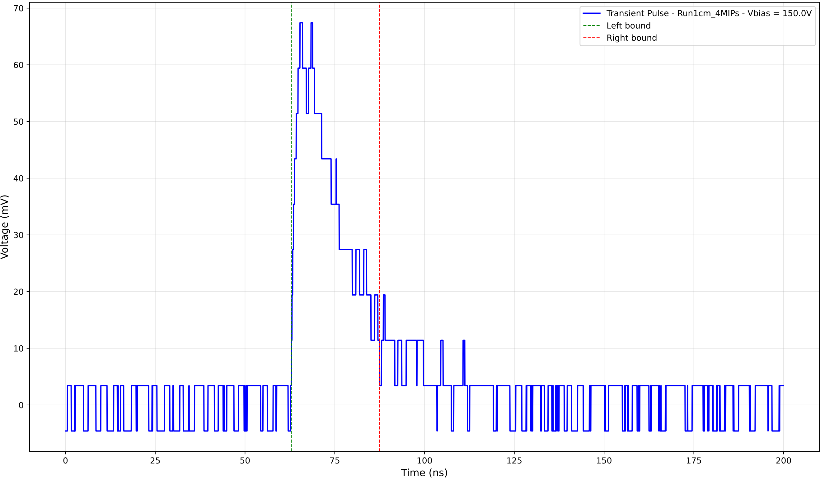
Transient Pulse - Sample: new1cm - Position: 1540.0 \mu\text{m} - Charge: 17.85 pC
