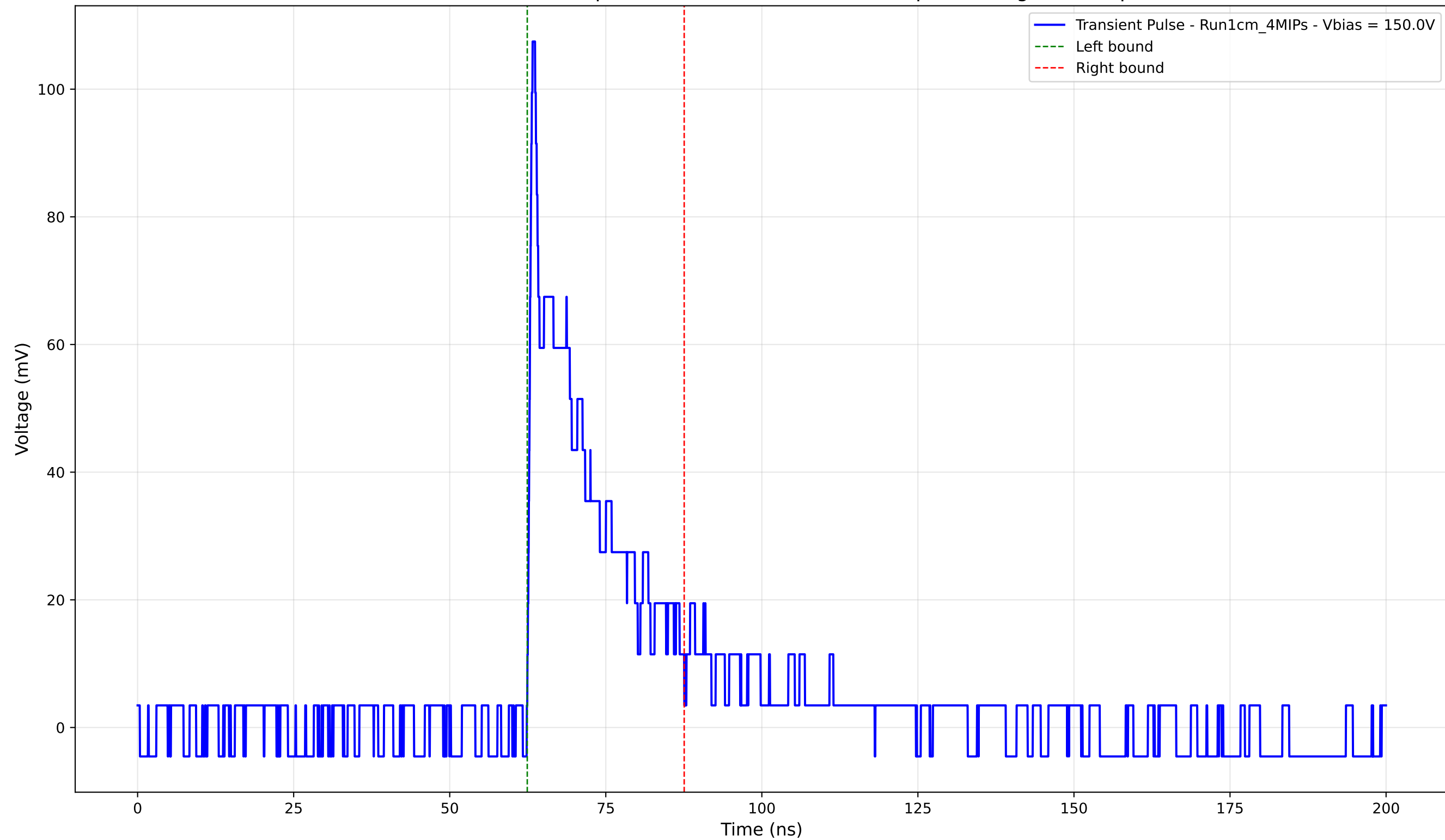
Transient Pulse - Sample: new1cm - Position: 2930.0 \mu\text{m} - Charge: 19.11 pC
