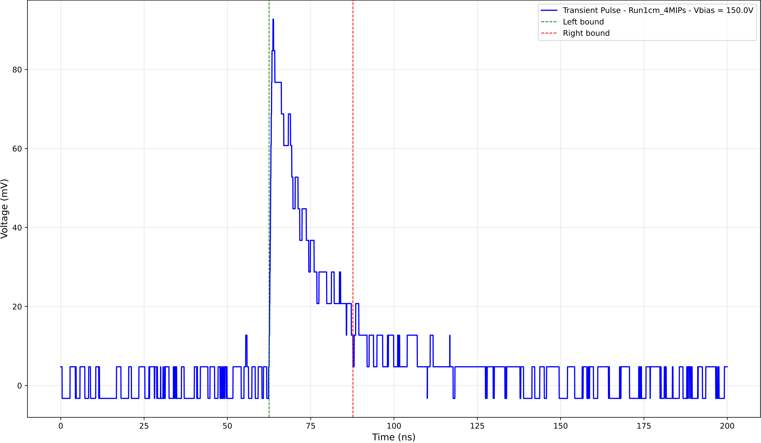
Transient Pulse - Sample: new1cm - Position: 3805.0 \mu\text{m} - Charge: 20.31 pC
