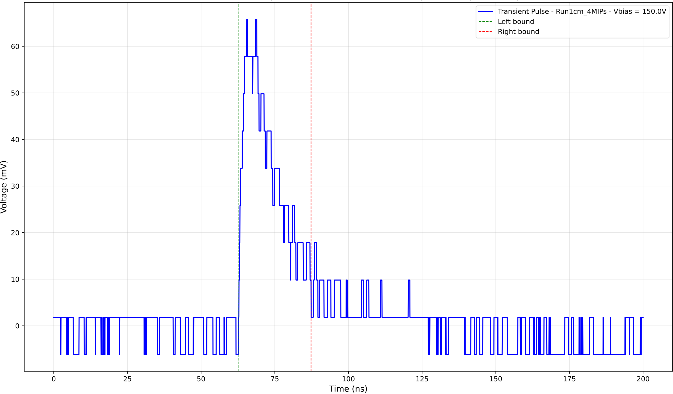
Transient Pulse - Sample: new1cm - Position: 1585.0 \mu\text{m} - Charge: 16.44 pC
