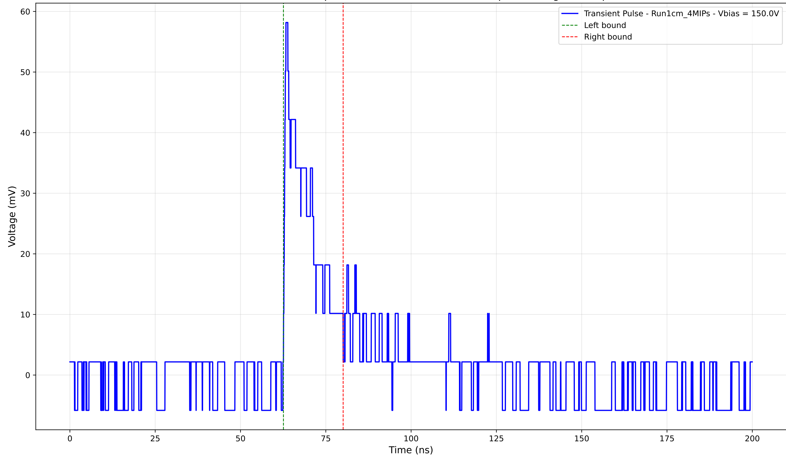
Transient Pulse - Sample: new1cm -Position: 3665.0 \mu\text{m} - Charge: 8.82 pC
