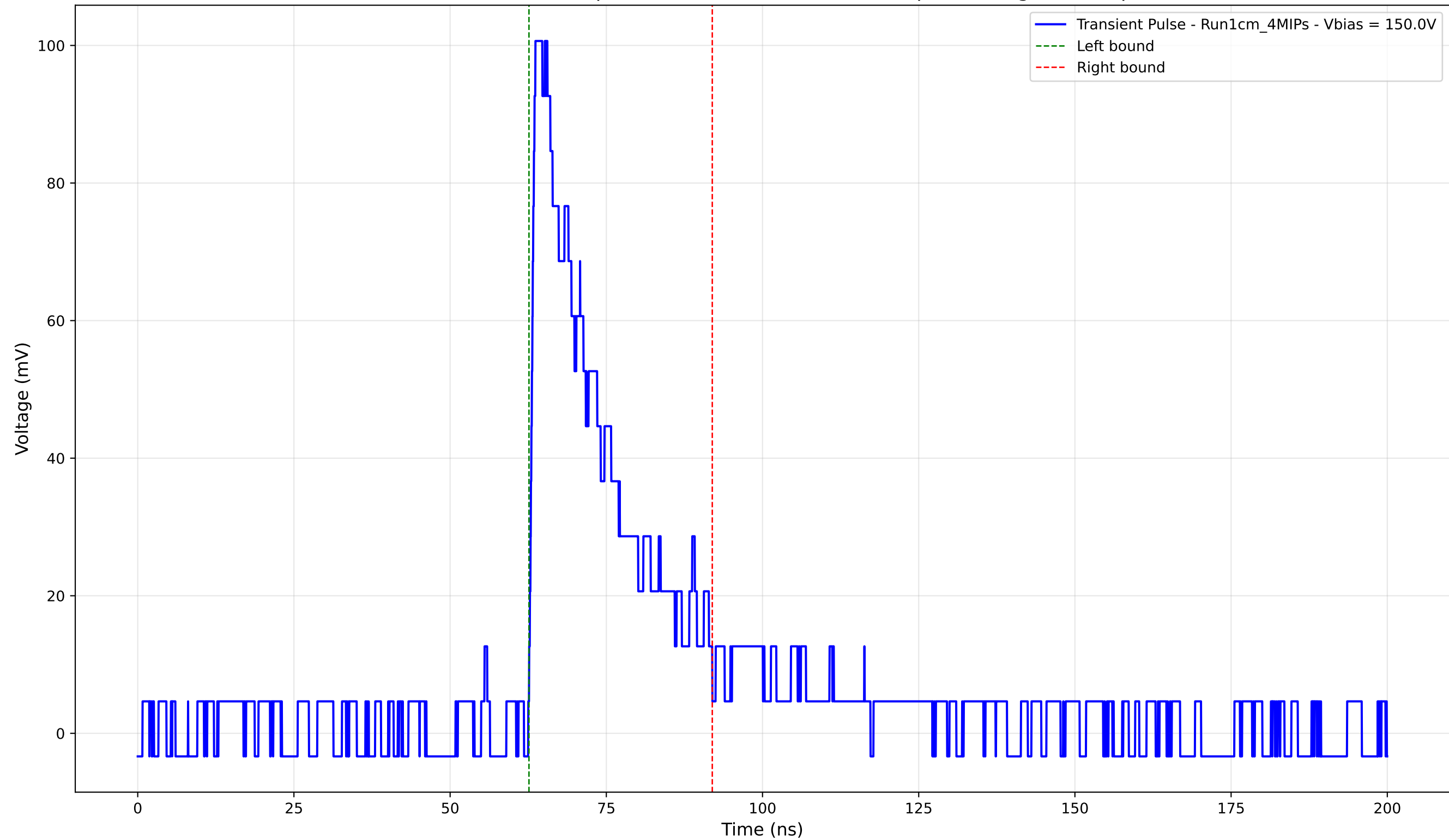
Transient Pulse - Sample: new1cm - Position: 4055.0 \mu\text{m} - Charge: 24.61 pC
