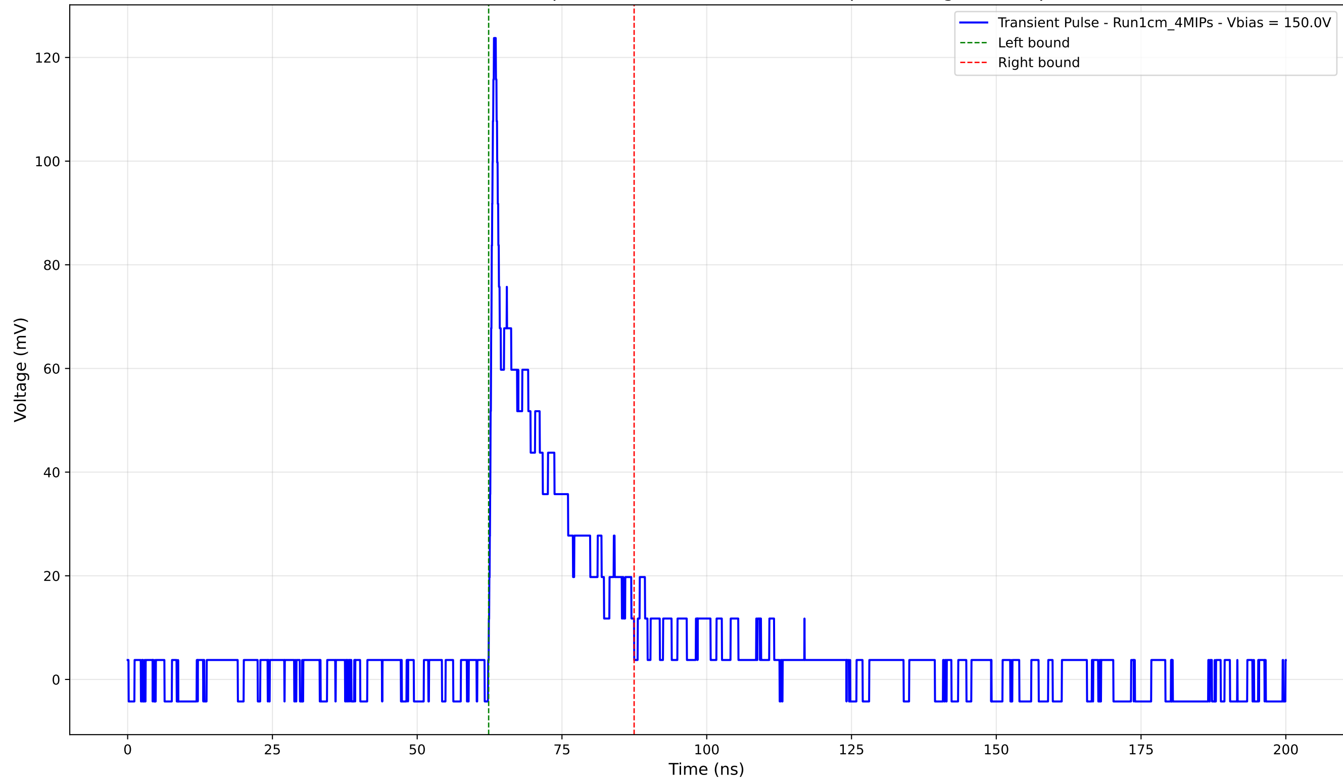
Transient Pulse - Sample: new1cm - Position: 3020.0 \mu\text{m} - Charge: 19.86 pC
