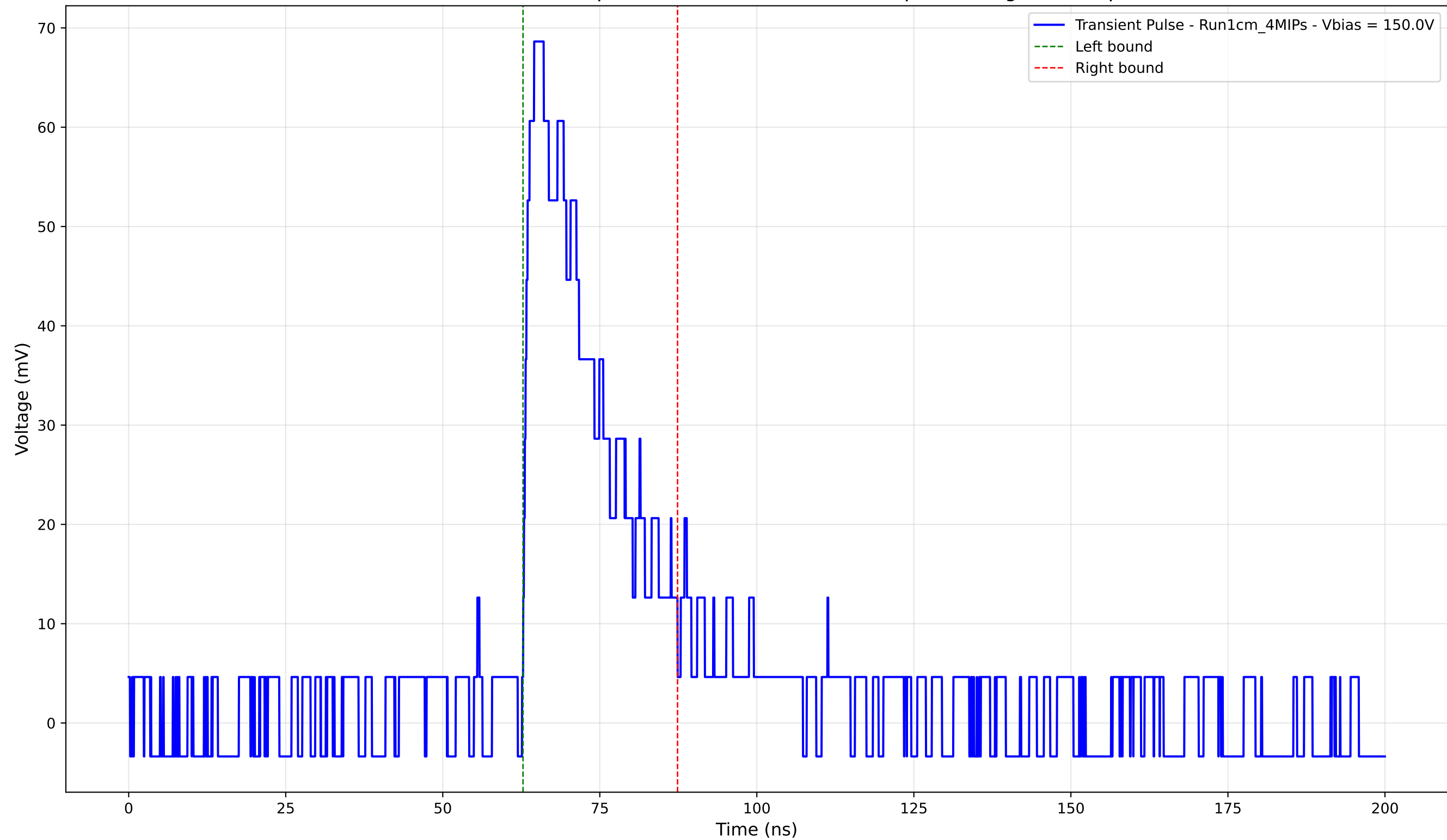
Transient Pulse - Sample: new1cm -Position: 895.0 \mu\text{m} - Charge: 17.09 pC
