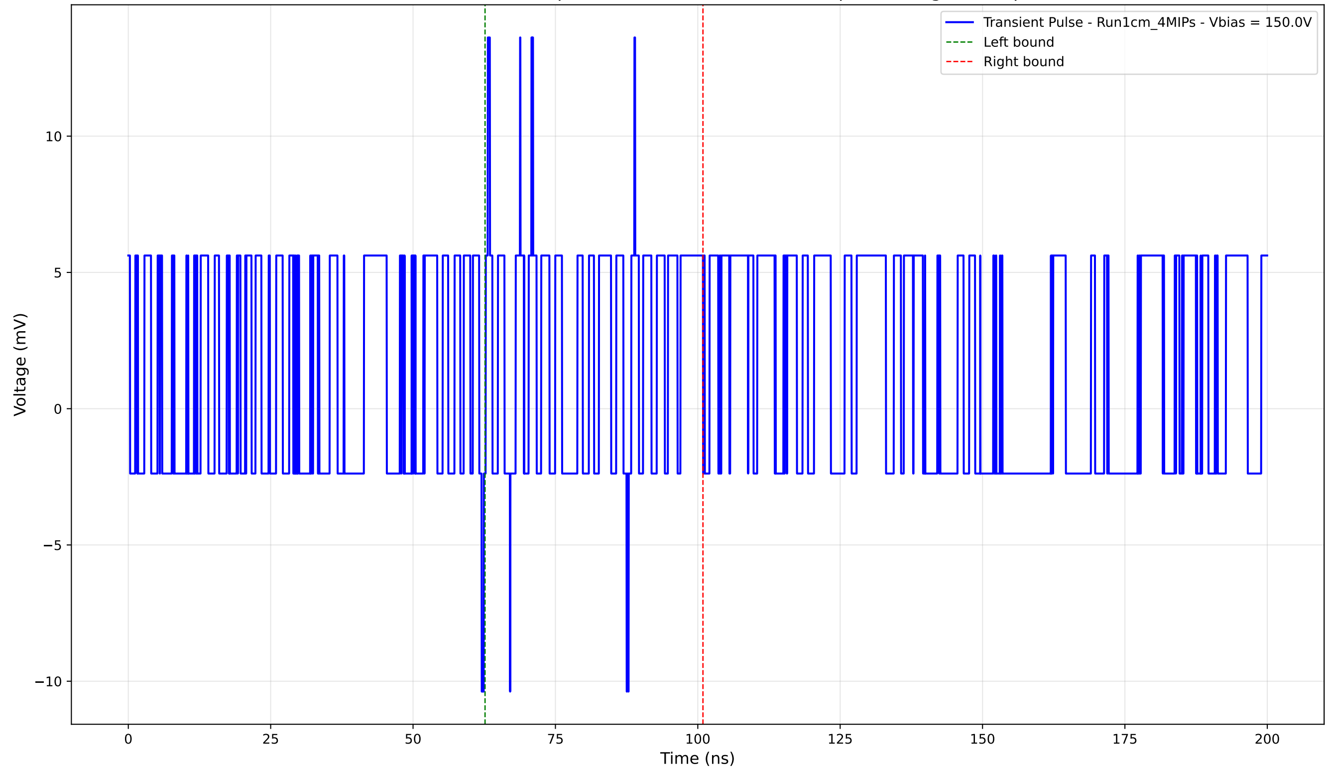
Transient Pulse - Sample: new1cm - Position: 165.0 \mu\text{m} - Charge: 1.95 pC
