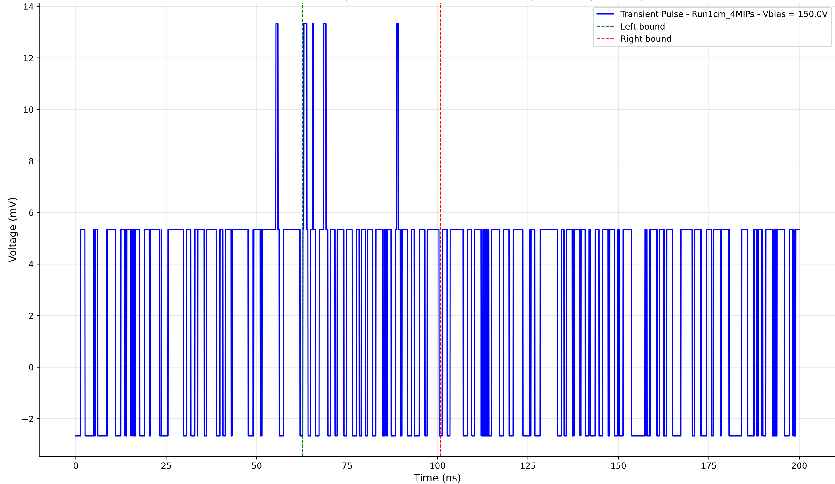
Transient Pulse - Sample: new1cm - Position: 5080.0 \mu\text{m} - Charge: 2.31 pC
