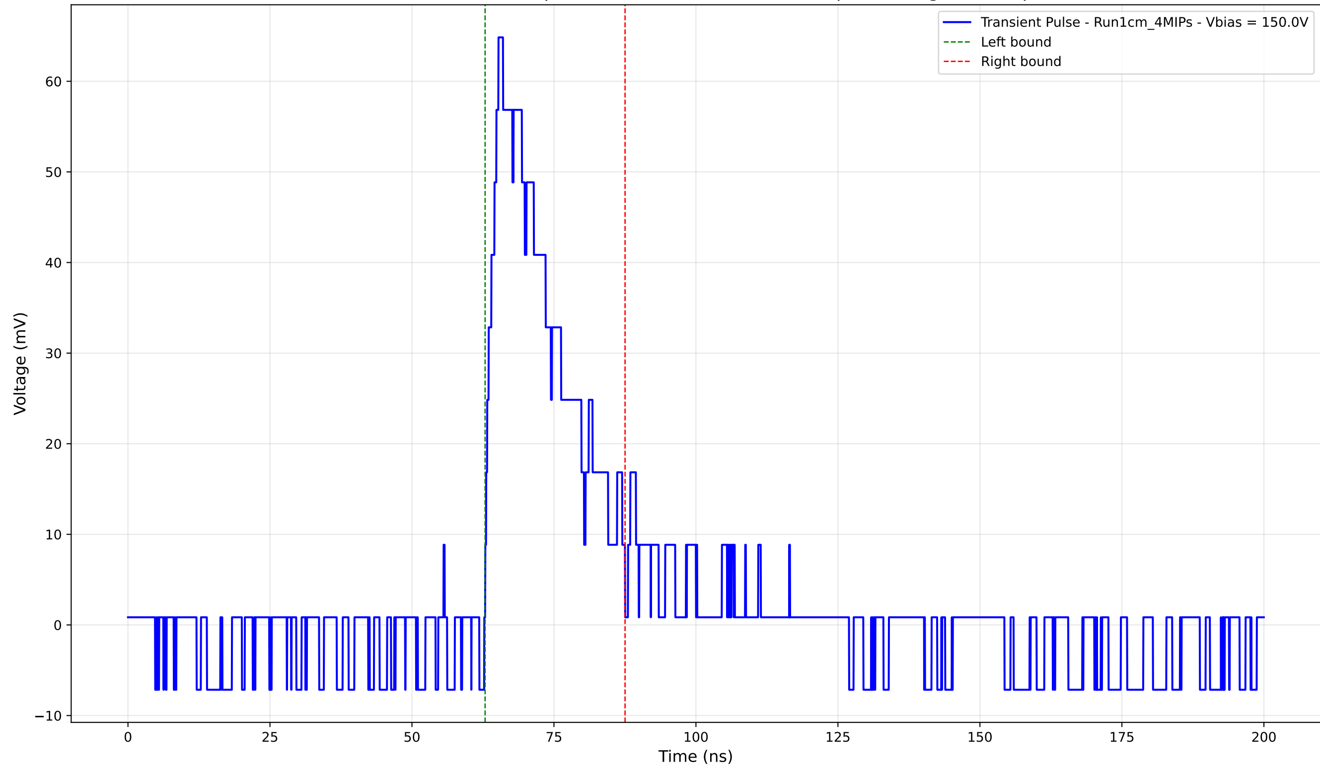
Transient Pulse - Sample: new1cm - Position: 1560.0 \mu\text{m} - Charge: 16.09 pC
