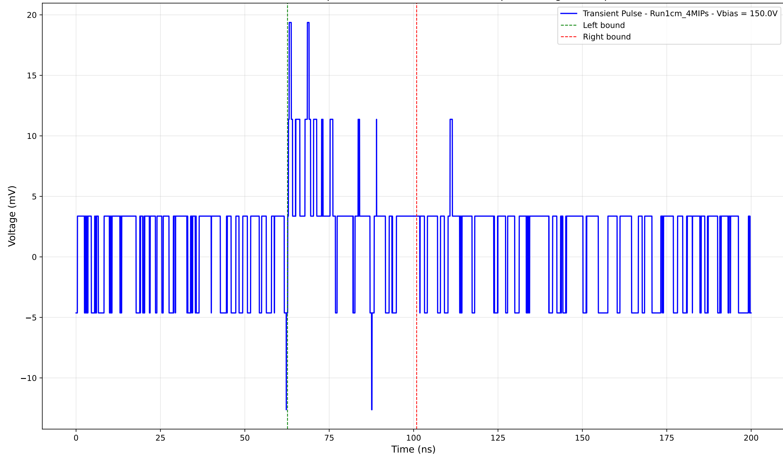
Transient Pulse - Sample: new1cm - Position: 4220.0 \mu\text{m} - Charge: 3.01 pC
