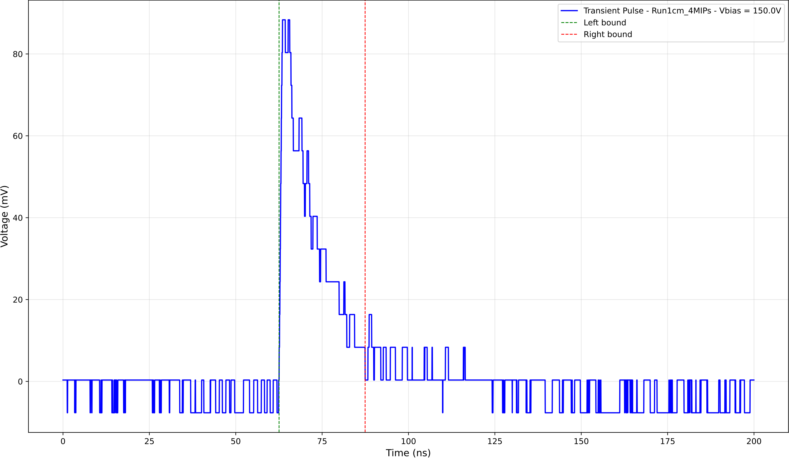
Transient Pulse - Sample: new1cm - Position: 4630.0 \mu\text{m} - Charge: 18.18 pC
