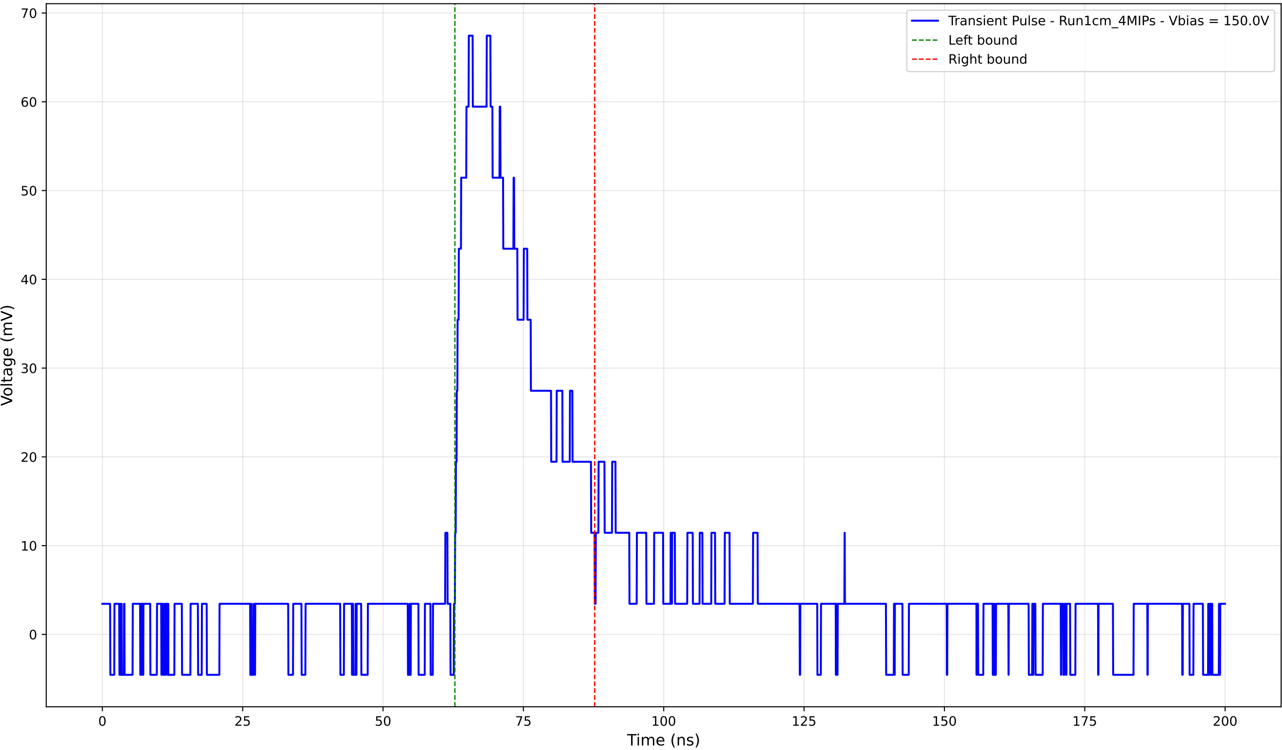
Transient Pulse - Sample: new1cm - Position: 1975.0 \mu\text{m} - Charge: 18.56 pC
