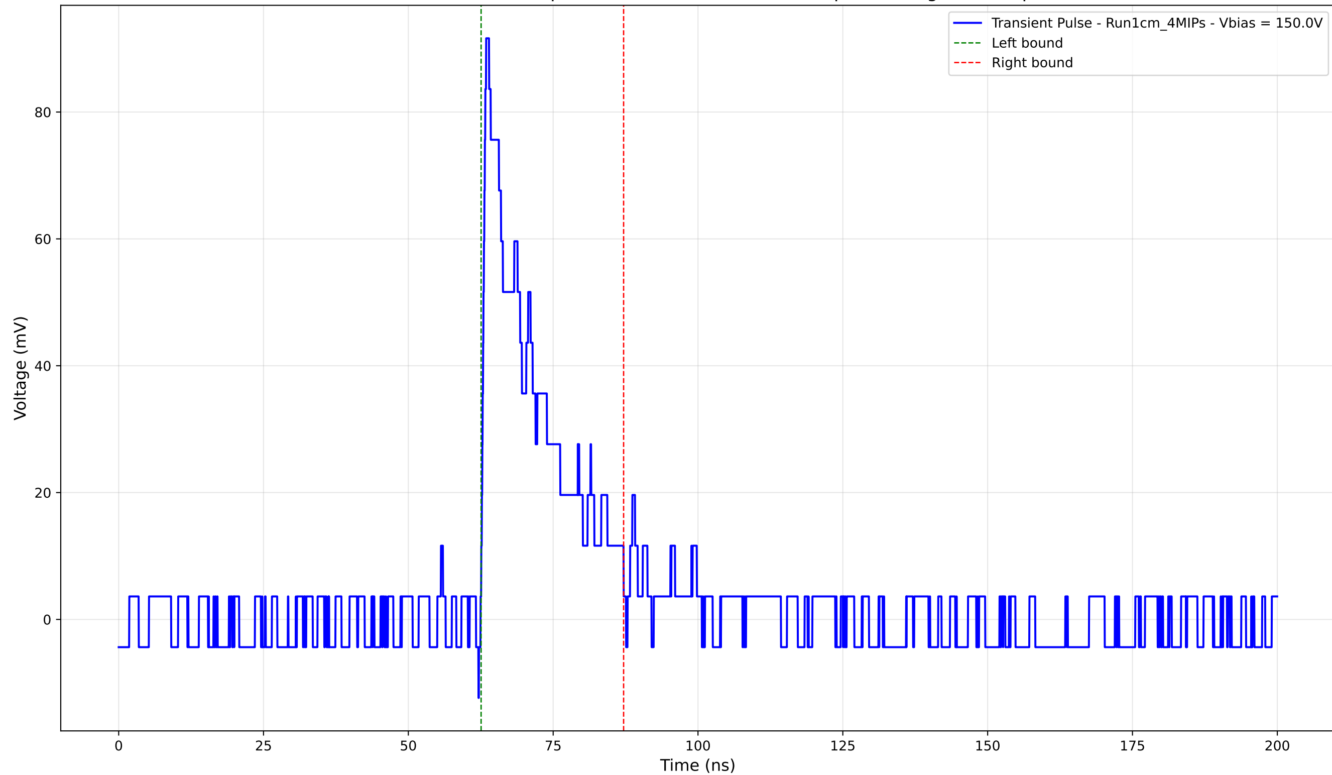
Transient Pulse - Sample: new1cm -Position: 365.0 \mu\text{m} - Charge: 16.81 pC
