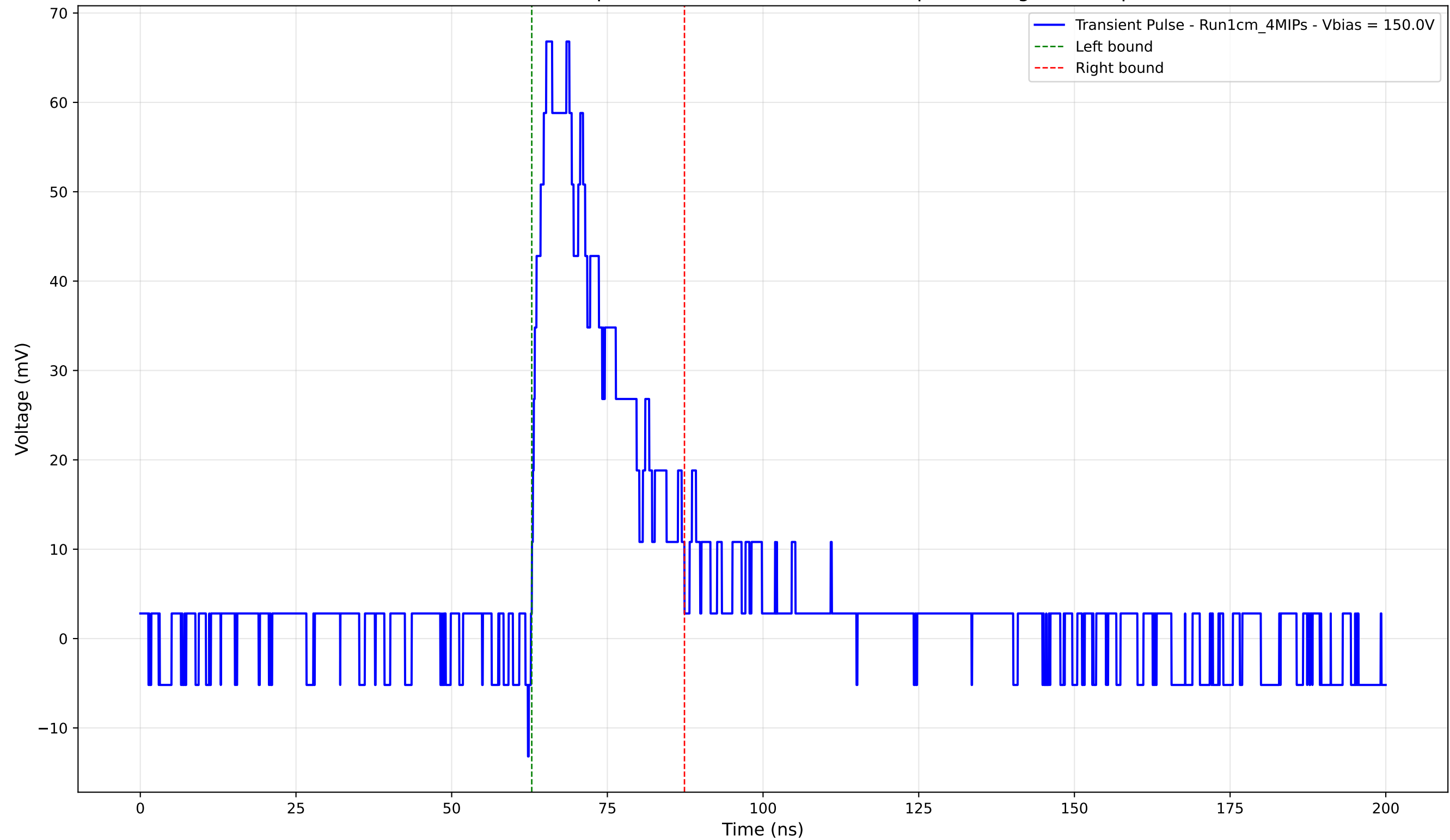
Transient Pulse - Sample: new1cm - Position: 1430.0 \mu\text{m} - Charge: 17.01 pC
