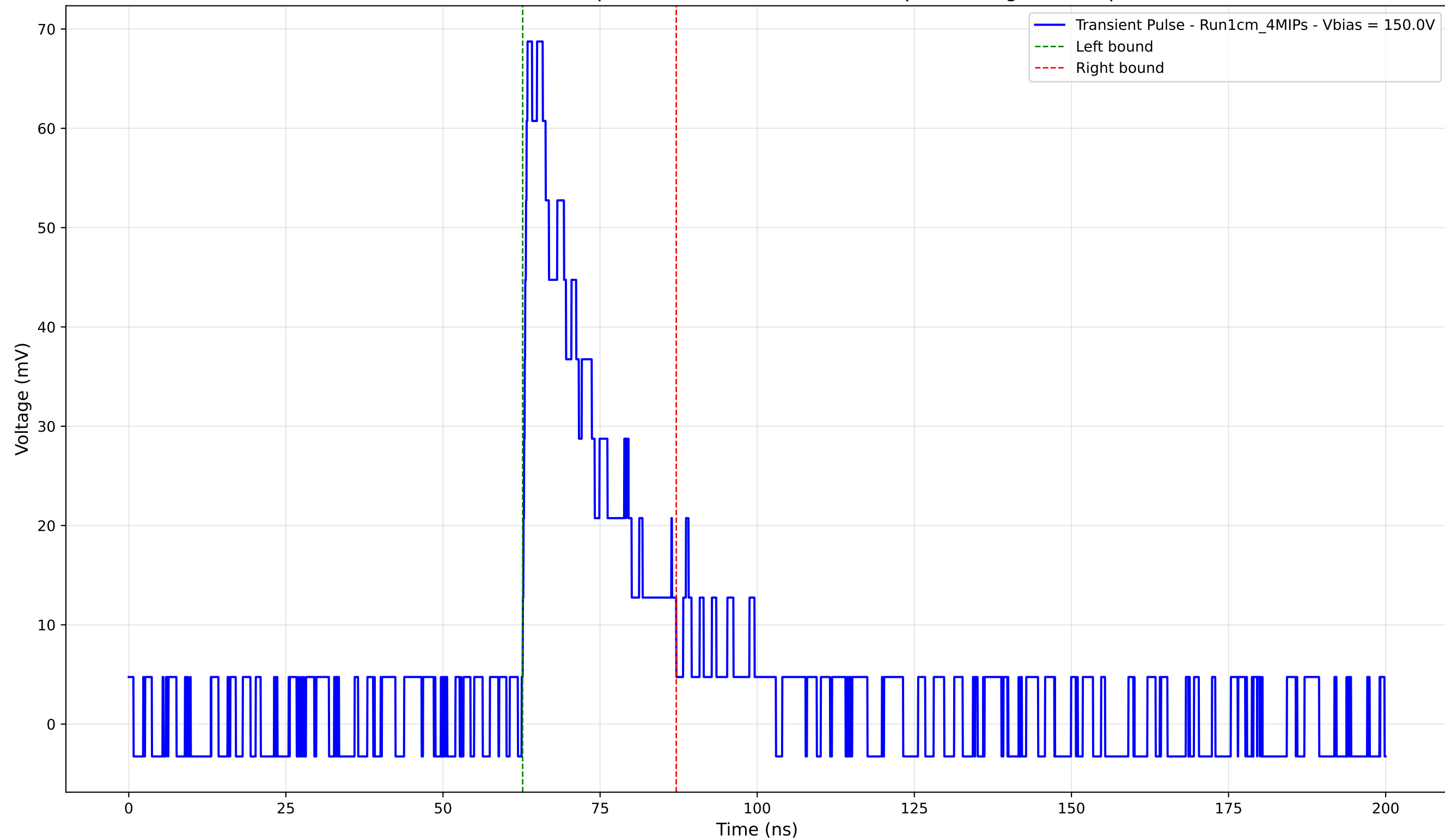
Transient Pulse - Sample: new1cm -Position: 595.0 \mu\text{m} - Charge: 15.48 pC
