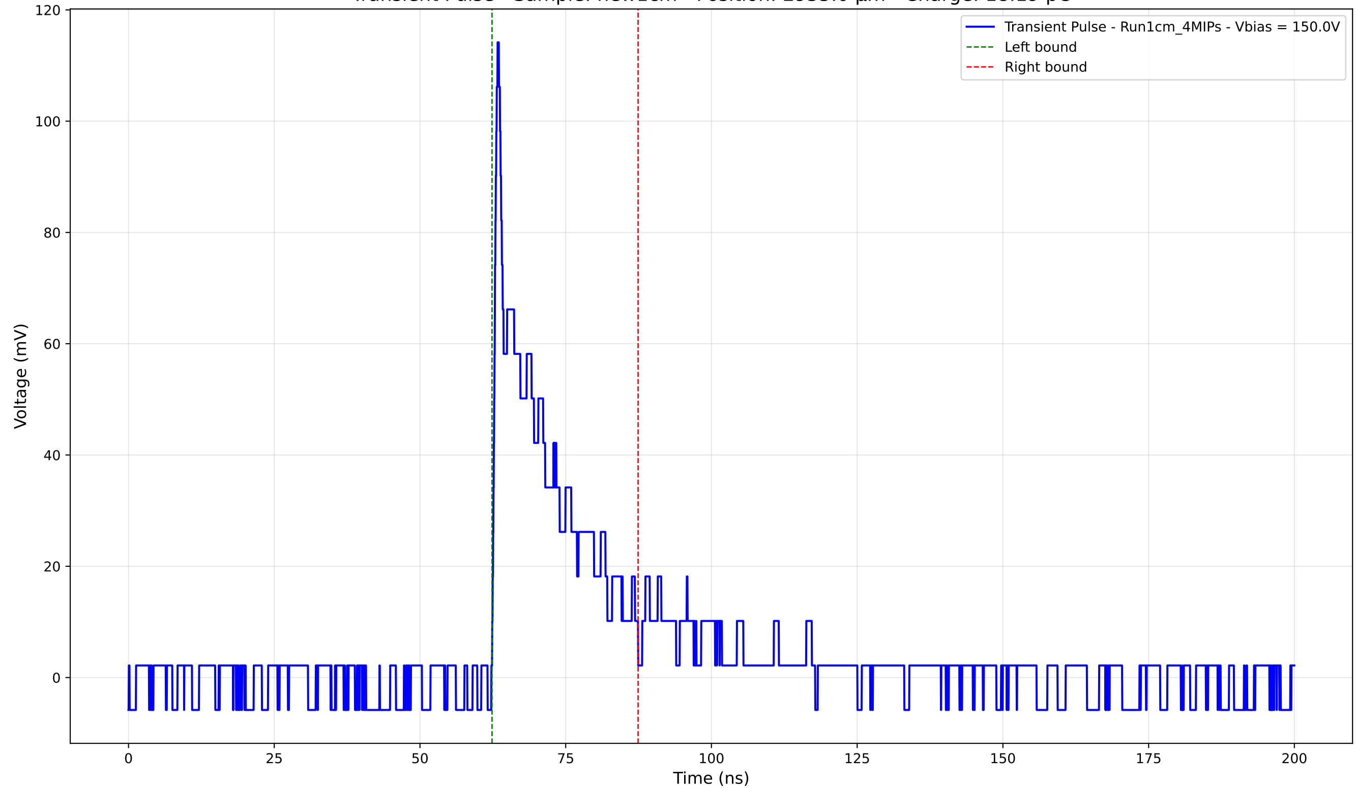
Transient Pulse - Sample: new1cm - Position: 2955.0 \mu\text{m} - Charge: 18.19 pC
