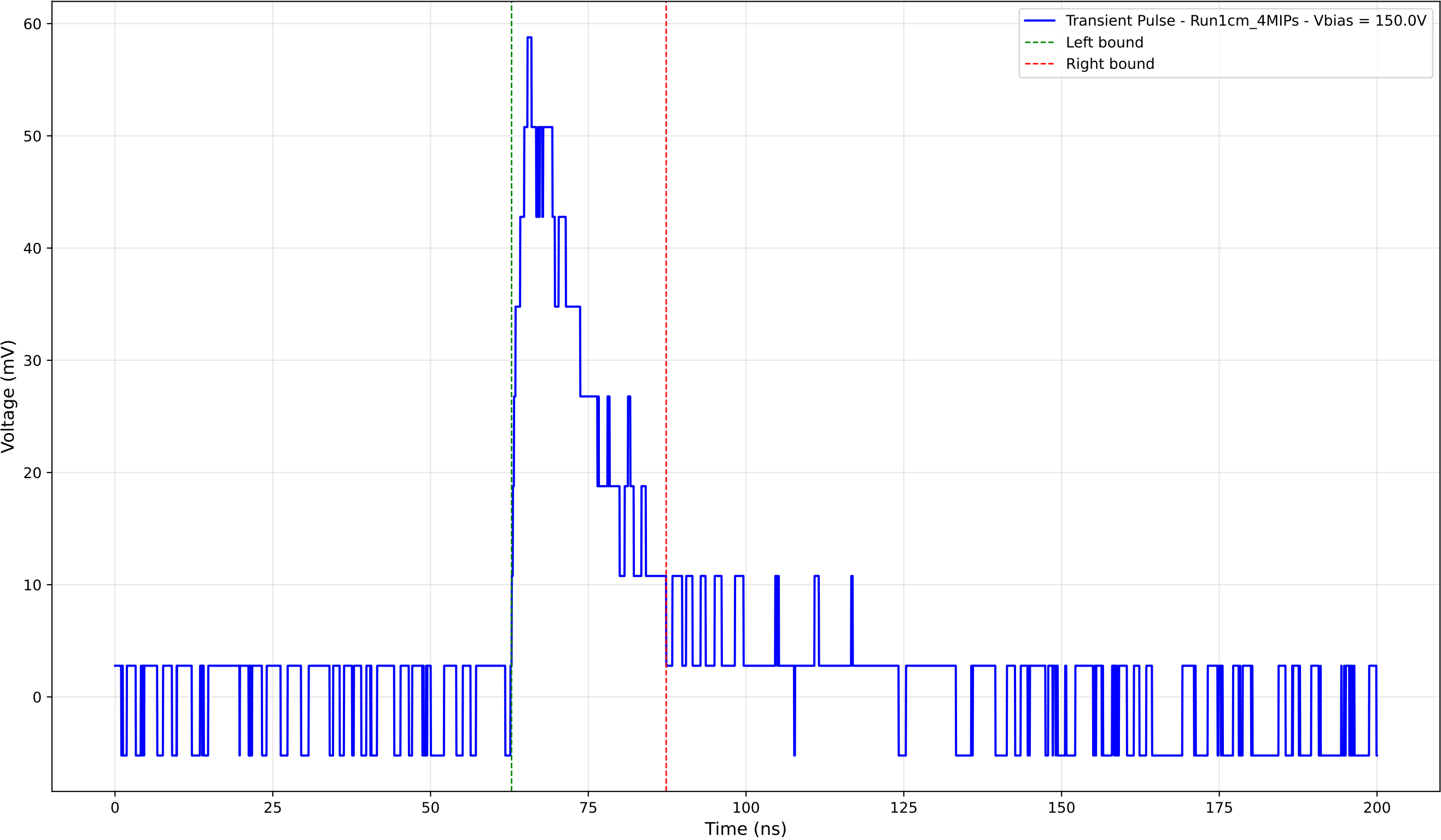
Transient Pulse - Sample: new1cm - Position: 1275.0 \mu\text{m} - Charge: 13.98 pC
