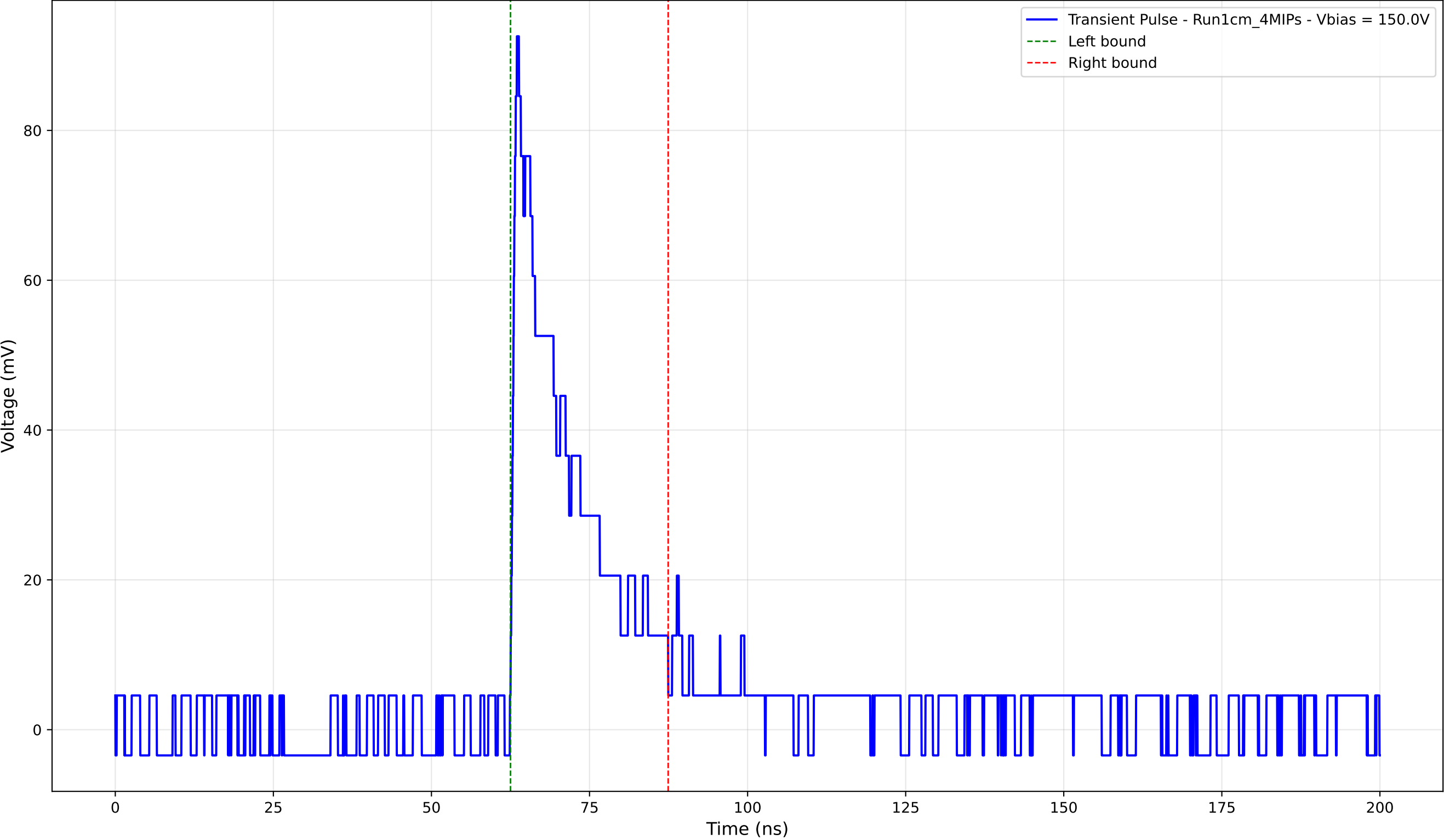
Transient Pulse - Sample: new1cm - Position: 4825.0 \mu\text{m} - Charge: 17.02 pC
