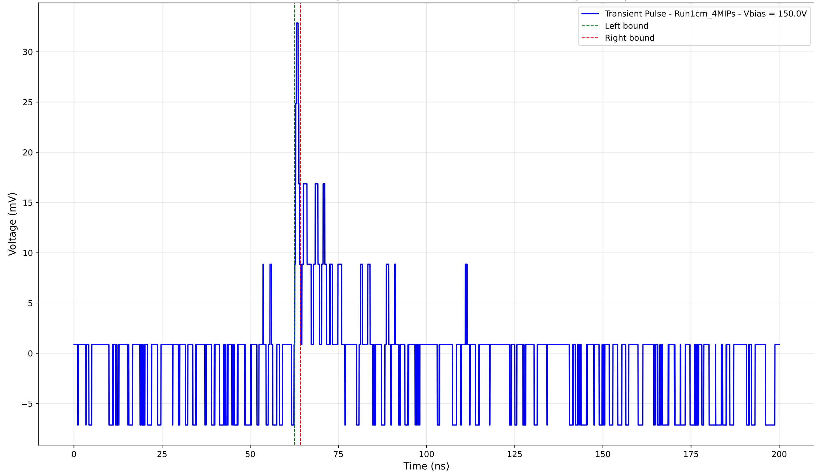
Transient Pulse - Sample: new1cm - Position: 3195.0 \mu\text{m} - Charge: 0.70 pC
