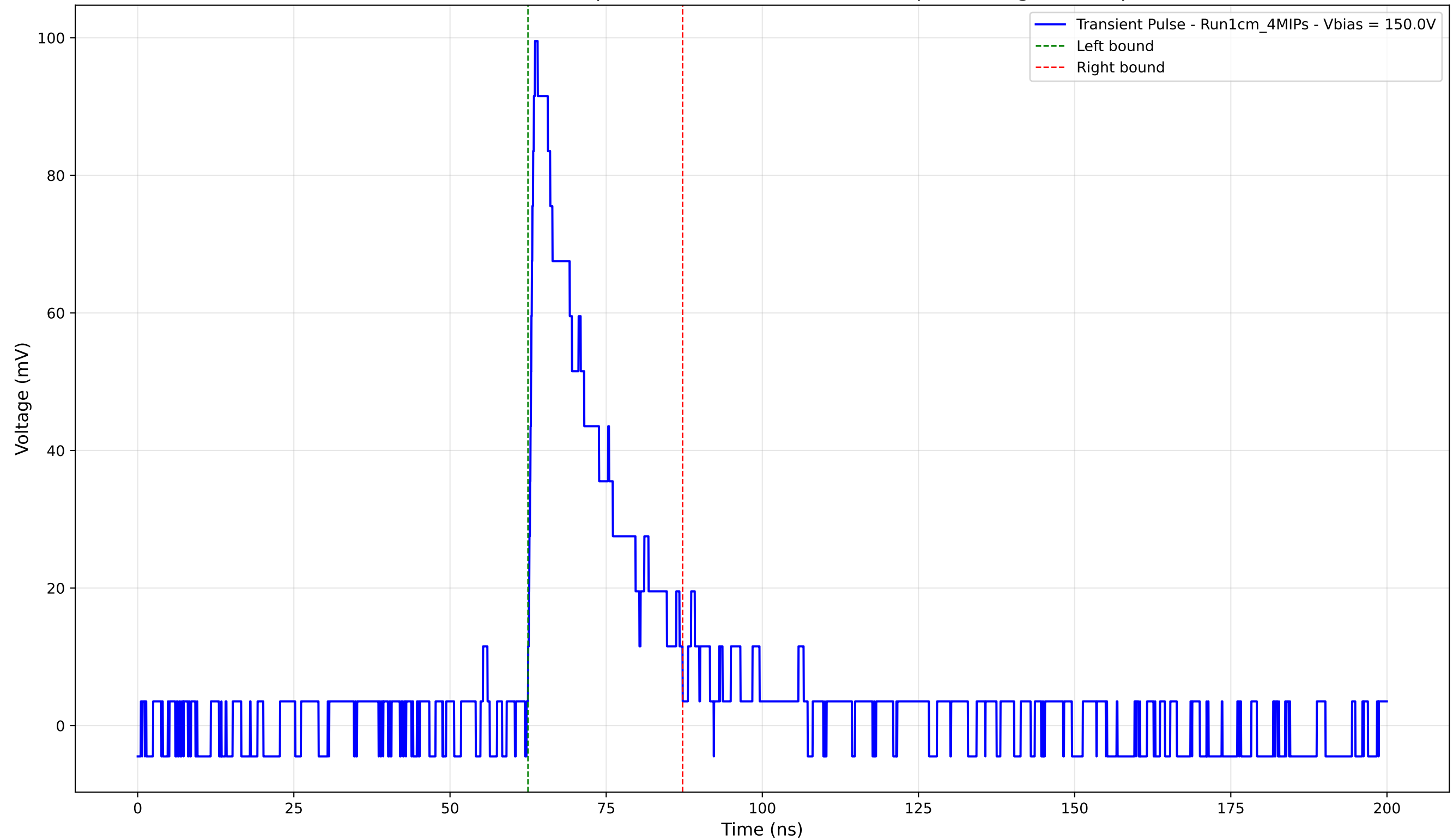
Transient Pulse - Sample: new1cm - Position: 4625.0 \mu\text{m} - Charge: 20.84 pC
