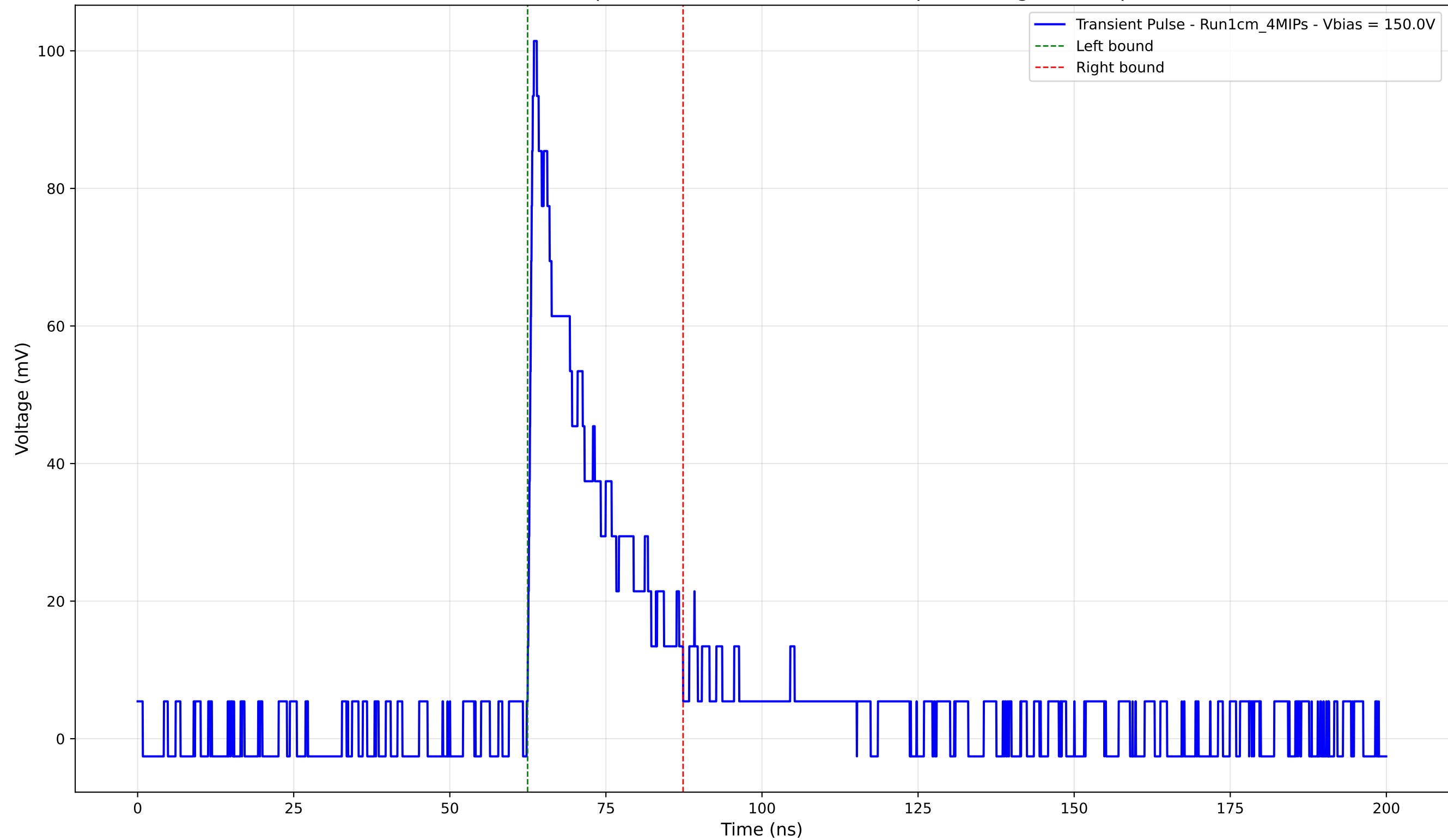
Transient Pulse - Sample: new1cm - Position: 4840.0 \mu\text{m} - Charge: 19.97 pC
