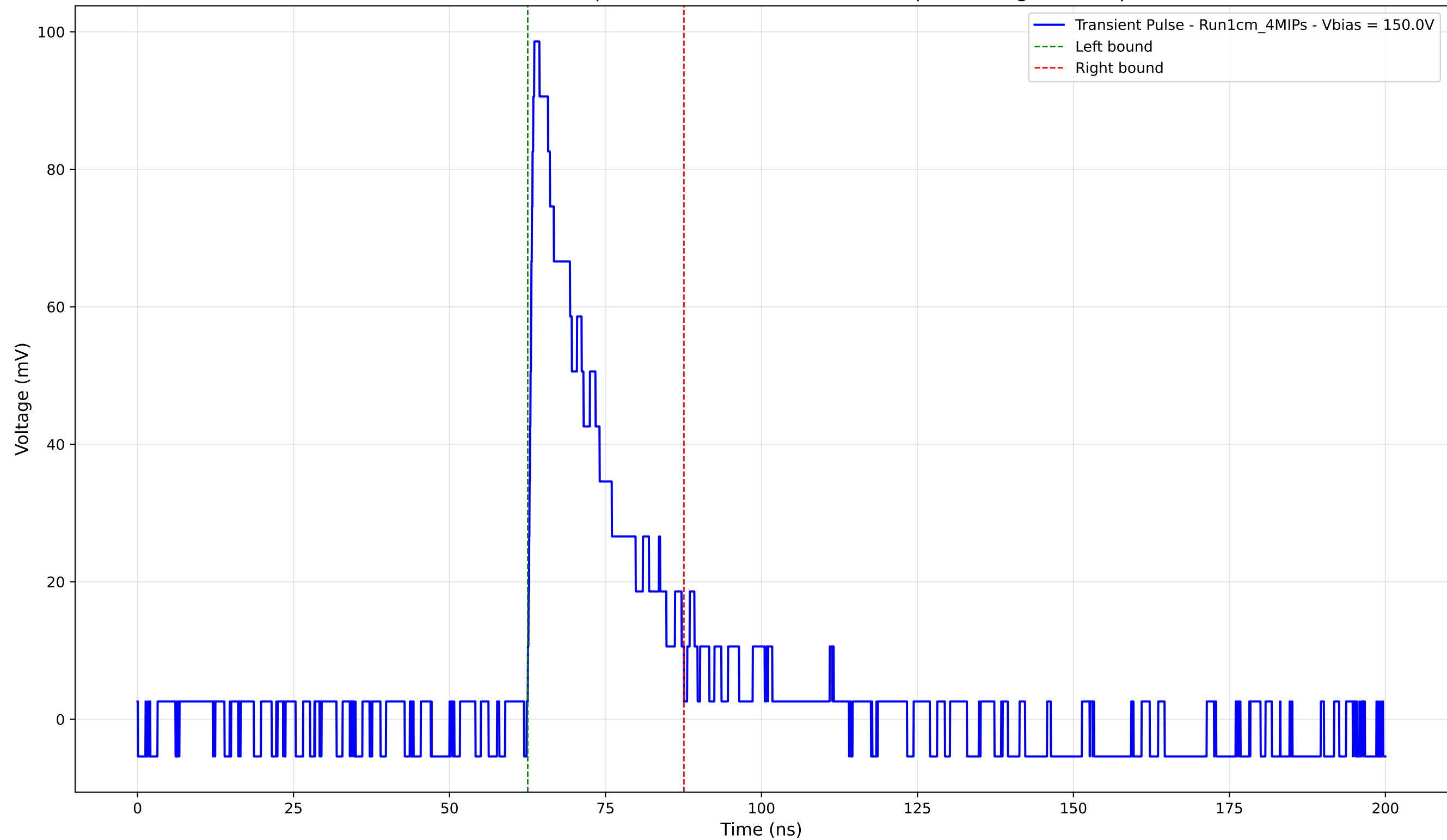
Transient Pulse - Sample: new1cm - Position: 4605.0 \mu\text{m} - Charge: 21.01 pC
