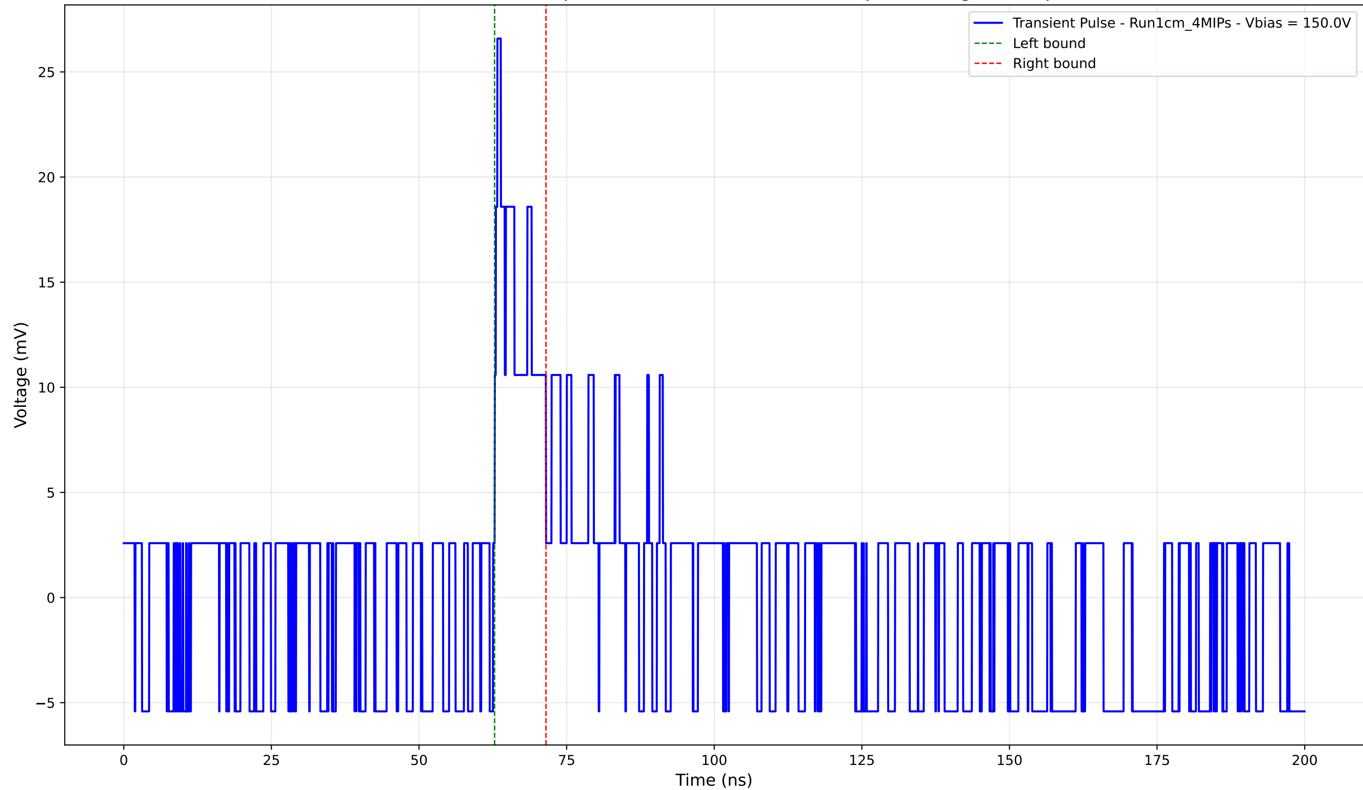
Transient Pulse - Sample: new1cm - Position: 4755.0 \mu\text{m} - Charge: 2.53 pC
