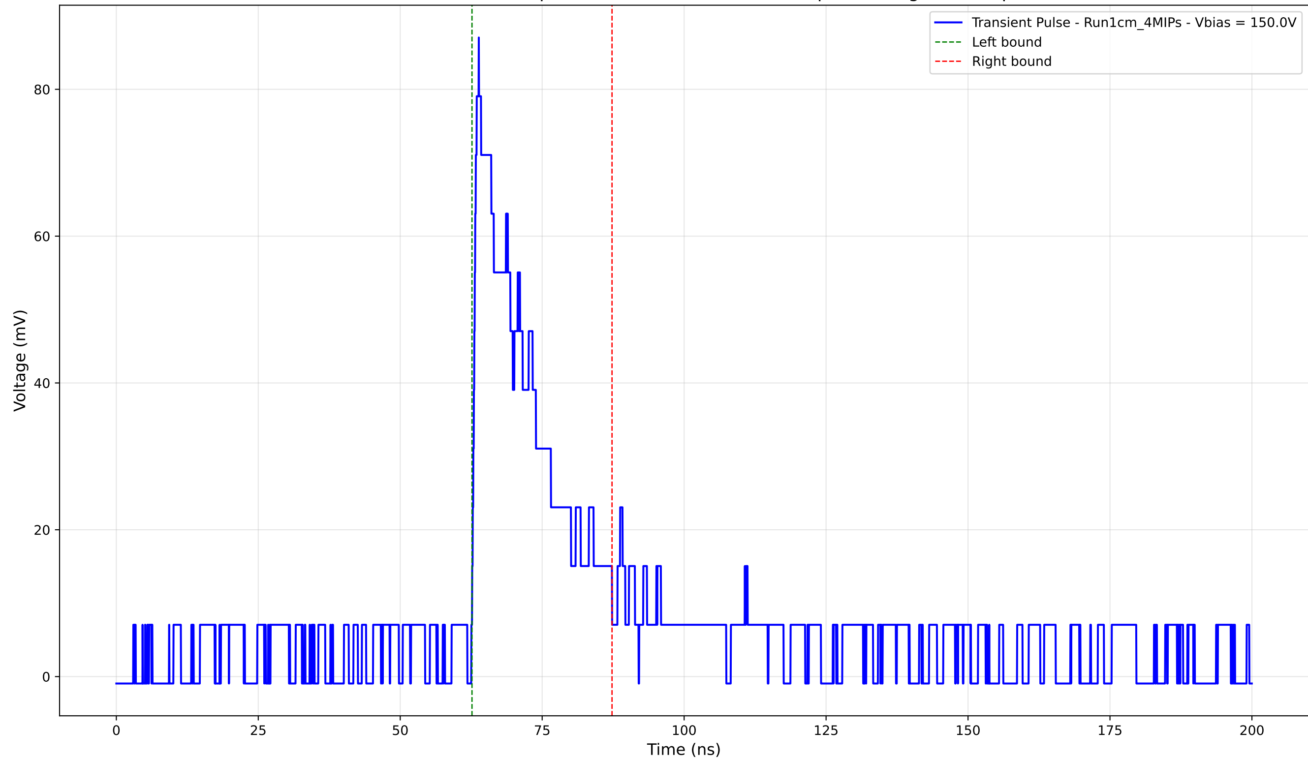
Transient Pulse - Sample: new1cm - Position: 565.0 \mu\text{m} - Charge: 18.04 pC
