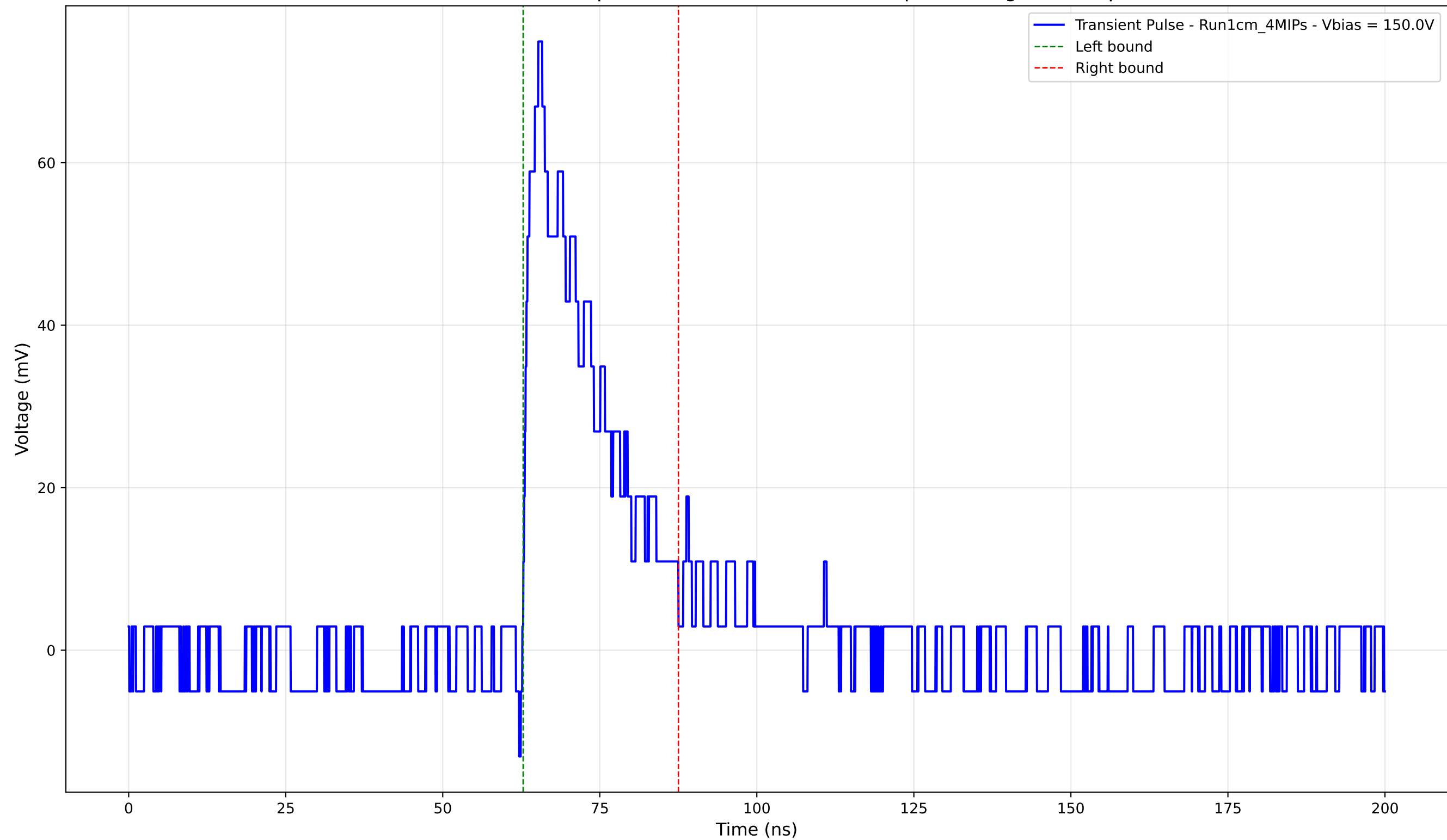
Transient Pulse - Sample: new1cm -Position: 855.0 \mu\text{m} - Charge: 16.50 pC
