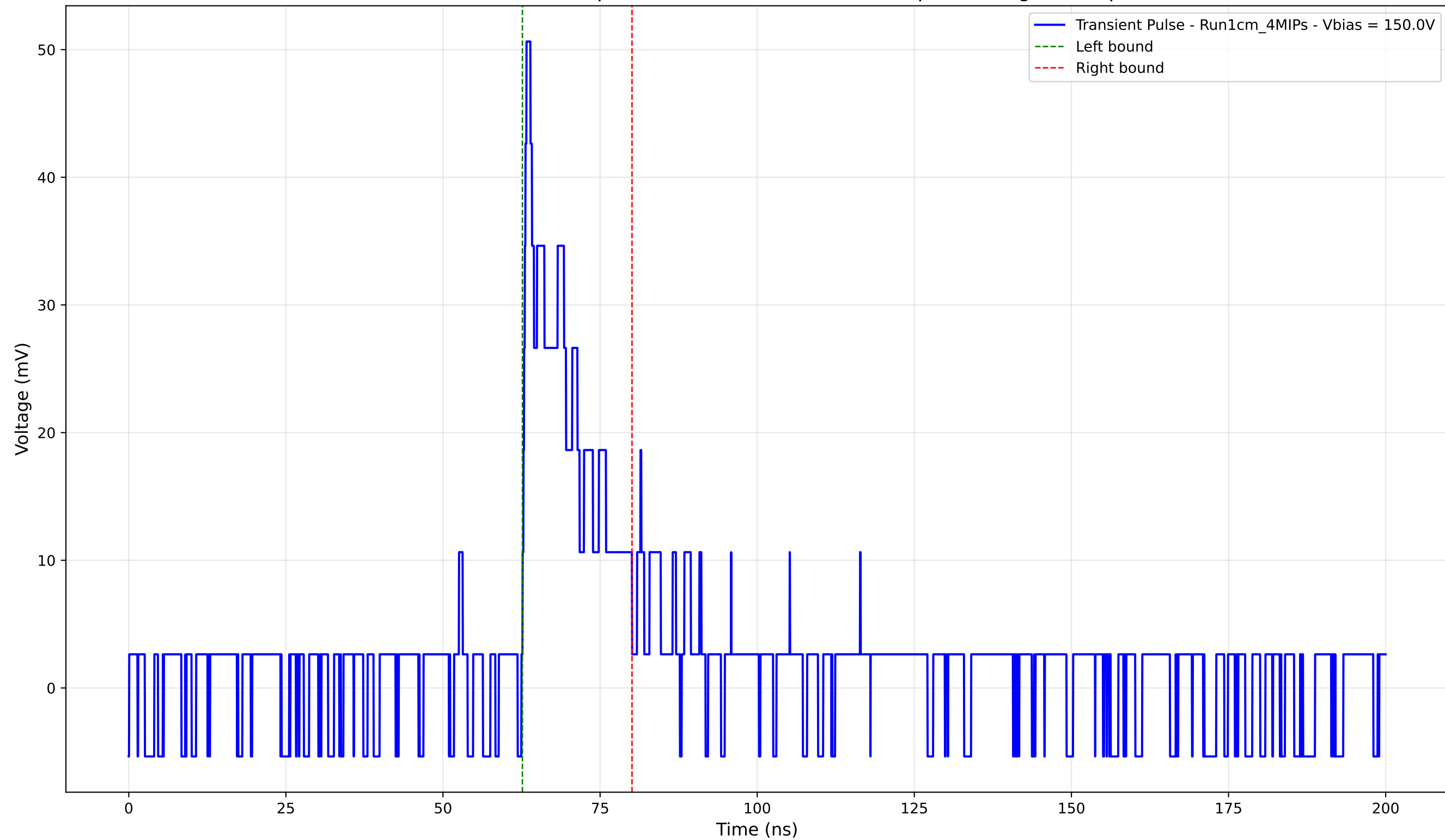
Transient Pulse - Sample: new1cm -Position: 3670.0 \mu\text{m} - Charge: 7.60 pC
