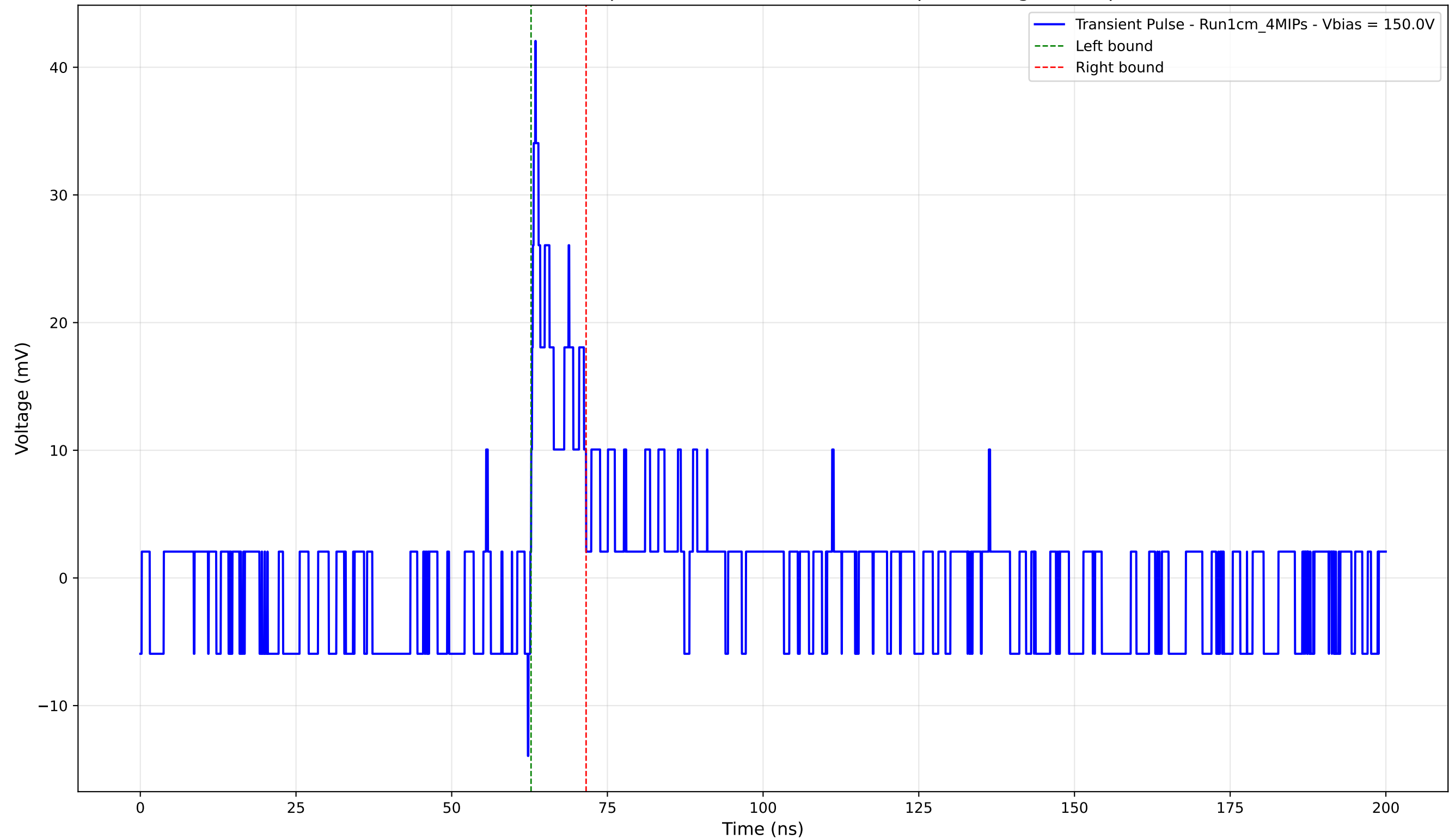
Transient Pulse - Sample: new1cm - Position: 225.0 \mu\text{m} - Charge: 3.16 pC
