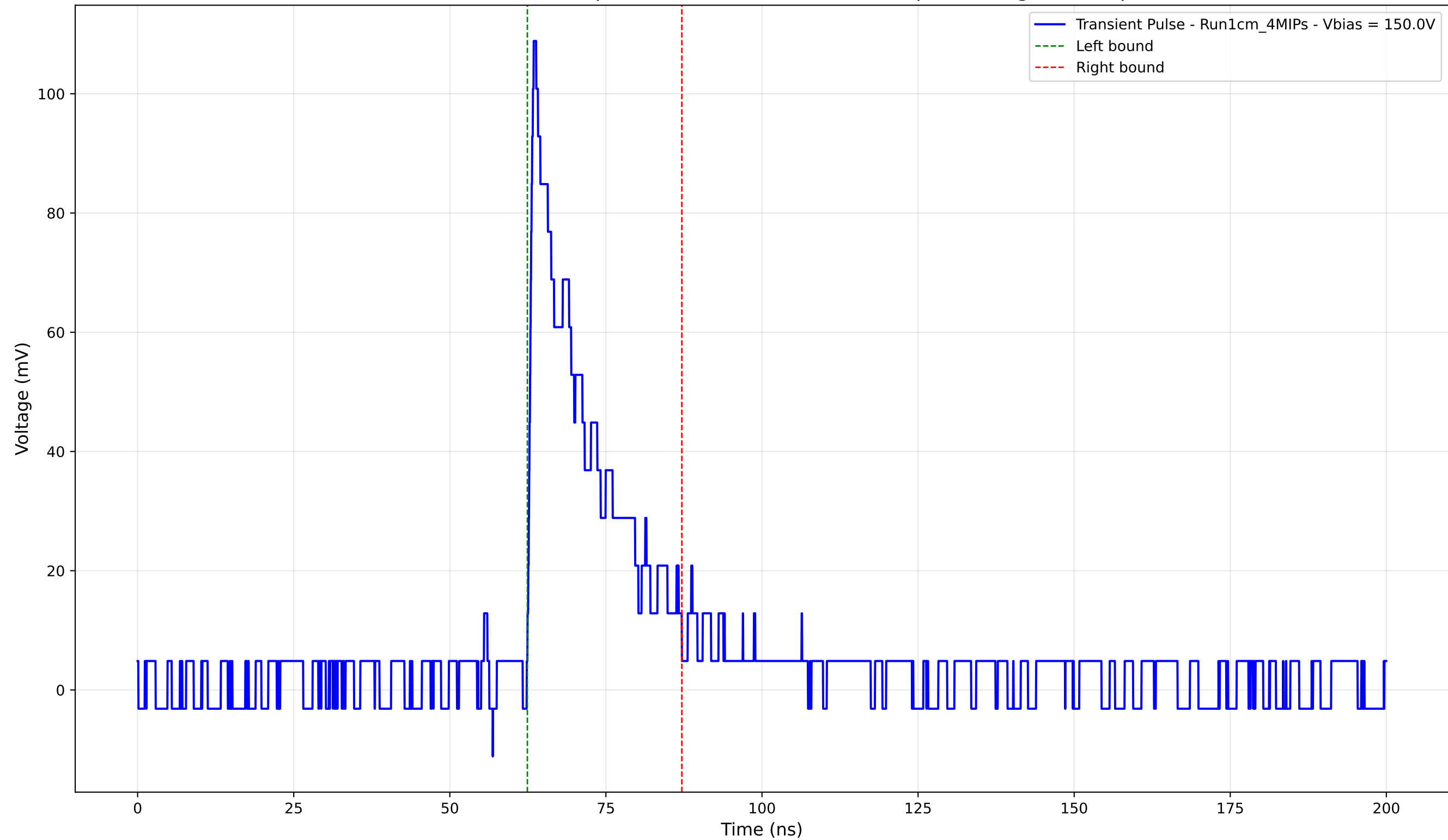
Transient Pulse - Sample: new1cm - Position: 4885.0 \mu\text{m} - Charge: 20.52 pC
