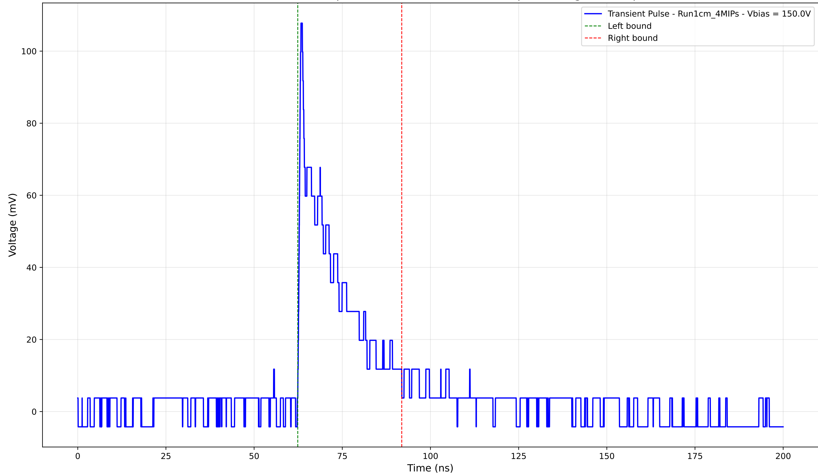
Transient Pulse - Sample: new1cm - Position: 2905.0 \mu\text{m} - Charge: 20.30 pC
