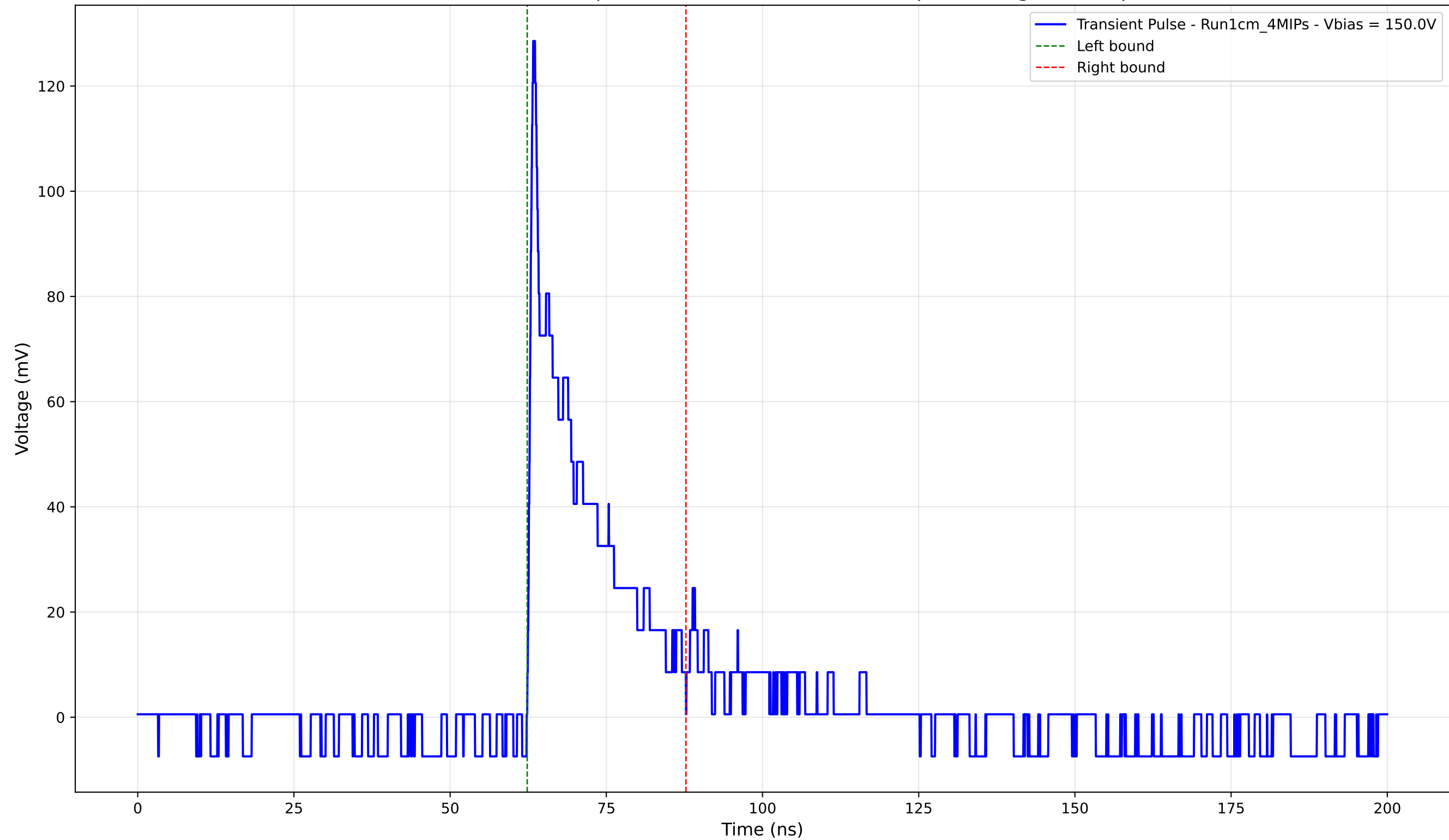
Transient Pulse - Sample: new1cm - Position: 3430.0 \mu\text{m} - Charge: 19.86 pC
