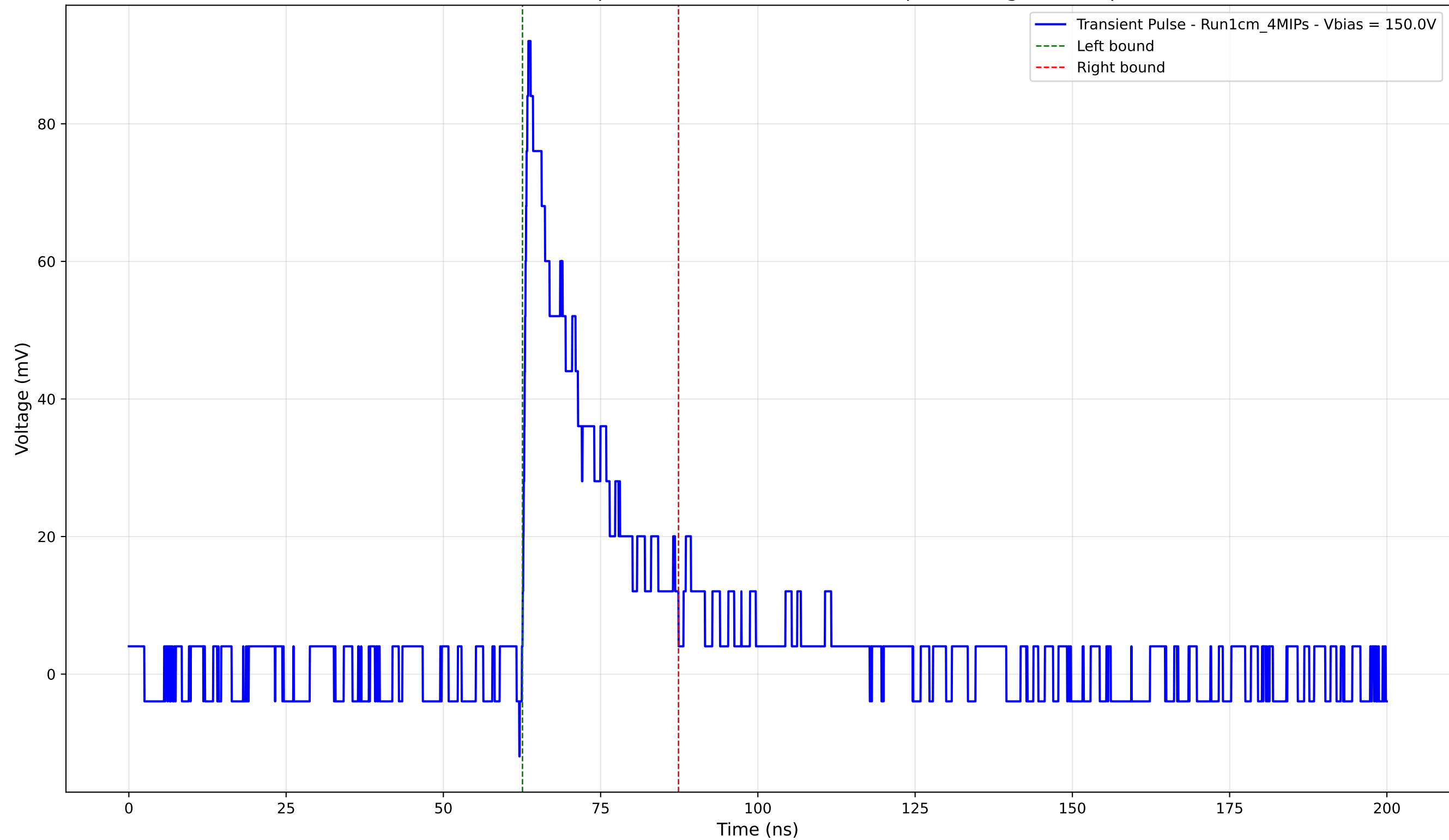
Transient Pulse - Sample: new1cm -Position: 460.0 \mu\text{m} - Charge: 17.60 pC
