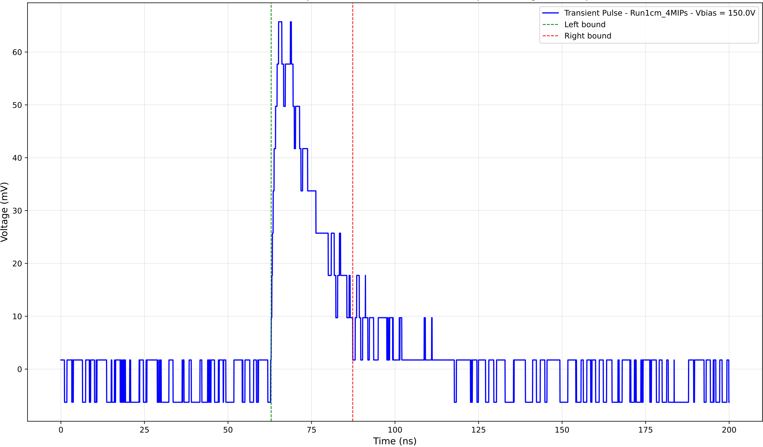
Transient Pulse - Sample: new1cm - Position: 1435.0 \mu\text{m} - Charge: 16.73 pC
