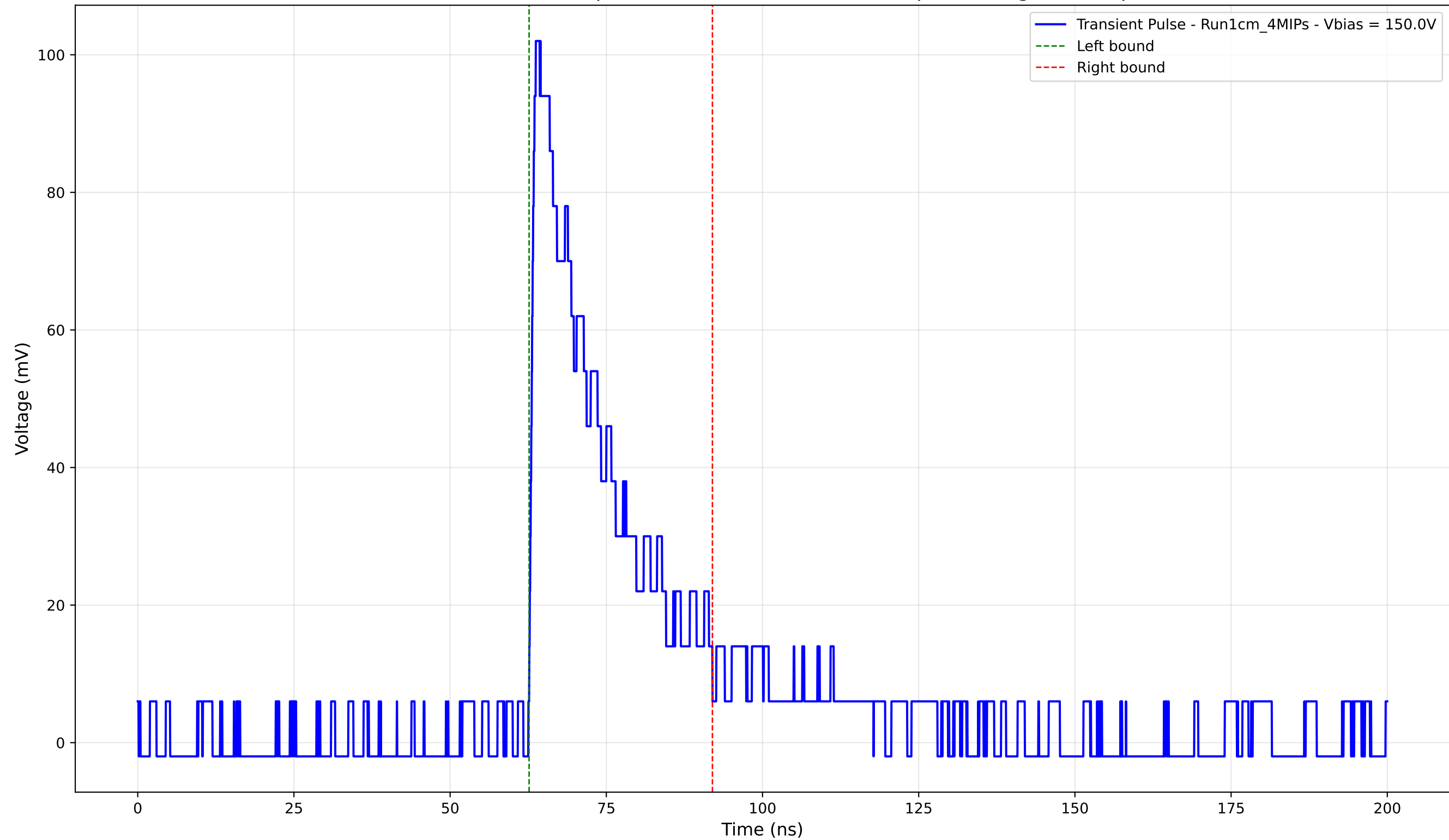
Transient Pulse - Sample: new1cm - Position: 3975.0 \mu\text{m} - Charge: 24.83 pC
