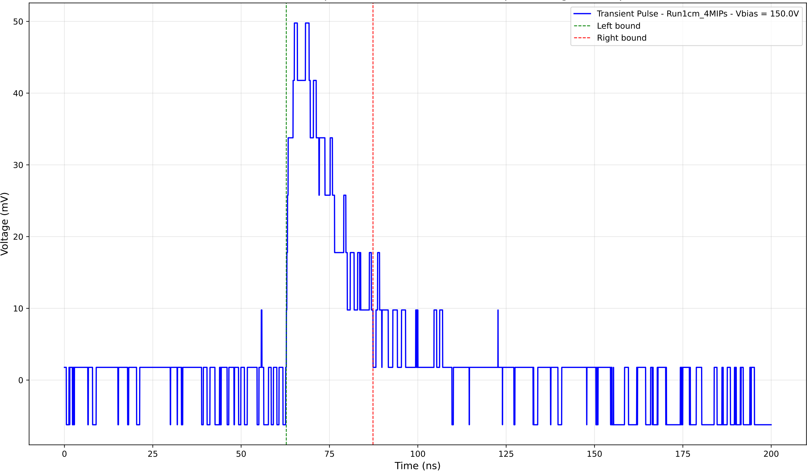
Transient Pulse - Sample: new1cm - Position: 2115.0 \mu\text{m} - Charge: 13.10 pC
