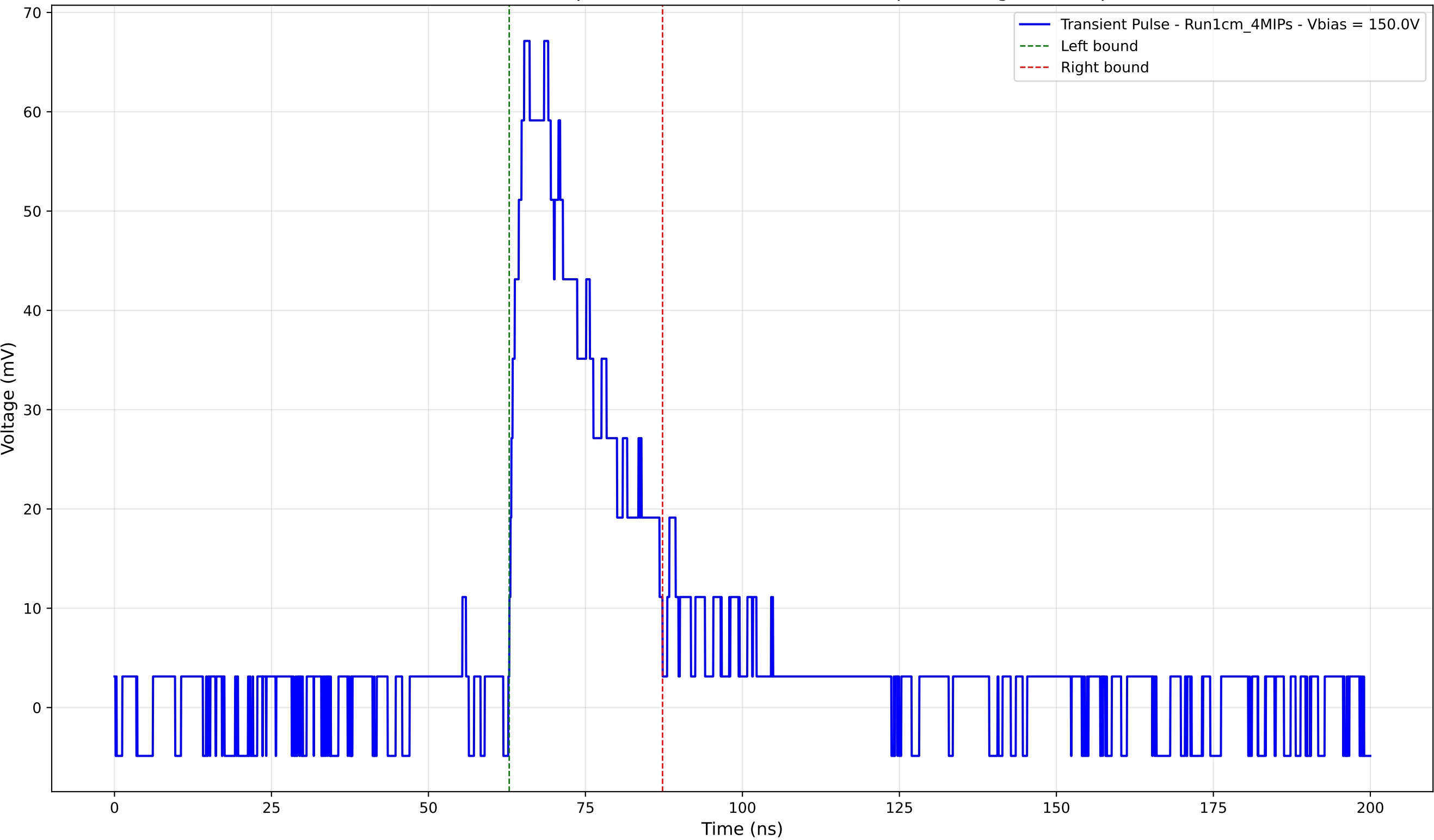
Transient Pulse - Sample: new1cm - Position: 1895.0 \mu\text{m} - Charge: 18.11 pC
