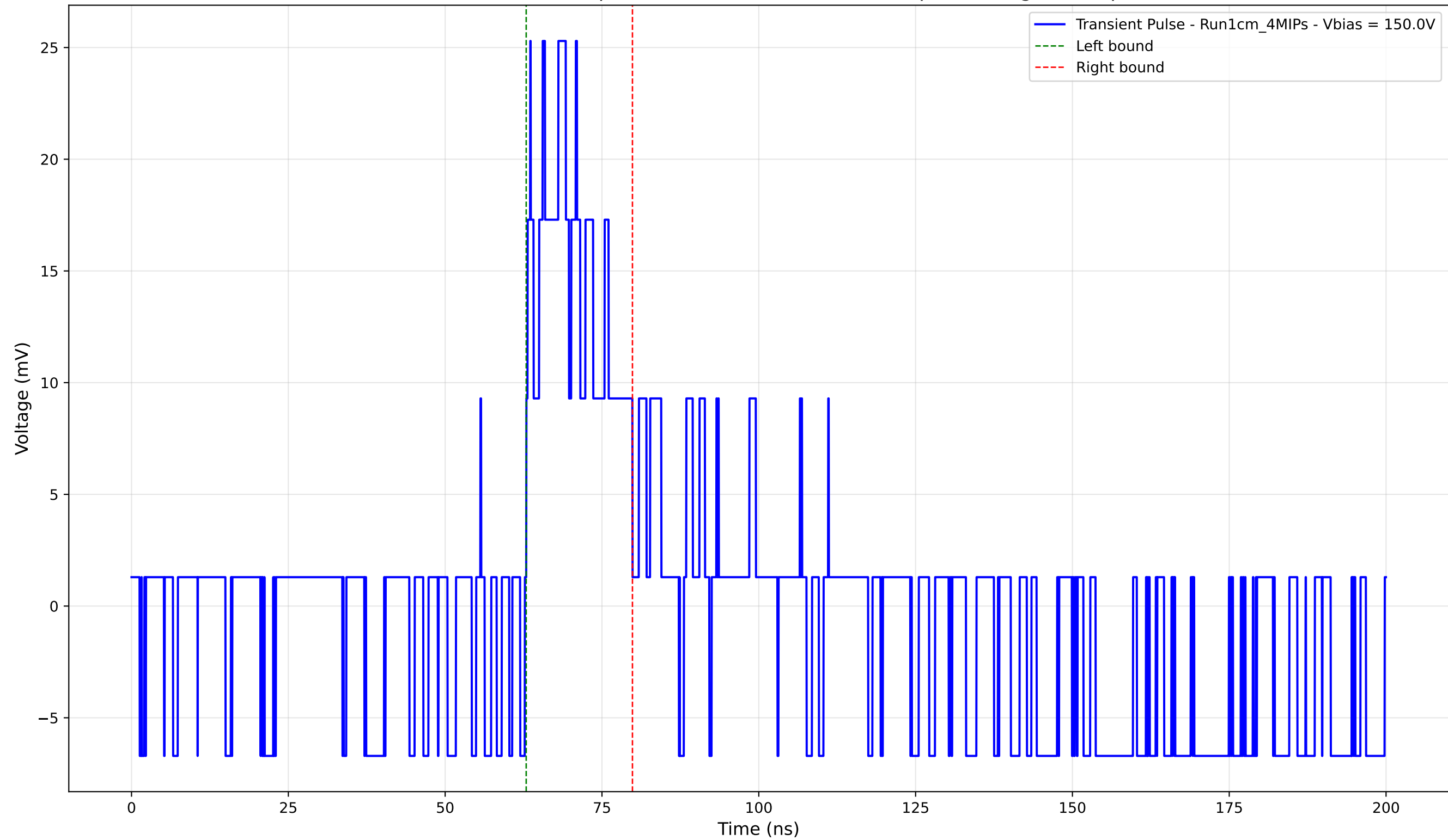
Transient Pulse - Sample: new1cm - Position: 2155.0 \mu\text{m} - Charge: 4.89 pC
