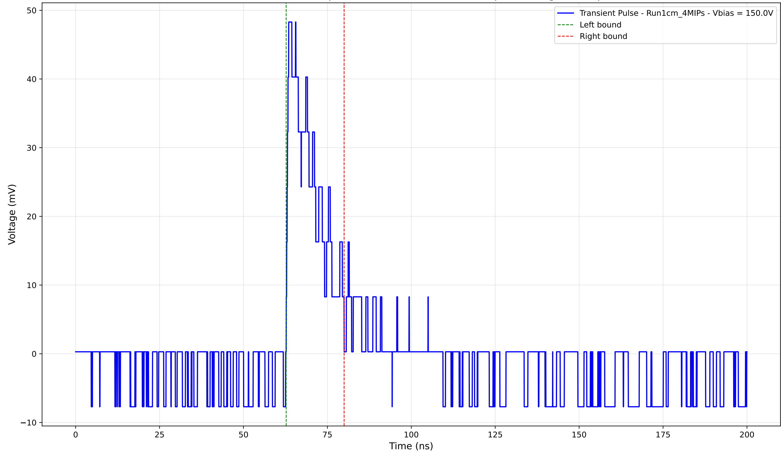
Transient Pulse - Sample: new1cm - Position: 620.0 \mu\text{m} - Charge: 8.52 pC
