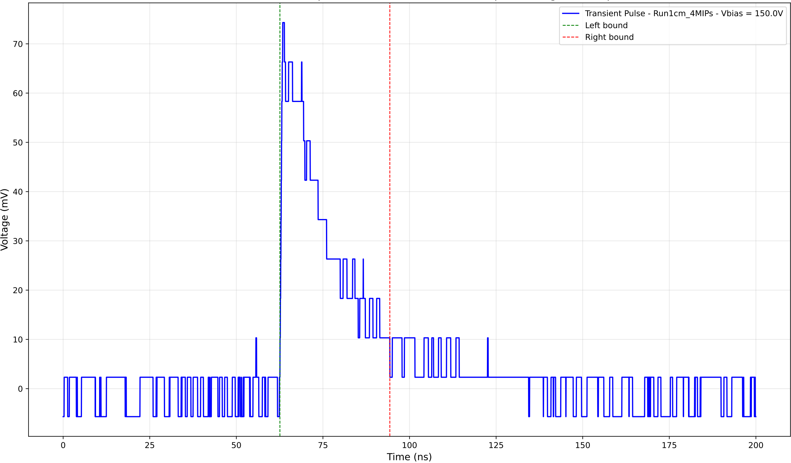
Transient Pulse - Sample: new1cm - Position: 2590.0 \mu\text{m} - Charge: 20.25 pC
