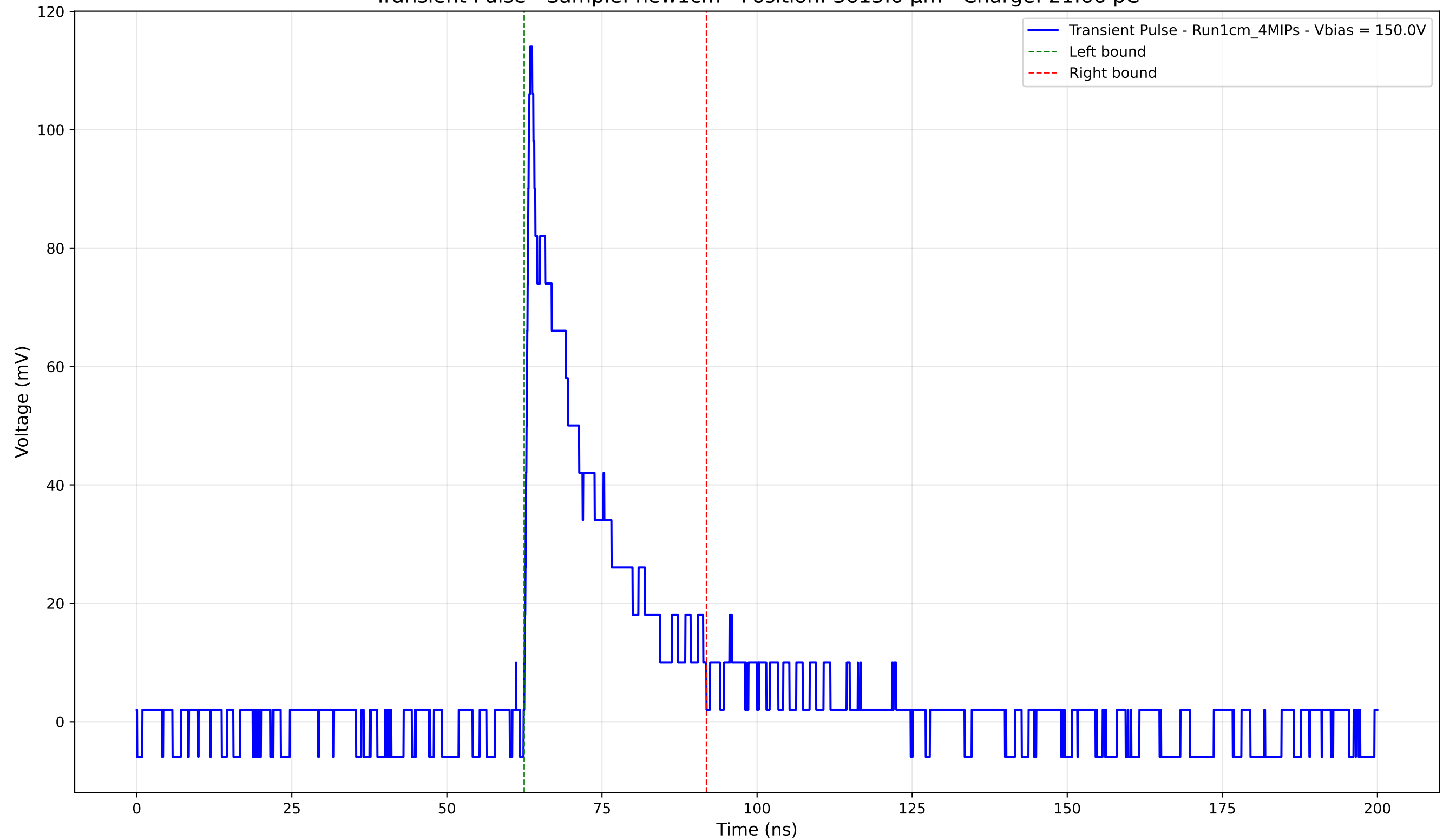
Transient Pulse - Sample: new1cm - Position: 3615.0 \mu\text{m} - Charge: 21.66 pC
