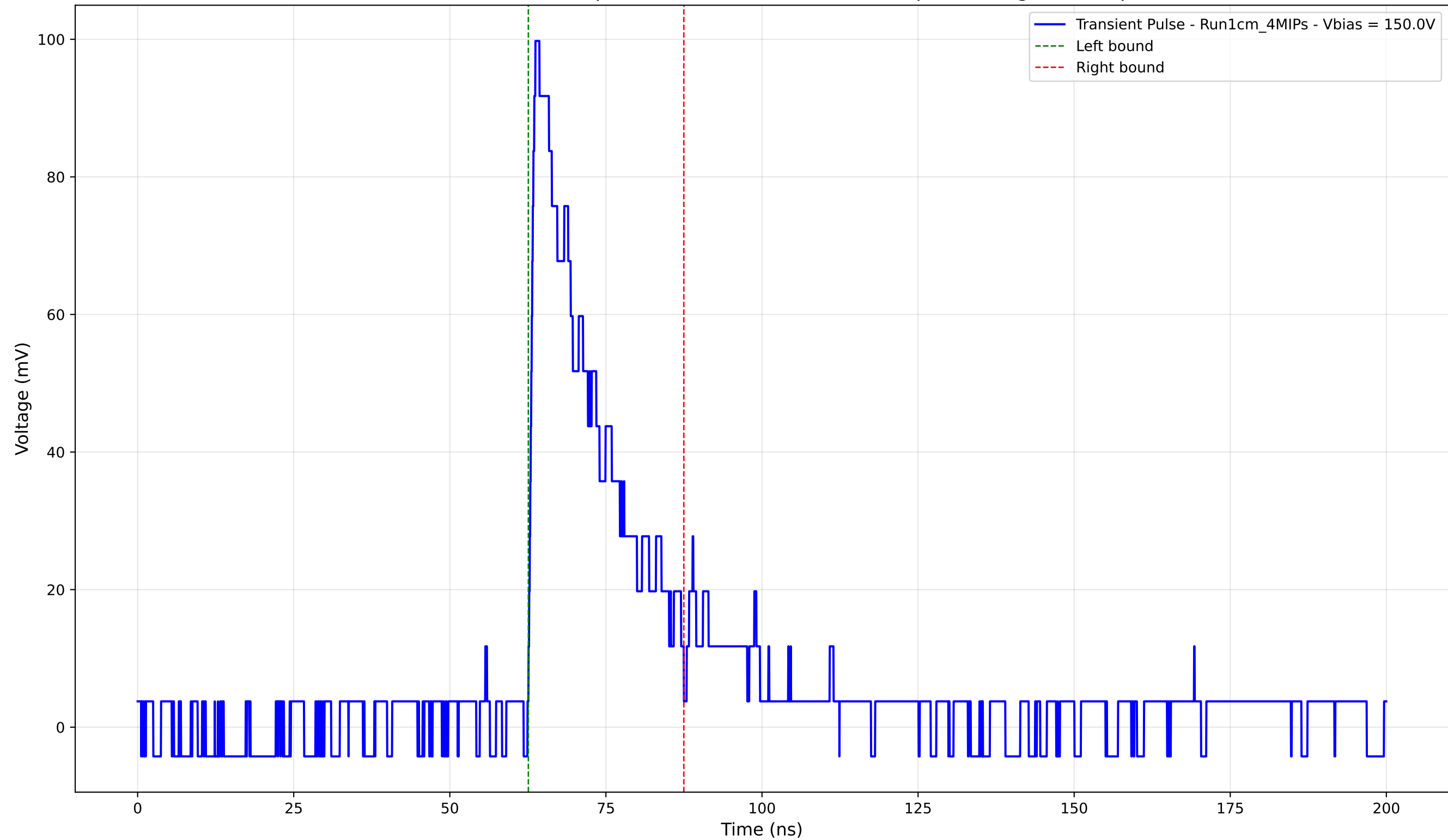
Transient Pulse - Sample: new1cm - Position: 3955.0 \mu\text{m} - Charge: 22.38 pC
