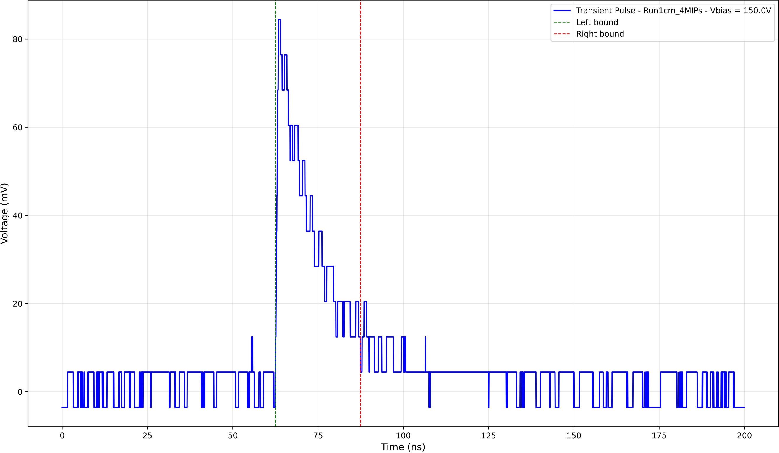
Transient Pulse - Sample: new1cm - Position: 3800.0 \mu\text{m} - Charge: 18.64 pC
