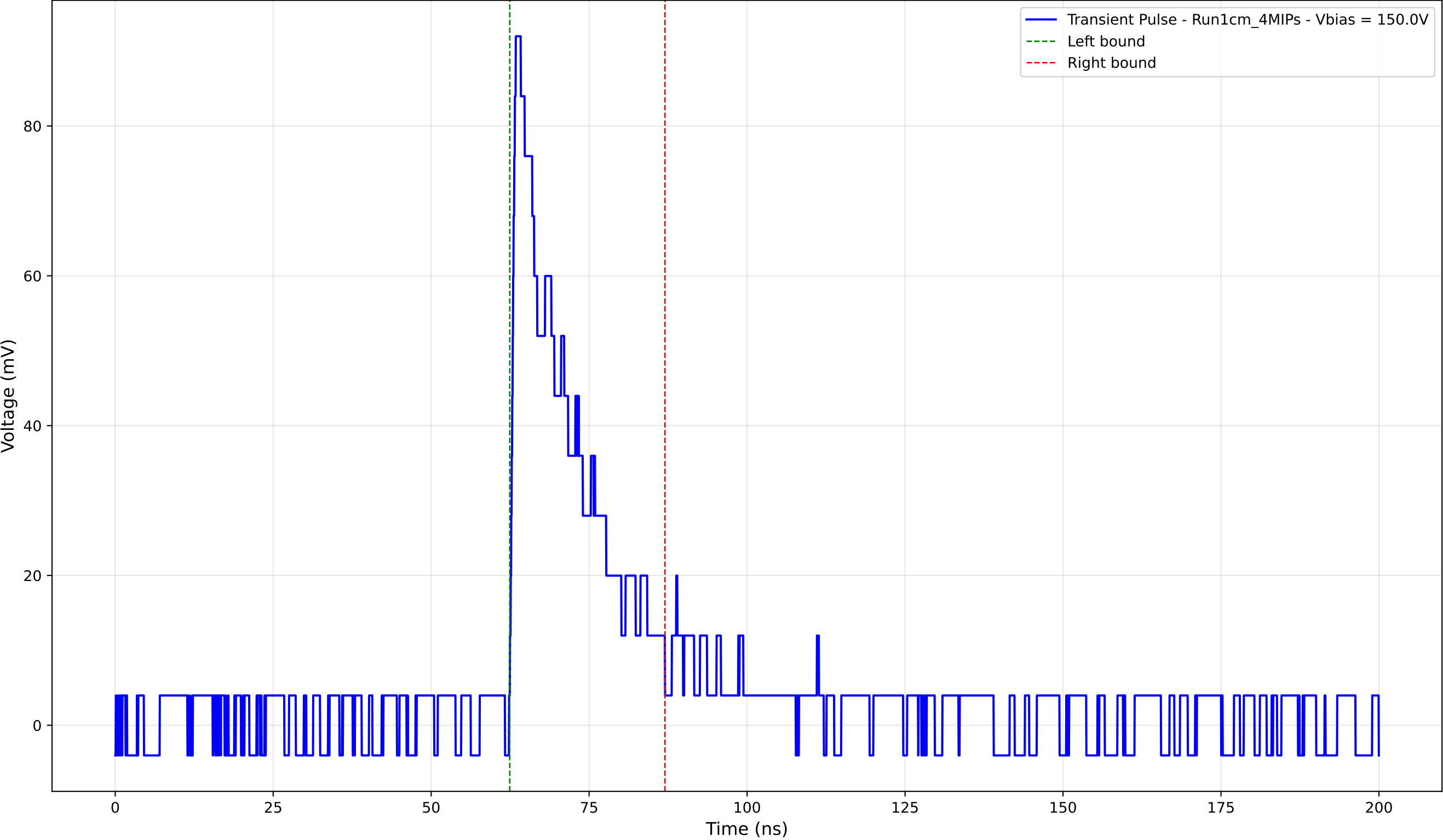
Transient Pulse - Sample: new1cm - Position: 4835.0 \mu\text{m} - Charge: 18.15 pC
