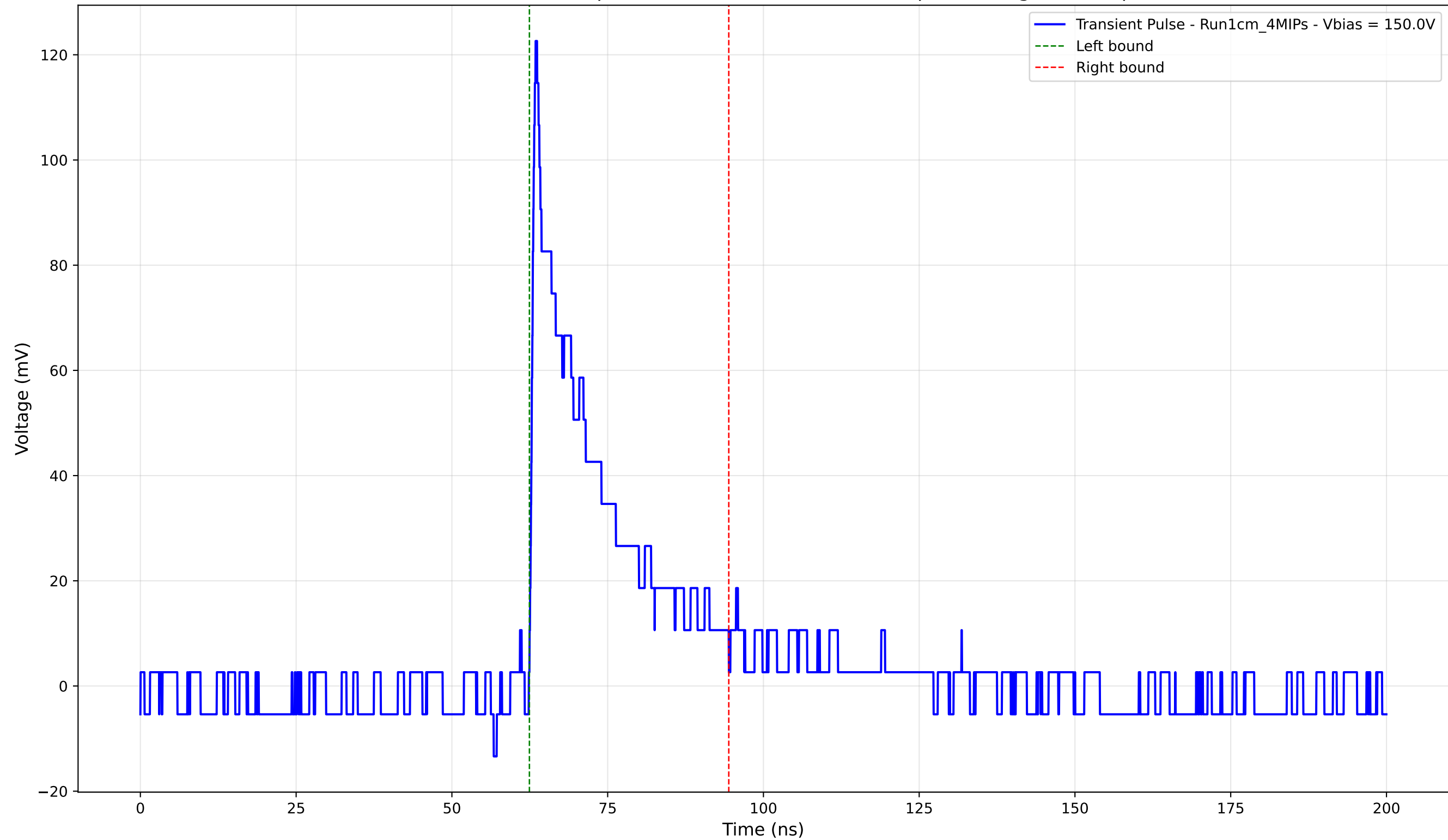
Transient Pulse - Sample: new1cm - Position: 3580.0 \mu\text{m} - Charge: 23.19 pC
