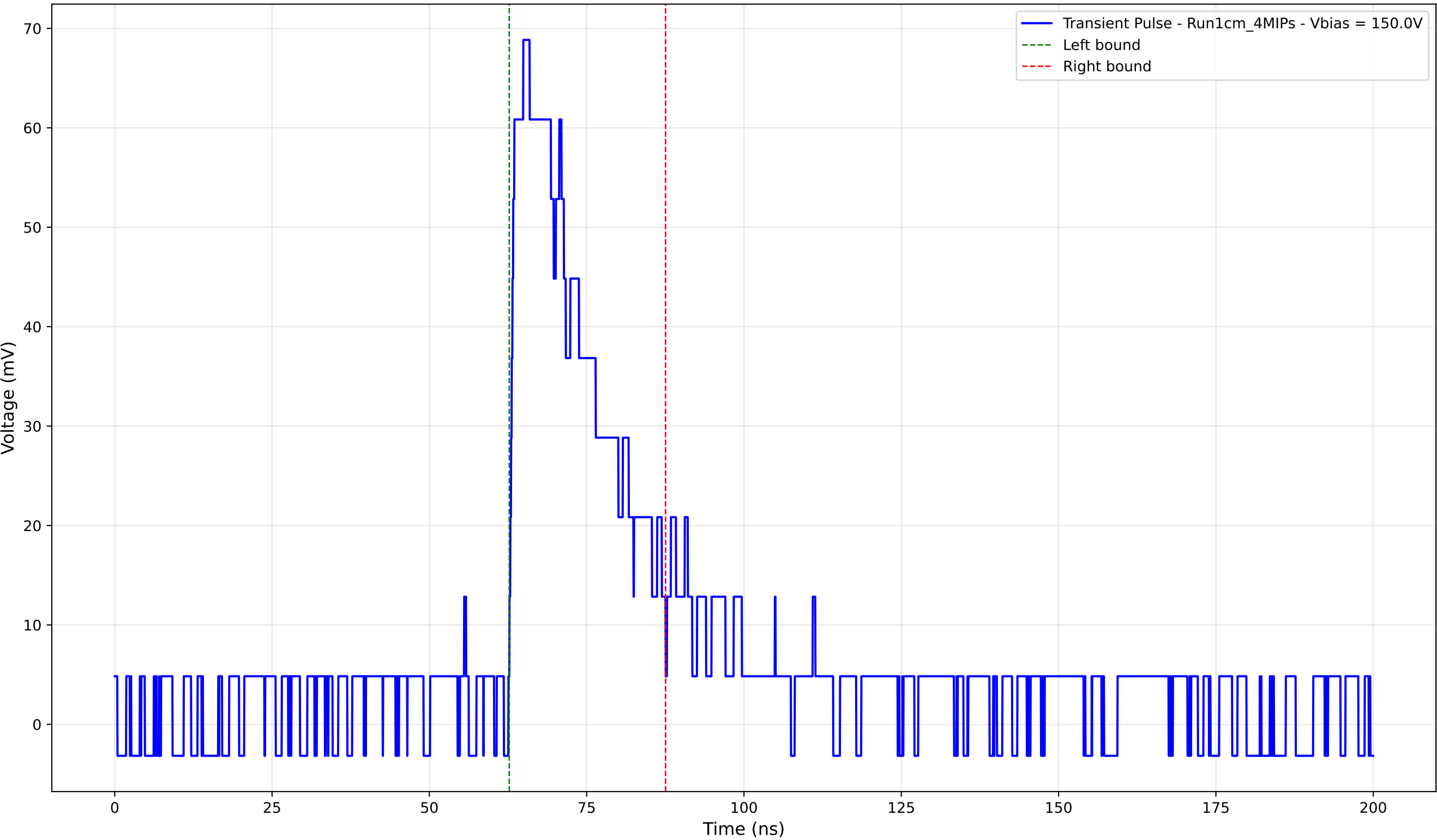
Transient Pulse - Sample: new1cm - Position: 2340.0 \mu\text{m} - Charge: 19.07 pC
