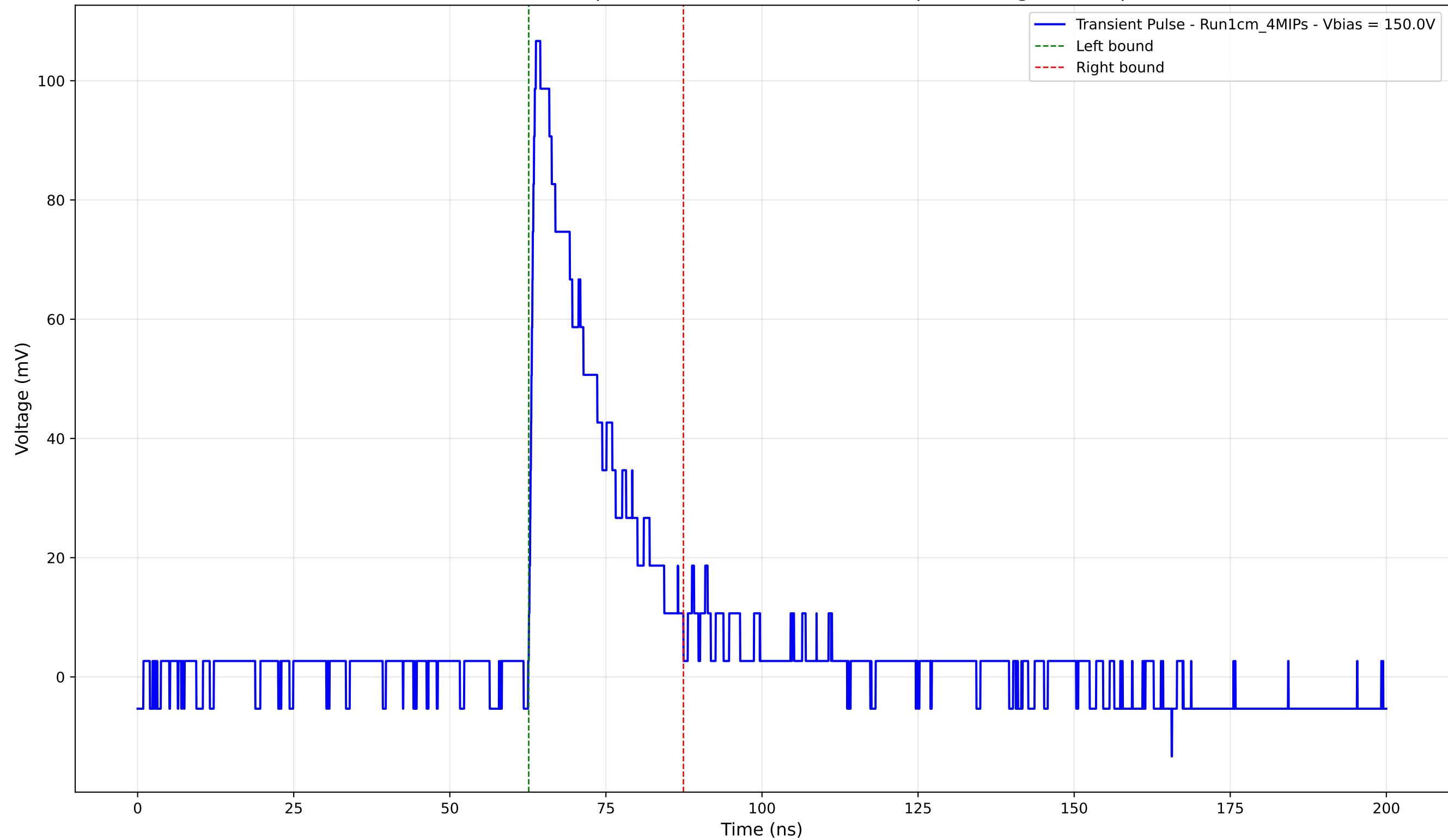
Transient Pulse - Sample: new1cm - Position: 4400.0 \mu\text{m} - Charge: 22.44 pC
