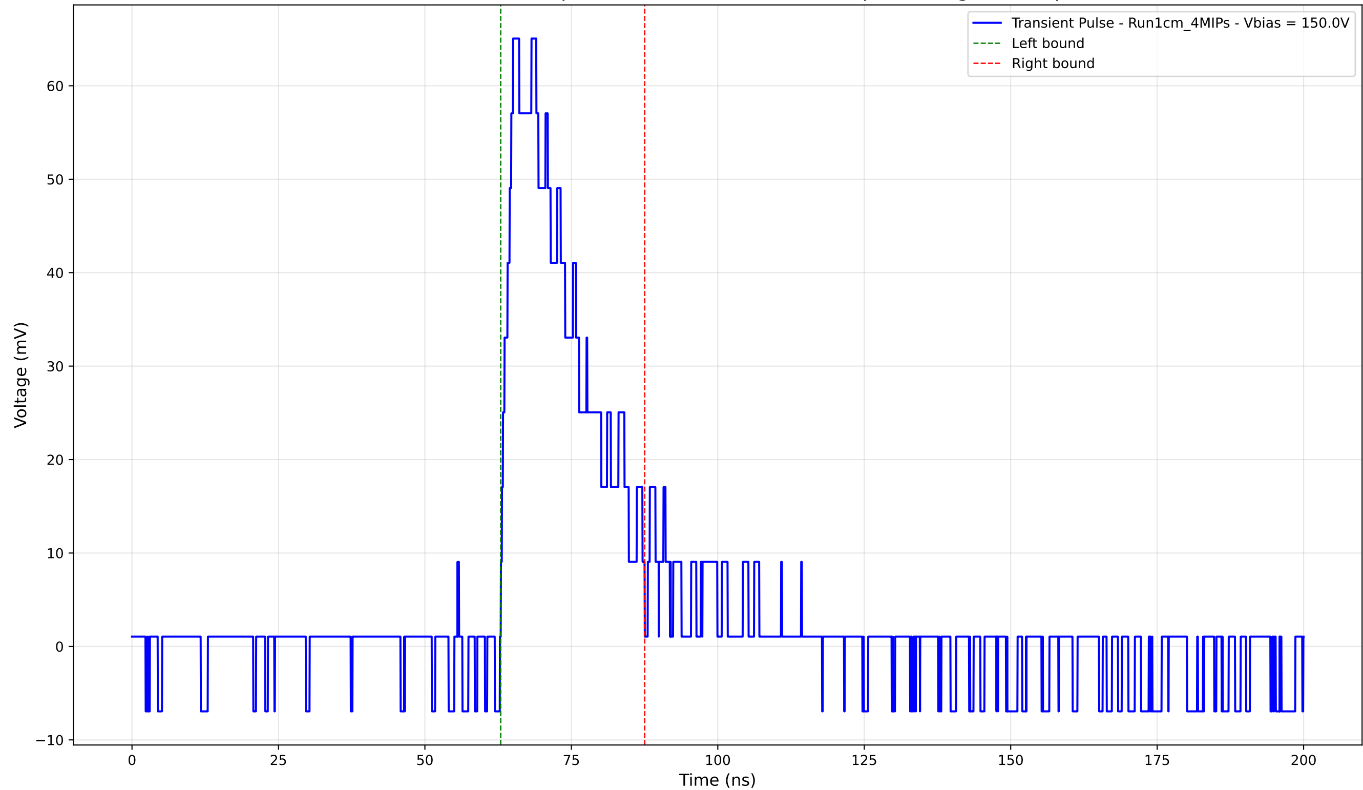
Transient Pulse - Sample: new1cm - Position: 1530.0 \mu\text{m} - Charge: 17.06 pC
