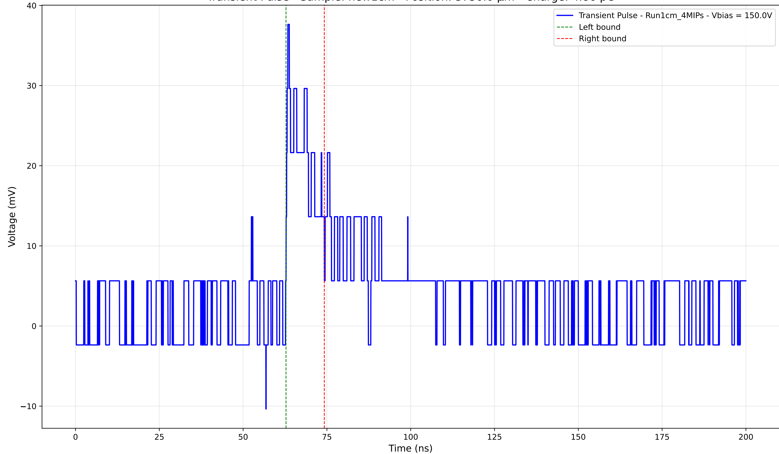
Transient Pulse - Sample: new1cm - Position: 3750.0 \mu\text{m} - Charge: 4.86 pC
