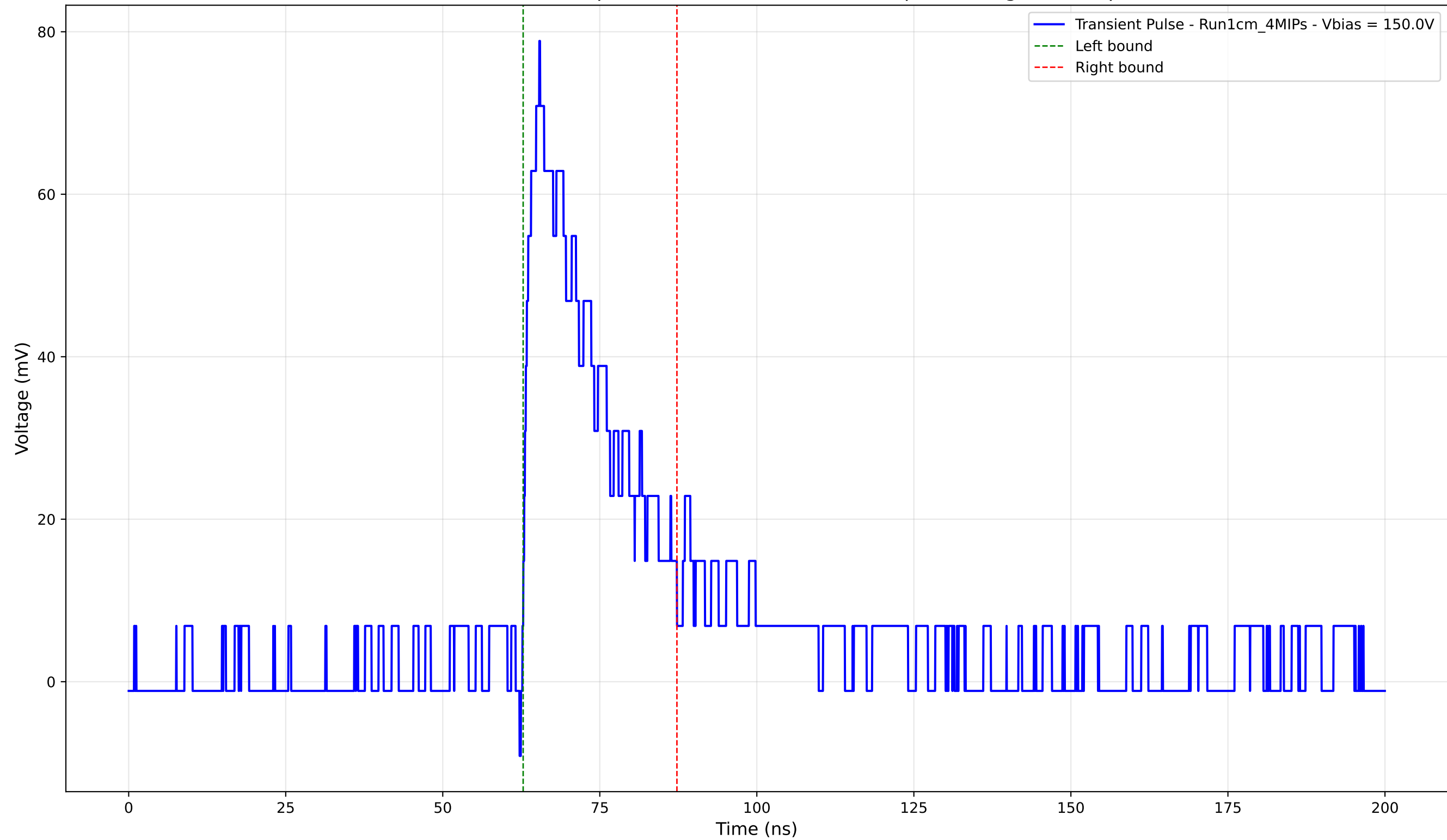
Transient Pulse - Sample: new1cm -Position: 985.0 \mu\text{m} - Charge: 18.72 pC
