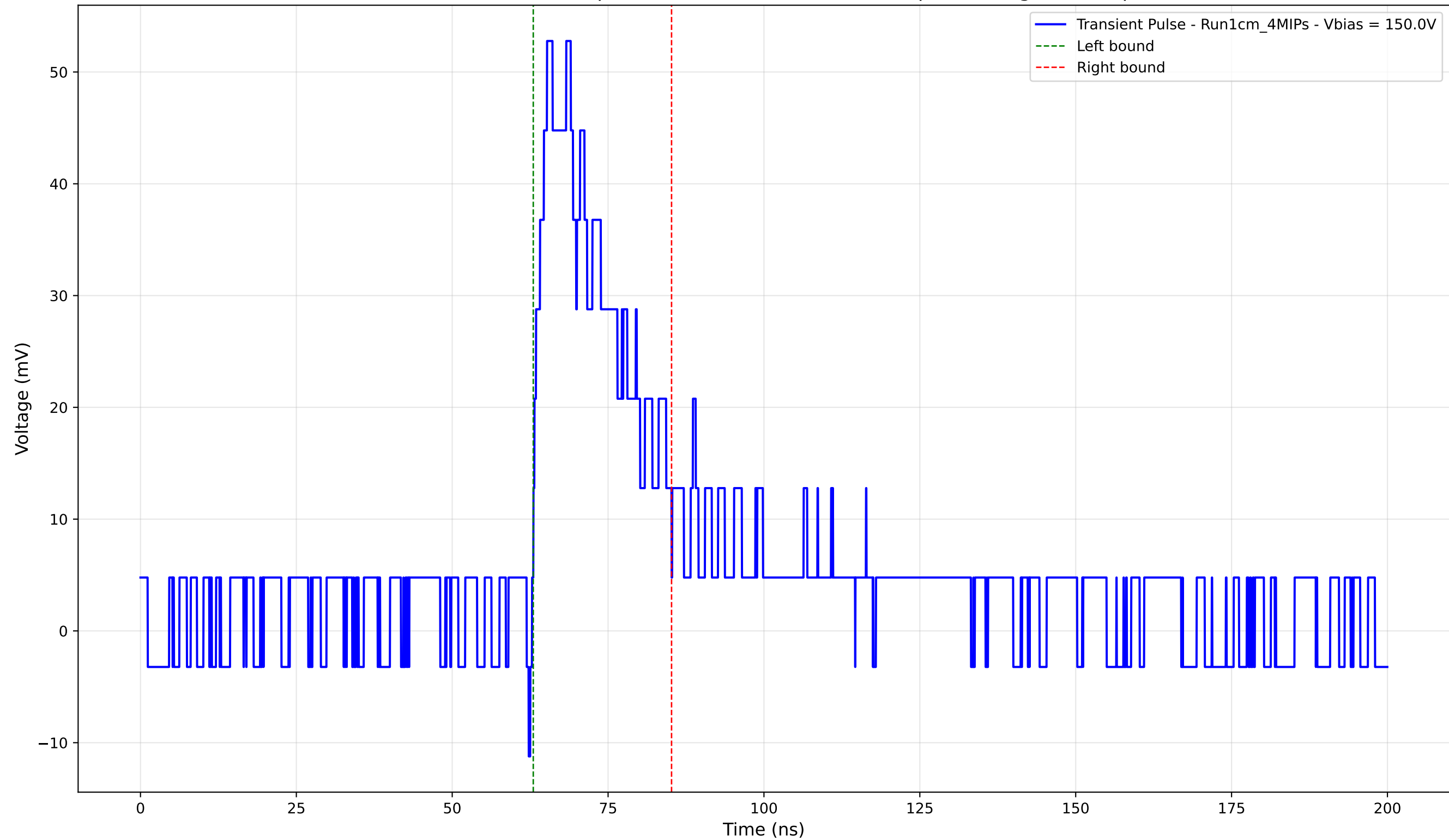
Transient Pulse - Sample: new1cm - Position: 1780.0 \mu\text{m} - Charge: 13.53 pC
