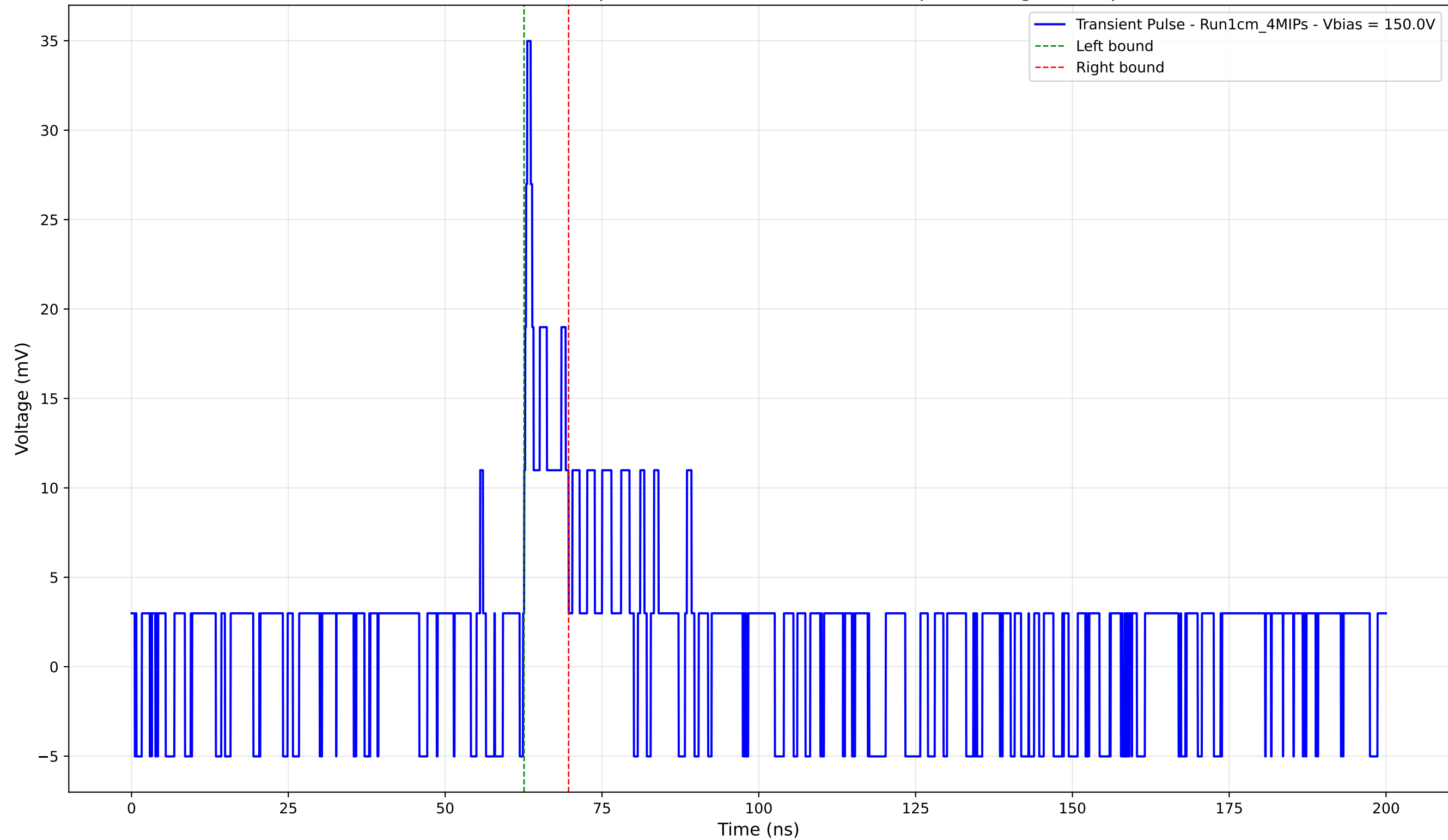
Transient Pulse - Sample: new1cm - Position: 3240.0 \mu\text{m} - Charge: 2.31 pC
