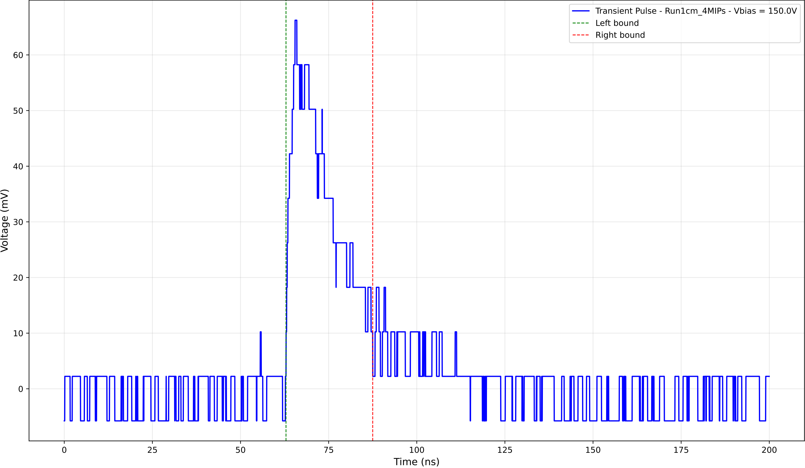
Transient Pulse - Sample: new1cm - Position: 1840.0 \mu\text{m} - Charge: 16.85 pC
