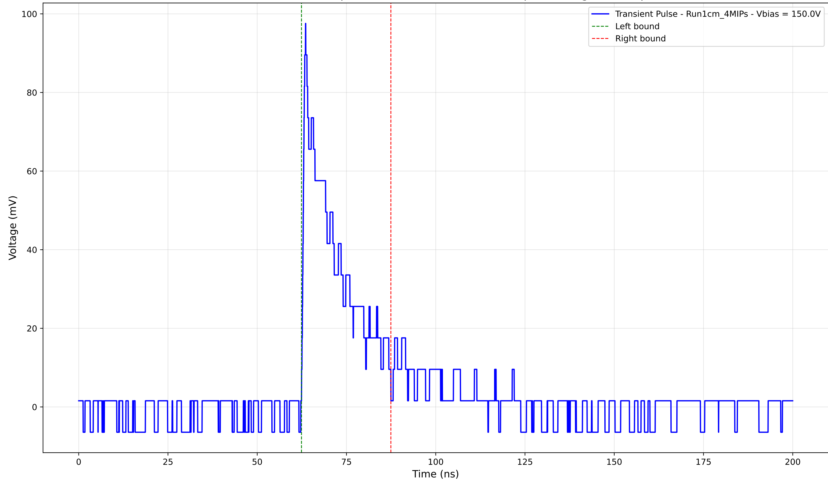
Transient Pulse - Sample: new1cm - Position: 3640.0 \mu\text{m} - Charge: 18.15 pC
