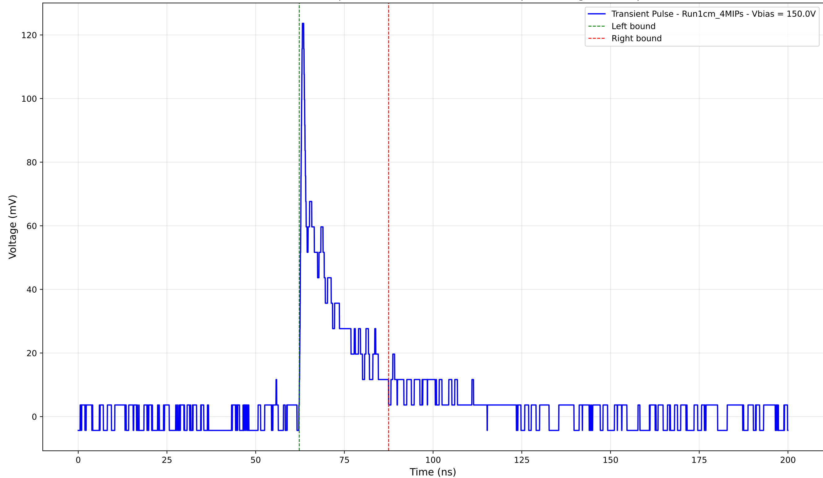
Transient Pulse - Sample: new1cm - Position: 3305.0 \mu\text{m} - Charge: 17.71 pC
