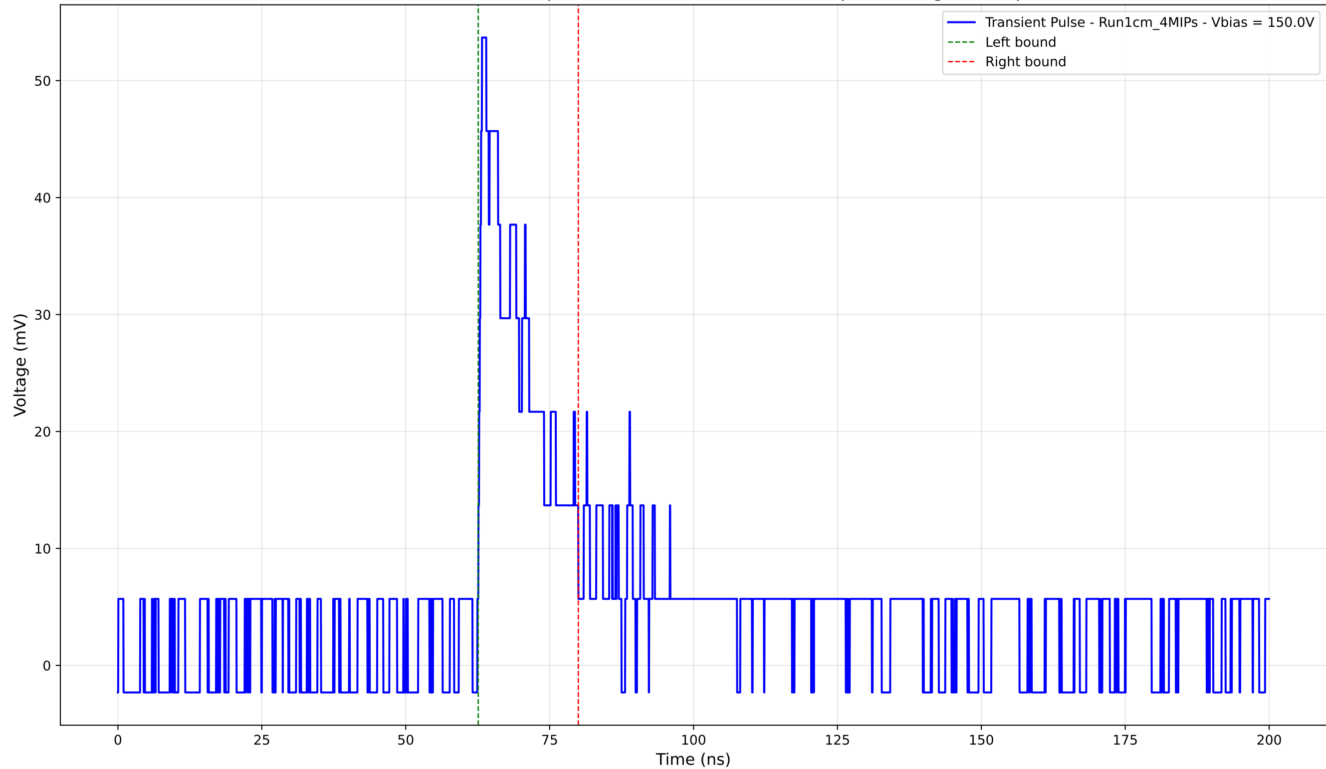
Transient Pulse - Sample: new1cm -Position: 4785.0 \mu\text{m} - Charge: 9.34 pC
