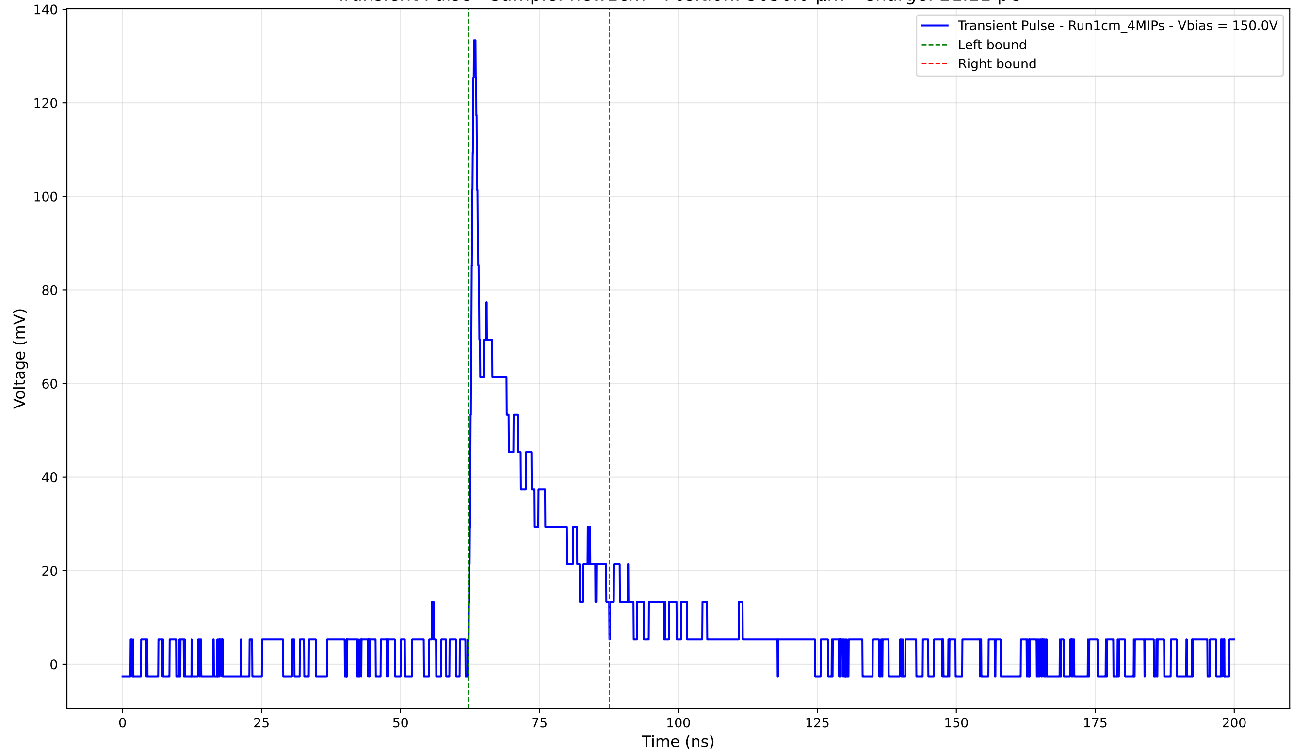
Transient Pulse - Sample: new1cm - Position: 3050.0 \mu\text{m} - Charge: 21.11 pC
