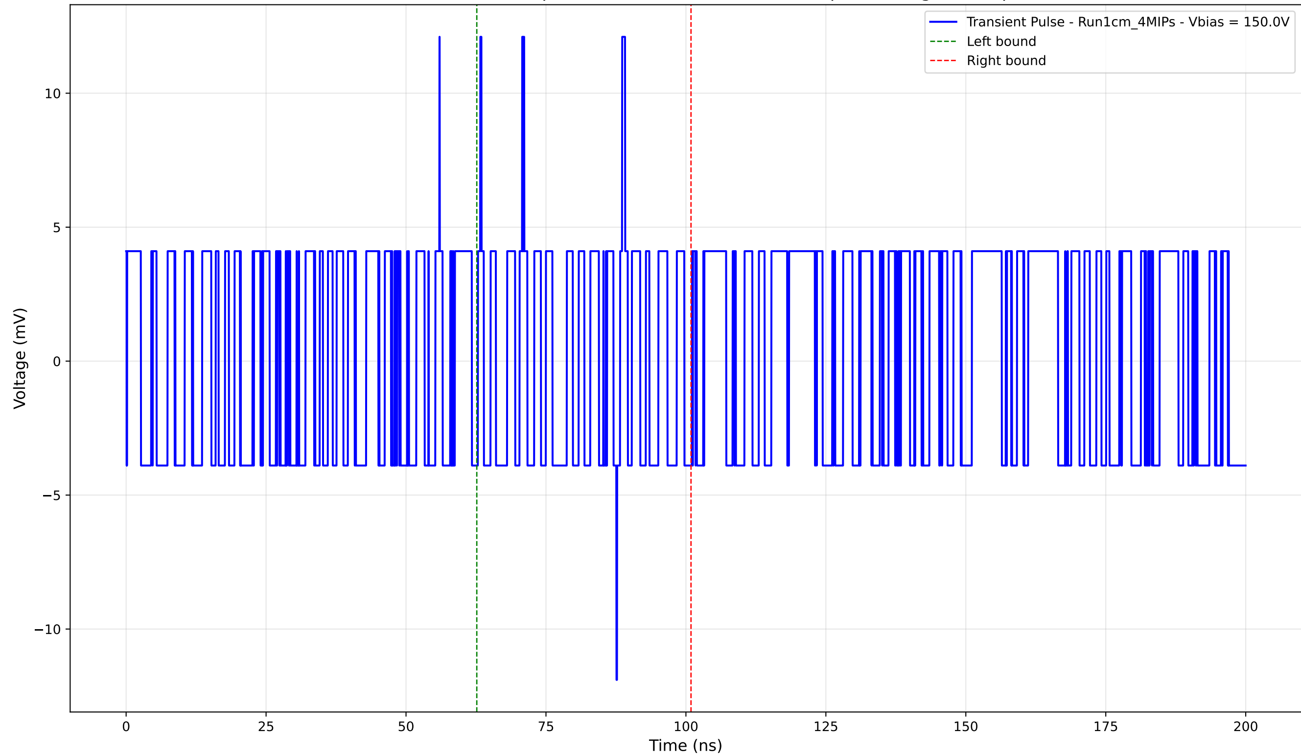
Transient Pulse - Sample: new1cm - Position: 5075.0 \mu\text{m} - Charge: 0.15 pC
