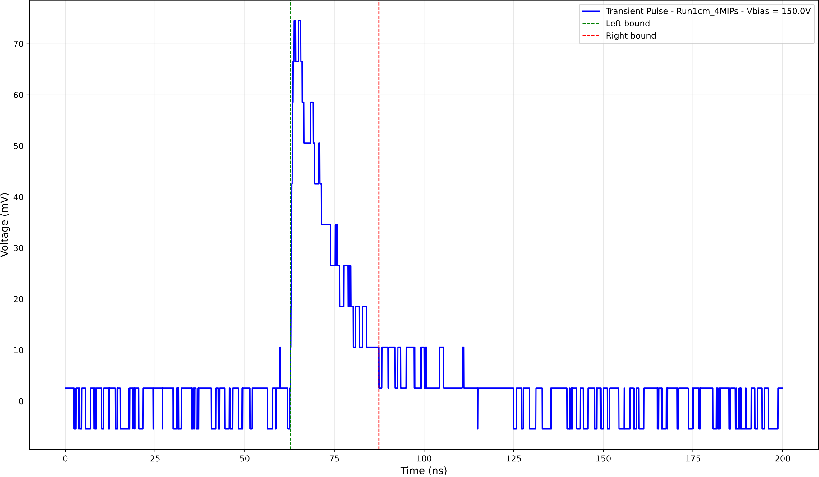
Transient Pulse - Sample: new1cm - Position: 4155.0 \mu\text{m} - Charge: 16.20 pC
