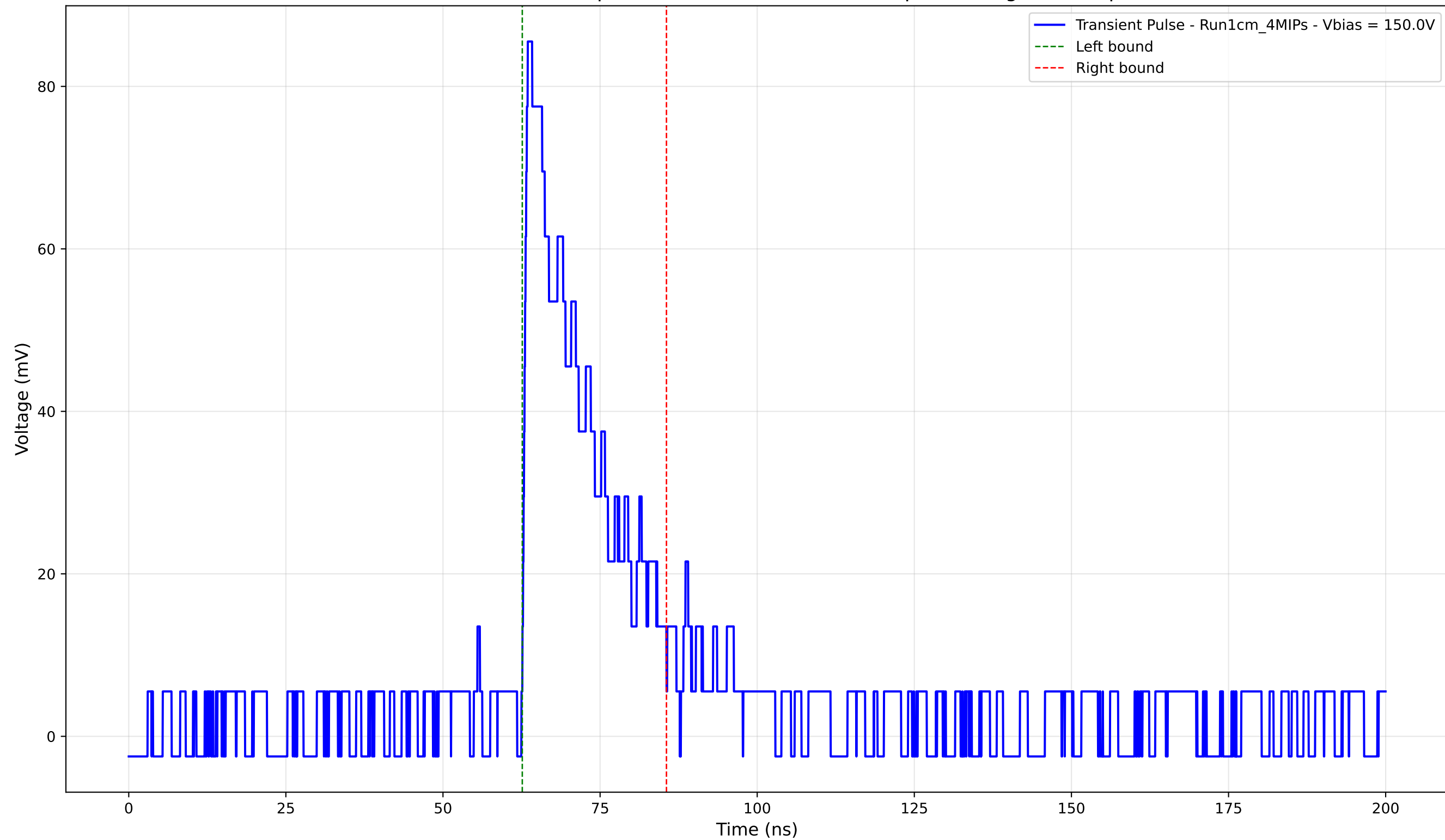
Transient Pulse - Sample: new1cm -Position: 515.0 \mu\text{m} - Charge: 18.10 pC
