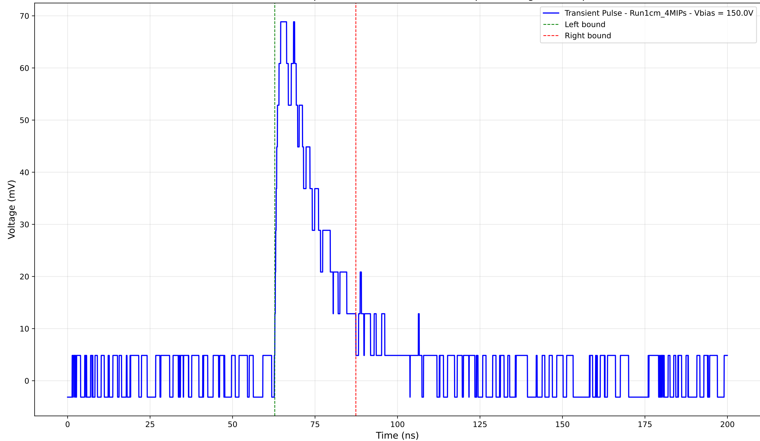
Transient Pulse - Sample: new1cm -Position: 965.0 \mu\text{m} - Charge: 17.83 pC
