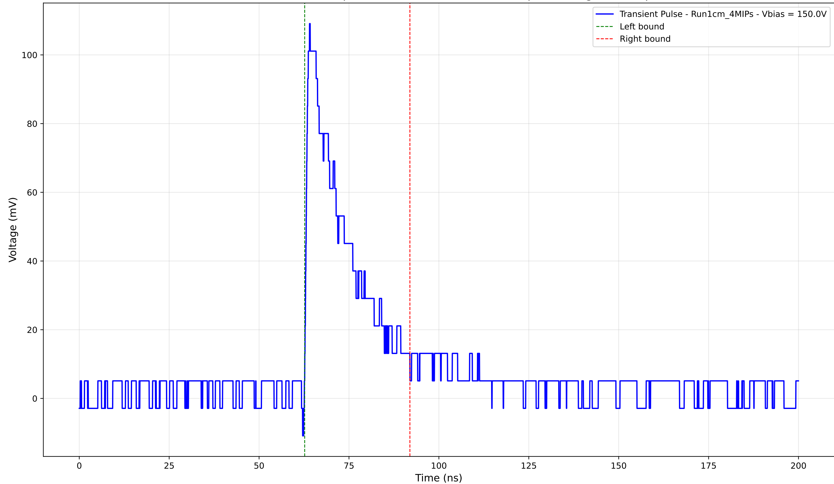
Transient Pulse - Sample: new1cm - Position: 4080.0 \mu\text{m} - Charge: 25.61 pC
