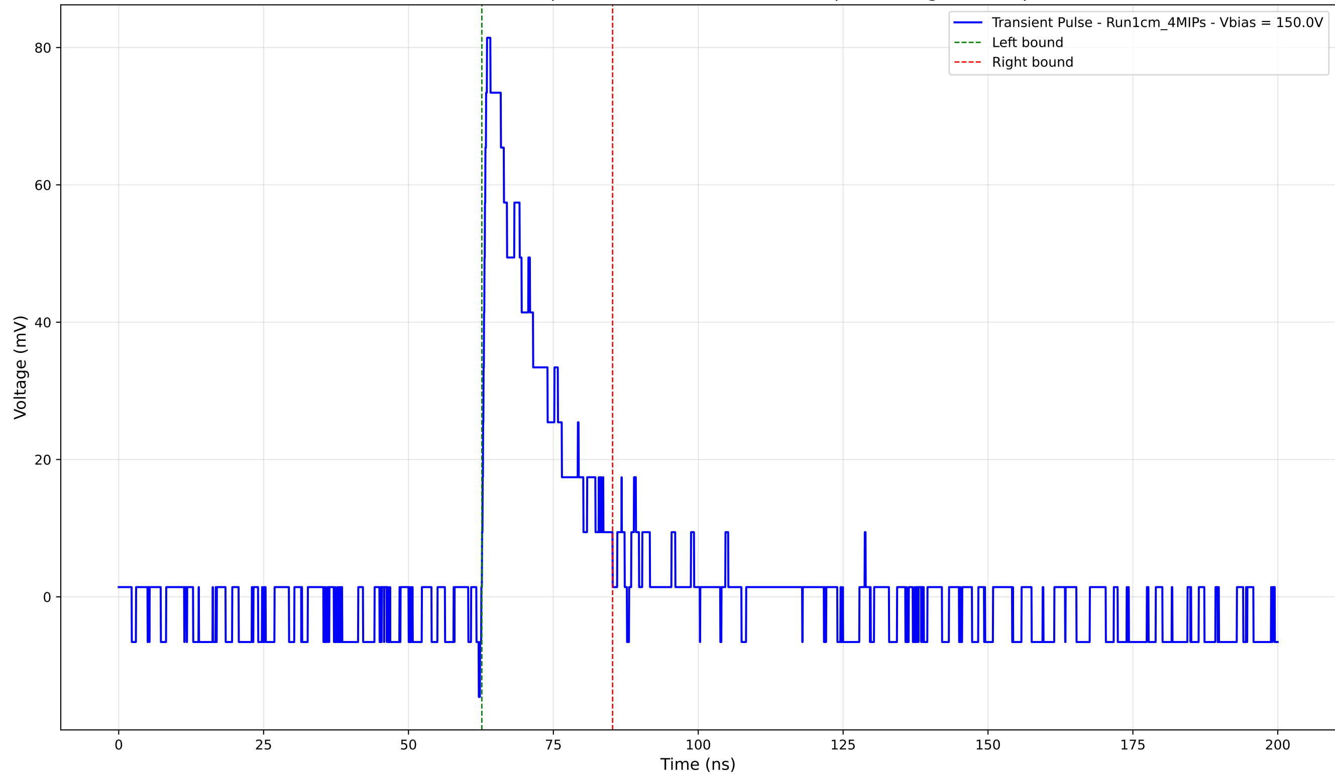
Transient Pulse - Sample: new1cm -Position: 535.0 \mu\text{m} - Charge: 15.59 pC
