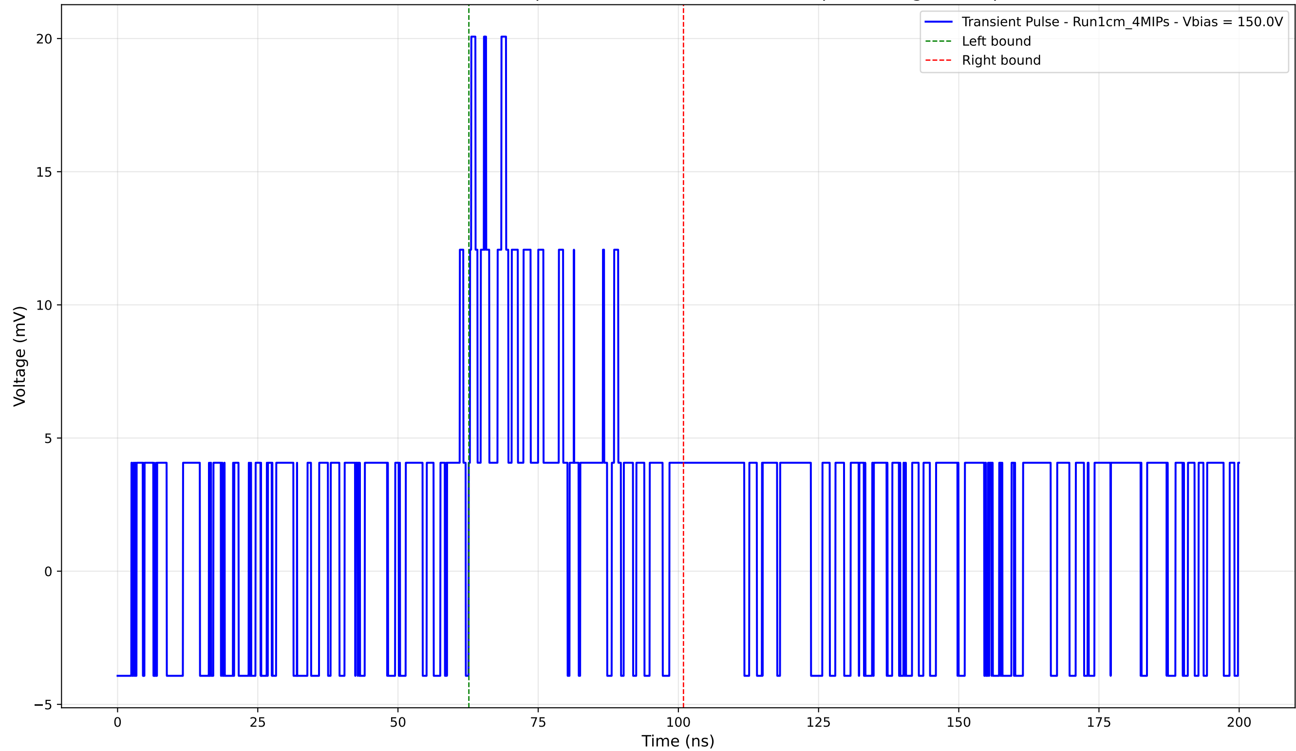
Transient Pulse - Sample: new1cm - Position: 2725.0 \mu\text{m} - Charge: 4.25 pC
