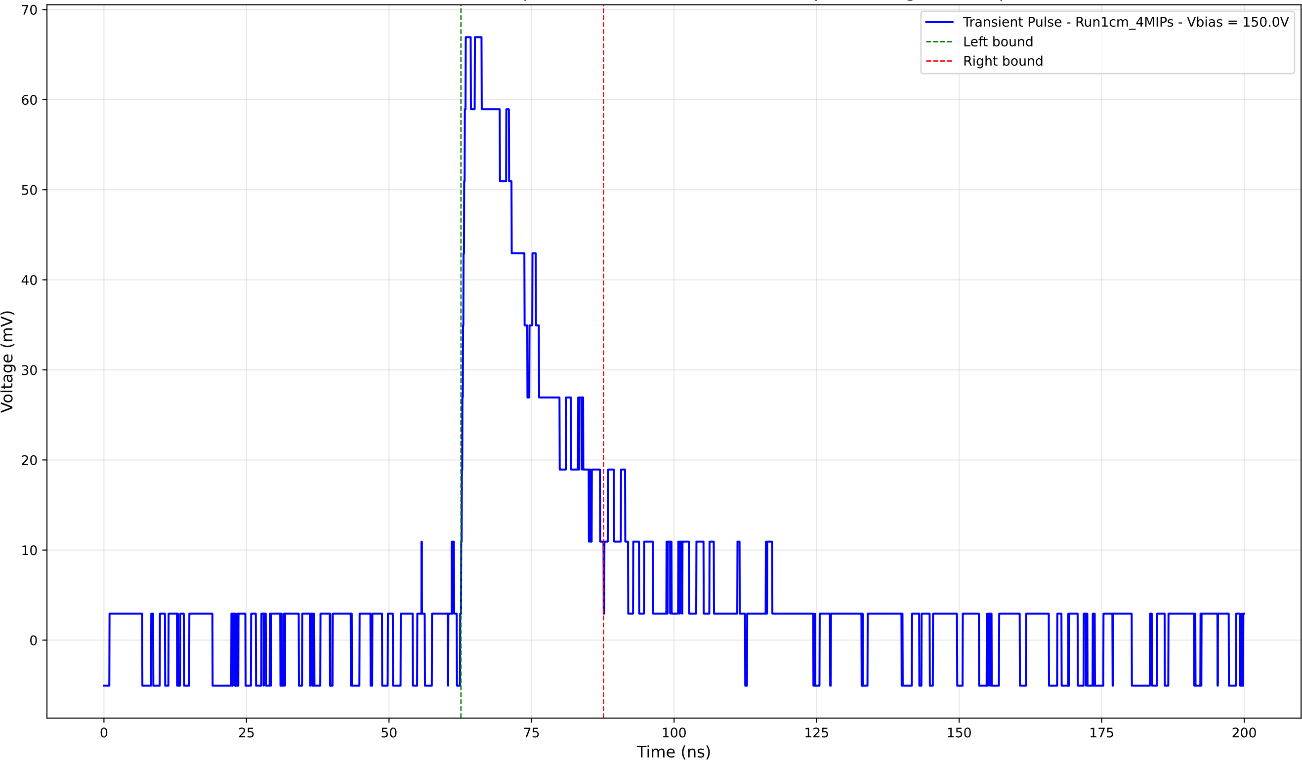
Transient Pulse - Sample: new1cm - Position: 2490.0 \mu\text{m} - Charge: 18.91 pC
