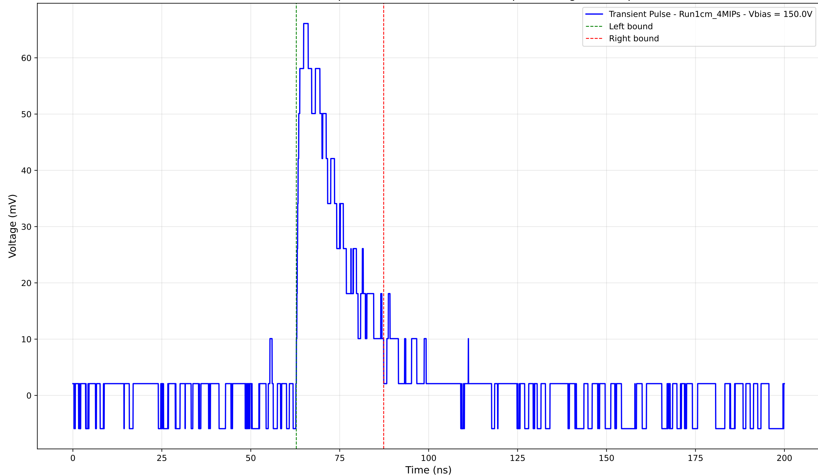
Transient Pulse - Sample: new1cm -Position: 915.0 \mu\text{m} - Charge: 16.21 pC
