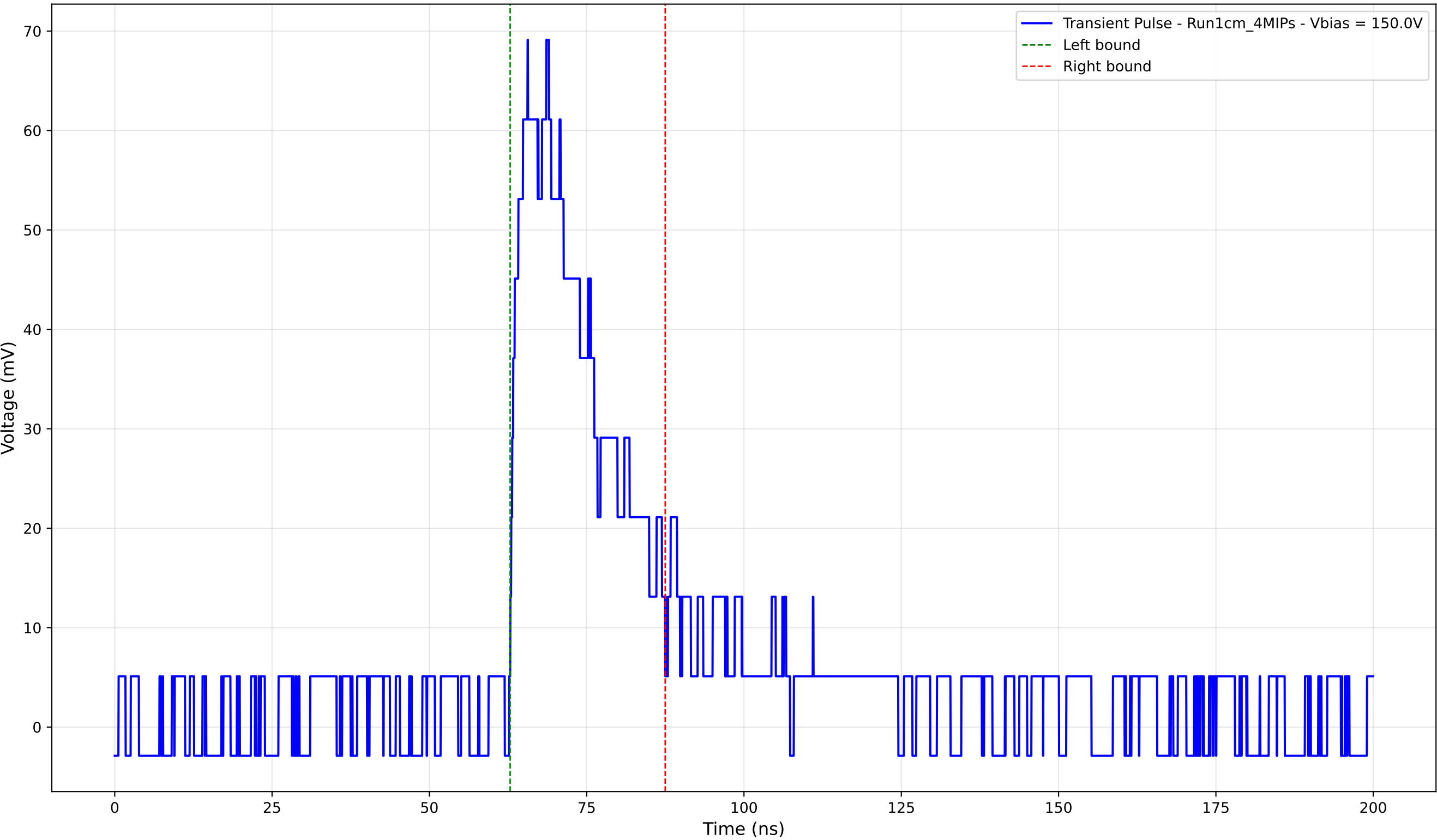
Transient Pulse - Sample: new1cm - Position: 2020.0 \mu\text{m} - Charge: 18.49 pC
