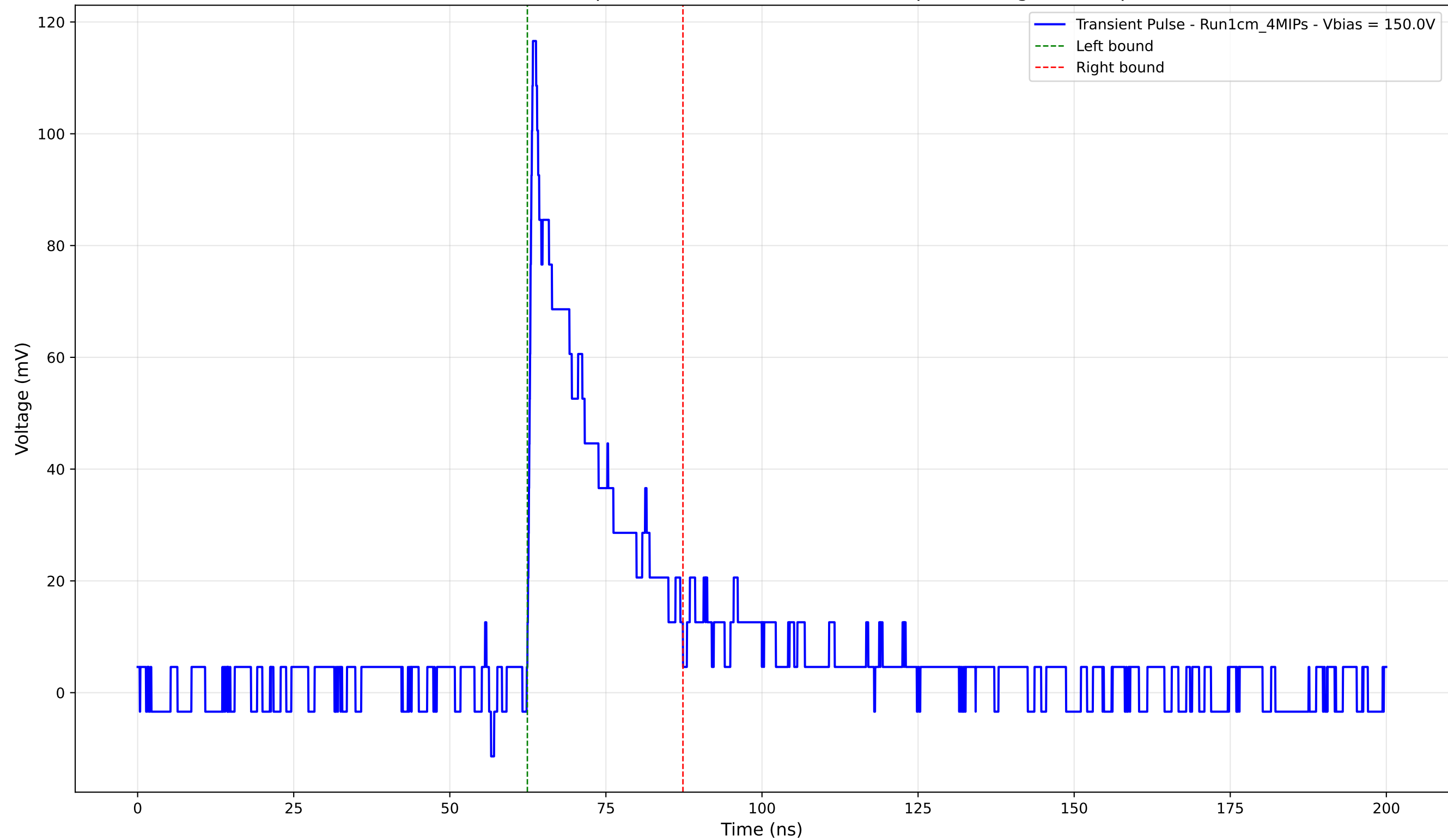
Transient Pulse - Sample: new1cm - Position: 3565.0 \mu\text{m} - Charge: 22.09 pC
