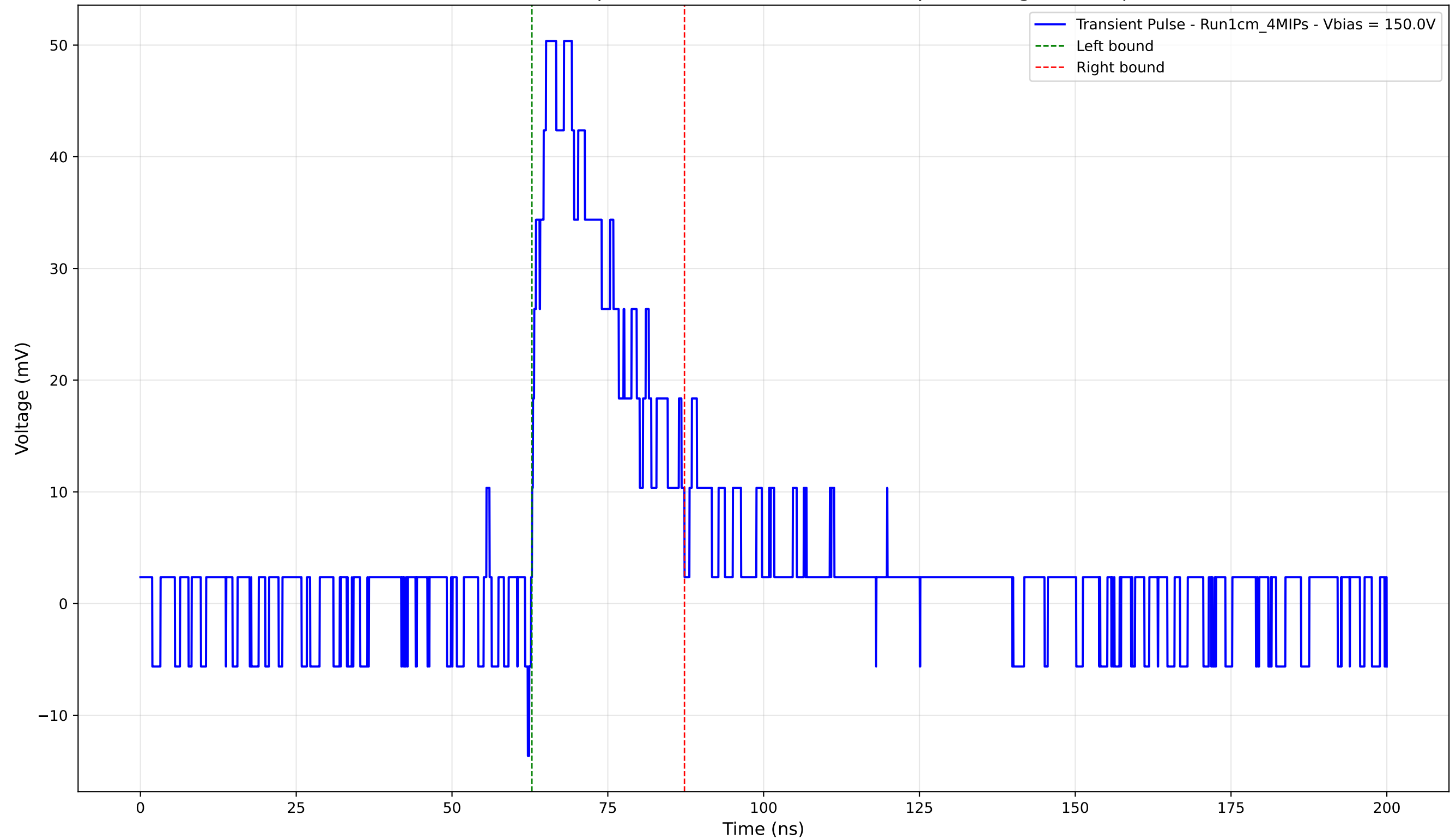
Transient Pulse - Sample: new1cm - Position: 1785.0 \mu\text{m} - Charge: 13.98 pC
