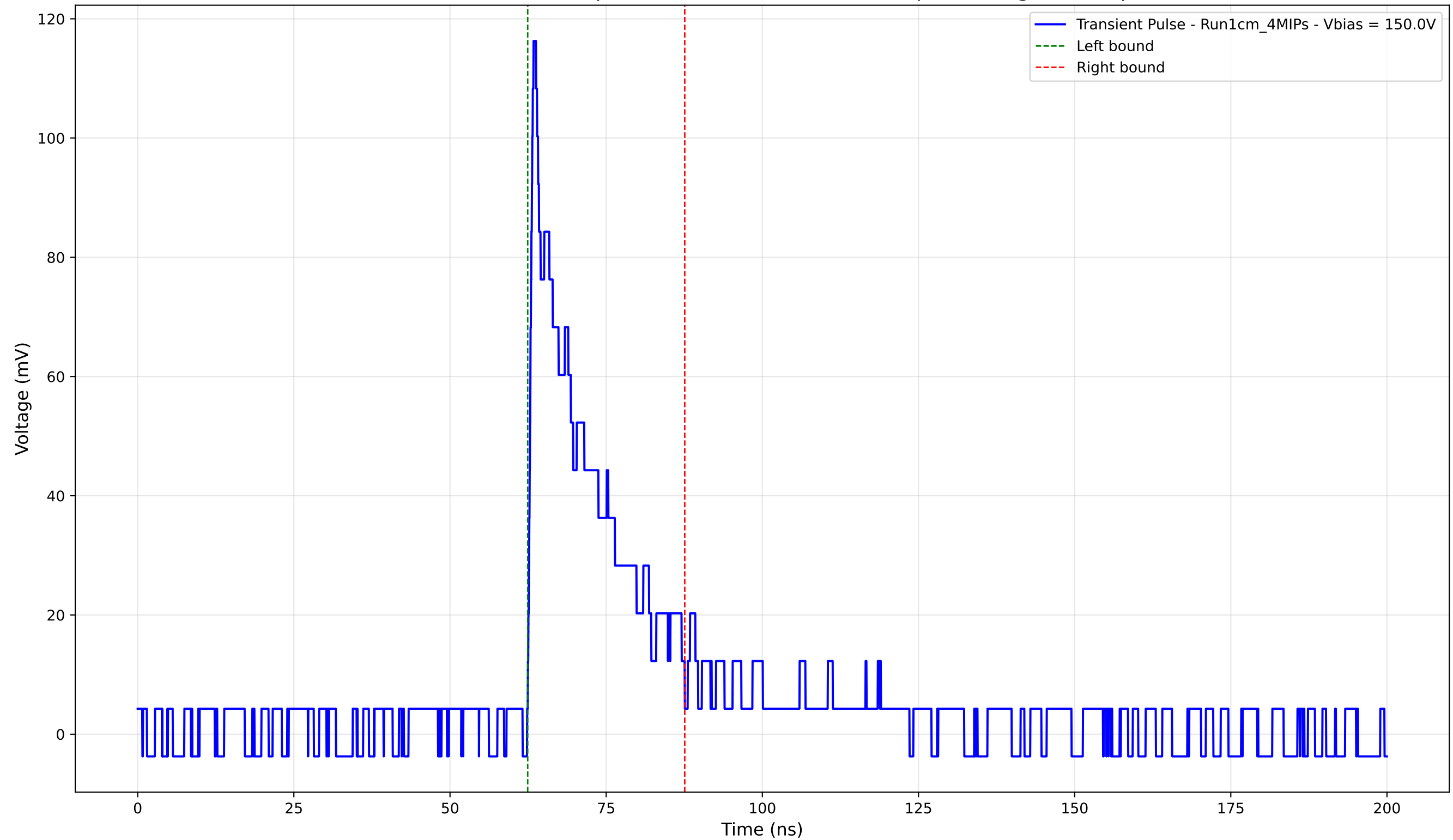
Transient Pulse - Sample: new1cm - Position: 3585.0 \mu\text{m} - Charge: 21.44 pC
