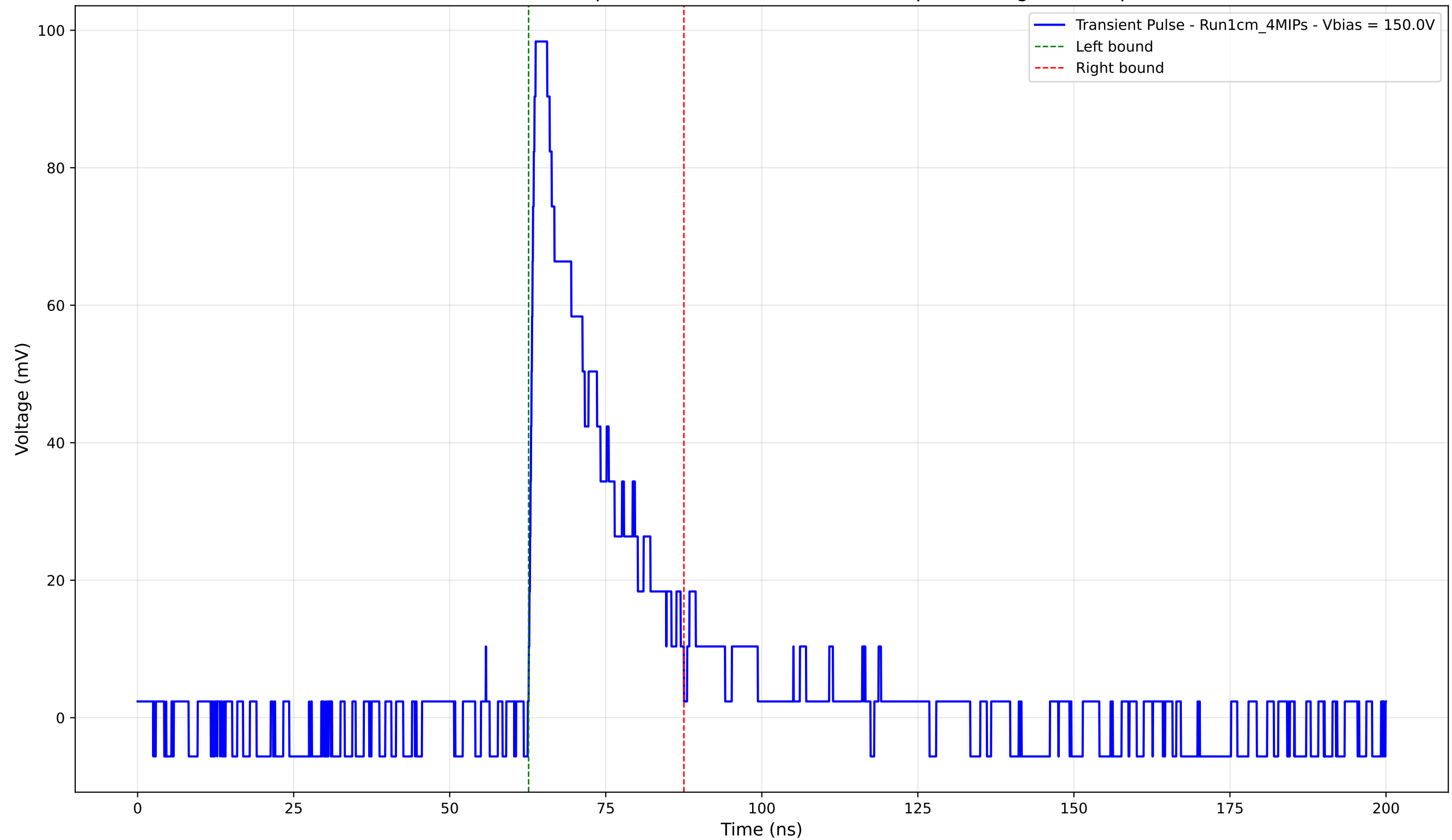
Transient Pulse - Sample: new1cm - Position: 4335.0 \mu\text{m} - Charge: 21.50 pC
