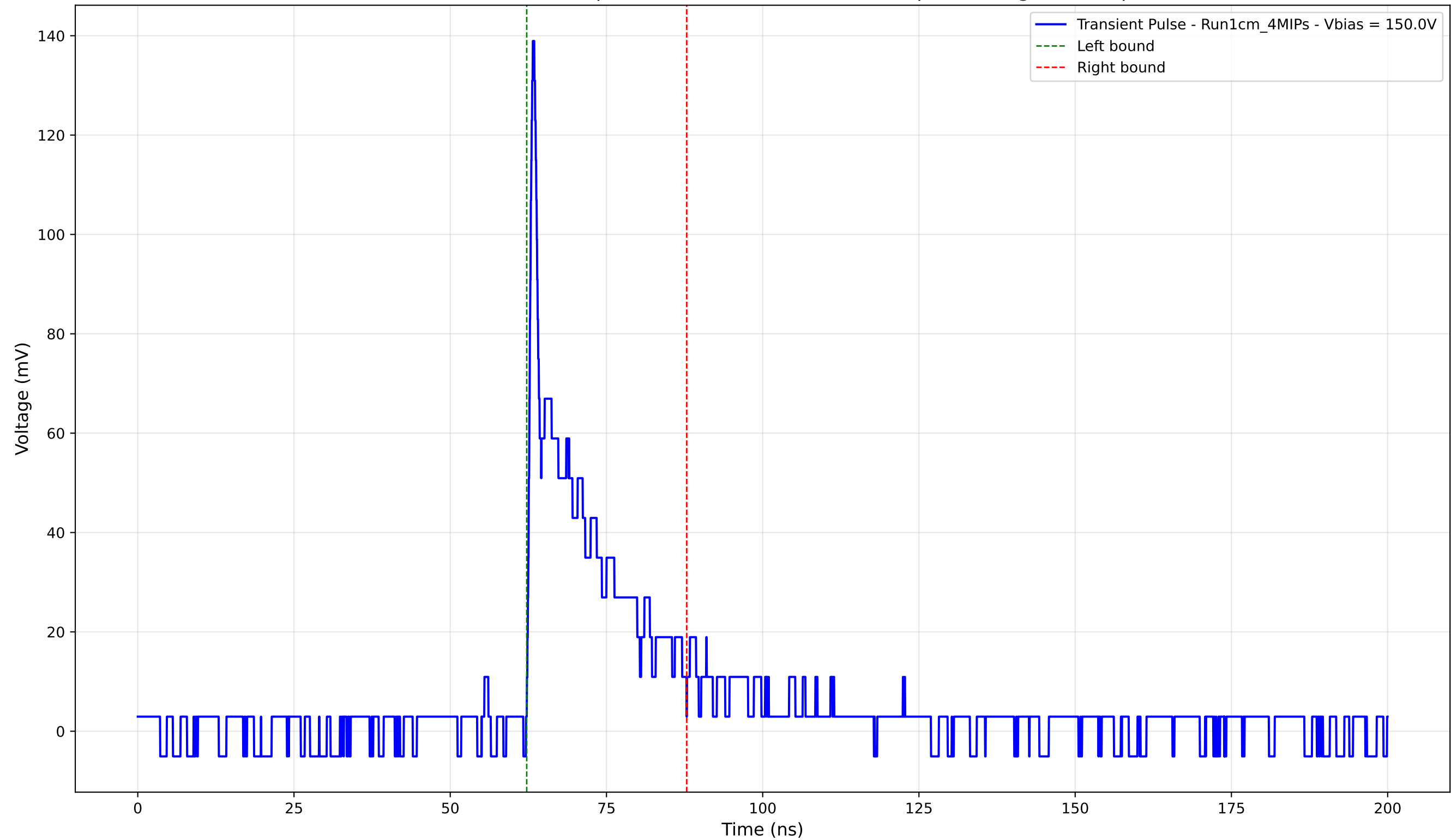
Transient Pulse - Sample: new1cm - Position: 3120.0 \mu\text{m} - Charge: 19.79 pC
