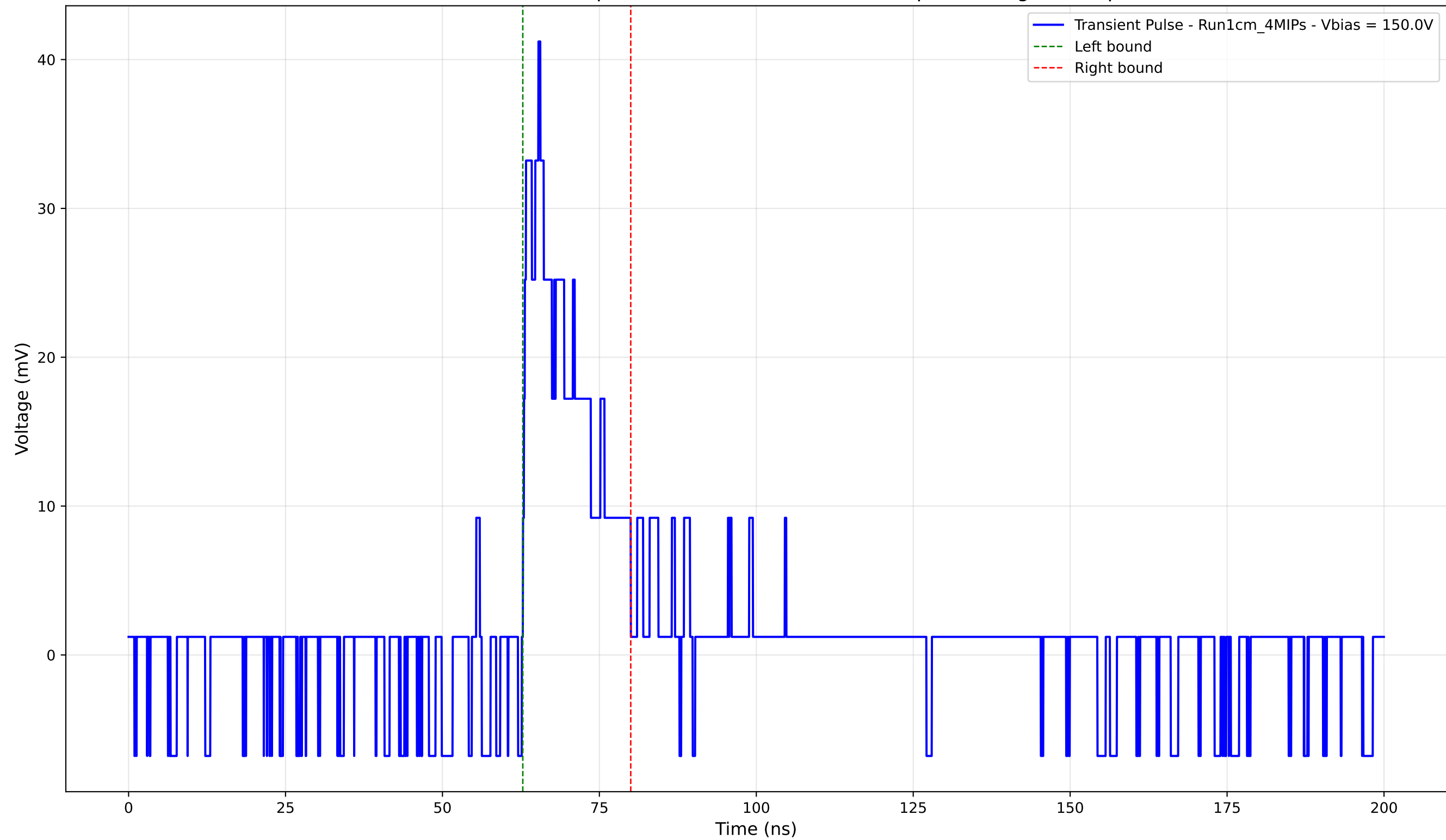
Transient Pulse - Sample: new1cm -Position: 4185.0 \mu\text{m} - Charge: 6.36 pC
