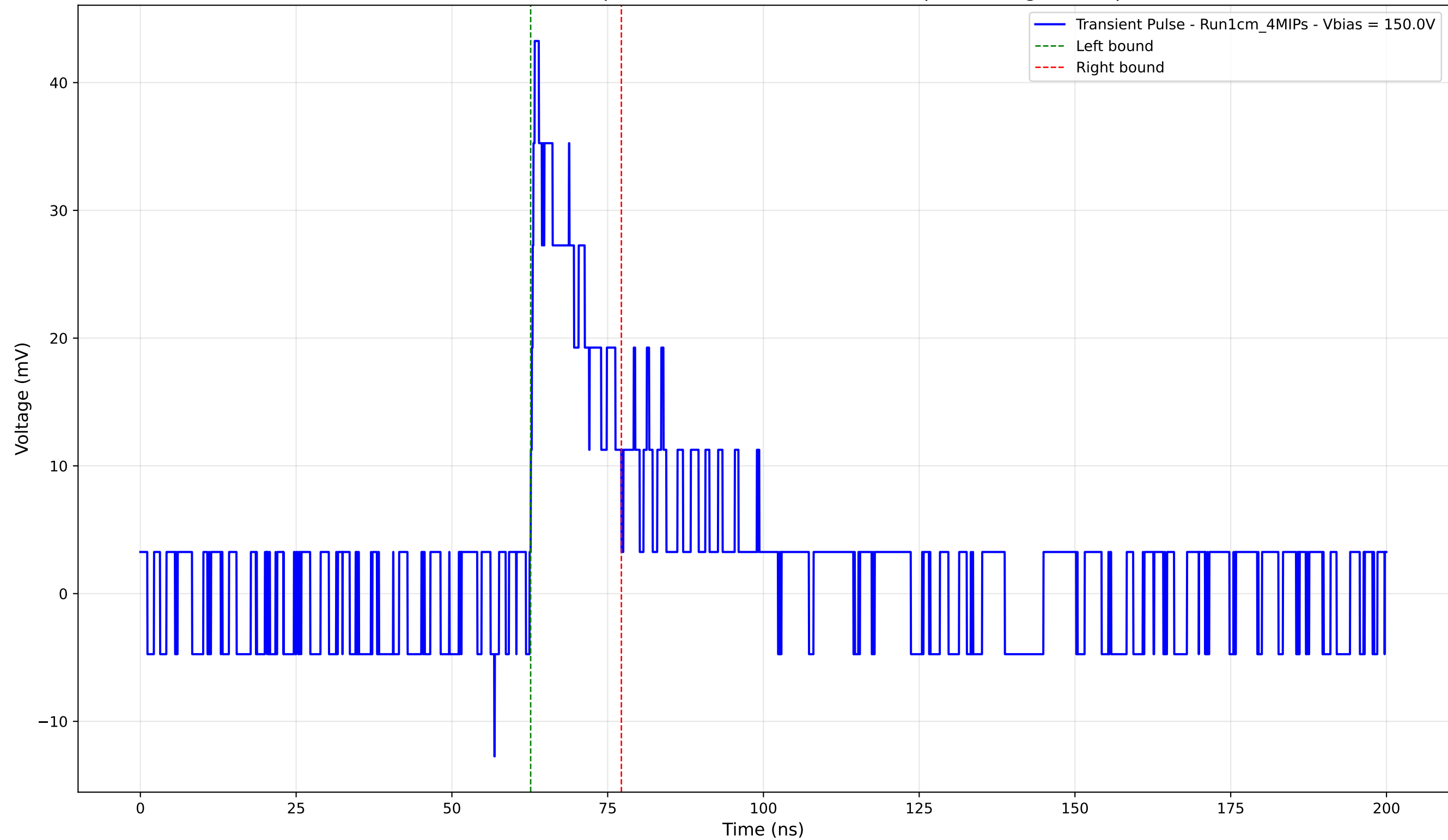
Transient Pulse - Sample: new1cm - Position: 3760.0 \mu\text{m} - Charge: 7.06 pC
