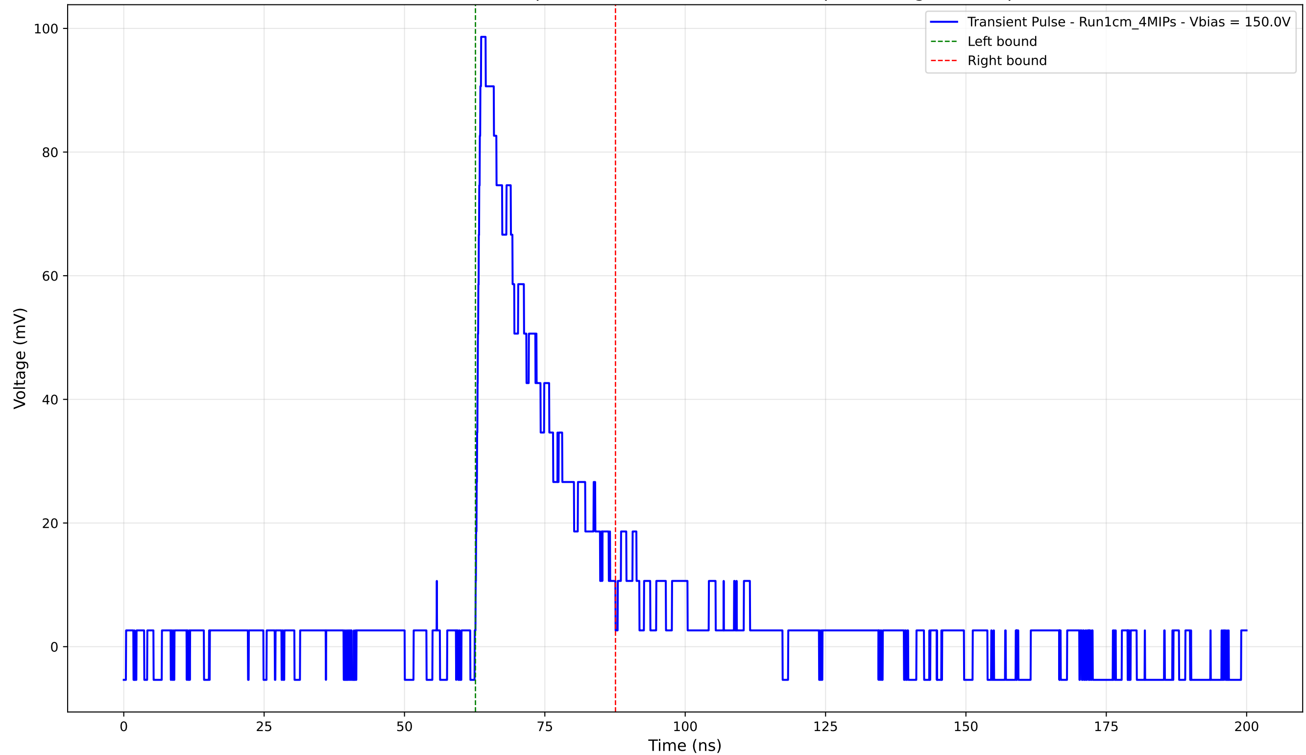
Transient Pulse - Sample: new1cm - Position: 4010.0 \mu\text{m} - Charge: 21.82 pC
