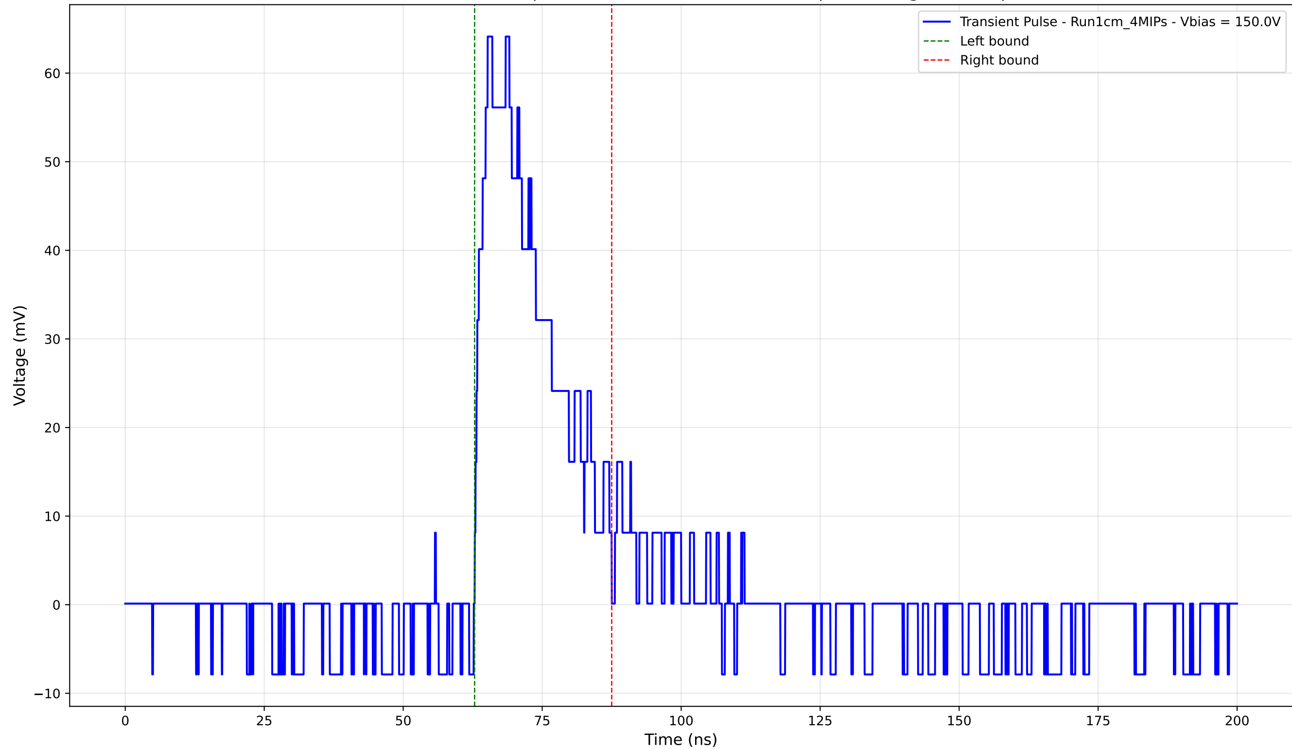
Transient Pulse - Sample: new1cm - Position: 1950.0 \mu\text{m} - Charge: 16.56 pC
