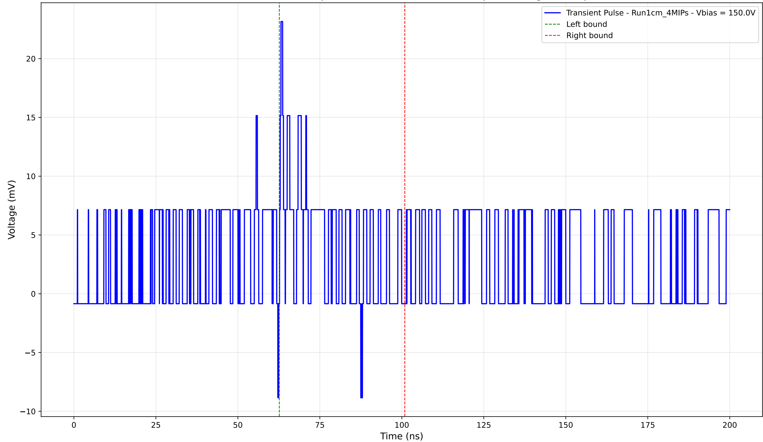
Transient Pulse - Sample: new1cm - Position: 195.0 \mu\text{m} - Charge: 3.35 pC
