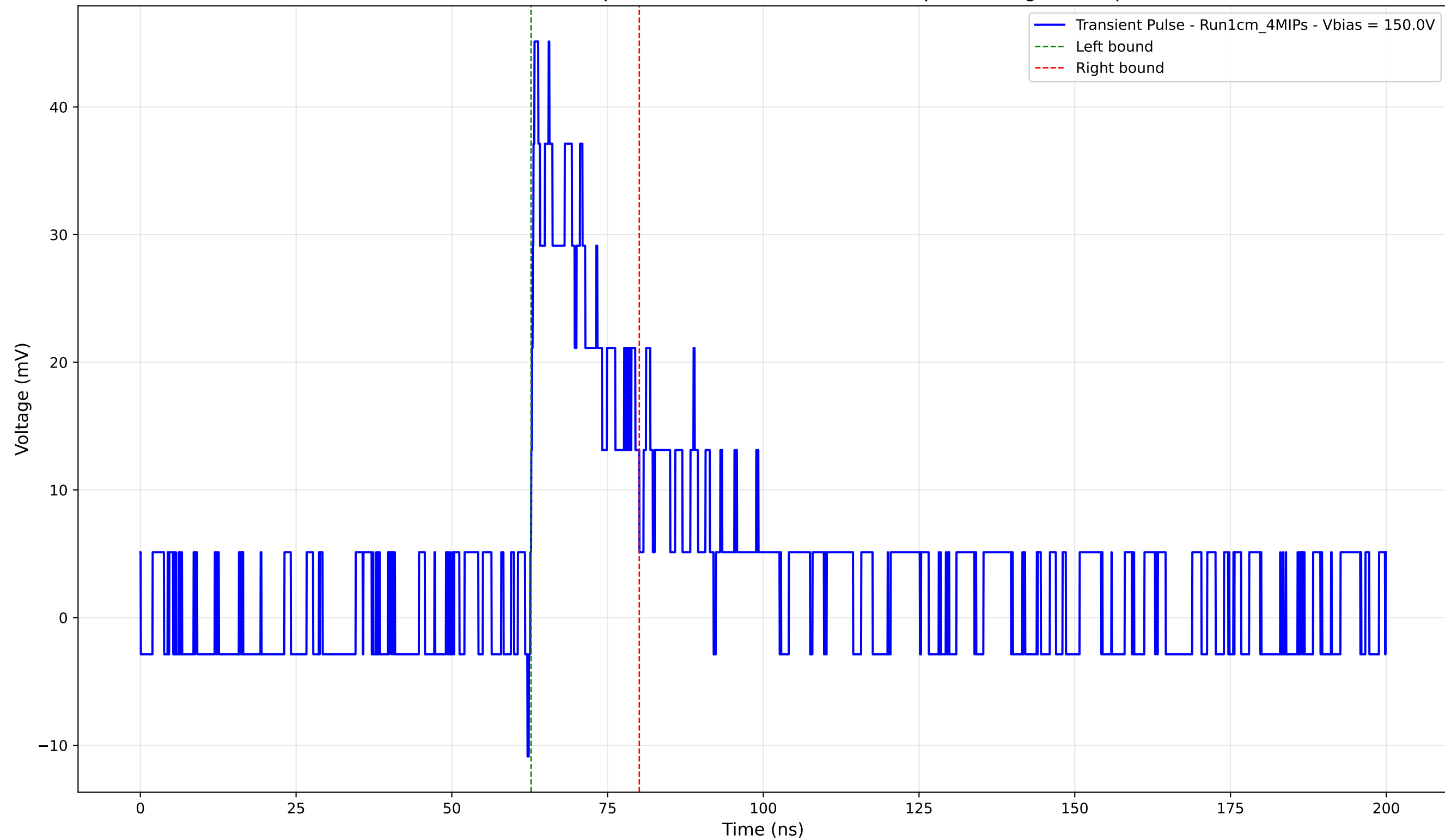
Transient Pulse - Sample: new1cm - Position: 2655.0 \mu\text{m} - Charge: 8.86 pC
