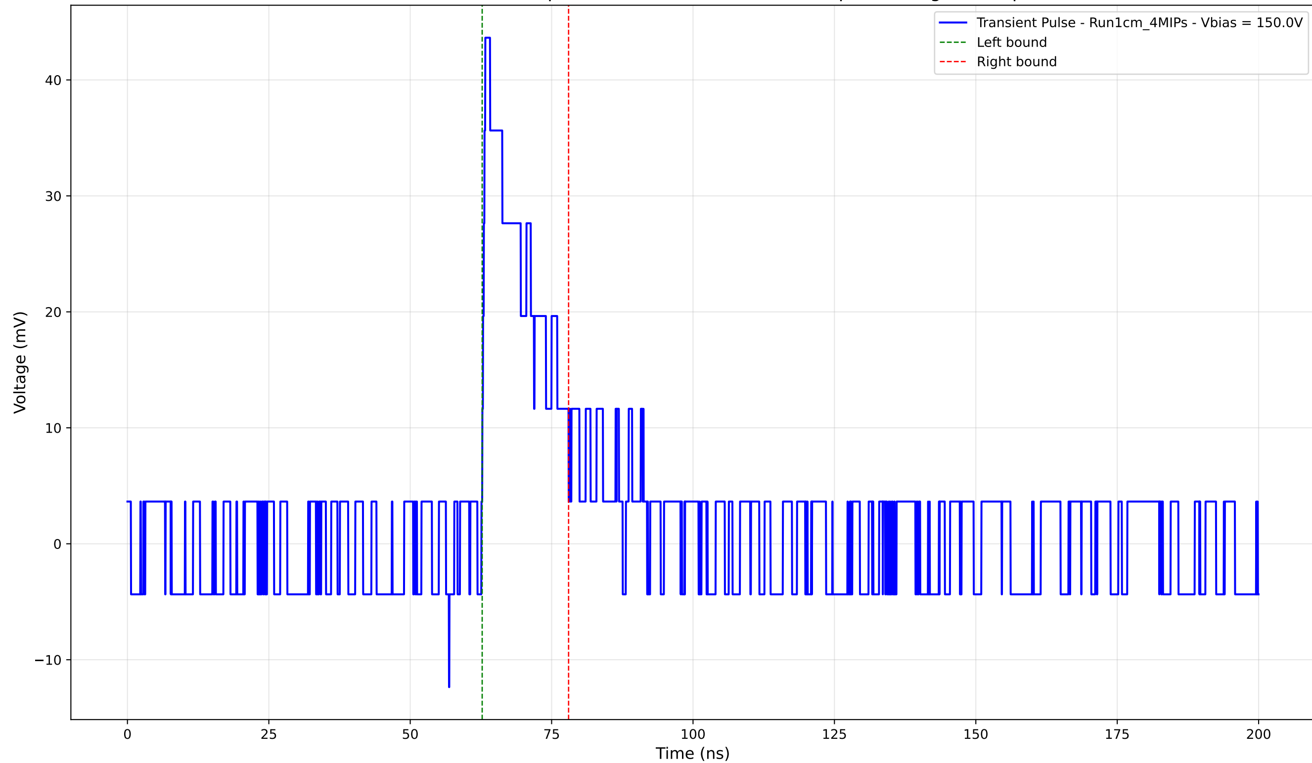
Transient Pulse - Sample: new1cm - Position: 4685.0 \mu\text{m} - Charge: 7.30 pC
