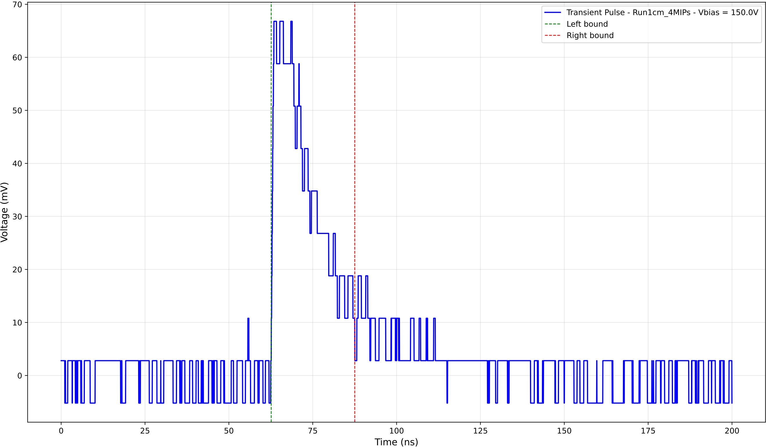
Transient Pulse - Sample: new1cm - Position: 2510.0 \mu\text{m} - Charge: 18.07 pC
