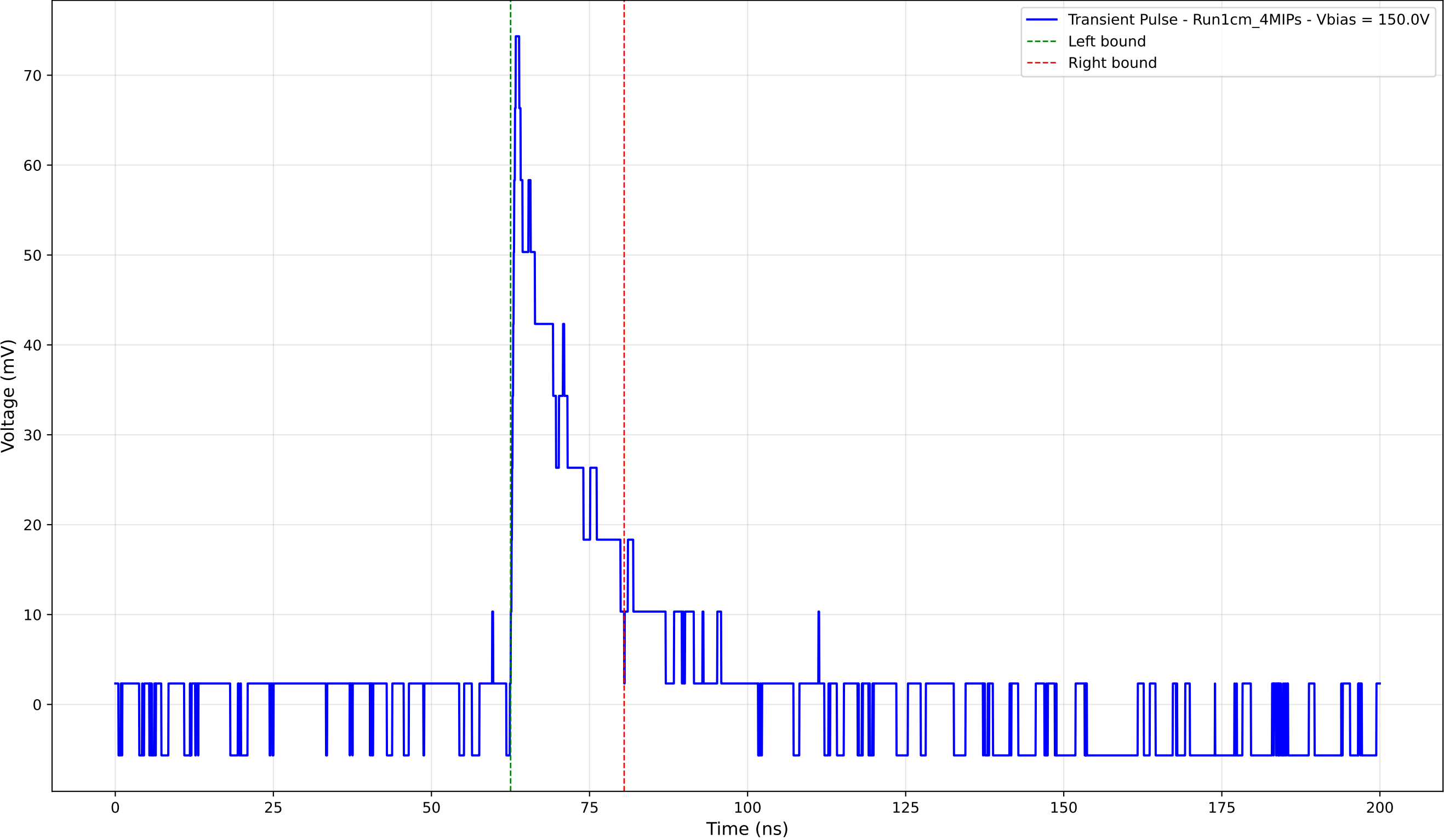
Transient Pulse - Sample: new1cm - Position: 3655.0 \mu\text{m} - Charge: 11.84 pC
