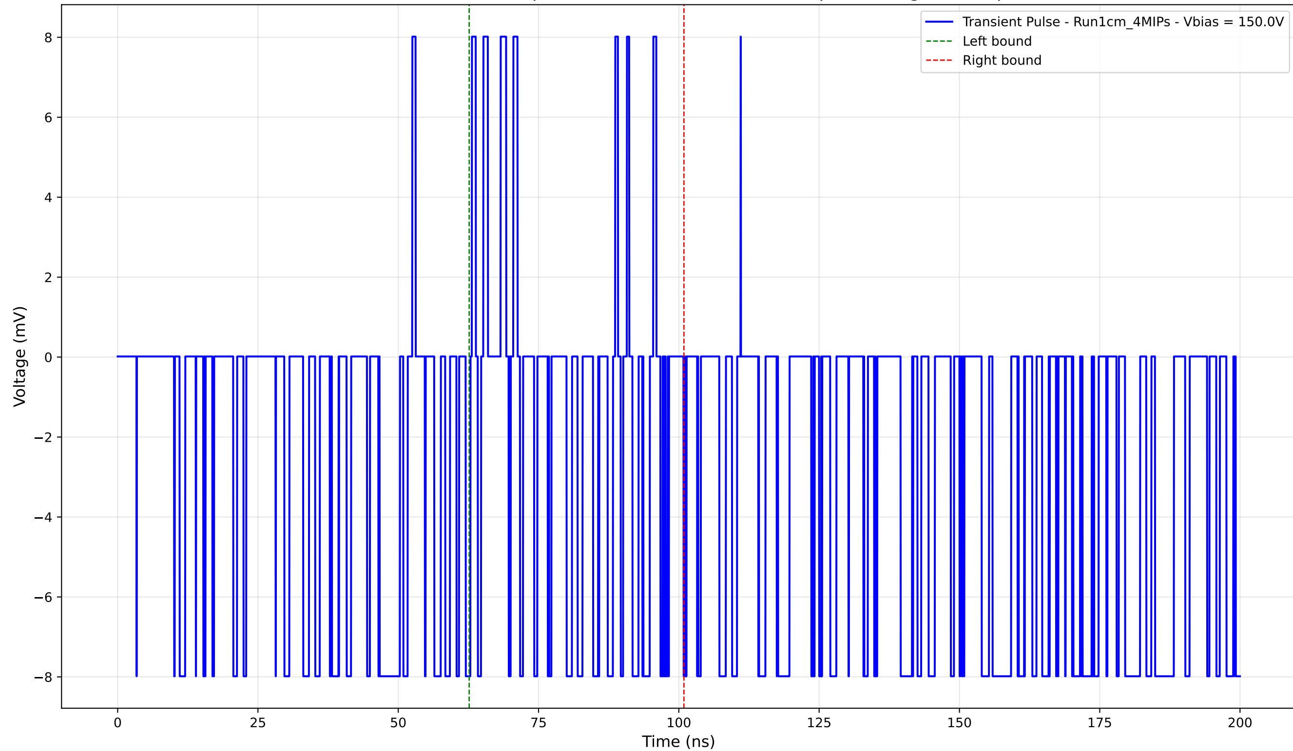
Transient Pulse - Sample: new1cm - Position: 1700.0 \mu\text{m} - Charge: -0.89 pC
