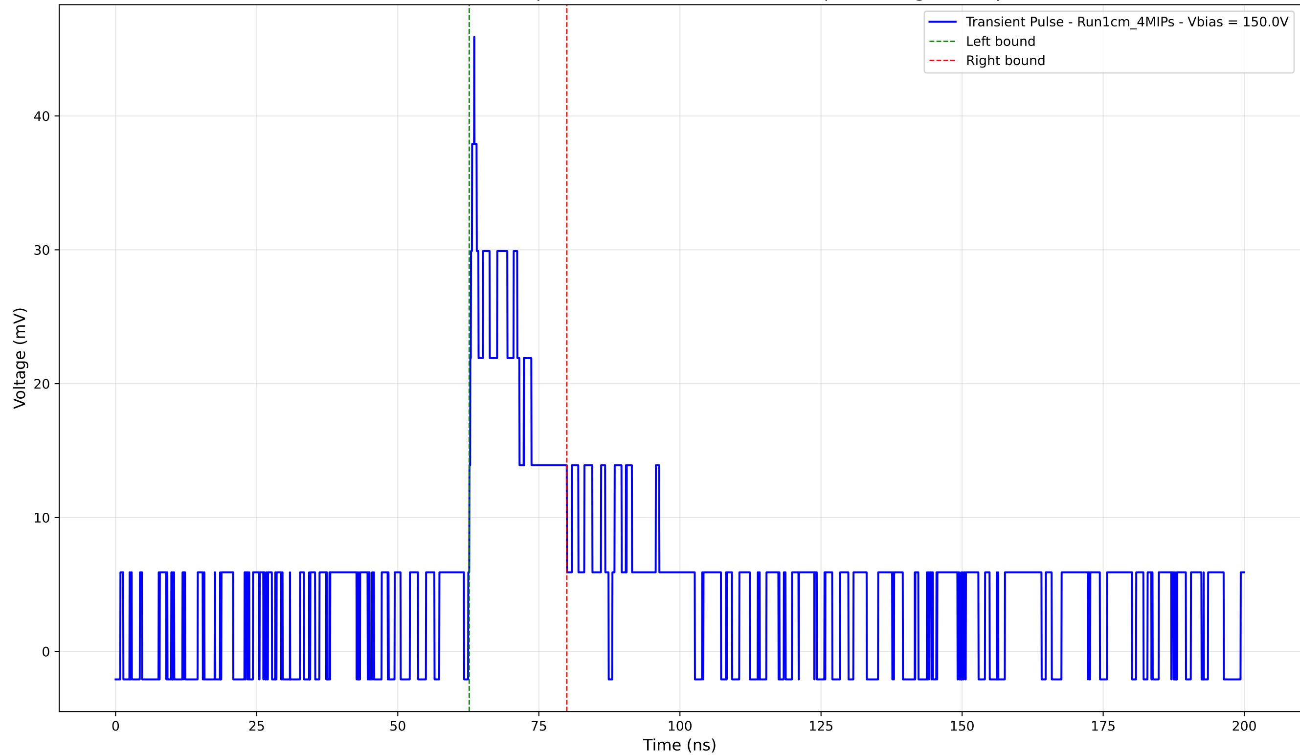
Transient Pulse - Sample: new1cm -Position: 2750.0 \mu\text{m} - Charge: 7.36 pC
