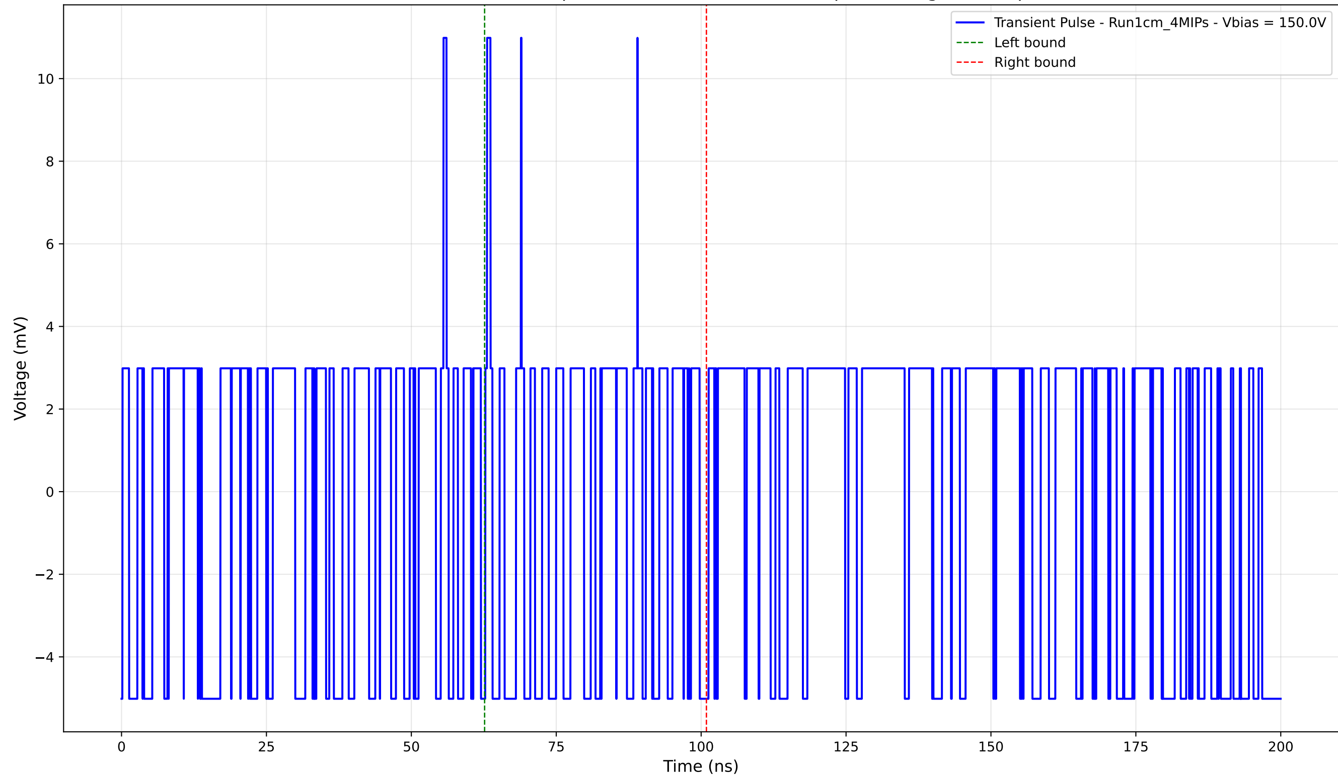
Transient Pulse - Sample: new1cm - Position: 10.0 \mu\text{m} - Charge: -0.11 pC
