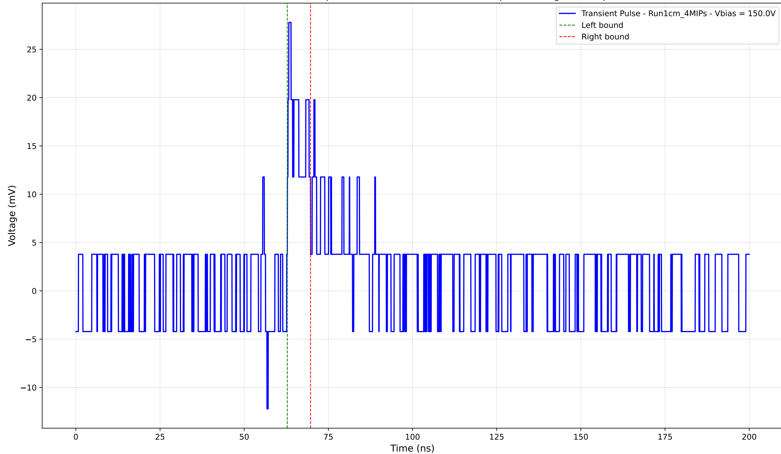
Transient Pulse - Sample: new1cm - Position: 4705.0 \mu\text{m} - Charge: 2.36 pC
