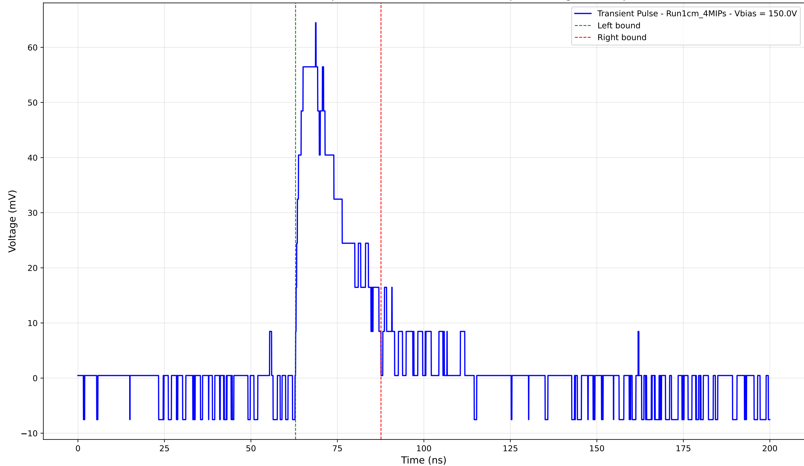
Transient Pulse - Sample: new1cm - Position: 1855.0 \mu\text{m} - Charge: 16.41 pC
