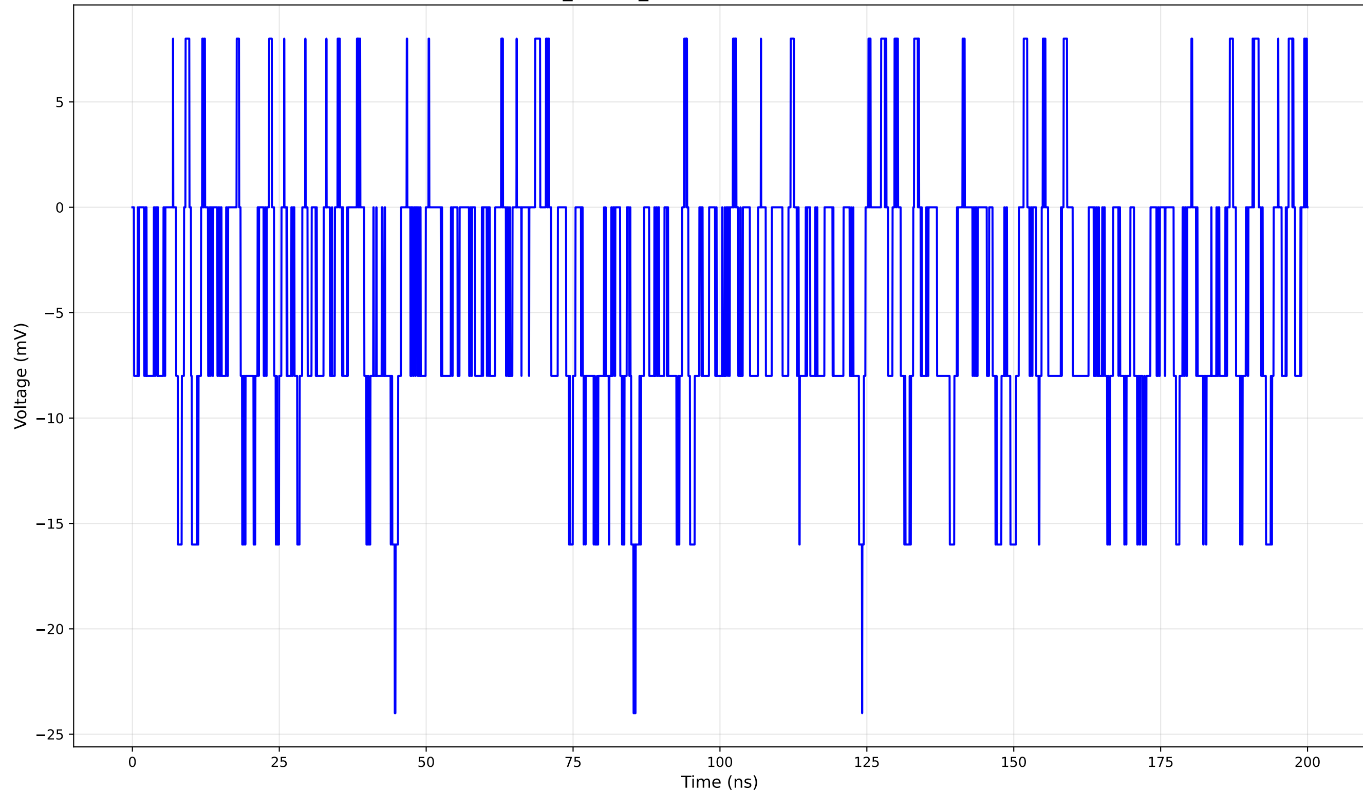
TCT Pulse Waveform - Run 2_0: 1cm_42-Position2 (Unknown V) - Rise Time: 0.00 ns (N/A)
