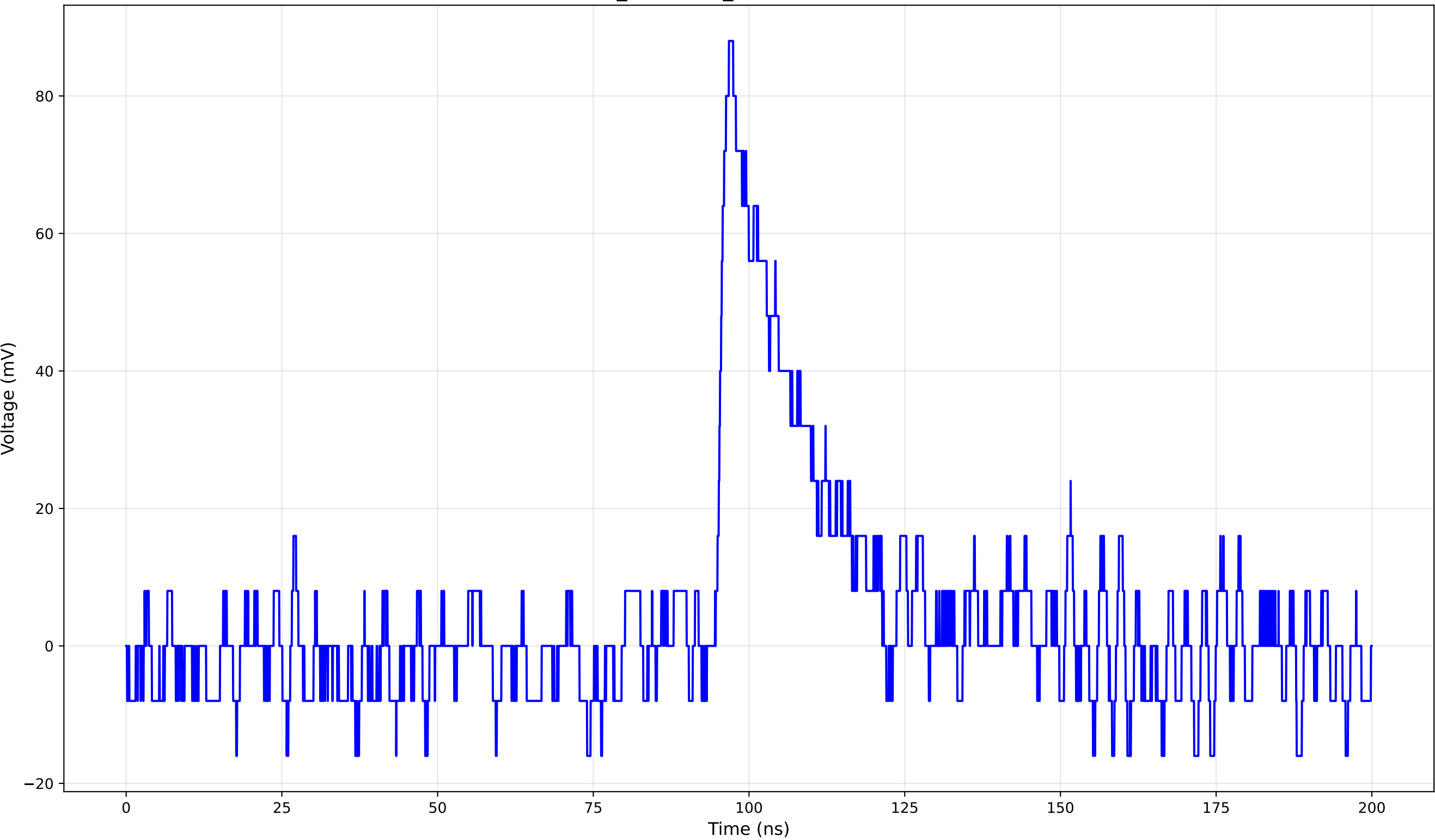
TCT Pulse Waveform - Run 2_100: 1cm_42-Position2 (100.0 V) - Rise Time: 1.64 ns
