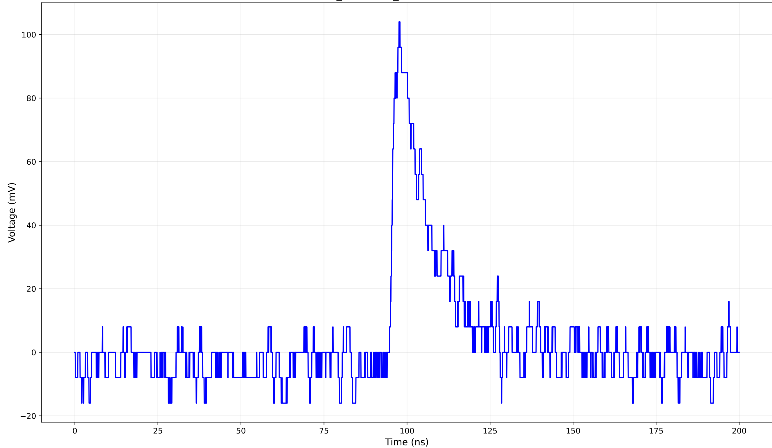
TCT Pulse Waveform - Run 2_110: 1cm_42-Position2 (110.0 V) - Rise Time: 2.50 ns
