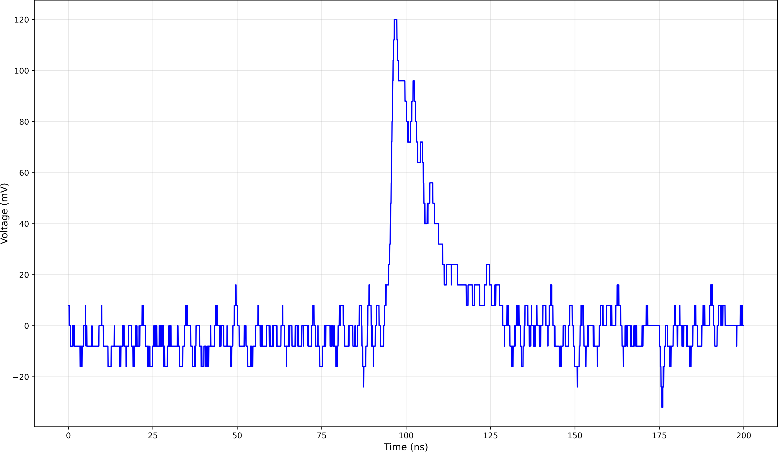
TCT Pulse Waveform - Run 2_120: 1cm_42-Position2 (120.0 V) - Rise Time: 2.66 ns
