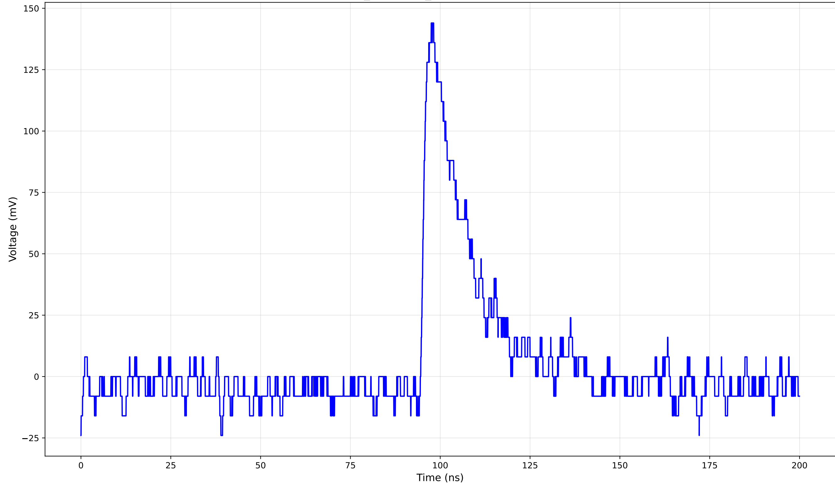
TCT Pulse Waveform - Run 2_130: 1cm_42-Position2 (130.0 V) - Rise Time: 2.13 ns
