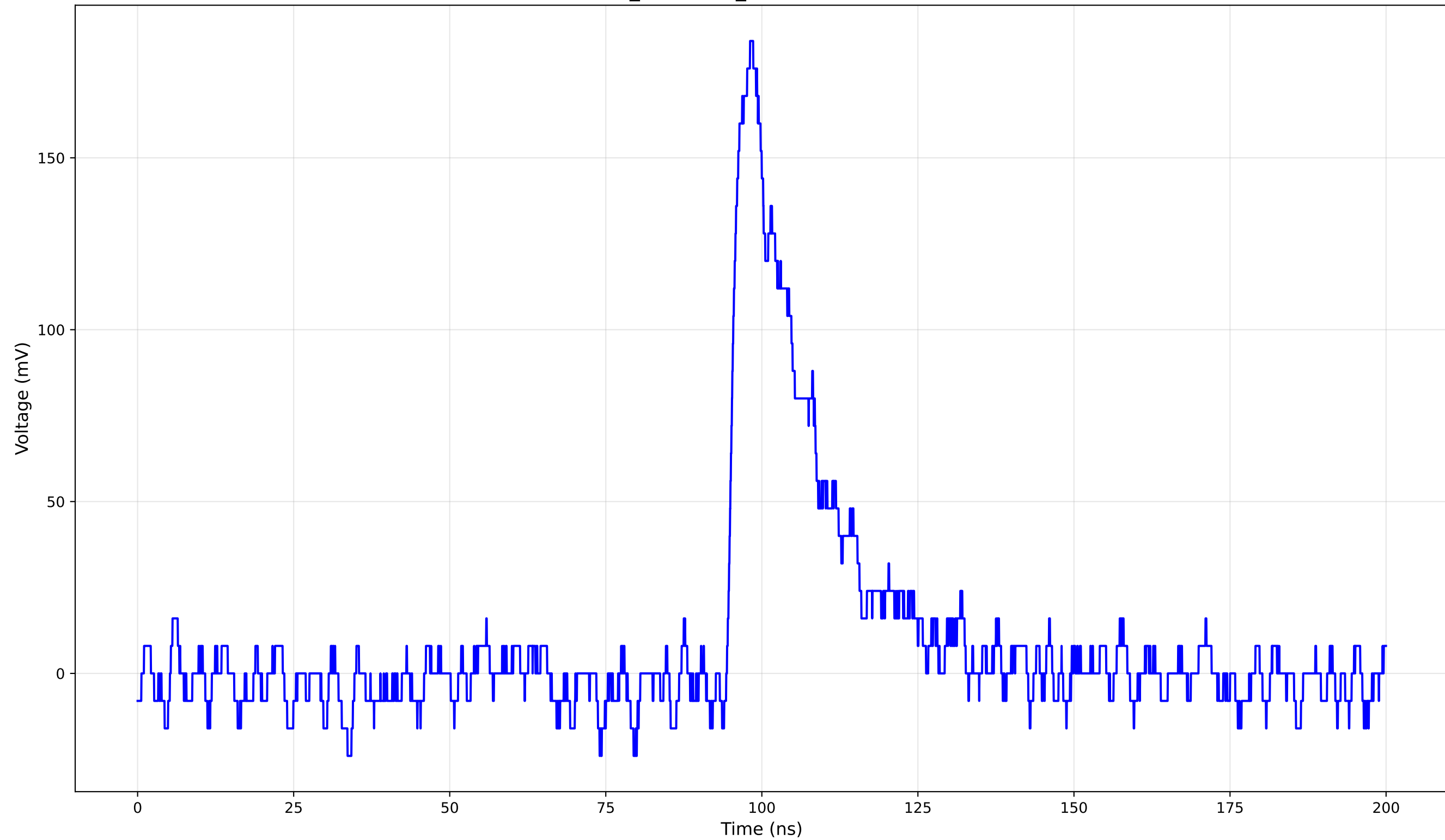
TCT Pulse Waveform - Run 2_140: 1cm_42-Position2 (140.0 V) - Rise Time: 2.20 ns
