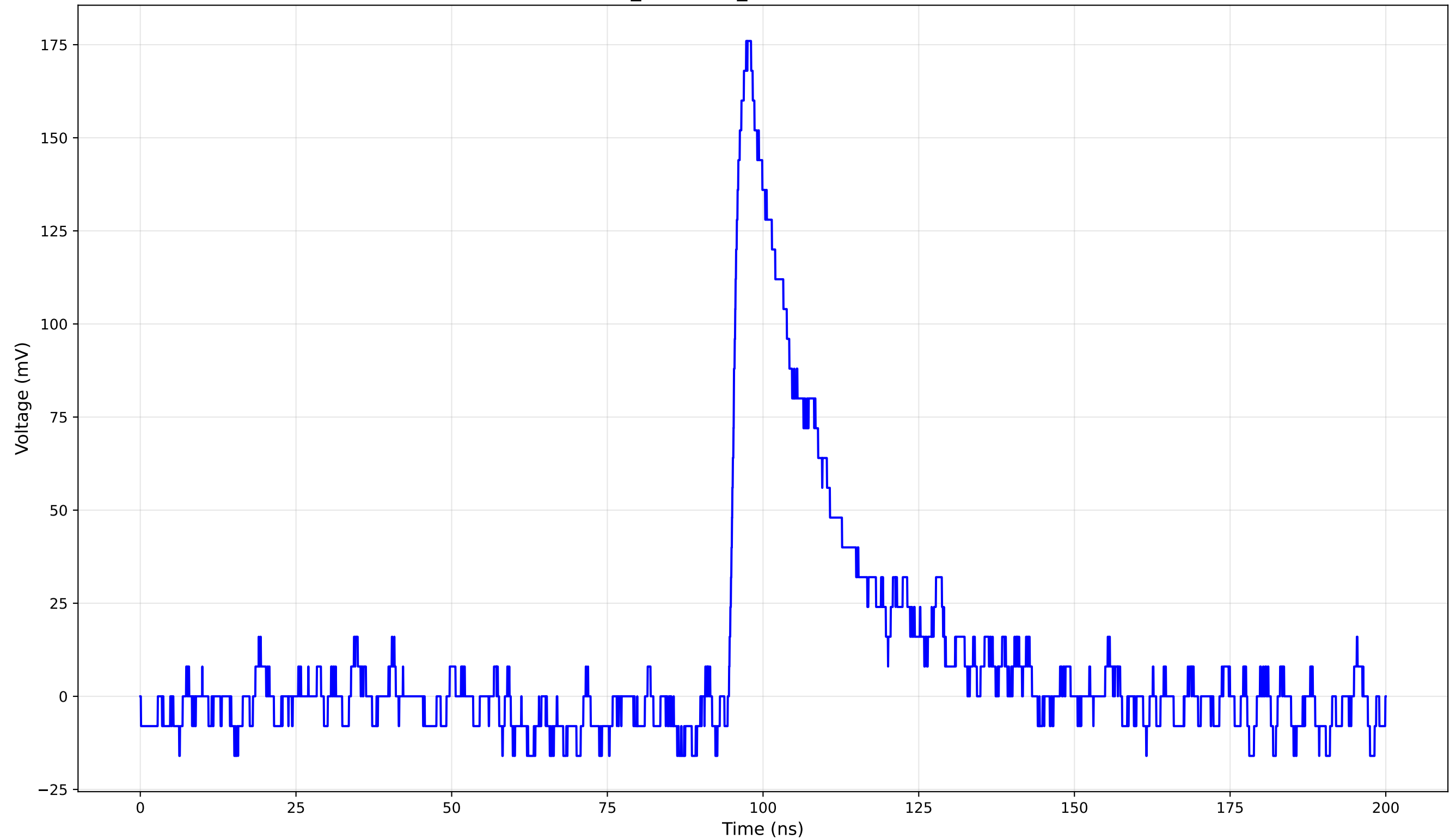
TCT Pulse Waveform - Run 2_141: 1cm_42-Position2 (141.0 V) - Rise Time: 1.91 ns
