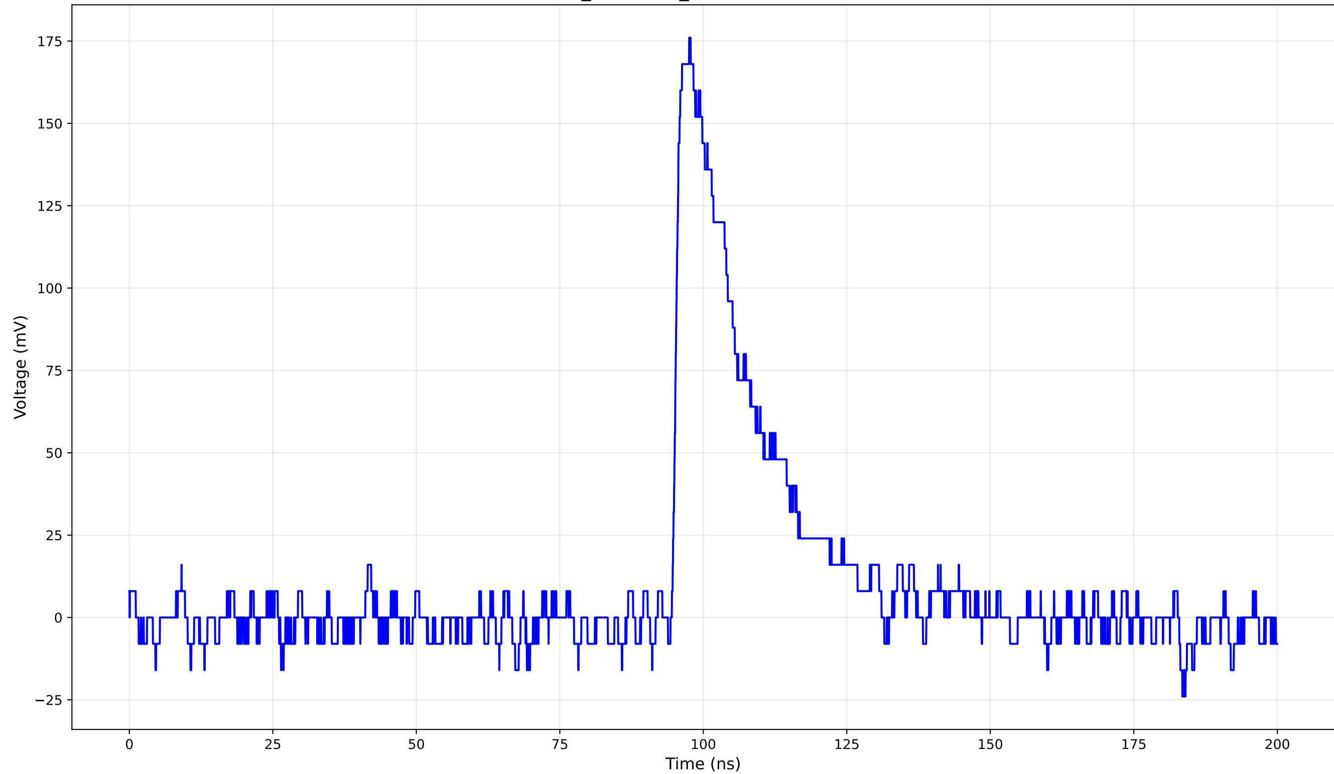
TCT Pulse Waveform - Run 2_142: 1cm_42-Position2 (142.0 V) - Rise Time: 1.28 ns
