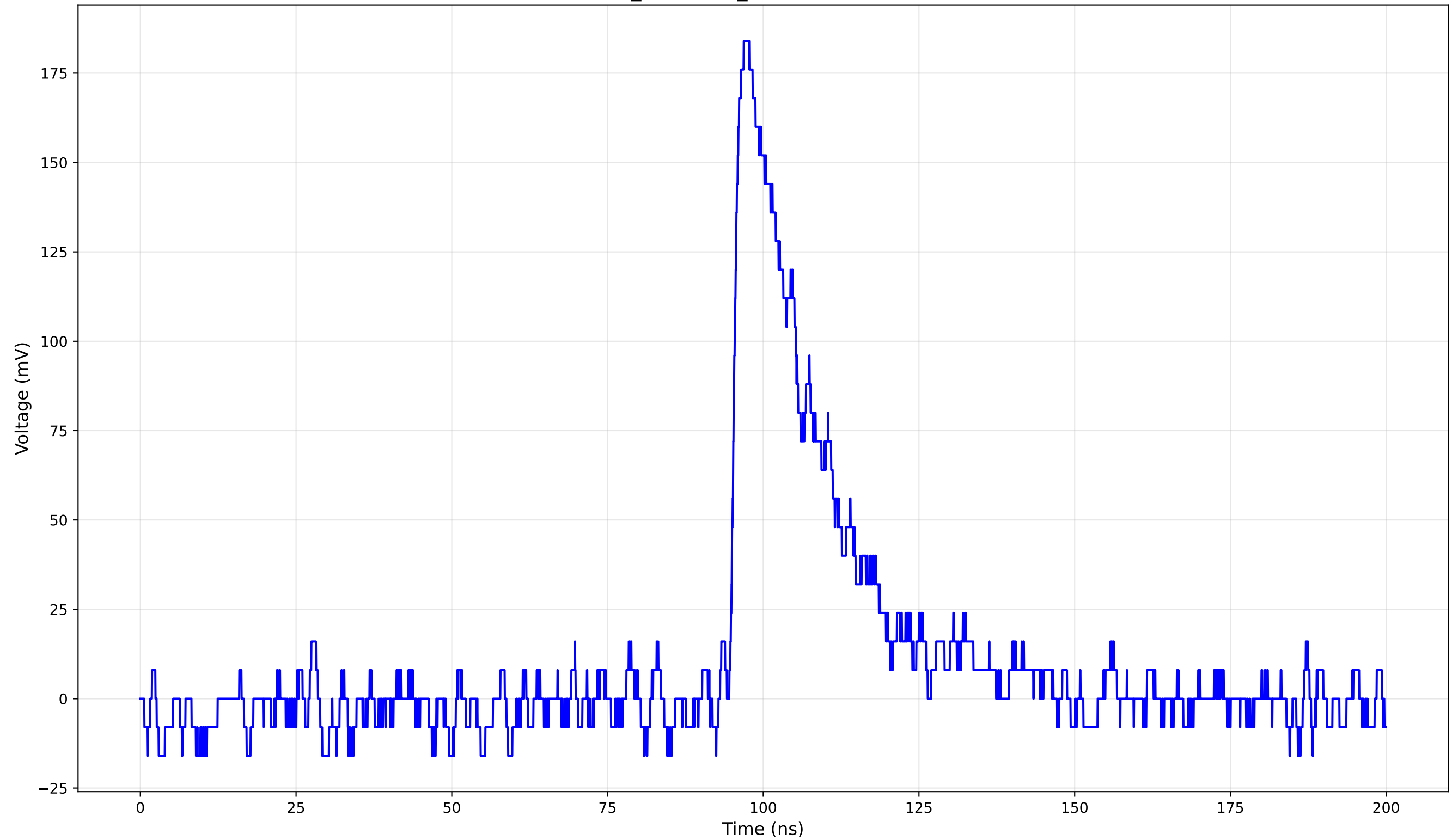
TCT Pulse Waveform - Run 2_143: 1cm_42-Position2 (143.0 V) - Rise Time: 1.41 ns
