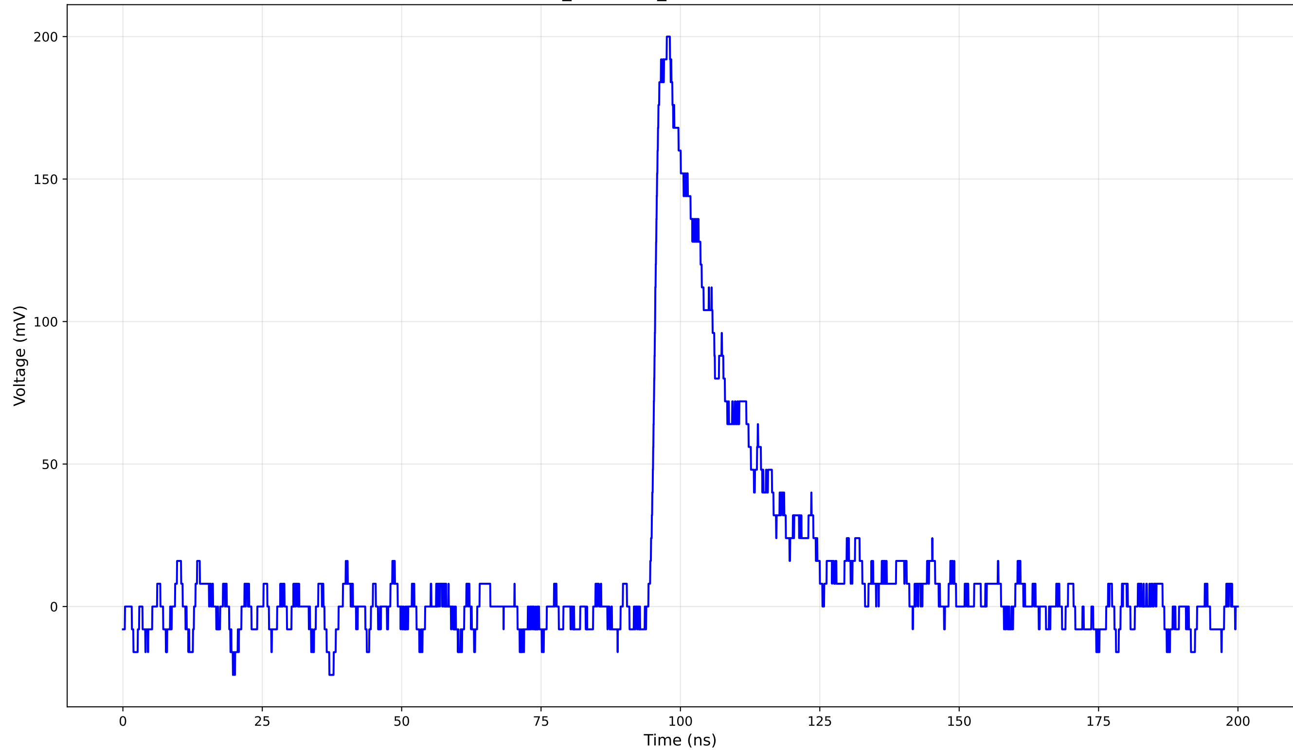
TCT Pulse Waveform - Run 2_144: 1cm_42-Position2 (144.0 V) - Rise Time: 1.50 ns
