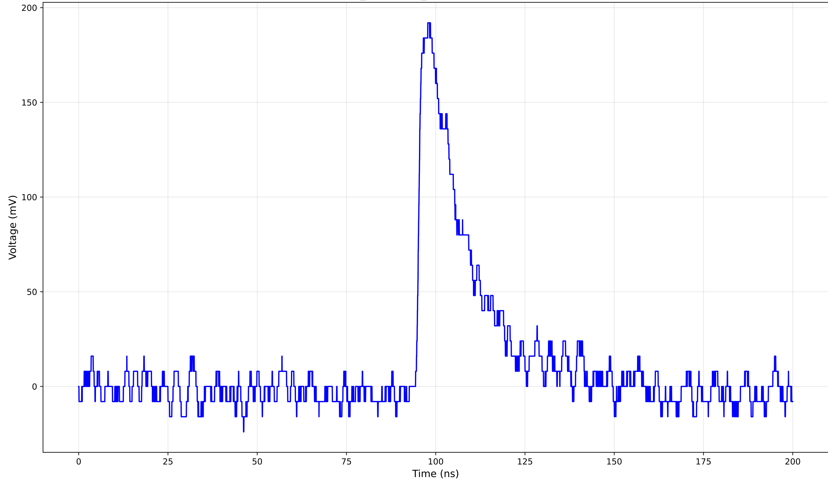
TCT Pulse Waveform - Run 2_145: 1cm_42-Position2 (145.0 V) - Rise Time: 1.39 ns
