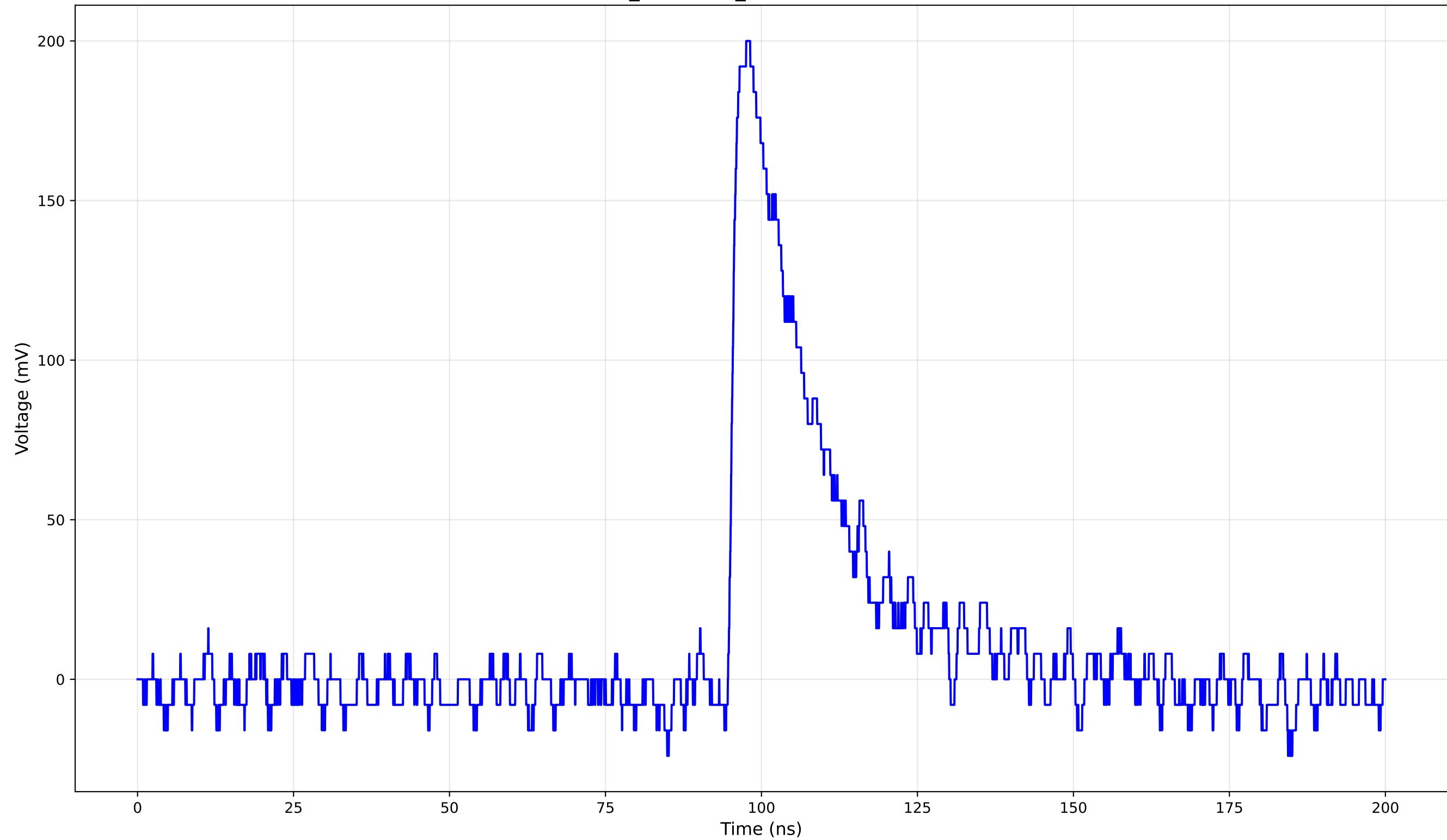
TCT Pulse Waveform - Run 2_146: 1cm_42-Position2 (146.0 V) - Rise Time: 1.42 ns
