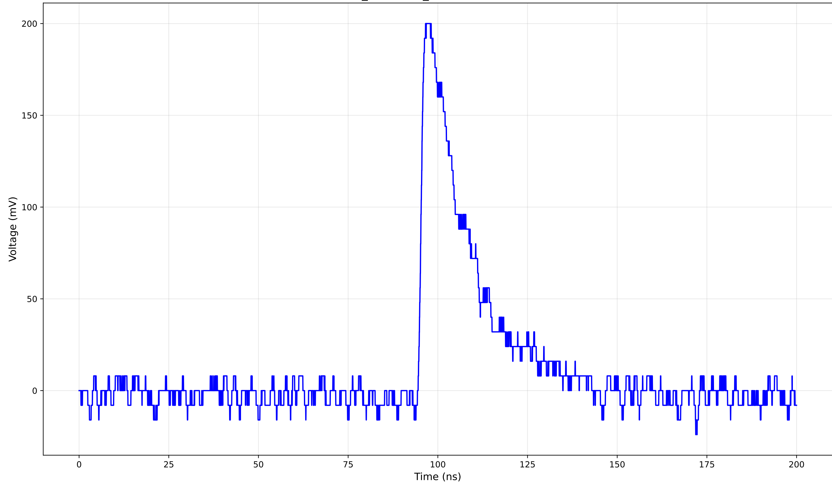
TCT Pulse Waveform - Run 2_147: 1cm_42-Position2 (147.0 V) - Rise Time: 1.40 ns
