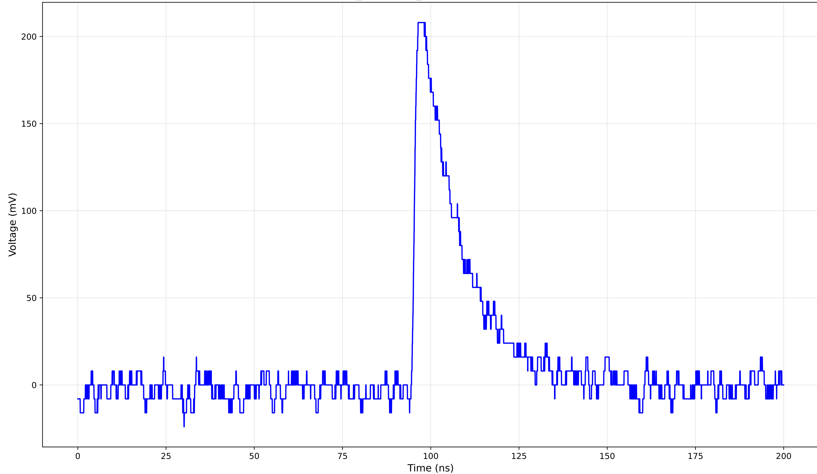
TCT Pulse Waveform - Run 2_148: 1cm_42-Position2 (148.0 V) - Rise Time: 1.32 ns
