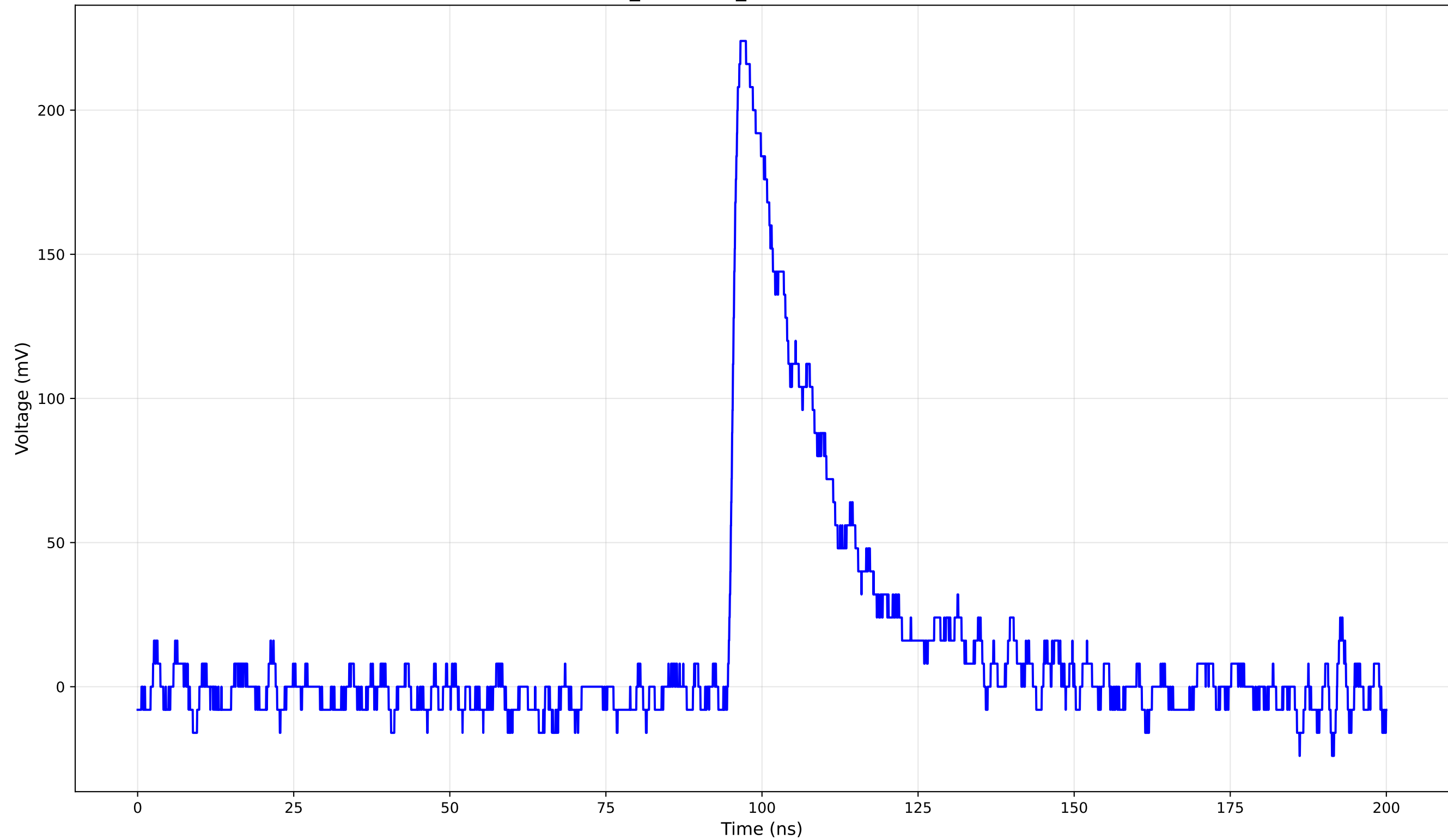
TCT Pulse Waveform - Run 2_149: 1cm_42-Position2 (149.0 V) - Rise Time: 1.37 ns
