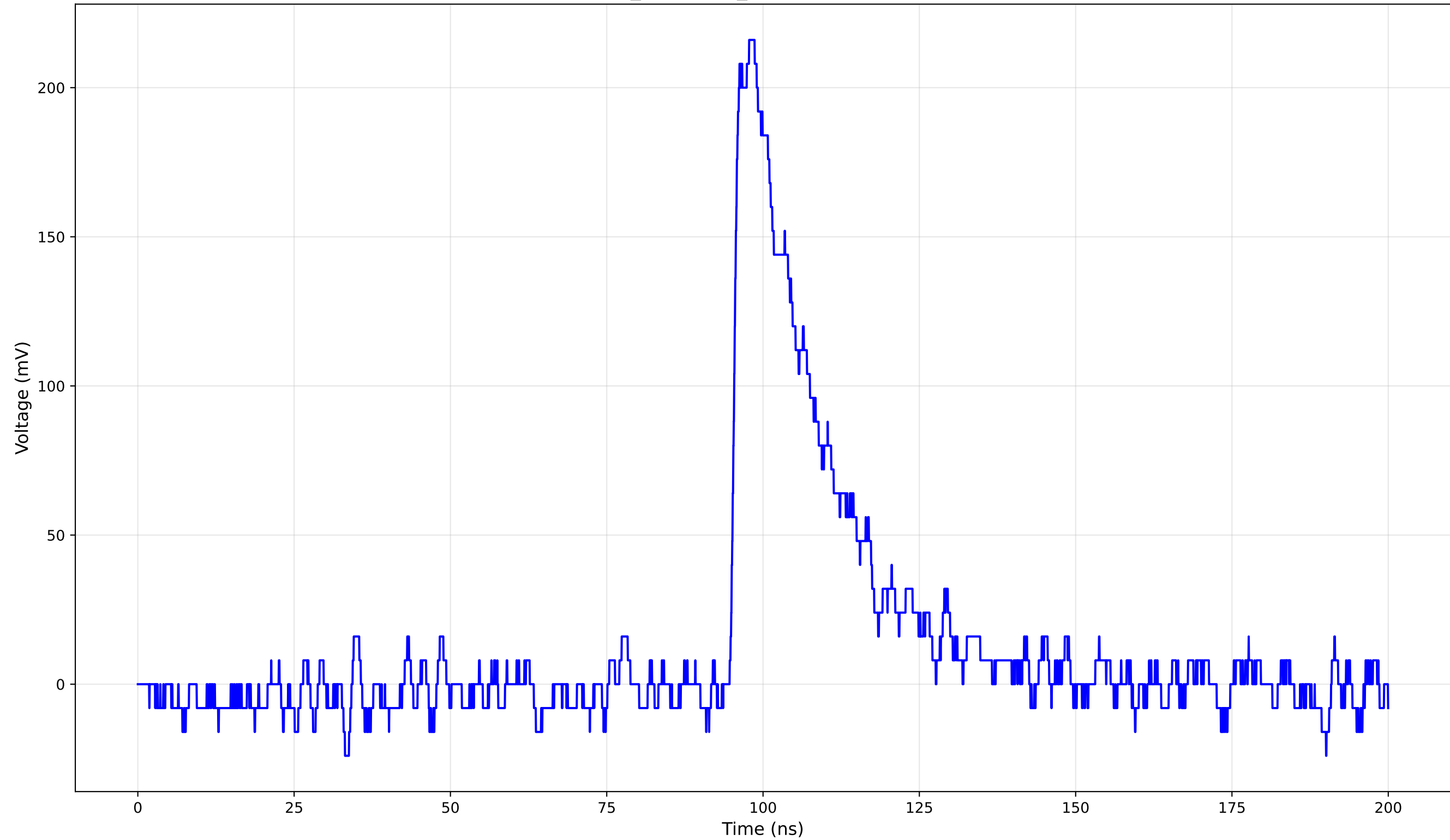
TCT Pulse Waveform - Run 2_150: 1cm_42-Position2 (150.0 V) - Rise Time: 1.23 ns
