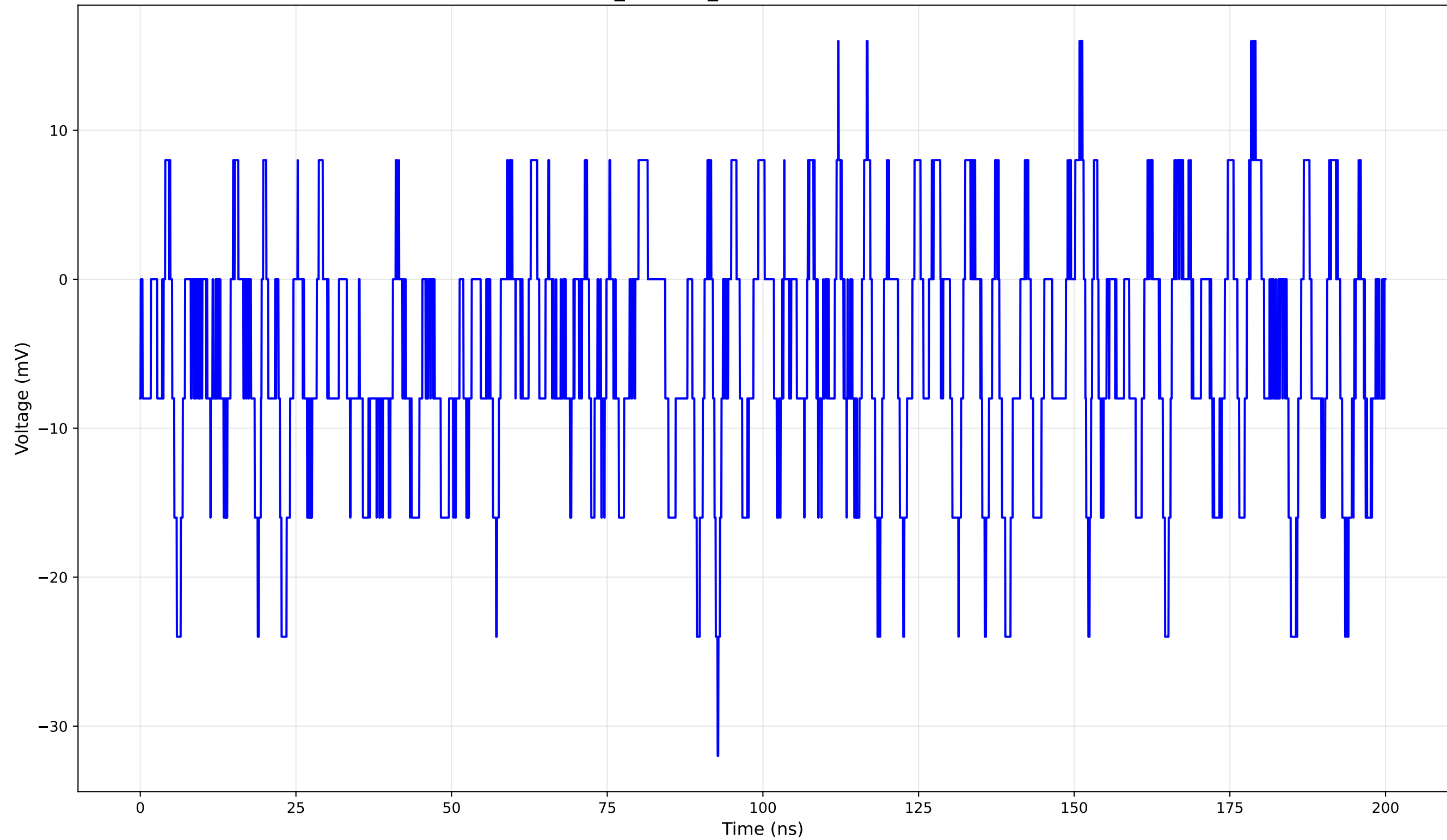
TCT Pulse Waveform - Run 2_20: 1cm_42-Position2 (20.0 V) - Rise Time: 0.00 ns (N/A)
