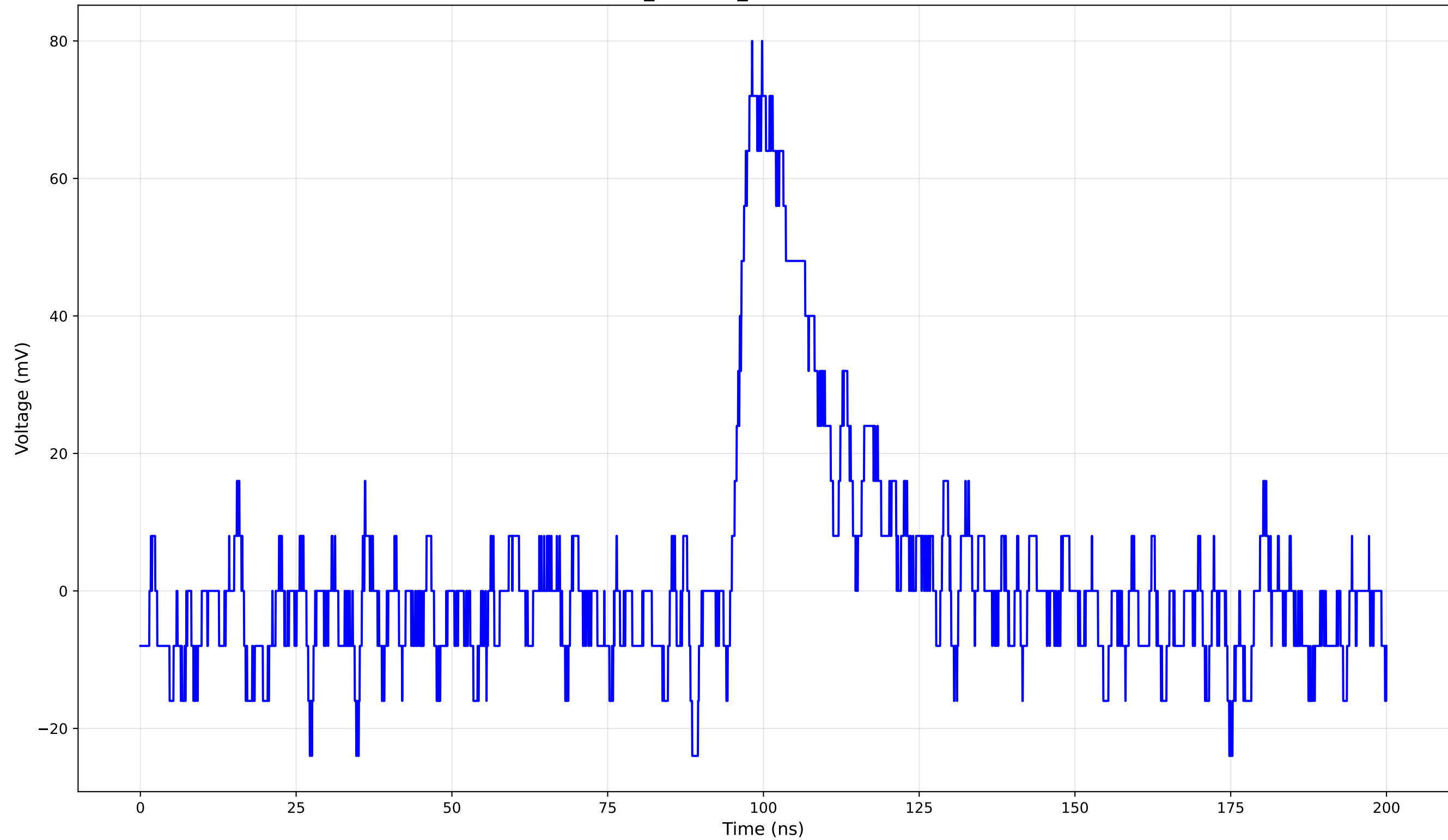
TCT Pulse Waveform - Run 2_40: 1cm_42-Position2 (40.0 V) - Rise Time: 2.82 ns
