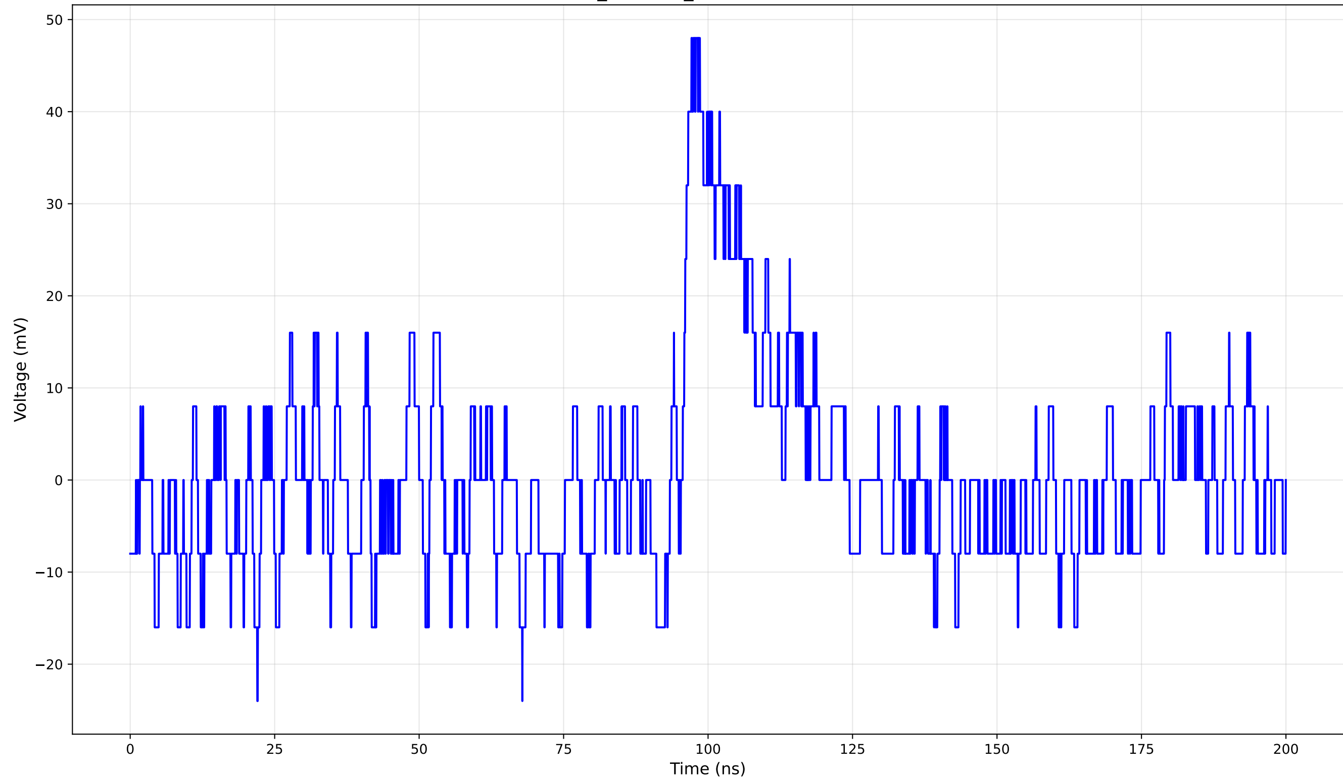
TCT Pulse Waveform - Run 2_50: 1cm_42-Position2 (50.0 V) - Rise Time: 1.84 ns
