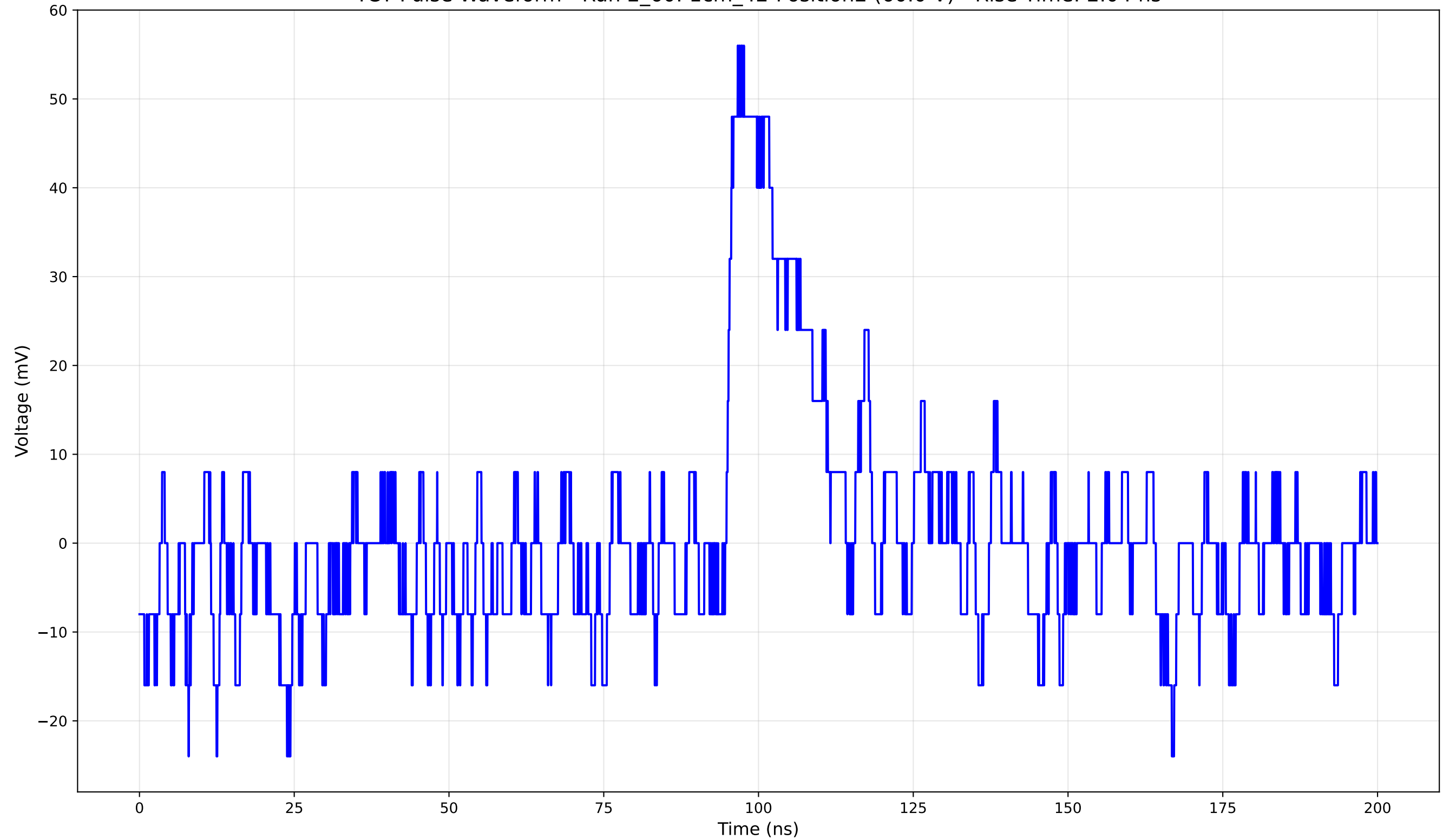
TCT Pulse Waveform - Run 2_60: 1cm_42-Position2 (60.0 V) - Rise Time: 2.04 ns
