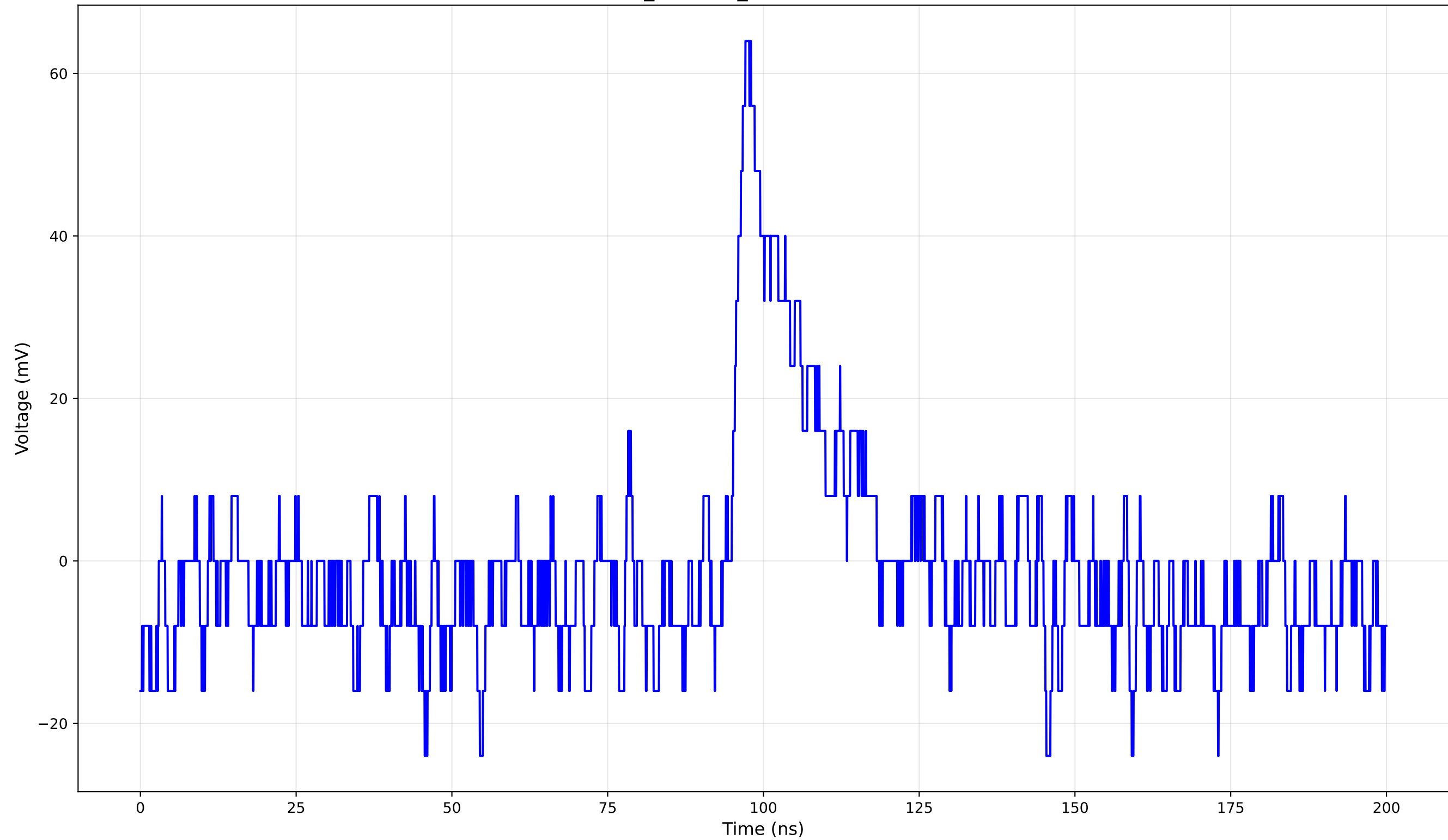
TCT Pulse Waveform - Run 2_70: 1cm_42-Position2 (70.0 V) - Rise Time: 2.20 ns
