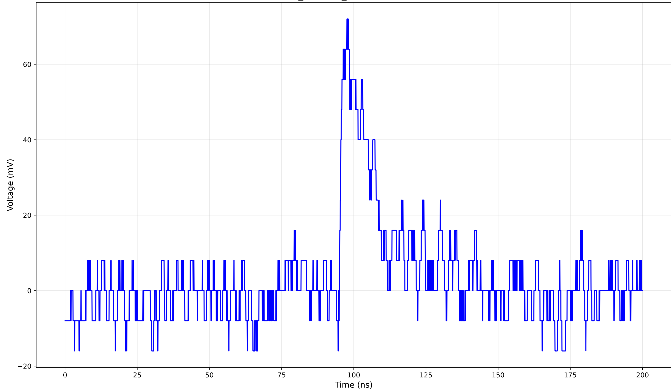
TCT Pulse Waveform - Run 2_80: 1cm_42-Position2 (80.0 V) - Rise Time: 2.55 ns
