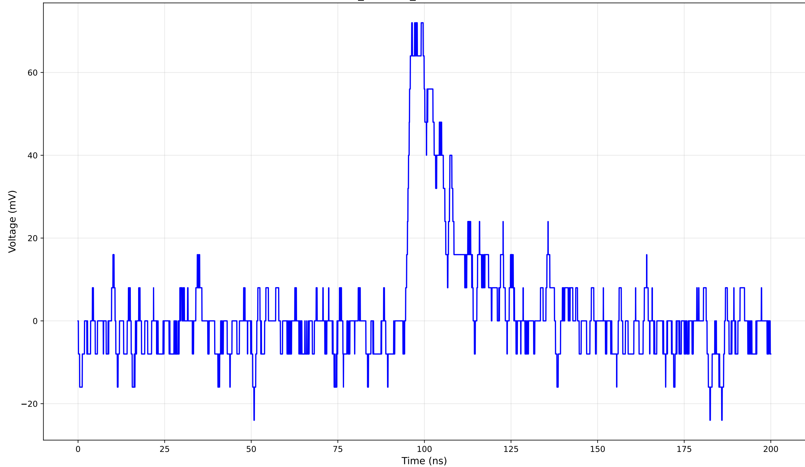
TCT Pulse Waveform - Run 2_90: 1cm_42-Position2 (90.0 V) - Rise Time: 1.75 ns
