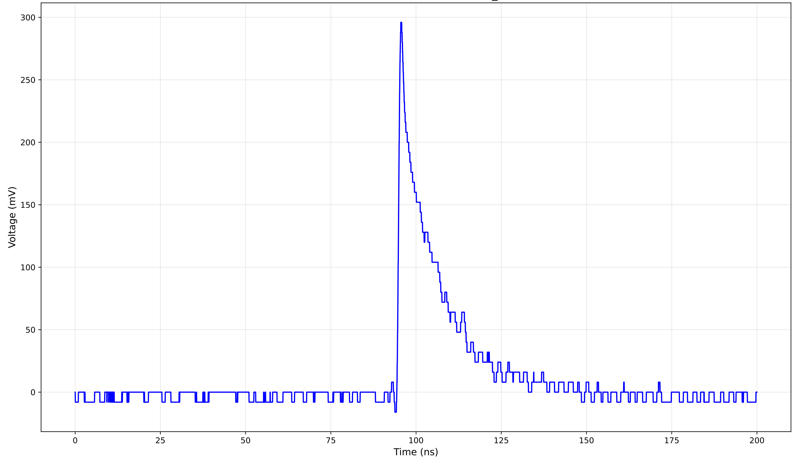
TCT Pulse Waveform - Run 3265um: 1cm_42 (150.0 V)
