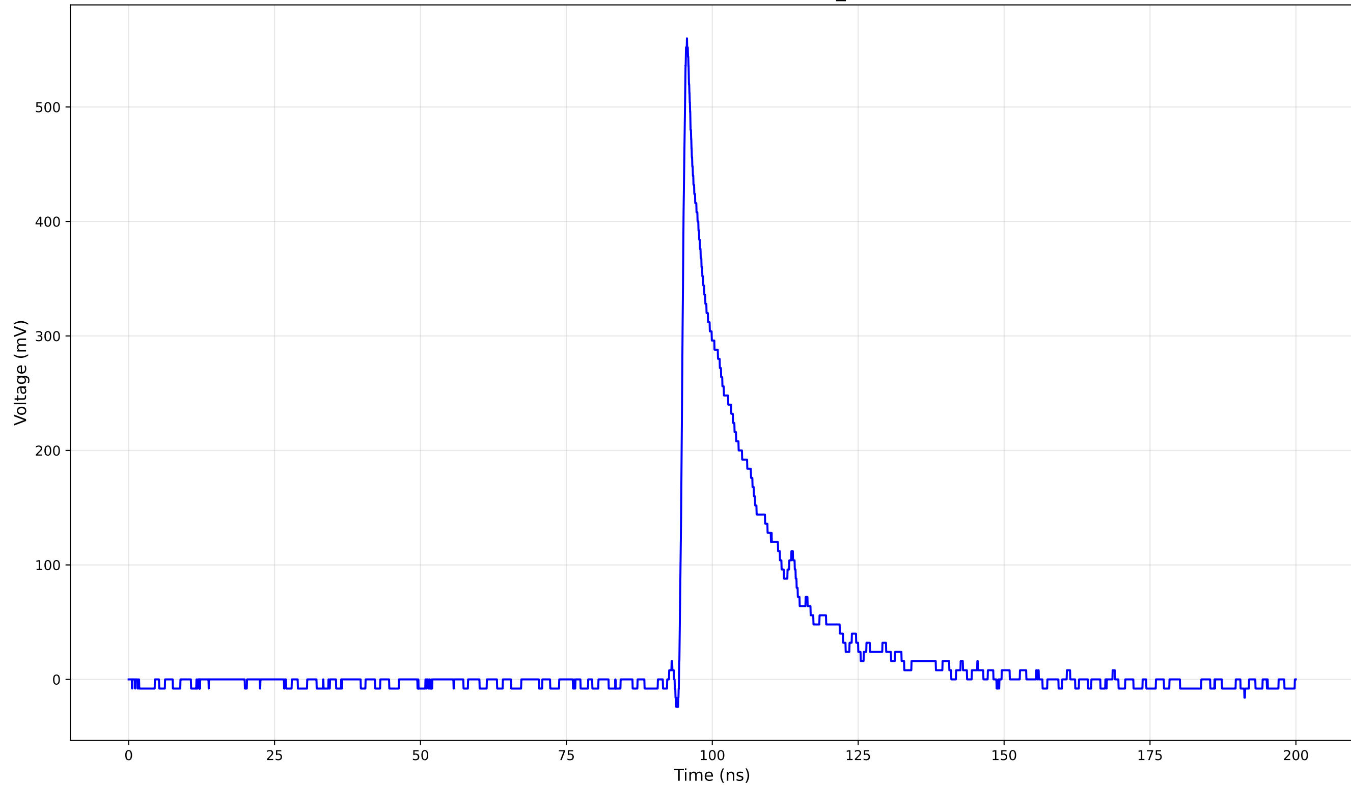
TCT Pulse Waveform - Run 395um: 1cm_42 (150.0 V)
