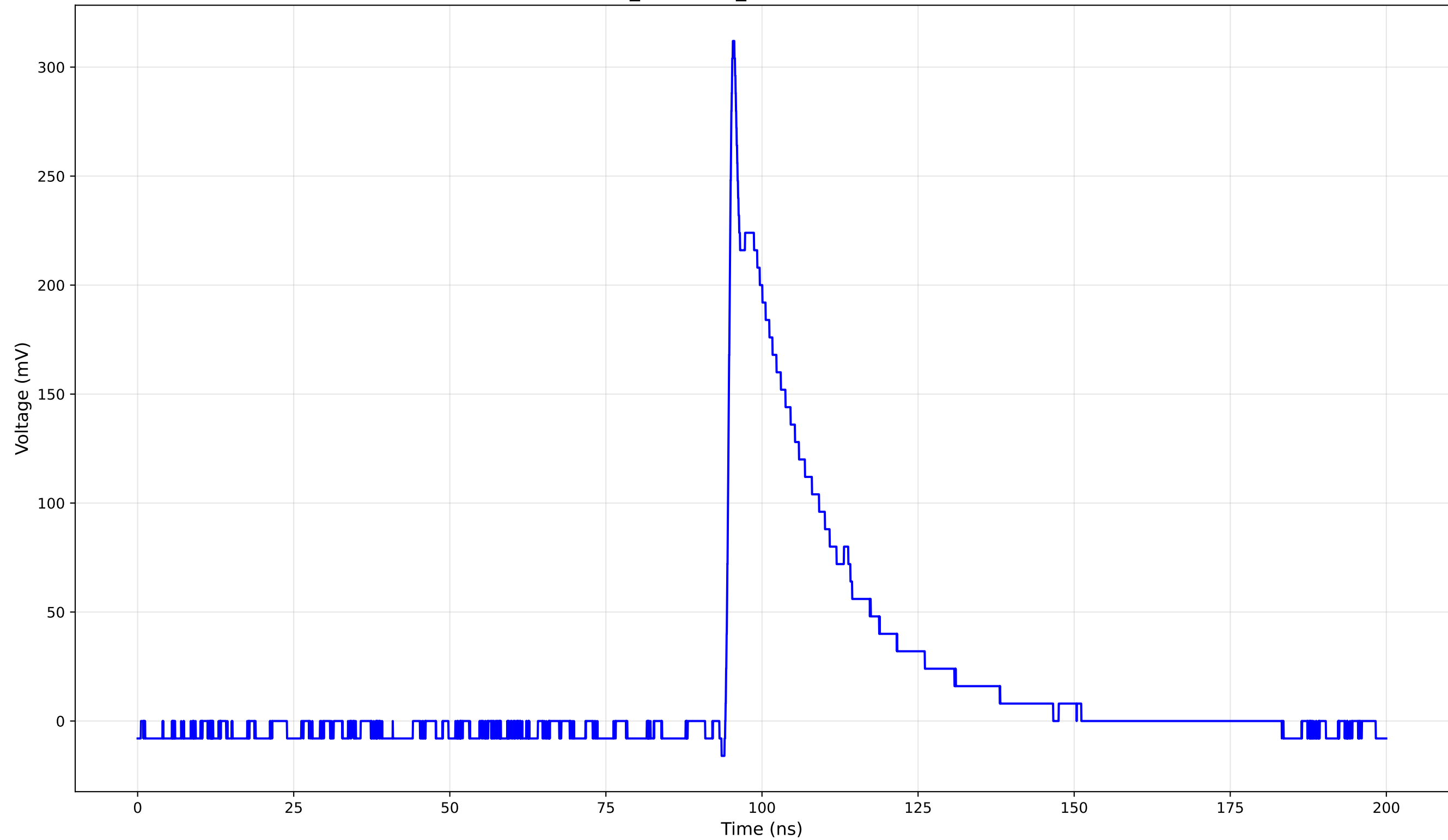
TCT Pulse Waveform - Run 3_100: 1cm_42-Position3 (100.0 V) - Rise Time: 0.86 ns
