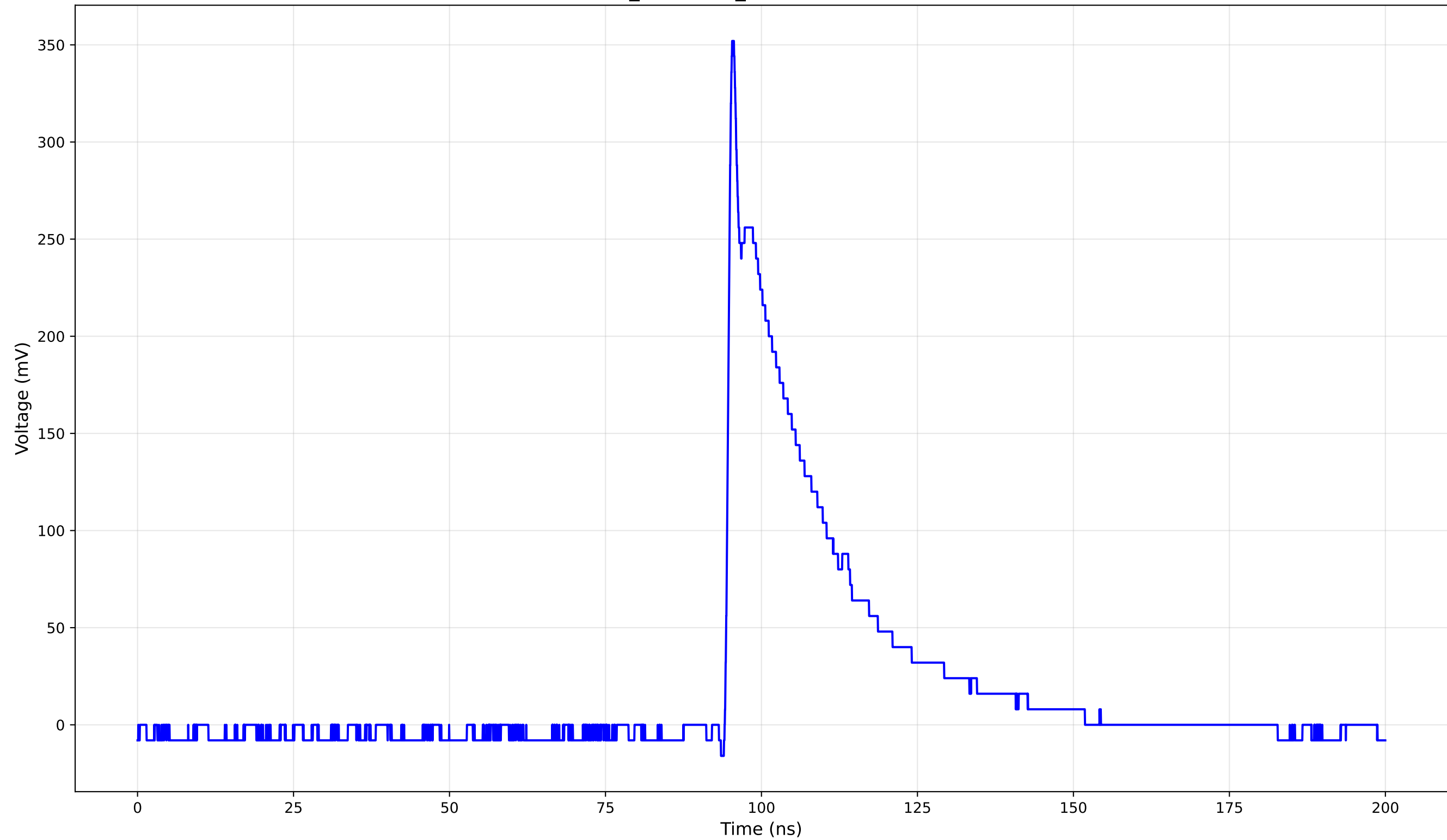
TCT Pulse Waveform - Run 3_110: 1cm_42-Position3 (110.0 V) - Rise Time: 0.84 ns
