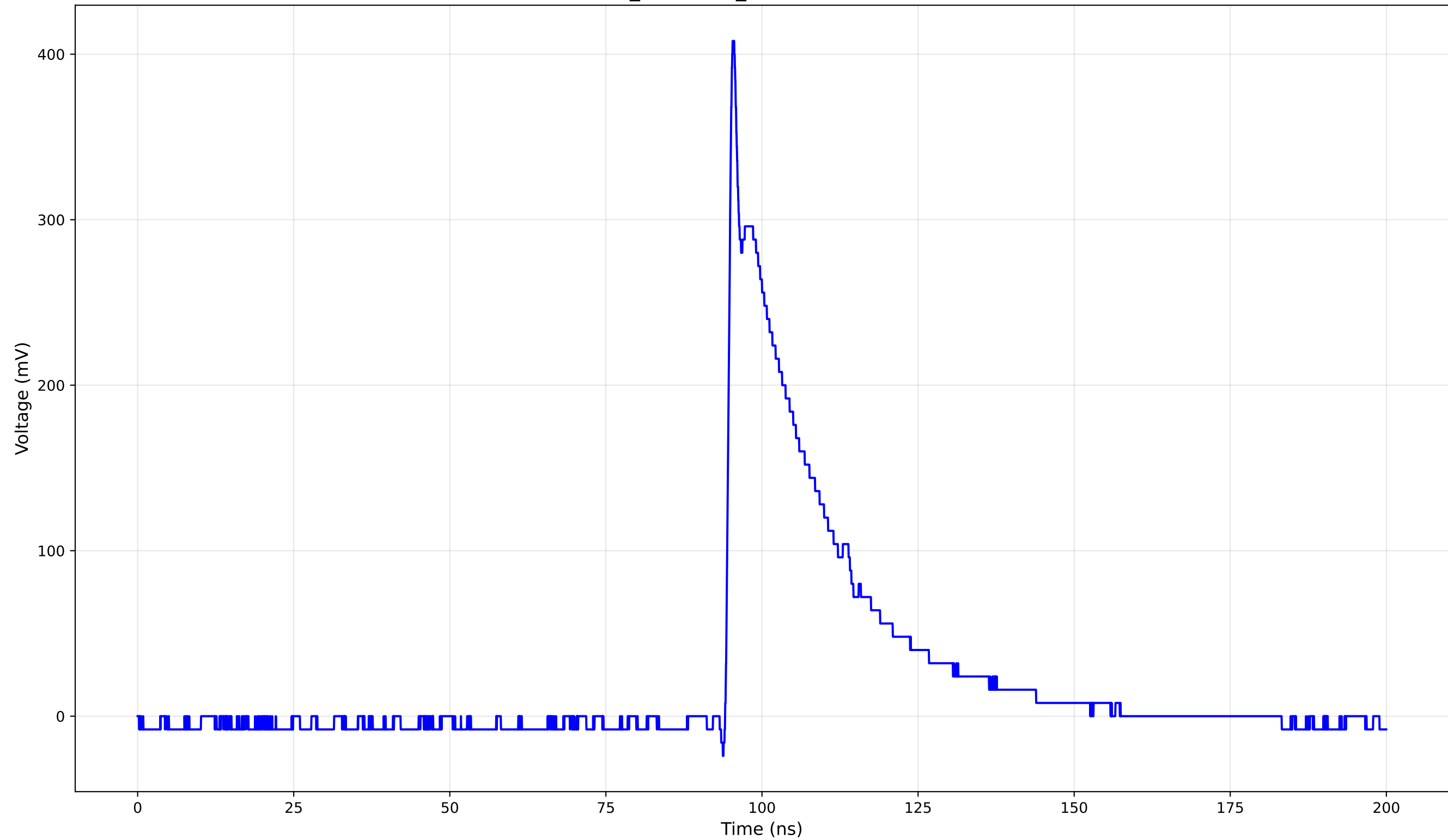
TCT Pulse Waveform - Run 3_120: 1cm_42-Position3 (120.0 V) - Rise Time: 0.81 ns
