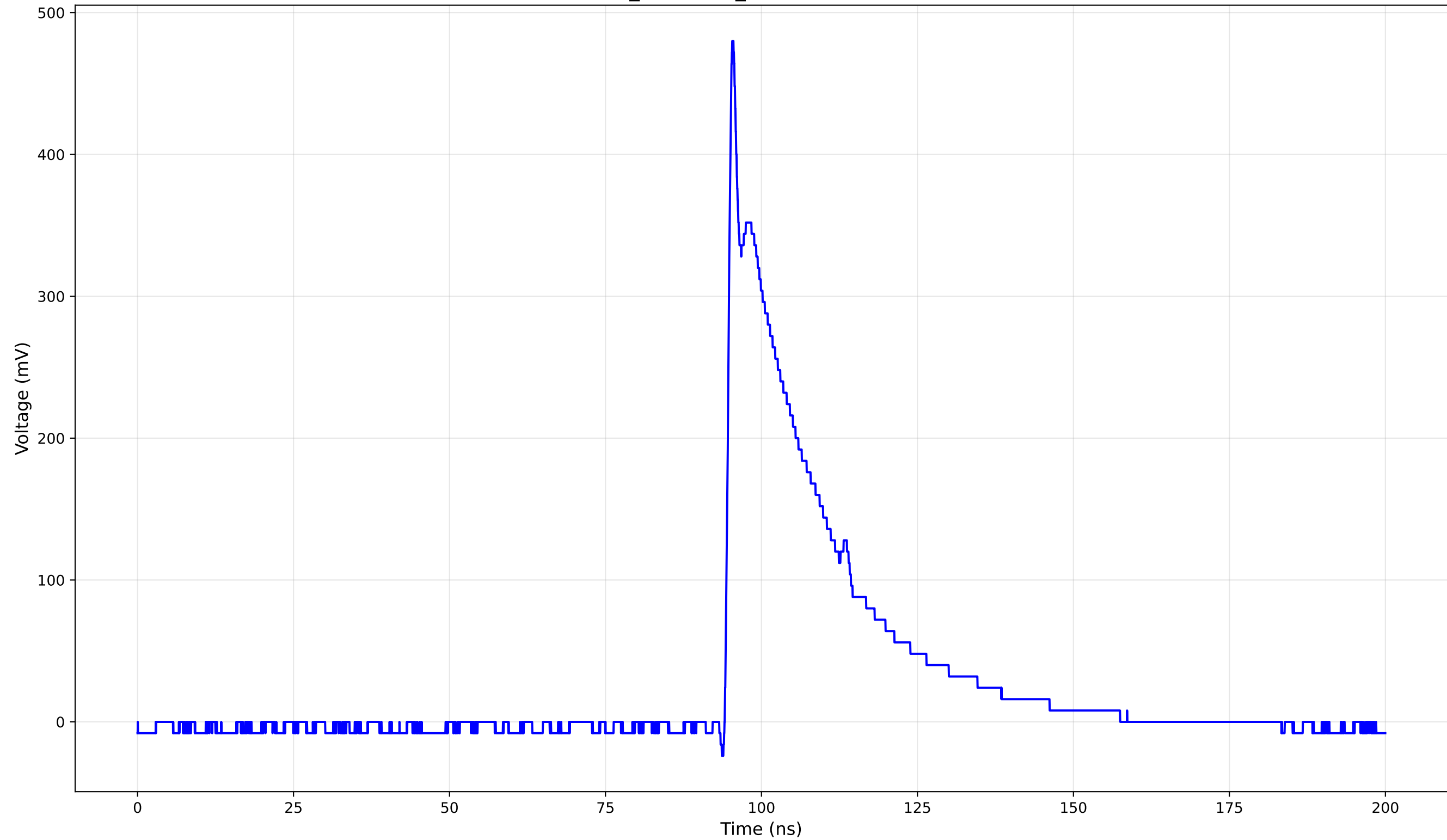
TCT Pulse Waveform - Run 3_130: 1cm_42-Position3 (130.0 V) - Rise Time: 0.81 ns
