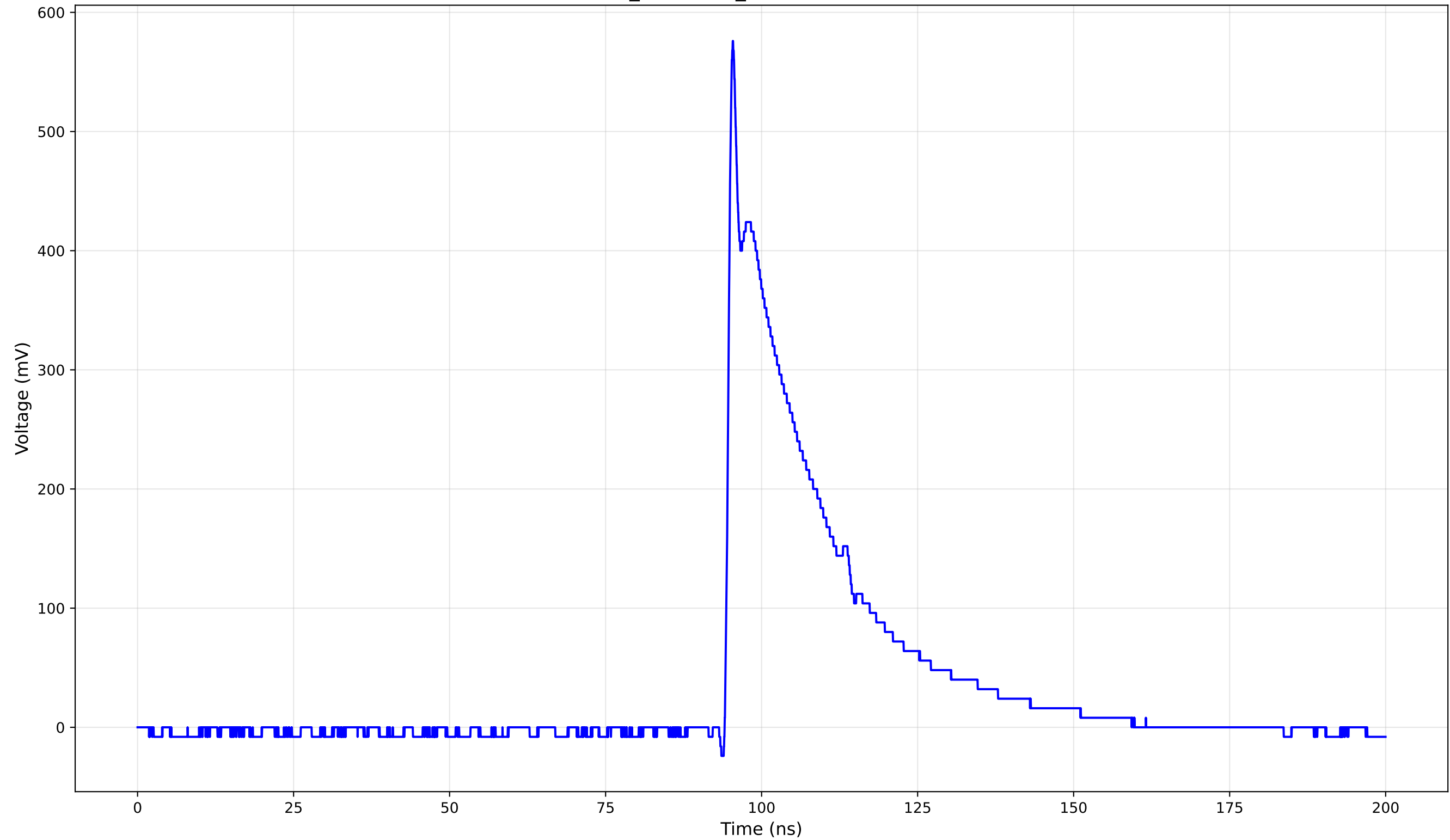
TCT Pulse Waveform - Run 3_140: 1cm_42-Position3 (140.0 V) - Rise Time: 0.83 ns
