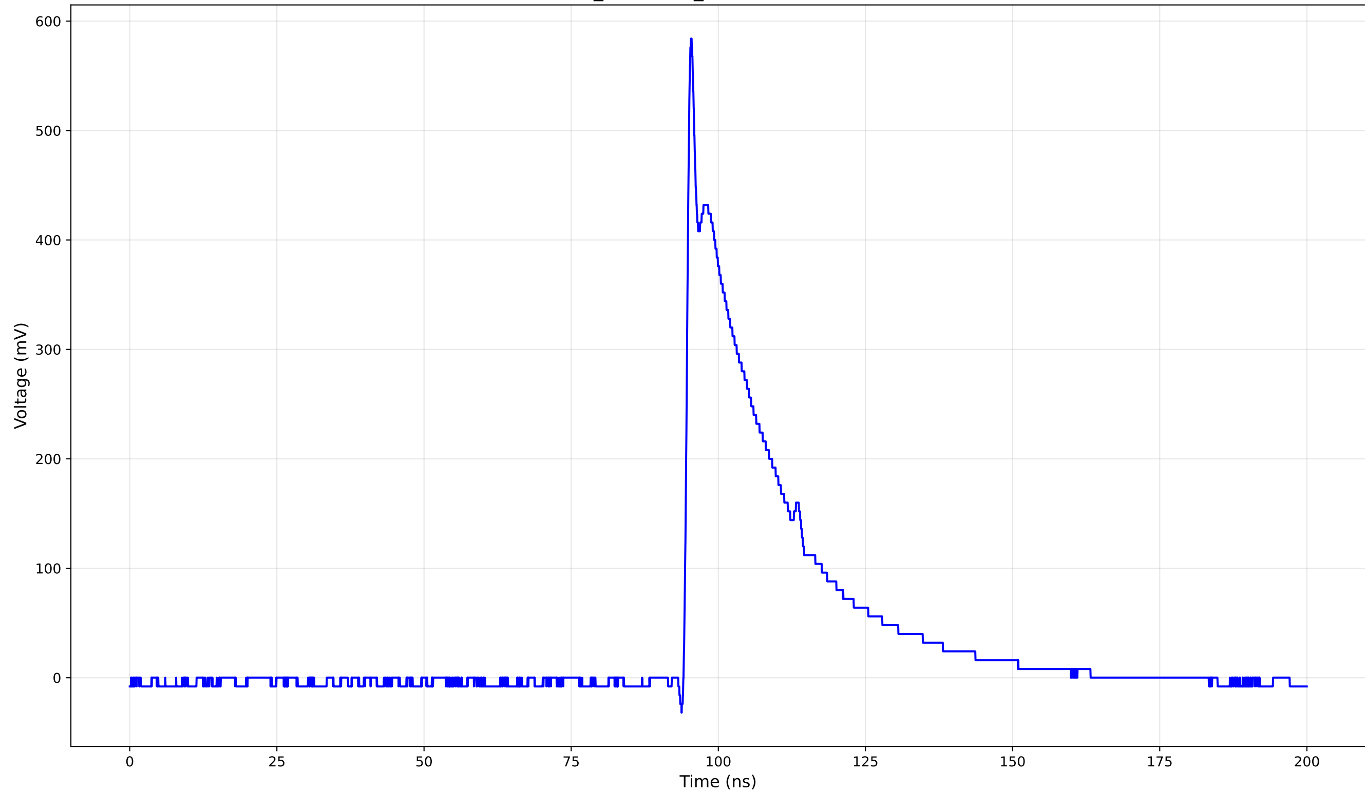
TCT Pulse Waveform - Run 3_141: 1cm_42-Position3 (141.0 V) - Rise Time: 0.82 ns
