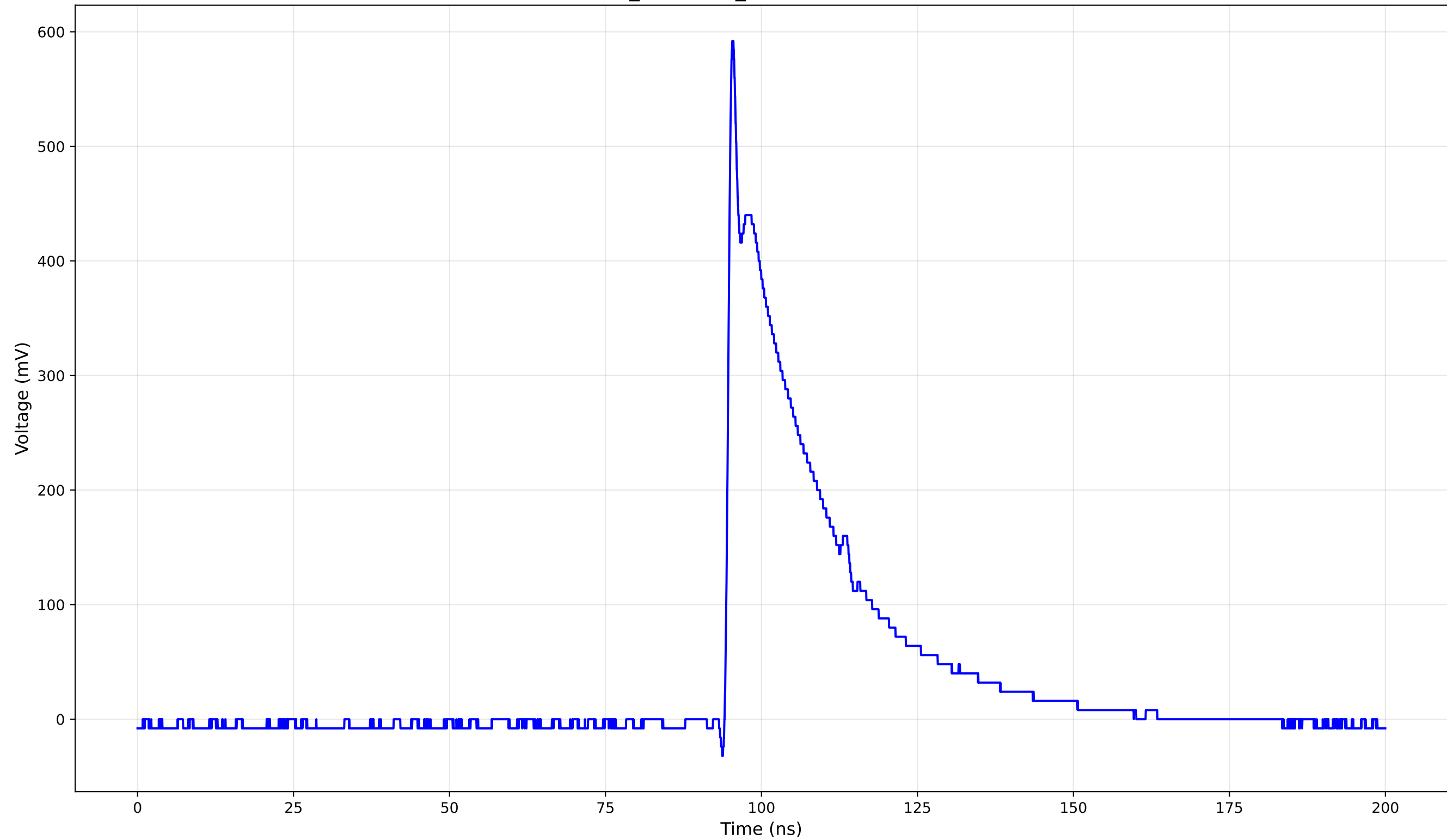
TCT Pulse Waveform - Run 3_142: 1cm_42-Position3 (142.0 V) - Rise Time: 0.82 ns
