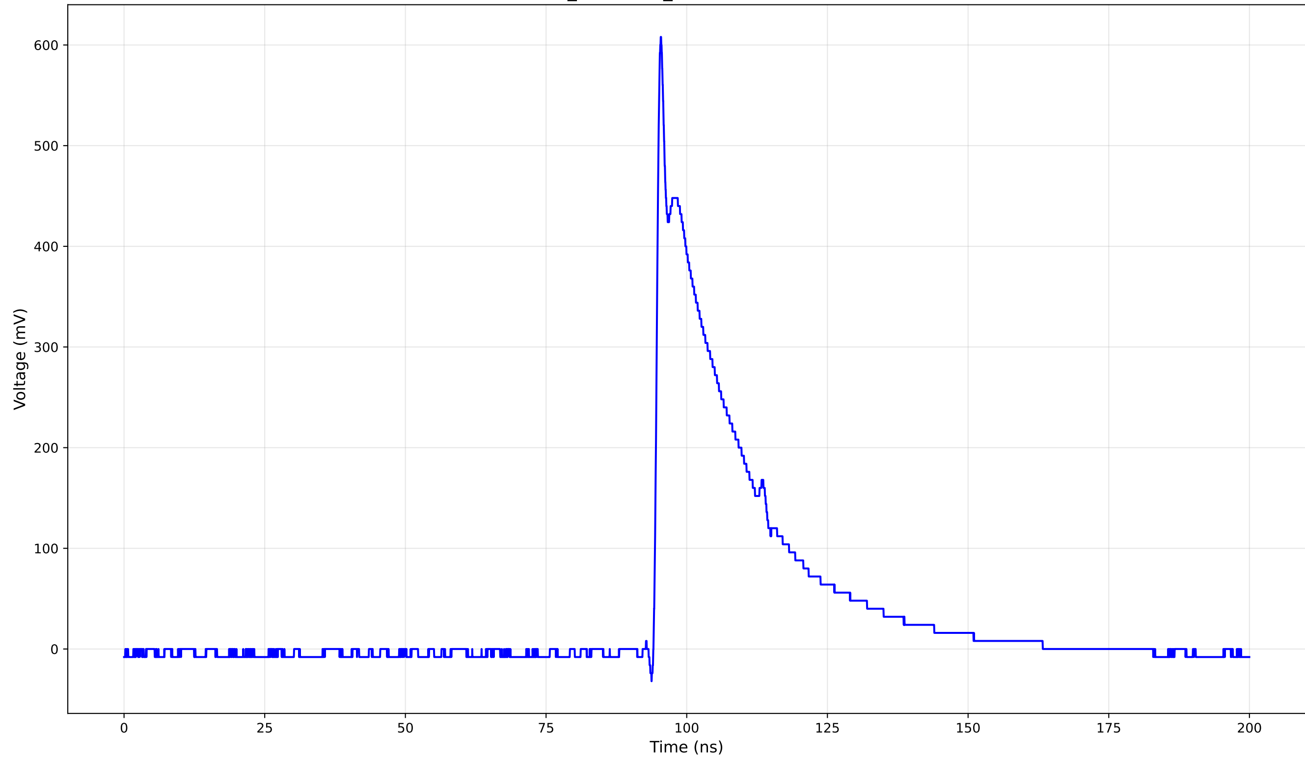
TCT Pulse Waveform - Run 3_143: 1cm_42-Position3 (143.0 V) - Rise Time: 0.82 ns
