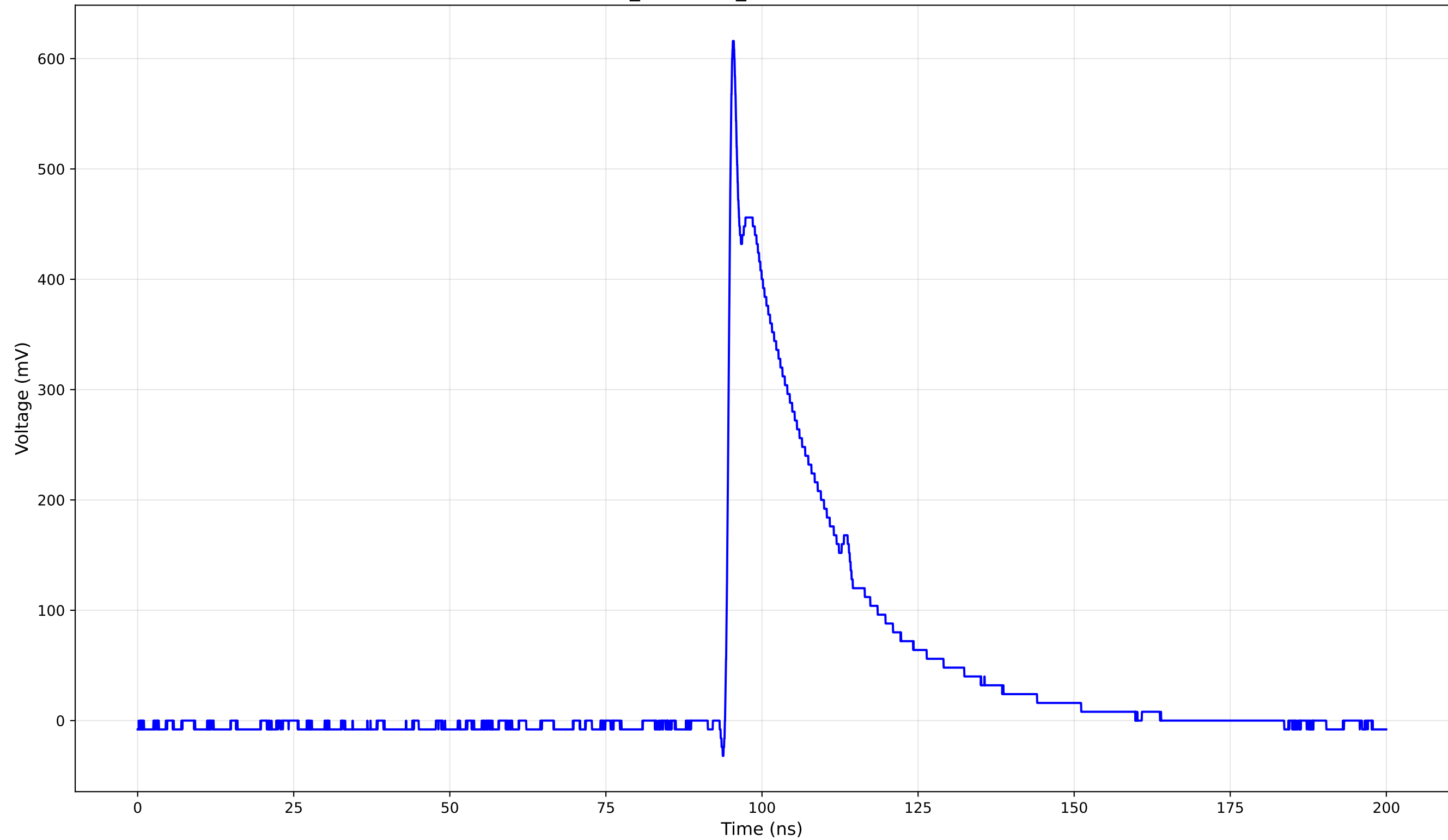
TCT Pulse Waveform - Run 3_144: 1cm_42-Position3 (144.0 V) - Rise Time: 0.80 ns
