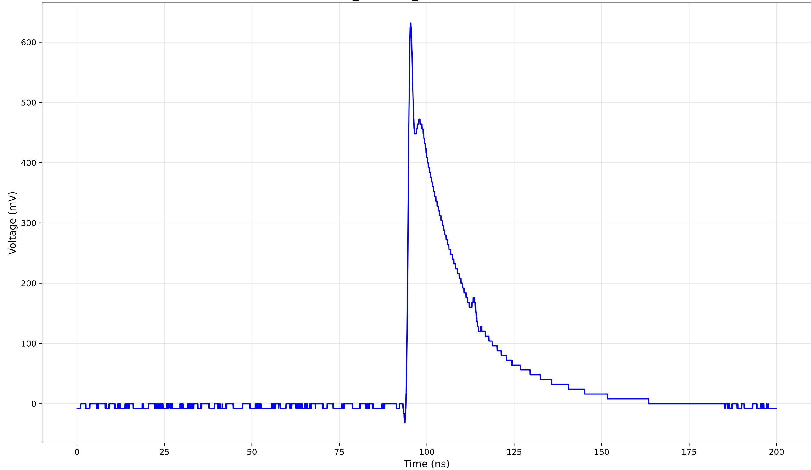
TCT Pulse Waveform - Run 3_145: 1cm_42-Position3 (145.0 V) - Rise Time: 0.83 ns
