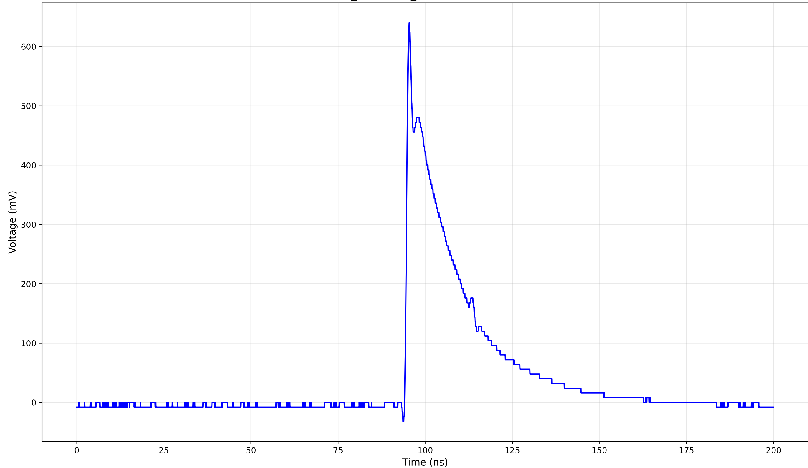
TCT Pulse Waveform - Run 3_146: 1cm_42-Position3 (146.0 V) - Rise Time: 0.83 ns
