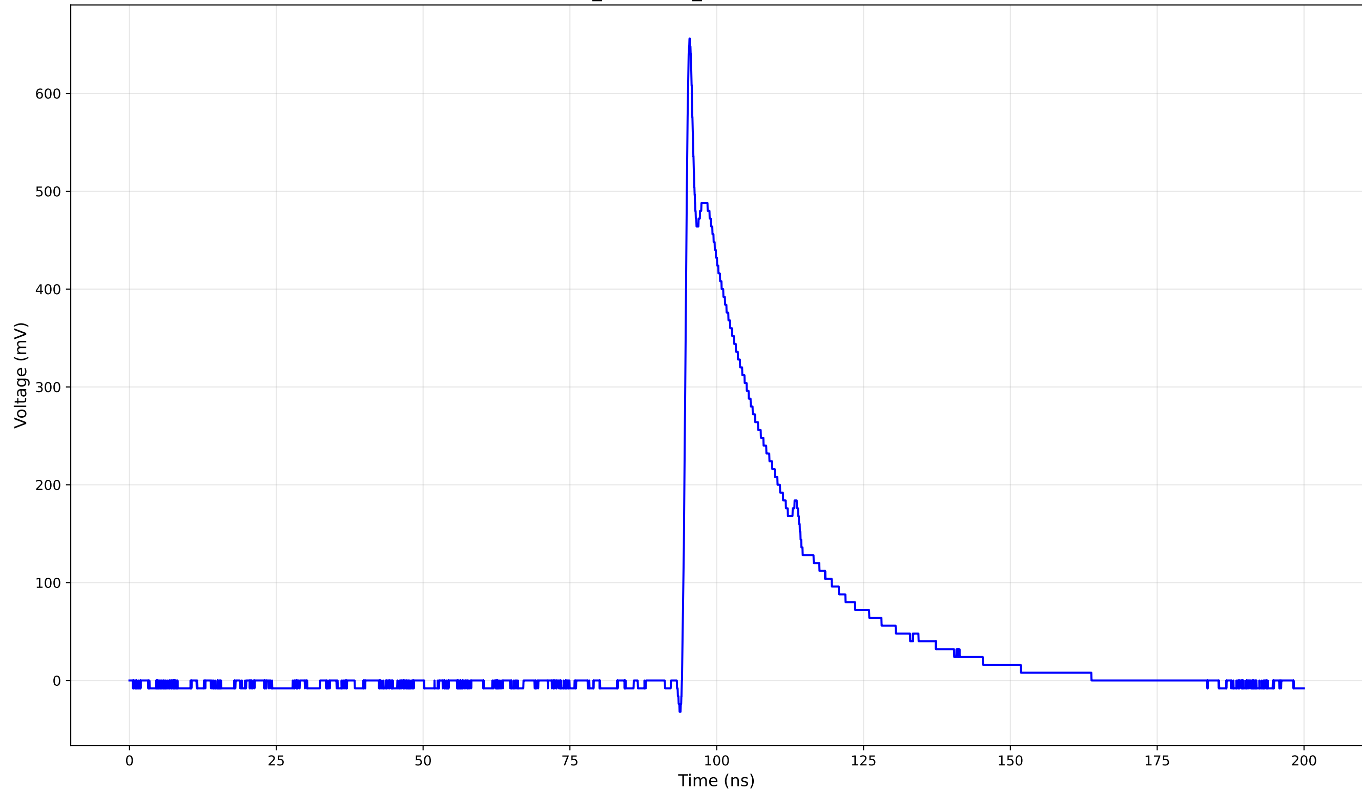
TCT Pulse Waveform - Run 3_147: 1cm_42-Position3 (147.0 V) - Rise Time: 0.82 ns
