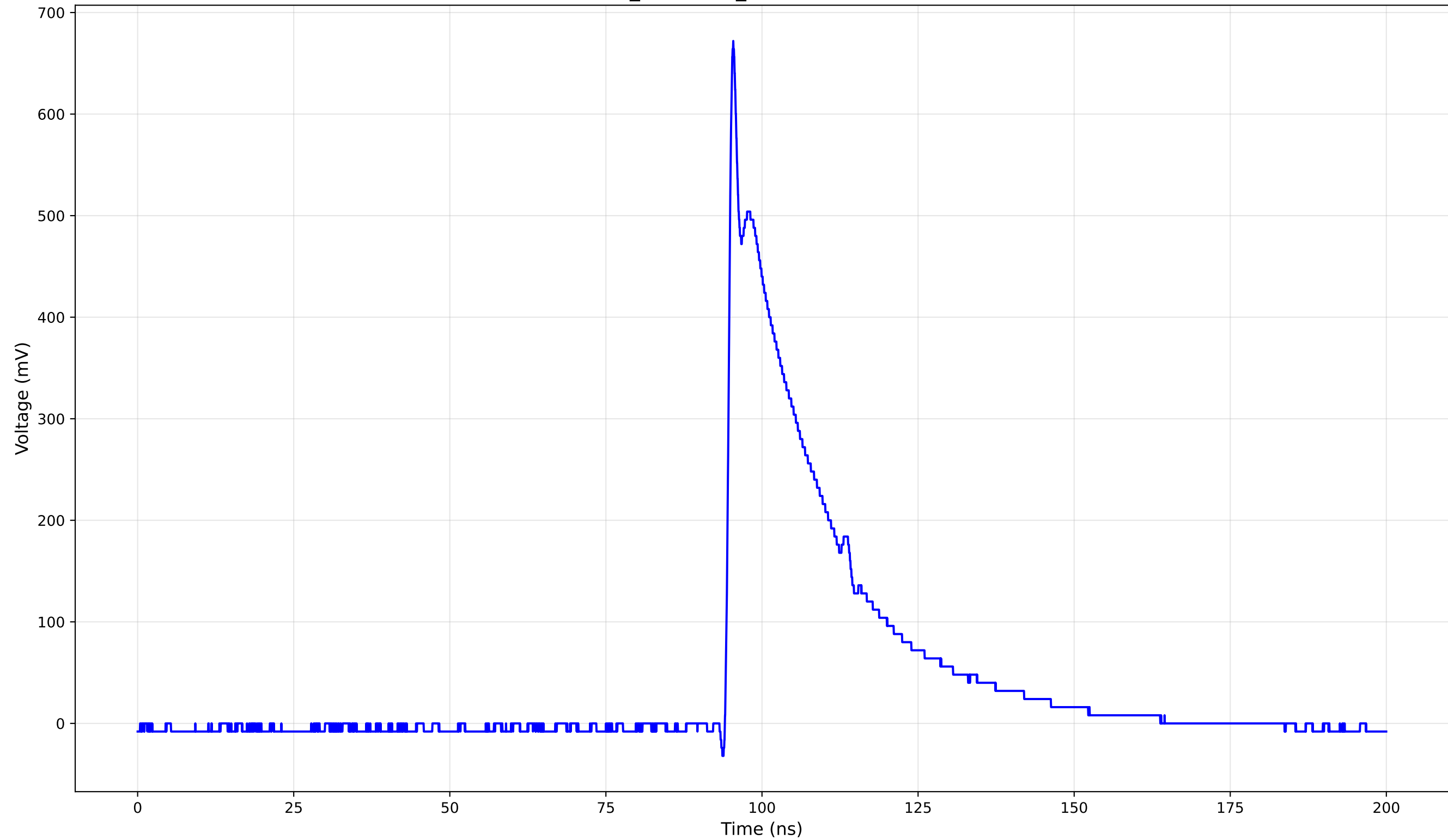
TCT Pulse Waveform - Run 3_148: 1cm_42-Position3 (148.0 V) - Rise Time: 0.82 ns
