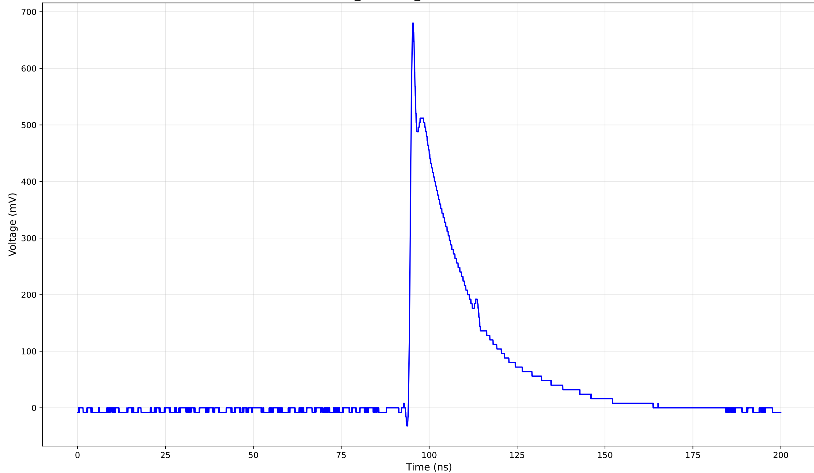
TCT Pulse Waveform - Run 3_149: 1cm_42-Position3 (149.0 V) - Rise Time: 0.81 ns
