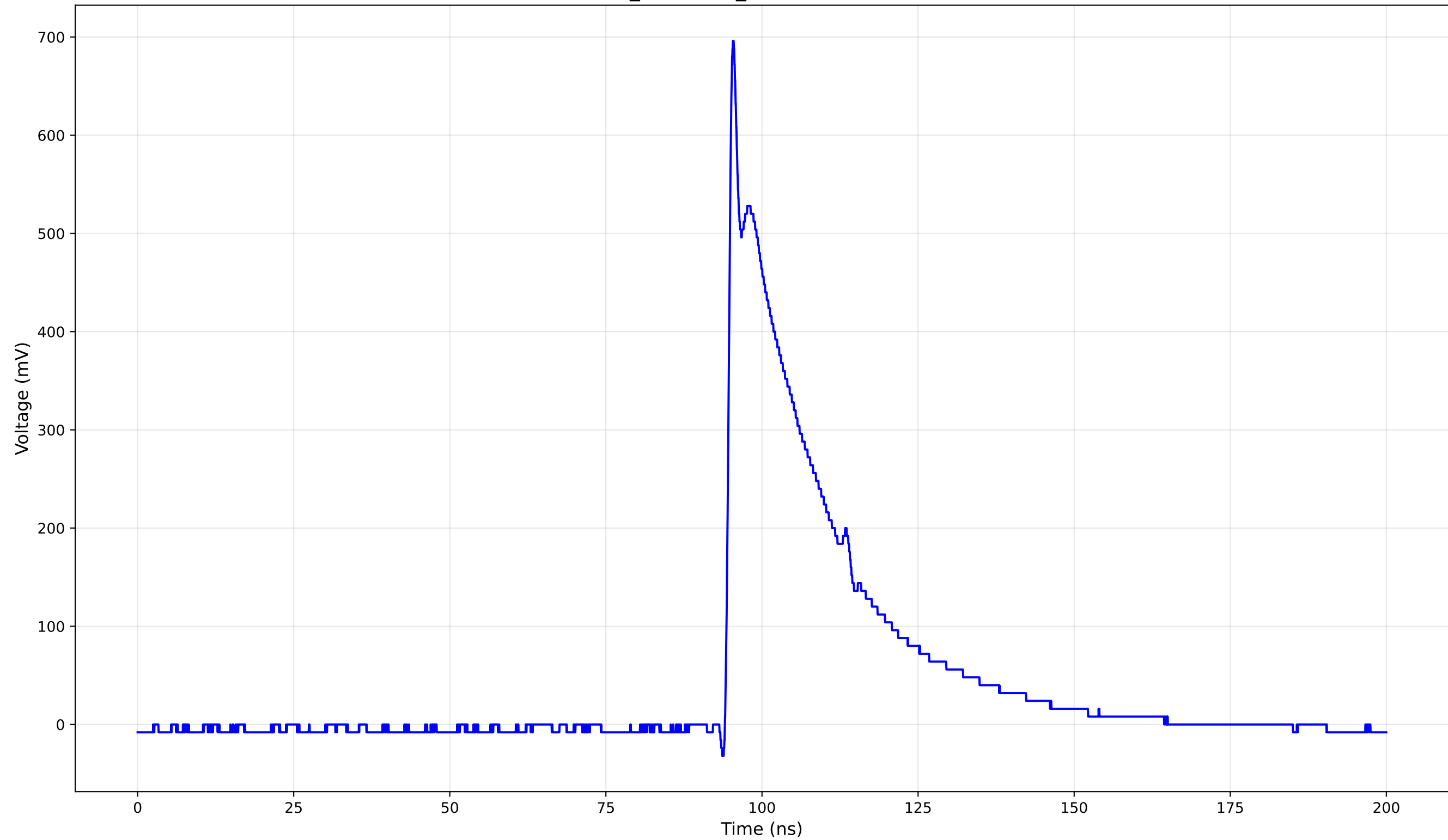
TCT Pulse Waveform - Run 3_150: 1cm_42-Position3 (150.0 V) - Rise Time: 0.82 ns
