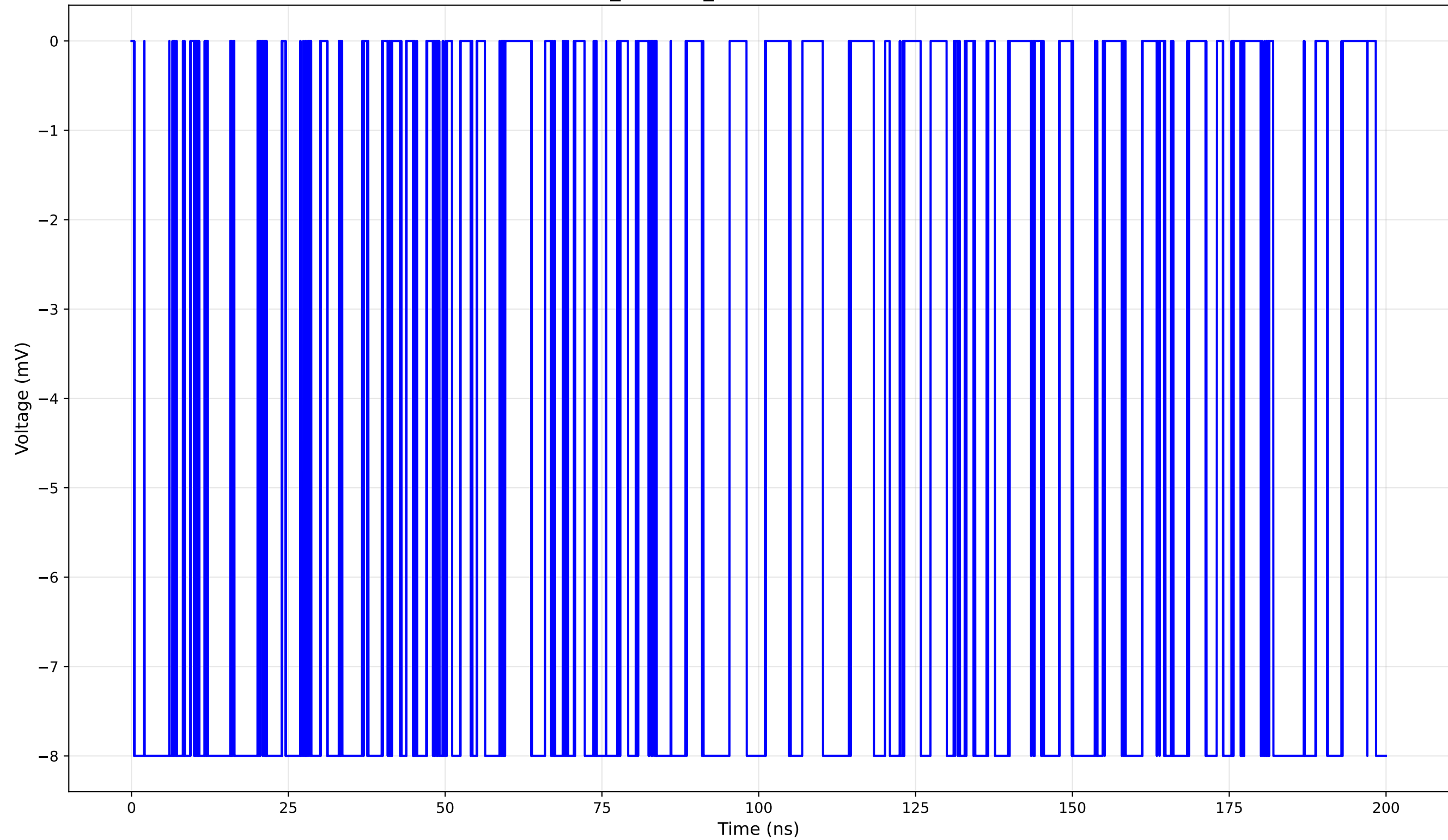
TCT Pulse Waveform - Run 3_20: 1cm_42-Position3 (20.0 V) - Rise Time: 0.00 ns (N/A)
