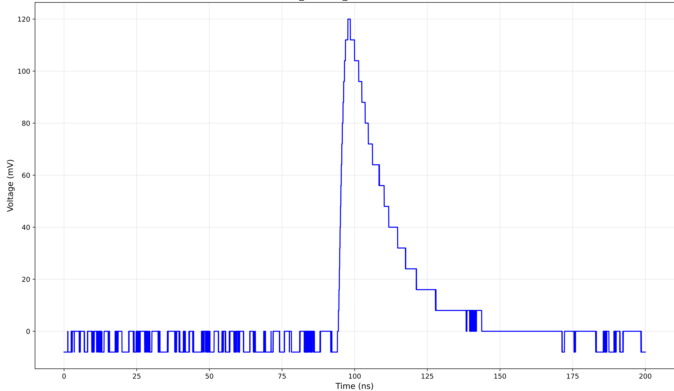
TCT Pulse Waveform - Run 3_40: 1cm_42-Position3 (40.0 V) - Rise Time: 2.26 ns
