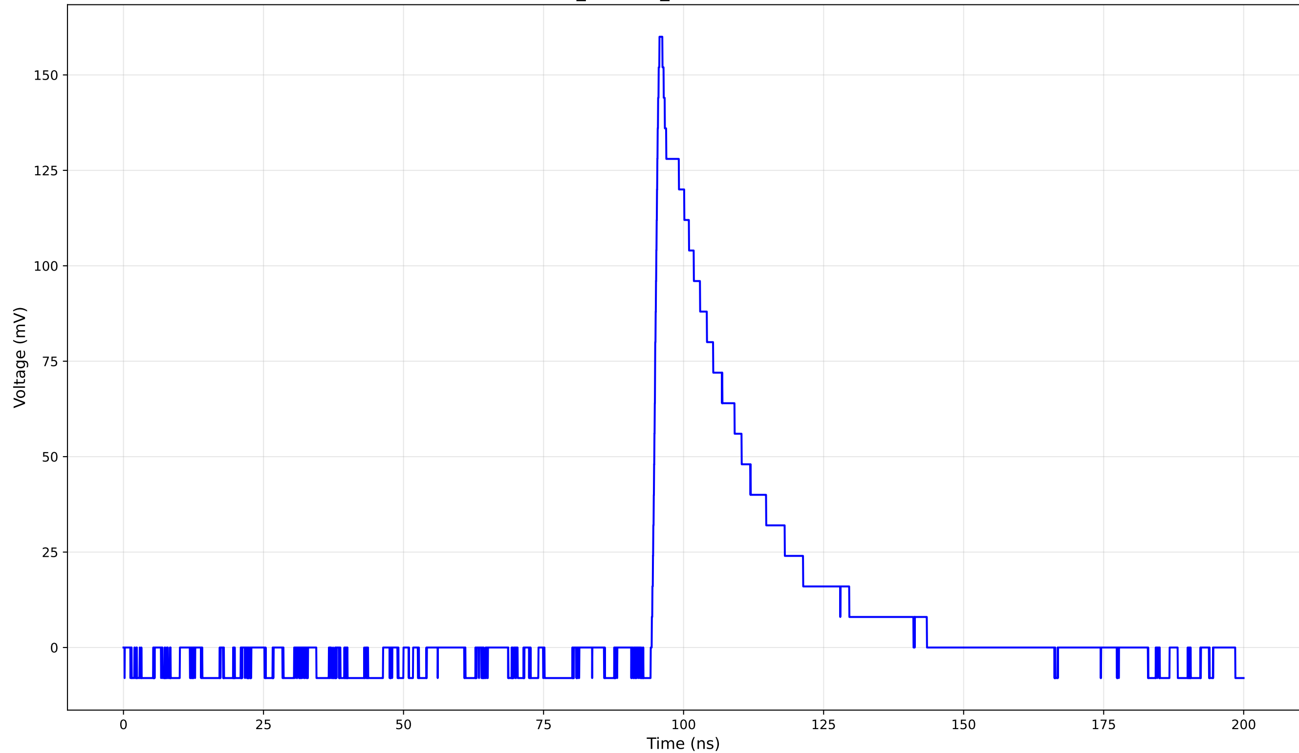
TCT Pulse Waveform - Run 3_50: 1cm_42-Position3 (50.0 V) - Rise Time: 1.03 ns
