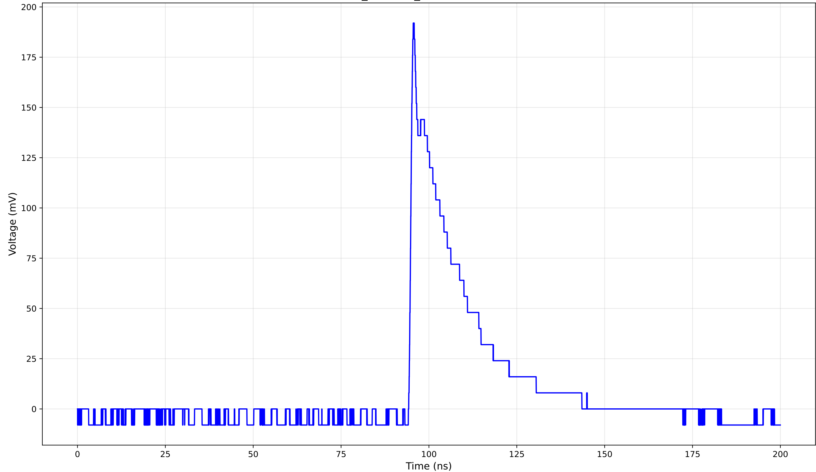
TCT Pulse Waveform - Run 3_60: 1cm_42-Position3 (60.0 V) - Rise Time: 0.96 ns
