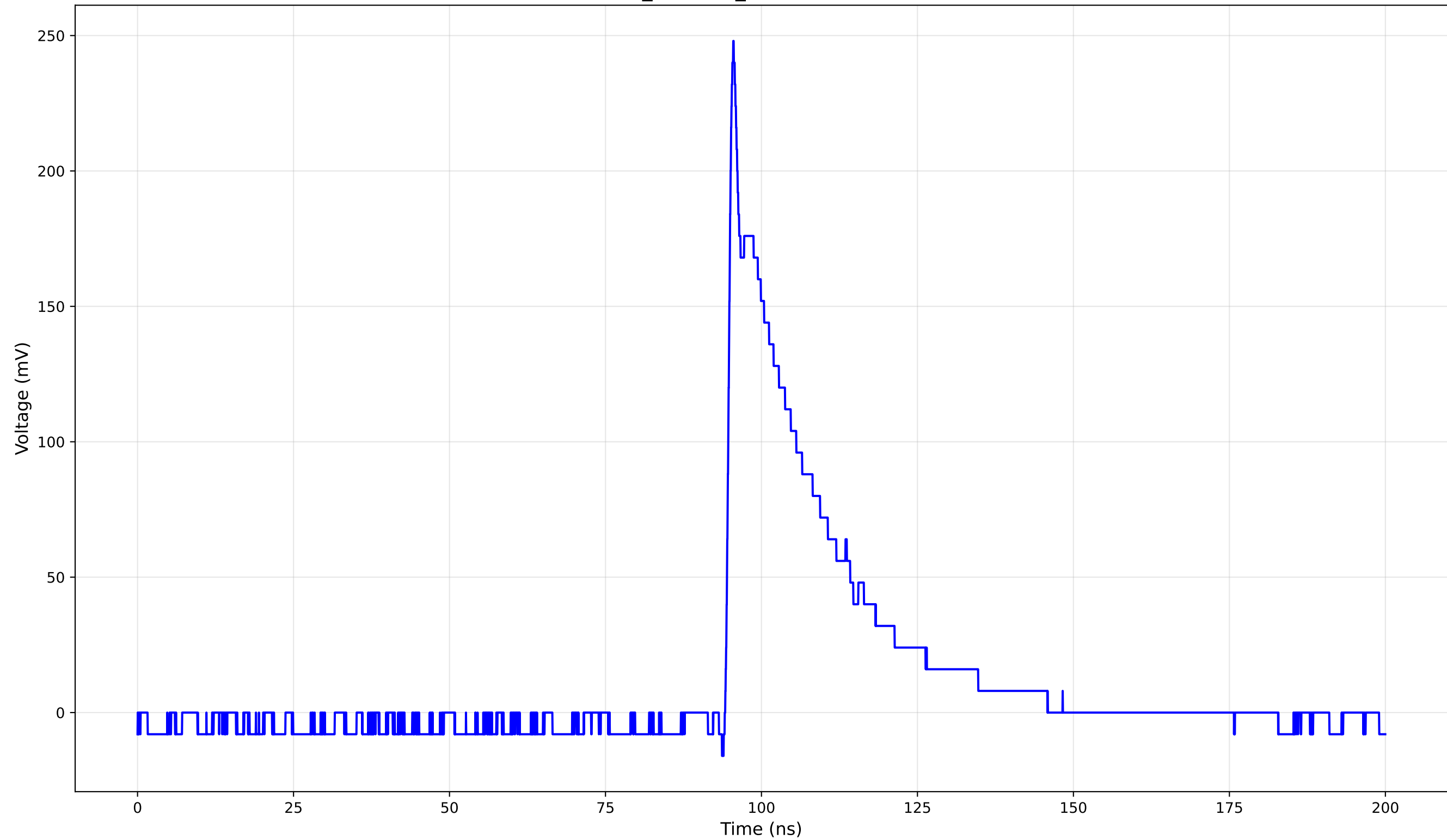
TCT Pulse Waveform - Run 3_70: 1cm_42-Position3 (70.0 V) - Rise Time: 0.87 ns
